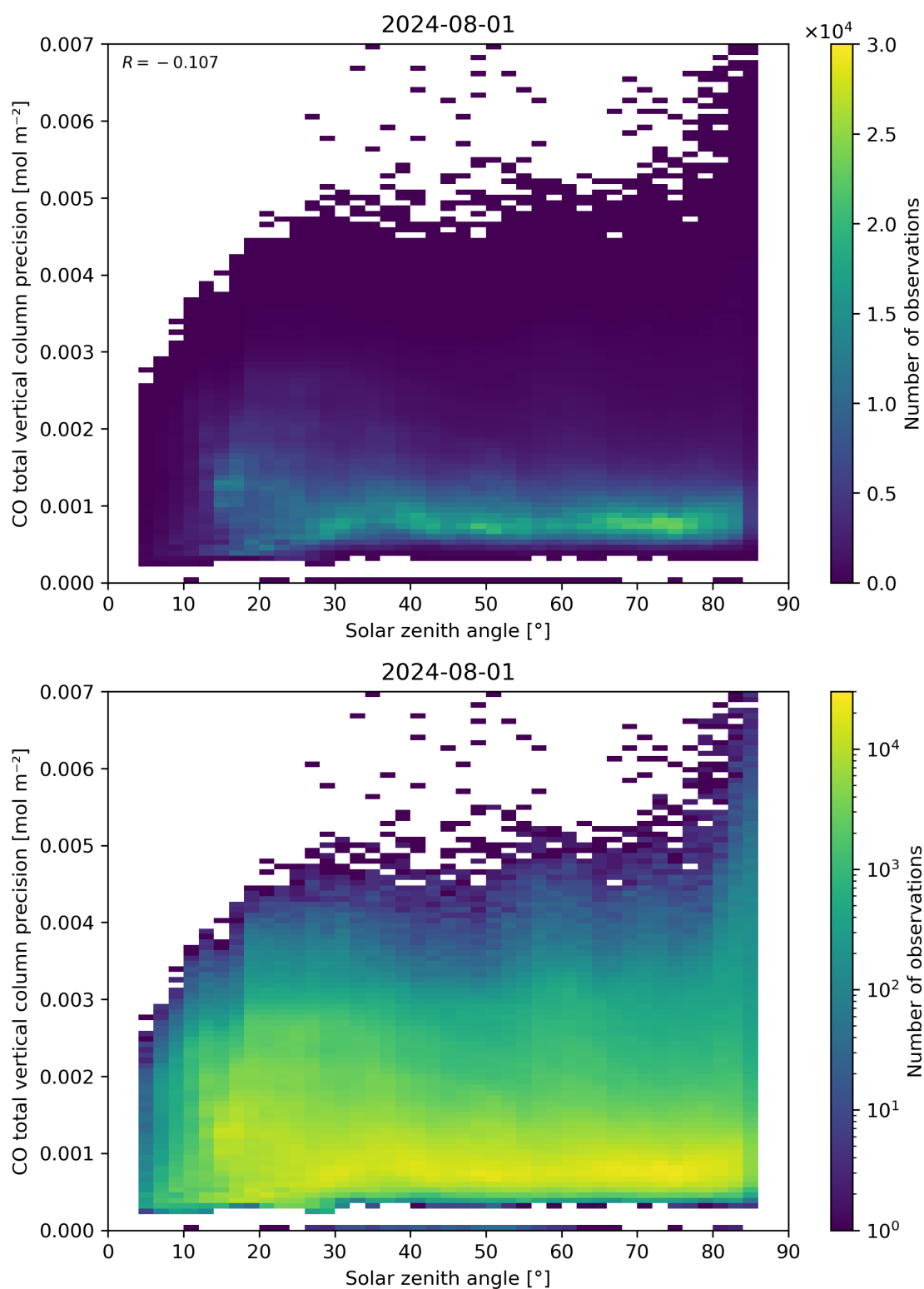
Figure 63: Scatter density plot of “Solar zenith angle” against “CO total vertical column precision” for 2024-07-31 to 2024-08-02.
