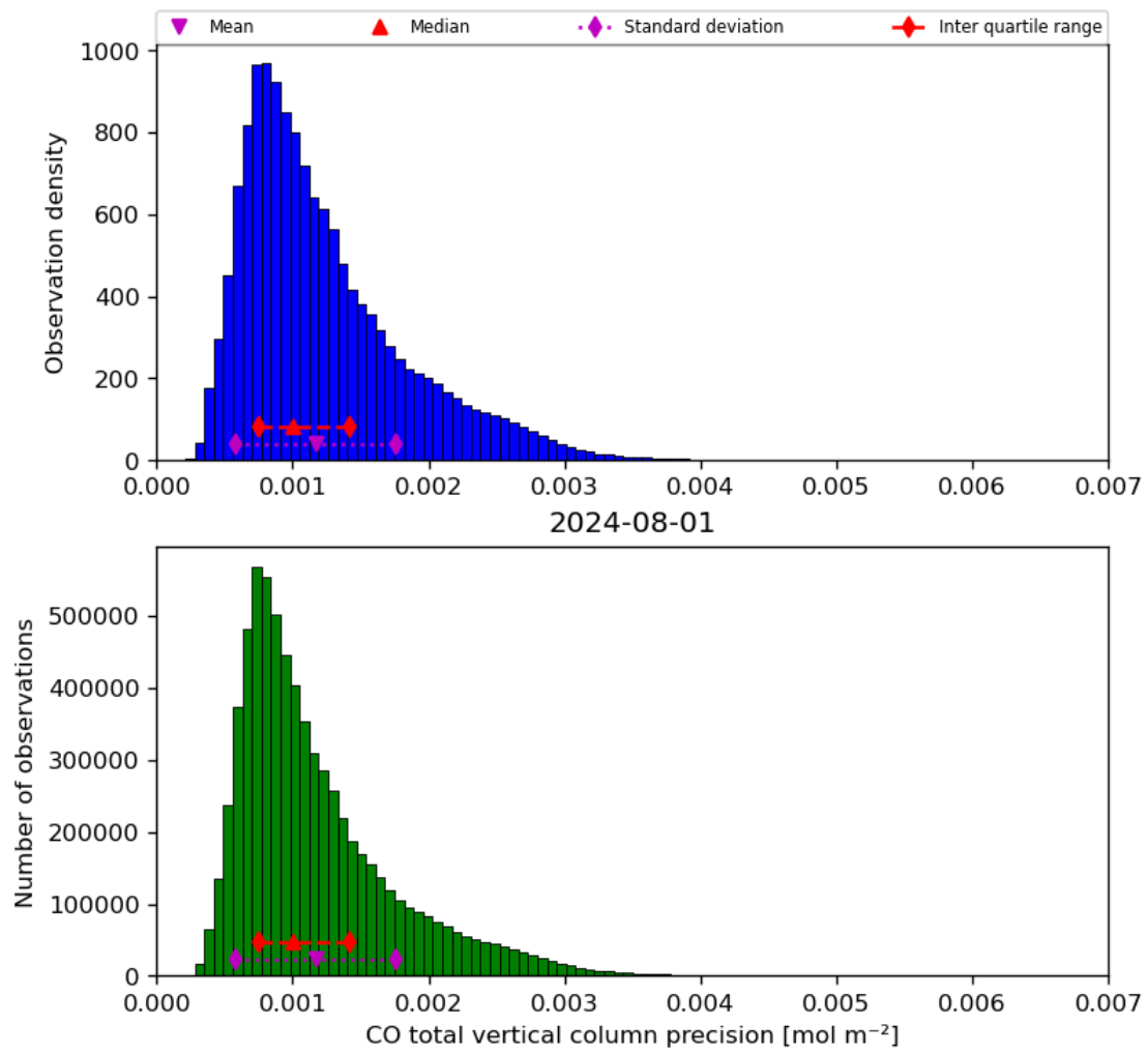
Figure 20: Histogram of “CO total vertical column precision” for 2024-07-31 to 2024-08-02
