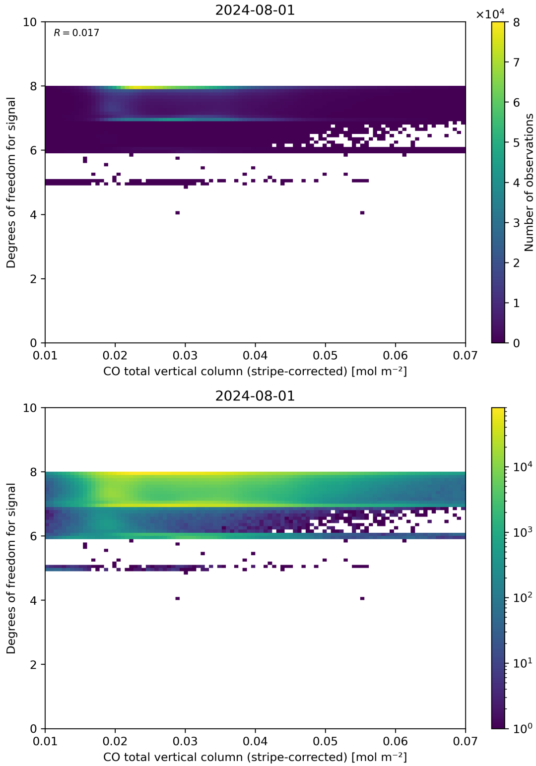
Figure 38: Scatter density plot of “CO total vertical column (stripe-corrected)” against “Degrees of freedom for signal” for 2024-07-31 to 2024-08-02.
