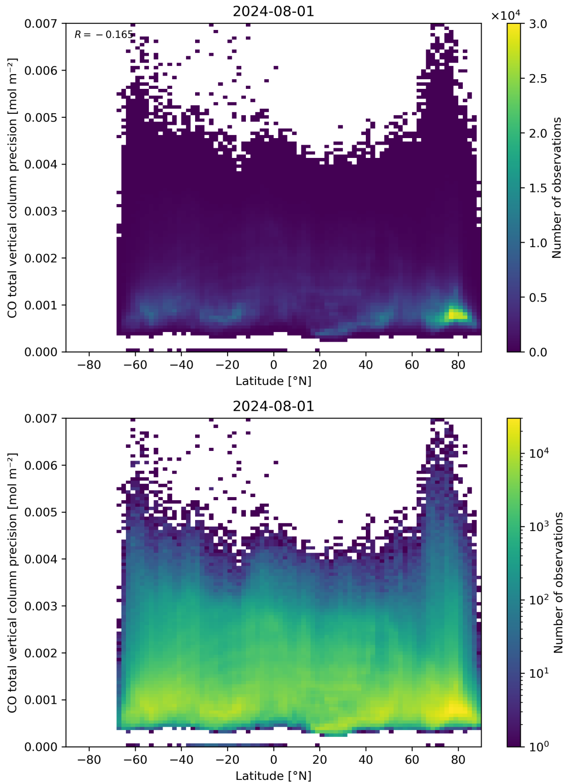
Figure 53: Scatter density plot of “Latitude” against “CO total vertical column precision” for 2024-07-31 to 2024-08-02.
