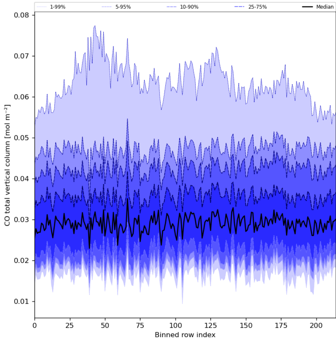
Figure 26: Along track statistics of “CO total vertical column” for 2024-07-31 to 2024-08-02
