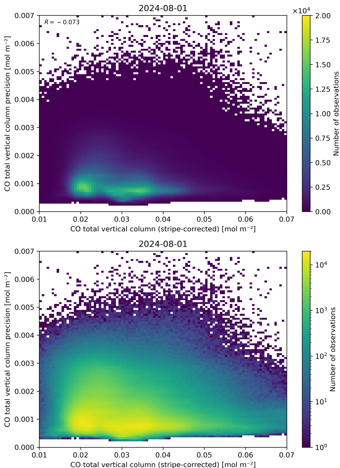
Figure 36: Scatter density plot of “CO total vertical column (stripe-corrected)” against “CO total vertical column precision” for 2024-07-31 to 2024-08-02.
