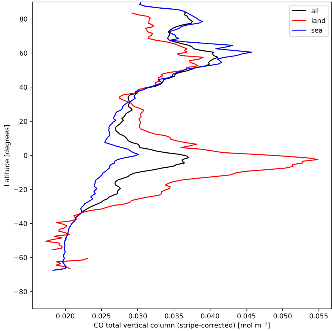
Figure 11: Zonal average of “CO total vertical column (stripe-corrected)” for 2024-07-31 to 2024-08-02.
