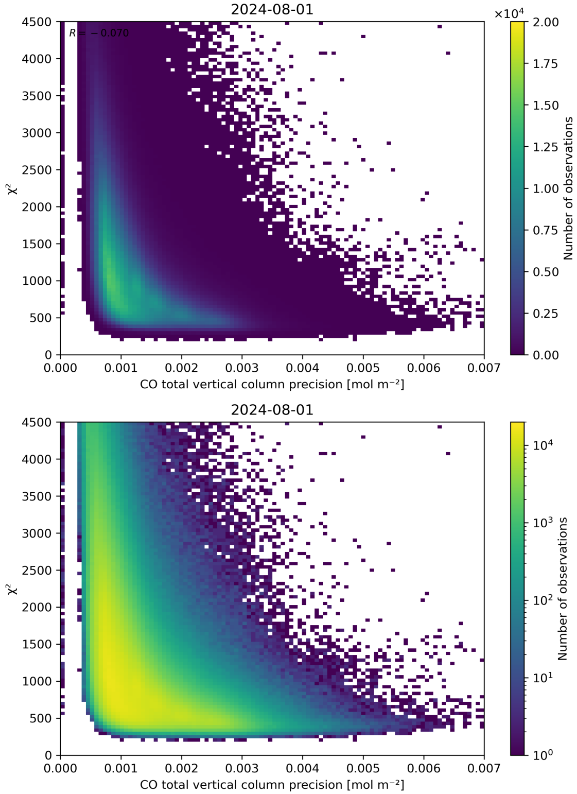
Figure 44: Scatter density plot of “CO total vertical column precision” against “ \chi^2 ” for 2024-07-31 to 2024-08-02.
