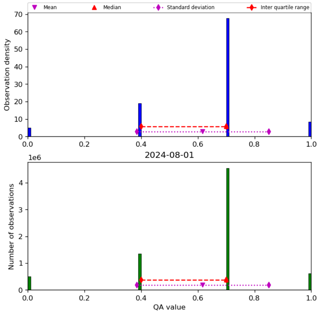
Figure 17: Histogram of “QA value” for 2024-07-31 to 2024-08-02
