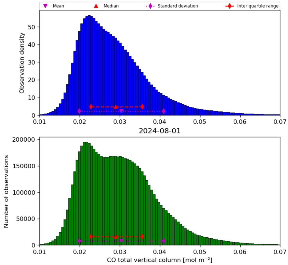
Figure 18: Histogram of “CO total vertical column” for 2024-07-31 to 2024-08-02
