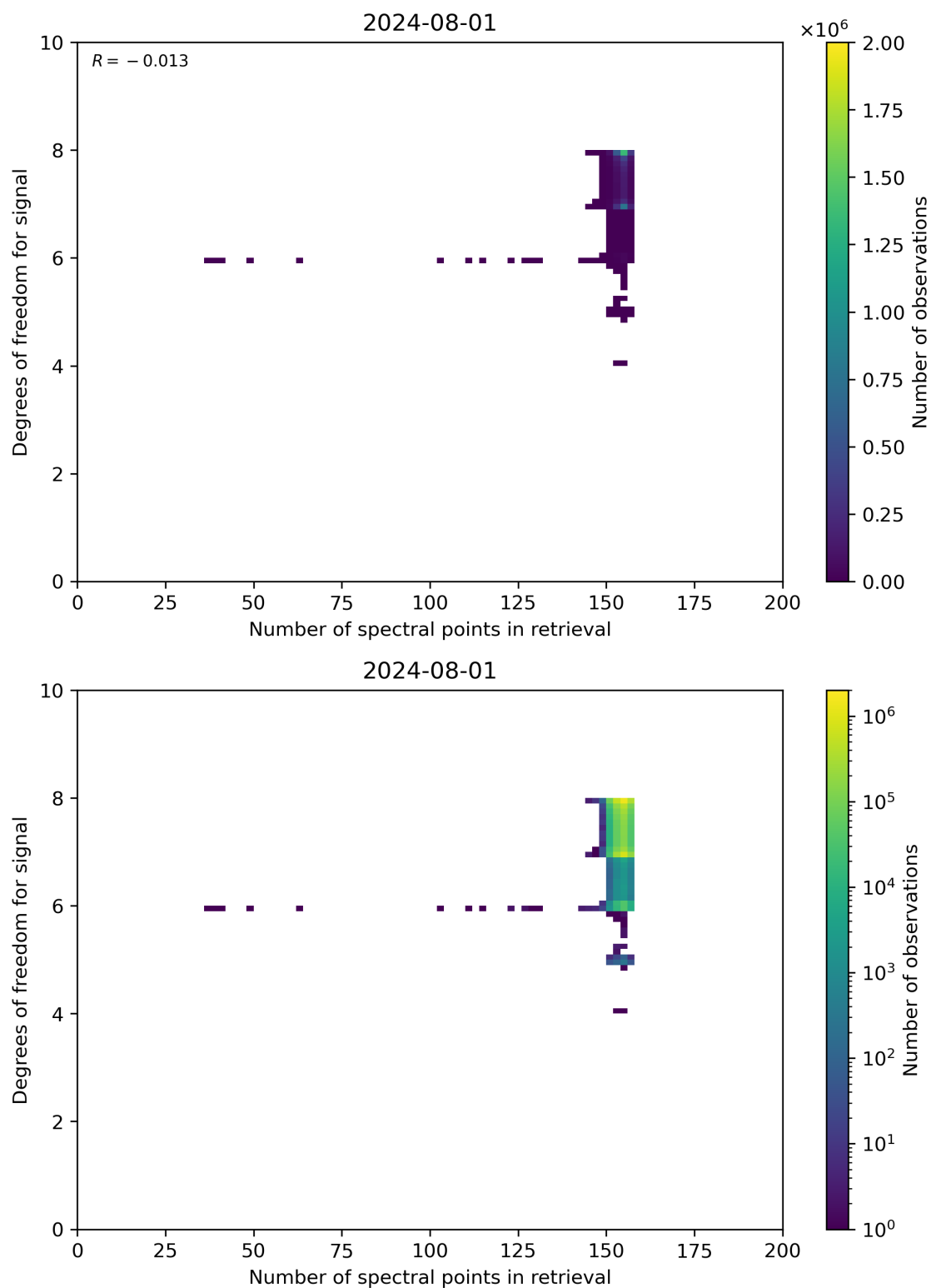
Figure 59: Scatter density plot of “Number of spectral points in retrieval” against “Degrees of freedom for signal” for 2024-07-31 to 2024-08-02.
