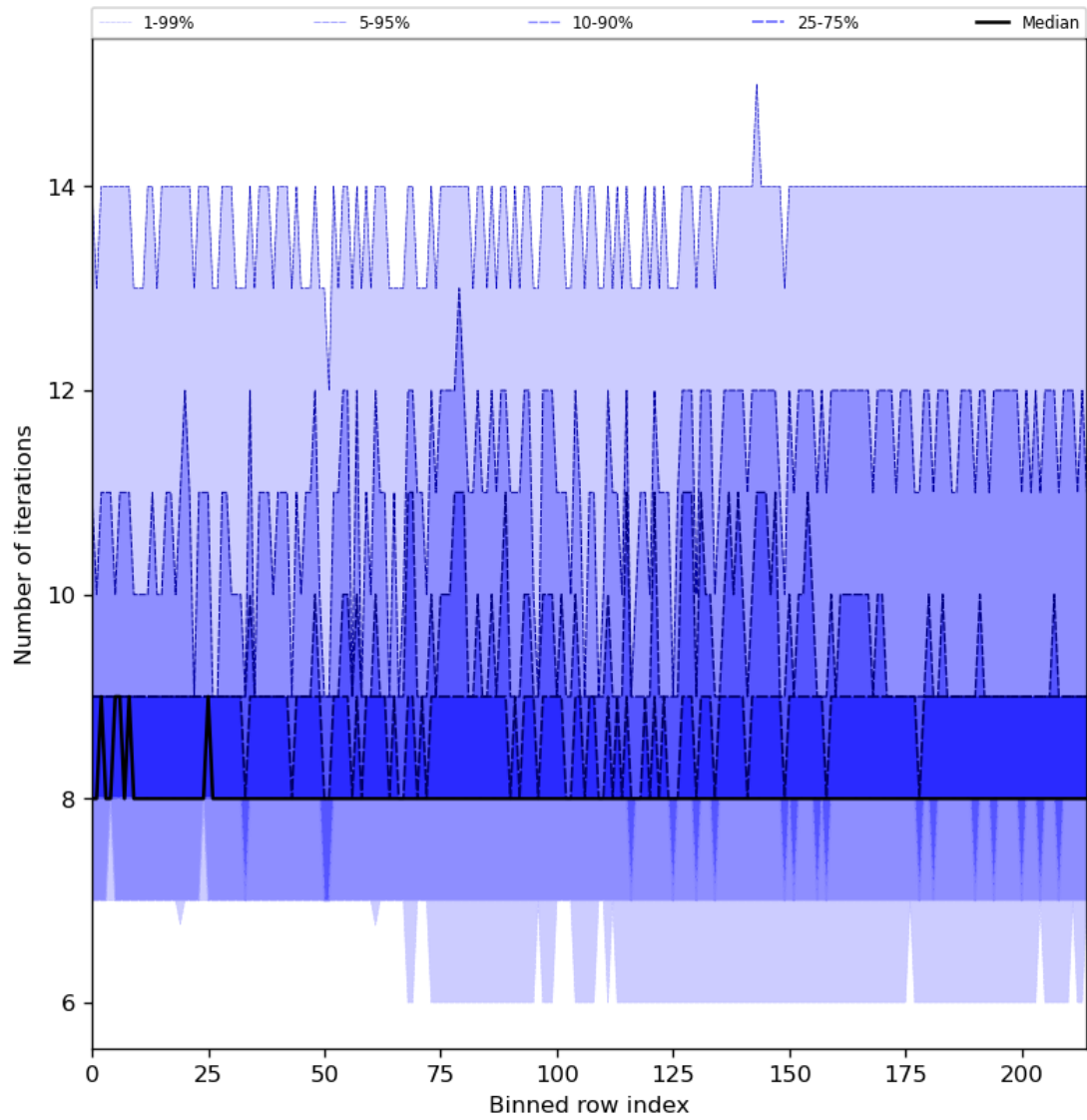
Figure 32: Along track statistics of “Number of iterations” for 2024-07-31 to 2024-08-02
