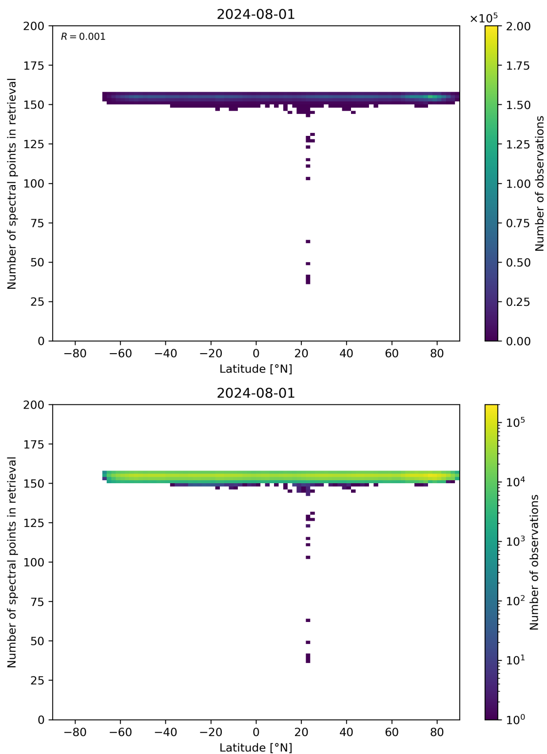
Figure 57: Scatter density plot of “Latitude” against “Number of spectral points in retrieval” for 2024-07-31 to 2024-08-02.
