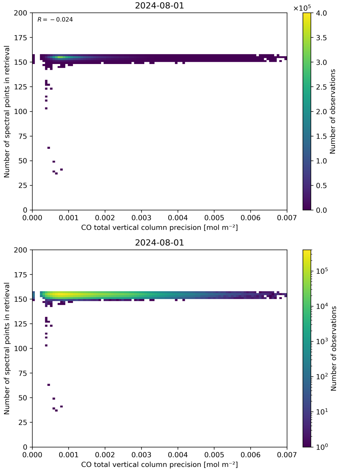
Figure 47: Scatter density plot of “CO total vertical column precision” against “Number of spectral points in retrieval” for 2024-07-31 to 2024-08-02.
