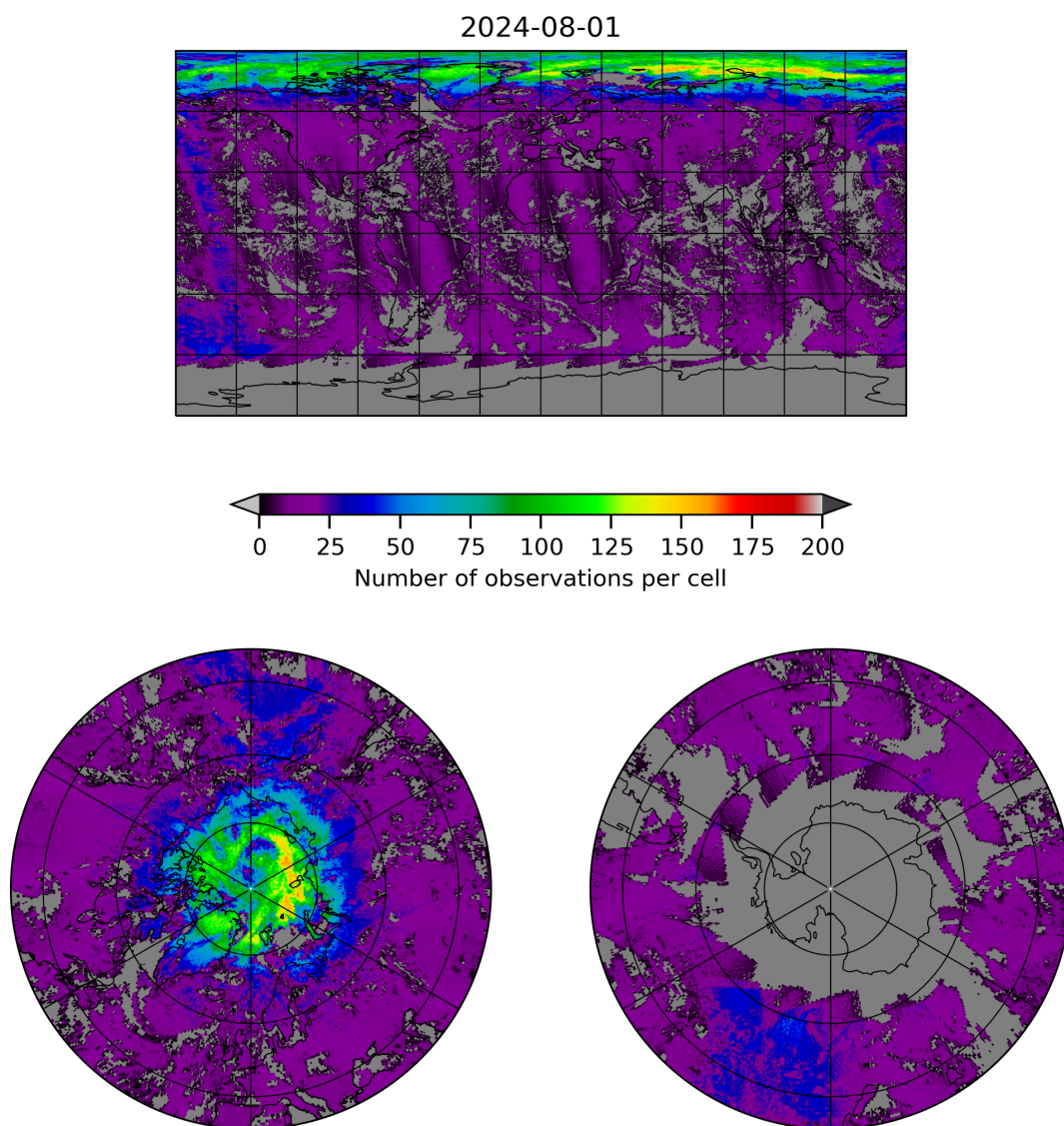
Figure 8: Map of the number of observations for 2024-07-31 to 2024-08-02
