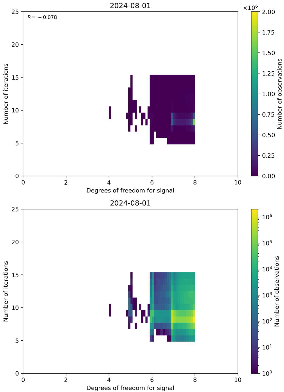
Figure 50: Scatter density plot of “Degrees of freedom for signal” against “Number of iterations” for 2024-07-31 to 2024-08-02.
