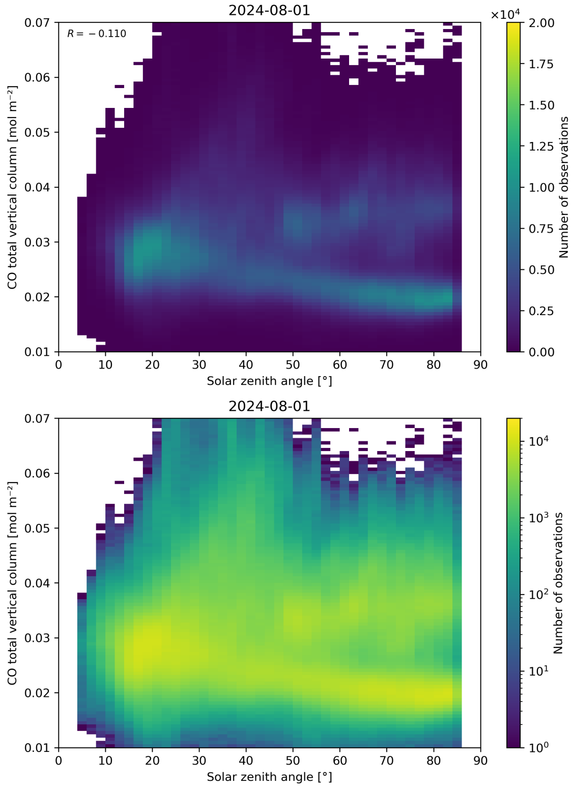
Figure 61: Scatter density plot of “Solar zenith angle” against “CO total vertical column” for 2024-07-31 to 2024-08-02.
