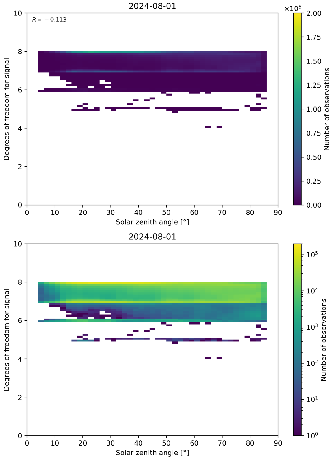
Figure 65: Scatter density plot of “Solar zenith angle” against “Degrees of freedom for signal” for 2024-07-31 to 2024-08-02.
