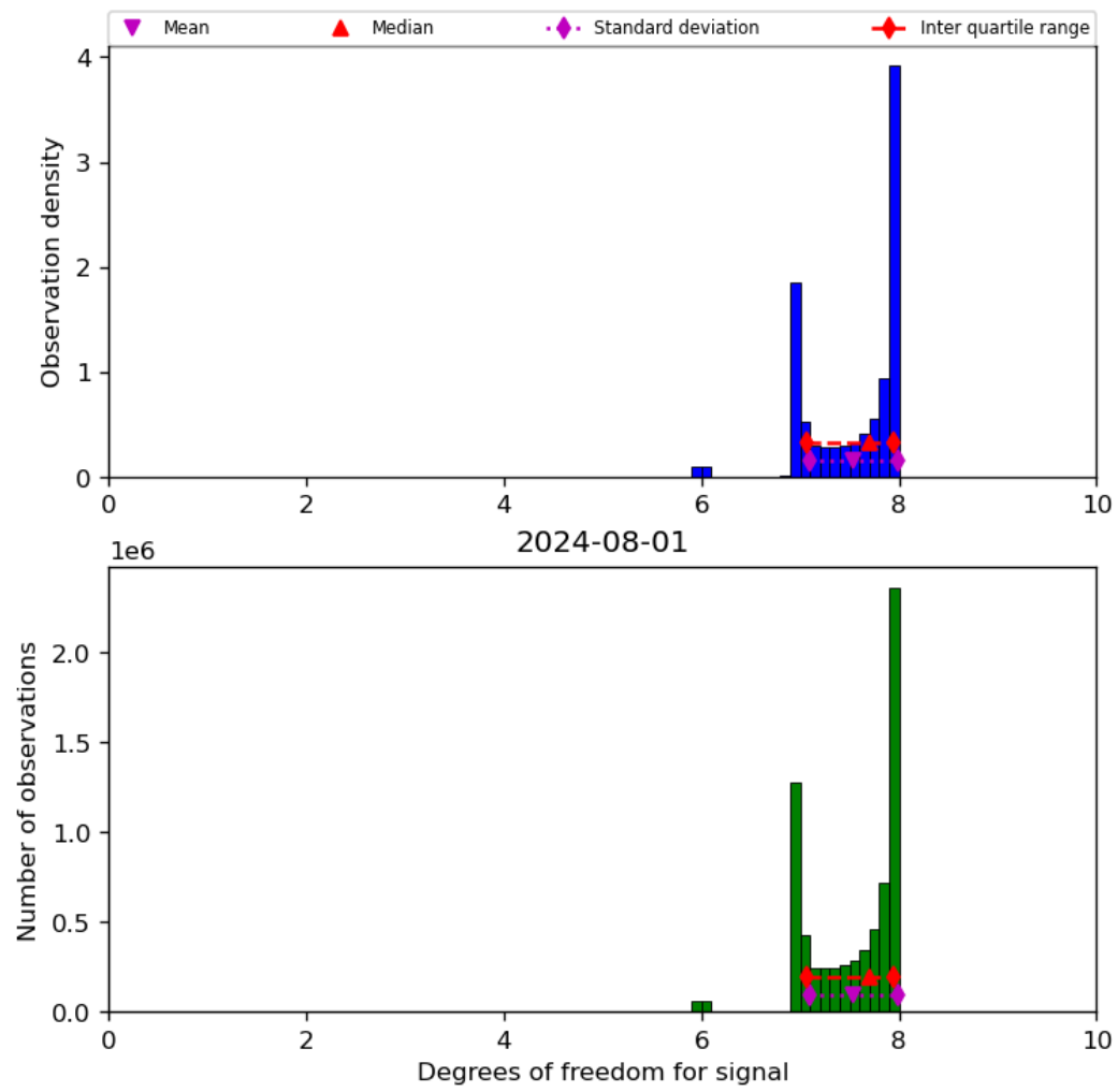
Figure 23: Histogram of “Degrees of freedom for signal” for 2024-07-31 to 2024-08-02
