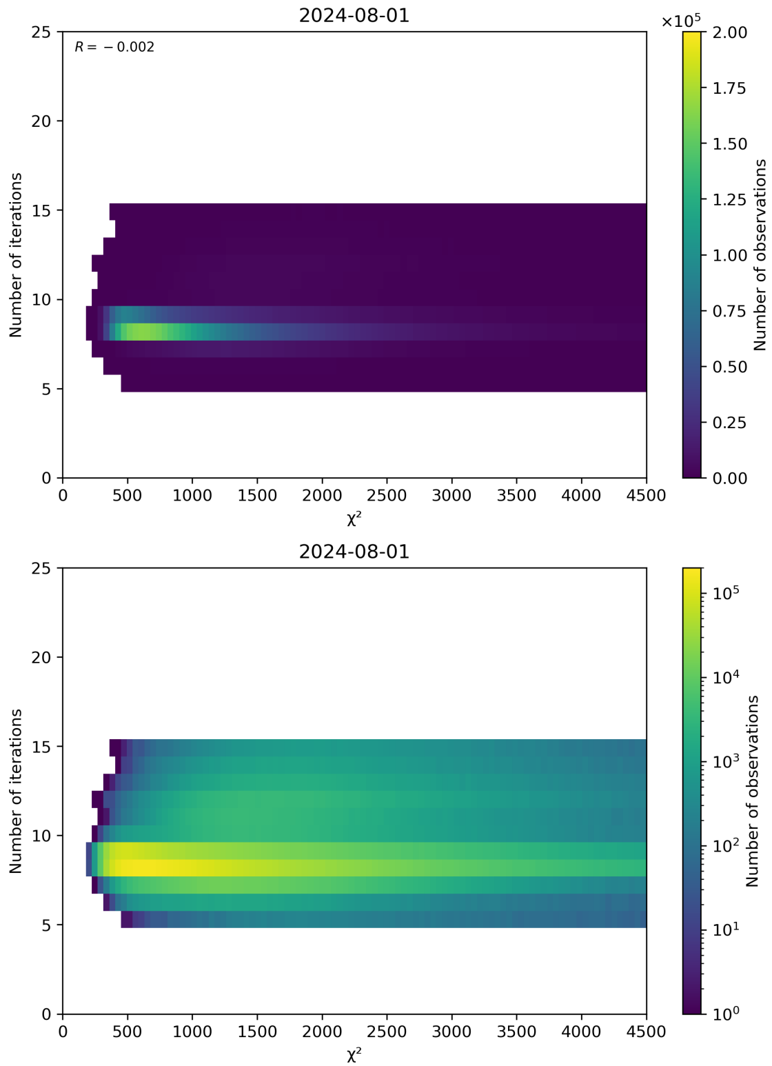
Figure 49: Scatter density plot of “ \chi^2 ” against “Number of iterations” for 2024-07-31 to 2024-08-02.
