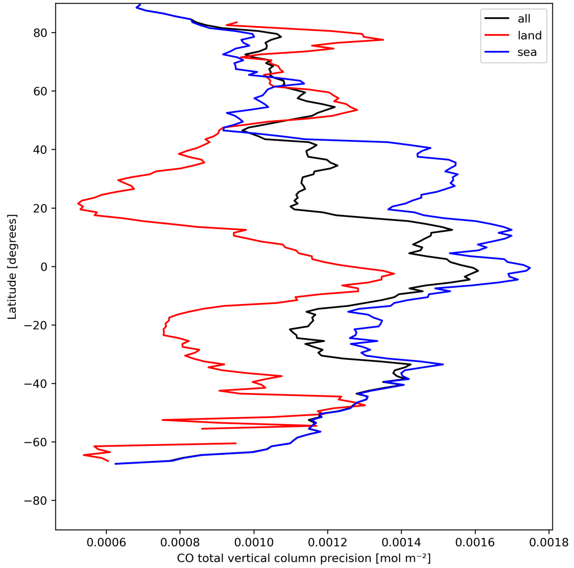
Figure 12: Zonal average of "CO total vertical column precision" for 2024-07-31 to 2024-08-02.
