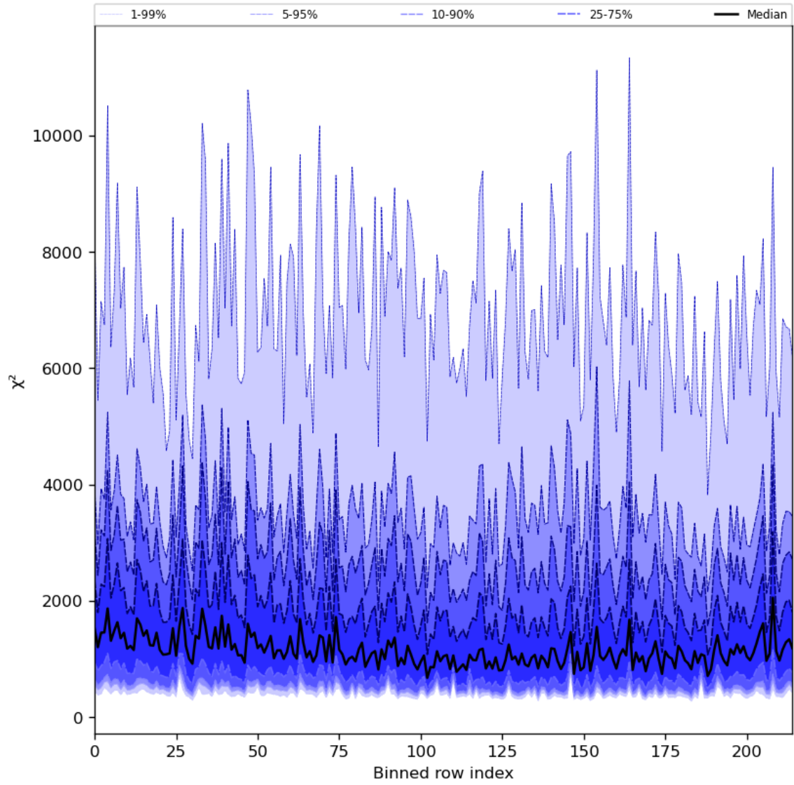
Figure 30: Along track statistics of “ \chi^2 ” for 2024-07-31 to 2024-08-02
