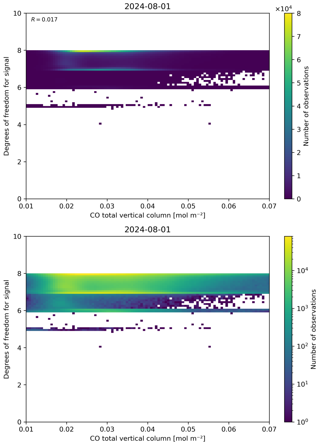
Figure 41: Scatter density plot of “CO total vertical column” against “Degrees of freedom for signal” for 2024-07-31 to 2024-08-02.
