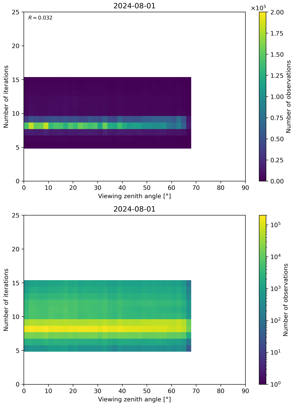
Figure 75: Scatter density plot of “Viewing zenith angle” against “Number of iterations” for 2024-07-31 to 2024-08-02.
