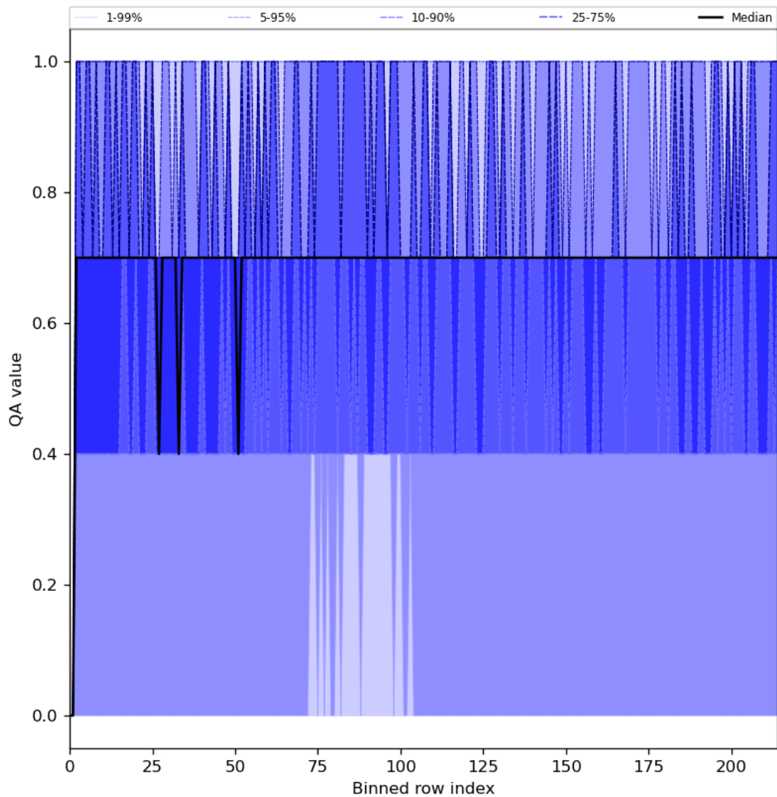
Figure 25: Along track statistics of “QA value” for 2024-07-31 to 2024-08-02
