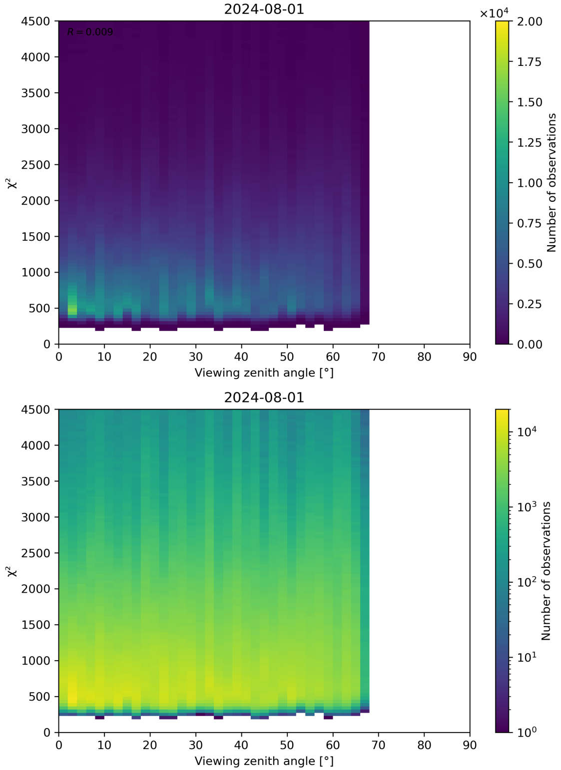
Figure 72: Scatter density plot of “Viewing zenith angle” against “ \chi^2 ” for 2024-07-31 to 2024-08-02.
