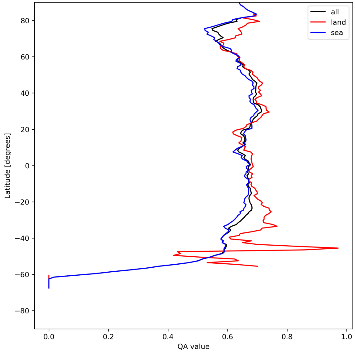
Figure 9: Zonal average of “QA value” for 2024-07-31 to 2024-08-02.
