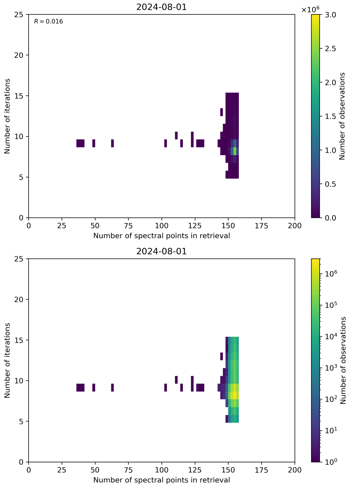
Figure 60: Scatter density plot of “Number of spectral points in retrieval” against “Number of iterations” for 2024-07-31 to 2024-08-02.
