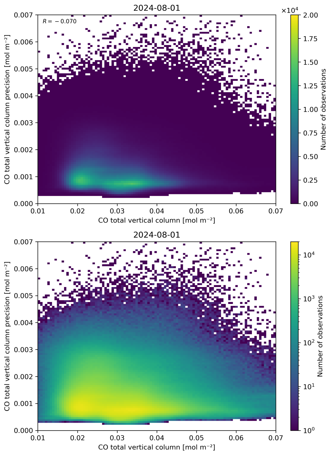
Figure 34: Scatter density plot of “CO total vertical column” against “CO total vertical column precision” for 2024-07-31 to 2024-08-02.
