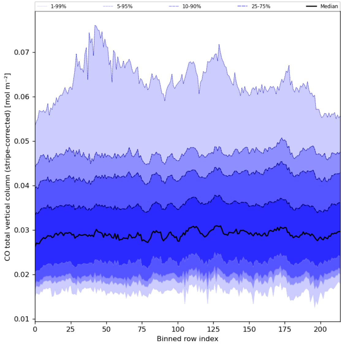
Figure 27: Along track statistics of “CO total vertical column (stripe-corrected)” for 2024-07-31 to 2024-08-02
