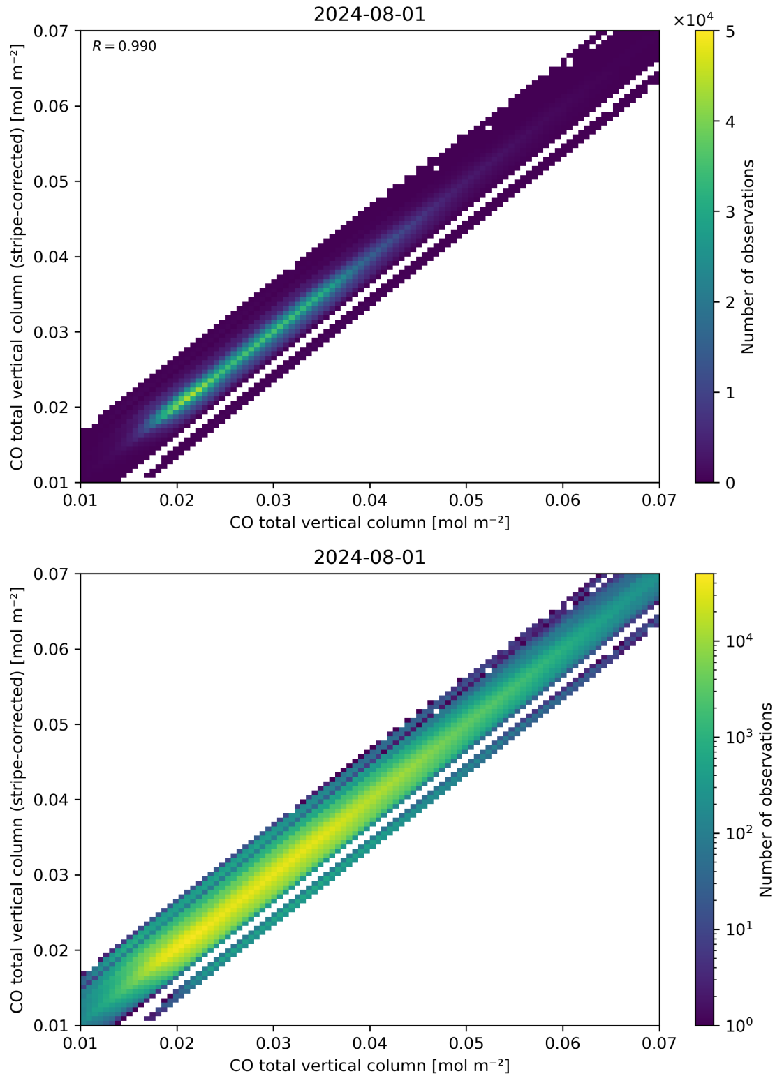
Figure 33: Scatter density plot of “CO total vertical column” against “CO total vertical column (stripe-corrected)” for 2024-07-31 to 2024-08-02.
