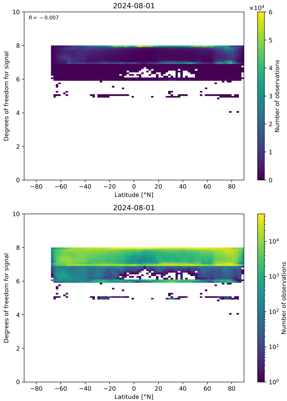
Figure 55: Scatter density plot of “Latitude” against “Degrees of freedom for signal” for 2024-07-31 to 2024-08-02.
