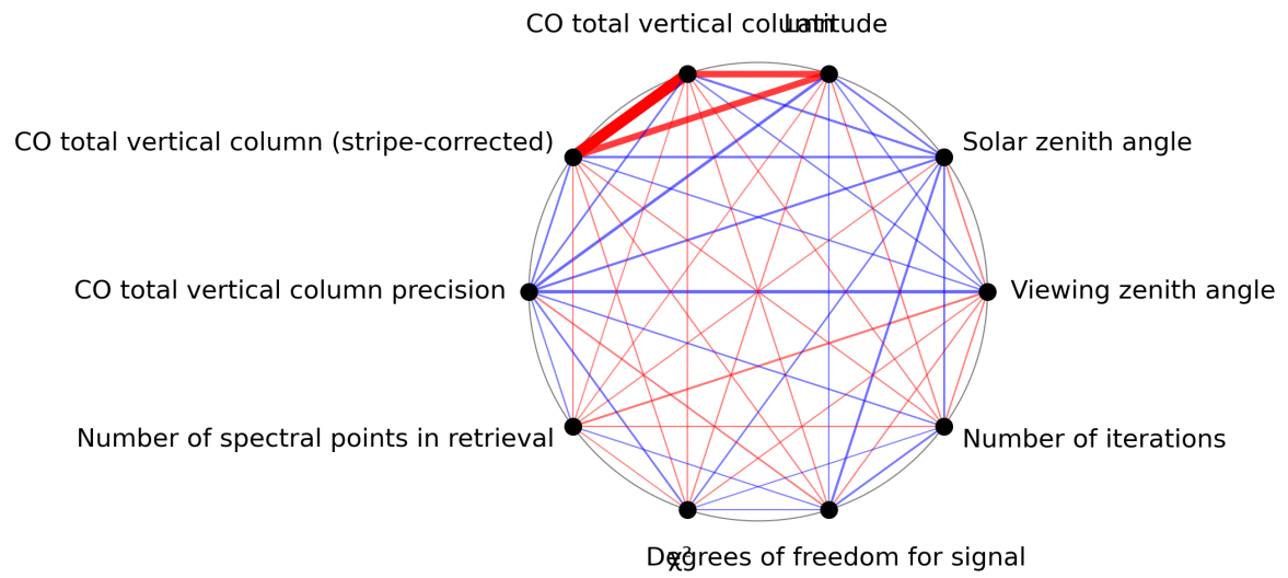
Figure 1: Map of correlation graph for 2024-07-31 to 2024-08-02.
