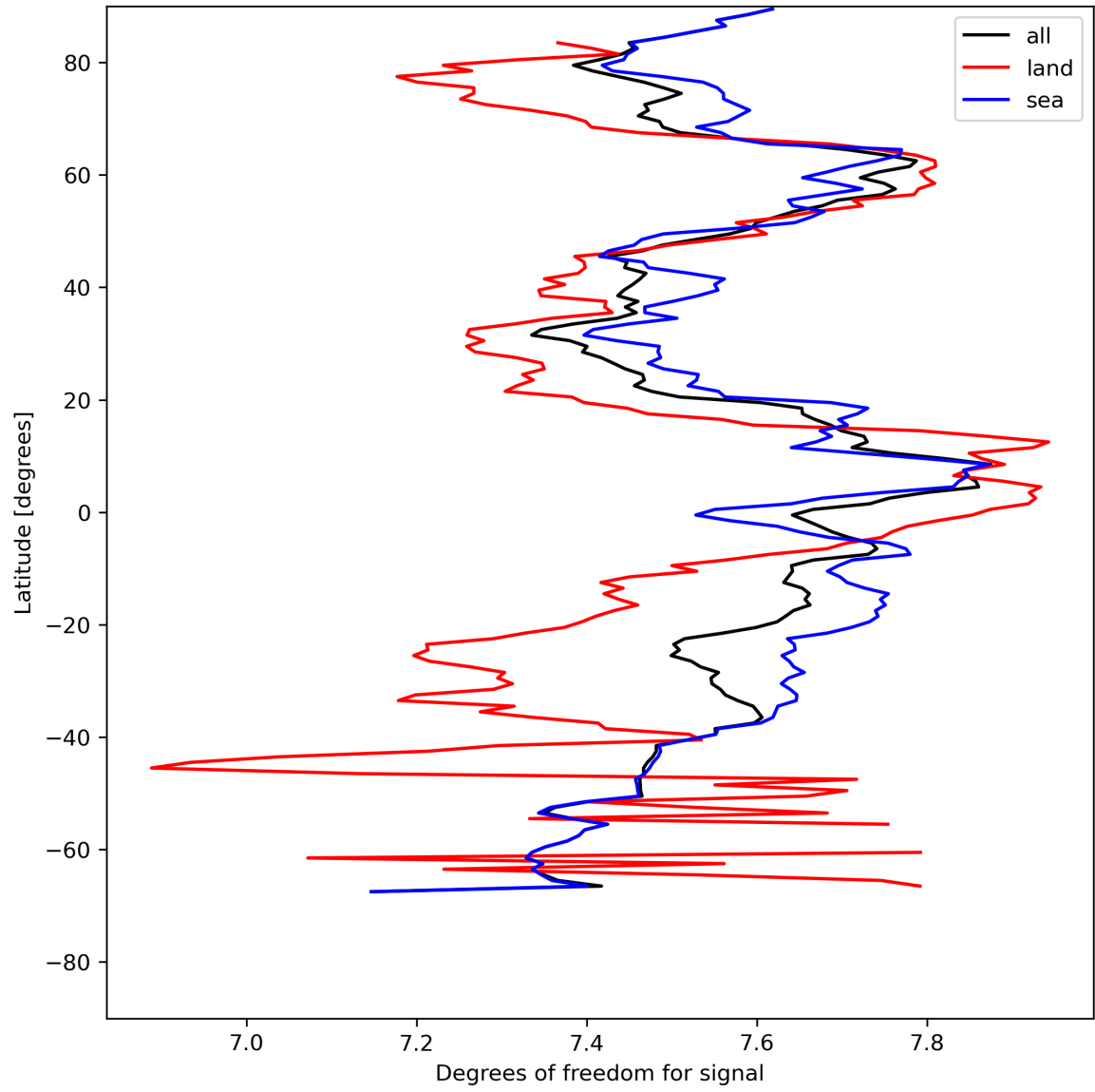
Figure 15: Zonal average of “Degrees of freedom for signal” for 2024-07-31 to 2024-08-02.
