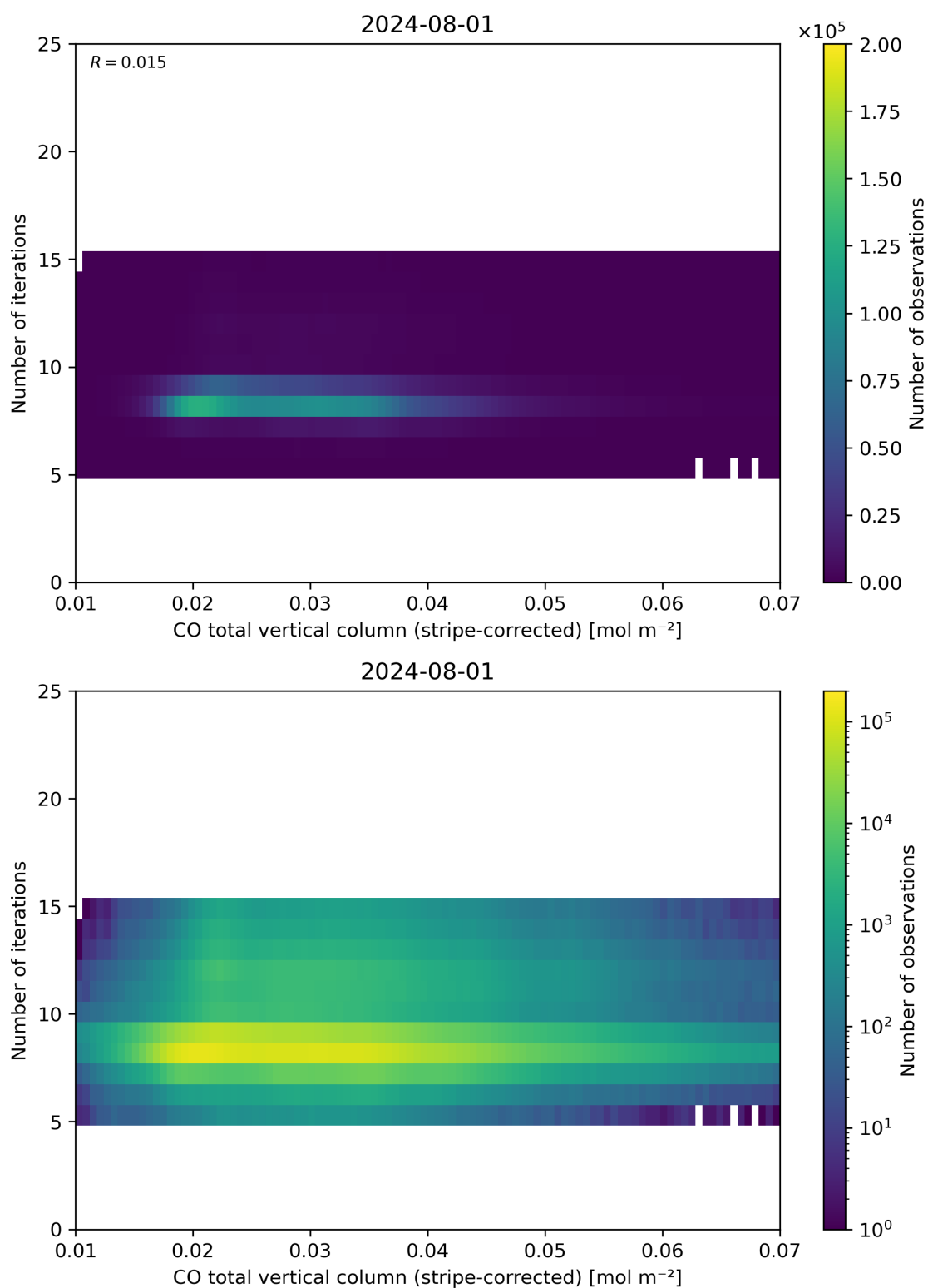
Figure 39: Scatter density plot of “CO total vertical column (stripe-corrected)” against “Number of iterations” for 2024-07-31 to 2024-08-02.
