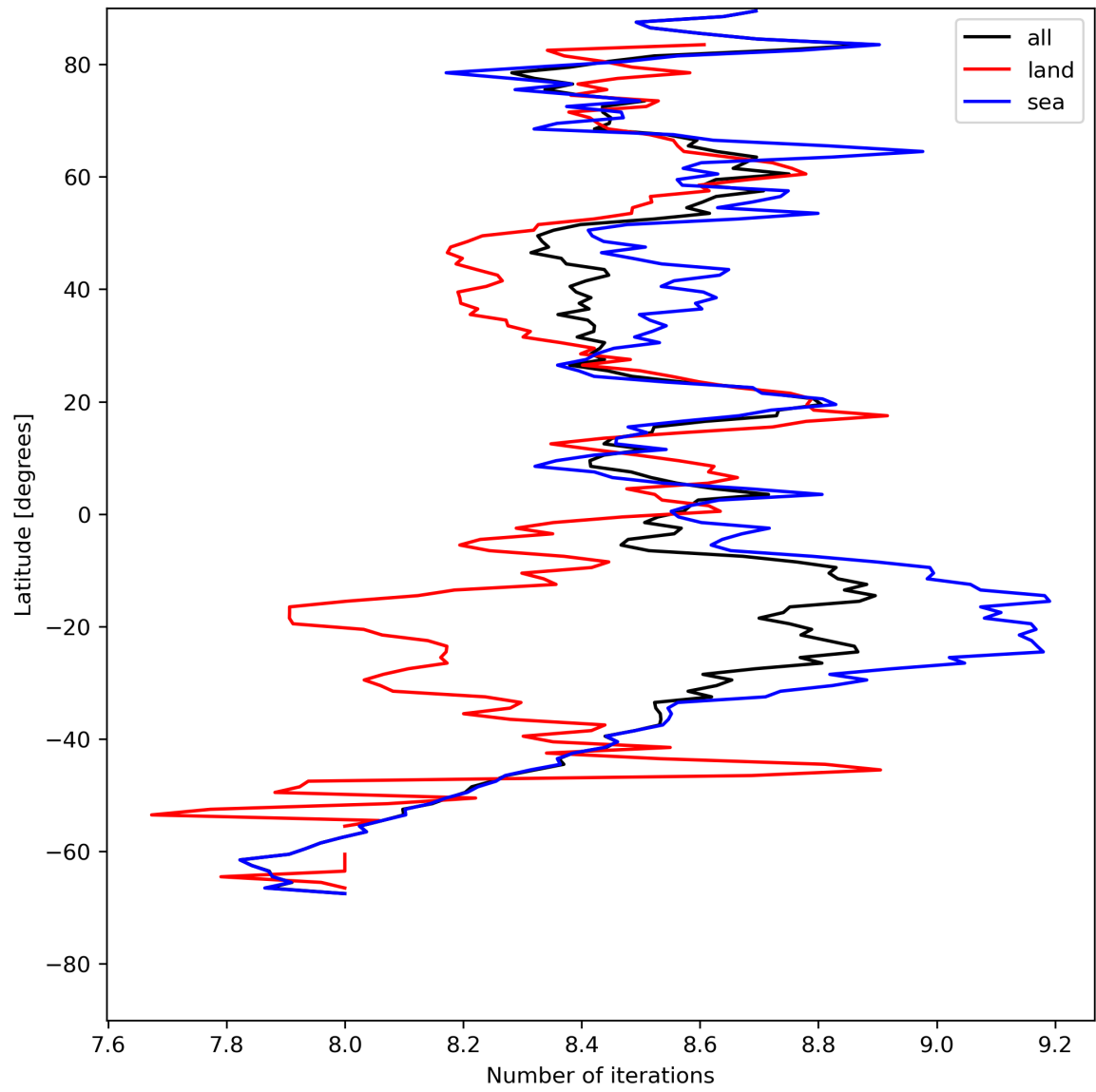
Figure 16: Zonal average of “Number of iterations” for 2024-07-31 to 2024-08-02.
