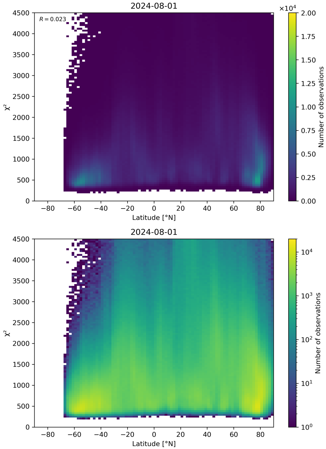
Figure 54: Scatter density plot of “Latitude” against “ \chi^2 ” for 2024-07-31 to 2024-08-02.
