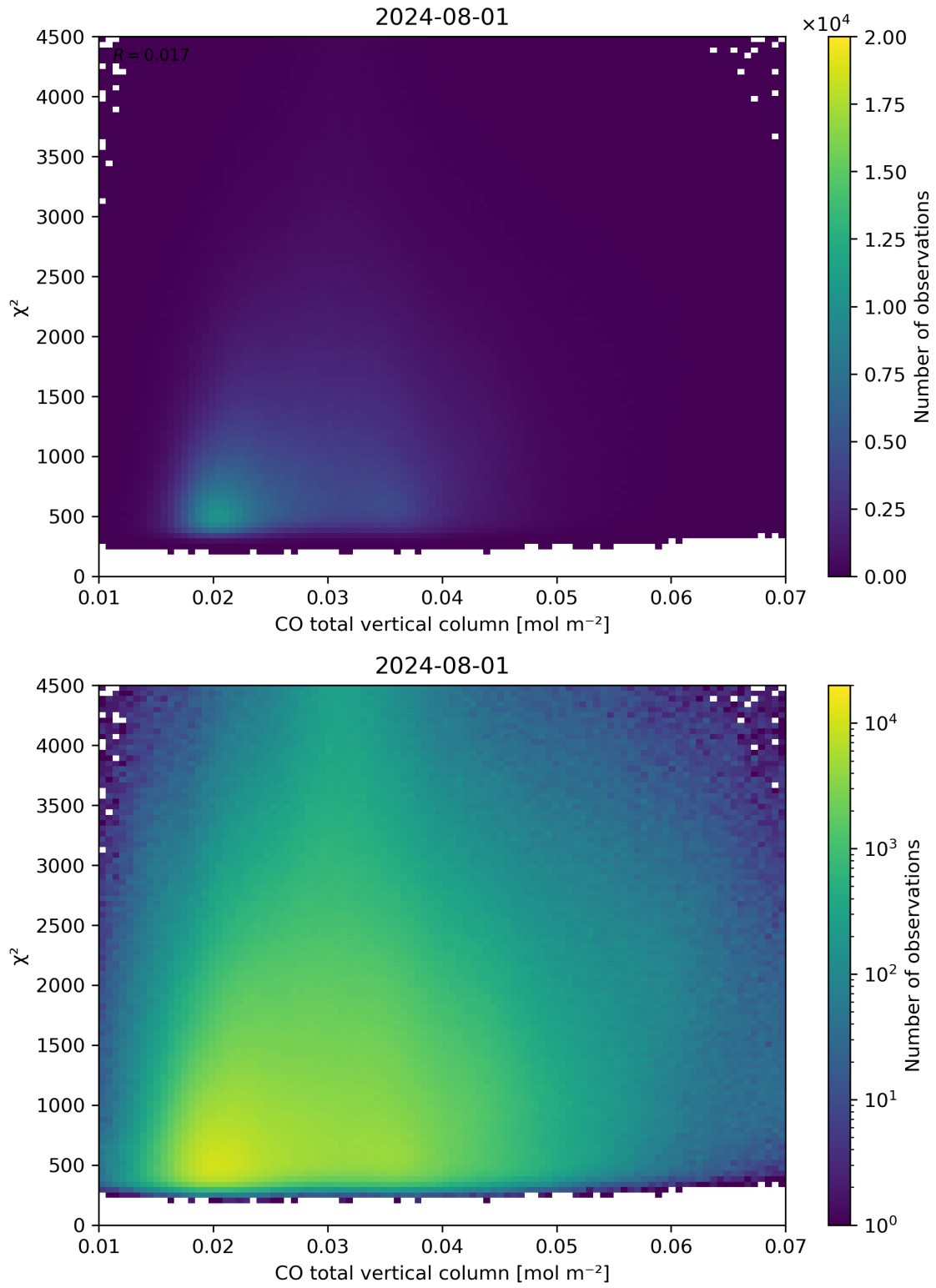
Figure 35: Scatter density plot of “CO total vertical column” against “ \chi^2 ” for 2024-07-31 to 2024-08-02.
