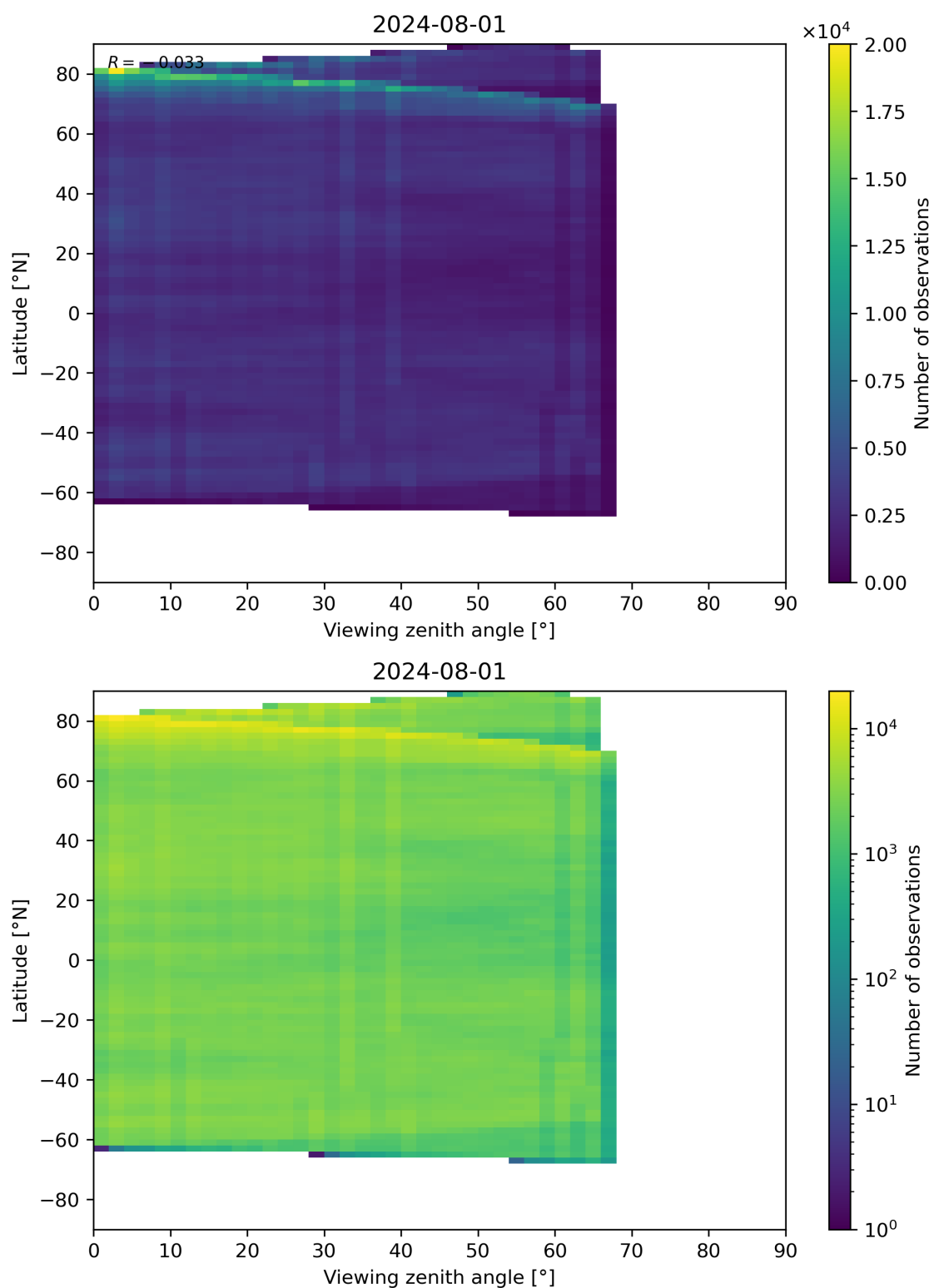
Figure 74: Scatter density plot of “Viewing zenith angle” against “Latitude” for 2024-07-31 to 2024-08-02.
