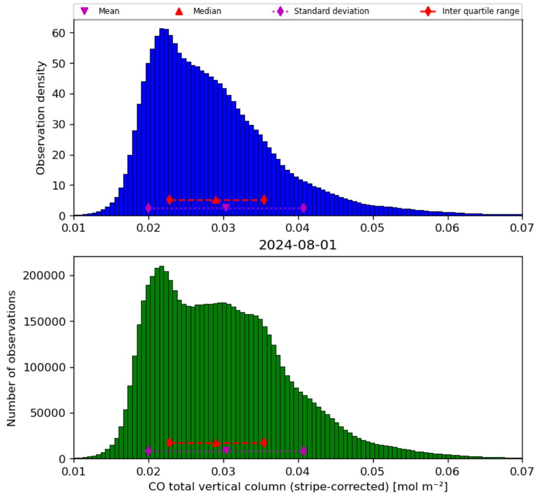
Figure 19: Histogram of “CO total vertical column (stripe-corrected)” for 2024-07-31 to 2024-08-02
