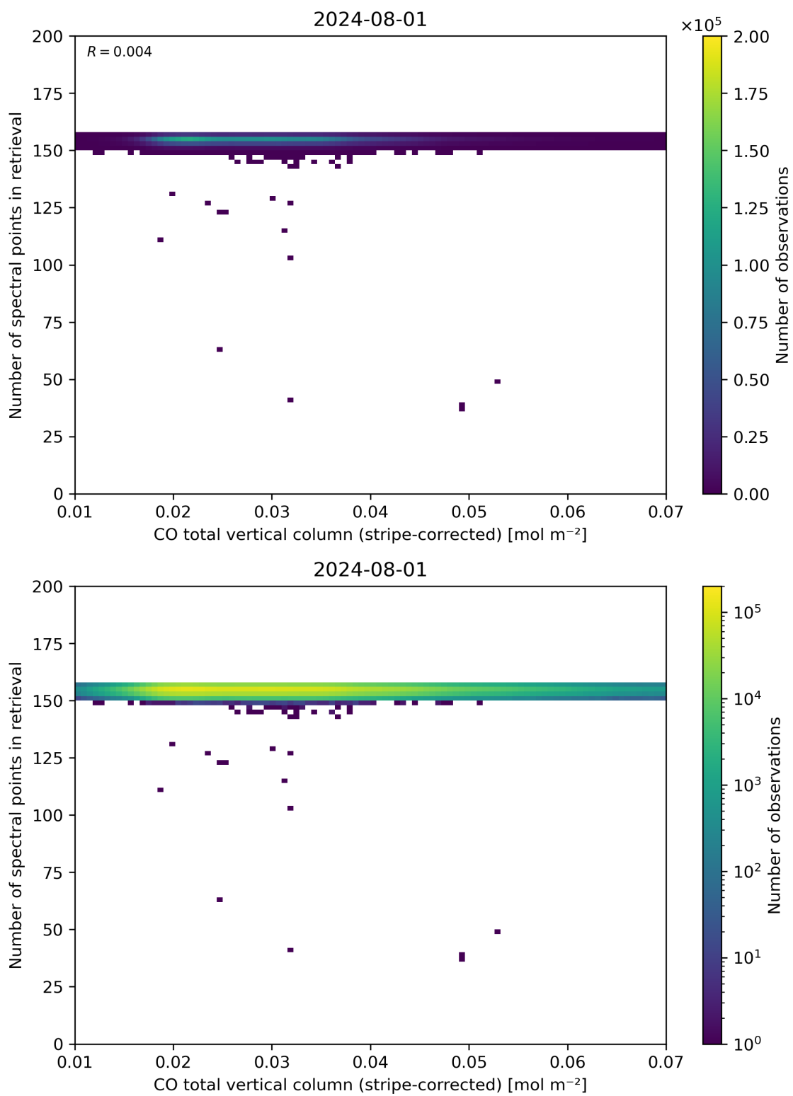
Figure 40: Scatter density plot of “CO total vertical column (stripe-corrected)” against “Number of spectral points in retrieval” for 2024-07-31 to 2024-08-02.
