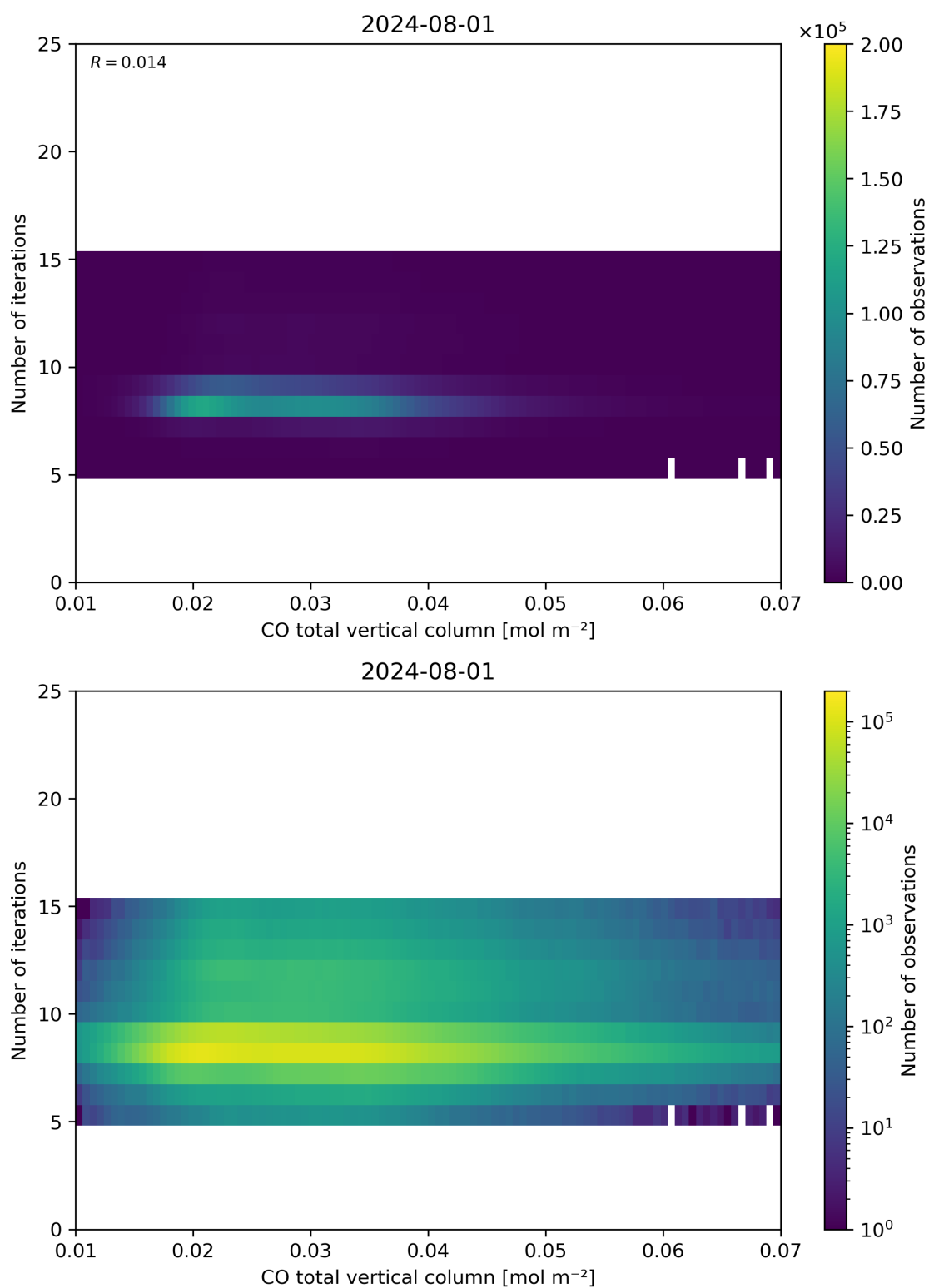
Figure 42: Scatter density plot of “CO total vertical column” against “Number of iterations” for 2024-07-31 to 2024-08-02.
