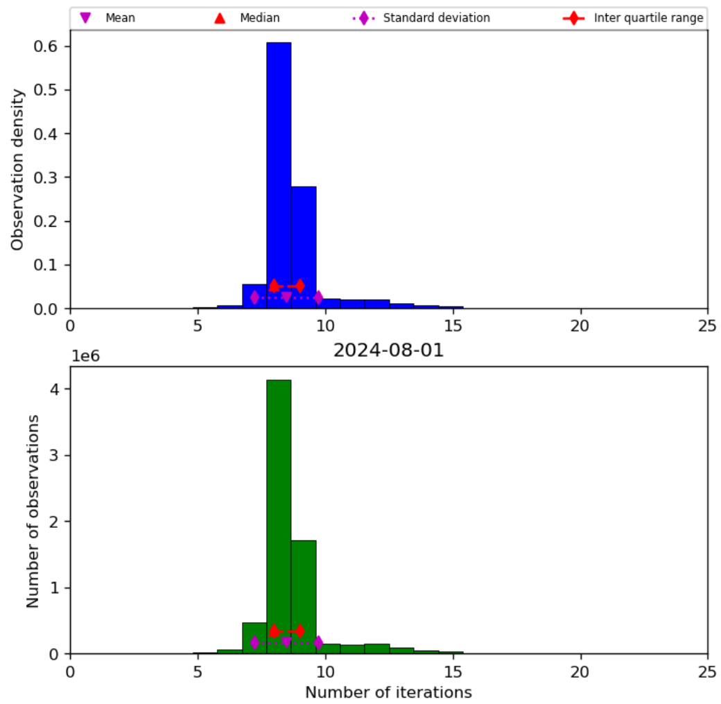
Figure 24: Histogram of “Number of iterations” for 2024-07-31 to 2024-08-02
