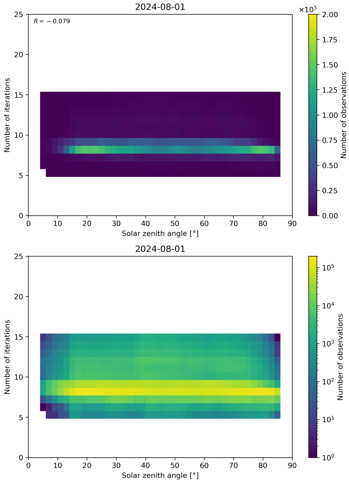
Figure 67: Scatter density plot of “Solar zenith angle” against “Number of iterations” for 2024-07-31 to 2024-08-02.
