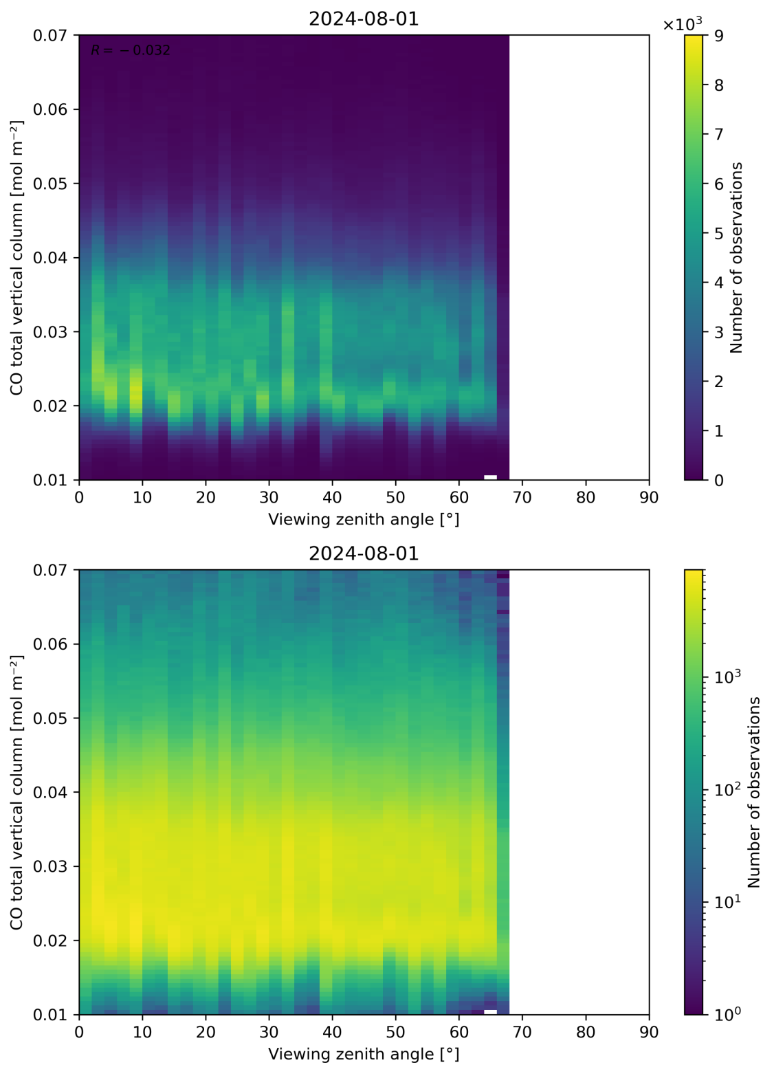
Figure 69: Scatter density plot of “Viewing zenith angle” against “CO total vertical column” for 2024-07-31 to 2024-08-02.
