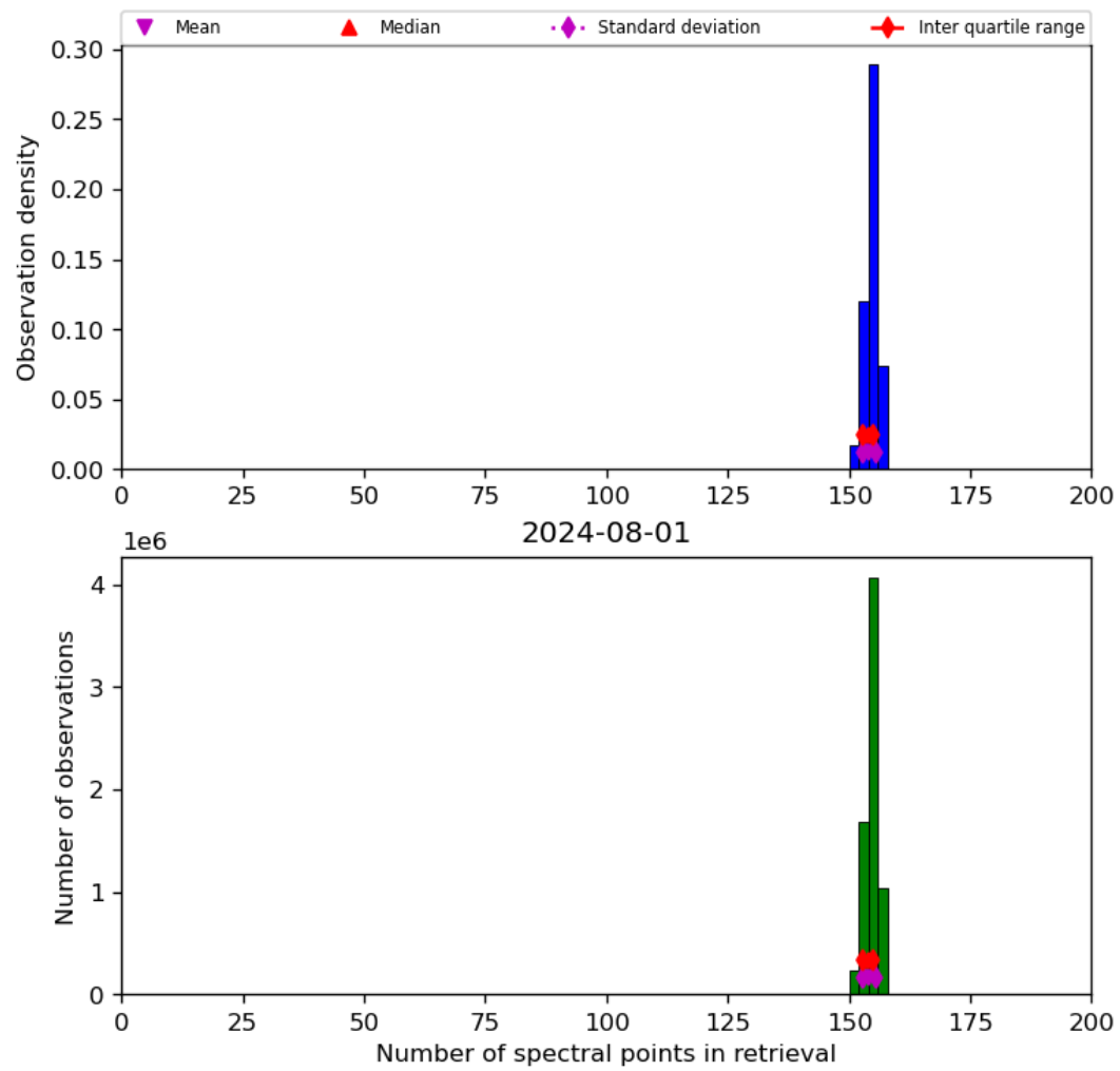
Figure 21: Histogram of “Number of spectral points in retrieval” for 2024-07-31 to 2024-08-02
