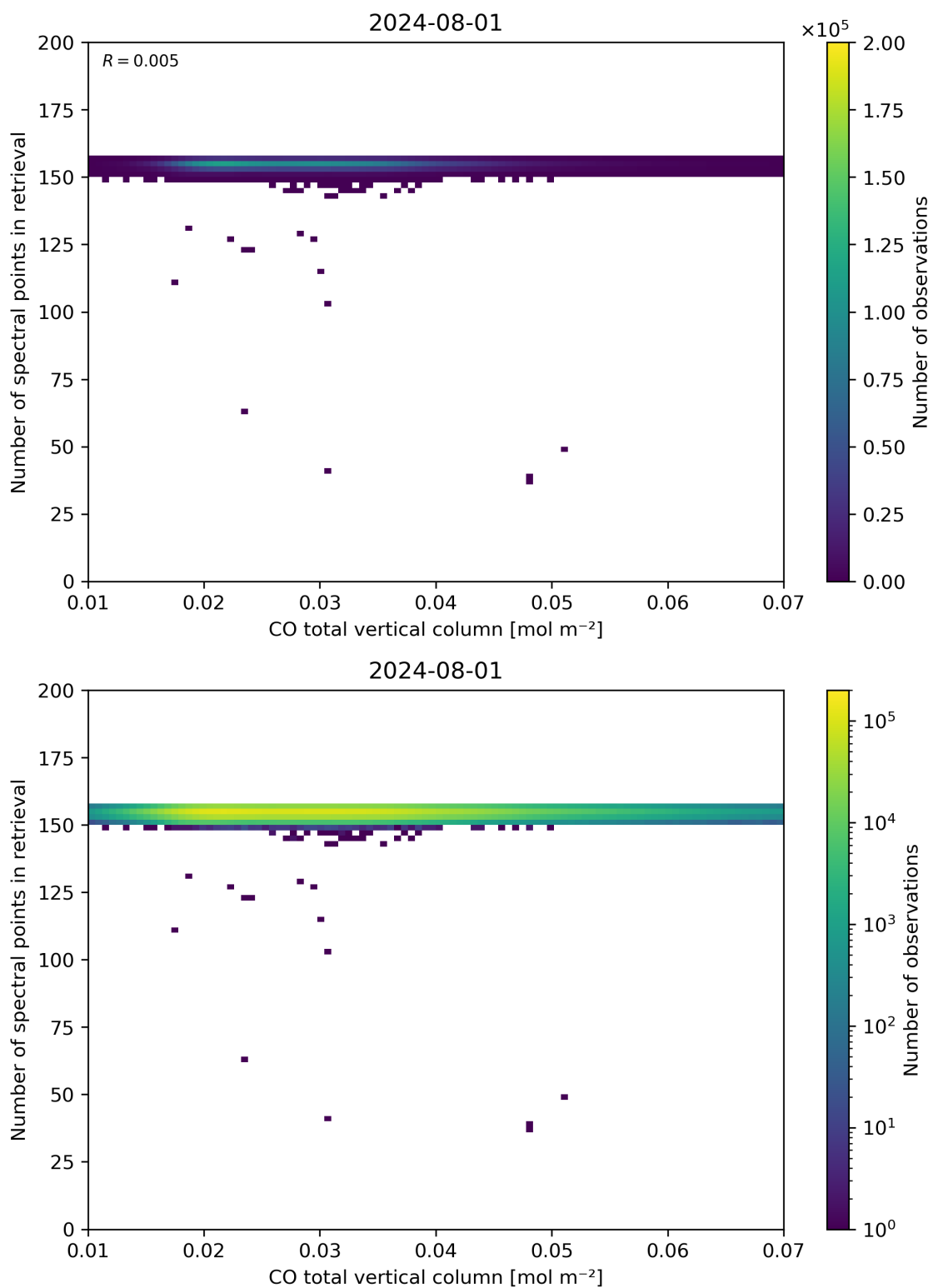
Figure 43: Scatter density plot of “CO total vertical column” against “Number of spectral points in retrieval” for 2024-07-31 to 2024-08-02.
