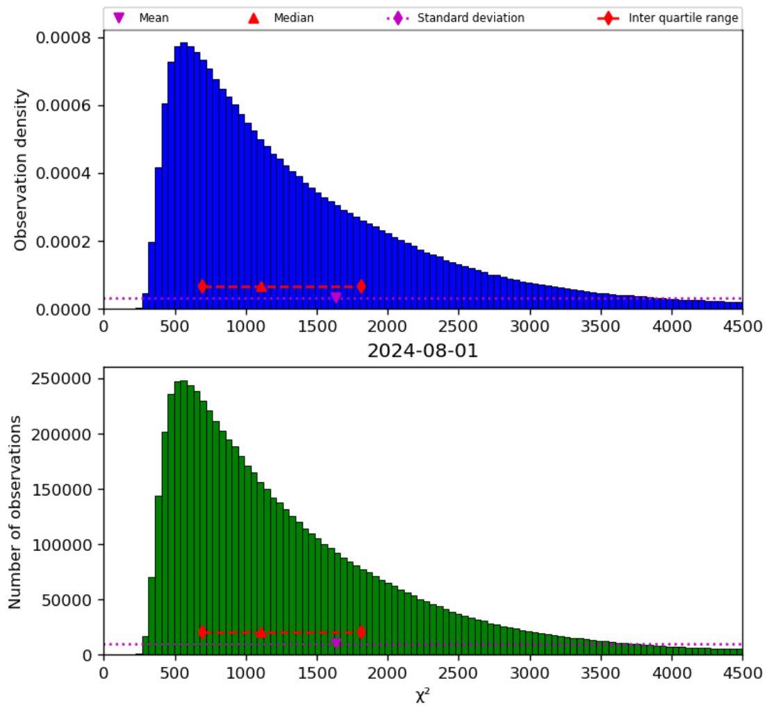
Figure 22: Histogram of “ \chi^2 ” for 2024-07-31 to 2024-08-02
