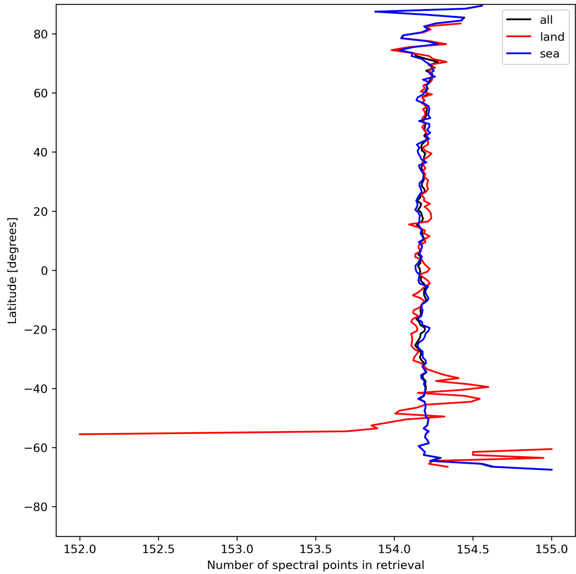
Figure 13: Zonal average of “Number of spectral points in retrieval” for 2024-07-31 to 2024-08-02.
