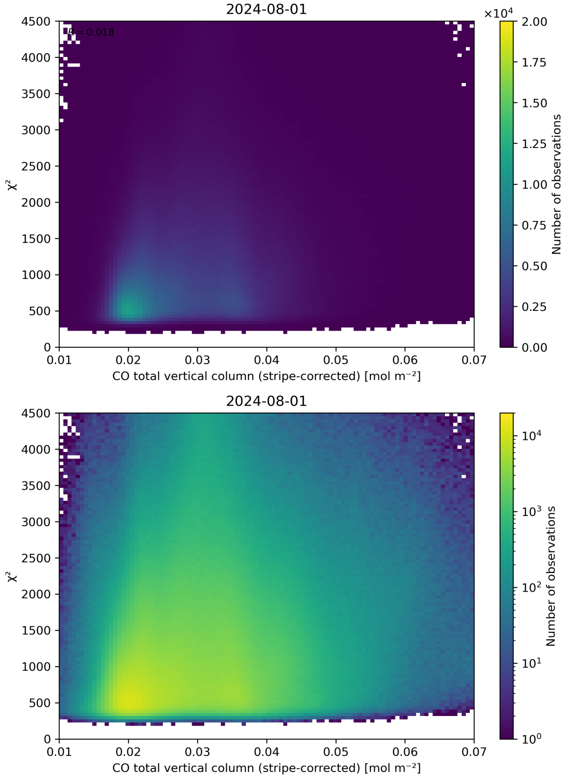
Figure 37: Scatter density plot of “CO total vertical column (stripe-corrected)” against “ \chi^2 ” for 2024-07-31 to 2024-08-02.
