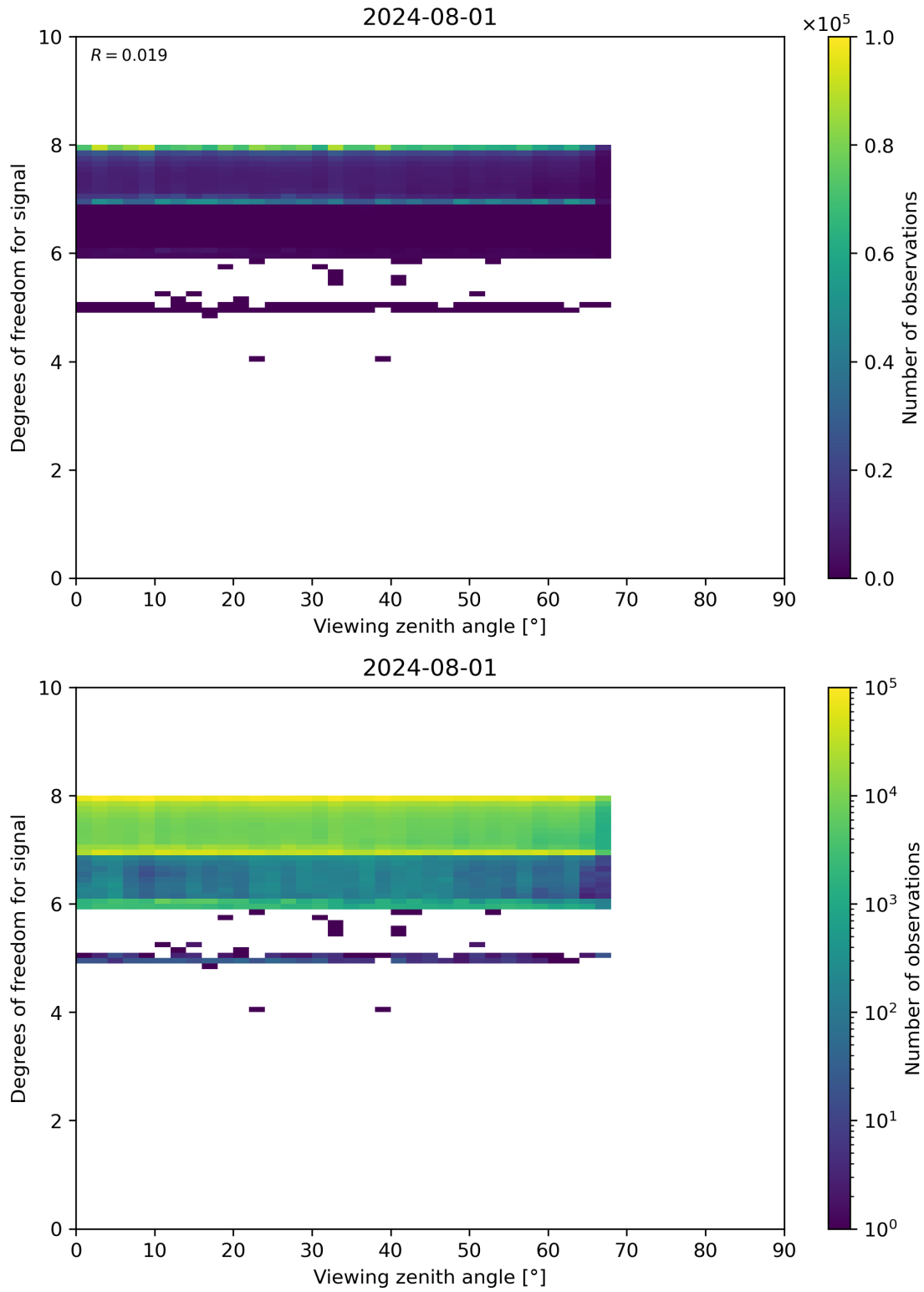
Figure 73: Scatter density plot of “Viewing zenith angle” against “Degrees of freedom for signal” for 2024-07-31 to 2024-08-02.
