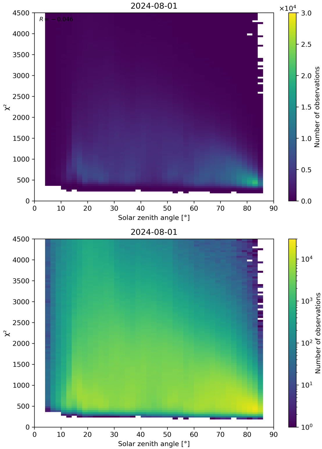
Figure 64: Scatter density plot of “Solar zenith angle” against “ \chi^2 ” for 2024-07-31 to 2024-08-02.
