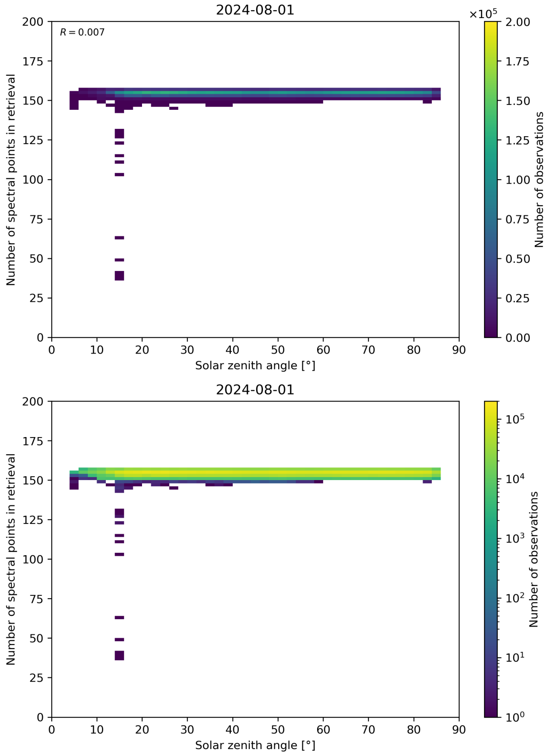
Figure 68: Scatter density plot of “Solar zenith angle” against “Number of spectral points in retrieval” for 2024-07-31 to 2024-08-02.
