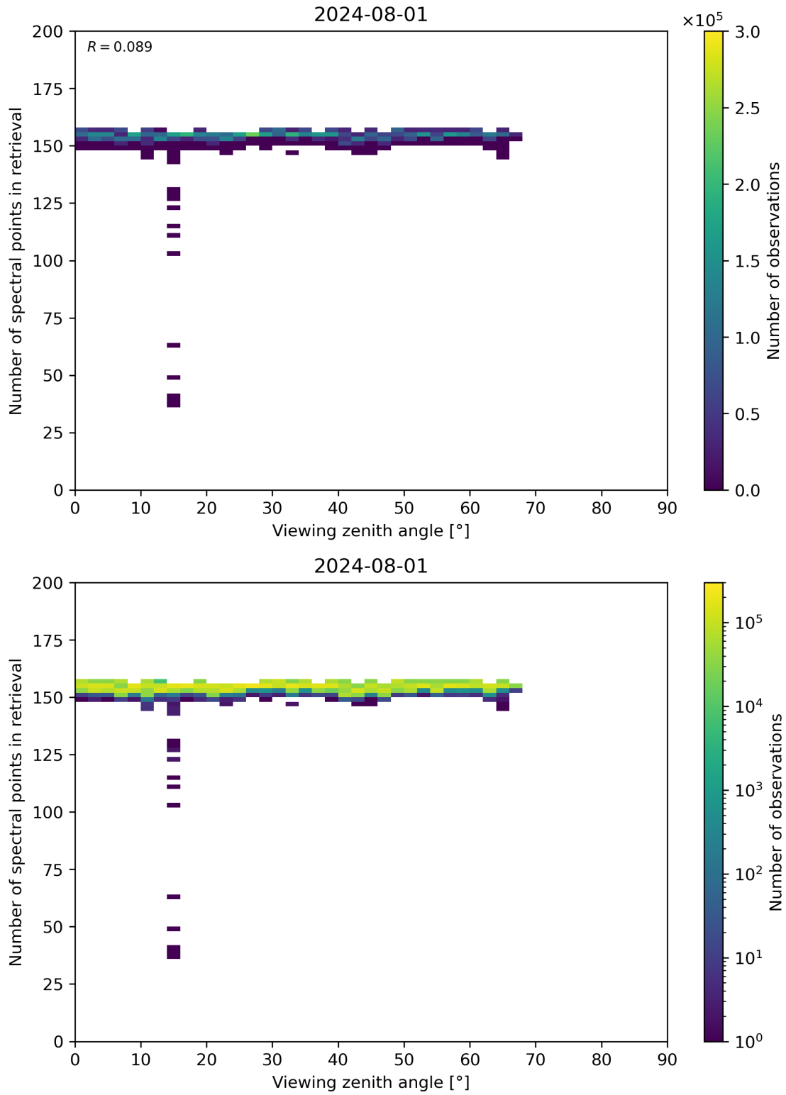
Figure 76: Scatter density plot of “Viewing zenith angle” against “Number of spectral points in retrieval” for 2024-07-31 to 2024-08-02.
