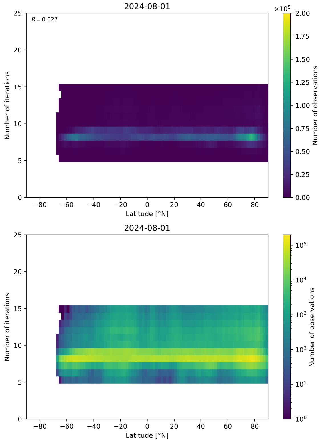
Figure 56: Scatter density plot of “Latitude” against “Number of iterations” for 2024-07-31 to 2024-08-02.
