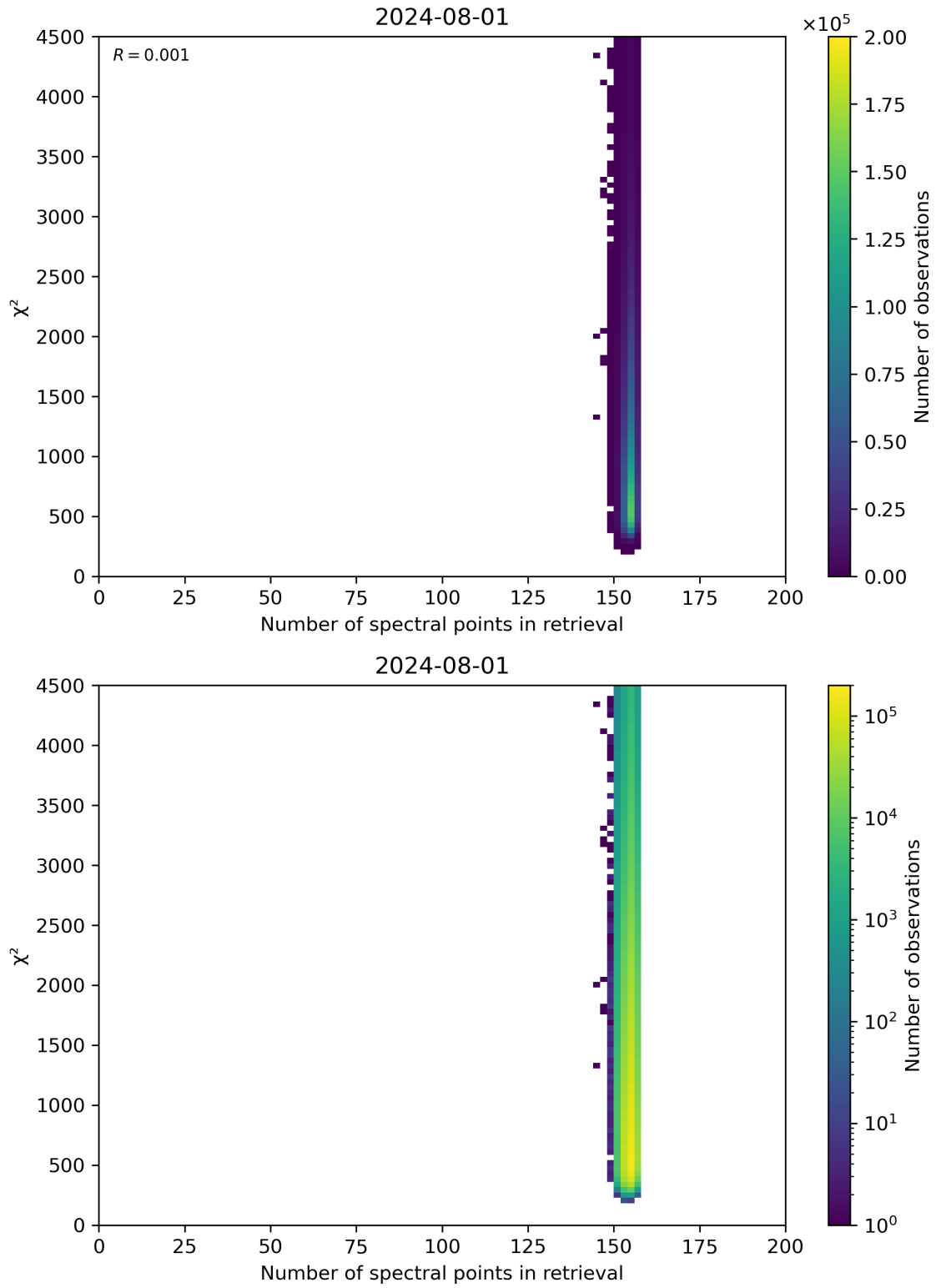
Figure 58: Scatter density plot of “Number of spectral points in retrieval” against “ \chi^2 ” for 2024-07-31 to 2024-08-02.
