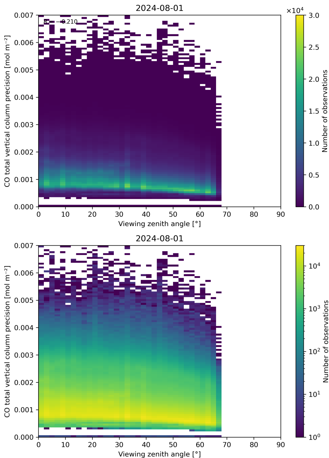
Figure 71: Scatter density plot of “Viewing zenith angle” against “CO total vertical column precision” for 2024-07-31 to 2024-08-02.
