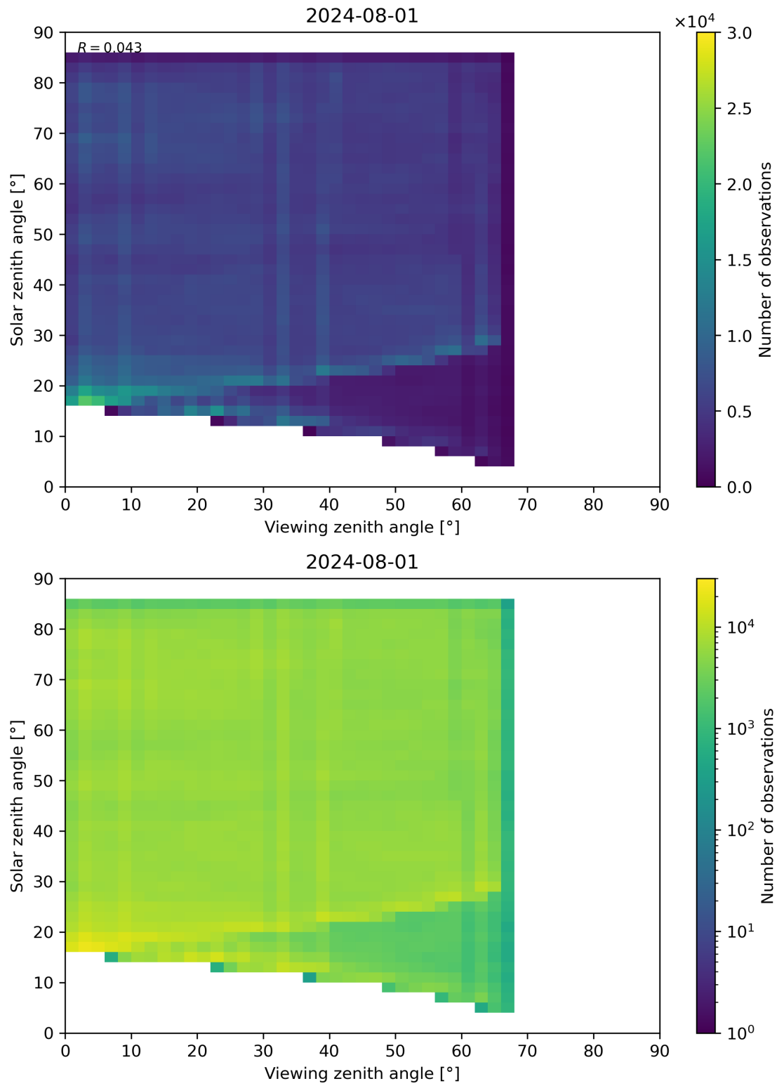
Figure 77: Scatter density plot of “Viewing zenith angle” against “Solar zenith angle” for 2024-07-31 to 2024-08-02.
