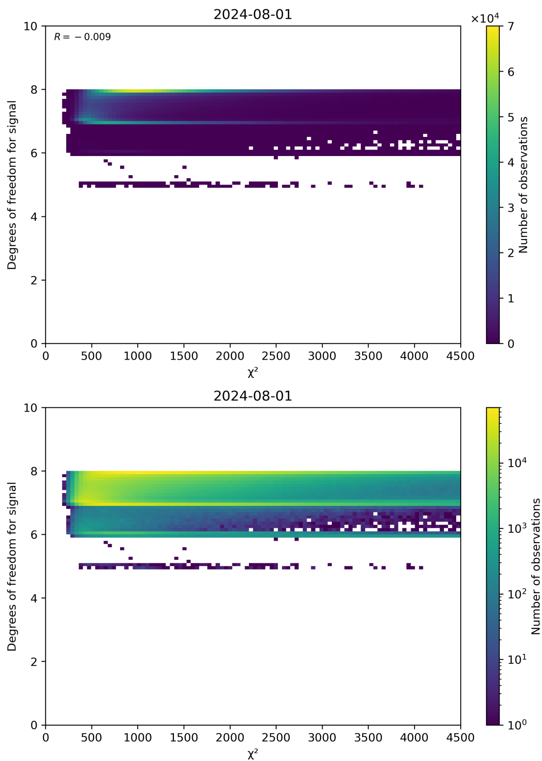
Figure 48: Scatter density plot of " \chi^2 " against "Degrees of freedom for signal" for 2024-07-31 to 2024-08-02.
