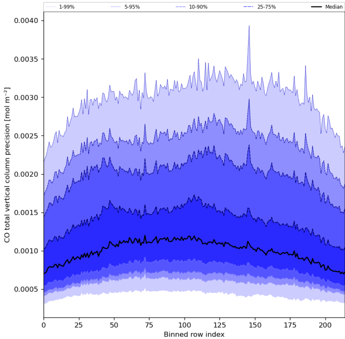
Figure 28: Along track statistics of “CO total vertical column precision” for 2024-07-31 to 2024-08-02
