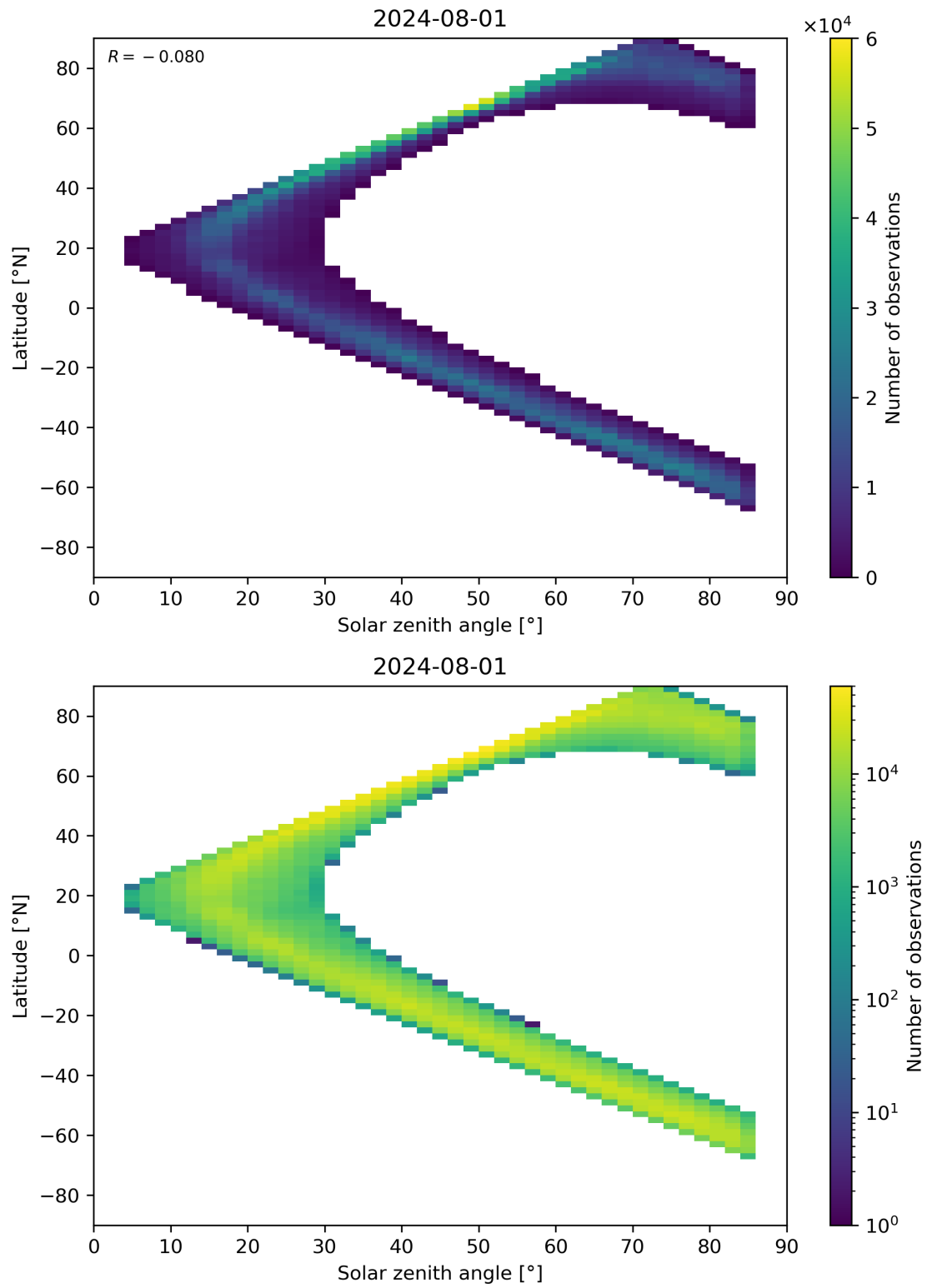
Figure 66: Scatter density plot of “Solar zenith angle” against “Latitude” for 2024-07-31 to 2024-08-02.
