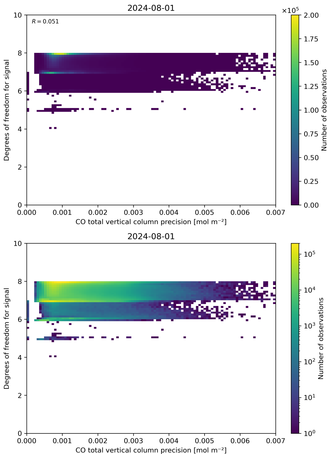
Figure 45: Scatter density plot of “CO total vertical column precision” against “Degrees of freedom for signal” for 2024-07-31 to 2024-08-02.
