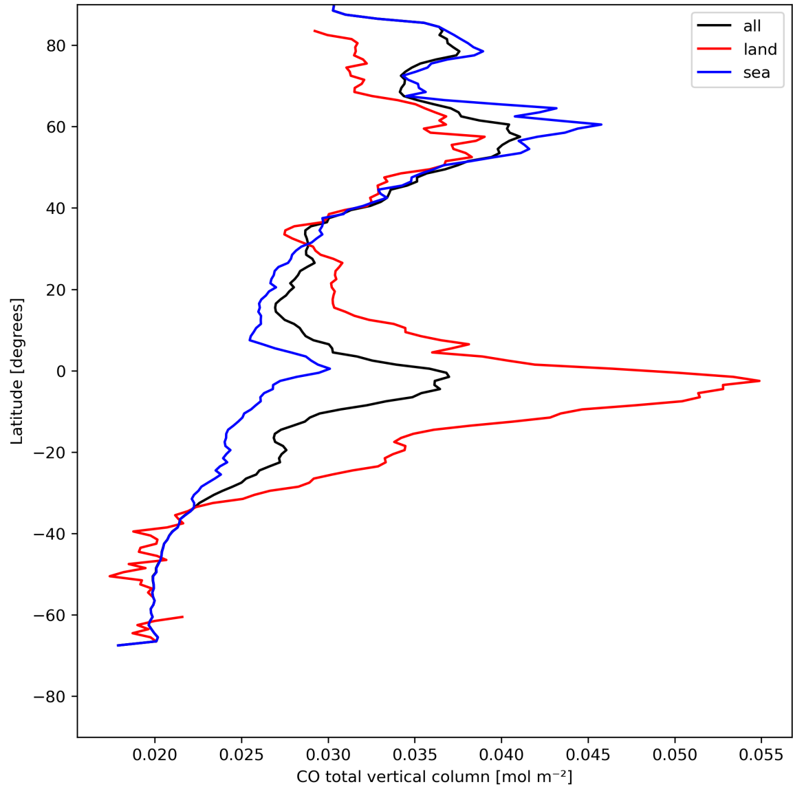
Figure 10: Zonal average of “CO total vertical column” for 2024-07-31 to 2024-08-02.
