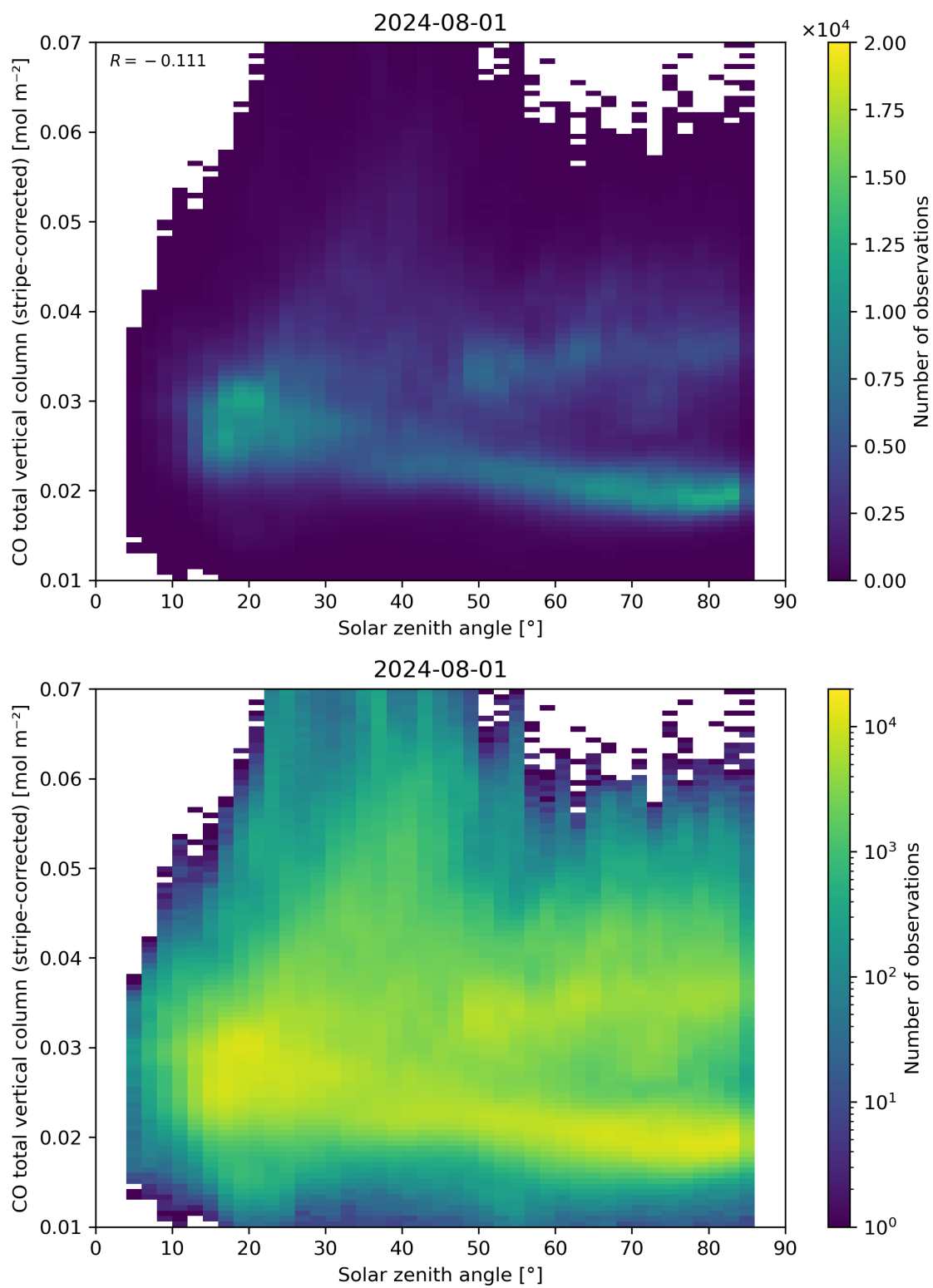
Figure 62: Scatter density plot of “Solar zenith angle” against “CO total vertical column (stripe-corrected)” for 2024-07-31 to 2024-08-02.
