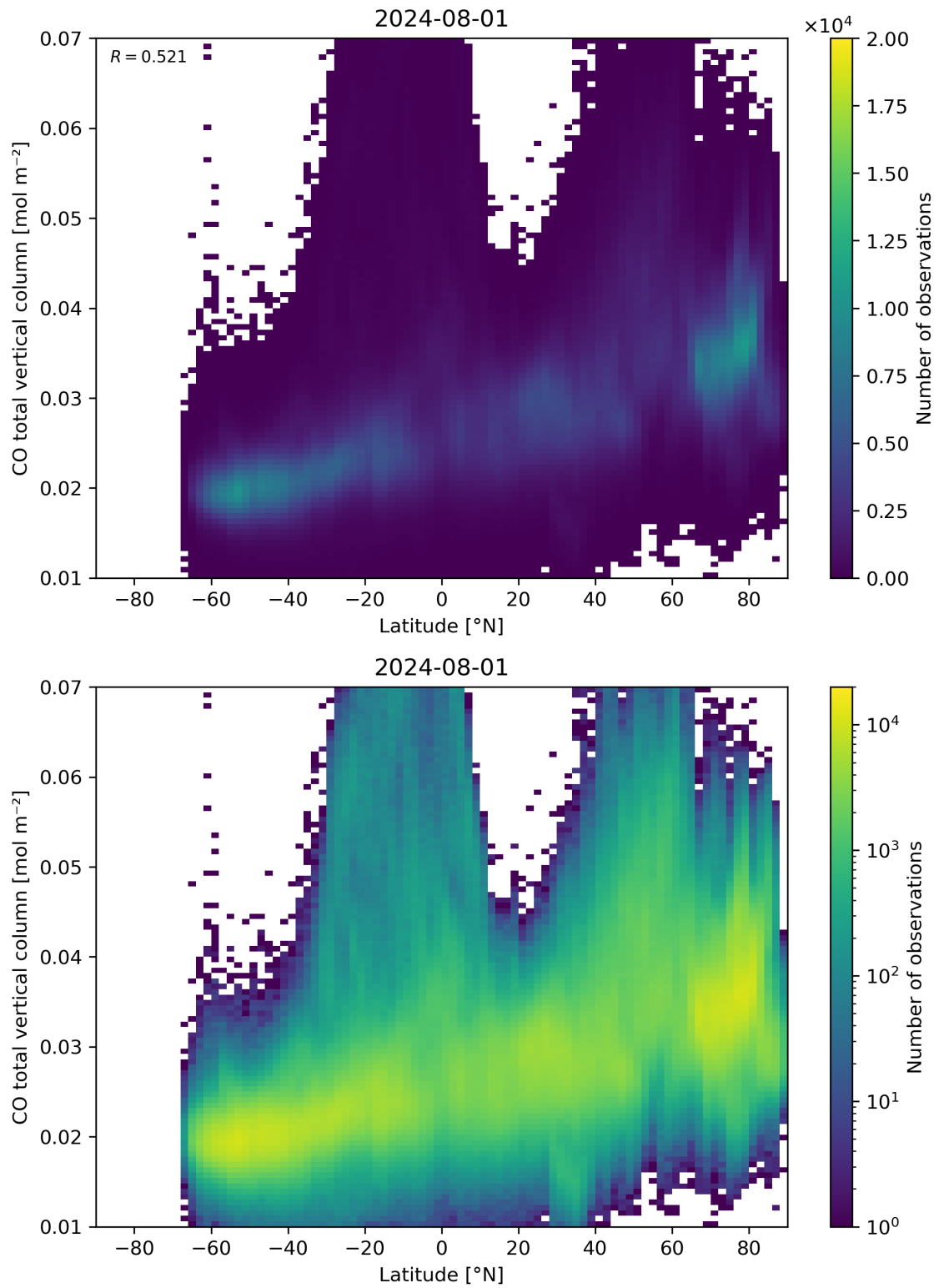
Figure 51: Scatter density plot of “Latitude” against “CO total vertical column” for 2024-07-31 to 2024-08-02.
