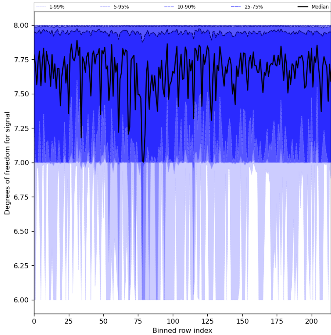
Figure 31: Along track statistics of “Degrees of freedom for signal” for 2024-07-31 to 2024-08-02
