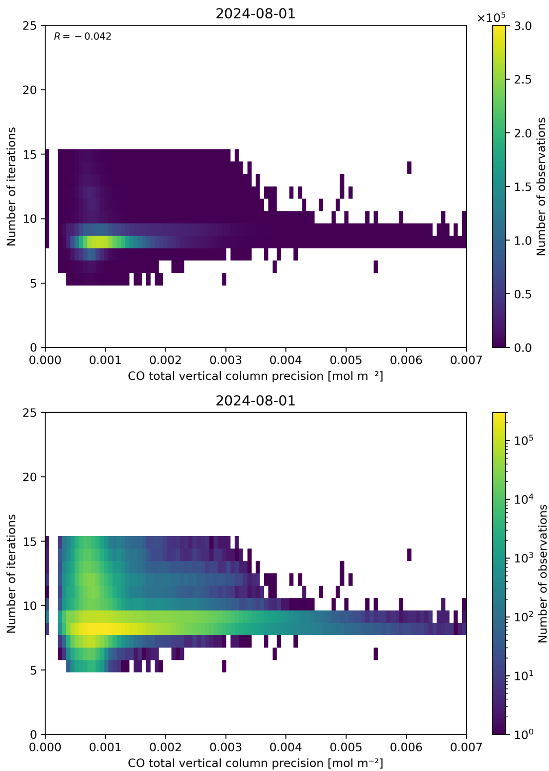
Figure 46: Scatter density plot of “CO total vertical column precision” against “Number of iterations” for 2024-07-31 to 2024-08-02.
