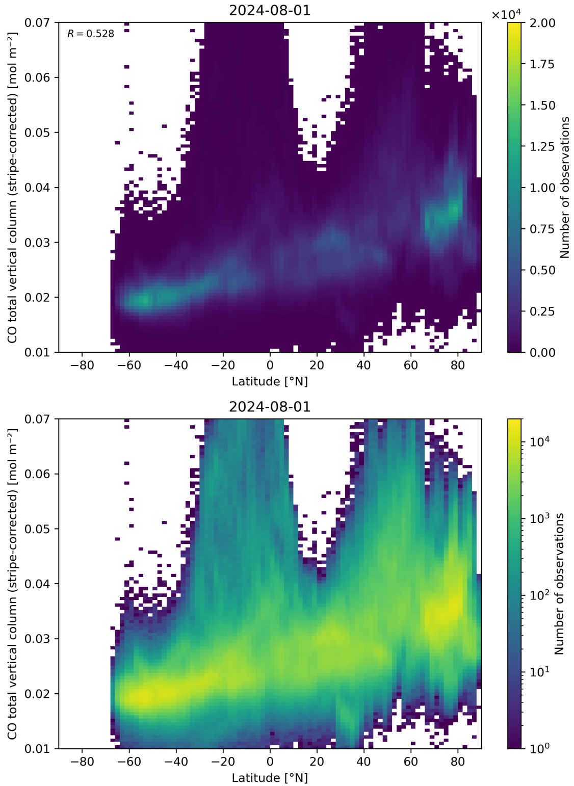
Figure 52: Scatter density plot of “Latitude” against “CO total vertical column (stripe-corrected)” for 2024-07-31 to 2024-08-02.
