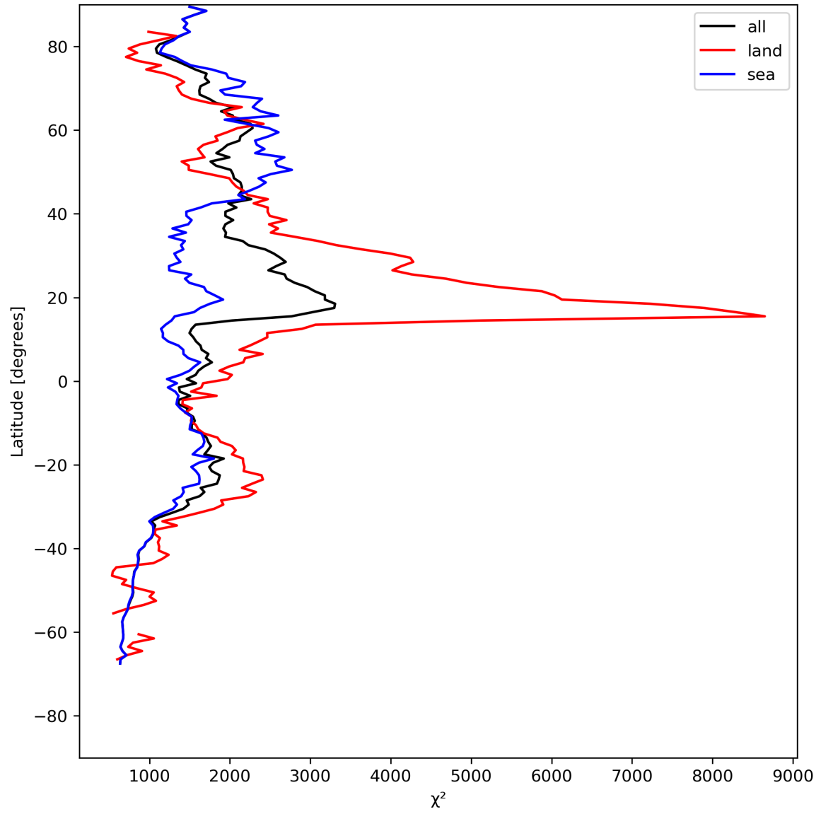
Figure 14: Zonal average of “ \chi^2 ” for 2024-07-31 to 2024-08-02.
