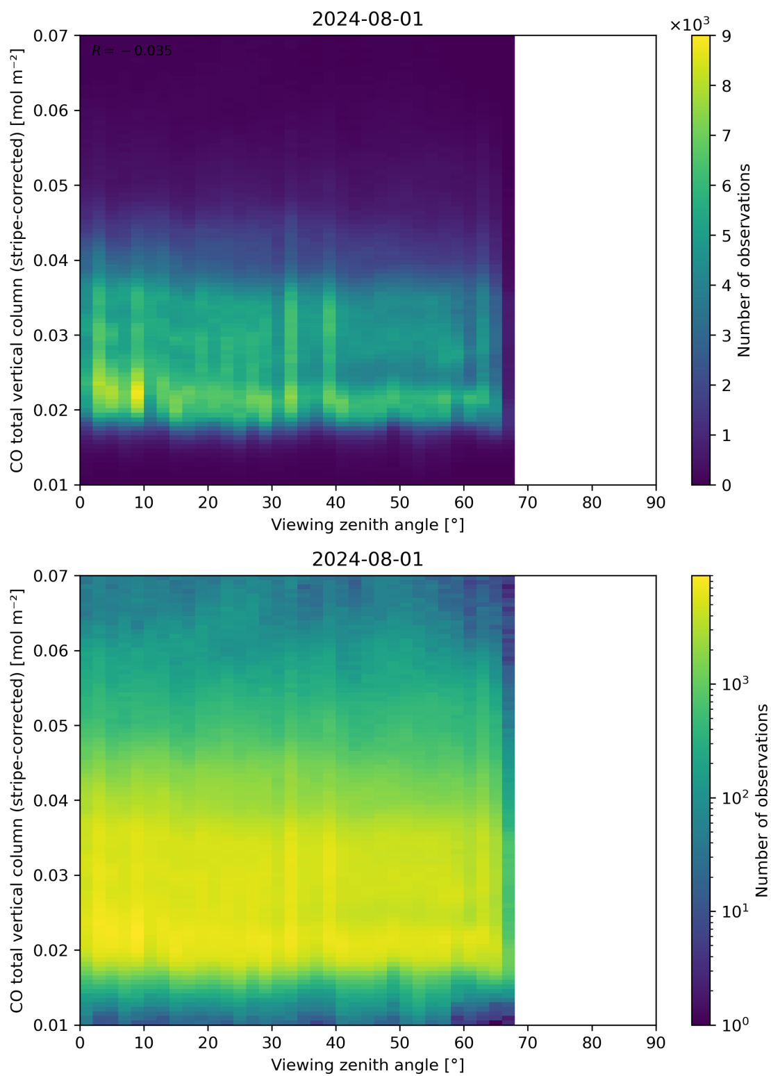
Figure 70: Scatter density plot of “Viewing zenith angle” against “CO total vertical column (stripe-corrected)” for 2024-07-31 to 2024-08-02.
