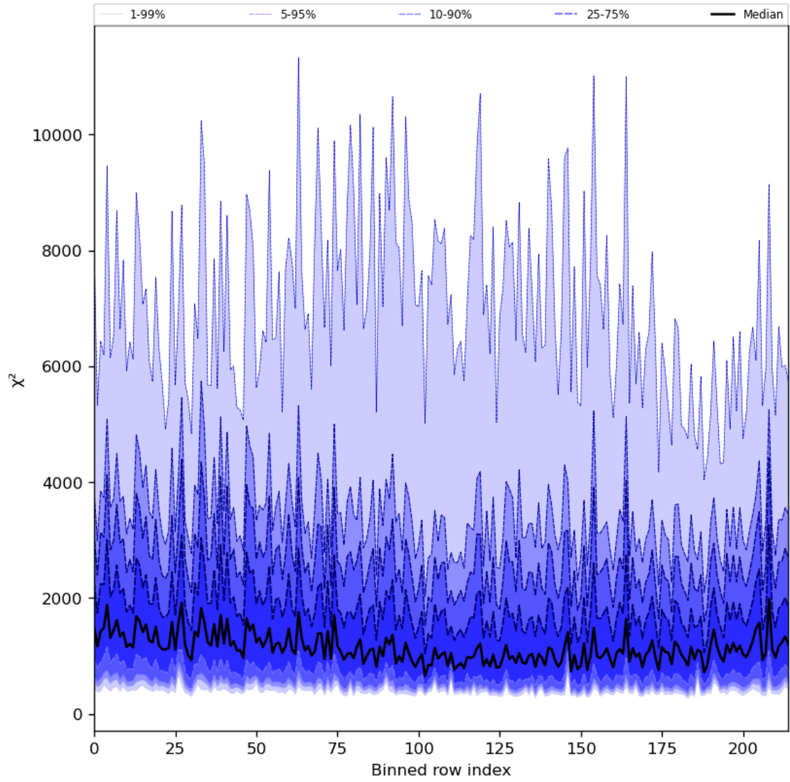
Figure 30: Along track statistics of “ \chi^2 ” for 2024-08-02 to 2024-08-04
