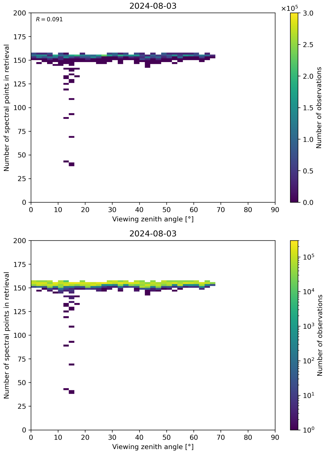
Figure 76: Scatter density plot of “Viewing zenith angle” against “Number of spectral points in retrieval” for 2024-08-02 to 2024-08-04.
