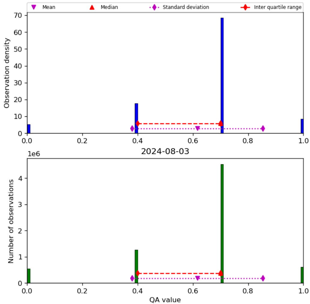
Figure 17: Histogram of “QA value” for 2024-08-02 to 2024-08-04
