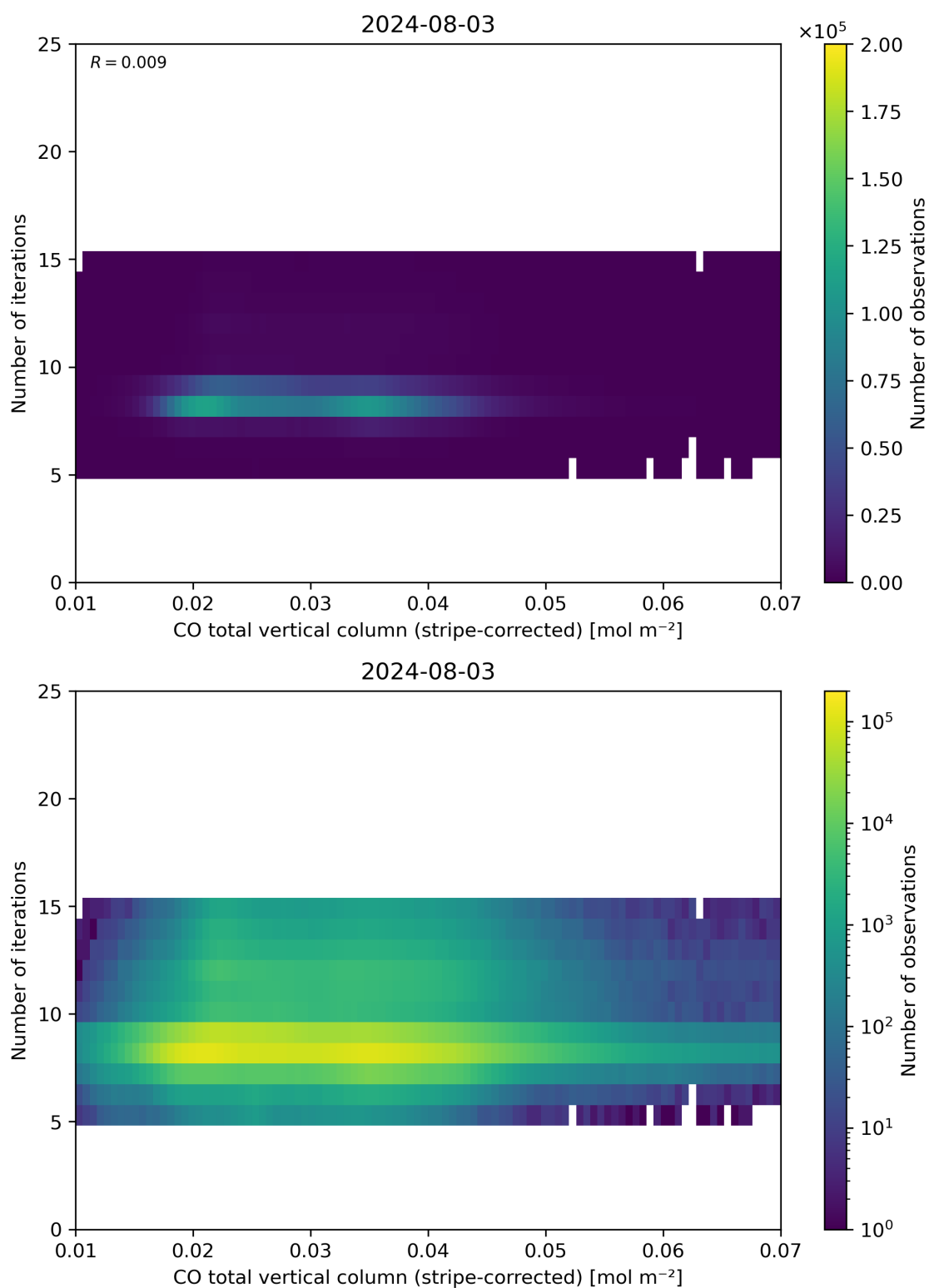
Figure 39: Scatter density plot of “CO total vertical column (stripe-corrected)” against “Number of iterations” for 2024-08-02 to 2024-08-04.
