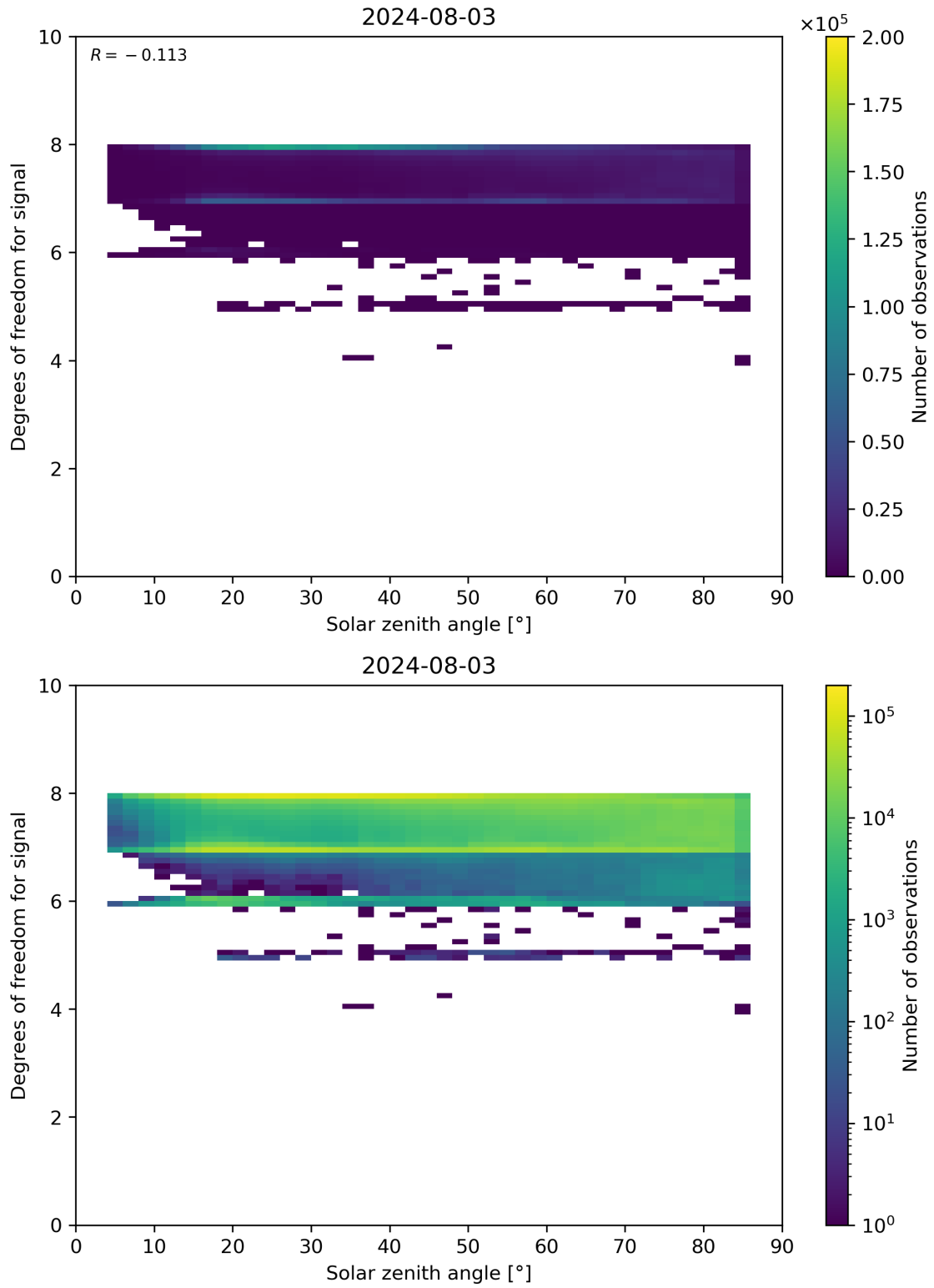
Figure 65: Scatter density plot of “Solar zenith angle” against “Degrees of freedom for signal” for 2024-08-02 to 2024-08-04.
