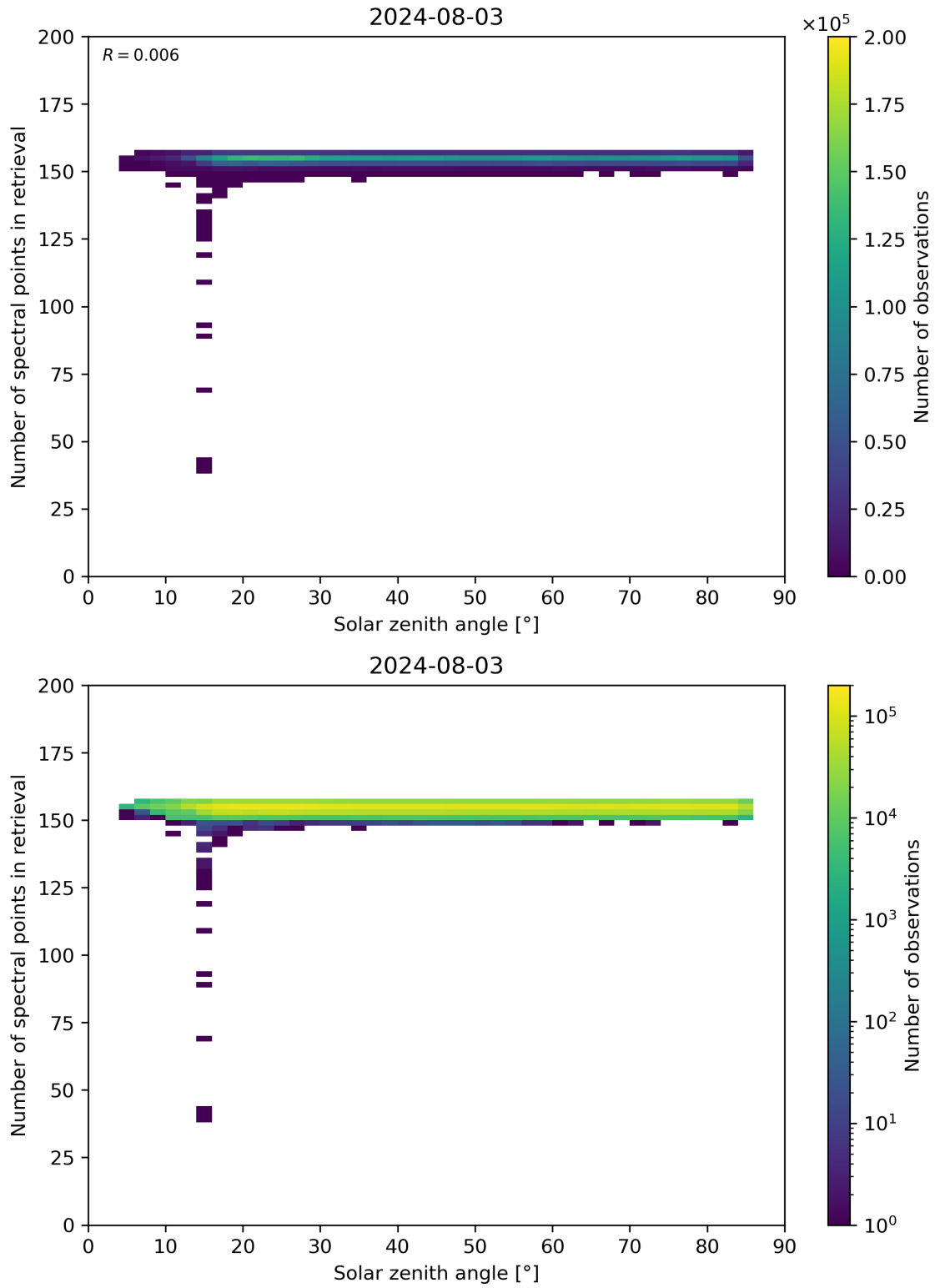
Figure 68: Scatter density plot of “Solar zenith angle” against “Number of spectral points in retrieval” for 2024-08-02 to 2024-08-04.
