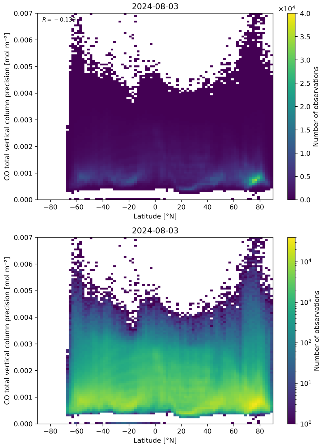
Figure 53: Scatter density plot of “Latitude” against “CO total vertical column precision” for 2024-08-02 to 2024-08-04.
