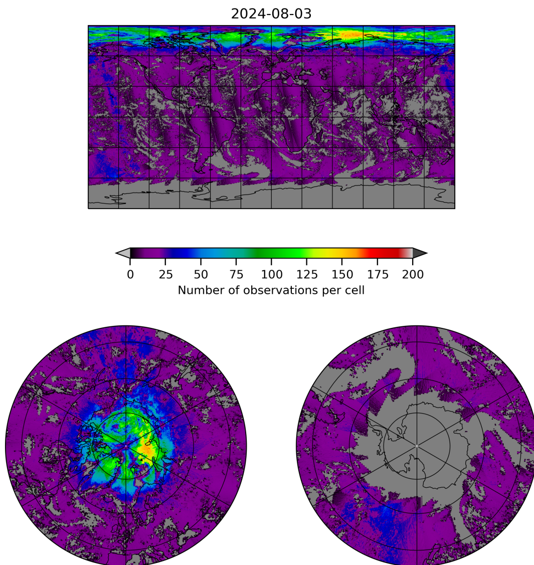
Figure 8: Map of the number of observations for 2024-08-02 to 2024-08-04
