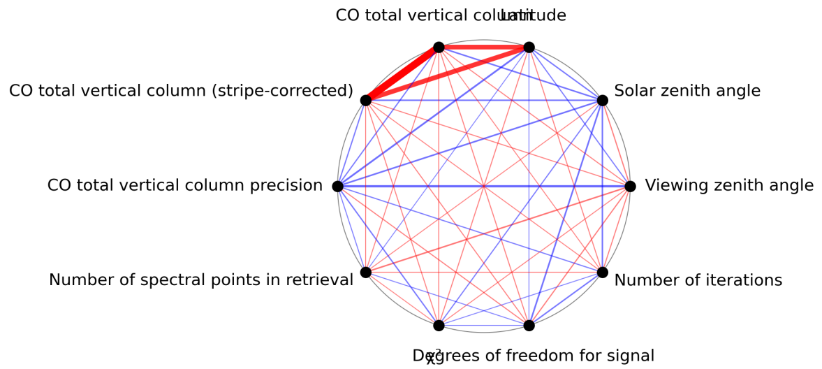
Figure 1: Map of correlation graph for 2024-08-02 to 2024-08-04.
