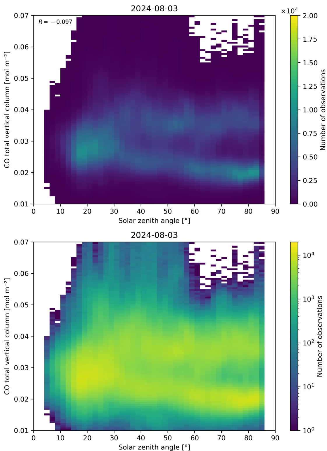
Figure 61: Scatter density plot of “Solar zenith angle” against “CO total vertical column” for 2024-08-02 to 2024-08-04.
