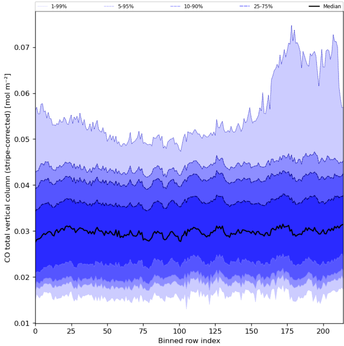
Figure 27: Along track statistics of “CO total vertical column (stripe-corrected)” for 2024-08-02 to 2024-08-04
