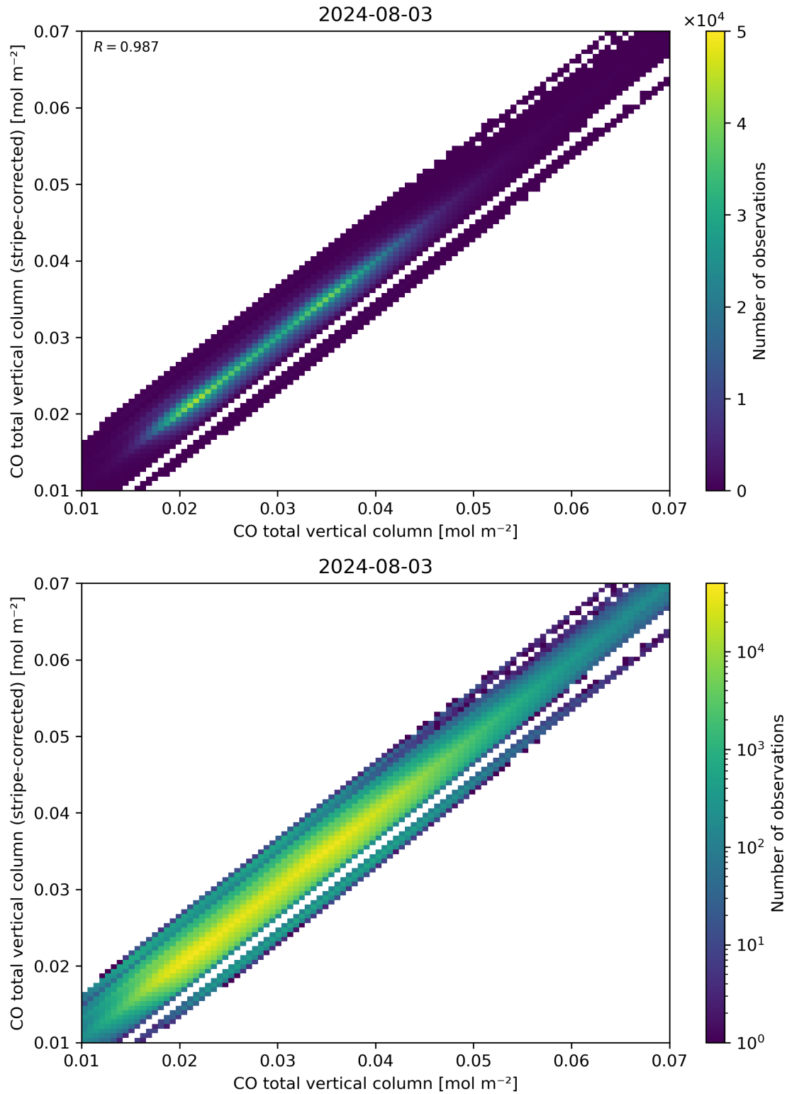
Figure 33: Scatter density plot of “CO total vertical column” against “CO total vertical column (stripe-corrected)” for 2024-08-02 to 2024-08-04.
