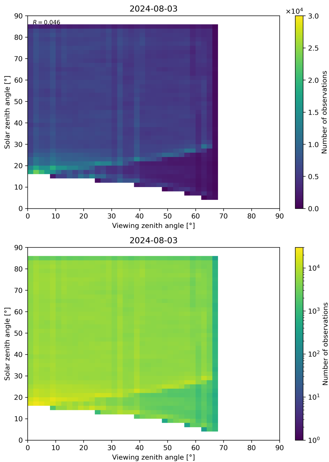
Figure 77: Scatter density plot of “Viewing zenith angle” against “Solar zenith angle” for 2024-08-02 to 2024-08-04.
