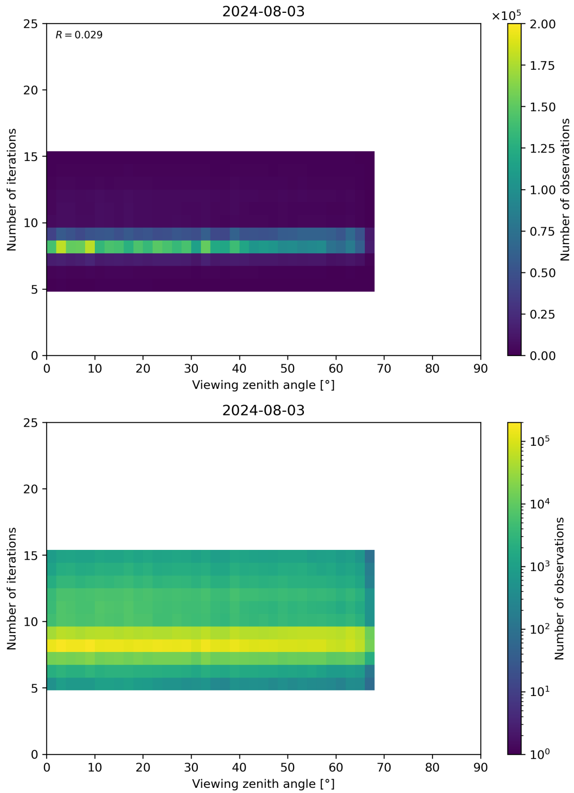
Figure 75: Scatter density plot of “Viewing zenith angle” against “Number of iterations” for 2024-08-02 to 2024-08-04.
