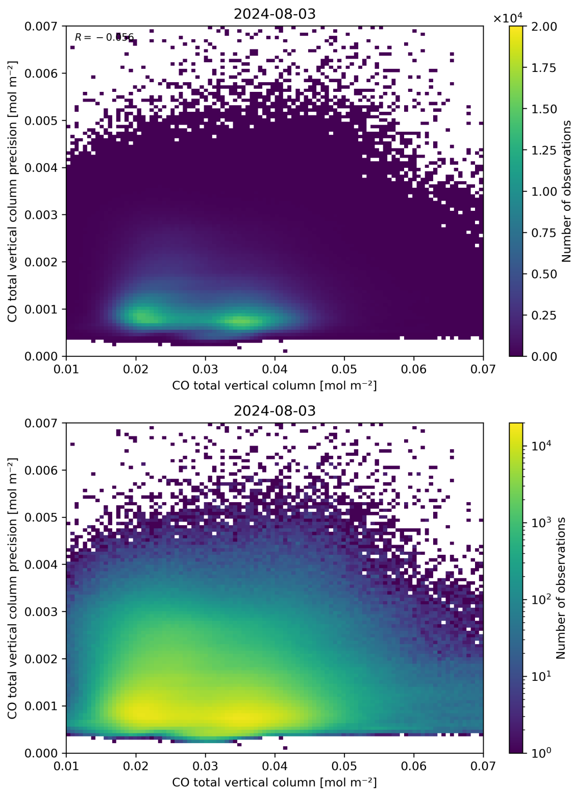
Figure 34: Scatter density plot of “CO total vertical column” against “CO total vertical column precision” for 2024-08-02 to 2024-08-04.
