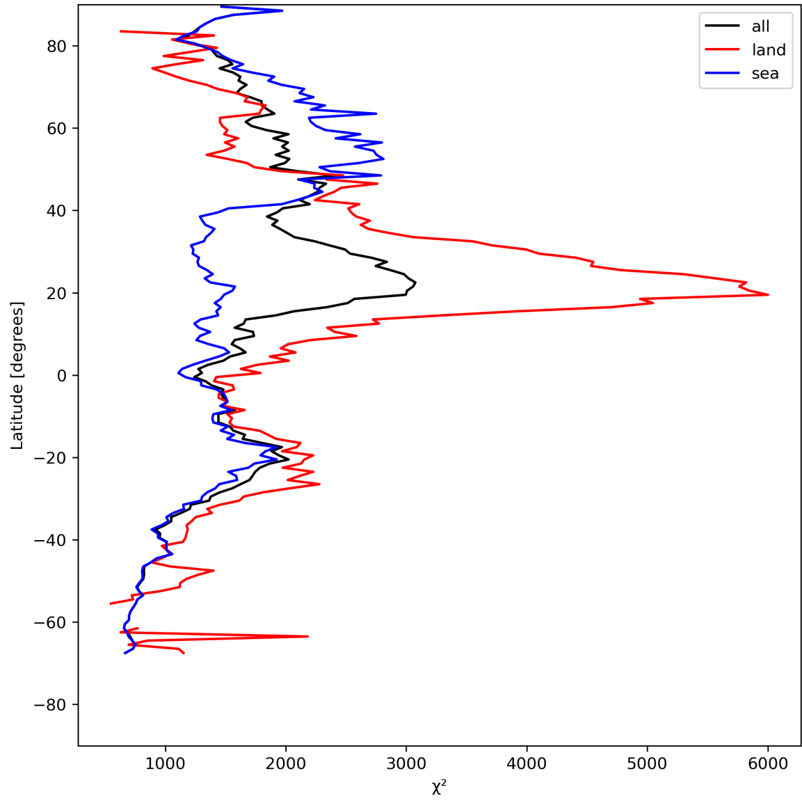
Figure 14: Zonal average of “ \chi^2 ” for 2024-08-02 to 2024-08-04.
