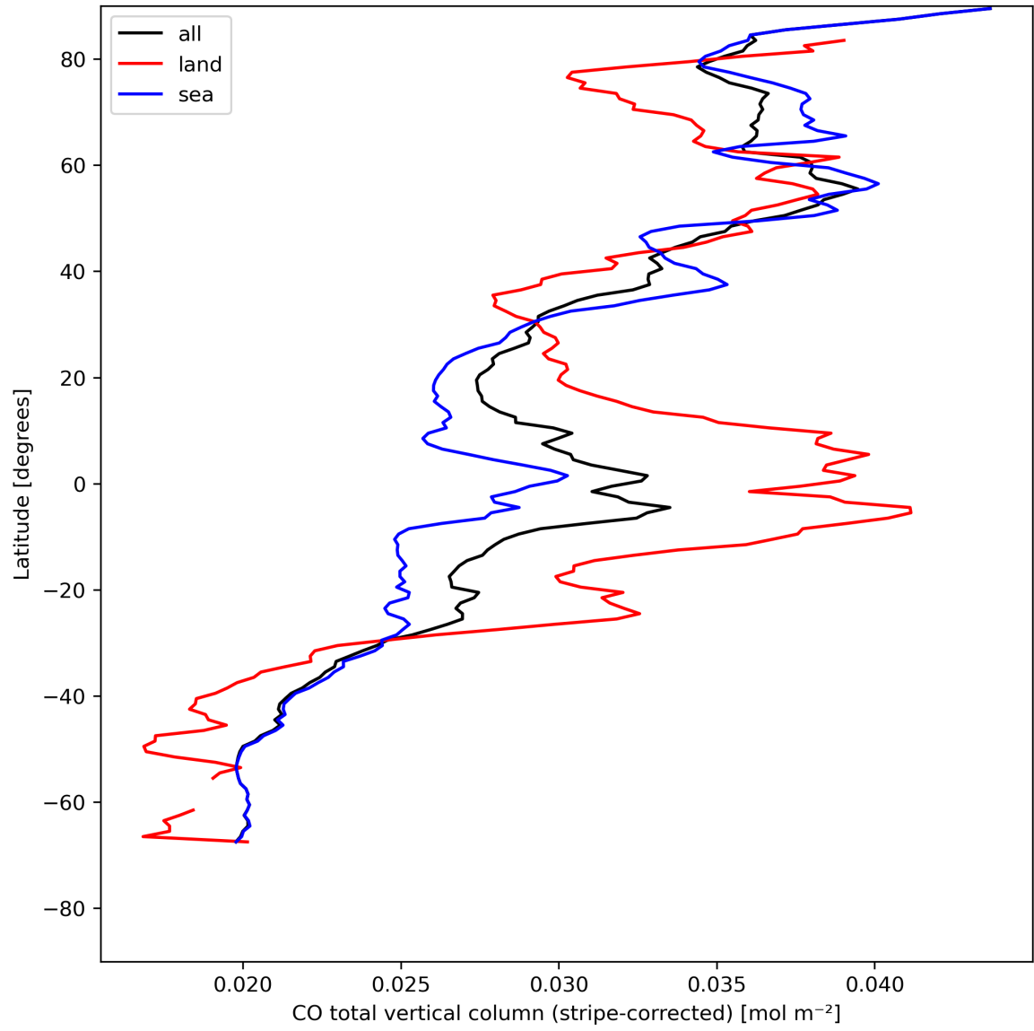
Figure 11: Zonal average of “CO total vertical column (stripe-corrected)” for 2024-08-02 to 2024-08-04.
