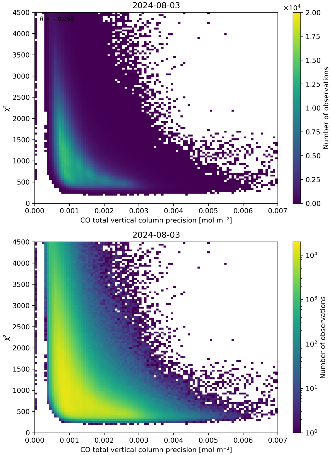
Figure 44: Scatter density plot of “CO total vertical column precision” against “ \chi^2 ” for 2024-08-02 to 2024-08-04.
