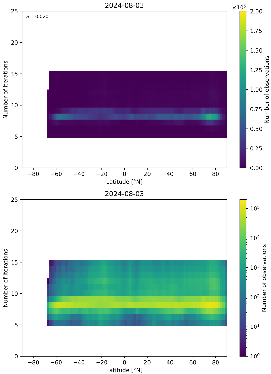
Figure 56: Scatter density plot of “Latitude” against “Number of iterations” for 2024-08-02 to 2024-08-04.
