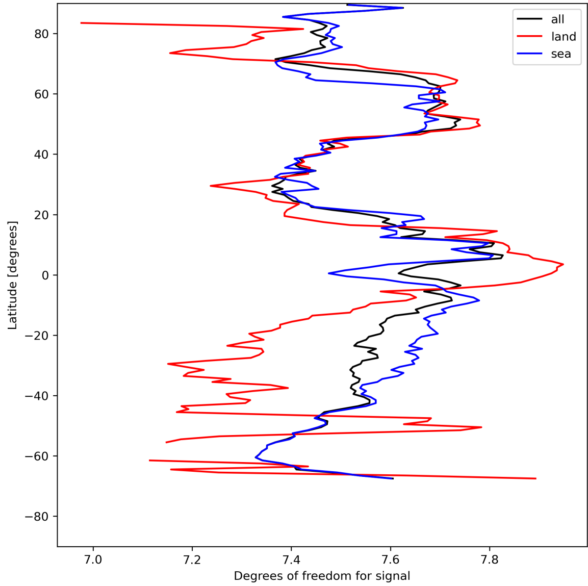
Figure 15: Zonal average of “Degrees of freedom for signal” for 2024-08-02 to 2024-08-04.
