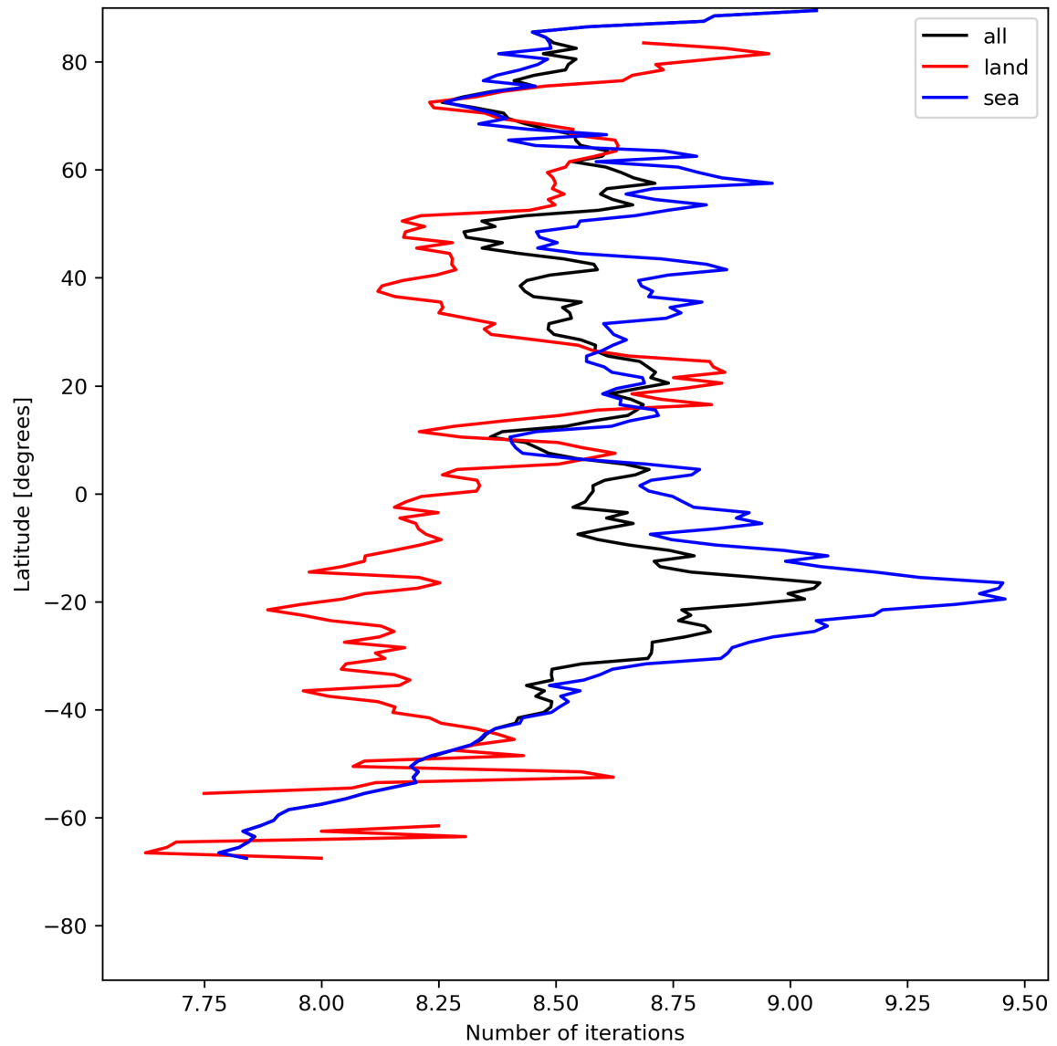
Figure 16: Zonal average of “Number of iterations” for 2024-08-02 to 2024-08-04.
