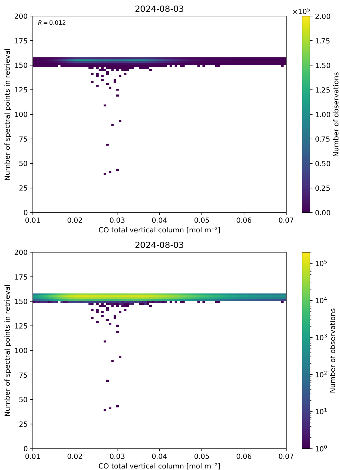
Figure 43: Scatter density plot of “CO total vertical column” against “Number of spectral points in retrieval” for 2024-08-02 to 2024-08-04.
