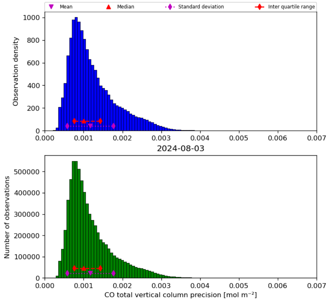
Figure 20: Histogram of “CO total vertical column precision” for 2024-08-02 to 2024-08-04
