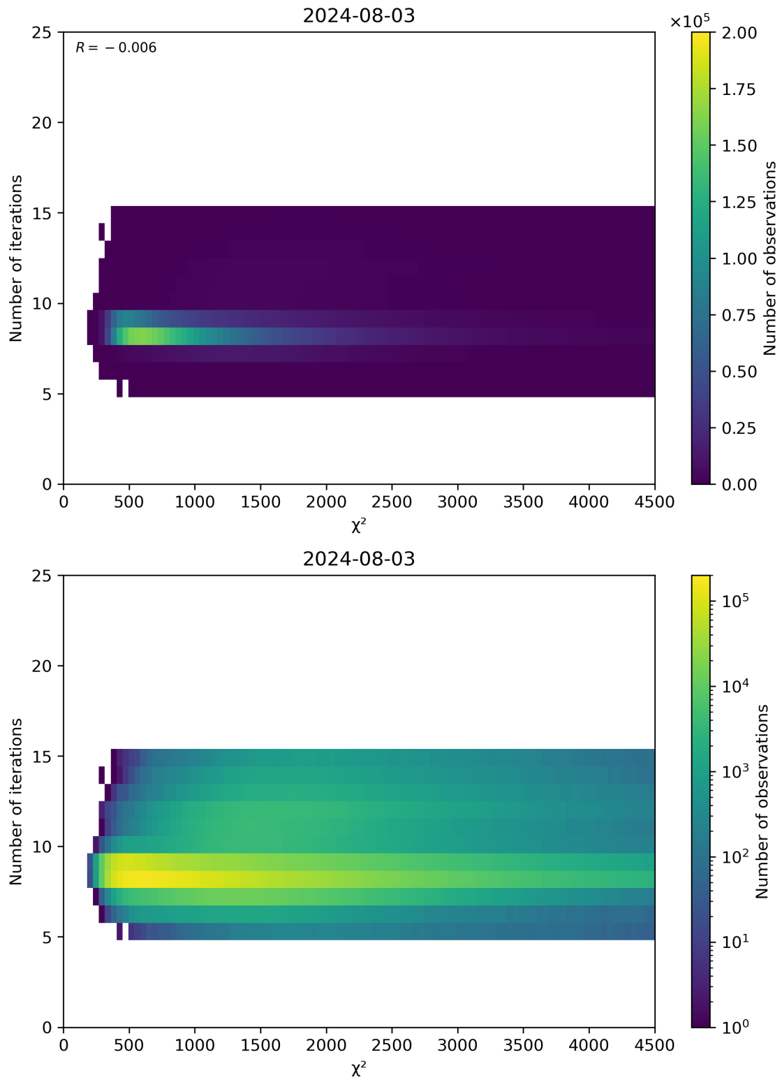
Figure 49: Scatter density plot of “ \chi^2 ” against “Number of iterations” for 2024-08-02 to 2024-08-04.
