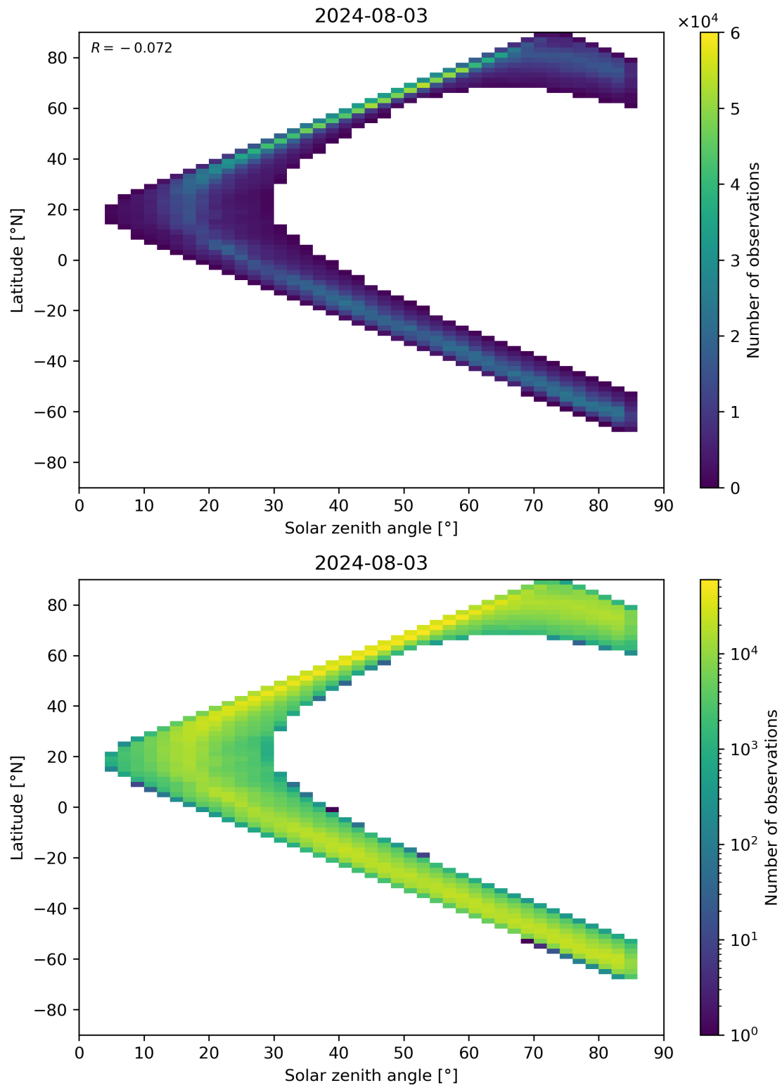
Figure 66: Scatter density plot of “Solar zenith angle” against “Latitude” for 2024-08-02 to 2024-08-04.
