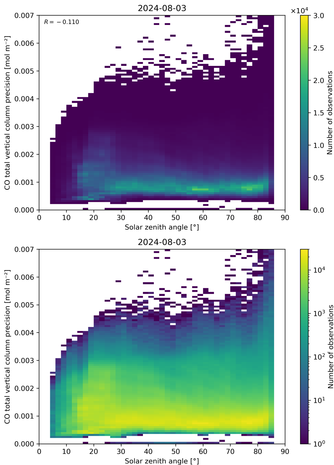
Figure 63: Scatter density plot of “Solar zenith angle” against “CO total vertical column precision” for 2024-08-02 to 2024-08-04.
