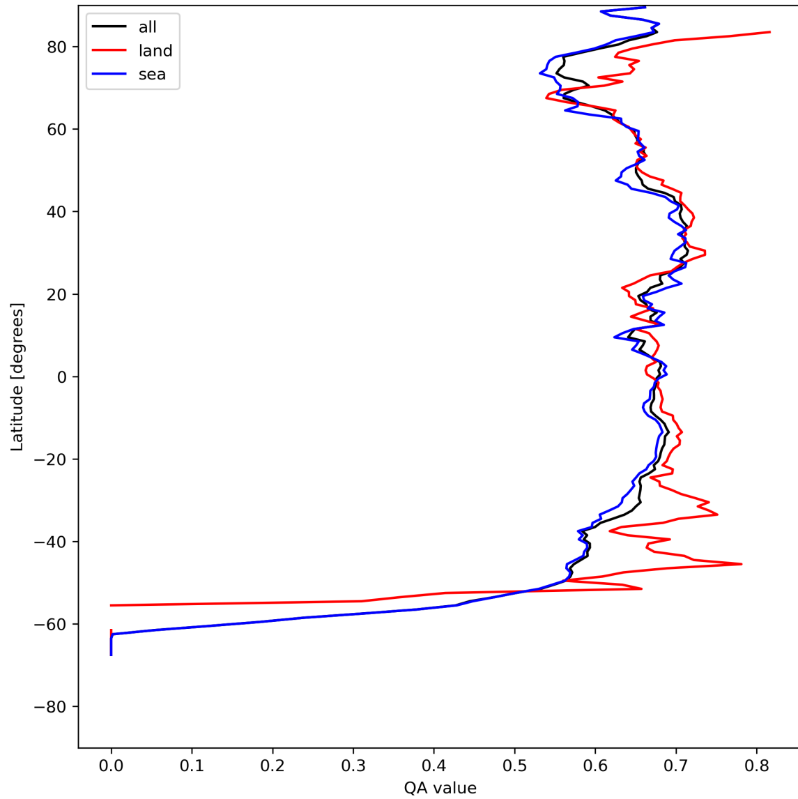
Figure 9: Zonal average of “QA value” for 2024-08-02 to 2024-08-04.
