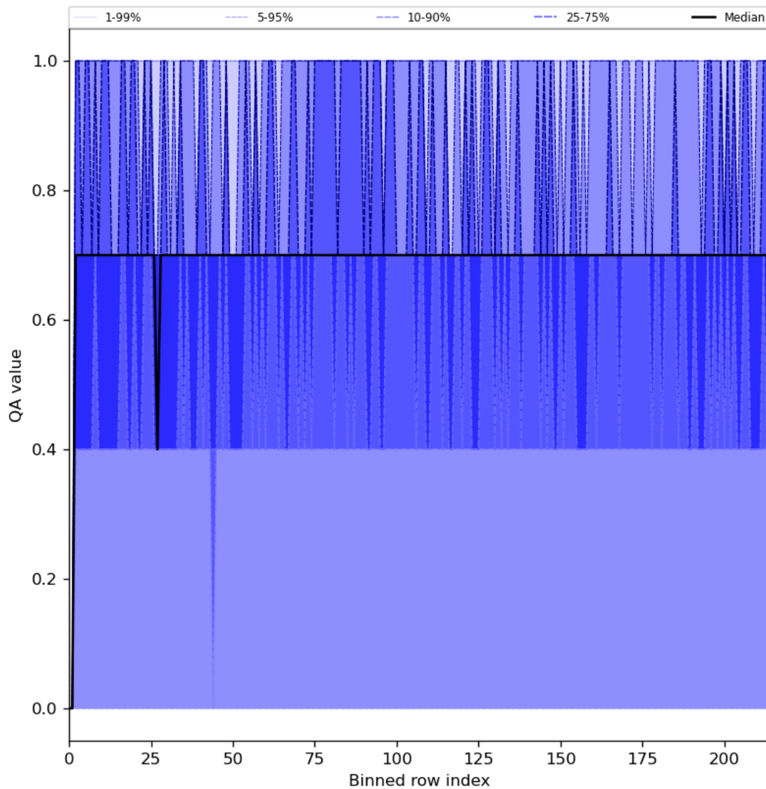
Figure 25: Along track statistics of “QA value” for 2024-08-02 to 2024-08-04
