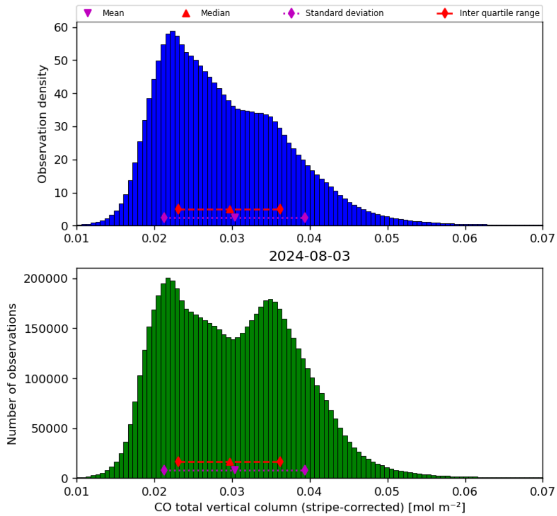
Figure 19: Histogram of “CO total vertical column (stripe-corrected)” for 2024-08-02 to 2024-08-04
