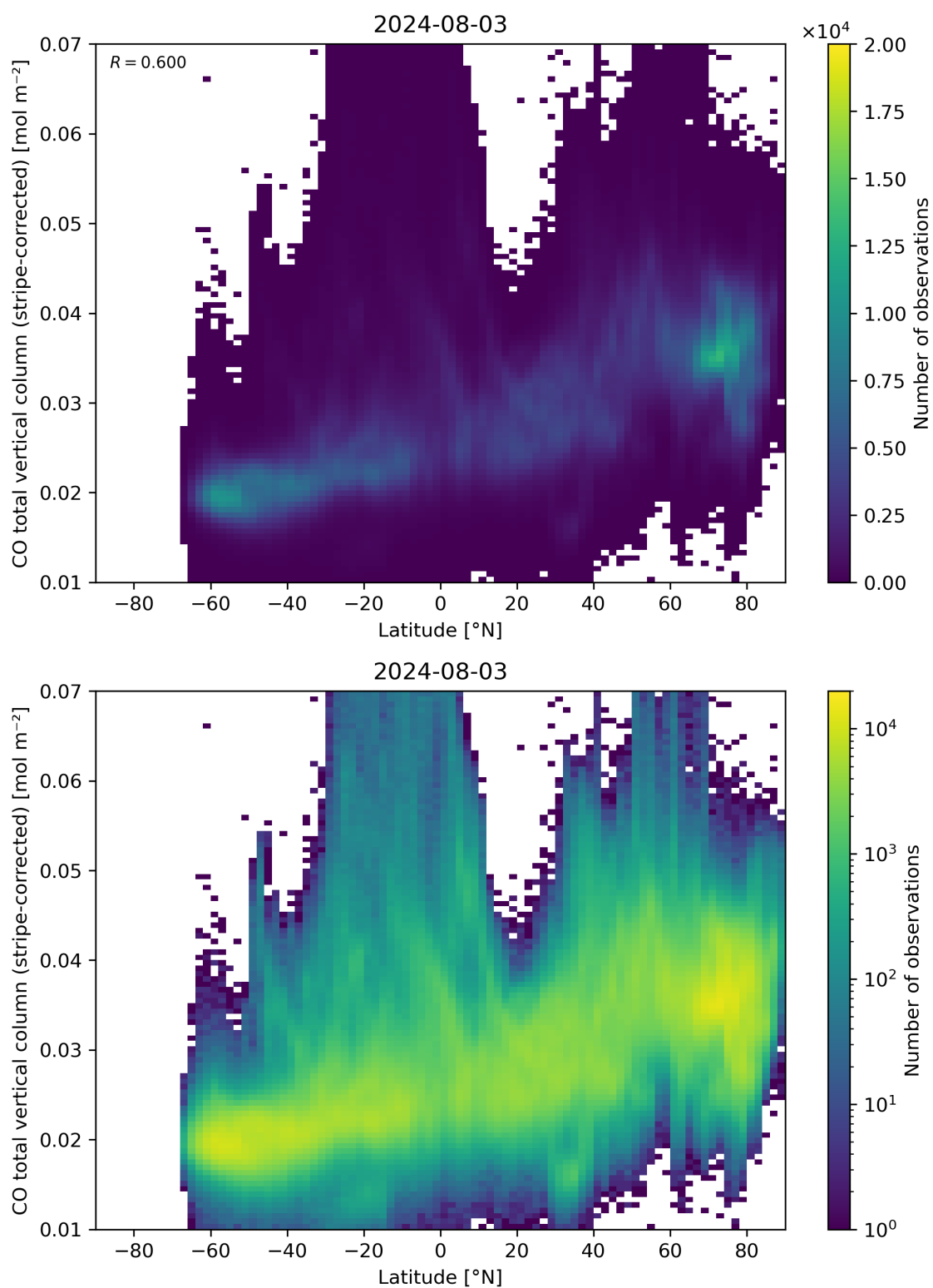
Figure 52: Scatter density plot of “Latitude” against “CO total vertical column (stripe-corrected)” for 2024-08-02 to 2024-08-04.
