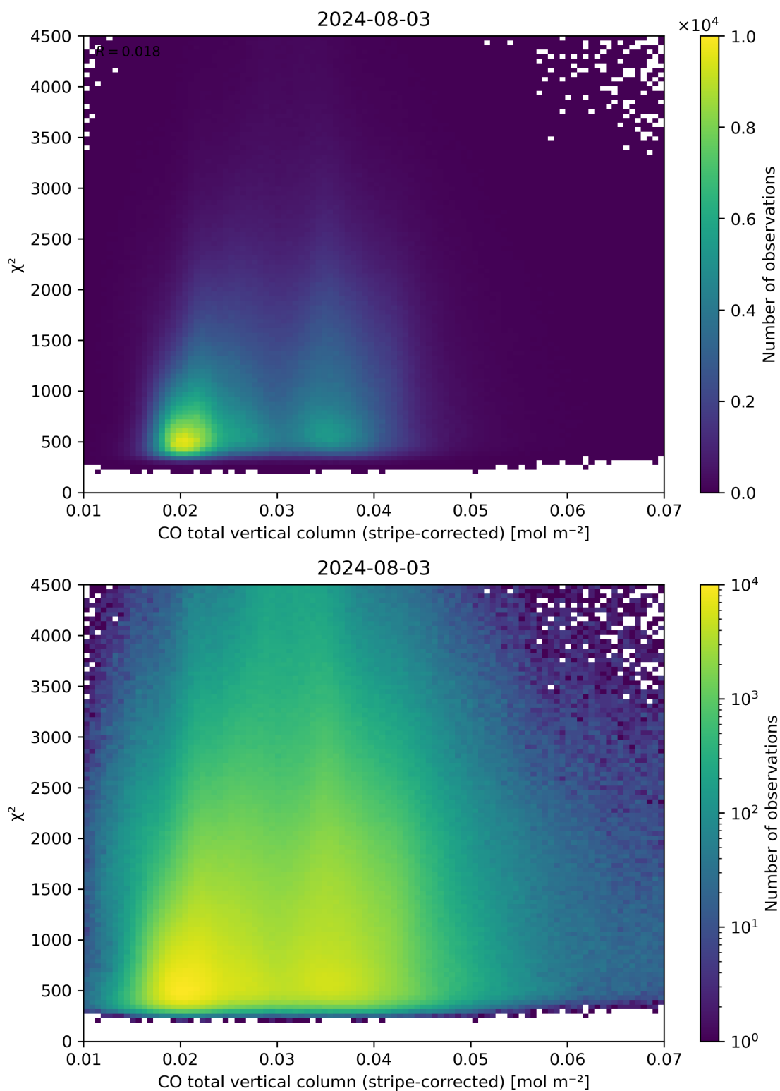
Figure 37: Scatter density plot of “CO total vertical column (stripe-corrected)” against “ \chi^2 ” for 2024-08-02 to 2024-08-04.
