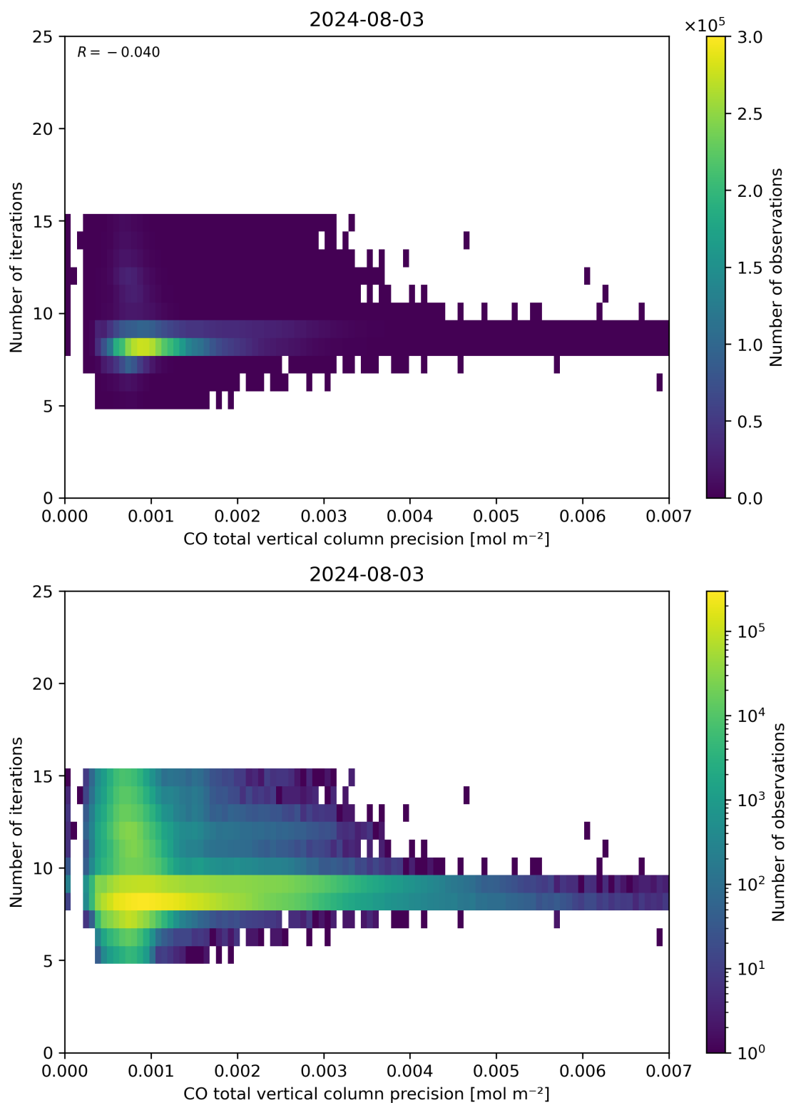
Figure 46: Scatter density plot of “CO total vertical column precision” against “Number of iterations” for 2024-08-02 to 2024-08-04.
