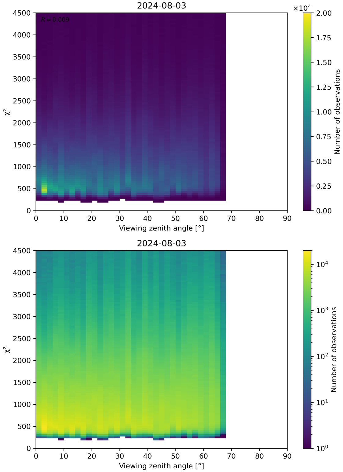
Figure 72: Scatter density plot of “Viewing zenith angle” against “ \chi^2 ” for 2024-08-02 to 2024-08-04.
