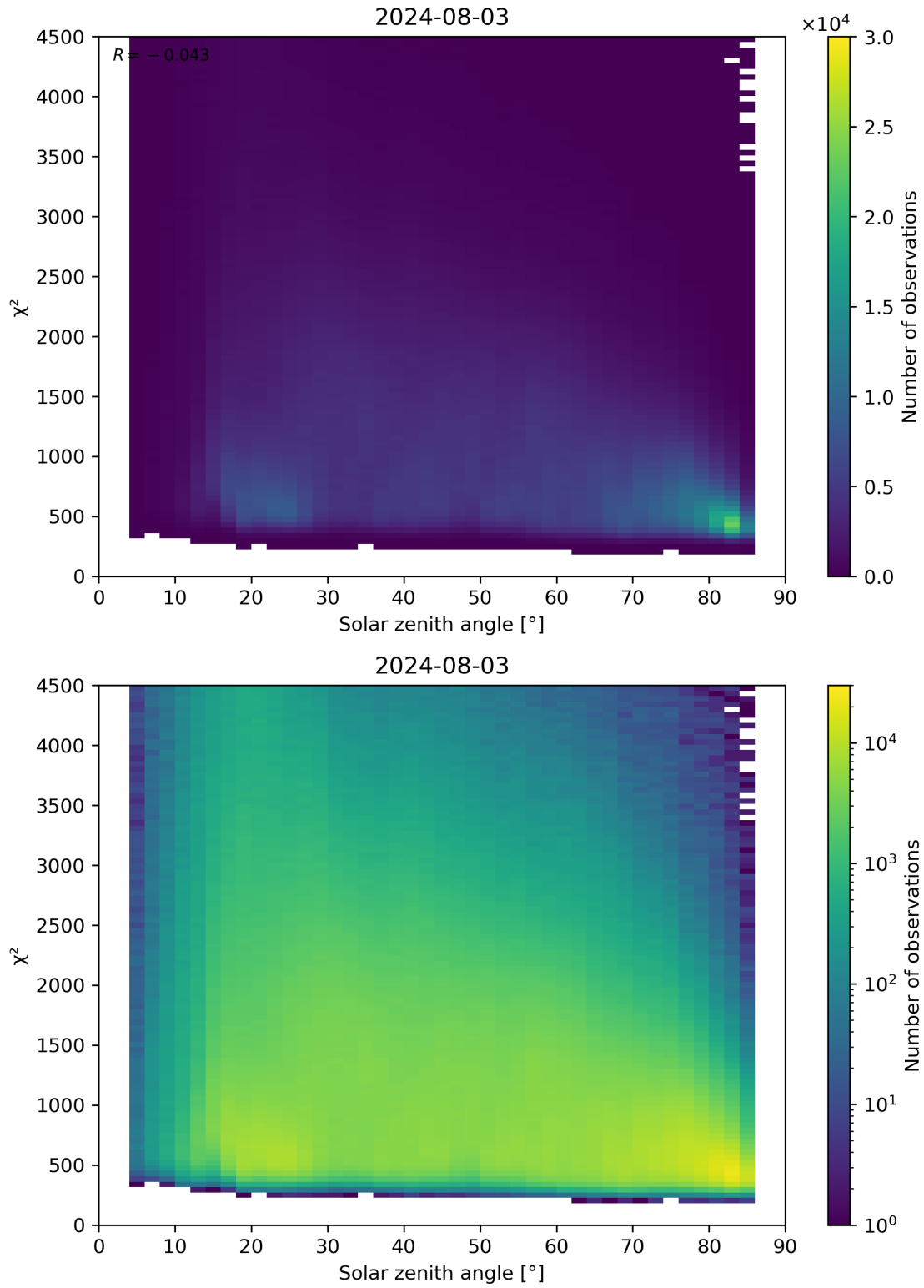
Figure 64: Scatter density plot of “Solar zenith angle” against “ \chi^2 ” for 2024-08-02 to 2024-08-04.
