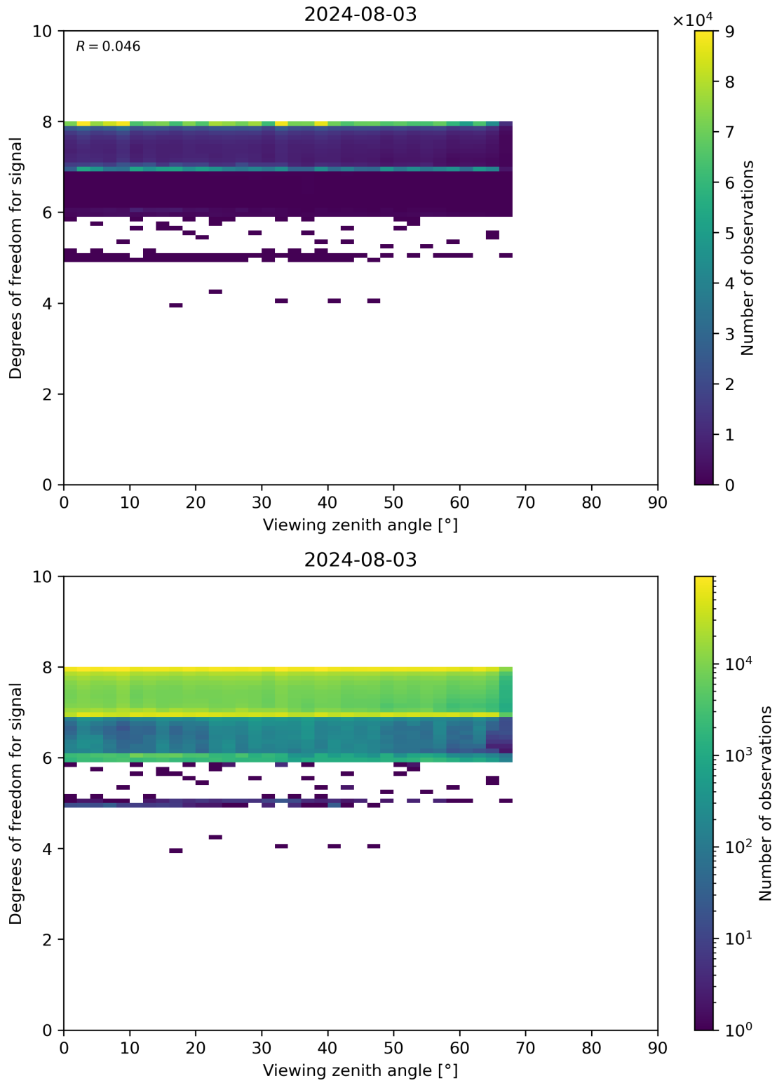
Figure 73: Scatter density plot of “Viewing zenith angle” against “Degrees of freedom for signal” for 2024-08-02 to 2024-08-04.
