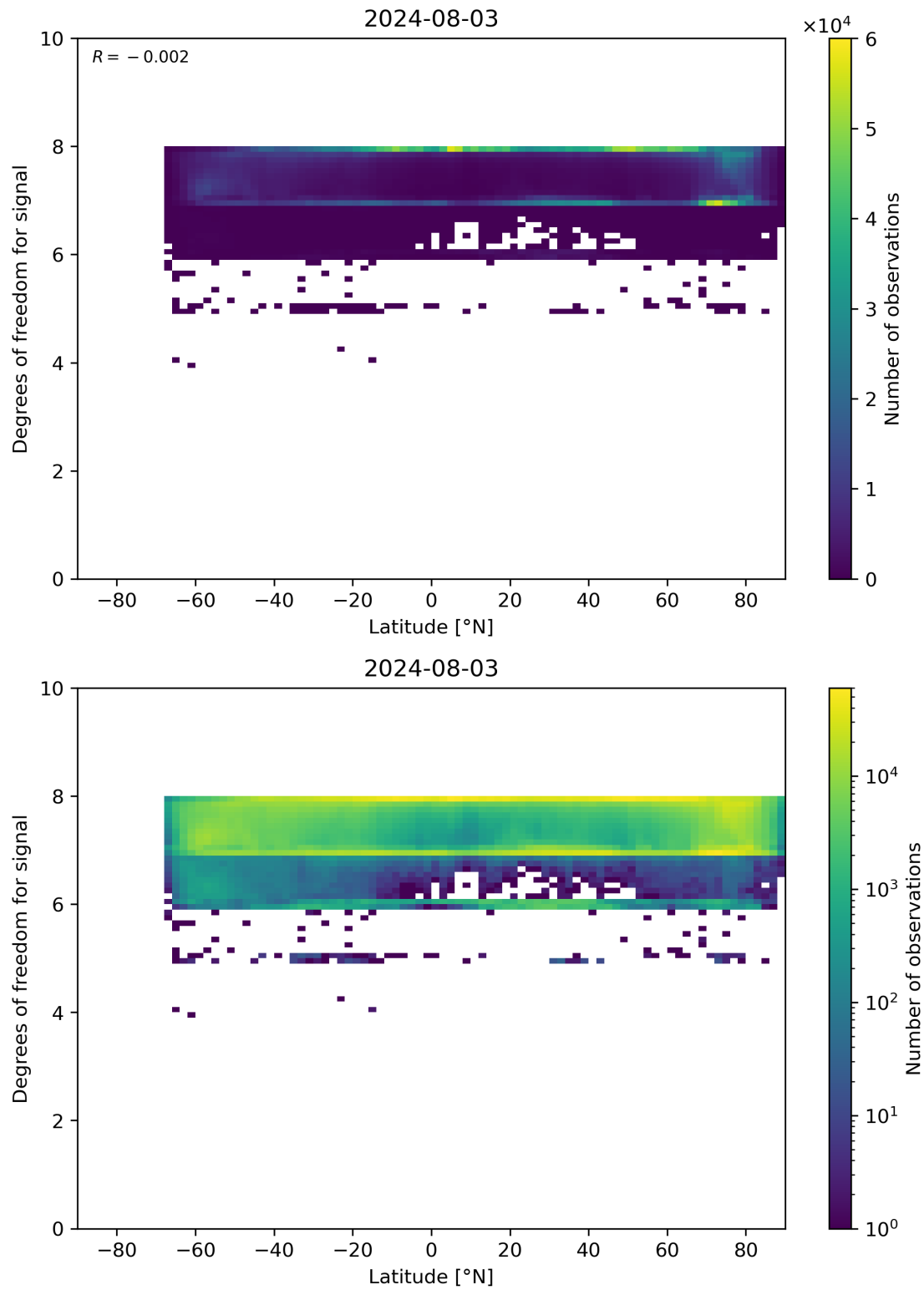
Figure 55: Scatter density plot of “Latitude” against “Degrees of freedom for signal” for 2024-08-02 to 2024-08-04.
