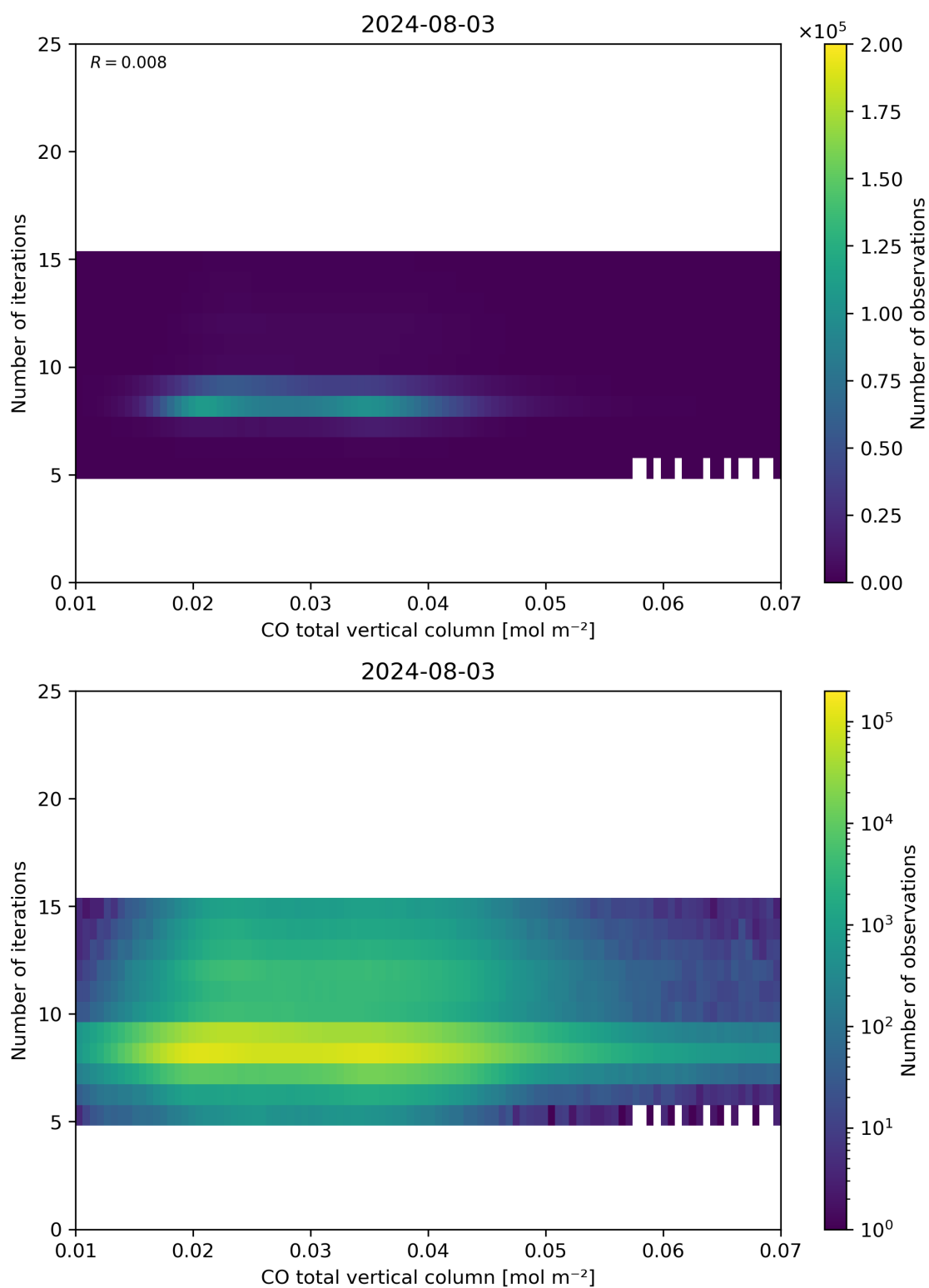
Figure 42: Scatter density plot of “CO total vertical column” against “Number of iterations” for 2024-08-02 to 2024-08-04.
