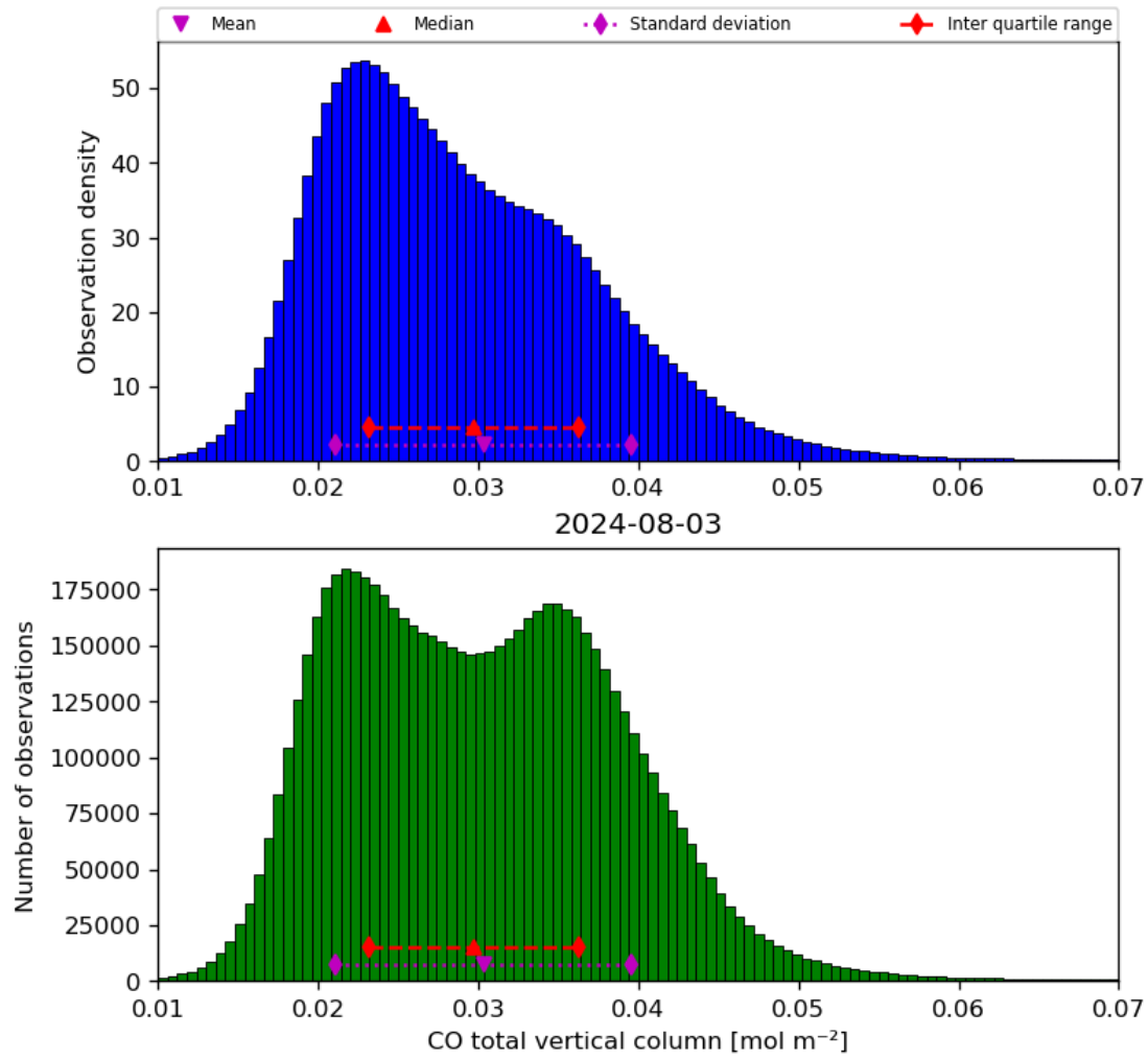
Figure 18: Histogram of “CO total vertical column” for 2024-08-02 to 2024-08-04
