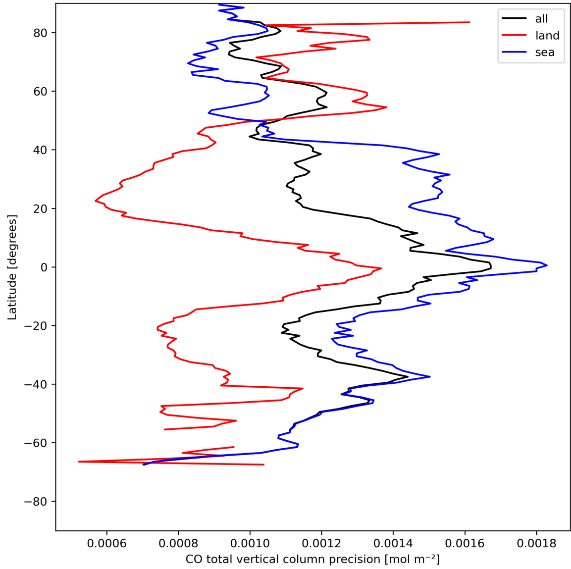
Figure 12: Zonal average of “CO total vertical column precision” for 2024-08-02 to 2024-08-04.
