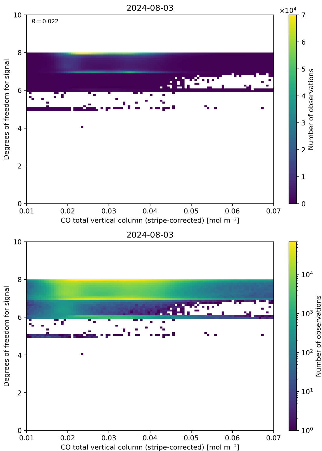
Figure 38: Scatter density plot of “CO total vertical column (stripe-corrected)” against “Degrees of freedom for signal” for 2024-08-02 to 2024-08-04.
