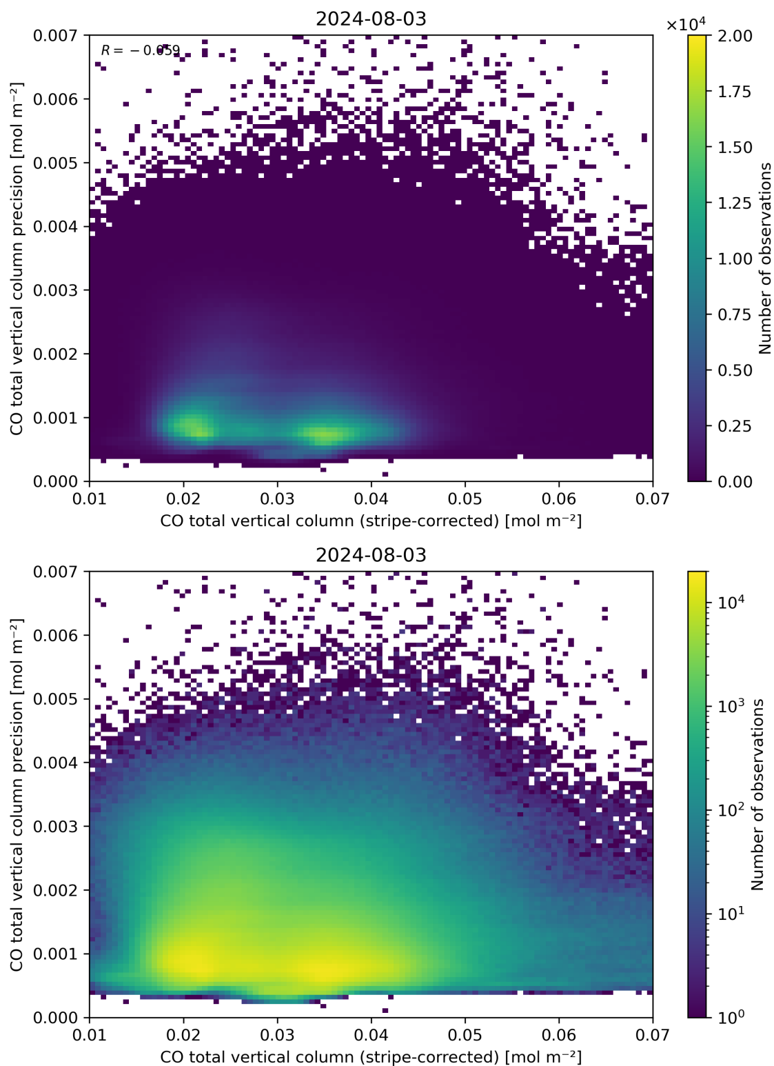
Figure 36: Scatter density plot of “CO total vertical column (stripe-corrected)” against “CO total vertical column precision” for 2024-08-02 to 2024-08-04.
