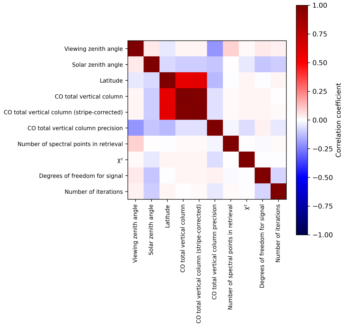
Figure 2: Map of correlation matrix for 2024-08-02 to 2024-08-04.
