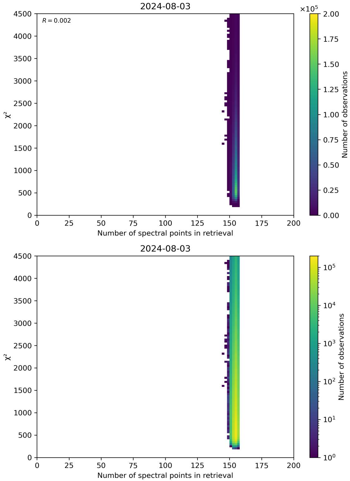
Figure 58: Scatter density plot of “Number of spectral points in retrieval” against “ \chi^2 ” for 2024-08-02 to 2024-08-04.
