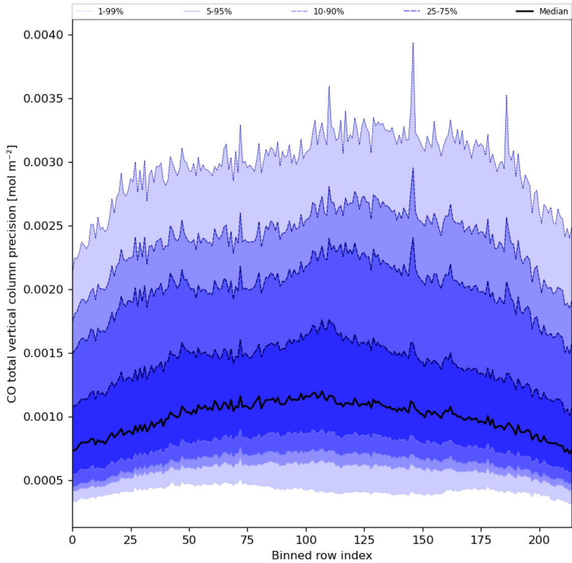
Figure 28: Along track statistics of “CO total vertical column precision” for 2024-08-02 to 2024-08-04
