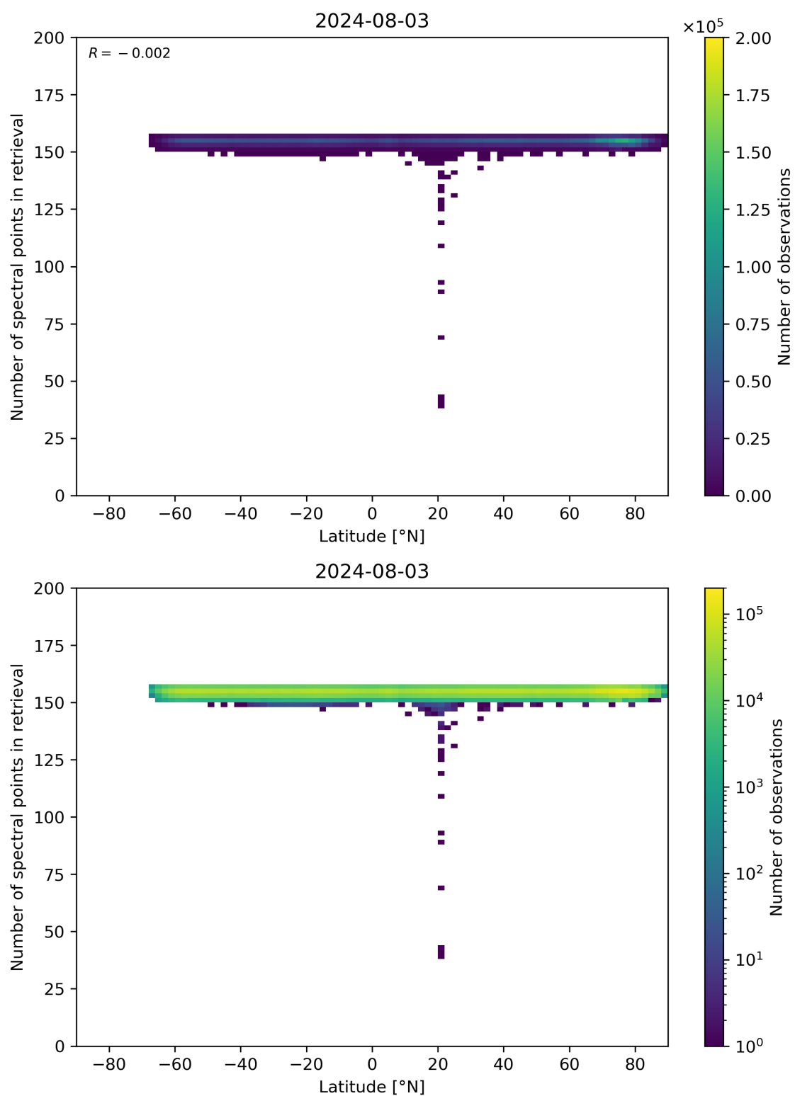
Figure 57: Scatter density plot of “Latitude” against “Number of spectral points in retrieval” for 2024-08-02 to 2024-08-04.
