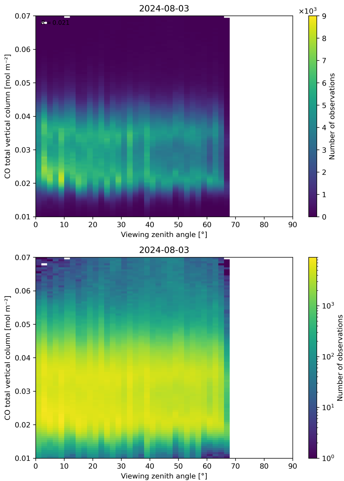
Figure 69: Scatter density plot of “Viewing zenith angle” against “CO total vertical column” for 2024-08-02 to 2024-08-04.
