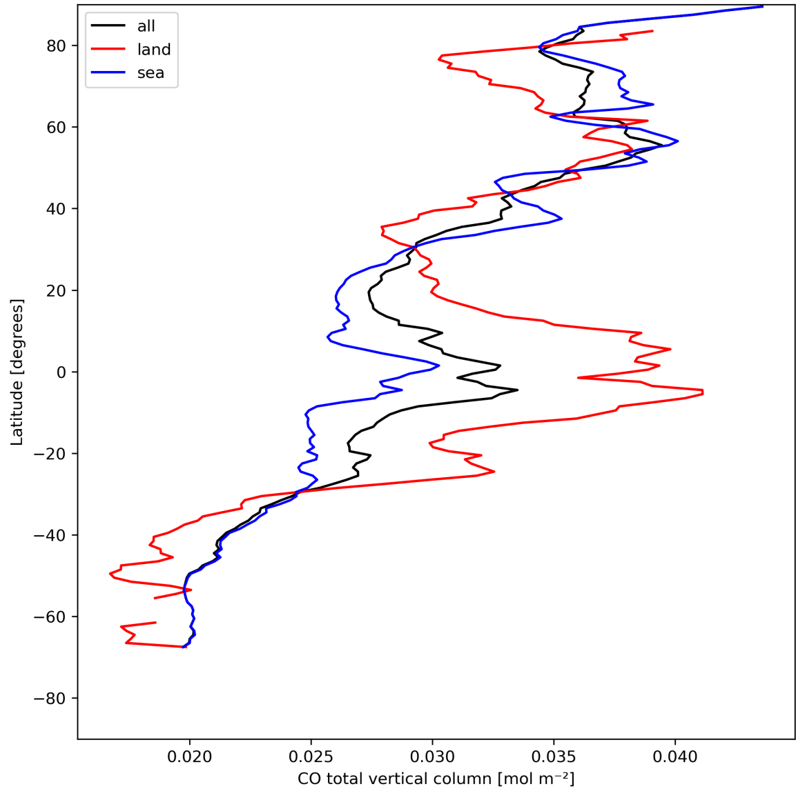
Figure 10: Zonal average of “CO total vertical column” for 2024-08-02 to 2024-08-04.
