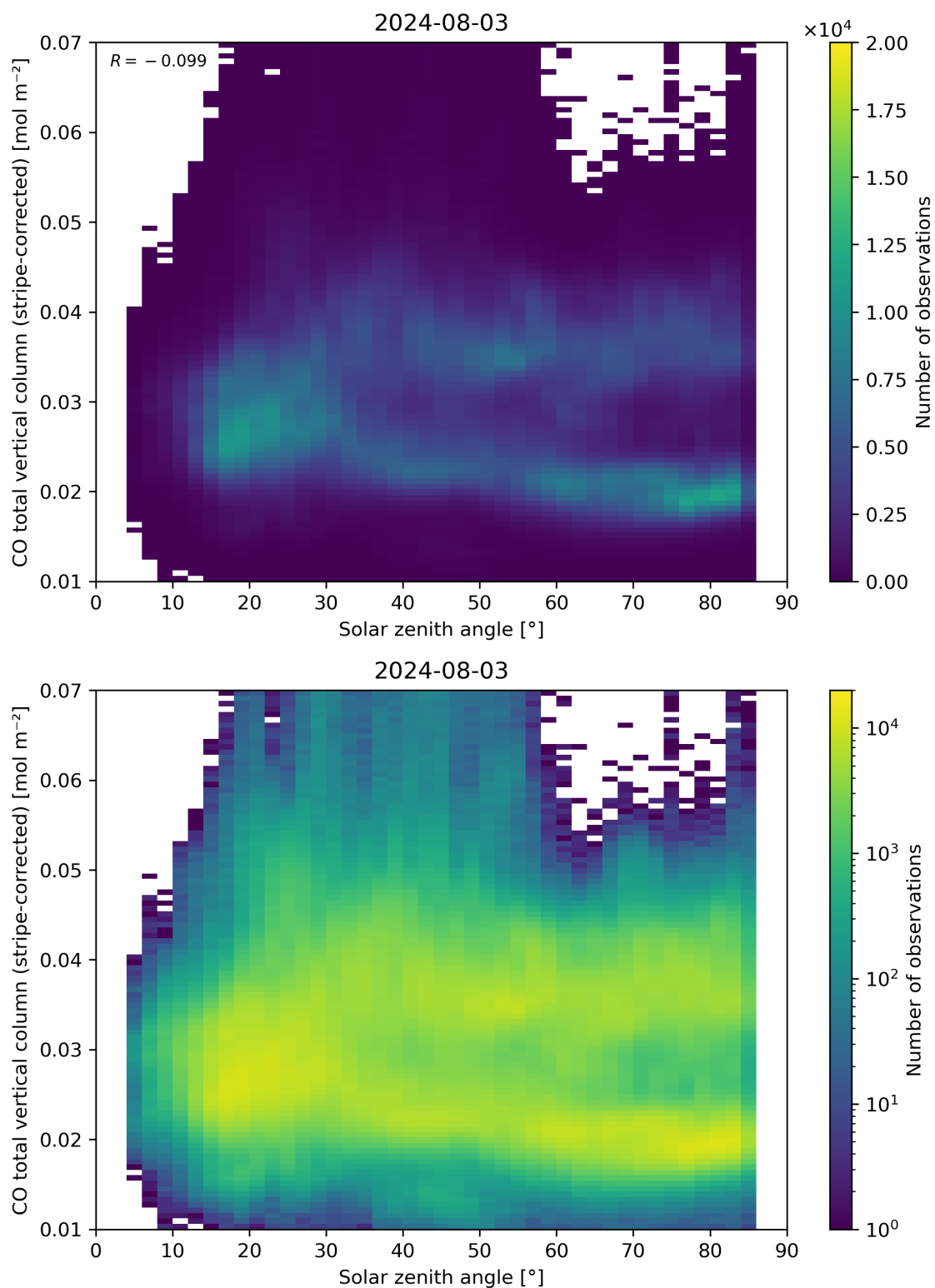
Figure 62: Scatter density plot of “Solar zenith angle” against “CO total vertical column (stripe-corrected)” for 2024-08-02 to 2024-08-04.
