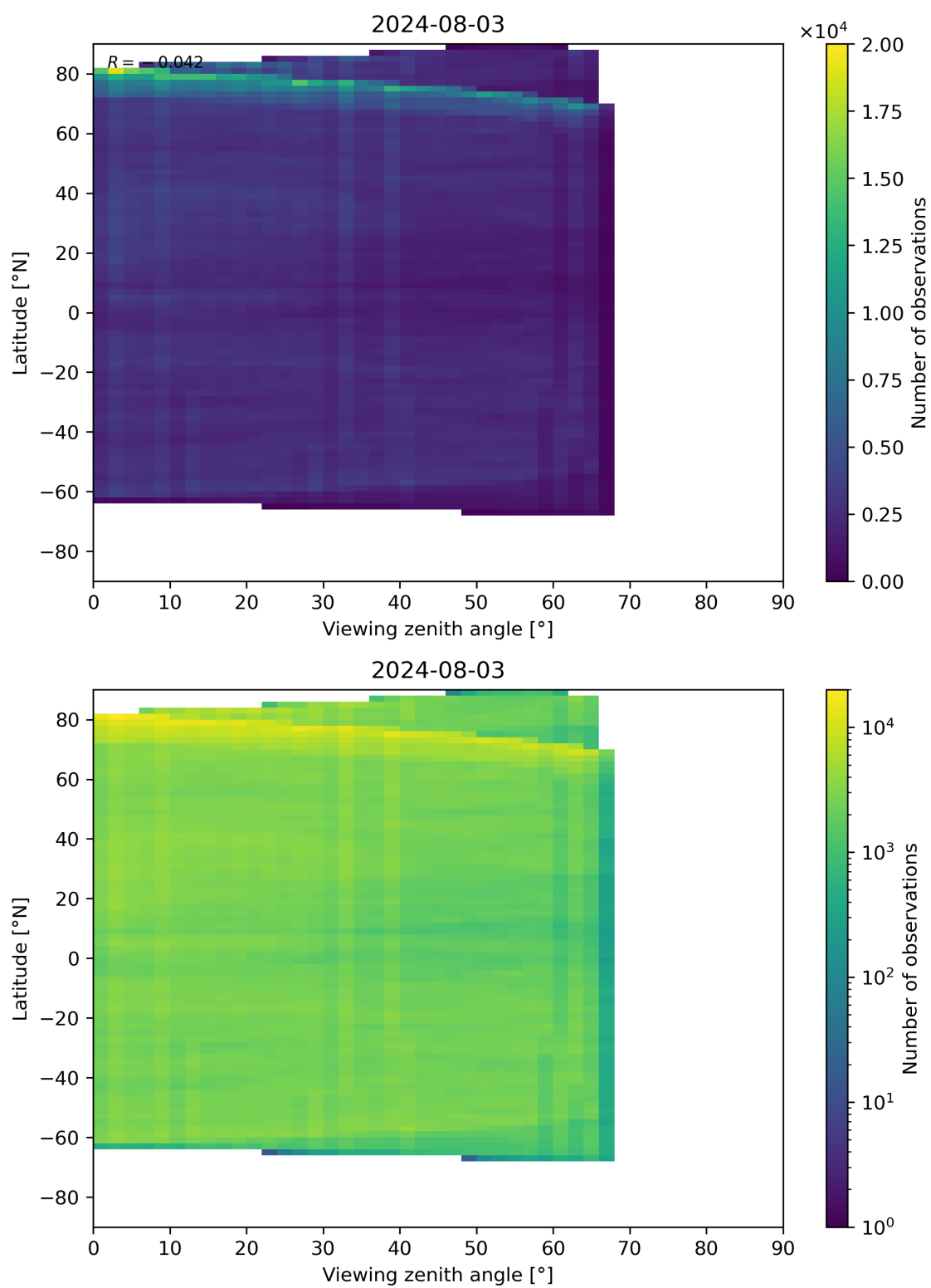
Figure 74: Scatter density plot of “Viewing zenith angle” against “Latitude” for 2024-08-02 to 2024-08-04.
