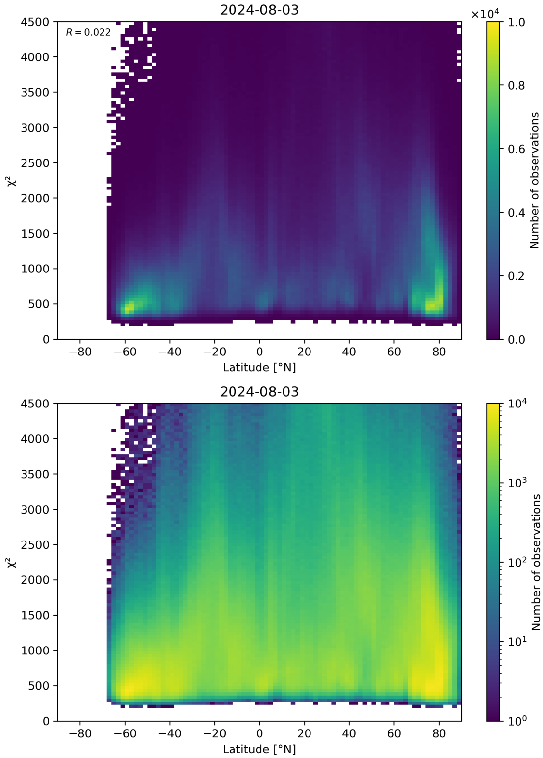
Figure 54: Scatter density plot of “Latitude” against “ \chi^2 ” for 2024-08-02 to 2024-08-04.
