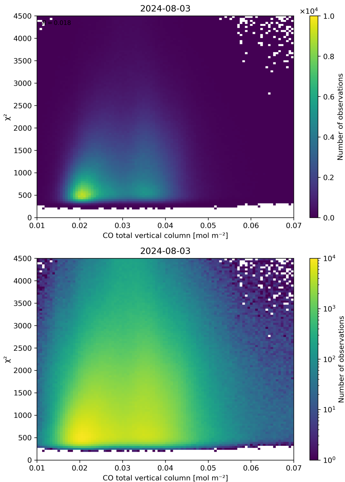
Figure 35: Scatter density plot of “CO total vertical column” against “ \chi^2 ” for 2024-08-02 to 2024-08-04.
