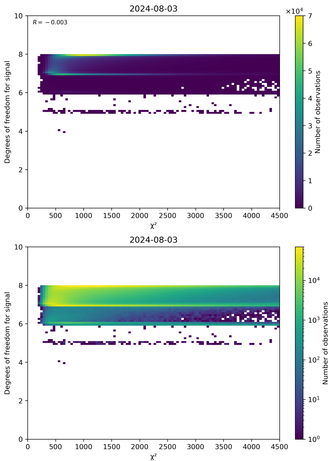
Figure 48: Scatter density plot of “ \chi^2 ” against “Degrees of freedom for signal” for 2024-08-02 to 2024-08-04.
