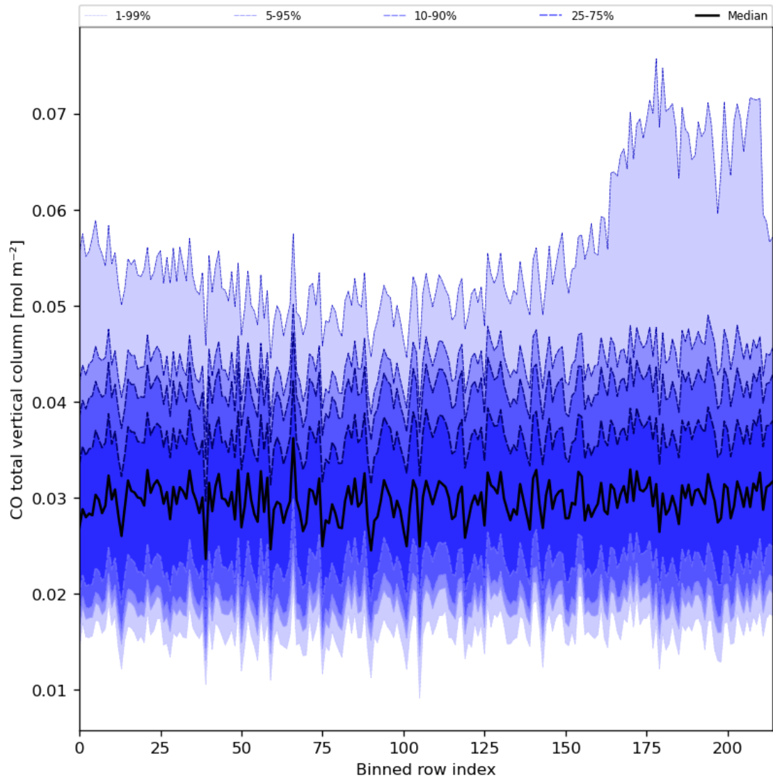
Figure 26: Along track statistics of “CO total vertical column” for 2024-08-02 to 2024-08-04
