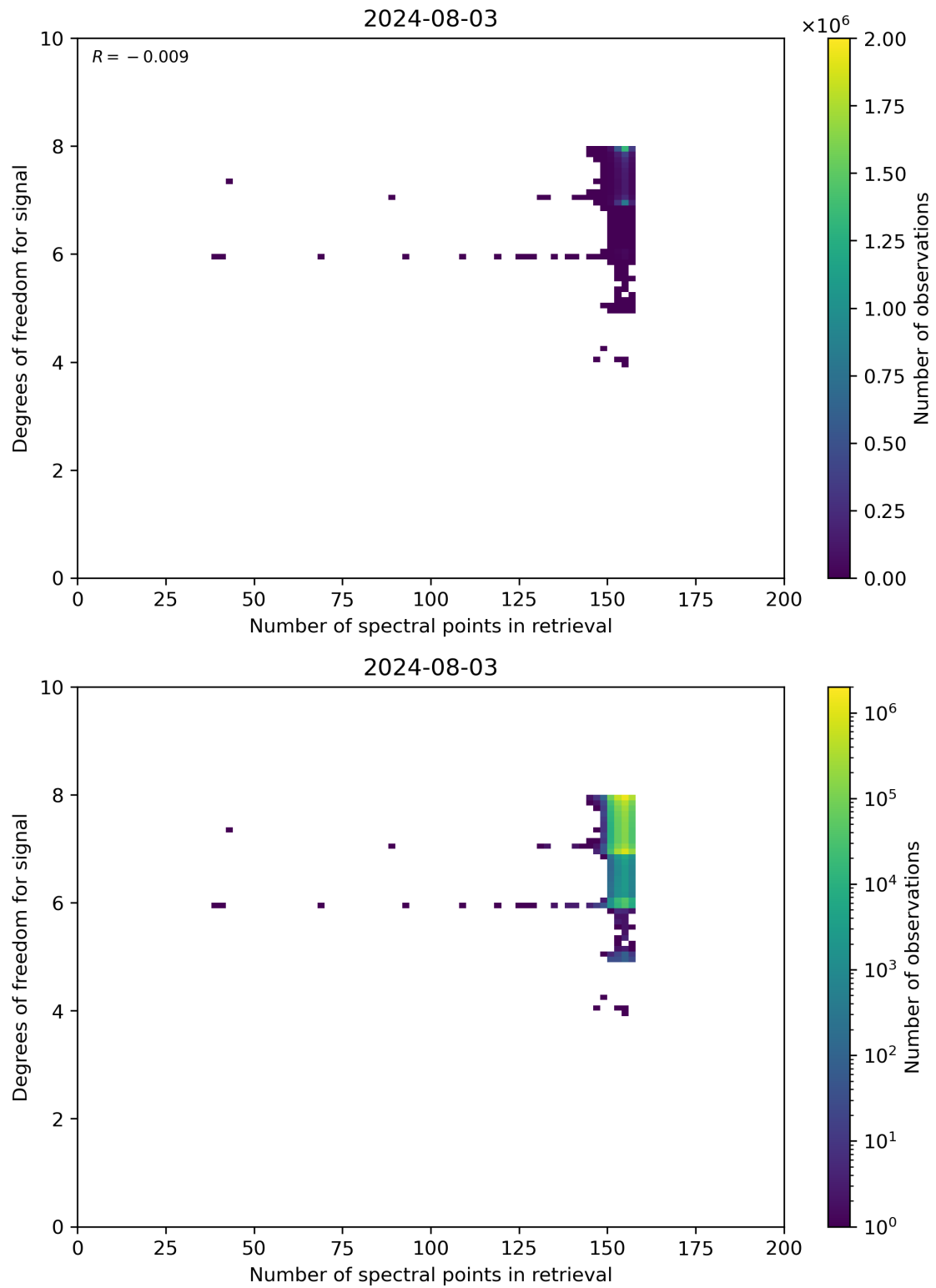
Figure 59: Scatter density plot of “Number of spectral points in retrieval” against “Degrees of freedom for signal” for 2024-08-02 to 2024-08-04.
