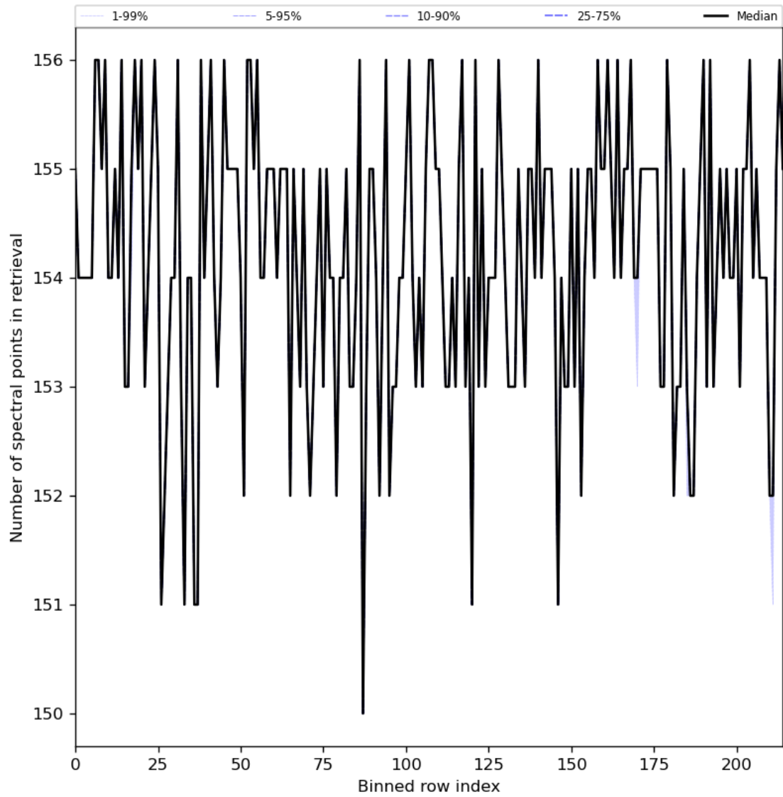
Figure 29: Along track statistics of “Number of spectral points in retrieval” for 2024-08-02 to 2024-08-04
