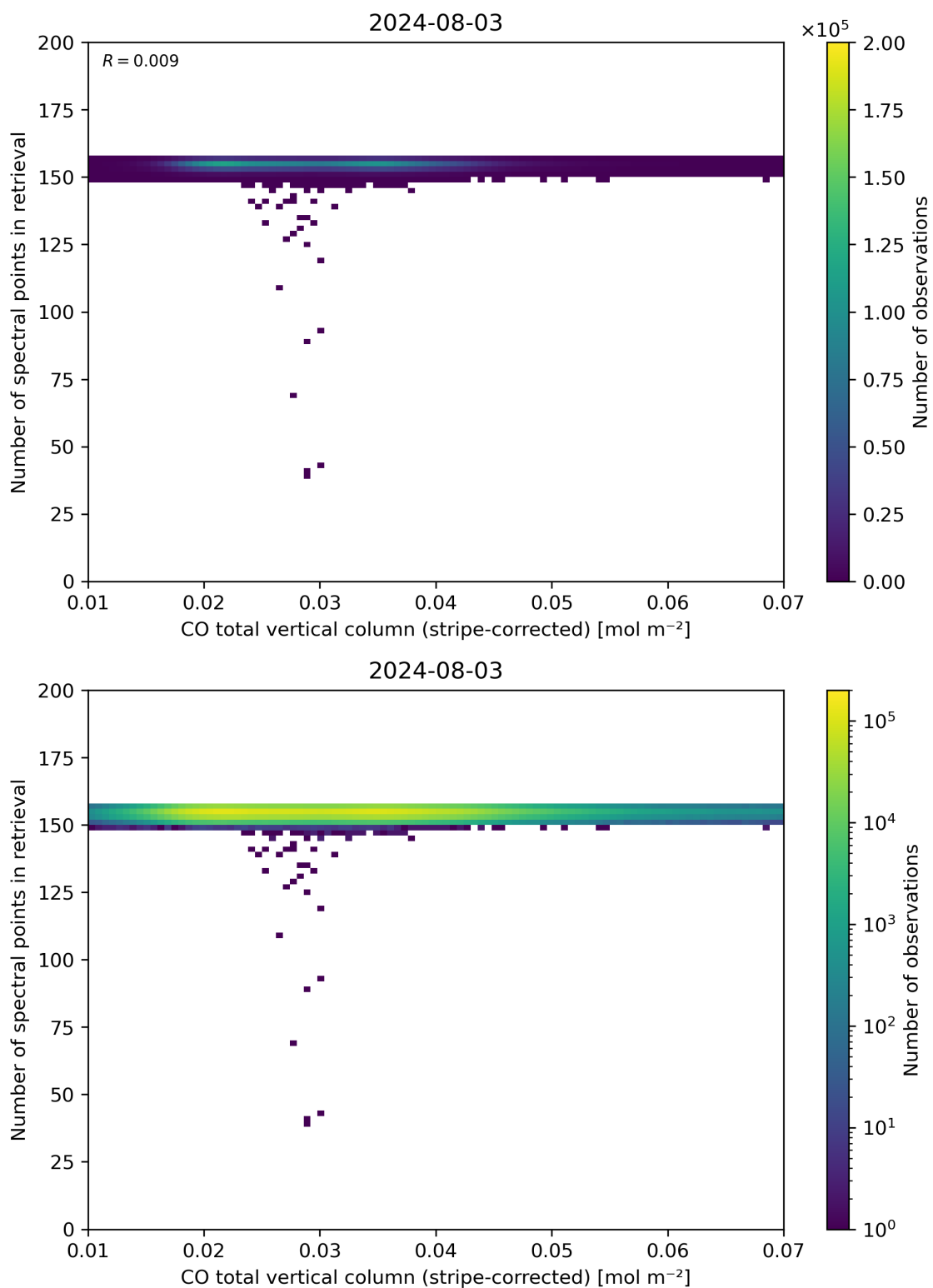
Figure 40: Scatter density plot of “CO total vertical column (stripe-corrected)” against “Number of spectral points in retrieval” for 2024-08-02 to 2024-08-04.
