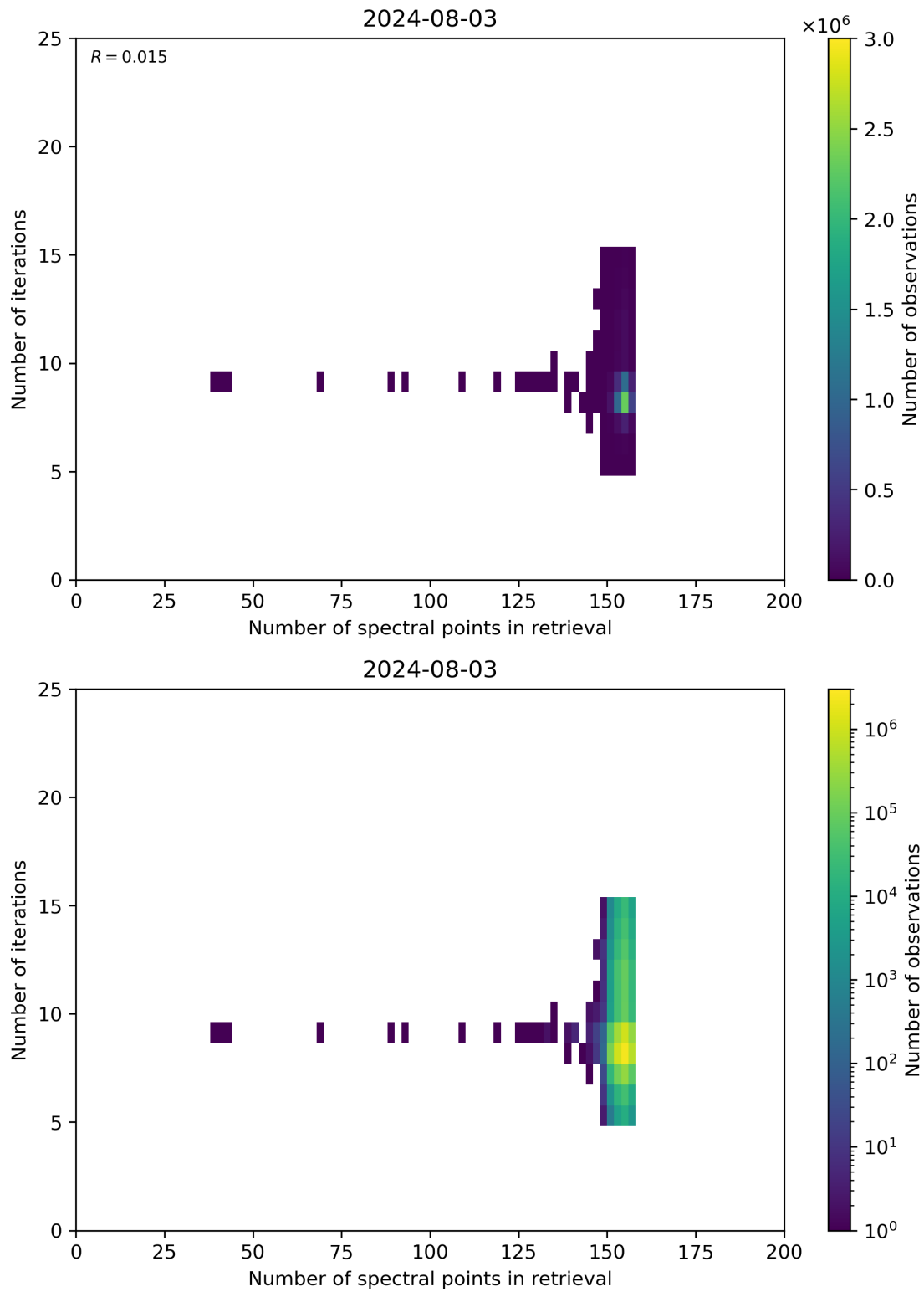
Figure 60: Scatter density plot of “Number of spectral points in retrieval” against “Number of iterations” for 2024-08-02 to 2024-08-04.
