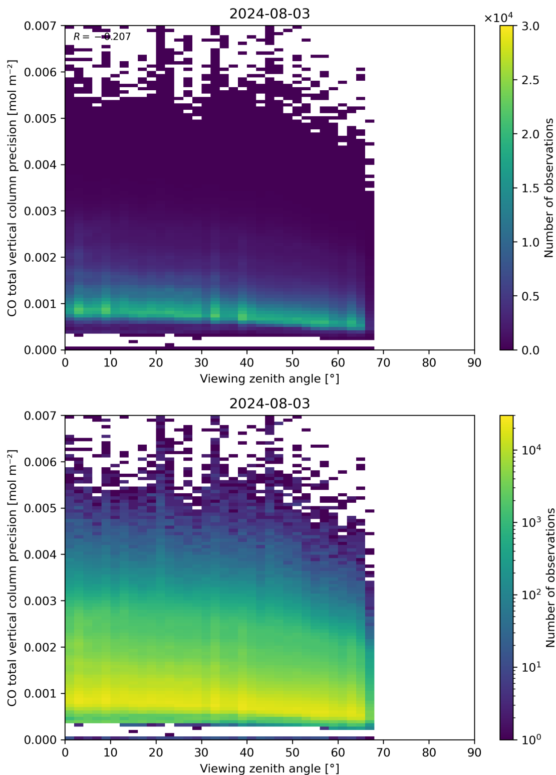
Figure 71: Scatter density plot of “Viewing zenith angle” against “CO total vertical column precision” for 2024-08-02 to 2024-08-04.
