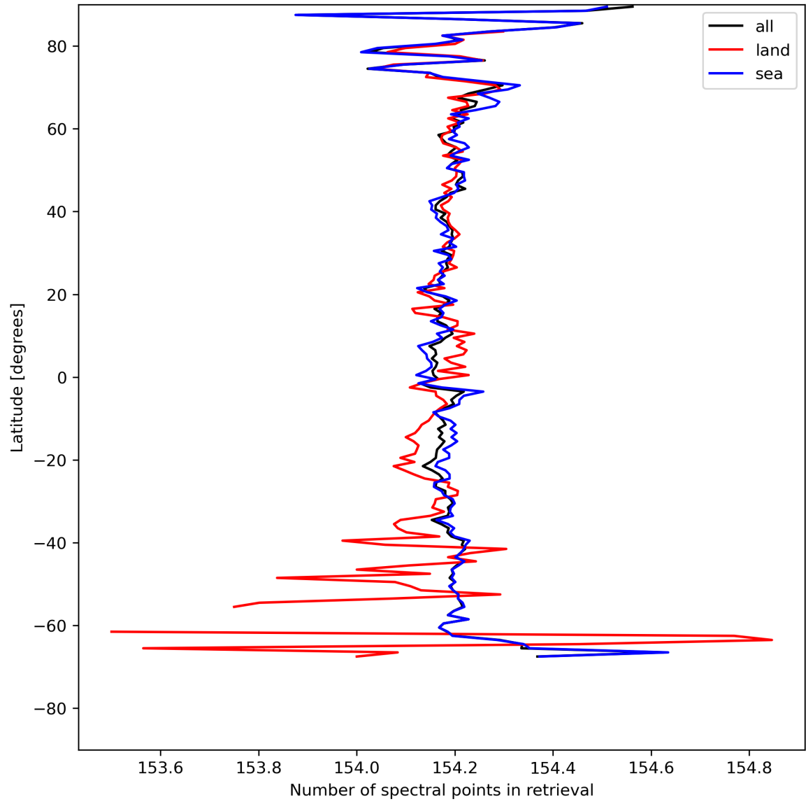
Figure 13: Zonal average of “Number of spectral points in retrieval” for 2024-08-02 to 2024-08-04.
