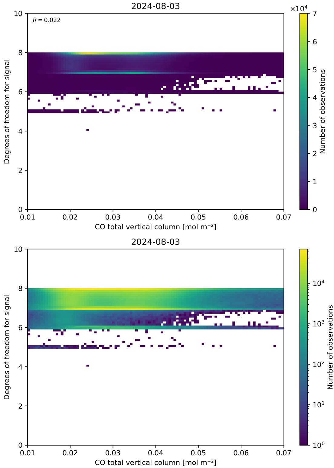
Figure 41: Scatter density plot of “CO total vertical column” against “Degrees of freedom for signal” for 2024-08-02 to 2024-08-04.
