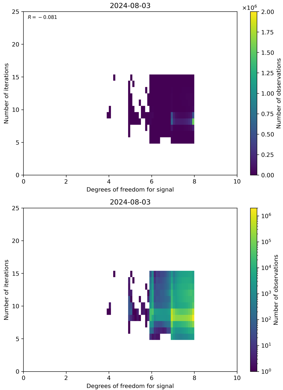
Figure 50: Scatter density plot of “Degrees of freedom for signal” against “Number of iterations” for 2024-08-02 to 2024-08-04.
