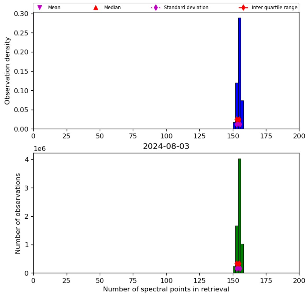
Figure 21: Histogram of “Number of spectral points in retrieval” for 2024-08-02 to 2024-08-04
