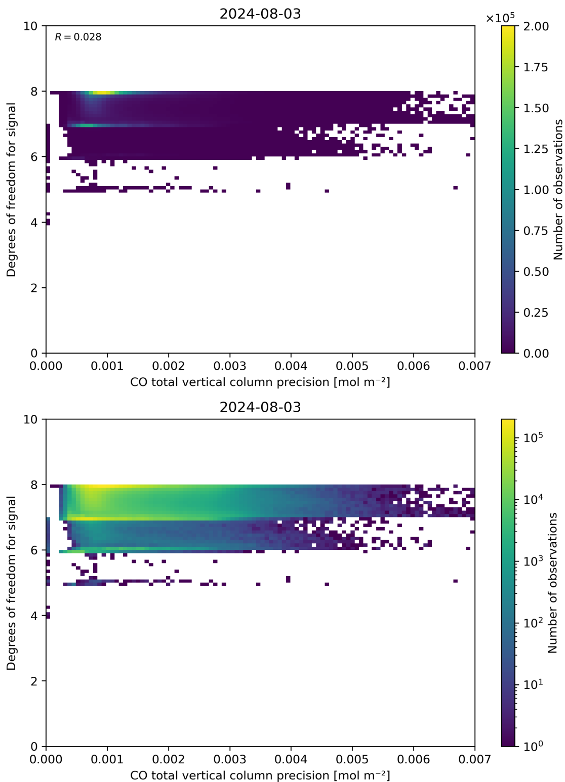
Figure 45: Scatter density plot of “CO total vertical column precision” against “Degrees of freedom for signal” for 2024-08-02 to 2024-08-04.
