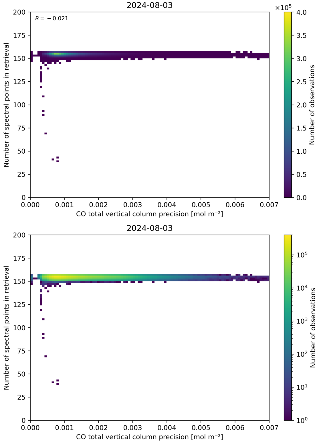
Figure 47: Scatter density plot of “CO total vertical column precision” against “Number of spectral points in retrieval” for 2024-08-02 to 2024-08-04.
