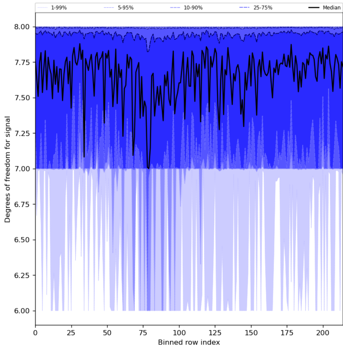
Figure 31: Along track statistics of “Degrees of freedom for signal” for 2024-08-02 to 2024-08-04
