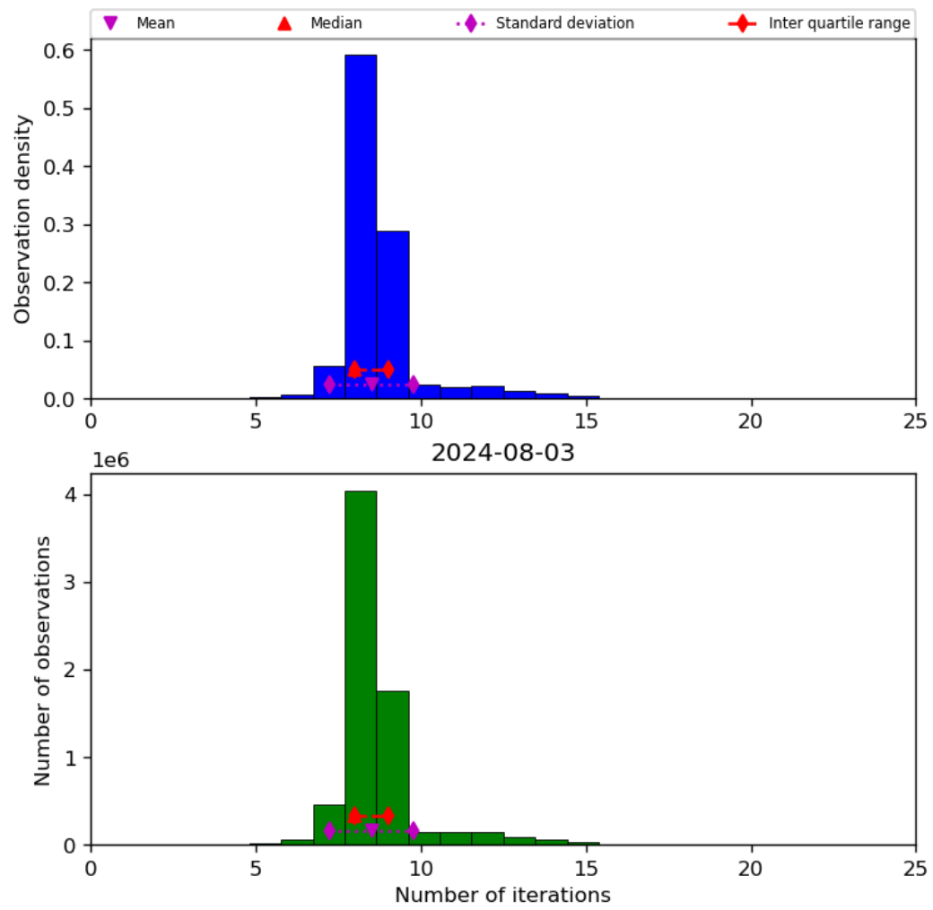
Figure 24: Histogram of “Number of iterations” for 2024-08-02 to 2024-08-04
