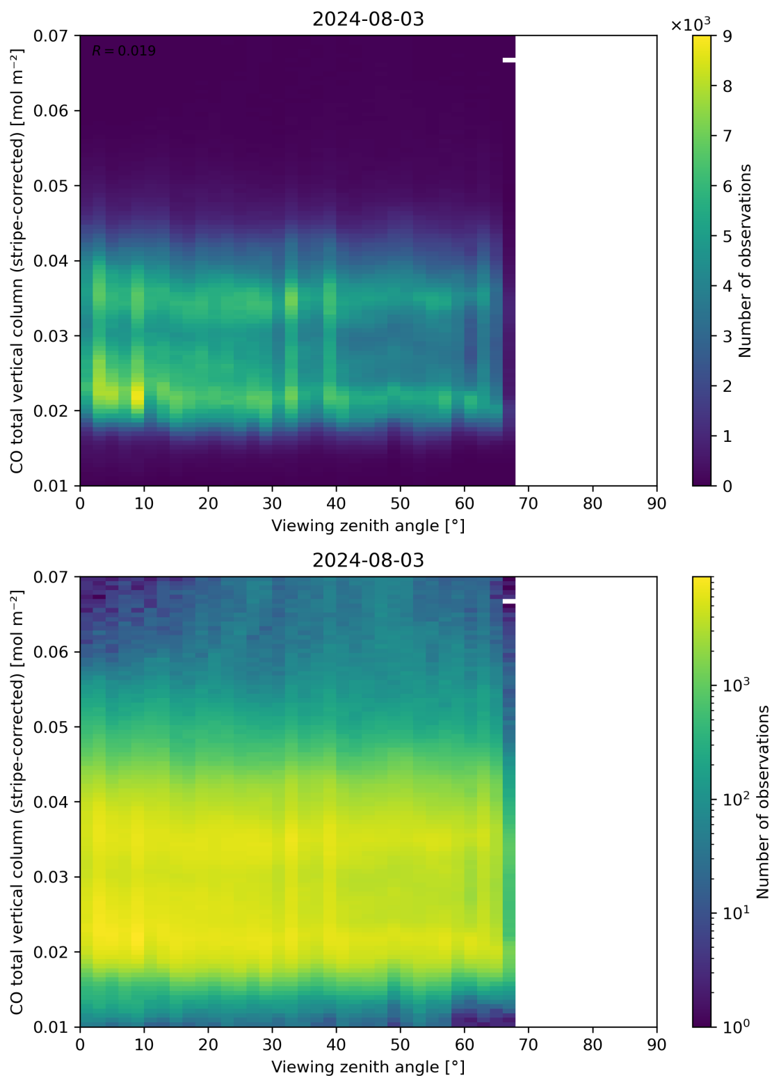
Figure 70: Scatter density plot of “Viewing zenith angle” against “CO total vertical column (stripe-corrected)” for 2024-08-02 to 2024-08-04.
