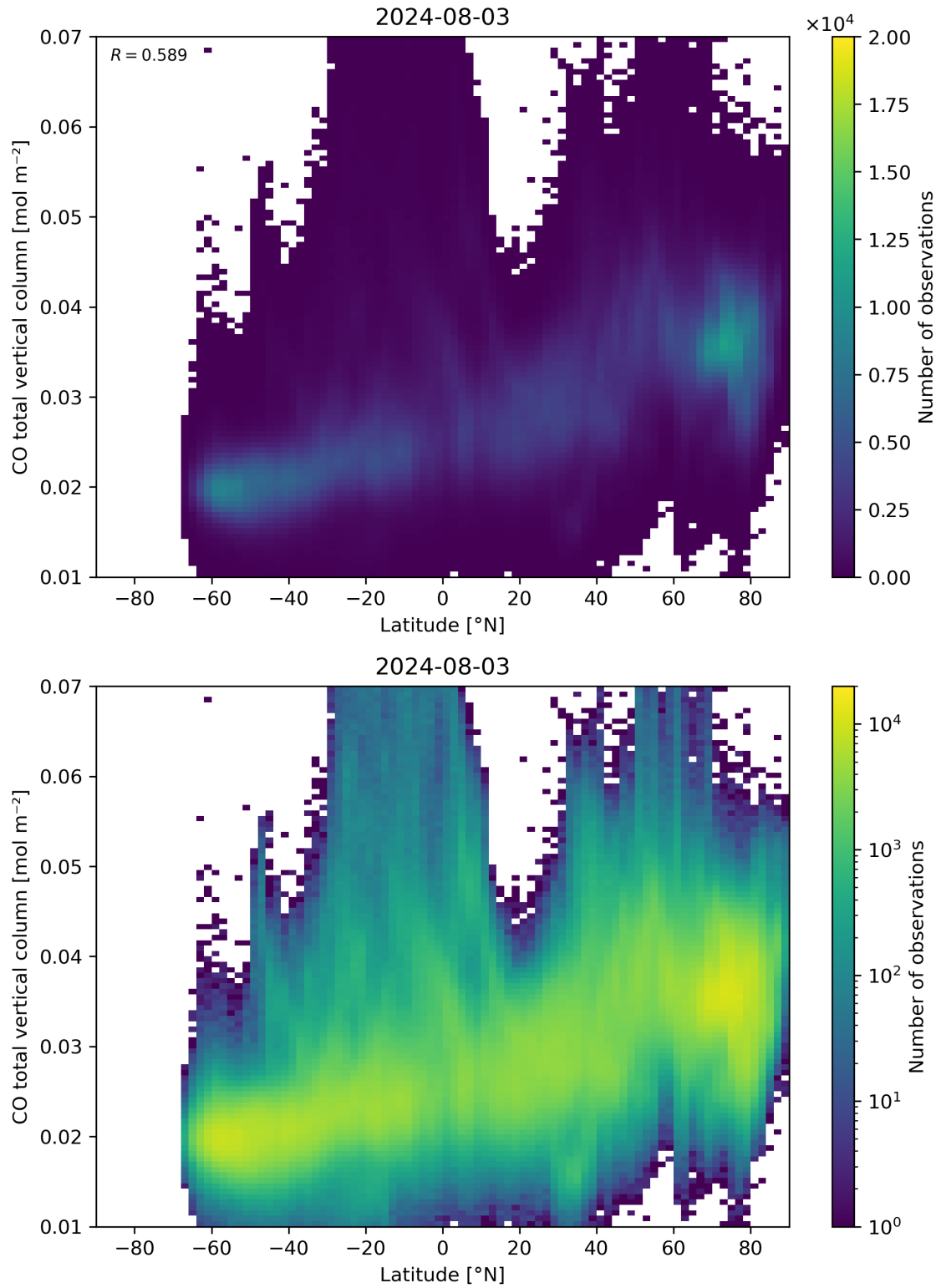
Figure 51: Scatter density plot of “Latitude” against “CO total vertical column” for 2024-08-02 to 2024-08-04.
