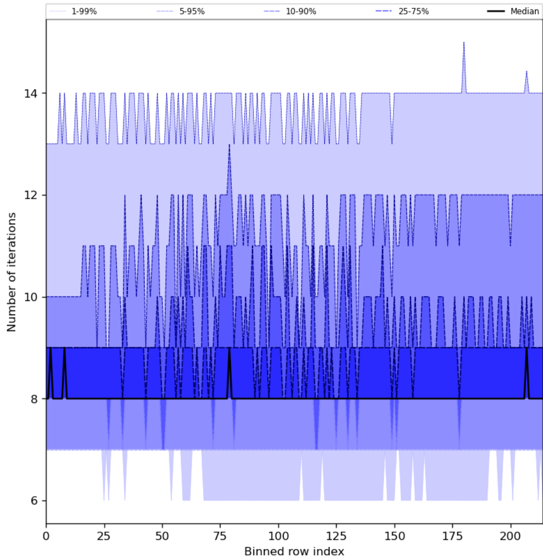
Figure 32: Along track statistics of “Number of iterations” for 2024-08-02 to 2024-08-04
