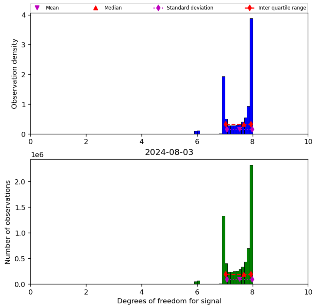
Figure 23: Histogram of “Degrees of freedom for signal” for 2024-08-02 to 2024-08-04
