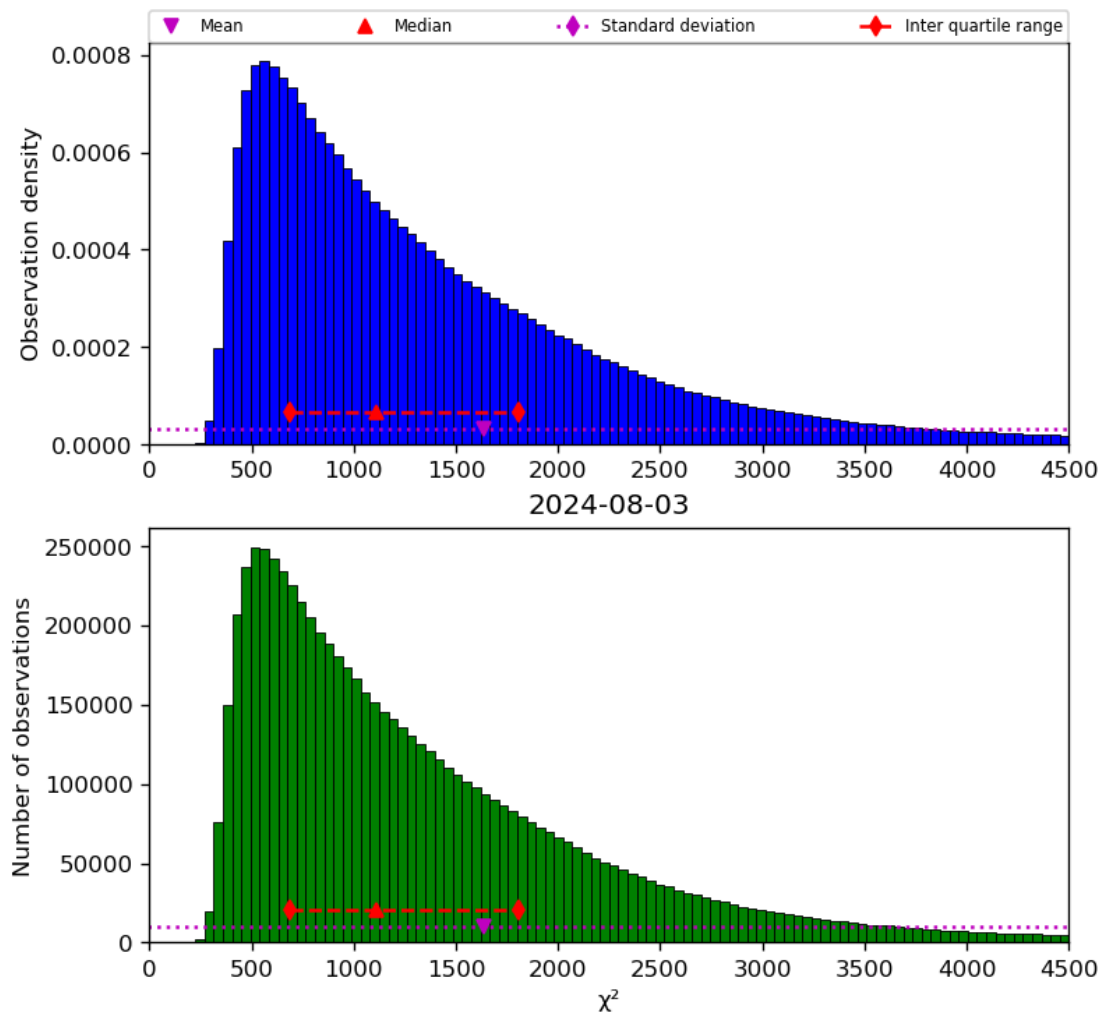
Figure 22: Histogram of “ \chi^2 ” for 2024-08-02 to 2024-08-04
