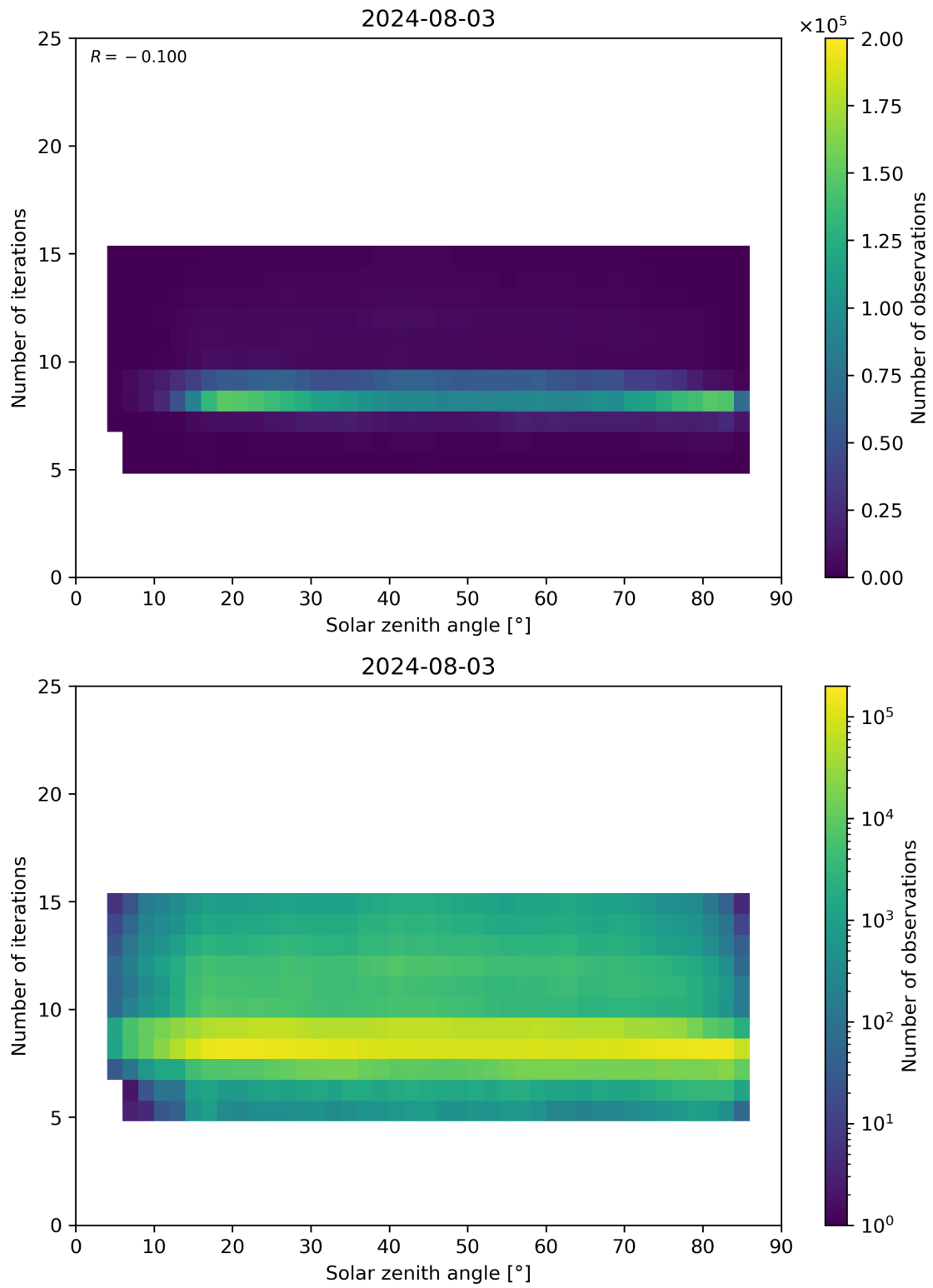
Figure 67: Scatter density plot of “Solar zenith angle” against “Number of iterations” for 2024-08-02 to 2024-08-04.
