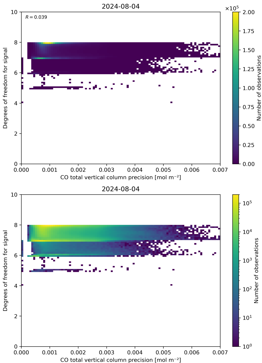
Figure 45: Scatter density plot of “CO total vertical column precision” against “Degrees of freedom for signal” for 2024-08-03 to 2024-08-05.
