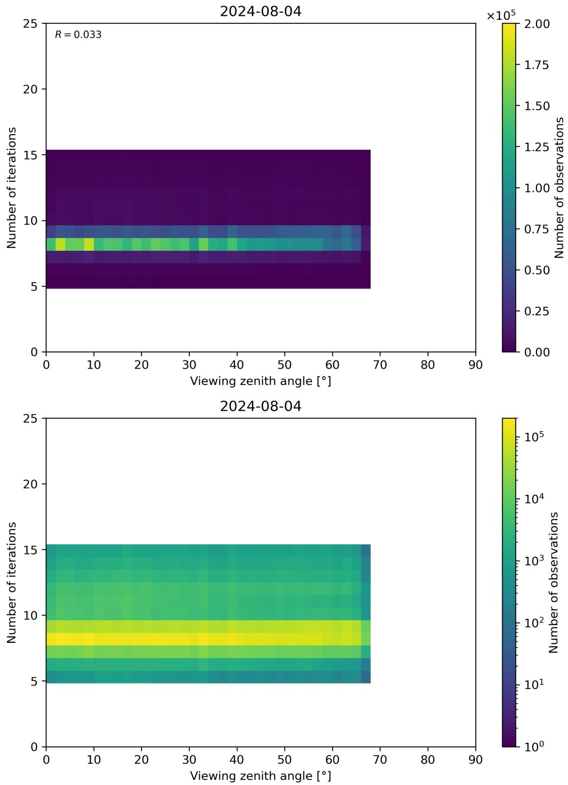
Figure 75: Scatter density plot of “Viewing zenith angle” against “Number of iterations” for 2024-08-03 to 2024-08-05.
