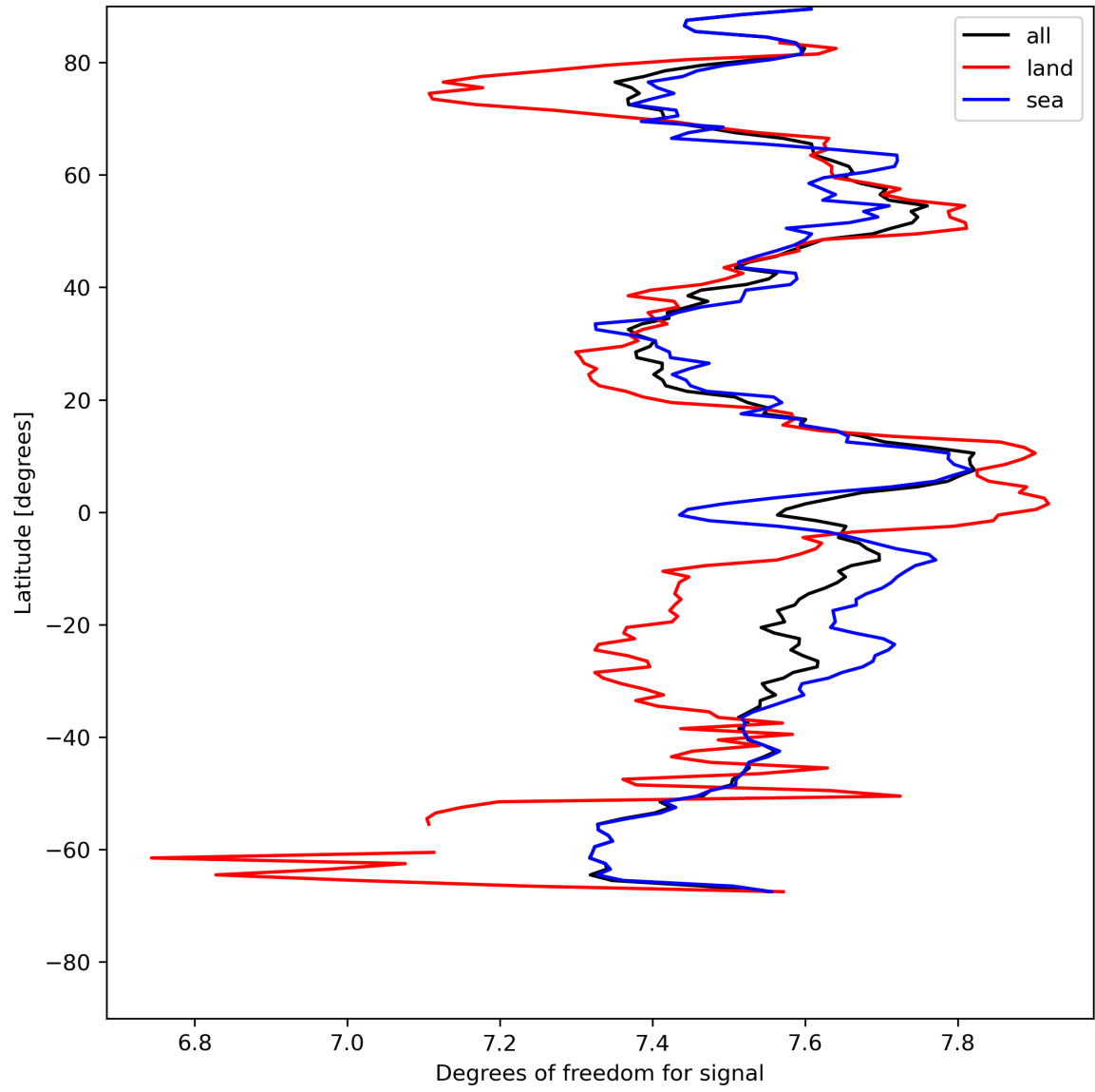
Figure 15: Zonal average of “Degrees of freedom for signal” for 2024-08-03 to 2024-08-05.
