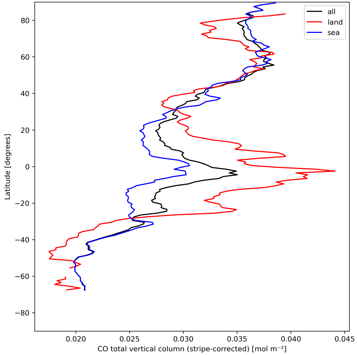
Figure 11: Zonal average of “CO total vertical column (stripe-corrected)” for 2024-08-03 to 2024-08-05.
