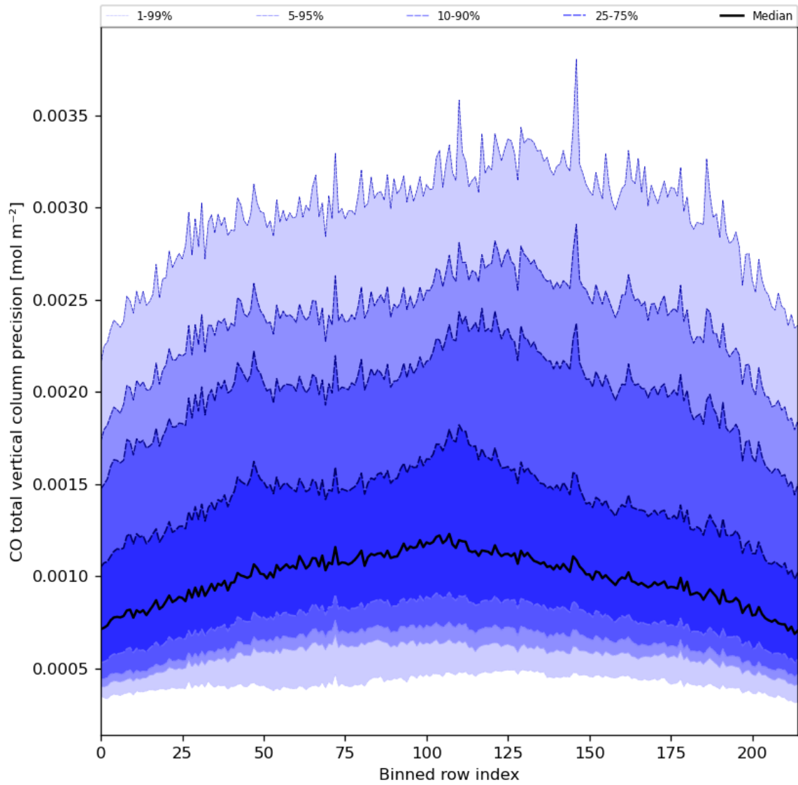
Figure 28: Along track statistics of “CO total vertical column precision” for 2024-08-03 to 2024-08-05
