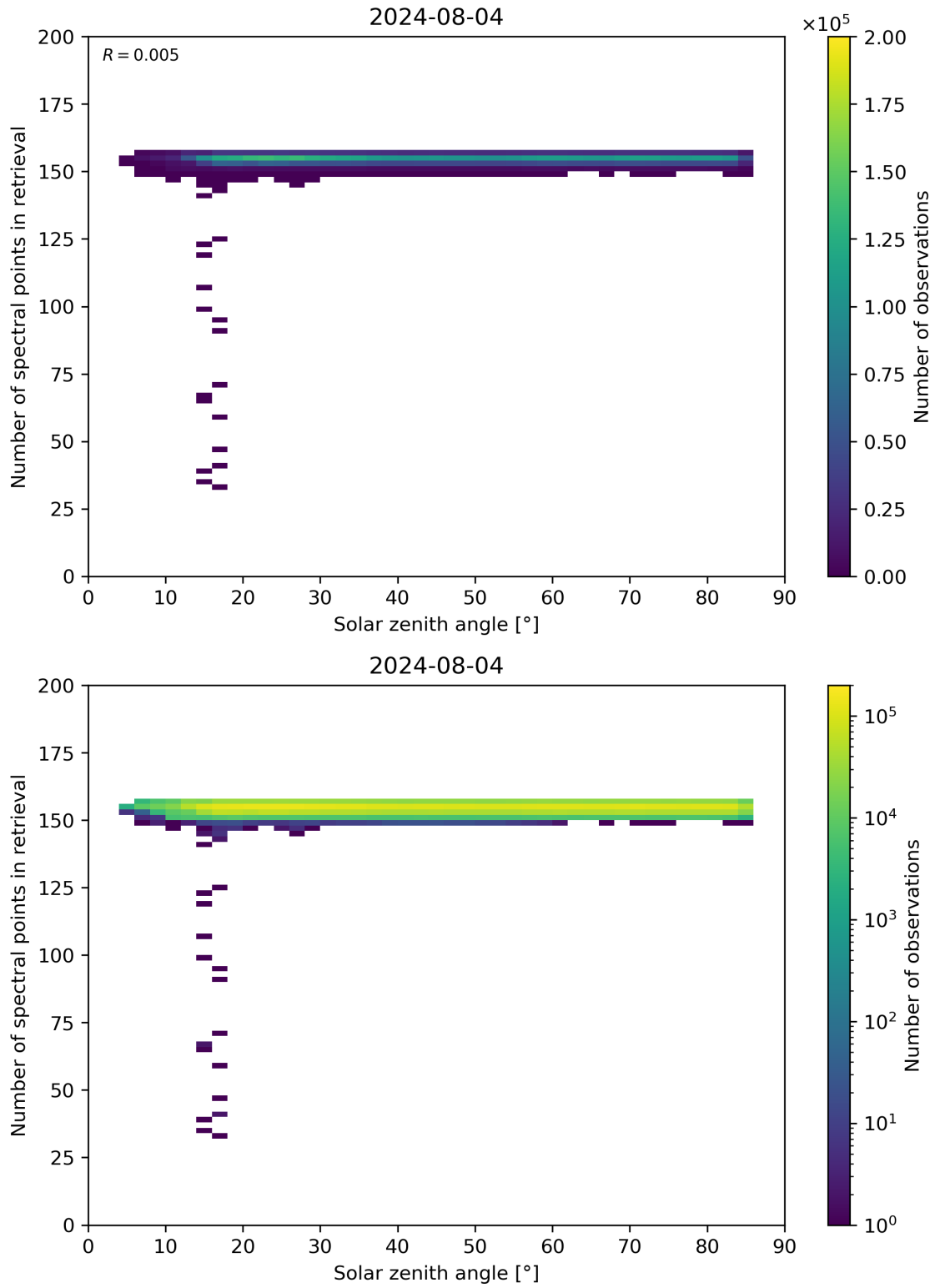
Figure 68: Scatter density plot of “Solar zenith angle” against “Number of spectral points in retrieval” for 2024-08-03 to 2024-08-05.
