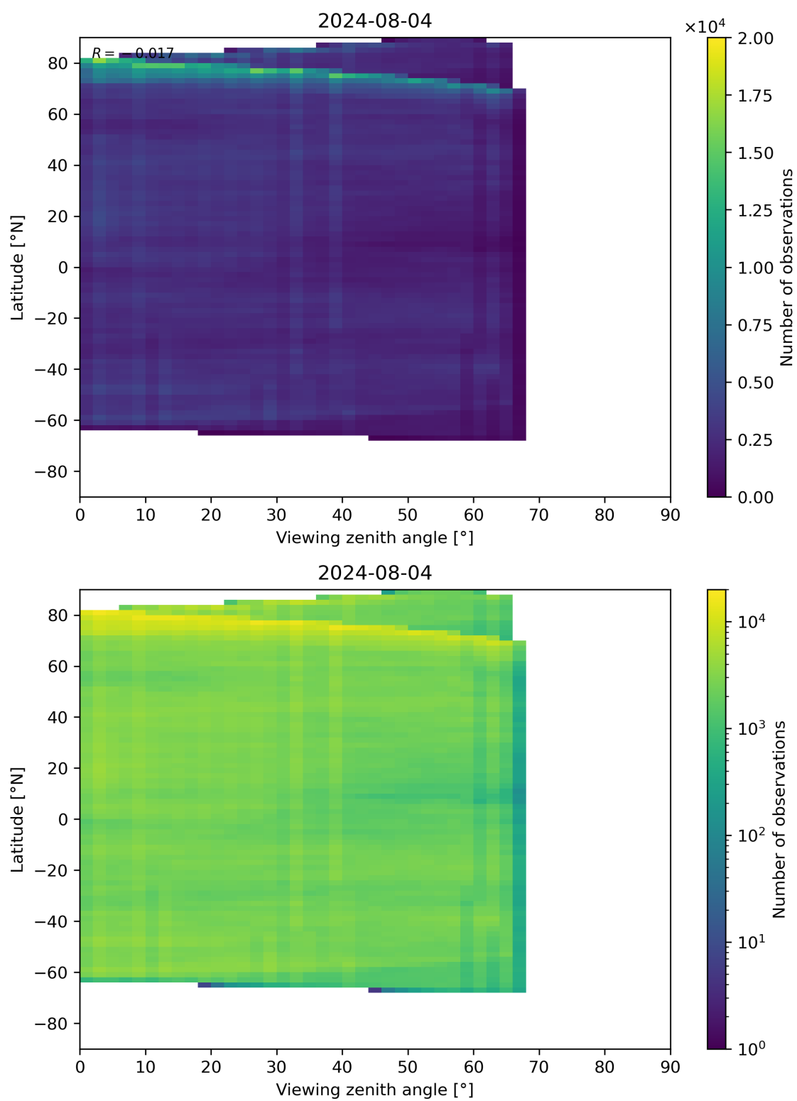
Figure 74: Scatter density plot of “Viewing zenith angle” against “Latitude” for 2024-08-03 to 2024-08-05.
