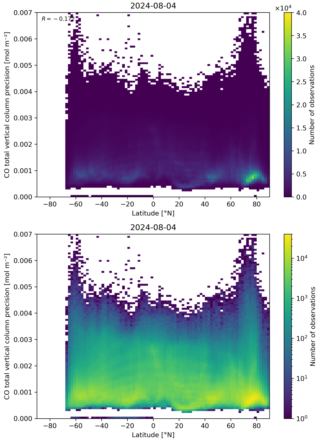
Figure 53: Scatter density plot of “Latitude” against “CO total vertical column precision” for 2024-08-03 to 2024-08-05.
