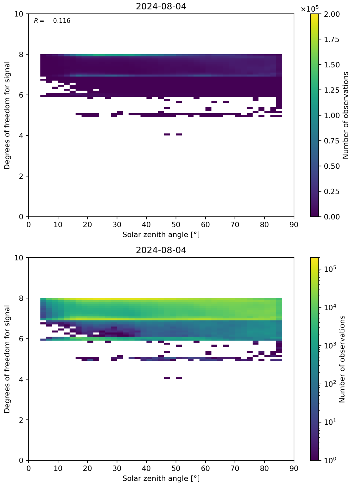
Figure 65: Scatter density plot of “Solar zenith angle” against “Degrees of freedom for signal” for 2024-08-03 to 2024-08-05.
