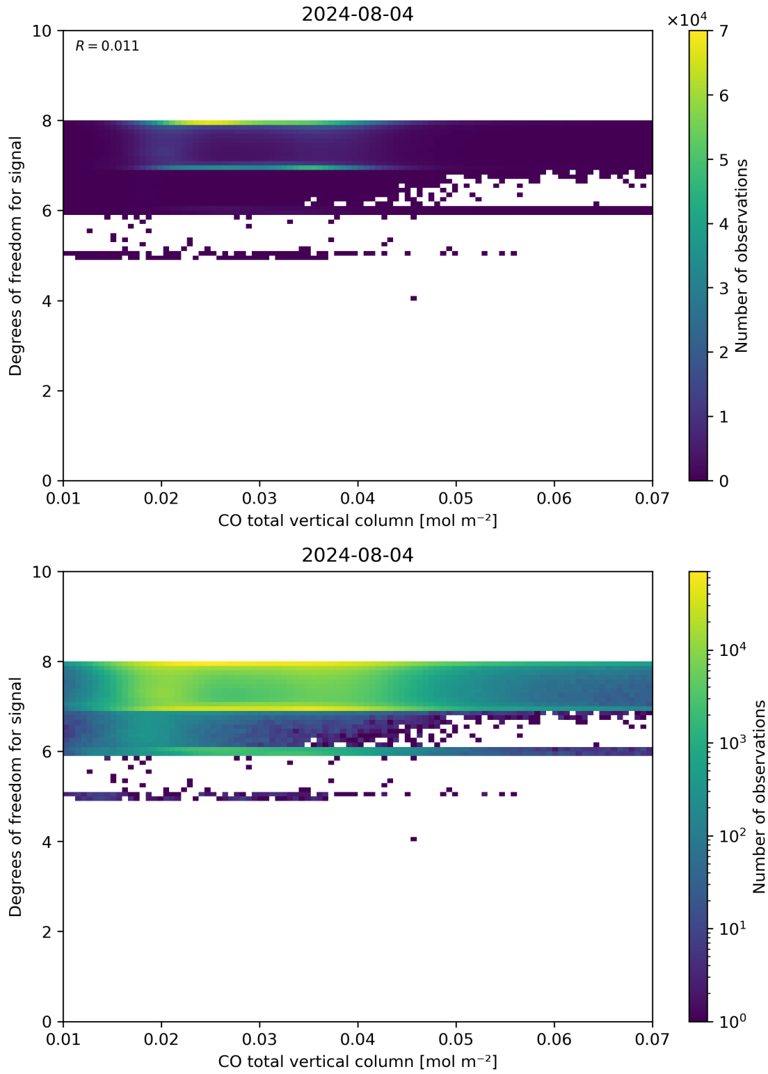
Figure 41: Scatter density plot of “CO total vertical column” against “Degrees of freedom for signal” for 2024-08-03 to 2024-08-05.
