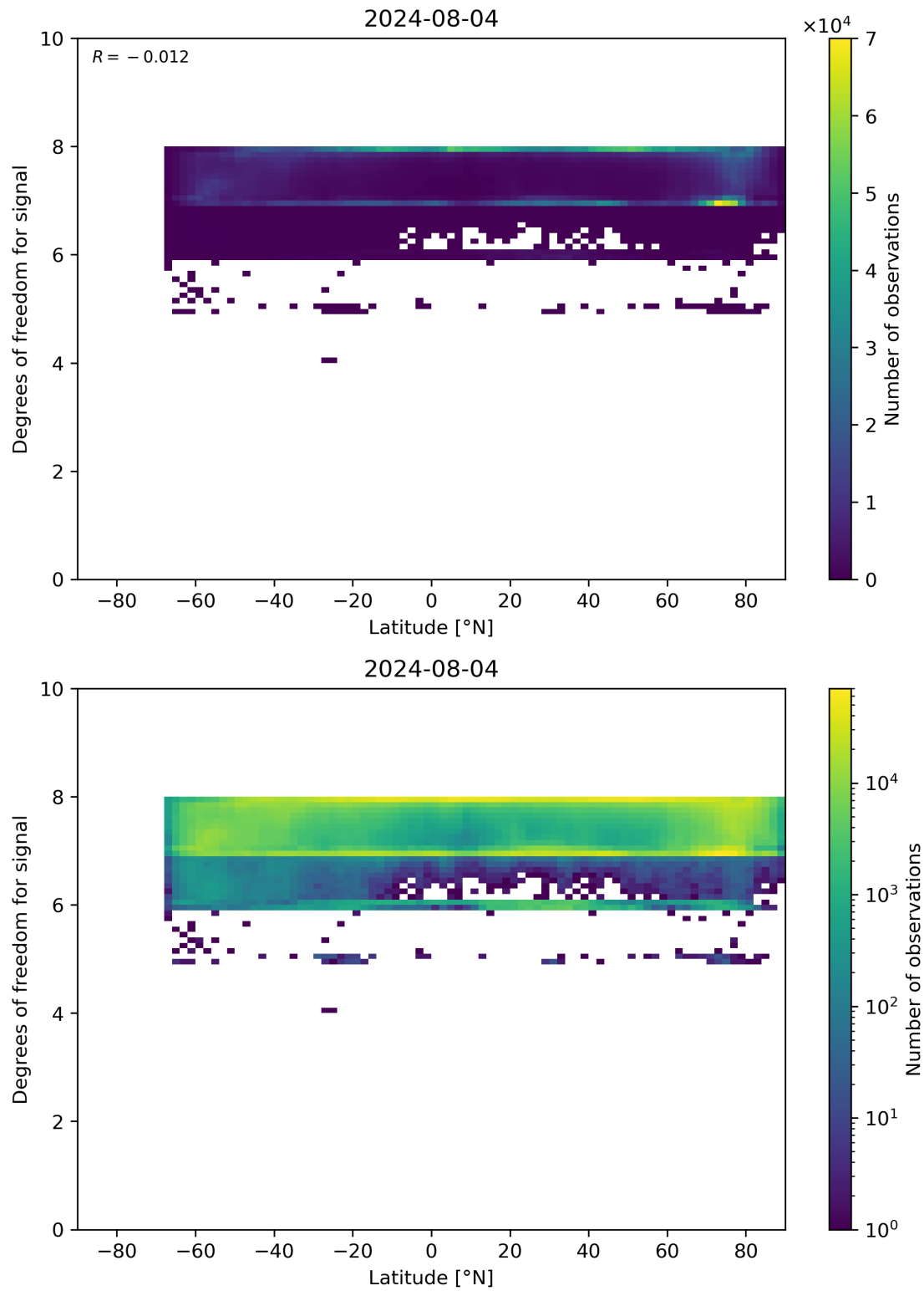
Figure 55: Scatter density plot of “Latitude” against “Degrees of freedom for signal” for 2024-08-03 to 2024-08-05.
