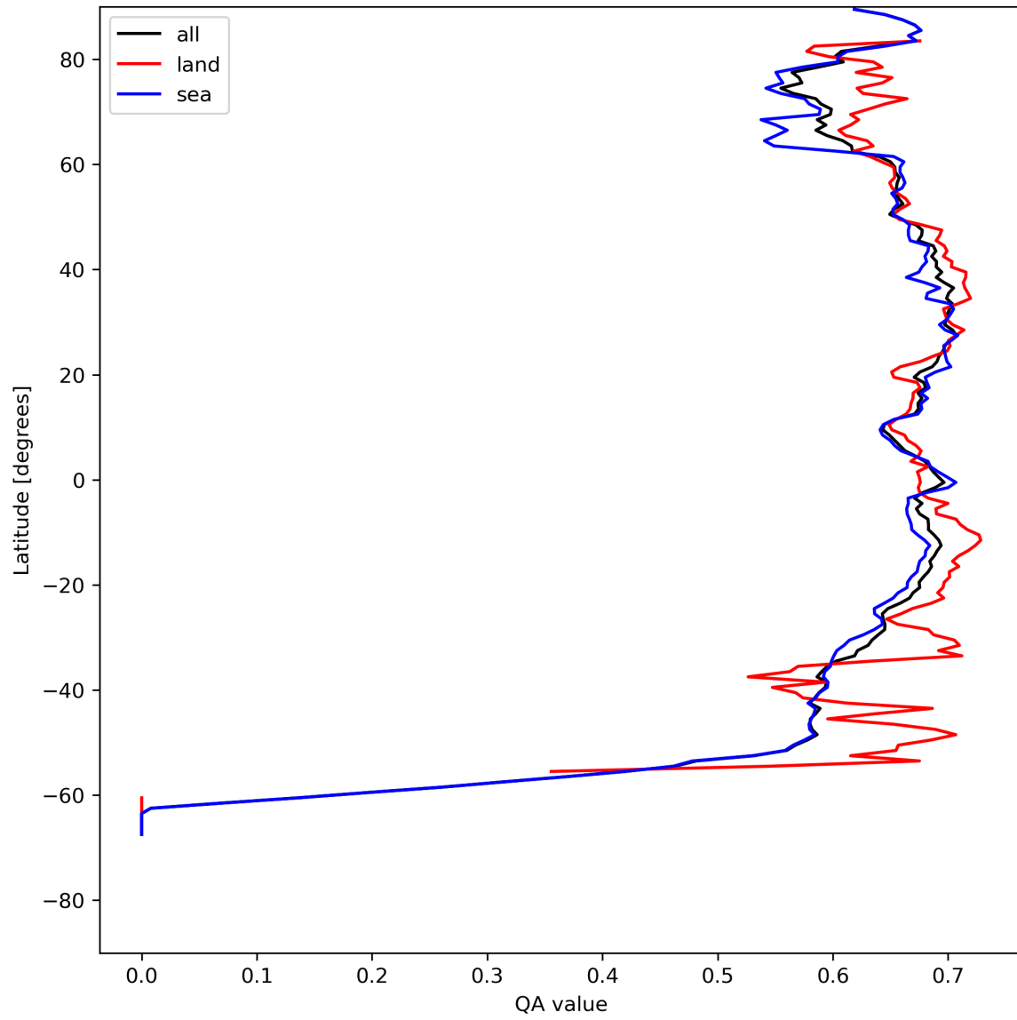
Figure 9: Zonal average of “QA value” for 2024-08-03 to 2024-08-05.
