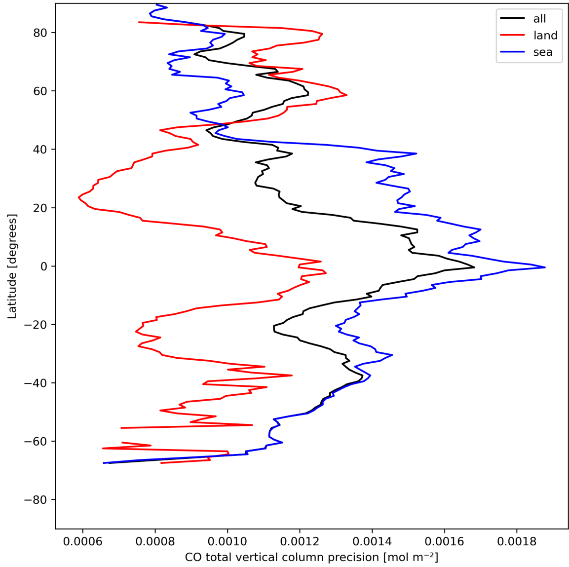
Figure 12: Zonal average of “CO total vertical column precision” for 2024-08-03 to 2024-08-05.
