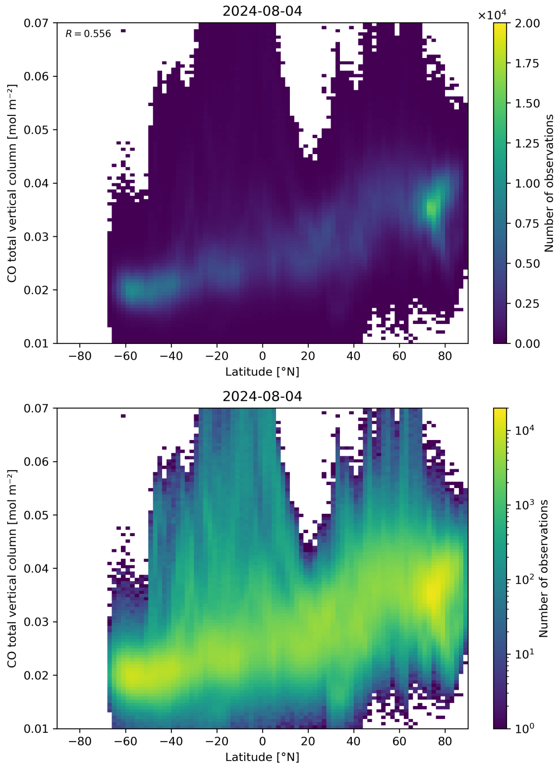
Figure 51: Scatter density plot of “Latitude” against “CO total vertical column” for 2024-08-03 to 2024-08-05.
