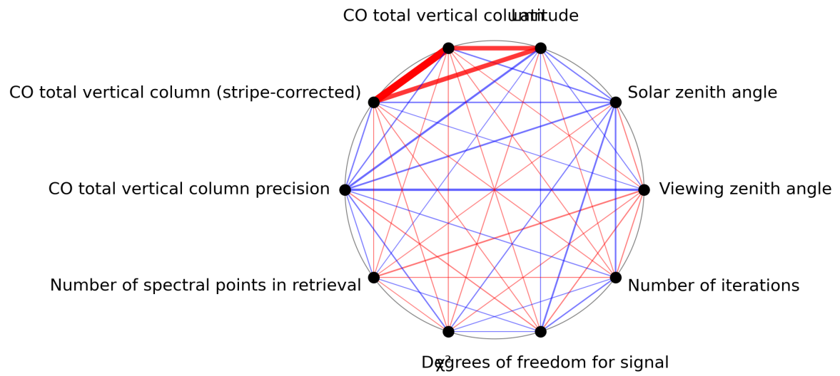
Figure 1: Map of correlation graph for 2024-08-03 to 2024-08-05.
