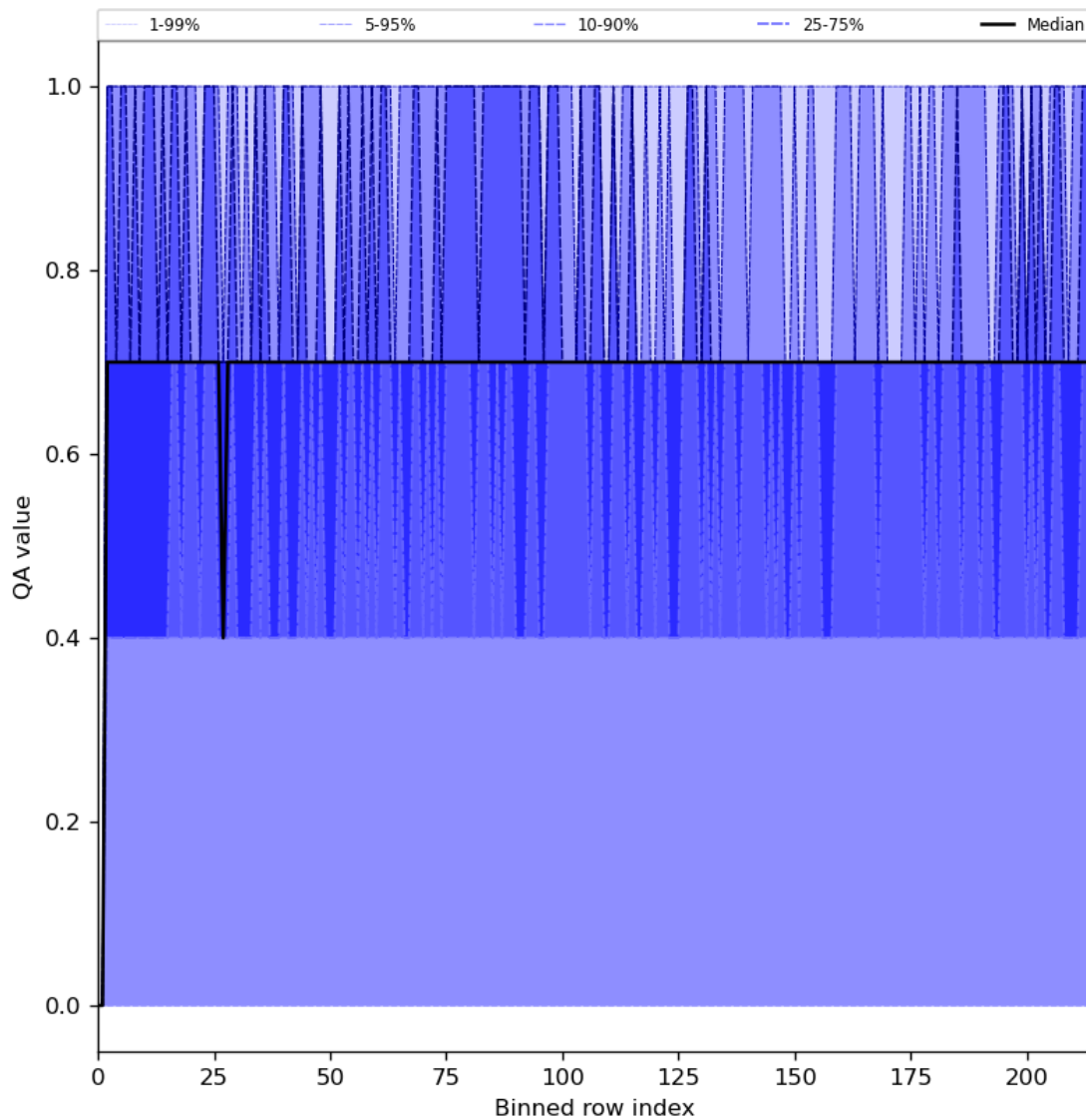
Figure 25: Along track statistics of “QA value” for 2024-08-03 to 2024-08-05
