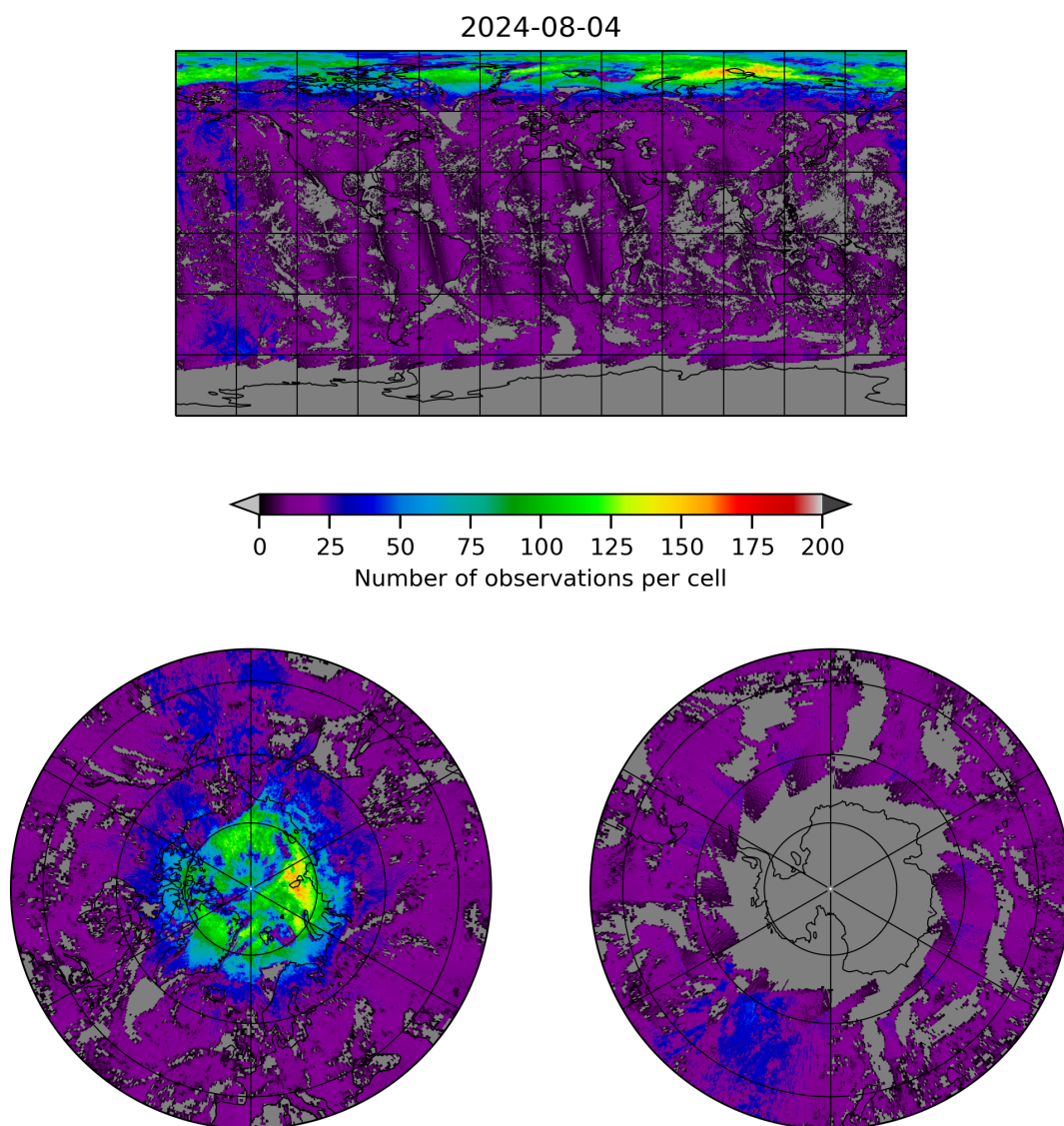
Figure 8: Map of the number of observations for 2024-08-03 to 2024-08-05
