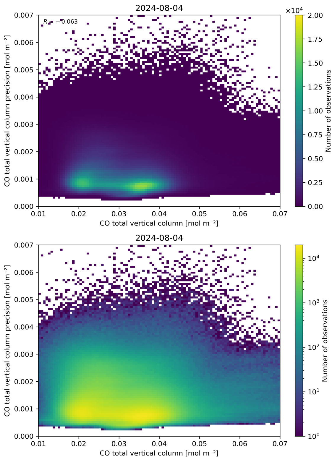
Figure 34: Scatter density plot of “CO total vertical column” against “CO total vertical column precision” for 2024-08-03 to 2024-08-05.
