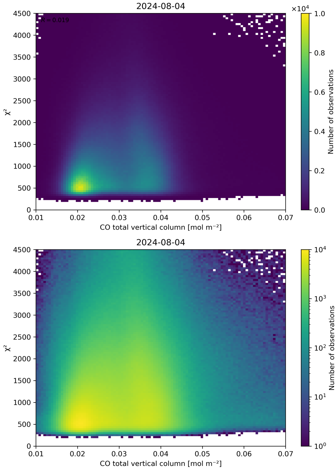
Figure 35: Scatter density plot of “CO total vertical column” against “ \chi^2 ” for 2024-08-03 to 2024-08-05.
