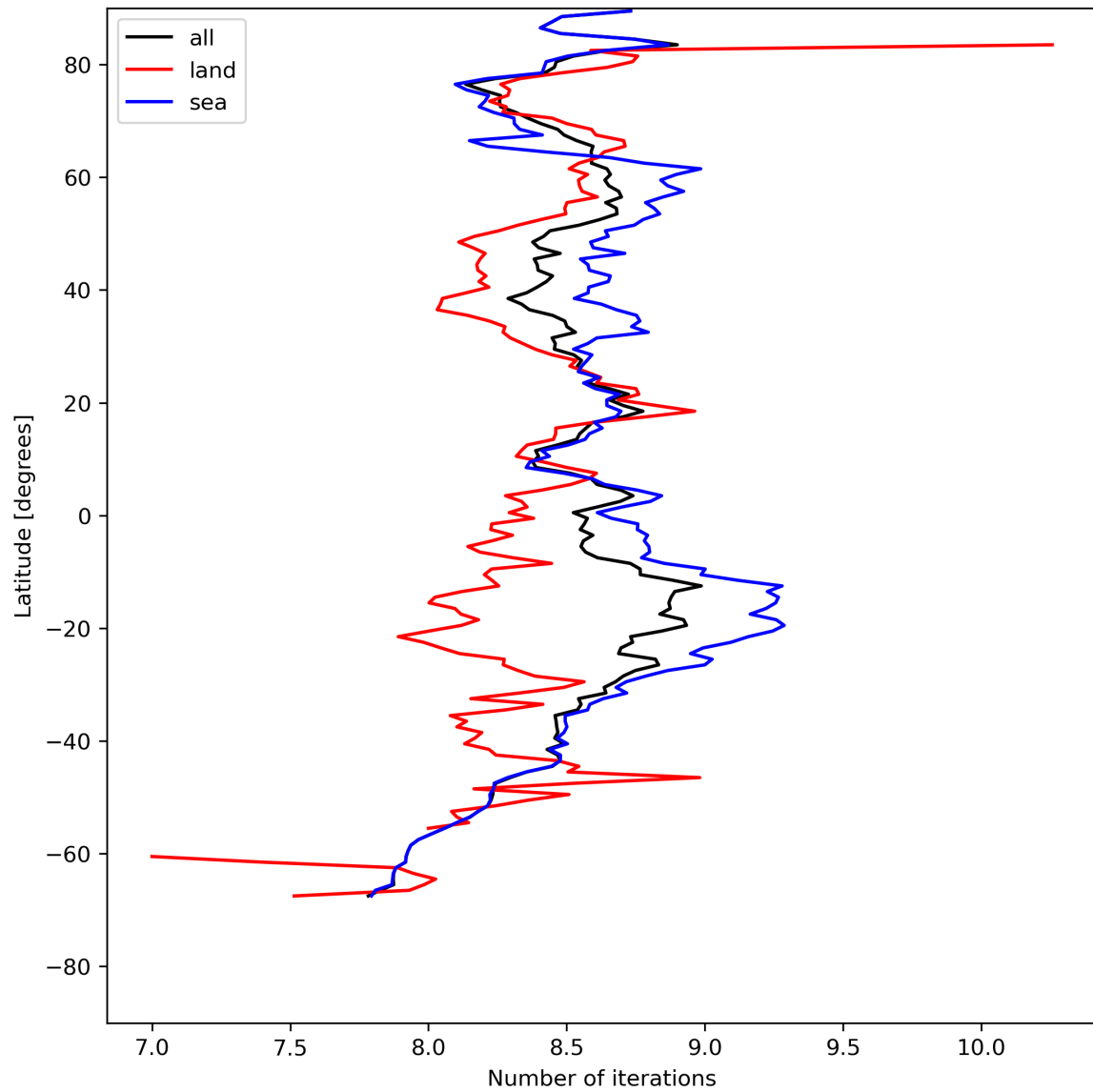
Figure 16: Zonal average of “Number of iterations” for 2024-08-03 to 2024-08-05.
