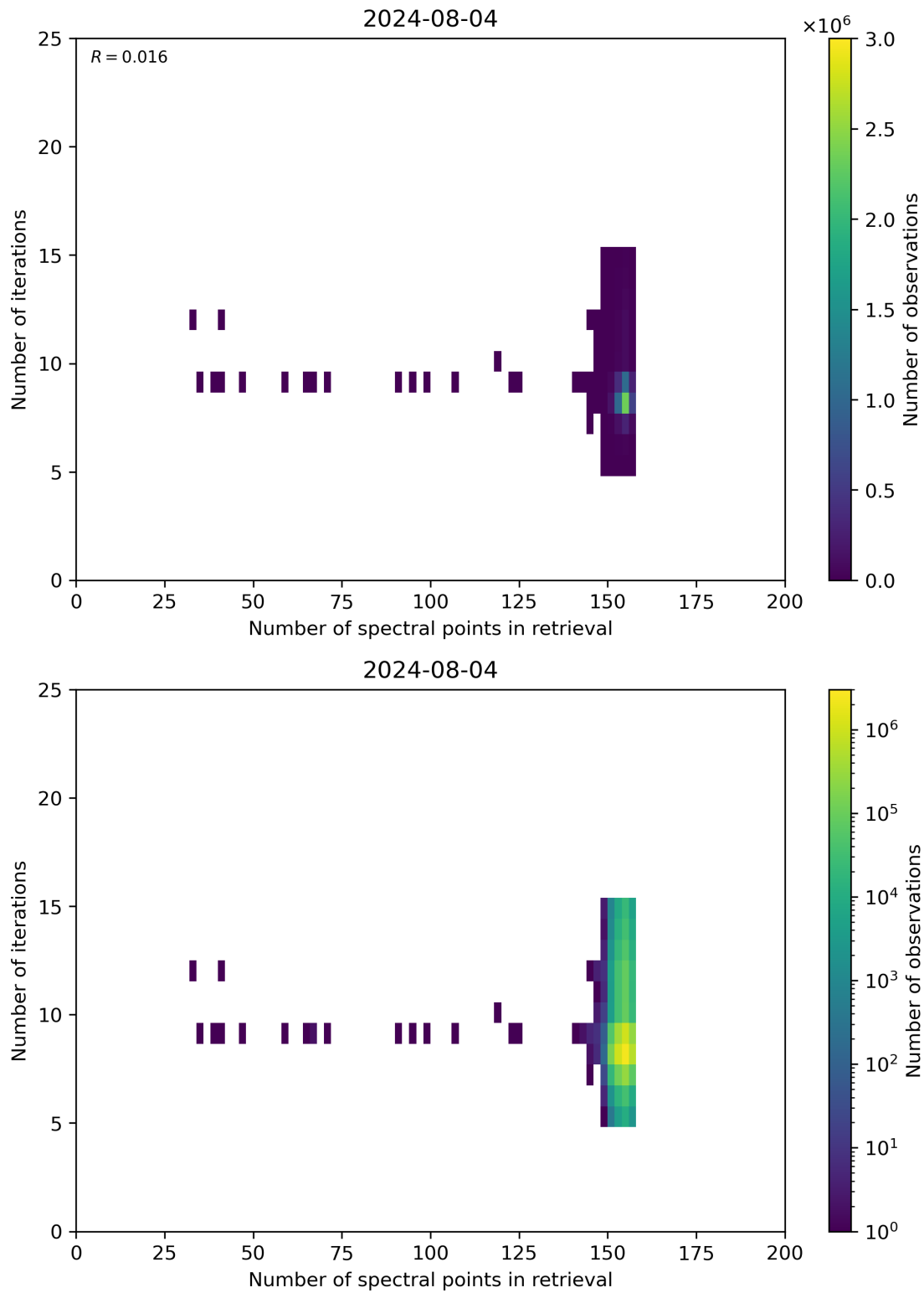
Figure 60: Scatter density plot of “Number of spectral points in retrieval” against “Number of iterations” for 2024-08-03 to 2024-08-05.
