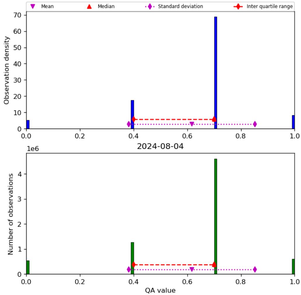
Figure 17: Histogram of “QA value” for 2024-08-03 to 2024-08-05
