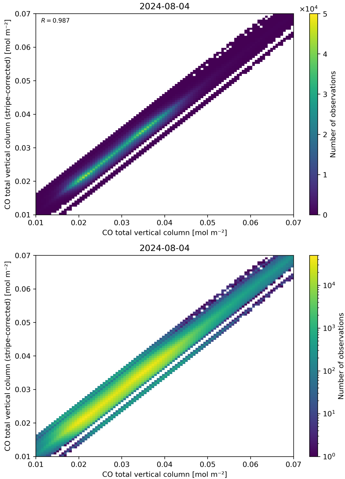
Figure 33: Scatter density plot of “CO total vertical column” against “CO total vertical column (stripe-corrected)” for 2024-08-03 to 2024-08-05.
