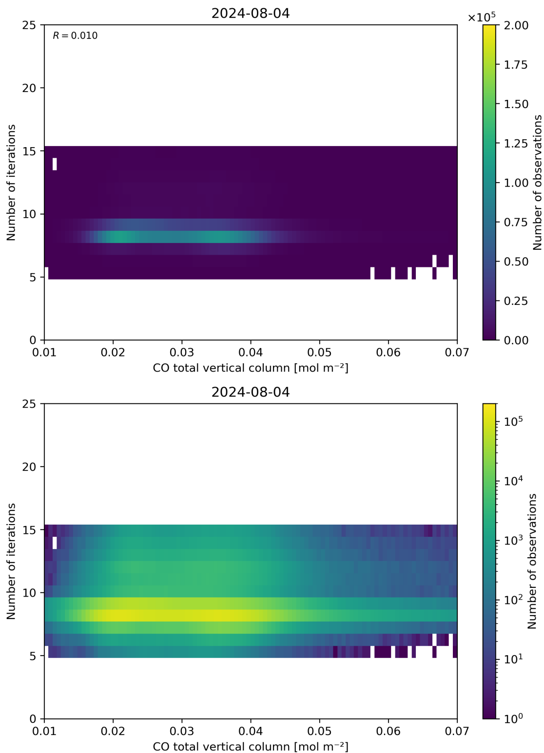
Figure 42: Scatter density plot of “CO total vertical column” against “Number of iterations” for 2024-08-03 to 2024-08-05.
