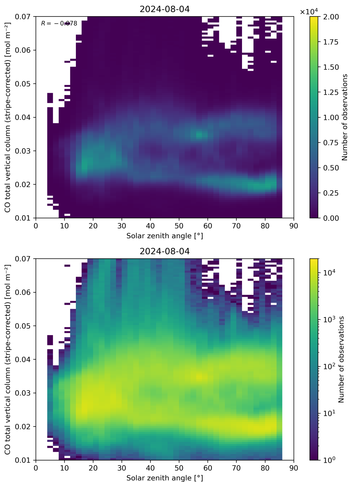
Figure 62: Scatter density plot of “Solar zenith angle” against “CO total vertical column (stripe-corrected)” for 2024-08-03 to 2024-08-05.
