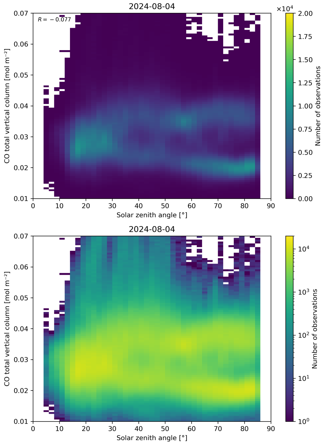
Figure 61: Scatter density plot of “Solar zenith angle” against “CO total vertical column” for 2024-08-03 to 2024-08-05.
