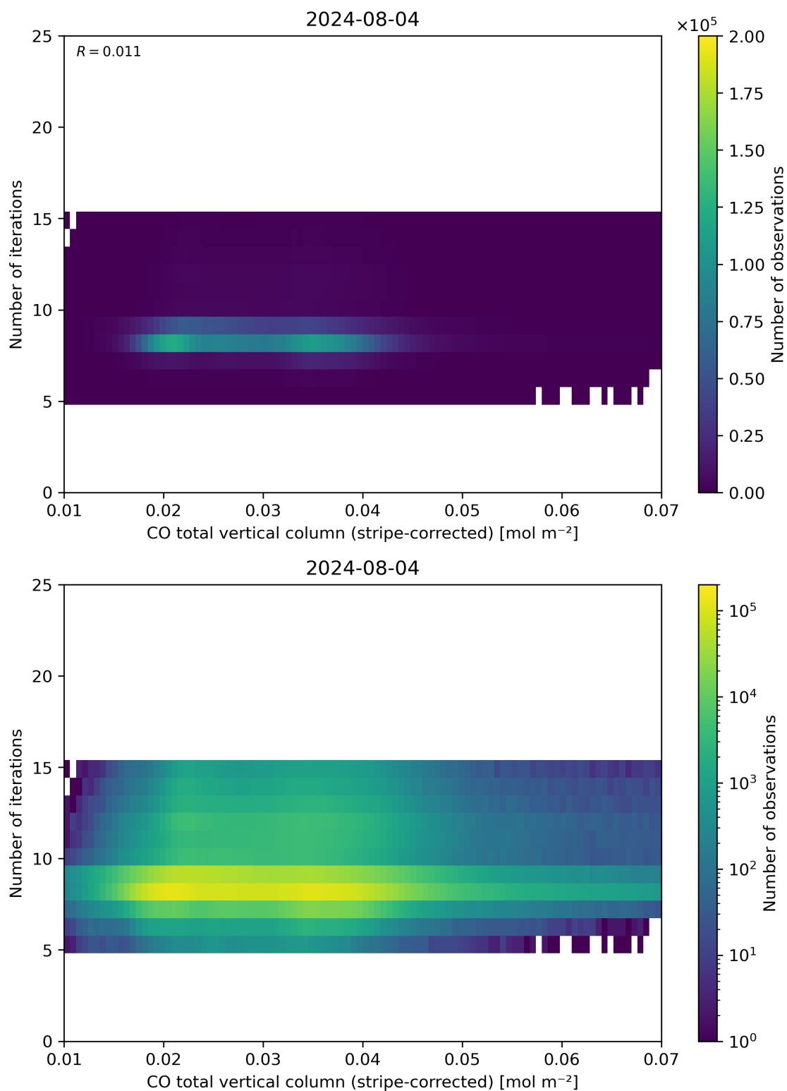
Figure 39: Scatter density plot of “CO total vertical column (stripe-corrected)” against “Number of iterations” for 2024-08-03 to 2024-08-05.
