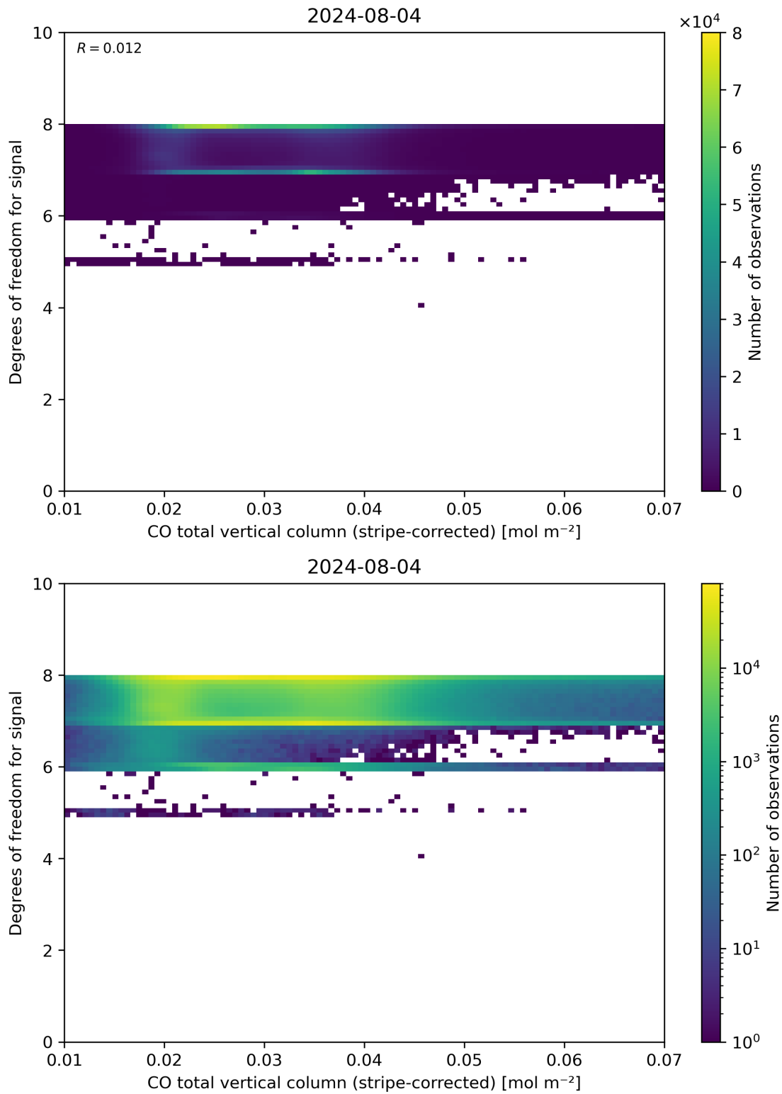
Figure 38: Scatter density plot of “CO total vertical column (stripe-corrected)” against “Degrees of freedom for signal” for 2024-08-03 to 2024-08-05.
