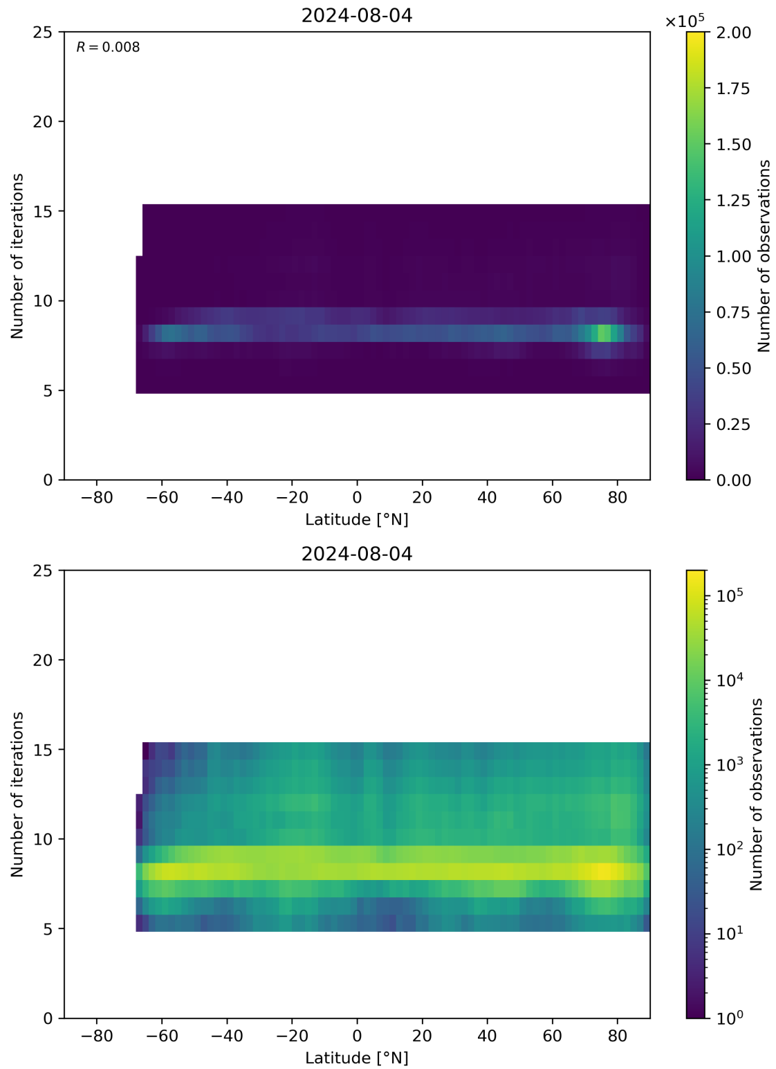
Figure 56: Scatter density plot of “Latitude” against “Number of iterations” for 2024-08-03 to 2024-08-05.
