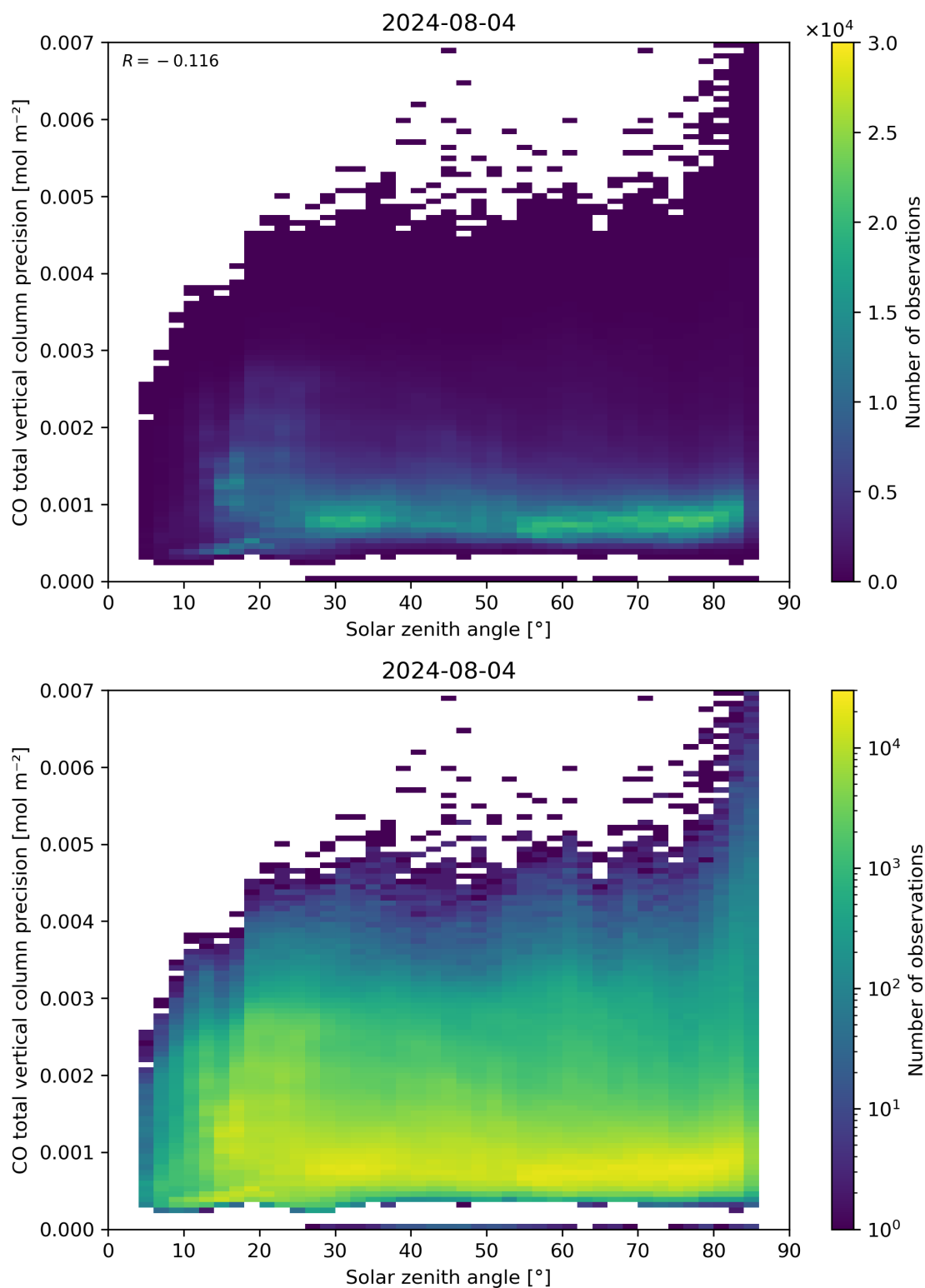
Figure 63: Scatter density plot of “Solar zenith angle” against “CO total vertical column precision” for 2024-08-03 to 2024-08-05.
