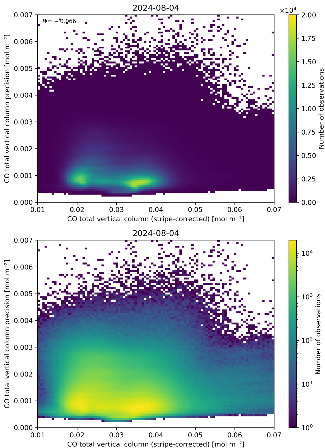
Figure 36: Scatter density plot of “CO total vertical column (stripe-corrected)” against “CO total vertical column precision” for 2024-08-03 to 2024-08-05.
