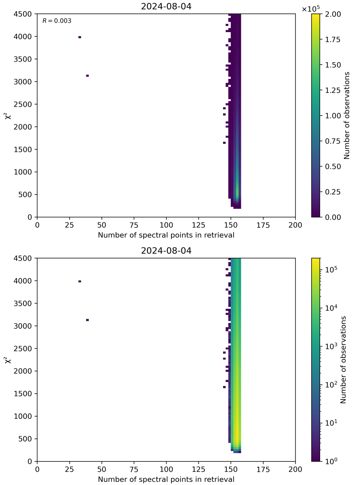
Figure 58: Scatter density plot of “Number of spectral points in retrieval” against “ \chi^2 ” for 2024-08-03 to 2024-08-05.
