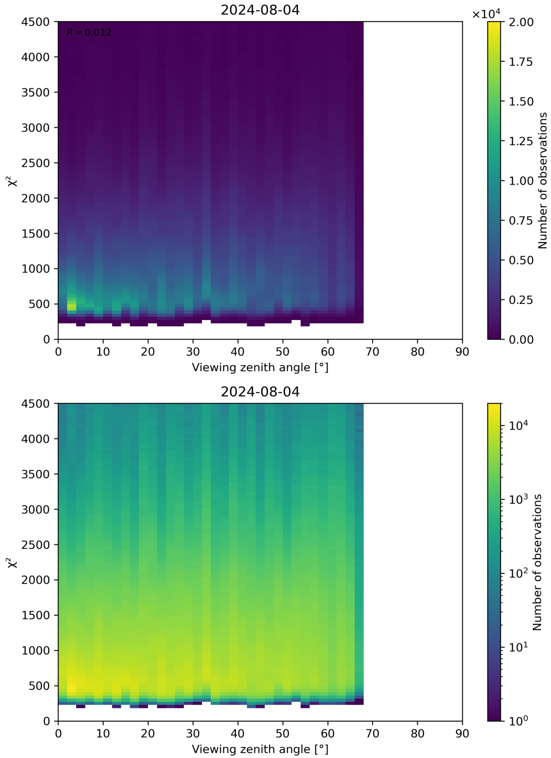
Figure 72: Scatter density plot of “Viewing zenith angle” against “ \chi^2 ” for 2024-08-03 to 2024-08-05.
