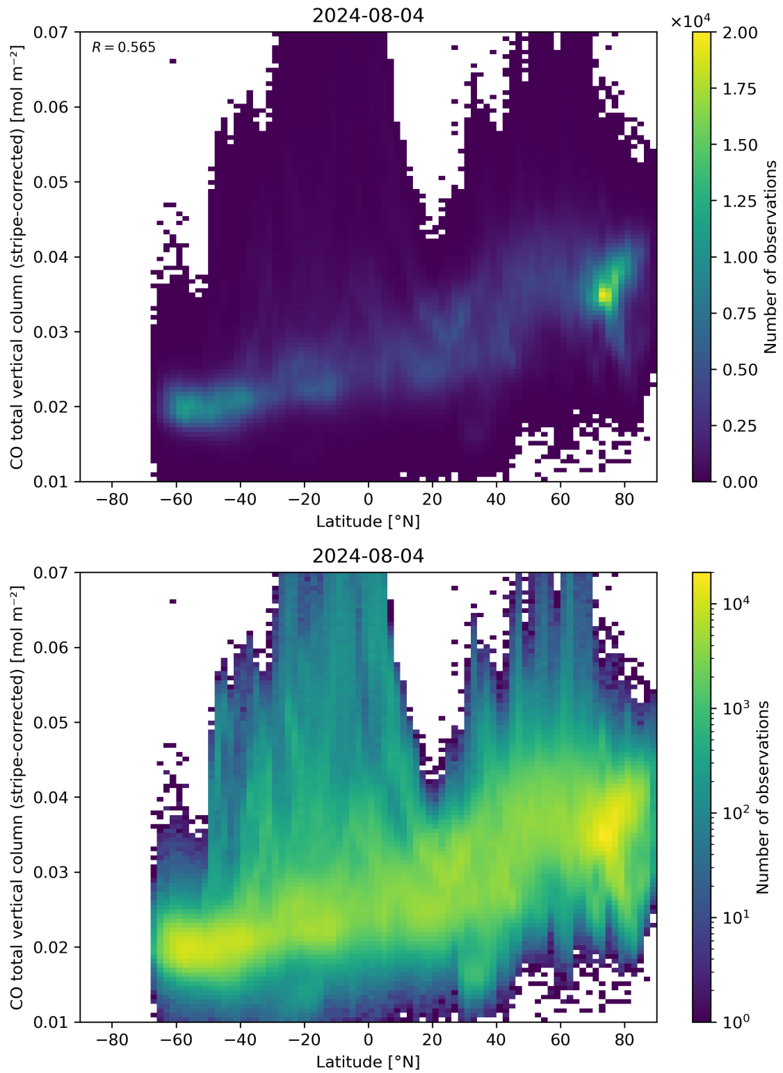
Figure 52: Scatter density plot of “Latitude” against “CO total vertical column (stripe-corrected)” for 2024-08-03 to 2024-08-05.
