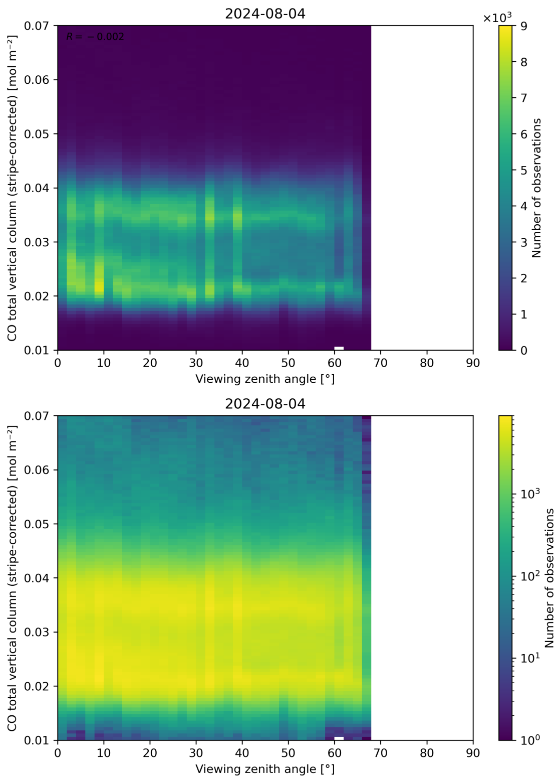
Figure 70: Scatter density plot of “Viewing zenith angle” against “CO total vertical column (stripe-corrected)” for 2024-08-03 to 2024-08-05.
