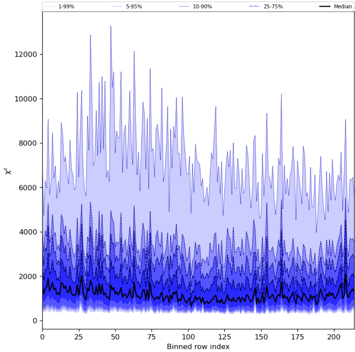
Figure 30: Along track statistics of “ \chi^2 ” for 2024-08-03 to 2024-08-05
