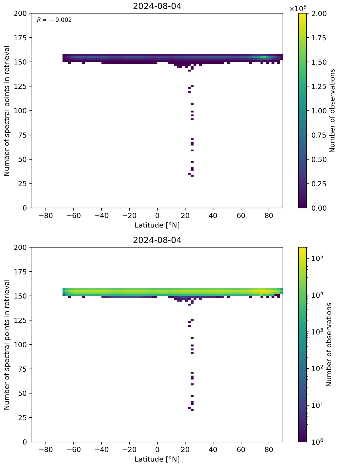
Figure 57: Scatter density plot of “Latitude” against “Number of spectral points in retrieval” for 2024-08-03 to 2024-08-05.
