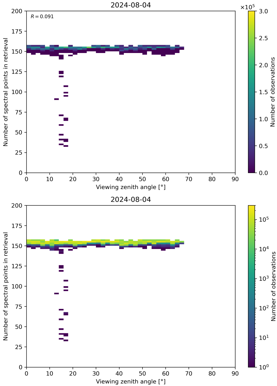
Figure 76: Scatter density plot of “Viewing zenith angle” against “Number of spectral points in retrieval” for 2024-08-03 to 2024-08-05.
