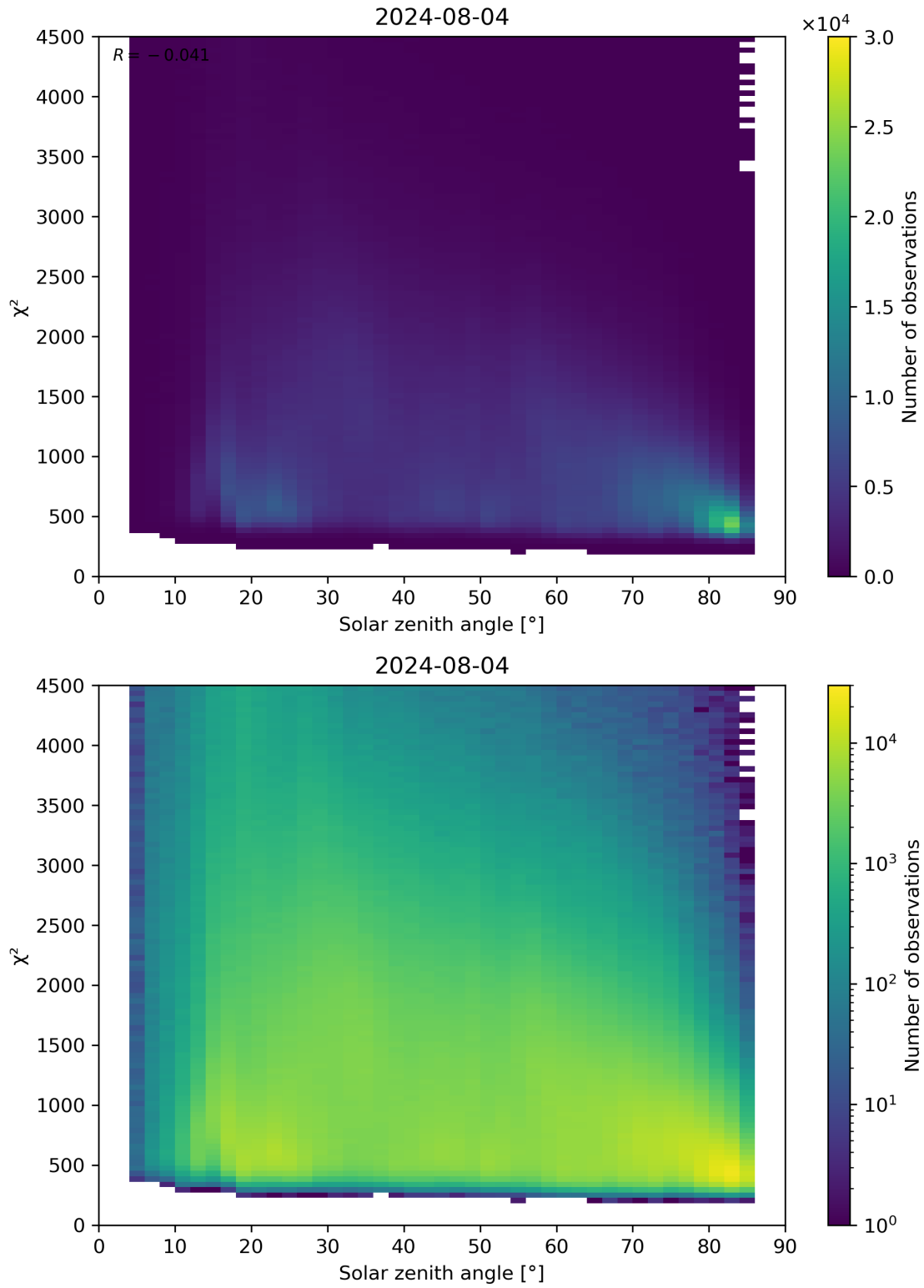
Figure 64: Scatter density plot of “Solar zenith angle” against “ \chi^2 ” for 2024-08-03 to 2024-08-05.
