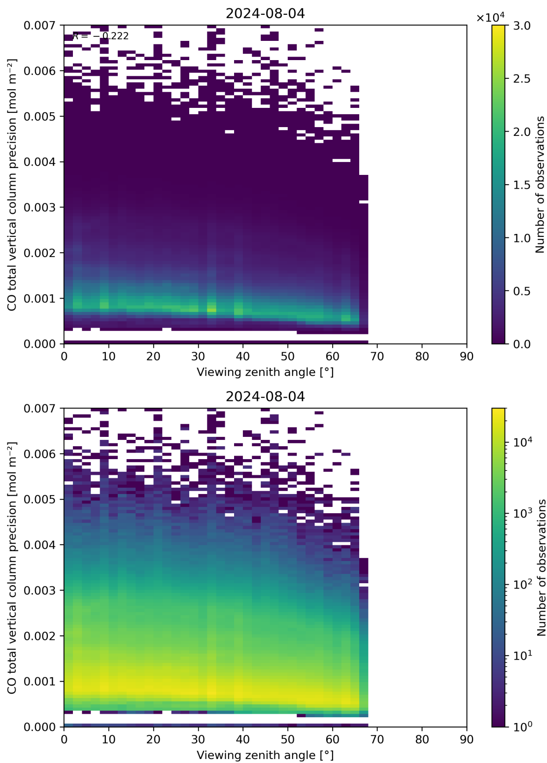
Figure 71: Scatter density plot of “Viewing zenith angle” against “CO total vertical column precision” for 2024-08-03 to 2024-08-05.
