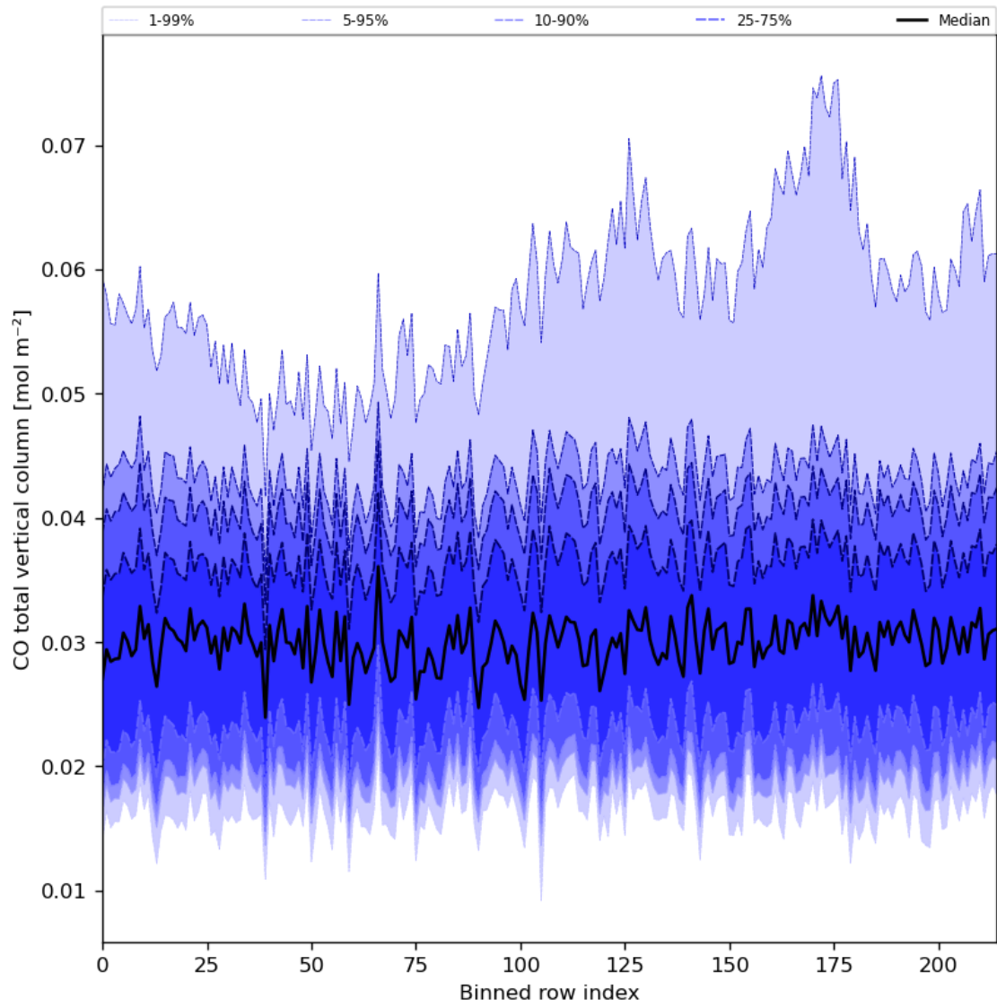
Figure 26: Along track statistics of “CO total vertical column” for 2024-08-03 to 2024-08-05
