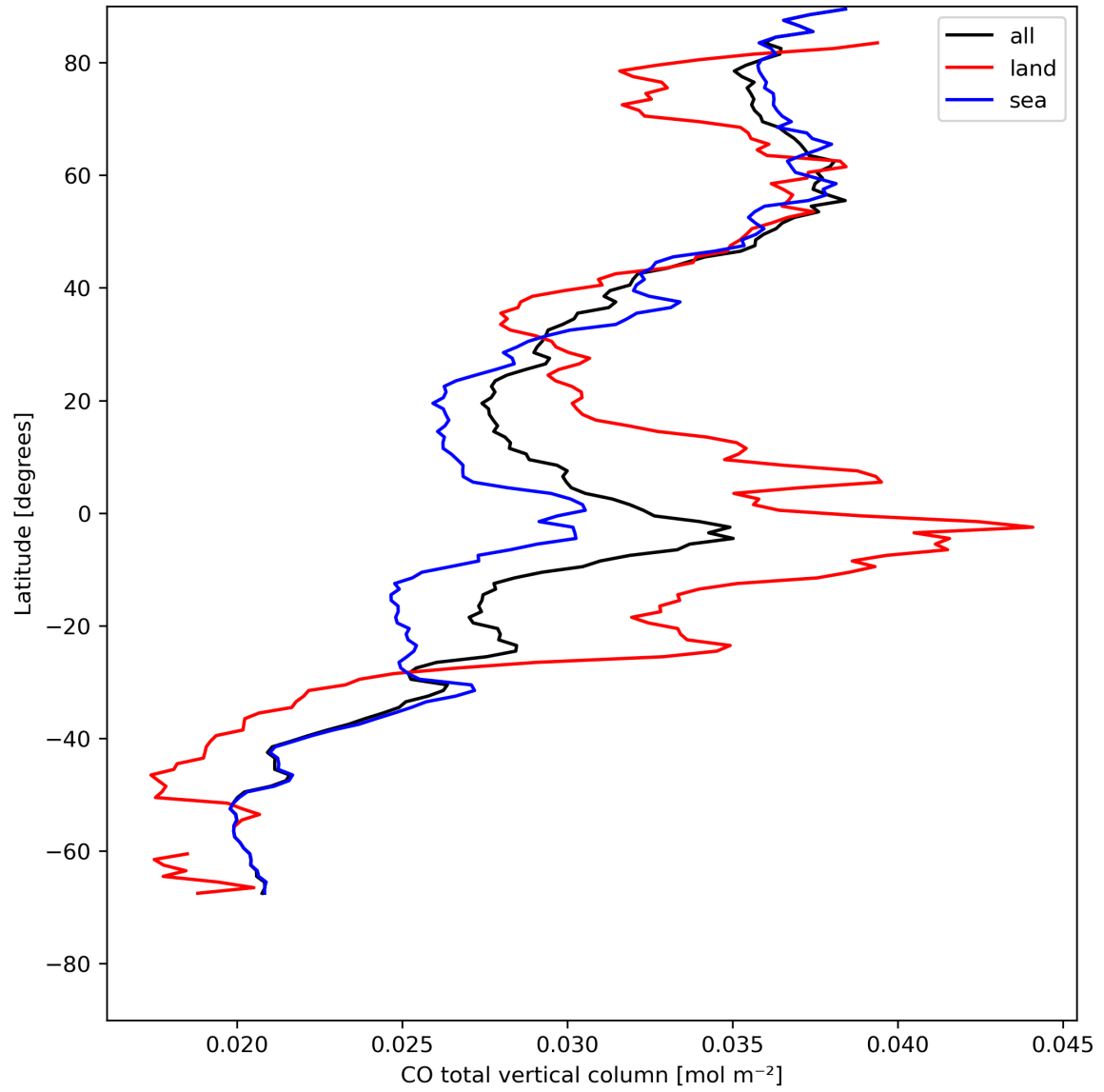
Figure 10: Zonal average of “CO total vertical column” for 2024-08-03 to 2024-08-05.
