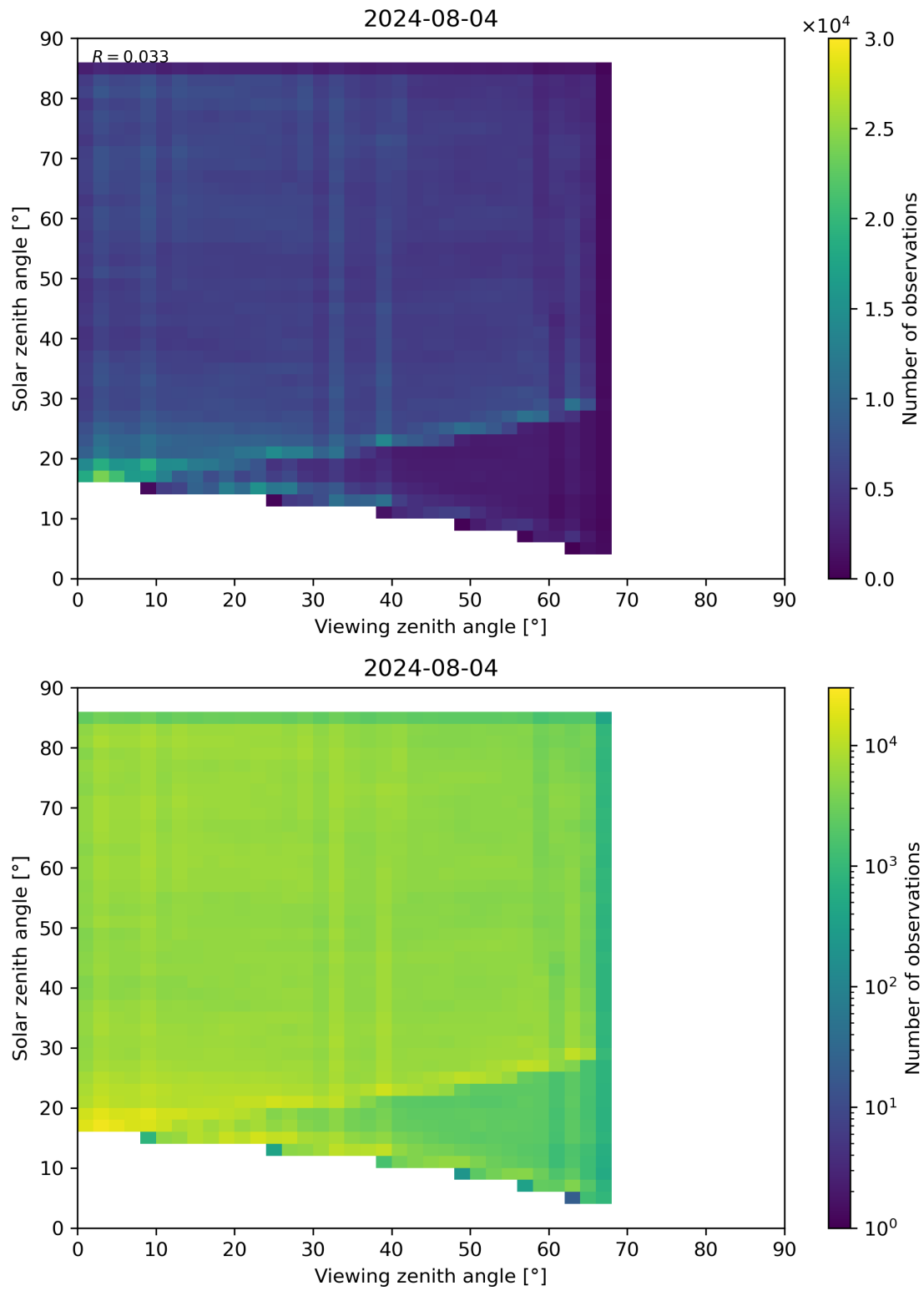
Figure 77: Scatter density plot of “Viewing zenith angle” against “Solar zenith angle” for 2024-08-03 to 2024-08-05.
