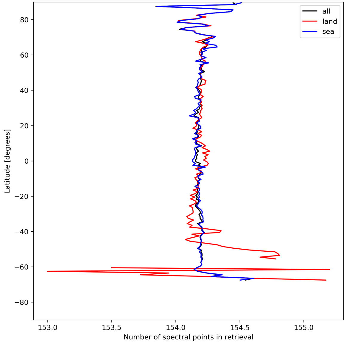
Figure 13: Zonal average of “Number of spectral points in retrieval” for 2024-08-03 to 2024-08-05.
