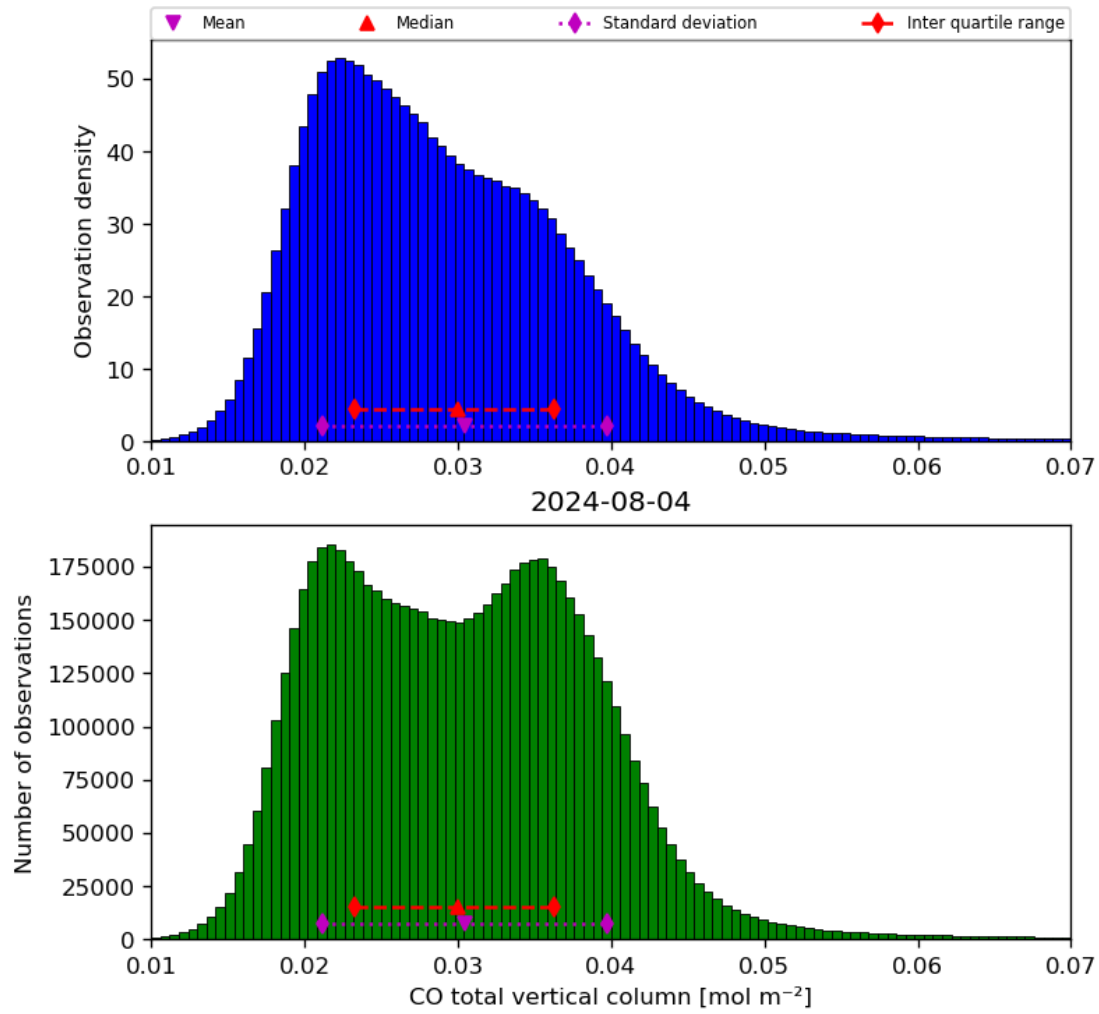
Figure 18: Histogram of “CO total vertical column” for 2024-08-03 to 2024-08-05
