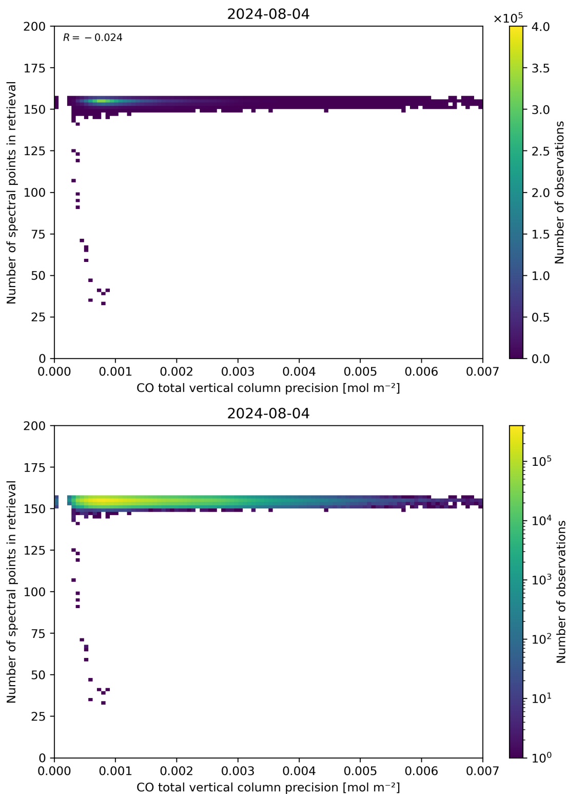
Figure 47: Scatter density plot of “CO total vertical column precision” against “Number of spectral points in retrieval” for 2024-08-03 to 2024-08-05.
