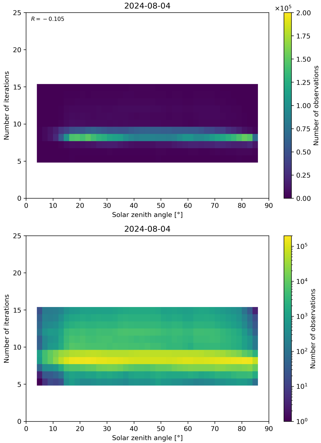
Figure 67: Scatter density plot of “Solar zenith angle” against “Number of iterations” for 2024-08-03 to 2024-08-05.
