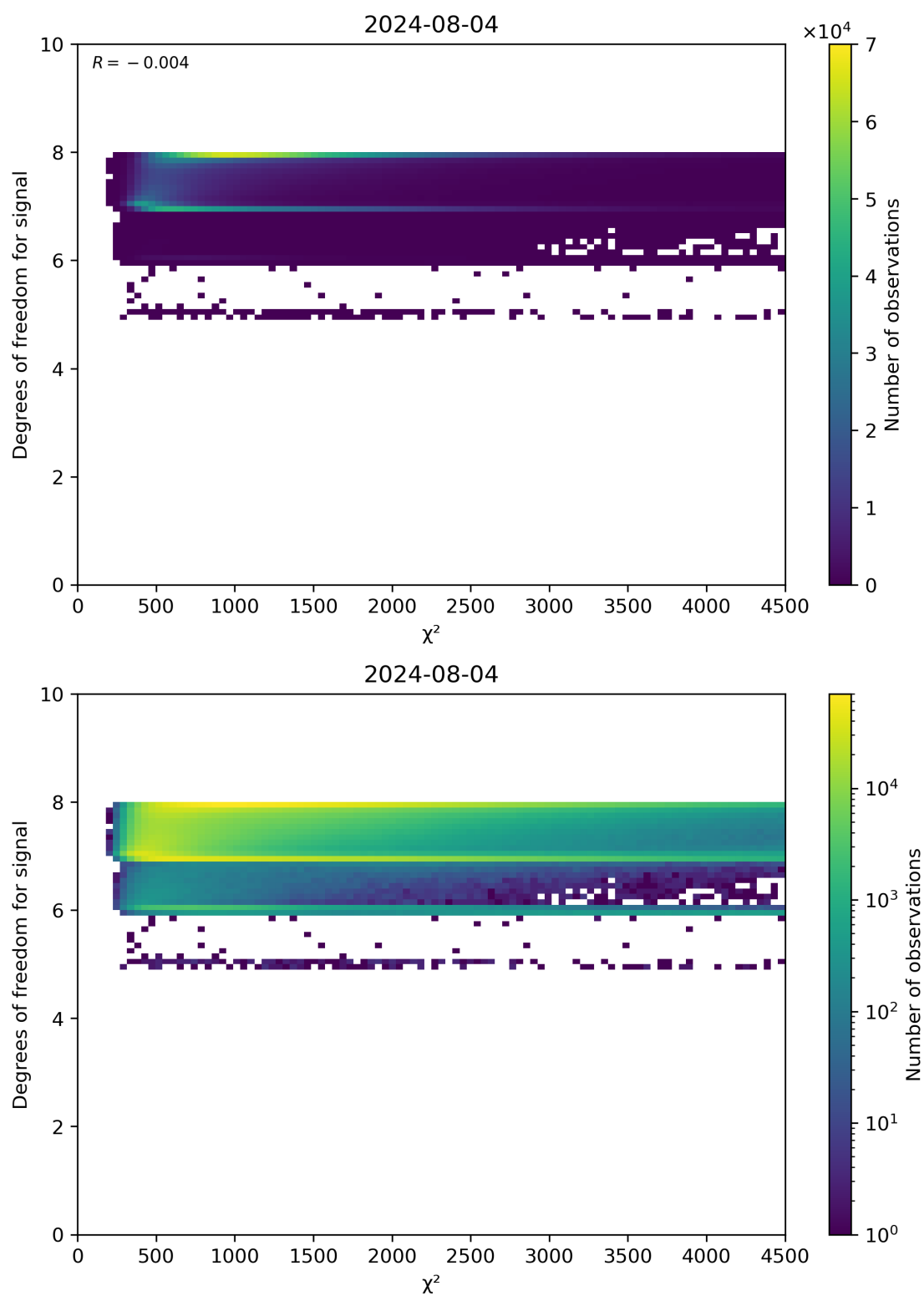
Figure 48: Scatter density plot of “ \chi^2 ” against “Degrees of freedom for signal” for 2024-08-03 to 2024-08-05.
