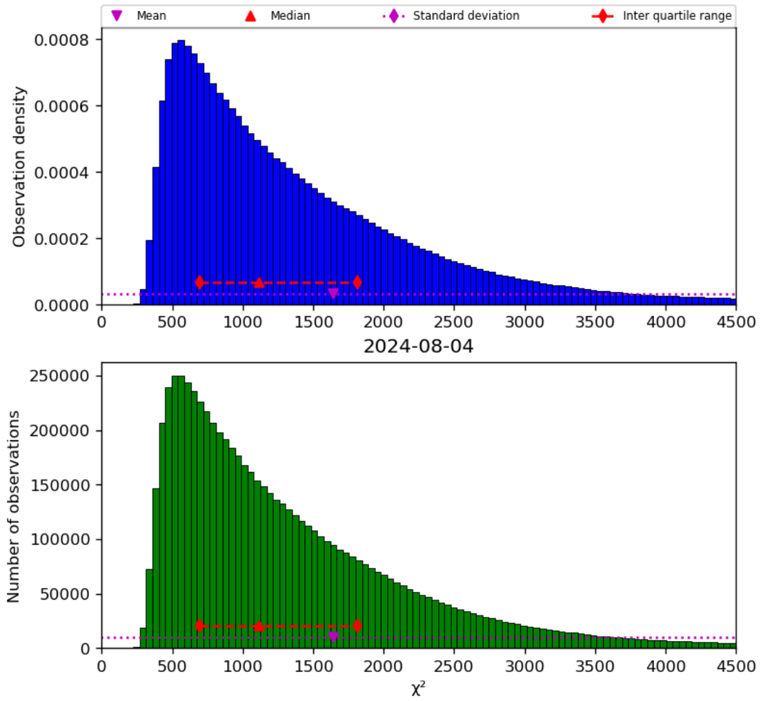
Figure 22: Histogram of “ \chi^2 ” for 2024-08-03 to 2024-08-05
