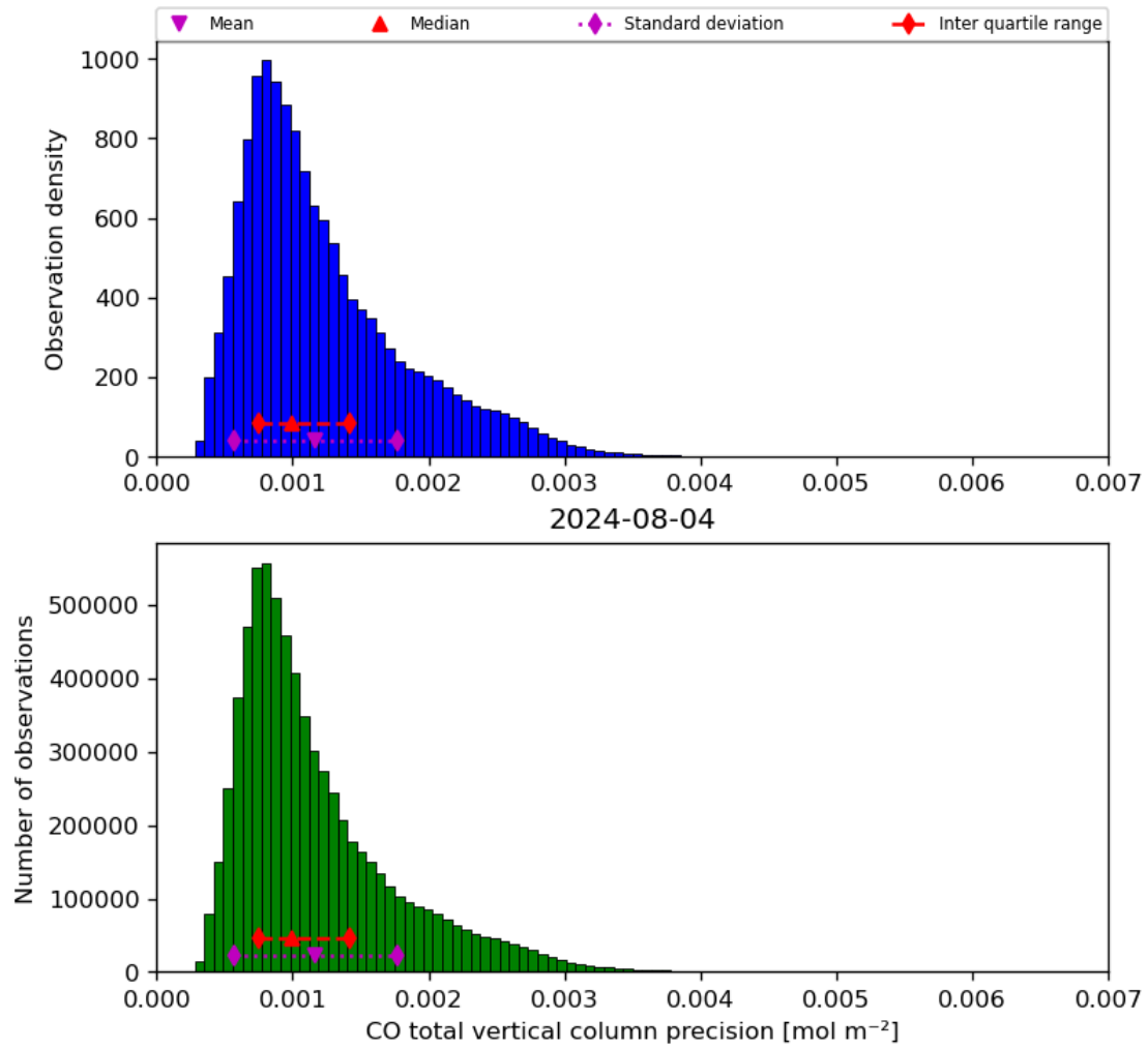
Figure 20: Histogram of “CO total vertical column precision” for 2024-08-03 to 2024-08-05
