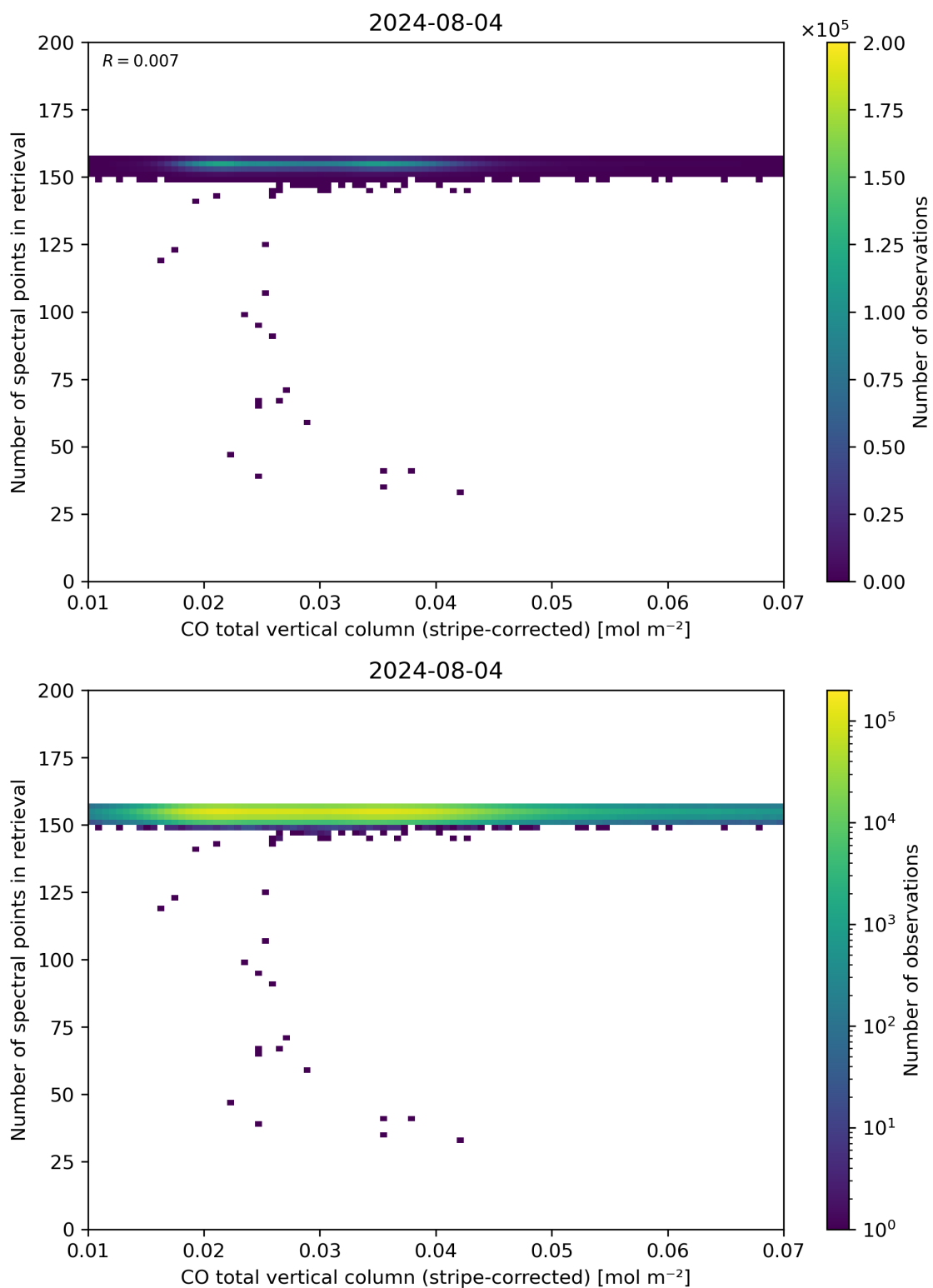
Figure 40: Scatter density plot of “CO total vertical column (stripe-corrected)” against “Number of spectral points in retrieval” for 2024-08-03 to 2024-08-05.
