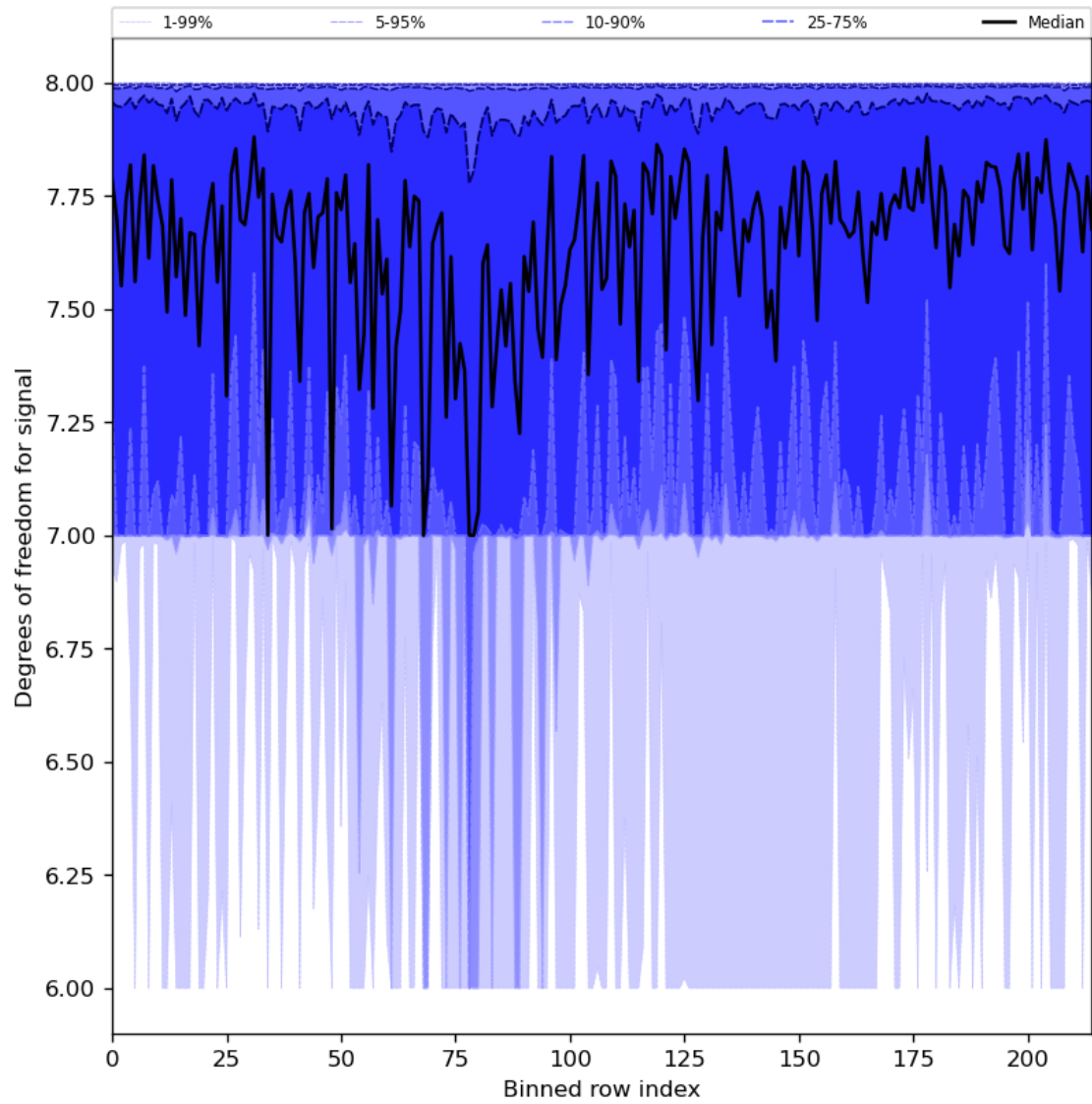
Figure 31: Along track statistics of “Degrees of freedom for signal” for 2024-08-03 to 2024-08-05
