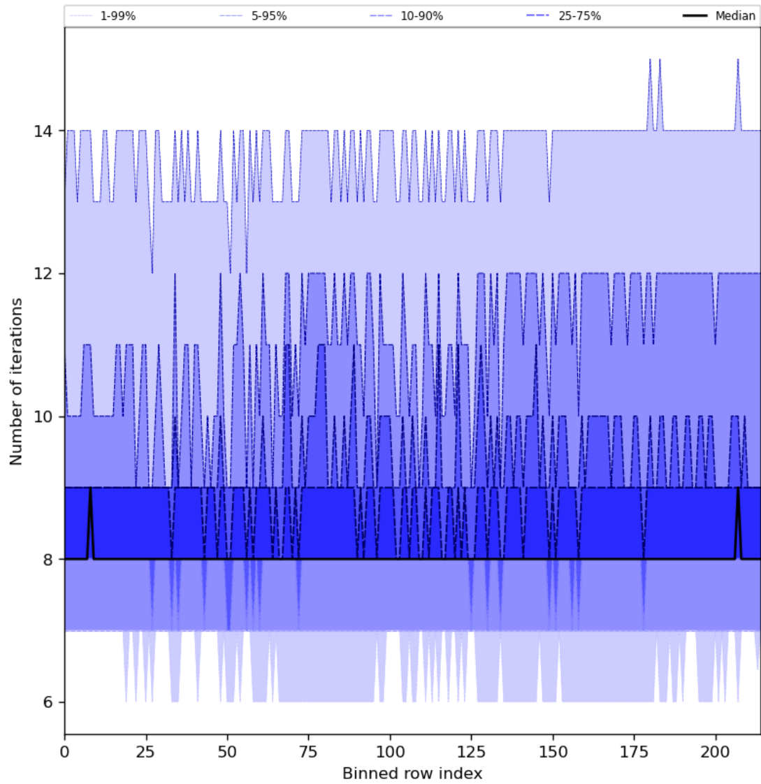
Figure 32: Along track statistics of “Number of iterations” for 2024-08-03 to 2024-08-05
