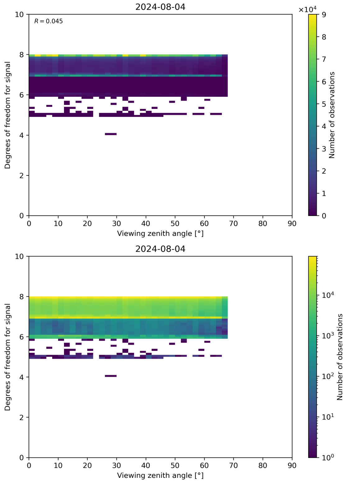
Figure 73: Scatter density plot of “Viewing zenith angle” against “Degrees of freedom for signal” for 2024-08-03 to 2024-08-05.
