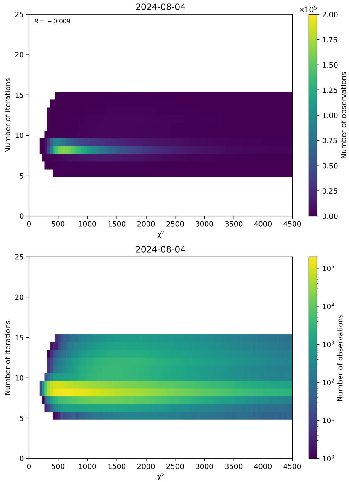
Figure 49: Scatter density plot of “ \chi^2 ” against “Number of iterations” for 2024-08-03 to 2024-08-05.
