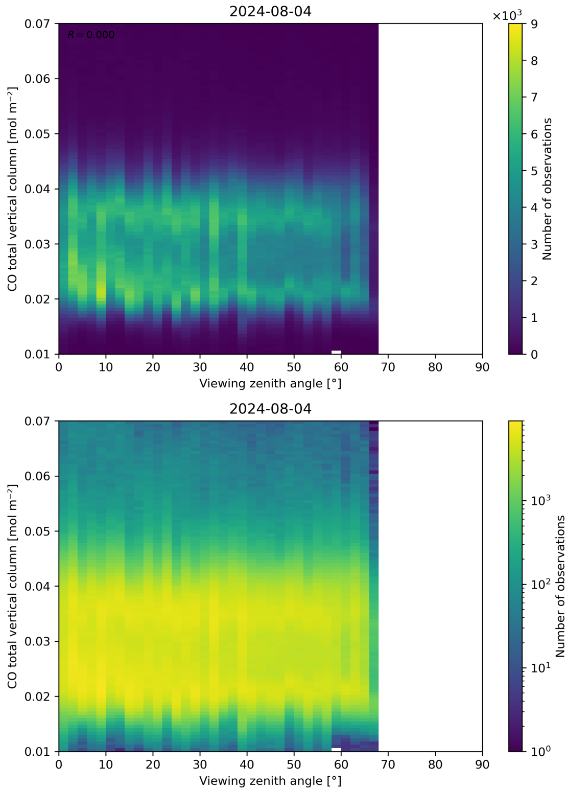
Figure 69: Scatter density plot of “Viewing zenith angle” against “CO total vertical column” for 2024-08-03 to 2024-08-05.
