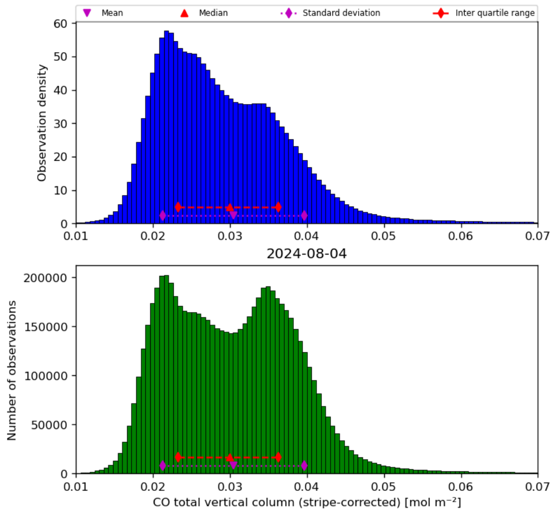
Figure 19: Histogram of “CO total vertical column (stripe-corrected)” for 2024-08-03 to 2024-08-05
