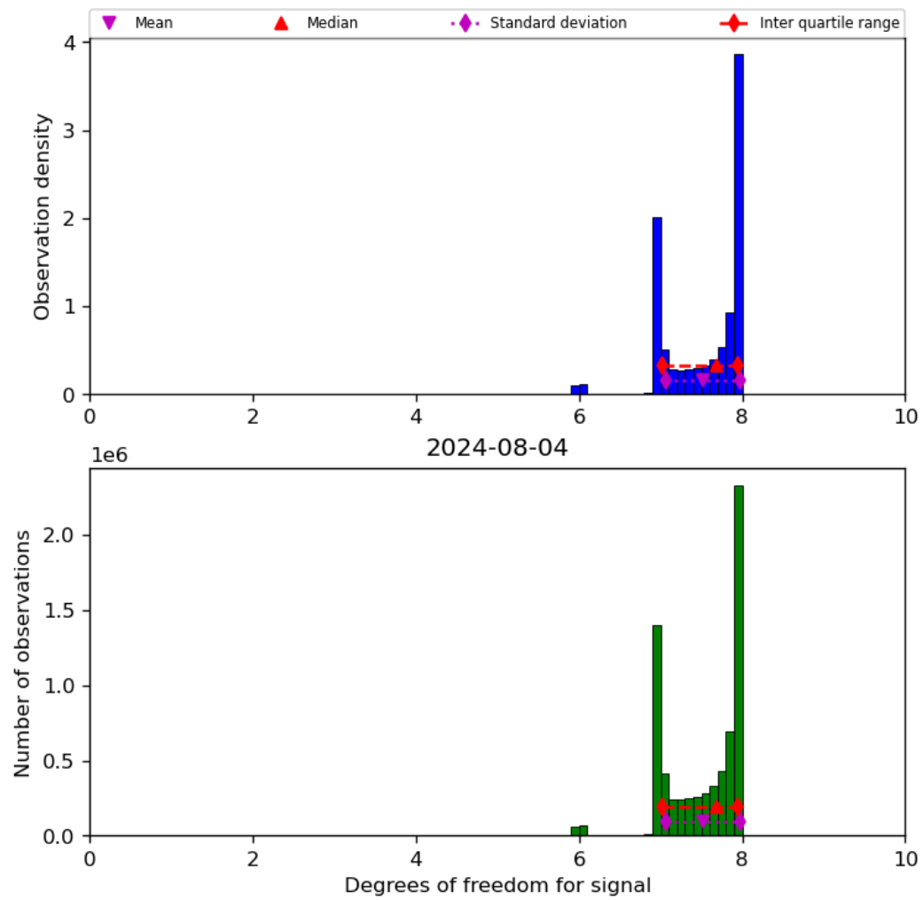
Figure 23: Histogram of “Degrees of freedom for signal” for 2024-08-03 to 2024-08-05
