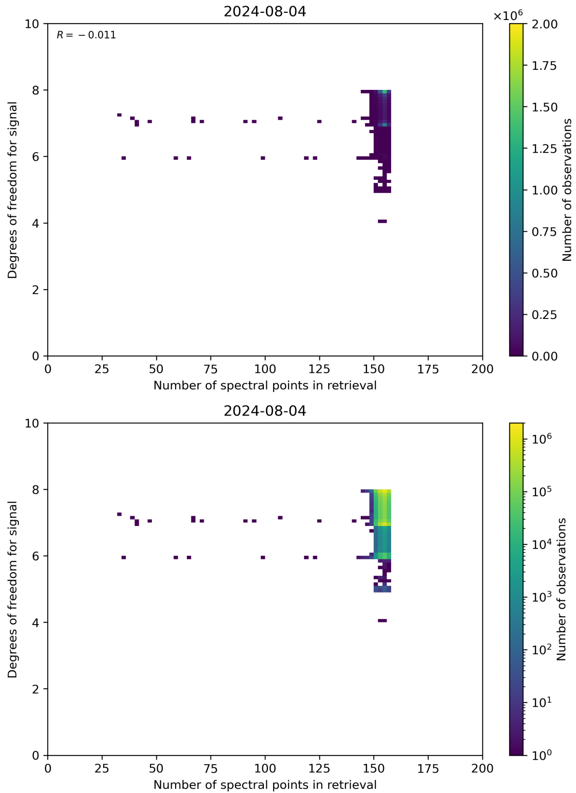
Figure 59: Scatter density plot of “Number of spectral points in retrieval” against “Degrees of freedom for signal” for 2024-08-03 to 2024-08-05.
