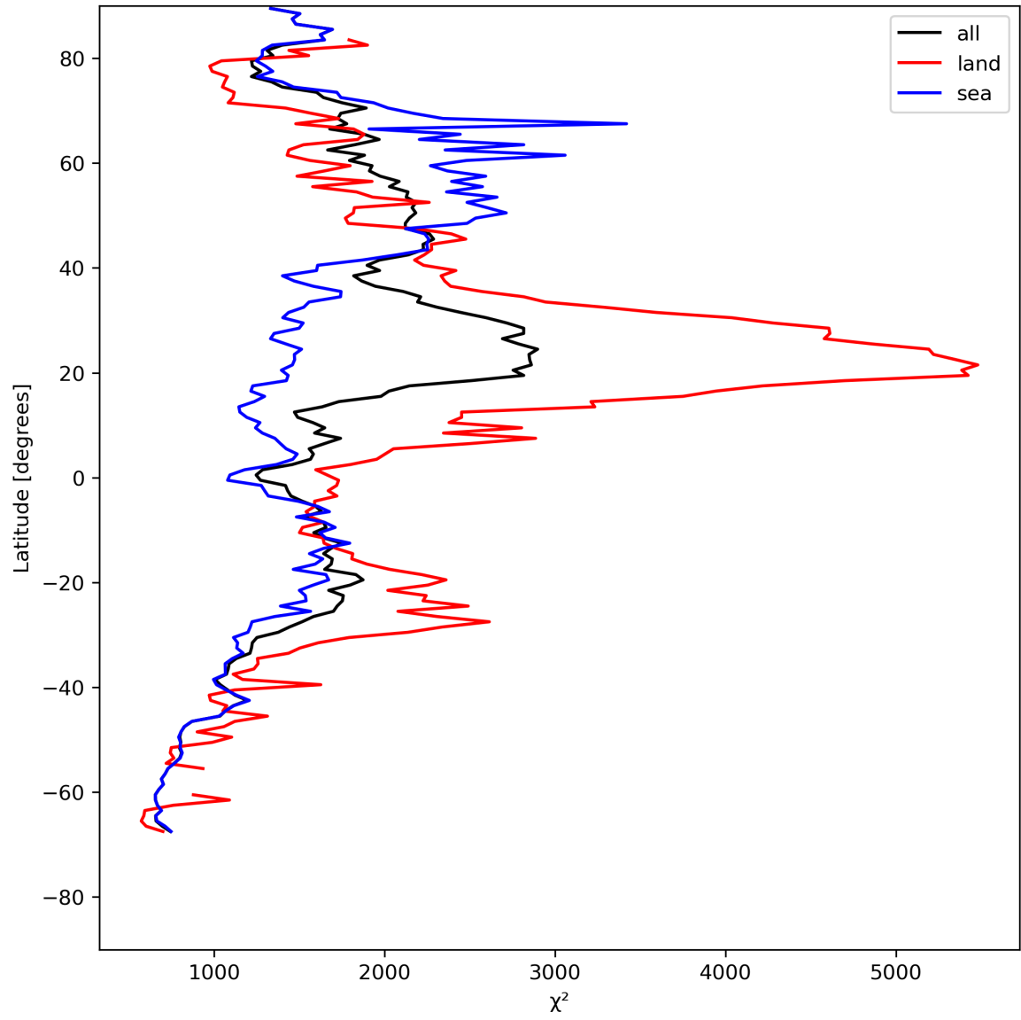
Figure 14: Zonal average of “ \chi^2 ” for 2024-08-03 to 2024-08-05.
