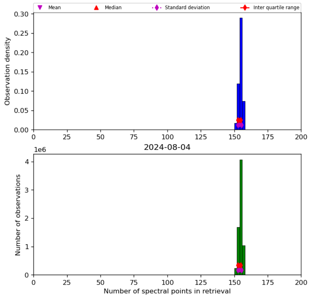
Figure 21: Histogram of “Number of spectral points in retrieval” for 2024-08-03 to 2024-08-05
