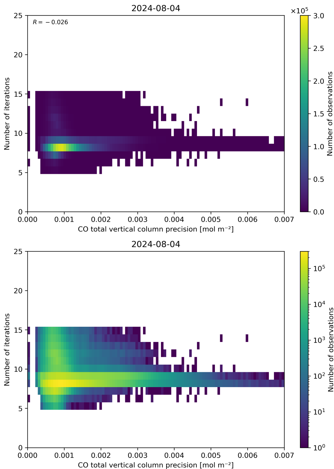
Figure 46: Scatter density plot of “CO total vertical column precision” against “Number of iterations” for 2024-08-03 to 2024-08-05.
