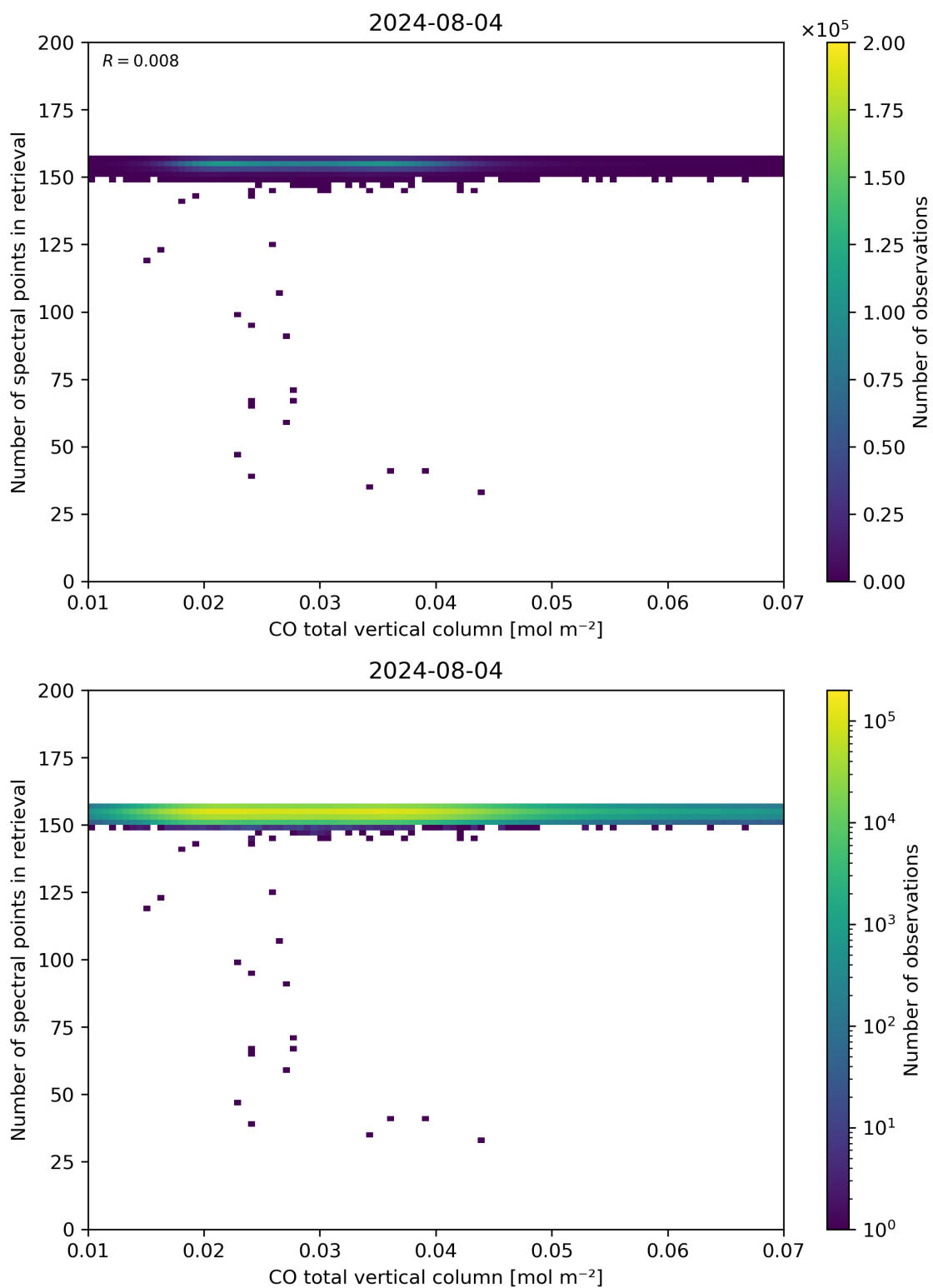
Figure 43: Scatter density plot of “CO total vertical column” against “Number of spectral points in retrieval” for 2024-08-03 to 2024-08-05.
