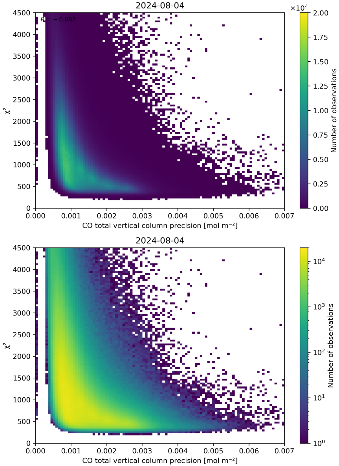
Figure 44: Scatter density plot of “CO total vertical column precision” against “ \chi^2 ” for 2024-08-03 to 2024-08-05.
