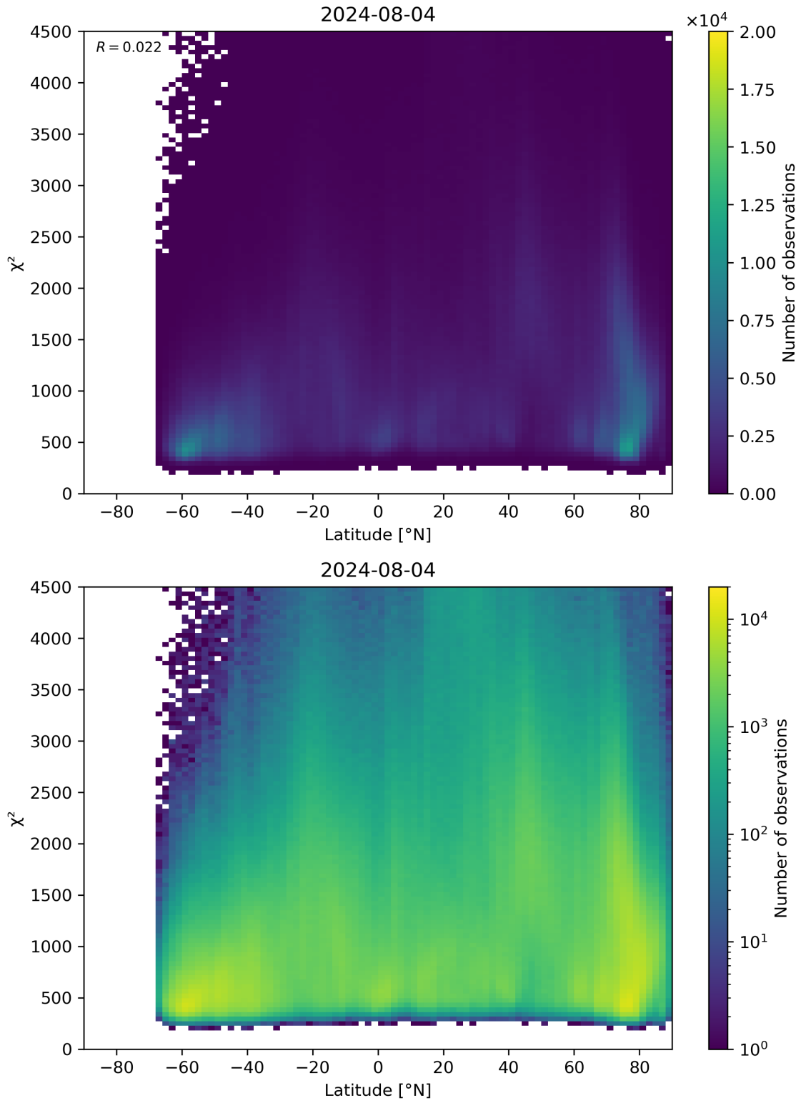
Figure 54: Scatter density plot of “Latitude” against “ \chi^2 ” for 2024-08-03 to 2024-08-05.
