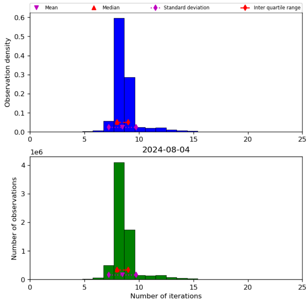
Figure 24: Histogram of “Number of iterations” for 2024-08-03 to 2024-08-05
