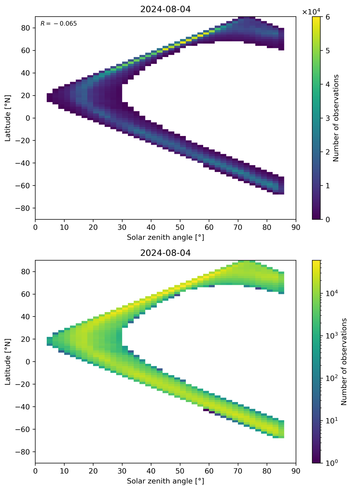
Figure 66: Scatter density plot of “Solar zenith angle” against “Latitude” for 2024-08-03 to 2024-08-05.
