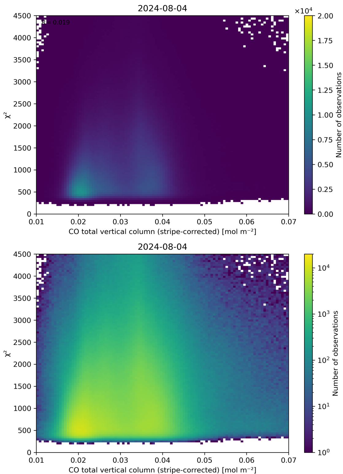
Figure 37: Scatter density plot of “CO total vertical column (stripe-corrected)” against “ \chi^2 ” for 2024-08-03 to 2024-08-05.
