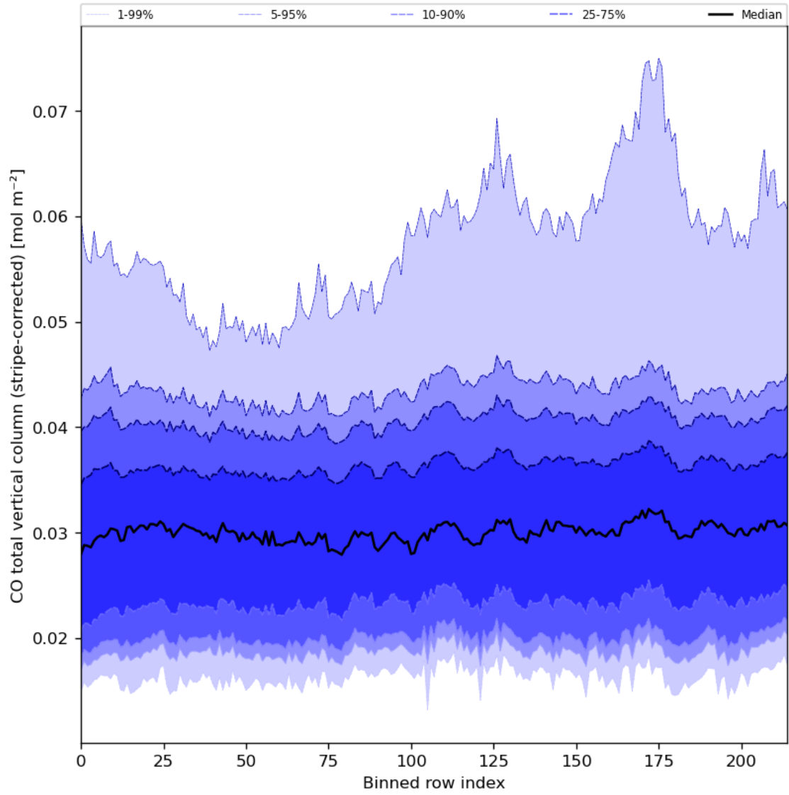
Figure 27: Along track statistics of “CO total vertical column (stripe-corrected)” for 2024-08-03 to 2024-08-05
