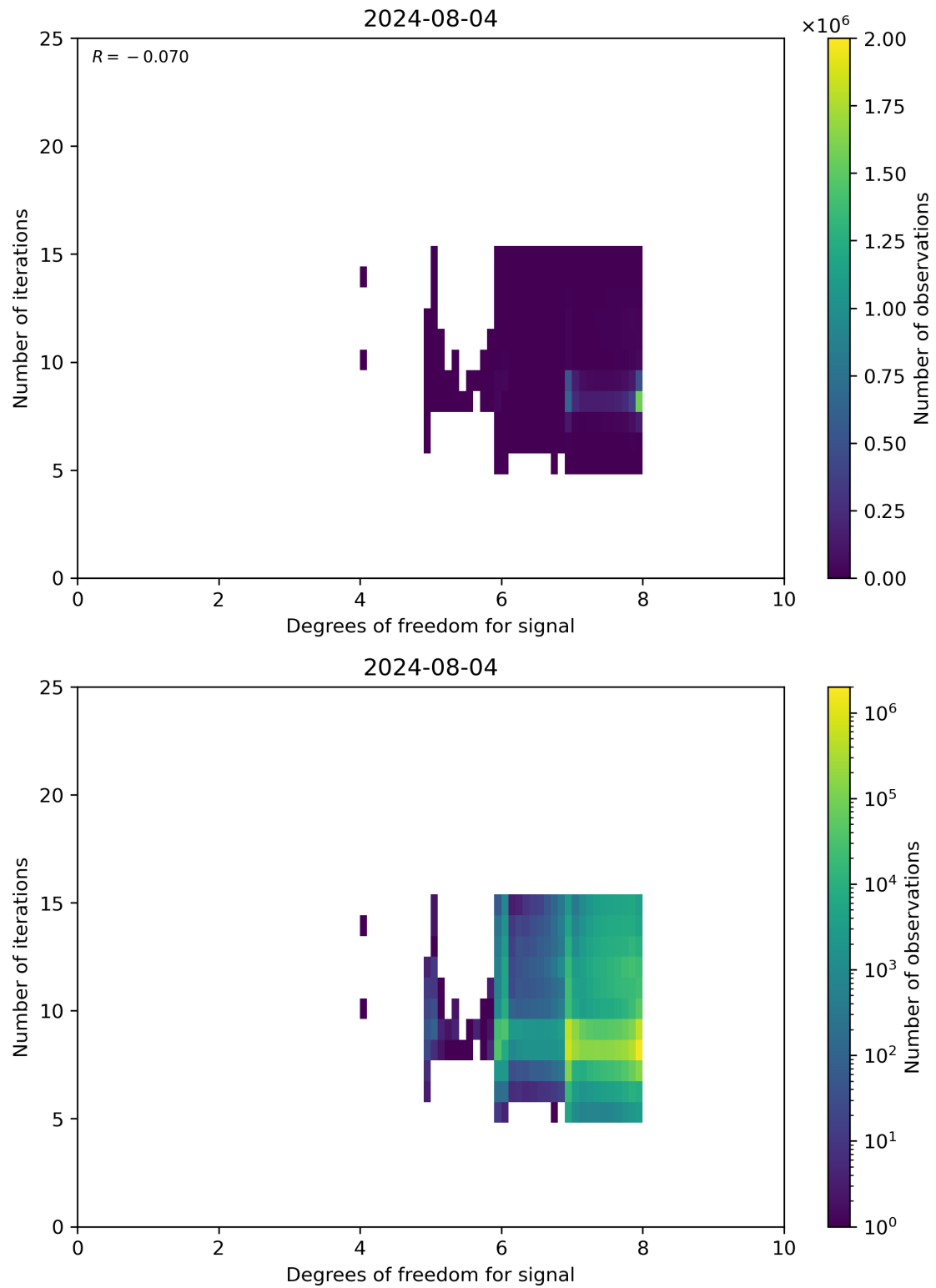
Figure 50: Scatter density plot of “Degrees of freedom for signal” against “Number of iterations” for 2024-08-03 to 2024-08-05.
