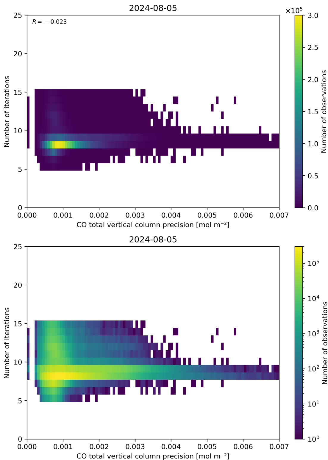
Figure 46: Scatter density plot of “CO total vertical column precision” against “Number of iterations” for 2024-08-04 to 2024-08-06.
