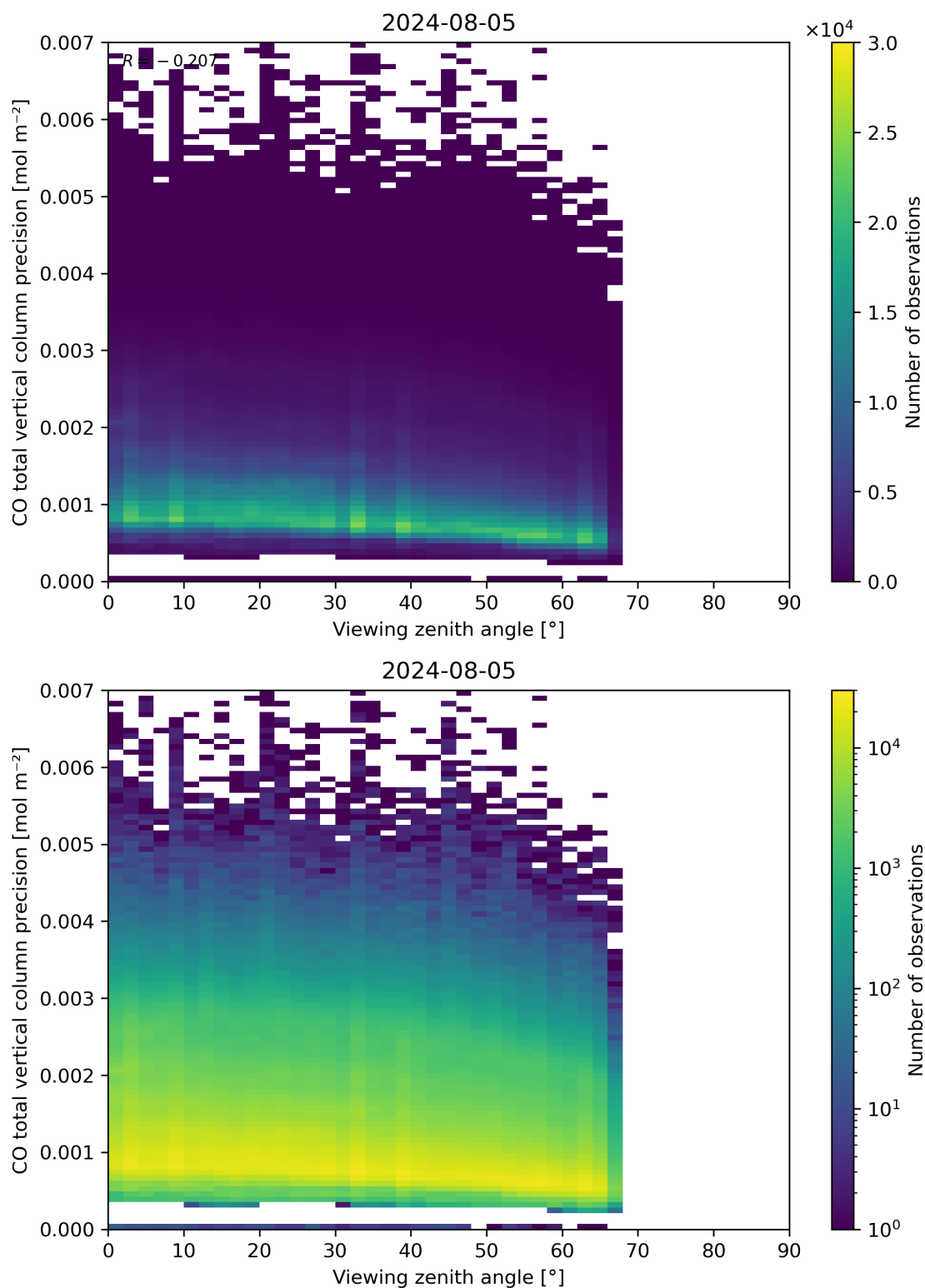
Figure 71: Scatter density plot of “Viewing zenith angle” against “CO total vertical column precision” for 2024-08-04 to 2024-08-06.
