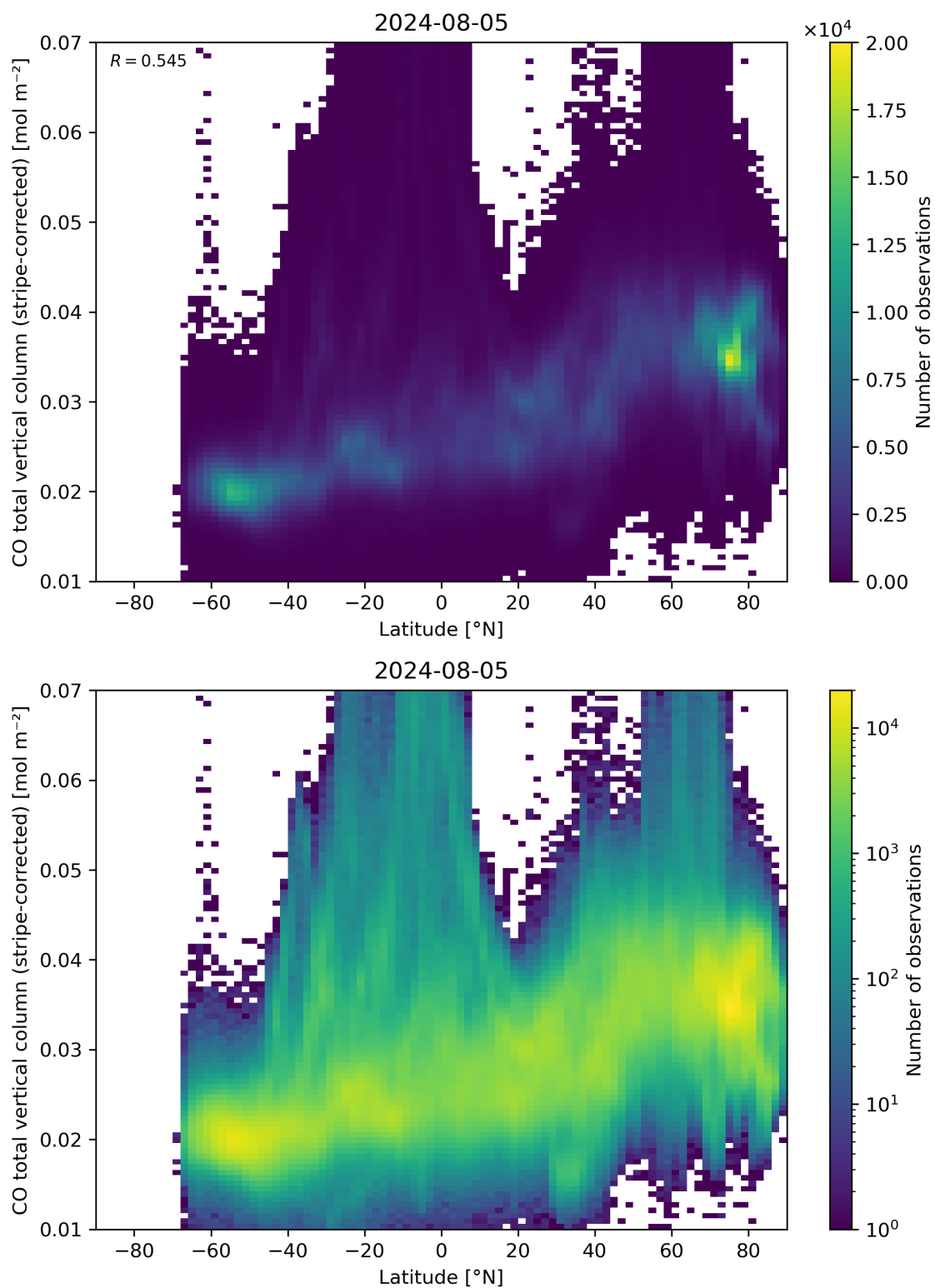
Figure 52: Scatter density plot of “Latitude” against “CO total vertical column (stripe-corrected)” for 2024-08-04 to 2024-08-06.
