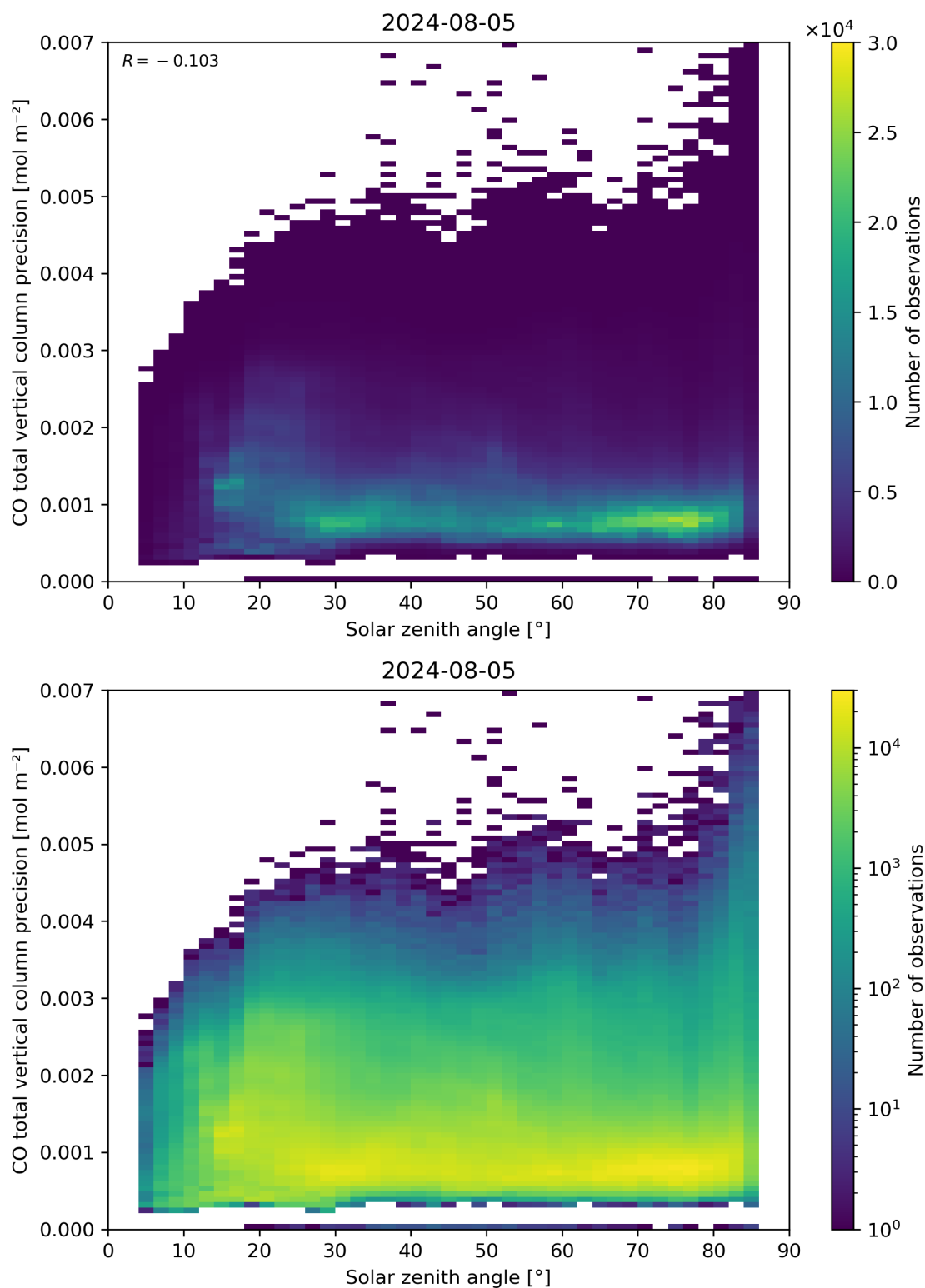
Figure 63: Scatter density plot of “Solar zenith angle” against “CO total vertical column precision” for 2024-08-04 to 2024-08-06.
