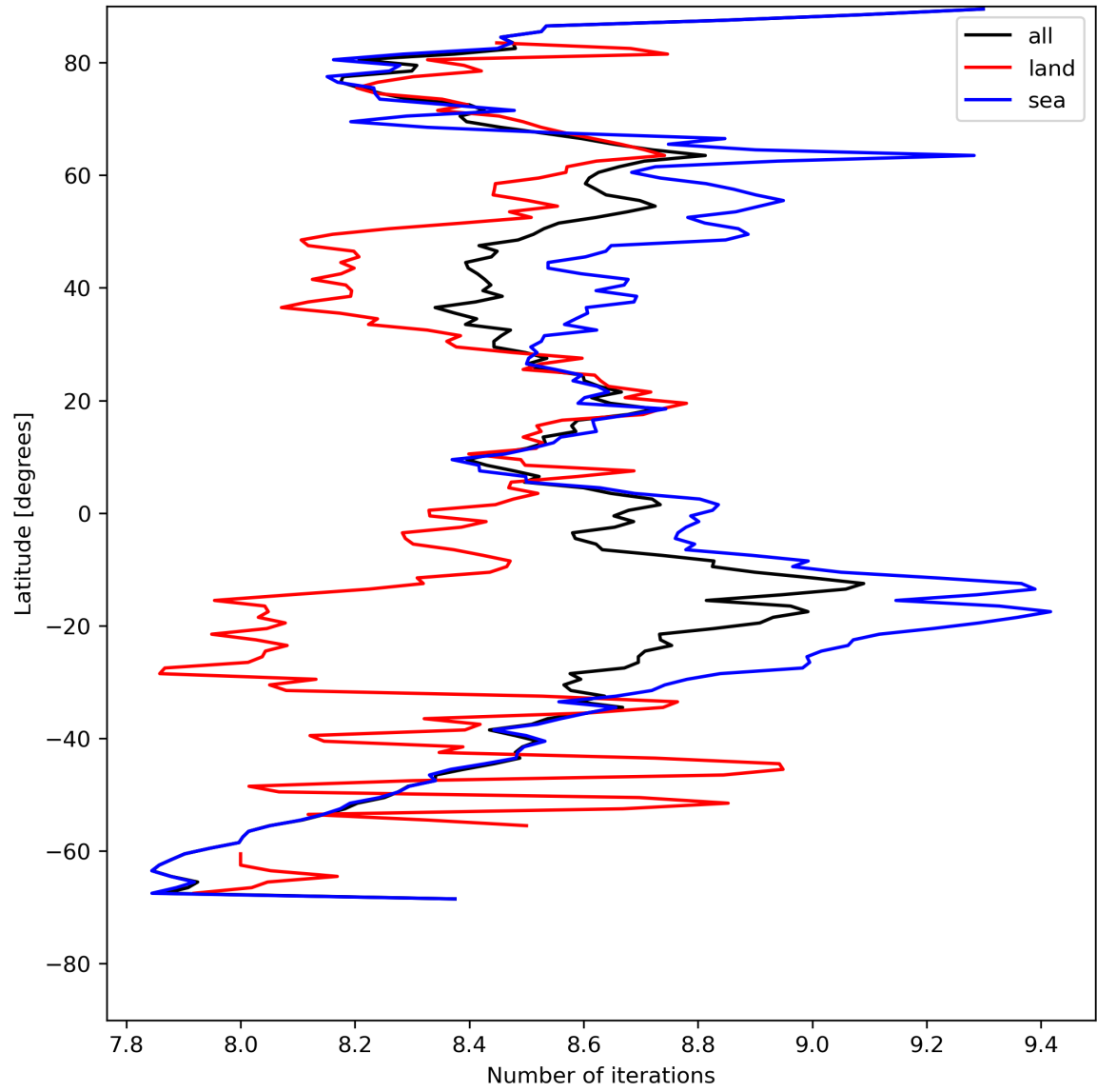
Figure 16: Zonal average of “Number of iterations” for 2024-08-04 to 2024-08-06.
