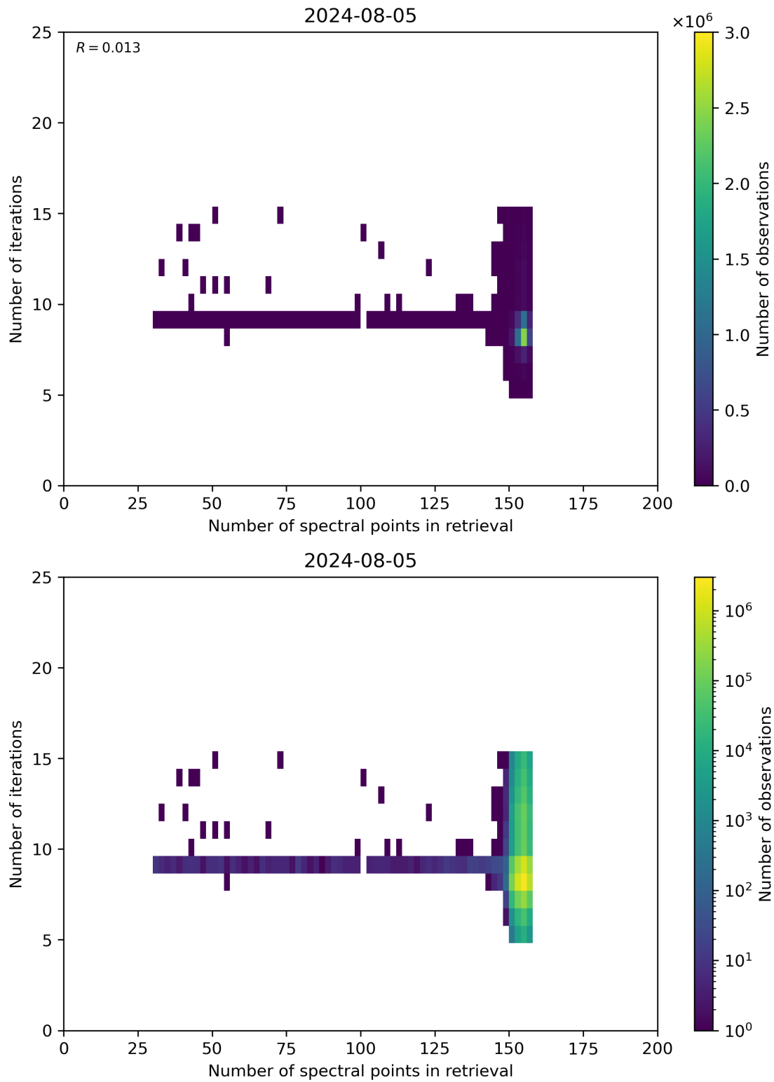
Figure 60: Scatter density plot of “Number of spectral points in retrieval” against “Number of iterations” for 2024-08-04 to 2024-08-06.
