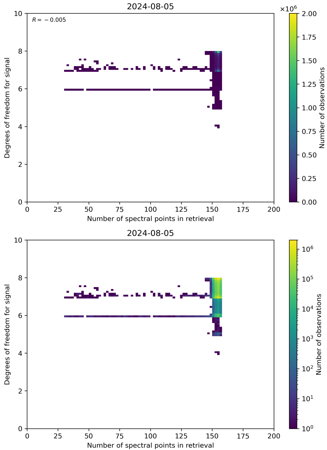
Figure 59: Scatter density plot of “Number of spectral points in retrieval” against “Degrees of freedom for signal” for 2024-08-04 to 2024-08-06.
