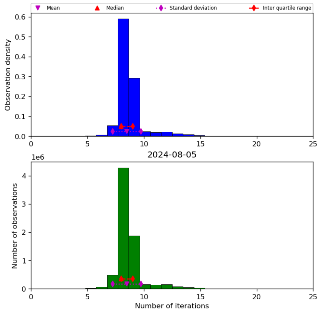
Figure 24: Histogram of “Number of iterations” for 2024-08-04 to 2024-08-06
