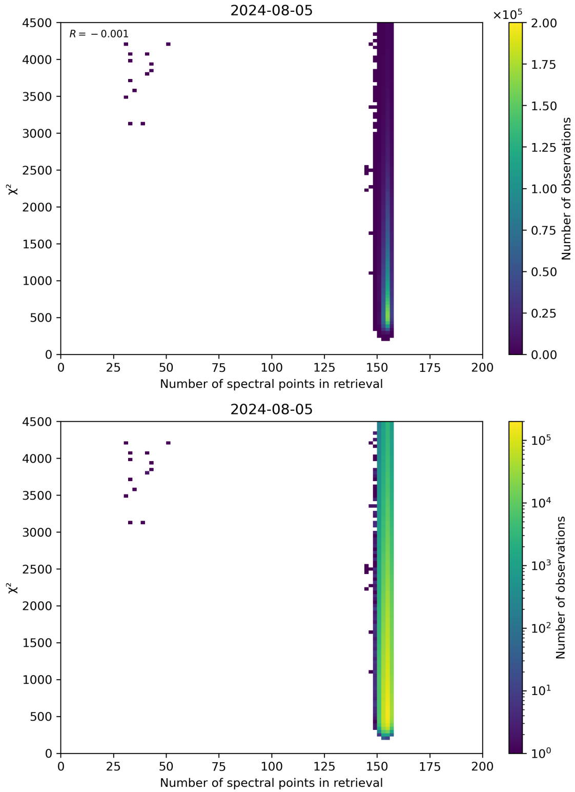
Figure 58: Scatter density plot of “Number of spectral points in retrieval” against “ \chi^2 ” for 2024-08-04 to 2024-08-06.
