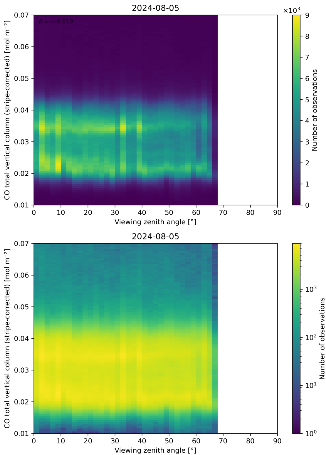
Figure 70: Scatter density plot of “Viewing zenith angle” against “CO total vertical column (stripe-corrected)” for 2024-08-04 to 2024-08-06.
