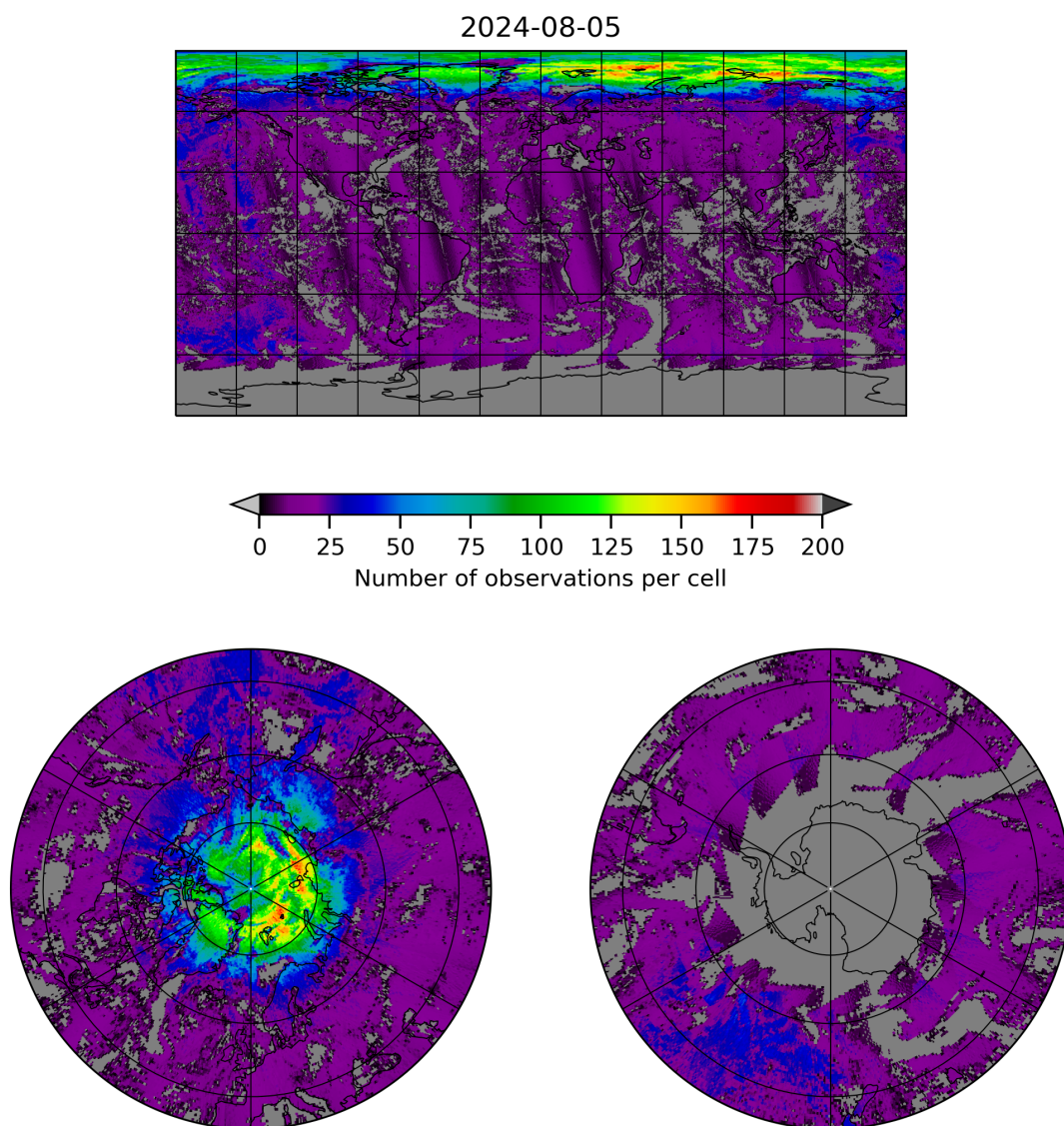
Figure 8: Map of the number of observations for 2024-08-04 to 2024-08-06
