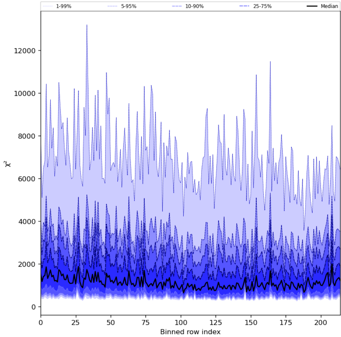
Figure 30: Along track statistics of “ \chi^2 ” for 2024-08-04 to 2024-08-06
