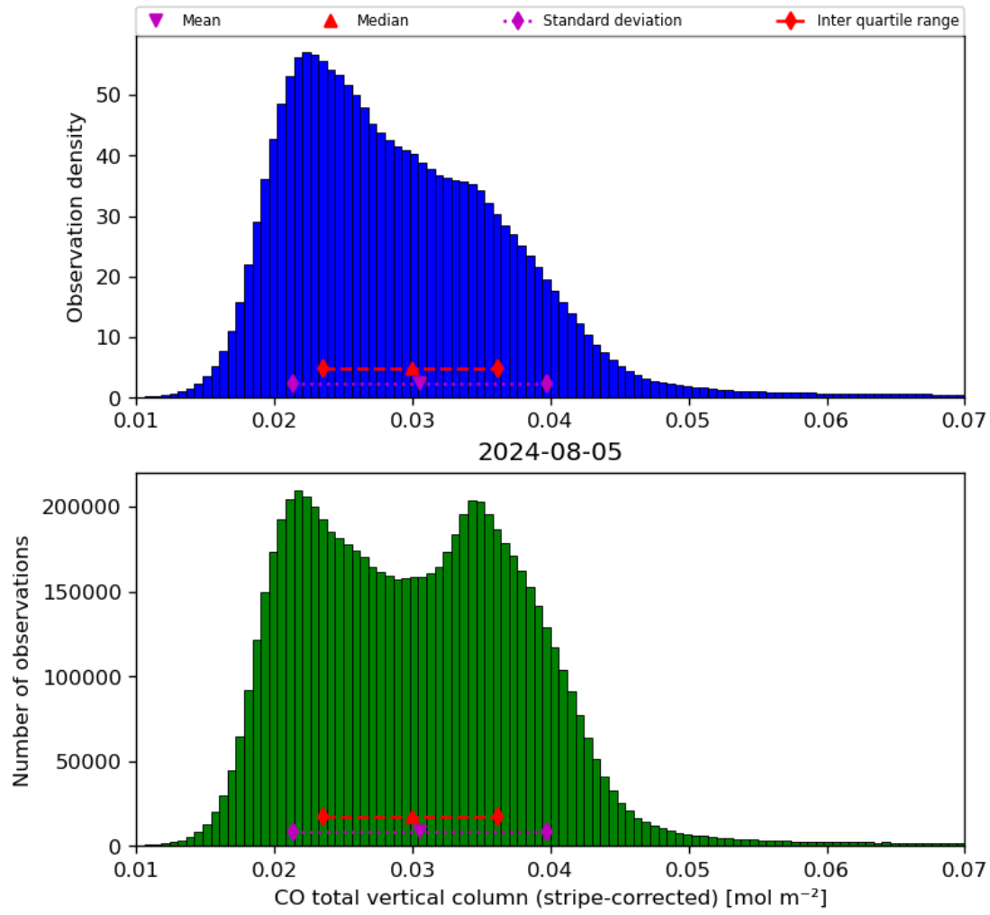
Figure 19: Histogram of “CO total vertical column (stripe-corrected)” for 2024-08-04 to 2024-08-06
