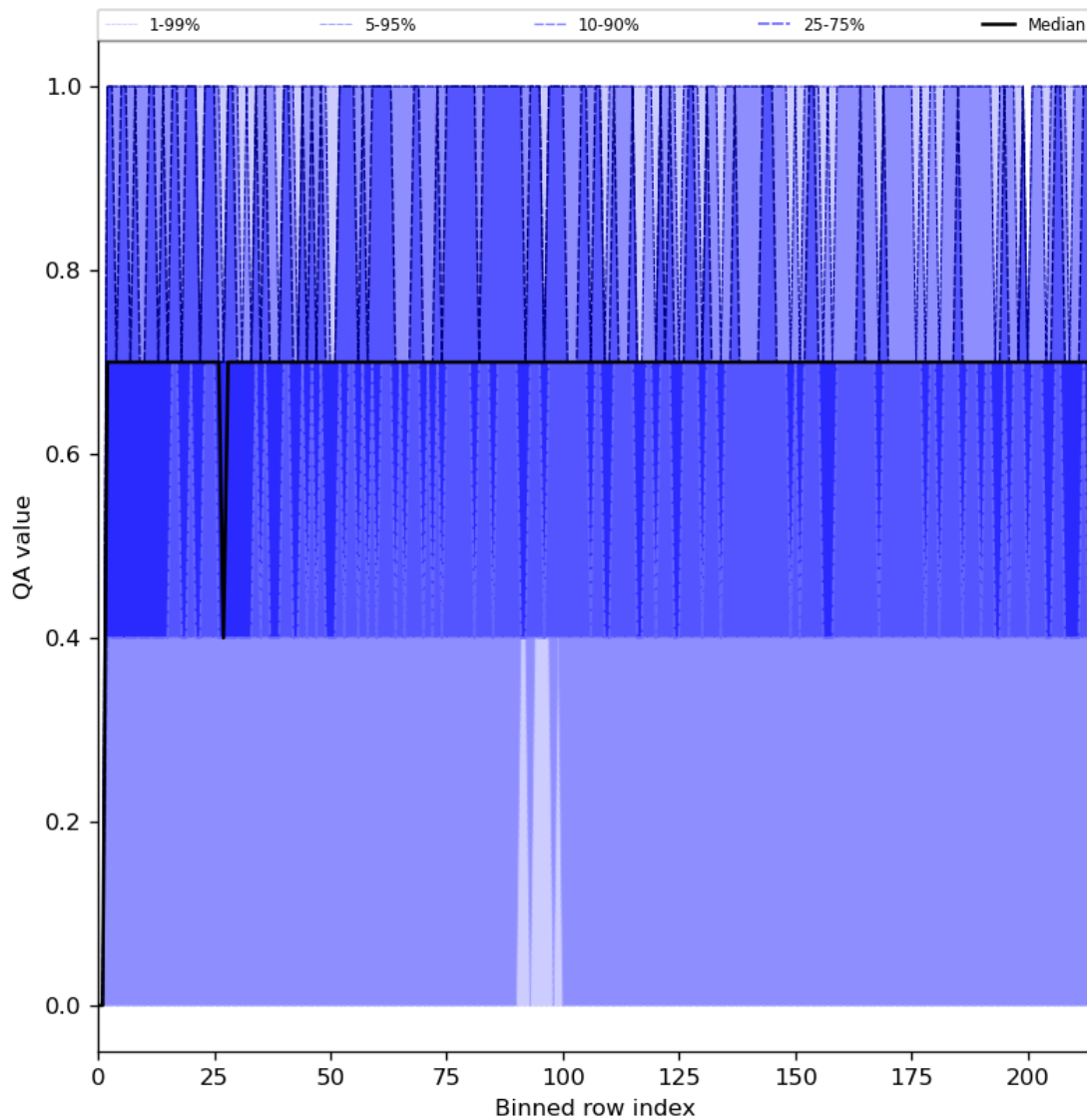
Figure 25: Along track statistics of “QA value” for 2024-08-04 to 2024-08-06
