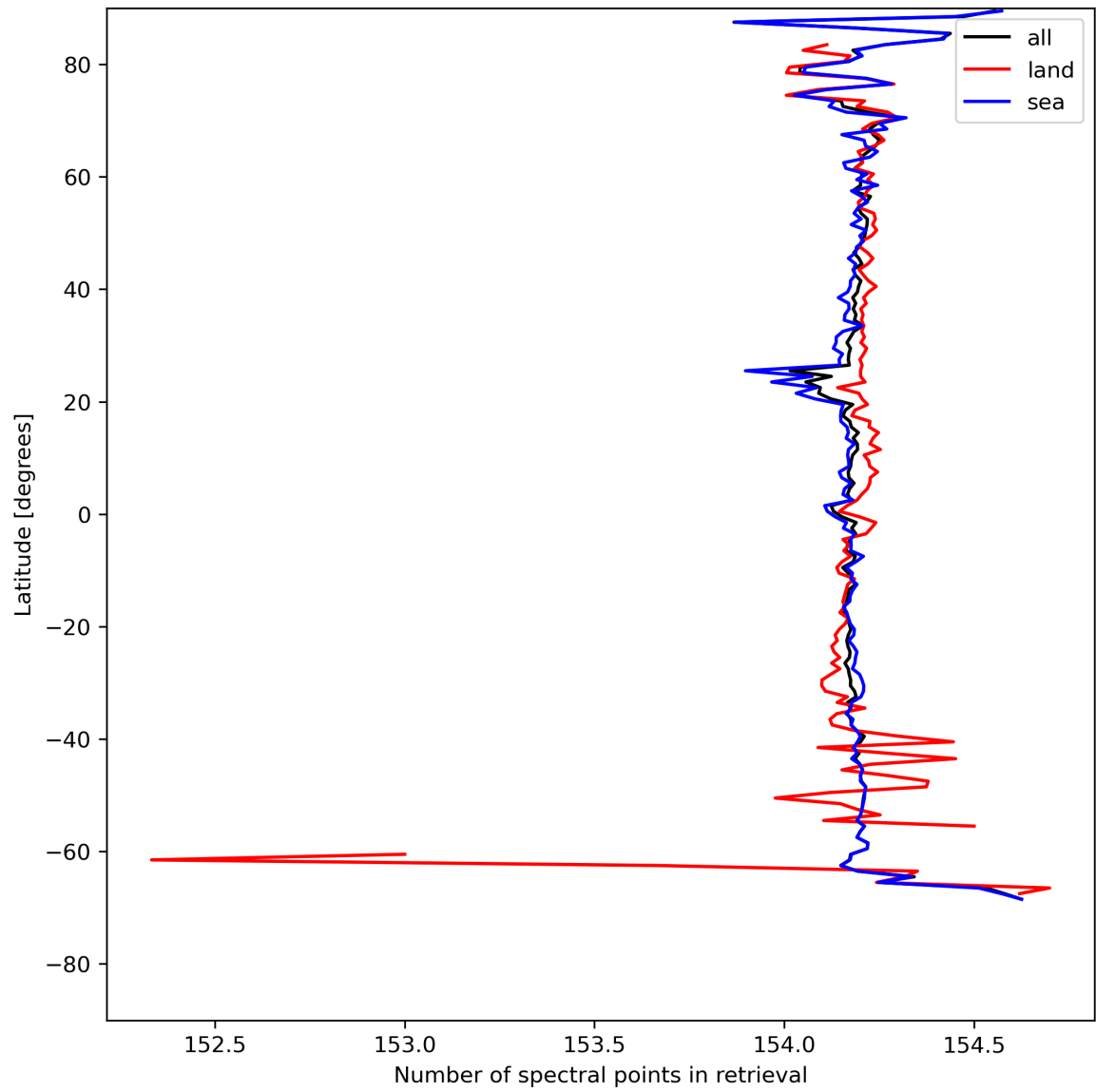
Figure 13: Zonal average of “Number of spectral points in retrieval” for 2024-08-04 to 2024-08-06.
