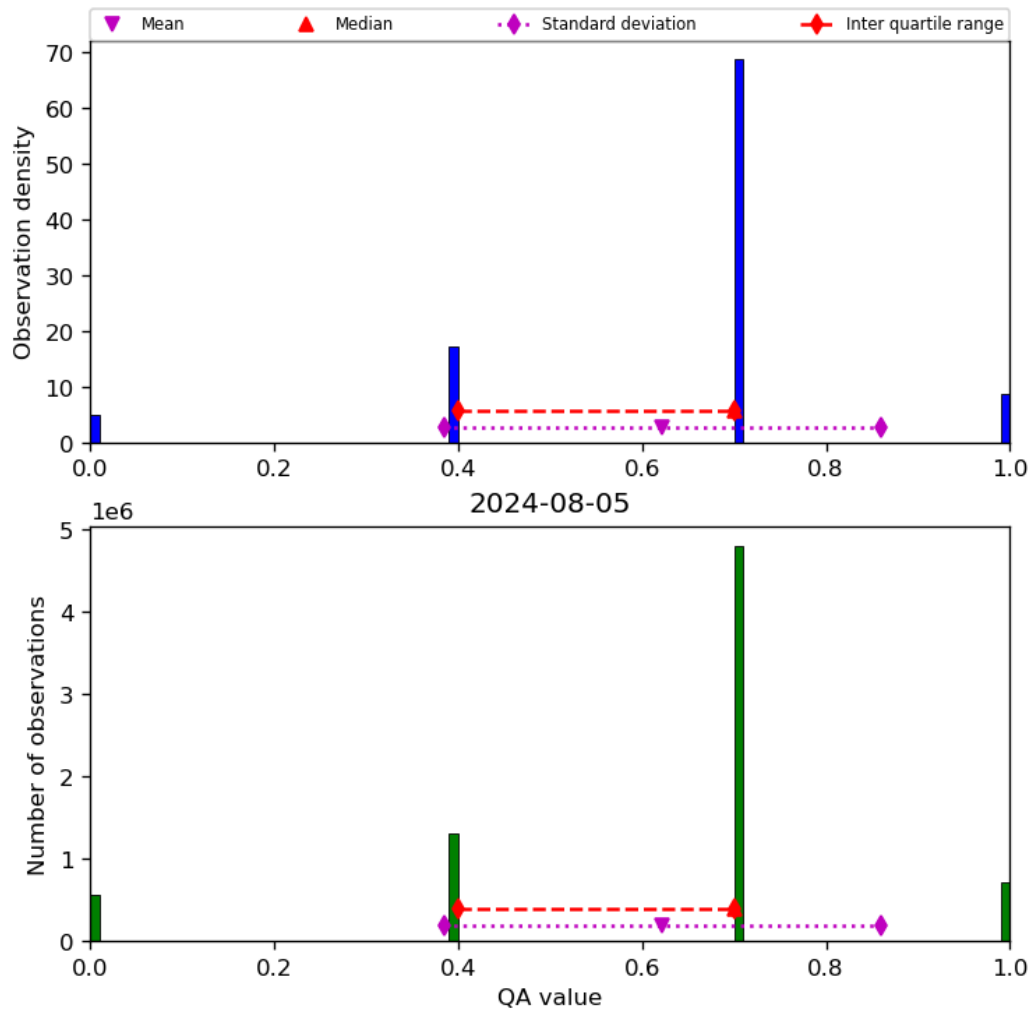
Figure 17: Histogram of “QA value” for 2024-08-04 to 2024-08-06
