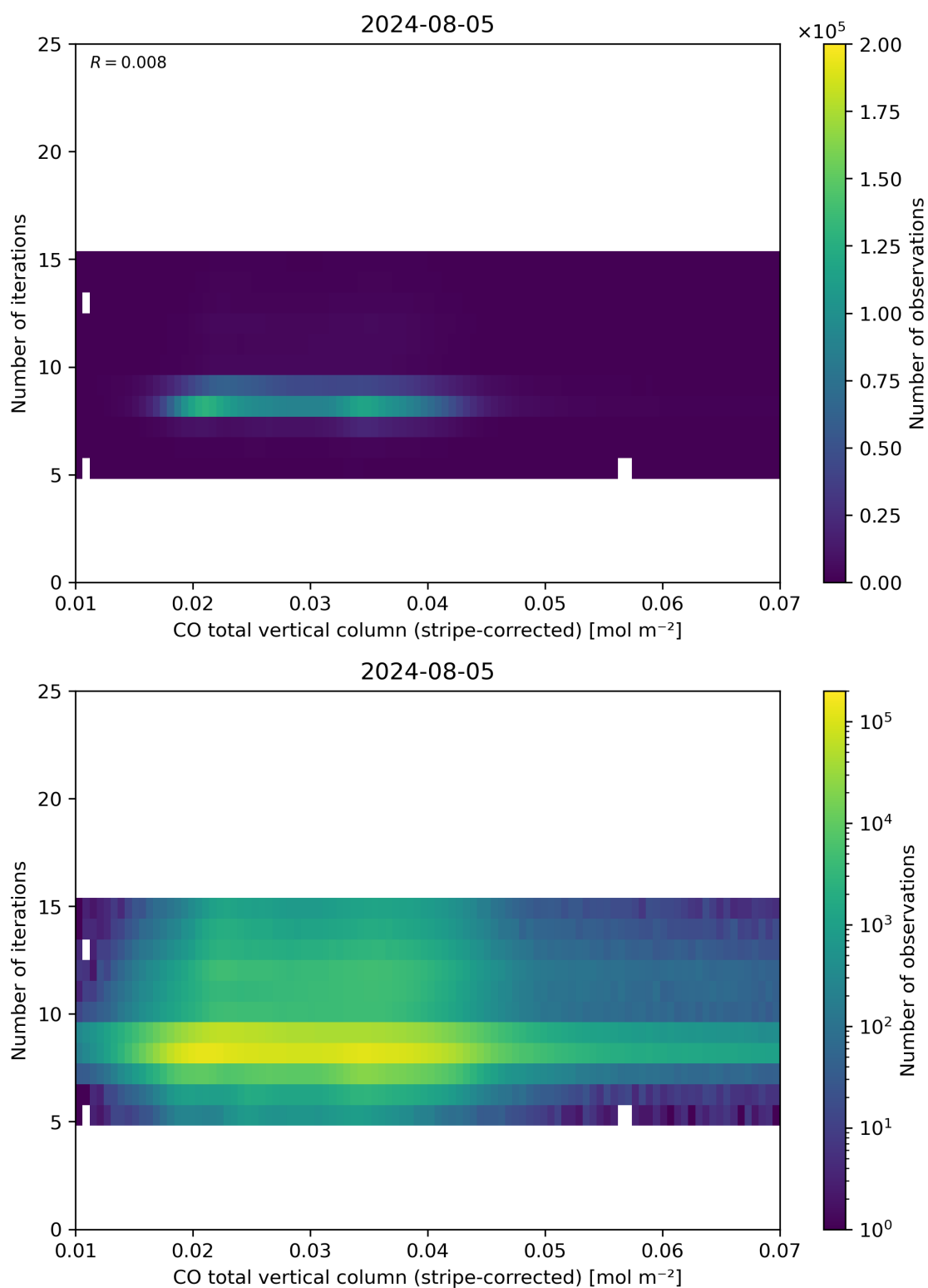
Figure 39: Scatter density plot of “CO total vertical column (stripe-corrected)” against “Number of iterations” for 2024-08-04 to 2024-08-06.
