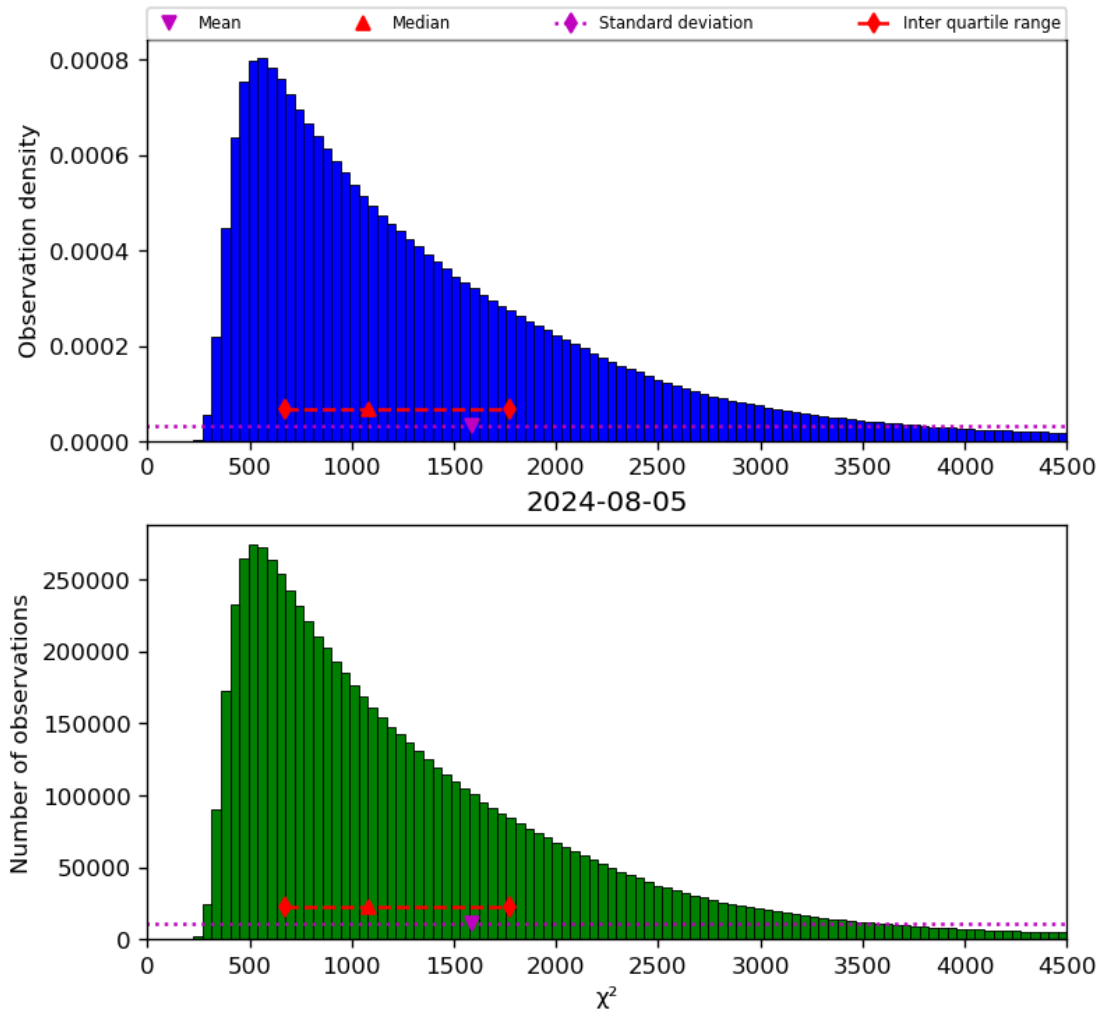
Figure 22: Histogram of “ \chi^2 ” for 2024-08-04 to 2024-08-06
