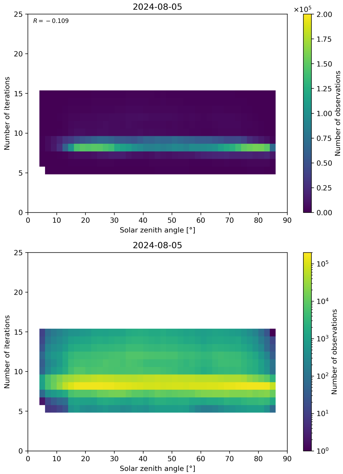
Figure 67: Scatter density plot of “Solar zenith angle” against “Number of iterations” for 2024-08-04 to 2024-08-06.
