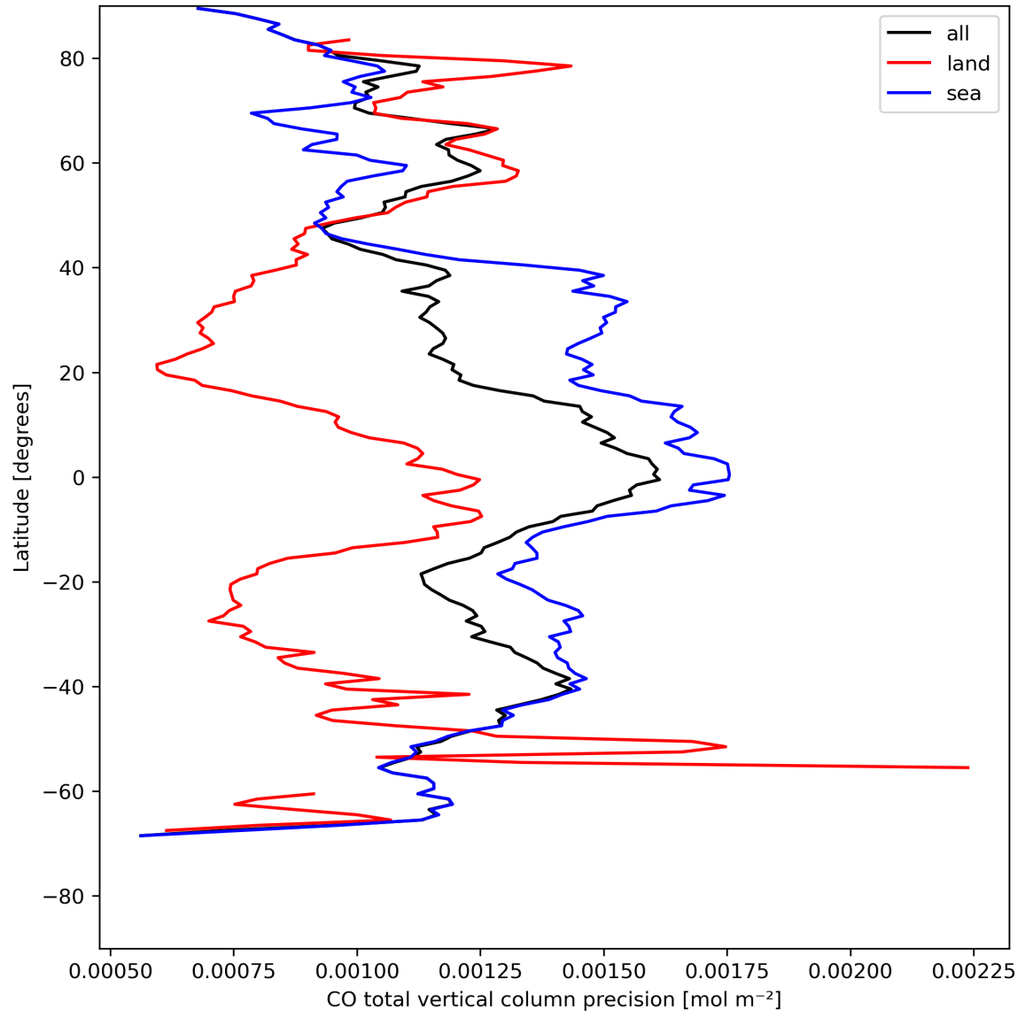
Figure 12: Zonal average of "CO total vertical column precision" for 2024-08-04 to 2024-08-06.
