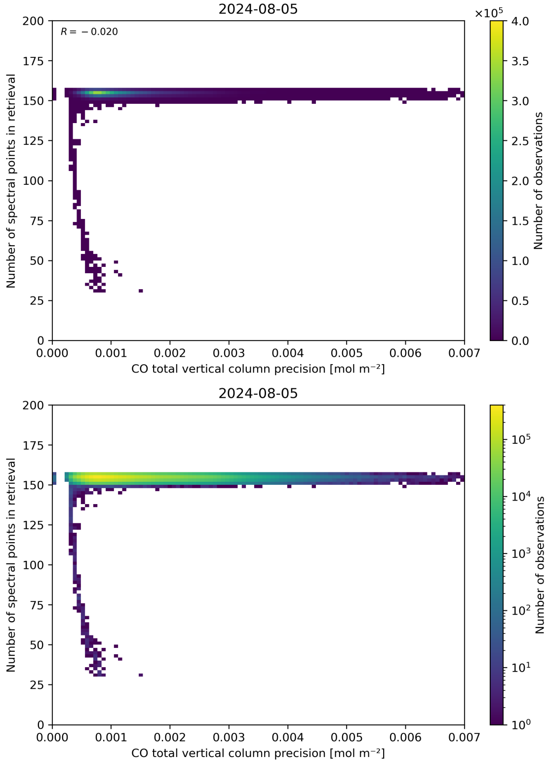
Figure 47: Scatter density plot of “CO total vertical column precision” against “Number of spectral points in retrieval” for 2024-08-04 to 2024-08-06.
