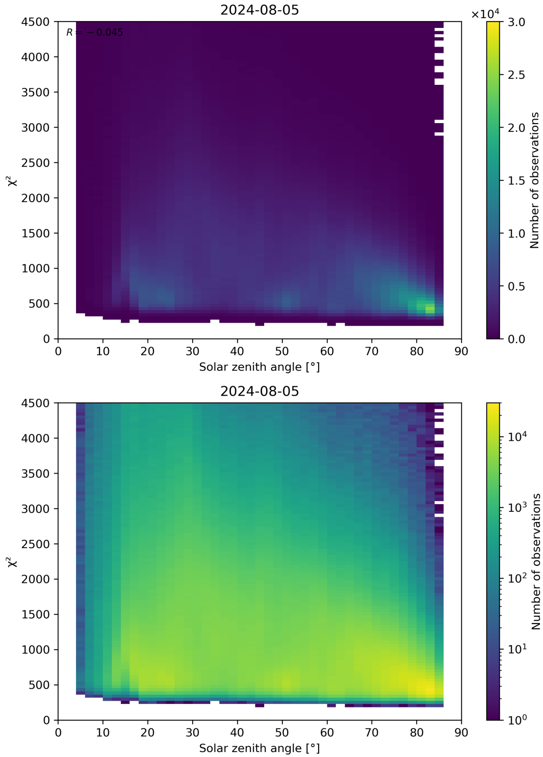
Figure 64: Scatter density plot of “Solar zenith angle” against “ \chi^2 ” for 2024-08-04 to 2024-08-06.
