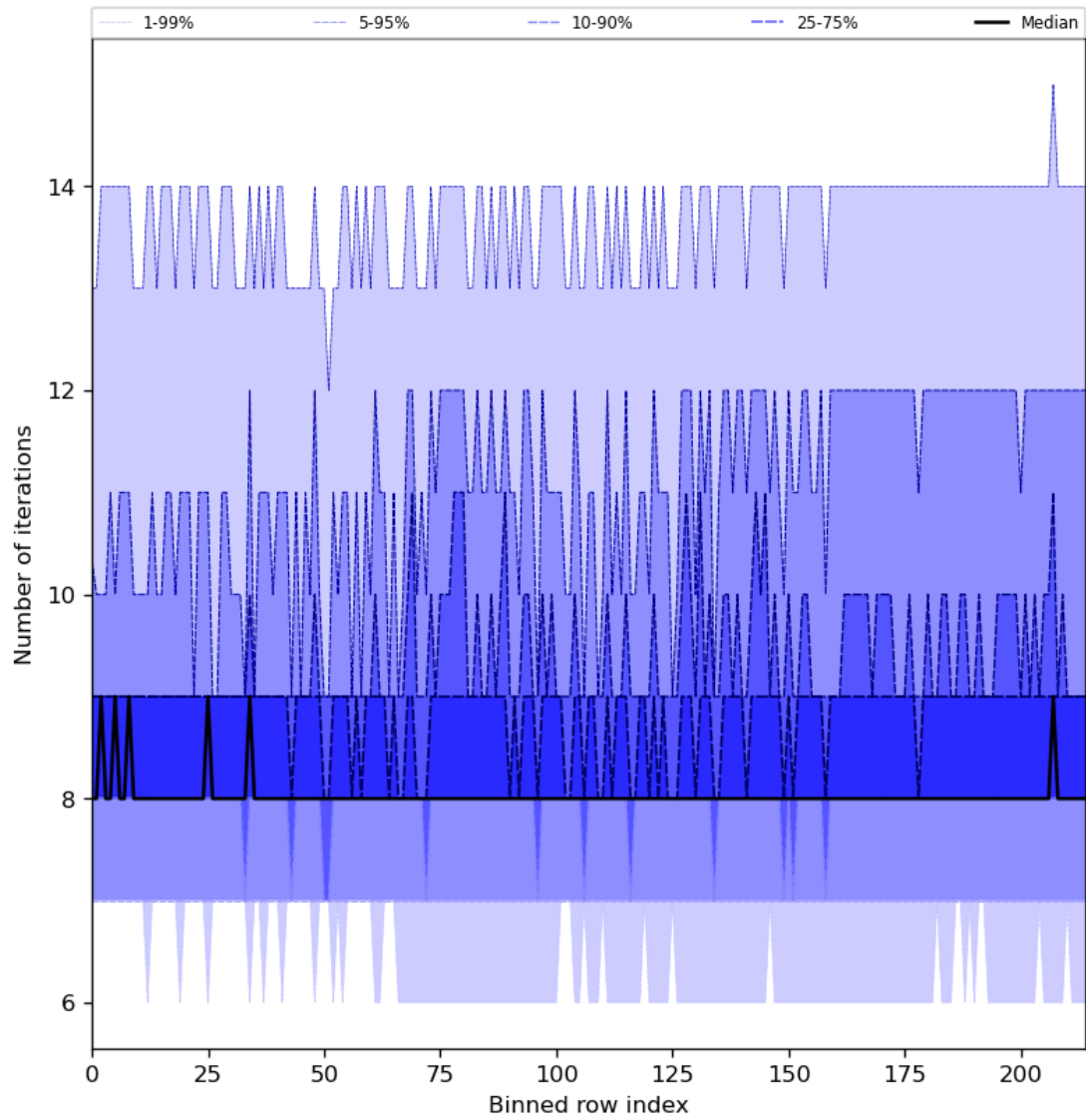
Figure 32: Along track statistics of “Number of iterations” for 2024-08-04 to 2024-08-06
