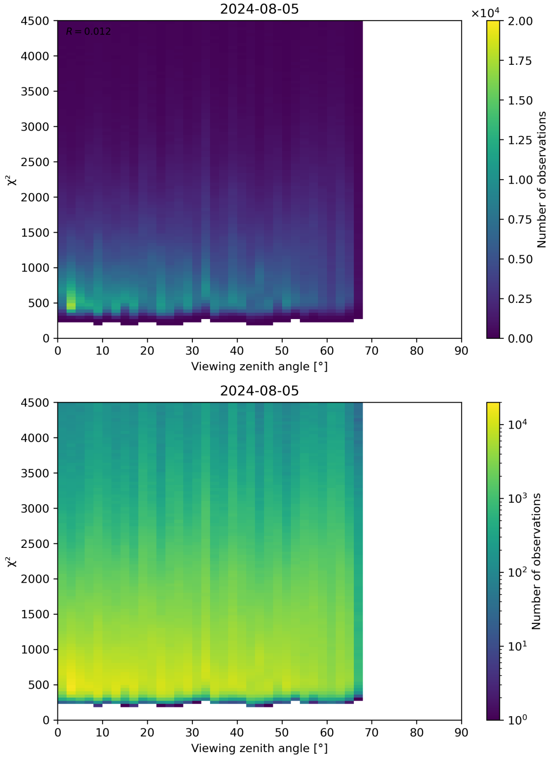
Figure 72: Scatter density plot of “Viewing zenith angle” against “ \chi^2 ” for 2024-08-04 to 2024-08-06.
