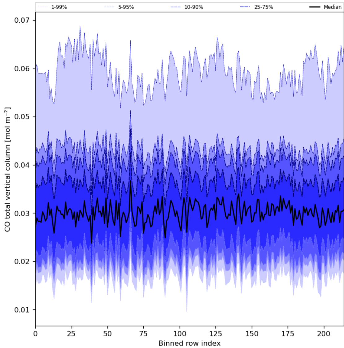
Figure 26: Along track statistics of “CO total vertical column” for 2024-08-04 to 2024-08-06
