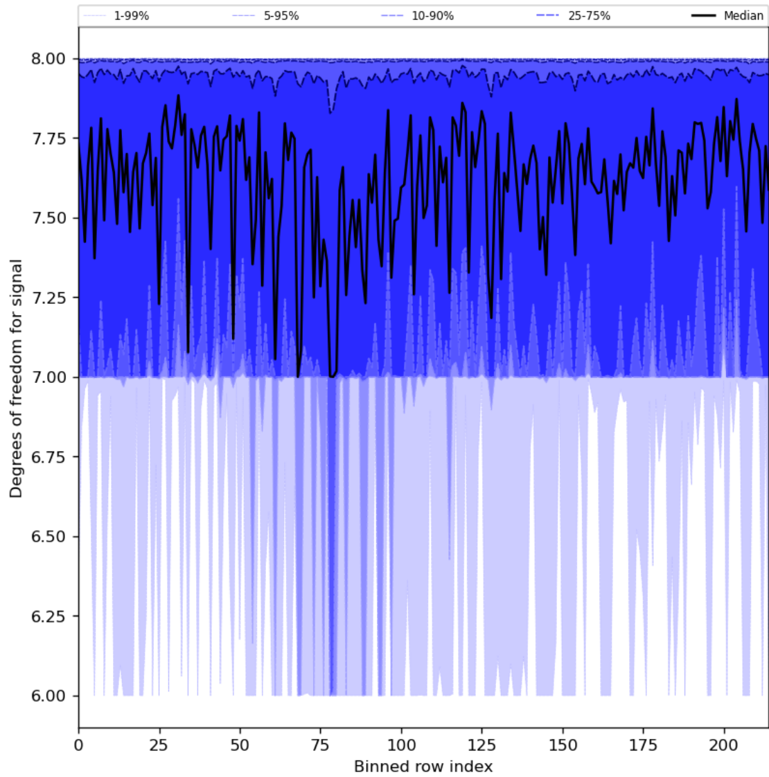
Figure 31: Along track statistics of “Degrees of freedom for signal” for 2024-08-04 to 2024-08-06
