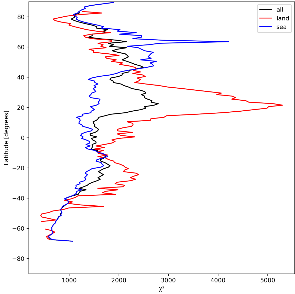
Figure 14: Zonal average of “ \chi^2 ” for 2024-08-04 to 2024-08-06.
