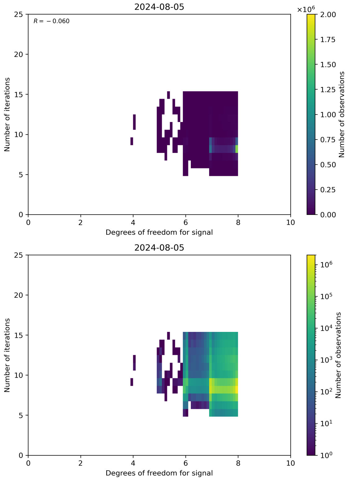
Figure 50: Scatter density plot of “Degrees of freedom for signal” against “Number of iterations” for 2024-08-04 to 2024-08-06.
