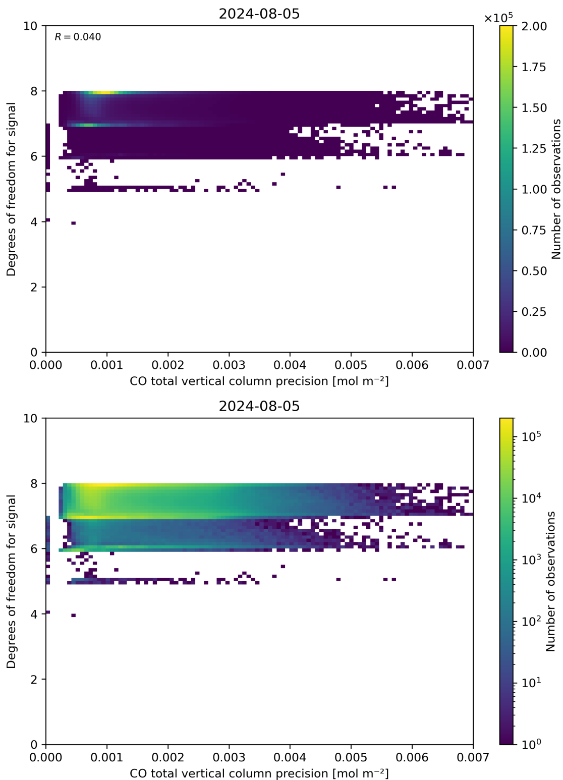
Figure 45: Scatter density plot of “CO total vertical column precision” against “Degrees of freedom for signal” for 2024-08-04 to 2024-08-06.
