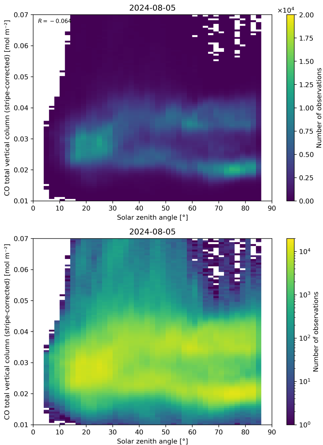
Figure 62: Scatter density plot of “Solar zenith angle” against “CO total vertical column (stripe-corrected)” for 2024-08-04 to 2024-08-06.
