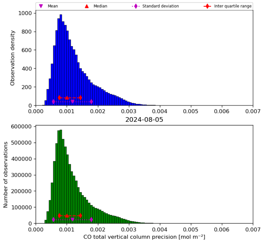
Figure 20: Histogram of “CO total vertical column precision” for 2024-08-04 to 2024-08-06
