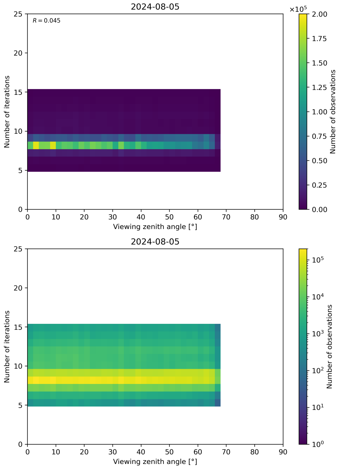
Figure 75: Scatter density plot of “Viewing zenith angle” against “Number of iterations” for 2024-08-04 to 2024-08-06.
