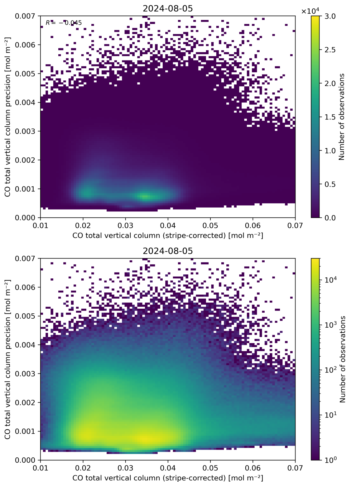
Figure 36: Scatter density plot of “CO total vertical column (stripe-corrected)” against “CO total vertical column precision” for 2024-08-04 to 2024-08-06.
