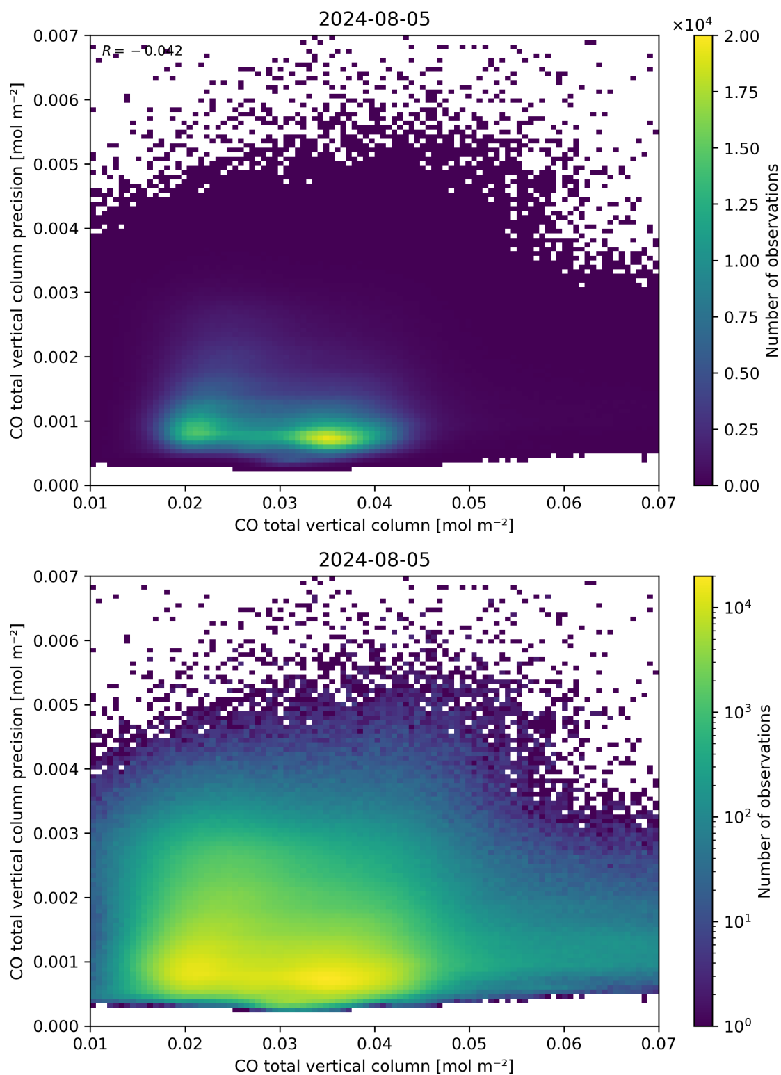
Figure 34: Scatter density plot of “CO total vertical column” against “CO total vertical column precision” for 2024-08-04 to 2024-08-06.
