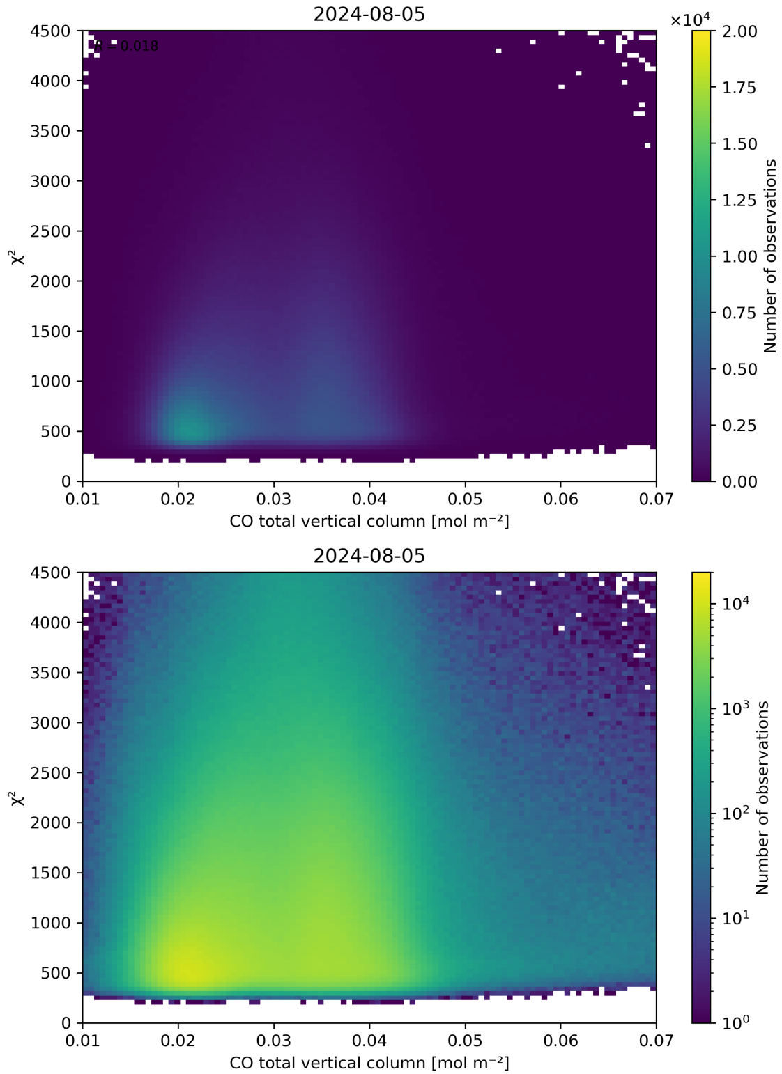
Figure 35: Scatter density plot of “CO total vertical column” against “ \chi^2 ” for 2024-08-04 to 2024-08-06.
