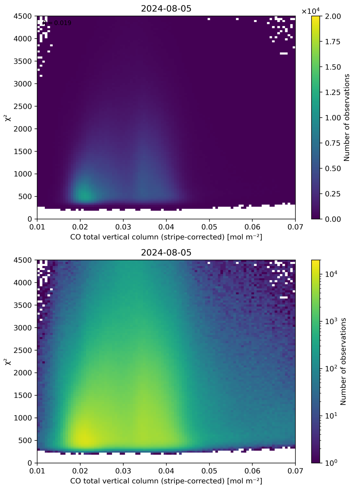
Figure 37: Scatter density plot of “CO total vertical column (stripe-corrected)” against “ \chi^2 ” for 2024-08-04 to 2024-08-06.
