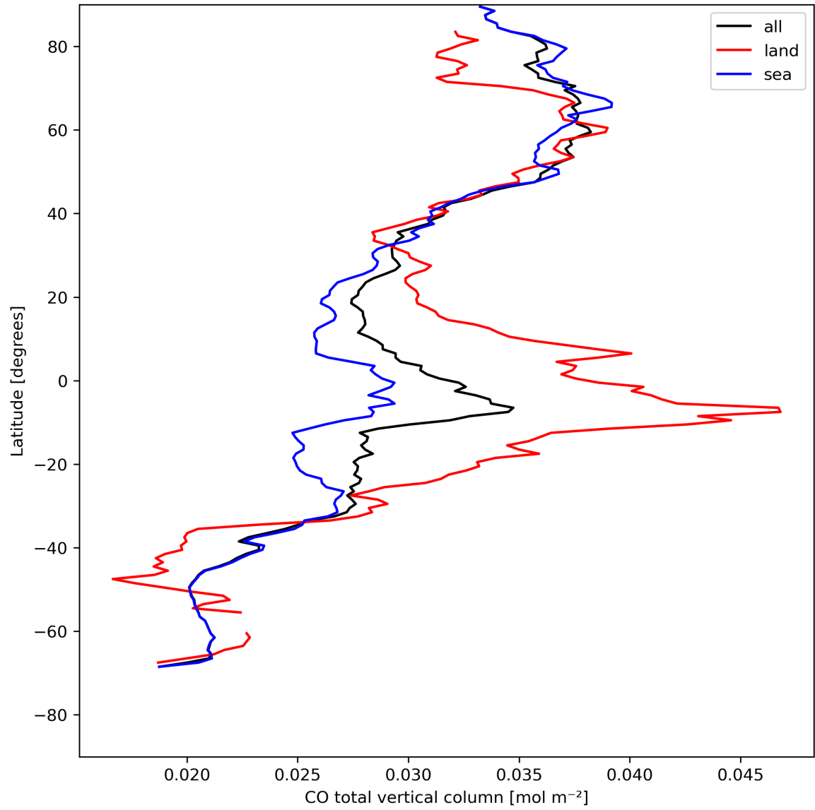
Figure 10: Zonal average of “CO total vertical column” for 2024-08-04 to 2024-08-06.
