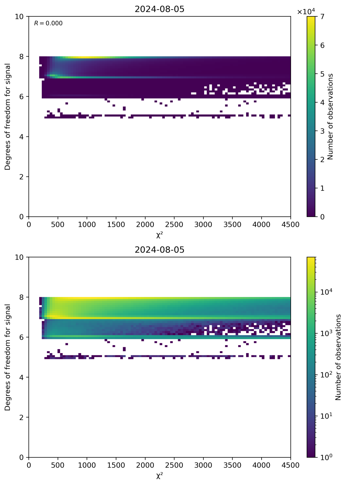
Figure 48: Scatter density plot of “ \chi^2 ” against “Degrees of freedom for signal” for 2024-08-04 to 2024-08-06.
