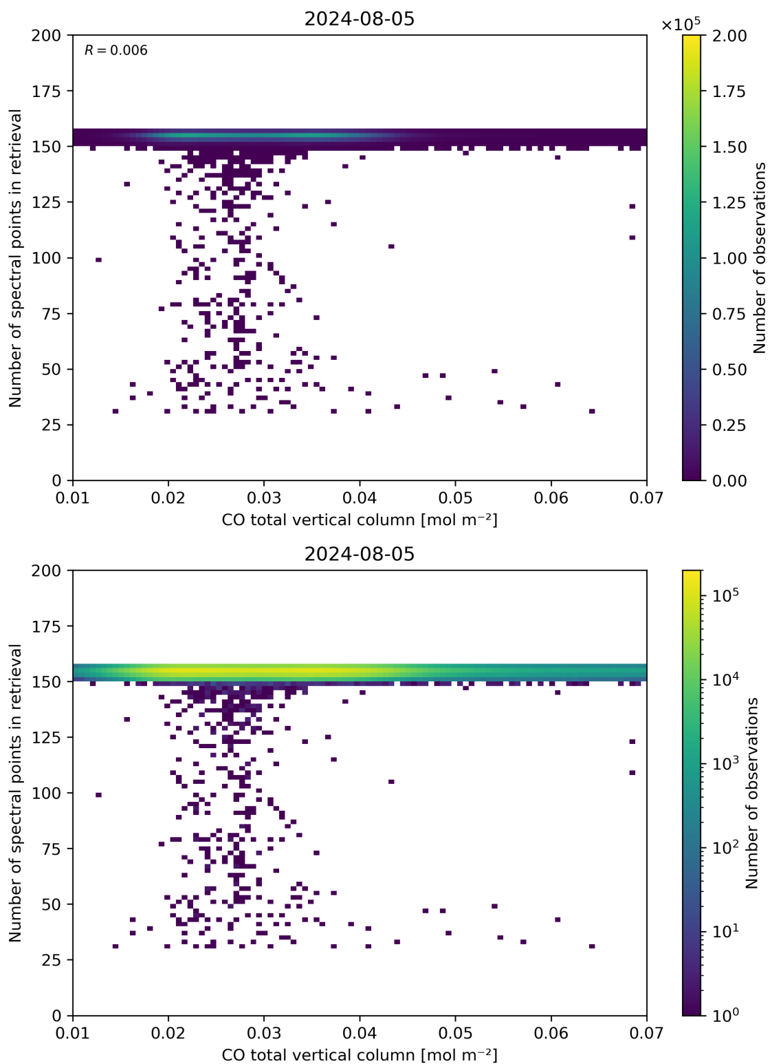
Figure 43: Scatter density plot of “CO total vertical column” against “Number of spectral points in retrieval” for 2024-08-04 to 2024-08-06.
