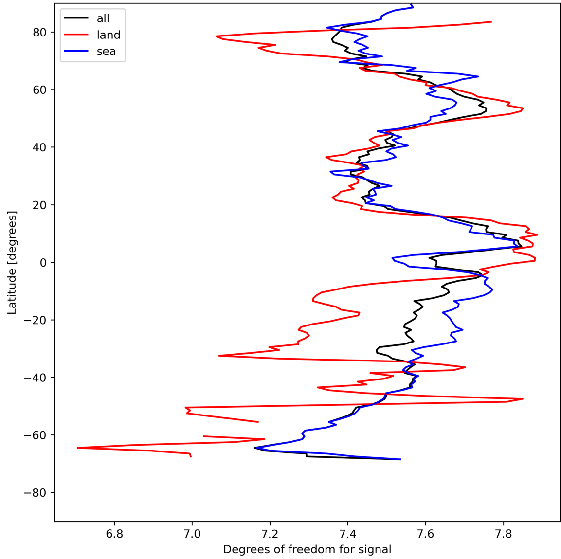
Figure 15: Zonal average of “Degrees of freedom for signal” for 2024-08-04 to 2024-08-06.
