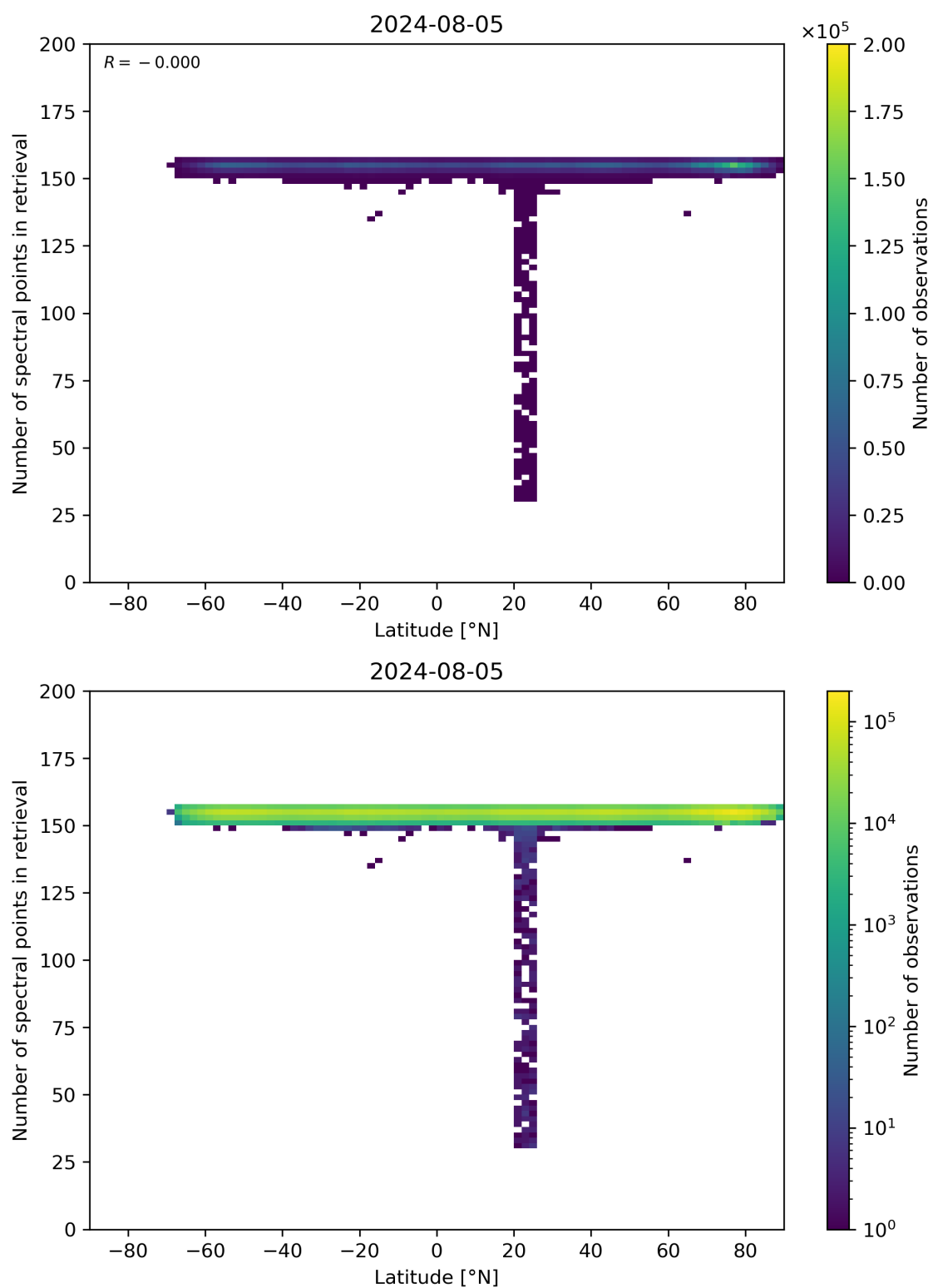
Figure 57: Scatter density plot of “Latitude” against “Number of spectral points in retrieval” for 2024-08-04 to 2024-08-06.
