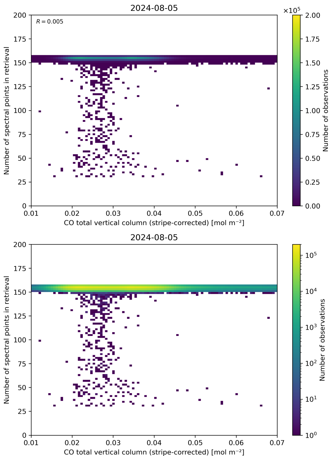
Figure 40: Scatter density plot of “CO total vertical column (stripe-corrected)” against “Number of spectral points in retrieval” for 2024-08-04 to 2024-08-06.
