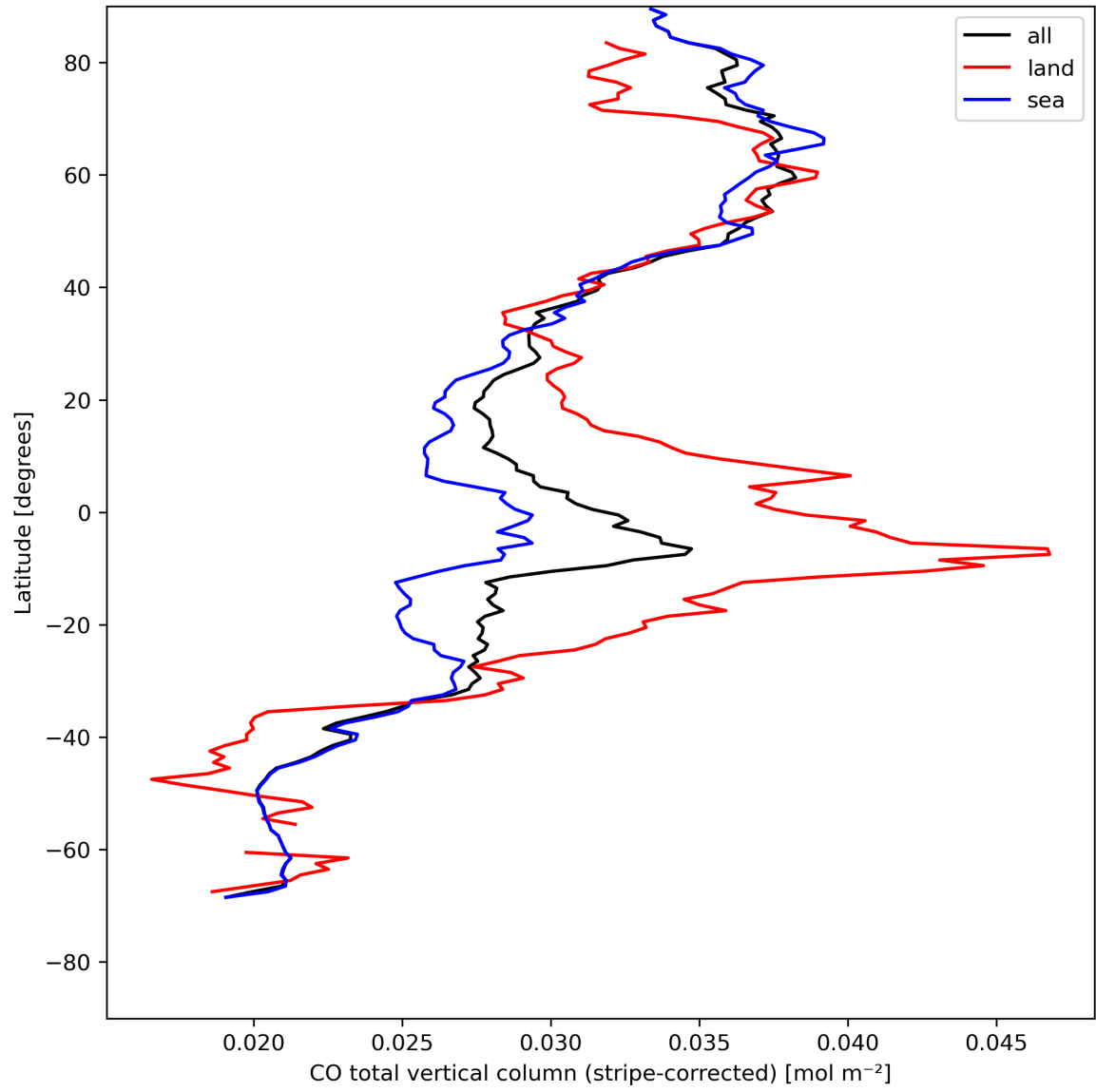
Figure 11: Zonal average of “CO total vertical column (stripe-corrected)” for 2024-08-04 to 2024-08-06.
