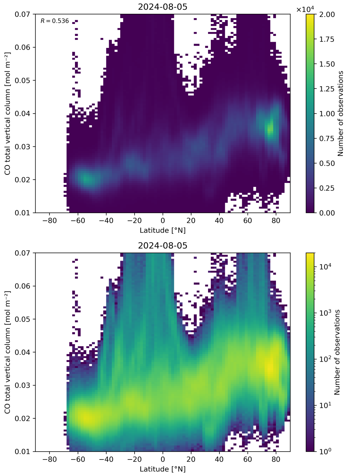
Figure 51: Scatter density plot of “Latitude” against “CO total vertical column” for 2024-08-04 to 2024-08-06.
