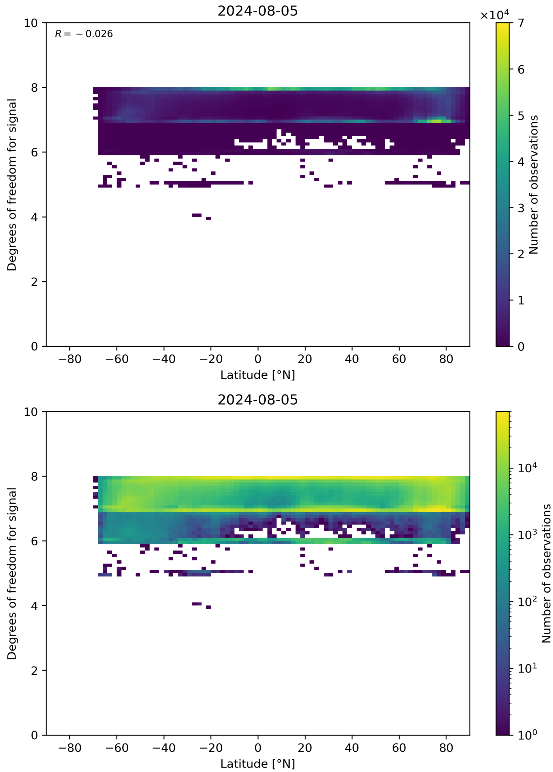
Figure 55: Scatter density plot of “Latitude” against “Degrees of freedom for signal” for 2024-08-04 to 2024-08-06.
