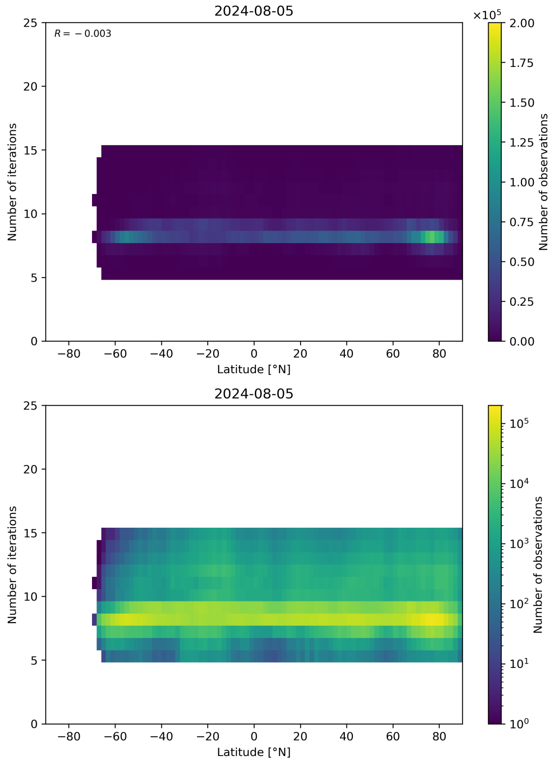
Figure 56: Scatter density plot of “Latitude” against “Number of iterations” for 2024-08-04 to 2024-08-06.
