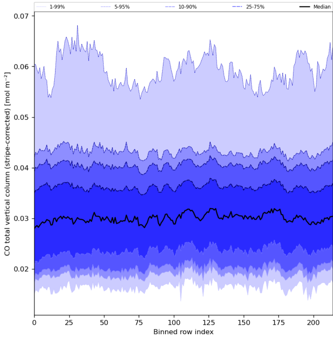
Figure 27: Along track statistics of “CO total vertical column (stripe-corrected)” for 2024-08-04 to 2024-08-06
