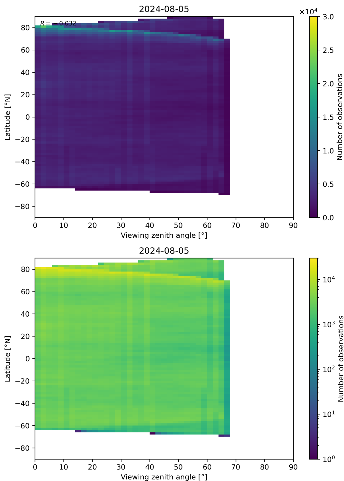
Figure 74: Scatter density plot of “Viewing zenith angle” against “Latitude” for 2024-08-04 to 2024-08-06.
