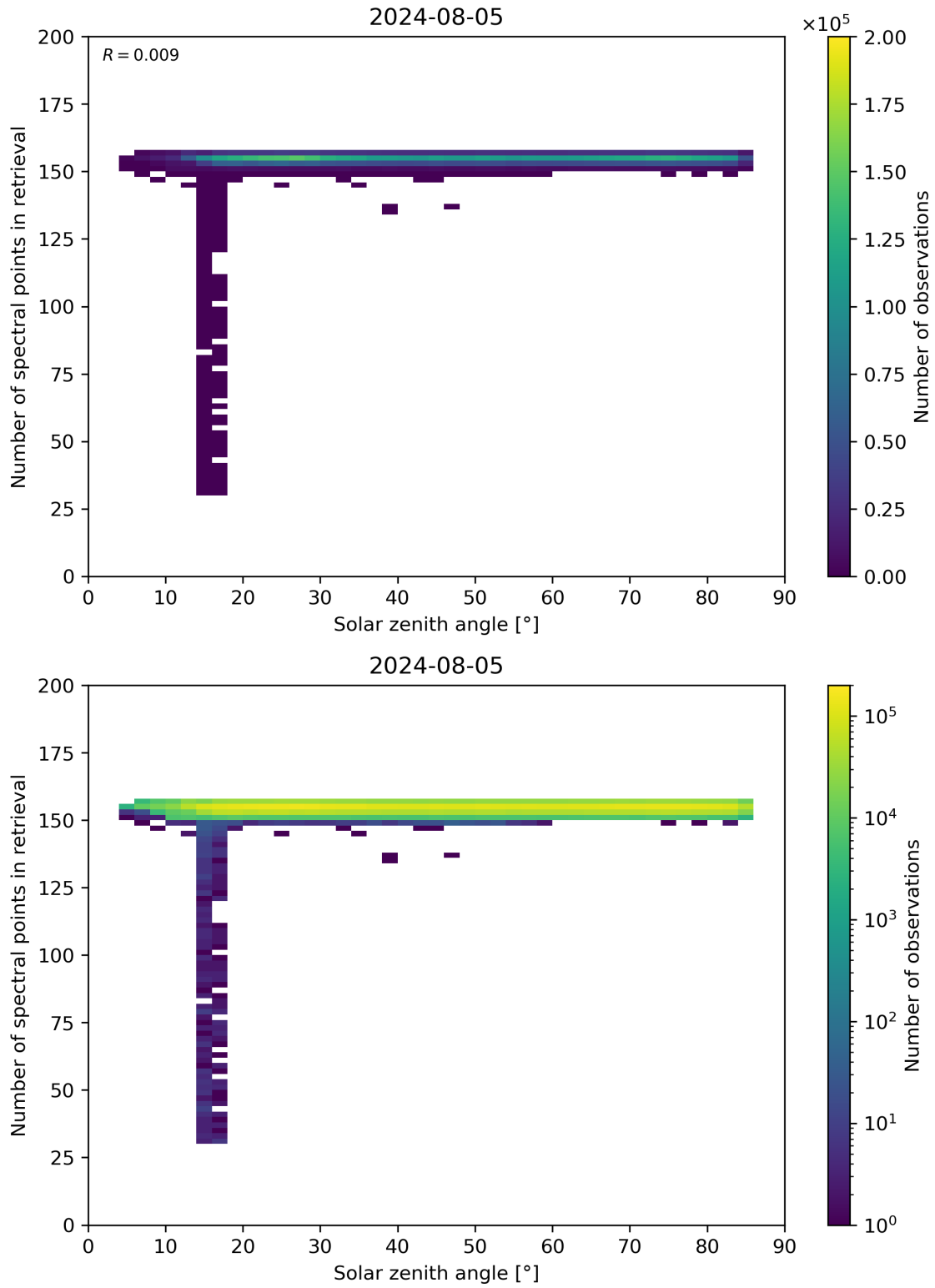
Figure 68: Scatter density plot of “Solar zenith angle” against “Number of spectral points in retrieval” for 2024-08-04 to 2024-08-06.
