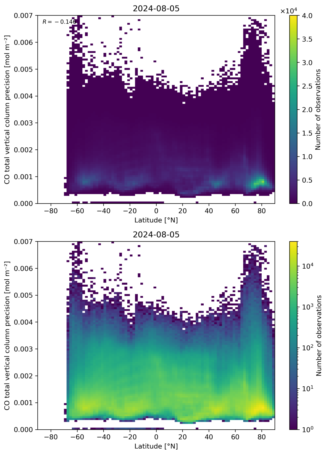
Figure 53: Scatter density plot of “Latitude” against “CO total vertical column precision” for 2024-08-04 to 2024-08-06.
