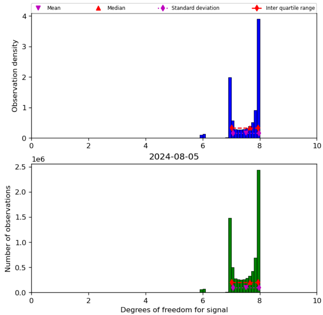
Figure 23: Histogram of “Degrees of freedom for signal” for 2024-08-04 to 2024-08-06
