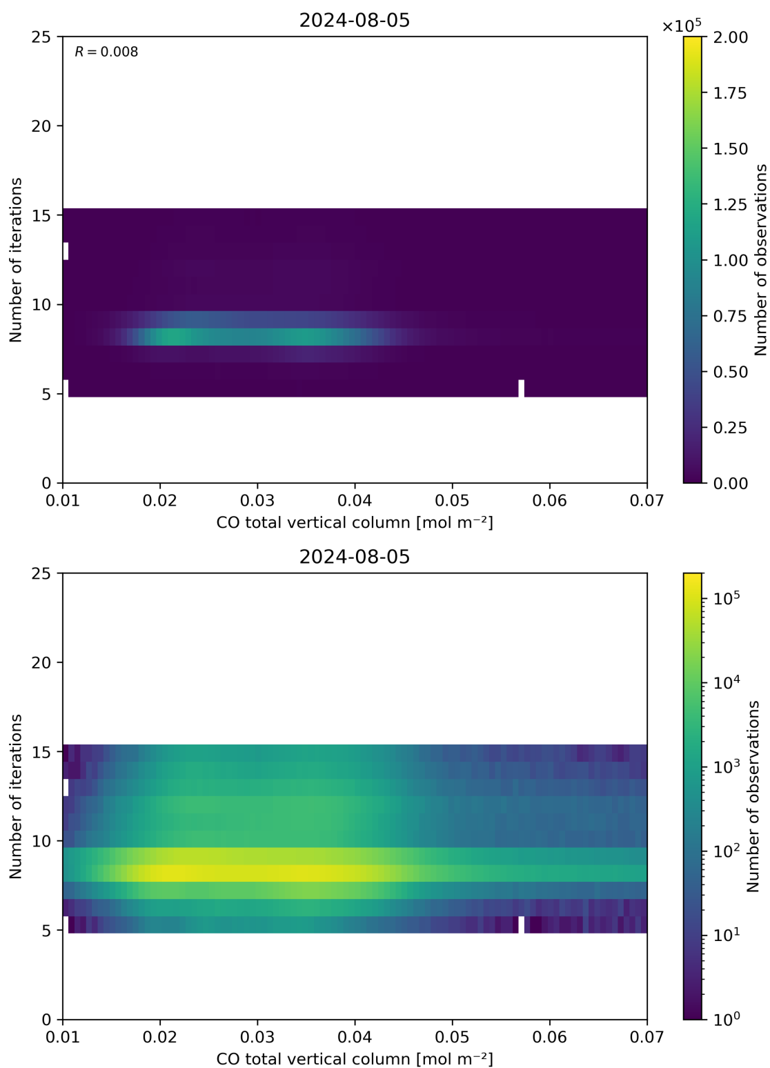
Figure 42: Scatter density plot of “CO total vertical column” against “Number of iterations” for 2024-08-04 to 2024-08-06.
