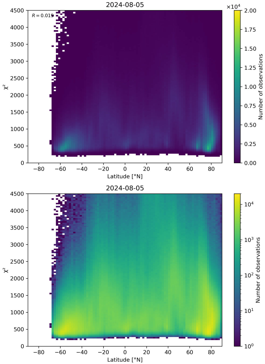
Figure 54: Scatter density plot of “Latitude” against “ \chi^2 ” for 2024-08-04 to 2024-08-06.
