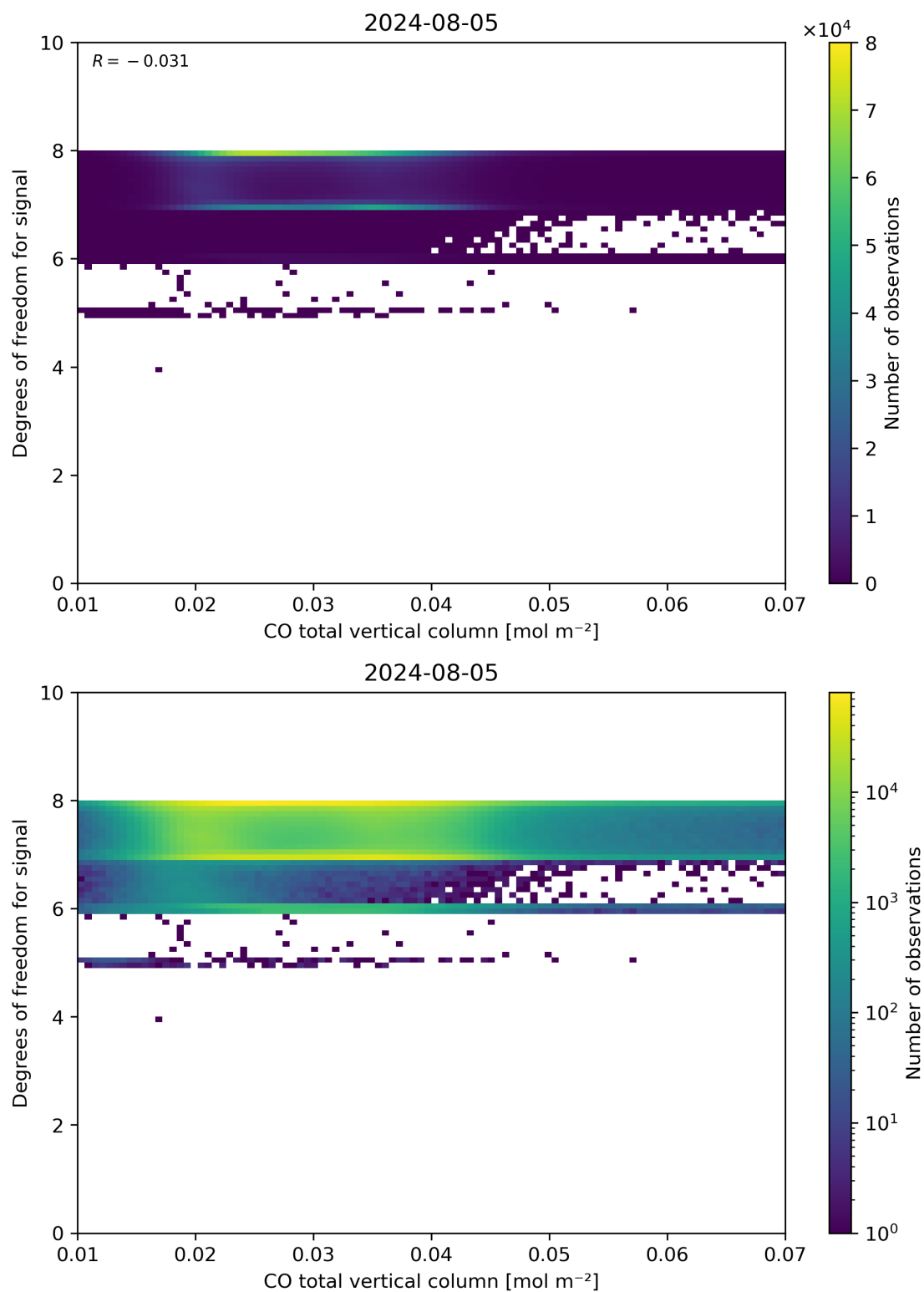
Figure 41: Scatter density plot of “CO total vertical column” against “Degrees of freedom for signal” for 2024-08-04 to 2024-08-06.
