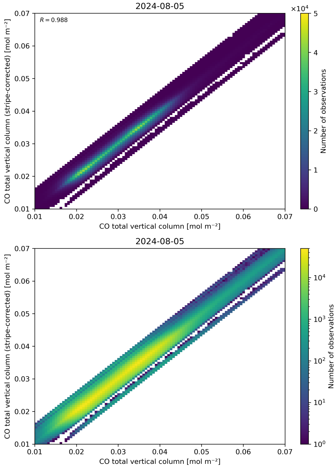
Figure 33: Scatter density plot of “CO total vertical column” against “CO total vertical column (stripe-corrected)” for 2024-08-04 to 2024-08-06.
