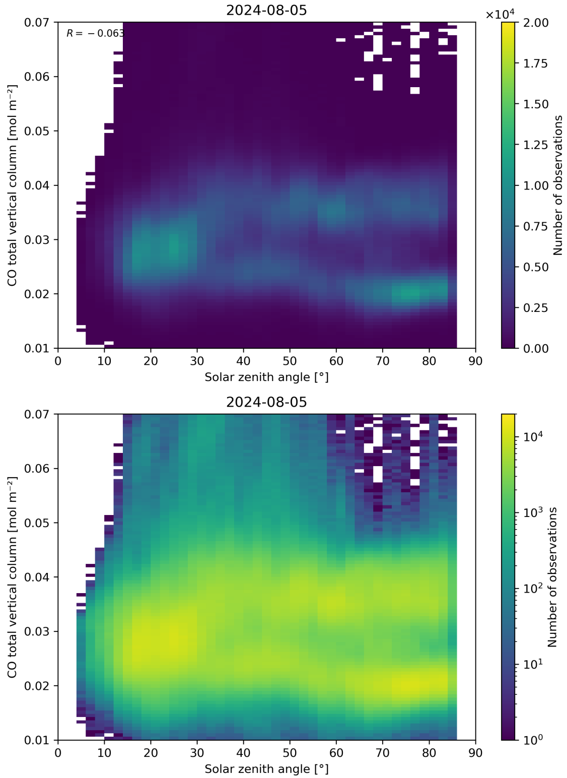
Figure 61: Scatter density plot of “Solar zenith angle” against “CO total vertical column” for 2024-08-04 to 2024-08-06.
