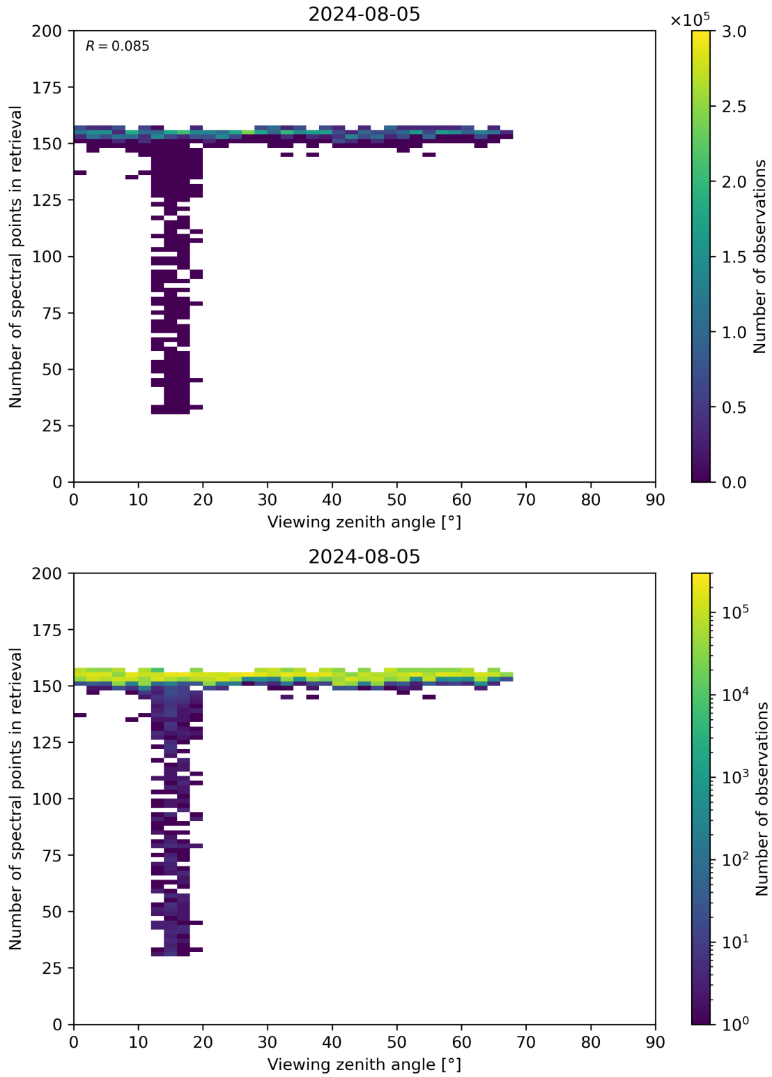
Figure 76: Scatter density plot of “Viewing zenith angle” against “Number of spectral points in retrieval” for 2024-08-04 to 2024-08-06.
