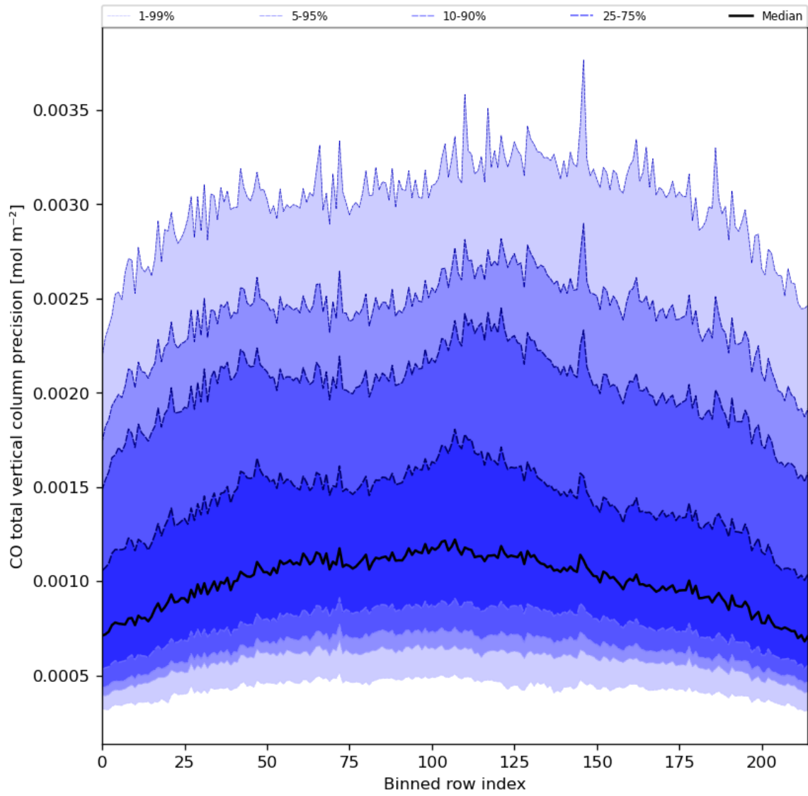
Figure 28: Along track statistics of “CO total vertical column precision” for 2024-08-04 to 2024-08-06
