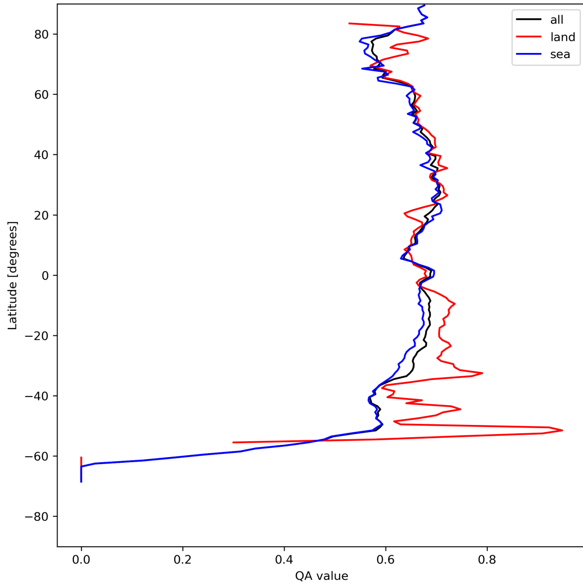
Figure 9: Zonal average of “QA value” for 2024-08-04 to 2024-08-06.
