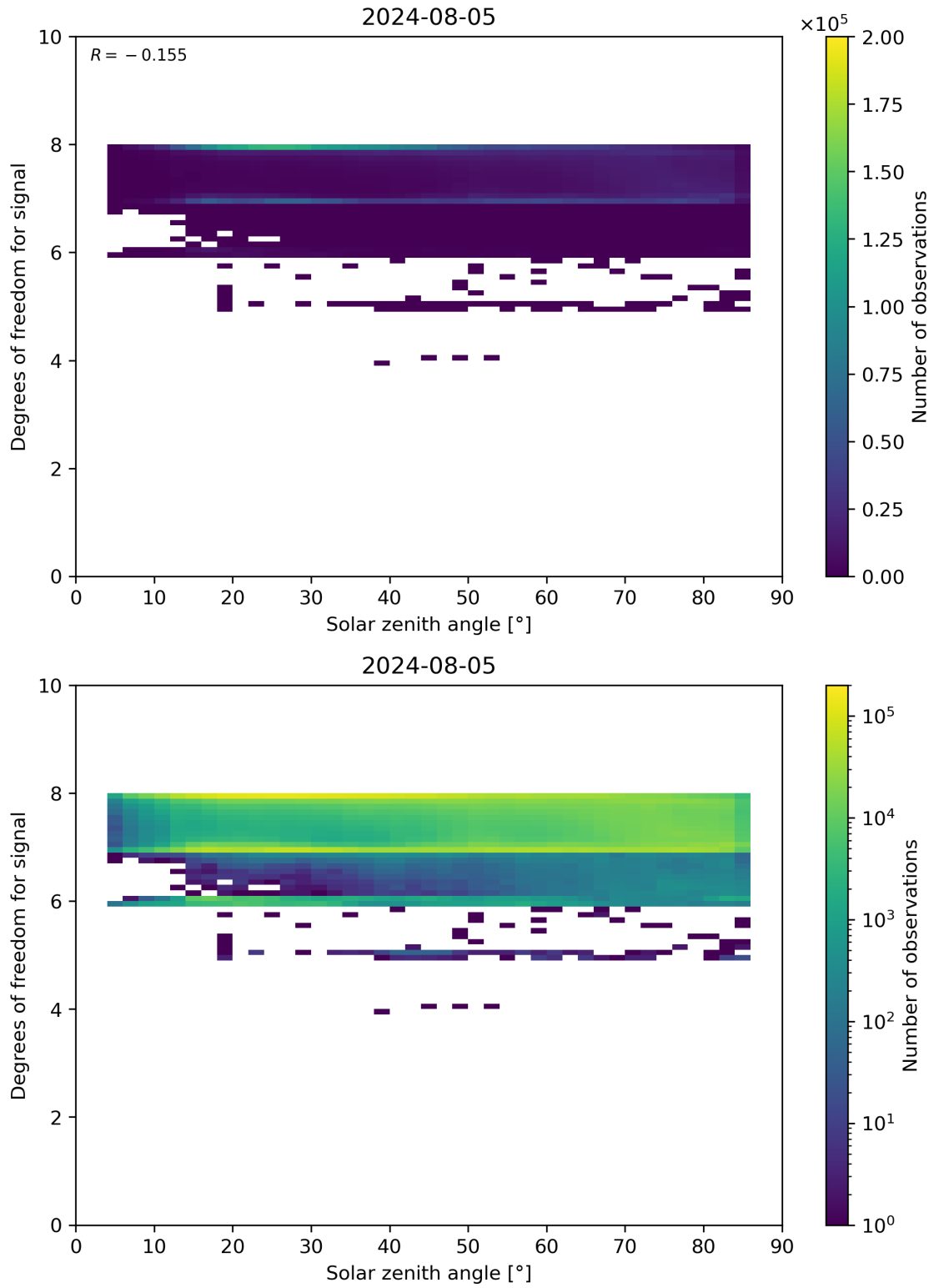
Figure 65: Scatter density plot of “Solar zenith angle” against “Degrees of freedom for signal” for 2024-08-04 to 2024-08-06.
