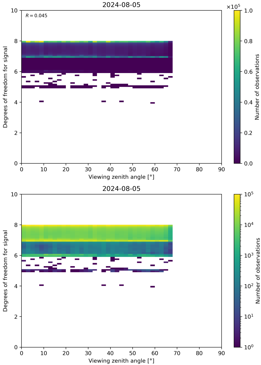
Figure 73: Scatter density plot of “Viewing zenith angle” against “Degrees of freedom for signal” for 2024-08-04 to 2024-08-06.
