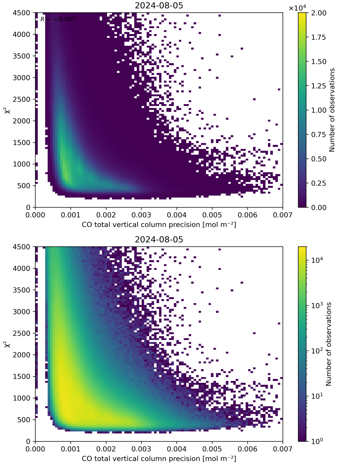
Figure 44: Scatter density plot of “CO total vertical column precision” against “ \chi^2 ” for 2024-08-04 to 2024-08-06.
