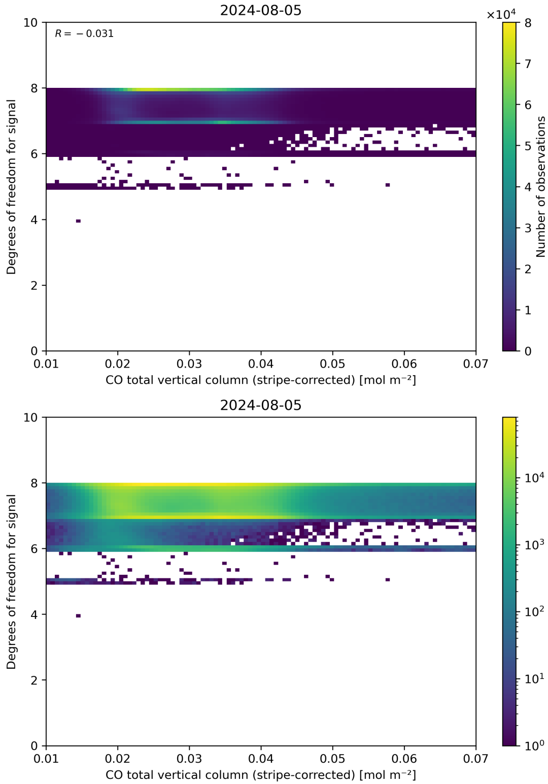
Figure 38: Scatter density plot of “CO total vertical column (stripe-corrected)” against “Degrees of freedom for signal” for 2024-08-04 to 2024-08-06.
