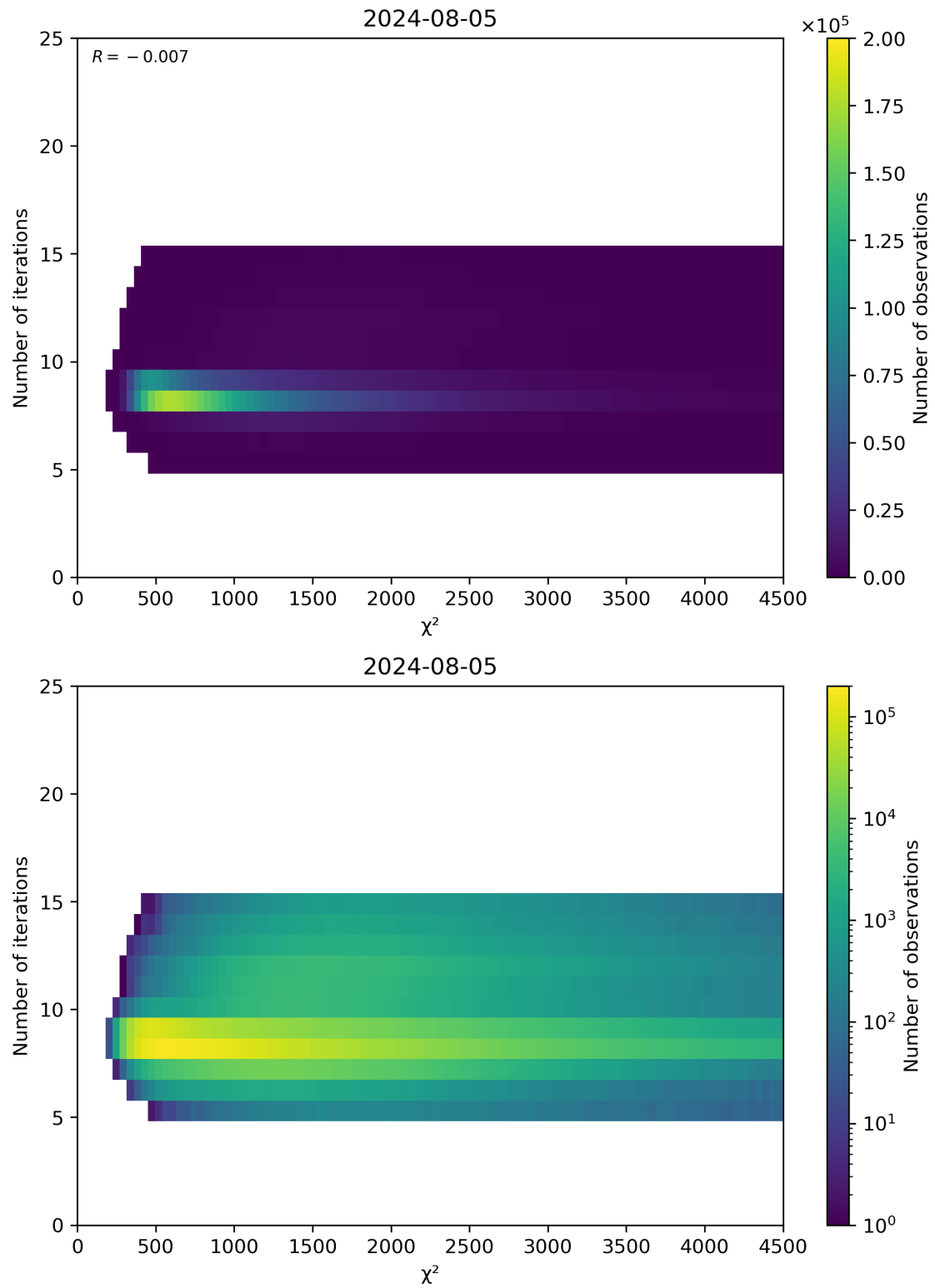
Figure 49: Scatter density plot of “ \chi^2 ” against “Number of iterations” for 2024-08-04 to 2024-08-06.
