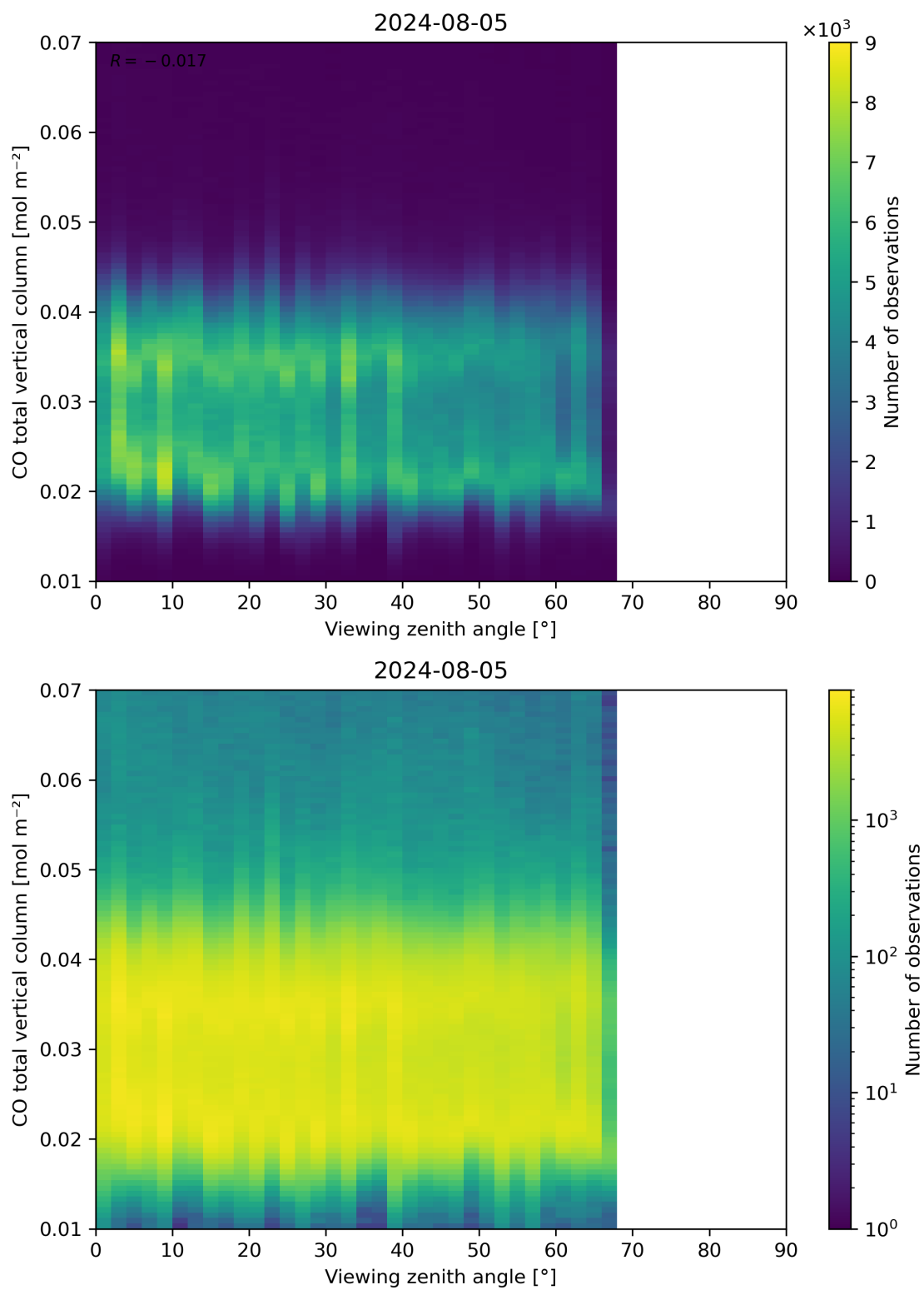
Figure 69: Scatter density plot of “Viewing zenith angle” against “CO total vertical column” for 2024-08-04 to 2024-08-06.
