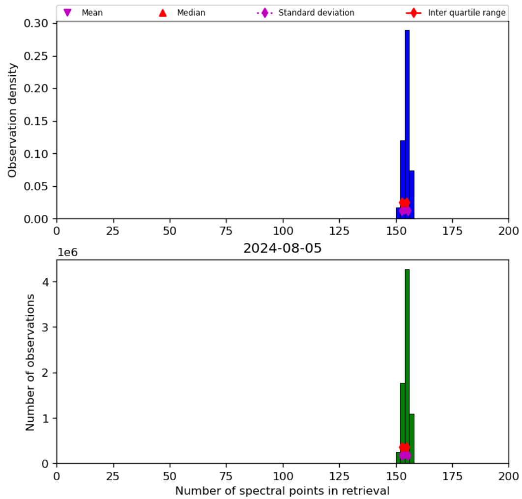
Figure 21: Histogram of “Number of spectral points in retrieval” for 2024-08-04 to 2024-08-06
