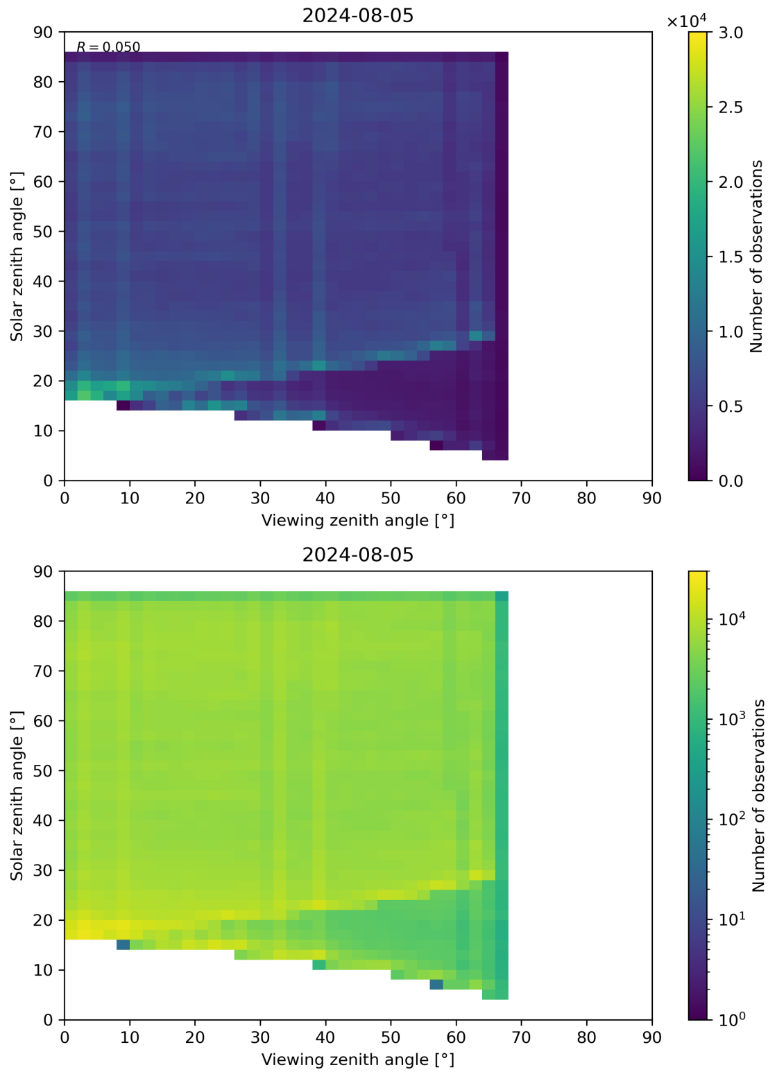
Figure 77: Scatter density plot of “Viewing zenith angle” against “Solar zenith angle” for 2024-08-04 to 2024-08-06.
