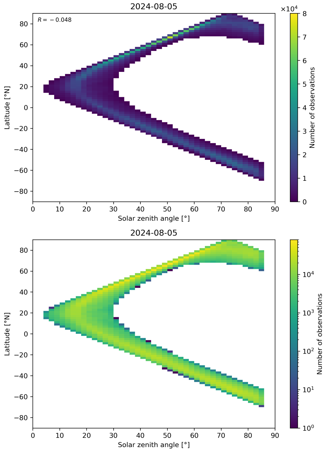
Figure 66: Scatter density plot of “Solar zenith angle” against “Latitude” for 2024-08-04 to 2024-08-06.
