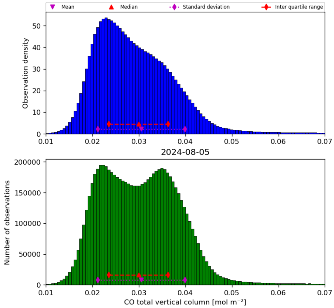
Figure 18: Histogram of “CO total vertical column” for 2024-08-04 to 2024-08-06
