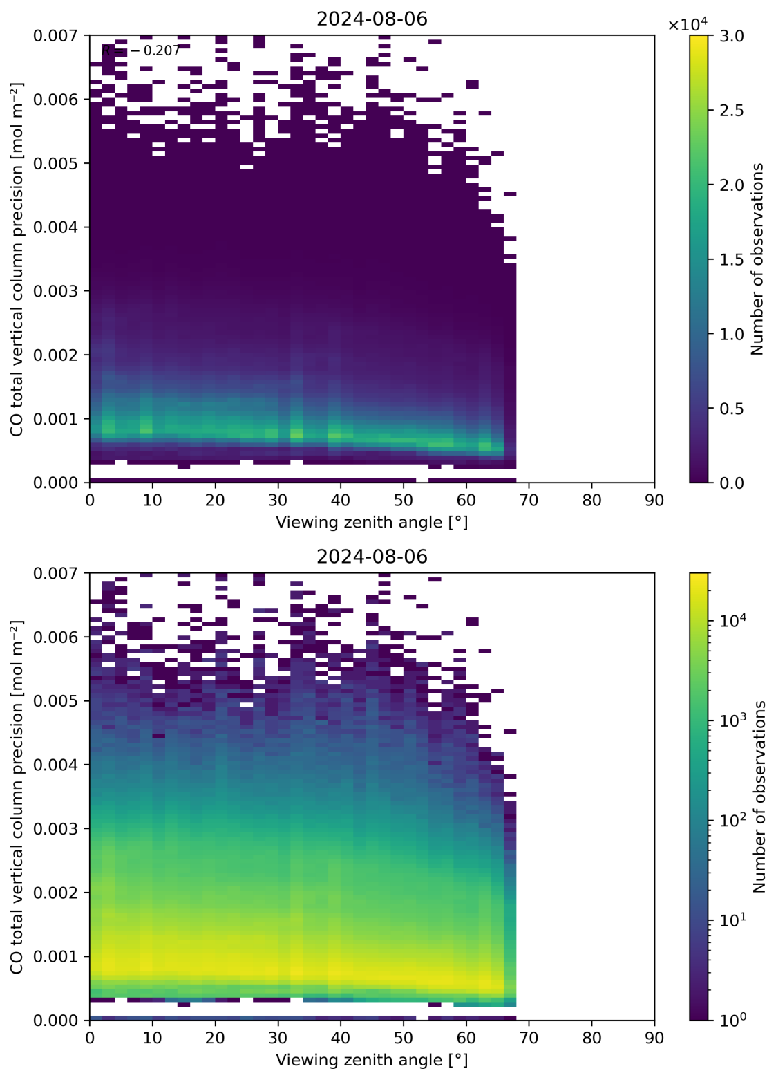
Figure 71: Scatter density plot of “Viewing zenith angle” against “CO total vertical column precision” for 2024-08-06 to 2024-08-07.
