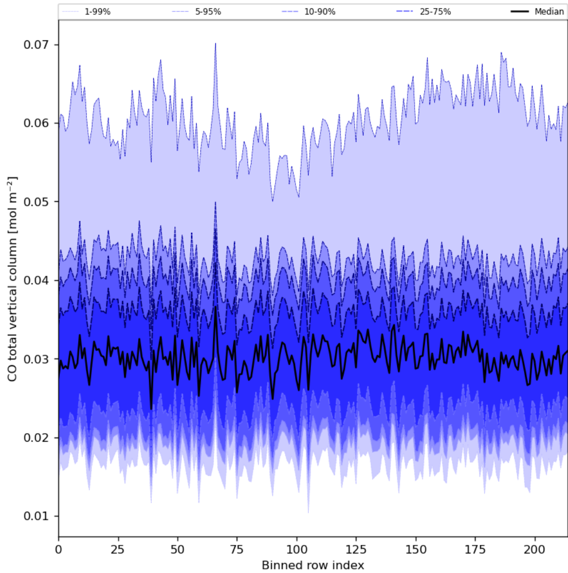
Figure 26: Along track statistics of “CO total vertical column” for 2024-08-06 to 2024-08-07
