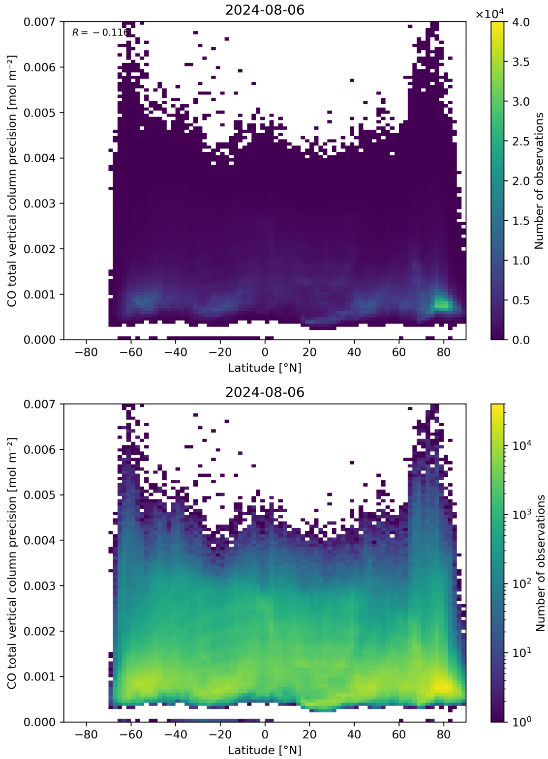
Figure 53: Scatter density plot of “Latitude” against “CO total vertical column precision” for 2024-08-06 to 2024-08-07.
