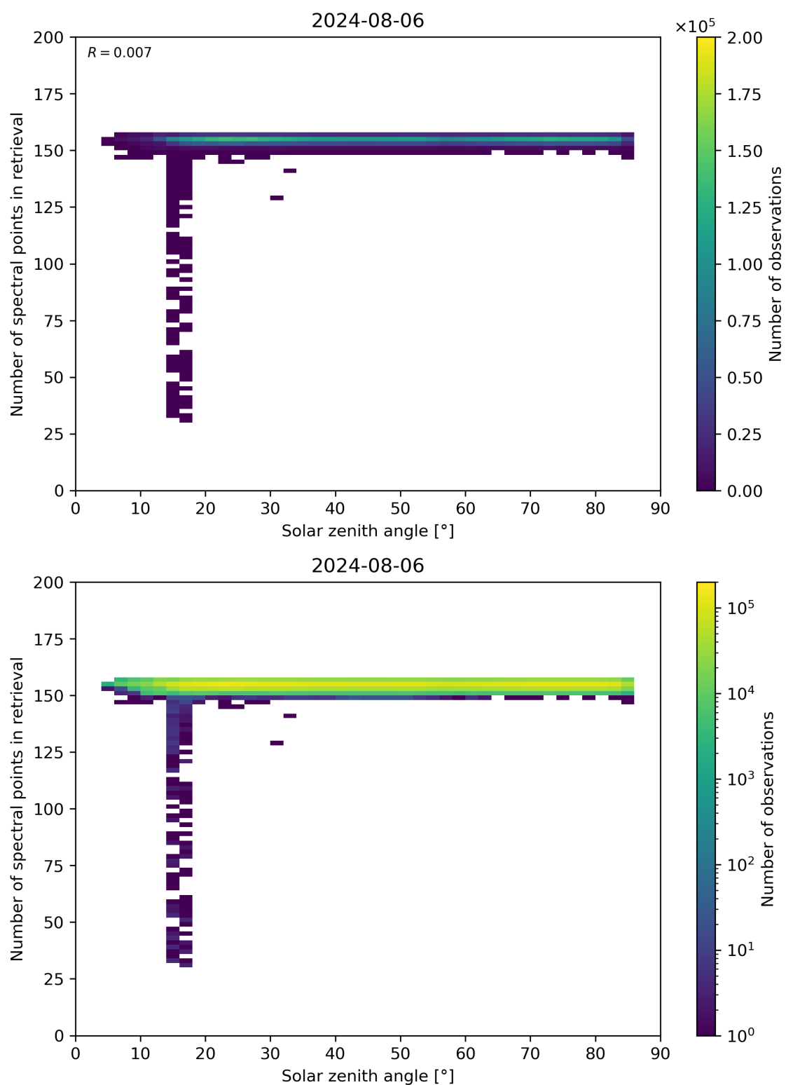
Figure 68: Scatter density plot of “Solar zenith angle” against “Number of spectral points in retrieval” for 2024-08-06 to 2024-08-07.
