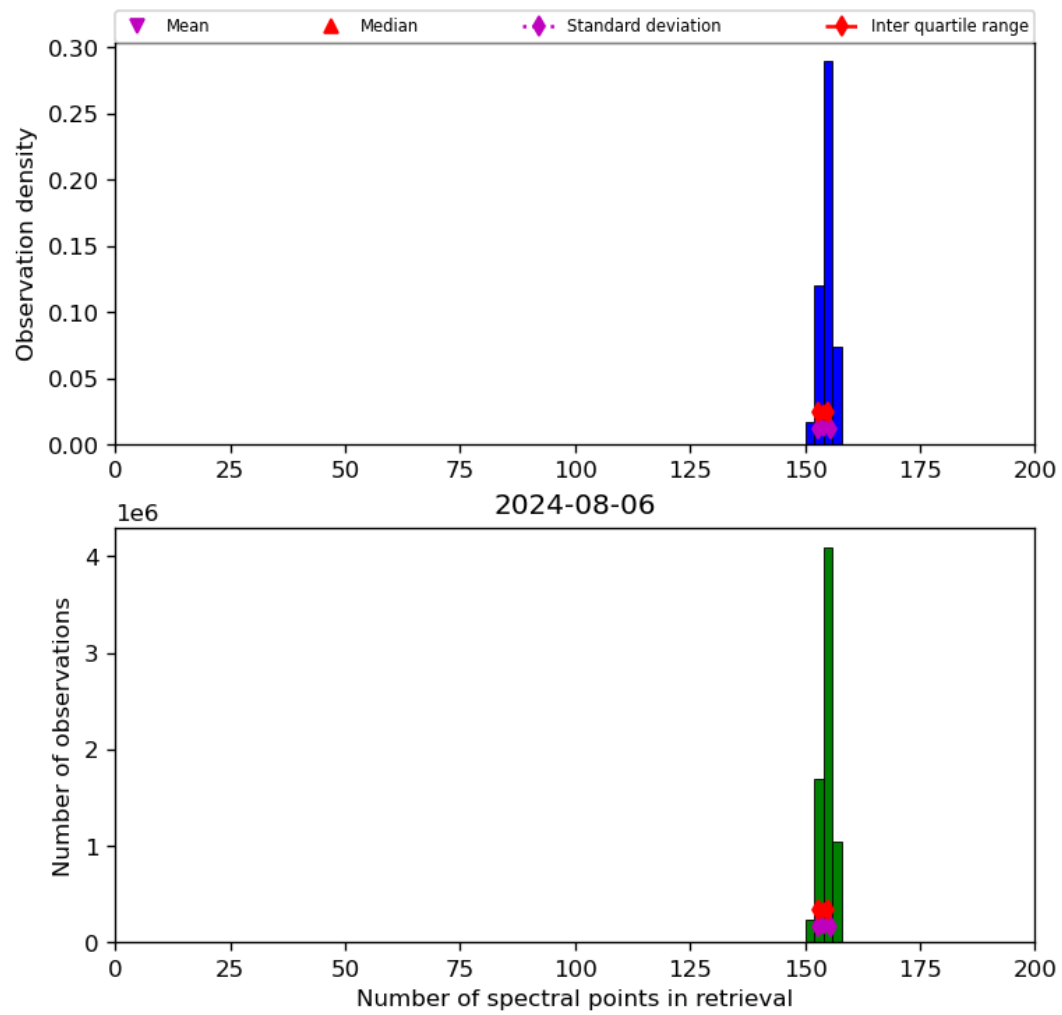
Figure 21: Histogram of “Number of spectral points in retrieval” for 2024-08-06 to 2024-08-07
