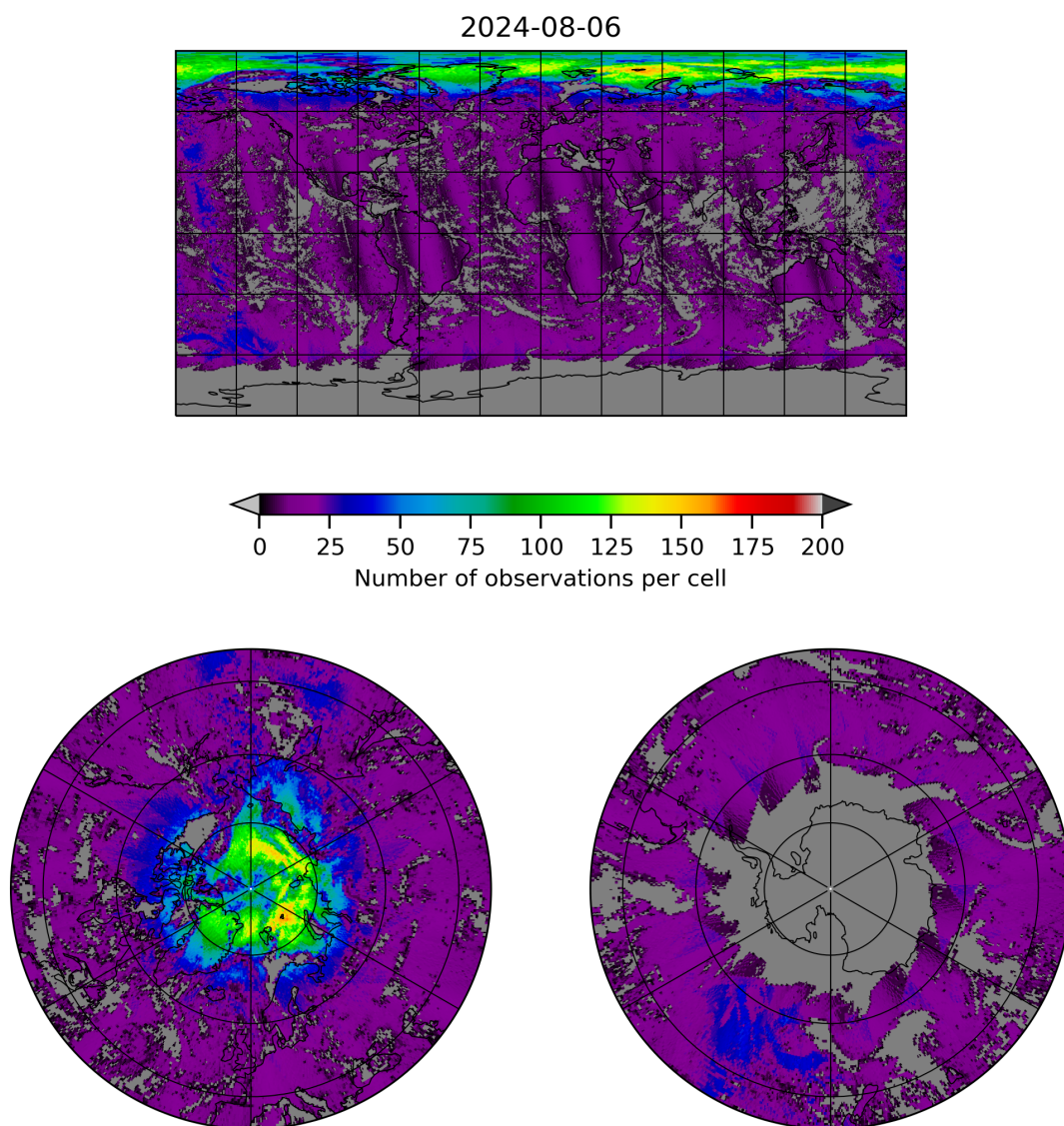
Figure 8: Map of the number of observations for 2024-08-06 to 2024-08-07
