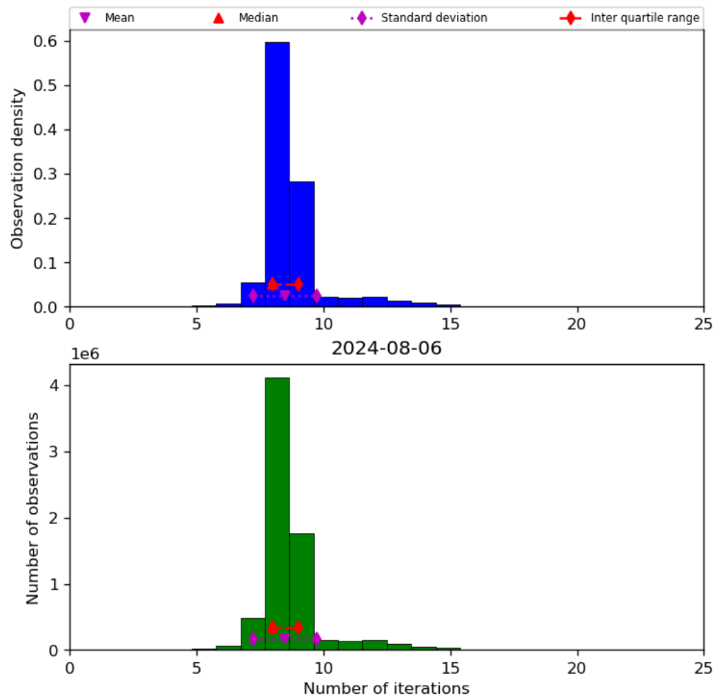
Figure 24: Histogram of “Number of iterations” for 2024-08-06 to 2024-08-07
