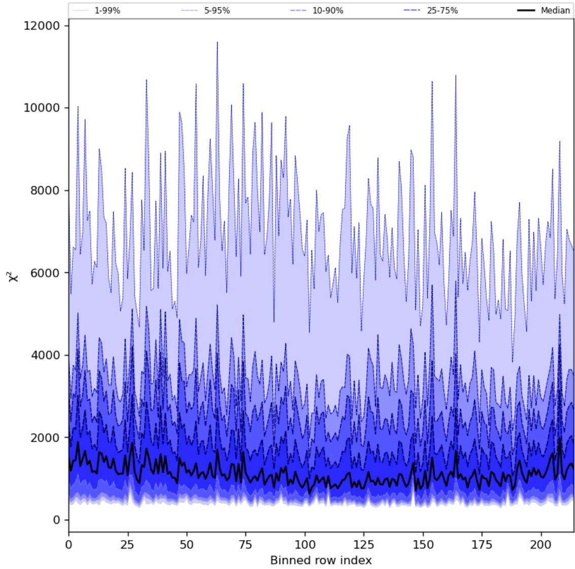
Figure 30: Along track statistics of “ \chi^2 ” for 2024-08-06 to 2024-08-07
