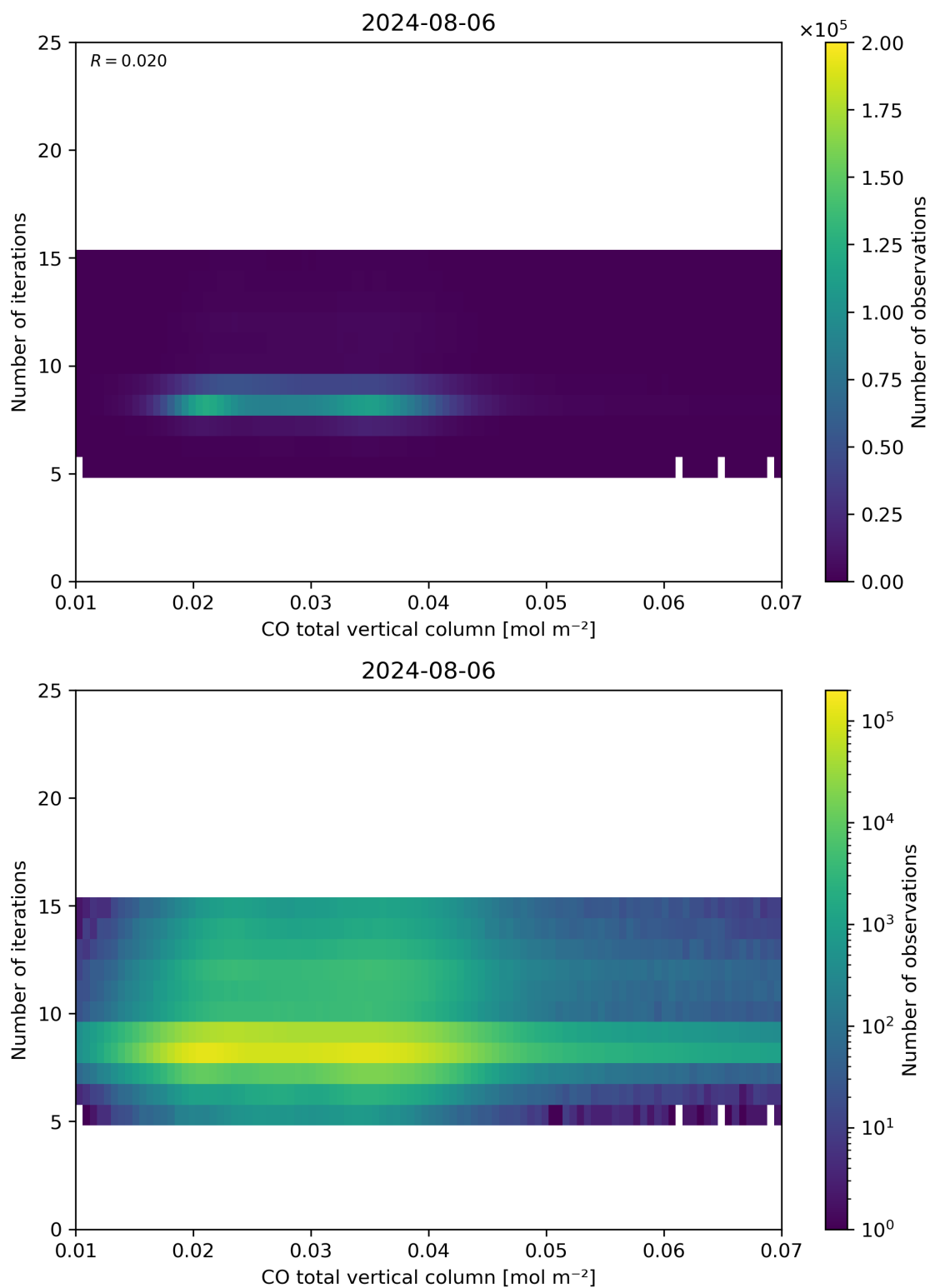
Figure 42: Scatter density plot of “CO total vertical column” against “Number of iterations” for 2024-08-06 to 2024-08-07.
