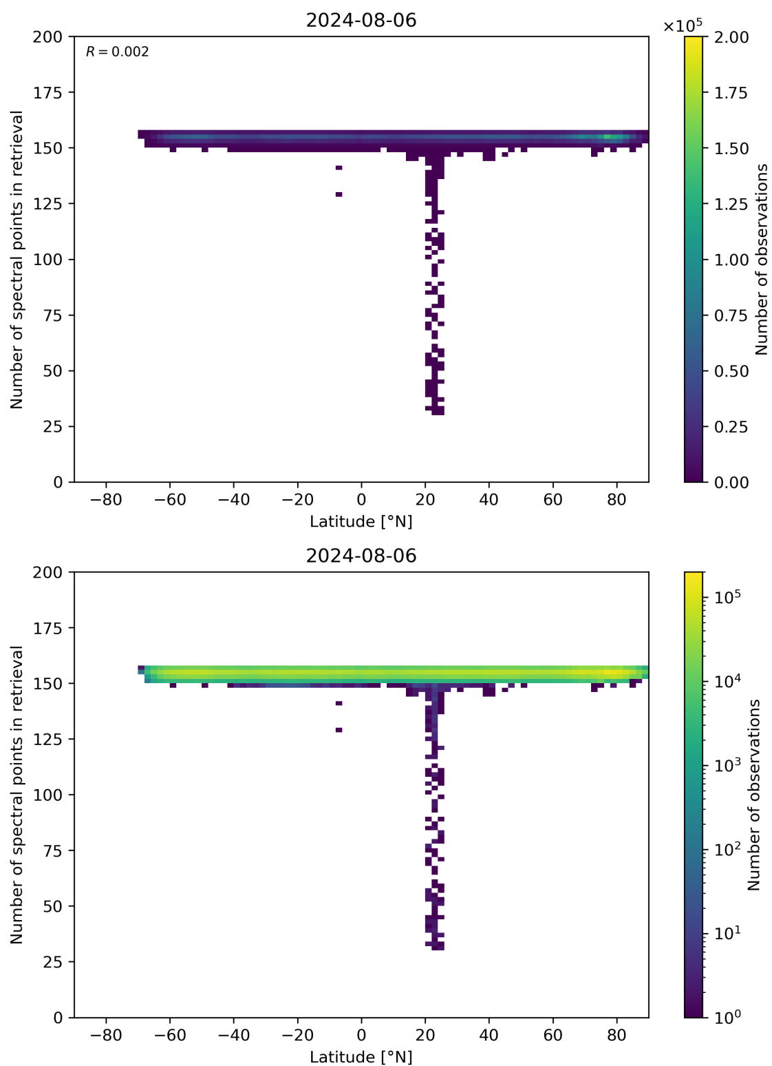
Figure 57: Scatter density plot of “Latitude” against “Number of spectral points in retrieval” for 2024-08-06 to 2024-08-07.
