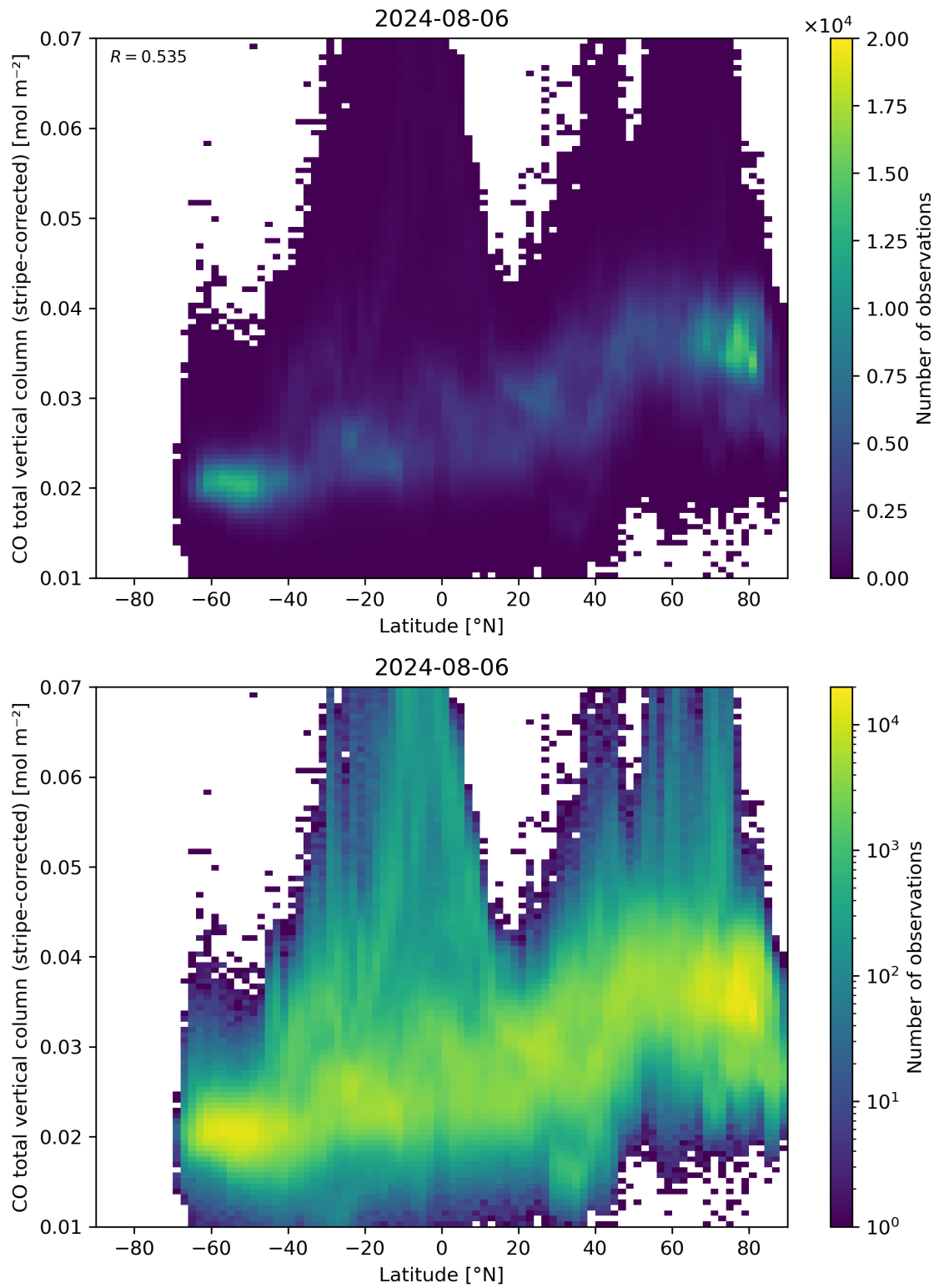
Figure 52: Scatter density plot of “Latitude” against “CO total vertical column (stripe-corrected)” for 2024-08-06 to 2024-08-07.
