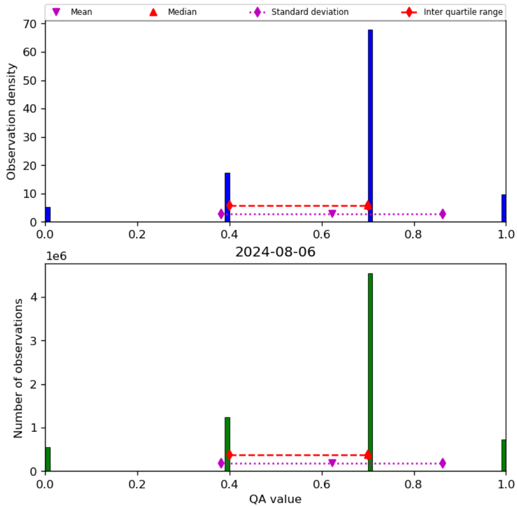
Figure 17: Histogram of “QA value” for 2024-08-06 to 2024-08-07
