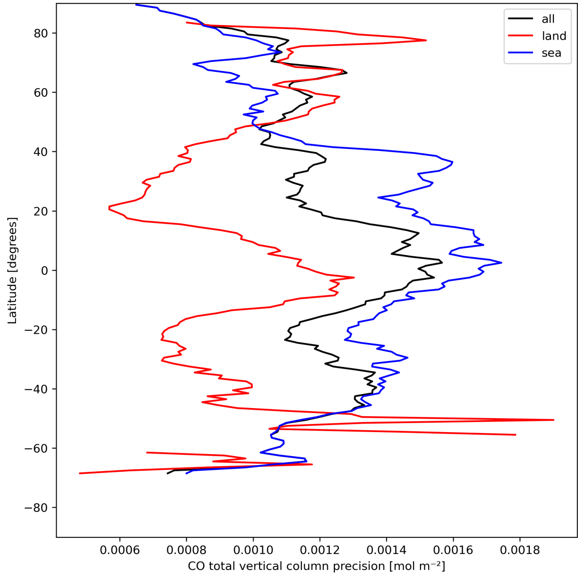
Figure 12: Zonal average of “CO total vertical column precision” for 2024-08-06 to 2024-08-07.
