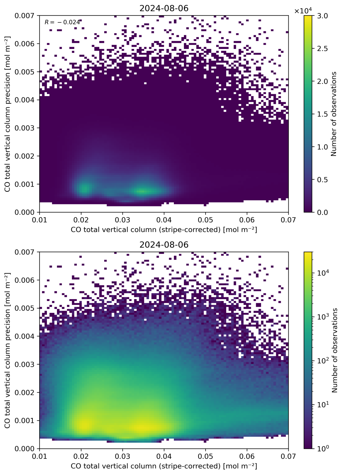
Figure 36: Scatter density plot of “CO total vertical column (stripe-corrected)” against “CO total vertical column precision” for 2024-08-06 to 2024-08-07.
