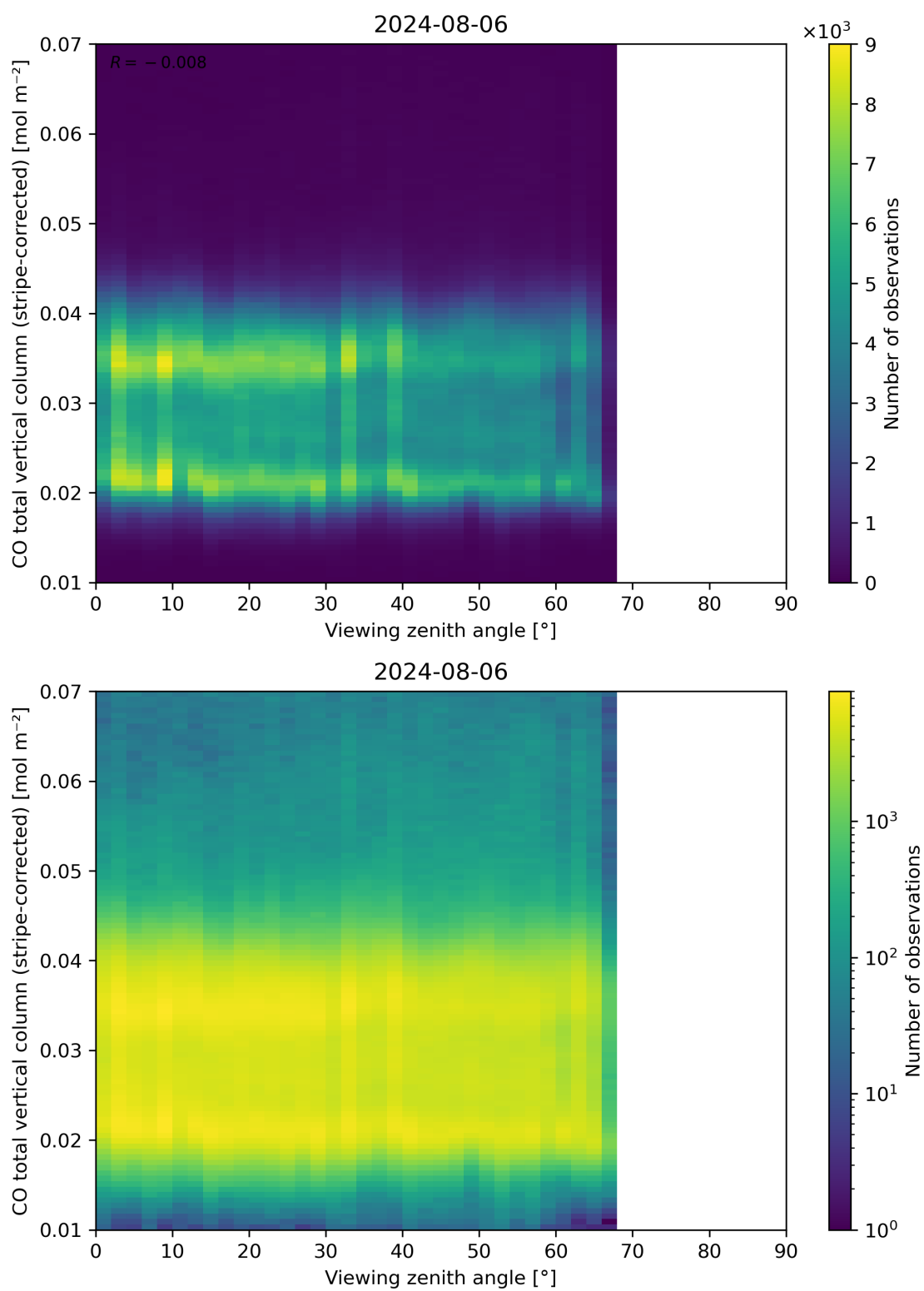
Figure 70: Scatter density plot of “Viewing zenith angle” against “CO total vertical column (stripe-corrected)” for 2024-08-06 to 2024-08-07.
