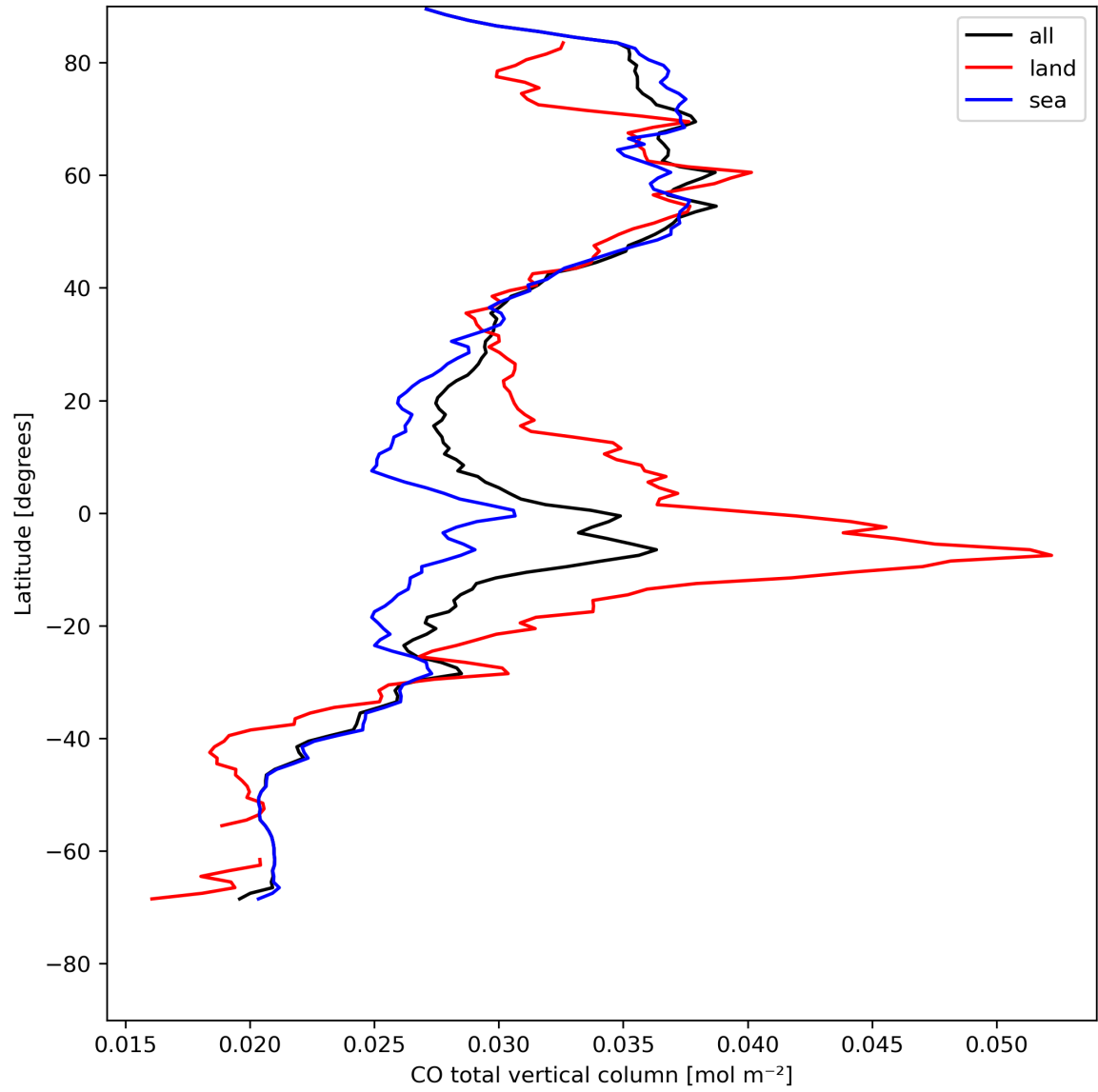
Figure 10: Zonal average of “CO total vertical column” for 2024-08-06 to 2024-08-07.
