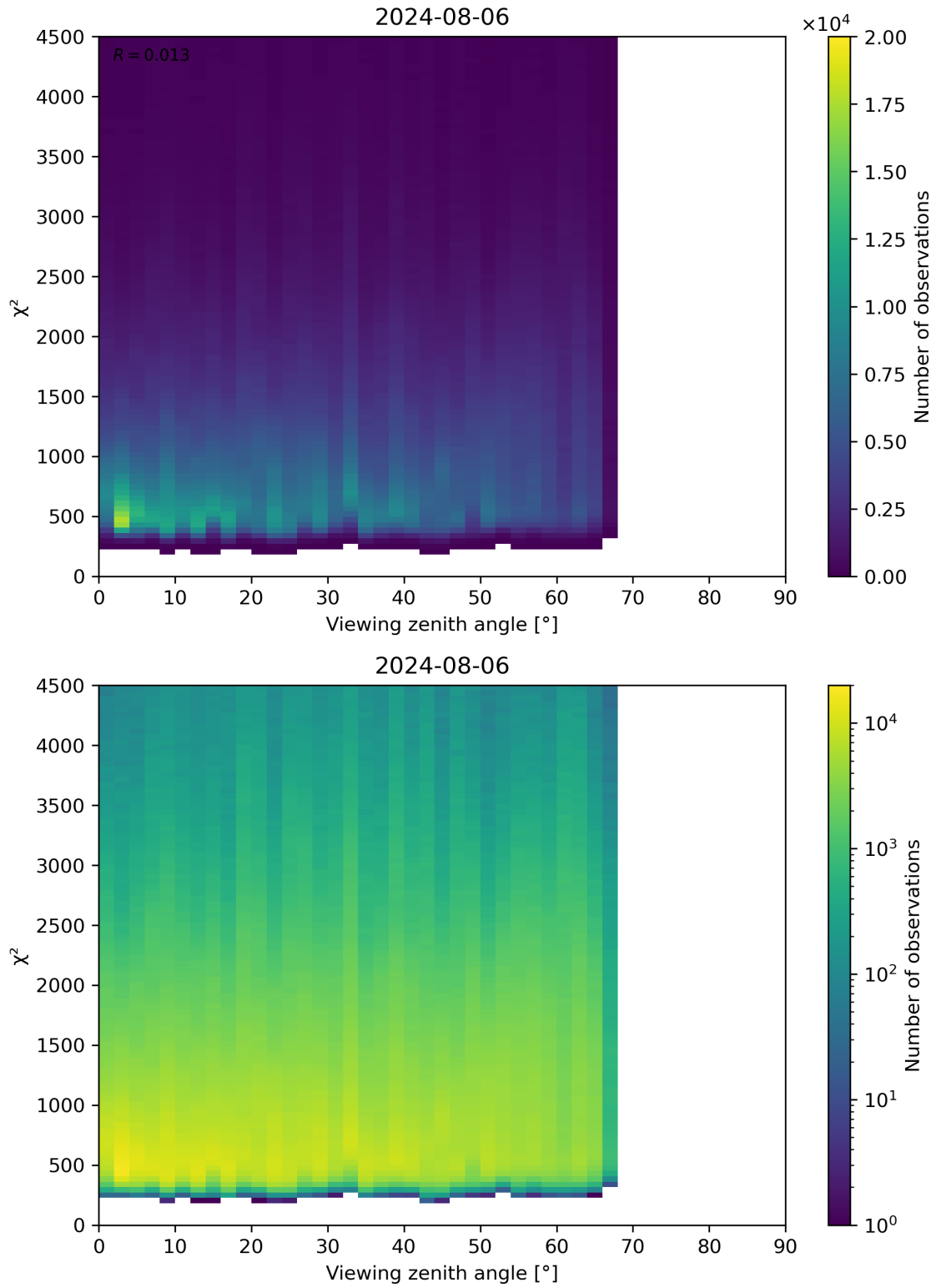
Figure 72: Scatter density plot of “Viewing zenith angle” against “ \chi^2 ” for 2024-08-06 to 2024-08-07.
