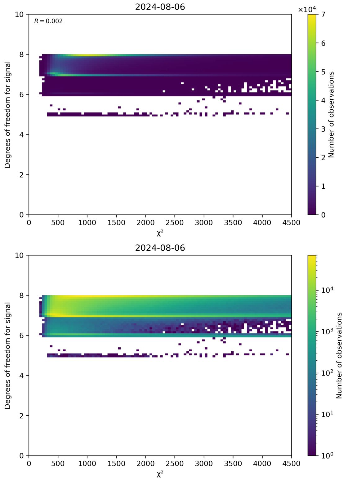
Figure 48: Scatter density plot of “ \chi^2 ” against “Degrees of freedom for signal” for 2024-08-06 to 2024-08-07.
