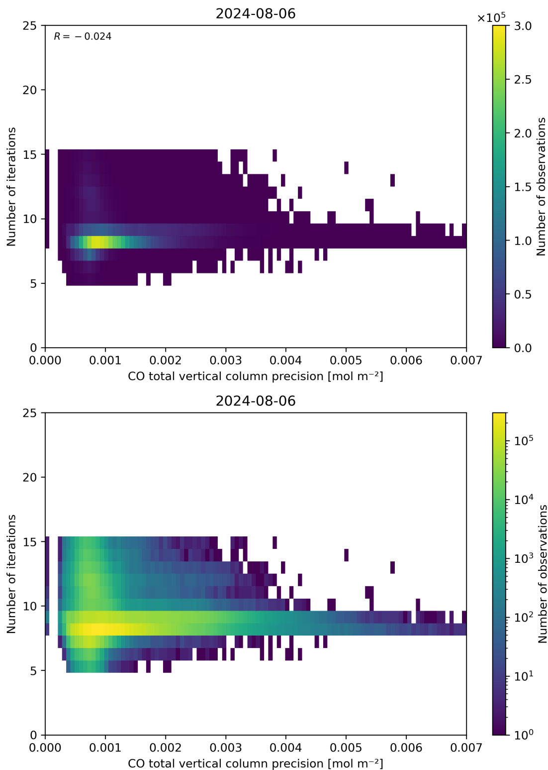
Figure 46: Scatter density plot of “CO total vertical column precision” against “Number of iterations” for 2024-08-06 to 2024-08-07.
