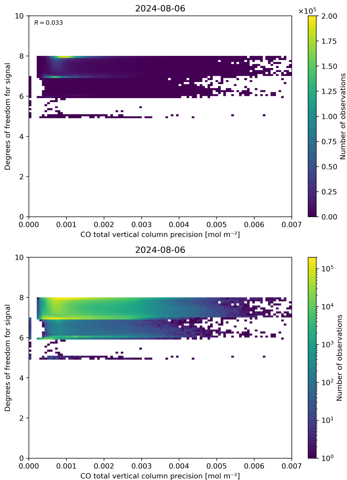
Figure 45: Scatter density plot of “CO total vertical column precision” against “Degrees of freedom for signal” for 2024-08-06 to 2024-08-07.
