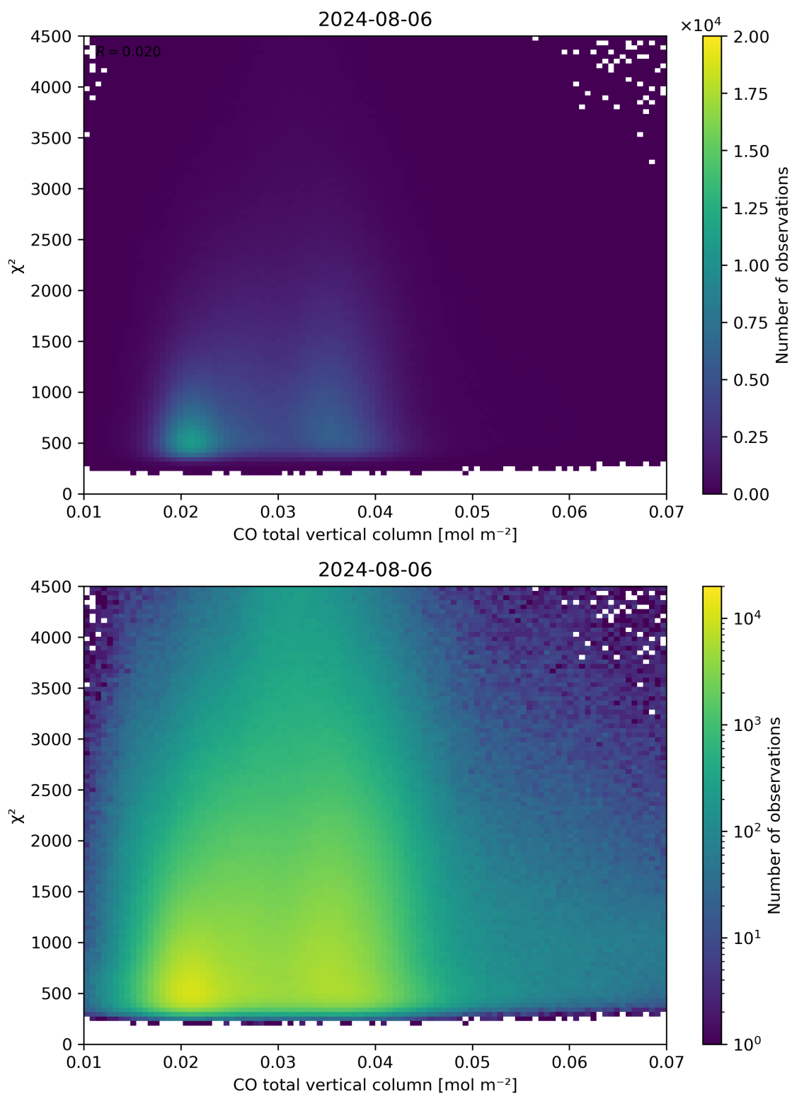
Figure 35: Scatter density plot of “CO total vertical column” against “ \chi^2 ” for 2024-08-06 to 2024-08-07.
