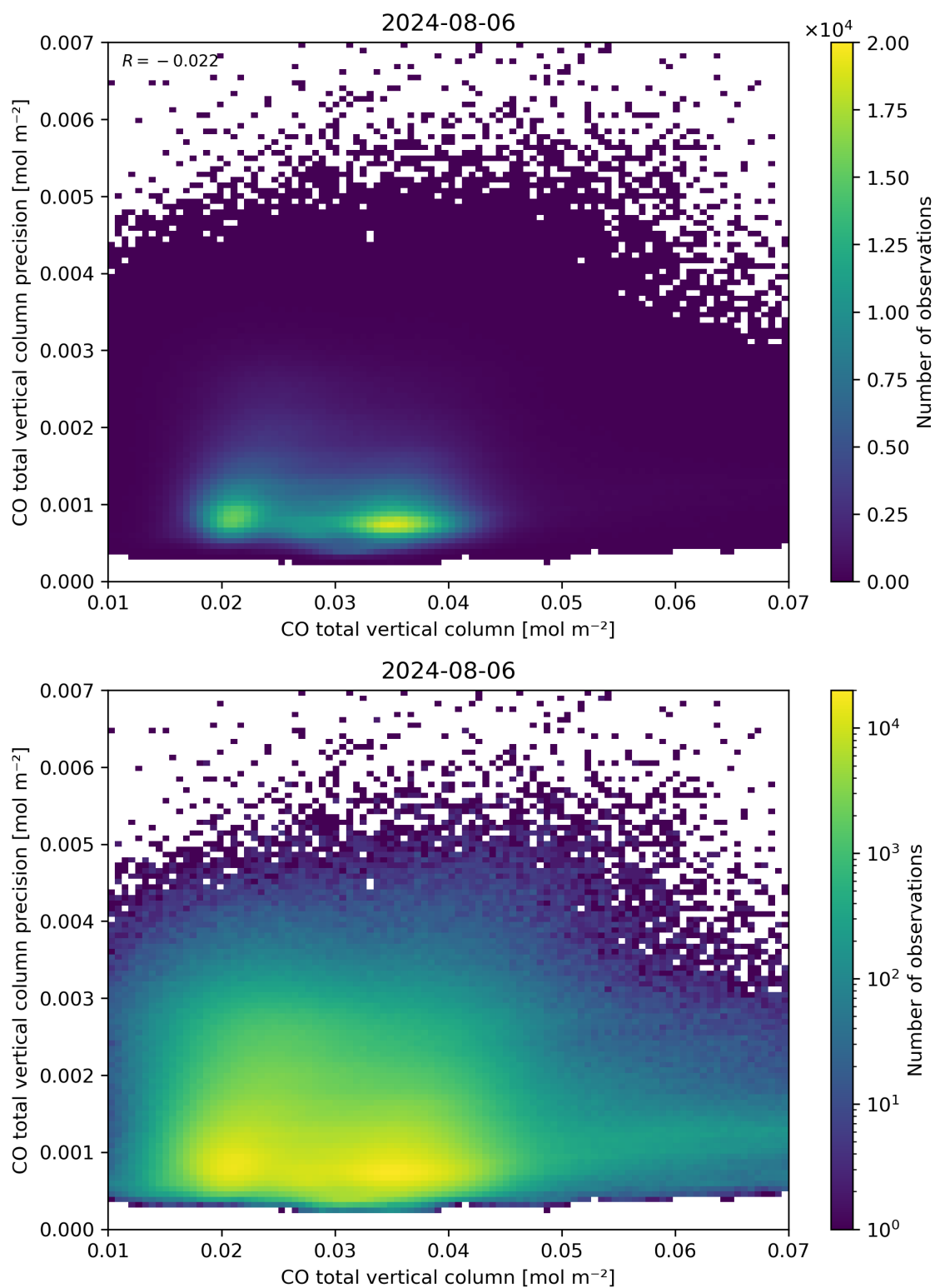
Figure 34: Scatter density plot of “CO total vertical column” against “CO total vertical column precision” for 2024-08-06 to 2024-08-07.
