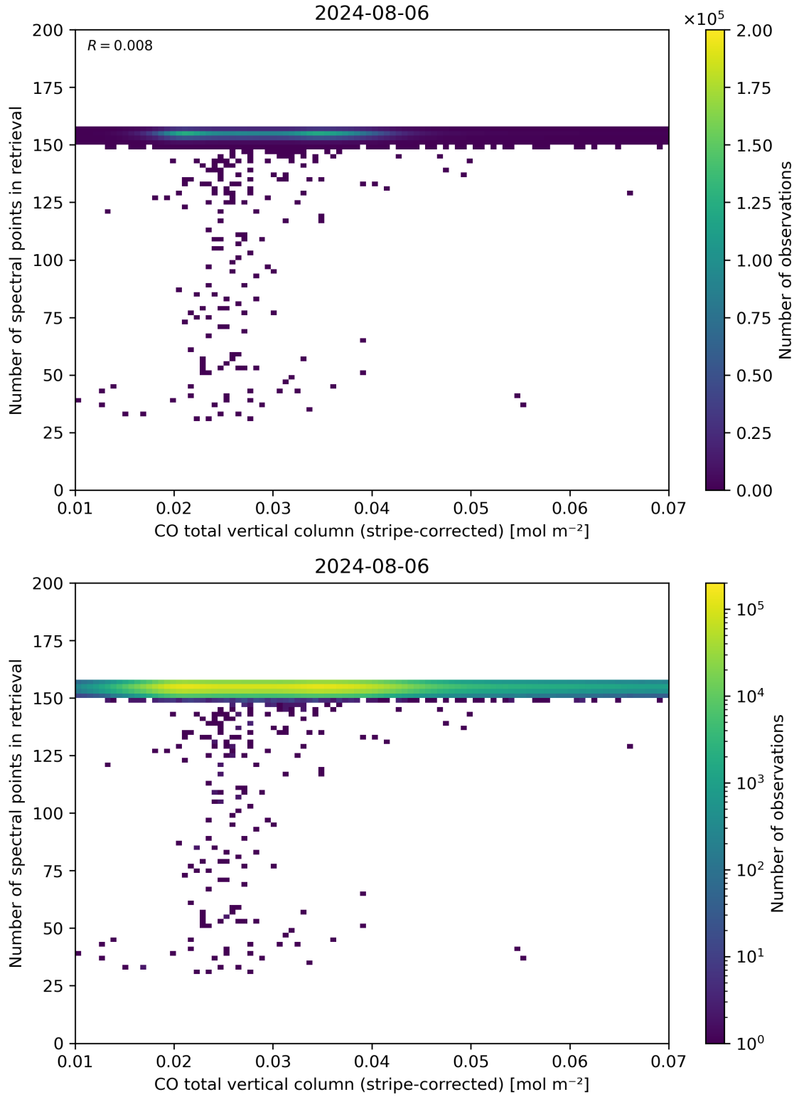
Figure 40: Scatter density plot of “CO total vertical column (stripe-corrected)” against “Number of spectral points in retrieval” for 2024-08-06 to 2024-08-07.
