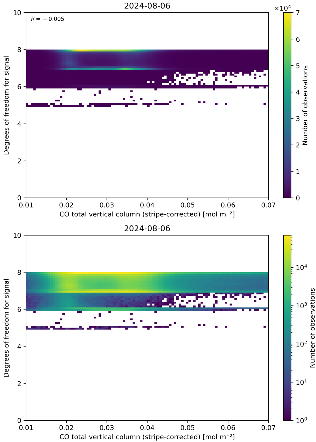
Figure 38: Scatter density plot of “CO total vertical column (stripe-corrected)” against “Degrees of freedom for signal” for 2024-08-06 to 2024-08-07.
