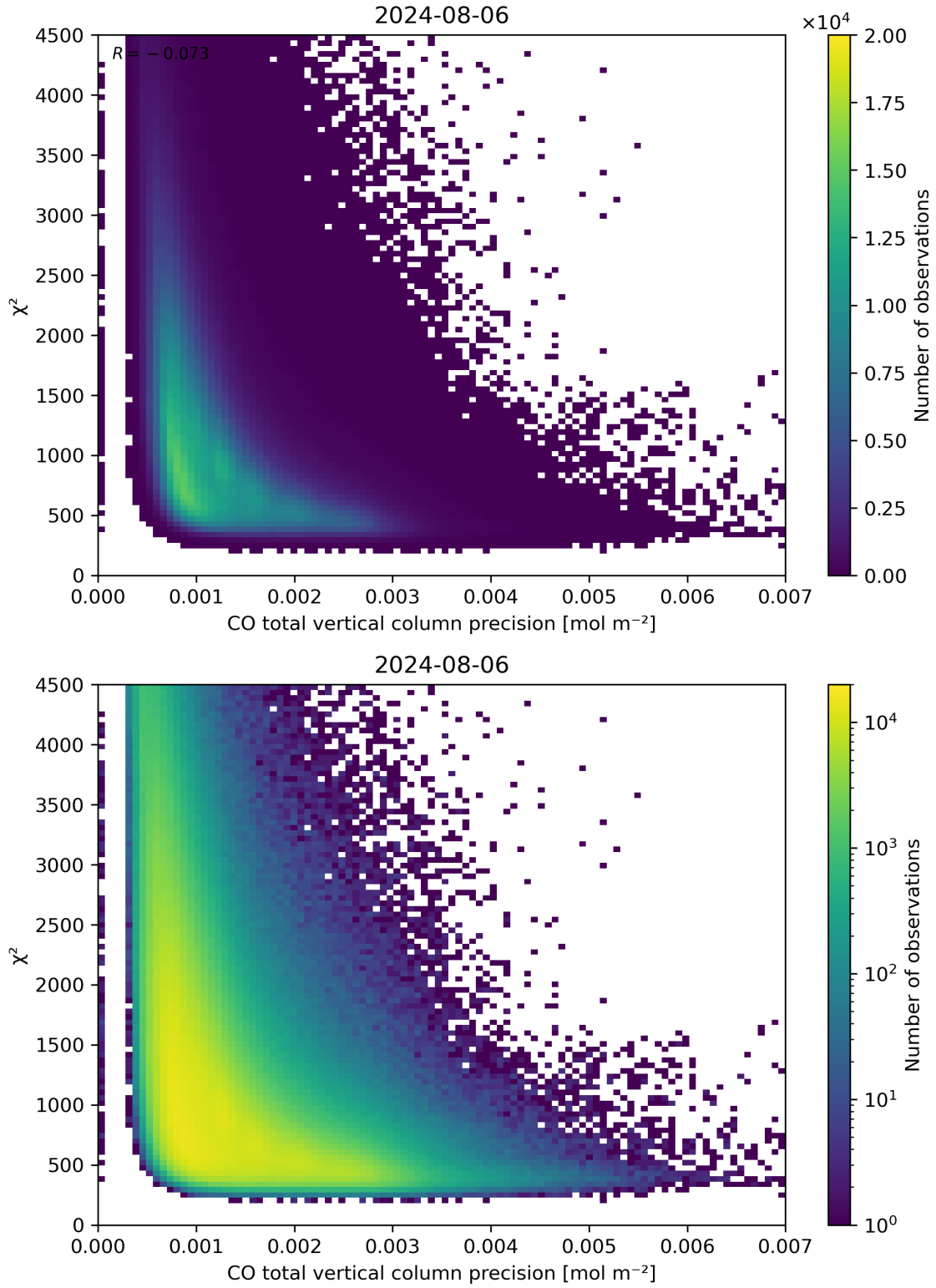
Figure 44: Scatter density plot of “CO total vertical column precision” against “ \chi^2 ” for 2024-08-06 to 2024-08-07.
