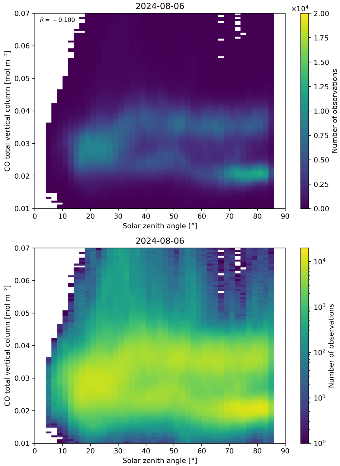
Figure 61: Scatter density plot of “Solar zenith angle” against “CO total vertical column” for 2024-08-06 to 2024-08-07.
