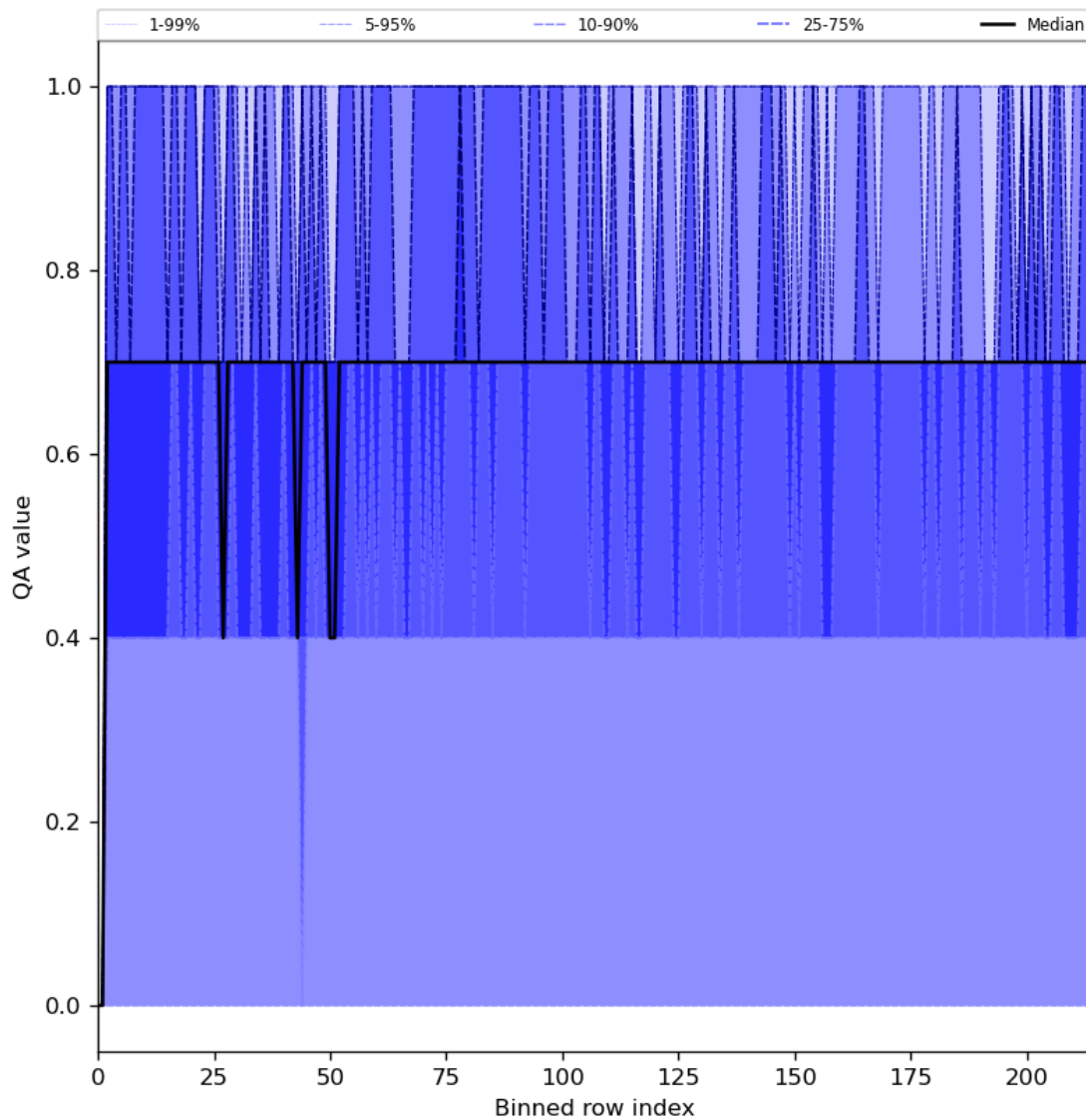
Figure 25: Along track statistics of “QA value” for 2024-08-06 to 2024-08-07
