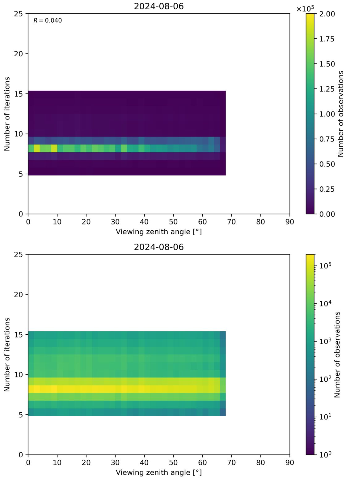
Figure 75: Scatter density plot of “Viewing zenith angle” against “Number of iterations” for 2024-08-06 to 2024-08-07.
