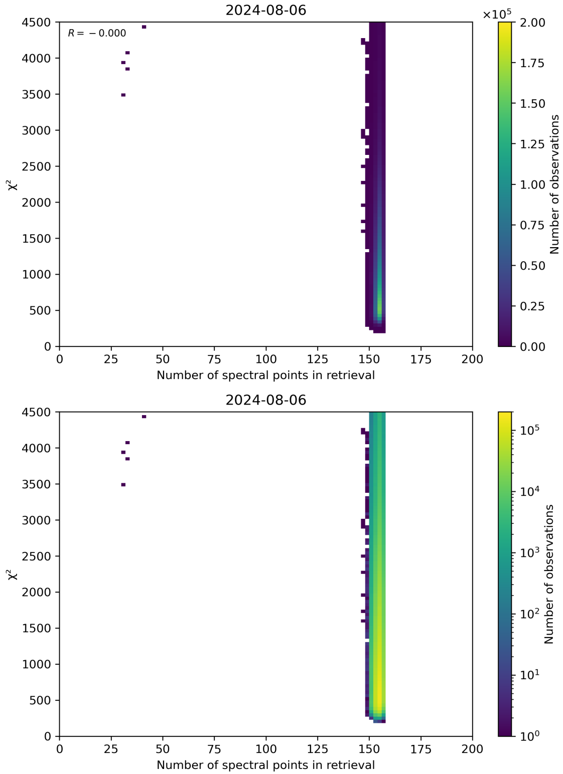
Figure 58: Scatter density plot of “Number of spectral points in retrieval” against “ \chi^2 ” for 2024-08-06 to 2024-08-07.
