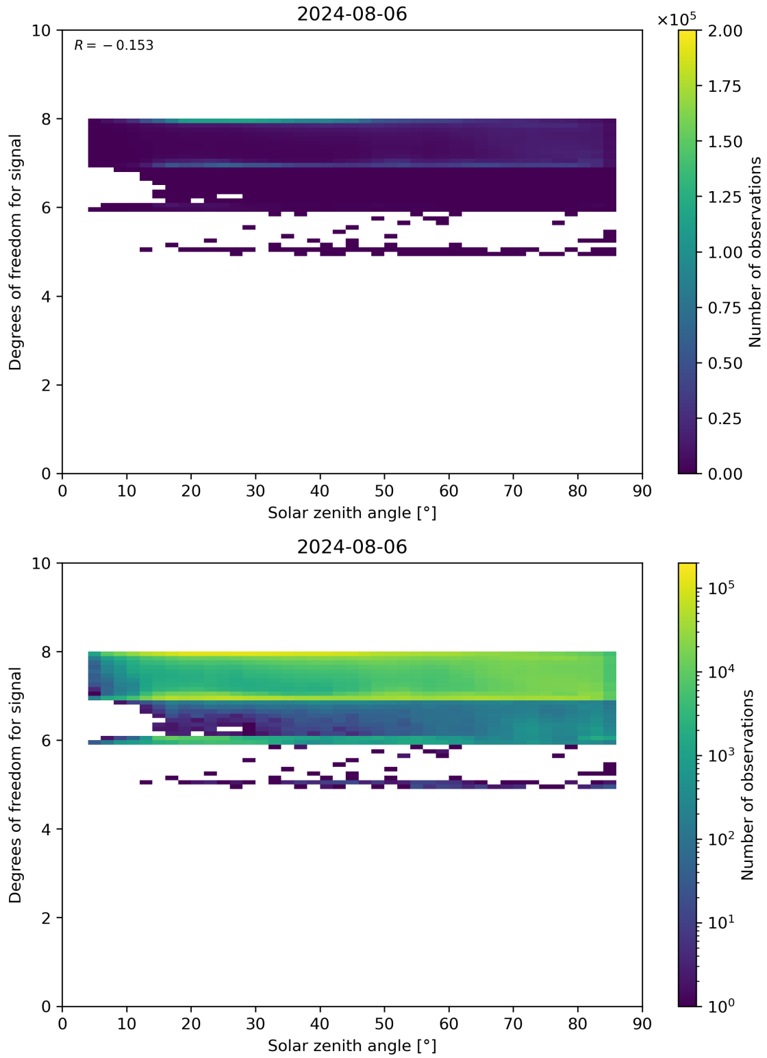
Figure 65: Scatter density plot of “Solar zenith angle” against “Degrees of freedom for signal” for 2024-08-06 to 2024-08-07.
