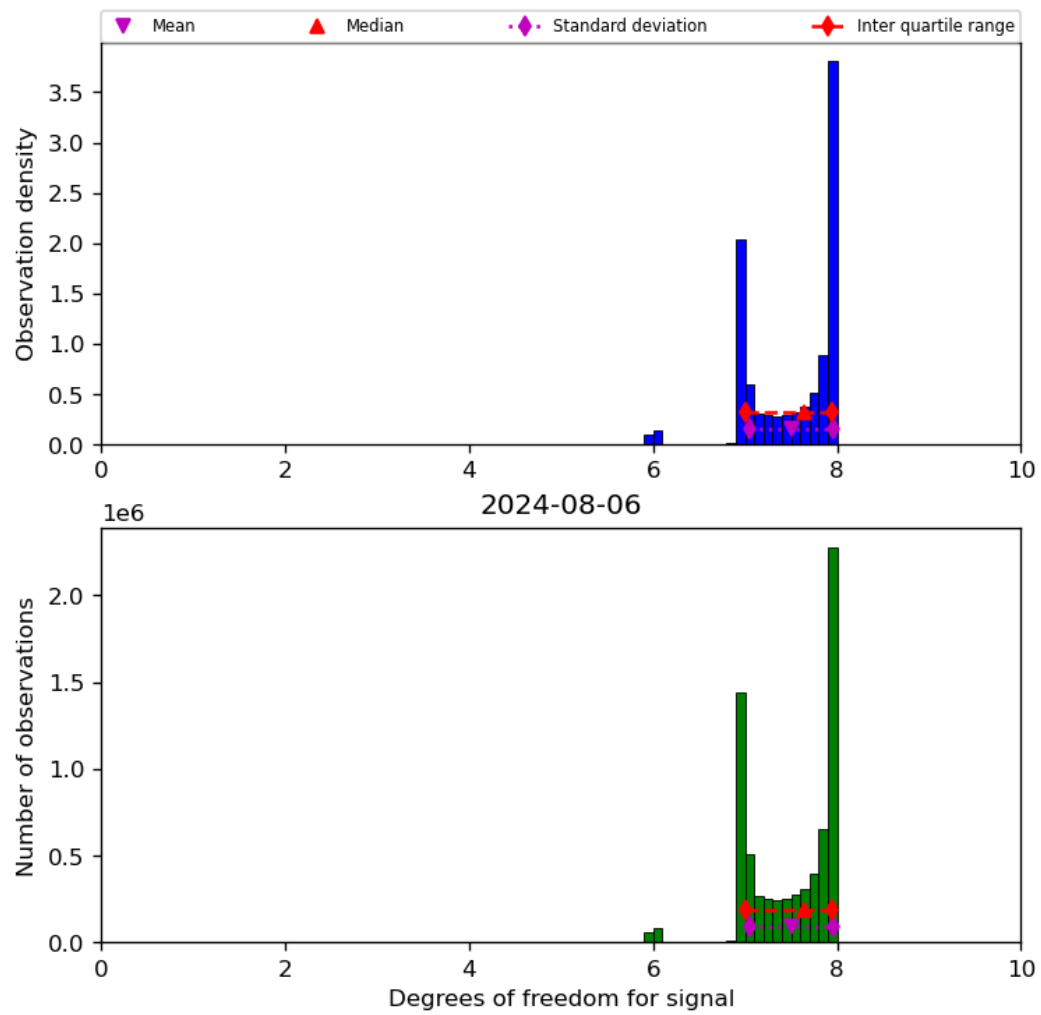
Figure 23: Histogram of “Degrees of freedom for signal” for 2024-08-06 to 2024-08-07
