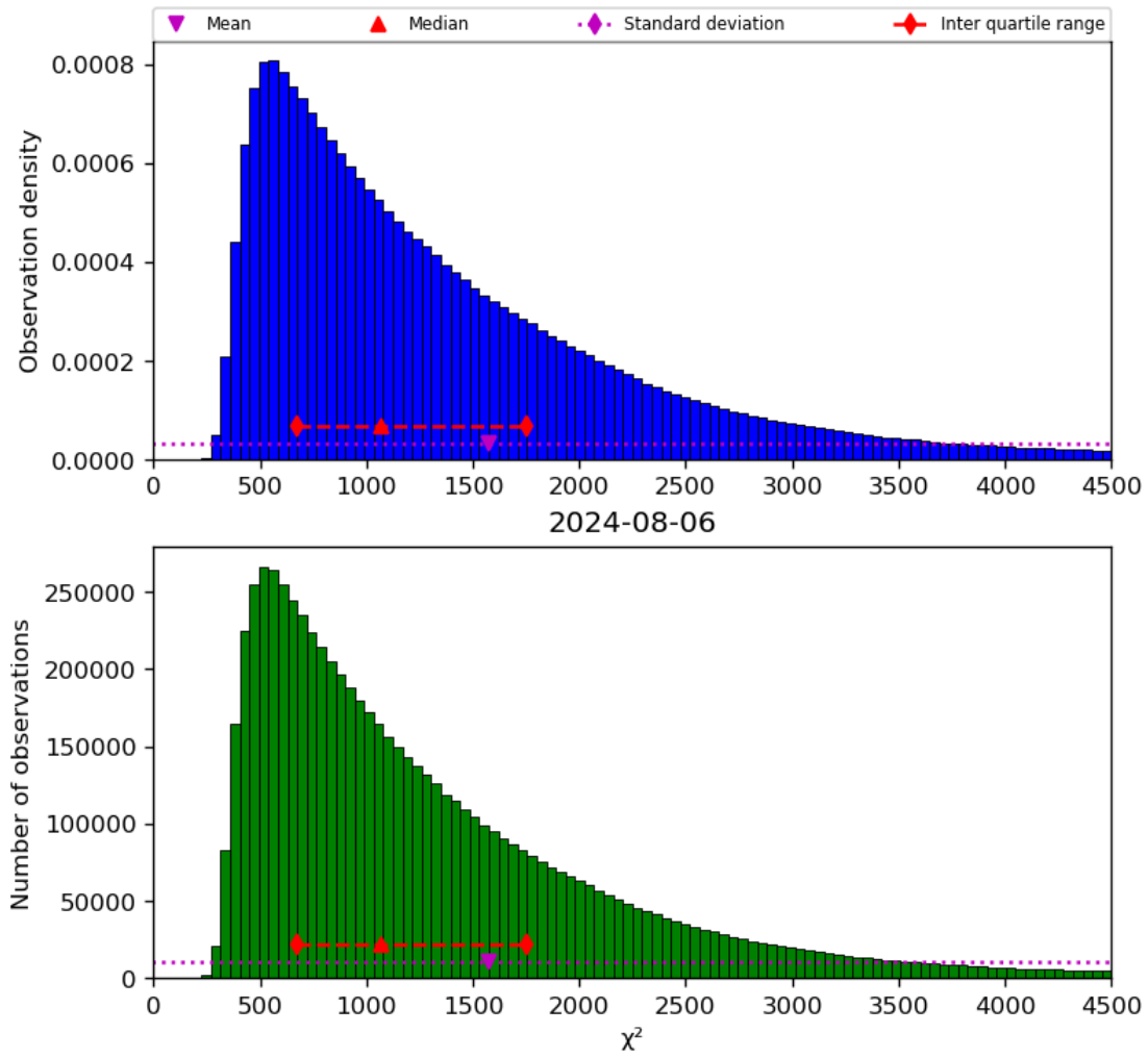
Figure 22: Histogram of “ \chi^2 ” for 2024-08-06 to 2024-08-07
