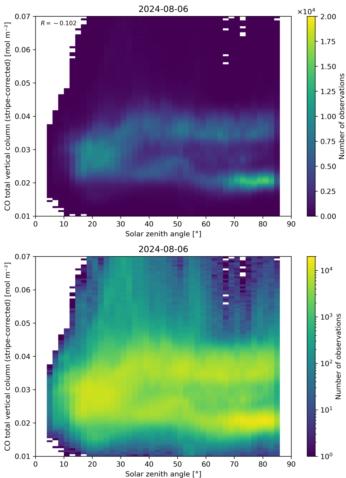
Figure 62: Scatter density plot of “Solar zenith angle” against “CO total vertical column (stripe-corrected)” for 2024-08-06 to 2024-08-07.
