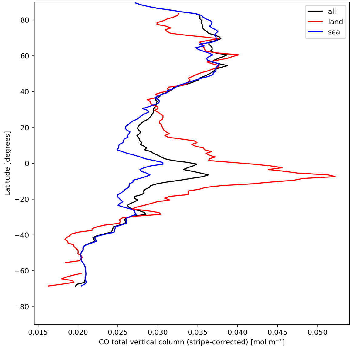
Figure 11: Zonal average of “CO total vertical column (stripe-corrected)” for 2024-08-06 to 2024-08-07.
