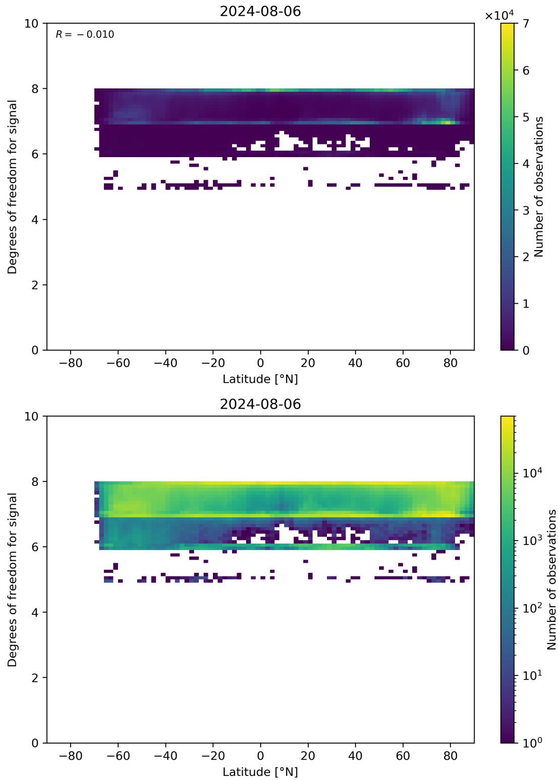
Figure 55: Scatter density plot of “Latitude” against “Degrees of freedom for signal” for 2024-08-06 to 2024-08-07.
