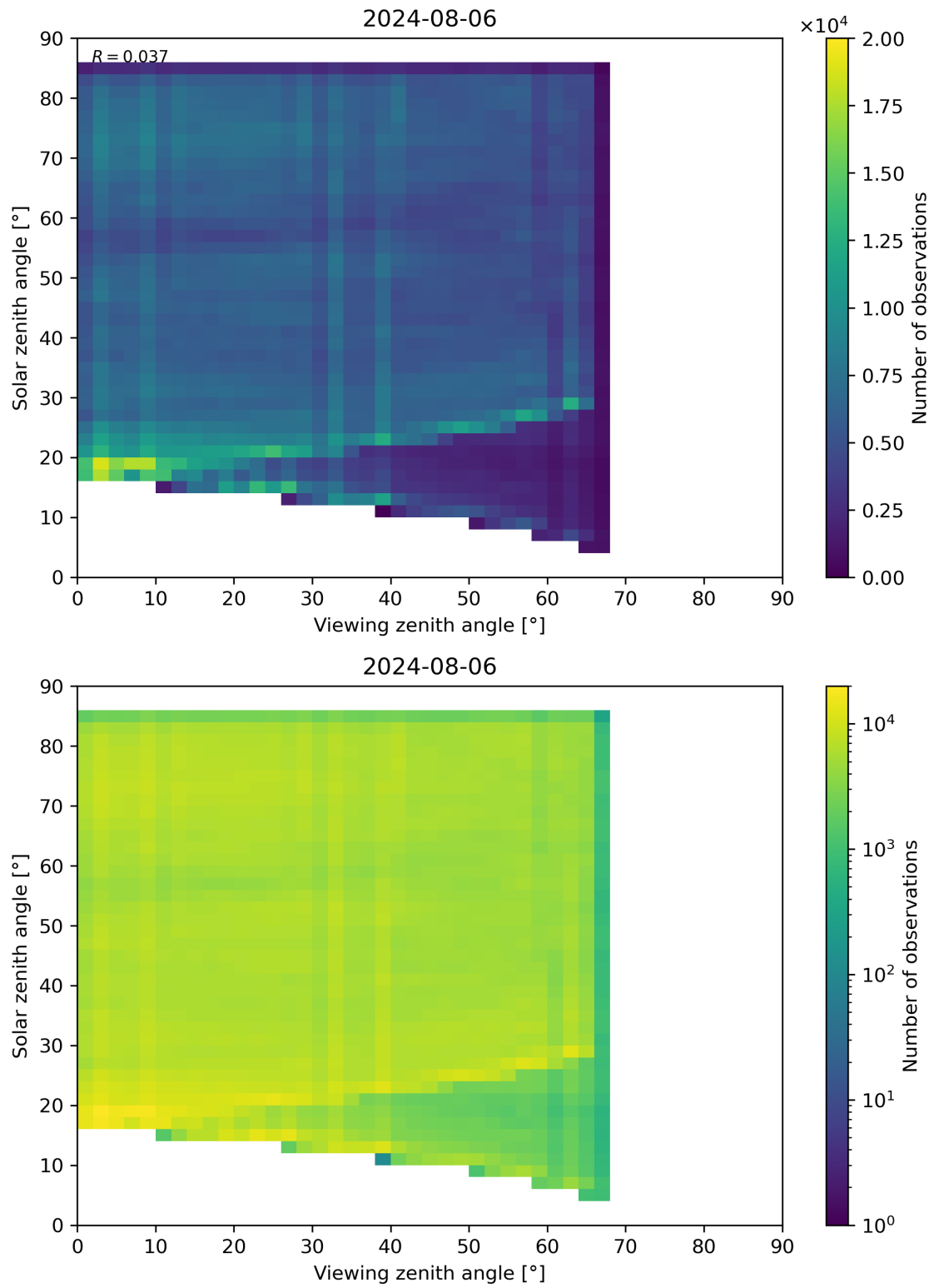
Figure 77: Scatter density plot of “Viewing zenith angle” against “Solar zenith angle” for 2024-08-06 to 2024-08-07.
