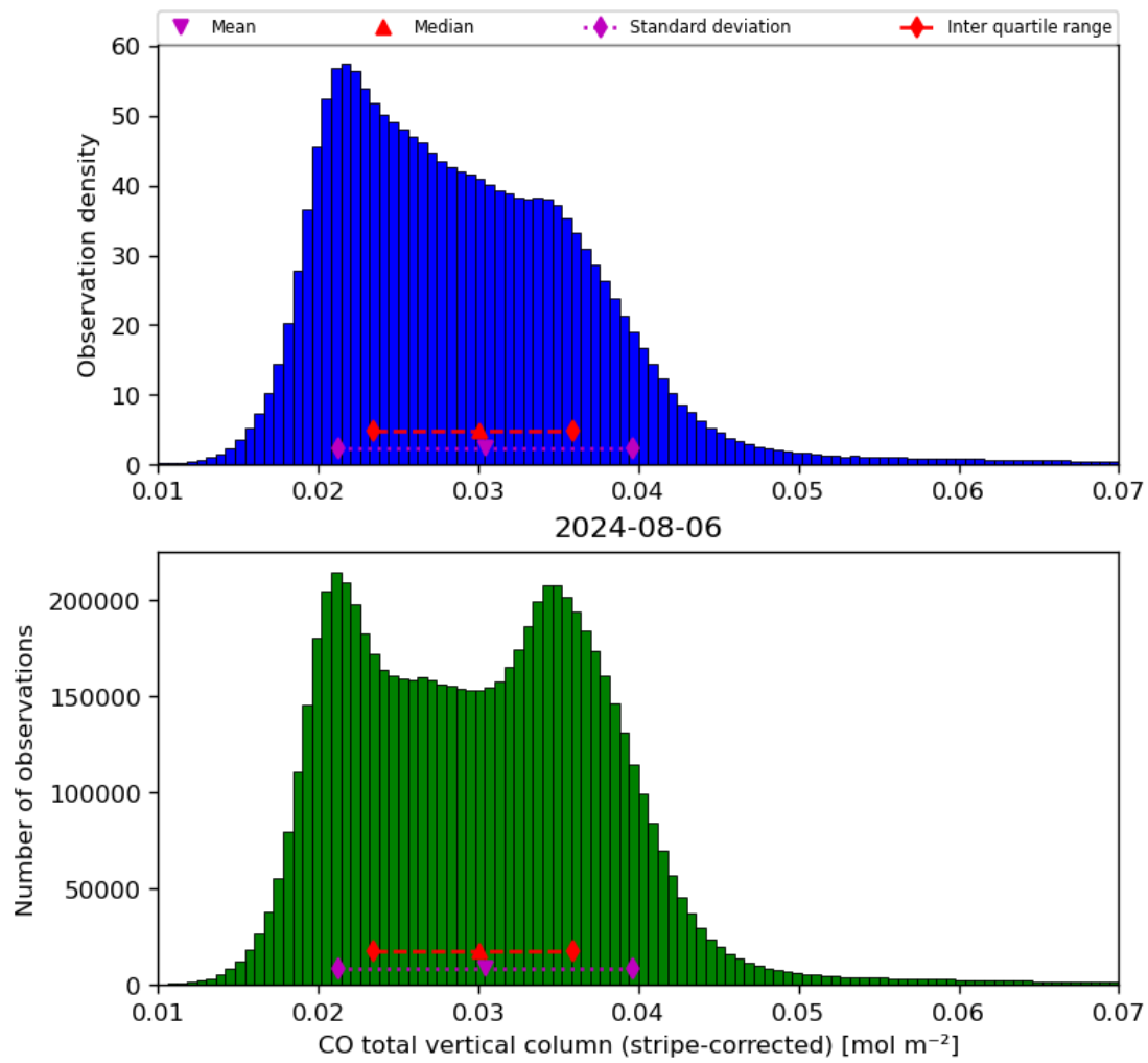
Figure 19: Histogram of “CO total vertical column (stripe-corrected)” for 2024-08-06 to 2024-08-07
