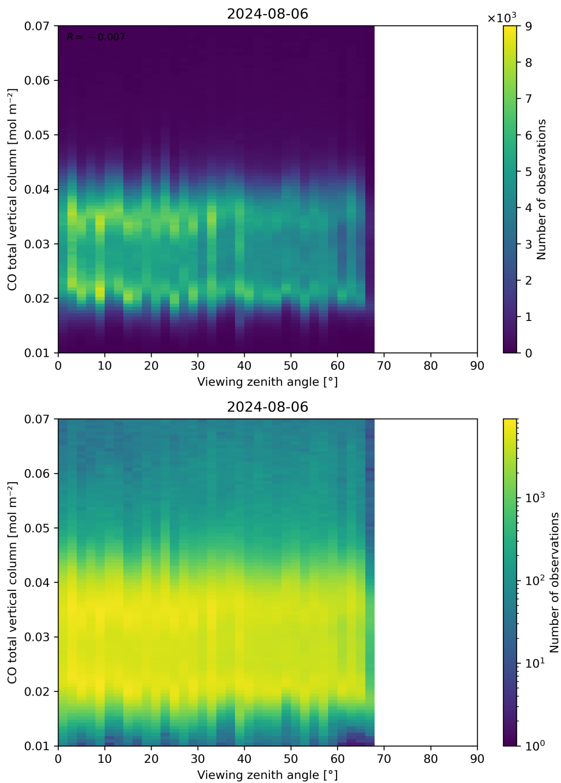
Figure 69: Scatter density plot of “Viewing zenith angle” against “CO total vertical column” for 2024-08-06 to 2024-08-07.
