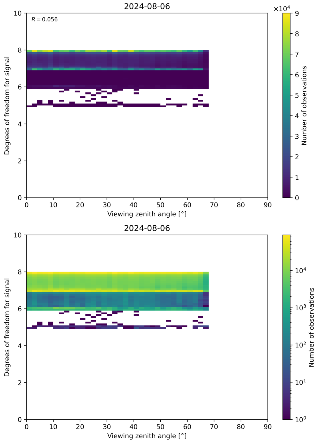
Figure 73: Scatter density plot of “Viewing zenith angle” against “Degrees of freedom for signal” for 2024-08-06 to 2024-08-07.
