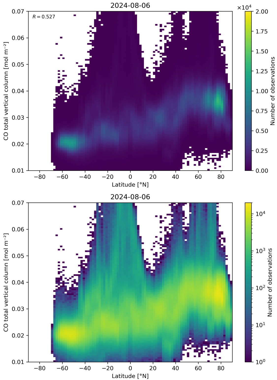
Figure 51: Scatter density plot of “Latitude” against “CO total vertical column” for 2024-08-06 to 2024-08-07.
