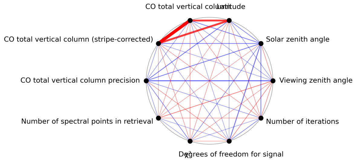
Figure 1: Map of correlation graph for 2024-08-06 to 2024-08-07.
