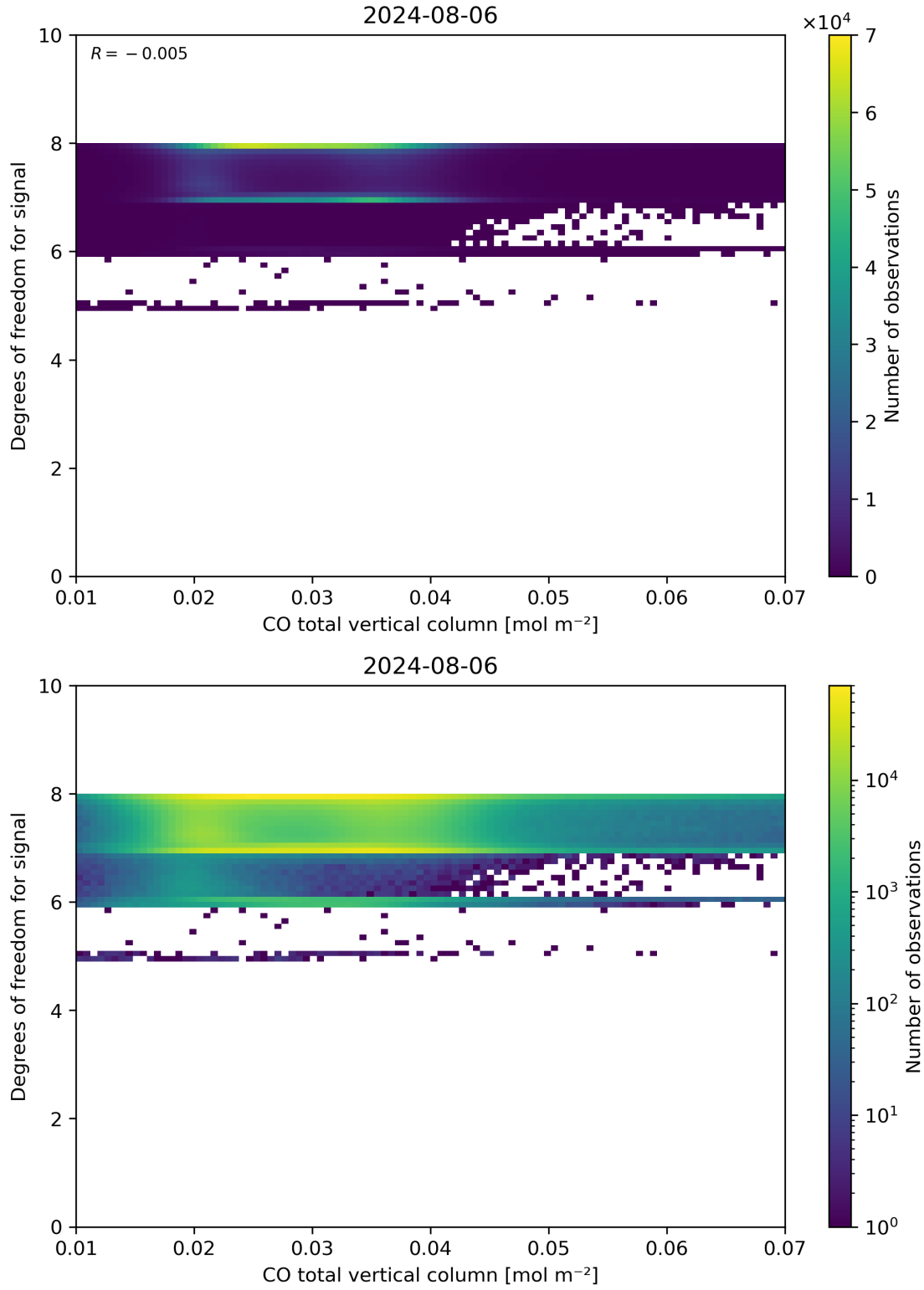
Figure 41: Scatter density plot of “CO total vertical column” against “Degrees of freedom for signal” for 2024-08-06 to 2024-08-07.
