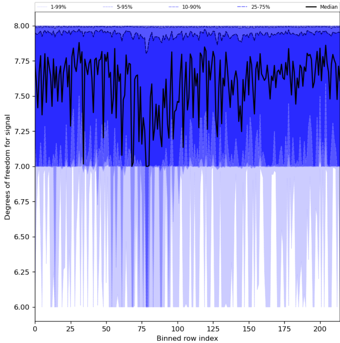
Figure 31: Along track statistics of “Degrees of freedom for signal” for 2024-08-06 to 2024-08-07
