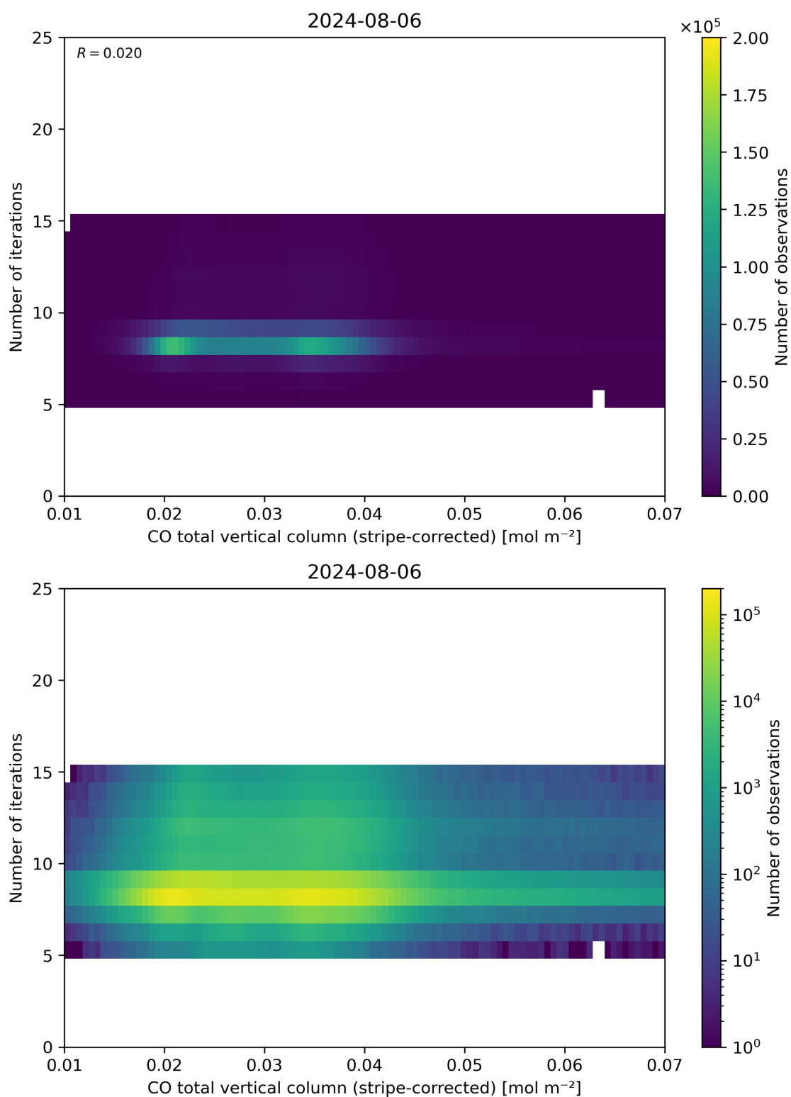
Figure 39: Scatter density plot of “CO total vertical column (stripe-corrected)” against “Number of iterations” for 2024-08-06 to 2024-08-07.
