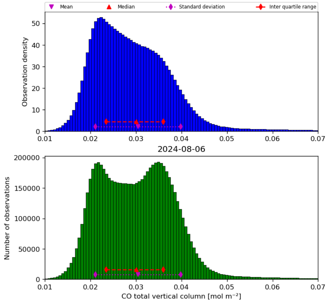
Figure 18: Histogram of “CO total vertical column” for 2024-08-06 to 2024-08-07
