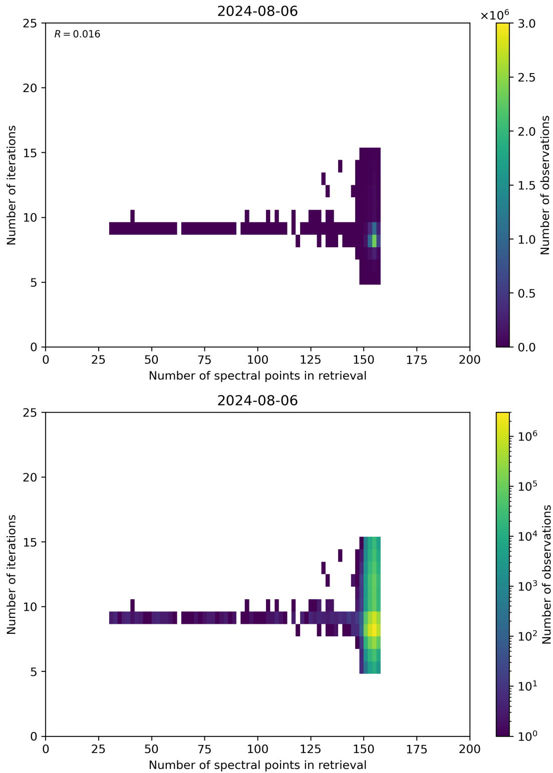
Figure 60: Scatter density plot of “Number of spectral points in retrieval” against “Number of iterations” for 2024-08-06 to 2024-08-07.
