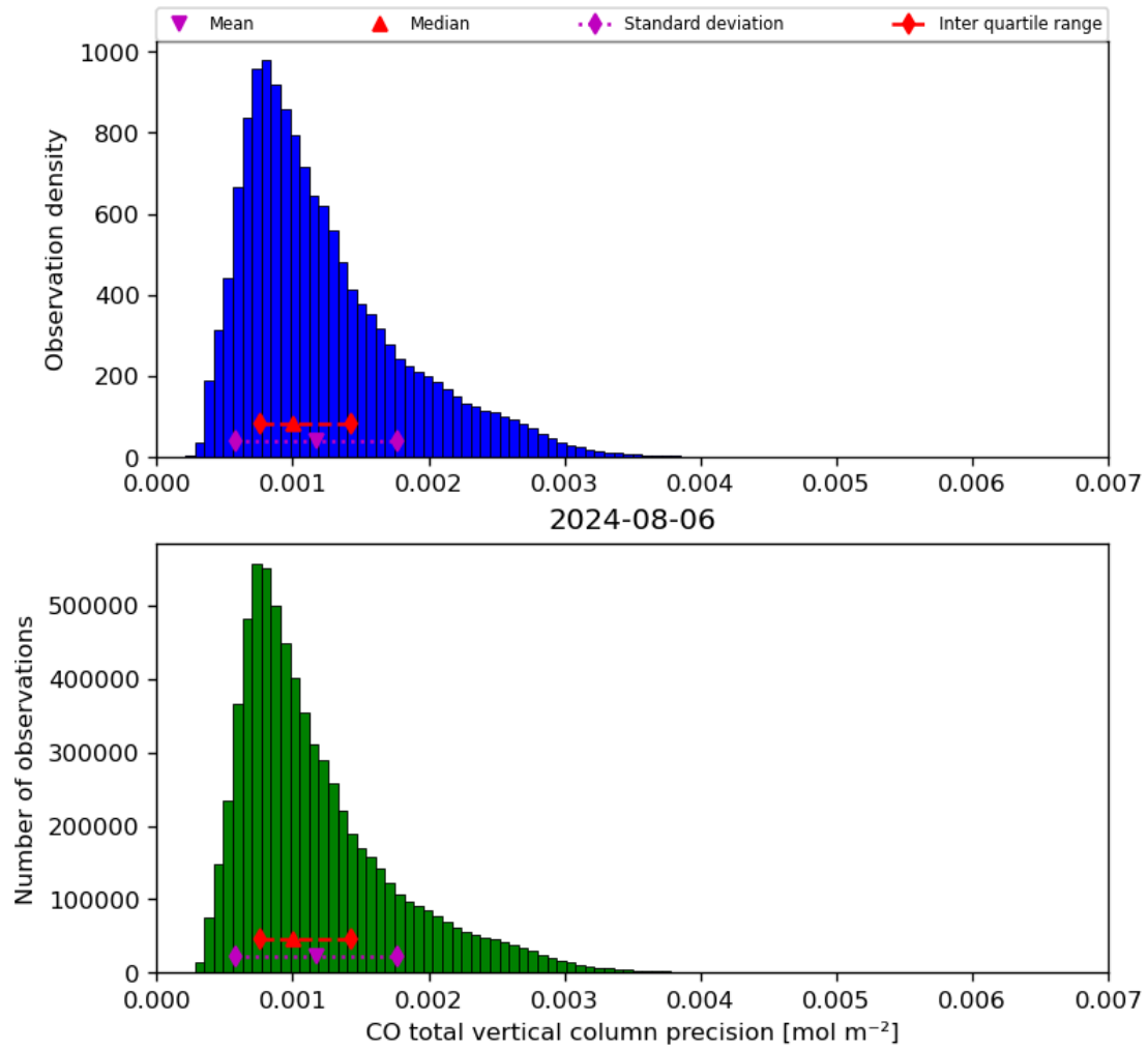
Figure 20: Histogram of “CO total vertical column precision” for 2024-08-06 to 2024-08-07
