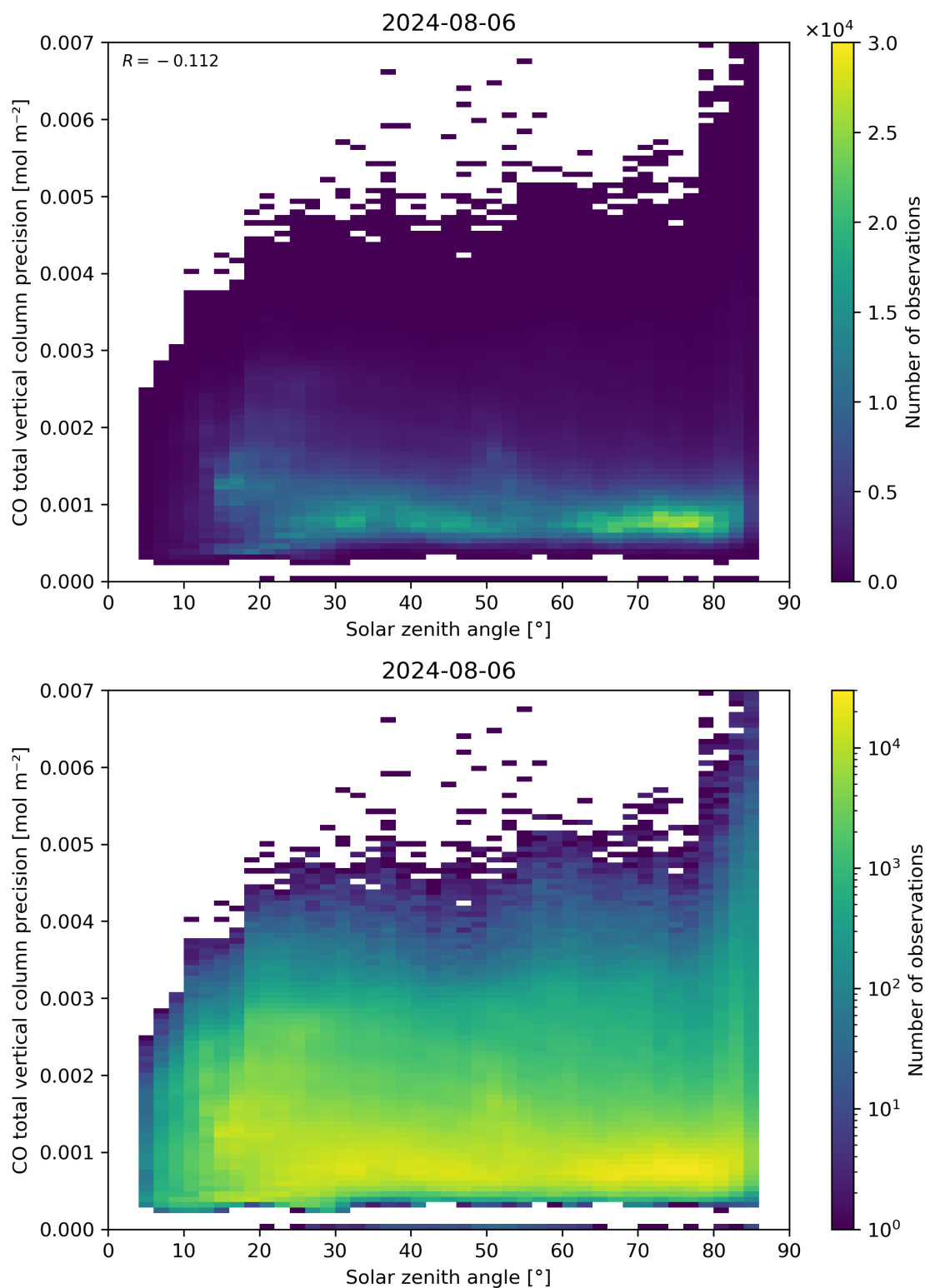
Figure 63: Scatter density plot of “Solar zenith angle” against “CO total vertical column precision” for 2024-08-06 to 2024-08-07.
