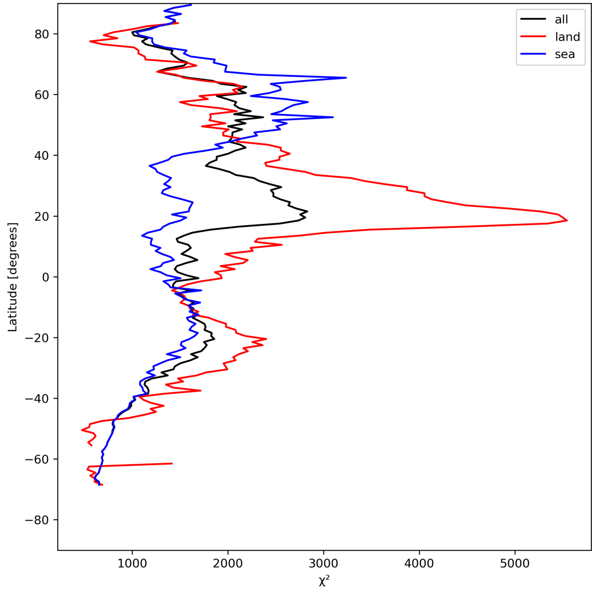
Figure 14: Zonal average of “ \chi^2 ” for 2024-08-06 to 2024-08-07.
