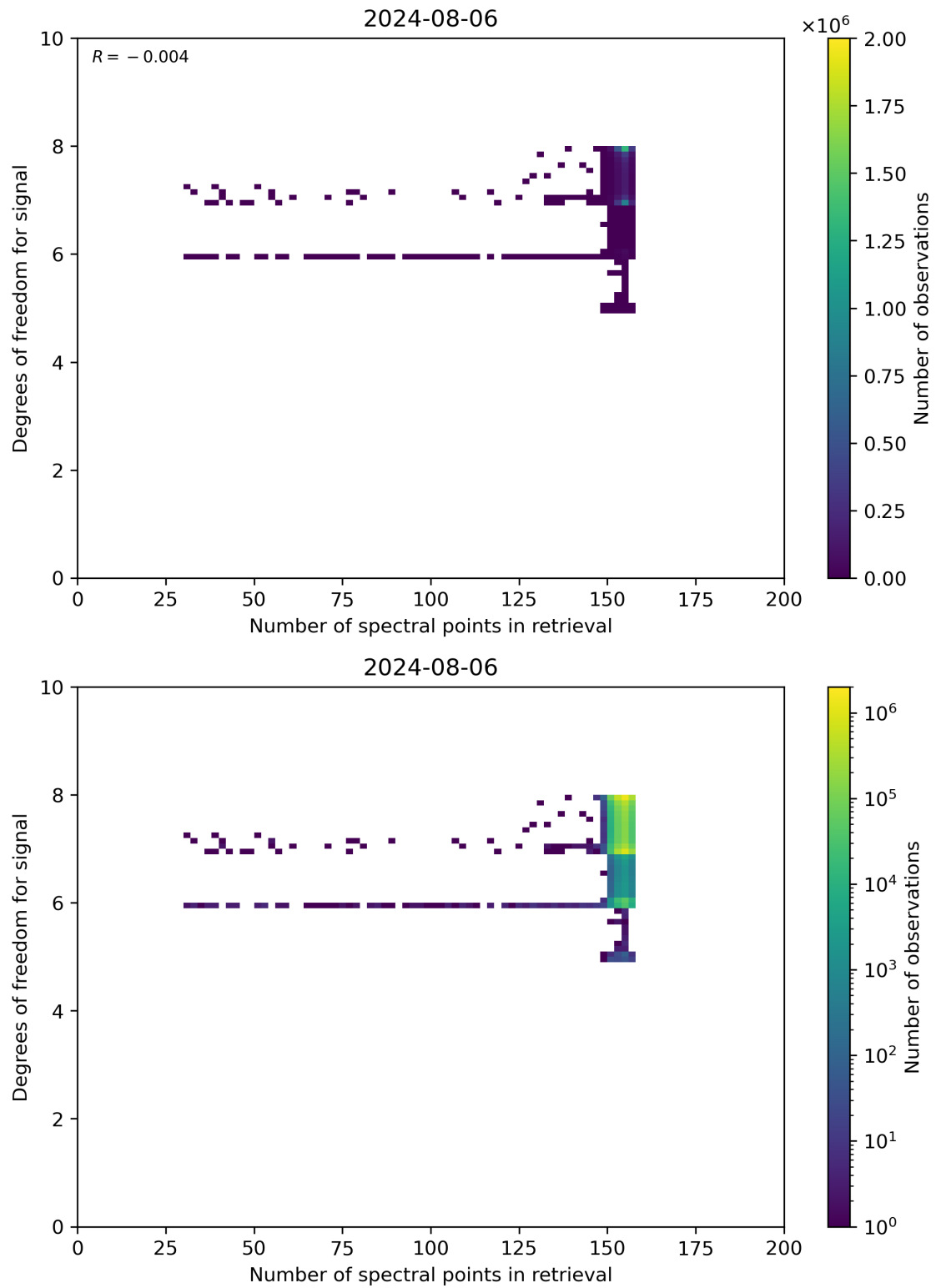
Figure 59: Scatter density plot of “Number of spectral points in retrieval” against “Degrees of freedom for signal” for 2024-08-06 to 2024-08-07.
