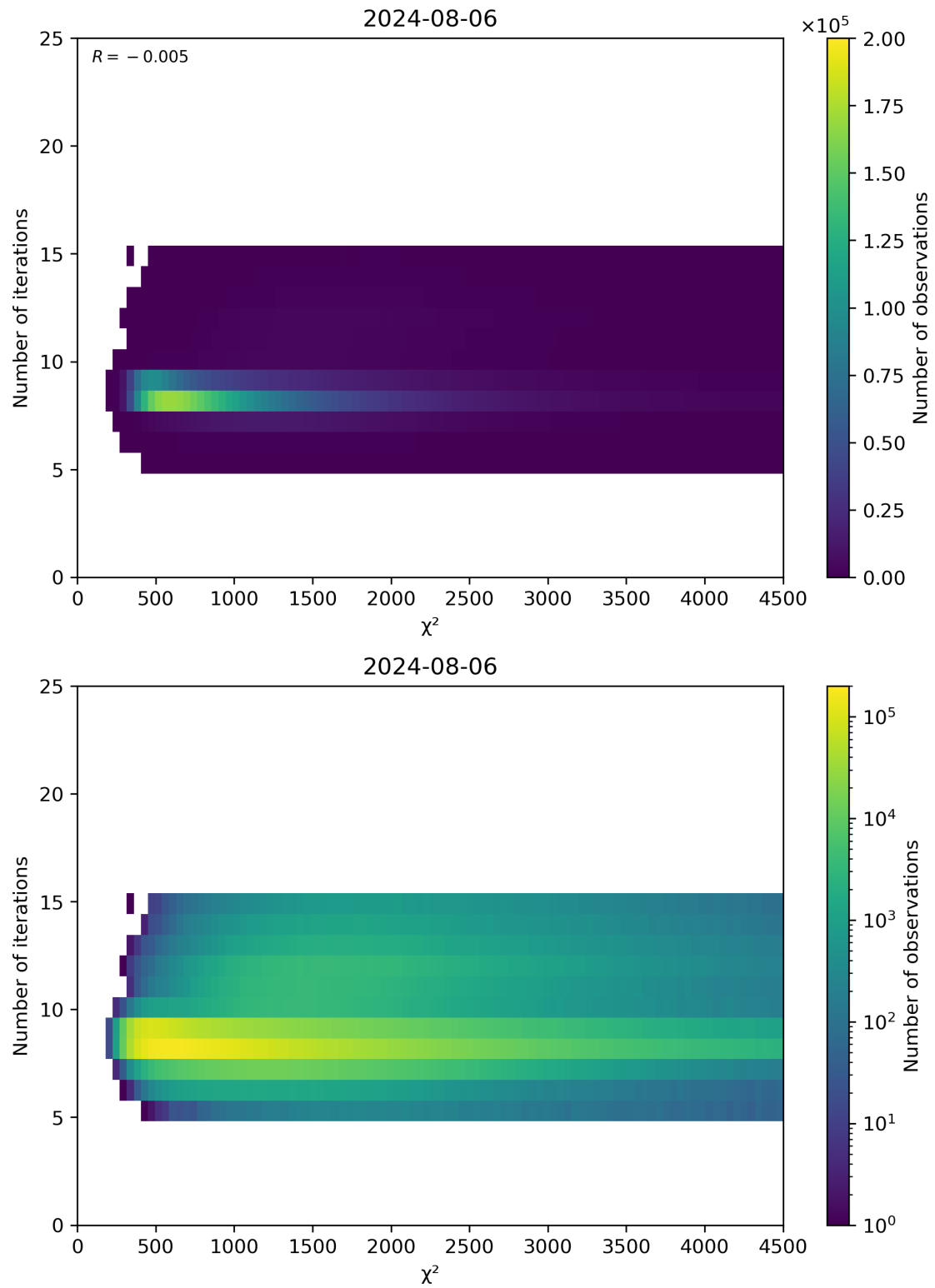
Figure 49: Scatter density plot of “ \chi^2 ” against “Number of iterations” for 2024-08-06 to 2024-08-07.
