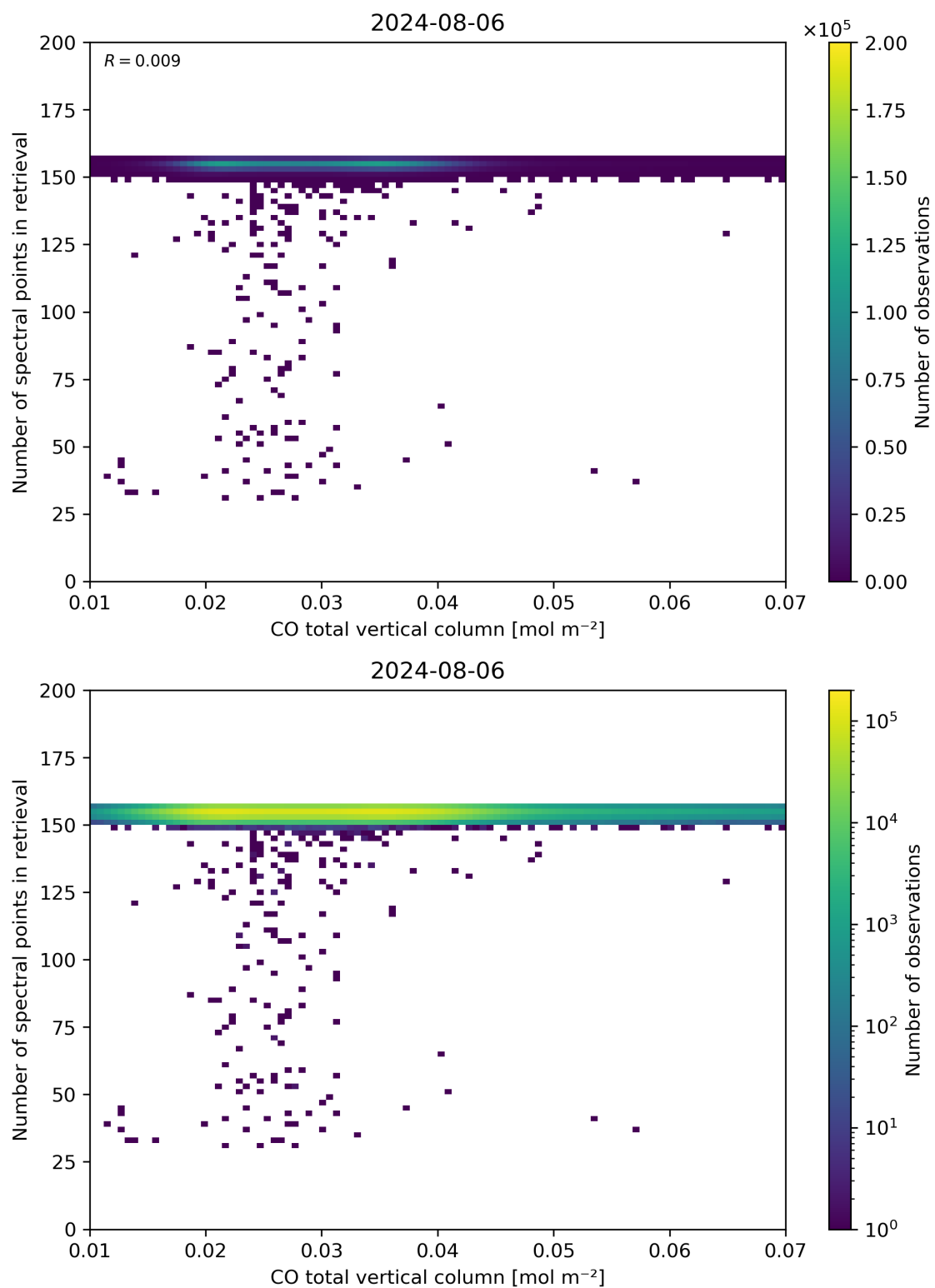
Figure 43: Scatter density plot of “CO total vertical column” against “Number of spectral points in retrieval” for 2024-08-06 to 2024-08-07.
