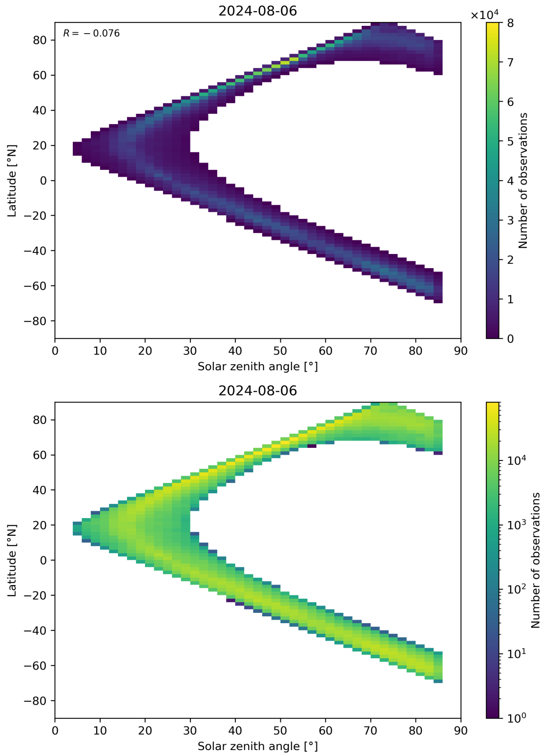
Figure 66: Scatter density plot of “Solar zenith angle” against “Latitude” for 2024-08-06 to 2024-08-07.
