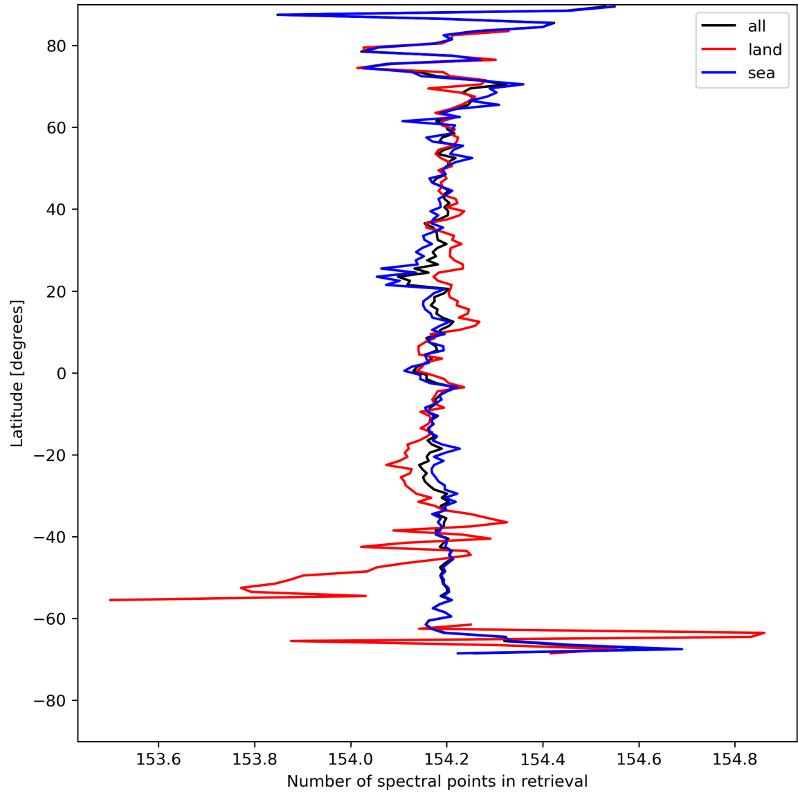
Figure 13: Zonal average of “Number of spectral points in retrieval” for 2024-08-06 to 2024-08-07.
