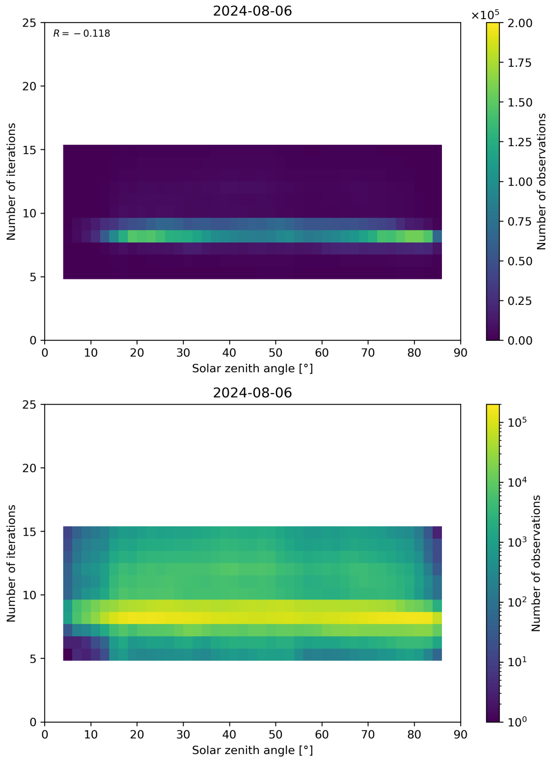
Figure 67: Scatter density plot of “Solar zenith angle” against “Number of iterations” for 2024-08-06 to 2024-08-07.
