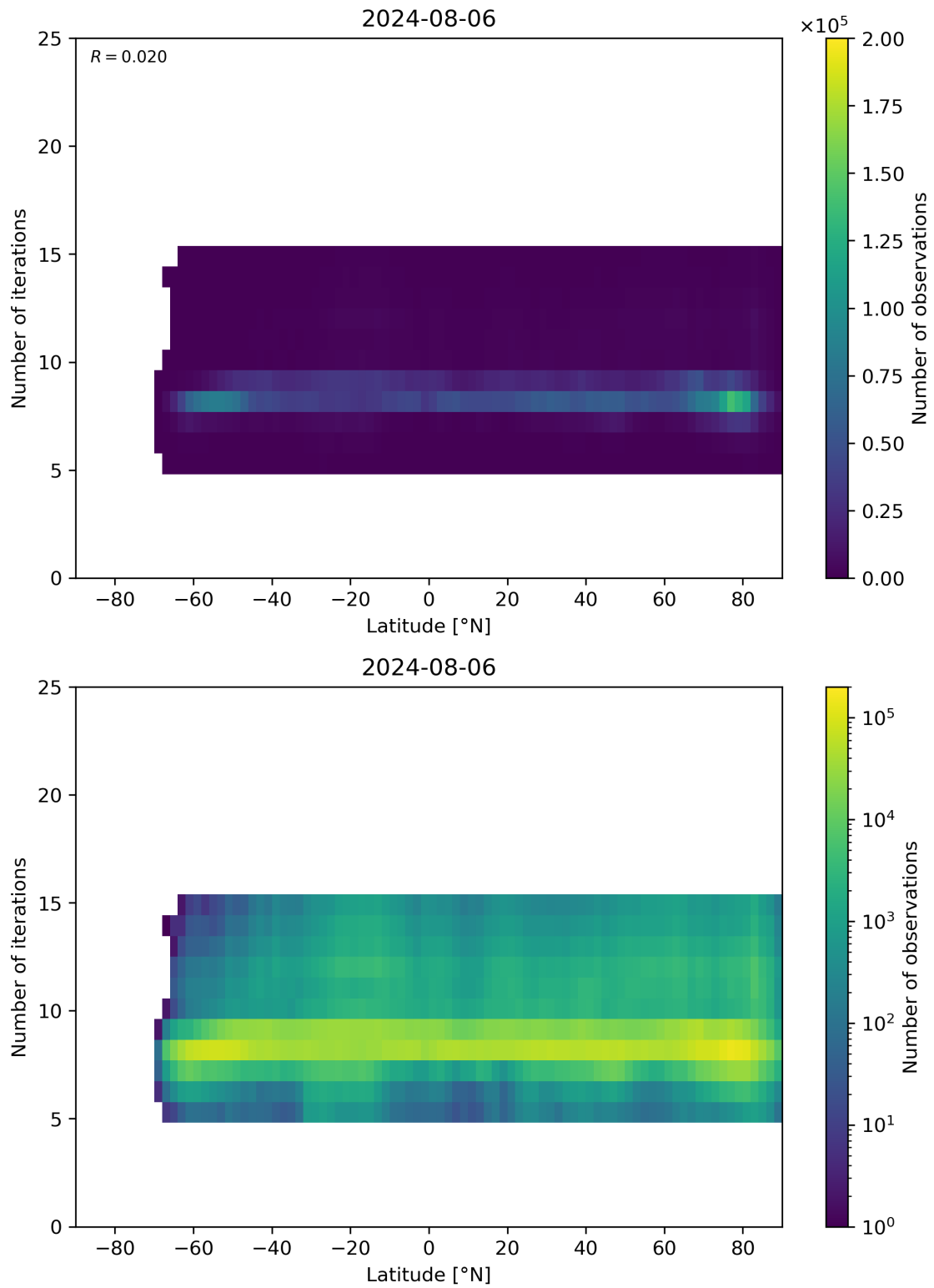
Figure 56: Scatter density plot of “Latitude” against “Number of iterations” for 2024-08-06 to 2024-08-07.
