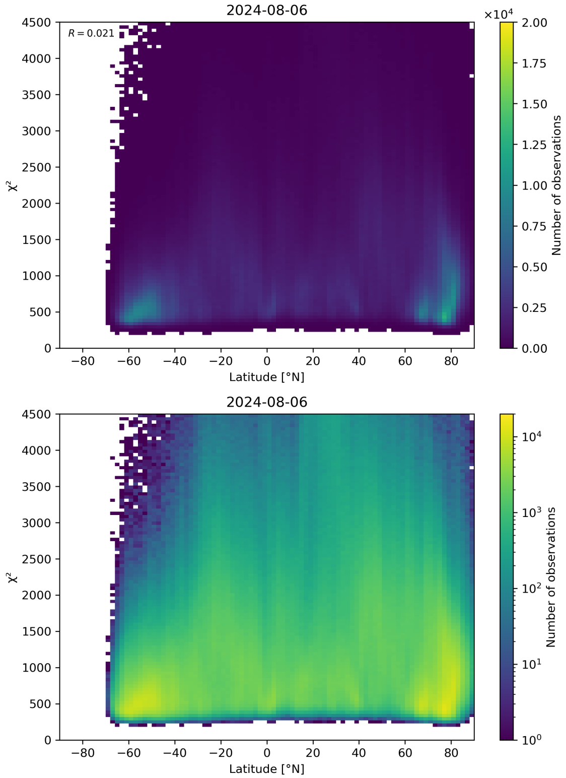
Figure 54: Scatter density plot of “Latitude” against “ \chi^2 ” for 2024-08-06 to 2024-08-07.
