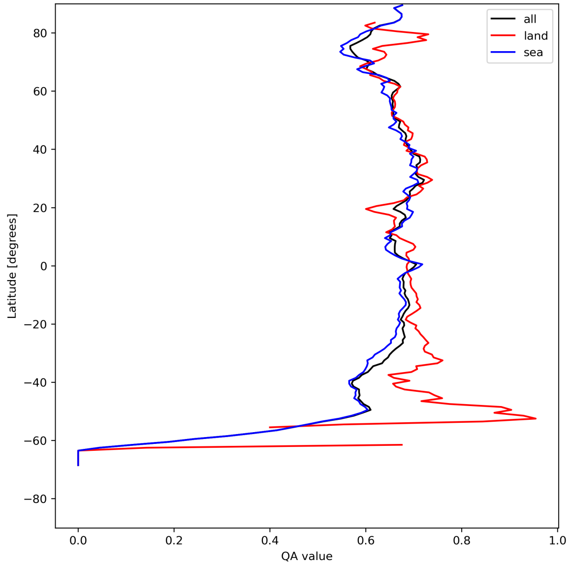
Figure 9: Zonal average of “QA value” for 2024-08-06 to 2024-08-07.
