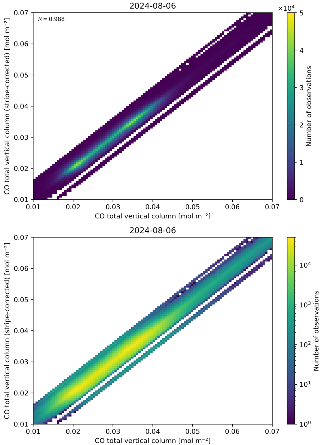
Figure 33: Scatter density plot of “CO total vertical column” against “CO total vertical column (stripe-corrected)” for 2024-08-06 to 2024-08-07.
