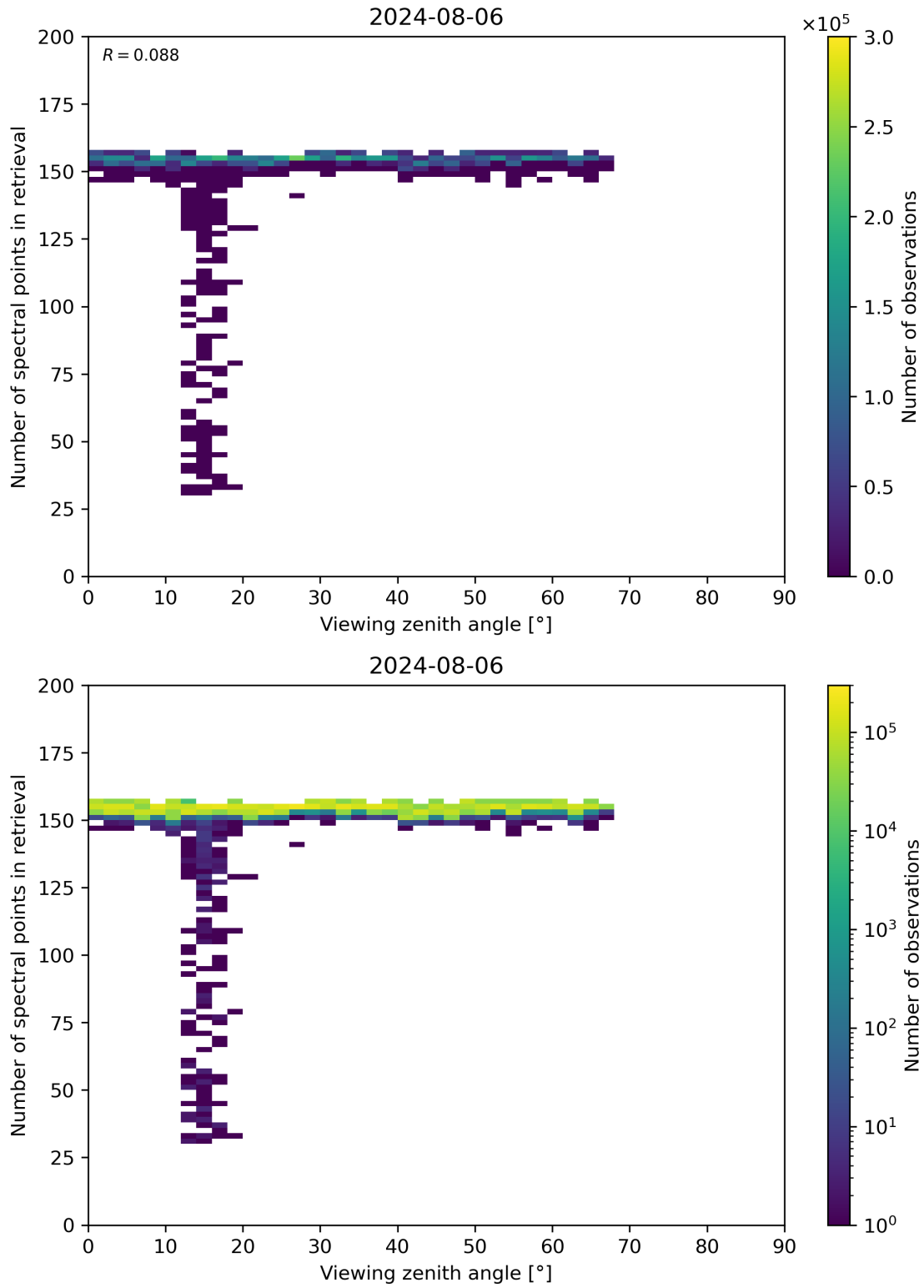
Figure 76: Scatter density plot of “Viewing zenith angle” against “Number of spectral points in retrieval” for 2024-08-06 to 2024-08-07.
