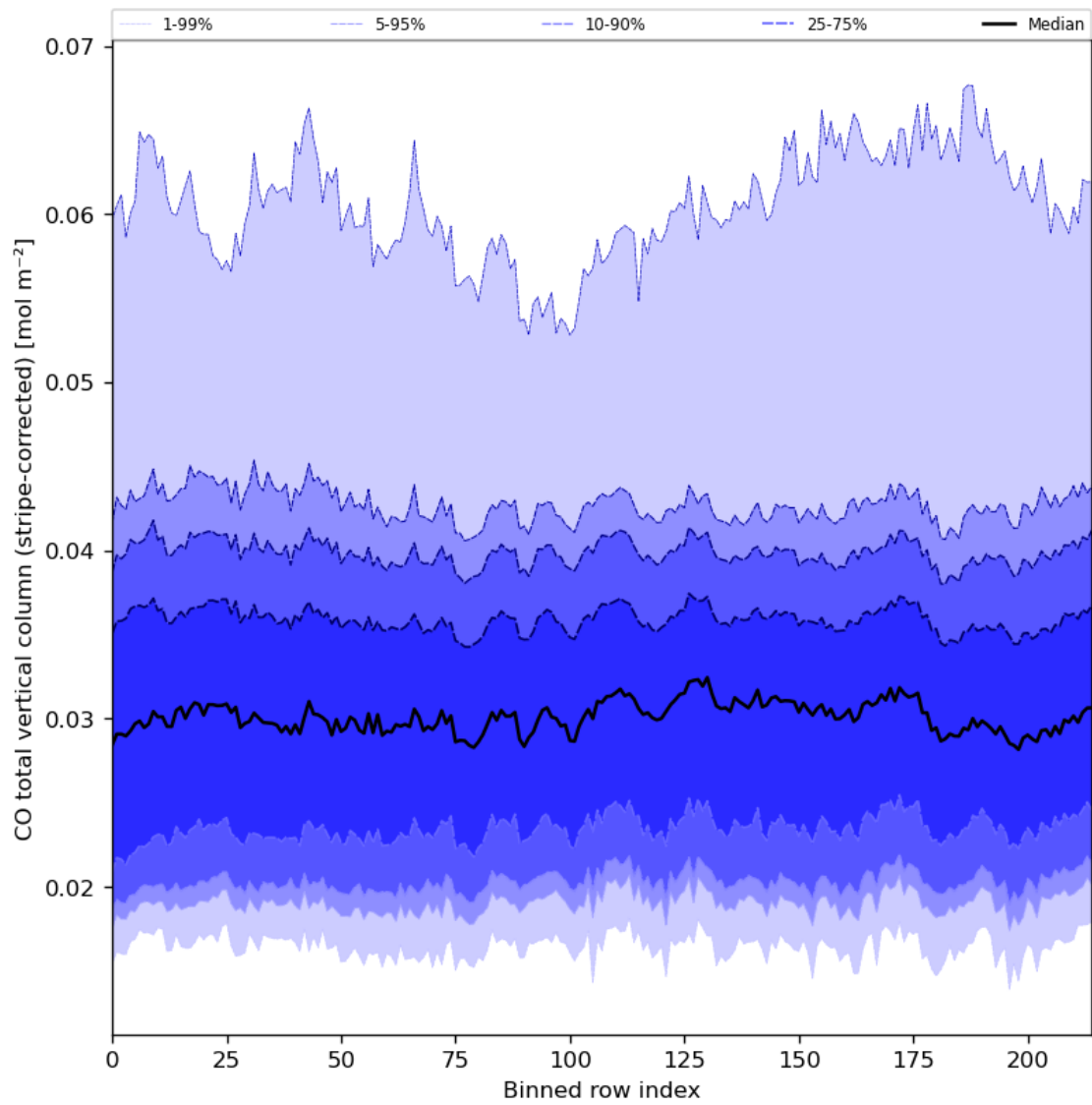
Figure 27: Along track statistics of “CO total vertical column (stripe-corrected)” for 2024-08-06 to 2024-08-07
