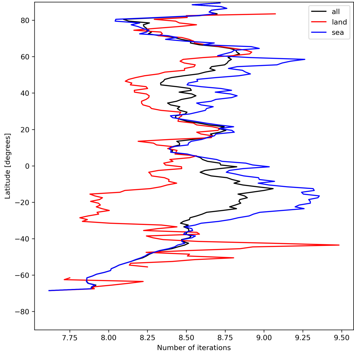
Figure 16: Zonal average of “Number of iterations” for 2024-08-06 to 2024-08-07.
