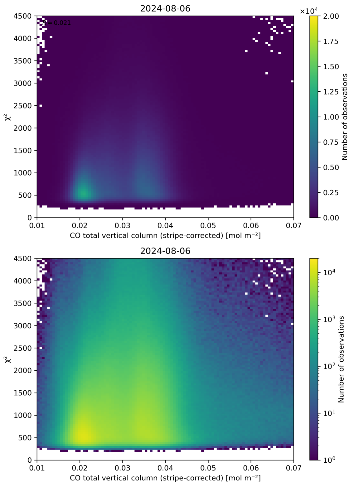
Figure 37: Scatter density plot of “CO total vertical column (stripe-corrected)” against “ \chi^2 ” for 2024-08-06 to 2024-08-07.
