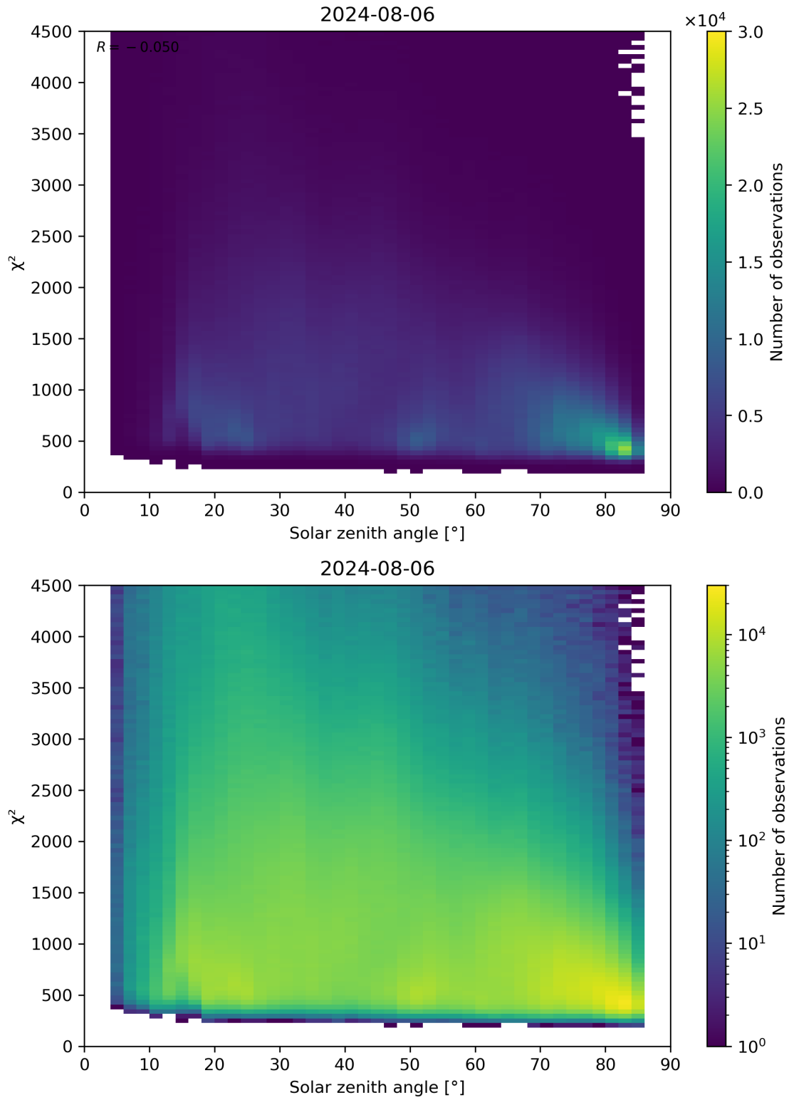
Figure 64: Scatter density plot of “Solar zenith angle” against “ \chi^2 ” for 2024-08-06 to 2024-08-07.
