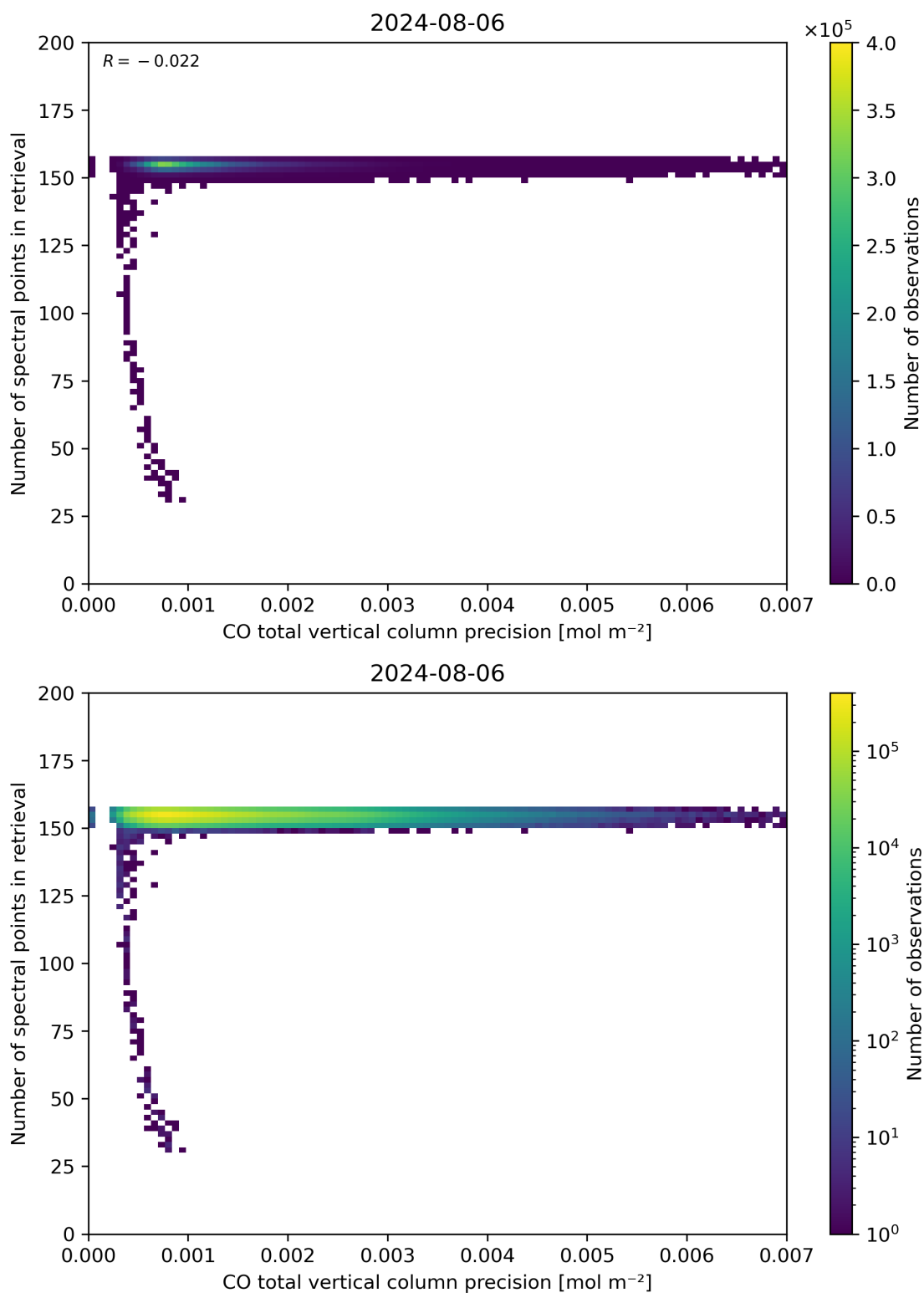
Figure 47: Scatter density plot of “CO total vertical column precision” against “Number of spectral points in retrieval” for 2024-08-06 to 2024-08-07.
