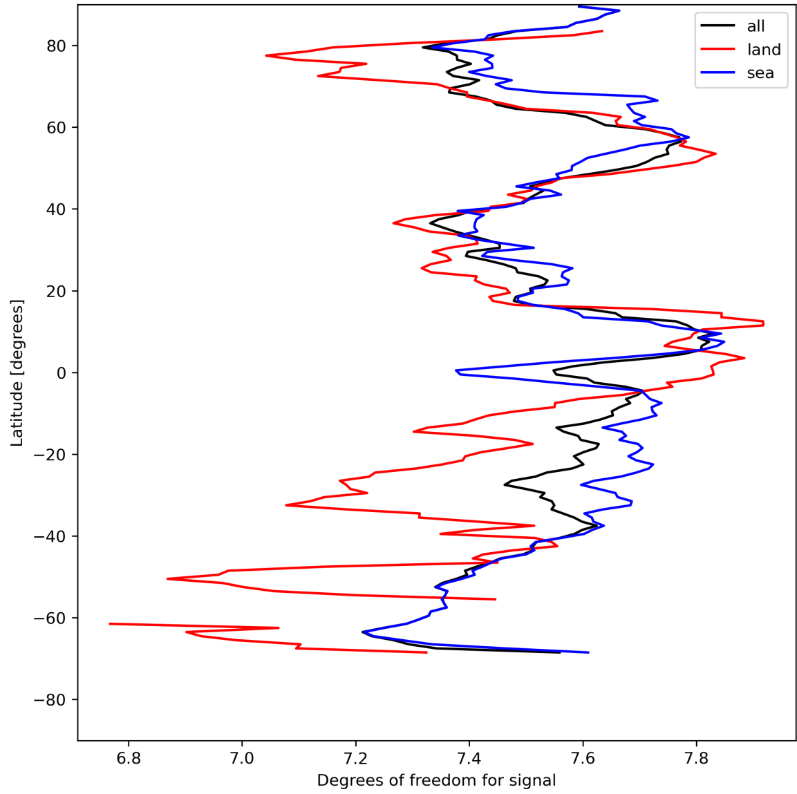
Figure 15: Zonal average of “Degrees of freedom for signal” for 2024-08-06 to 2024-08-07.
