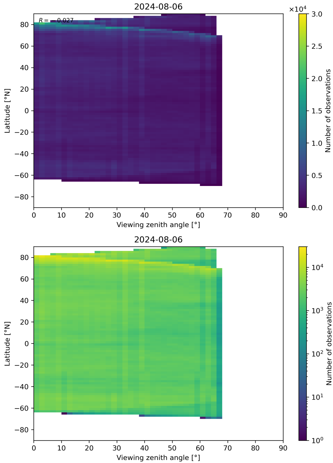
Figure 74: Scatter density plot of “Viewing zenith angle” against “Latitude” for 2024-08-06 to 2024-08-07.
