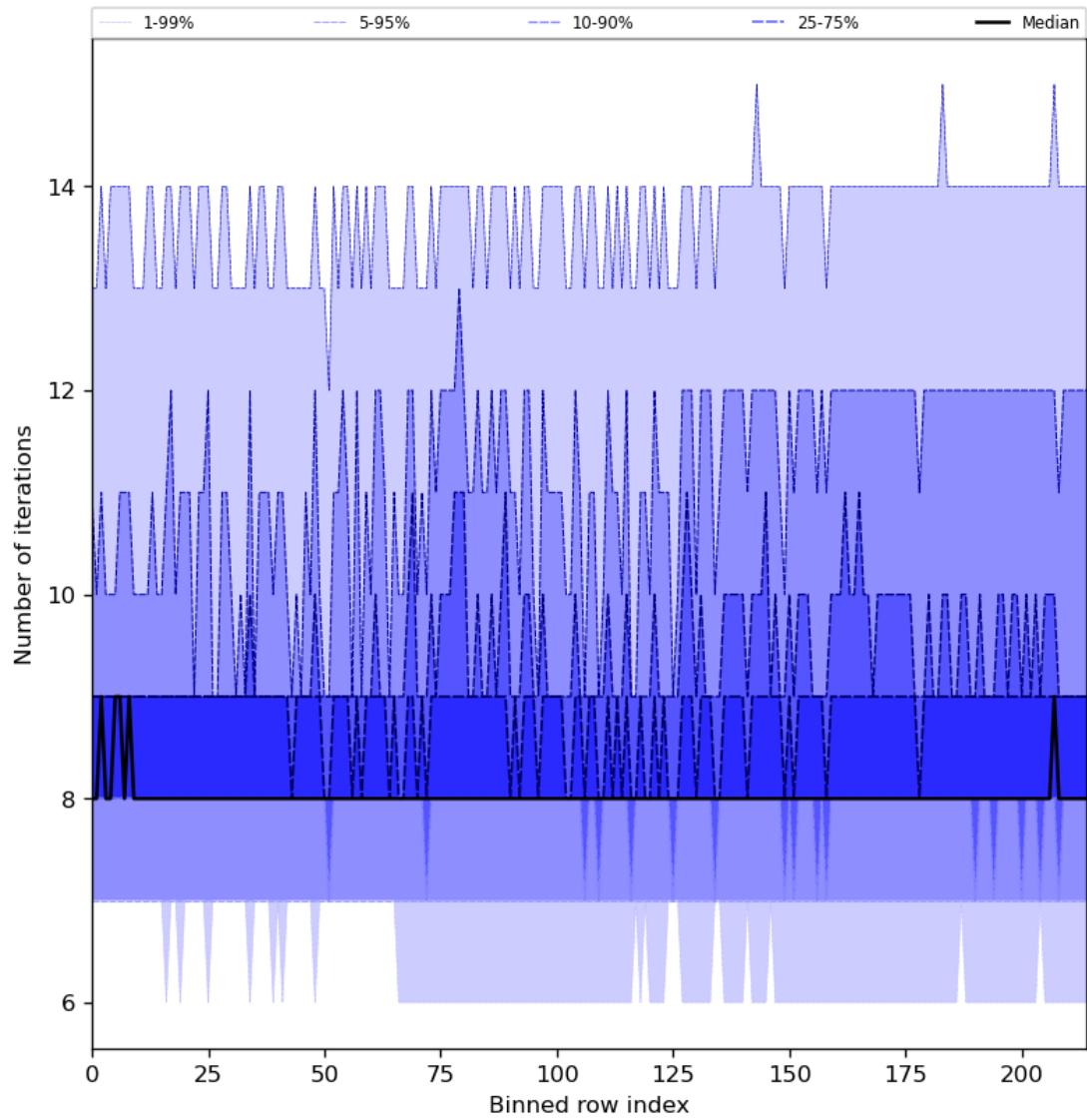
Figure 32: Along track statistics of “Number of iterations” for 2024-08-06 to 2024-08-07
