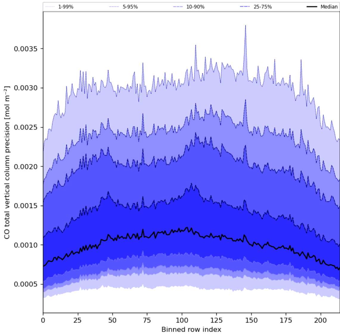
Figure 28: Along track statistics of “CO total vertical column precision” for 2024-08-06 to 2024-08-07
