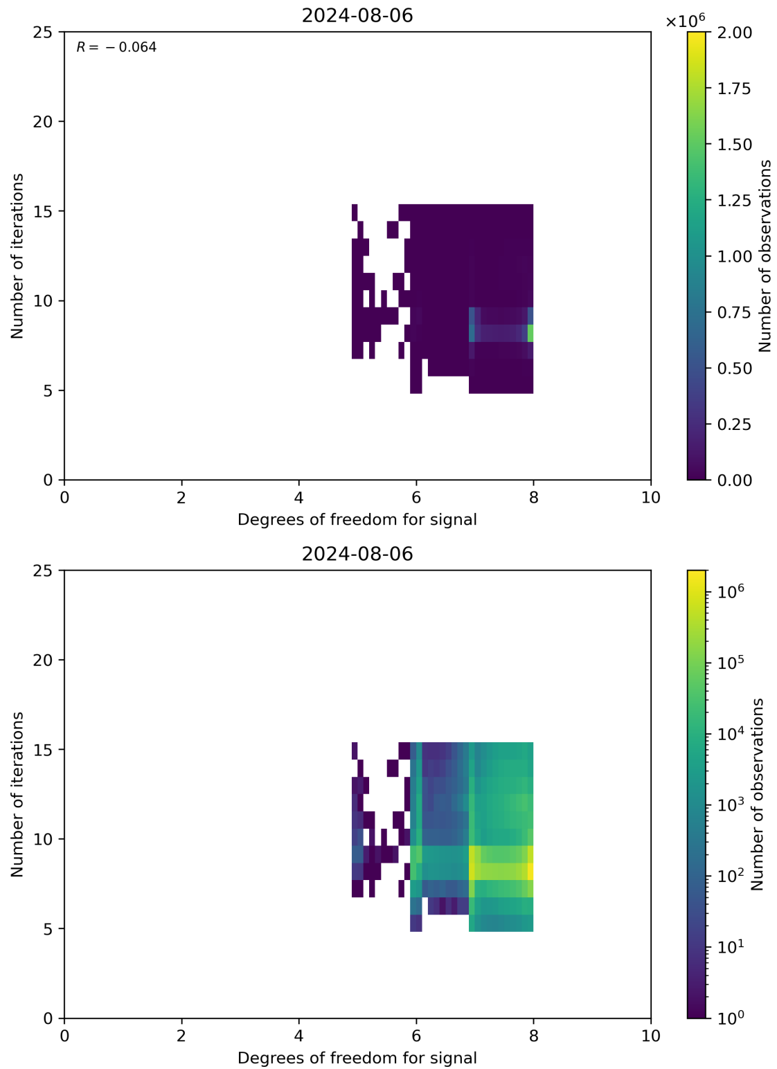
Figure 50: Scatter density plot of “Degrees of freedom for signal” against “Number of iterations” for 2024-08-06 to 2024-08-07.
