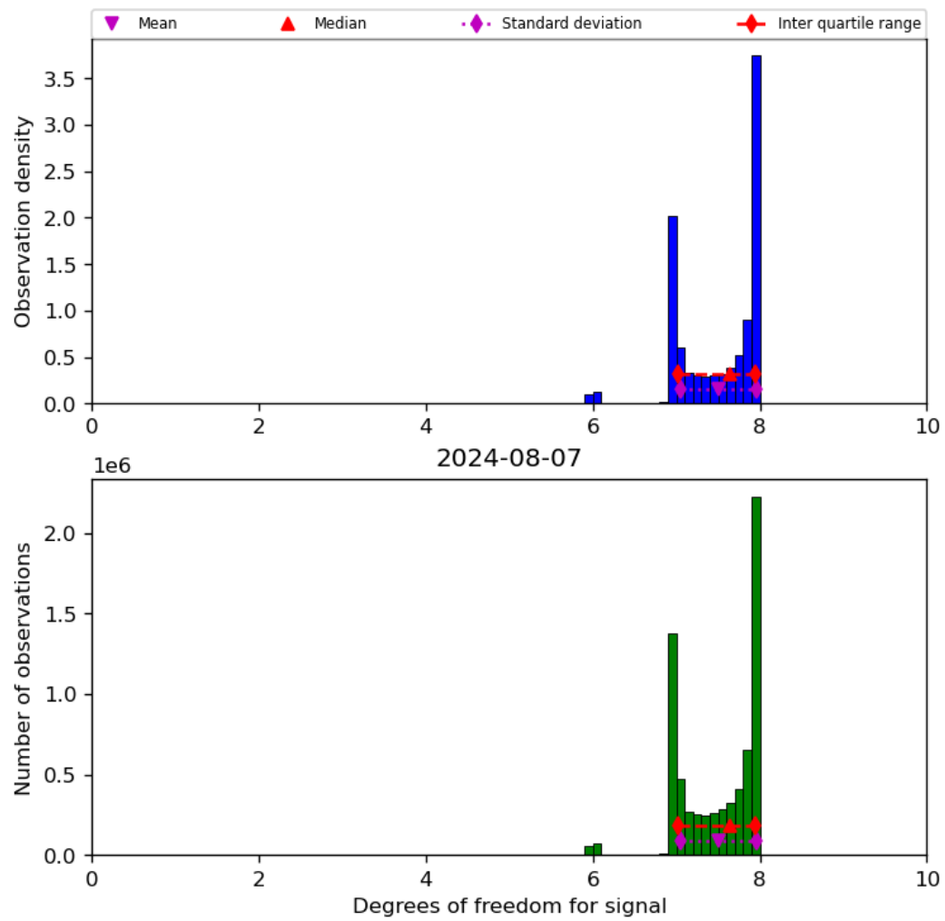
Figure 23: Histogram of “Degrees of freedom for signal” for 2024-08-06 to 2024-08-08
