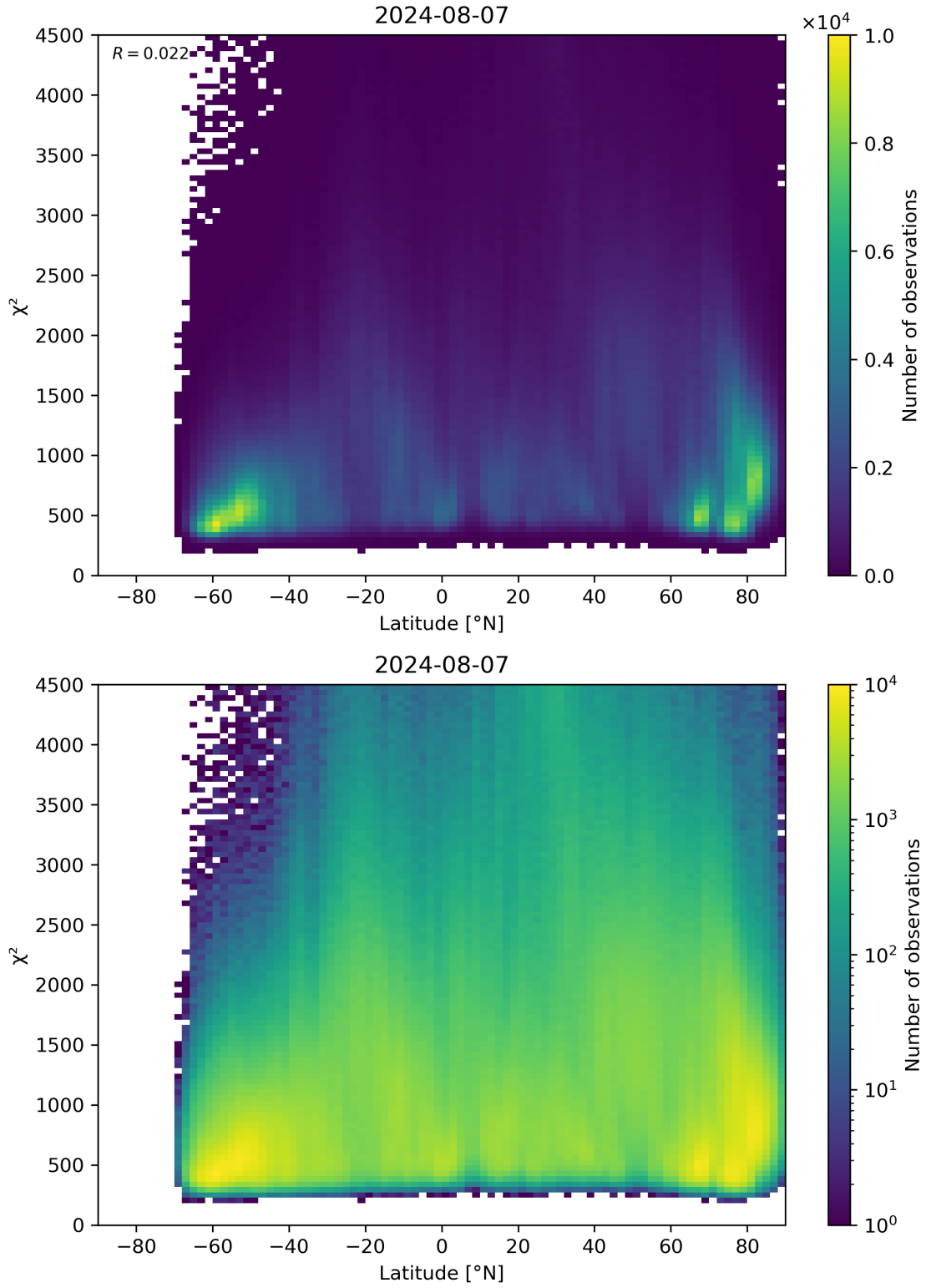
Figure 54: Scatter density plot of “Latitude” against “ \chi^2 ” for 2024-08-06 to 2024-08-08.
