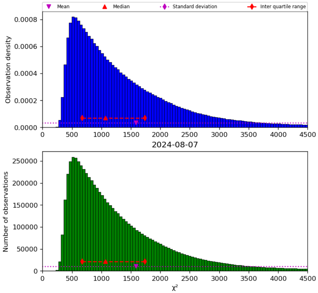
Figure 22: Histogram of “ \chi^2 ” for 2024-08-06 to 2024-08-08
