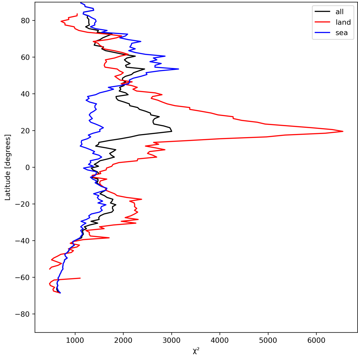
Figure 14: Zonal average of “ \chi^2 ” for 2024-08-06 to 2024-08-08.
