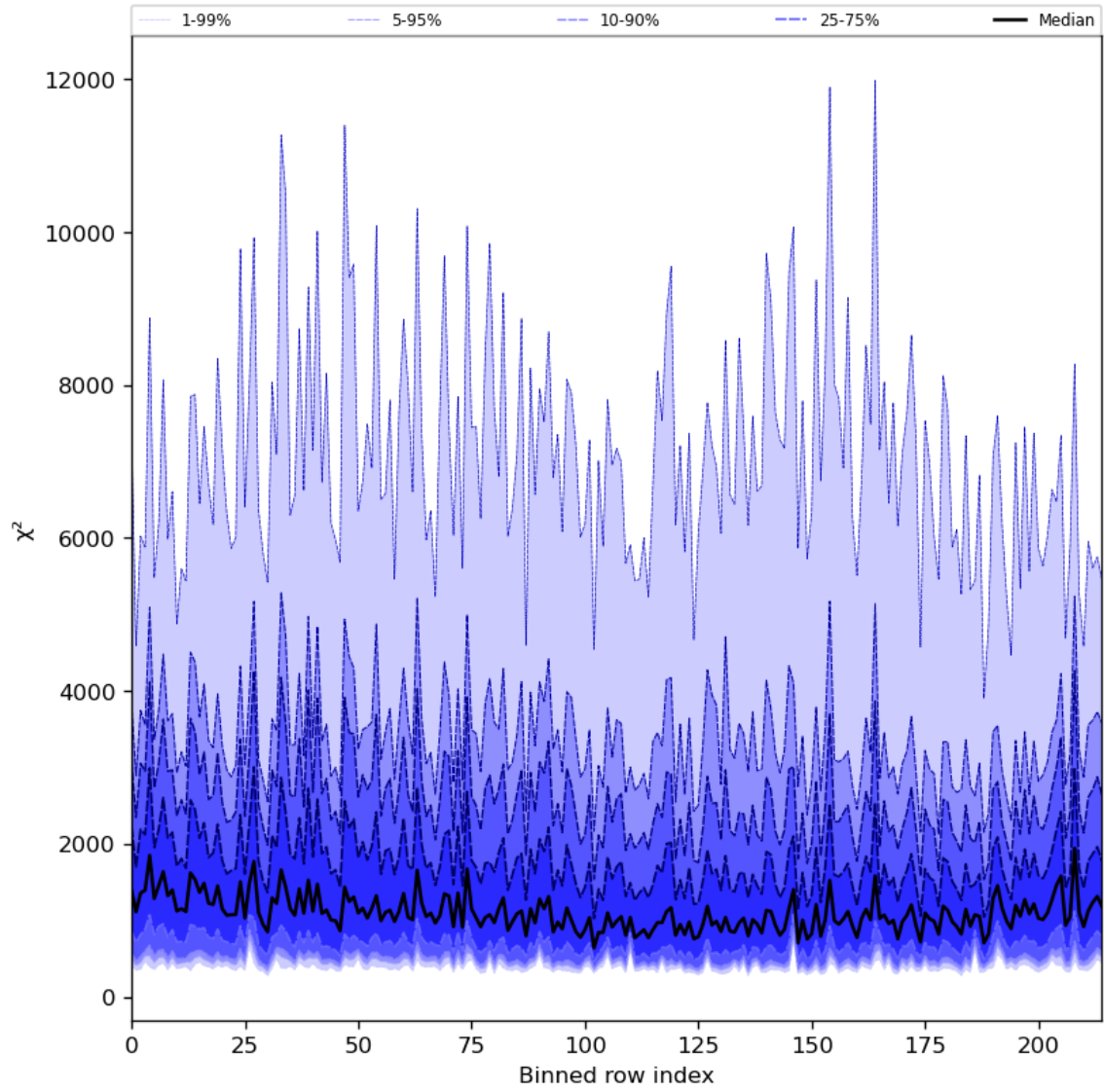
Figure 30: Along track statistics of “ \chi^2 ” for 2024-08-06 to 2024-08-08
