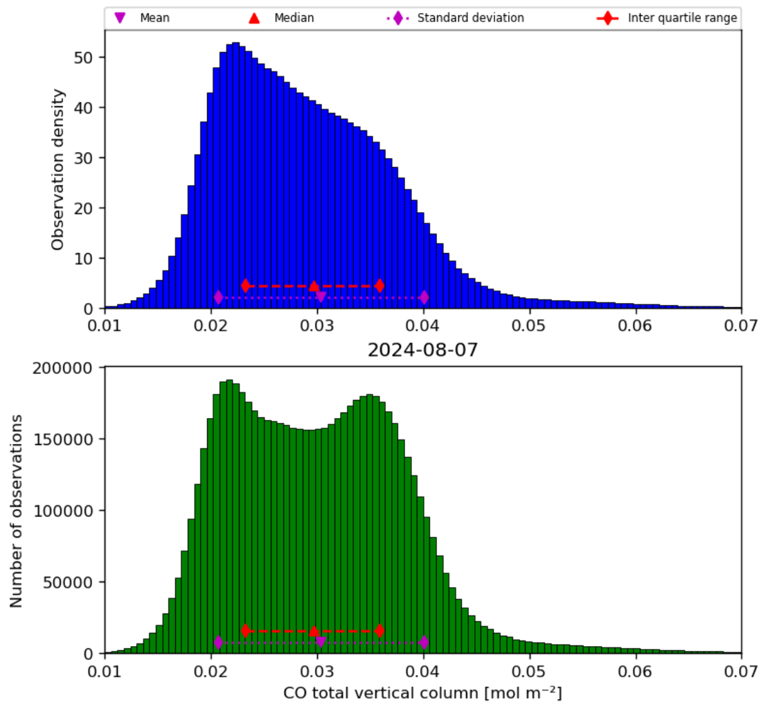
Figure 18: Histogram of “CO total vertical column” for 2024-08-06 to 2024-08-08
