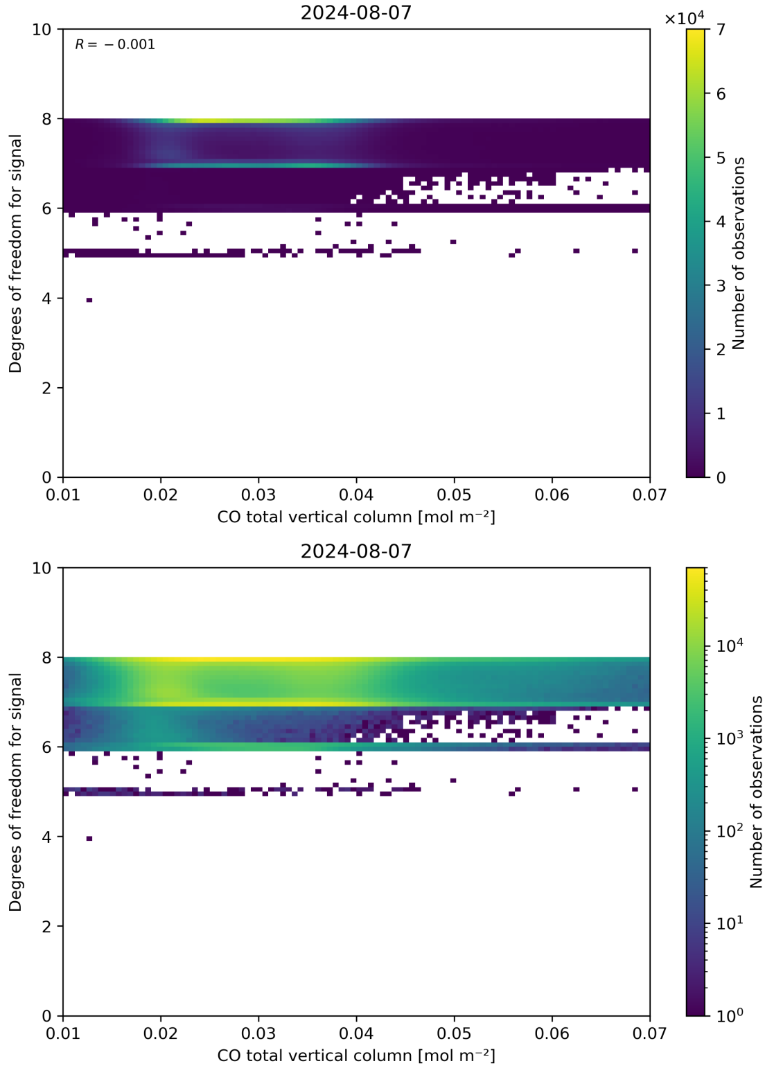
Figure 41: Scatter density plot of “CO total vertical column” against “Degrees of freedom for signal” for 2024-08-06 to 2024-08-08.
