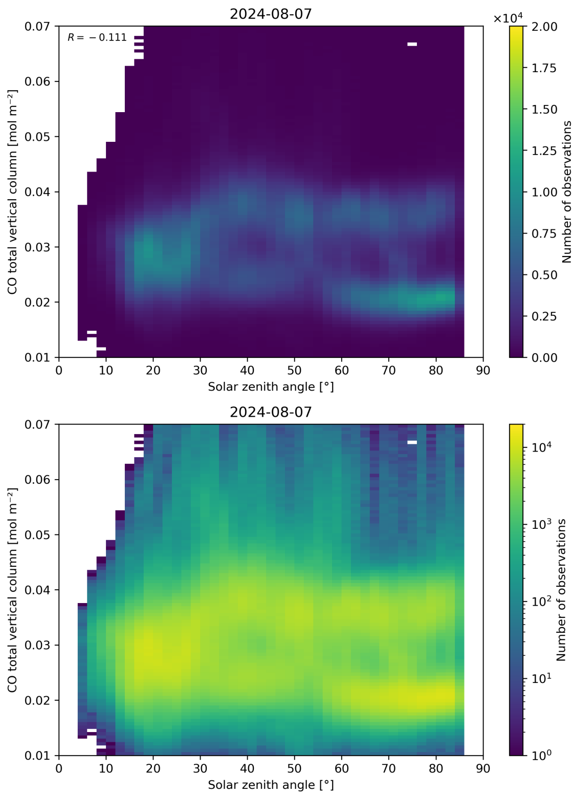
Figure 61: Scatter density plot of “Solar zenith angle” against “CO total vertical column” for 2024-08-06 to 2024-08-08.
