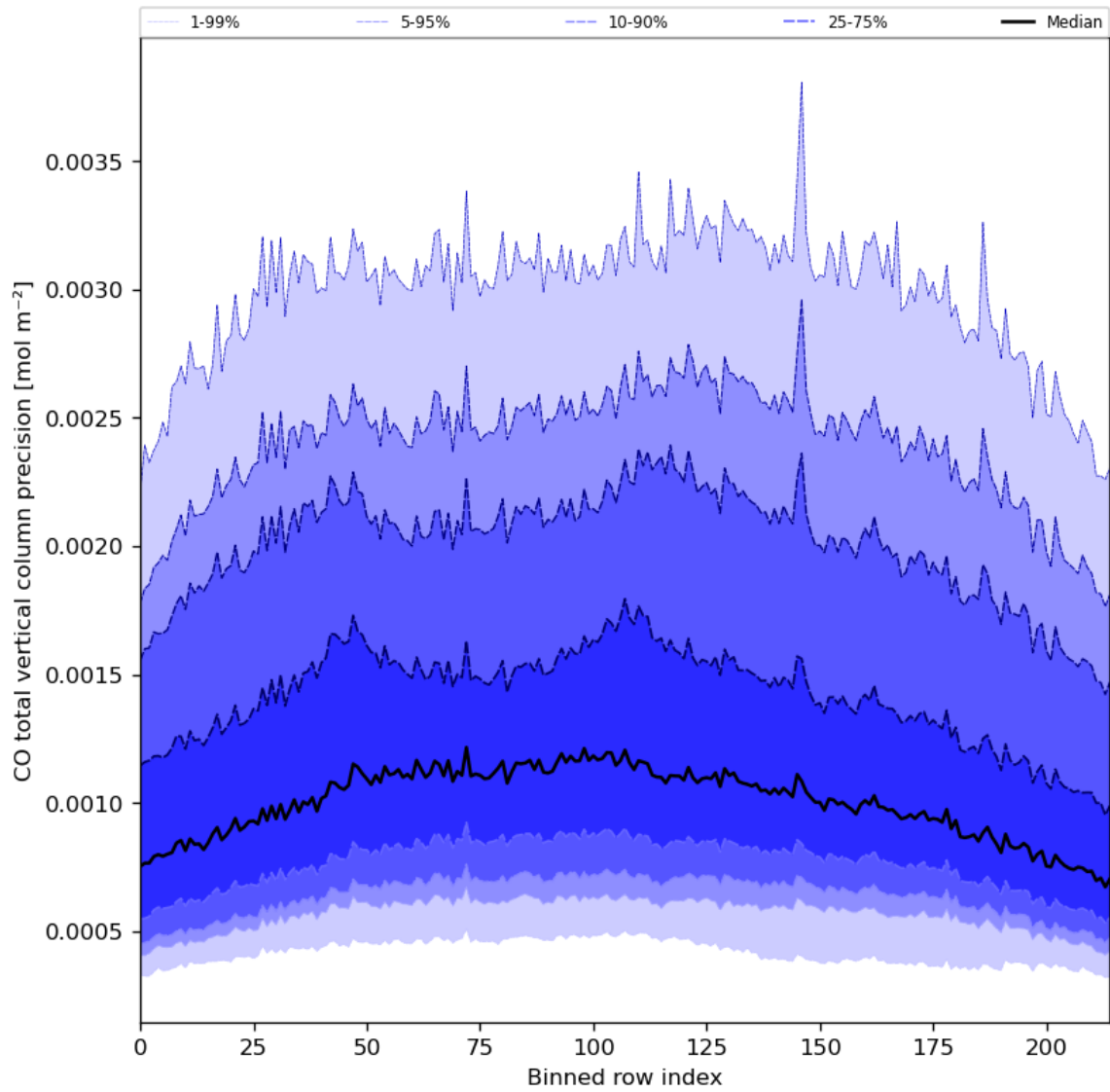
Figure 28: Along track statistics of “CO total vertical column precision” for 2024-08-06 to 2024-08-08
