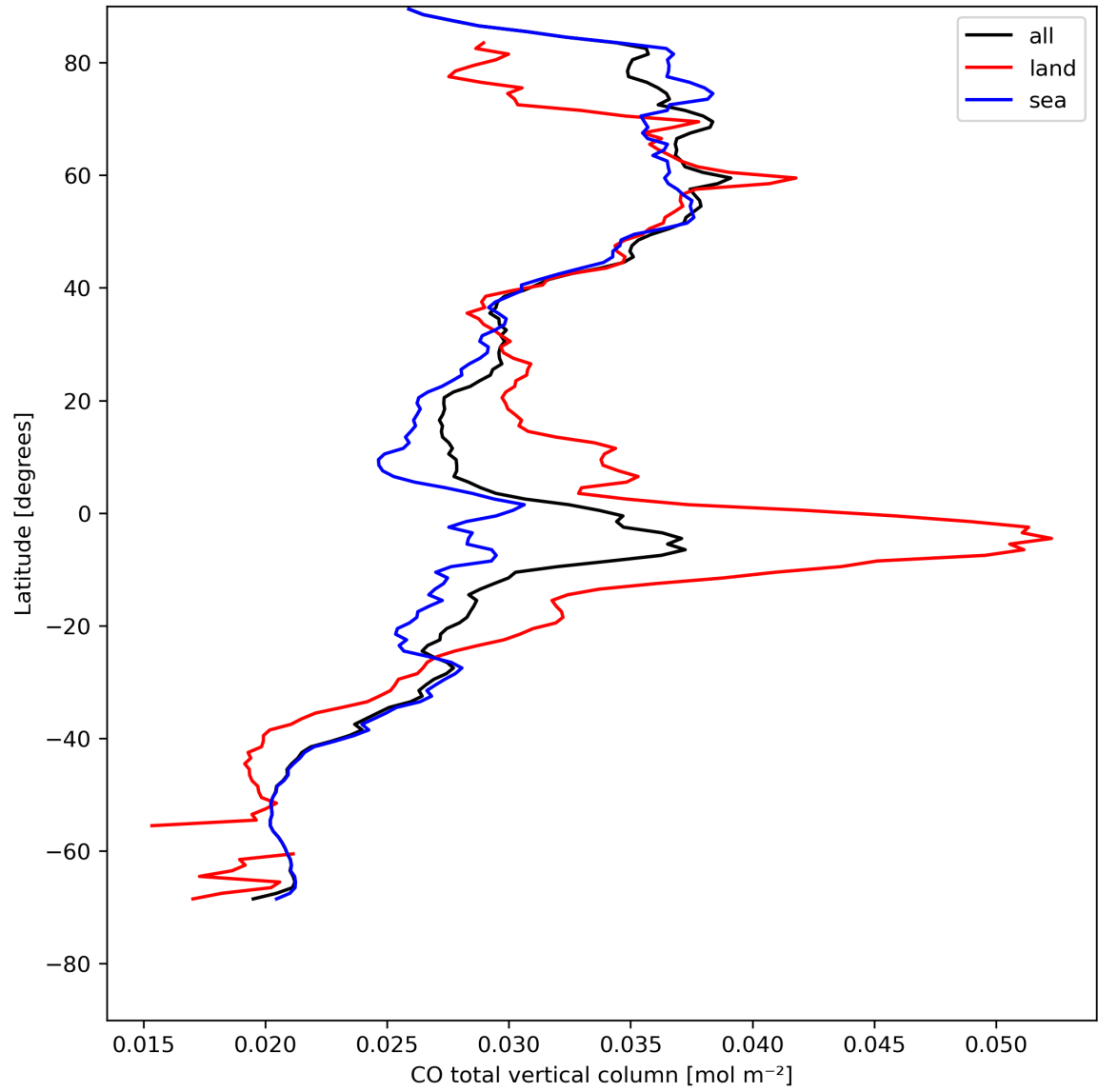
Figure 10: Zonal average of “CO total vertical column” for 2024-08-06 to 2024-08-08.
