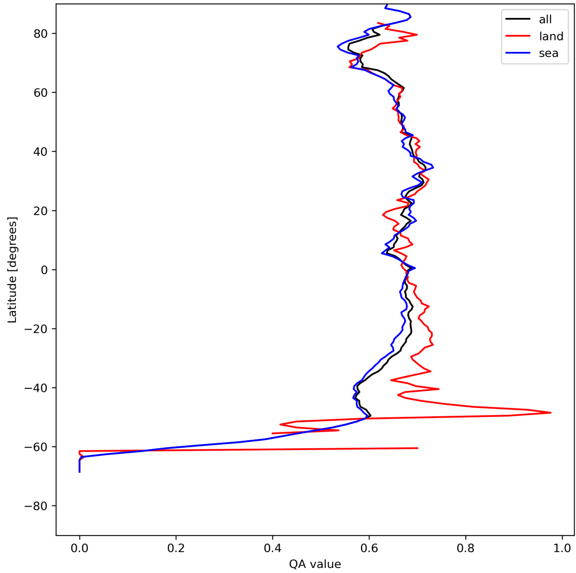
Figure 9: Zonal average of “QA value” for 2024-08-06 to 2024-08-08.
