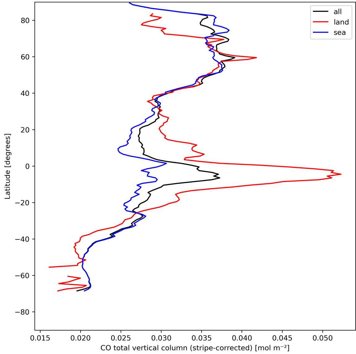
Figure 11: Zonal average of “CO total vertical column (stripe-corrected)” for 2024-08-06 to 2024-08-08.
