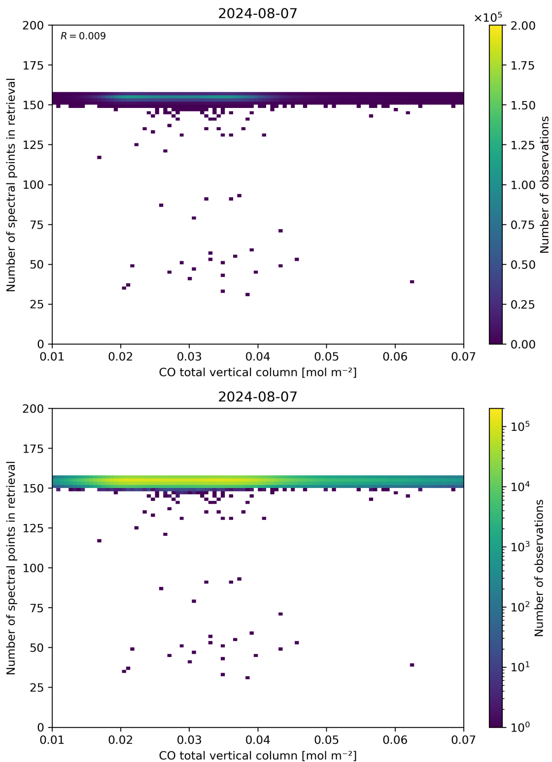
Figure 43: Scatter density plot of “CO total vertical column” against “Number of spectral points in retrieval” for 2024-08-06 to 2024-08-08.
