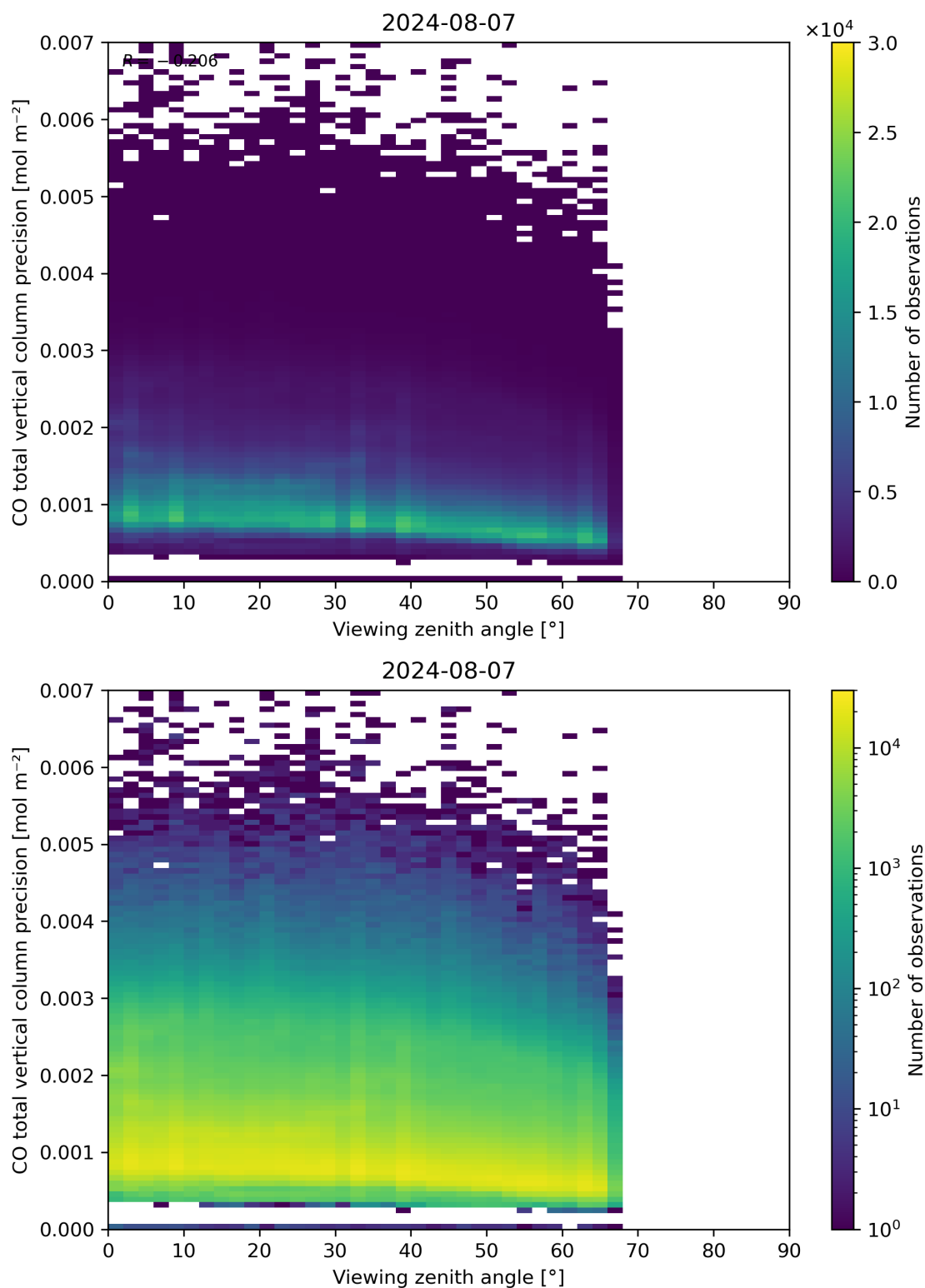
Figure 71: Scatter density plot of “Viewing zenith angle” against “CO total vertical column precision” for 2024-08-06 to 2024-08-08.
