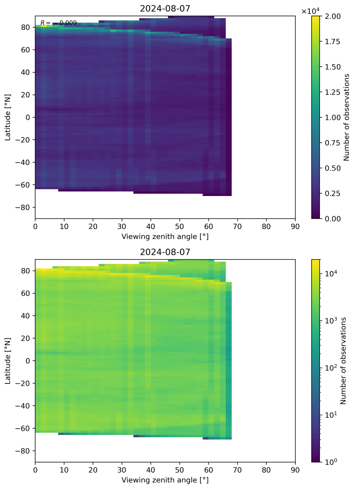
Figure 74: Scatter density plot of “Viewing zenith angle” against “Latitude” for 2024-08-06 to 2024-08-08.
