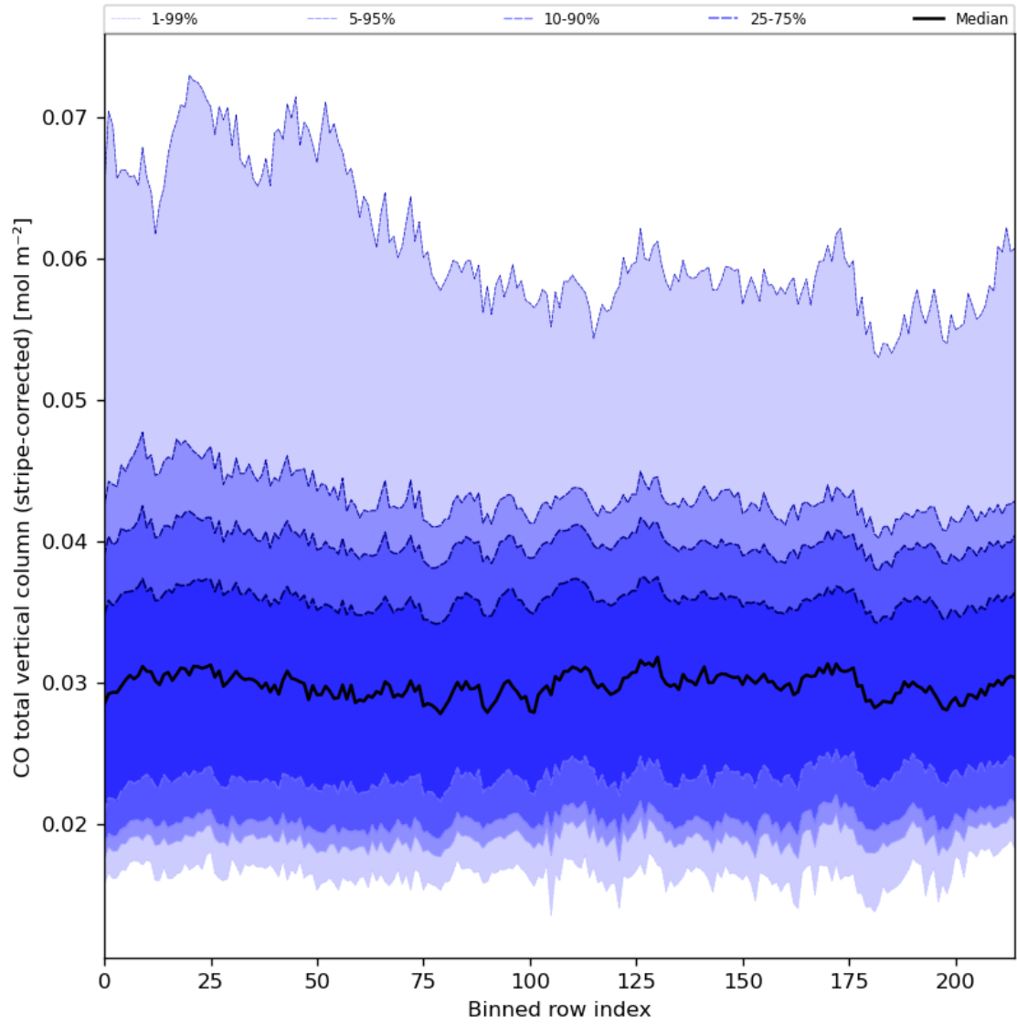
Figure 27: Along track statistics of “CO total vertical column (stripe-corrected)” for 2024-08-06 to 2024-08-08
