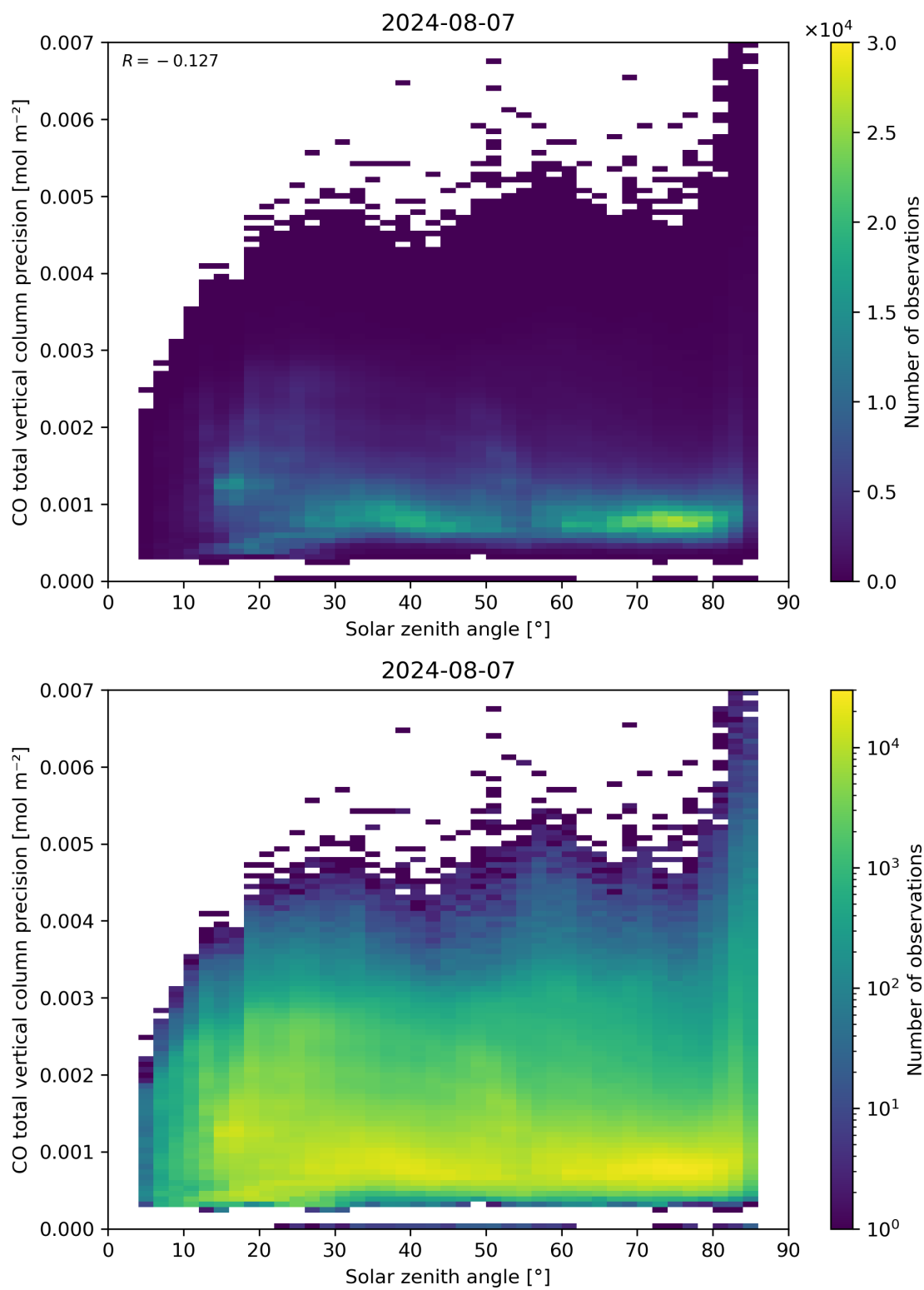
Figure 63: Scatter density plot of “Solar zenith angle” against “CO total vertical column precision” for 2024-08-06 to 2024-08-08.
