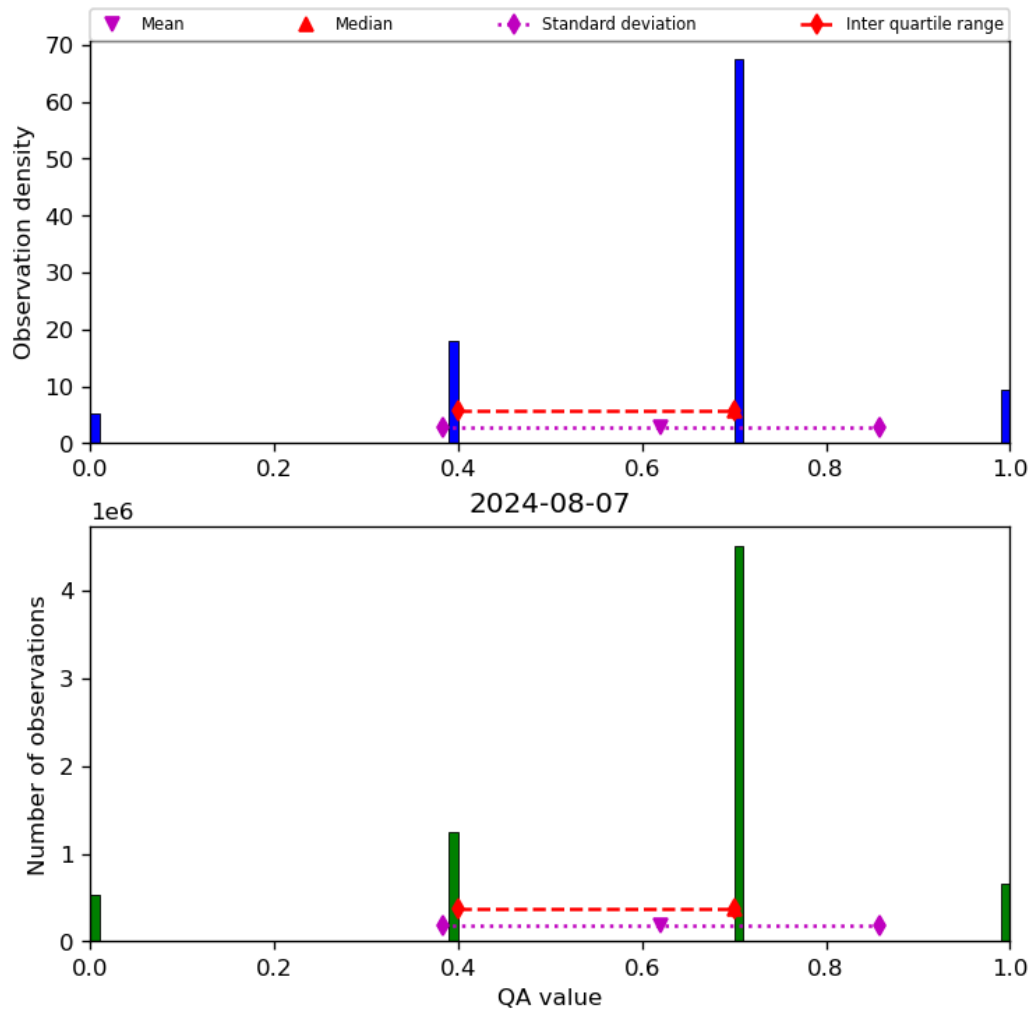
Figure 17: Histogram of “QA value” for 2024-08-06 to 2024-08-08
