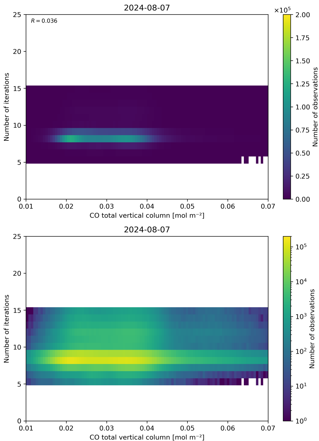
Figure 42: Scatter density plot of “CO total vertical column” against “Number of iterations” for 2024-08-06 to 2024-08-08.
