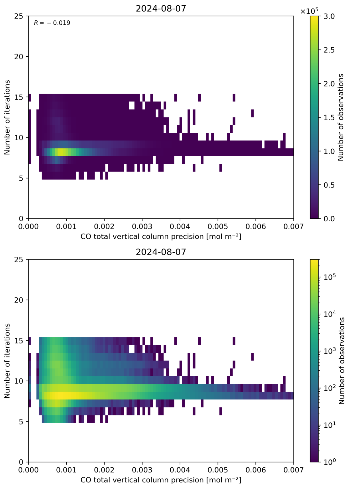
Figure 46: Scatter density plot of “CO total vertical column precision” against “Number of iterations” for 2024-08-06 to 2024-08-08.
