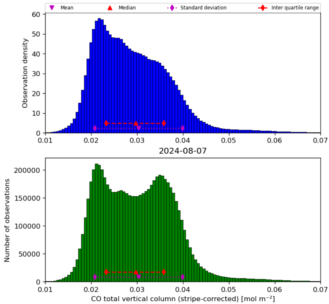
Figure 19: Histogram of “CO total vertical column (stripe-corrected)” for 2024-08-06 to 2024-08-08
