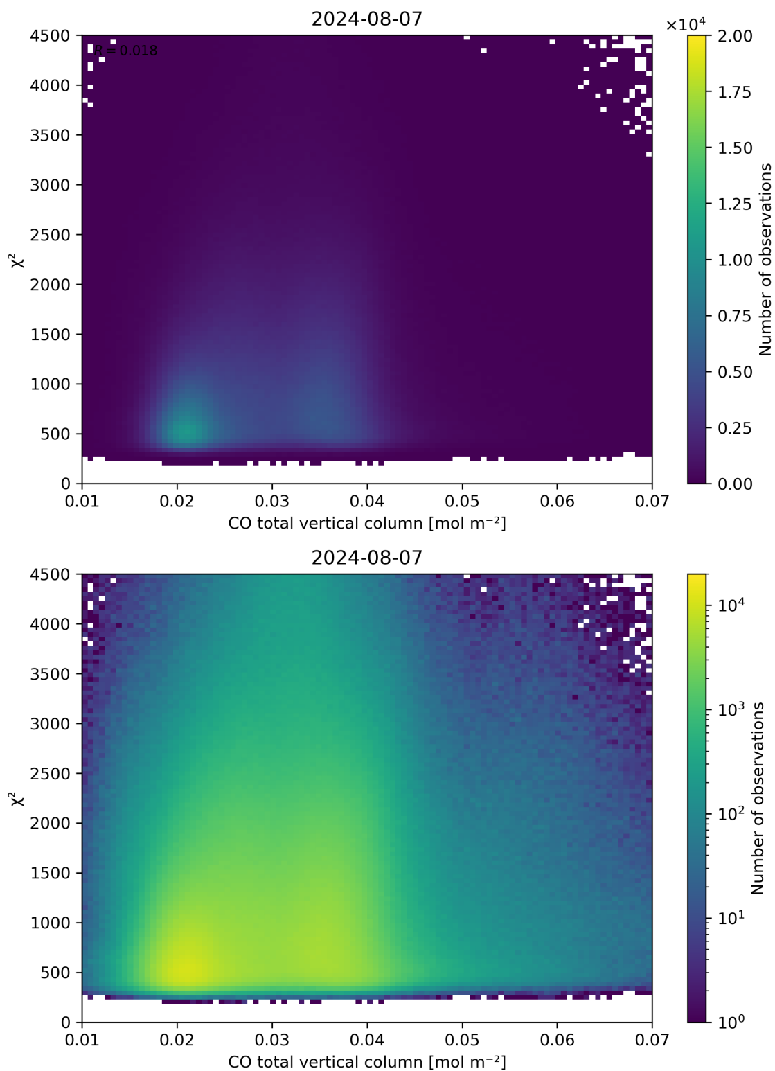
Figure 35: Scatter density plot of “CO total vertical column” against “ \chi^2 ” for 2024-08-06 to 2024-08-08.
