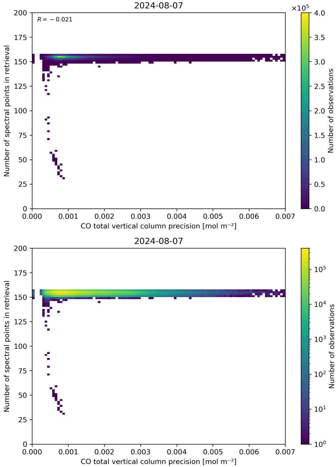
Figure 47: Scatter density plot of “CO total vertical column precision” against “Number of spectral points in retrieval” for 2024-08-06 to 2024-08-08.
