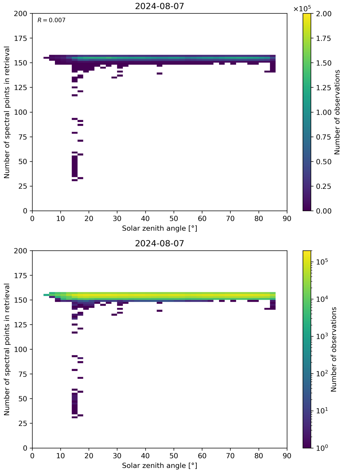
Figure 68: Scatter density plot of “Solar zenith angle” against “Number of spectral points in retrieval” for 2024-08-06 to 2024-08-08.
