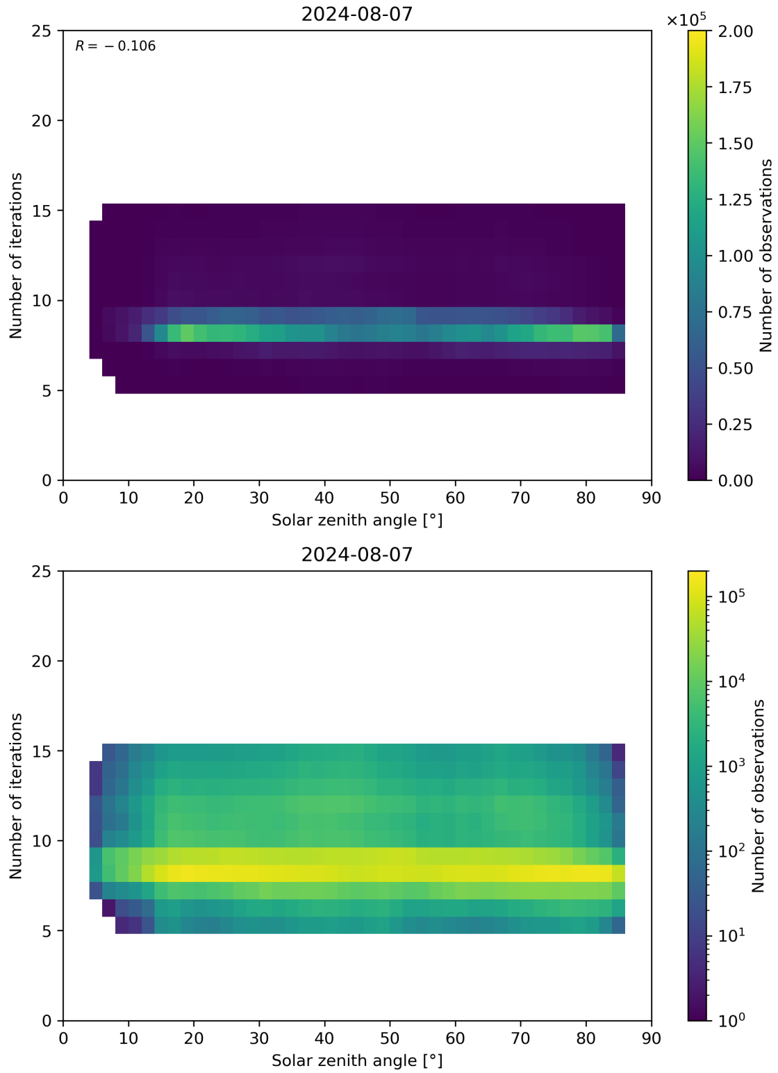
Figure 67: Scatter density plot of “Solar zenith angle” against “Number of iterations” for 2024-08-06 to 2024-08-08.
