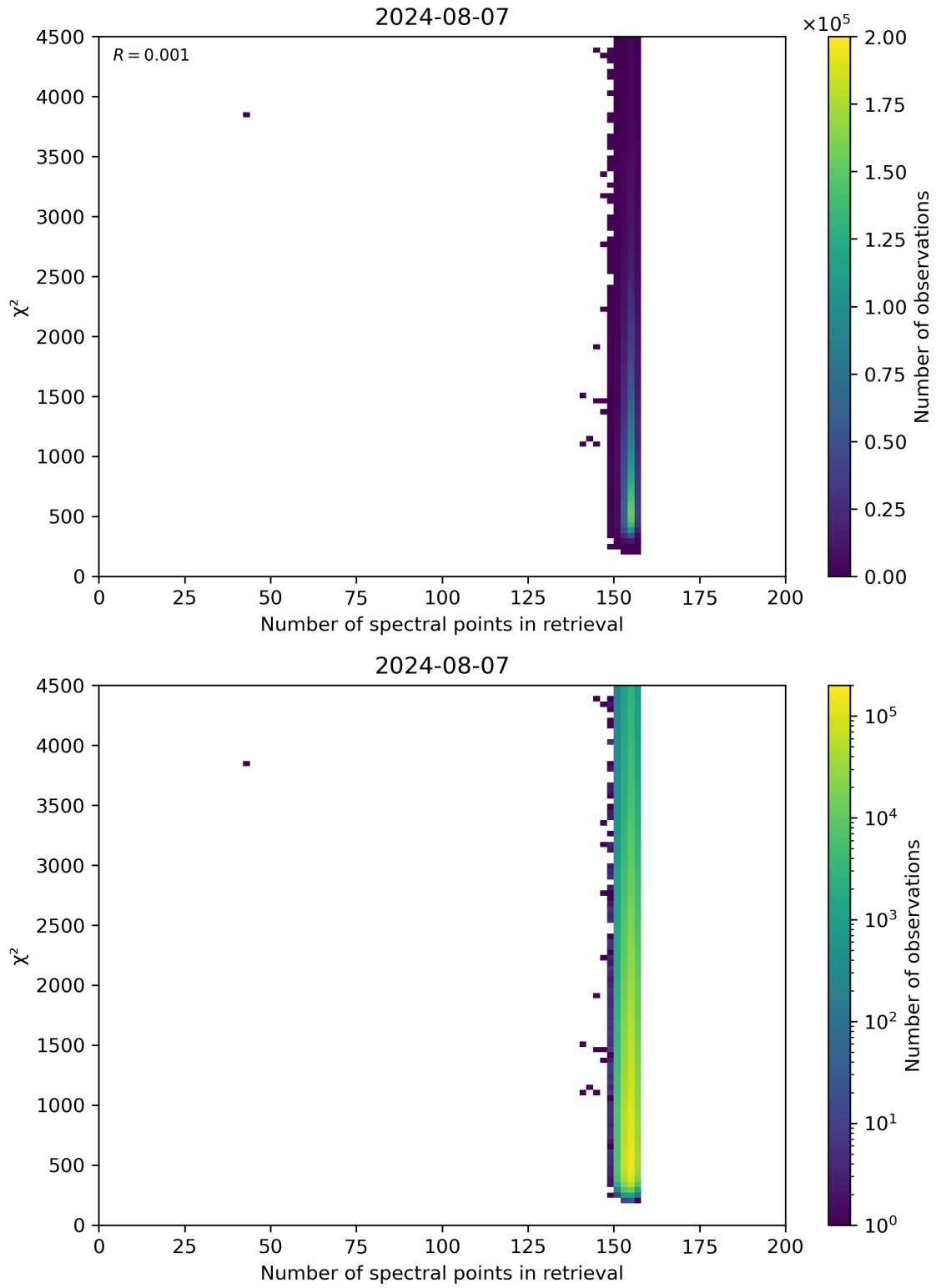
Figure 58: Scatter density plot of “Number of spectral points in retrieval” against “ \chi^2 ” for 2024-08-06 to 2024-08-08.
