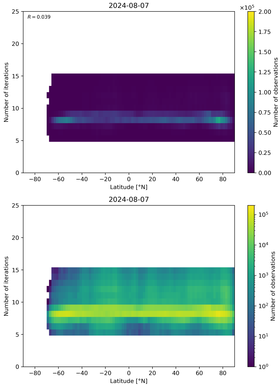
Figure 56: Scatter density plot of “Latitude” against “Number of iterations” for 2024-08-06 to 2024-08-08.
