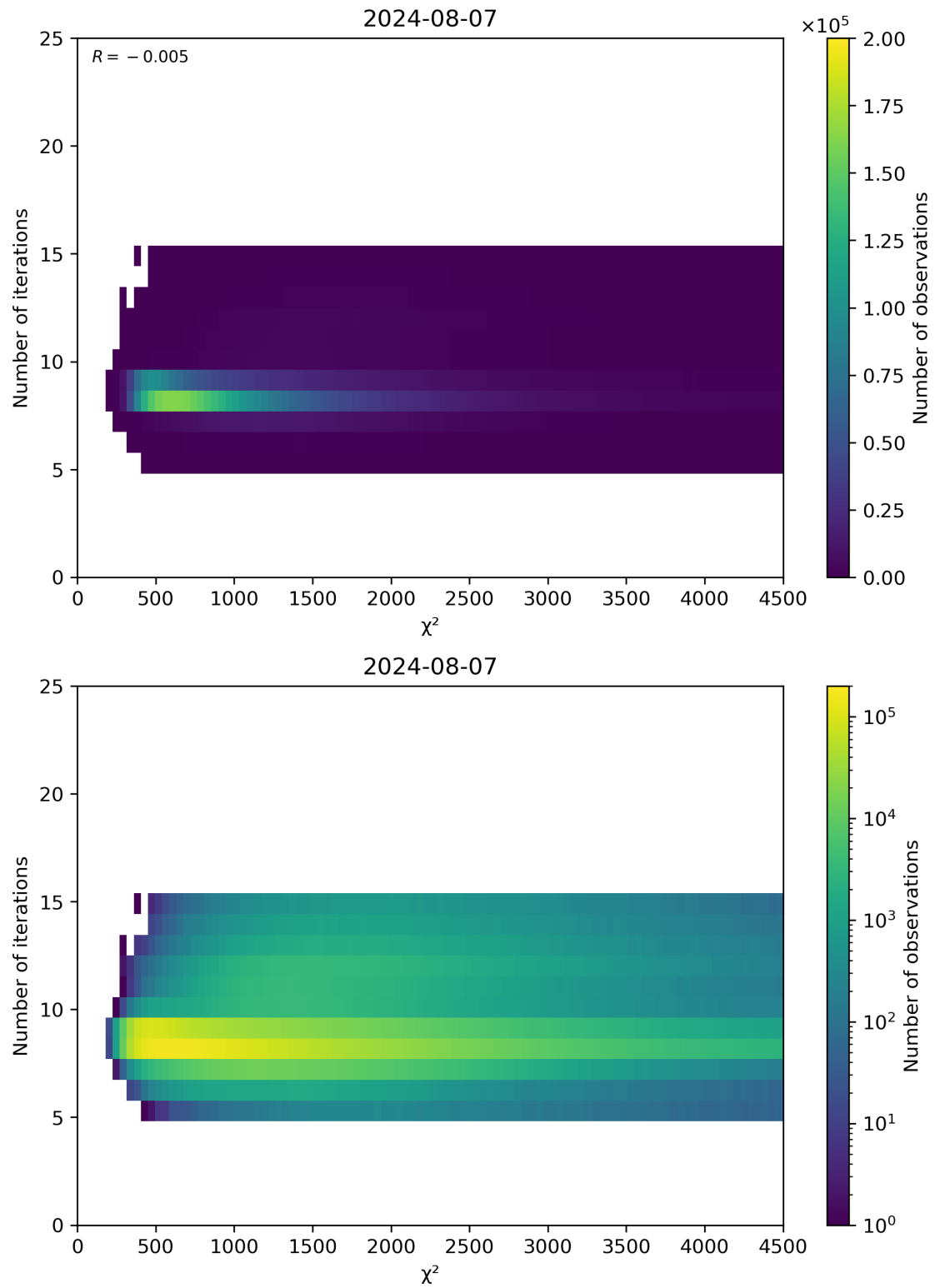
Figure 49: Scatter density plot of “ \chi^2 ” against “Number of iterations” for 2024-08-06 to 2024-08-08.
