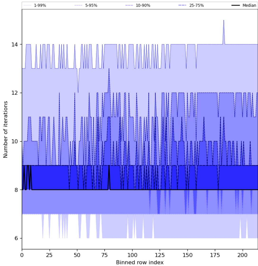
Figure 32: Along track statistics of “Number of iterations” for 2024-08-06 to 2024-08-08
