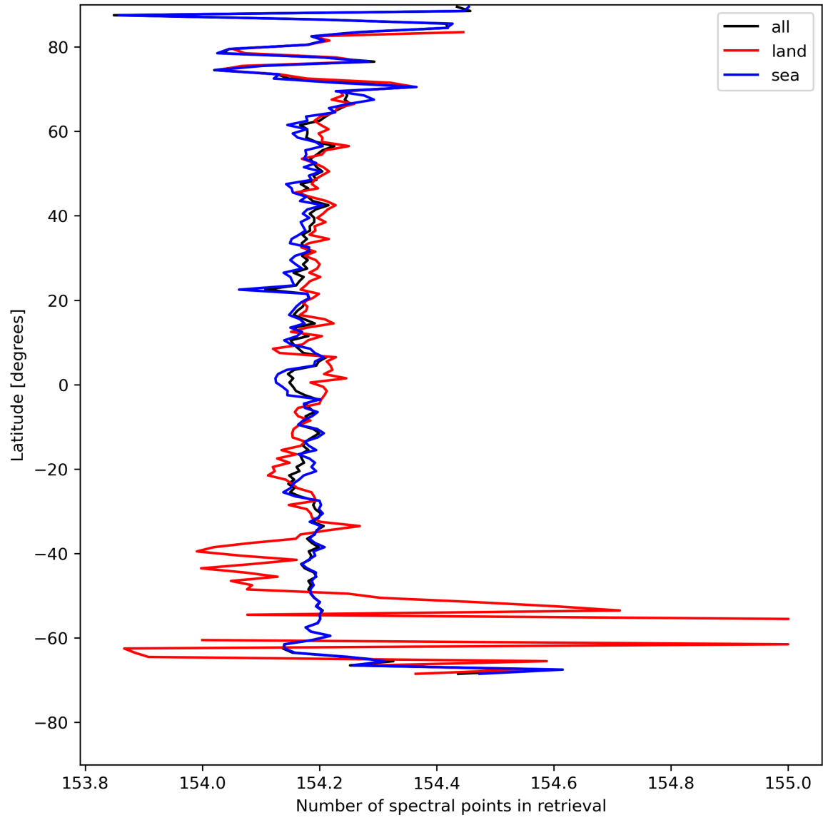
Figure 13: Zonal average of “Number of spectral points in retrieval” for 2024-08-06 to 2024-08-08.
