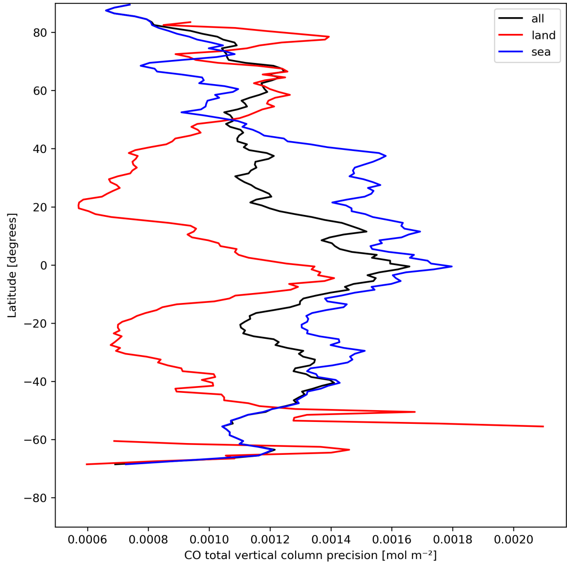
Figure 12: Zonal average of “CO total vertical column precision” for 2024-08-06 to 2024-08-08.
