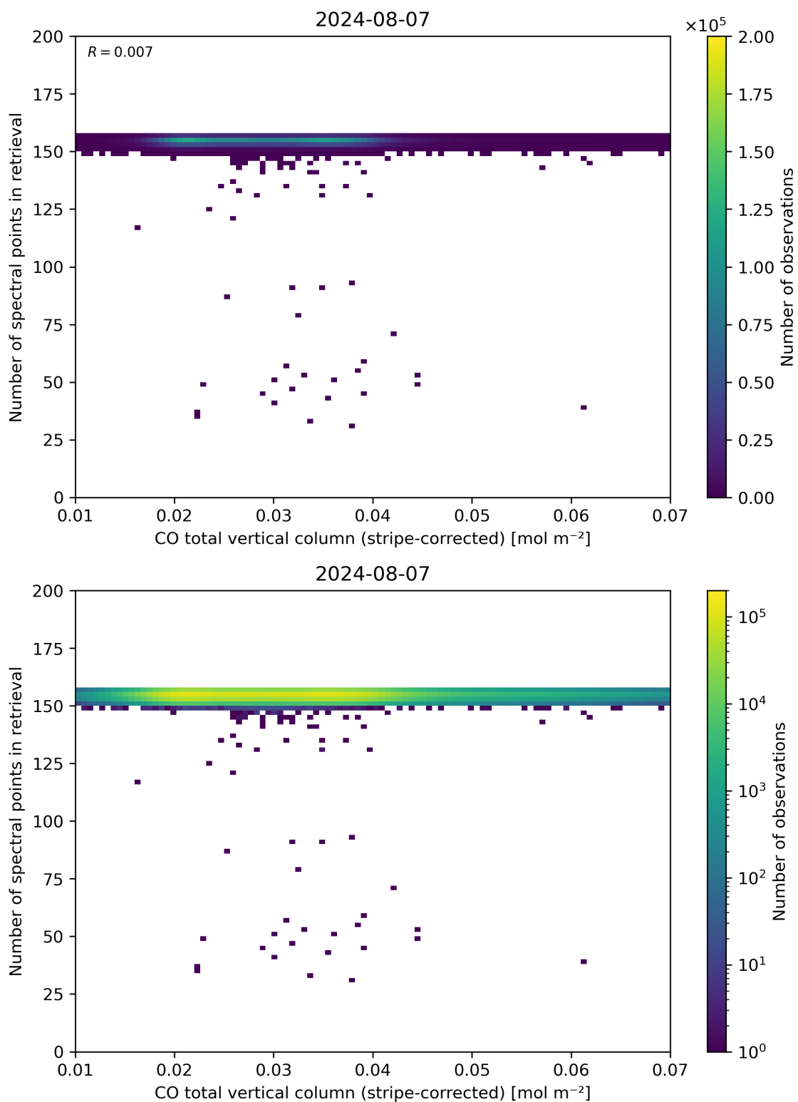
Figure 40: Scatter density plot of “CO total vertical column (stripe-corrected)” against “Number of spectral points in retrieval” for 2024-08-06 to 2024-08-08.
