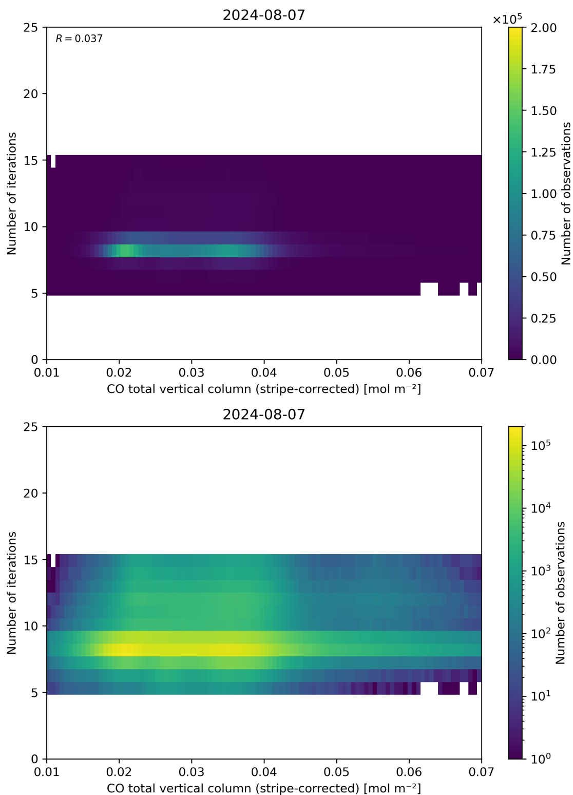
Figure 39: Scatter density plot of “CO total vertical column (stripe-corrected)” against “Number of iterations” for 2024-08-06 to 2024-08-08.
