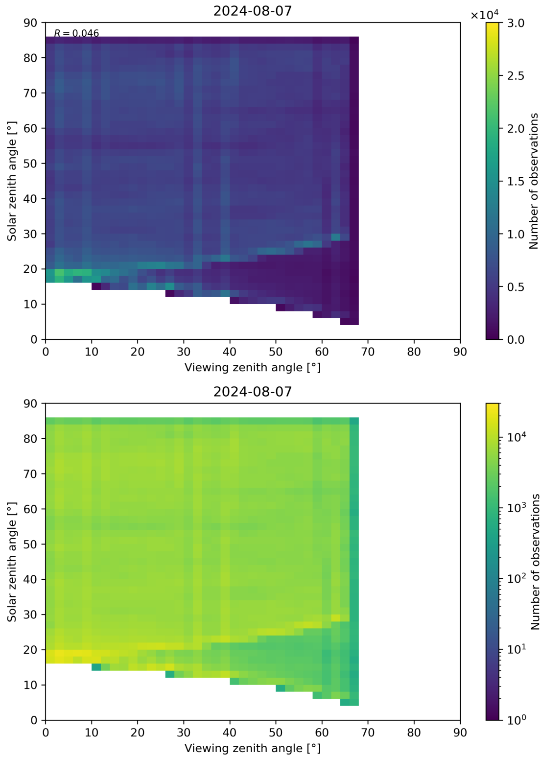
Figure 77: Scatter density plot of “Viewing zenith angle” against “Solar zenith angle” for 2024-08-06 to 2024-08-08.
