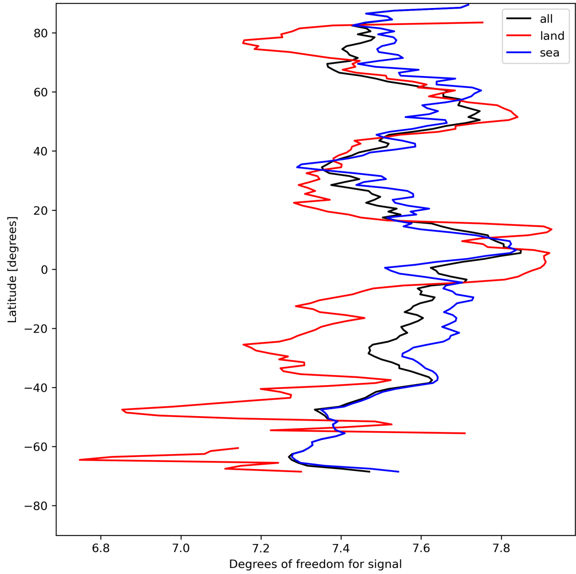
Figure 15: Zonal average of “Degrees of freedom for signal” for 2024-08-06 to 2024-08-08.
