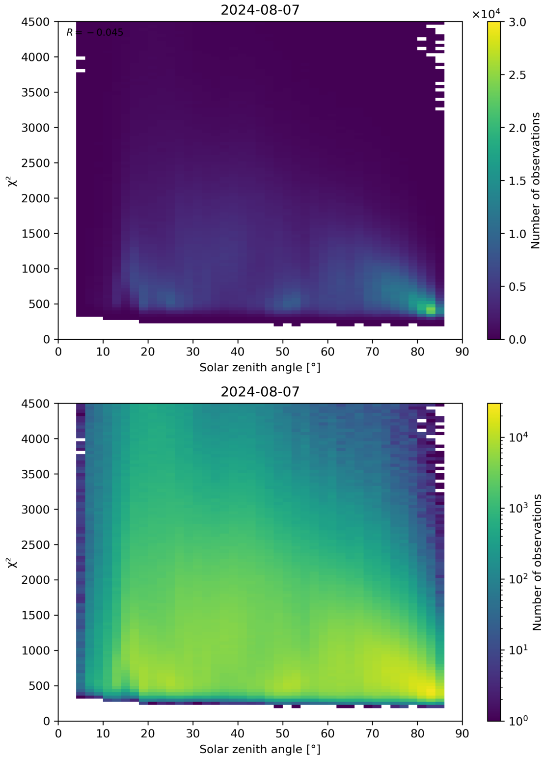
Figure 64: Scatter density plot of “Solar zenith angle” against “ \chi^2 ” for 2024-08-06 to 2024-08-08.
