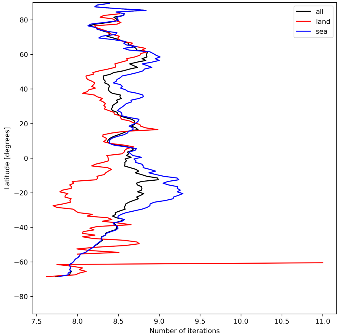
Figure 16: Zonal average of “Number of iterations” for 2024-08-06 to 2024-08-08.
