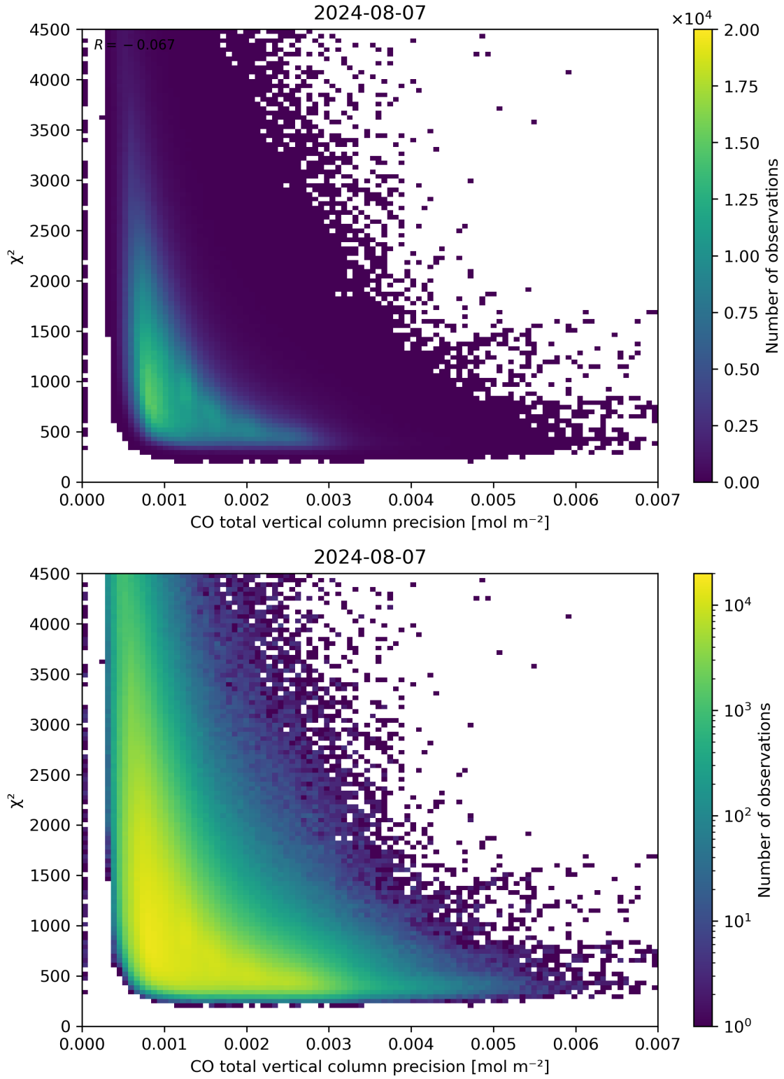
Figure 44: Scatter density plot of “CO total vertical column precision” against “ \chi^2 ” for 2024-08-06 to 2024-08-08.
