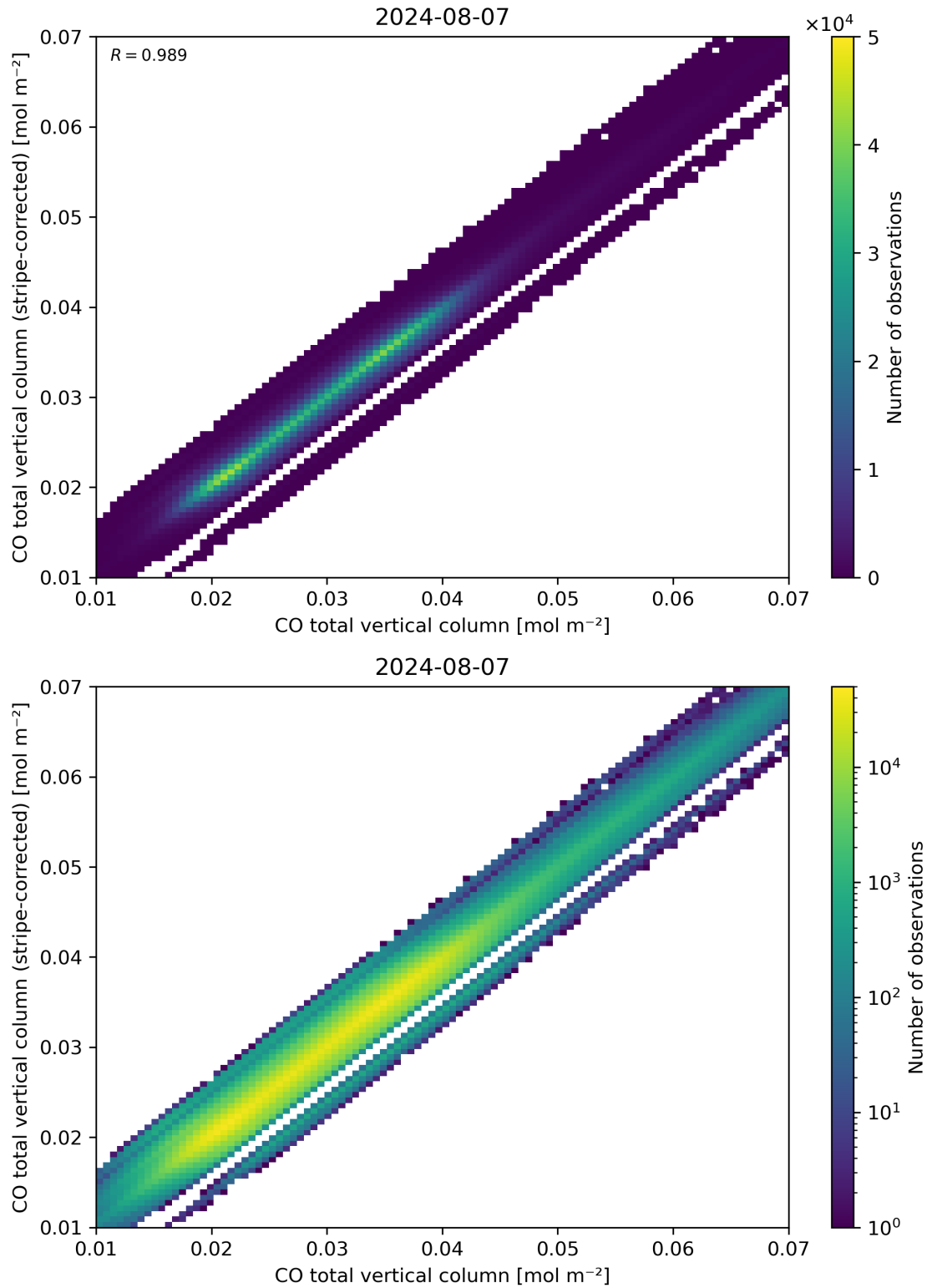
Figure 33: Scatter density plot of “CO total vertical column” against “CO total vertical column (stripe-corrected)” for 2024-08-06 to 2024-08-08.
