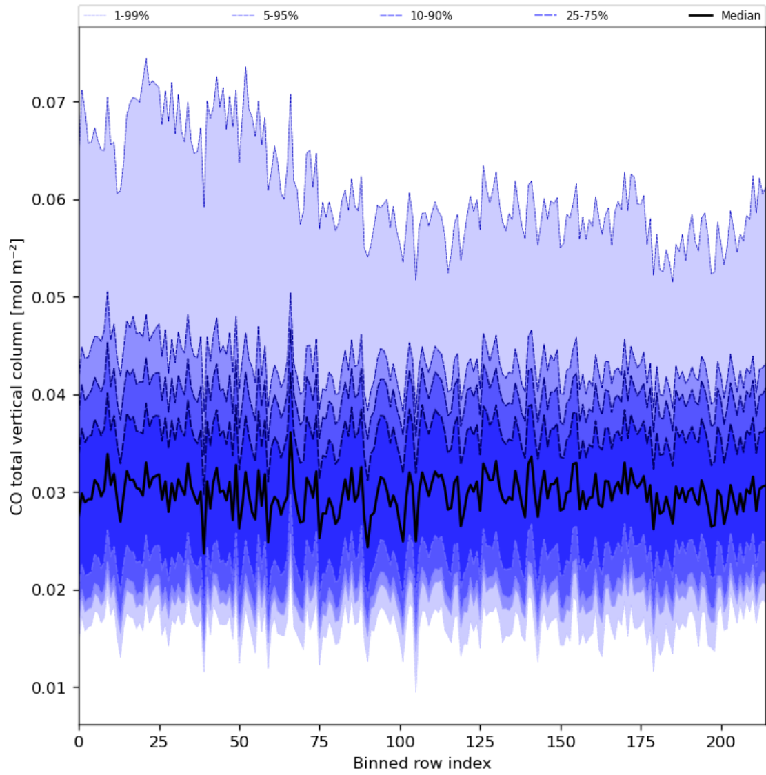
Figure 26: Along track statistics of “CO total vertical column” for 2024-08-06 to 2024-08-08
