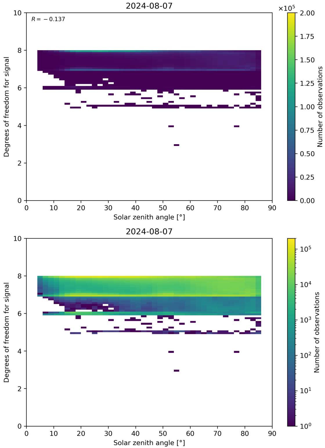
Figure 65: Scatter density plot of “Solar zenith angle” against “Degrees of freedom for signal” for 2024-08-06 to 2024-08-08.
