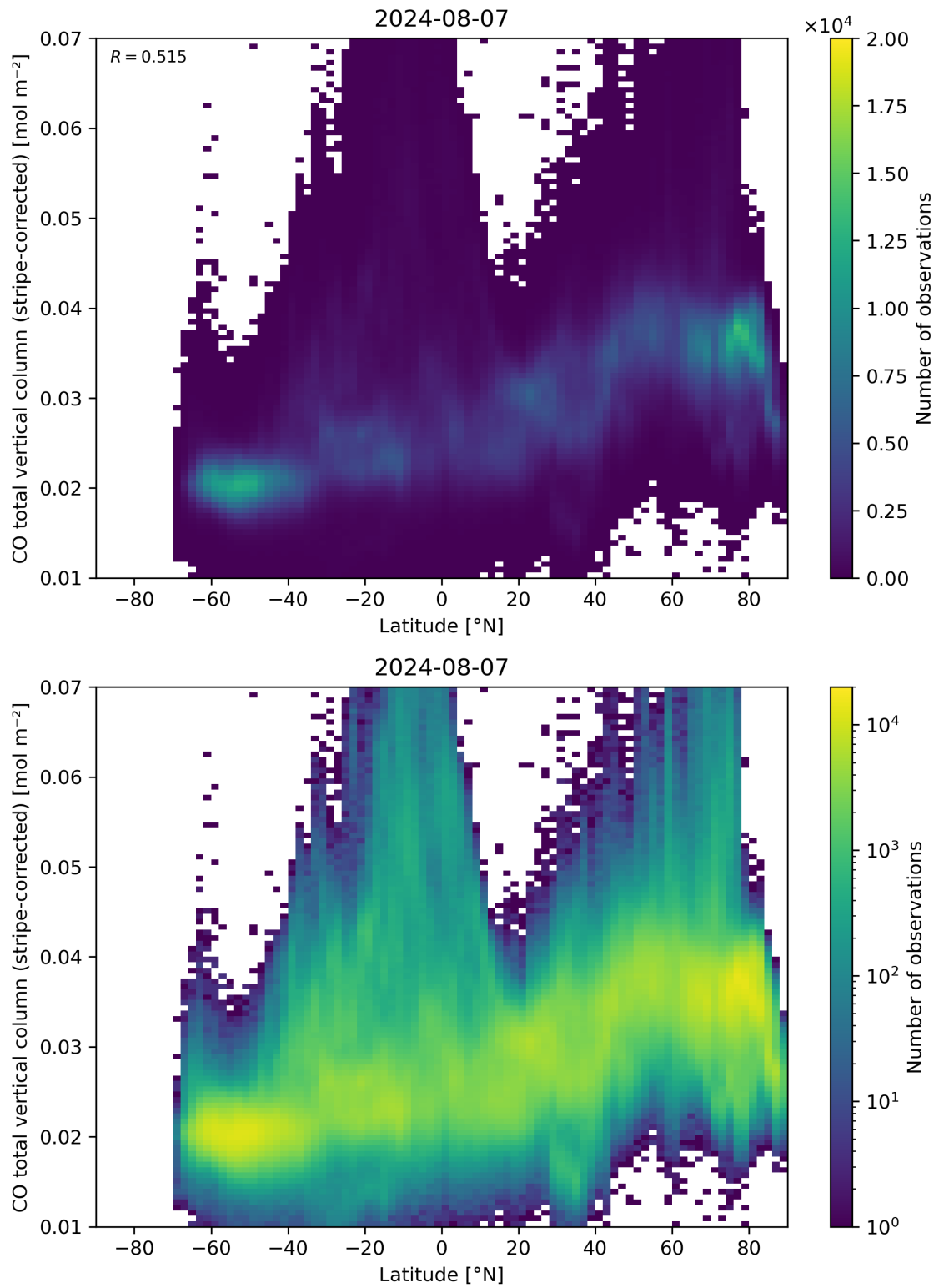
Figure 52: Scatter density plot of “Latitude” against “CO total vertical column (stripe-corrected)” for 2024-08-06 to 2024-08-08.
