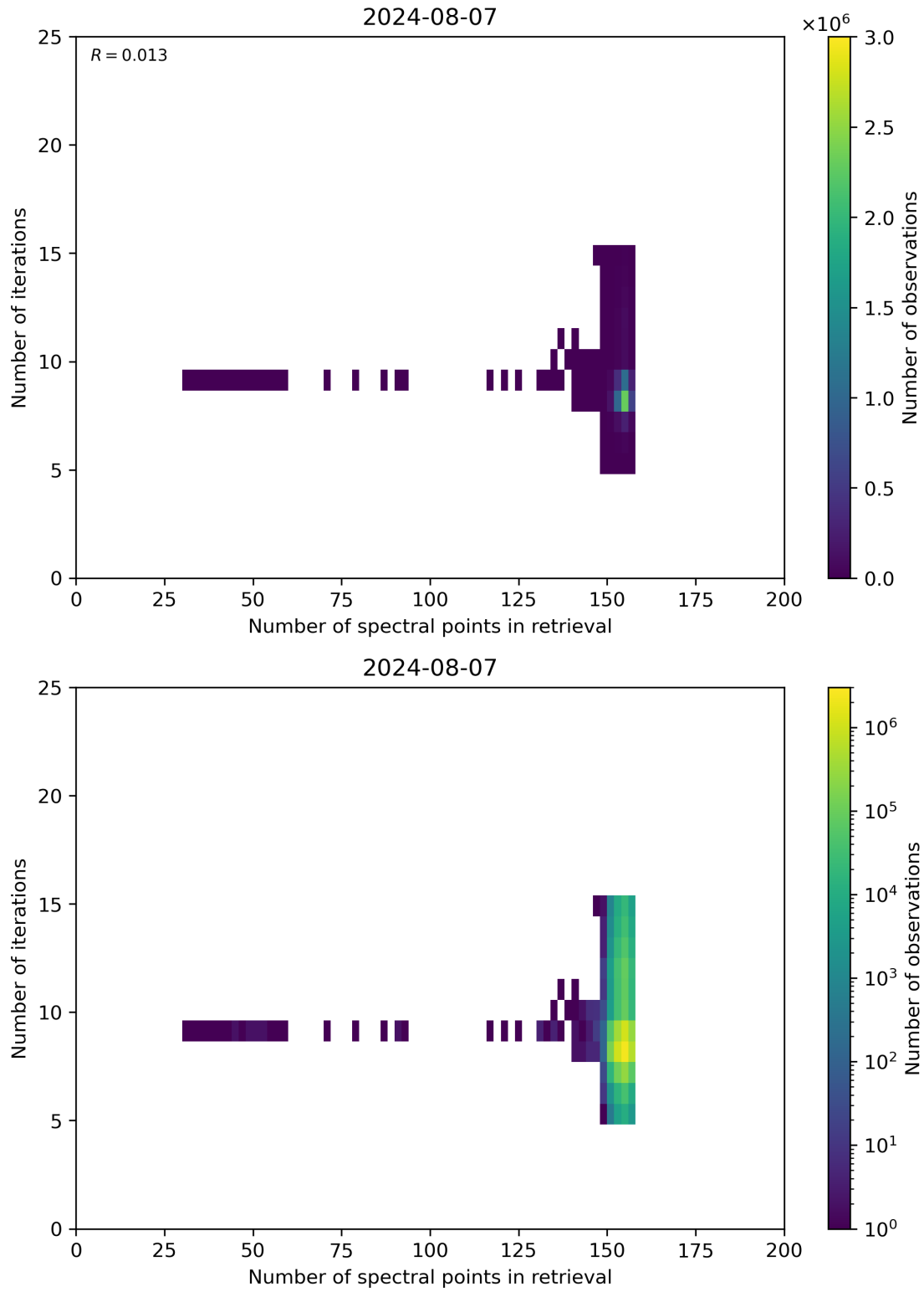
Figure 60: Scatter density plot of “Number of spectral points in retrieval” against “Number of iterations” for 2024-08-06 to 2024-08-08.
