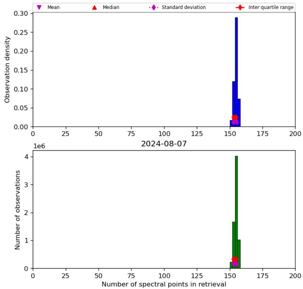
Figure 21: Histogram of “Number of spectral points in retrieval” for 2024-08-06 to 2024-08-08
