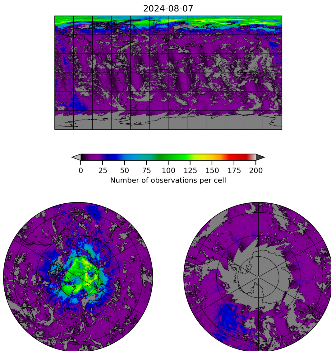
Figure 8: Map of the number of observations for 2024-08-06 to 2024-08-08
