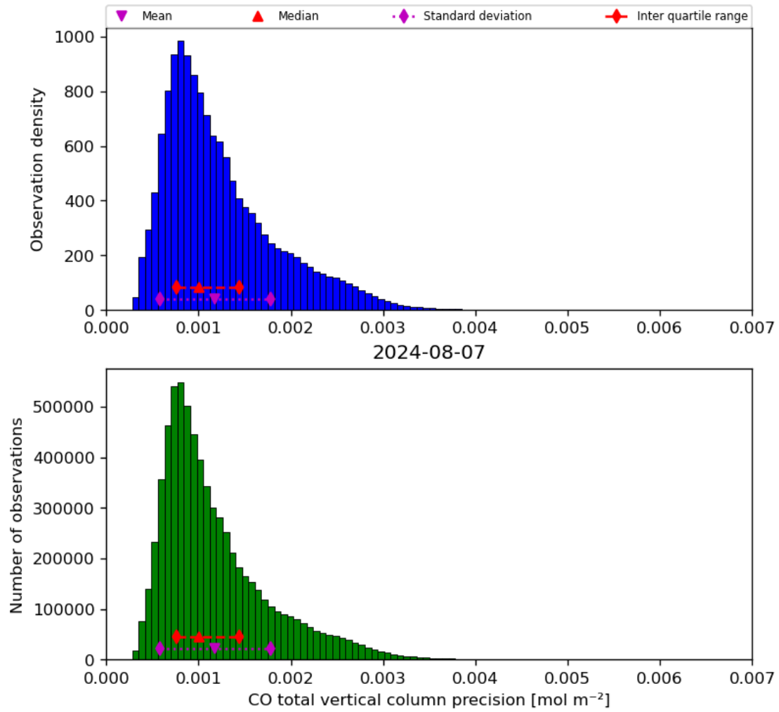
Figure 20: Histogram of “CO total vertical column precision” for 2024-08-06 to 2024-08-08
