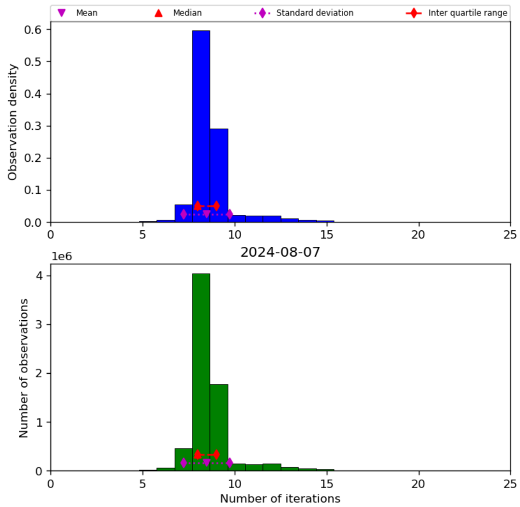
Figure 24: Histogram of “Number of iterations” for 2024-08-06 to 2024-08-08
