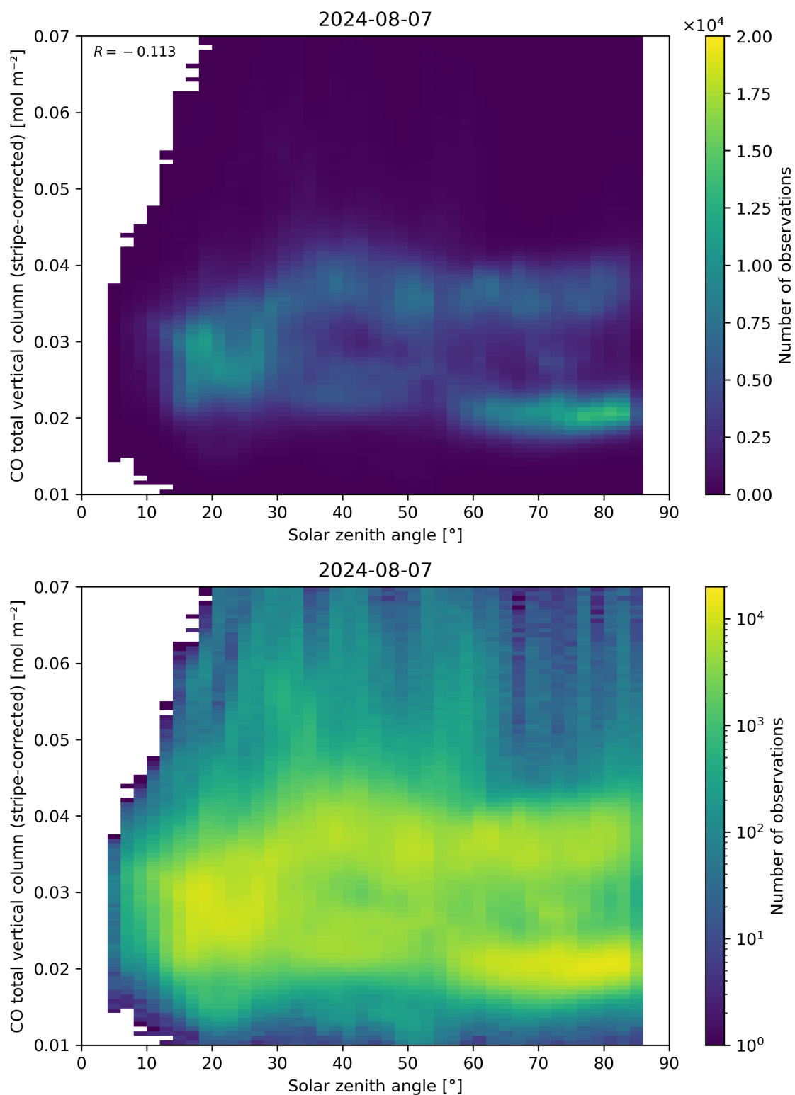
Figure 62: Scatter density plot of “Solar zenith angle” against “CO total vertical column (stripe-corrected)” for 2024-08-06 to 2024-08-08.
