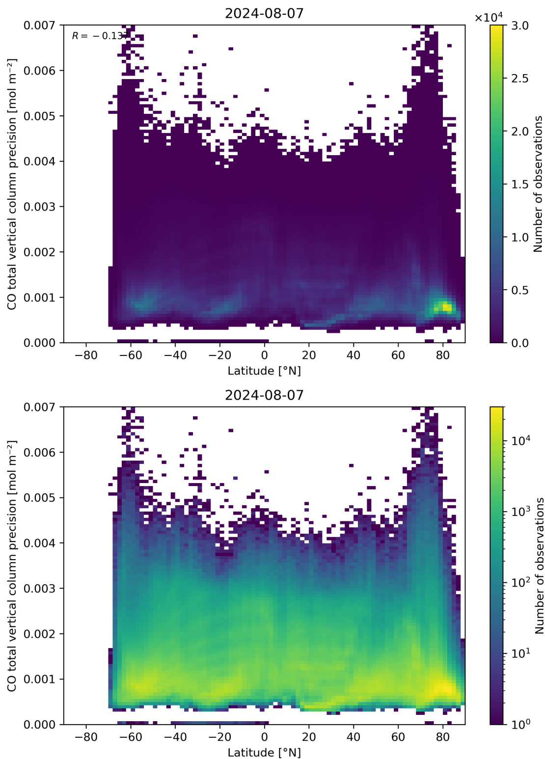
Figure 53: Scatter density plot of “Latitude” against “CO total vertical column precision” for 2024-08-06 to 2024-08-08.
