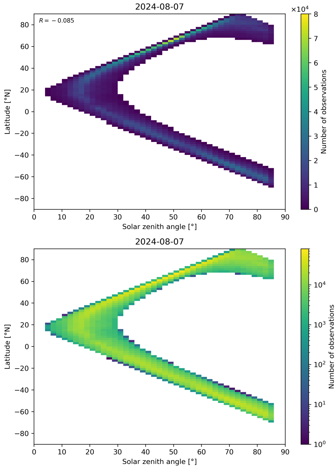
Figure 66: Scatter density plot of “Solar zenith angle” against “Latitude” for 2024-08-06 to 2024-08-08.
