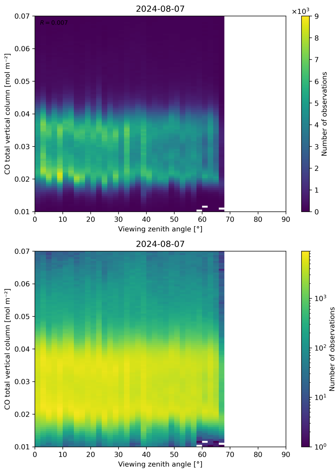
Figure 69: Scatter density plot of “Viewing zenith angle” against “CO total vertical column” for 2024-08-06 to 2024-08-08.
