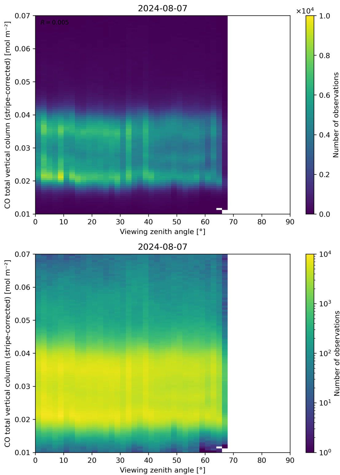
Figure 70: Scatter density plot of “Viewing zenith angle” against “CO total vertical column (stripe-corrected)” for 2024-08-06 to 2024-08-08.
