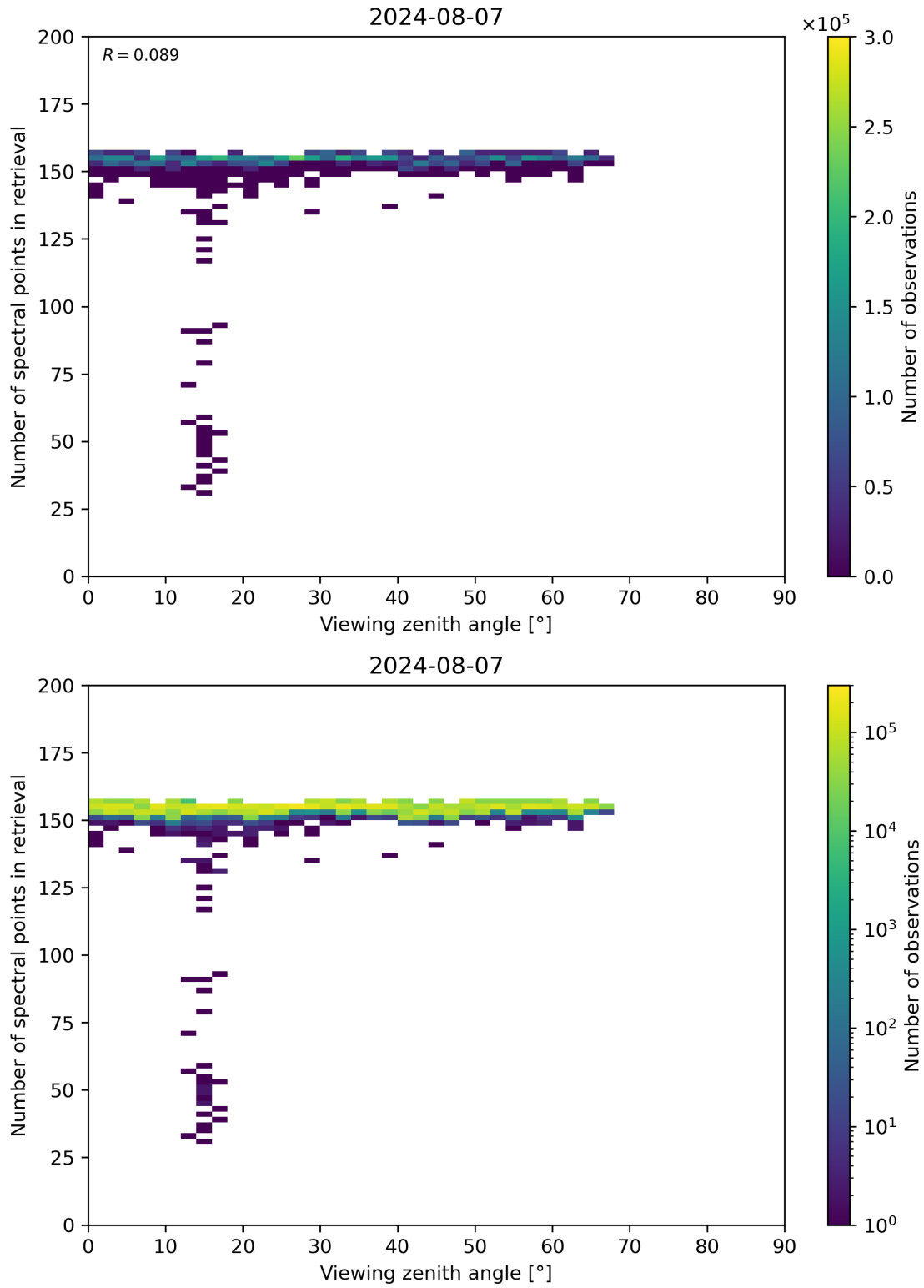
Figure 76: Scatter density plot of “Viewing zenith angle” against “Number of spectral points in retrieval” for 2024-08-06 to 2024-08-08.
