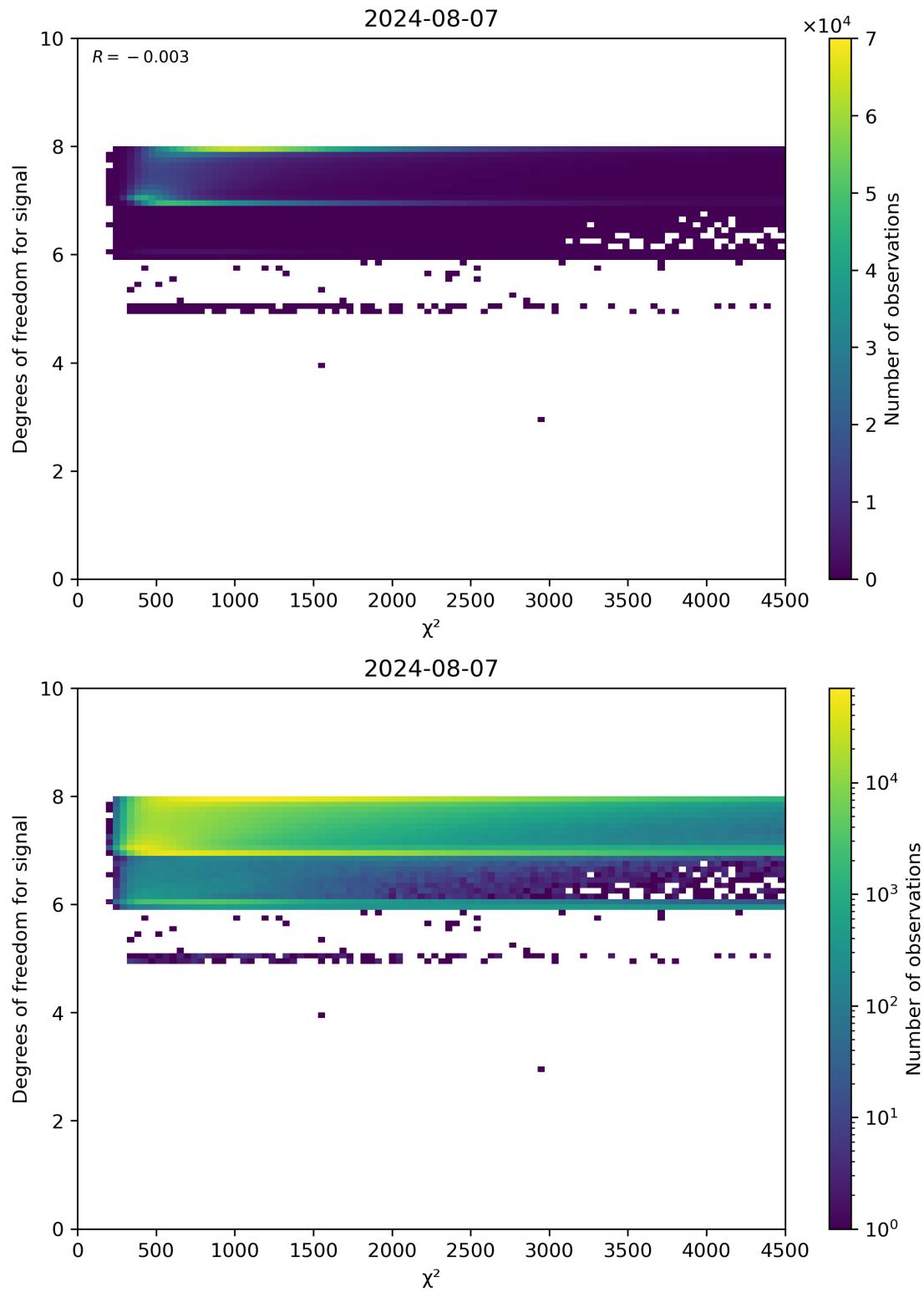
Figure 48: Scatter density plot of “ \chi^2 ” against “Degrees of freedom for signal” for 2024-08-06 to 2024-08-08.
