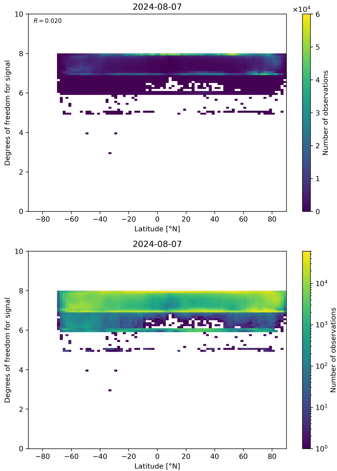
Figure 55: Scatter density plot of “Latitude” against “Degrees of freedom for signal” for 2024-08-06 to 2024-08-08.
