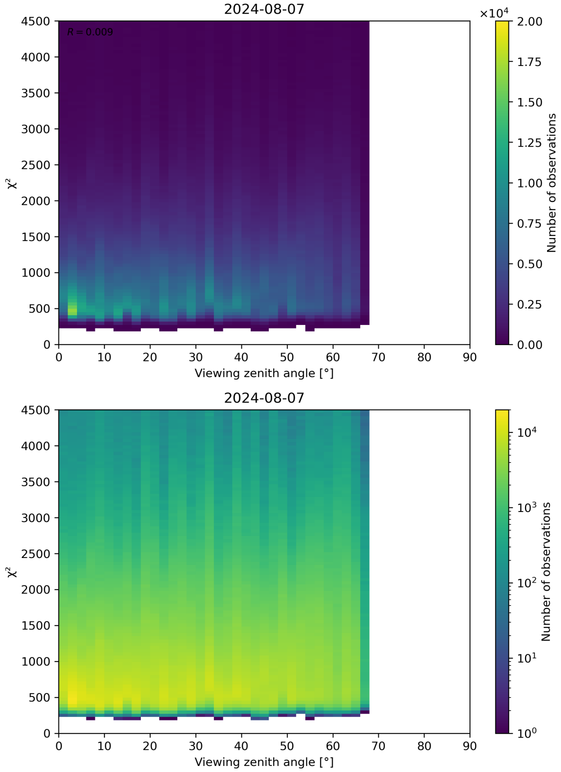
Figure 72: Scatter density plot of “Viewing zenith angle” against “ \chi^2 ” for 2024-08-06 to 2024-08-08.
