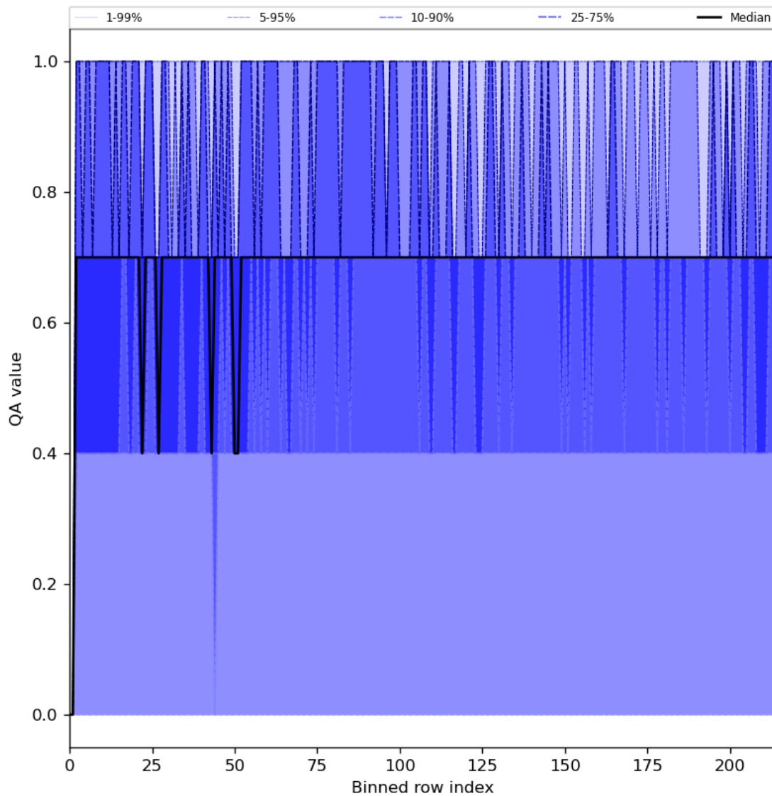
Figure 25: Along track statistics of “QA value” for 2024-08-06 to 2024-08-08
