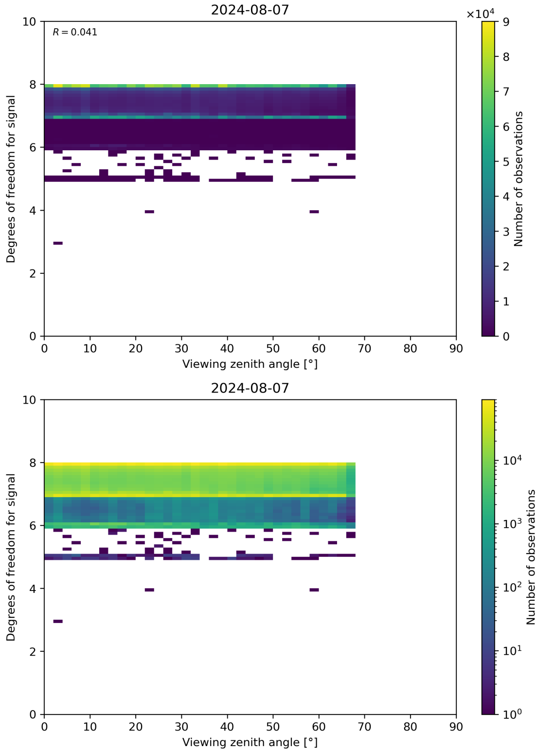
Figure 73: Scatter density plot of “Viewing zenith angle” against “Degrees of freedom for signal” for 2024-08-06 to 2024-08-08.
