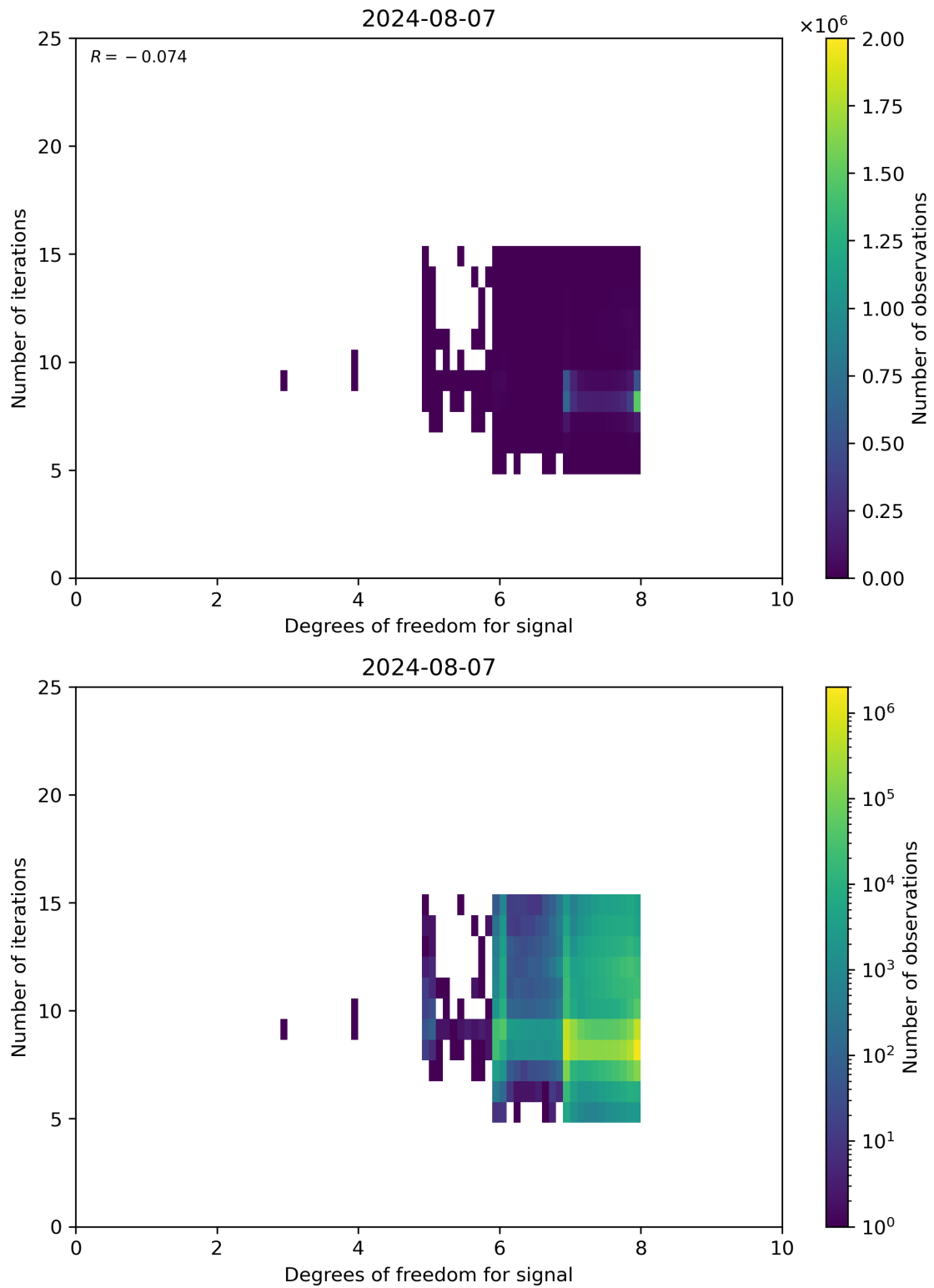
Figure 50: Scatter density plot of “Degrees of freedom for signal” against “Number of iterations” for 2024-08-06 to 2024-08-08.
