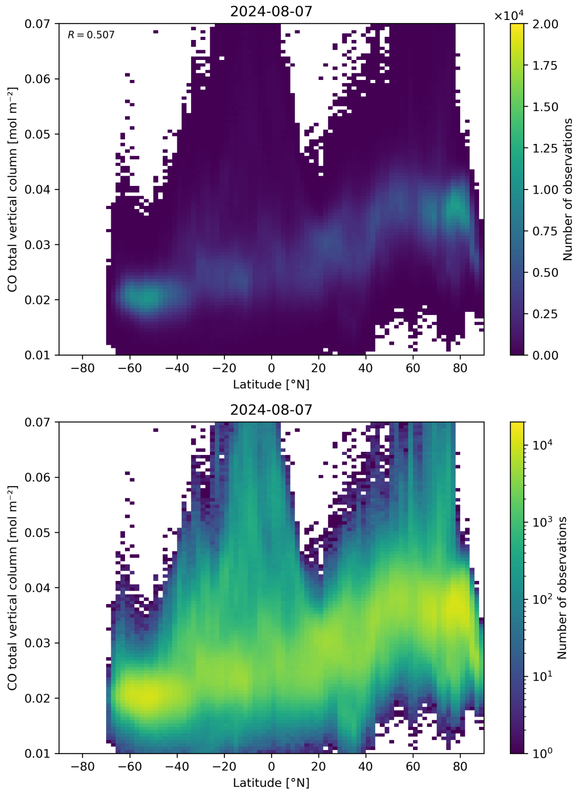
Figure 51: Scatter density plot of “Latitude” against “CO total vertical column” for 2024-08-06 to 2024-08-08.
