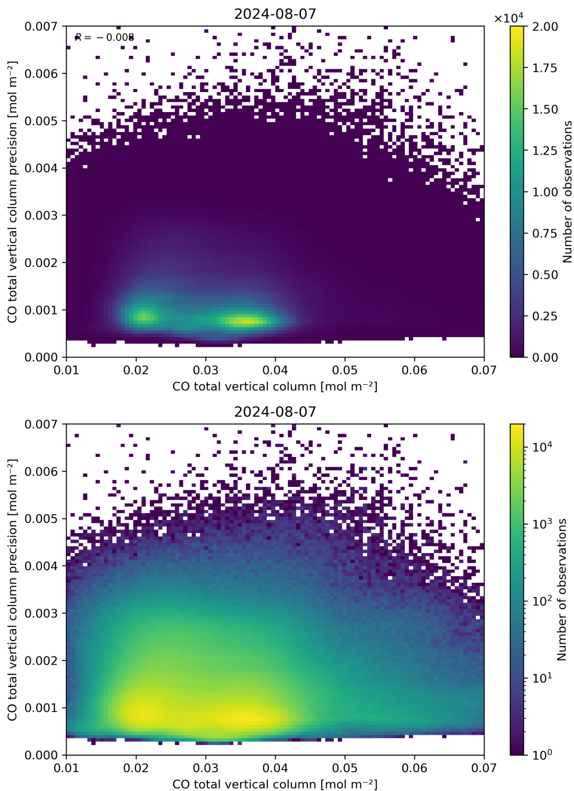
Figure 34: Scatter density plot of “CO total vertical column” against “CO total vertical column precision” for 2024-08-06 to 2024-08-08.
