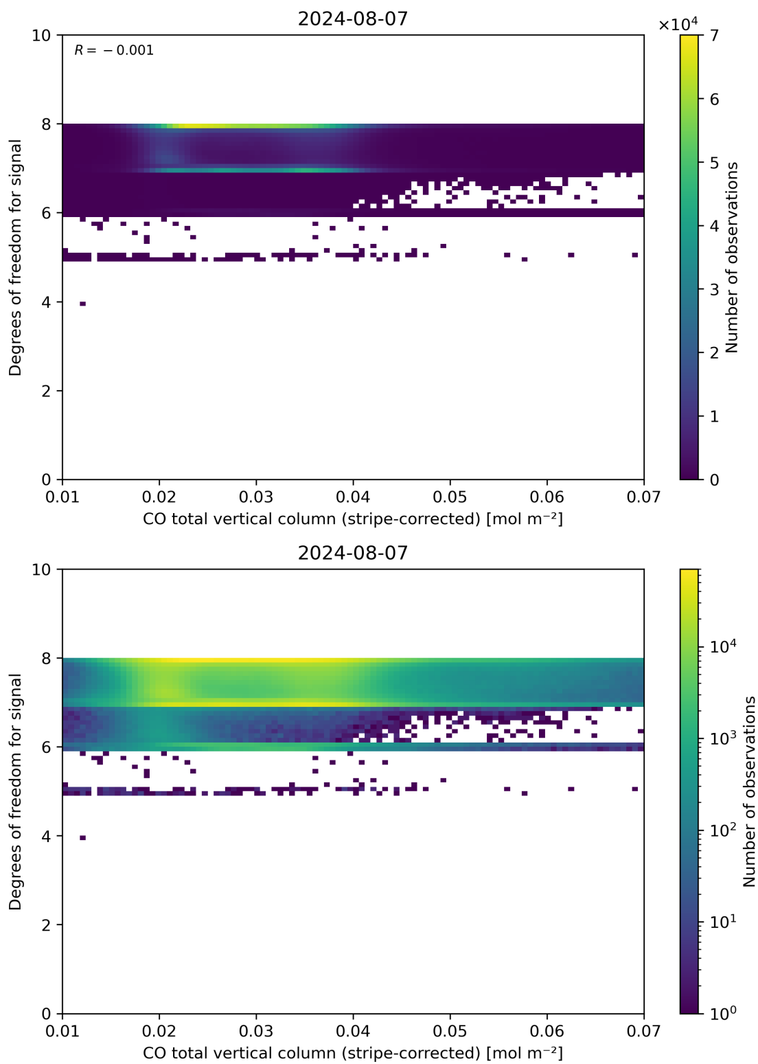
Figure 38: Scatter density plot of “CO total vertical column (stripe-corrected)” against “Degrees of freedom for signal” for 2024-08-06 to 2024-08-08.
