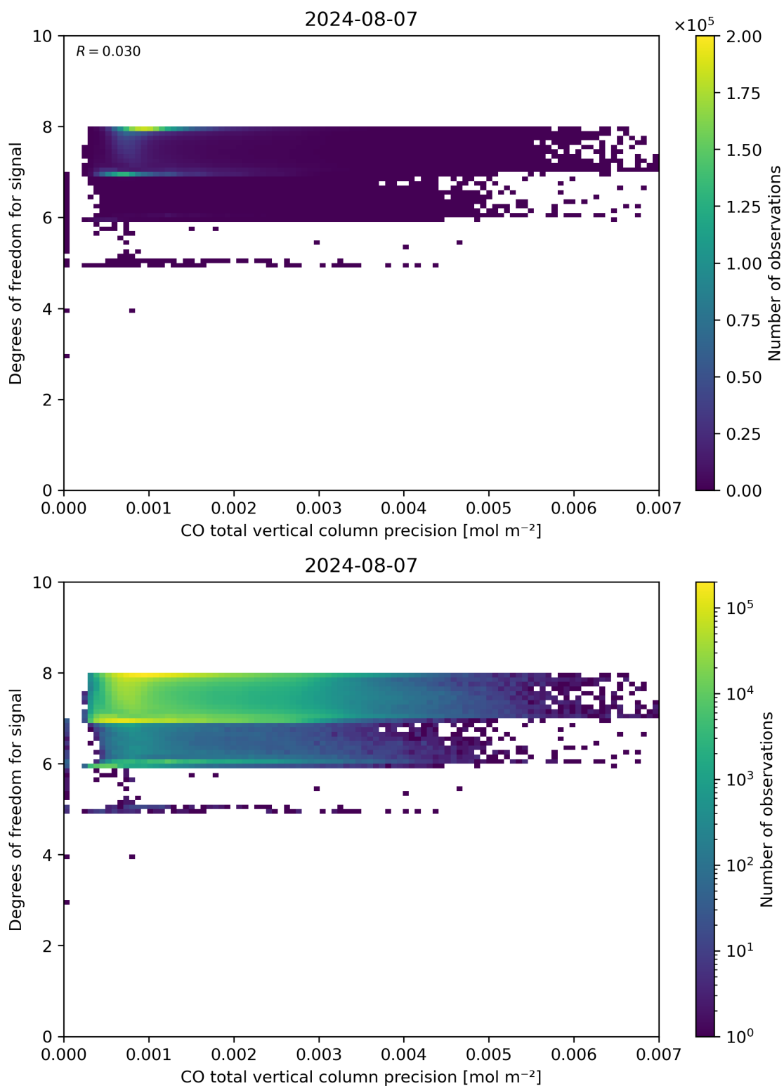
Figure 45: Scatter density plot of “CO total vertical column precision” against “Degrees of freedom for signal” for 2024-08-06 to 2024-08-08.
