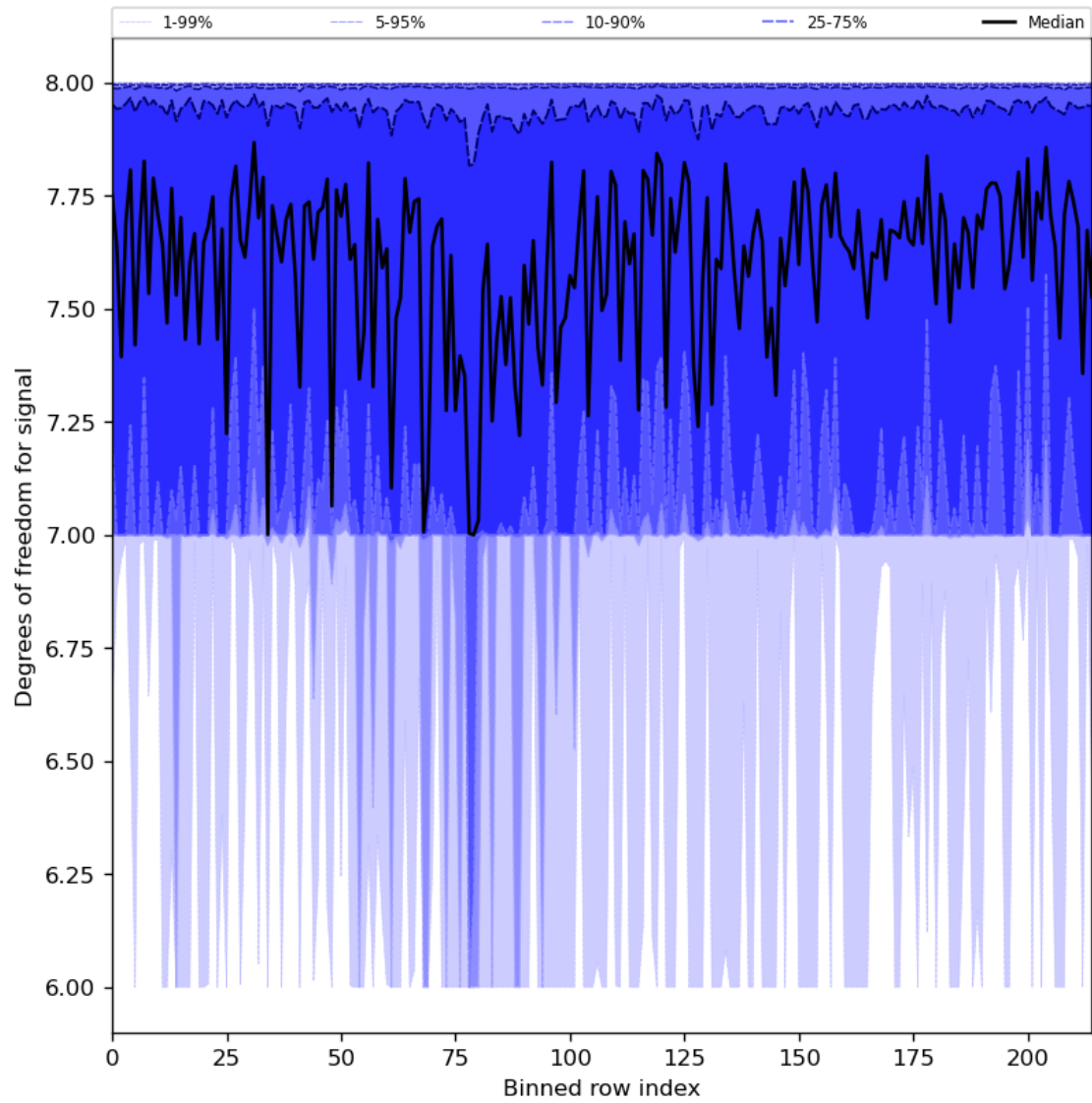
Figure 31: Along track statistics of “Degrees of freedom for signal” for 2024-08-06 to 2024-08-08
