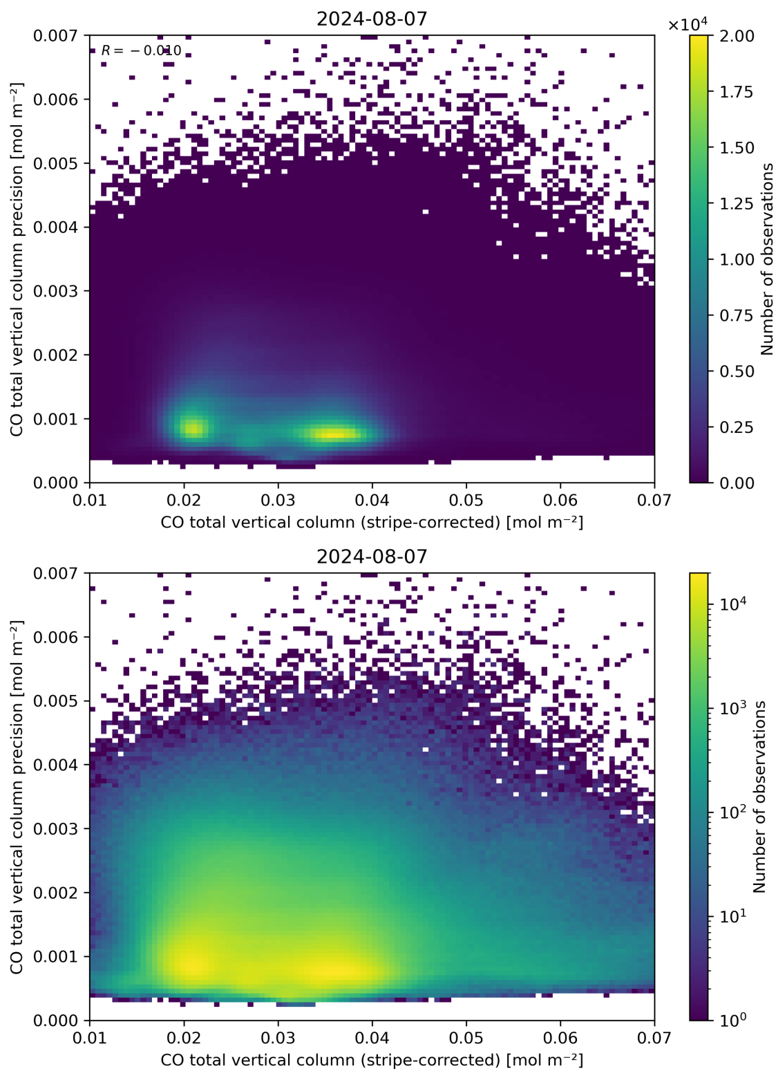
Figure 36: Scatter density plot of “CO total vertical column (stripe-corrected)” against “CO total vertical column precision” for 2024-08-06 to 2024-08-08.
