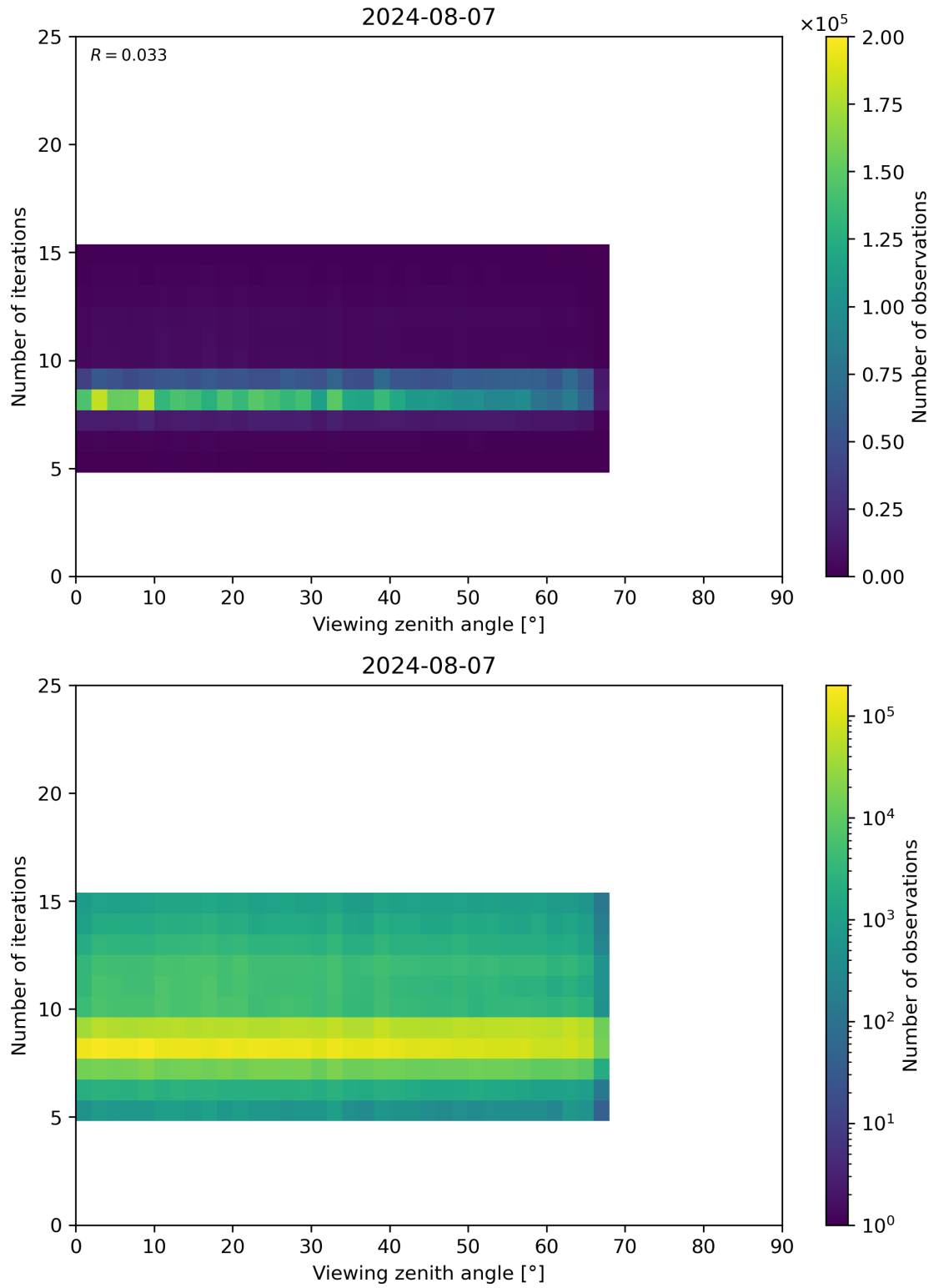
Figure 75: Scatter density plot of “Viewing zenith angle” against “Number of iterations” for 2024-08-06 to 2024-08-08.
