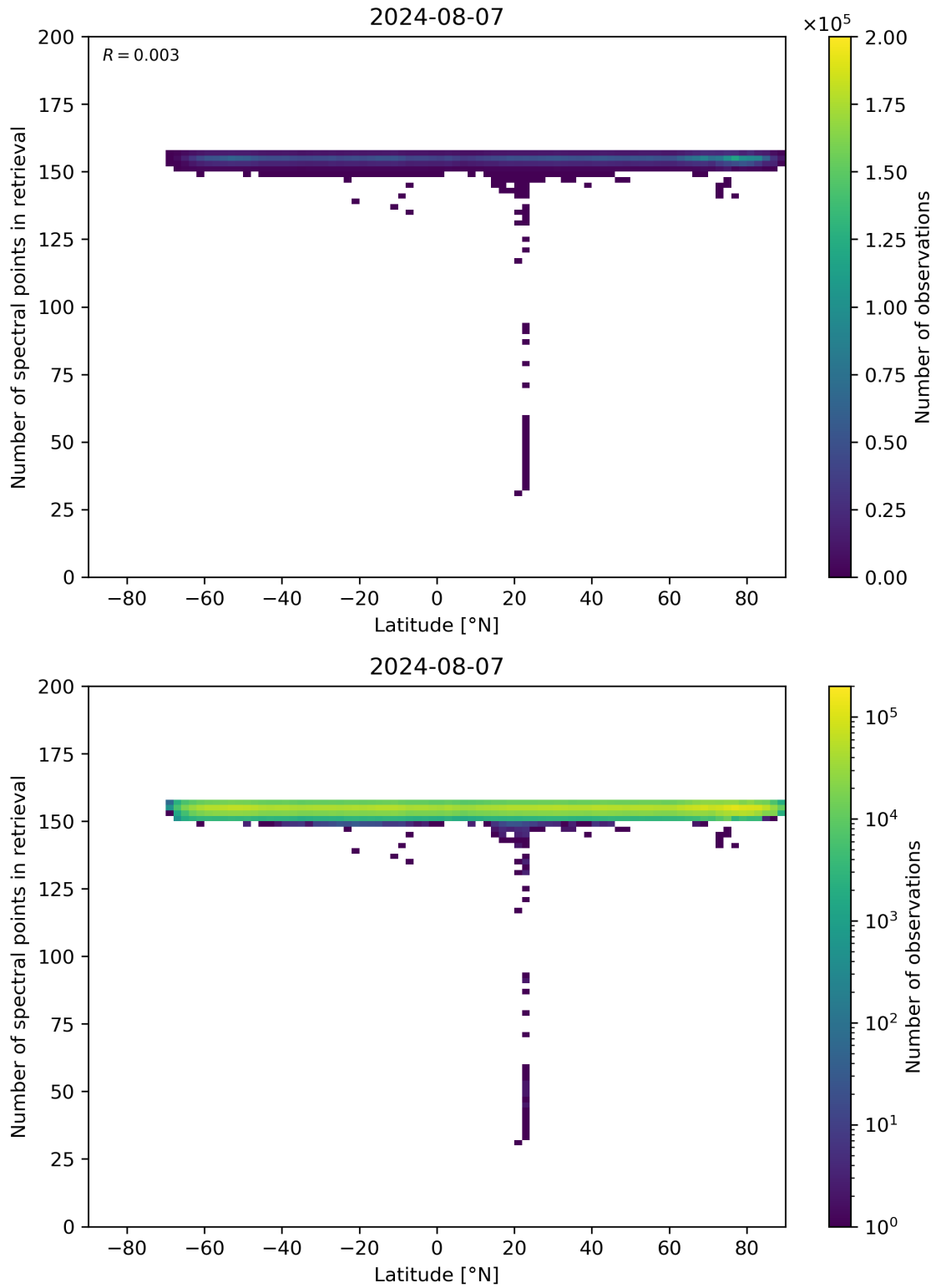
Figure 57: Scatter density plot of “Latitude” against “Number of spectral points in retrieval” for 2024-08-06 to 2024-08-08.
