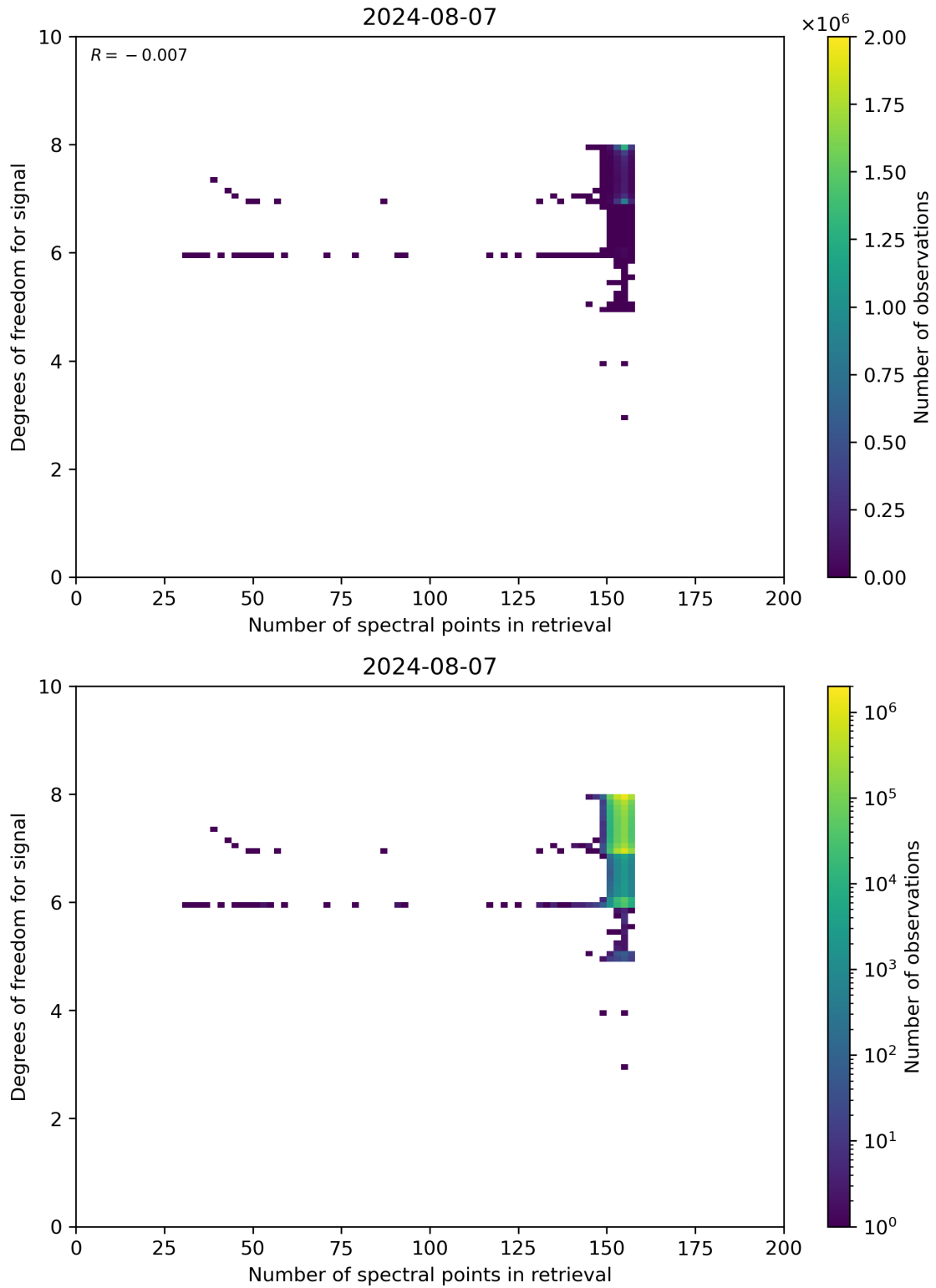
Figure 59: Scatter density plot of “Number of spectral points in retrieval” against “Degrees of freedom for signal” for 2024-08-06 to 2024-08-08.
