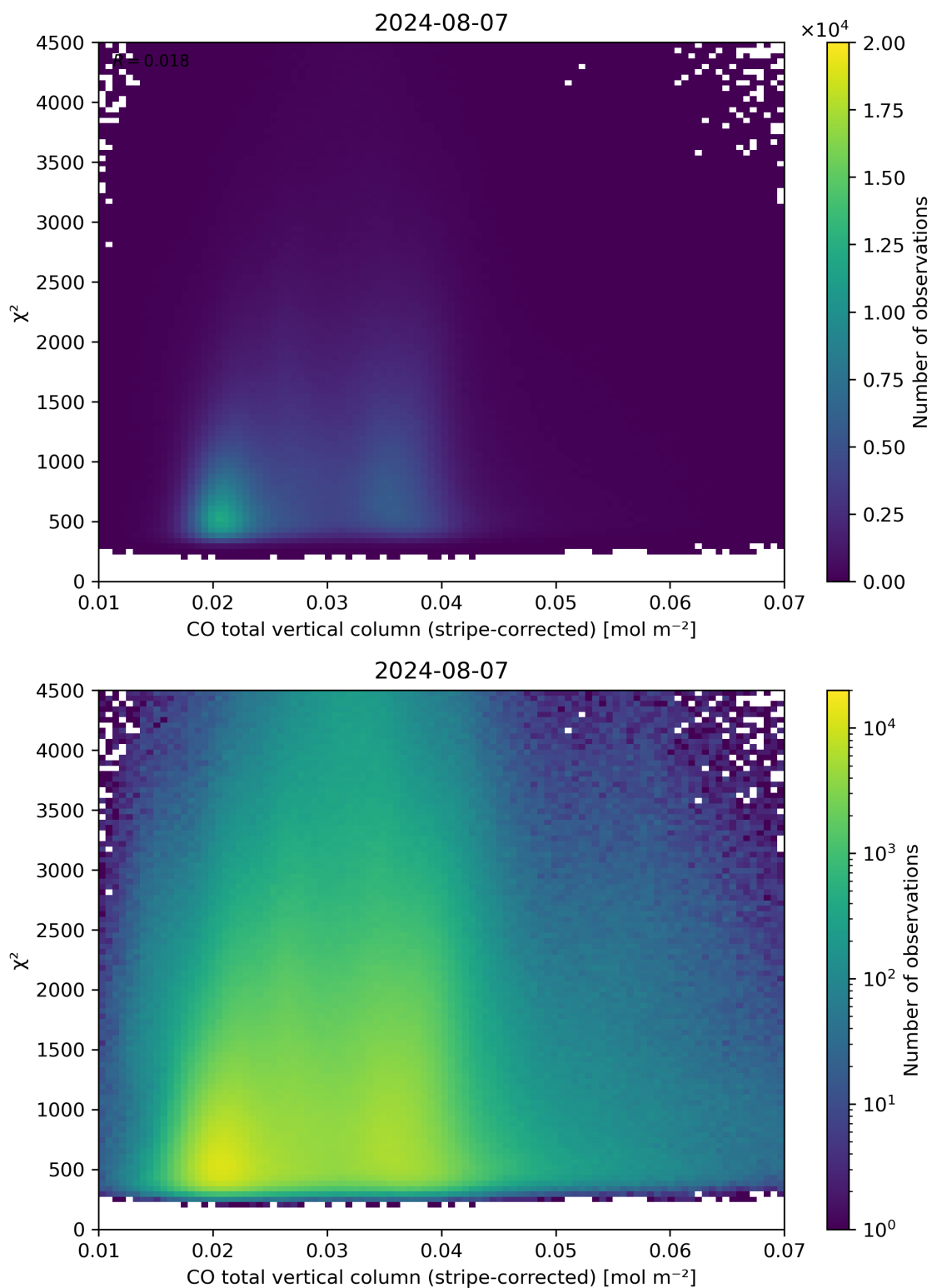
Figure 37: Scatter density plot of “CO total vertical column (stripe-corrected)” against “ \chi^2 ” for 2024-08-06 to 2024-08-08.
