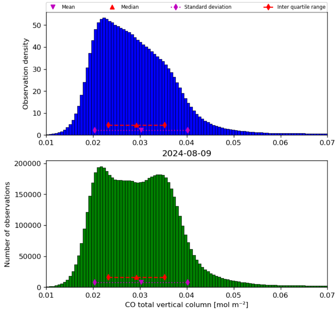
Figure 18: Histogram of “CO total vertical column” for 2024-08-08 to 2024-08-10
