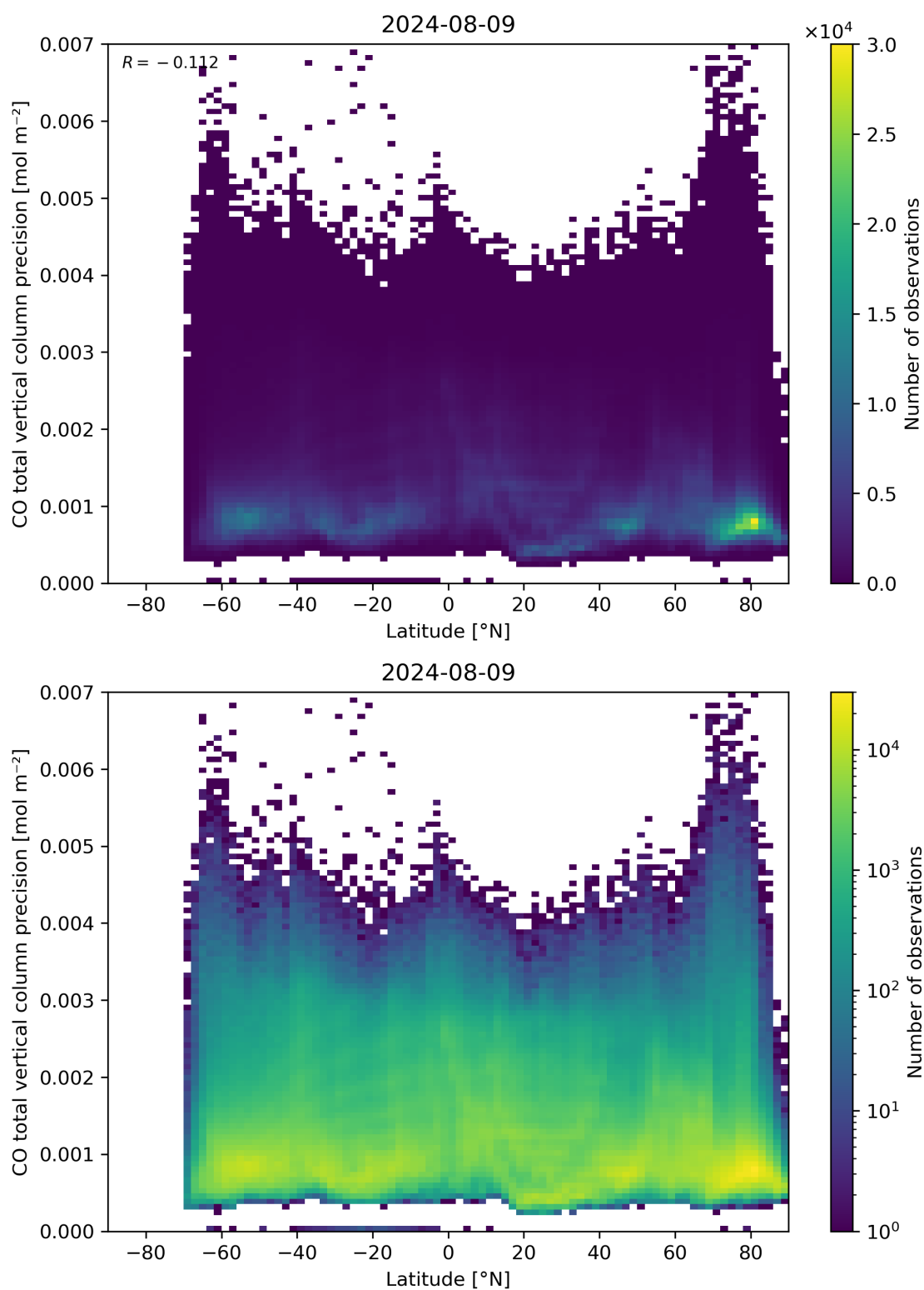
Figure 53: Scatter density plot of “Latitude” against “CO total vertical column precision” for 2024-08-08 to 2024-08-10.
