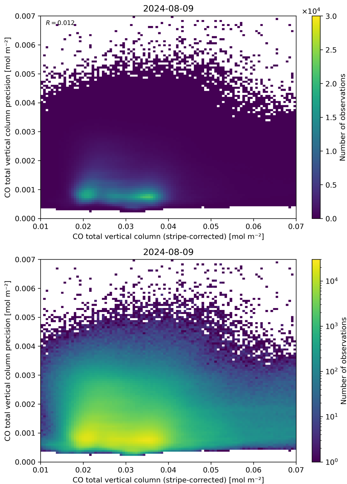
Figure 36: Scatter density plot of “CO total vertical column (stripe-corrected)” against “CO total vertical column precision” for 2024-08-08 to 2024-08-10.
