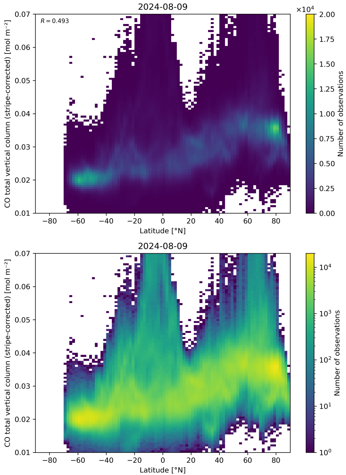
Figure 52: Scatter density plot of “Latitude” against “CO total vertical column (stripe-corrected)” for 2024-08-08 to 2024-08-10.
