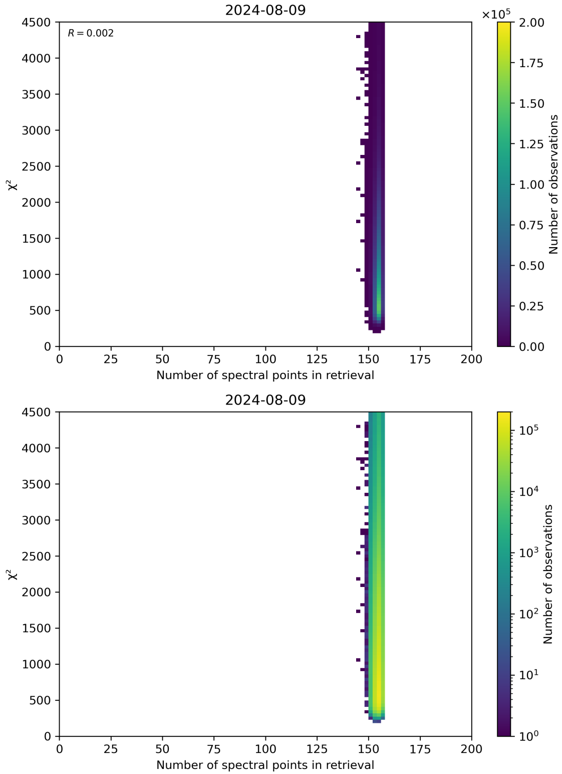
Figure 58: Scatter density plot of “Number of spectral points in retrieval” against “ \chi^2 ” for 2024-08-08 to 2024-08-10.
