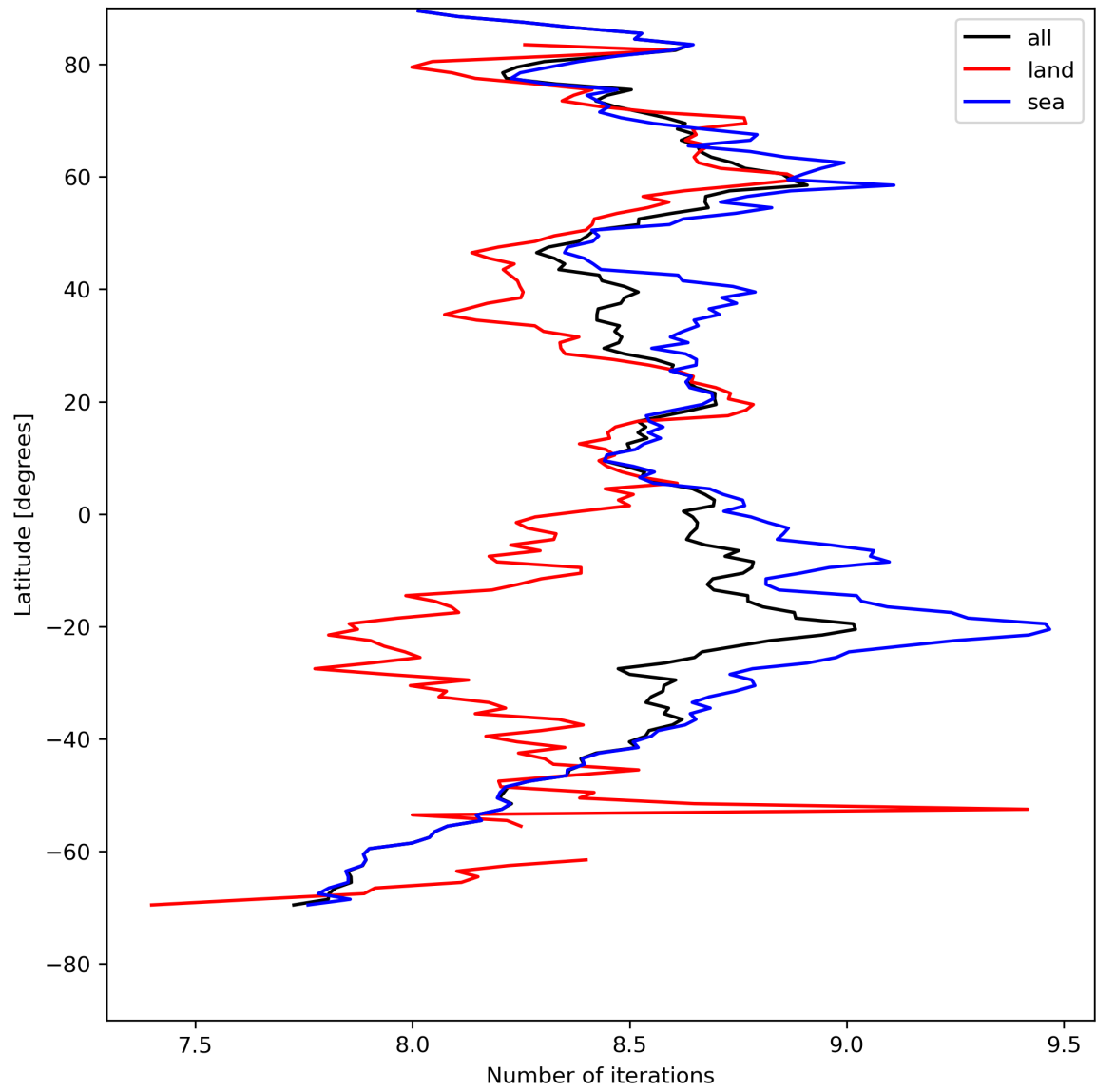
Figure 16: Zonal average of “Number of iterations” for 2024-08-08 to 2024-08-10.
