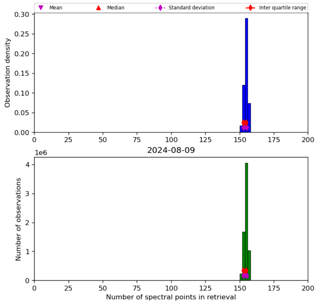
Figure 21: Histogram of “Number of spectral points in retrieval” for 2024-08-08 to 2024-08-10
