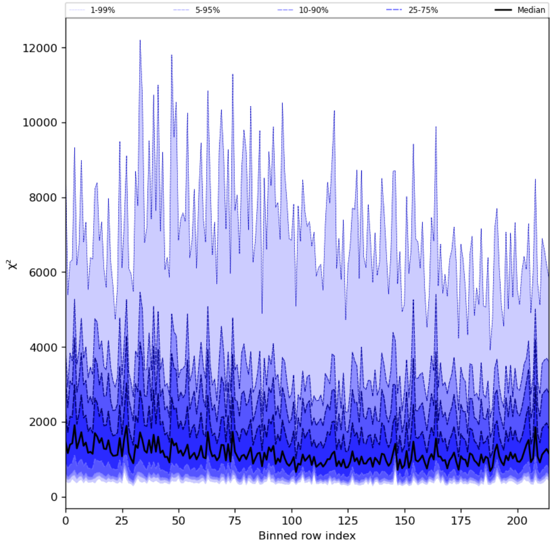
Figure 30: Along track statistics of “ \chi^2 ” for 2024-08-08 to 2024-08-10
