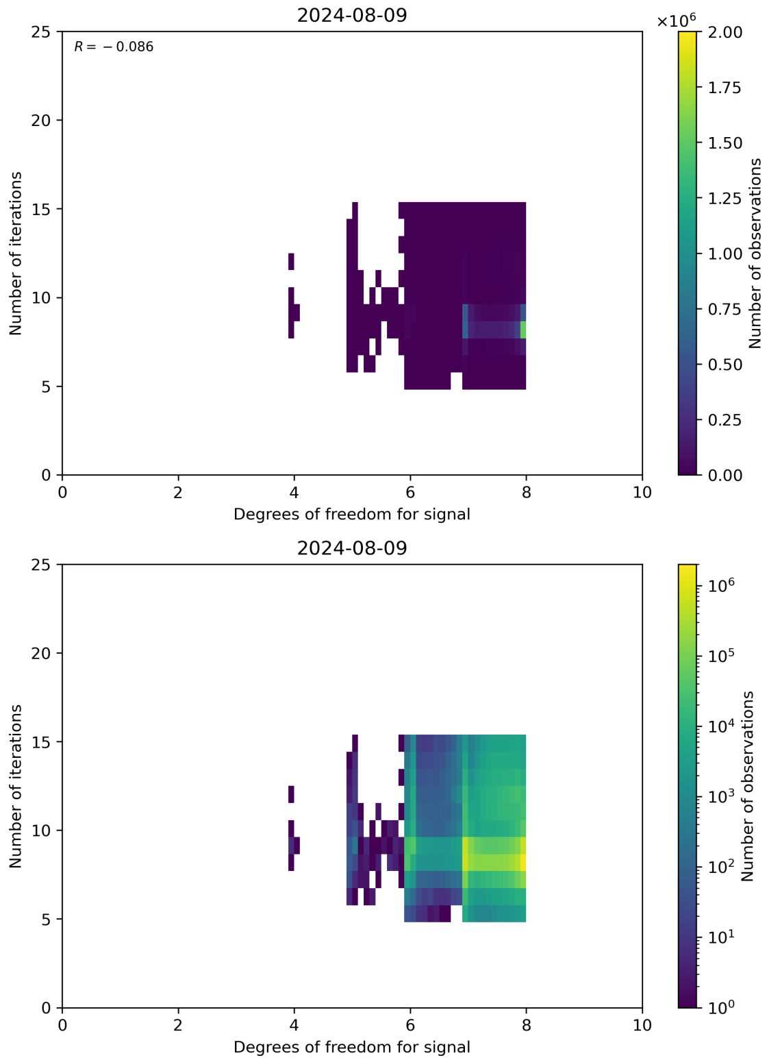
Figure 50: Scatter density plot of “Degrees of freedom for signal” against “Number of iterations” for 2024-08-08 to 2024-08-10.
