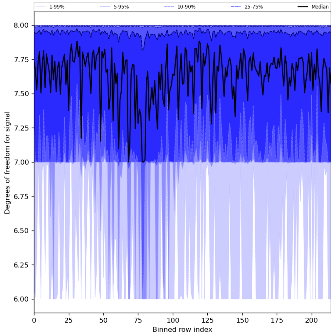
Figure 31: Along track statistics of “Degrees of freedom for signal” for 2024-08-08 to 2024-08-10
