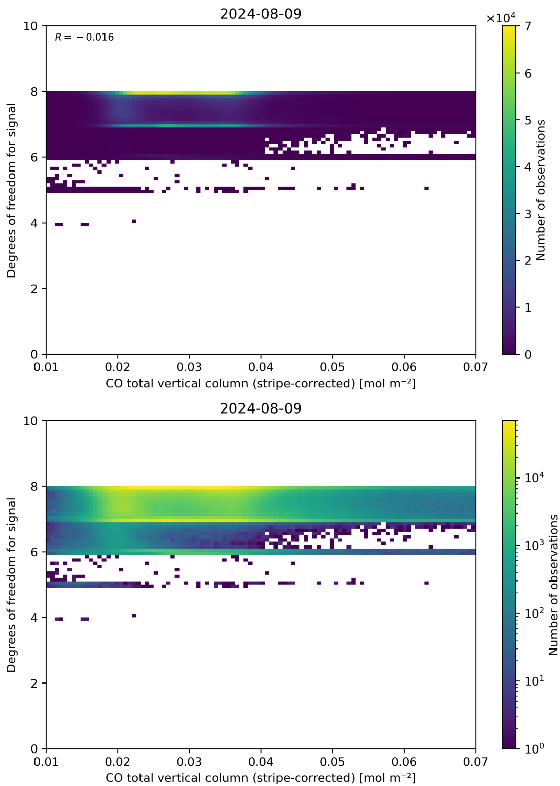
Figure 38: Scatter density plot of “CO total vertical column (stripe-corrected)” against “Degrees of freedom for signal” for 2024-08-08 to 2024-08-10.
