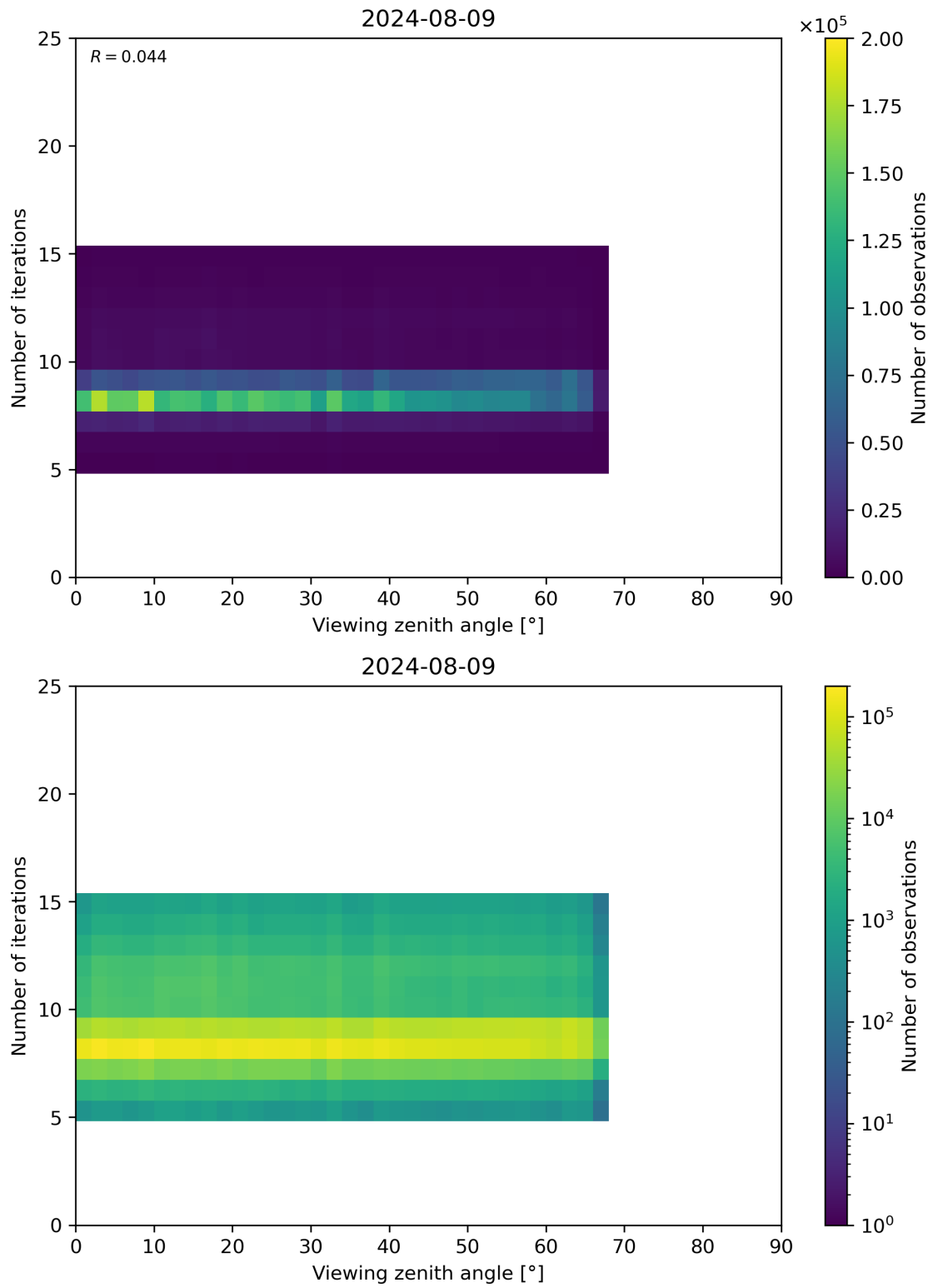
Figure 75: Scatter density plot of “Viewing zenith angle” against “Number of iterations” for 2024-08-08 to 2024-08-10.
