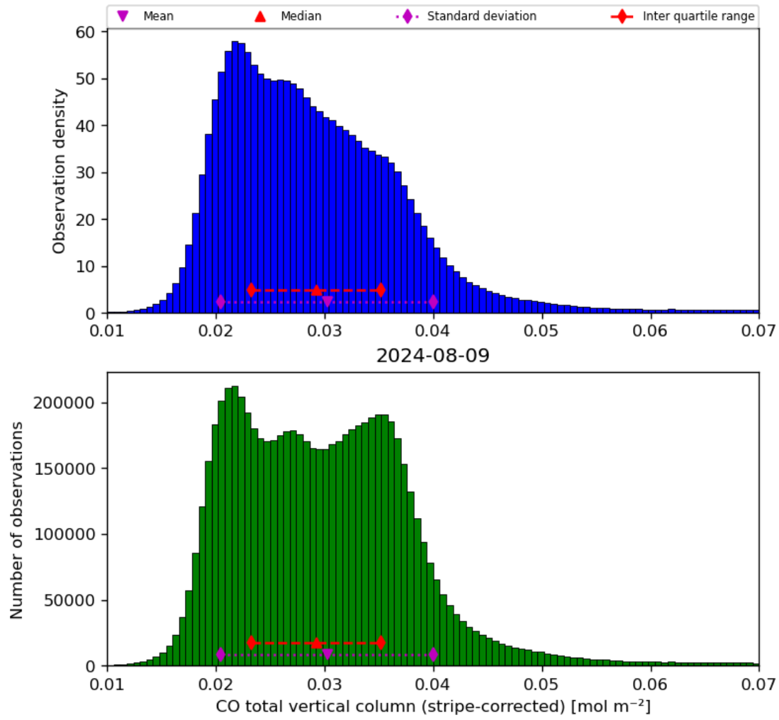
Figure 19: Histogram of “CO total vertical column (stripe-corrected)” for 2024-08-08 to 2024-08-10
