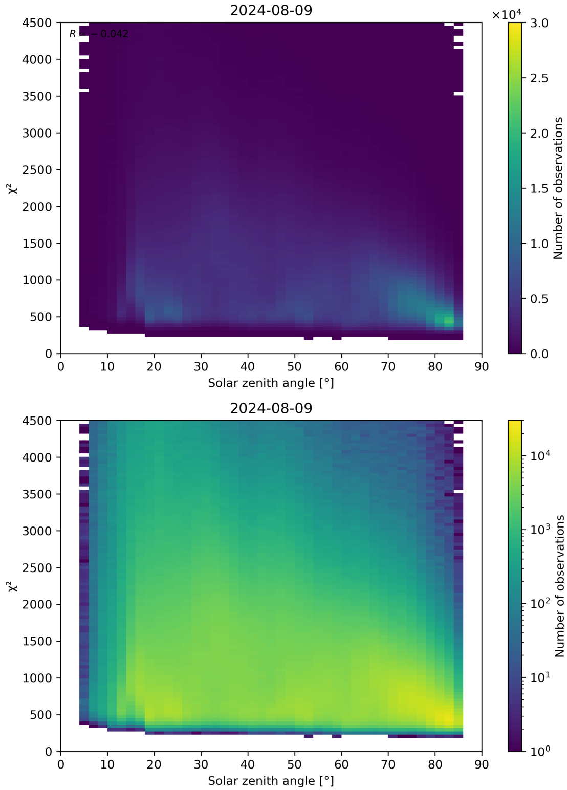
Figure 64: Scatter density plot of “Solar zenith angle” against “ \chi^2 ” for 2024-08-08 to 2024-08-10.
