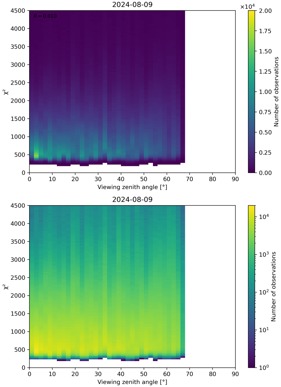
Figure 72: Scatter density plot of “Viewing zenith angle” against “ \chi^2 ” for 2024-08-08 to 2024-08-10.
