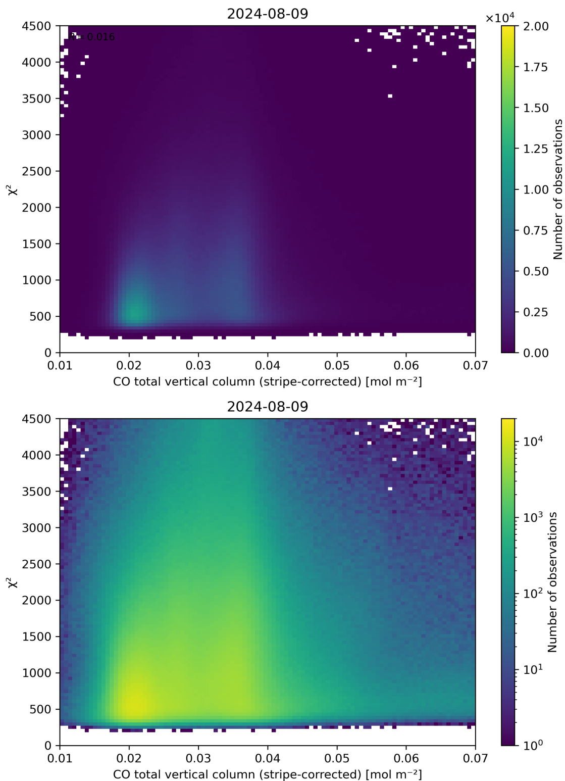
Figure 37: Scatter density plot of “CO total vertical column (stripe-corrected)” against “ \chi^2 ” for 2024-08-08 to 2024-08-10.
