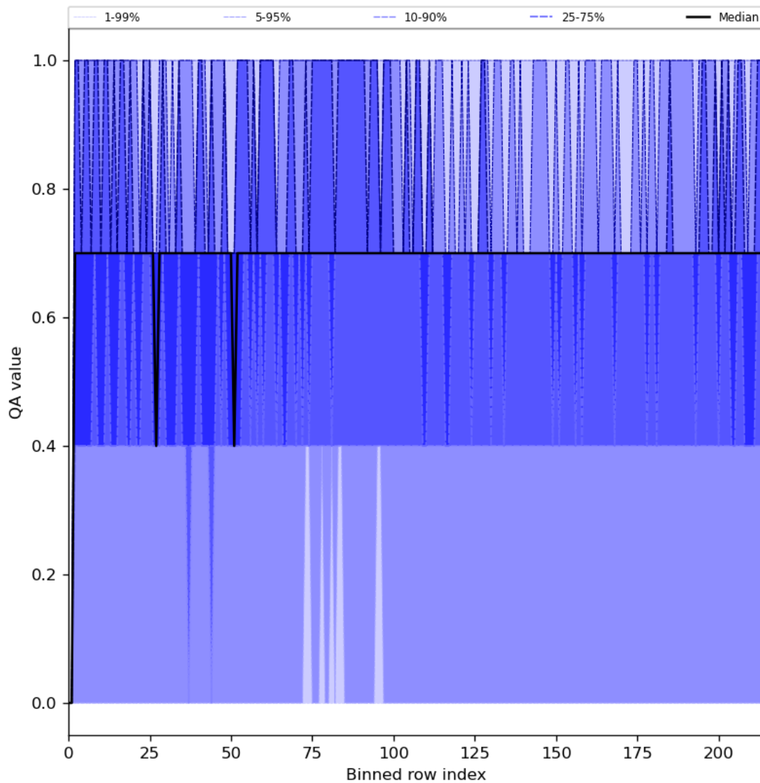
Figure 25: Along track statistics of “QA value” for 2024-08-08 to 2024-08-10
