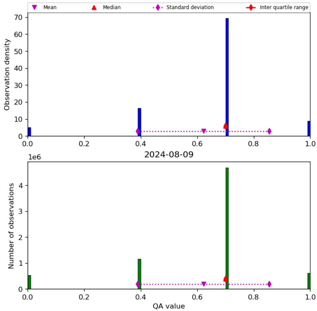
Figure 17: Histogram of “QA value” for 2024-08-08 to 2024-08-10
