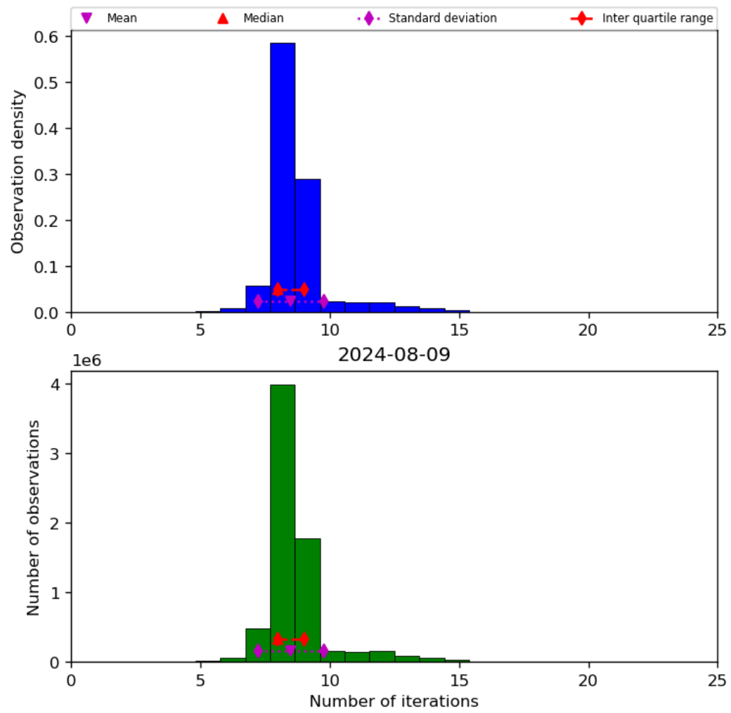
Figure 24: Histogram of “Number of iterations” for 2024-08-08 to 2024-08-10
