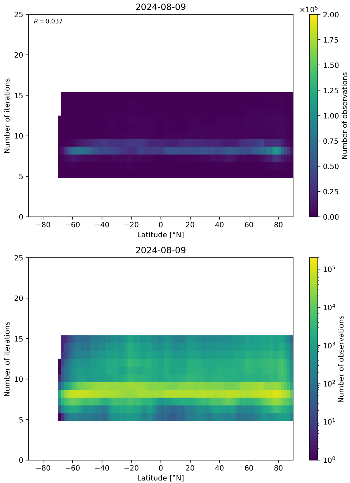
Figure 56: Scatter density plot of “Latitude” against “Number of iterations” for 2024-08-08 to 2024-08-10.
