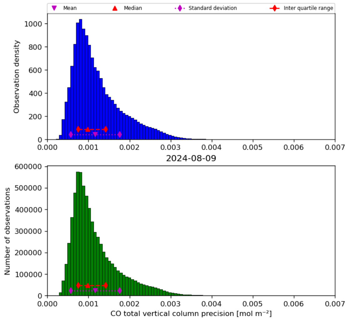
Figure 20: Histogram of “CO total vertical column precision” for 2024-08-08 to 2024-08-10
