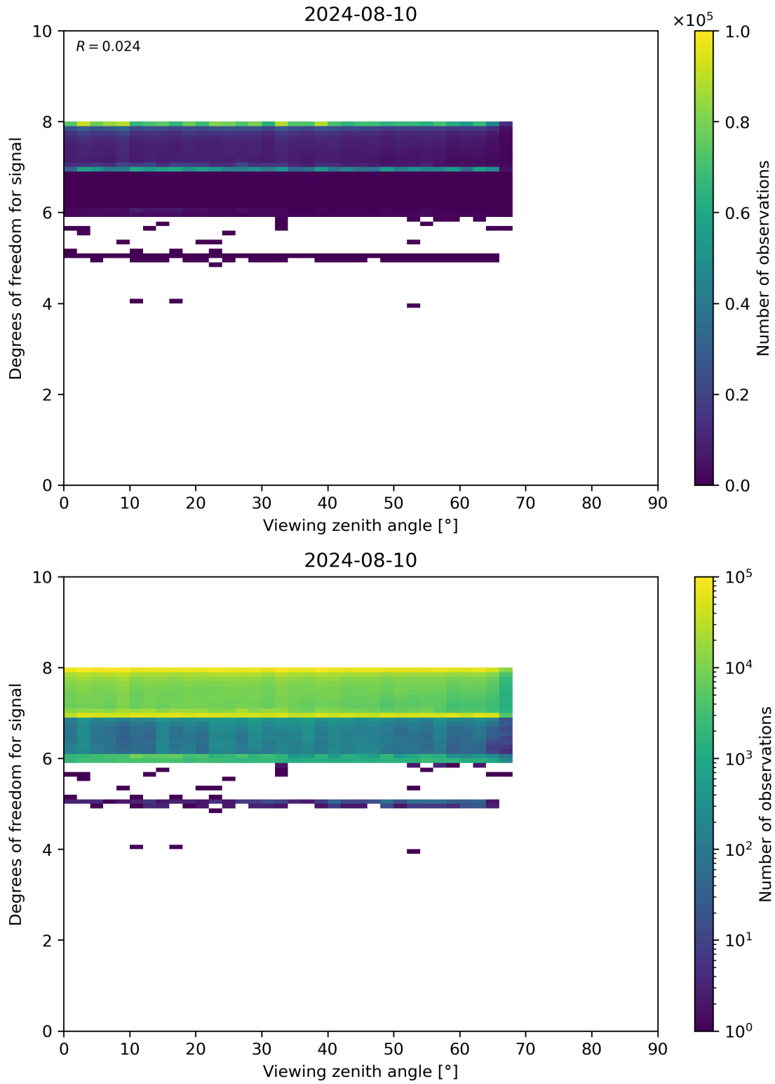
Figure 73: Scatter density plot of “Viewing zenith angle” against “Degrees of freedom for signal” for 2024-08-09 to 2024-08-11.
