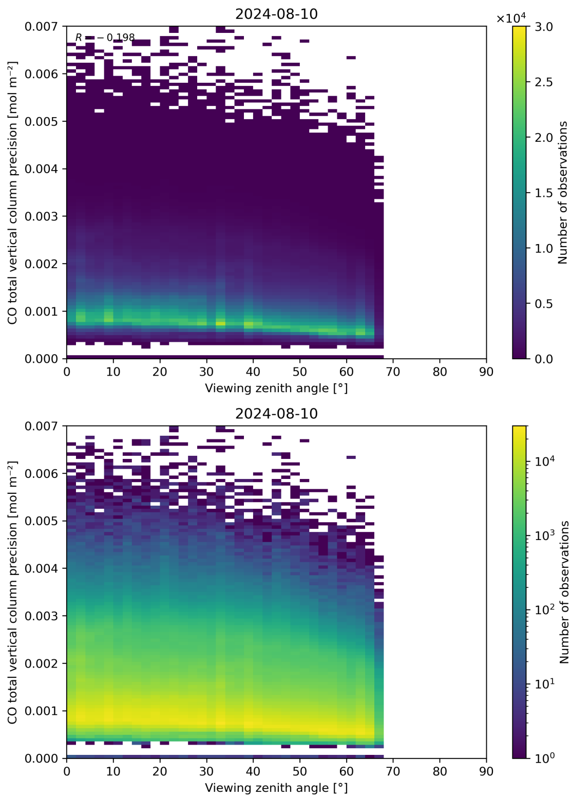
Figure 71: Scatter density plot of “Viewing zenith angle” against “CO total vertical column precision” for 2024-08-09 to 2024-08-11.
