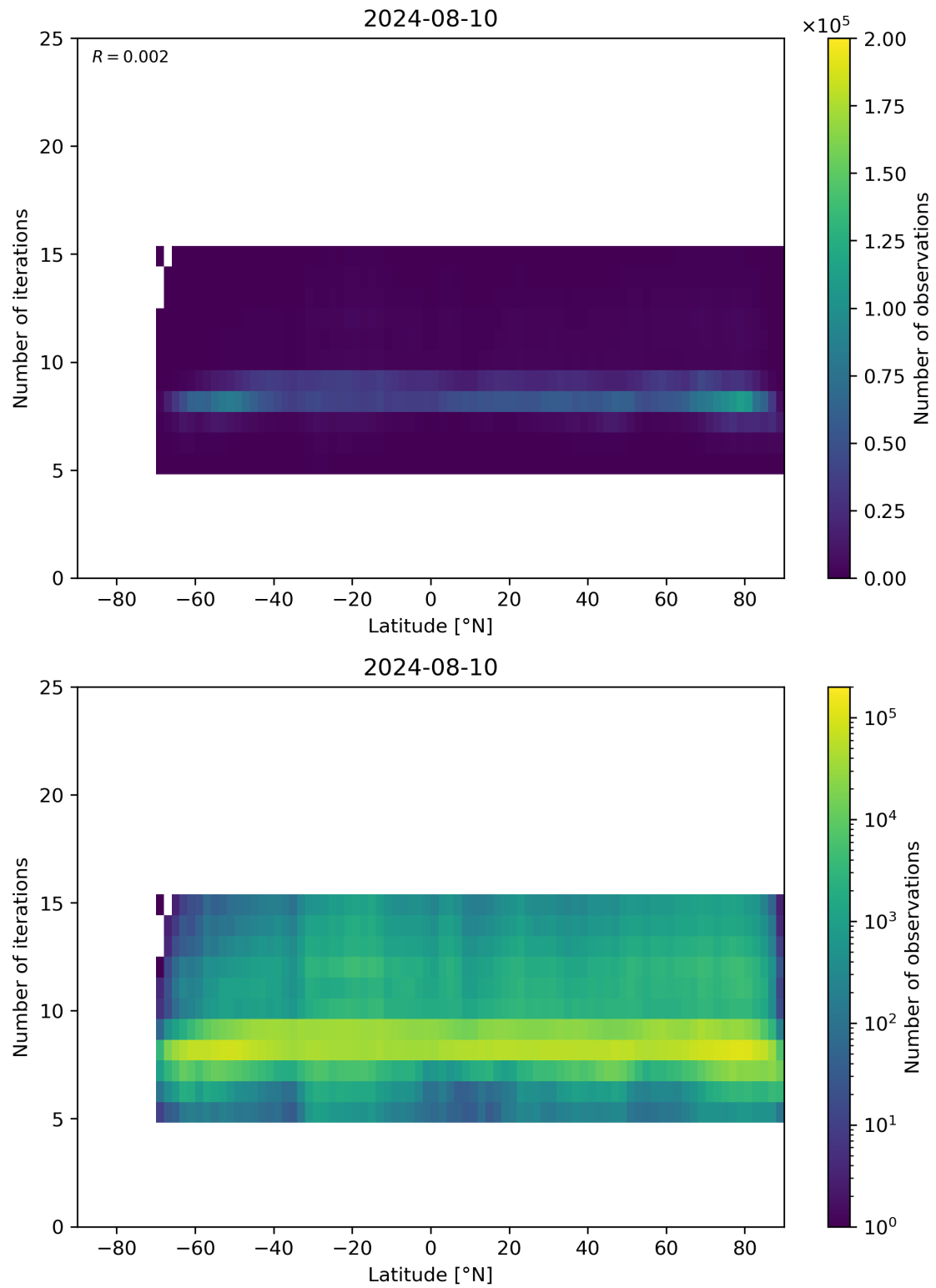
Figure 56: Scatter density plot of “Latitude” against “Number of iterations” for 2024-08-09 to 2024-08-11.
