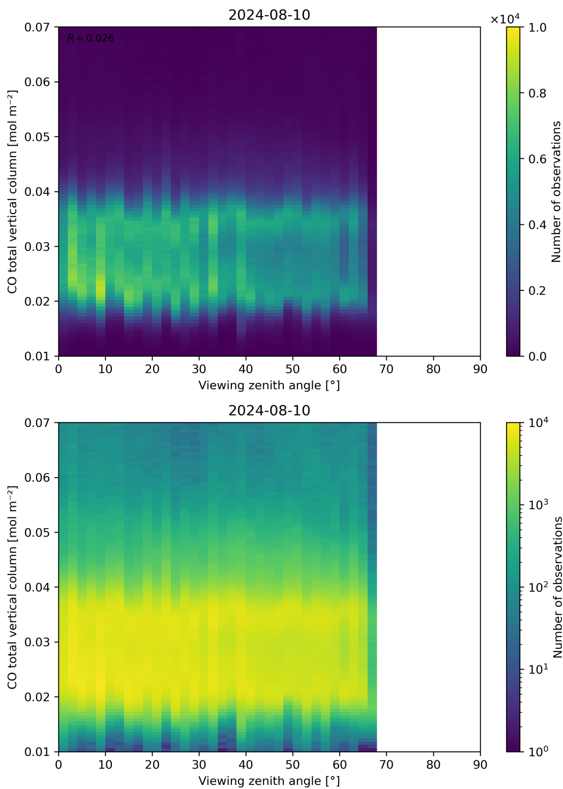
Figure 69: Scatter density plot of “Viewing zenith angle” against “CO total vertical column” for 2024-08-09 to 2024-08-11.
