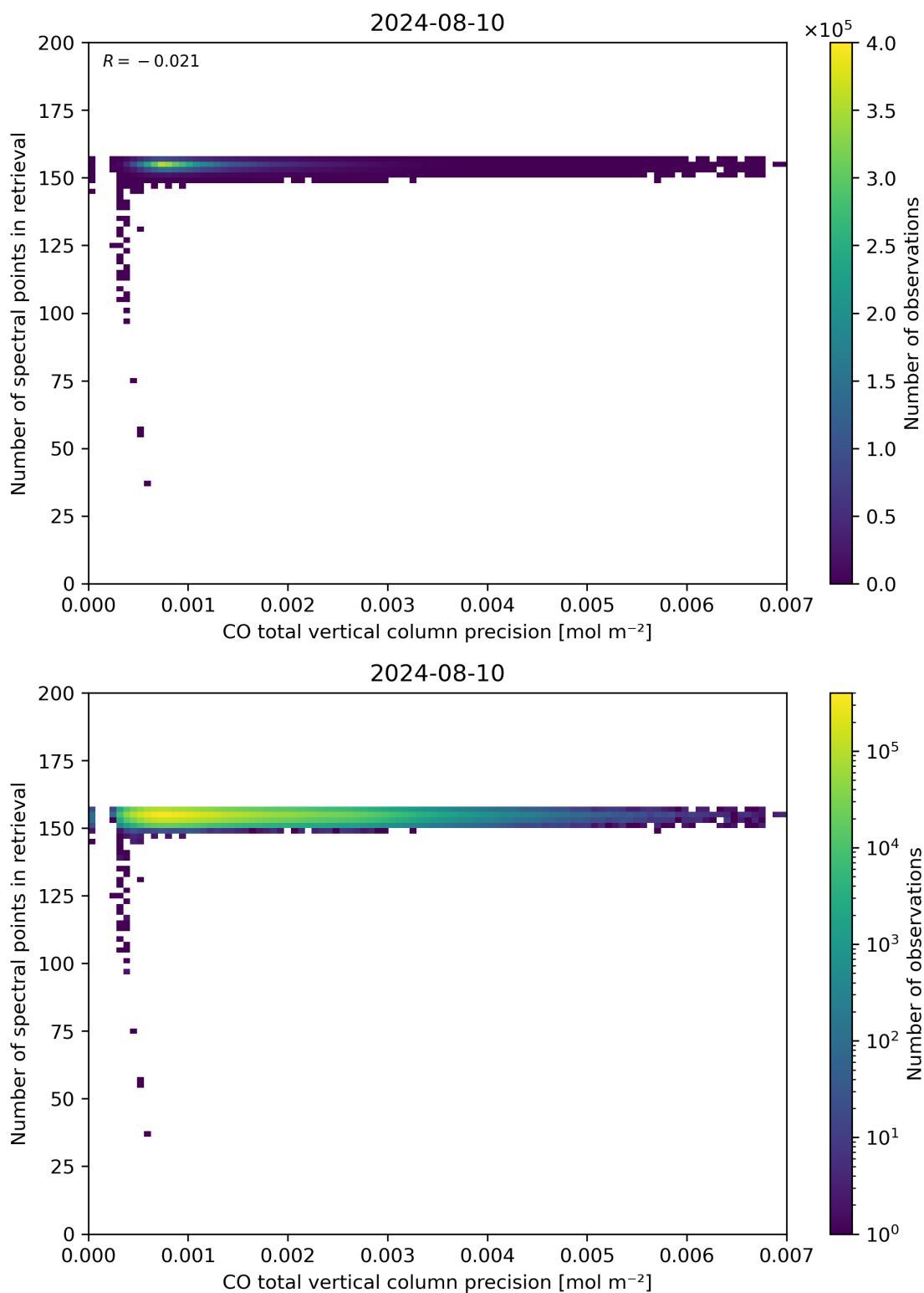
Figure 47: Scatter density plot of “CO total vertical column precision” against “Number of spectral points in retrieval” for 2024-08-09 to 2024-08-11.
