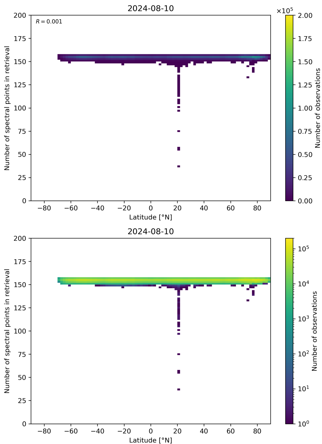
Figure 57: Scatter density plot of “Latitude” against “Number of spectral points in retrieval” for 2024-08-09 to 2024-08-11.
