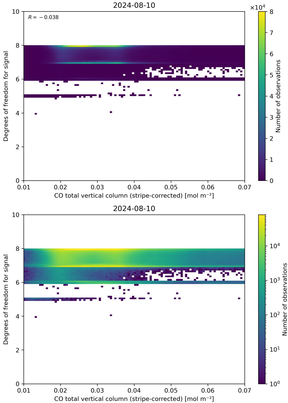
Figure 38: Scatter density plot of “CO total vertical column (stripe-corrected)” against “Degrees of freedom for signal” for 2024-08-09 to 2024-08-11.
