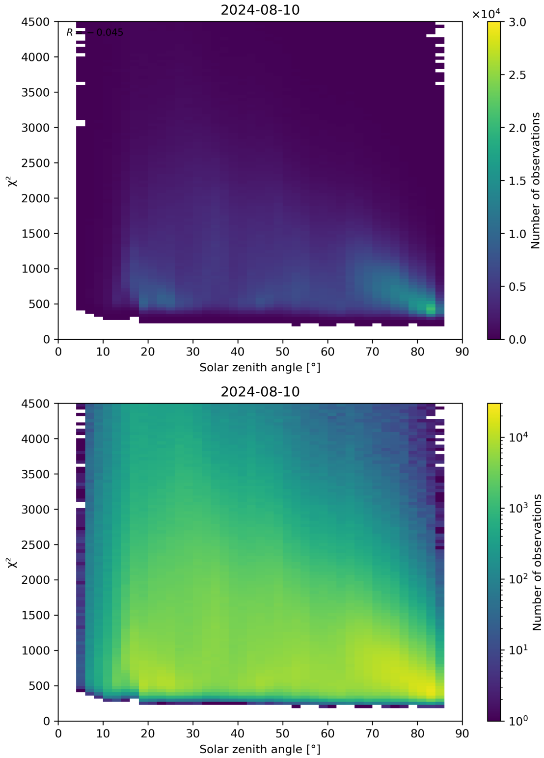
Figure 64: Scatter density plot of “Solar zenith angle” against “ \chi^2 ” for 2024-08-09 to 2024-08-11.
