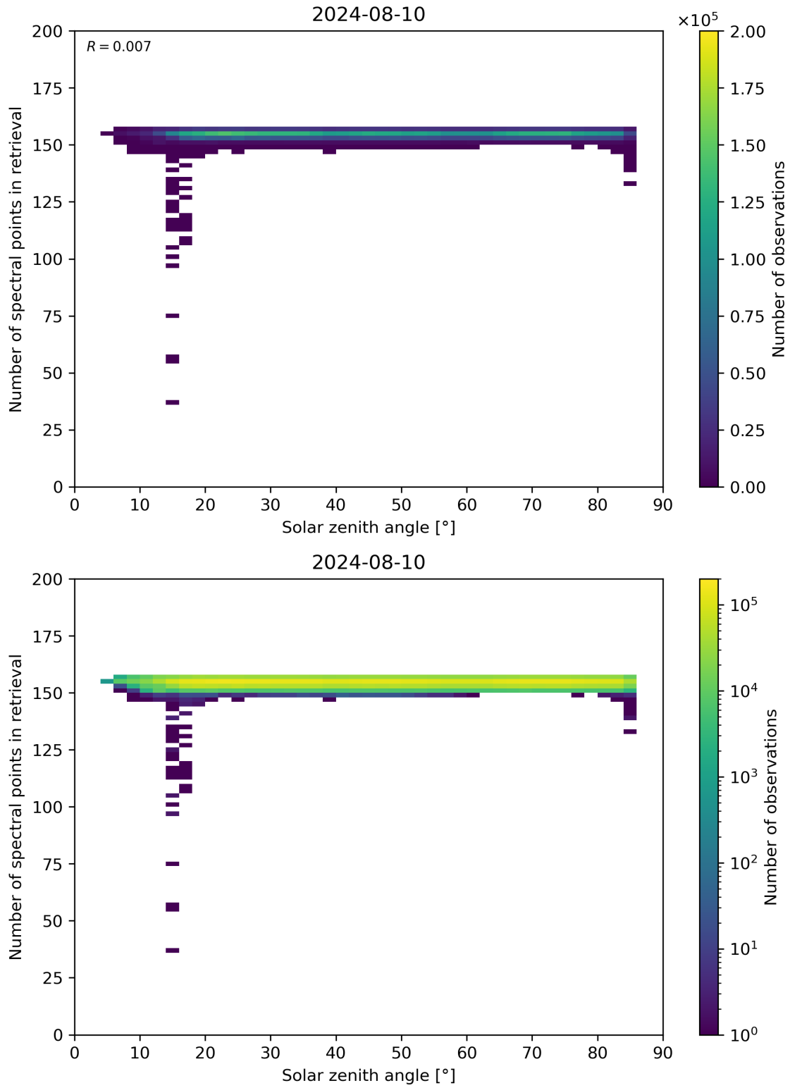
Figure 68: Scatter density plot of “Solar zenith angle” against “Number of spectral points in retrieval” for 2024-08-09 to 2024-08-11.
