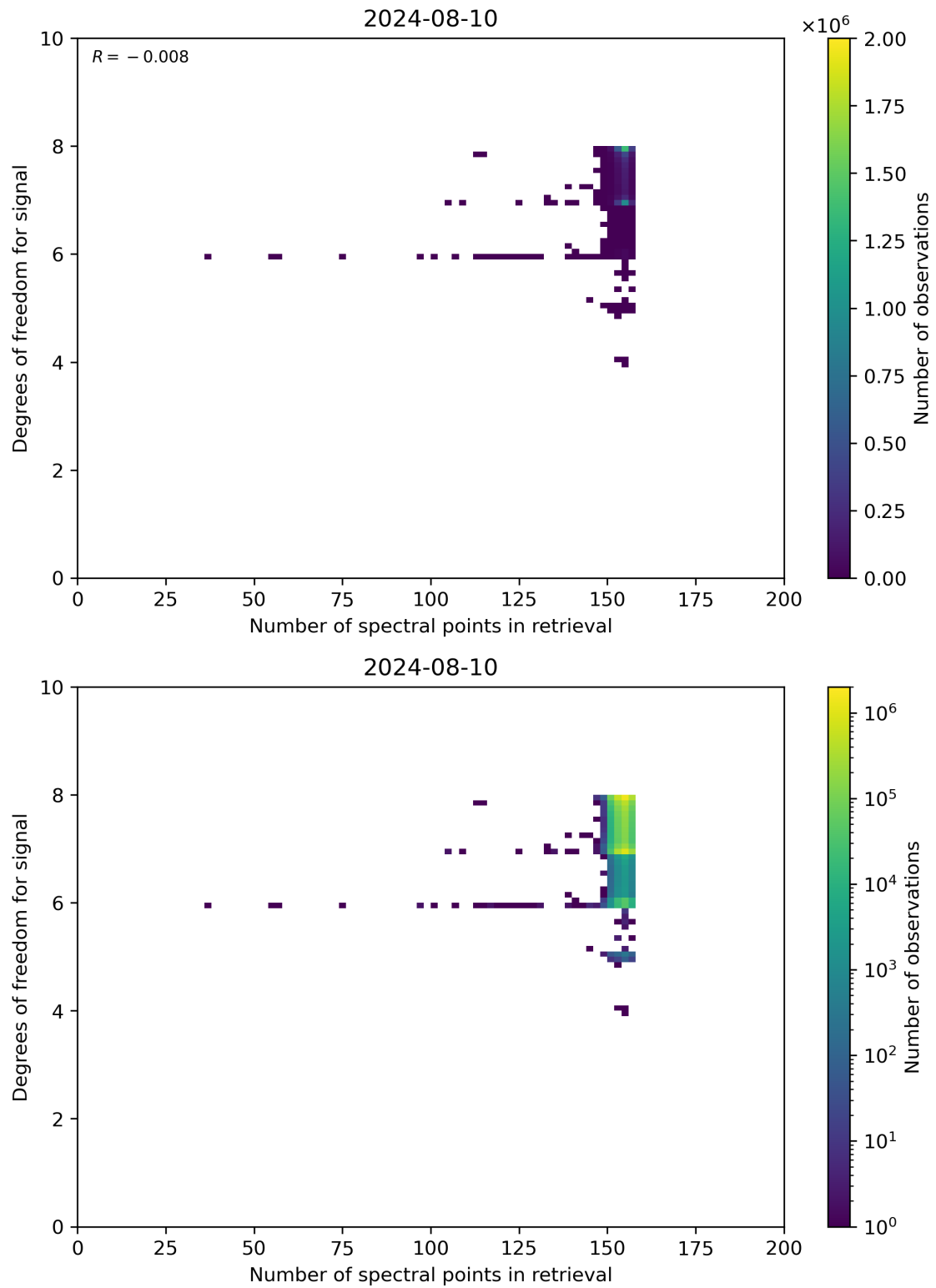
Figure 59: Scatter density plot of “Number of spectral points in retrieval” against “Degrees of freedom for signal” for 2024-08-09 to 2024-08-11.
