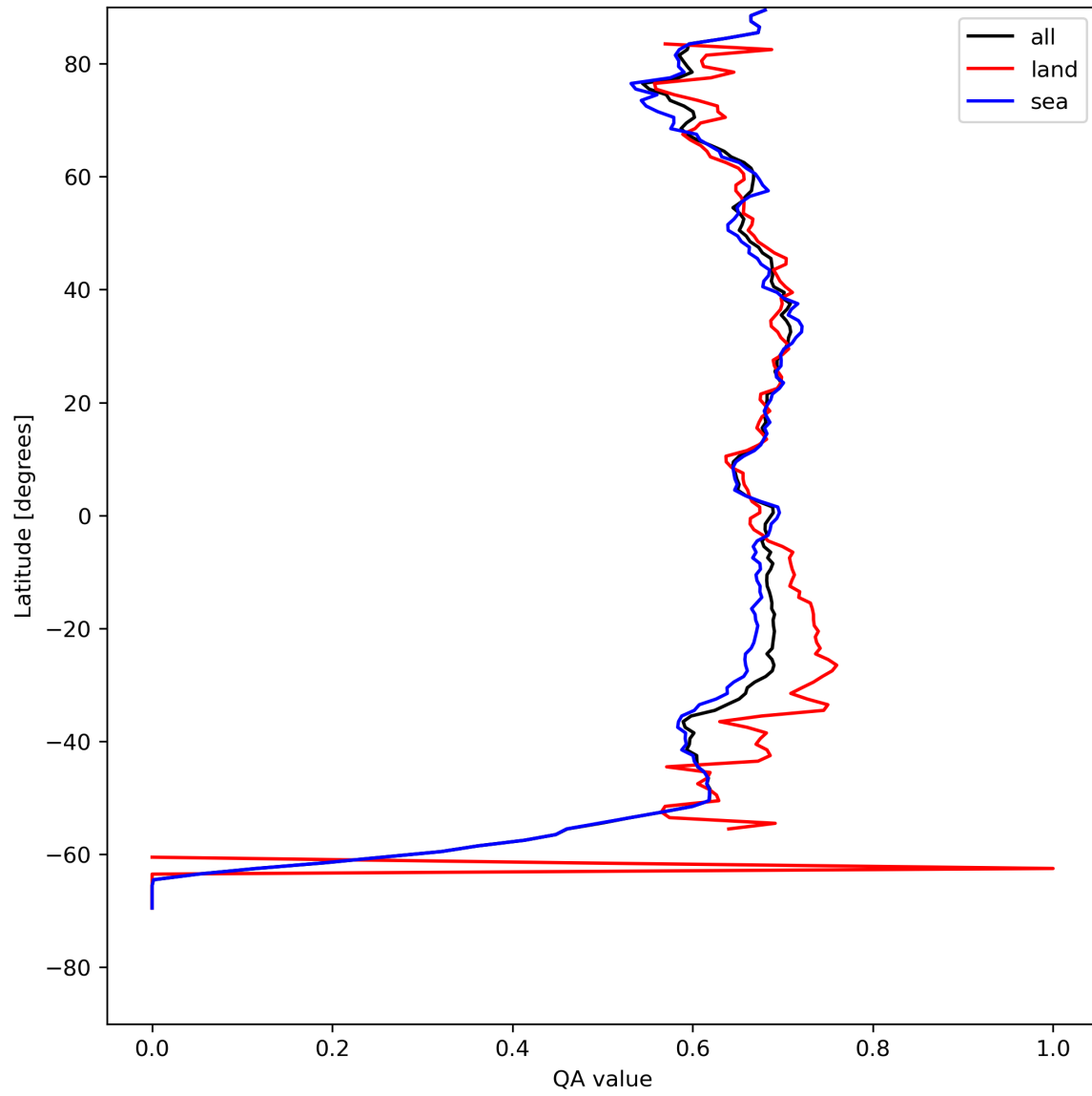
Figure 9: Zonal average of “QA value” for 2024-08-09 to 2024-08-11.
