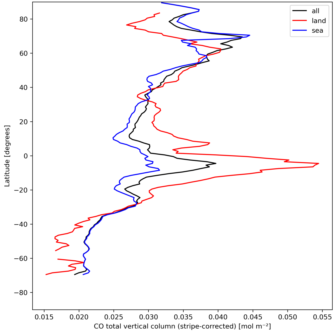
Figure 11: Zonal average of “CO total vertical column (stripe-corrected)” for 2024-08-09 to 2024-08-11.
