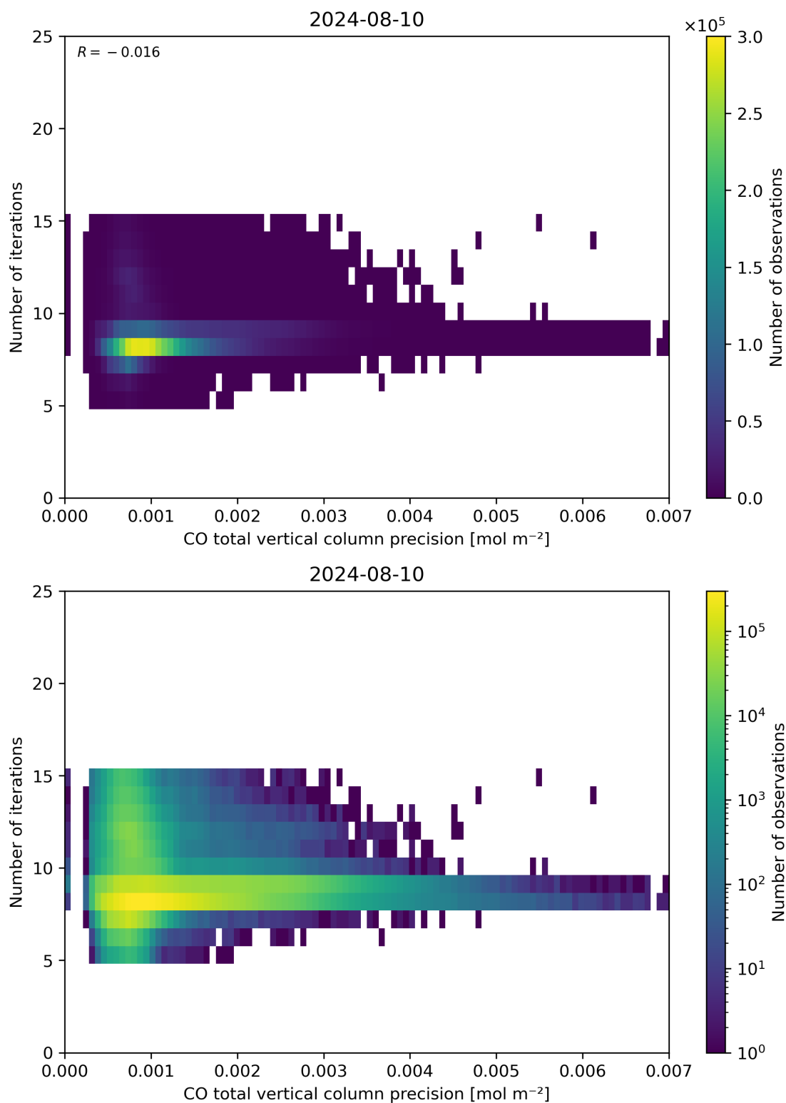
Figure 46: Scatter density plot of “CO total vertical column precision” against “Number of iterations” for 2024-08-09 to 2024-08-11.
