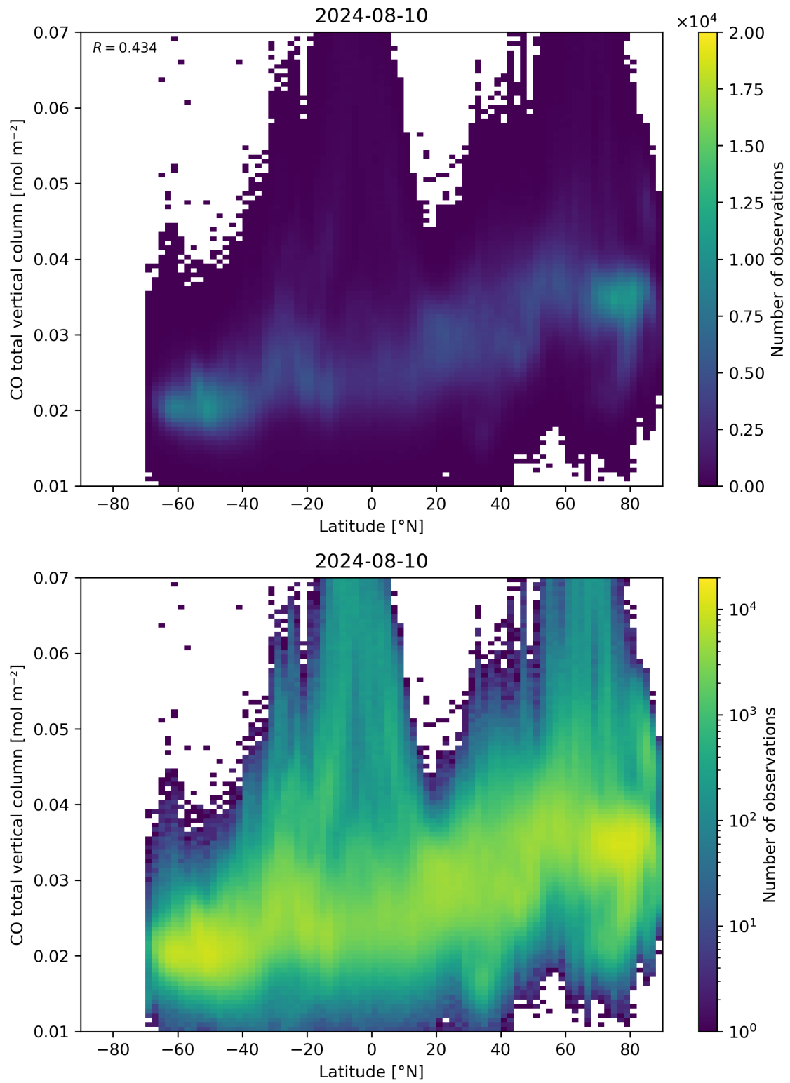
Figure 51: Scatter density plot of “Latitude” against “CO total vertical column” for 2024-08-09 to 2024-08-11.
