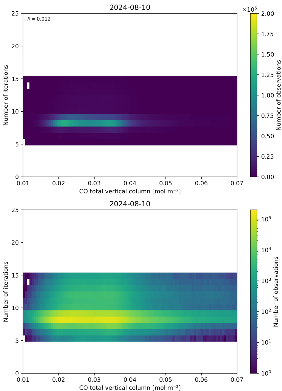
Figure 42: Scatter density plot of “CO total vertical column” against “Number of iterations” for 2024-08-09 to 2024-08-11.
