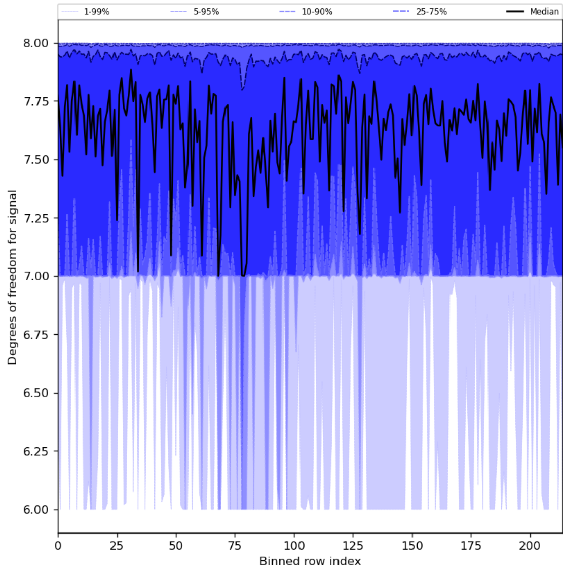
Figure 31: Along track statistics of “Degrees of freedom for signal” for 2024-08-09 to 2024-08-11
