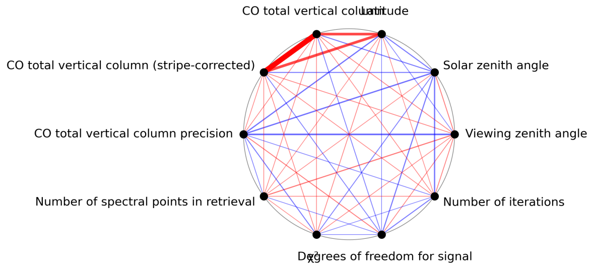
Figure 1: Map of correlation graph for 2024-08-09 to 2024-08-11.
