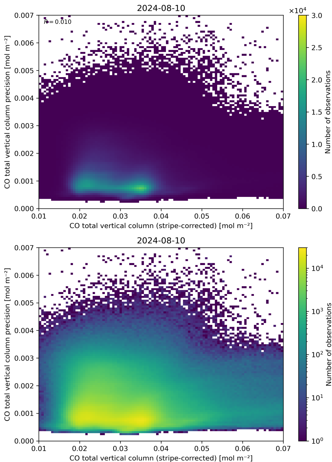
Figure 36: Scatter density plot of “CO total vertical column (stripe-corrected)” against “CO total vertical column precision” for 2024-08-09 to 2024-08-11.
