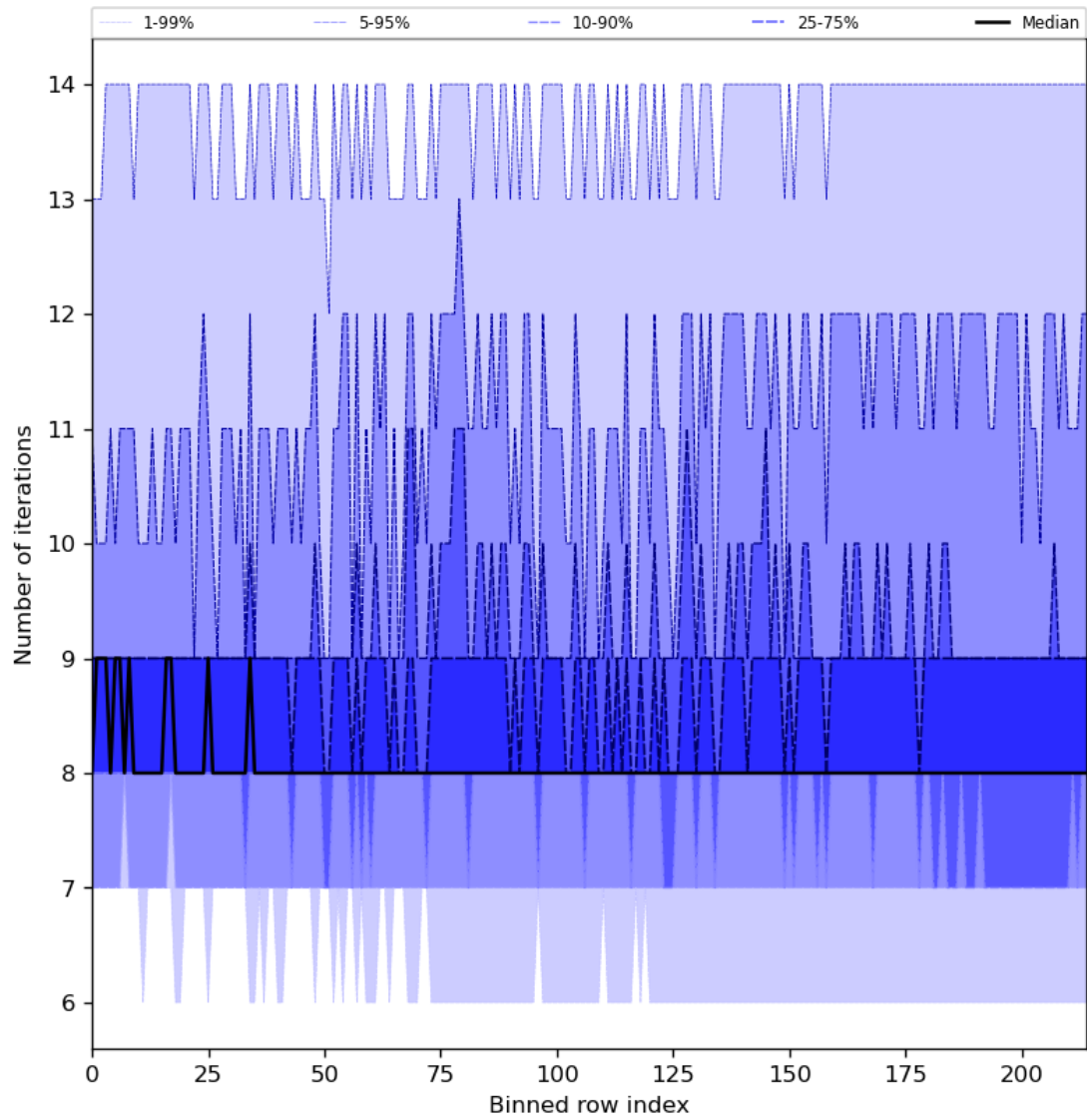
Figure 32: Along track statistics of “Number of iterations” for 2024-08-09 to 2024-08-11
