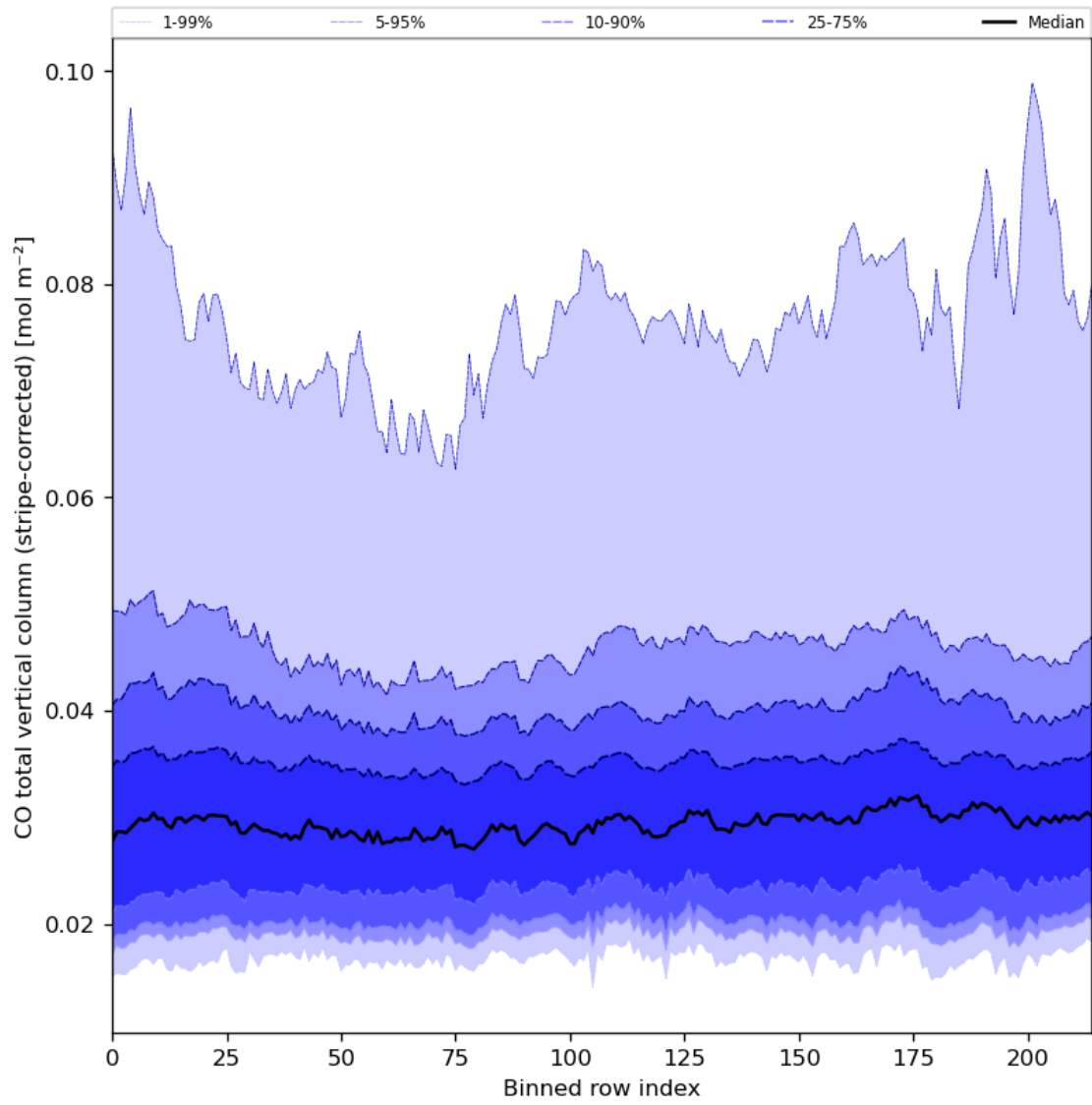
Figure 27: Along track statistics of “CO total vertical column (stripe-corrected)” for 2024-08-09 to 2024-08-11
