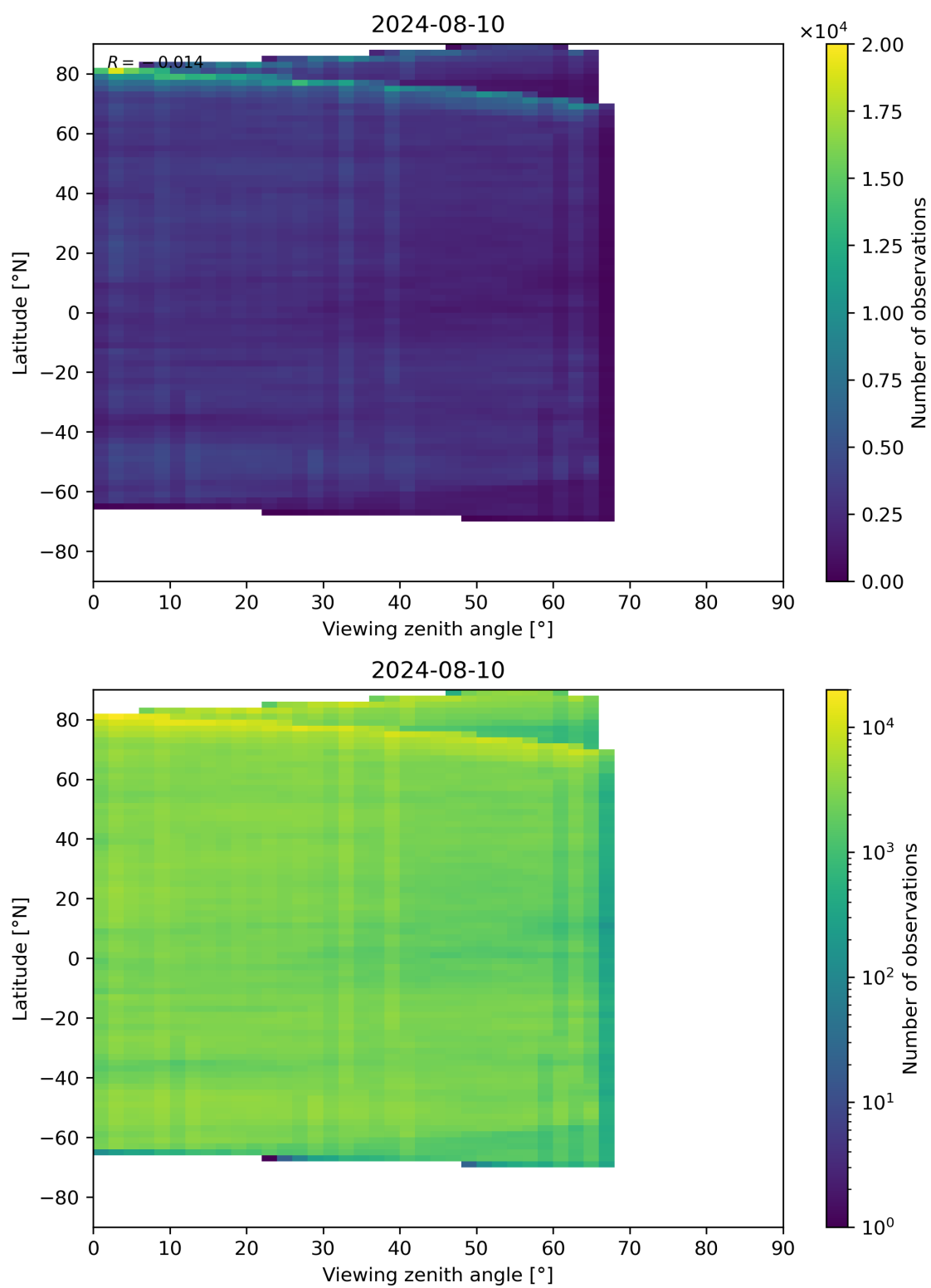
Figure 74: Scatter density plot of “Viewing zenith angle” against “Latitude” for 2024-08-09 to 2024-08-11.
