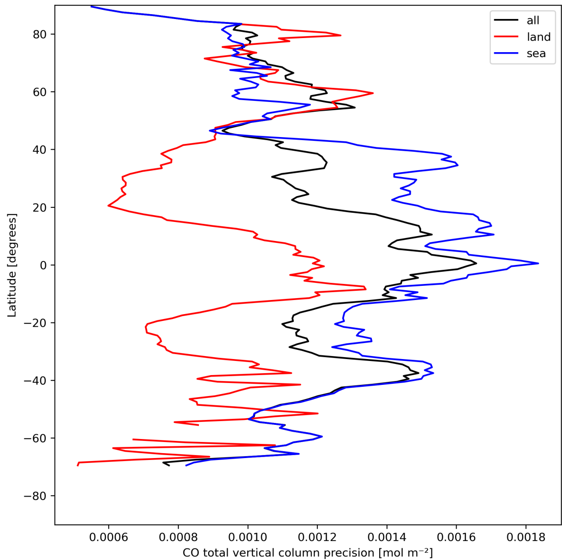
Figure 12: Zonal average of “CO total vertical column precision” for 2024-08-09 to 2024-08-11.
