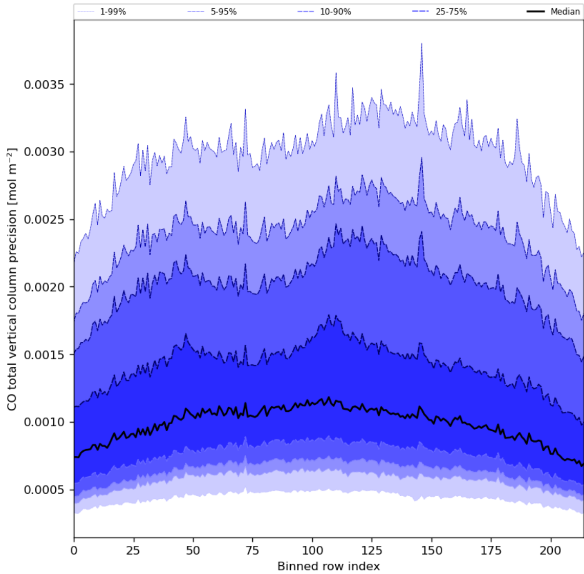
Figure 28: Along track statistics of “CO total vertical column precision” for 2024-08-09 to 2024-08-11
