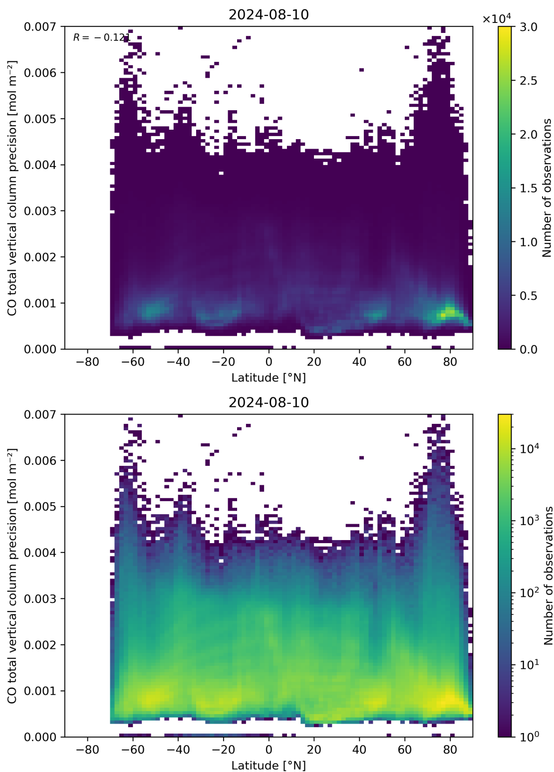
Figure 53: Scatter density plot of “Latitude” against “CO total vertical column precision” for 2024-08-09 to 2024-08-11.
