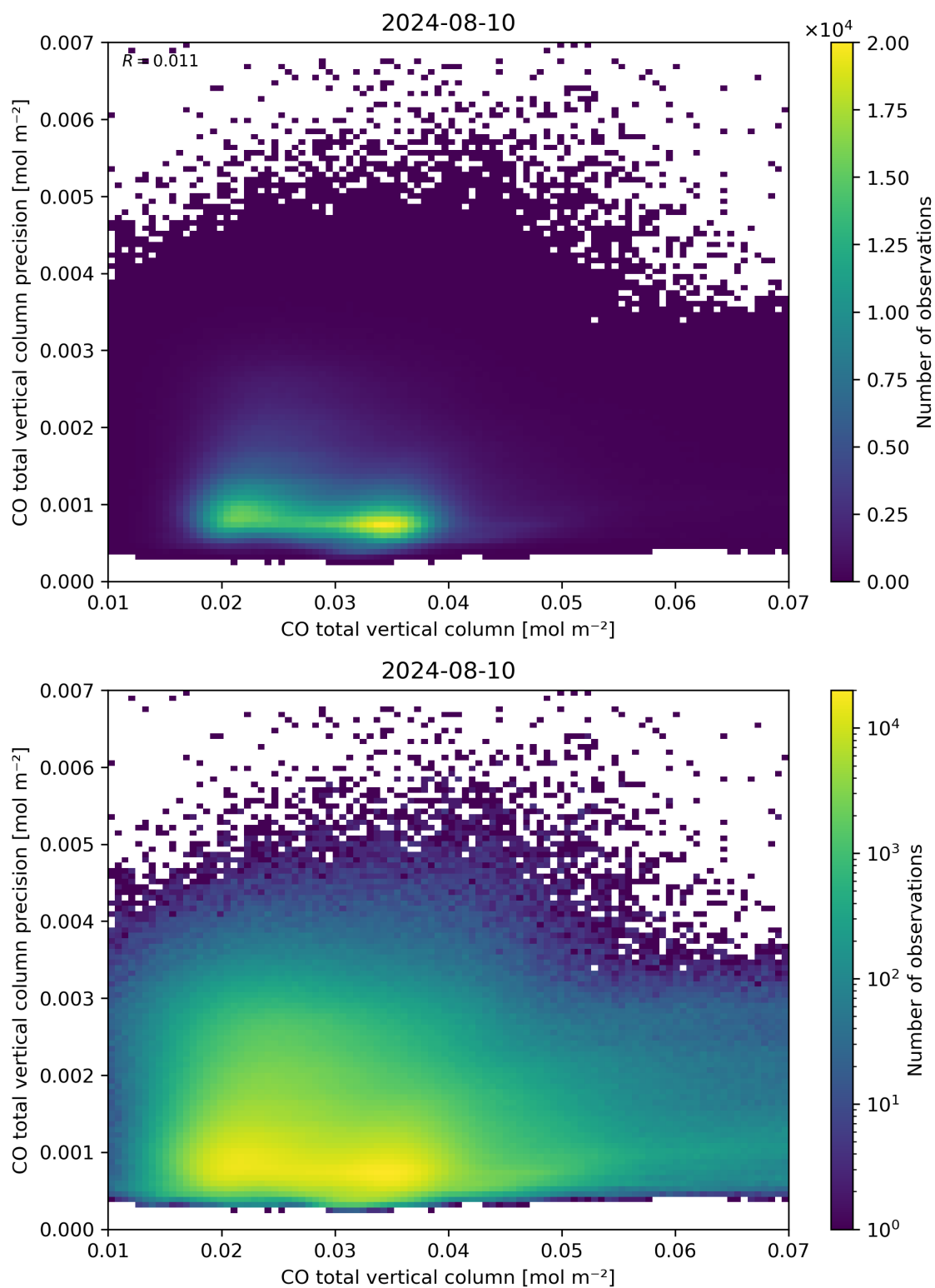
Figure 34: Scatter density plot of “CO total vertical column” against “CO total vertical column precision” for 2024-08-09 to 2024-08-11.
