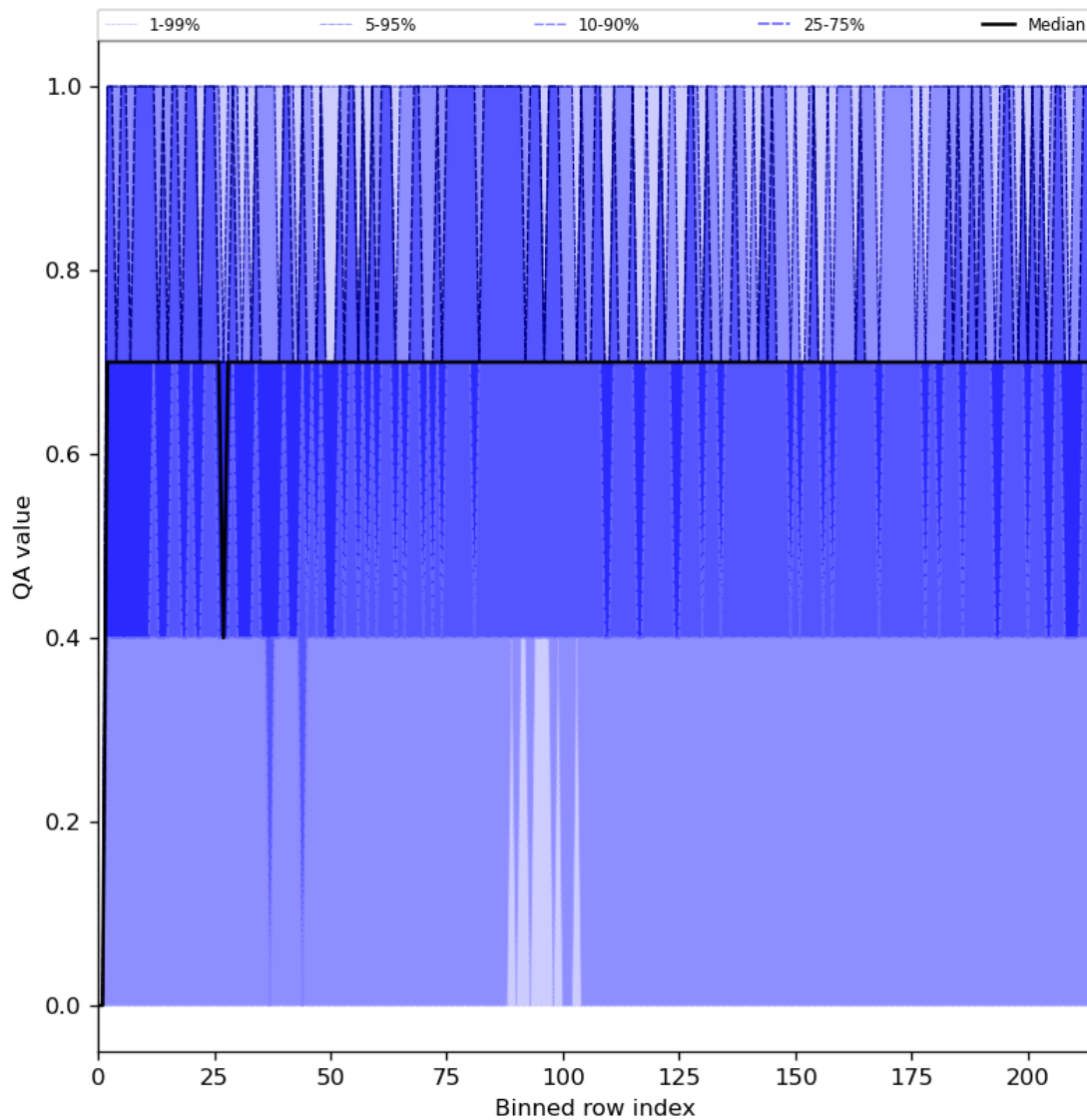
Figure 25: Along track statistics of “QA value” for 2024-08-09 to 2024-08-11
