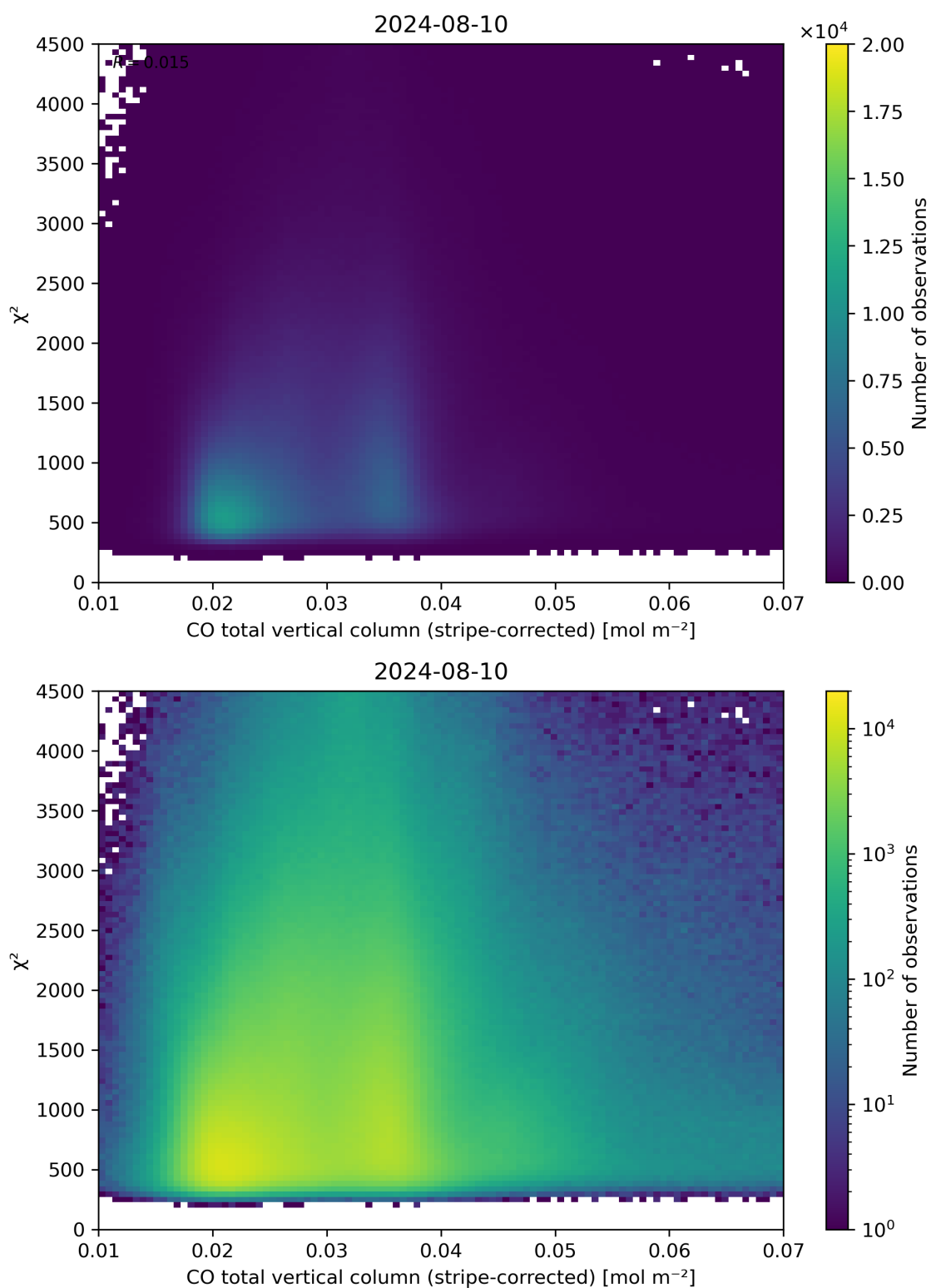
Figure 37: Scatter density plot of “CO total vertical column (stripe-corrected)” against “ \chi^2 ” for 2024-08-09 to 2024-08-11.
