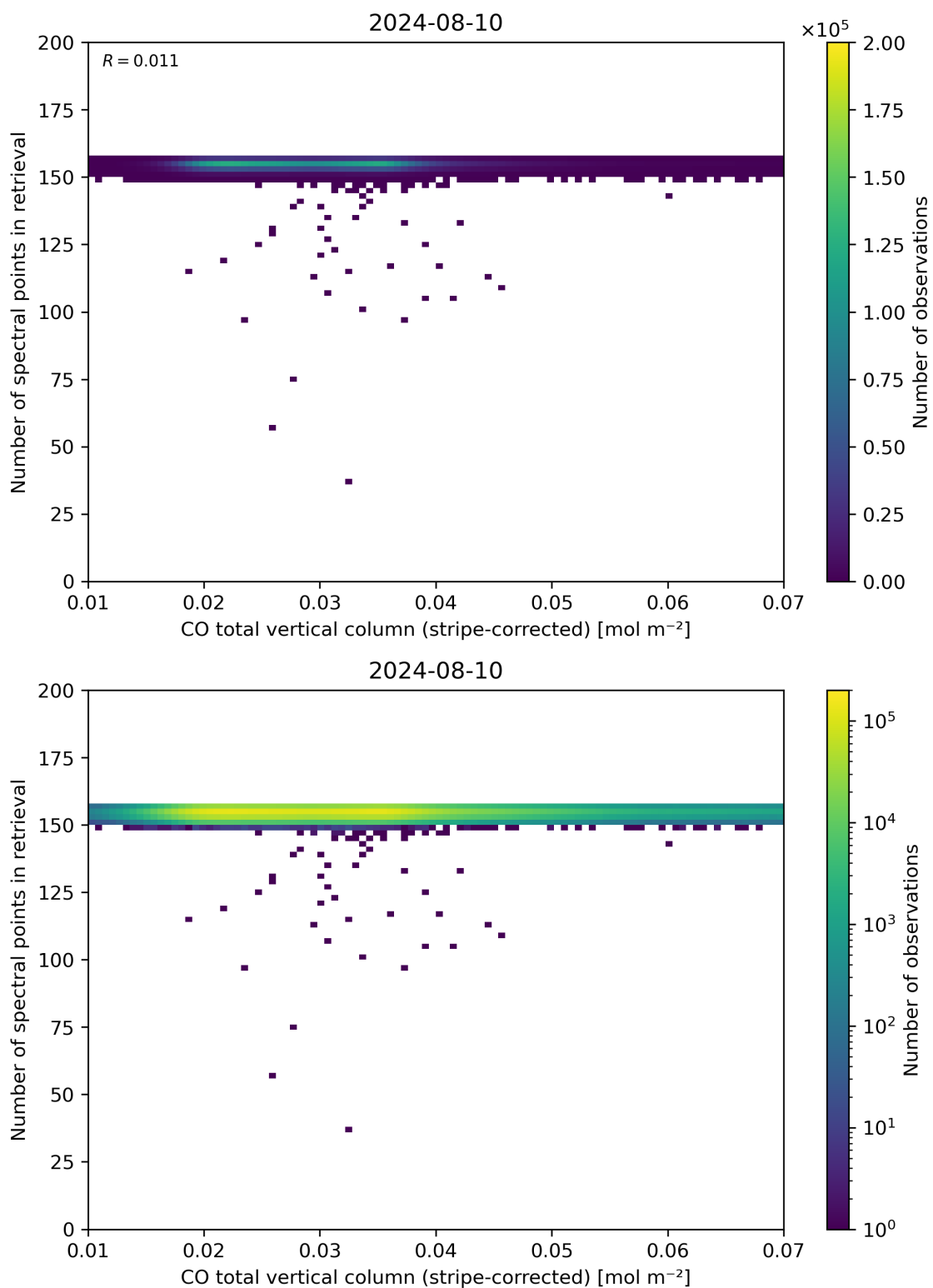
Figure 40: Scatter density plot of “CO total vertical column (stripe-corrected)” against “Number of spectral points in retrieval” for 2024-08-09 to 2024-08-11.
