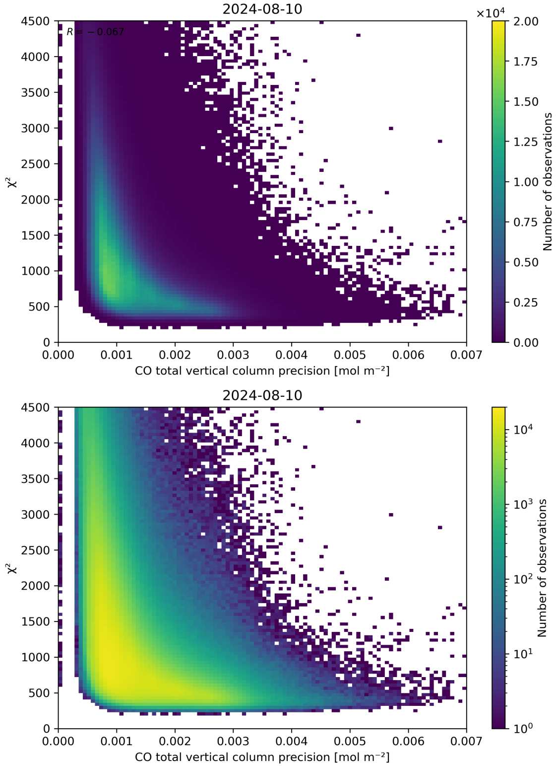
Figure 44: Scatter density plot of “CO total vertical column precision” against “ \chi^2 ” for 2024-08-09 to 2024-08-11.
