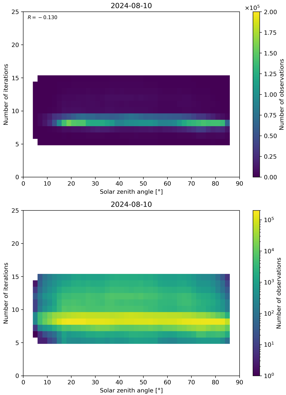
Figure 67: Scatter density plot of “Solar zenith angle” against “Number of iterations” for 2024-08-09 to 2024-08-11.
