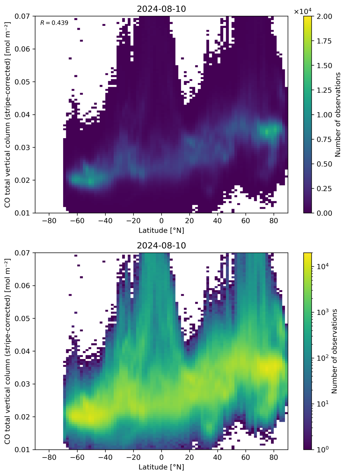
Figure 52: Scatter density plot of “Latitude” against “CO total vertical column (stripe-corrected)” for 2024-08-09 to 2024-08-11.
