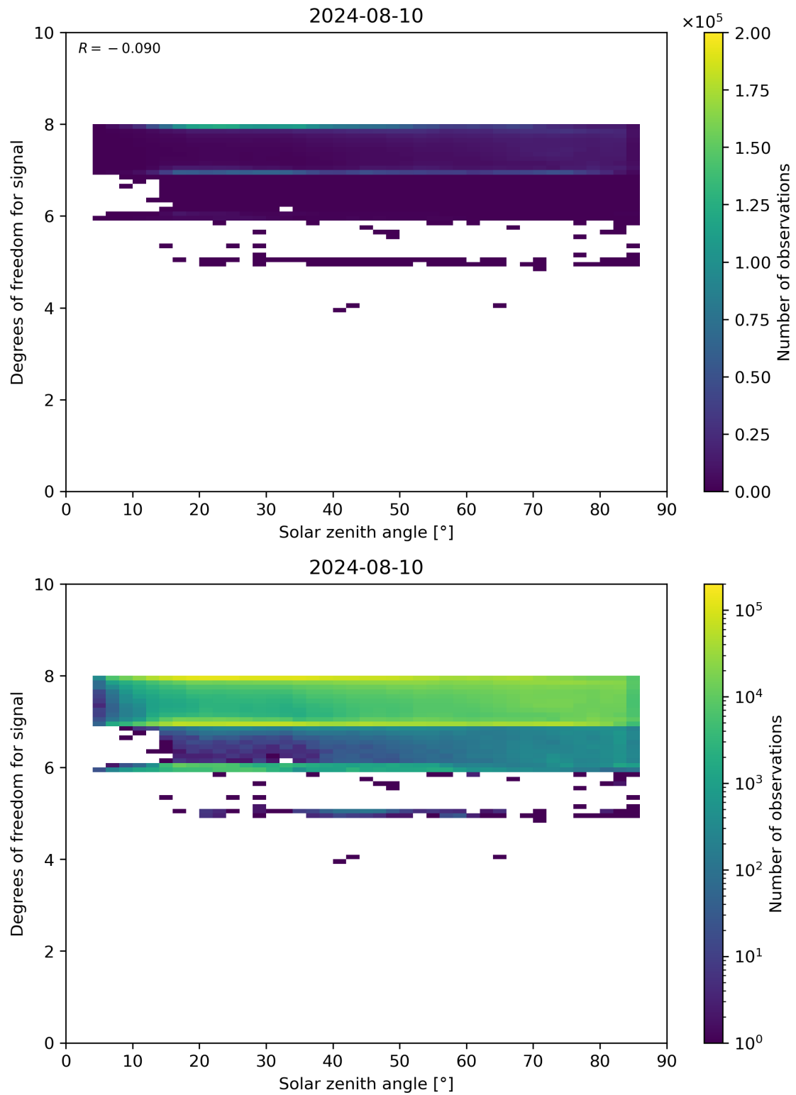
Figure 65: Scatter density plot of “Solar zenith angle” against “Degrees of freedom for signal” for 2024-08-09 to 2024-08-11.
