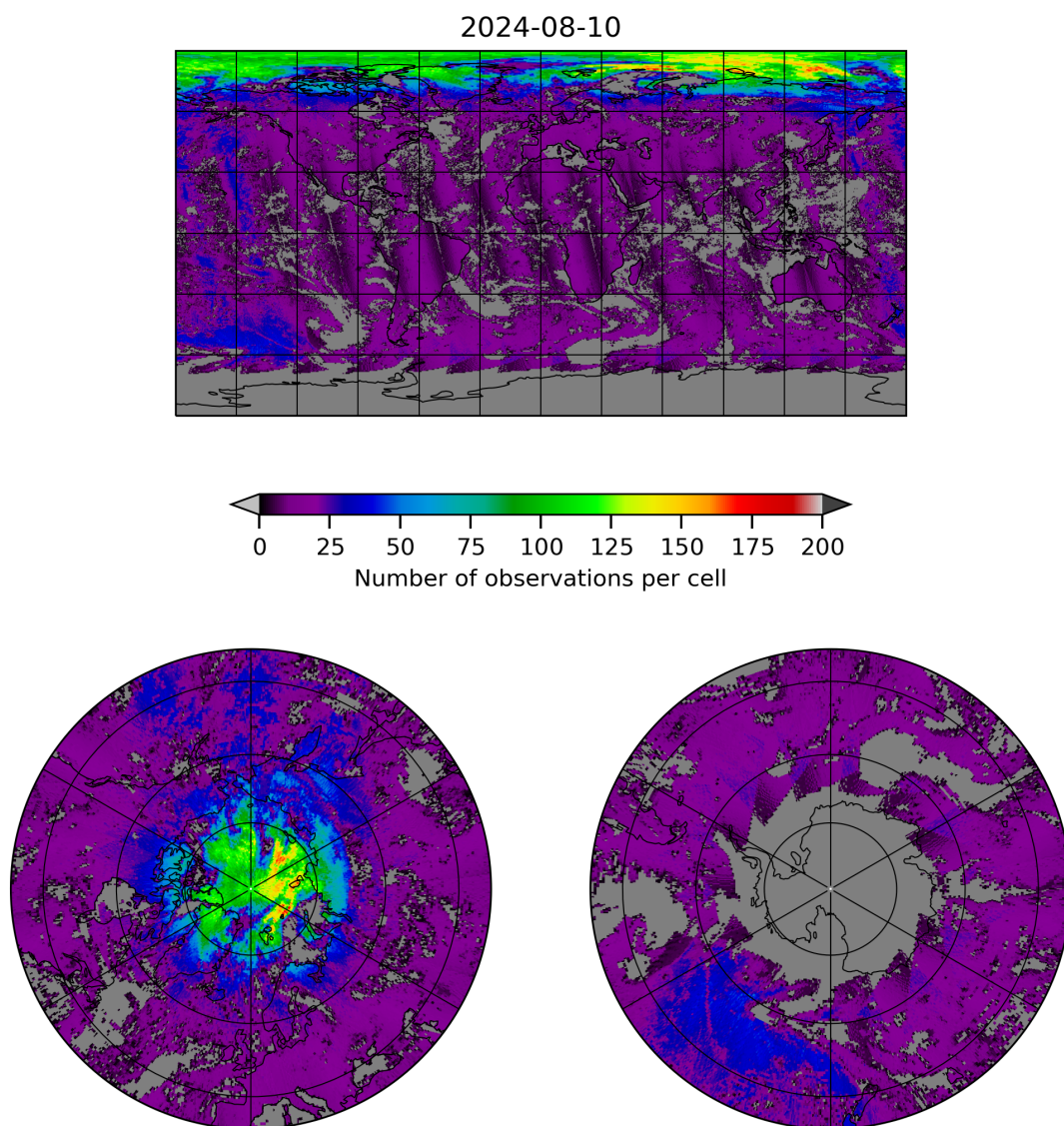
Figure 8: Map of the number of observations for 2024-08-09 to 2024-08-11
