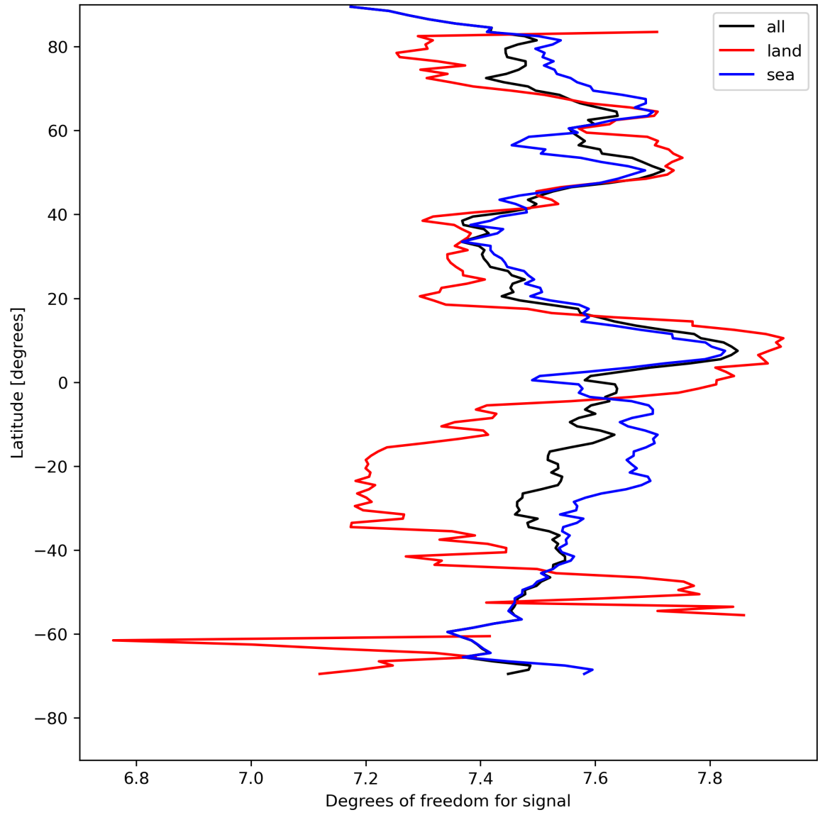
Figure 15: Zonal average of “Degrees of freedom for signal” for 2024-08-09 to 2024-08-11.
