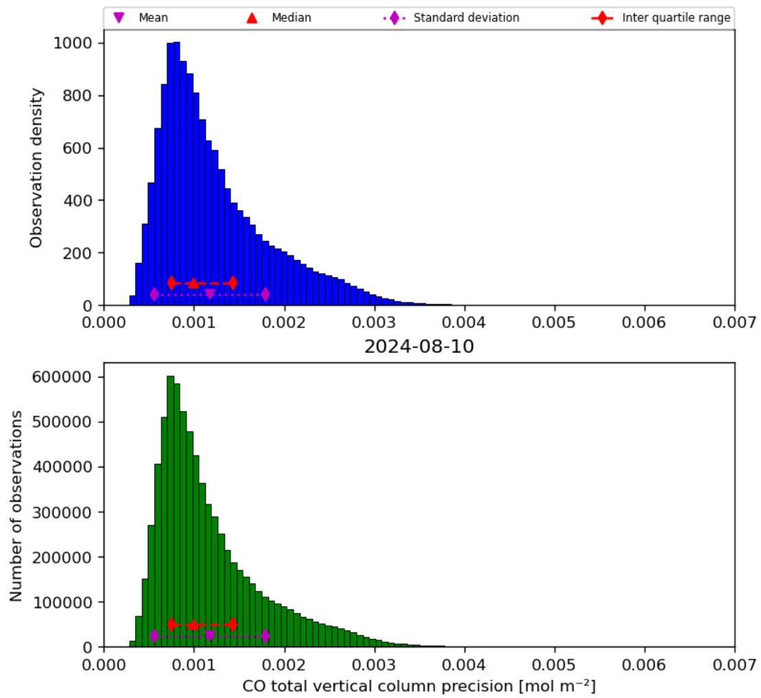
Figure 20: Histogram of “CO total vertical column precision” for 2024-08-09 to 2024-08-11
