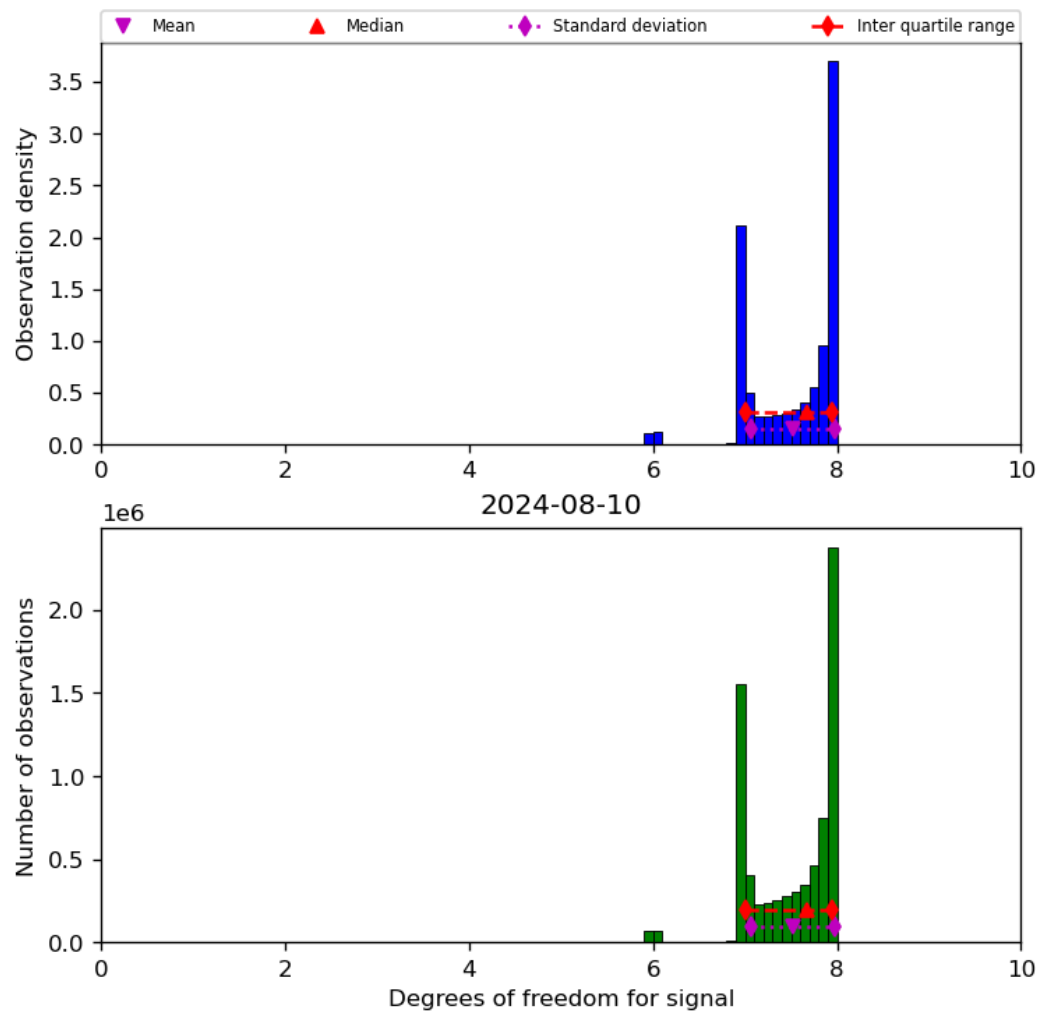
Figure 23: Histogram of “Degrees of freedom for signal” for 2024-08-09 to 2024-08-11
