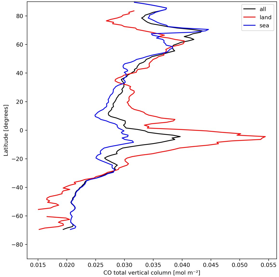
Figure 10: Zonal average of “CO total vertical column” for 2024-08-09 to 2024-08-11.
