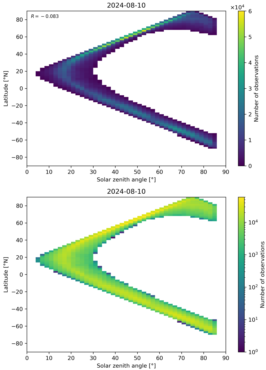
Figure 66: Scatter density plot of “Solar zenith angle” against “Latitude” for 2024-08-09 to 2024-08-11.
