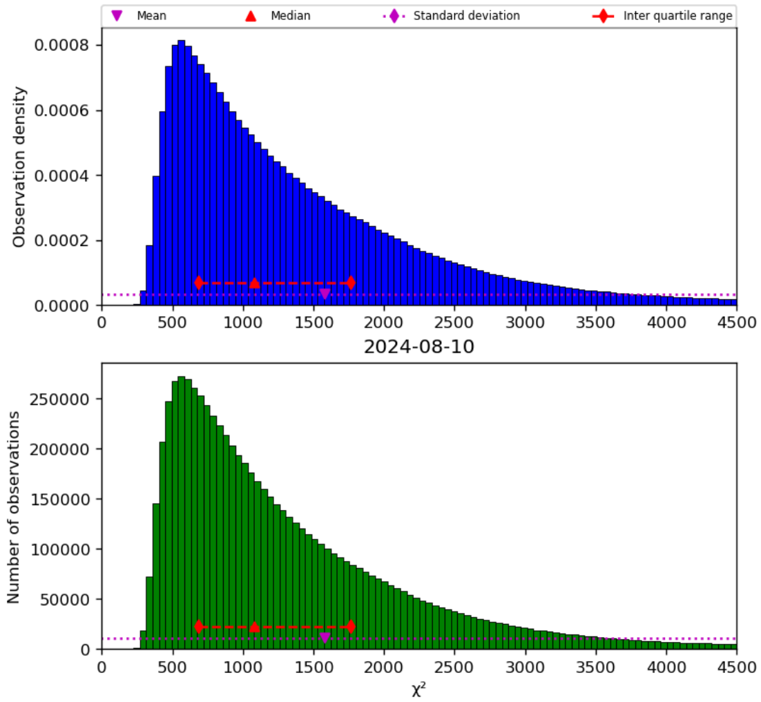
Figure 22: Histogram of “ \chi^2 ” for 2024-08-09 to 2024-08-11
