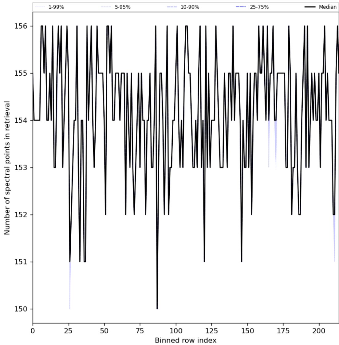
Figure 29: Along track statistics of “Number of spectral points in retrieval” for 2024-08-09 to 2024-08-11
