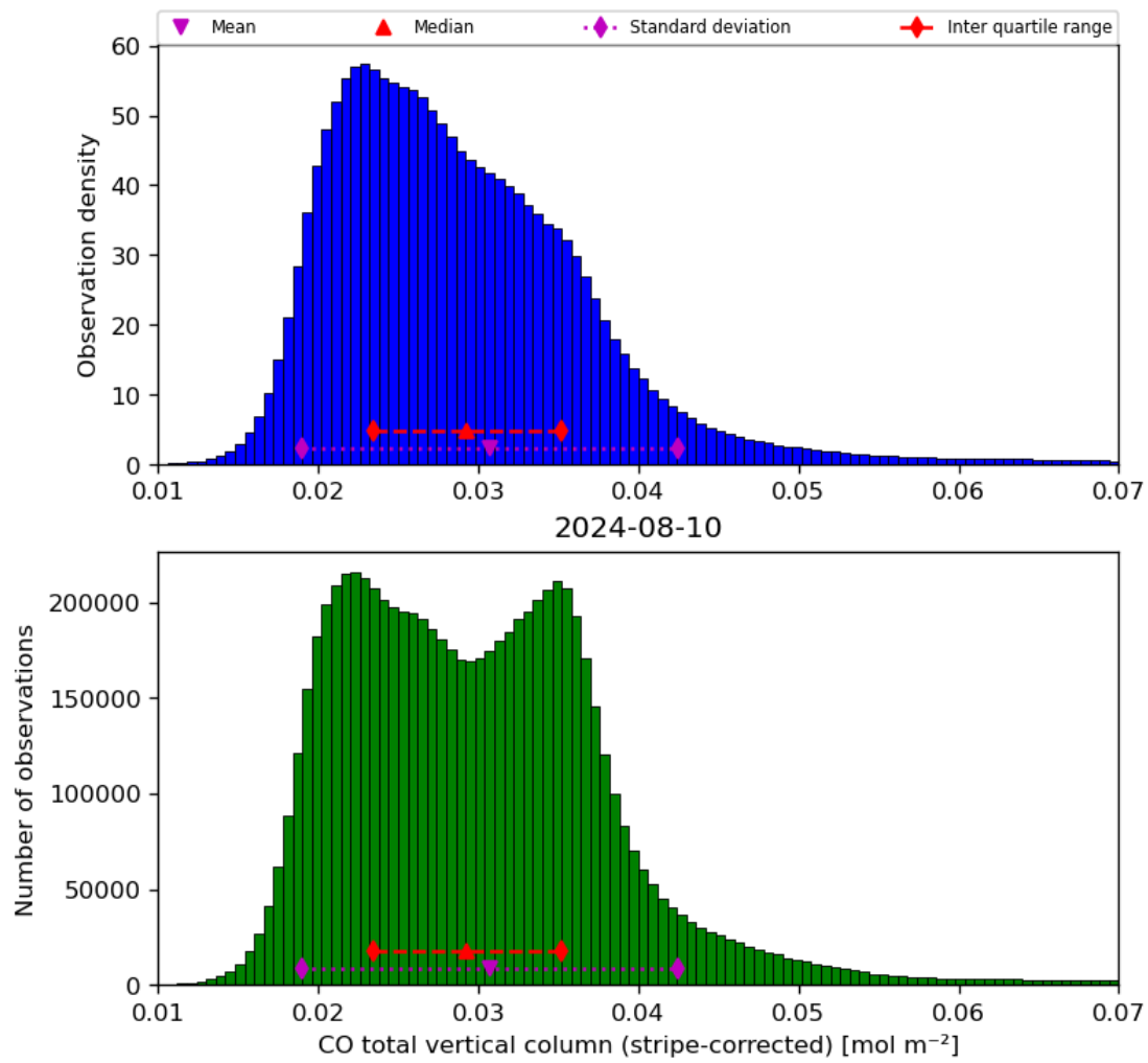
Figure 19: Histogram of “CO total vertical column (stripe-corrected)” for 2024-08-09 to 2024-08-11
