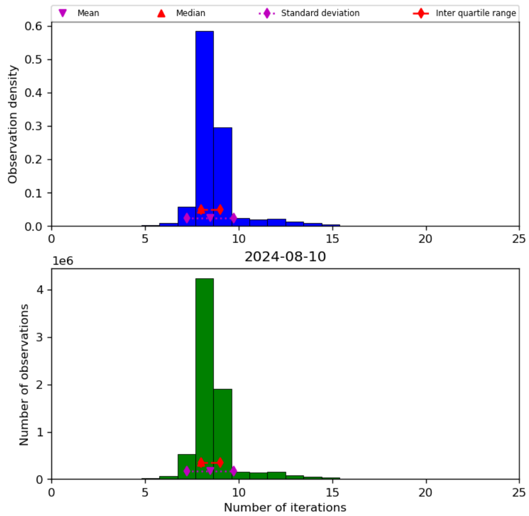
Figure 24: Histogram of “Number of iterations” for 2024-08-09 to 2024-08-11
