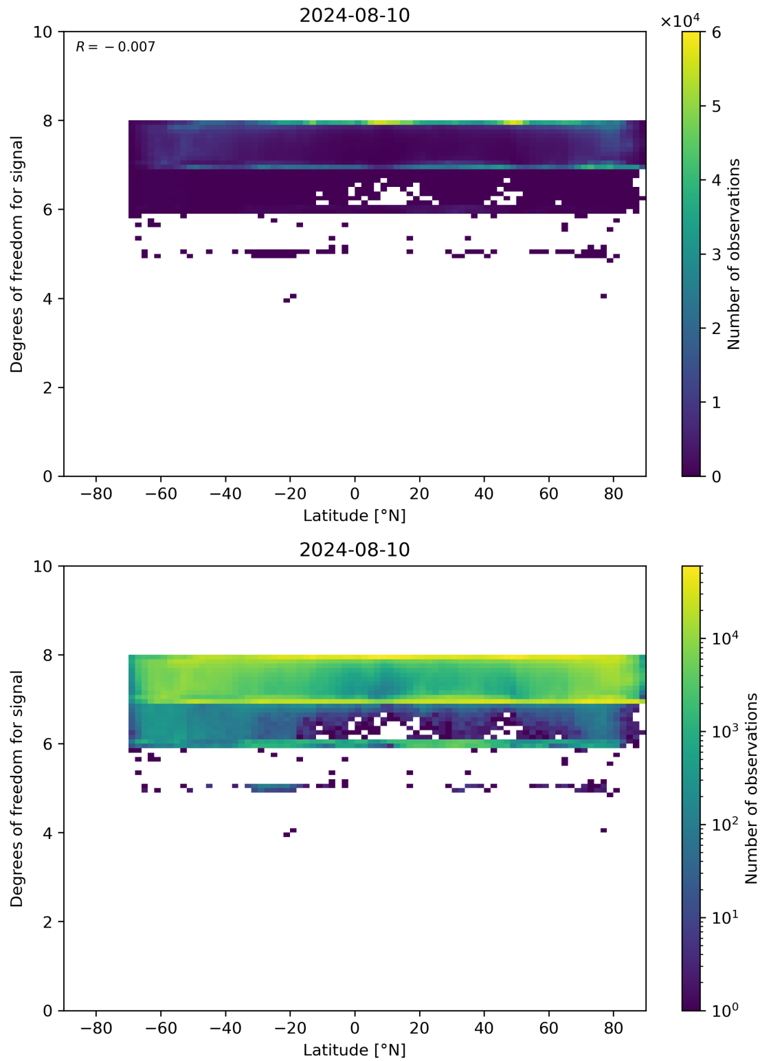
Figure 55: Scatter density plot of “Latitude” against “Degrees of freedom for signal” for 2024-08-09 to 2024-08-11.
