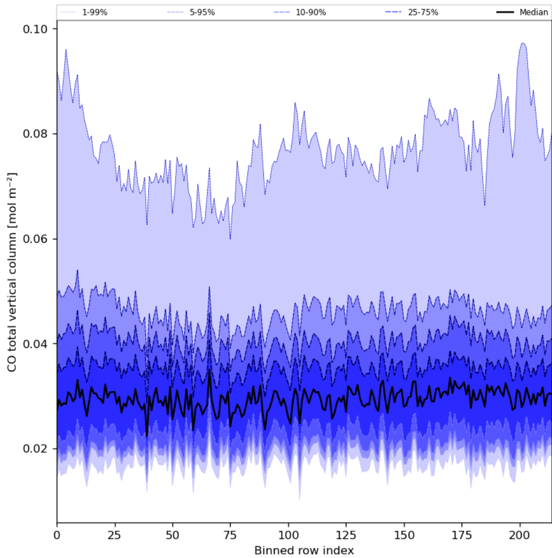
Figure 26: Along track statistics of “CO total vertical column” for 2024-08-09 to 2024-08-11
