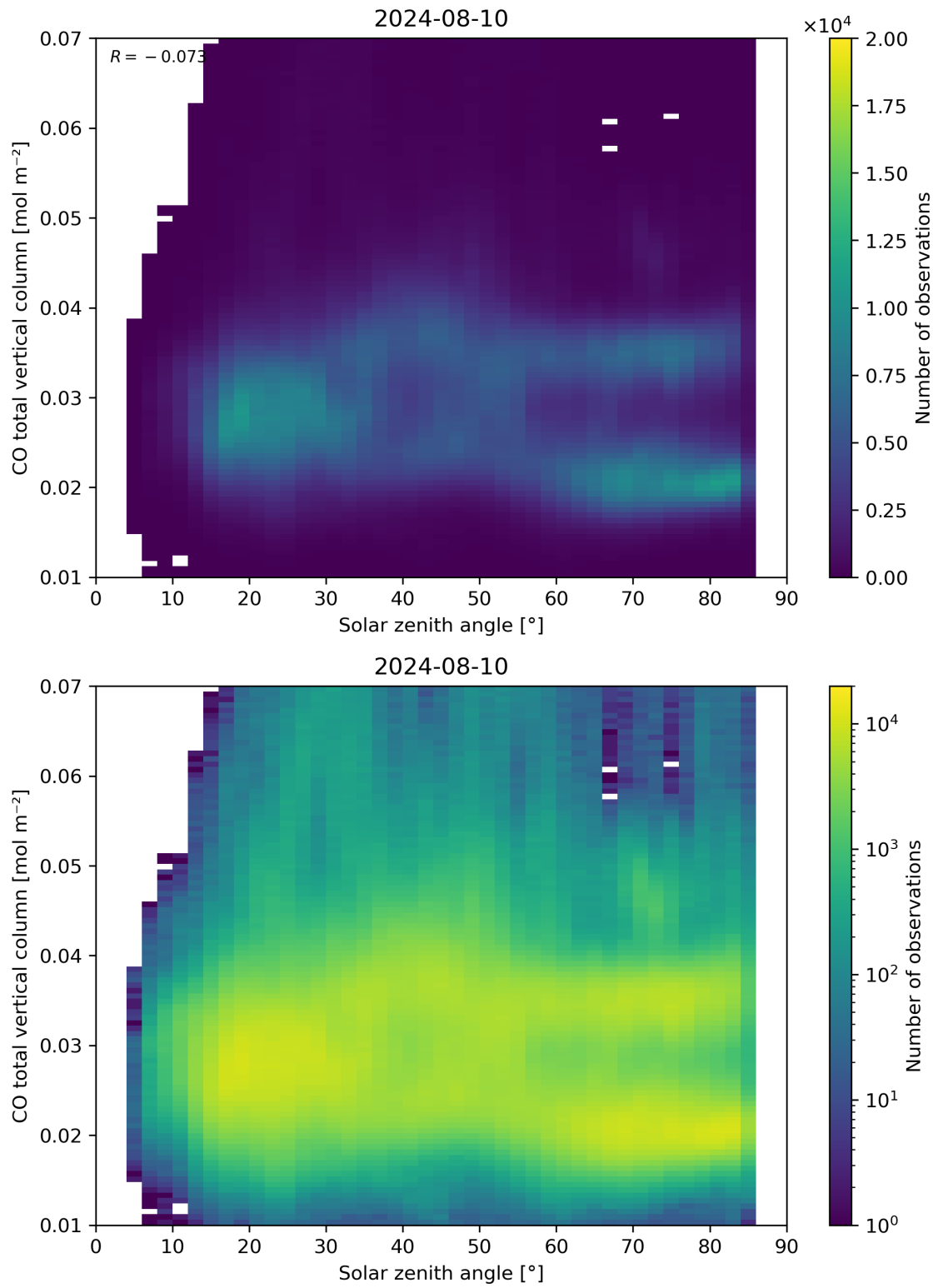
Figure 61: Scatter density plot of “Solar zenith angle” against “CO total vertical column” for 2024-08-09 to 2024-08-11.
