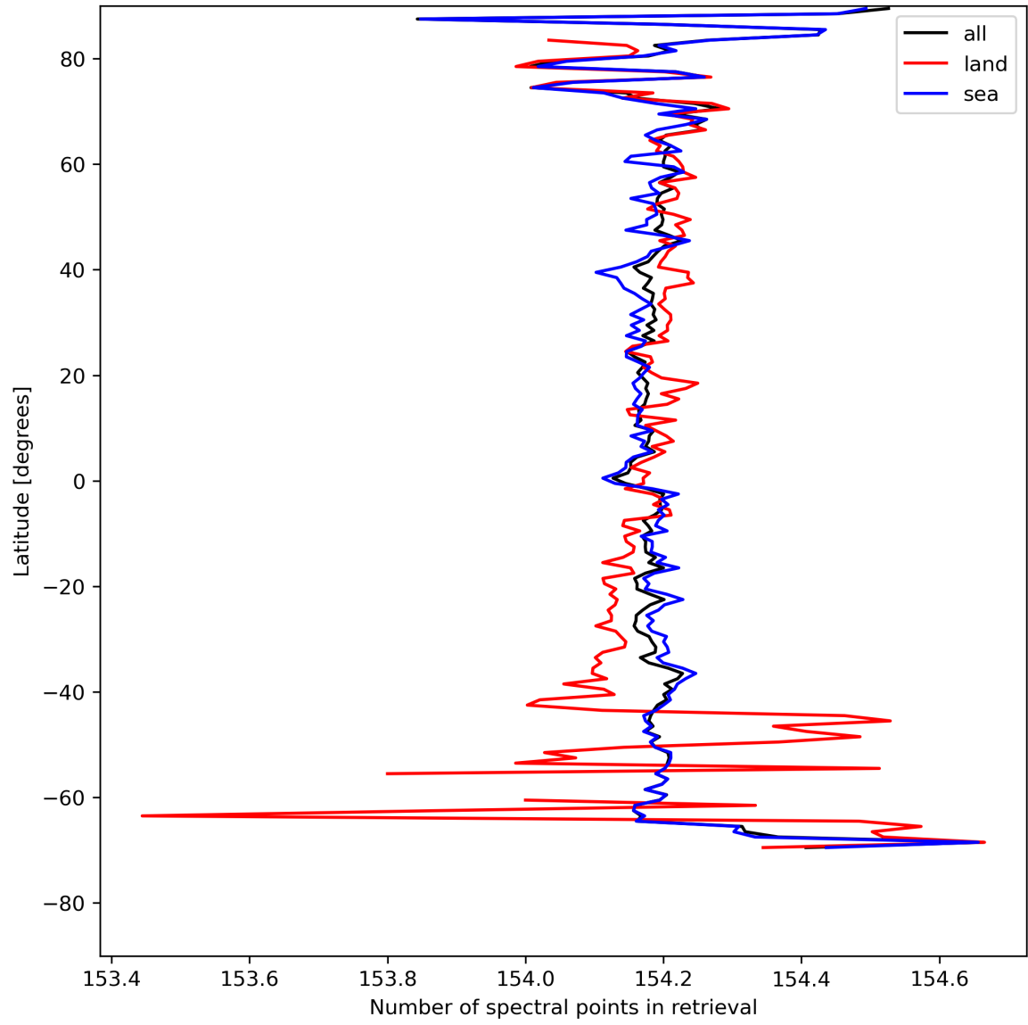
Figure 13: Zonal average of “Number of spectral points in retrieval” for 2024-08-09 to 2024-08-11.
