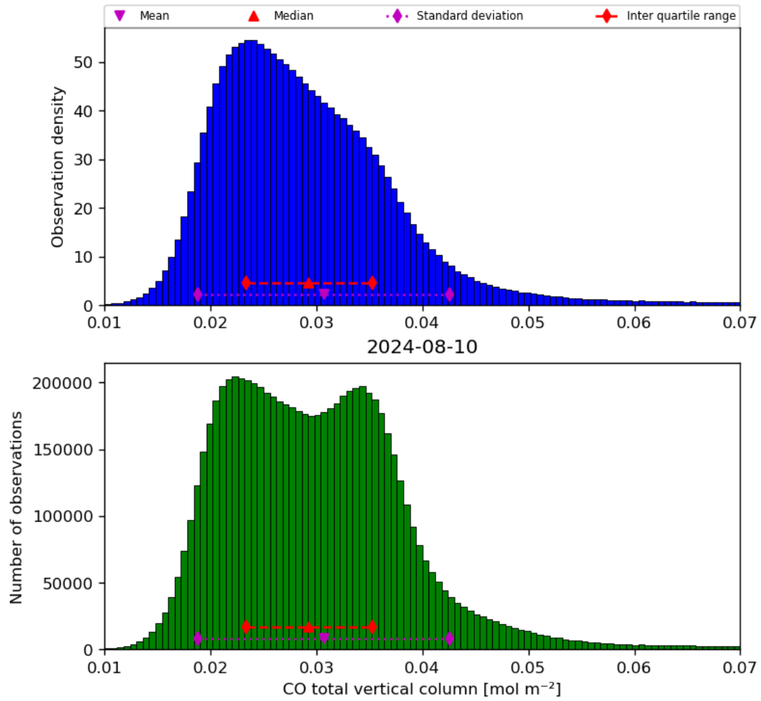
Figure 18: Histogram of “CO total vertical column” for 2024-08-09 to 2024-08-11
