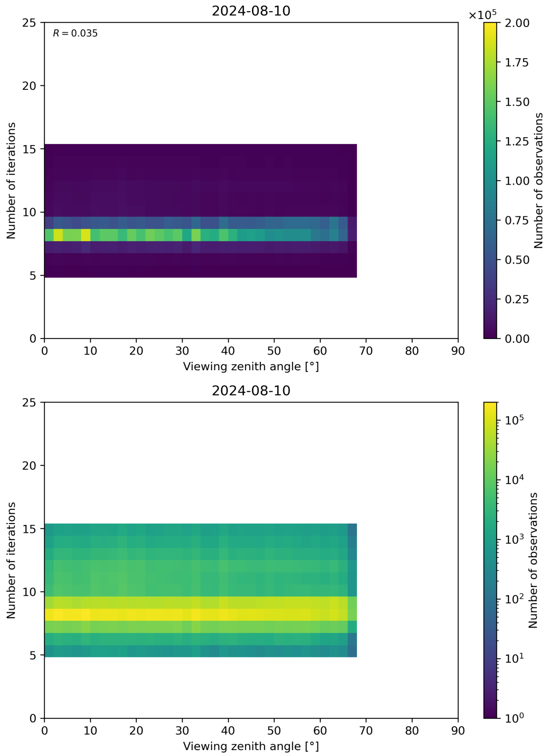
Figure 75: Scatter density plot of “Viewing zenith angle” against “Number of iterations” for 2024-08-09 to 2024-08-11.
