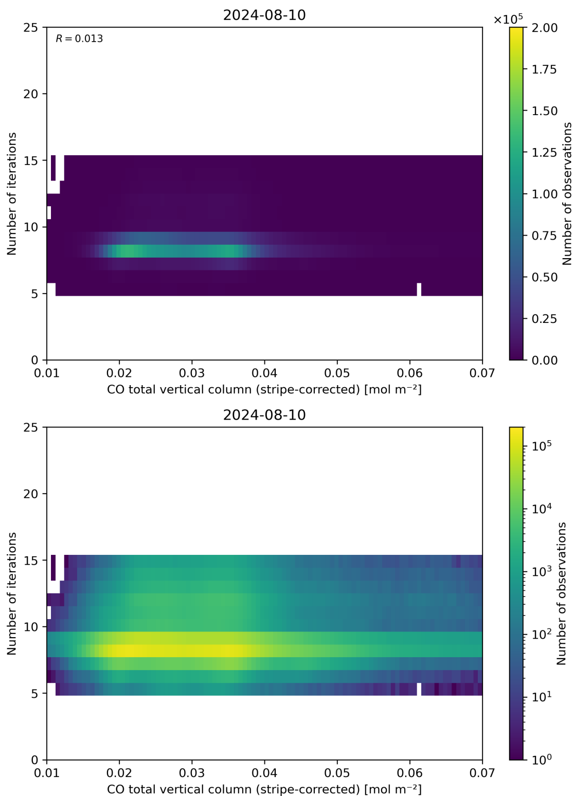
Figure 39: Scatter density plot of “CO total vertical column (stripe-corrected)” against “Number of iterations” for 2024-08-09 to 2024-08-11.
