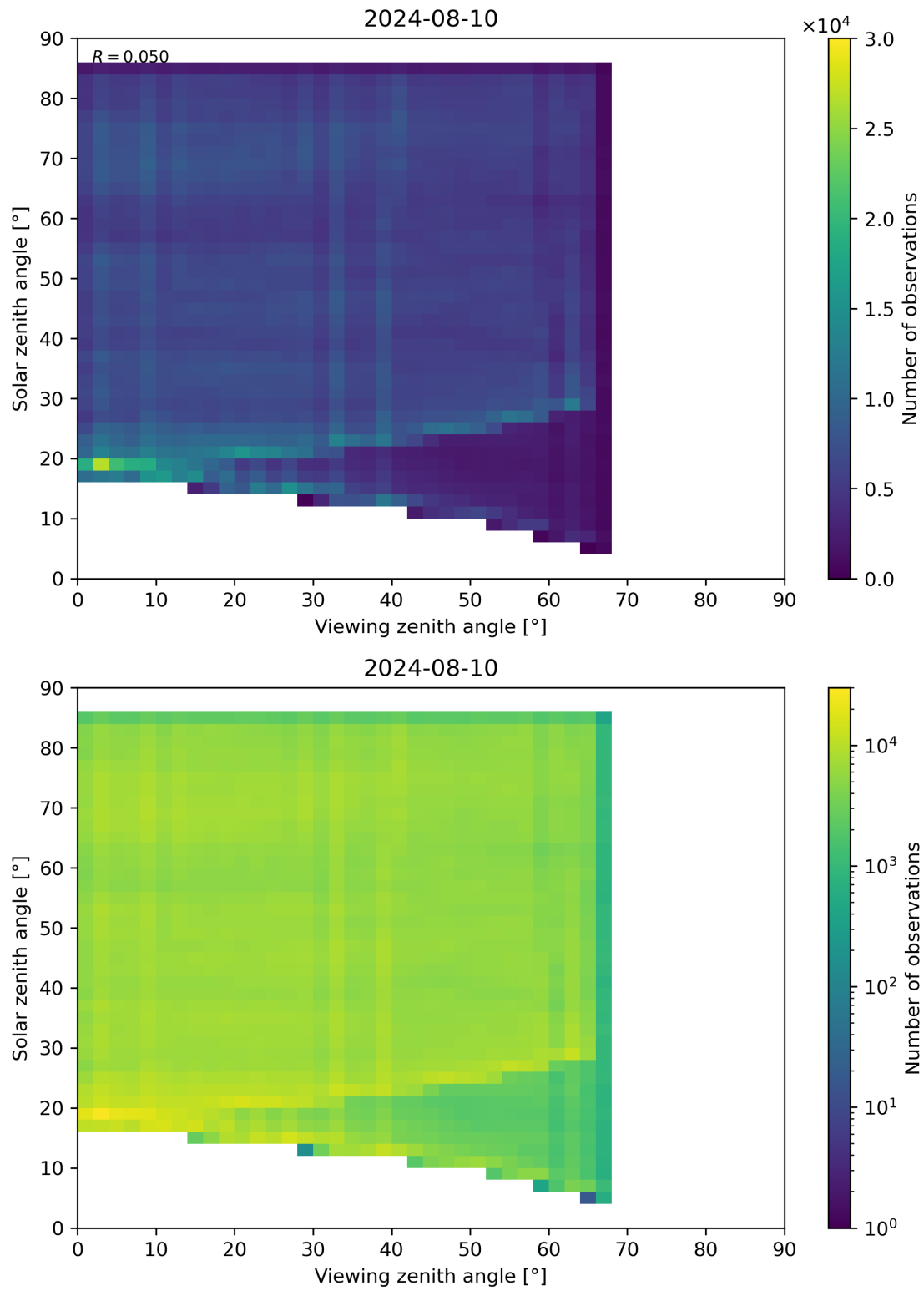
Figure 77: Scatter density plot of “Viewing zenith angle” against “Solar zenith angle” for 2024-08-09 to 2024-08-11.
