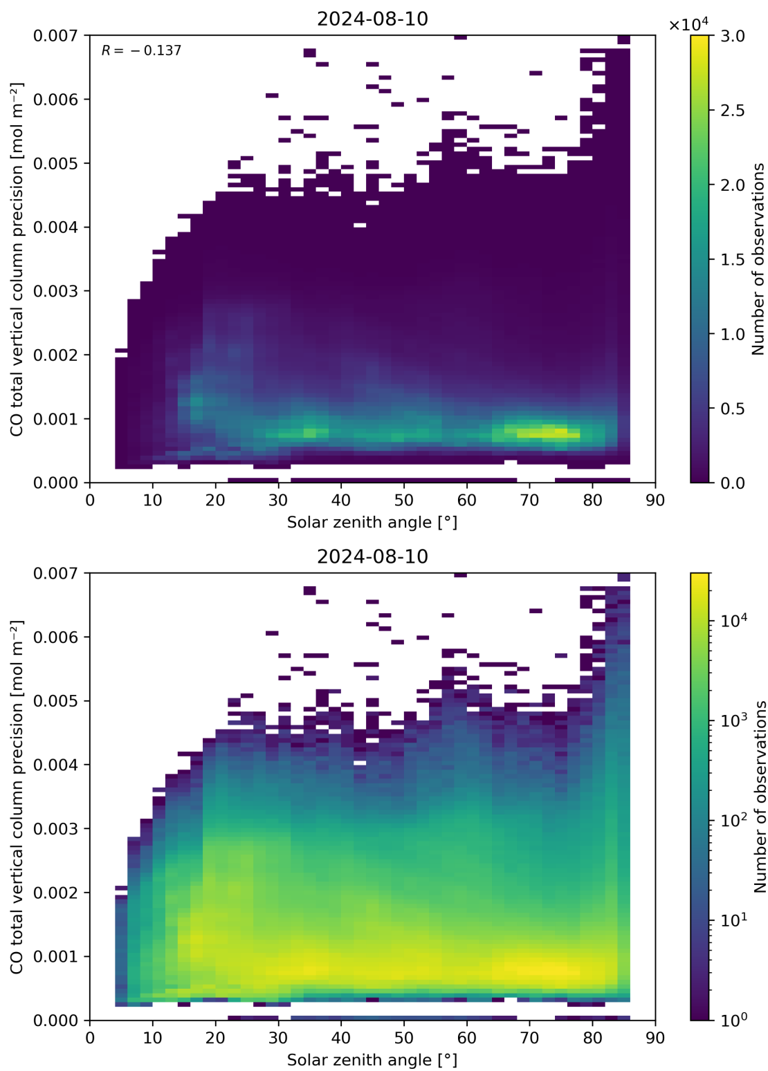
Figure 63: Scatter density plot of “Solar zenith angle” against “CO total vertical column precision” for 2024-08-09 to 2024-08-11.
