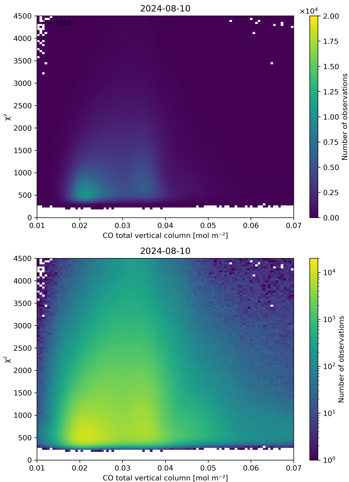
Figure 35: Scatter density plot of “CO total vertical column” against “ \chi^2 ” for 2024-08-09 to 2024-08-11.
