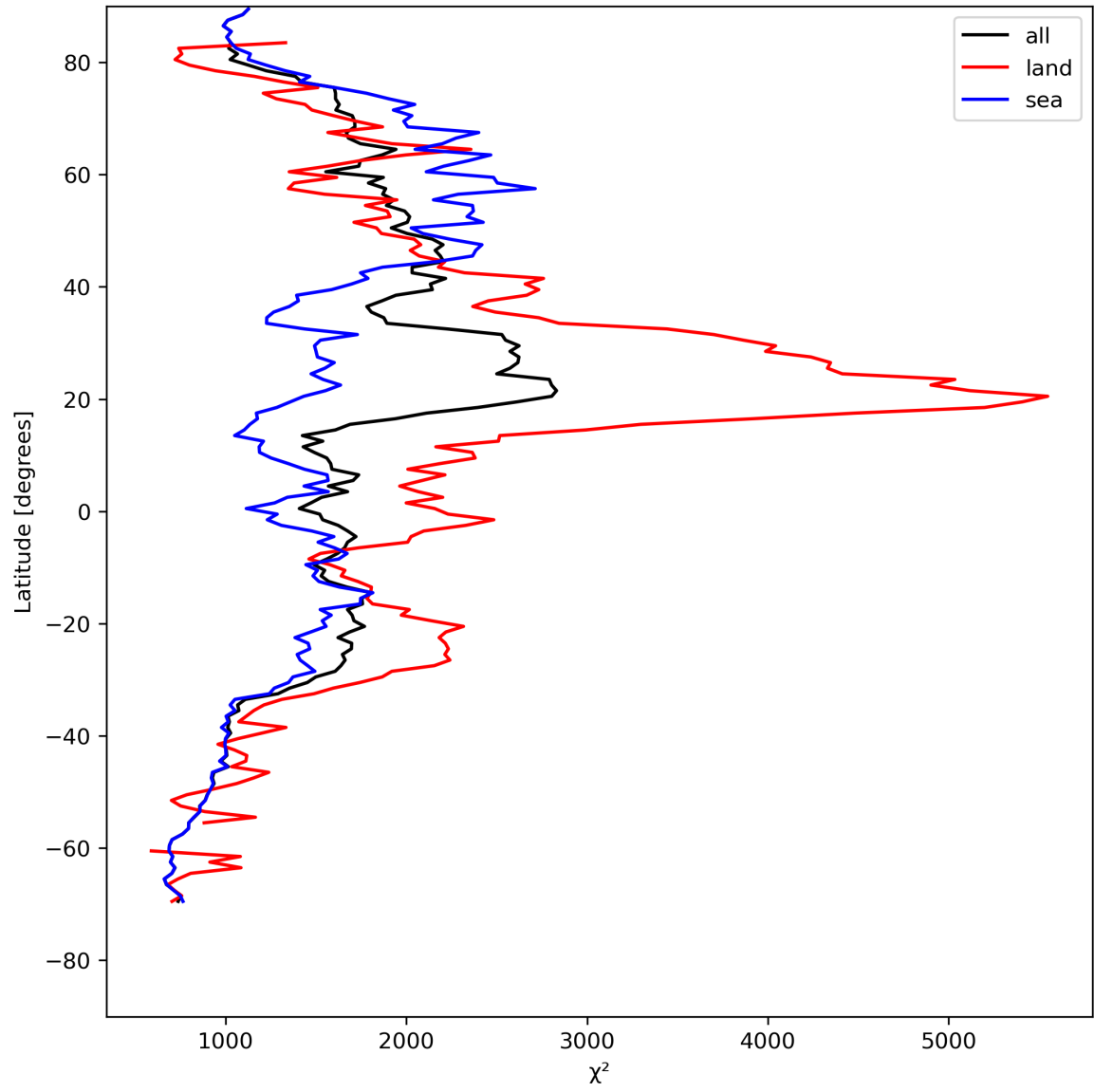
Figure 14: Zonal average of “ \chi^2 ” for 2024-08-09 to 2024-08-11.
