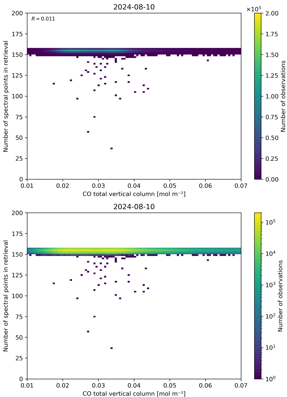
Figure 43: Scatter density plot of “CO total vertical column” against “Number of spectral points in retrieval” for 2024-08-09 to 2024-08-11.
