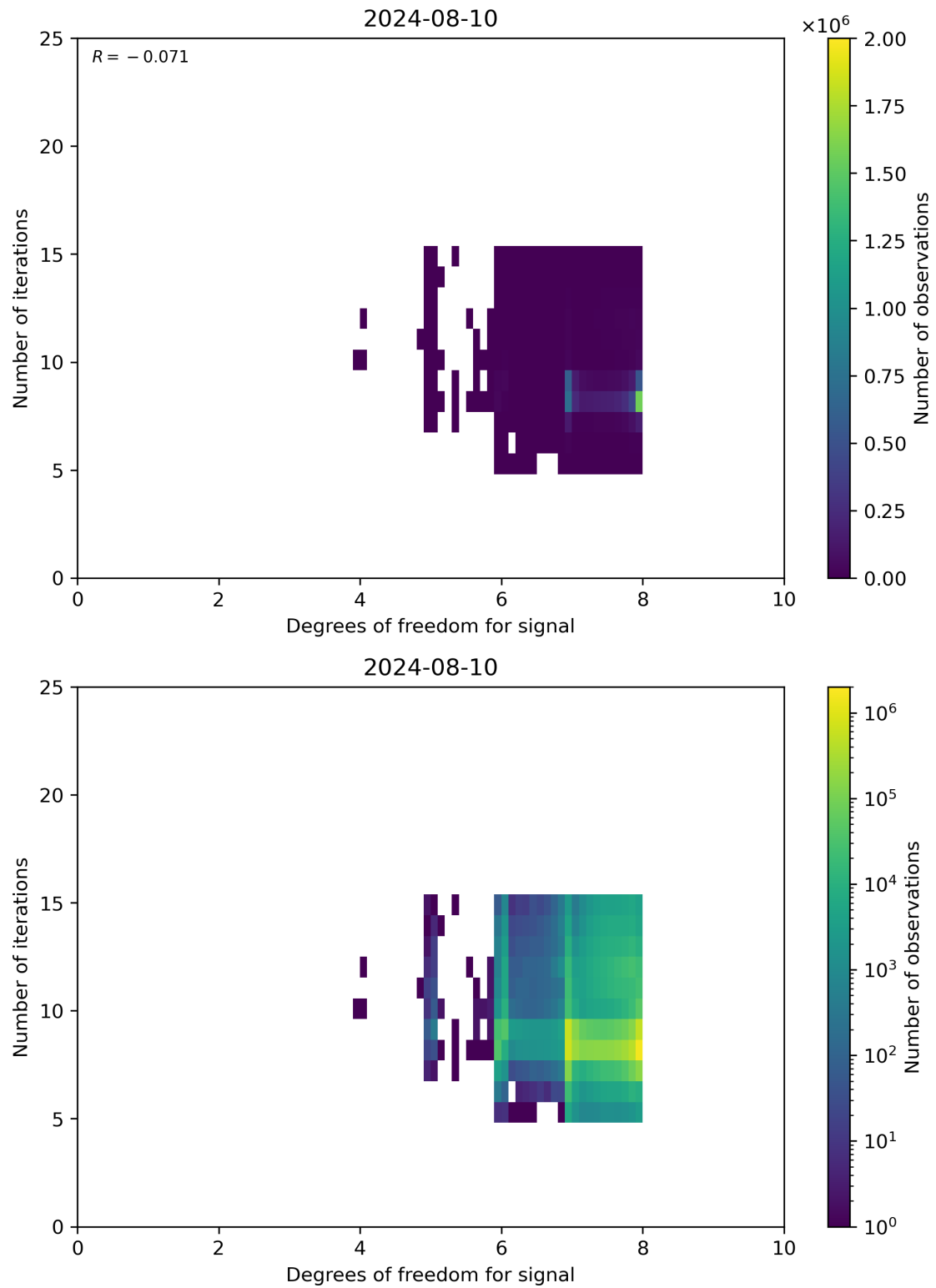
Figure 50: Scatter density plot of “Degrees of freedom for signal” against “Number of iterations” for 2024-08-09 to 2024-08-11.
