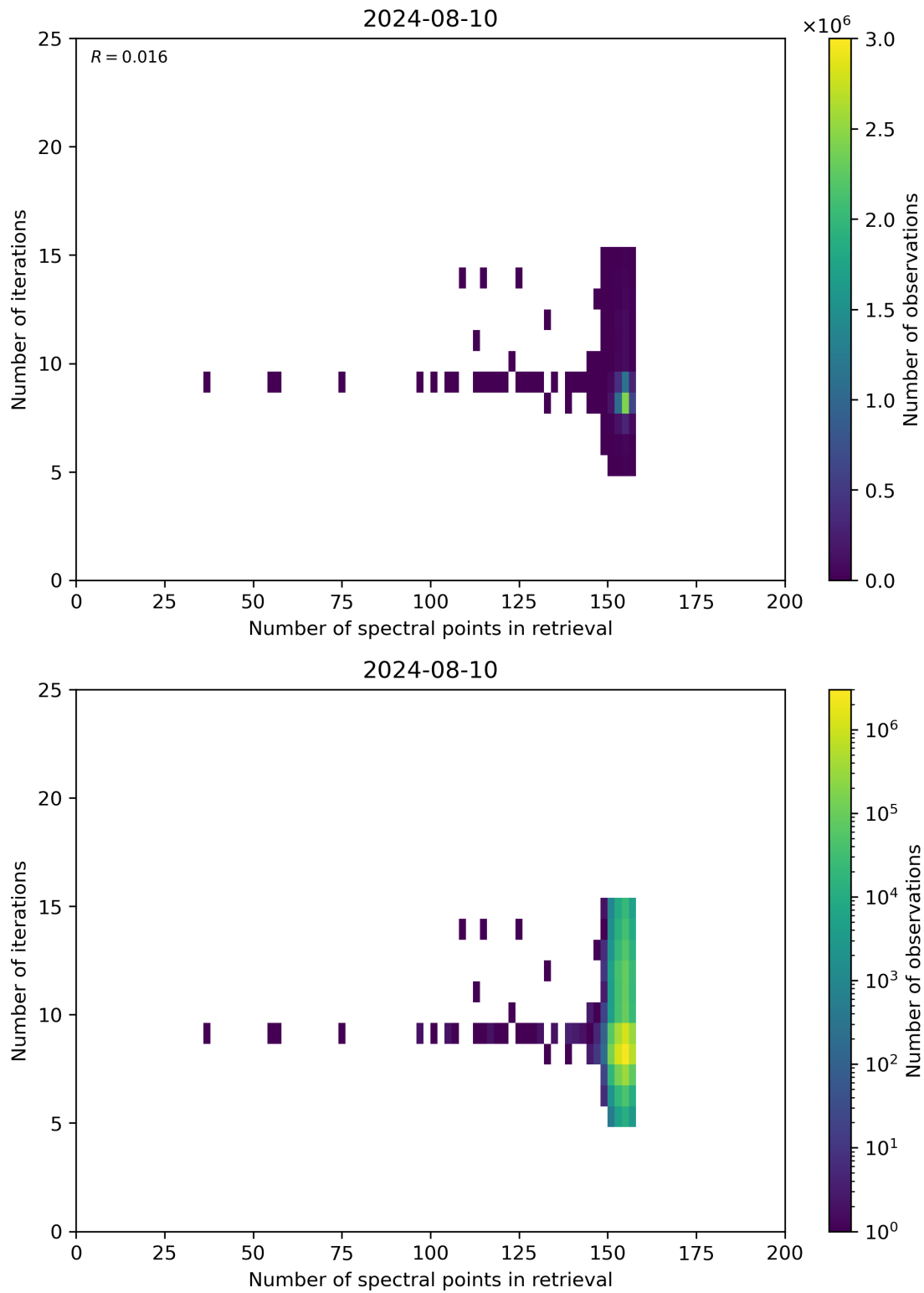
Figure 60: Scatter density plot of “Number of spectral points in retrieval” against “Number of iterations” for 2024-08-09 to 2024-08-11.
