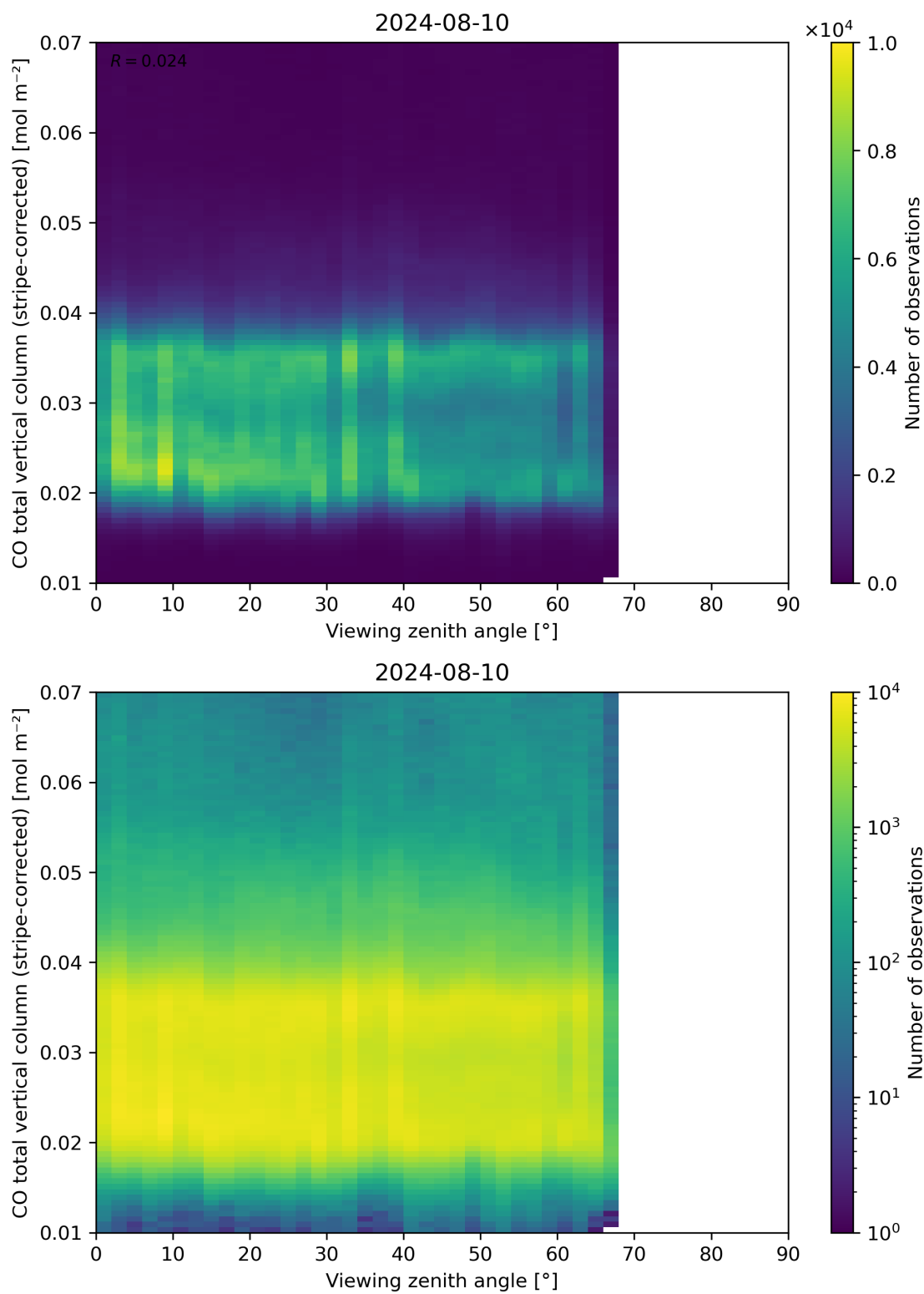
Figure 70: Scatter density plot of “Viewing zenith angle” against “CO total vertical column (stripe-corrected)” for 2024-08-09 to 2024-08-11.
