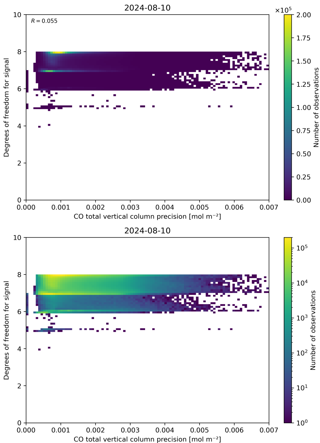
Figure 45: Scatter density plot of “CO total vertical column precision” against “Degrees of freedom for signal” for 2024-08-09 to 2024-08-11.
