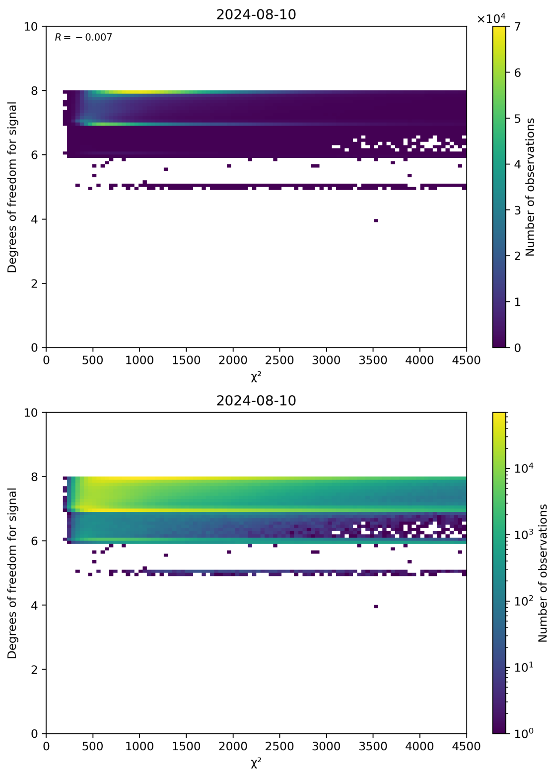
Figure 48: Scatter density plot of “ \chi^2 ” against “Degrees of freedom for signal” for 2024-08-09 to 2024-08-11.
