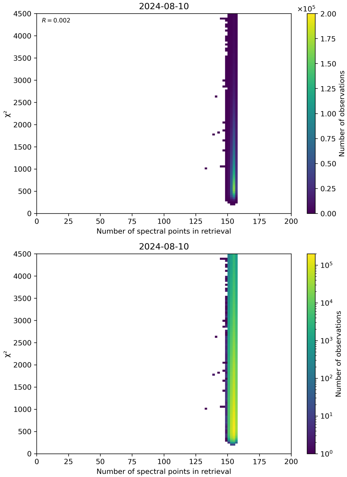
Figure 58: Scatter density plot of “Number of spectral points in retrieval” against “ \chi^2 ” for 2024-08-09 to 2024-08-11.
