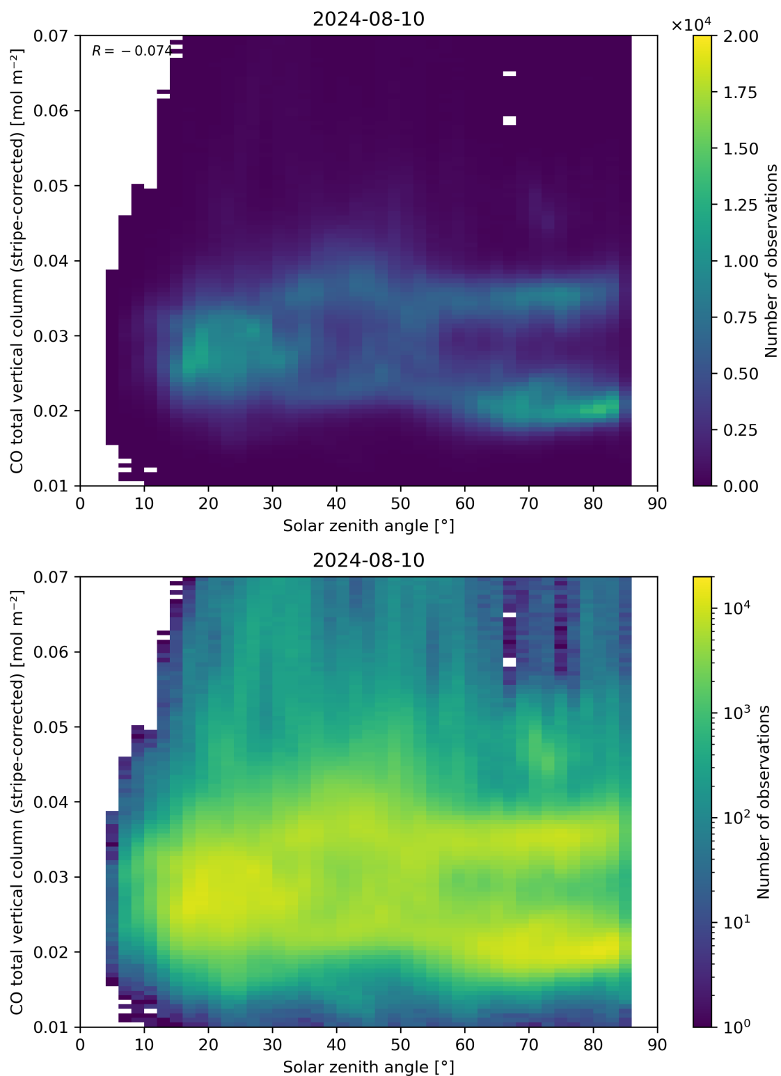
Figure 62: Scatter density plot of “Solar zenith angle” against “CO total vertical column (stripe-corrected)” for 2024-08-09 to 2024-08-11.
