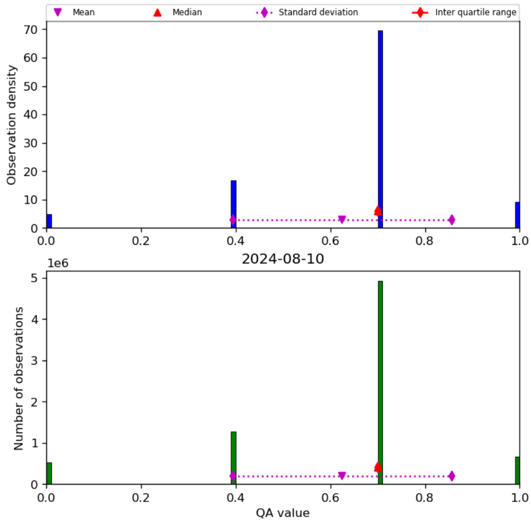
Figure 17: Histogram of “QA value” for 2024-08-09 to 2024-08-11
