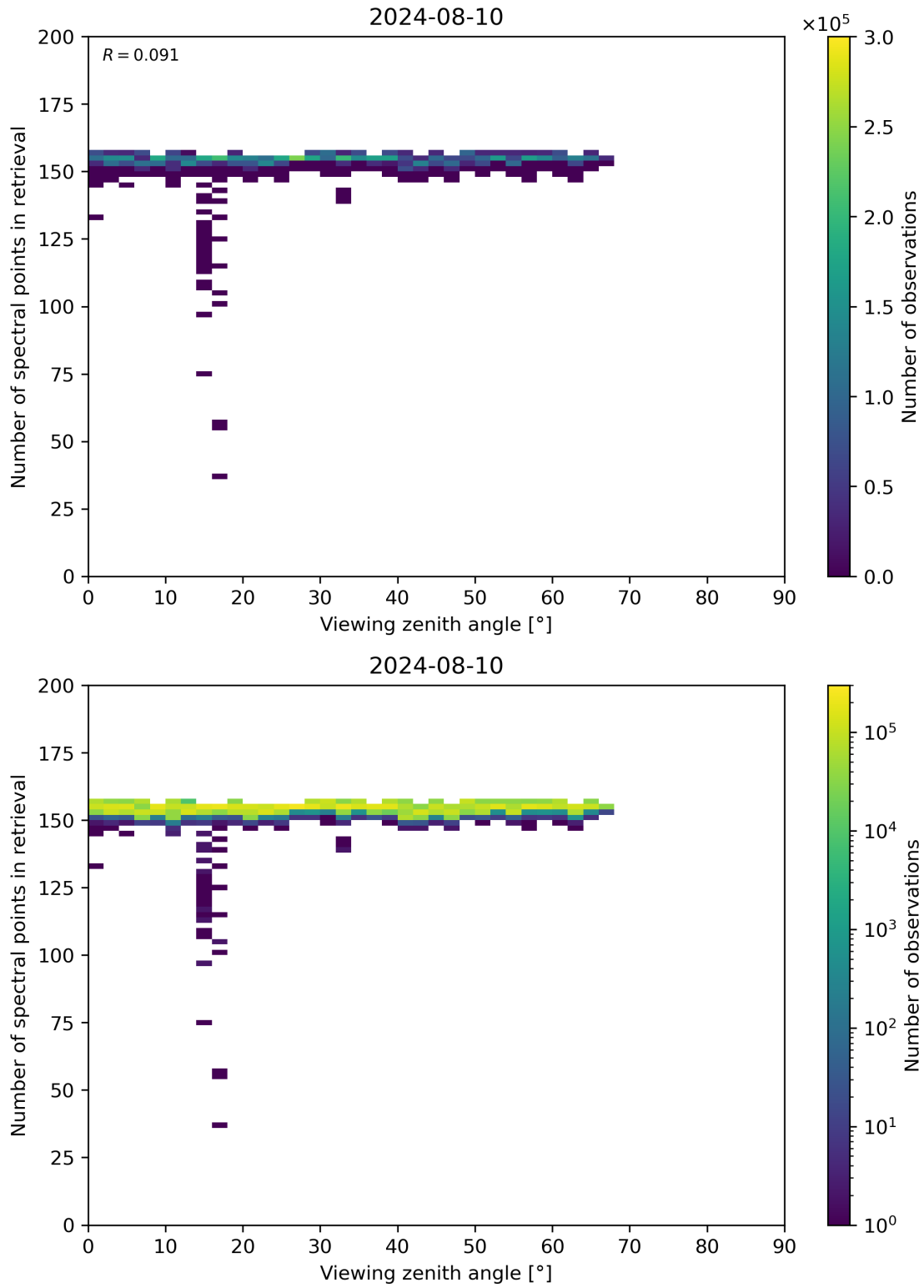
Figure 76: Scatter density plot of “Viewing zenith angle” against “Number of spectral points in retrieval” for 2024-08-09 to 2024-08-11.
