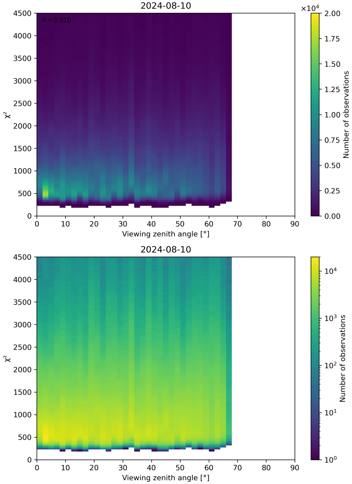
Figure 72: Scatter density plot of “Viewing zenith angle” against “ \chi^2 ” for 2024-08-09 to 2024-08-11.
