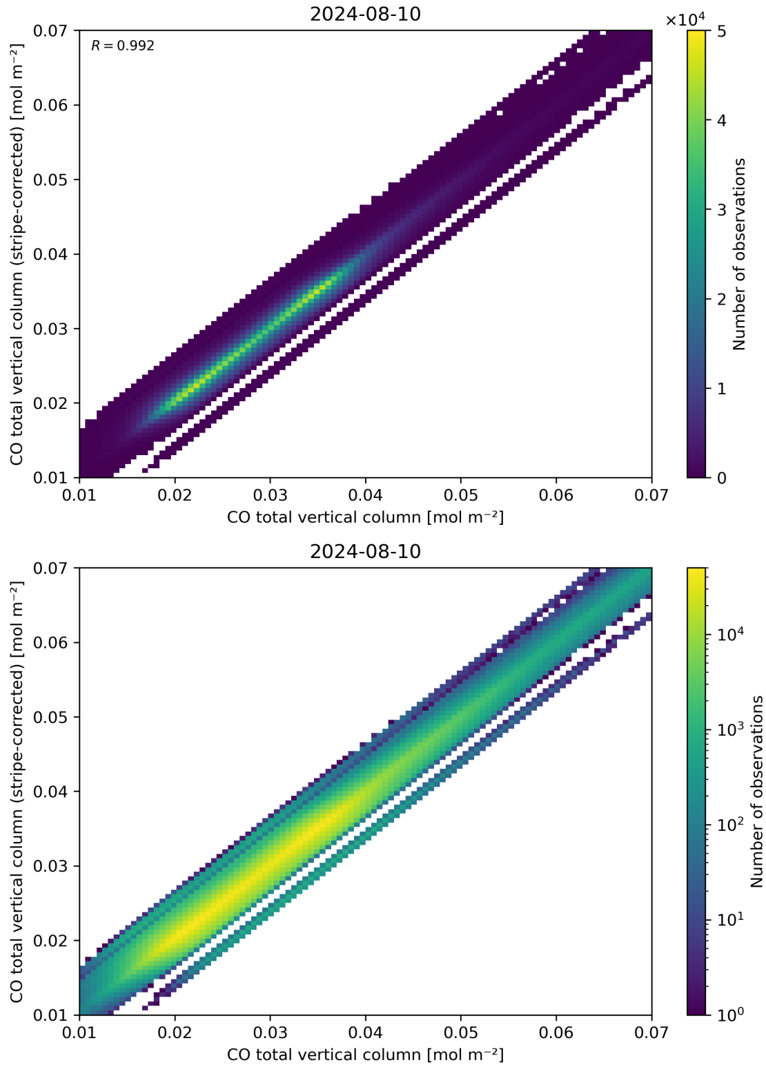
Figure 33: Scatter density plot of “CO total vertical column” against “CO total vertical column (stripe-corrected)” for 2024-08-09 to 2024-08-11.
