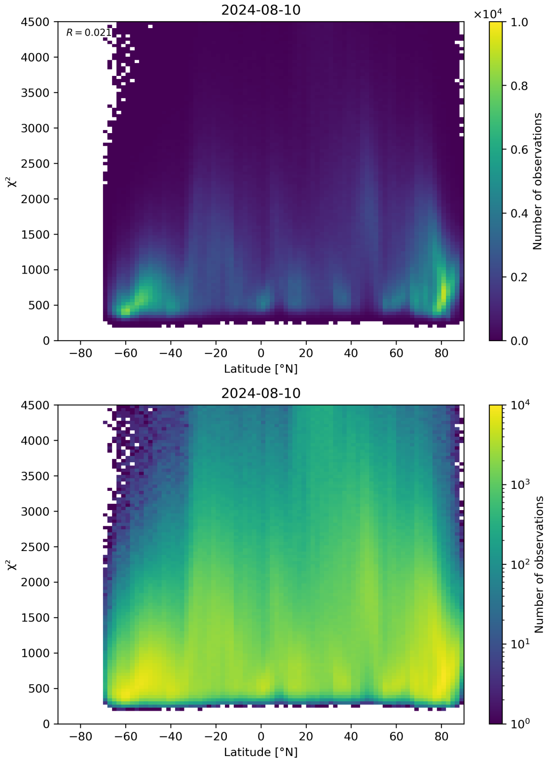
Figure 54: Scatter density plot of “Latitude” against “ \chi^2 ” for 2024-08-09 to 2024-08-11.
