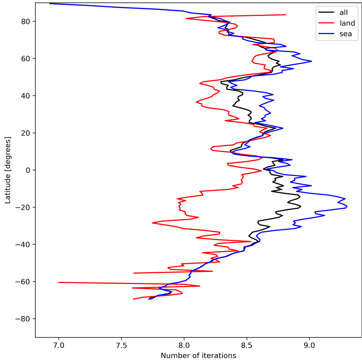
Figure 16: Zonal average of “Number of iterations” for 2024-08-09 to 2024-08-11.
