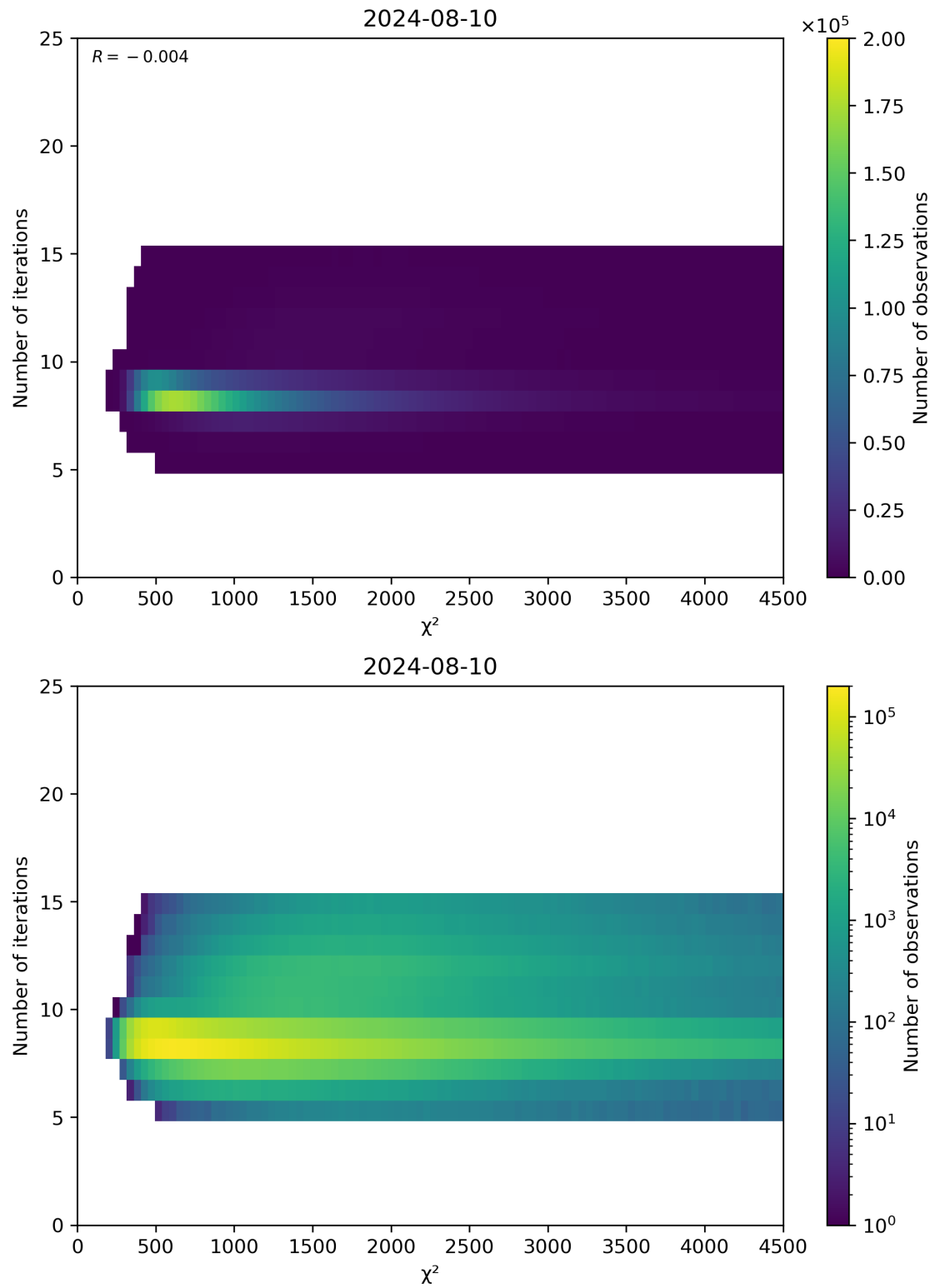
Figure 49: Scatter density plot of “ \chi^2 ” against “Number of iterations” for 2024-08-09 to 2024-08-11.
