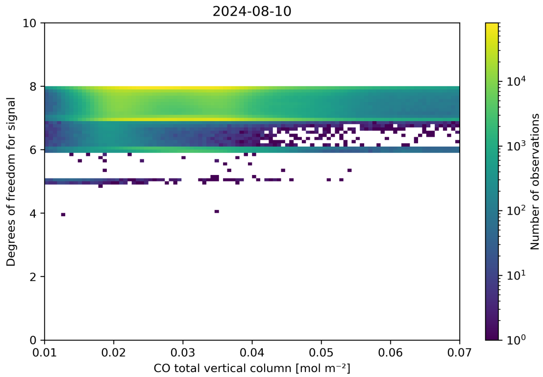
Figure 41: Scatter density plot of “CO total vertical column” against “Degrees of freedom for signal” for 2024-08-09 to 2024-08-11.
