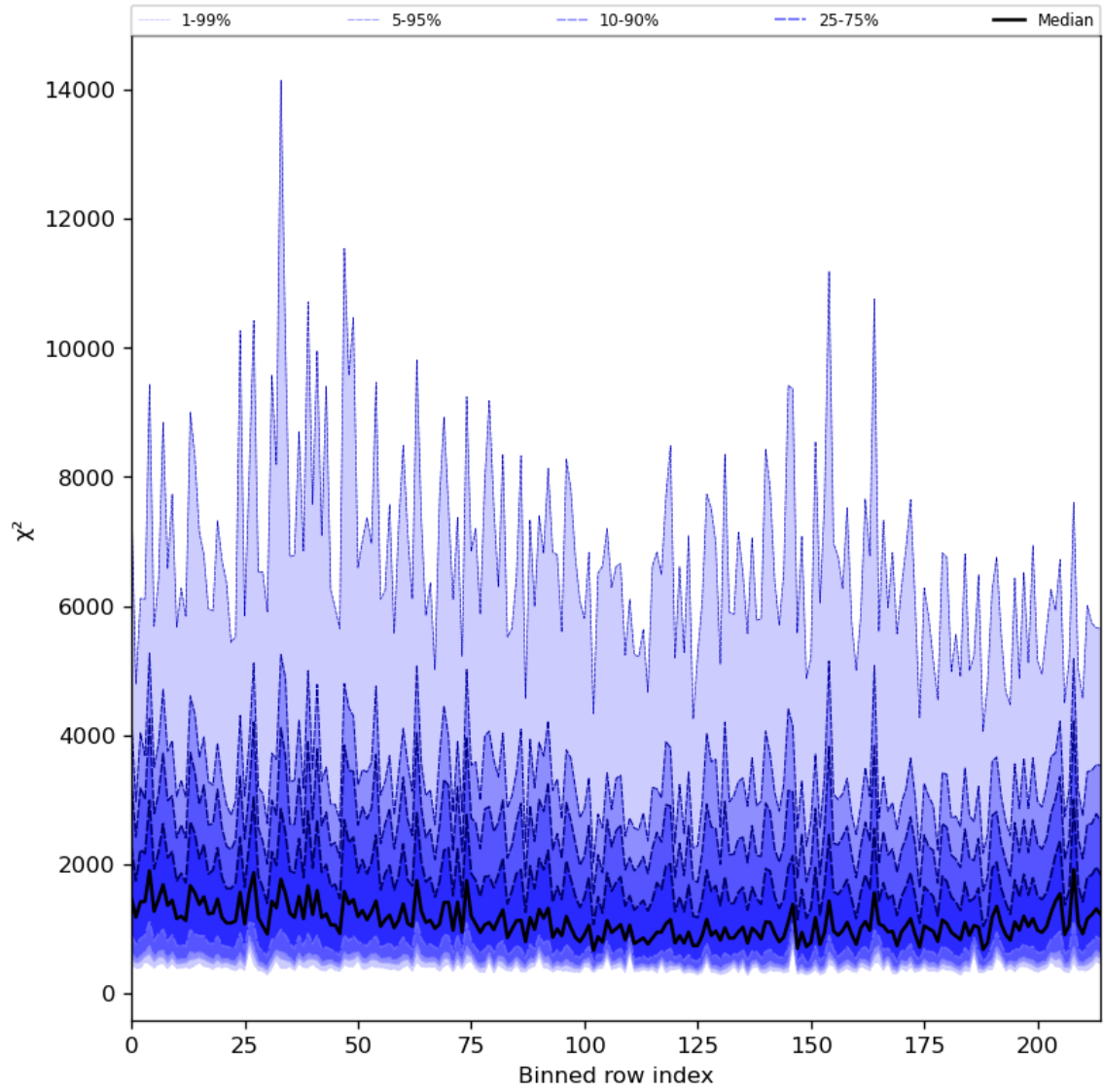
Figure 30: Along track statistics of “ \chi^2 ” for 2024-08-09 to 2024-08-11
