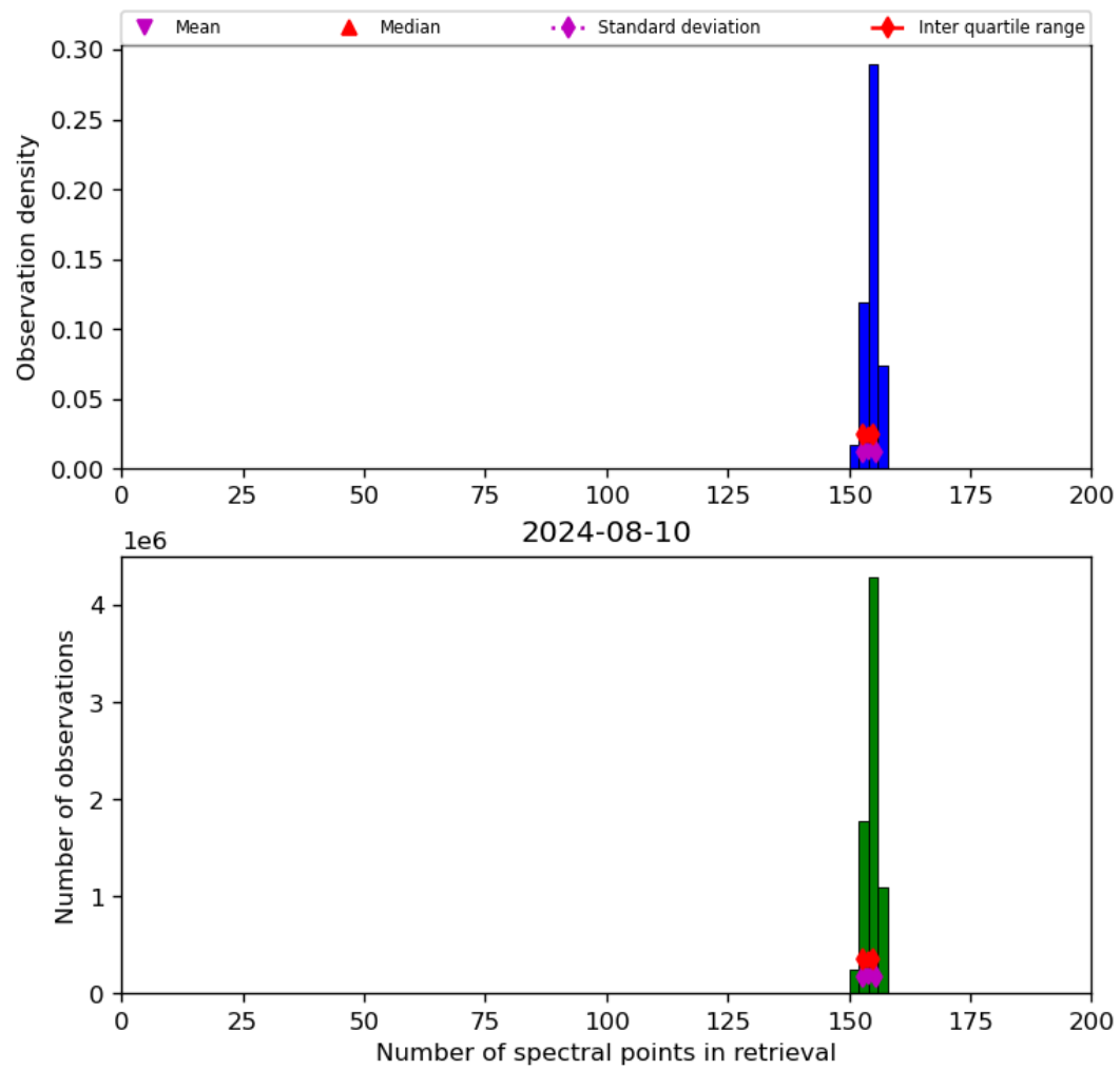
Figure 21: Histogram of “Number of spectral points in retrieval” for 2024-08-09 to 2024-08-11
