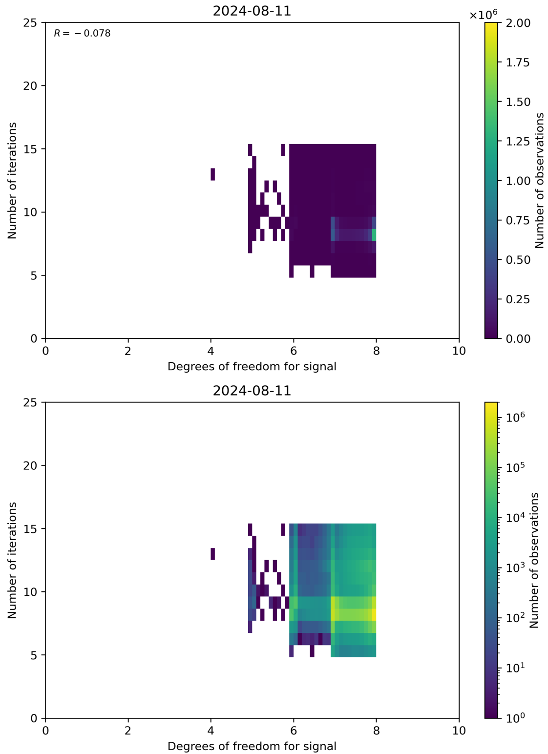
Figure 50: Scatter density plot of “Degrees of freedom for signal” against “Number of iterations” for 2024-08-11 to 2024-08-11.
