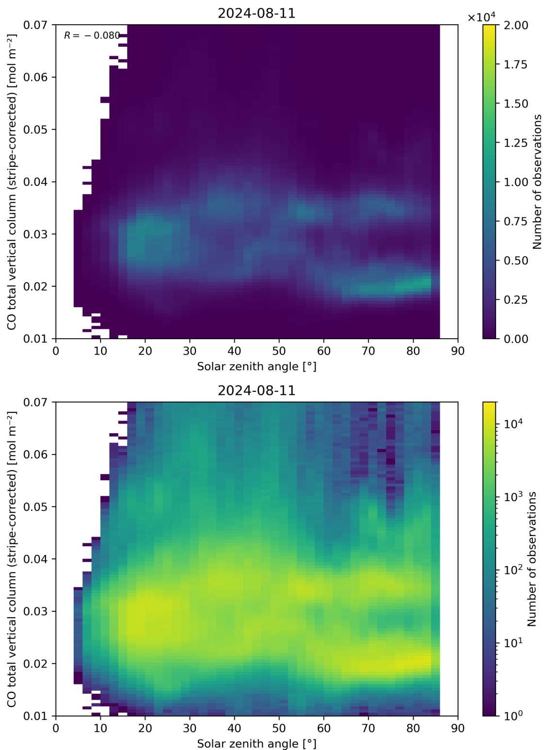
Figure 62: Scatter density plot of “Solar zenith angle” against “CO total vertical column (stripe-corrected)” for 2024-08-11 to 2024-08-11.
