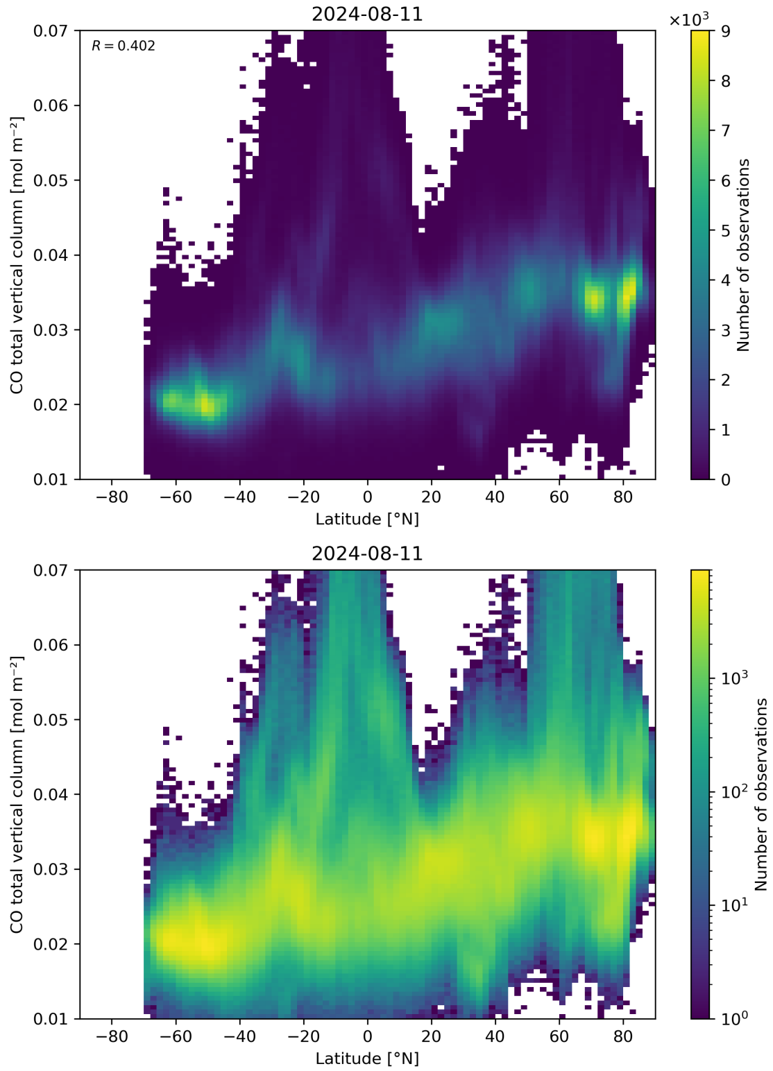
Figure 51: Scatter density plot of “Latitude” against “CO total vertical column” for 2024-08-11 to 2024-08-11.
