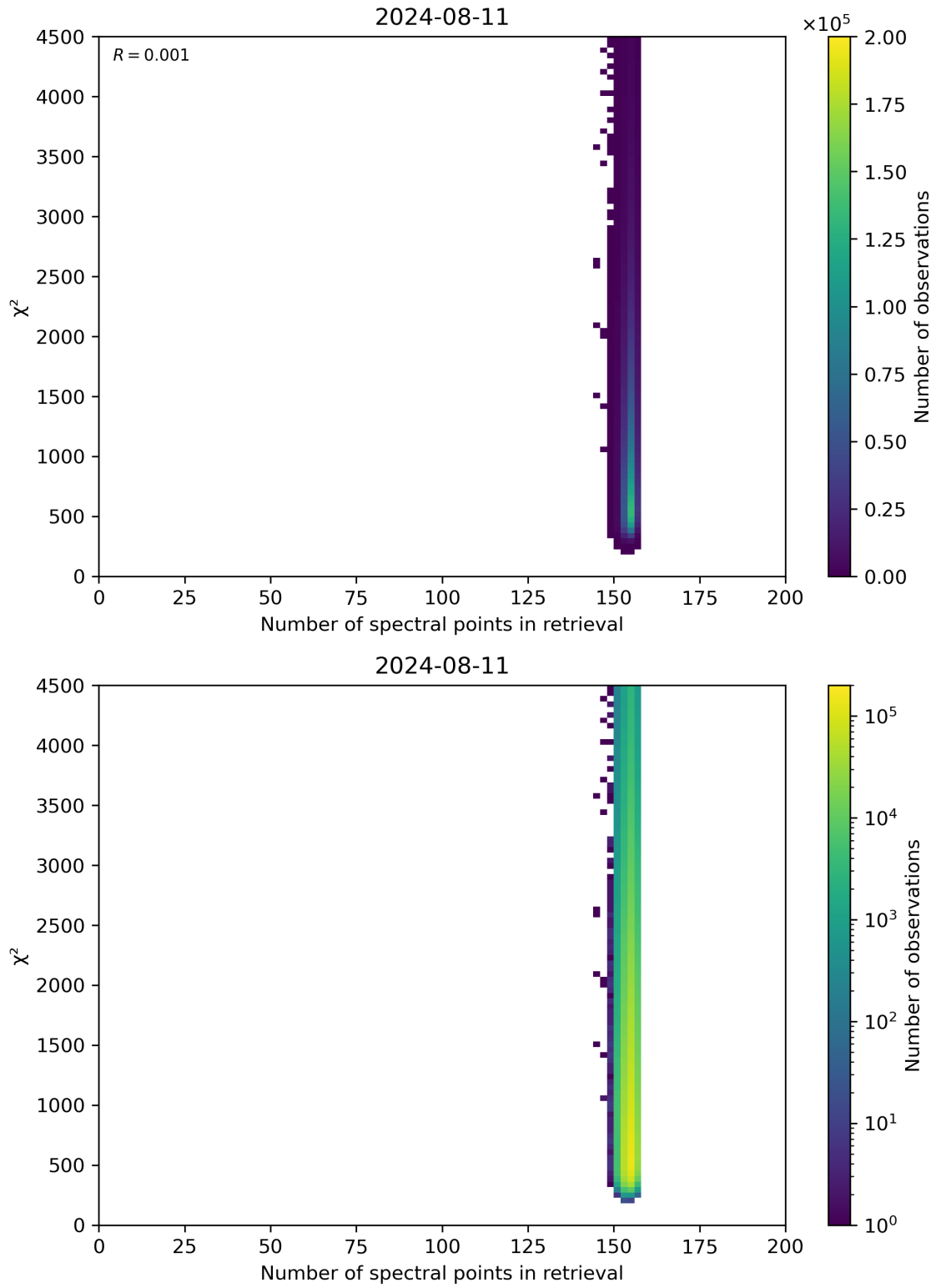
Figure 58: Scatter density plot of “Number of spectral points in retrieval” against “ \chi^2 ” for 2024-08-11 to 2024-08-11.
