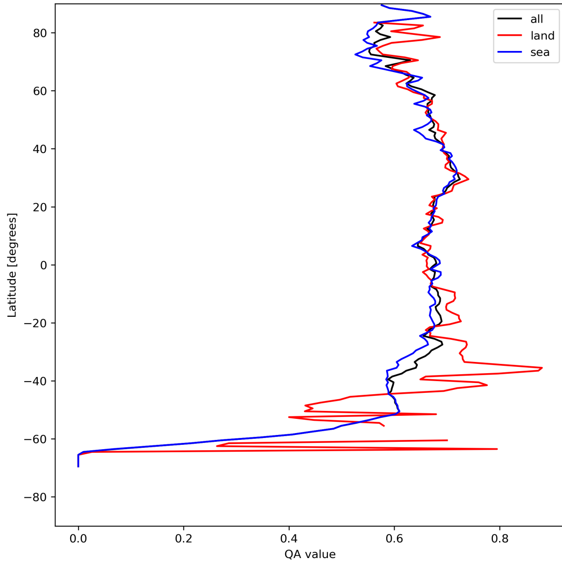
Figure 9: Zonal average of “QA value” for 2024-08-11 to 2024-08-11.
