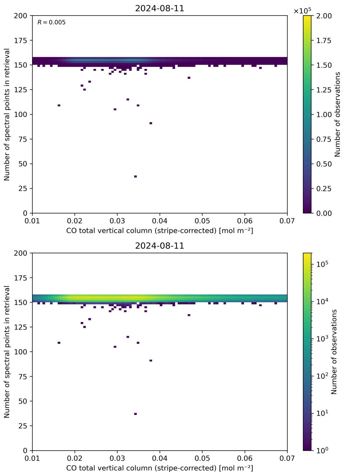
Figure 40: Scatter density plot of “CO total vertical column (stripe-corrected)” against “Number of spectral points in retrieval” for 2024-08-11 to 2024-08-11.
