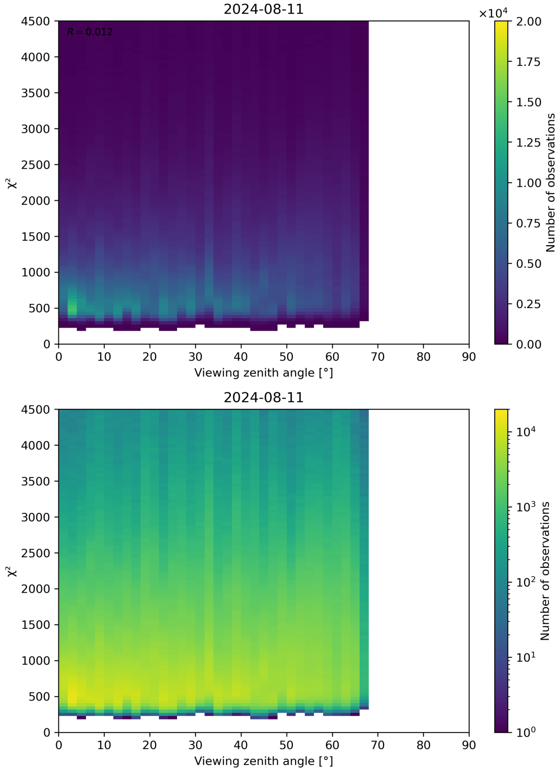
Figure 72: Scatter density plot of “Viewing zenith angle” against “ \chi^2 ” for 2024-08-11 to 2024-08-11.
