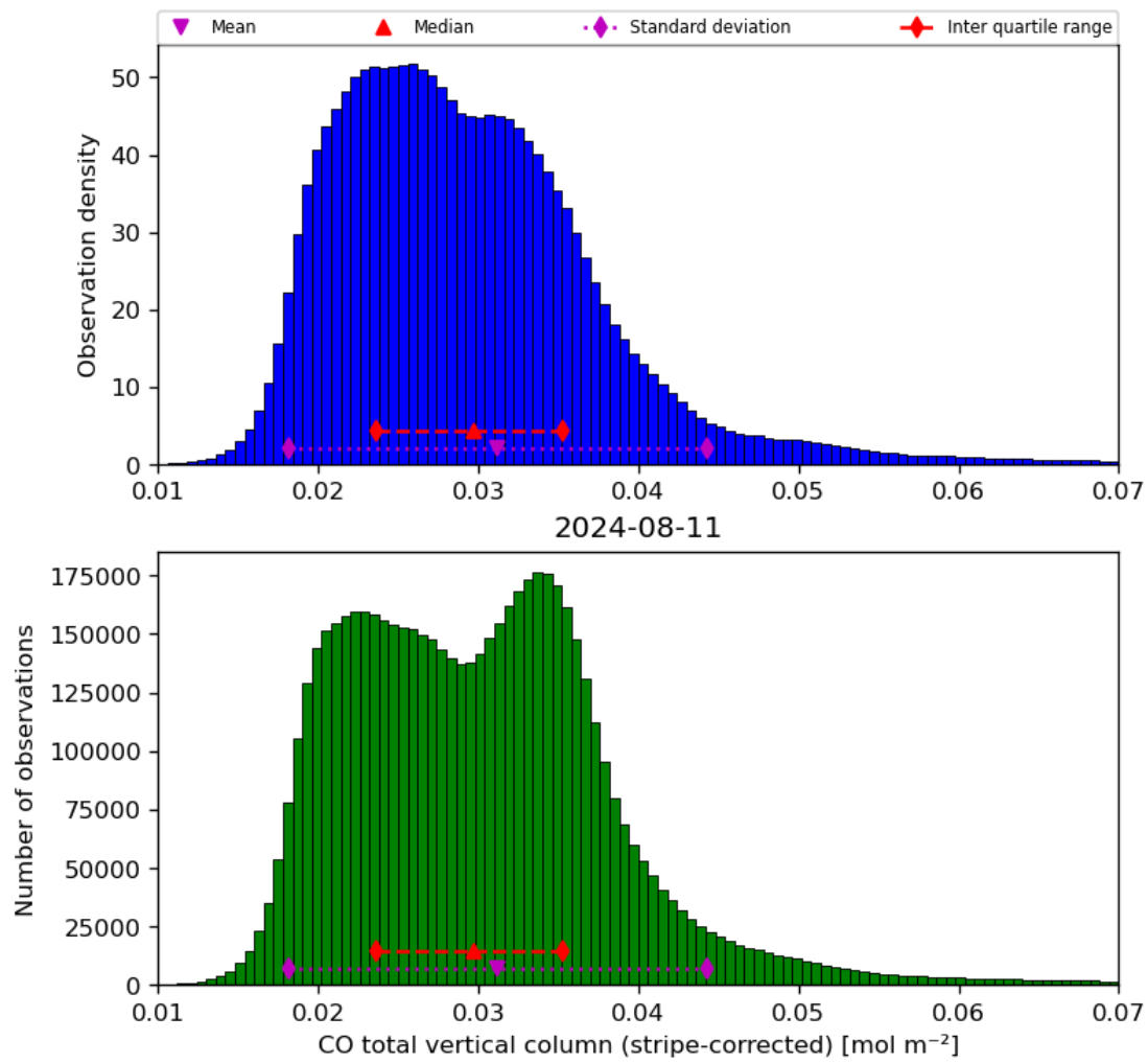
Figure 19: Histogram of “CO total vertical column (stripe-corrected)” for 2024-08-11 to 2024-08-11
