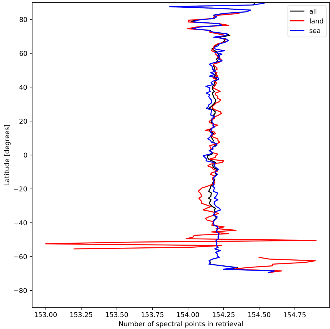
Figure 13: Zonal average of “Number of spectral points in retrieval” for 2024-08-11 to 2024-08-11.
