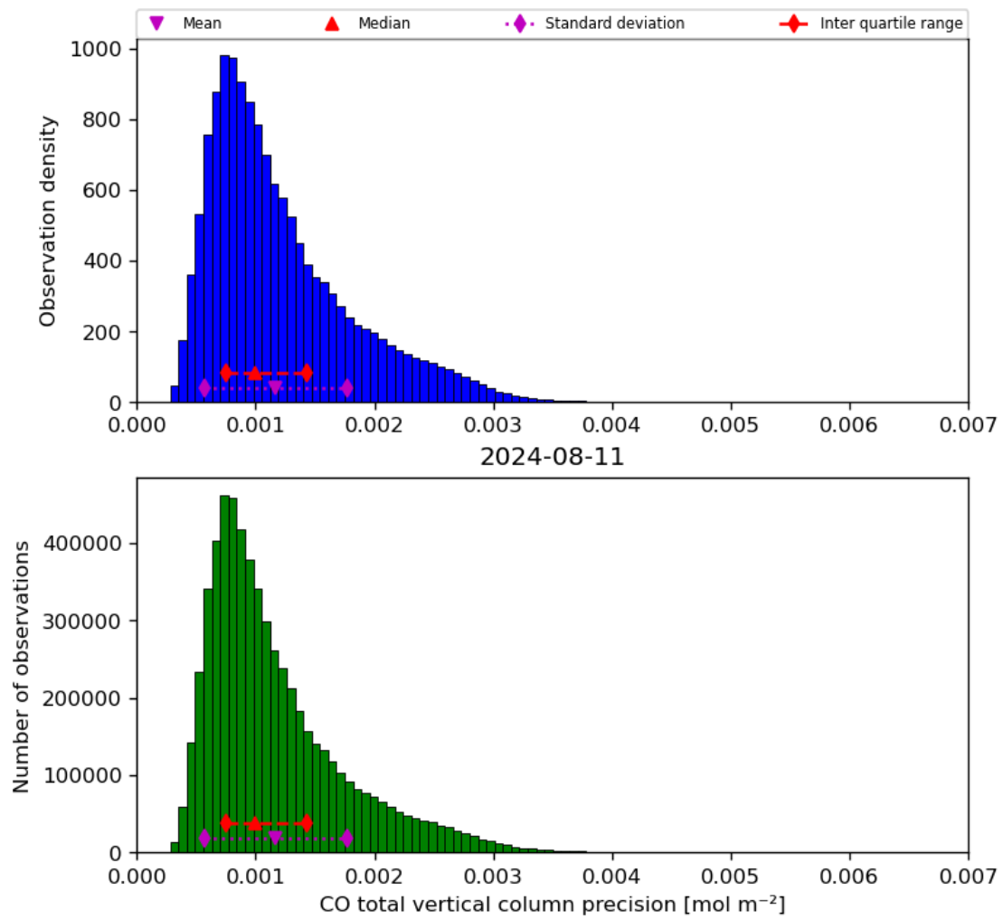
Figure 20: Histogram of “CO total vertical column precision” for 2024-08-11 to 2024-08-11
