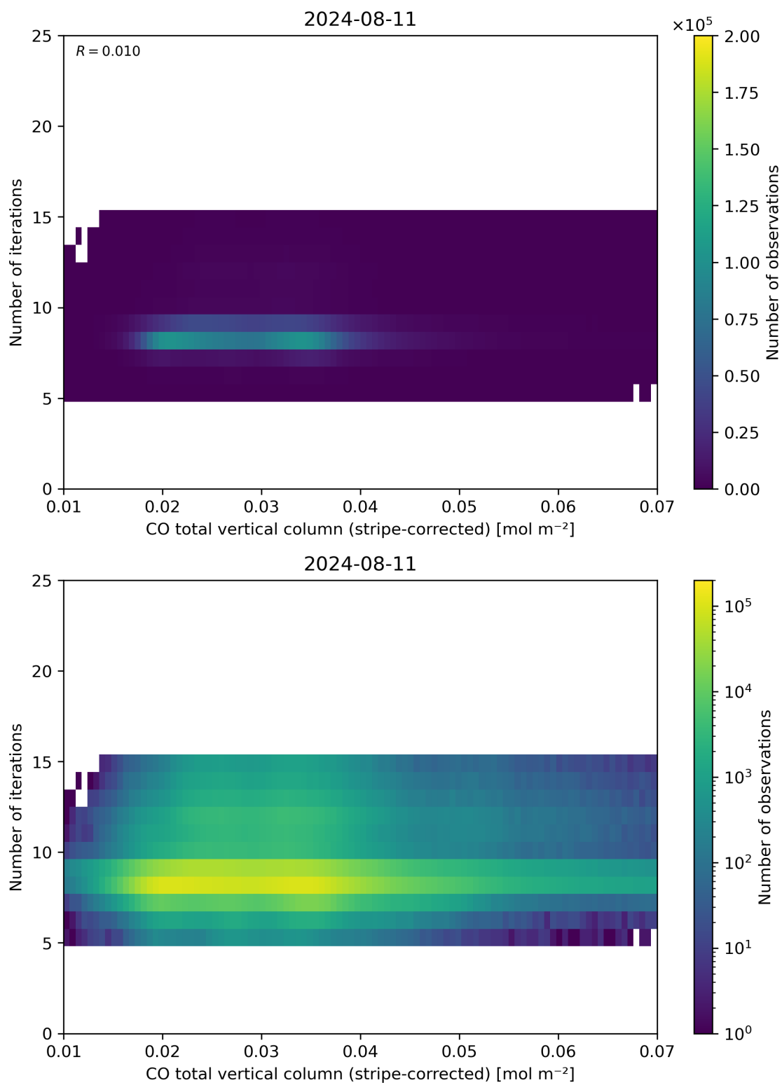
Figure 39: Scatter density plot of “CO total vertical column (stripe-corrected)” against “Number of iterations” for 2024-08-11 to 2024-08-11.
