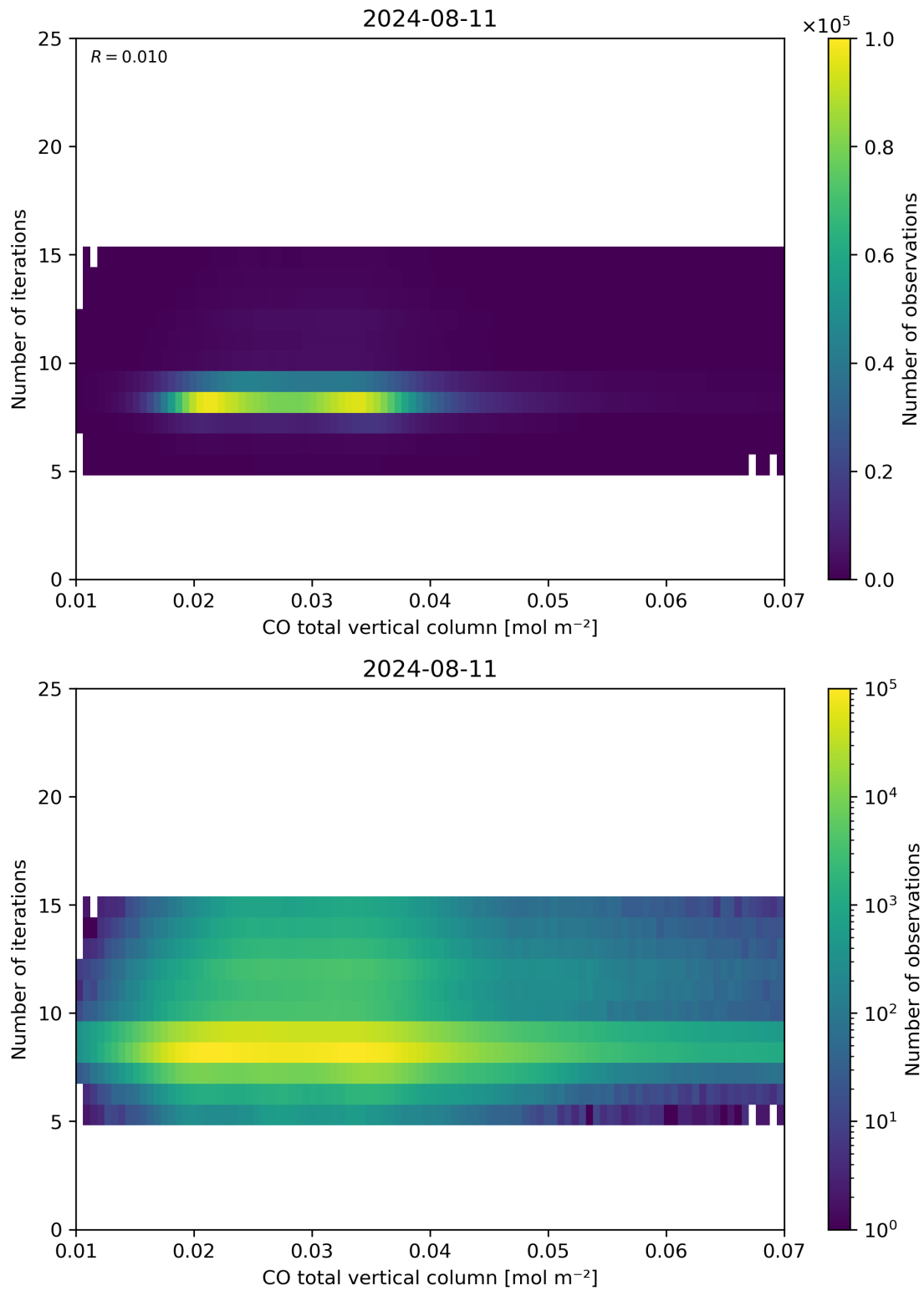
Figure 42: Scatter density plot of “CO total vertical column” against “Number of iterations” for 2024-08-11 to 2024-08-11.
