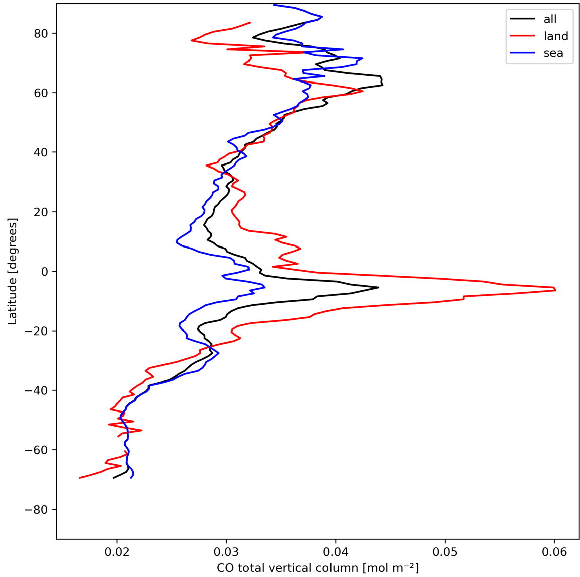
Figure 10: Zonal average of “CO total vertical column” for 2024-08-11 to 2024-08-11.
