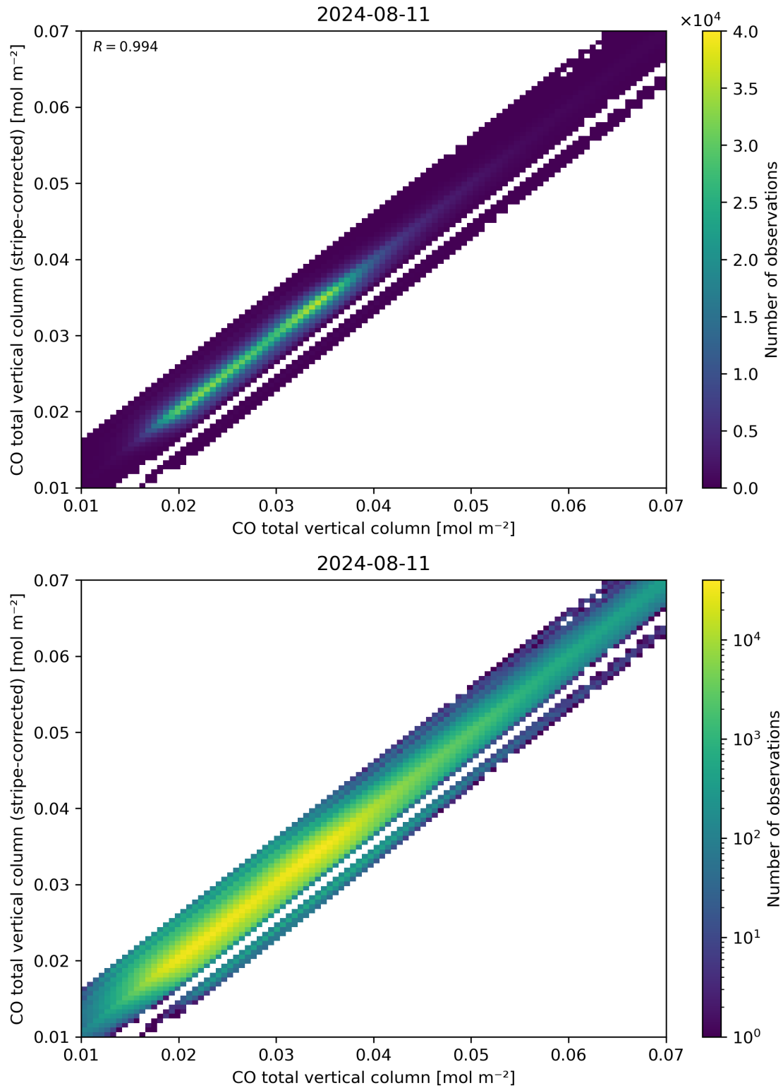
Figure 33: Scatter density plot of “CO total vertical column” against “CO total vertical column (stripe-corrected)” for 2024-08-11 to 2024-08-11.
