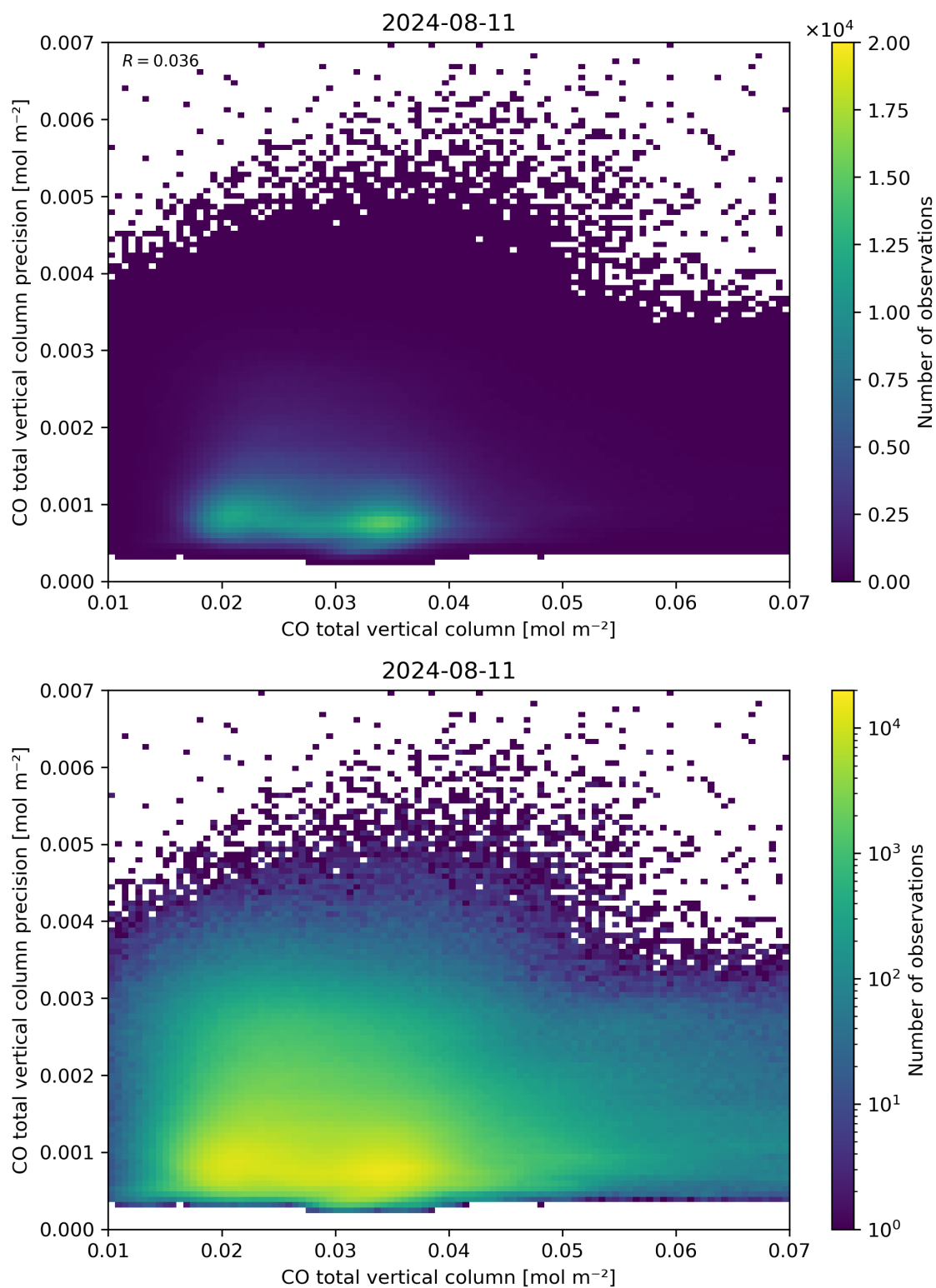
Figure 34: Scatter density plot of “CO total vertical column” against “CO total vertical column precision” for 2024-08-11 to 2024-08-11.
