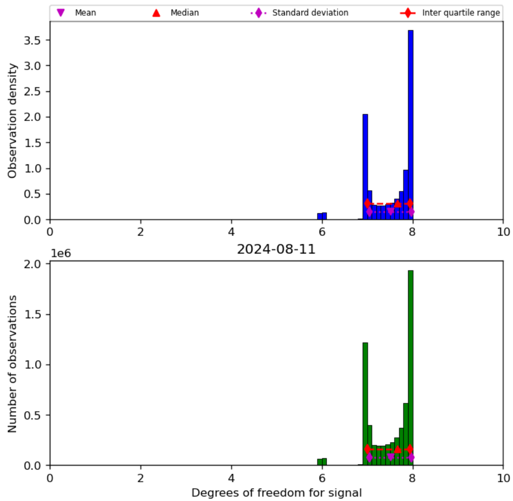
Figure 23: Histogram of “Degrees of freedom for signal” for 2024-08-11 to 2024-08-11
