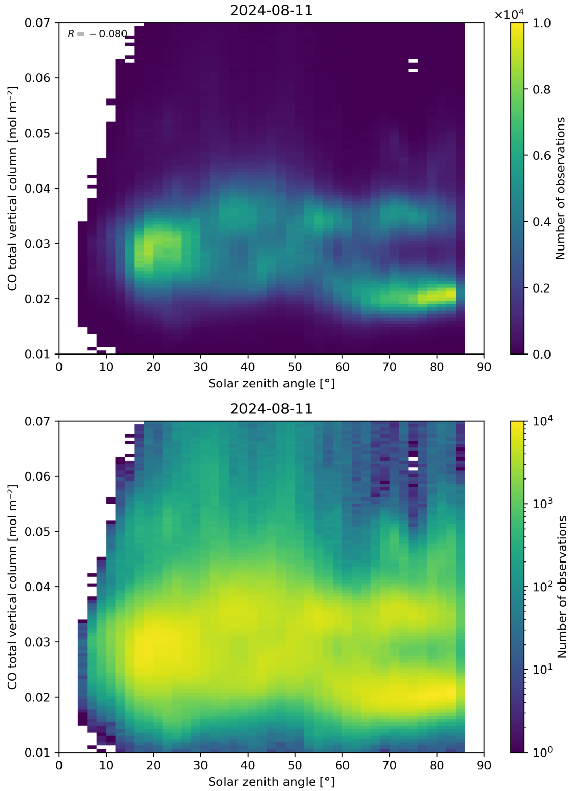
Figure 61: Scatter density plot of “Solar zenith angle” against “CO total vertical column” for 2024-08-11 to 2024-08-11.
