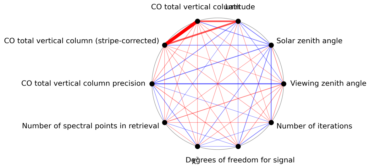
Figure 1: Map of correlation graph for 2024-08-11 to 2024-08-11.
