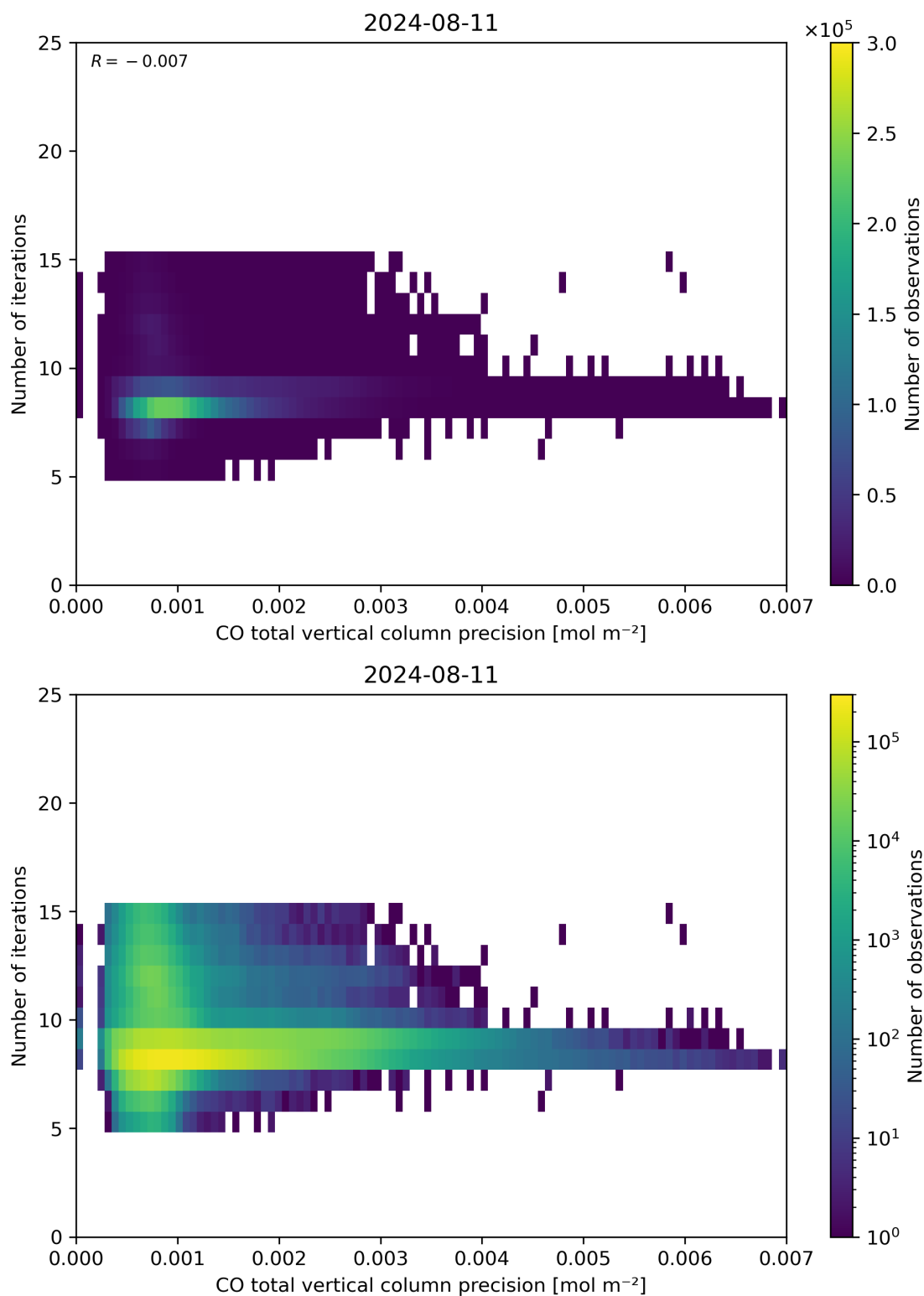
Figure 46: Scatter density plot of “CO total vertical column precision” against “Number of iterations” for 2024-08-11 to 2024-08-11.
