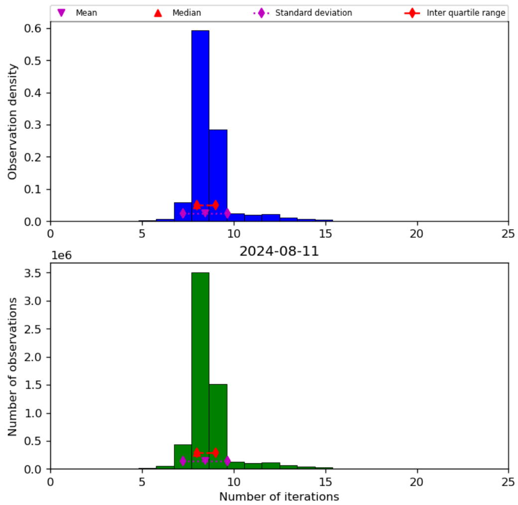
Figure 24: Histogram of “Number of iterations” for 2024-08-11 to 2024-08-11
