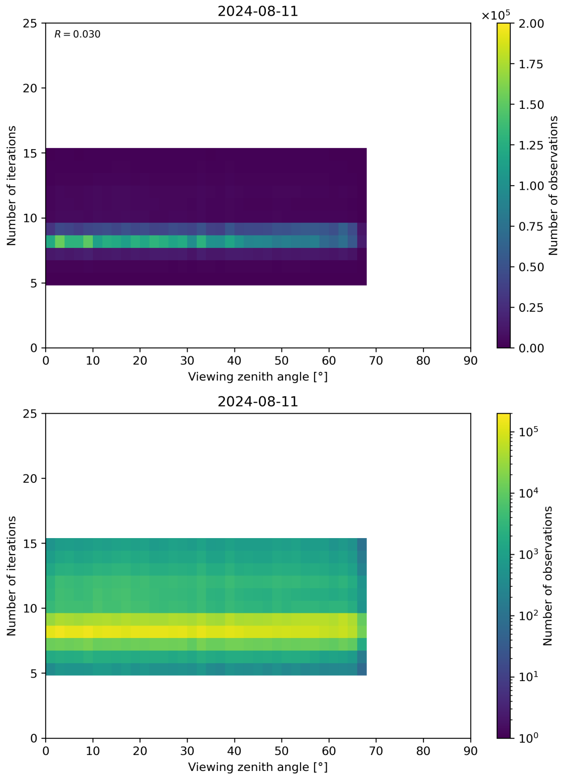
Figure 75: Scatter density plot of “Viewing zenith angle” against “Number of iterations” for 2024-08-11 to 2024-08-11.
