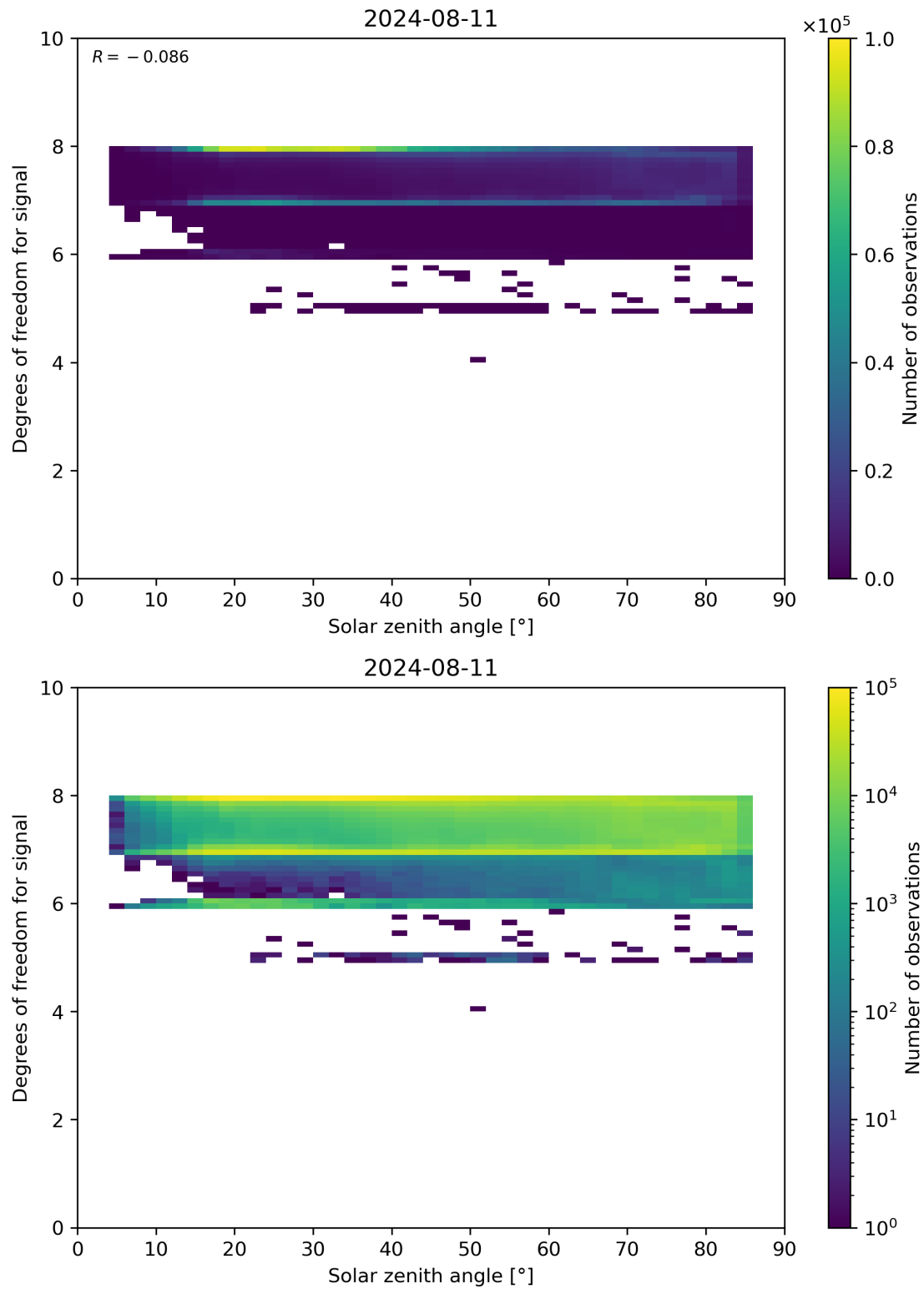
Figure 65: Scatter density plot of “Solar zenith angle” against “Degrees of freedom for signal” for 2024-08-11 to 2024-08-11.
