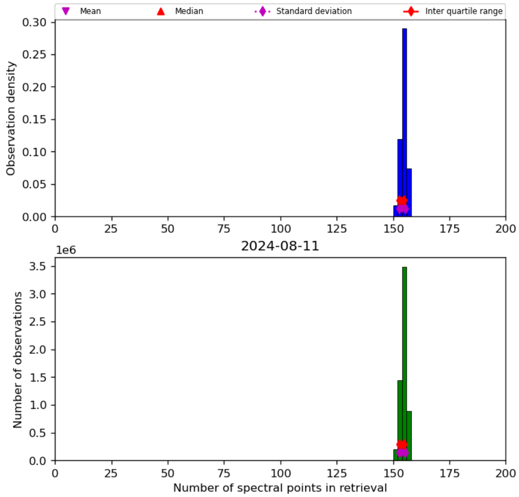
Figure 21: Histogram of “Number of spectral points in retrieval” for 2024-08-11 to 2024-08-11
