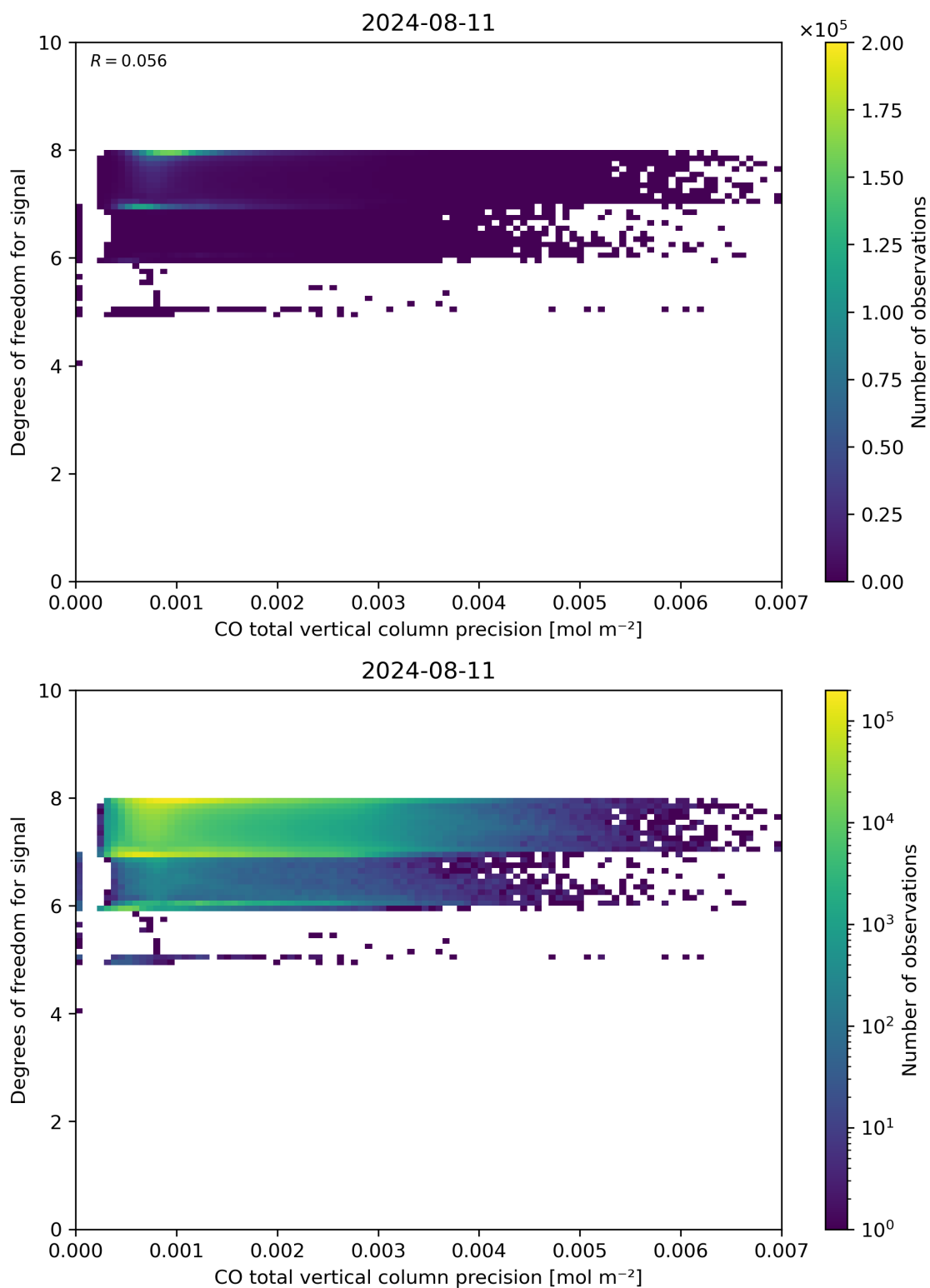
Figure 45: Scatter density plot of “CO total vertical column precision” against “Degrees of freedom for signal” for 2024-08-11 to 2024-08-11.
