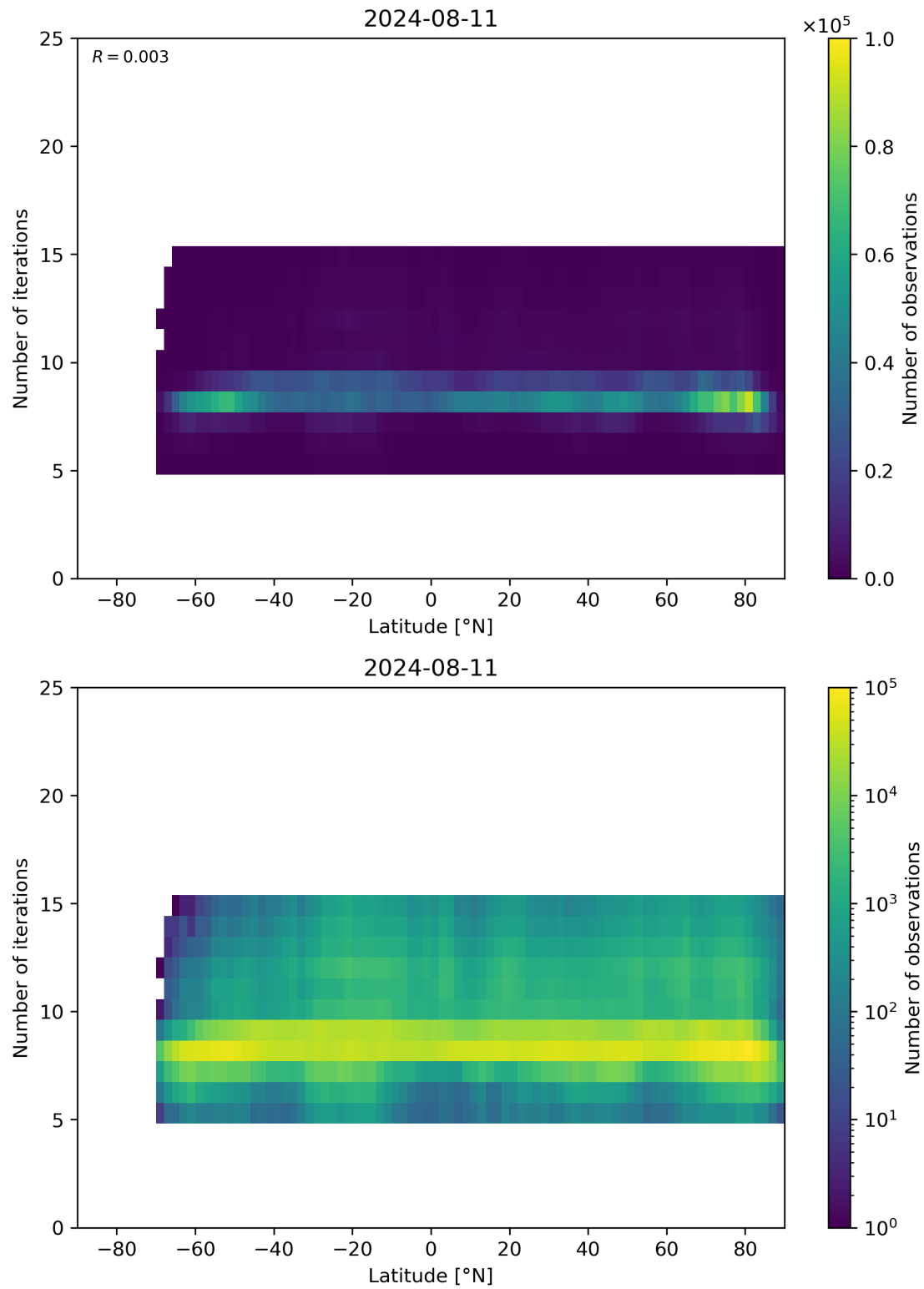
Figure 56: Scatter density plot of “Latitude” against “Number of iterations” for 2024-08-11 to 2024-08-11.
