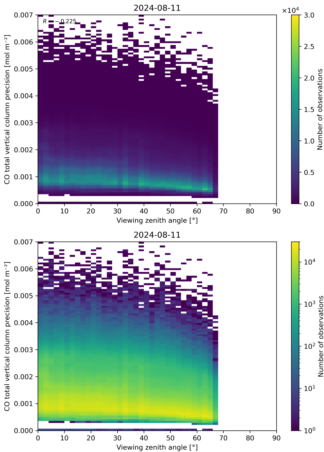
Figure 71: Scatter density plot of “Viewing zenith angle” against “CO total vertical column precision” for 2024-08-11 to 2024-08-11.
