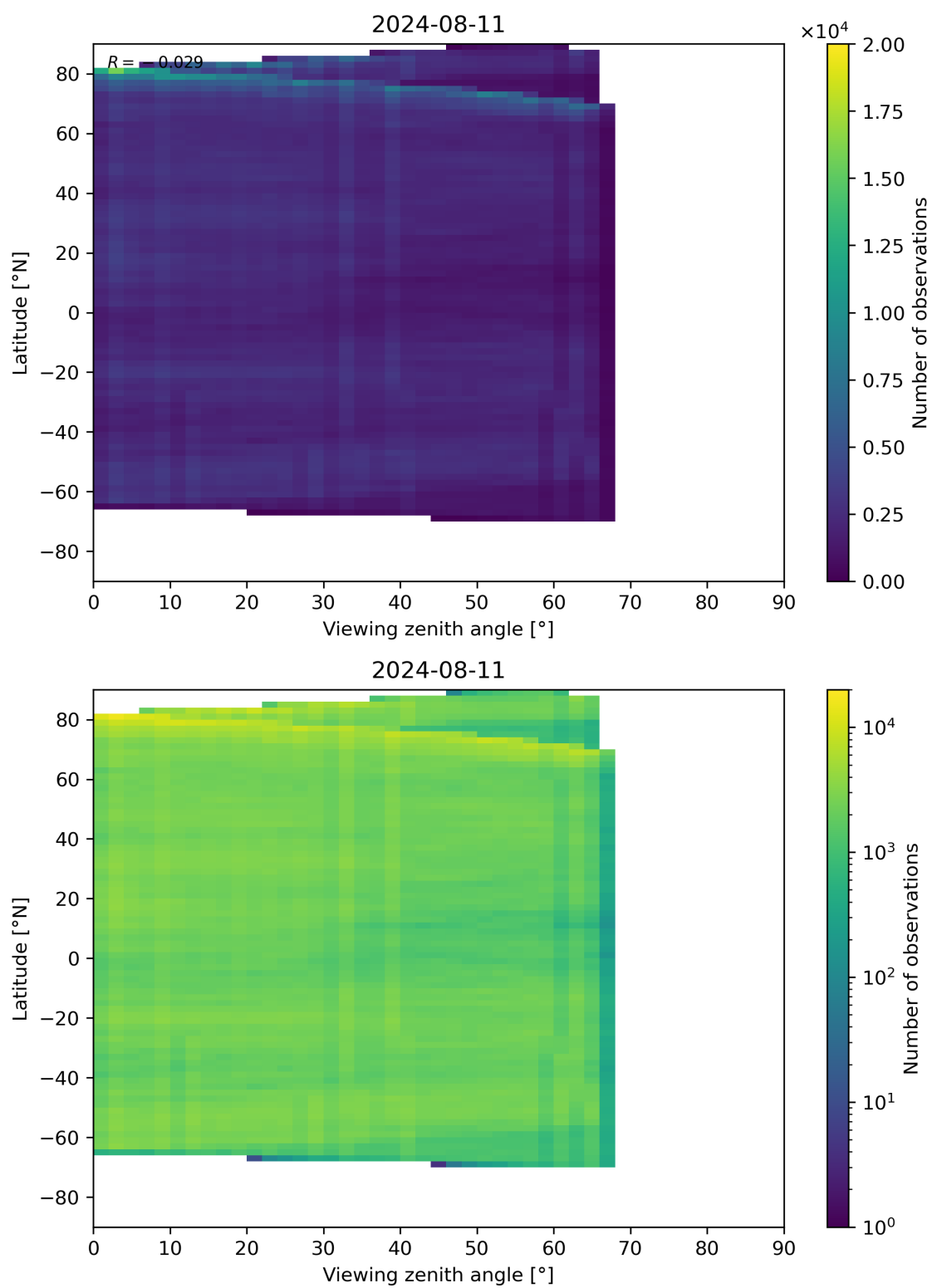
Figure 74: Scatter density plot of “Viewing zenith angle” against “Latitude” for 2024-08-11 to 2024-08-11.
