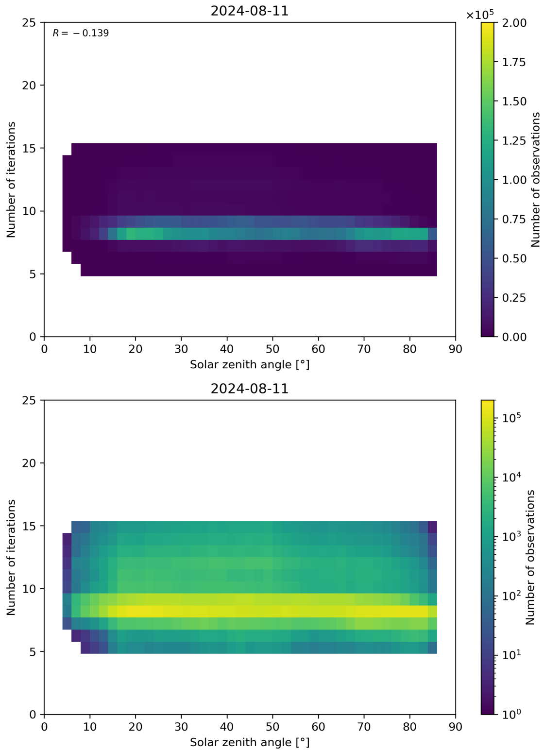
Figure 67: Scatter density plot of “Solar zenith angle” against “Number of iterations” for 2024-08-11 to 2024-08-11.
