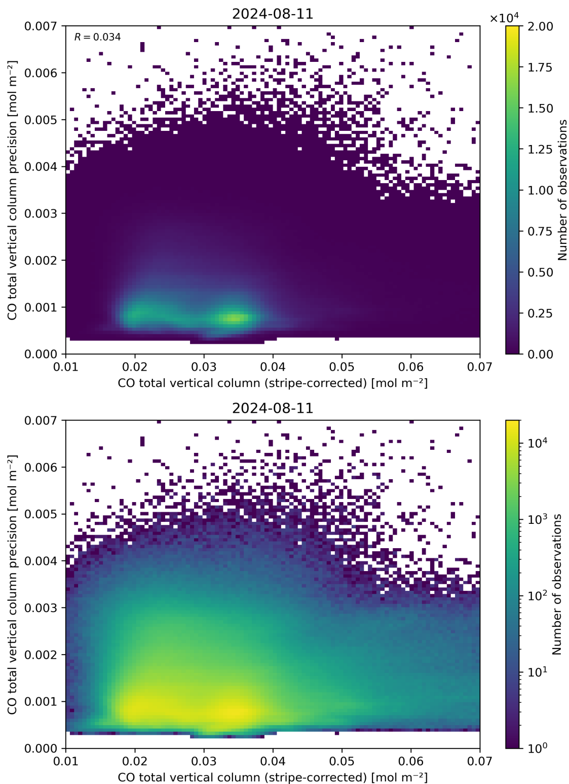
Figure 36: Scatter density plot of “CO total vertical column (stripe-corrected)” against “CO total vertical column precision” for 2024-08-11 to 2024-08-11.
