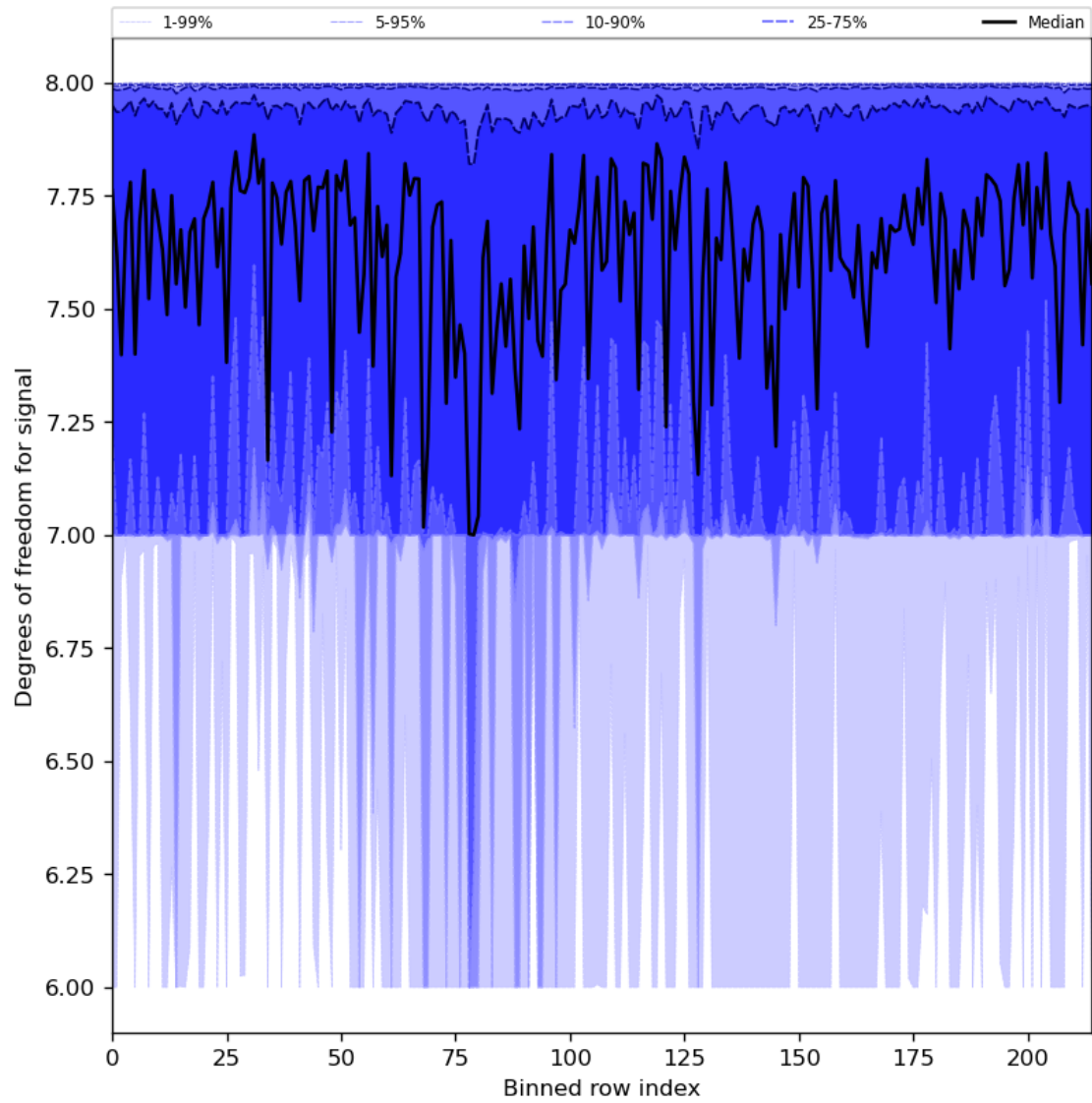
Figure 31: Along track statistics of “Degrees of freedom for signal” for 2024-08-11 to 2024-08-11
