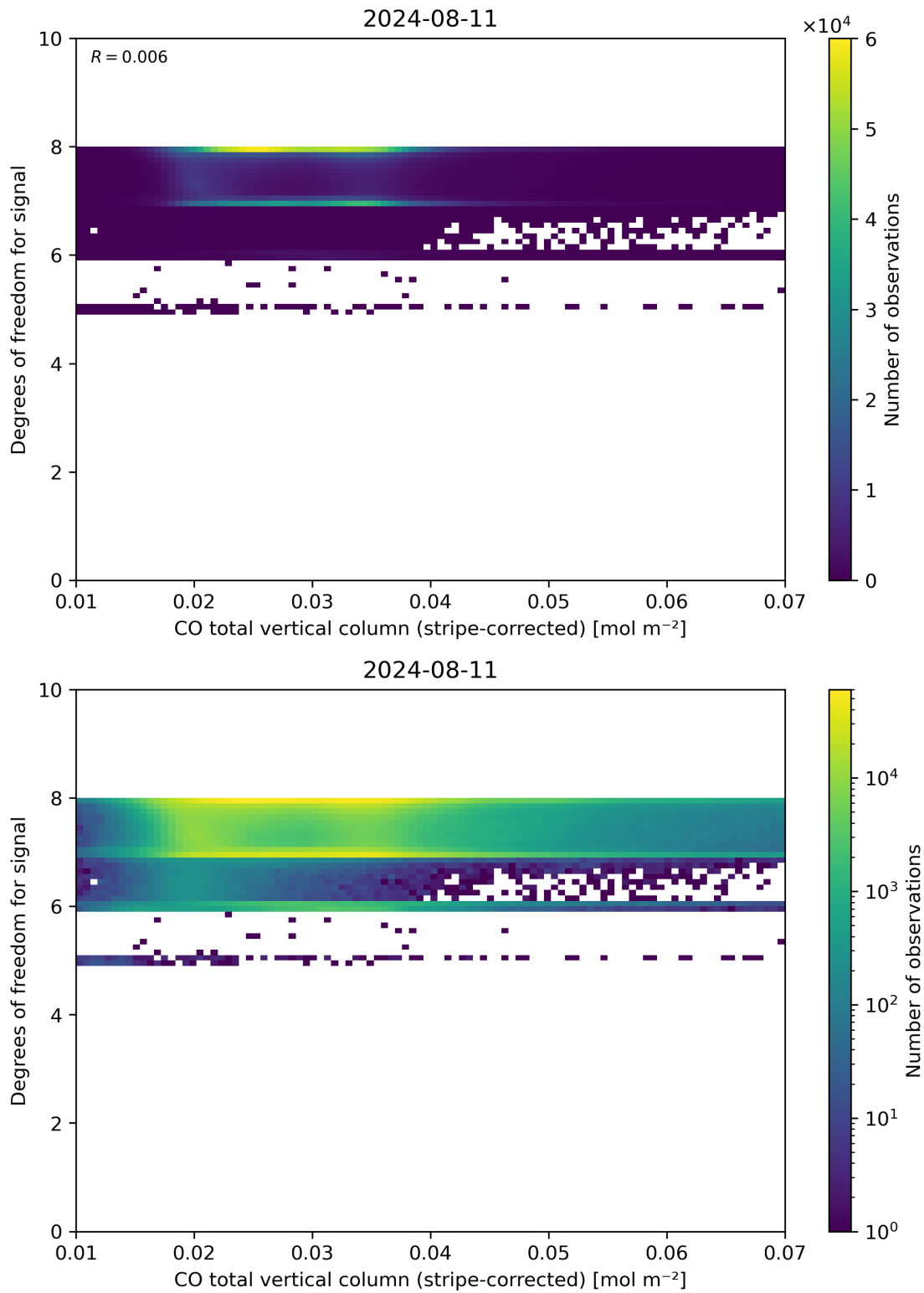
Figure 38: Scatter density plot of “CO total vertical column (stripe-corrected)” against “Degrees of freedom for signal” for 2024-08-11 to 2024-08-11.
