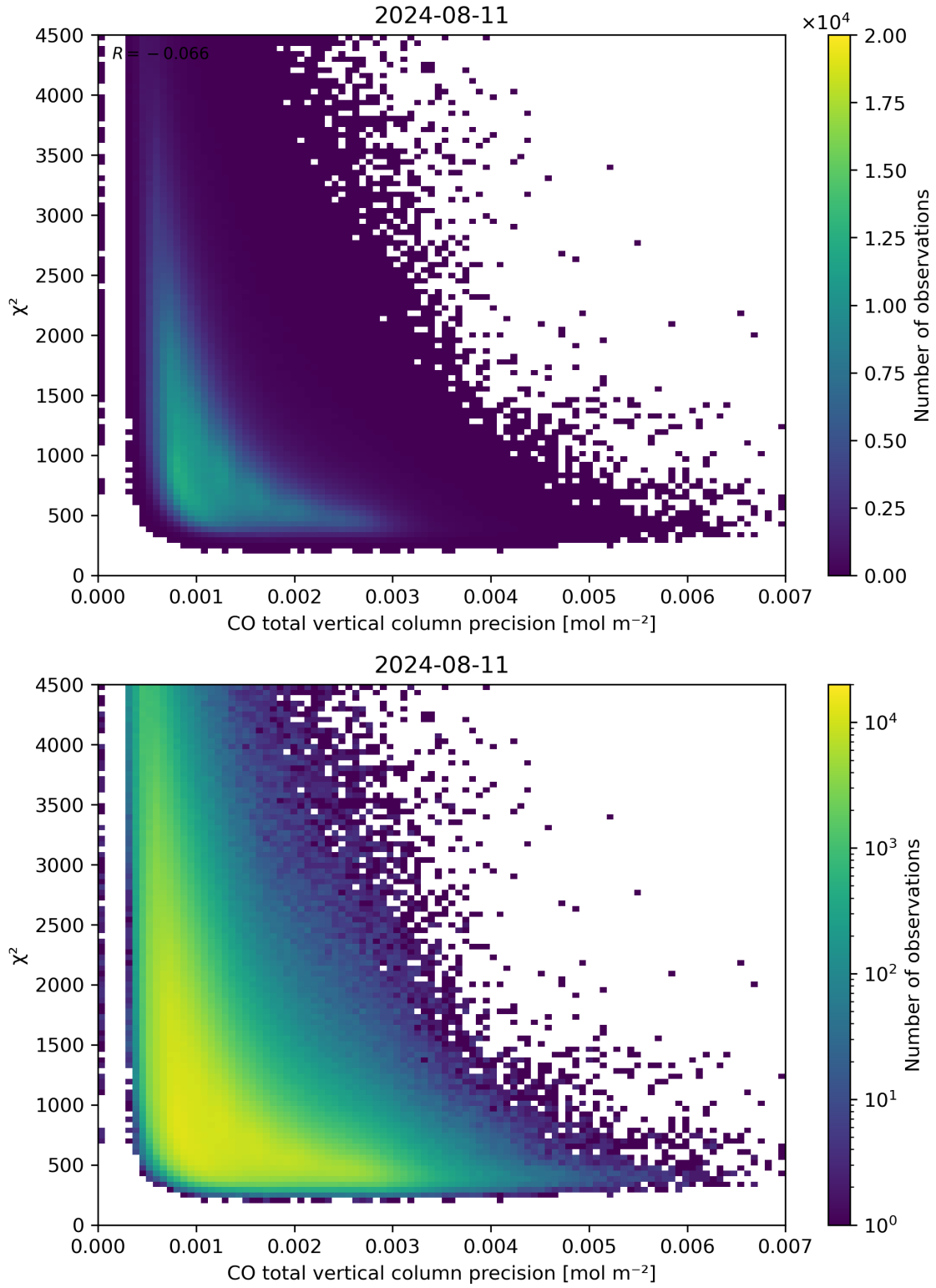
Figure 44: Scatter density plot of “CO total vertical column precision” against “ \chi^2 ” for 2024-08-11 to 2024-08-11.
