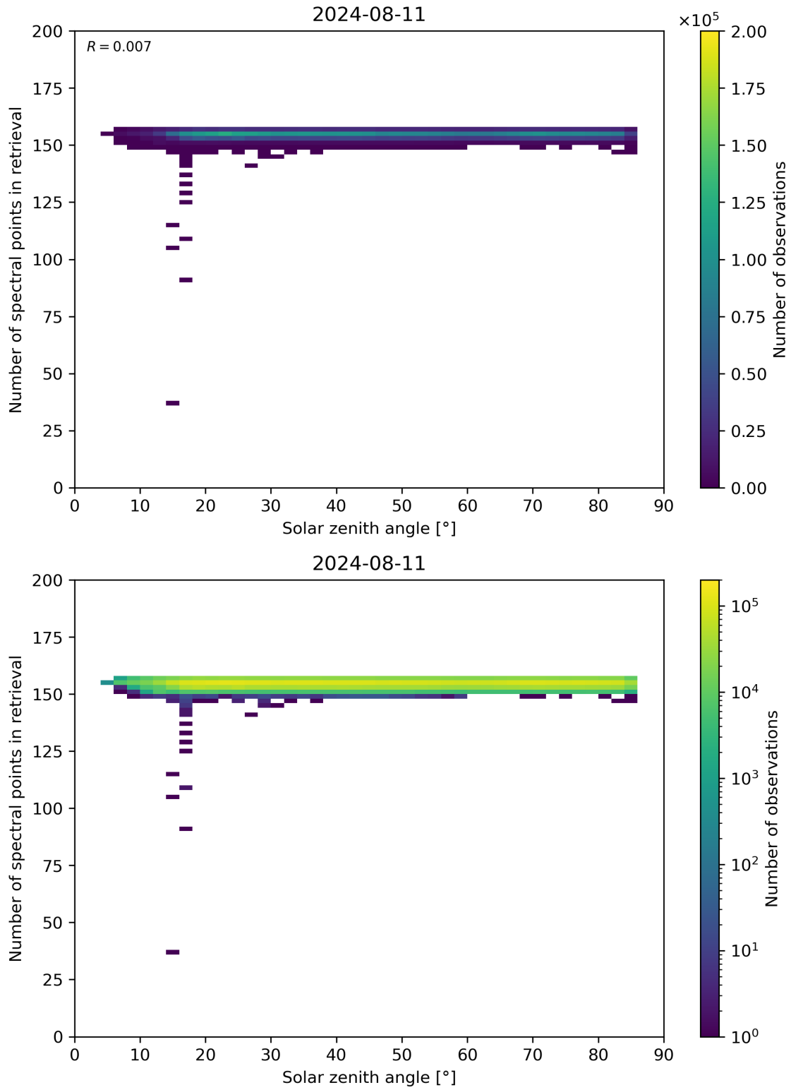
Figure 68: Scatter density plot of “Solar zenith angle” against “Number of spectral points in retrieval” for 2024-08-11 to 2024-08-11.
