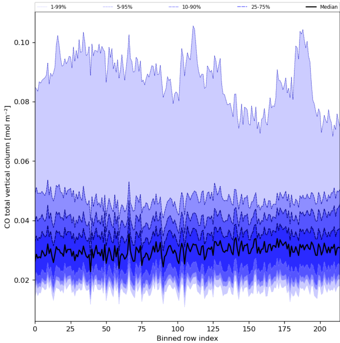
Figure 26: Along track statistics of “CO total vertical column” for 2024-08-11 to 2024-08-11
