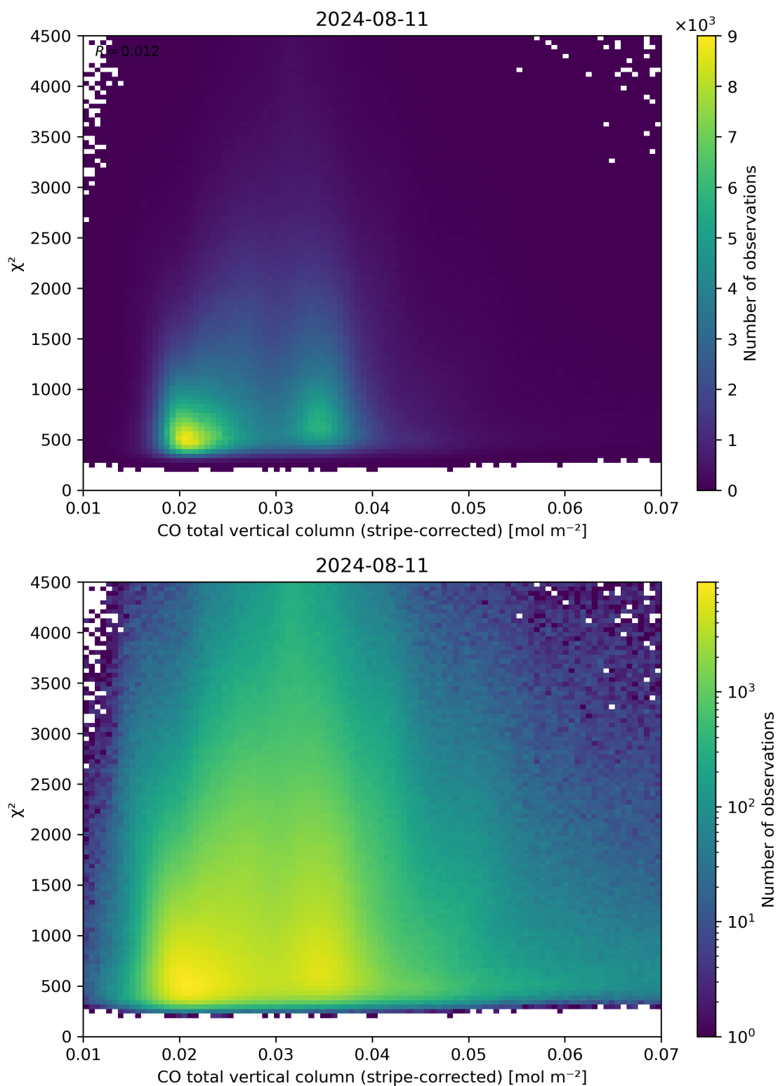
Figure 37: Scatter density plot of “CO total vertical column (stripe-corrected)” against “ \chi^2 ” for 2024-08-11 to 2024-08-11.
