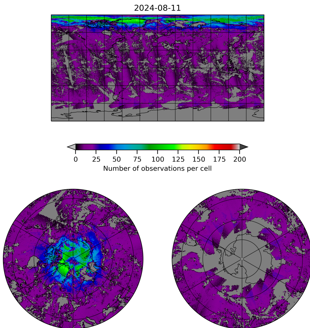
Figure 8: Map of the number of observations for 2024-08-11 to 2024-08-11
