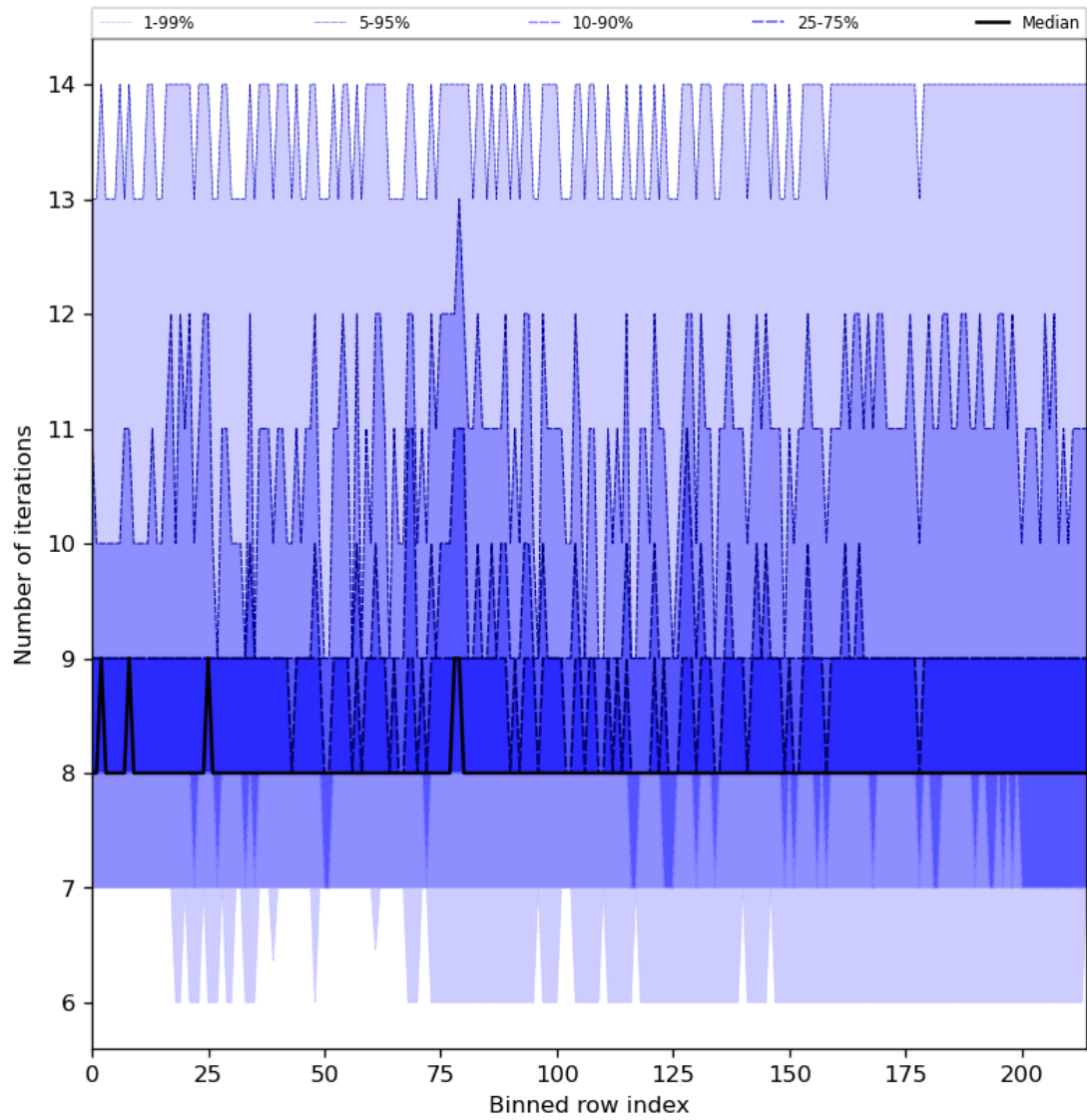
Figure 32: Along track statistics of “Number of iterations” for 2024-08-11 to 2024-08-11
