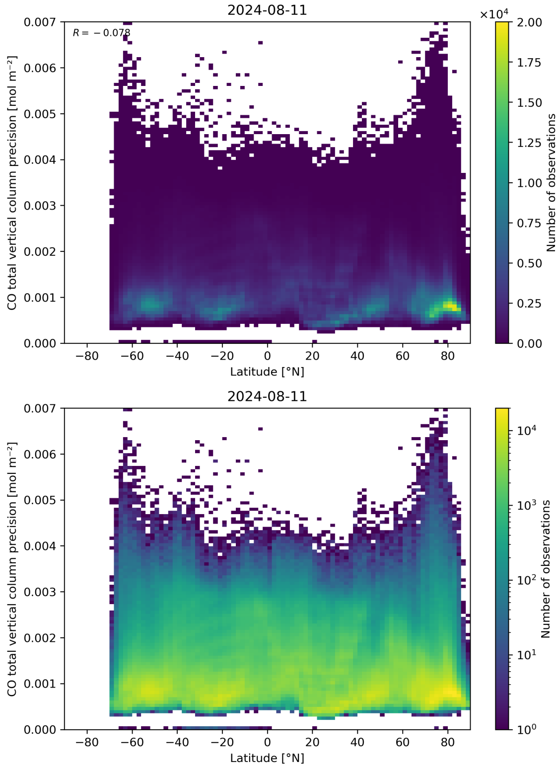
Figure 53: Scatter density plot of “Latitude” against “CO total vertical column precision” for 2024-08-11 to 2024-08-11.
