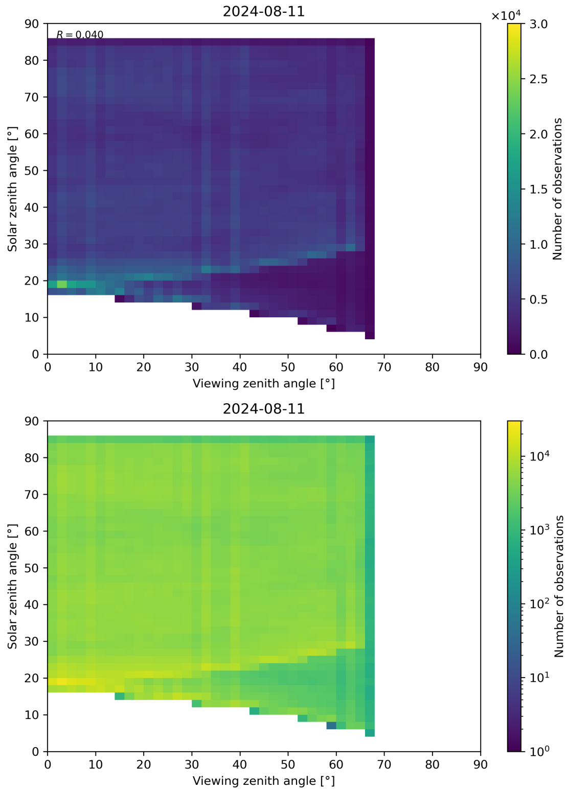
Figure 77: Scatter density plot of “Viewing zenith angle” against “Solar zenith angle” for 2024-08-11 to 2024-08-11.
