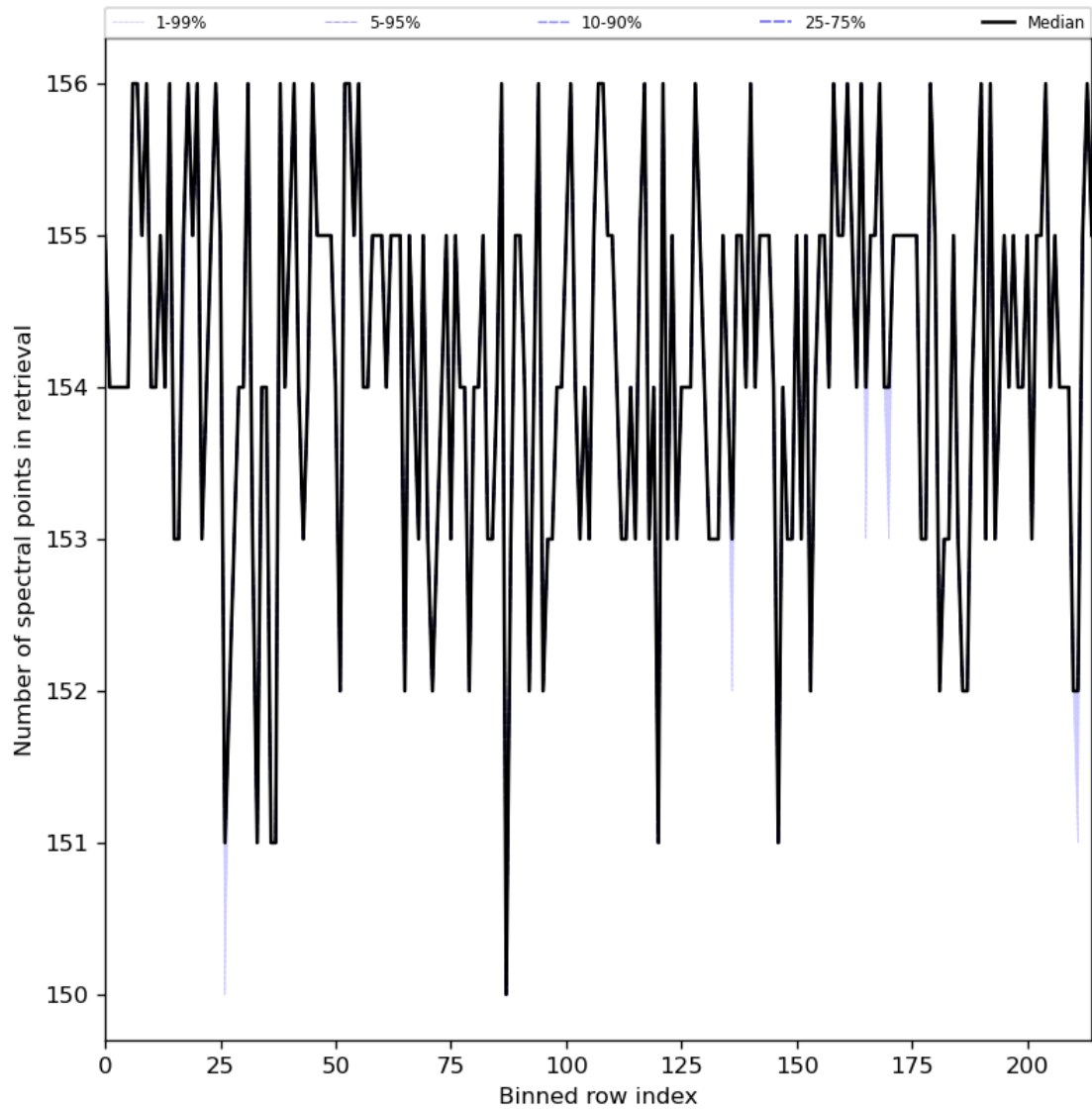
Figure 29: Along track statistics of “Number of spectral points in retrieval” for 2024-08-11 to 2024-08-11
