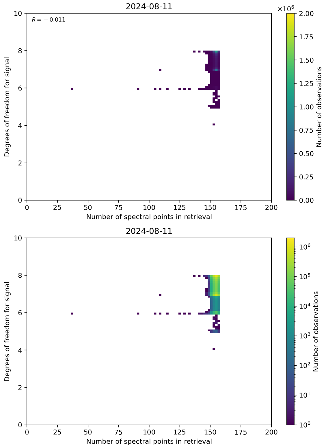
Figure 59: Scatter density plot of “Number of spectral points in retrieval” against “Degrees of freedom for signal” for 2024-08-11 to 2024-08-11.
