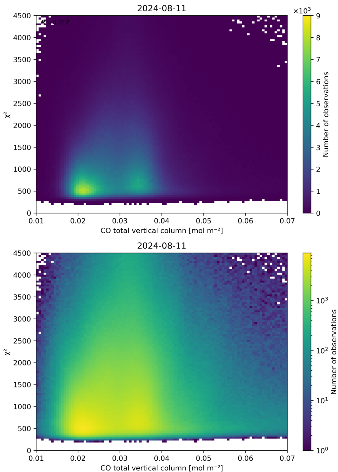
Figure 35: Scatter density plot of “CO total vertical column” against “ \chi^2 ” for 2024-08-11 to 2024-08-11.
