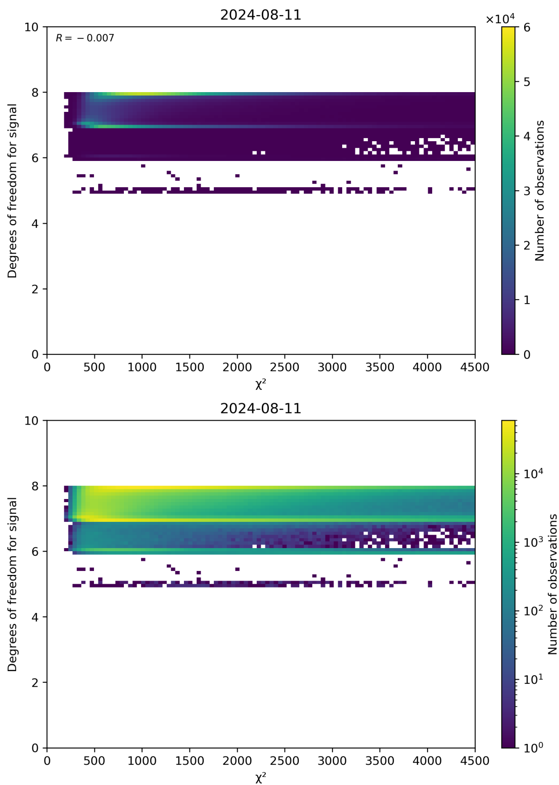
Figure 48: Scatter density plot of “ \chi^2 ” against “Degrees of freedom for signal” for 2024-08-11 to 2024-08-11.
