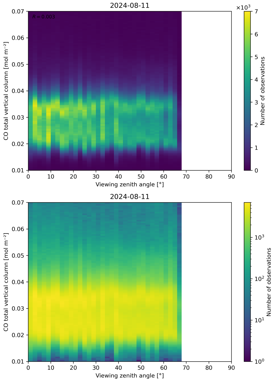
Figure 69: Scatter density plot of “Viewing zenith angle” against “CO total vertical column” for 2024-08-11 to 2024-08-11.
