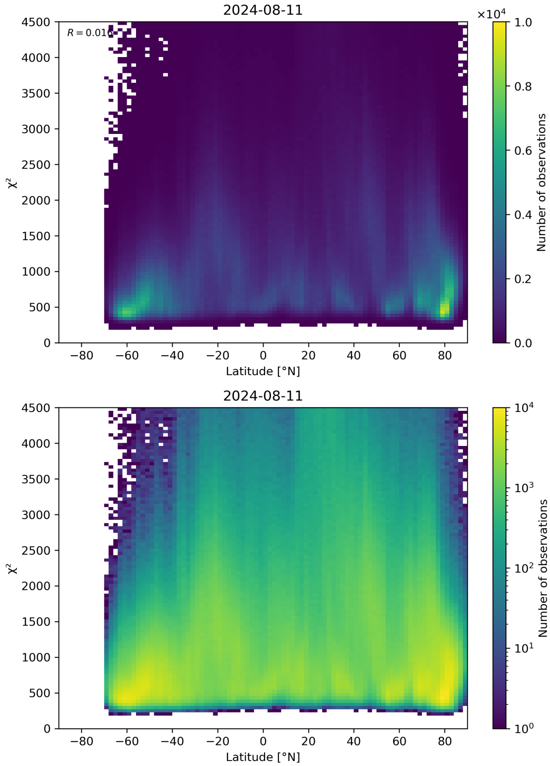
Figure 54: Scatter density plot of “Latitude” against “ \chi^2 ” for 2024-08-11 to 2024-08-11.
