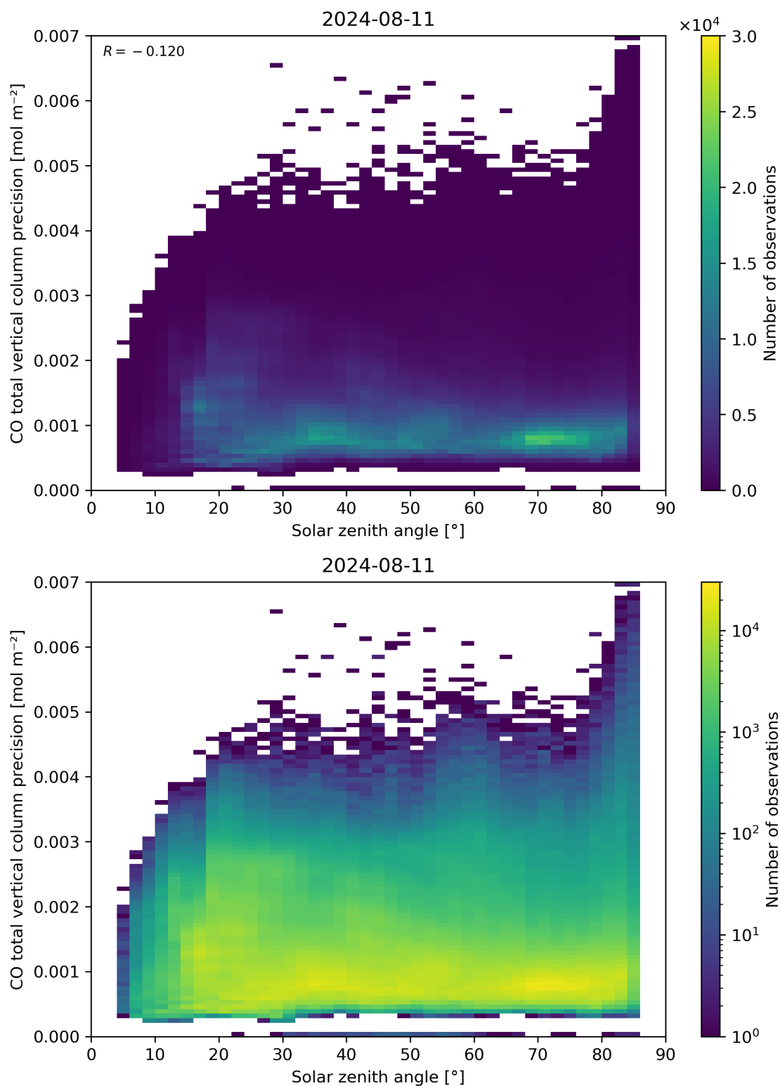
Figure 63: Scatter density plot of “Solar zenith angle” against “CO total vertical column precision” for 2024-08-11 to 2024-08-11.
