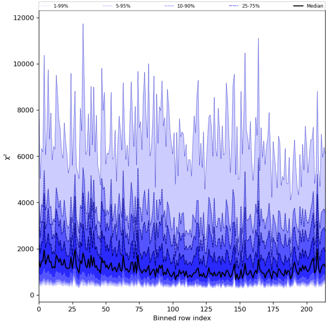
Figure 30: Along track statistics of “ \chi^2 ” for 2024-08-11 to 2024-08-11
