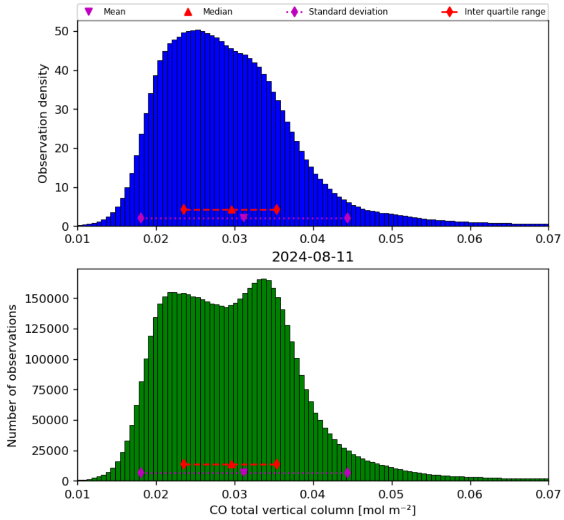
Figure 18: Histogram of “CO total vertical column” for 2024-08-11 to 2024-08-11
