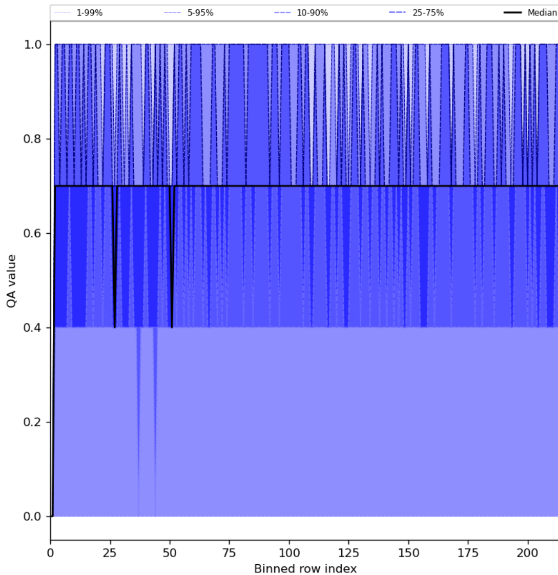
Figure 25: Along track statistics of “QA value” for 2024-08-11 to 2024-08-11
