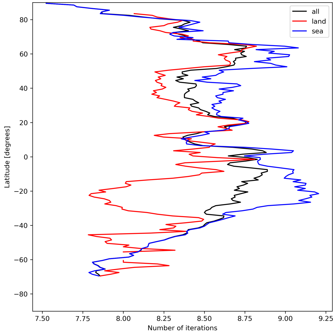
Figure 16: Zonal average of “Number of iterations” for 2024-08-11 to 2024-08-11.
