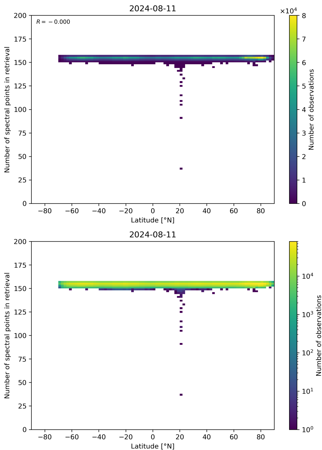
Figure 57: Scatter density plot of “Latitude” against “Number of spectral points in retrieval” for 2024-08-11 to 2024-08-11.
