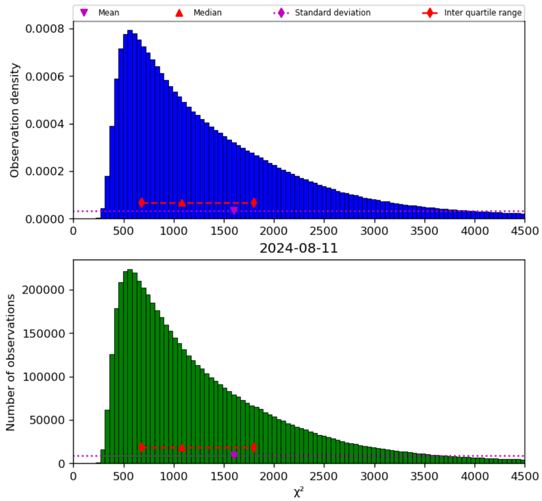
Figure 22: Histogram of “ \chi^2 ” for 2024-08-11 to 2024-08-11
