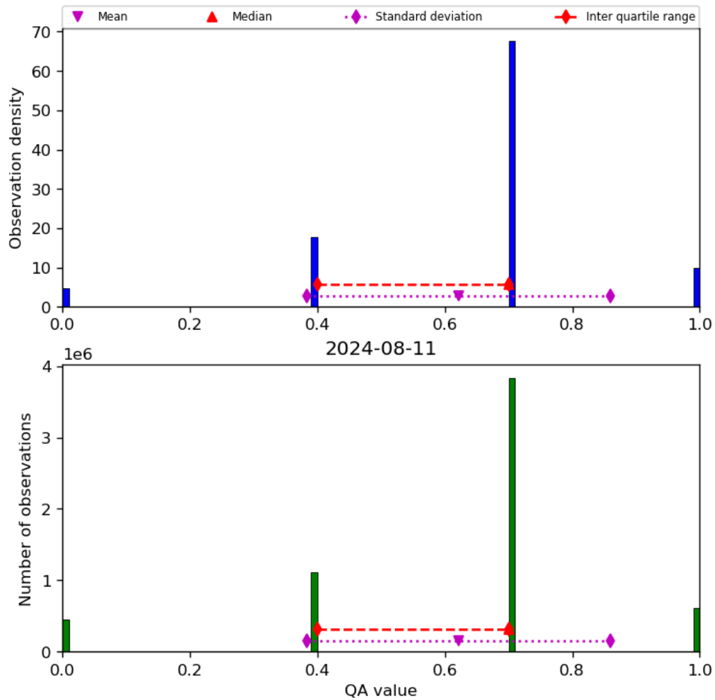
Figure 17: Histogram of “QA value” for 2024-08-11 to 2024-08-11
