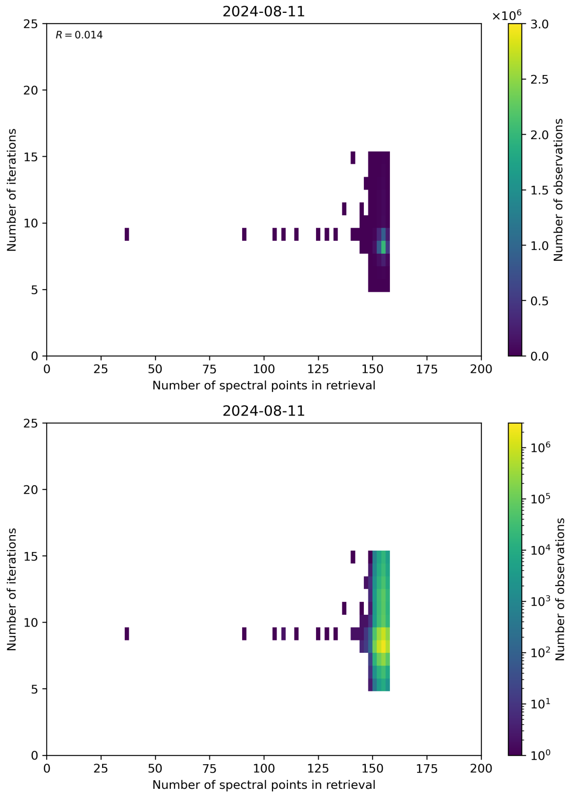
Figure 60: Scatter density plot of “Number of spectral points in retrieval” against “Number of iterations” for 2024-08-11 to 2024-08-11.
