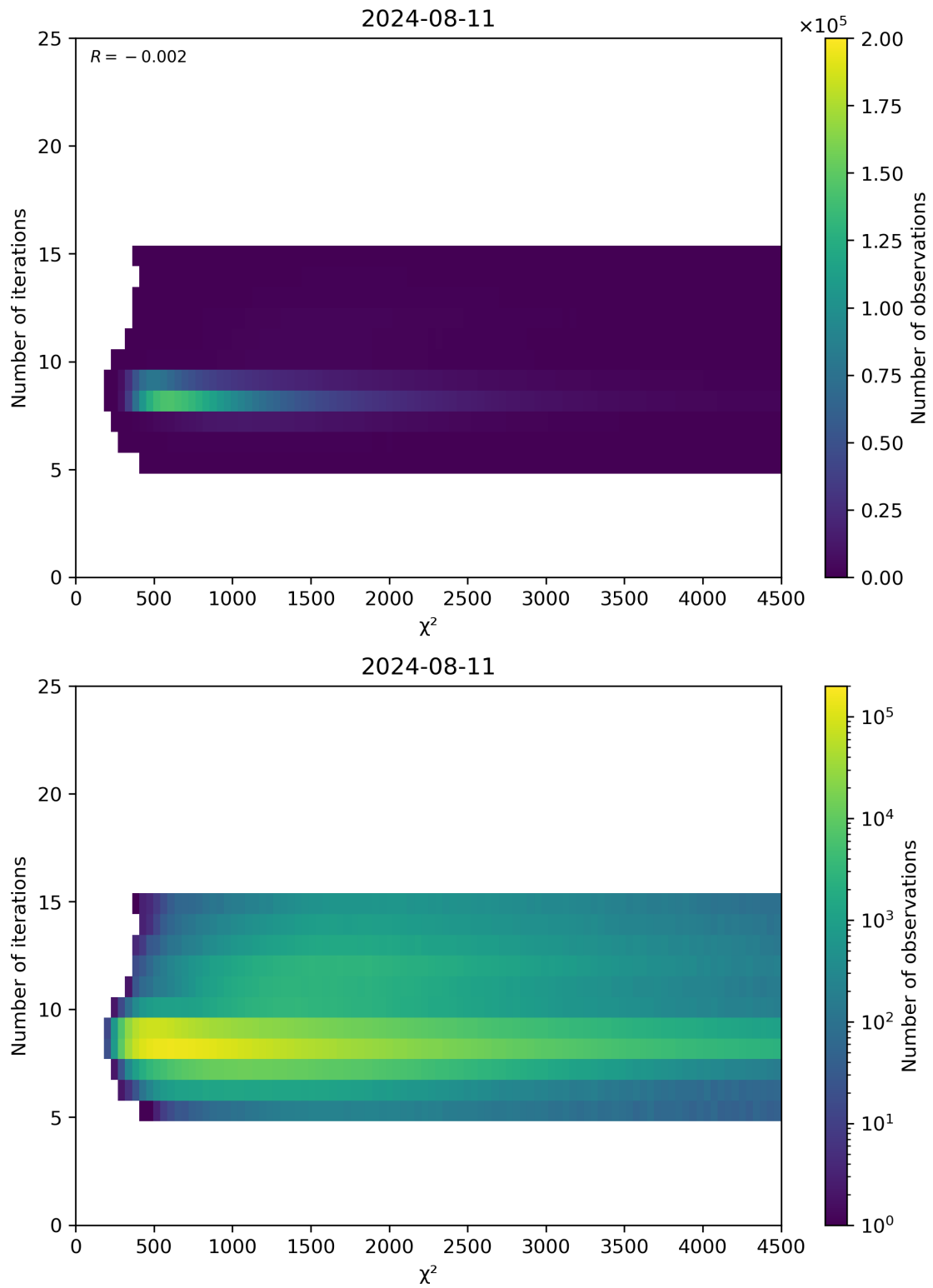
Figure 49: Scatter density plot of “ \chi^2 ” against “Number of iterations” for 2024-08-11 to 2024-08-11.
