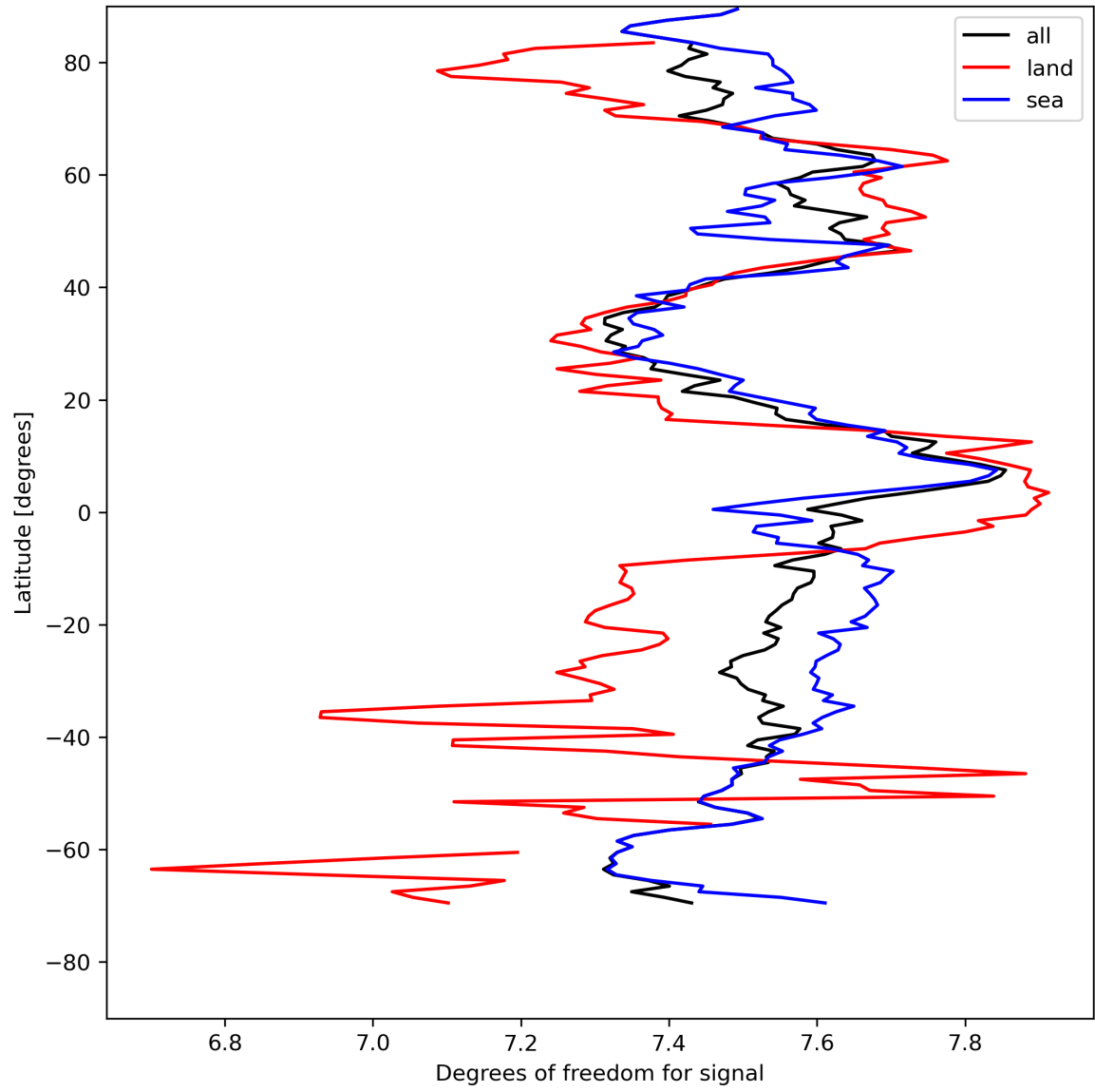
Figure 15: Zonal average of “Degrees of freedom for signal” for 2024-08-11 to 2024-08-11.
