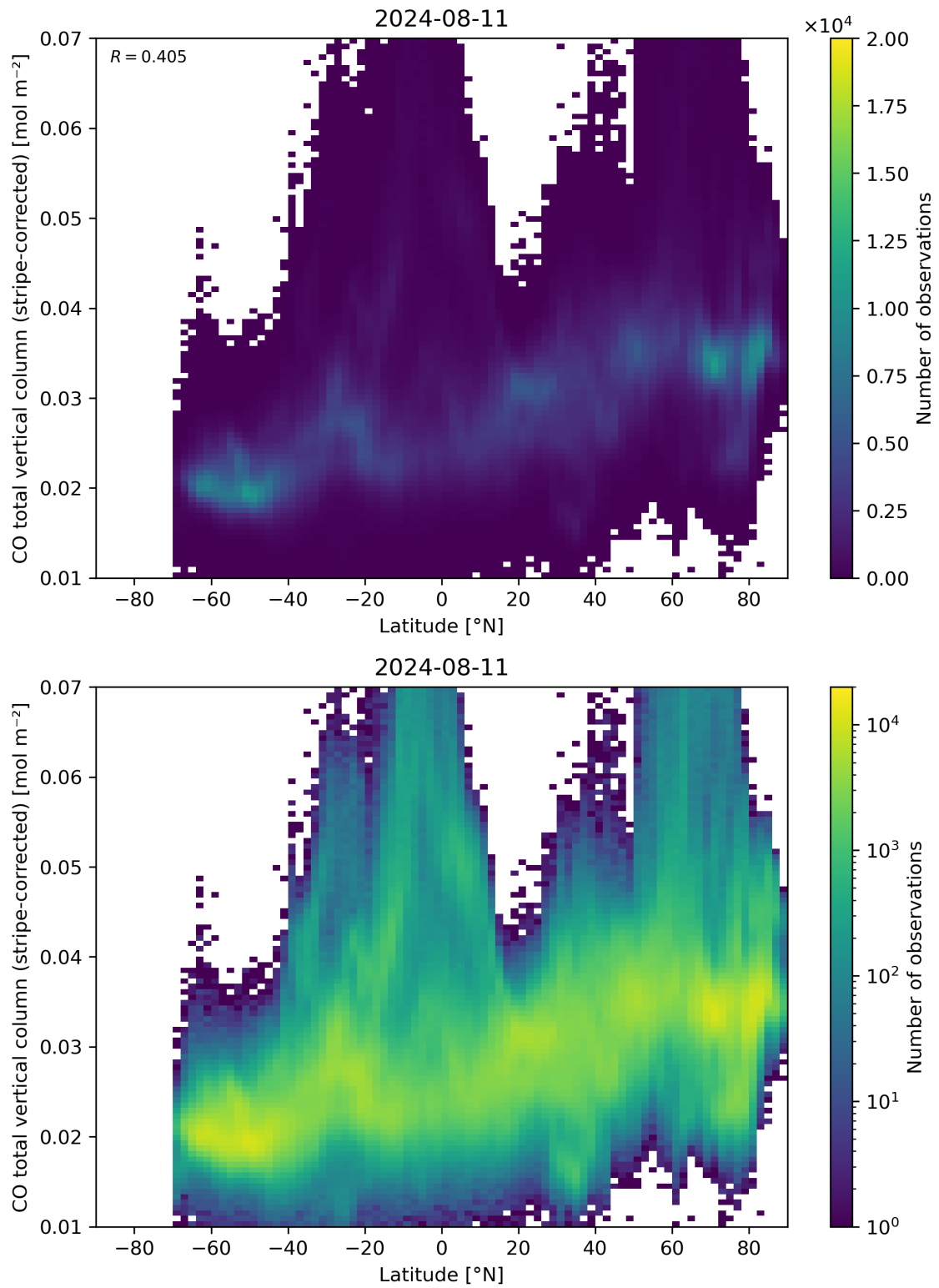
Figure 52: Scatter density plot of “Latitude” against “CO total vertical column (stripe-corrected)” for 2024-08-11 to 2024-08-11.
