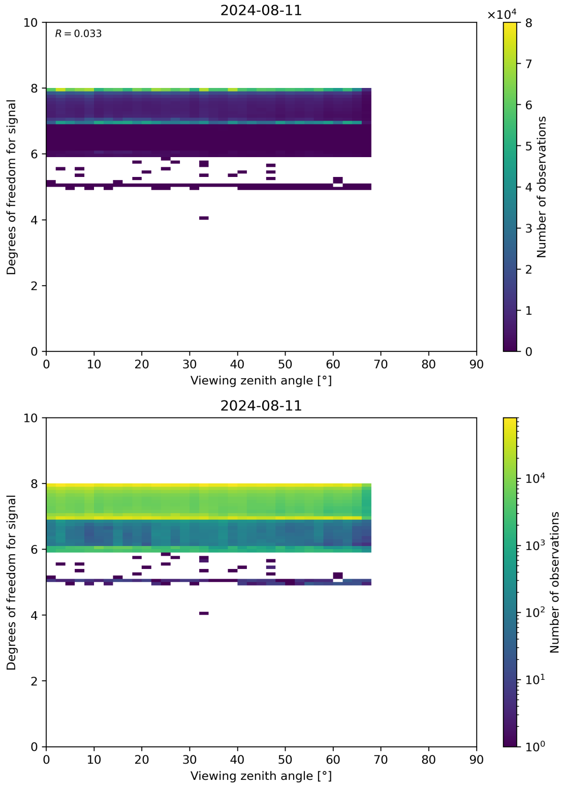
Figure 73: Scatter density plot of “Viewing zenith angle” against “Degrees of freedom for signal” for 2024-08-11 to 2024-08-11.
