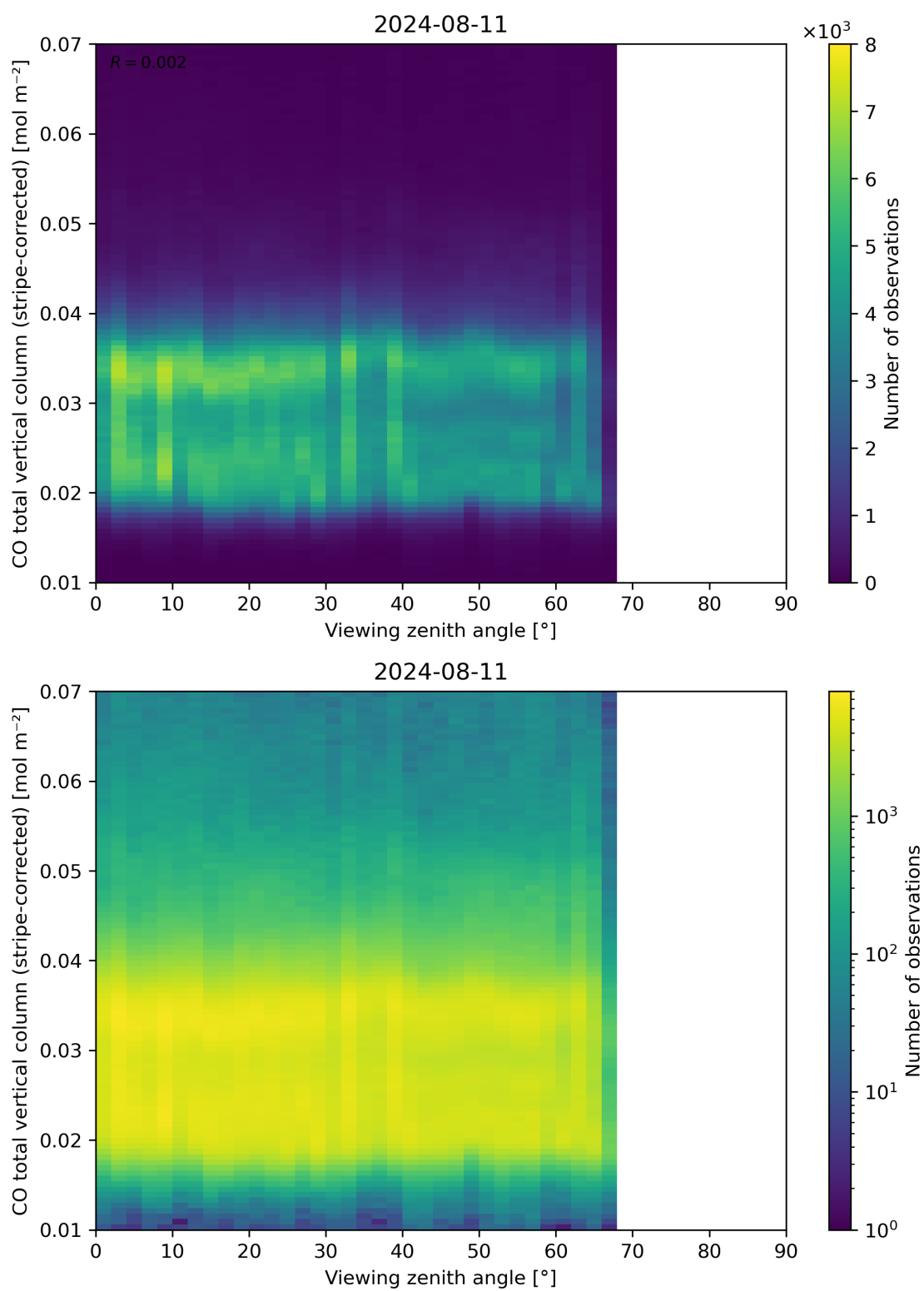
Figure 70: Scatter density plot of “Viewing zenith angle” against “CO total vertical column (stripe-corrected)” for 2024-08-11 to 2024-08-11.
