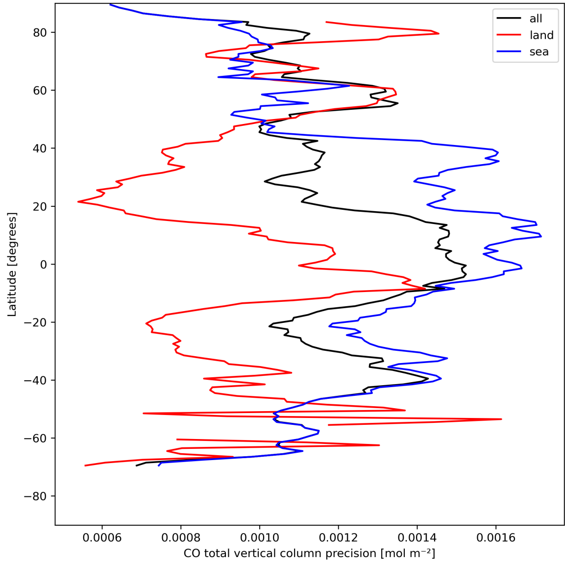
Figure 12: Zonal average of "CO total vertical column precision" for 2024-08-11 to 2024-08-11.
