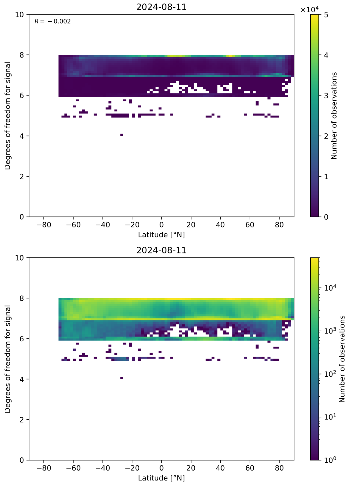
Figure 55: Scatter density plot of “Latitude” against “Degrees of freedom for signal” for 2024-08-11 to 2024-08-11.
