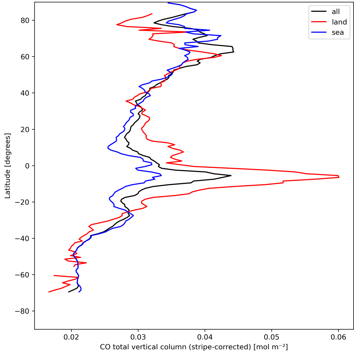
Figure 11: Zonal average of “CO total vertical column (stripe-corrected)” for 2024-08-11 to 2024-08-11.
