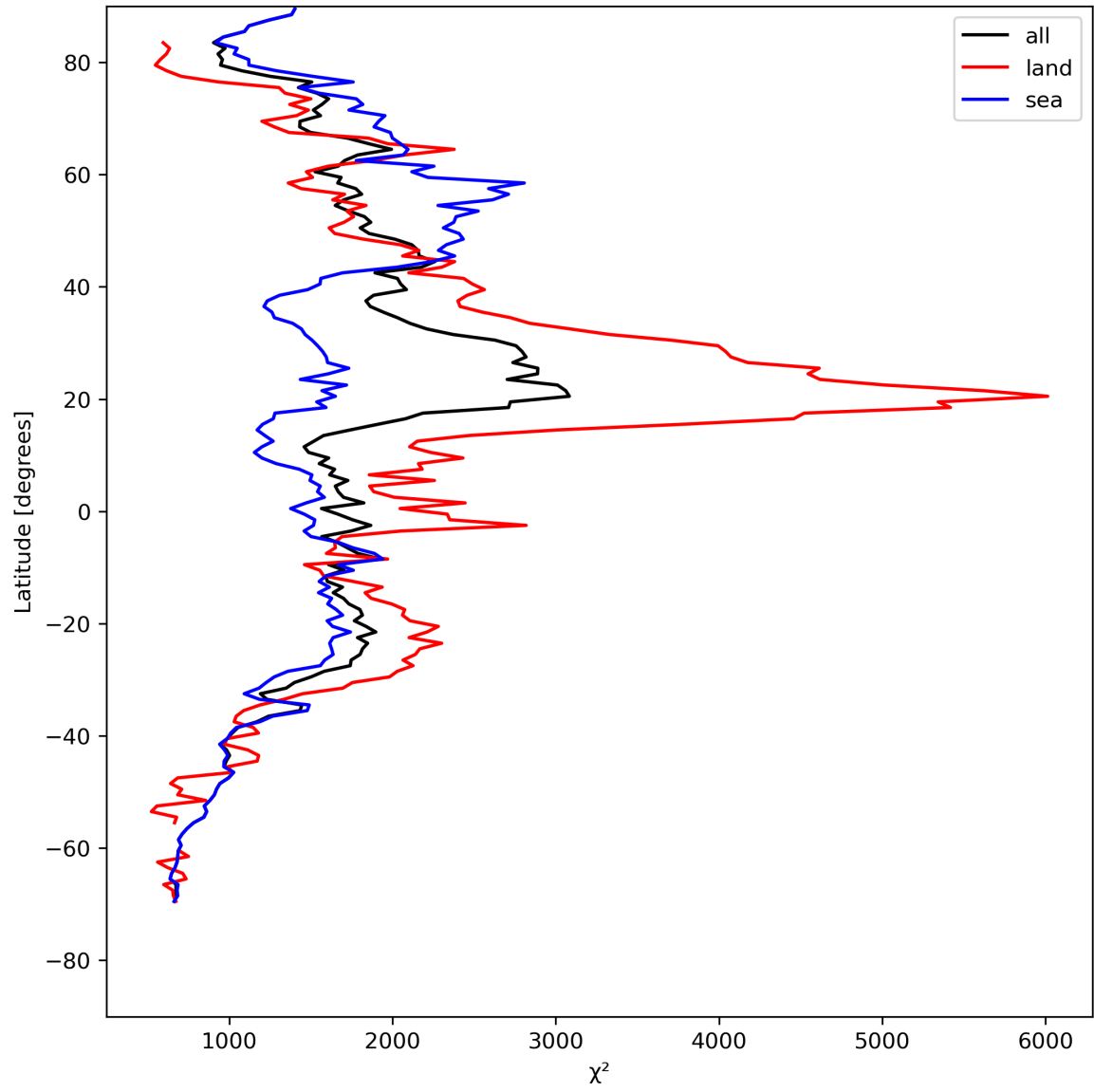
Figure 14: Zonal average of “ \chi^2 ” for 2024-08-11 to 2024-08-11.
