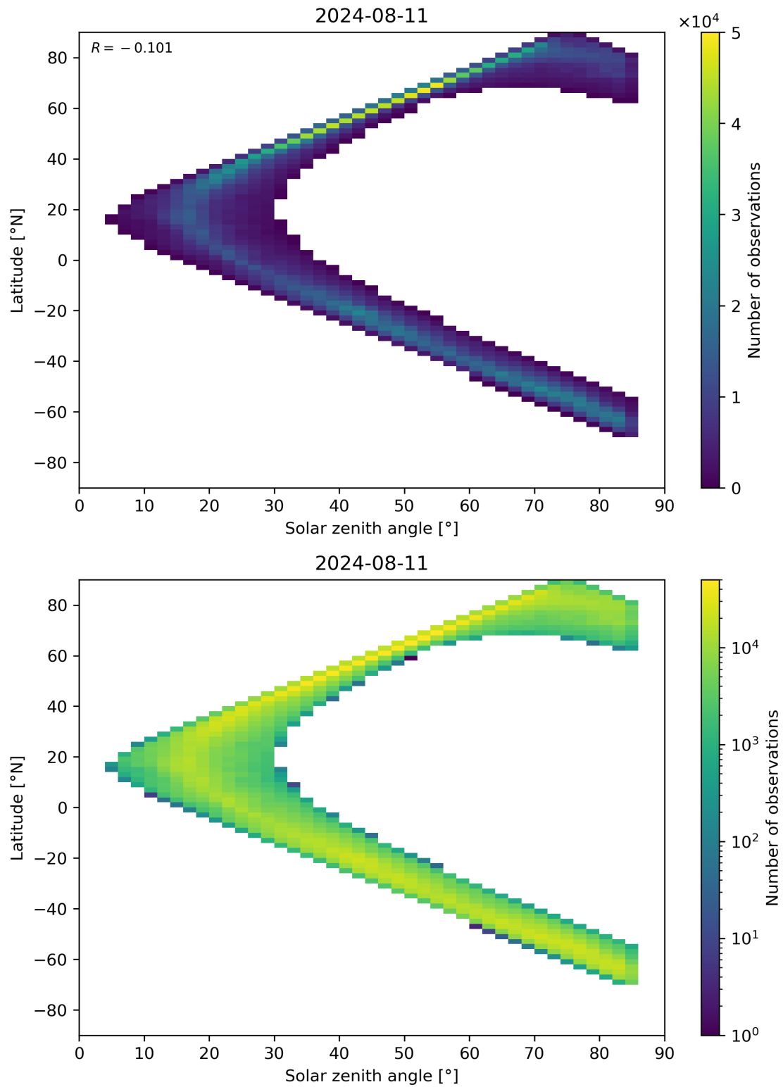
Figure 66: Scatter density plot of “Solar zenith angle” against “Latitude” for 2024-08-11 to 2024-08-11.
