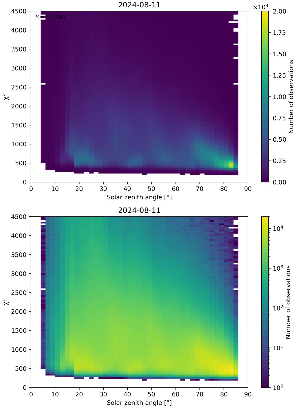
Figure 64: Scatter density plot of “Solar zenith angle” against “ \chi^2 ” for 2024-08-11 to 2024-08-11.
