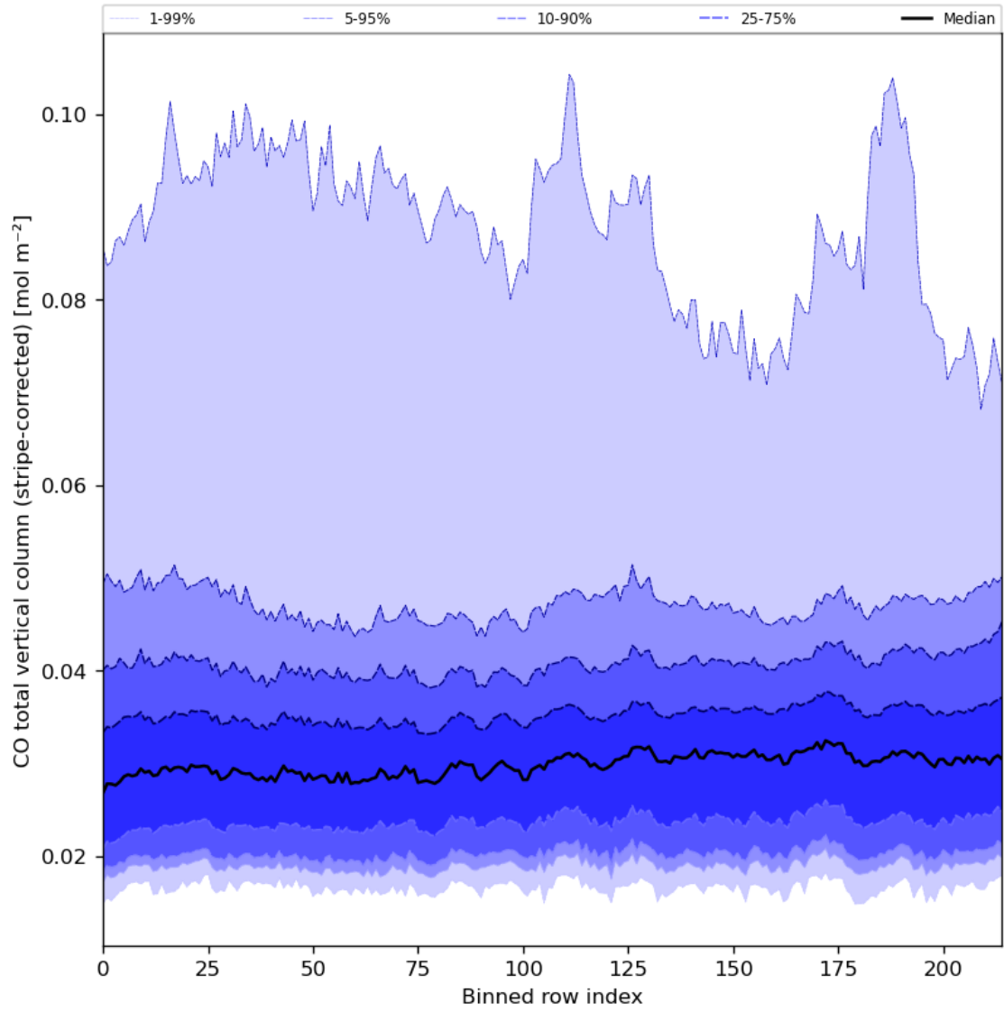
Figure 27: Along track statistics of “CO total vertical column (stripe-corrected)” for 2024-08-11 to 2024-08-11
