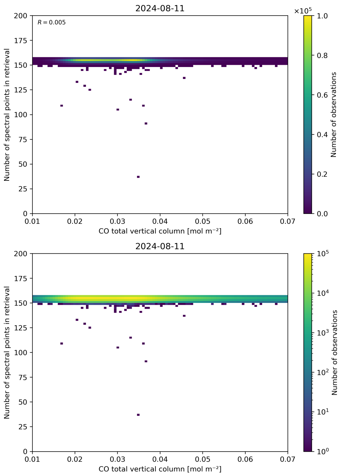
Figure 43: Scatter density plot of “CO total vertical column” against “Number of spectral points in retrieval” for 2024-08-11 to 2024-08-11.
