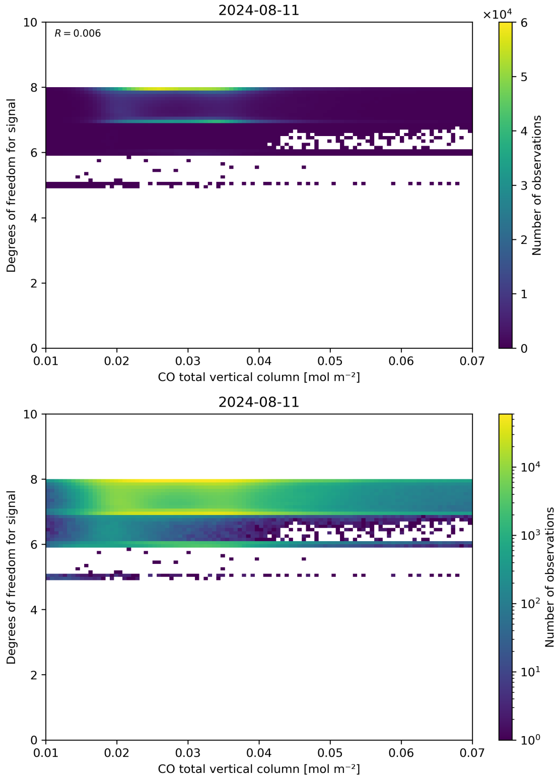
Figure 41: Scatter density plot of “CO total vertical column” against “Degrees of freedom for signal” for 2024-08-11 to 2024-08-11.
