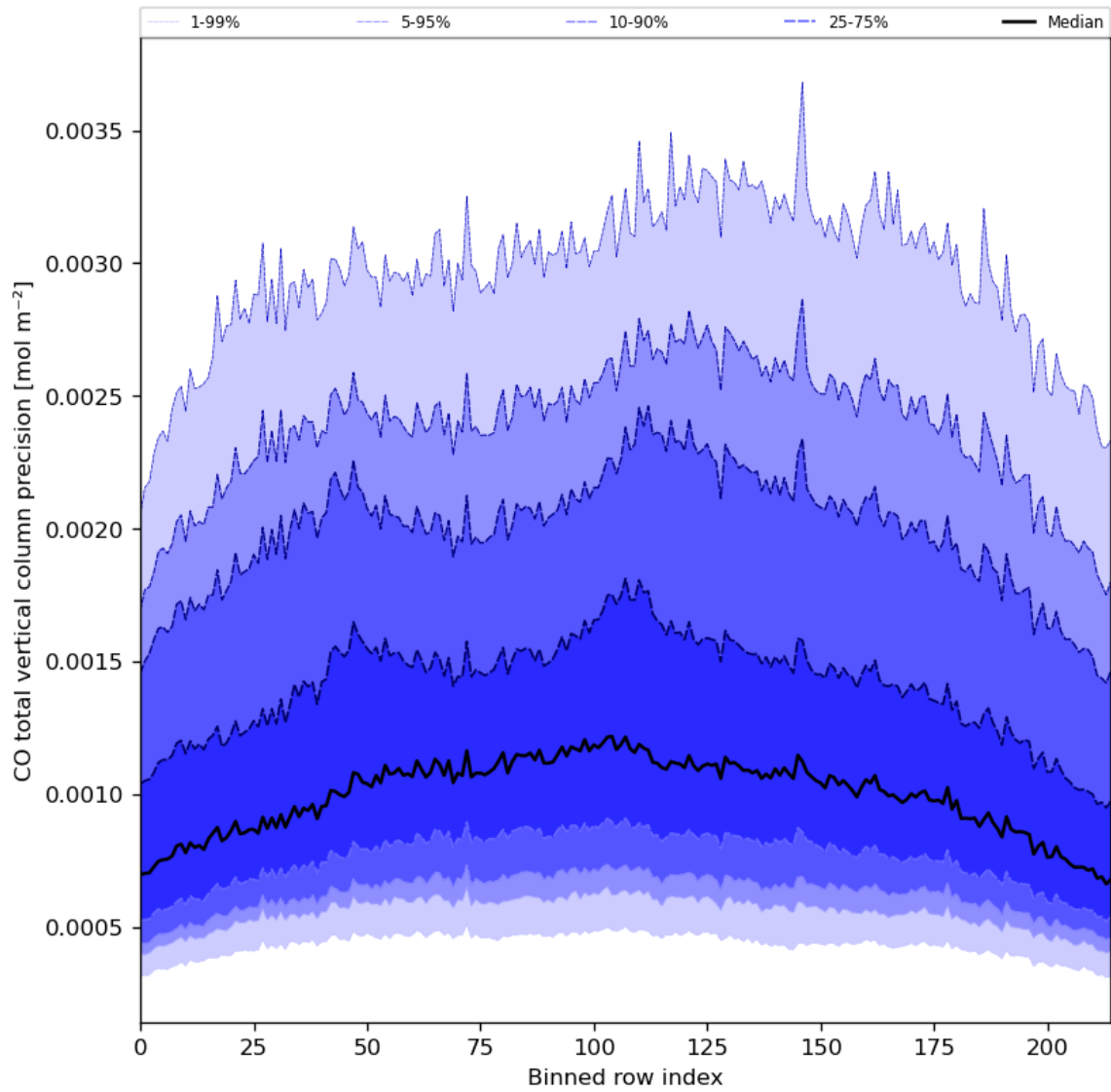
Figure 28: Along track statistics of “CO total vertical column precision” for 2024-08-11 to 2024-08-11
