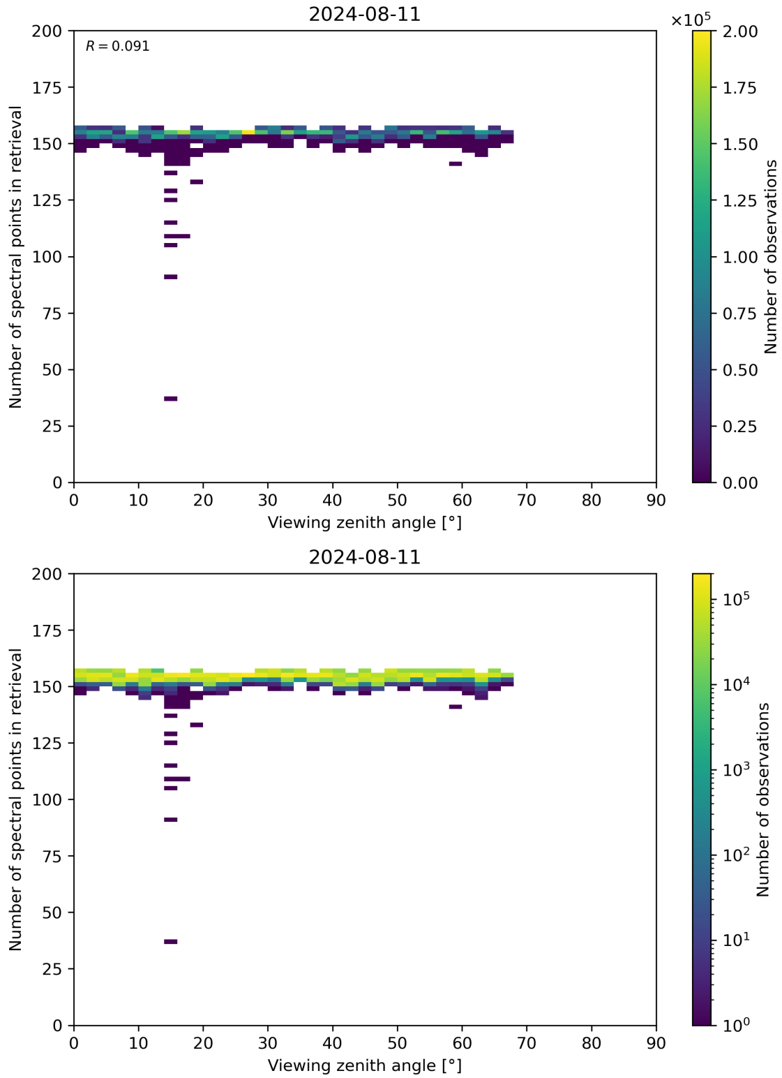
Figure 76: Scatter density plot of “Viewing zenith angle” against “Number of spectral points in retrieval” for 2024-08-11 to 2024-08-11.
