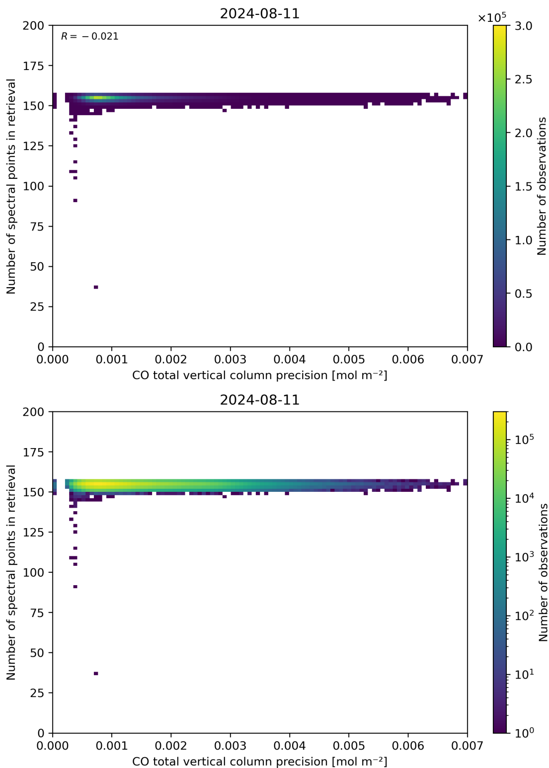
Figure 47: Scatter density plot of “CO total vertical column precision” against “Number of spectral points in retrieval” for 2024-08-11 to 2024-08-11.
