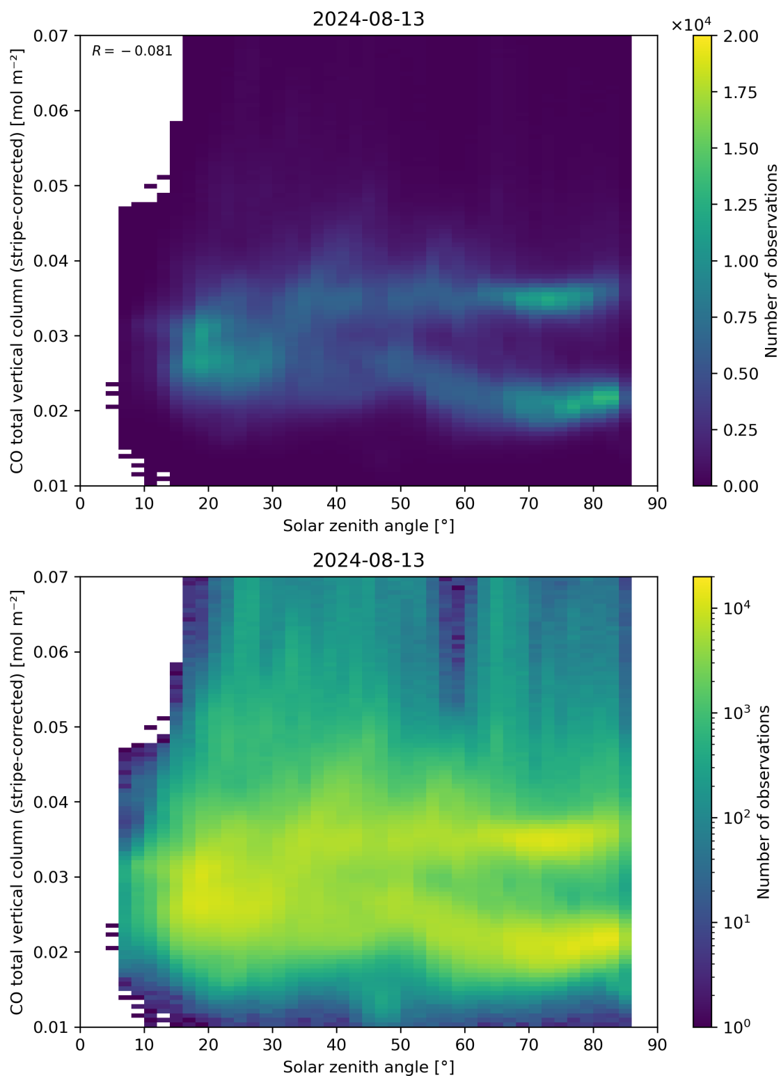
Figure 62: Scatter density plot of “Solar zenith angle” against “CO total vertical column (stripe-corrected)” for 2024-08-12 to 2024-08-14.
