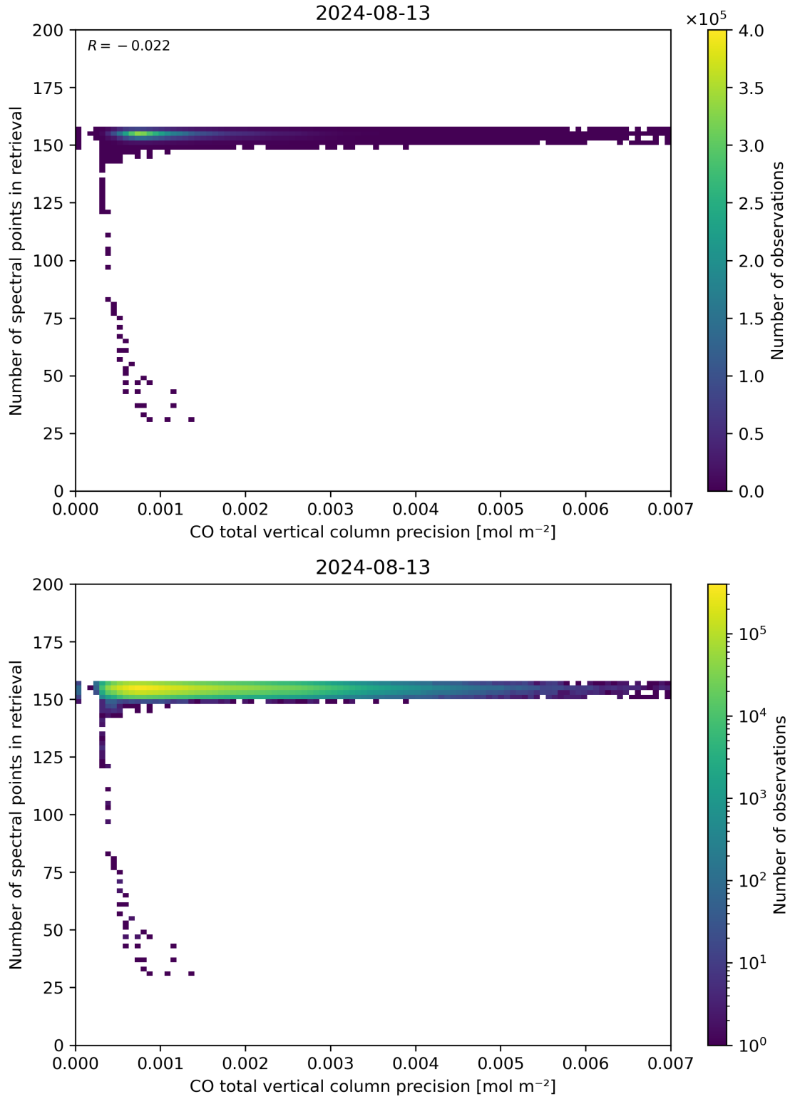
Figure 47: Scatter density plot of “CO total vertical column precision” against “Number of spectral points in retrieval” for 2024-08-12 to 2024-08-14.
