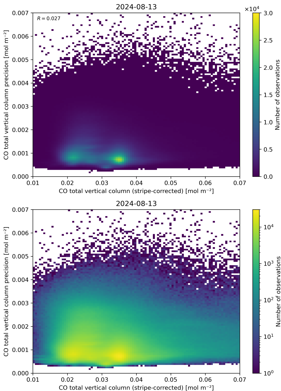
Figure 36: Scatter density plot of “CO total vertical column (stripe-corrected)” against “CO total vertical column precision” for 2024-08-12 to 2024-08-14.
