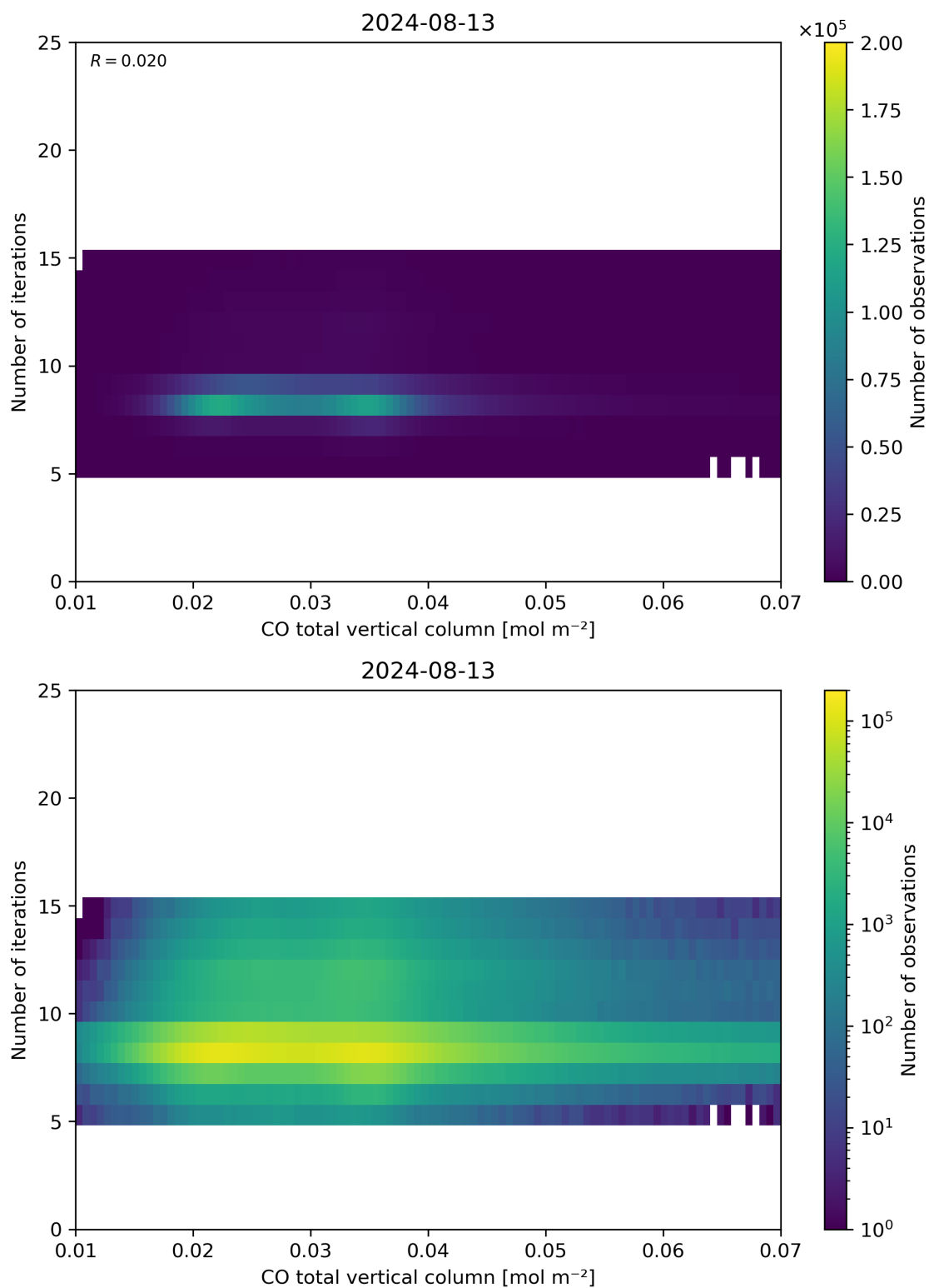
Figure 42: Scatter density plot of “CO total vertical column” against “Number of iterations” for 2024-08-12 to 2024-08-14.
