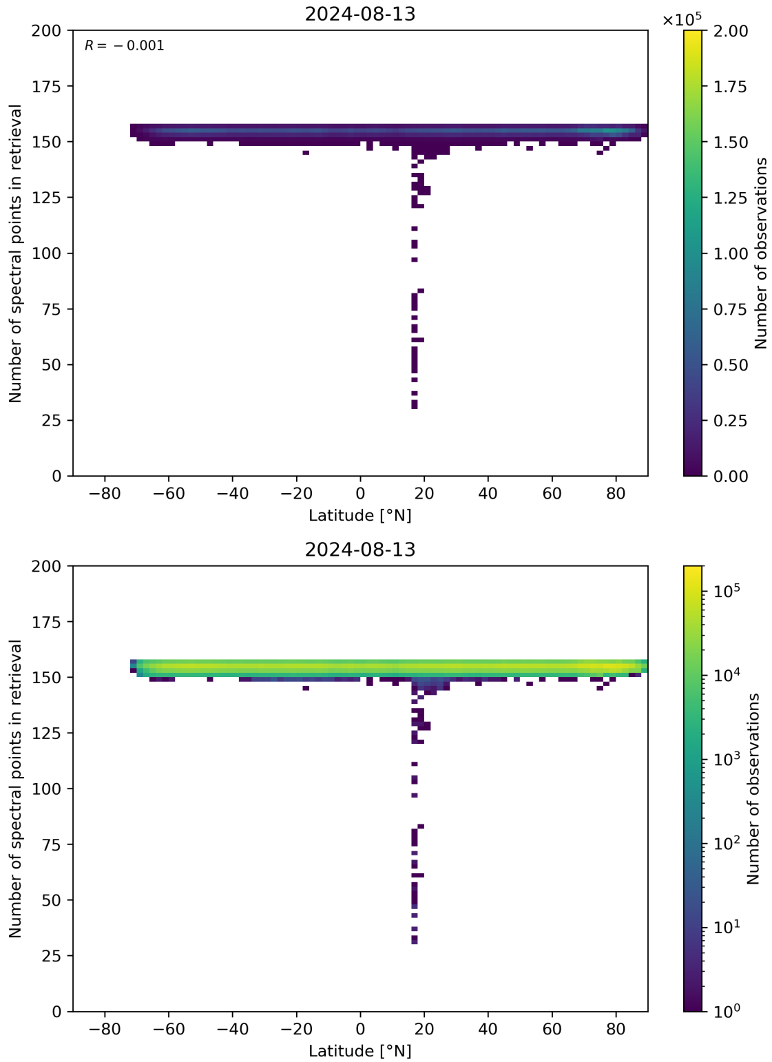
Figure 57: Scatter density plot of “Latitude” against “Number of spectral points in retrieval” for 2024-08-12 to 2024-08-14.
