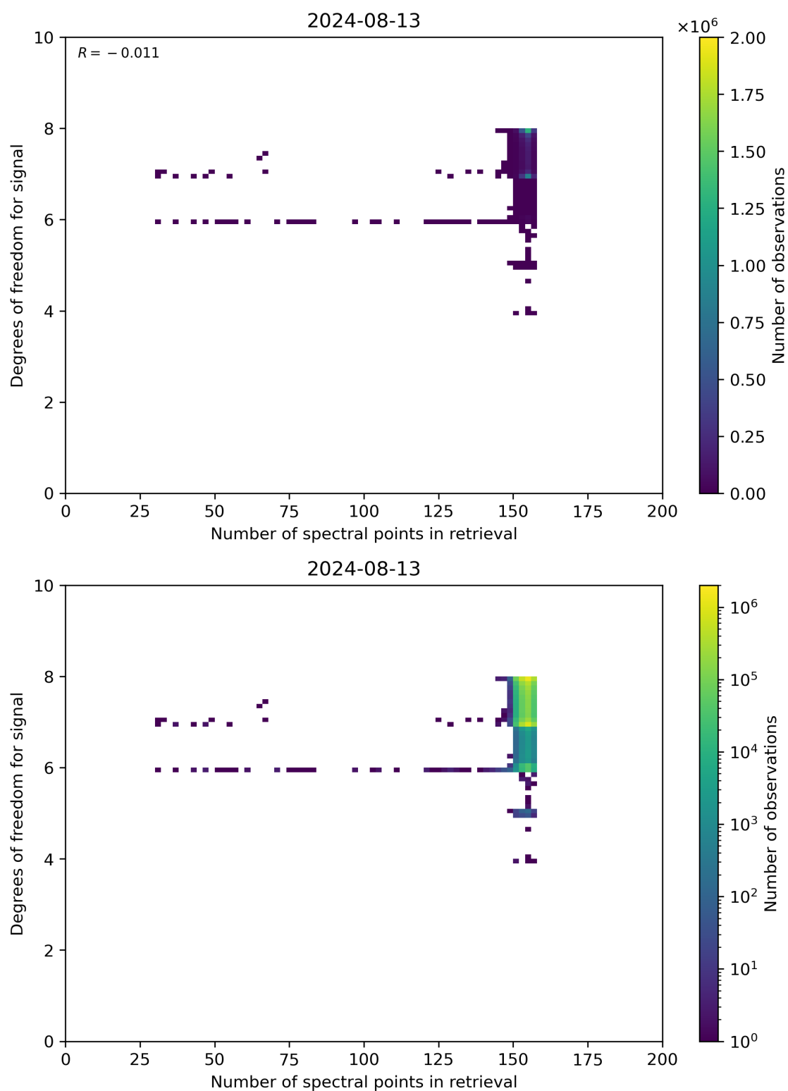
Figure 59: Scatter density plot of “Number of spectral points in retrieval” against “Degrees of freedom for signal” for 2024-08-12 to 2024-08-14.
