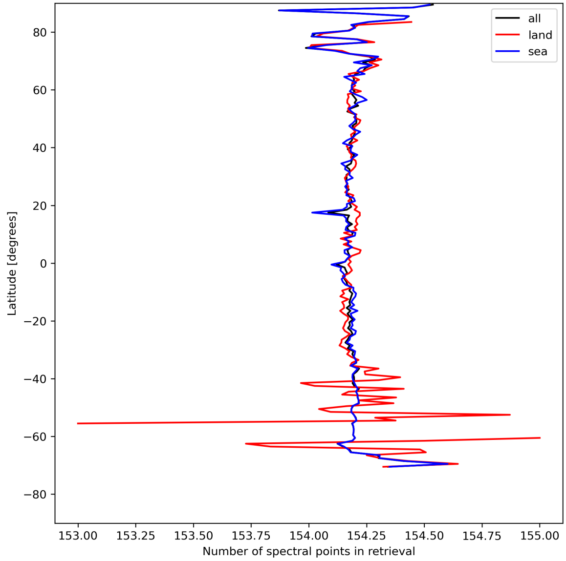
Figure 13: Zonal average of “Number of spectral points in retrieval” for 2024-08-12 to 2024-08-14.
