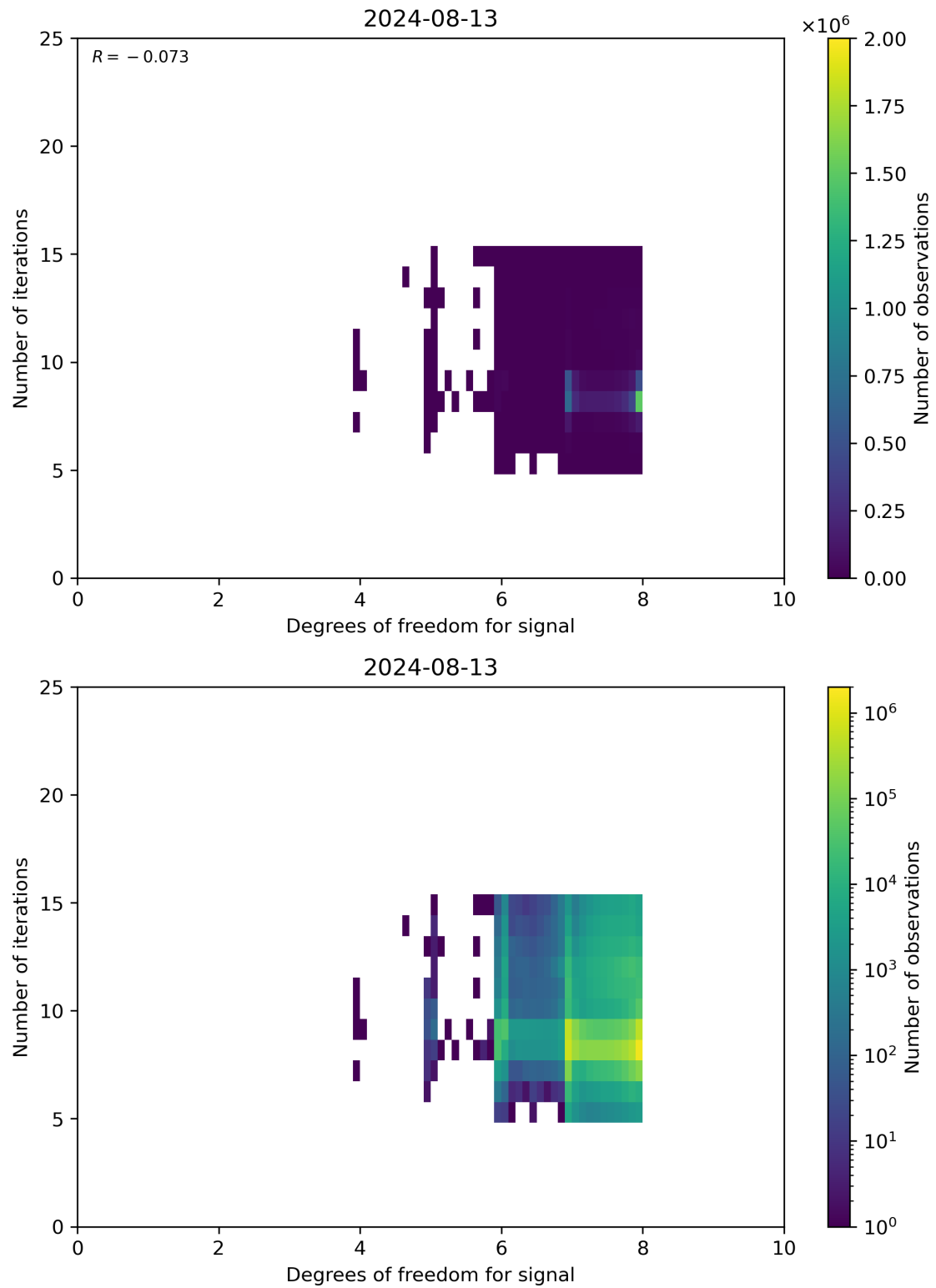
Figure 50: Scatter density plot of “Degrees of freedom for signal” against “Number of iterations” for 2024-08-12 to 2024-08-14.
