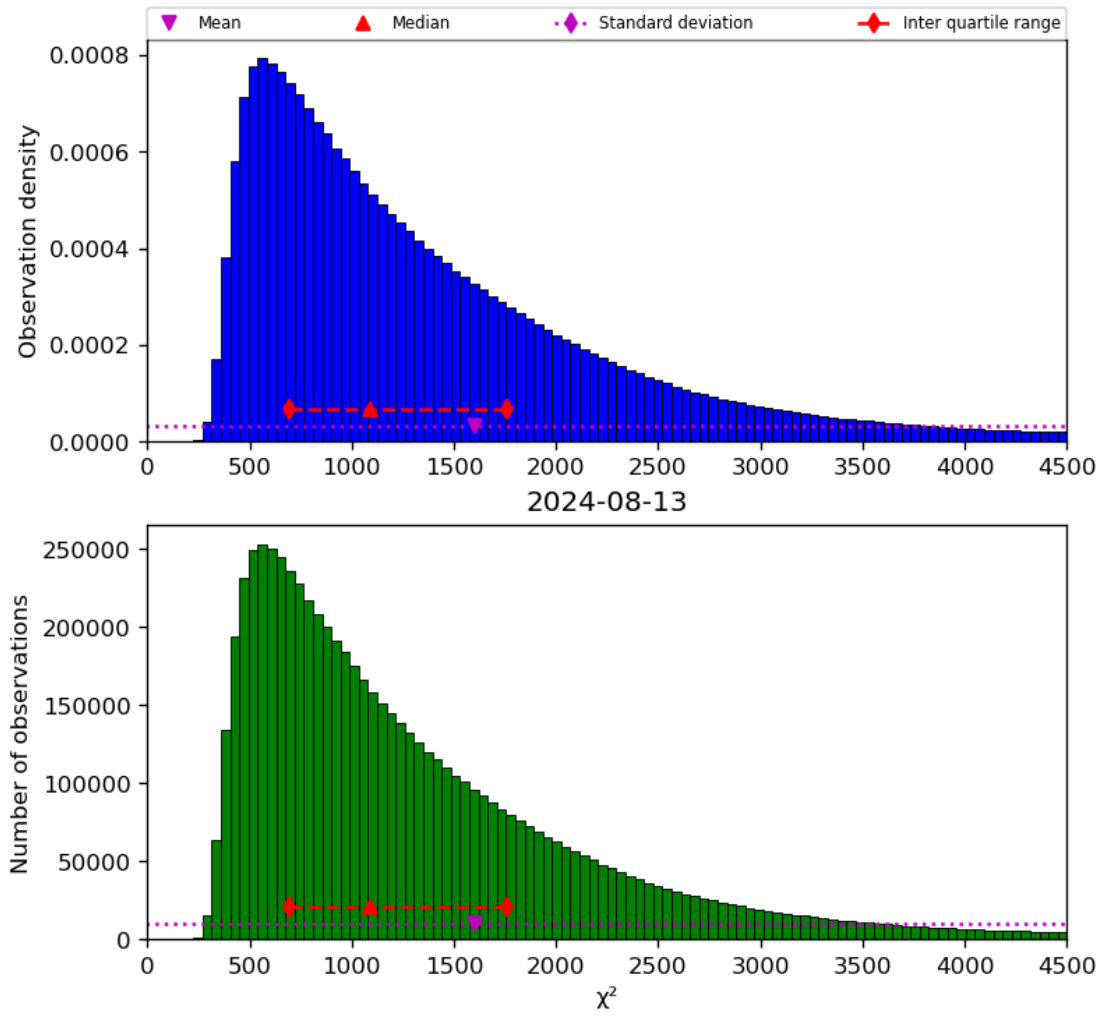
Figure 22: Histogram of “ \chi^2 ” for 2024-08-12 to 2024-08-14
