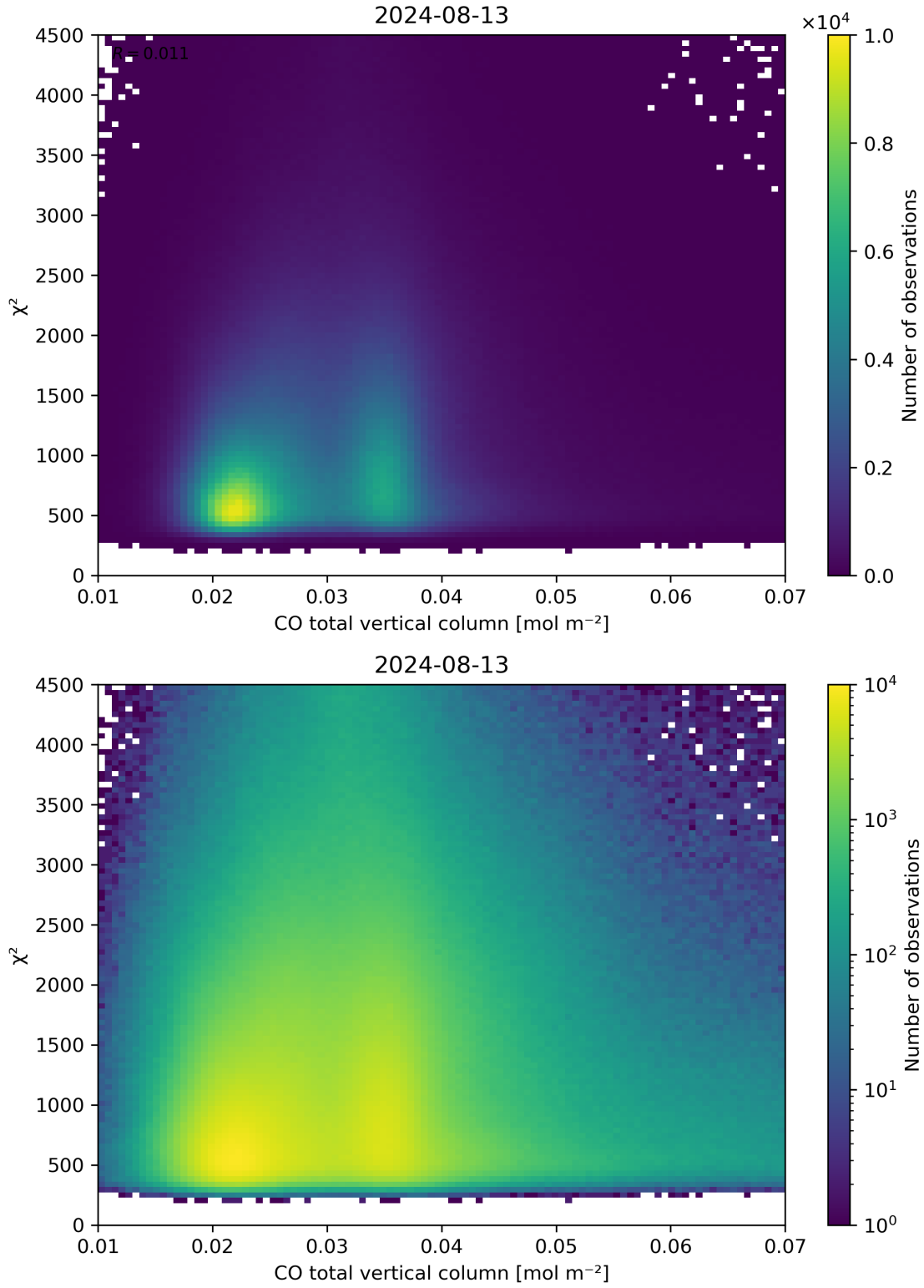
Figure 35: Scatter density plot of “CO total vertical column” against “ \chi^2 ” for 2024-08-12 to 2024-08-14.
