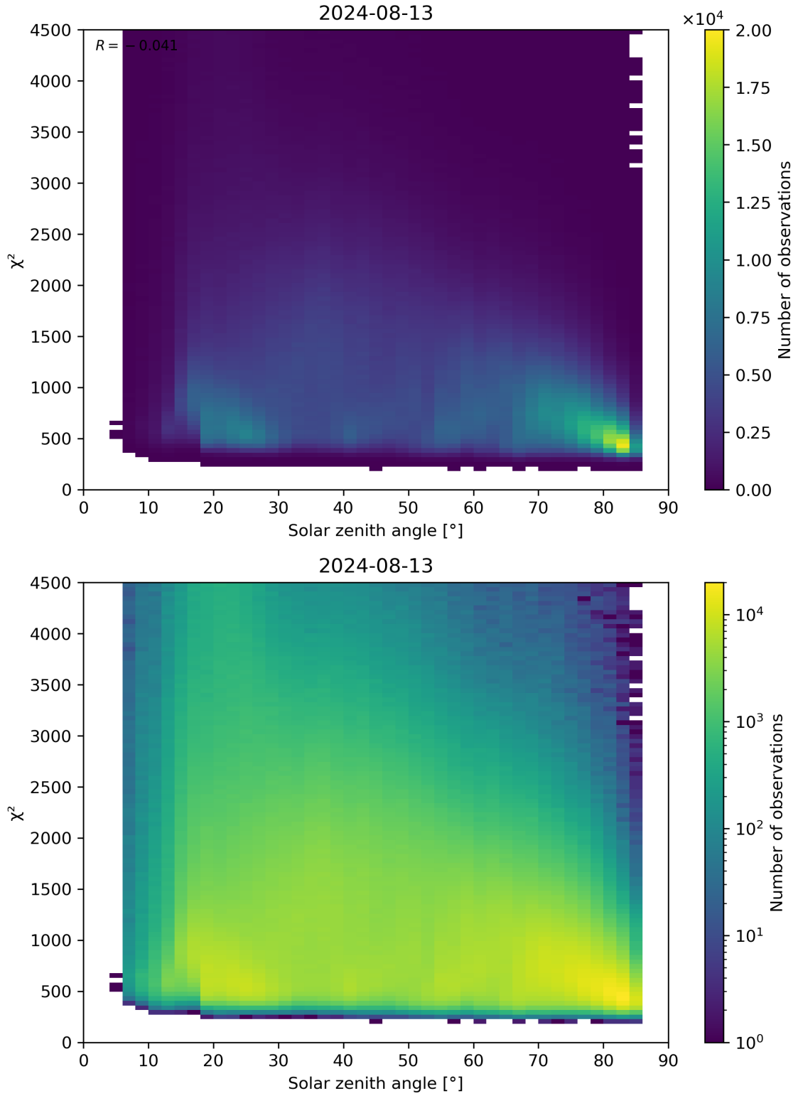
Figure 64: Scatter density plot of “Solar zenith angle” against “ \chi^2 ” for 2024-08-12 to 2024-08-14.
