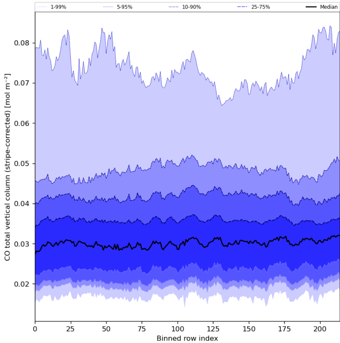
Figure 27: Along track statistics of “CO total vertical column (stripe-corrected)” for 2024-08-12 to 2024-08-14
