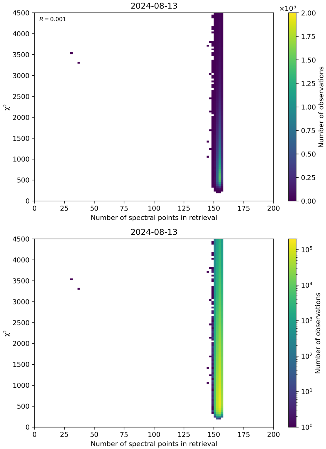
Figure 58: Scatter density plot of “Number of spectral points in retrieval” against “ \chi^2 ” for 2024-08-12 to 2024-08-14.
