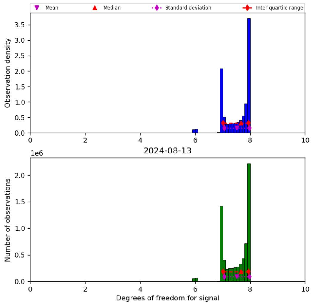
Figure 23: Histogram of “Degrees of freedom for signal” for 2024-08-12 to 2024-08-14
