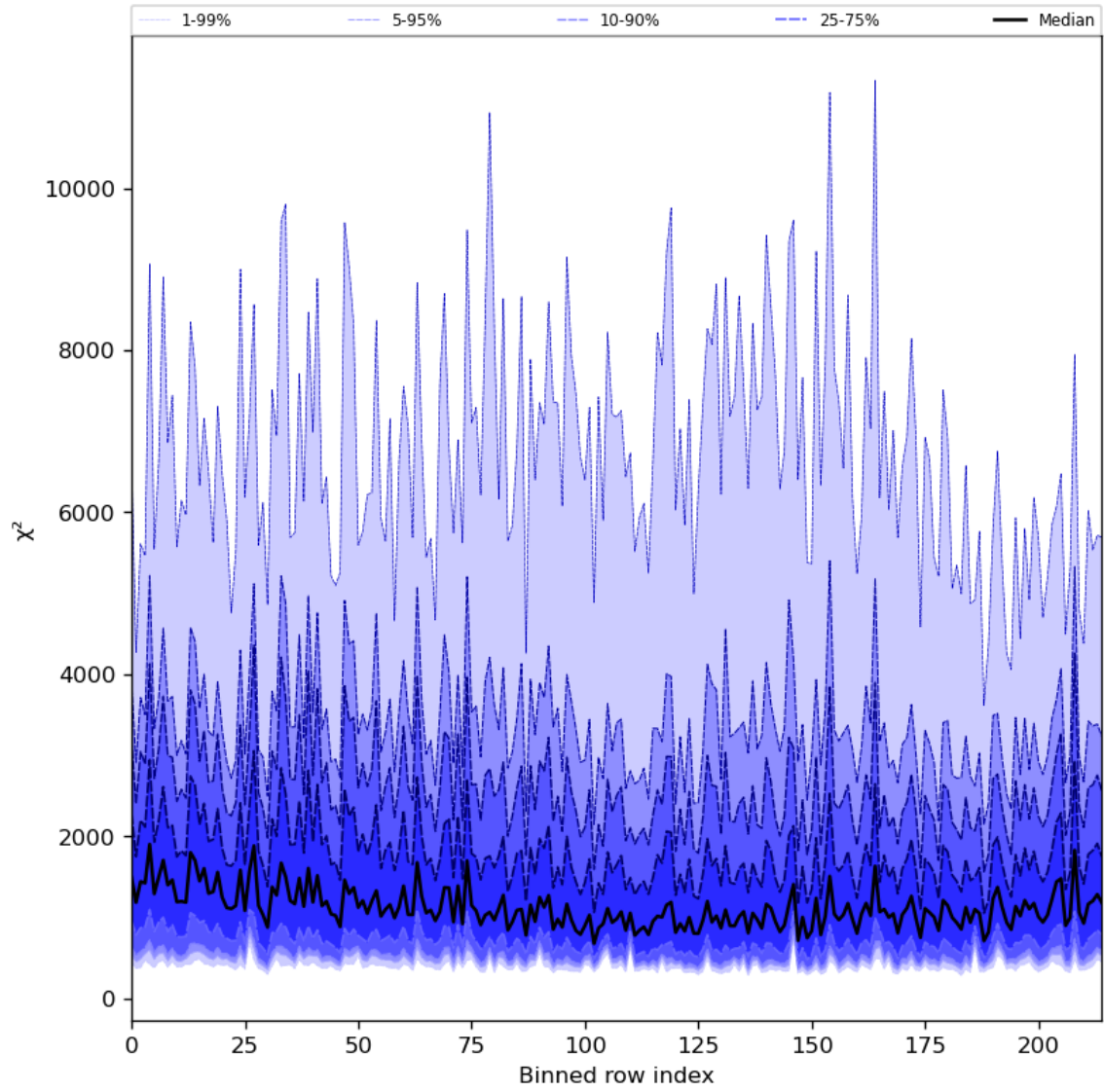
Figure 30: Along track statistics of “ \chi^2 ” for 2024-08-12 to 2024-08-14
