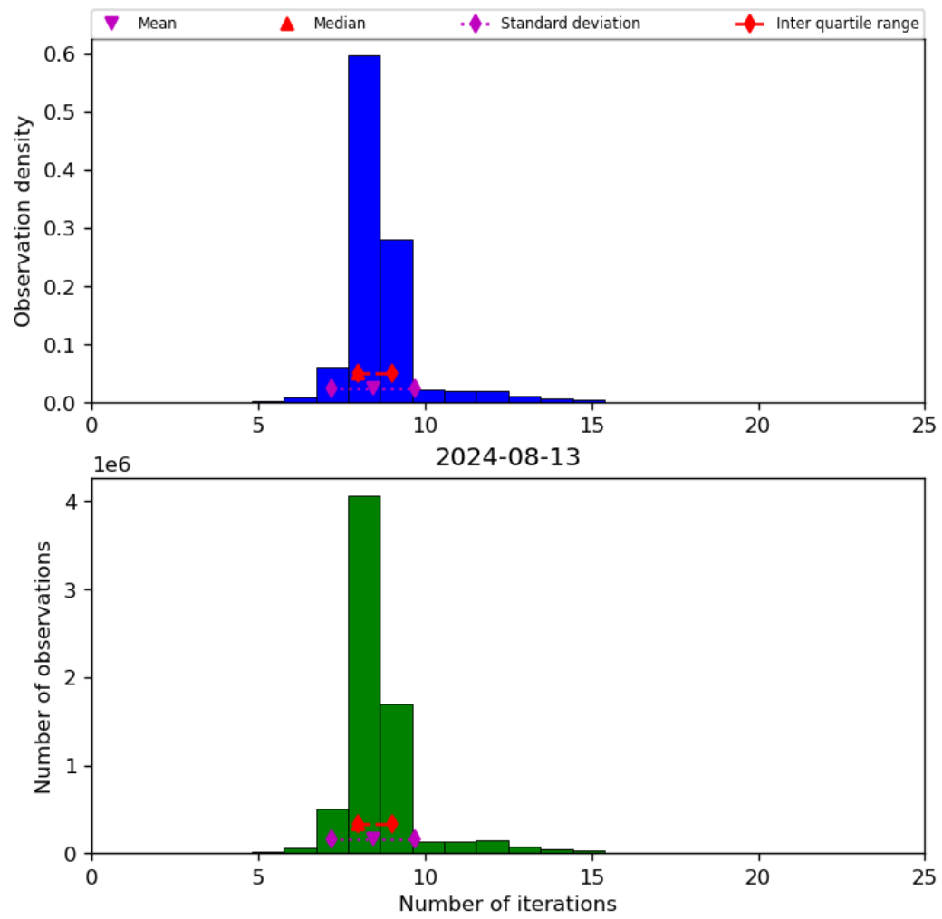
Figure 24: Histogram of “Number of iterations” for 2024-08-12 to 2024-08-14
