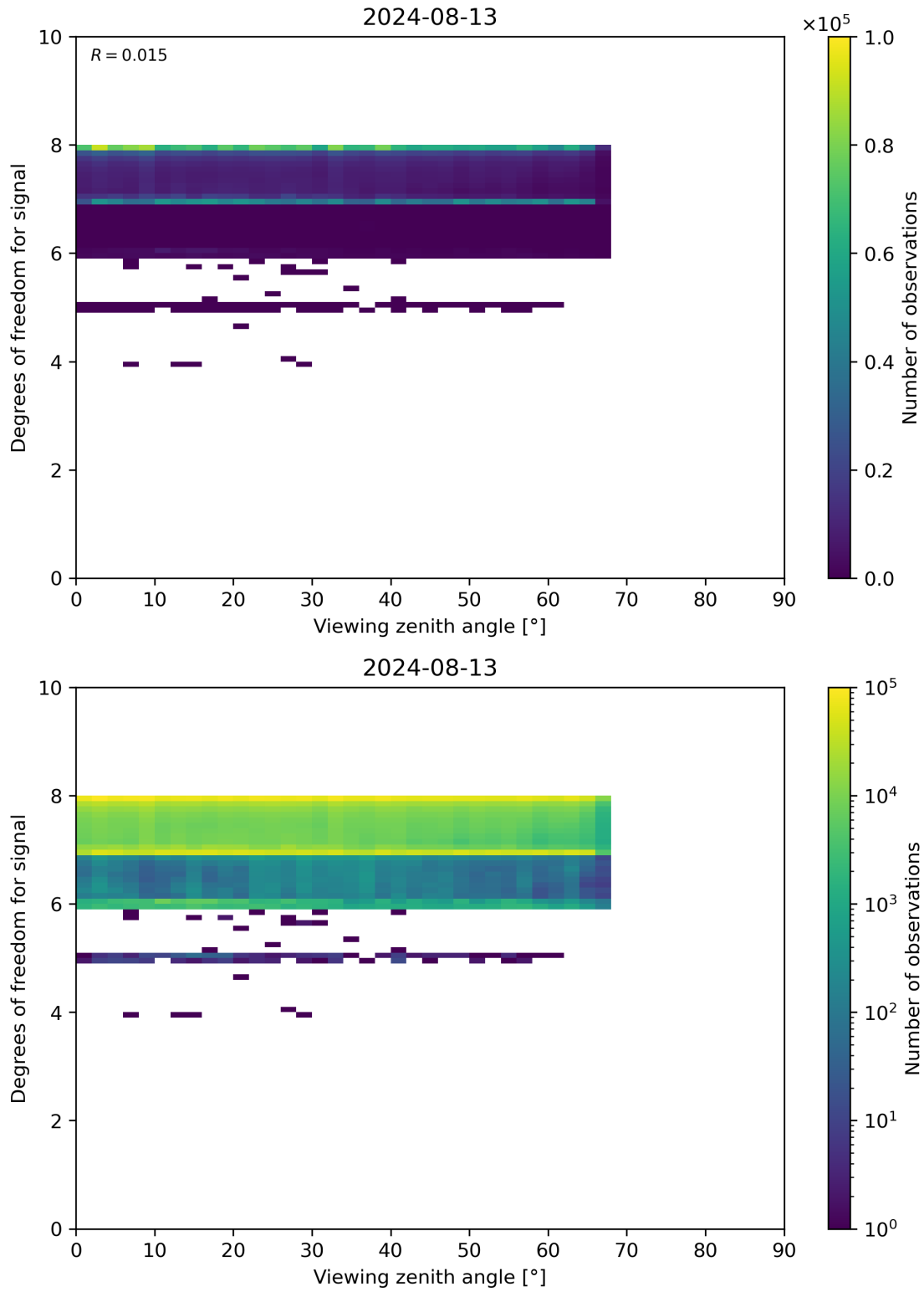
Figure 73: Scatter density plot of “Viewing zenith angle” against “Degrees of freedom for signal” for 2024-08-12 to 2024-08-14.
