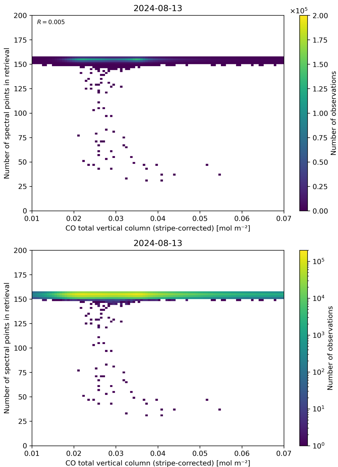
Figure 40: Scatter density plot of “CO total vertical column (stripe-corrected)” against “Number of spectral points in retrieval” for 2024-08-12 to 2024-08-14.
