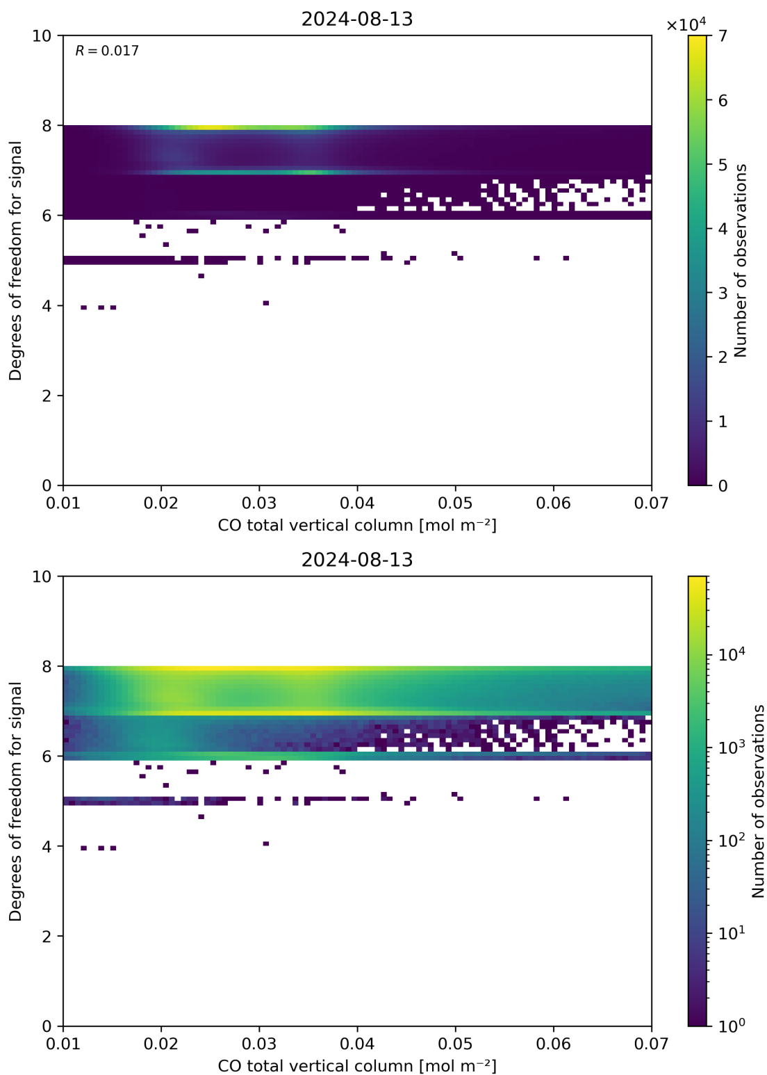
Figure 41: Scatter density plot of “CO total vertical column” against “Degrees of freedom for signal” for 2024-08-12 to 2024-08-14.
