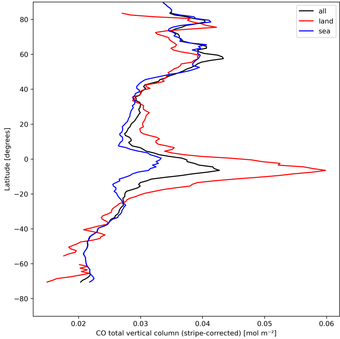
Figure 11: Zonal average of “CO total vertical column (stripe-corrected)” for 2024-08-12 to 2024-08-14.
