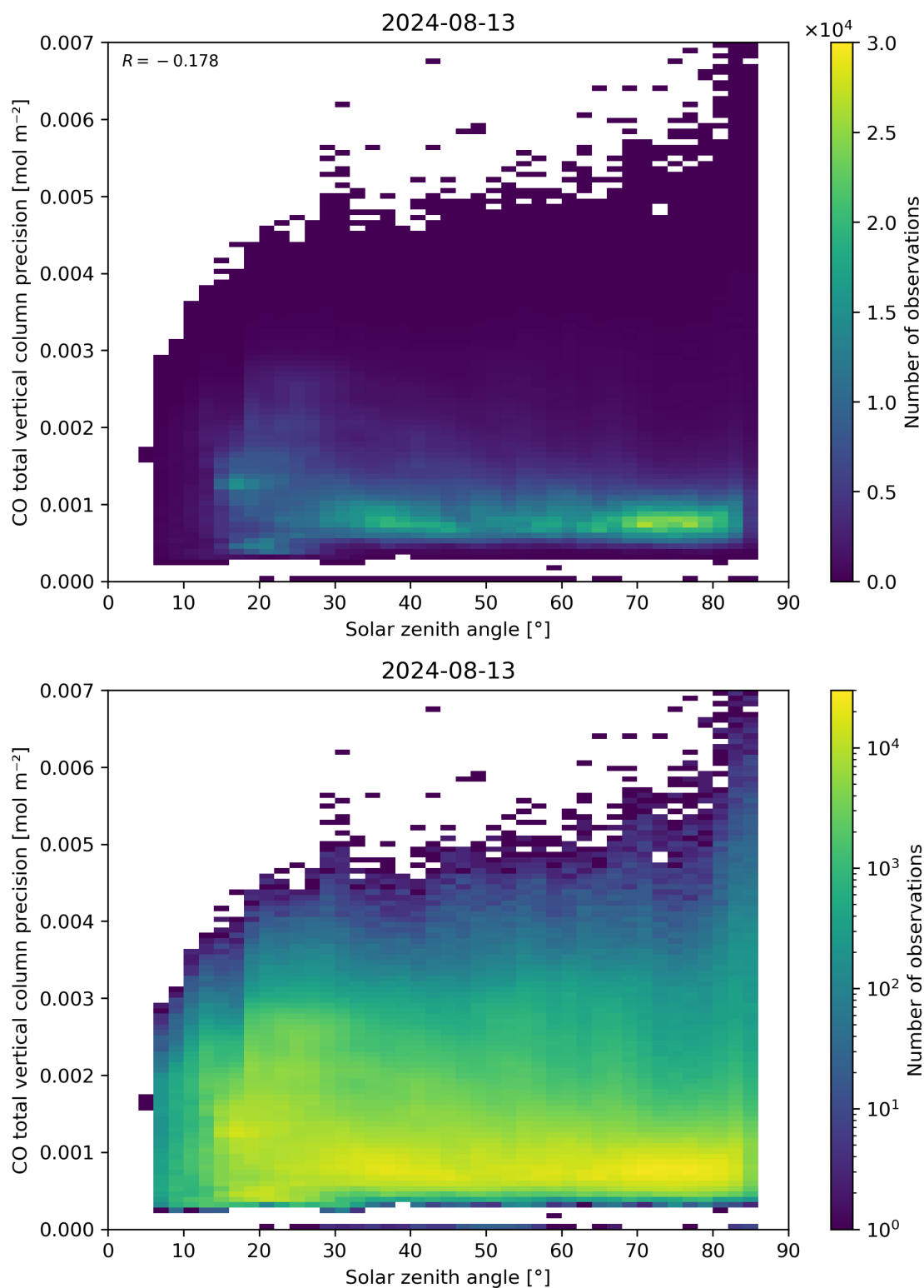
Figure 63: Scatter density plot of “Solar zenith angle” against “CO total vertical column precision” for 2024-08-12 to 2024-08-14.
