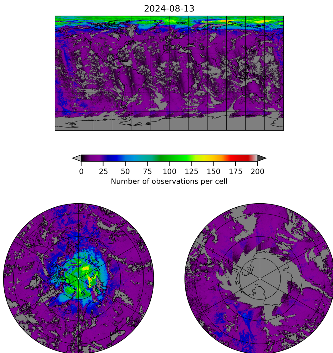
Figure 8: Map of the number of observations for 2024-08-12 to 2024-08-14
