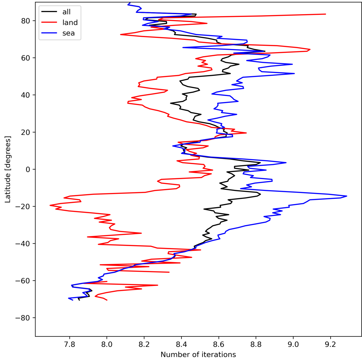
Figure 16: Zonal average of “Number of iterations” for 2024-08-12 to 2024-08-14.
