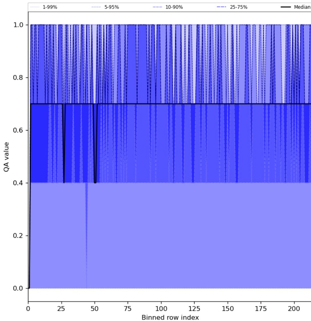
Figure 25: Along track statistics of “QA value” for 2024-08-12 to 2024-08-14
