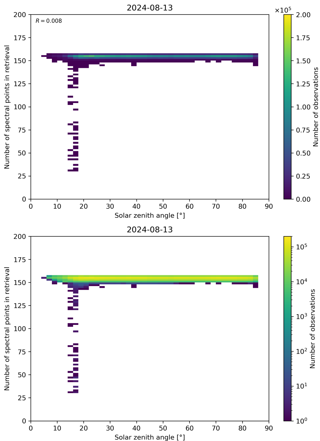
Figure 68: Scatter density plot of “Solar zenith angle” against “Number of spectral points in retrieval” for 2024-08-12 to 2024-08-14.
