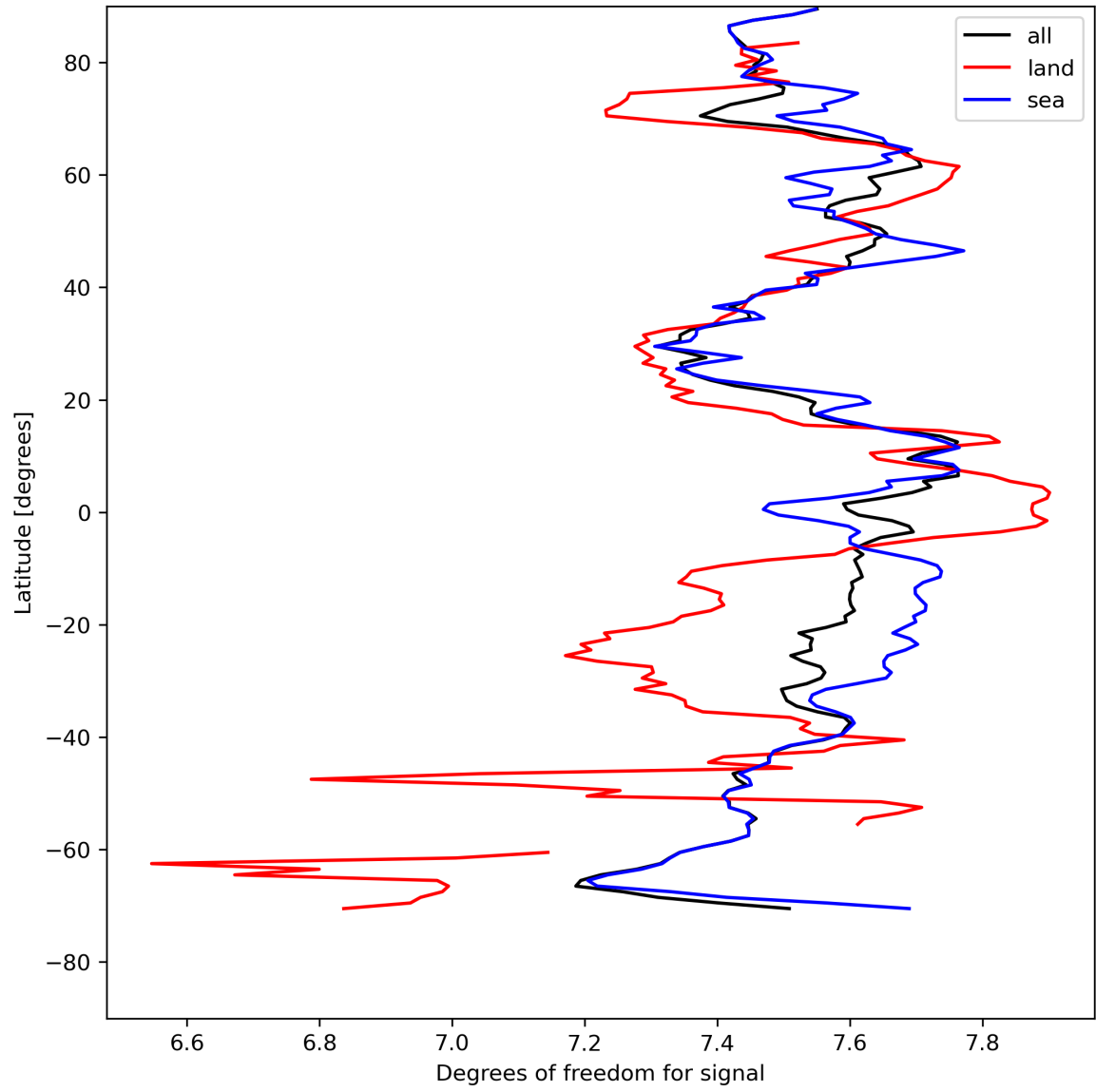
Figure 15: Zonal average of “Degrees of freedom for signal” for 2024-08-12 to 2024-08-14.
