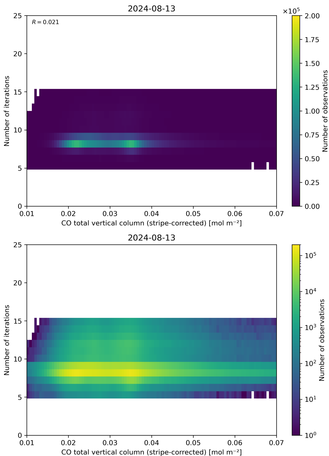
Figure 39: Scatter density plot of “CO total vertical column (stripe-corrected)” against “Number of iterations” for 2024-08-12 to 2024-08-14.
