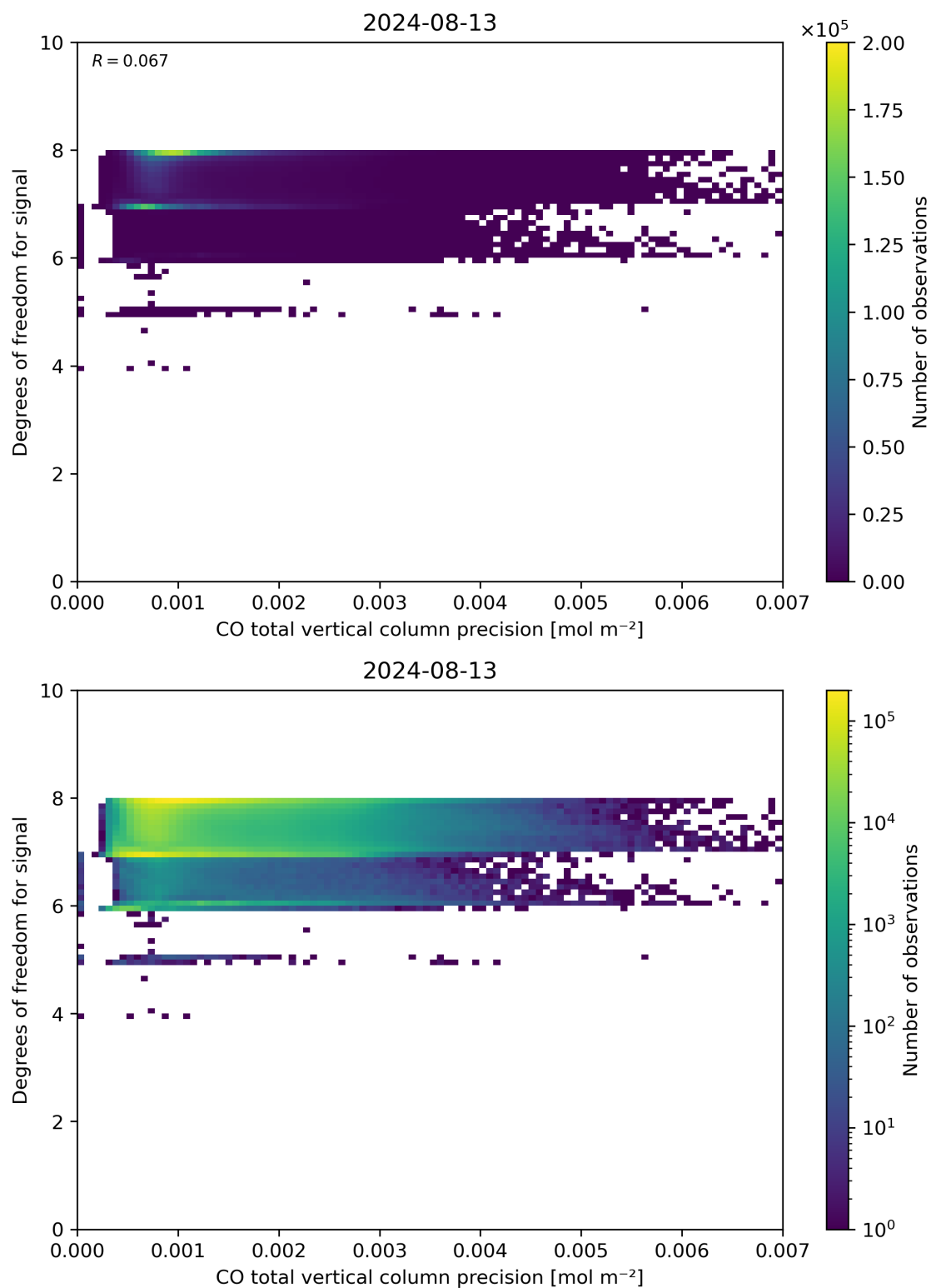
Figure 45: Scatter density plot of “CO total vertical column precision” against “Degrees of freedom for signal” for 2024-08-12 to 2024-08-14.
