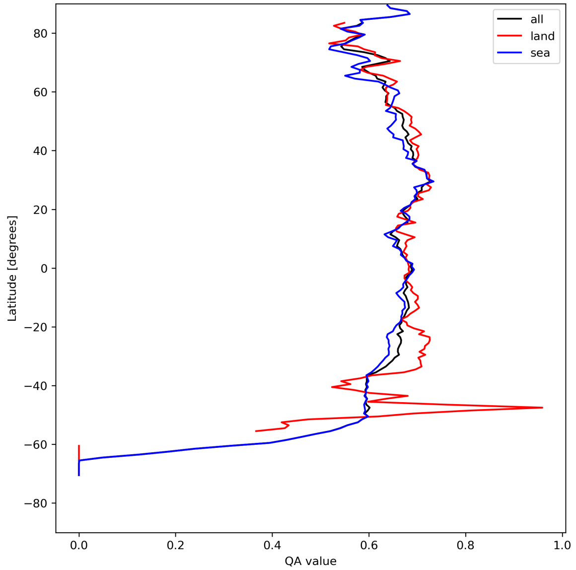
Figure 9: Zonal average of “QA value” for 2024-08-12 to 2024-08-14.
