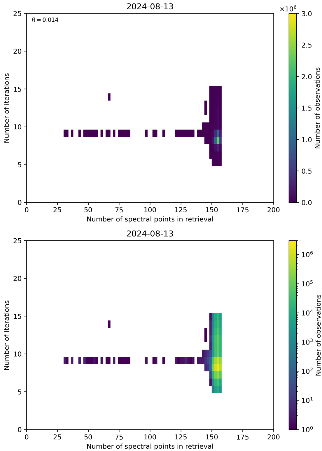
Figure 60: Scatter density plot of “Number of spectral points in retrieval” against “Number of iterations” for 2024-08-12 to 2024-08-14.
