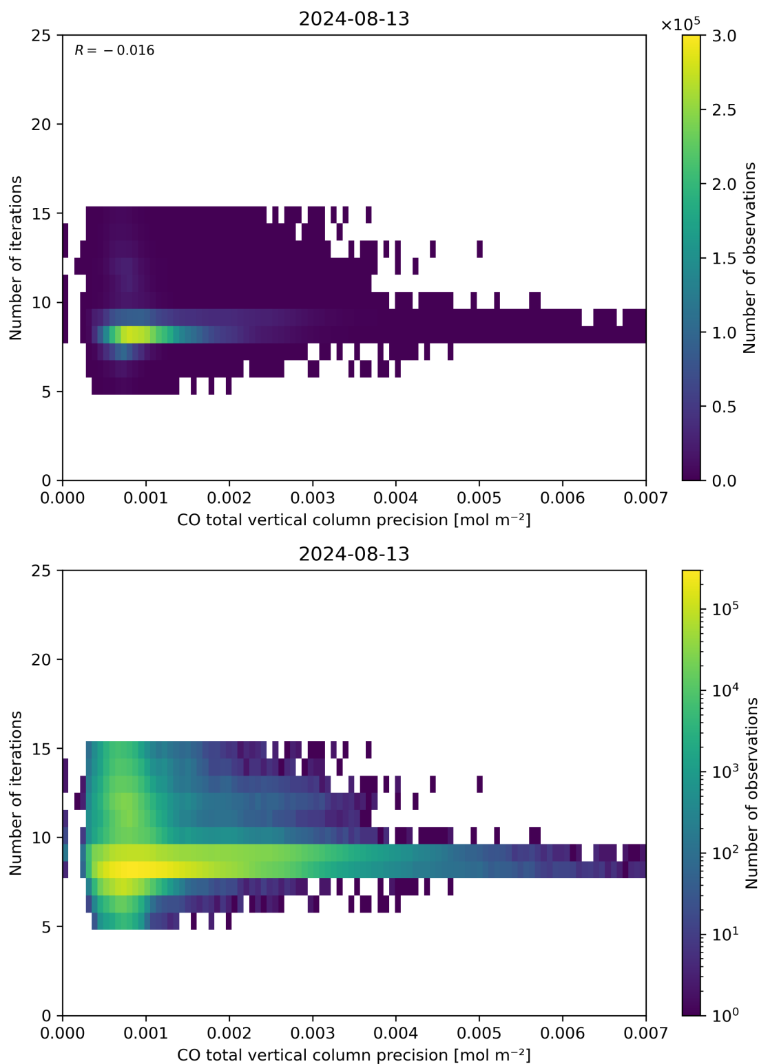
Figure 46: Scatter density plot of “CO total vertical column precision” against “Number of iterations” for 2024-08-12 to 2024-08-14.
