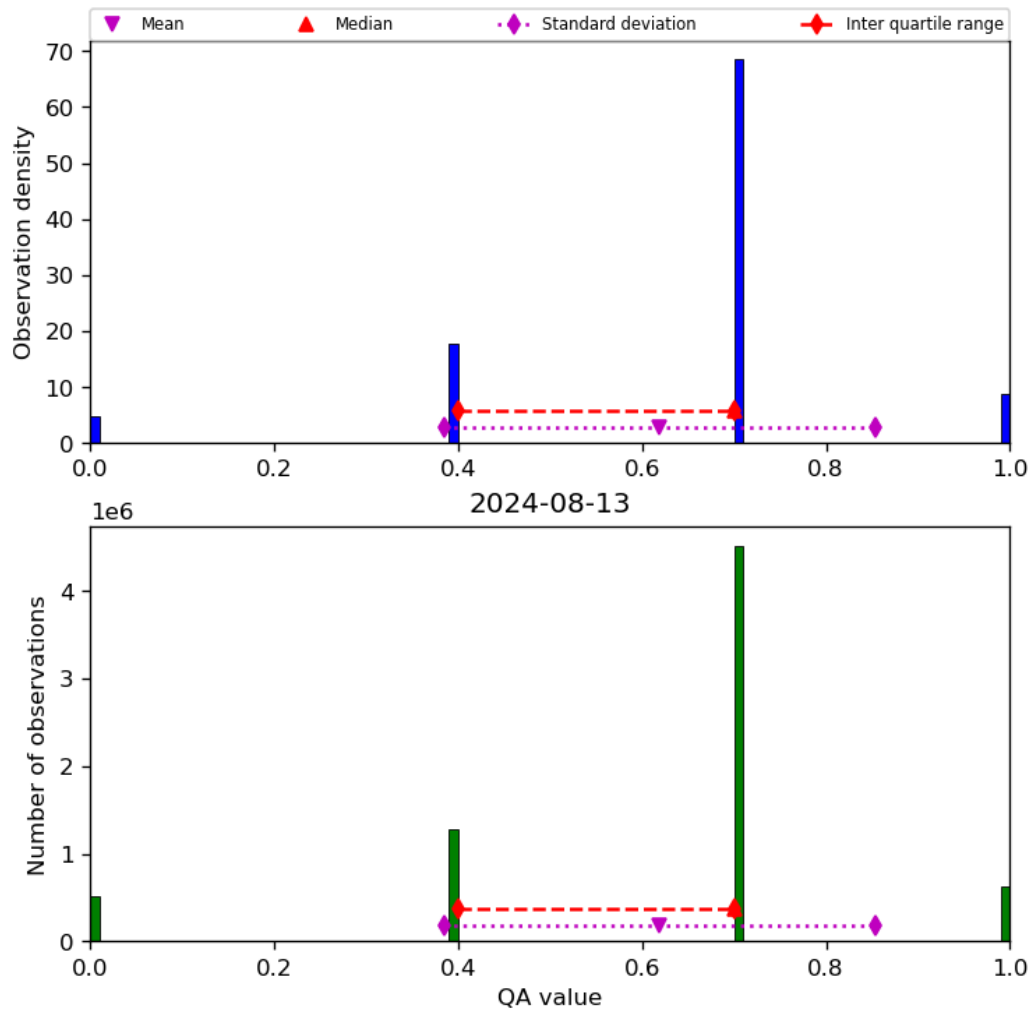
Figure 17: Histogram of “QA value” for 2024-08-12 to 2024-08-14
