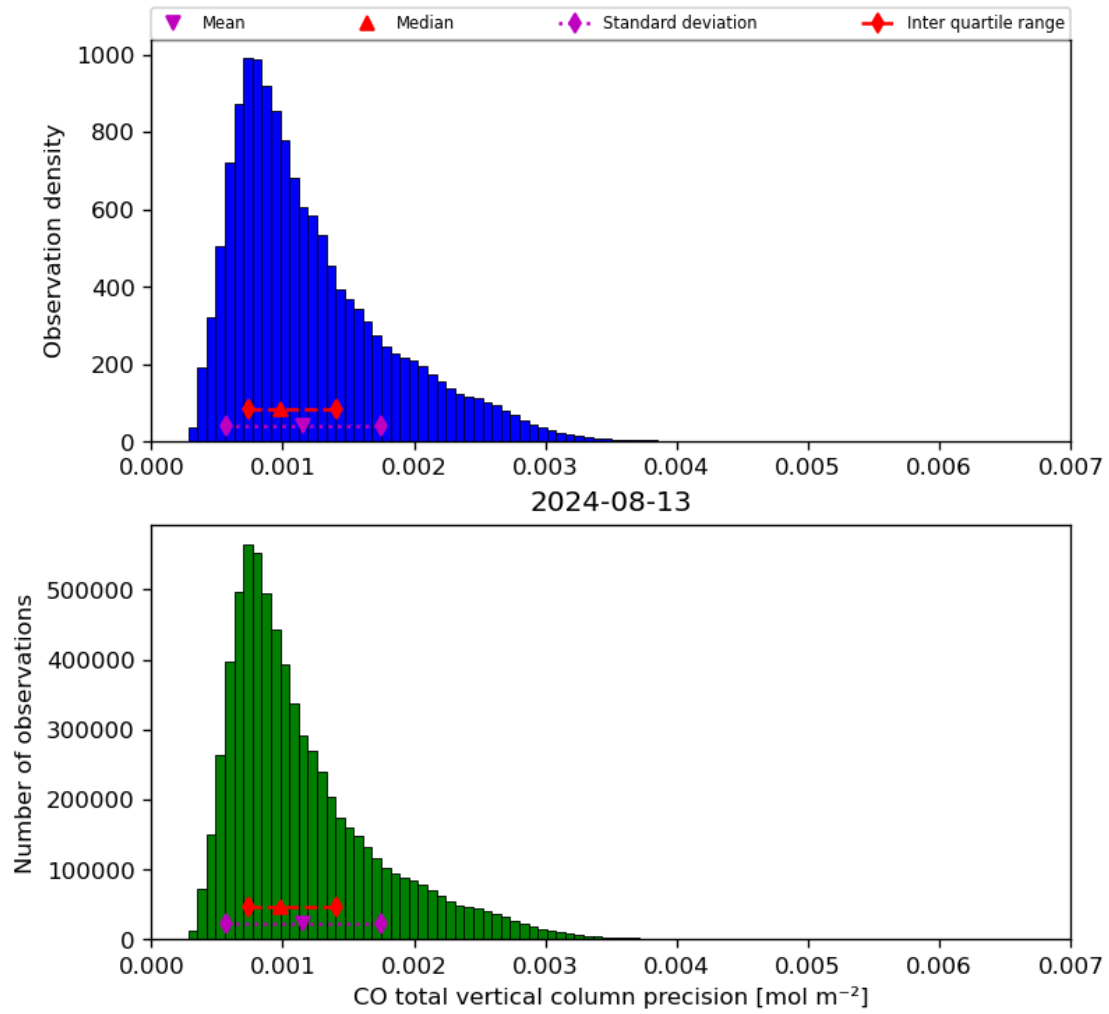
Figure 20: Histogram of “CO total vertical column precision” for 2024-08-12 to 2024-08-14
