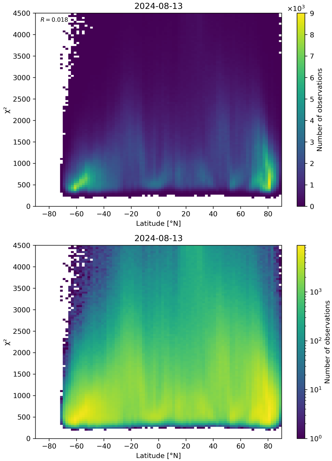
Figure 54: Scatter density plot of “Latitude” against “ \chi^2 ” for 2024-08-12 to 2024-08-14.
