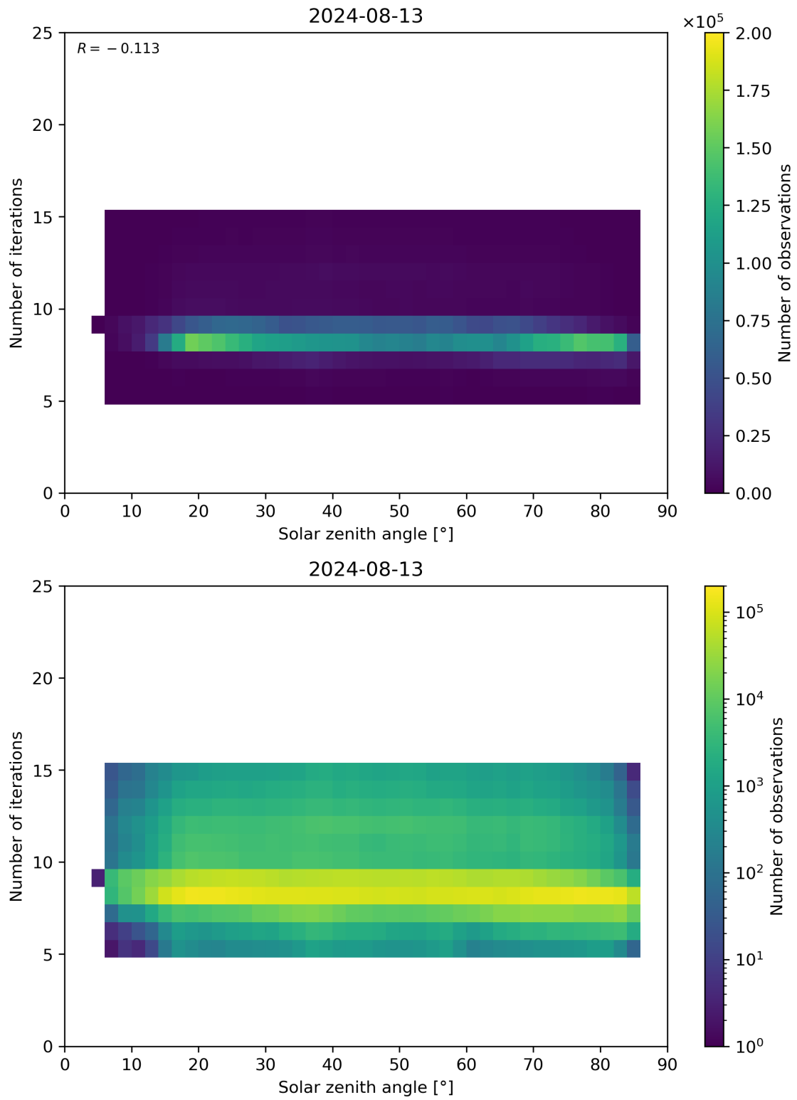
Figure 67: Scatter density plot of “Solar zenith angle” against “Number of iterations” for 2024-08-12 to 2024-08-14.
