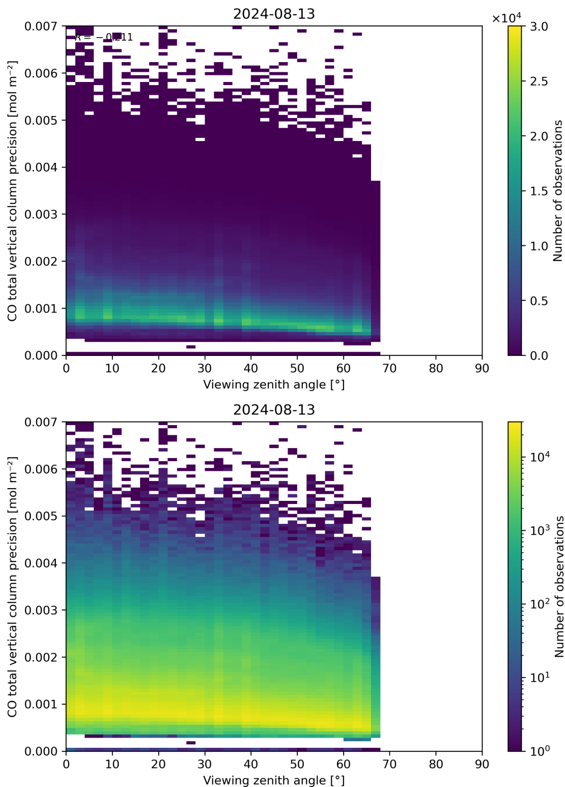
Figure 71: Scatter density plot of “Viewing zenith angle” against “CO total vertical column precision” for 2024-08-12 to 2024-08-14.
