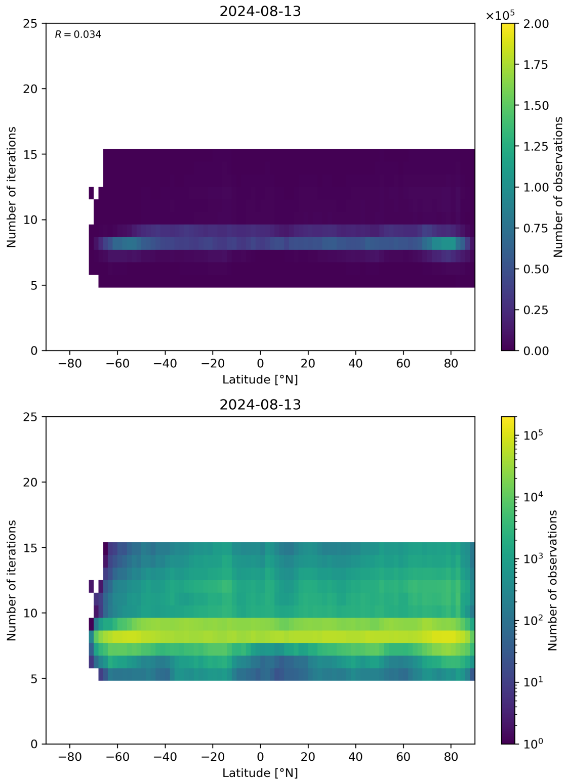
Figure 56: Scatter density plot of “Latitude” against “Number of iterations” for 2024-08-12 to 2024-08-14.
