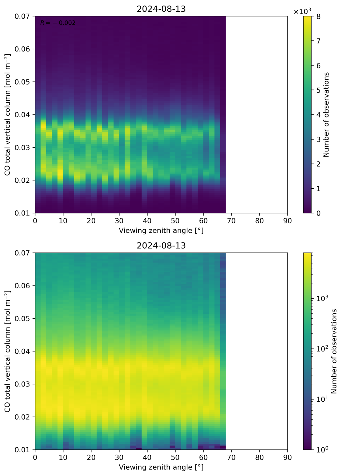
Figure 69: Scatter density plot of “Viewing zenith angle” against “CO total vertical column” for 2024-08-12 to 2024-08-14.
