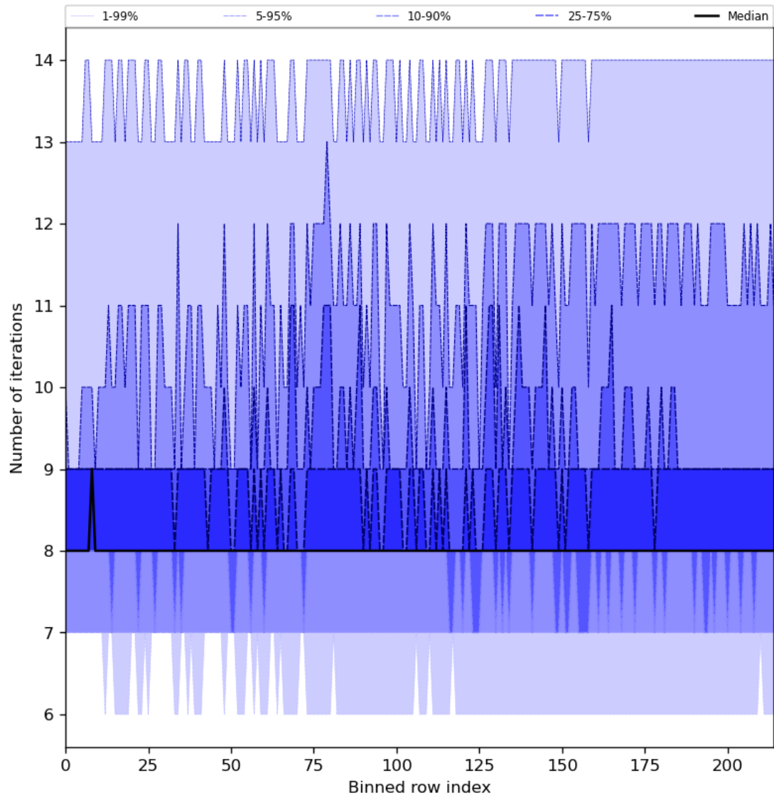
Figure 32: Along track statistics of “Number of iterations” for 2024-08-12 to 2024-08-14
