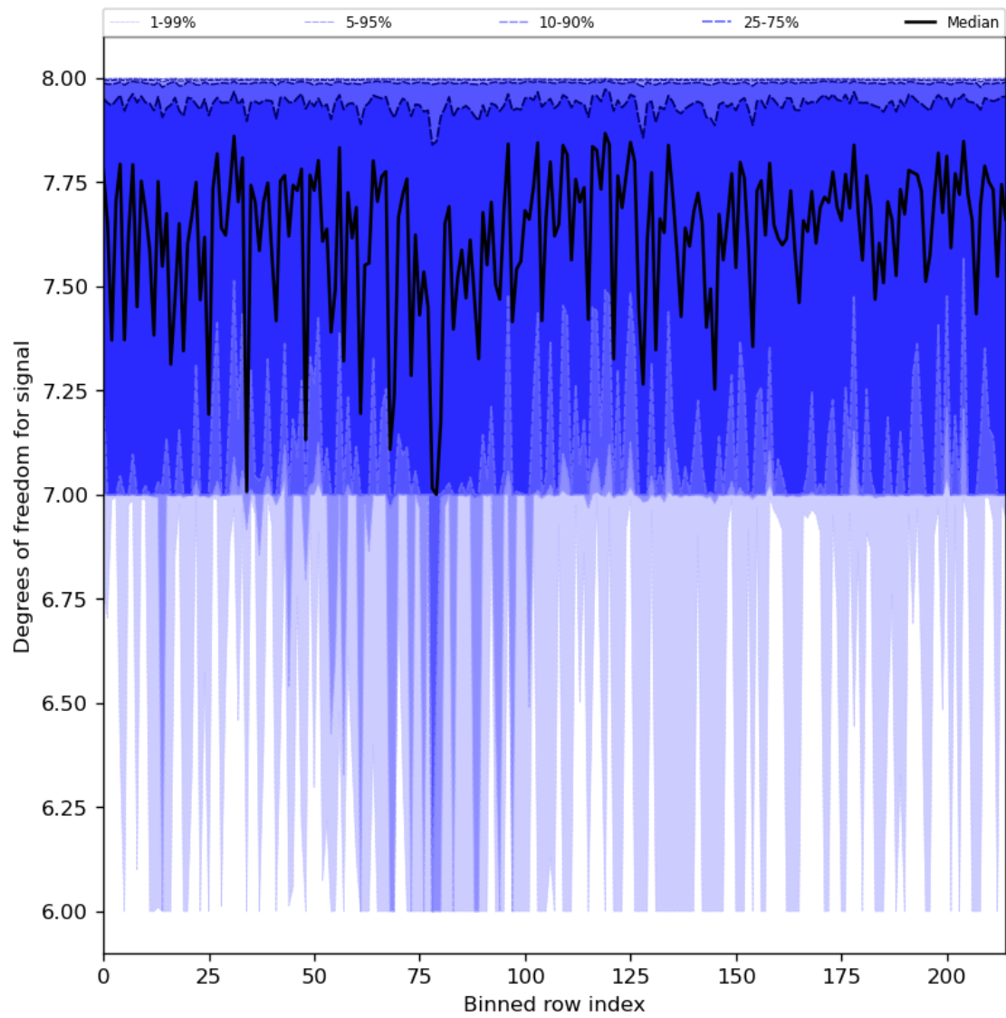
Figure 31: Along track statistics of “Degrees of freedom for signal” for 2024-08-12 to 2024-08-14
