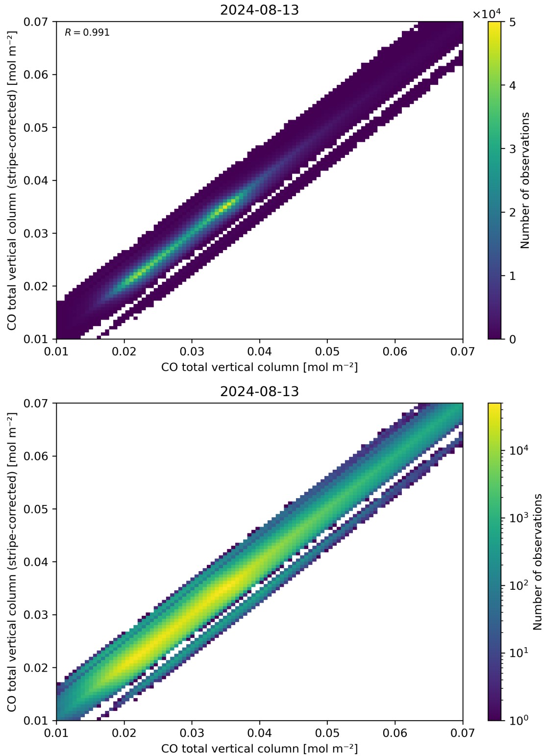
Figure 33: Scatter density plot of “CO total vertical column” against “CO total vertical column (stripe-corrected)” for 2024-08-12 to 2024-08-14.
