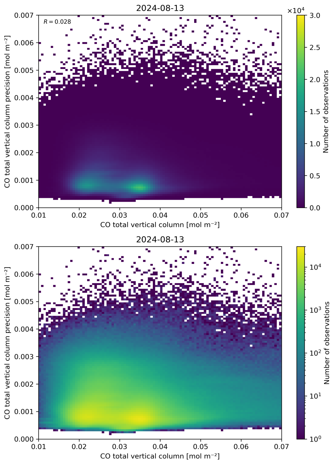
Figure 34: Scatter density plot of “CO total vertical column” against “CO total vertical column precision” for 2024-08-12 to 2024-08-14.
