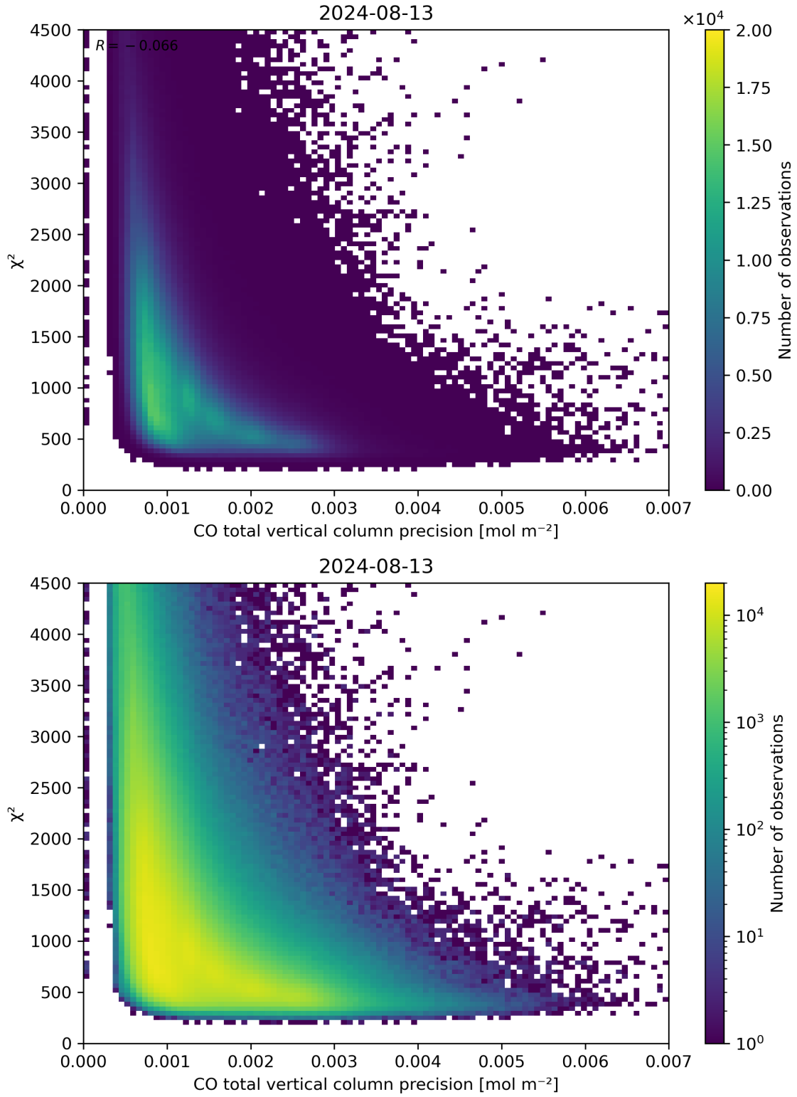
Figure 44: Scatter density plot of “CO total vertical column precision” against “ \chi^2 ” for 2024-08-12 to 2024-08-14.
