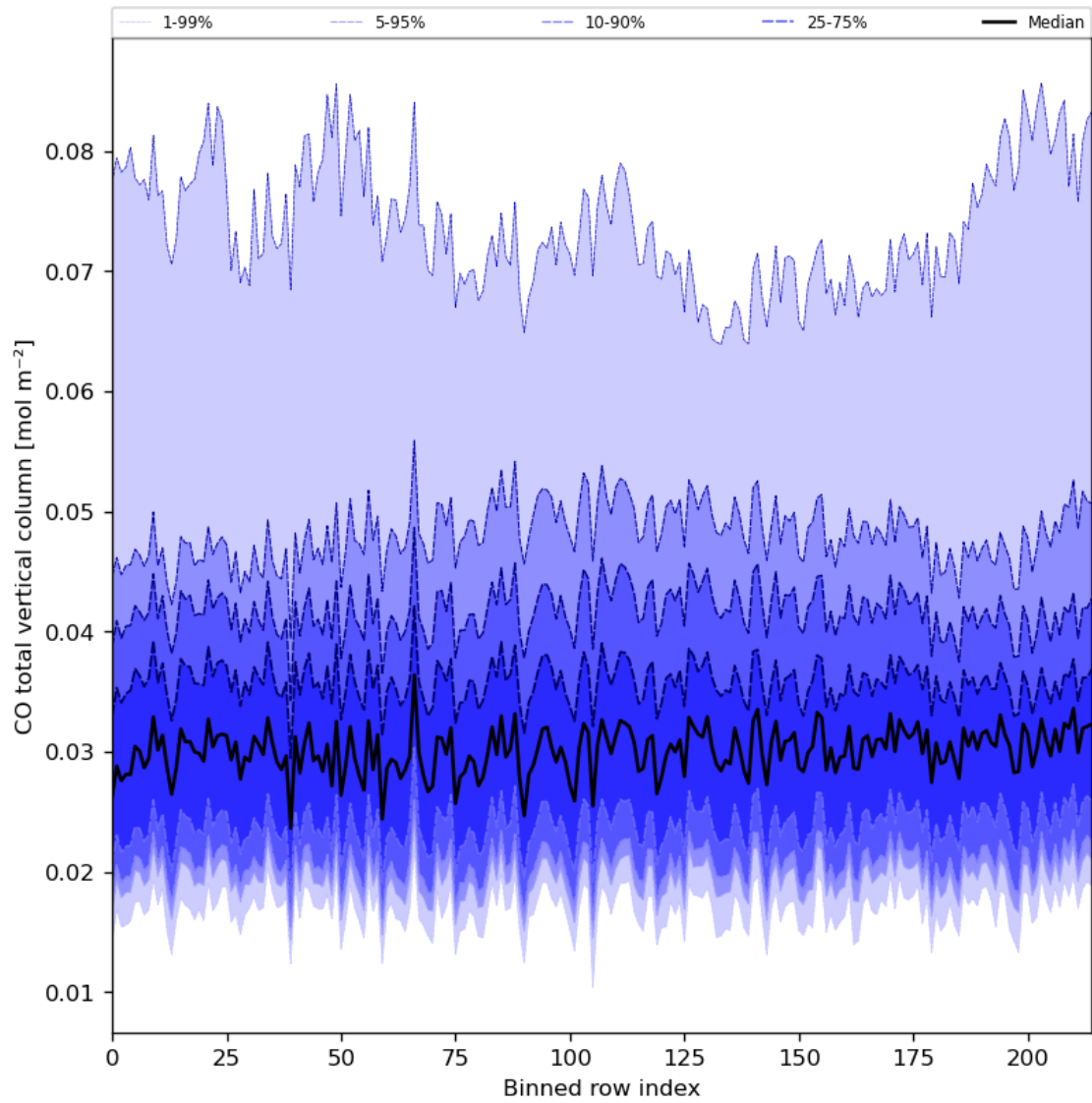
Figure 26: Along track statistics of “CO total vertical column” for 2024-08-12 to 2024-08-14
