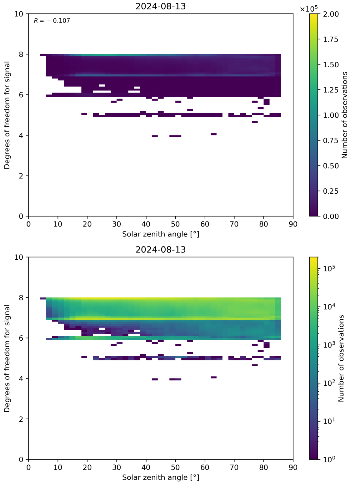
Figure 65: Scatter density plot of “Solar zenith angle” against “Degrees of freedom for signal” for 2024-08-12 to 2024-08-14.
