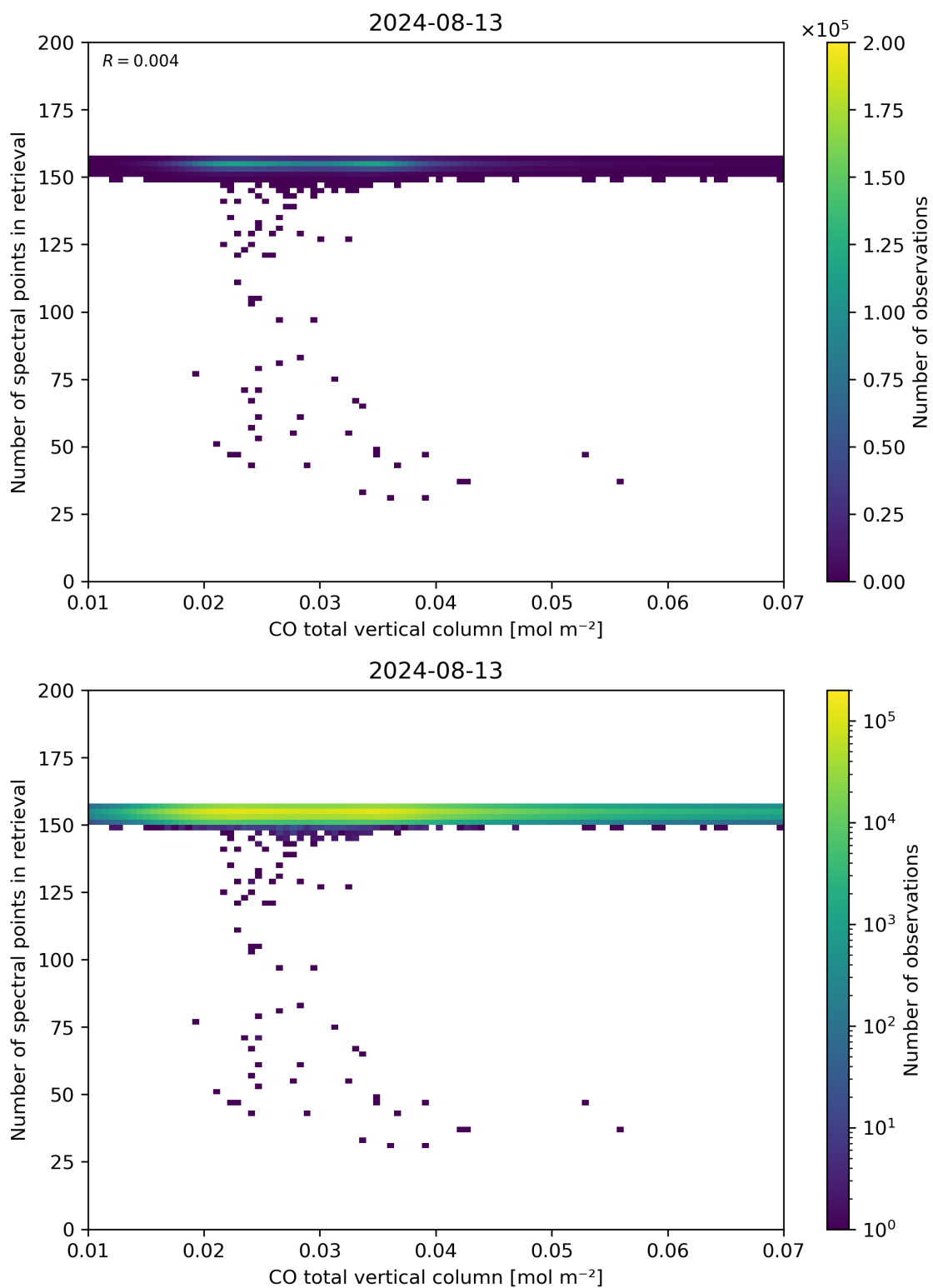
Figure 43: Scatter density plot of “CO total vertical column” against “Number of spectral points in retrieval” for 2024-08-12 to 2024-08-14.
