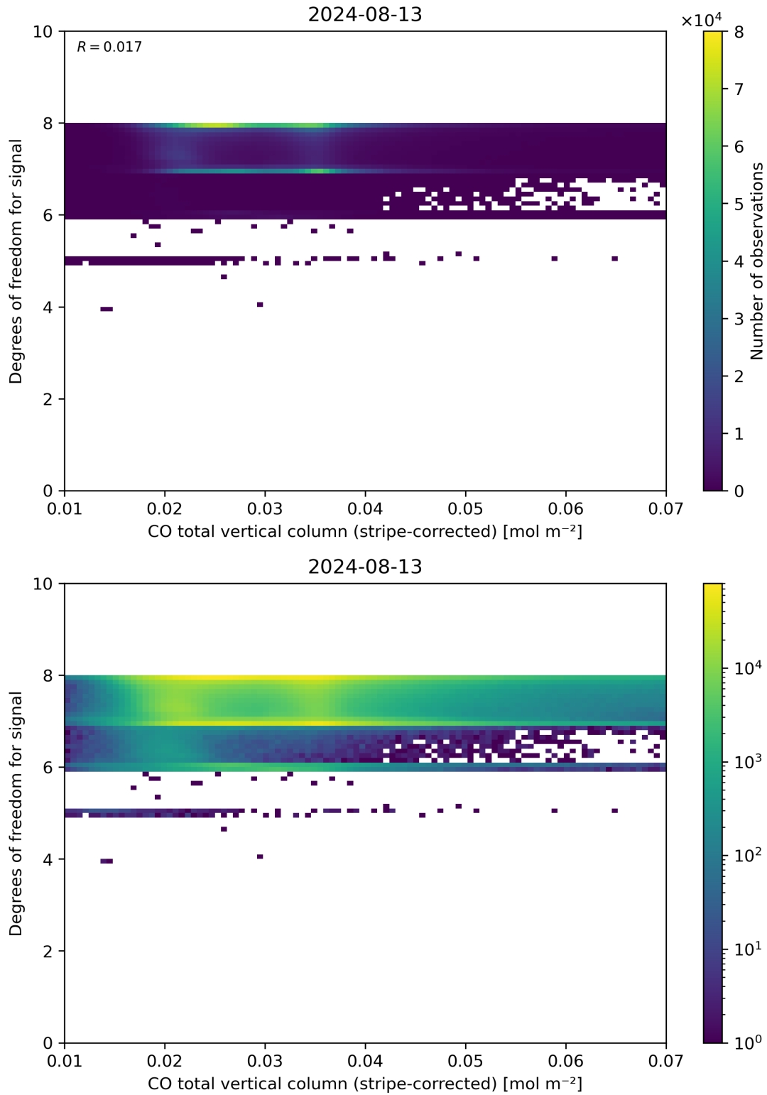
Figure 38: Scatter density plot of “CO total vertical column (stripe-corrected)” against “Degrees of freedom for signal” for 2024-08-12 to 2024-08-14.
