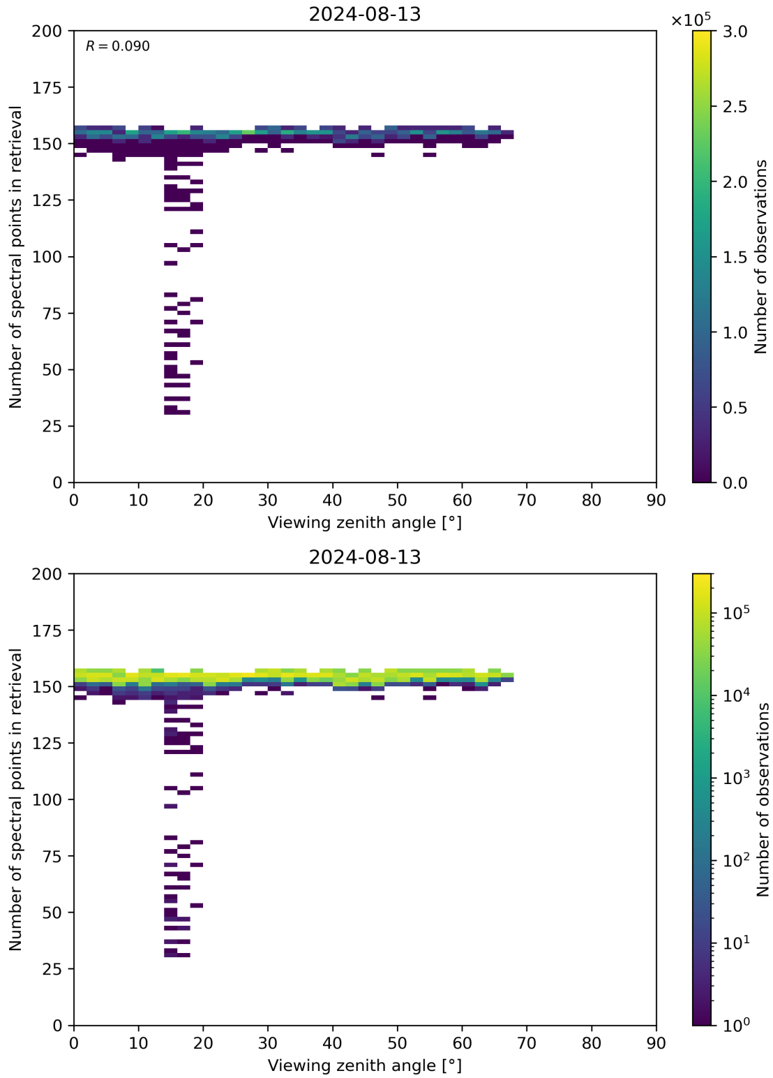
Figure 76: Scatter density plot of “Viewing zenith angle” against “Number of spectral points in retrieval” for 2024-08-12 to 2024-08-14.
