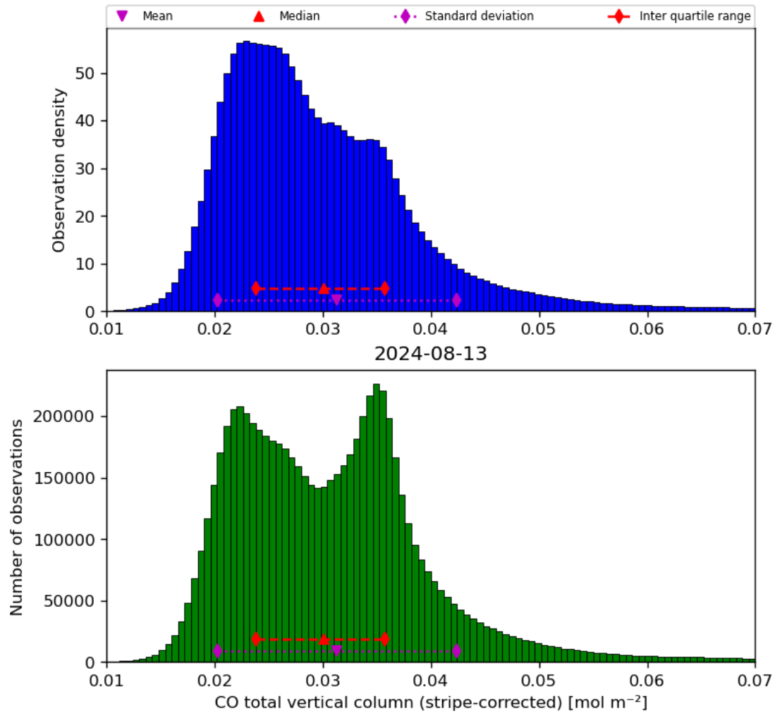
Figure 19: Histogram of “CO total vertical column (stripe-corrected)” for 2024-08-12 to 2024-08-14
