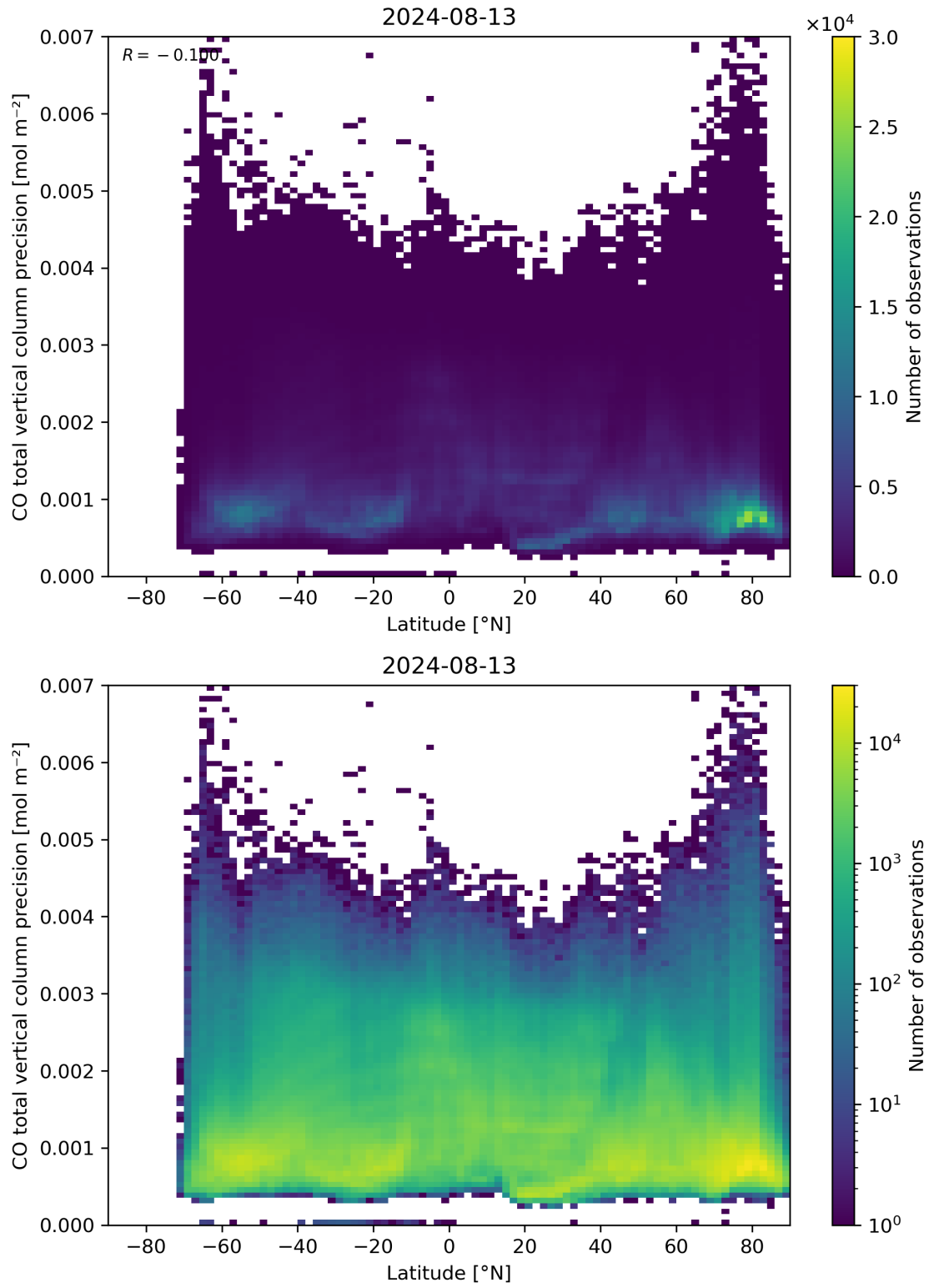
Figure 53: Scatter density plot of “Latitude” against “CO total vertical column precision” for 2024-08-12 to 2024-08-14.
