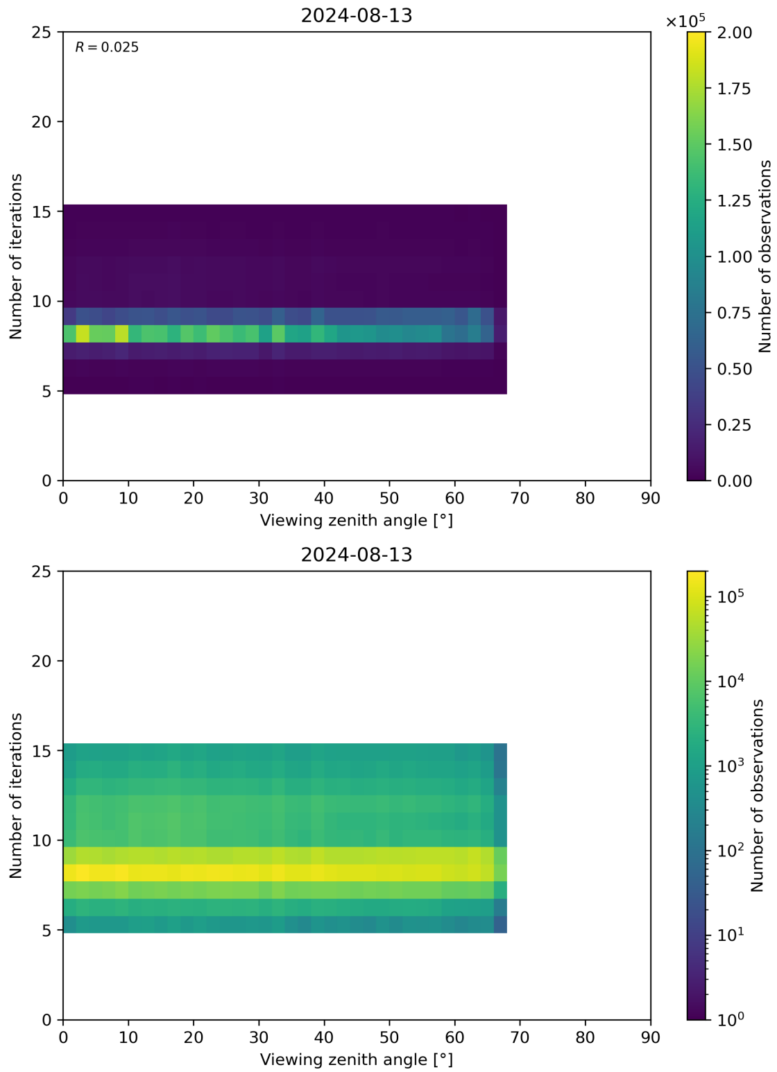
Figure 75: Scatter density plot of “Viewing zenith angle” against “Number of iterations” for 2024-08-12 to 2024-08-14.
