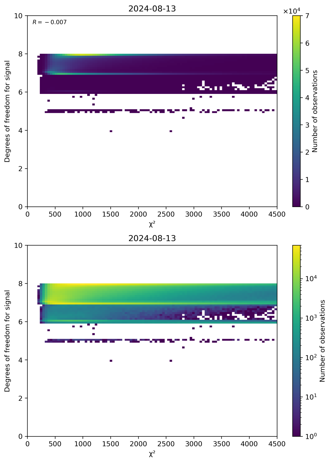
Figure 48: Scatter density plot of “ \chi^2 ” against “Degrees of freedom for signal” for 2024-08-12 to 2024-08-14.
