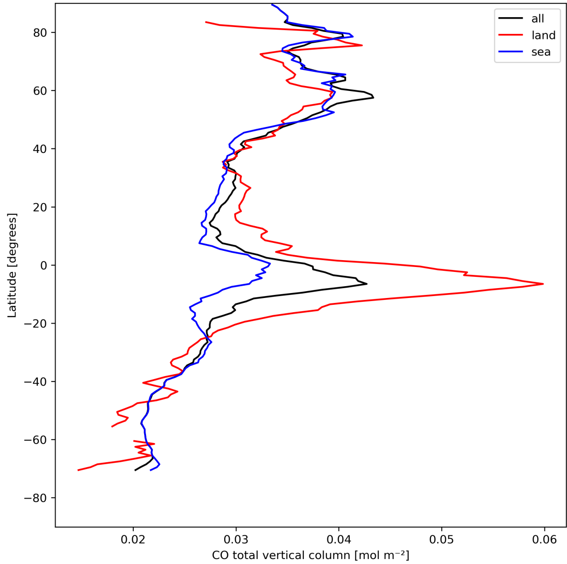
Figure 10: Zonal average of “CO total vertical column” for 2024-08-12 to 2024-08-14.
