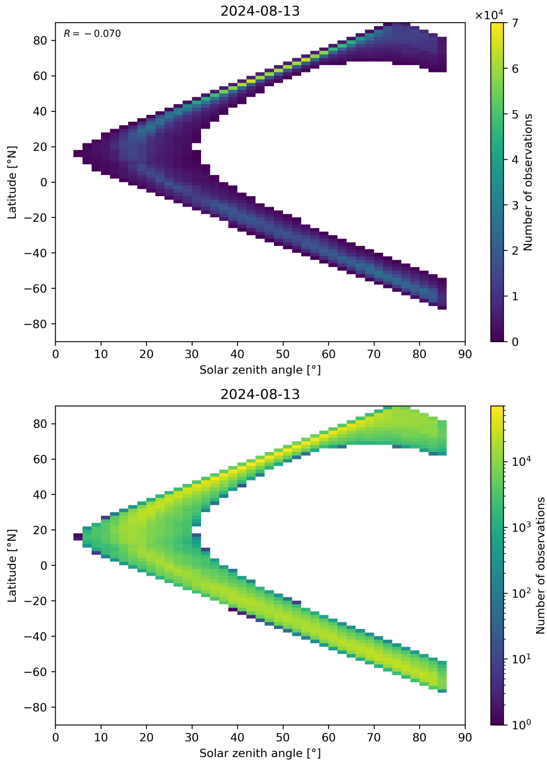
Figure 66: Scatter density plot of “Solar zenith angle” against “Latitude” for 2024-08-12 to 2024-08-14.
