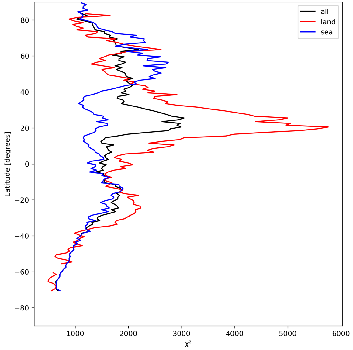
Figure 14: Zonal average of “ \chi^2 ” for 2024-08-12 to 2024-08-14.
