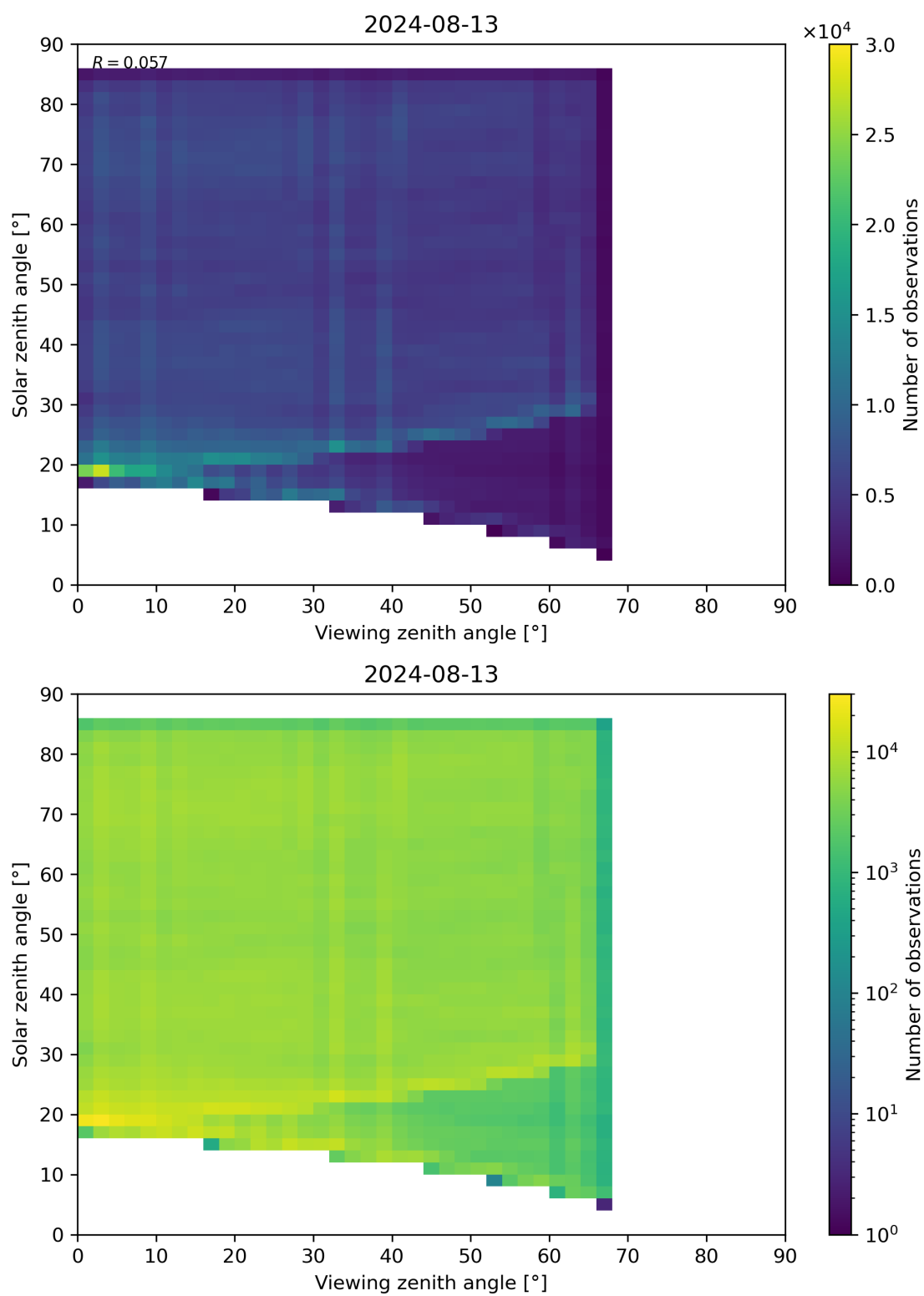
Figure 77: Scatter density plot of “Viewing zenith angle” against “Solar zenith angle” for 2024-08-12 to 2024-08-14.
