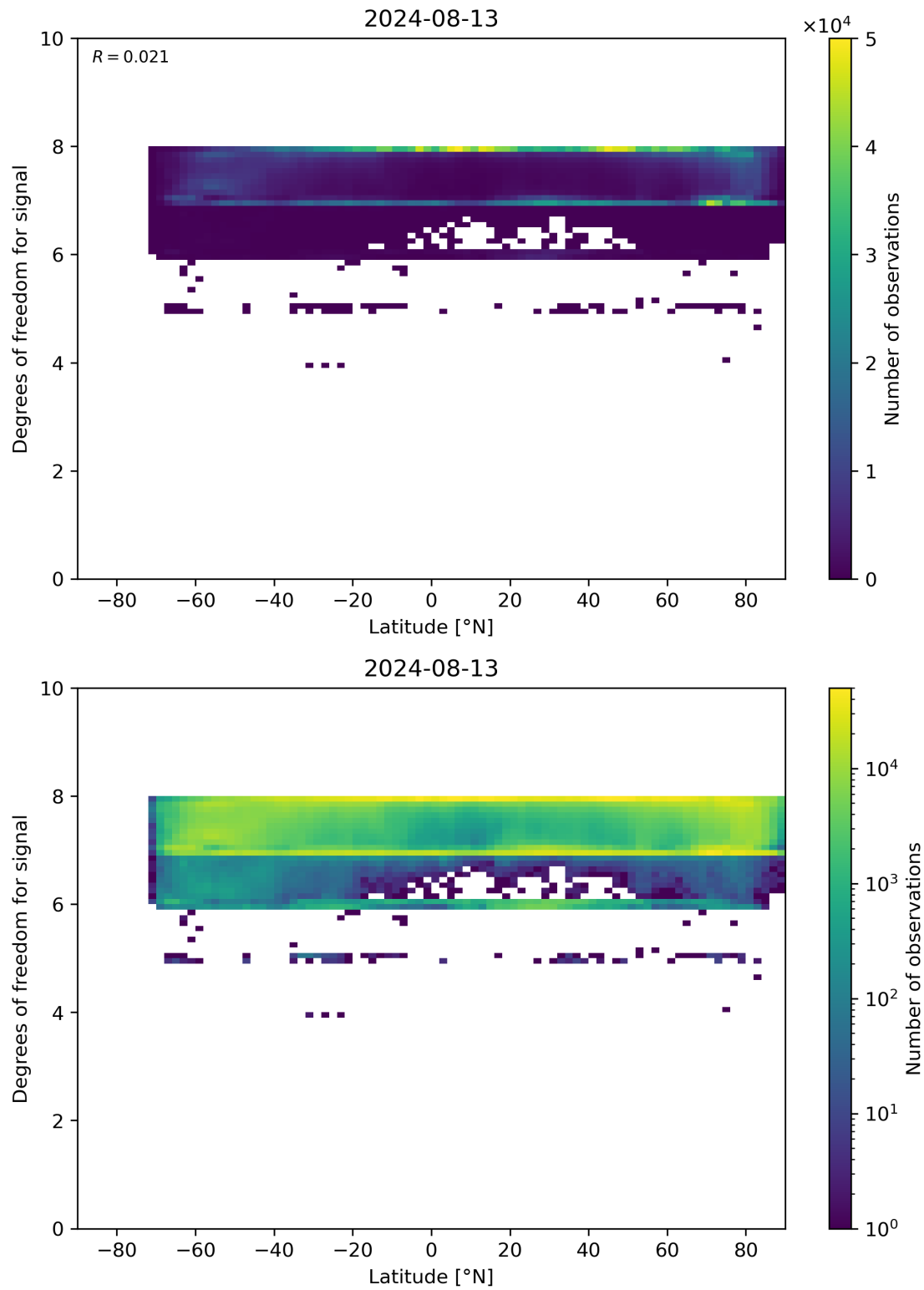
Figure 55: Scatter density plot of “Latitude” against “Degrees of freedom for signal” for 2024-08-12 to 2024-08-14.
