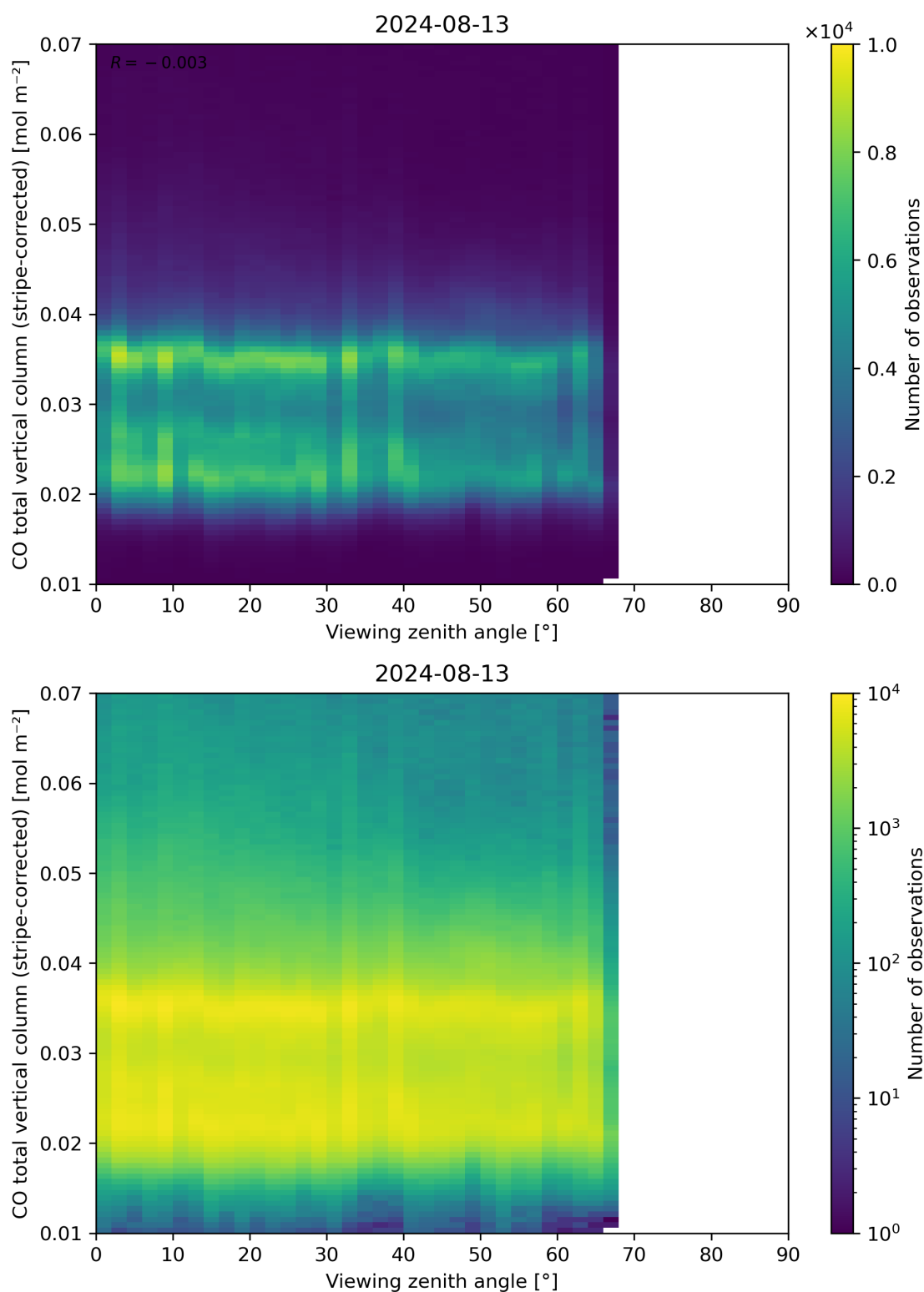
Figure 70: Scatter density plot of “Viewing zenith angle” against “CO total vertical column (stripe-corrected)” for 2024-08-12 to 2024-08-14.
