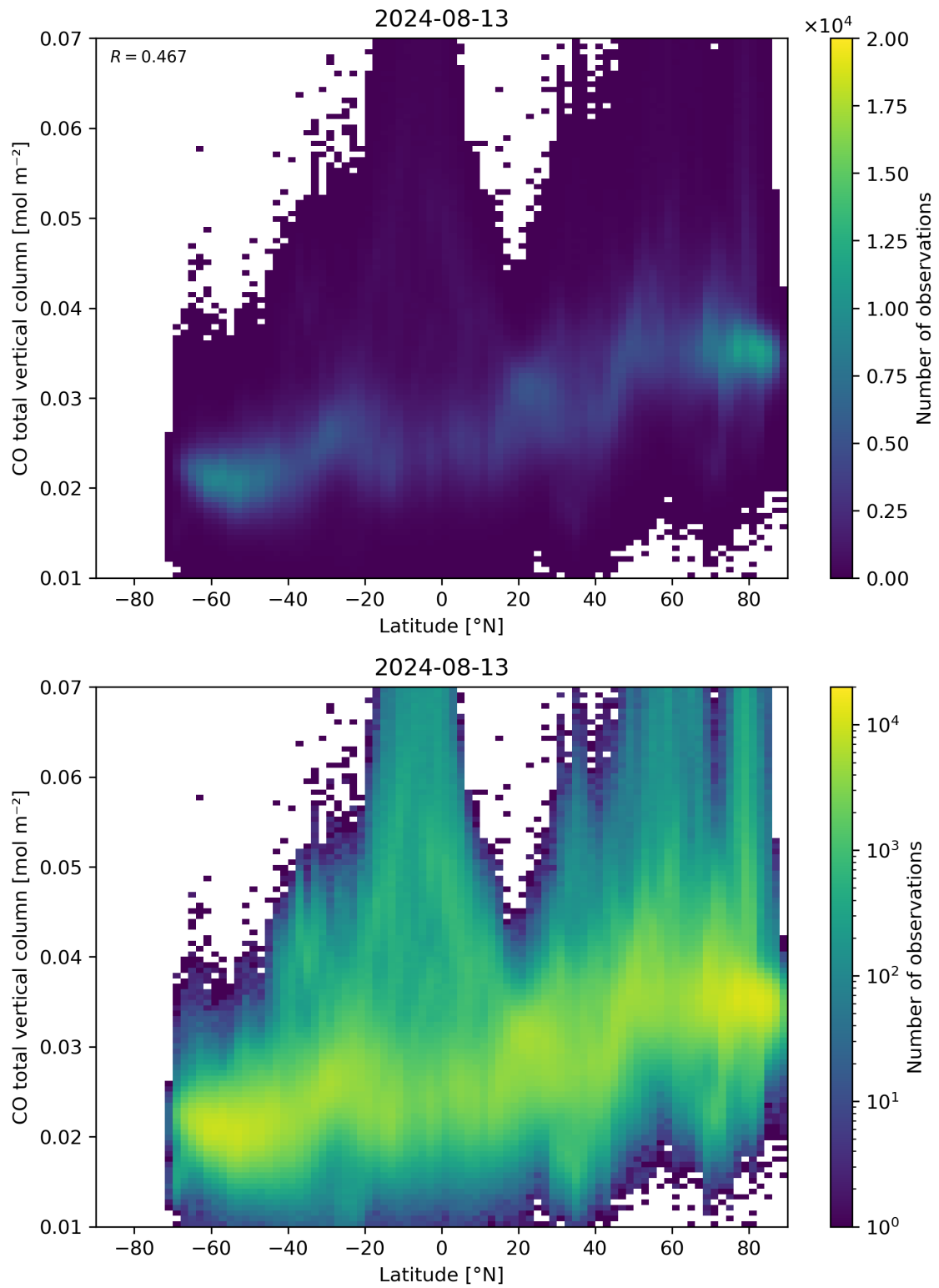
Figure 51: Scatter density plot of “Latitude” against “CO total vertical column” for 2024-08-12 to 2024-08-14.
