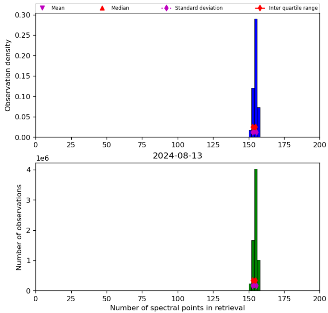
Figure 21: Histogram of “Number of spectral points in retrieval” for 2024-08-12 to 2024-08-14
