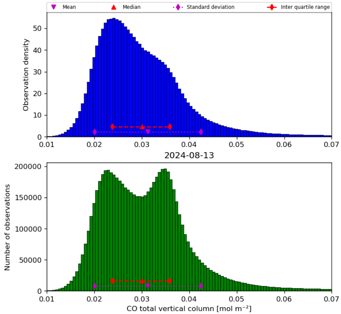
Figure 18: Histogram of “CO total vertical column” for 2024-08-12 to 2024-08-14
