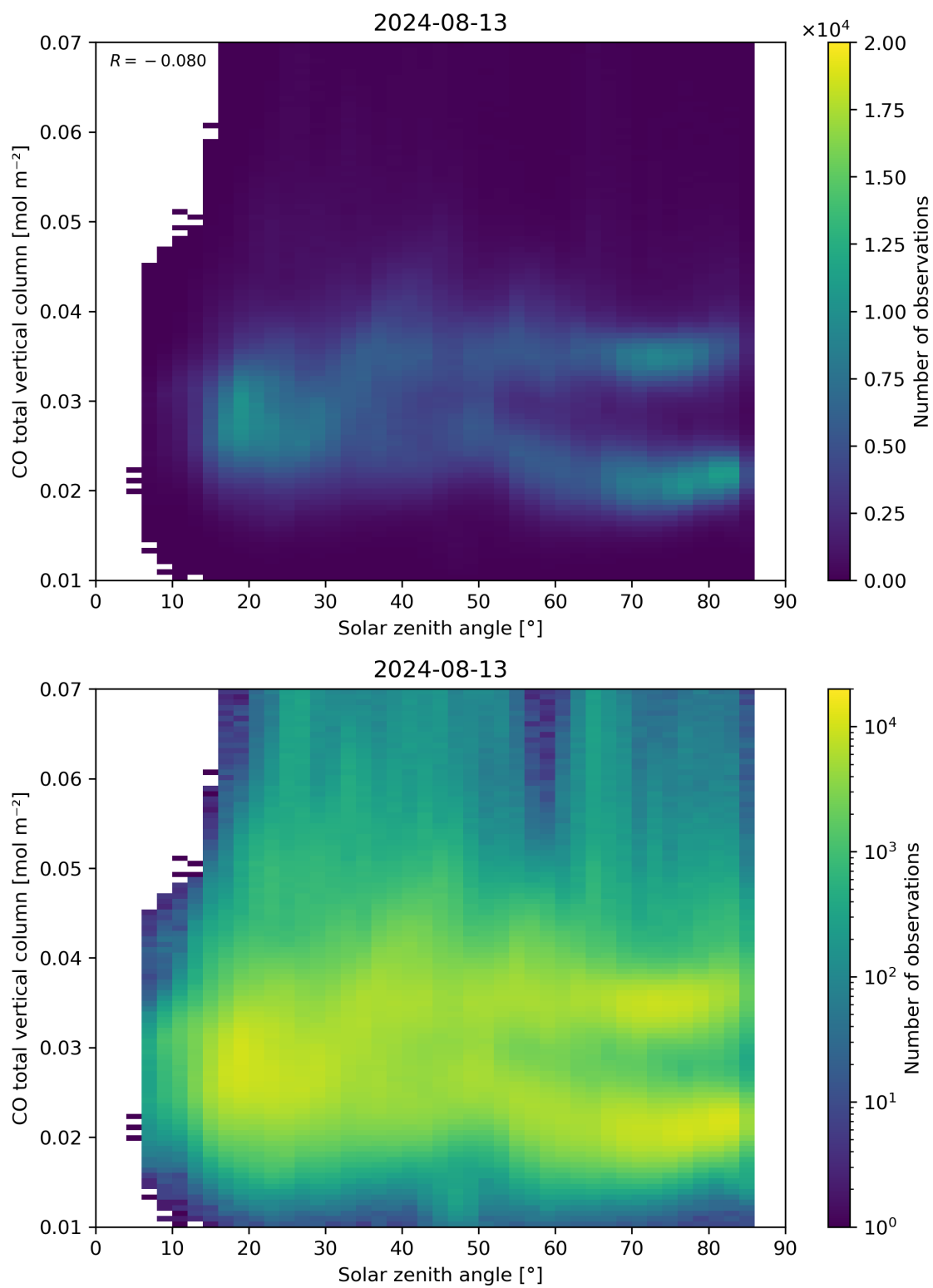
Figure 61: Scatter density plot of “Solar zenith angle” against “CO total vertical column” for 2024-08-12 to 2024-08-14.
