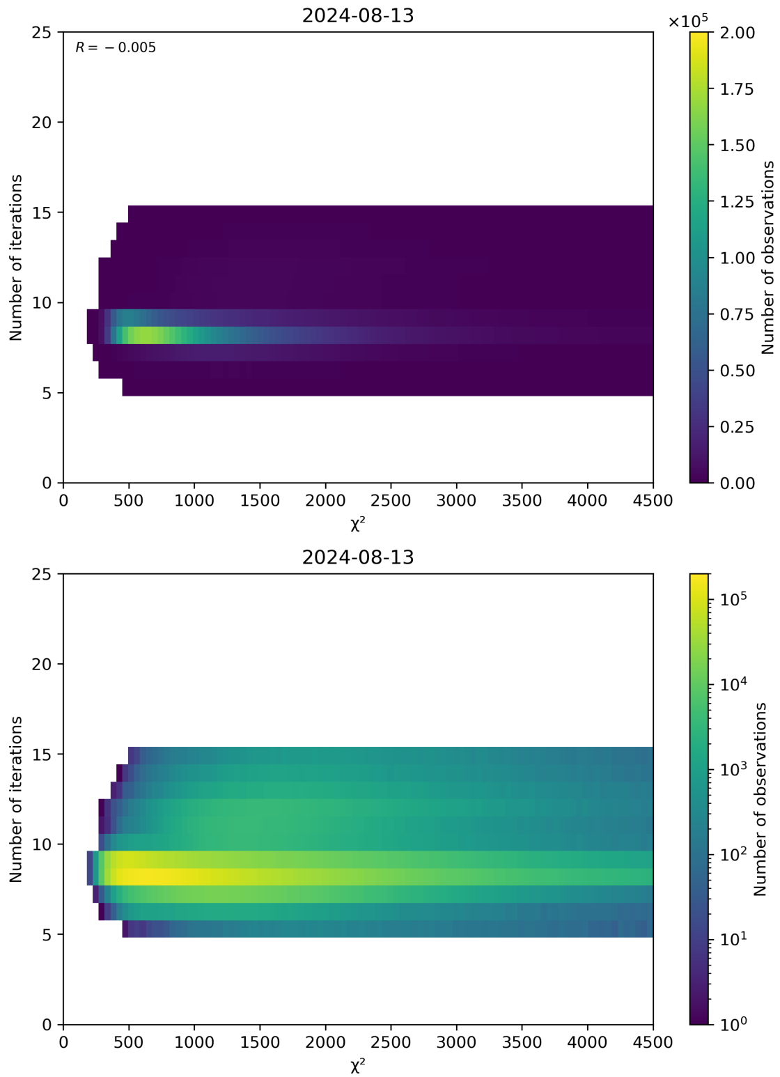
Figure 49: Scatter density plot of “ \chi^2 ” against “Number of iterations” for 2024-08-12 to 2024-08-14.
