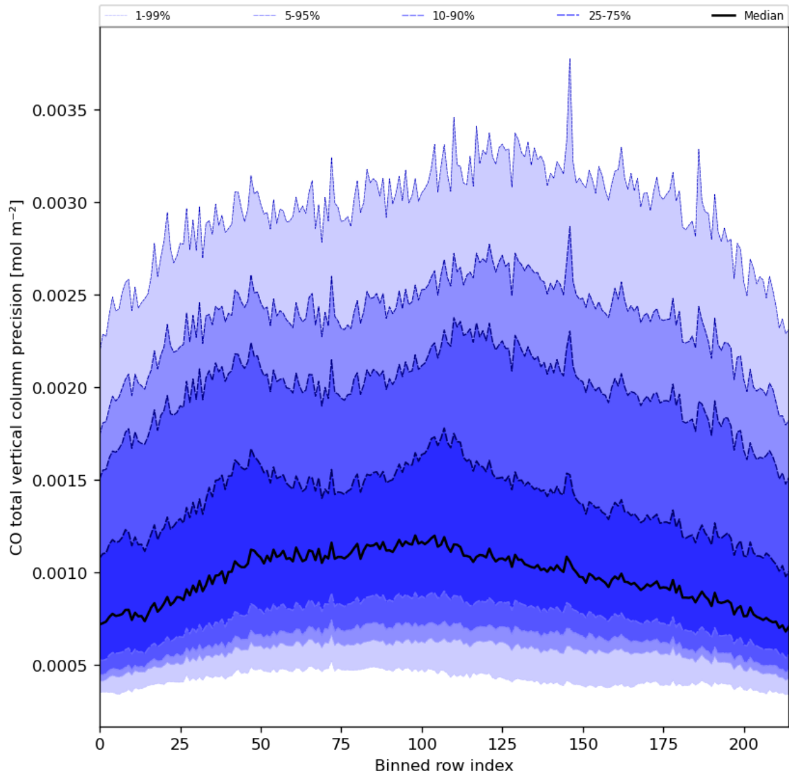
Figure 28: Along track statistics of “CO total vertical column precision” for 2024-08-12 to 2024-08-14
