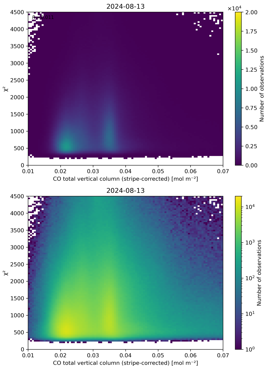
Figure 37: Scatter density plot of “CO total vertical column (stripe-corrected)” against “ \chi^2 ” for 2024-08-12 to 2024-08-14.
