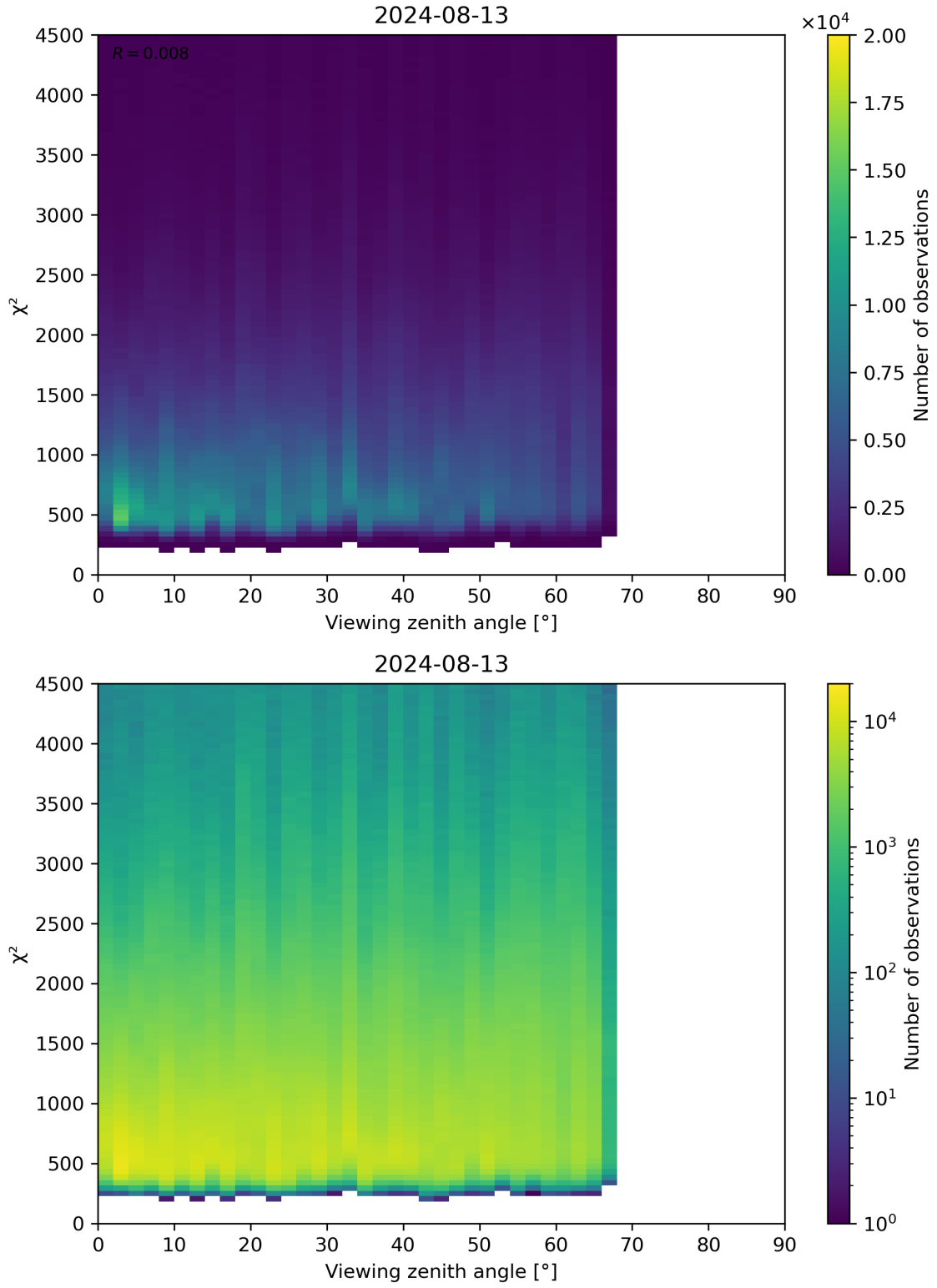
Figure 72: Scatter density plot of “Viewing zenith angle” against “ \chi^2 ” for 2024-08-12 to 2024-08-14.
