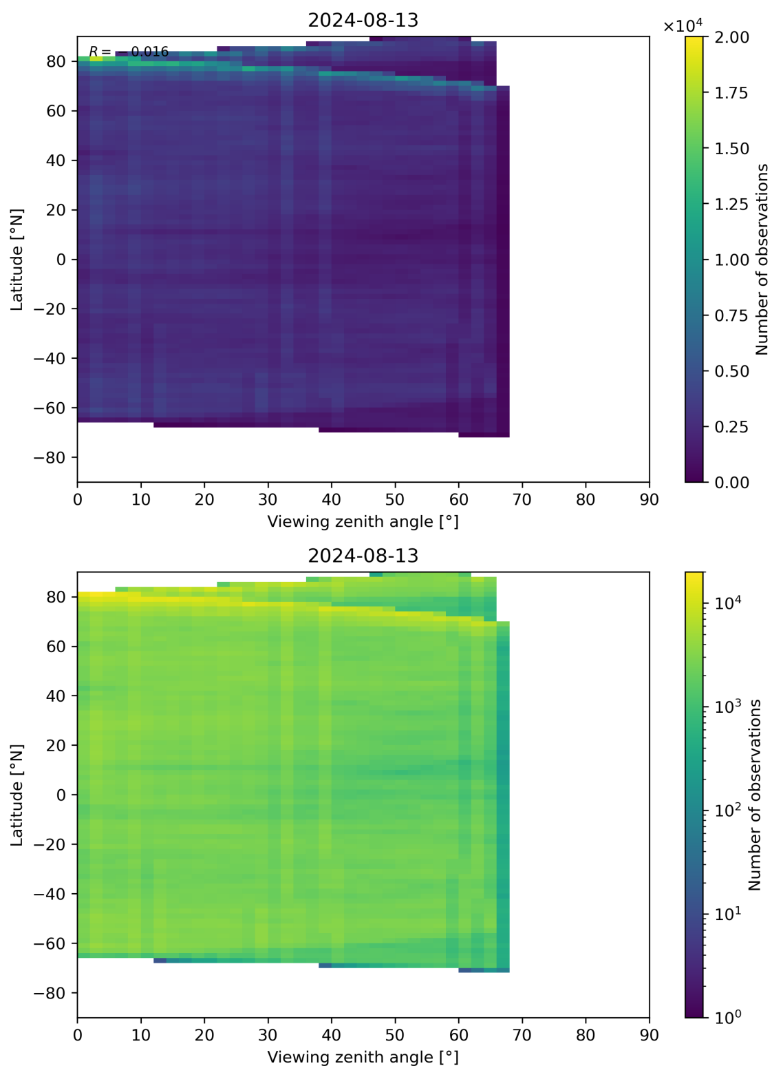
Figure 74: Scatter density plot of “Viewing zenith angle” against “Latitude” for 2024-08-12 to 2024-08-14.
