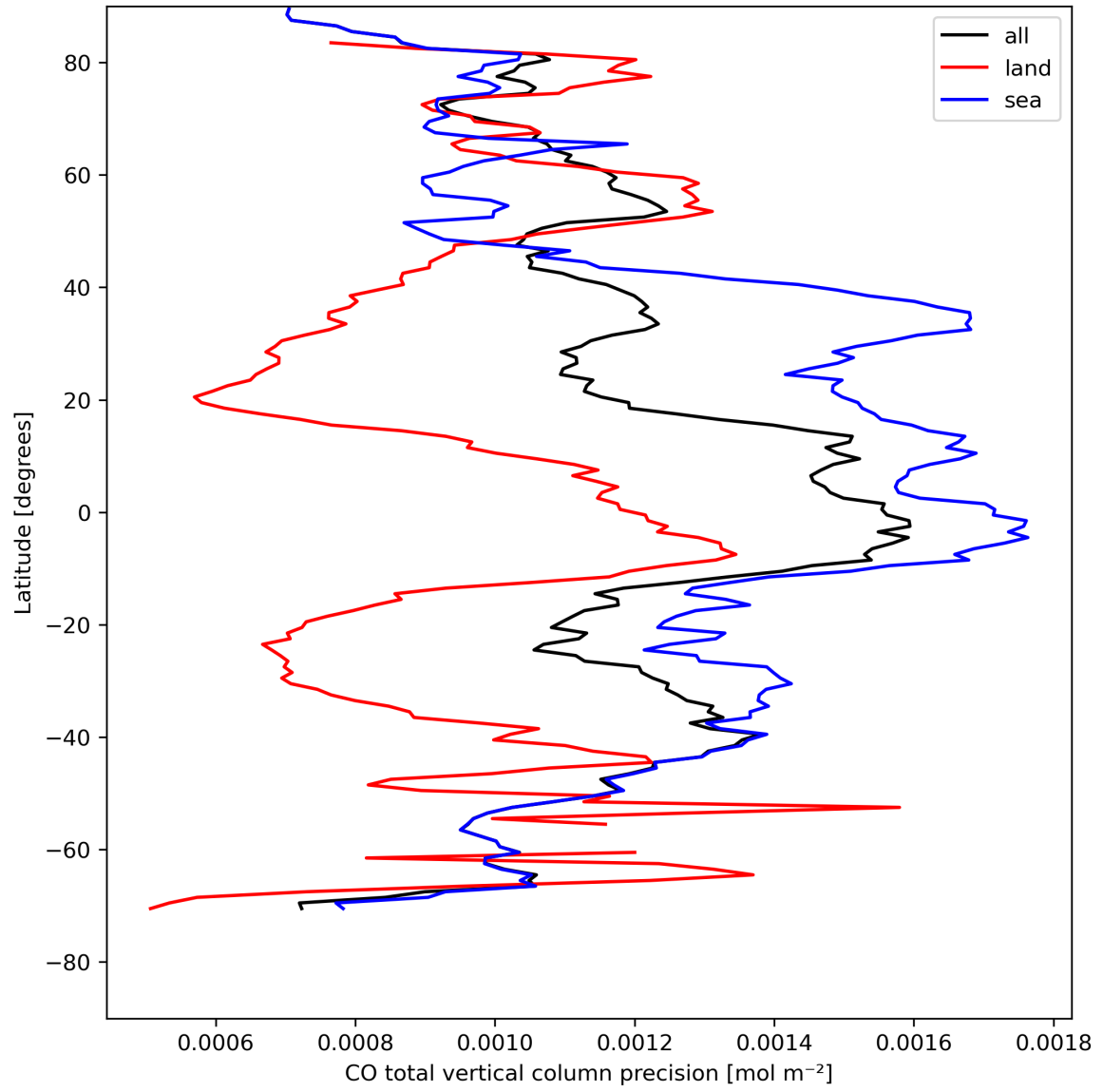
Figure 12: Zonal average of “CO total vertical column precision” for 2024-08-12 to 2024-08-14.
