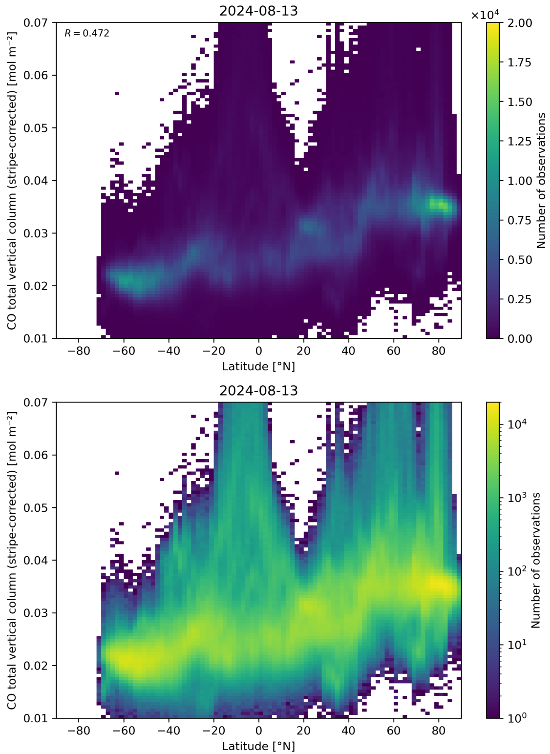
Figure 52: Scatter density plot of “Latitude” against “CO total vertical column (stripe-corrected)” for 2024-08-12 to 2024-08-14.
