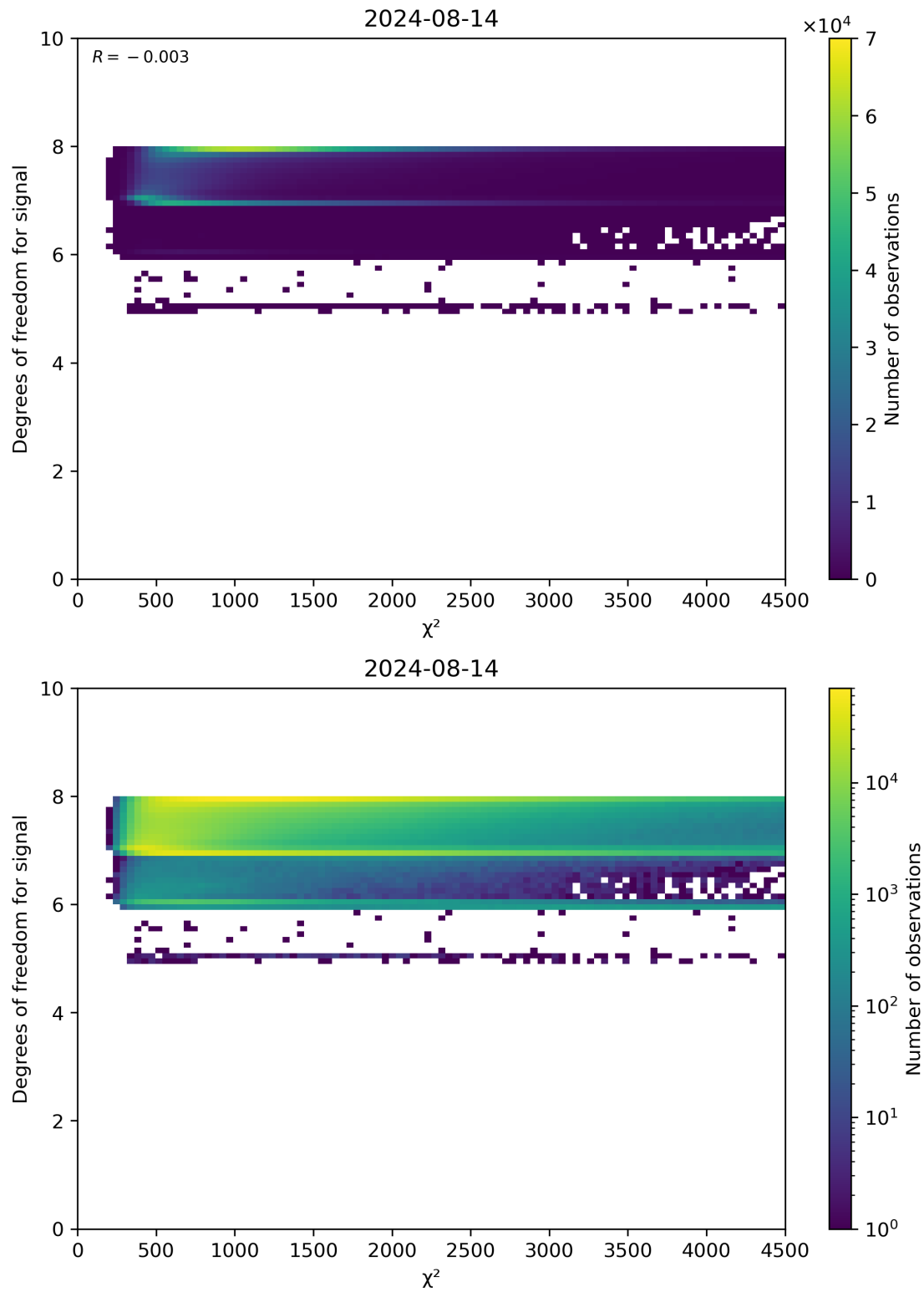
Figure 48: Scatter density plot of “ \chi^2 ” against “Degrees of freedom for signal” for 2024-08-13 to 2024-08-15.
