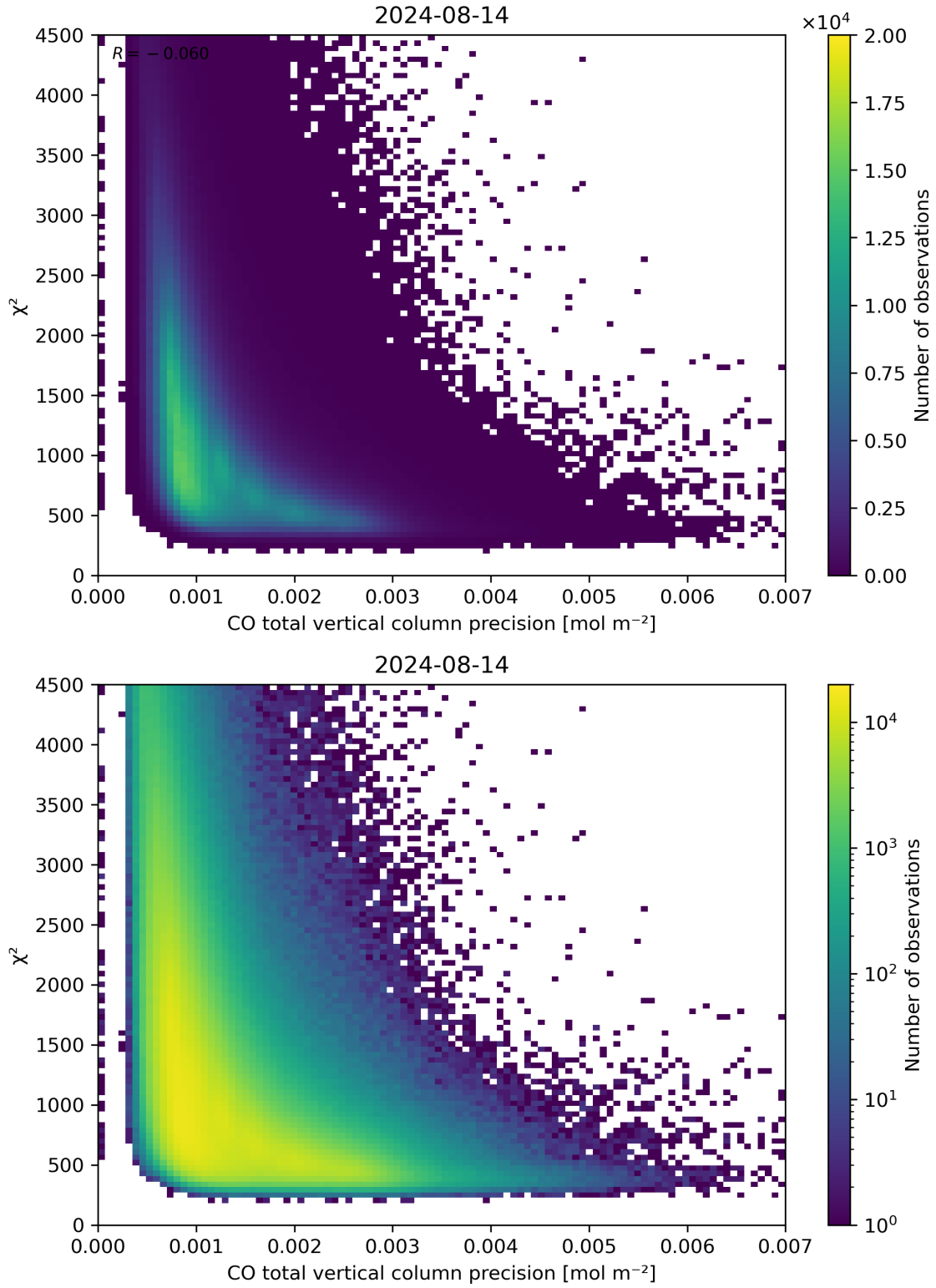
Figure 44: Scatter density plot of “CO total vertical column precision” against “ \chi^2 ” for 2024-08-13 to 2024-08-15.
