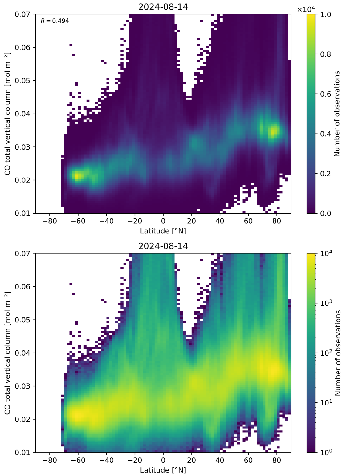
Figure 51: Scatter density plot of “Latitude” against “CO total vertical column” for 2024-08-13 to 2024-08-15.
