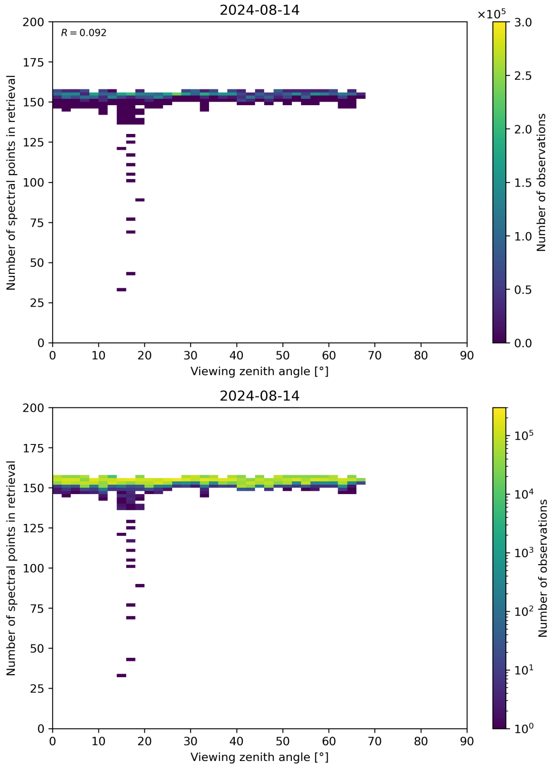
Figure 76: Scatter density plot of “Viewing zenith angle” against “Number of spectral points in retrieval” for 2024-08-13 to 2024-08-15.
