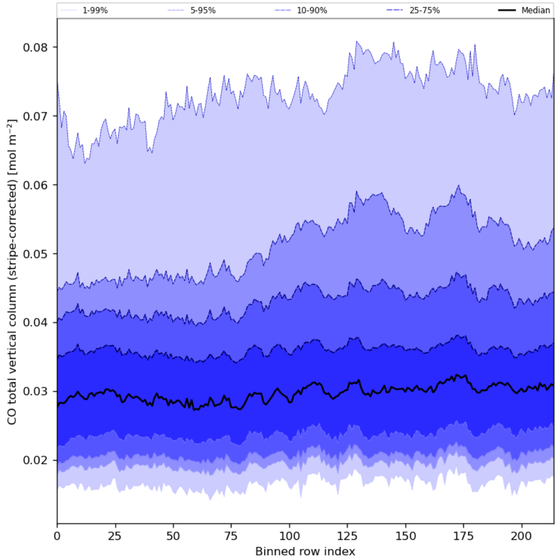
Figure 27: Along track statistics of “CO total vertical column (stripe-corrected)” for 2024-08-13 to 2024-08-15
