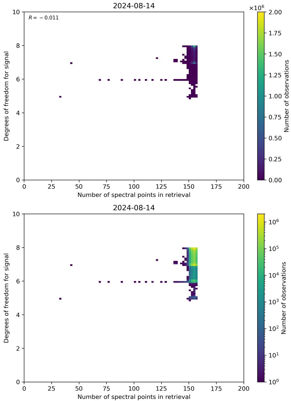
Figure 59: Scatter density plot of “Number of spectral points in retrieval” against “Degrees of freedom for signal” for 2024-08-13 to 2024-08-15.
