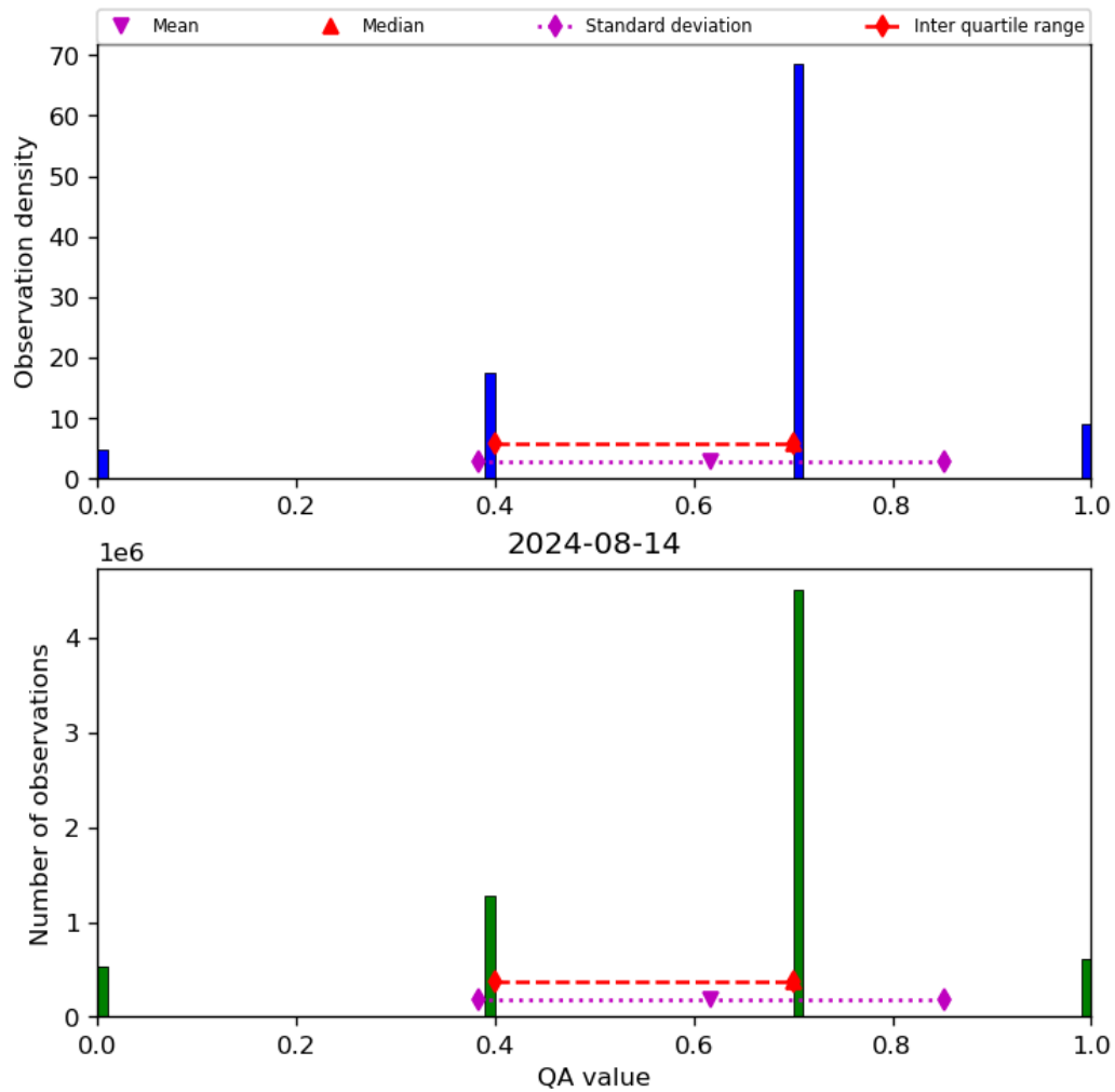
Figure 17: Histogram of “QA value” for 2024-08-13 to 2024-08-15
