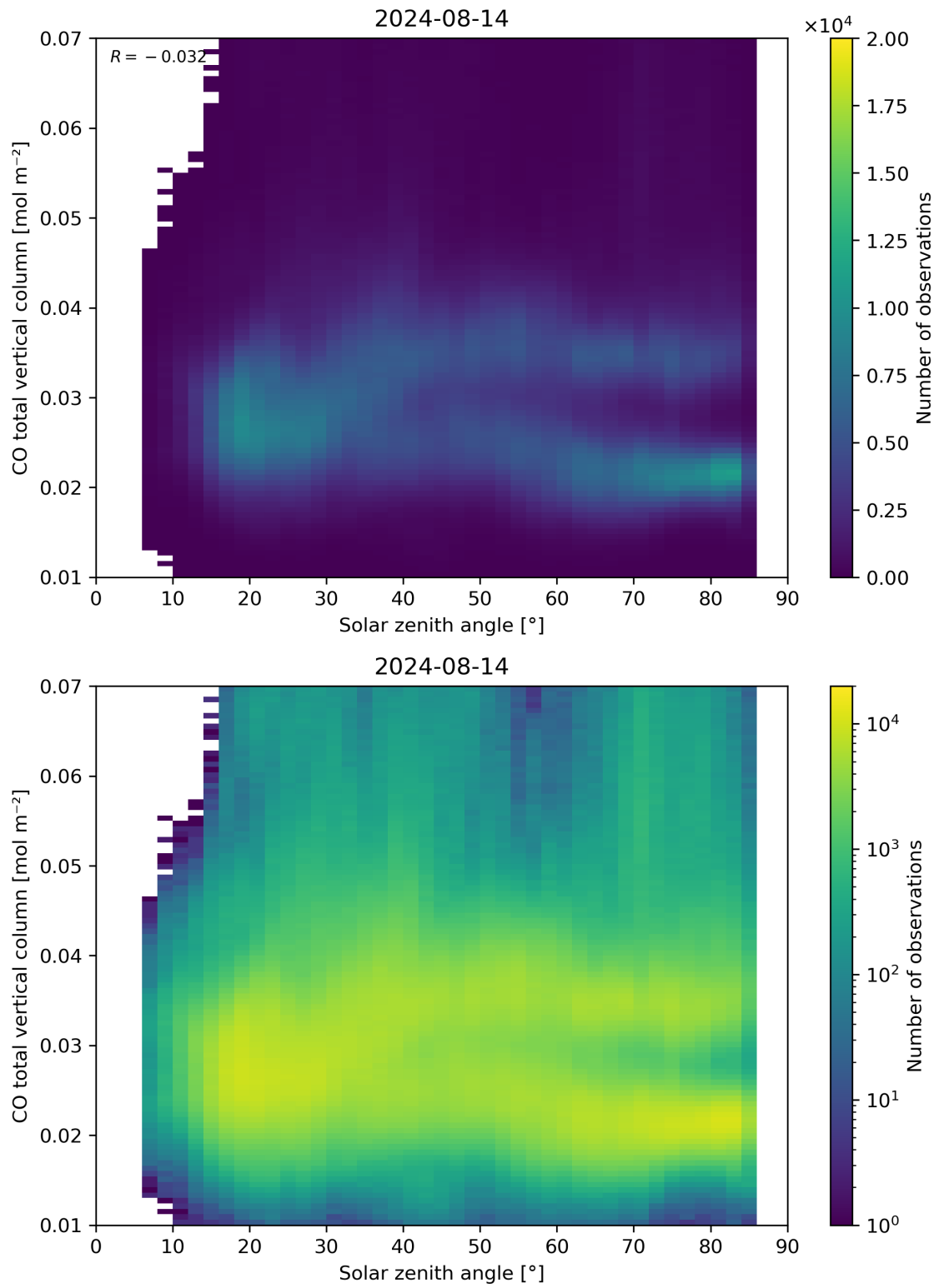
Figure 61: Scatter density plot of “Solar zenith angle” against “CO total vertical column” for 2024-08-13 to 2024-08-15.
