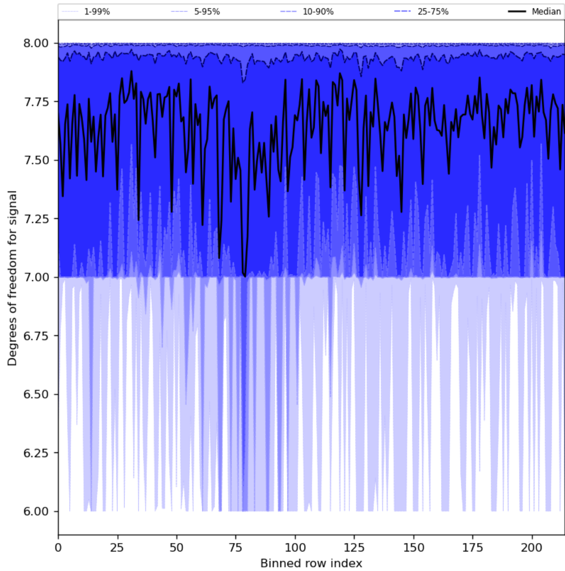
Figure 31: Along track statistics of “Degrees of freedom for signal” for 2024-08-13 to 2024-08-15
