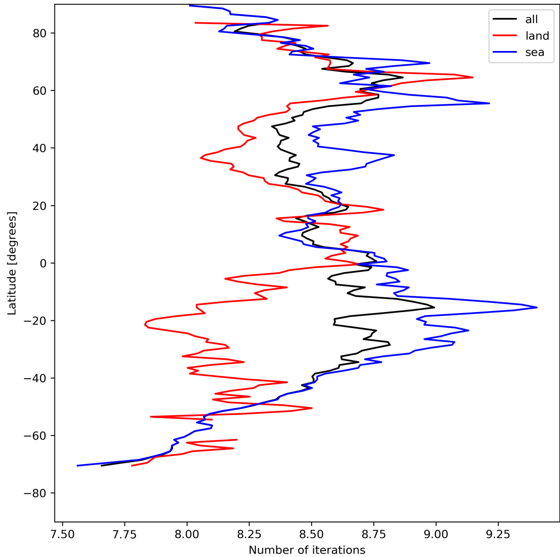
Figure 16: Zonal average of “Number of iterations” for 2024-08-13 to 2024-08-15.
