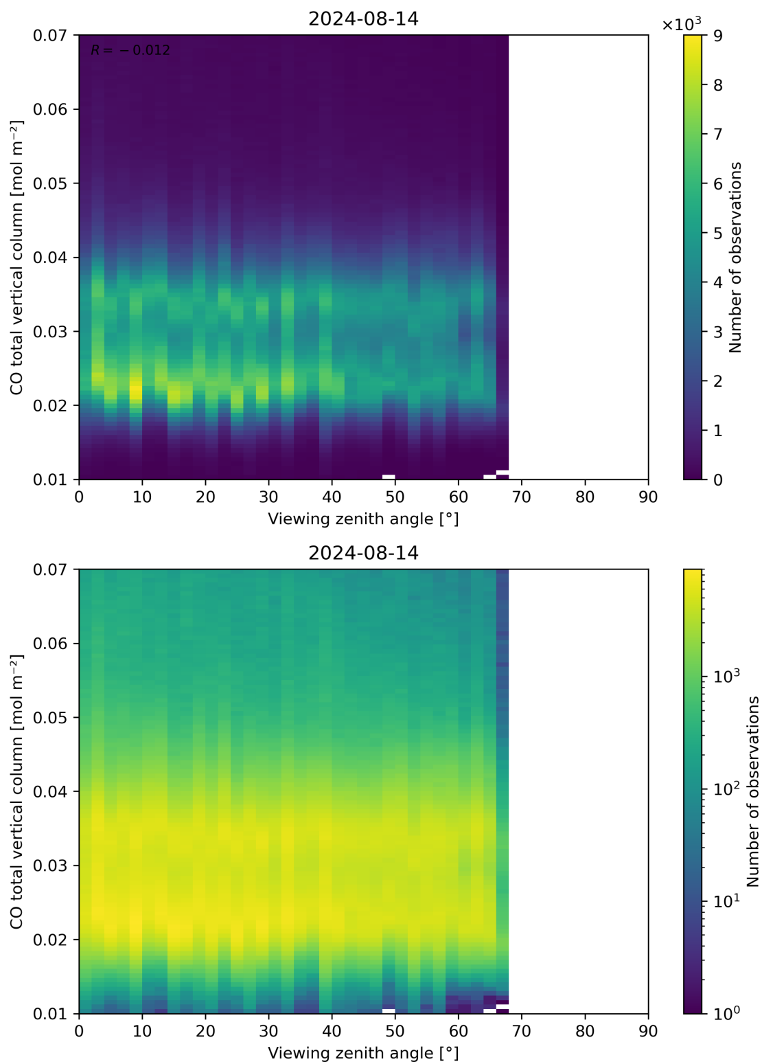
Figure 69: Scatter density plot of “Viewing zenith angle” against “CO total vertical column” for 2024-08-13 to 2024-08-15.
