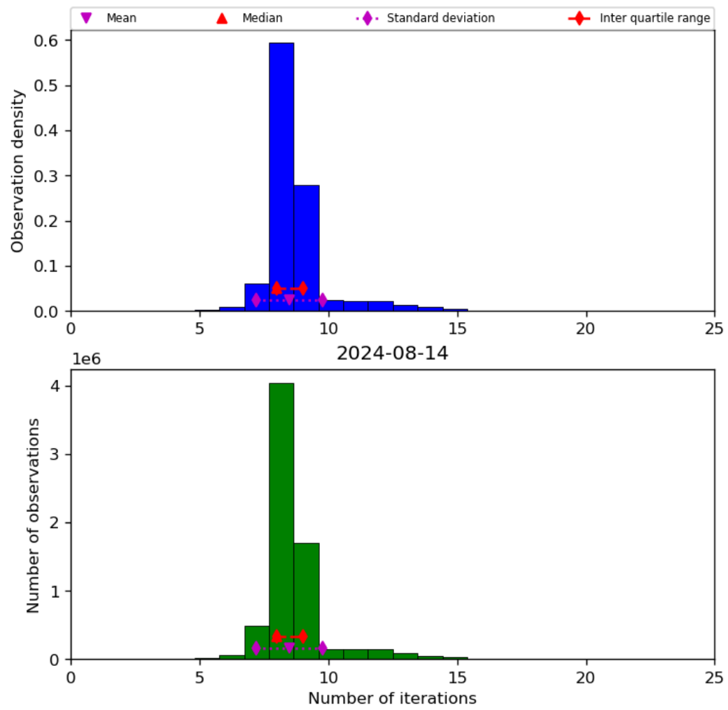
Figure 24: Histogram of “Number of iterations” for 2024-08-13 to 2024-08-15
