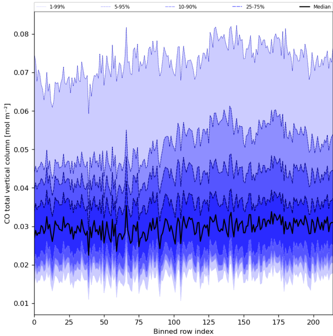
Figure 26: Along track statistics of “CO total vertical column” for 2024-08-13 to 2024-08-15
