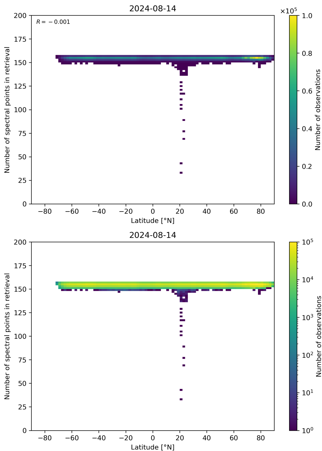
Figure 57: Scatter density plot of “Latitude” against “Number of spectral points in retrieval” for 2024-08-13 to 2024-08-15.
