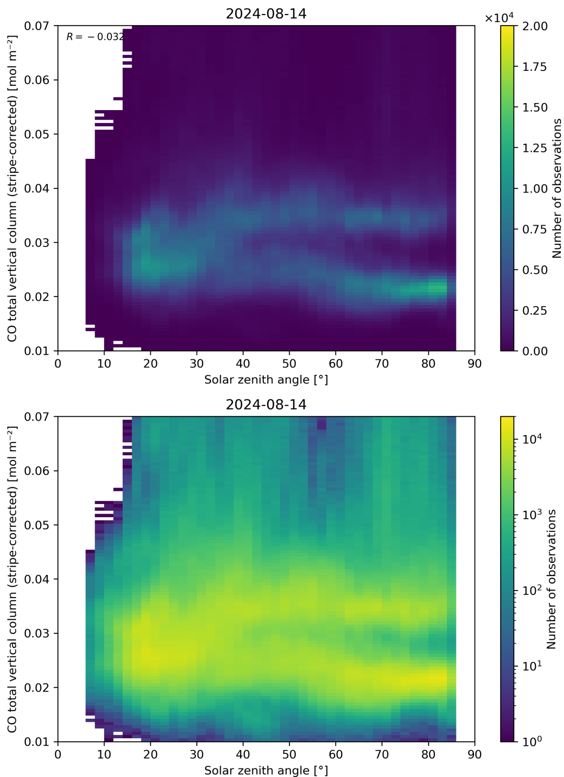
Figure 62: Scatter density plot of “Solar zenith angle” against “CO total vertical column (stripe-corrected)” for 2024-08-13 to 2024-08-15.
