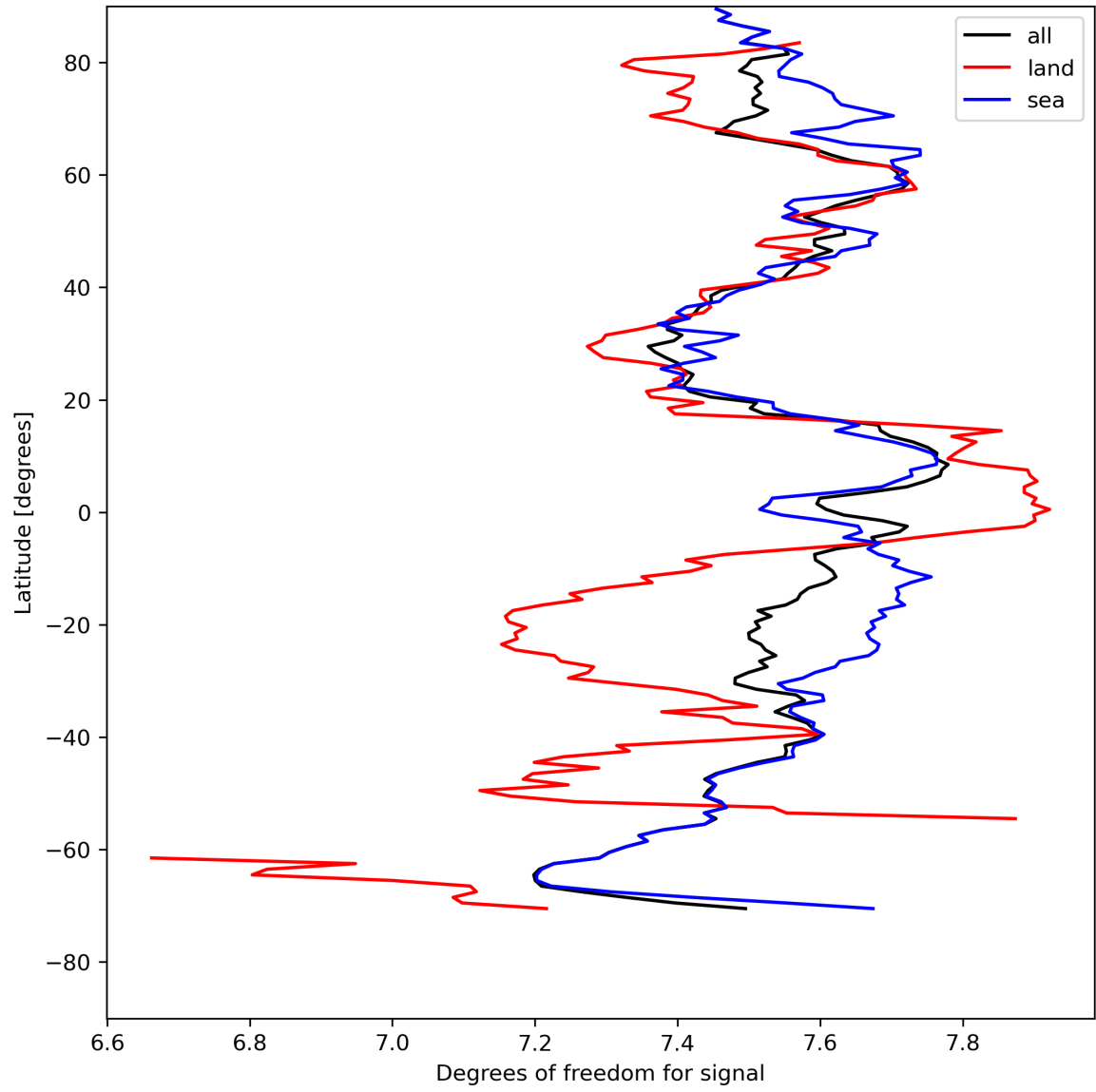
Figure 15: Zonal average of “Degrees of freedom for signal” for 2024-08-13 to 2024-08-15.
