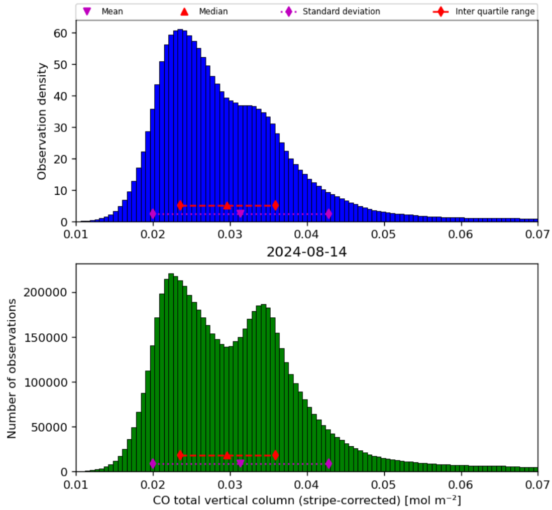
Figure 19: Histogram of “CO total vertical column (stripe-corrected)” for 2024-08-13 to 2024-08-15
