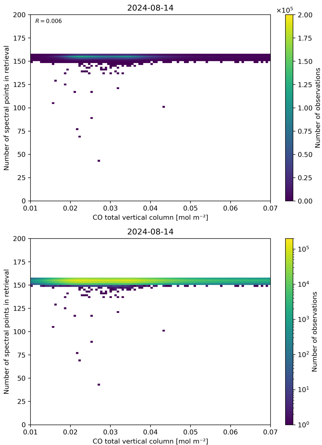
Figure 43: Scatter density plot of “CO total vertical column” against “Number of spectral points in retrieval” for 2024-08-13 to 2024-08-15.
