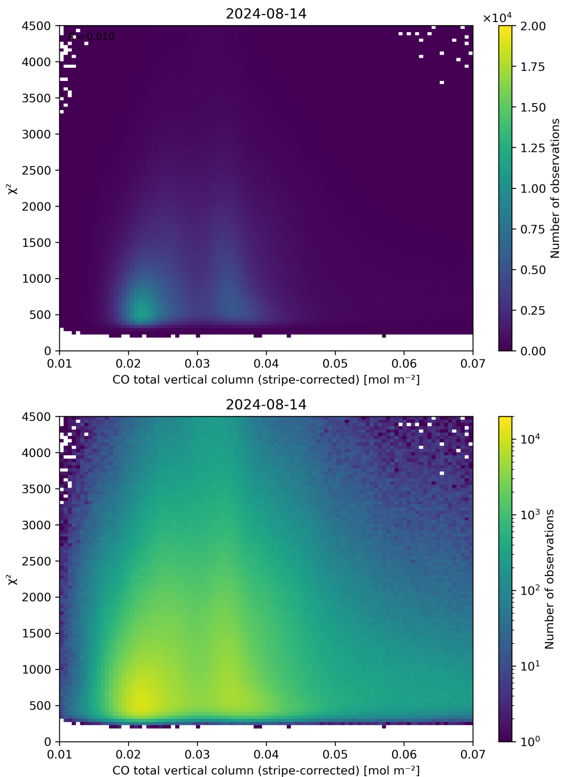
Figure 37: Scatter density plot of “CO total vertical column (stripe-corrected)” against “ \chi^2 ” for 2024-08-13 to 2024-08-15.
