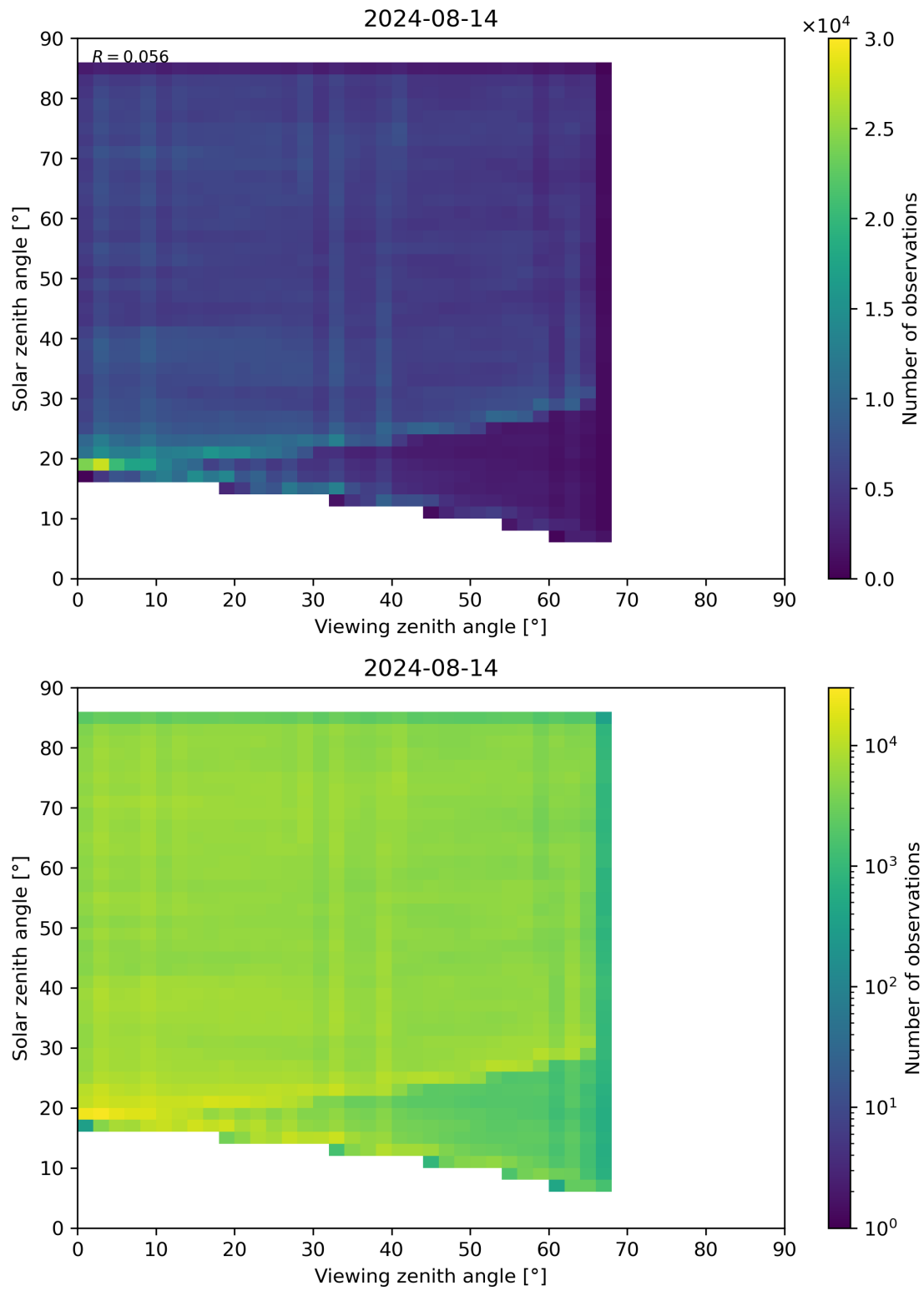
Figure 77: Scatter density plot of “Viewing zenith angle” against “Solar zenith angle” for 2024-08-13 to 2024-08-15.
