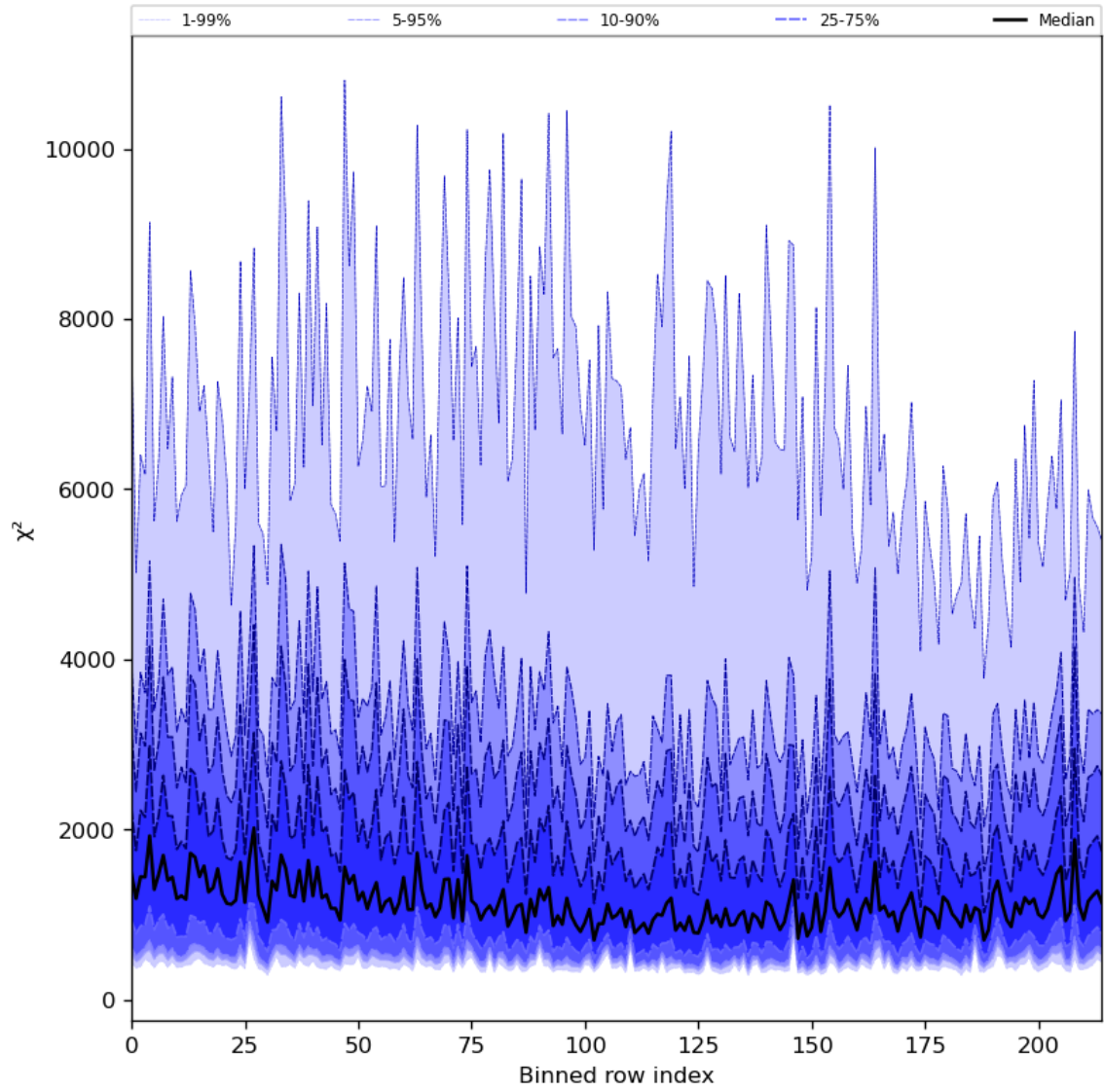
Figure 30: Along track statistics of “ \chi^2 ” for 2024-08-13 to 2024-08-15
