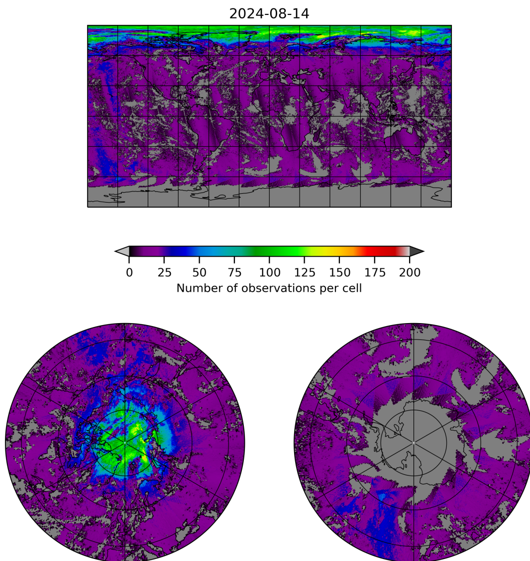
Figure 8: Map of the number of observations for 2024-08-13 to 2024-08-15
