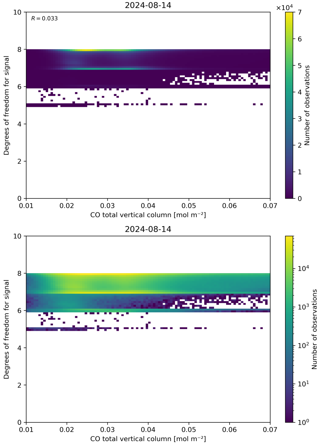
Figure 41: Scatter density plot of “CO total vertical column” against “Degrees of freedom for signal” for 2024-08-13 to 2024-08-15.
