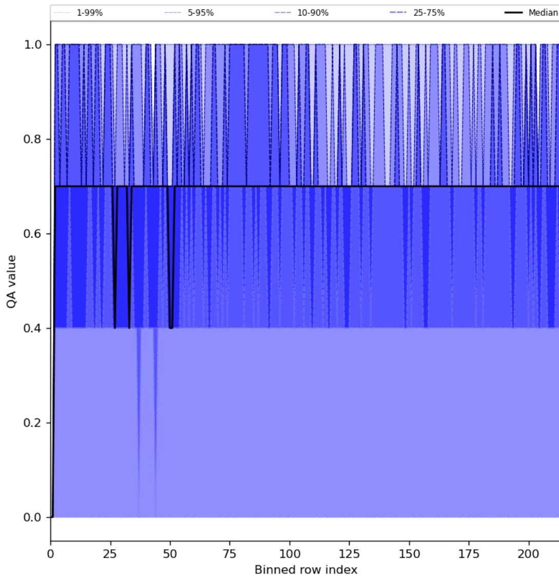
Figure 25: Along track statistics of “QA value” for 2024-08-13 to 2024-08-15
