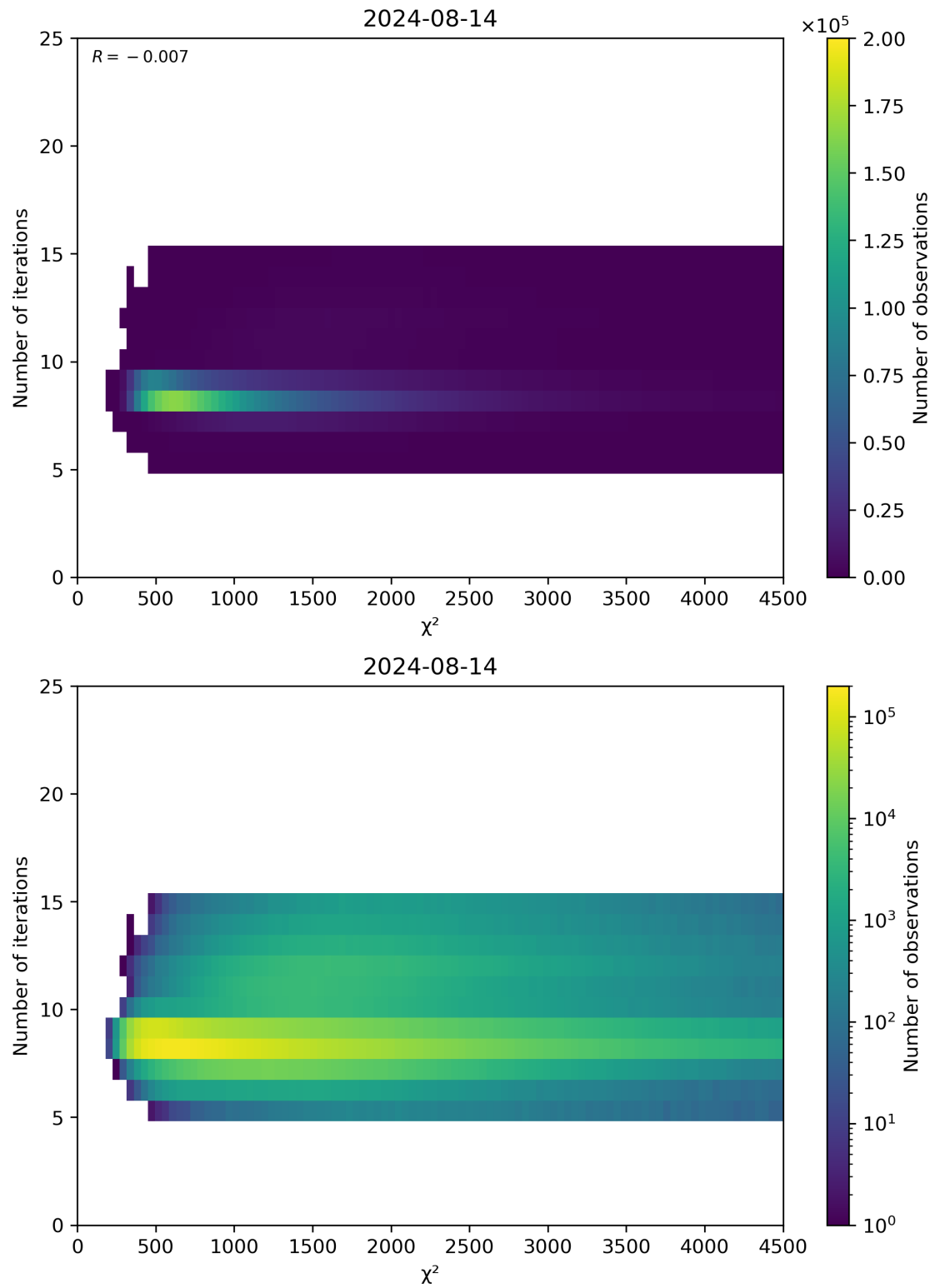
Figure 49: Scatter density plot of “ \chi^2 ” against “Number of iterations” for 2024-08-13 to 2024-08-15.
