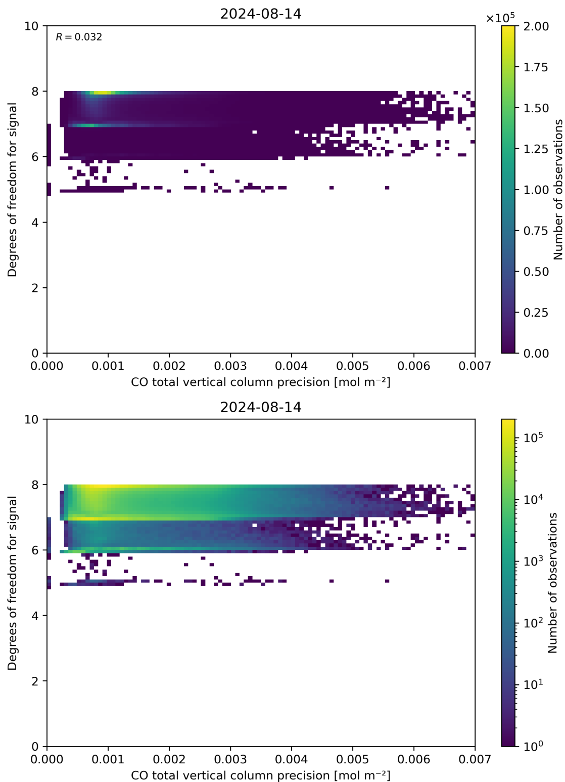
Figure 45: Scatter density plot of “CO total vertical column precision” against “Degrees of freedom for signal” for 2024-08-13 to 2024-08-15.
