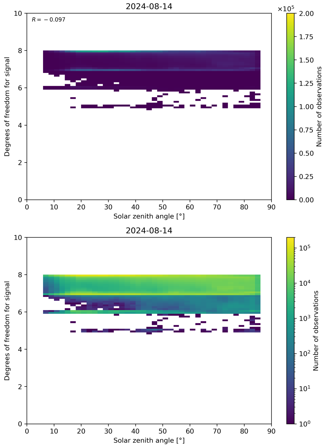
Figure 65: Scatter density plot of “Solar zenith angle” against “Degrees of freedom for signal” for 2024-08-13 to 2024-08-15.
