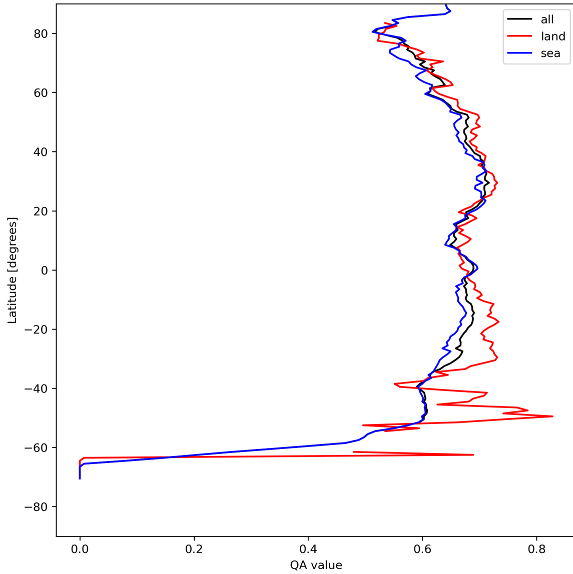
Figure 9: Zonal average of “QA value” for 2024-08-13 to 2024-08-15.
