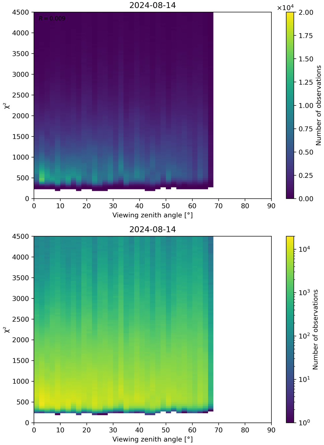
Figure 72: Scatter density plot of “Viewing zenith angle” against “ \chi^2 ” for 2024-08-13 to 2024-08-15.
