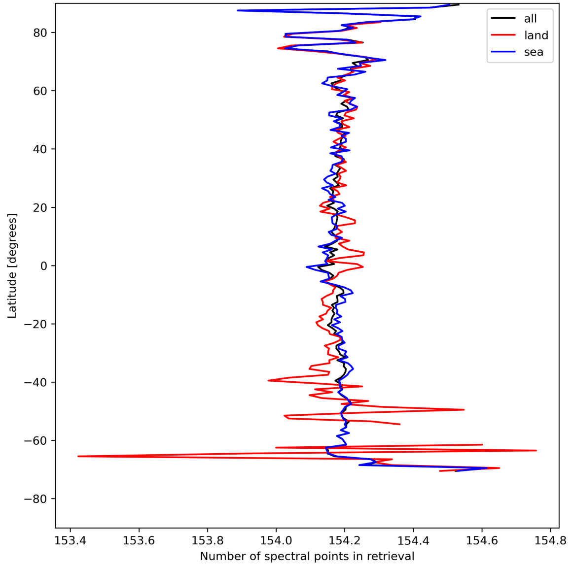
Figure 13: Zonal average of “Number of spectral points in retrieval” for 2024-08-13 to 2024-08-15.
