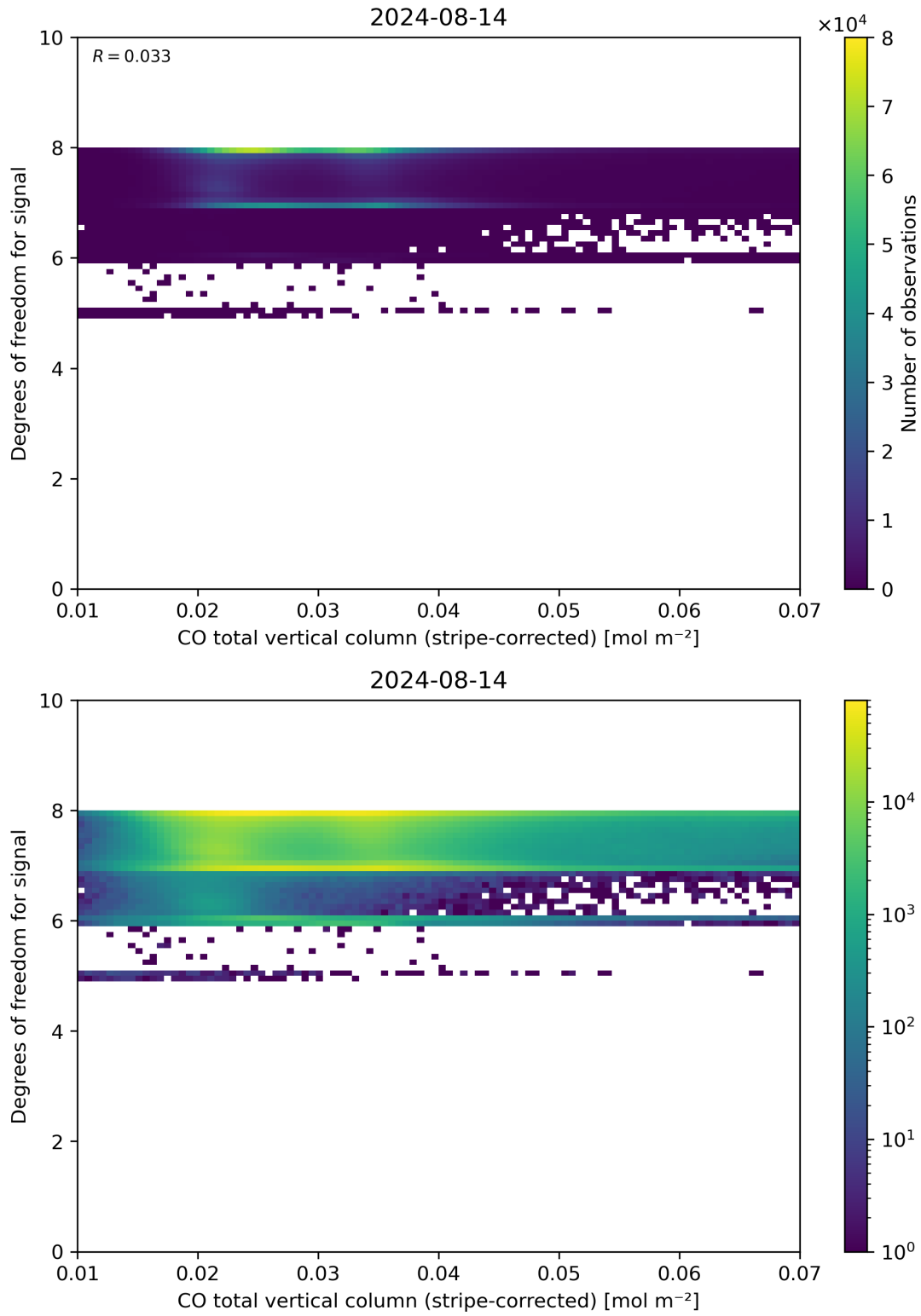
Figure 38: Scatter density plot of “CO total vertical column (stripe-corrected)” against “Degrees of freedom for signal” for 2024-08-13 to 2024-08-15.
