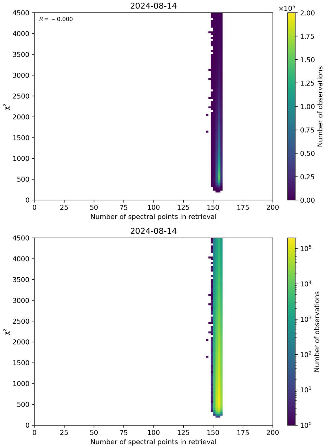
Figure 58: Scatter density plot of “Number of spectral points in retrieval” against “ \chi^2 ” for 2024-08-13 to 2024-08-15.
