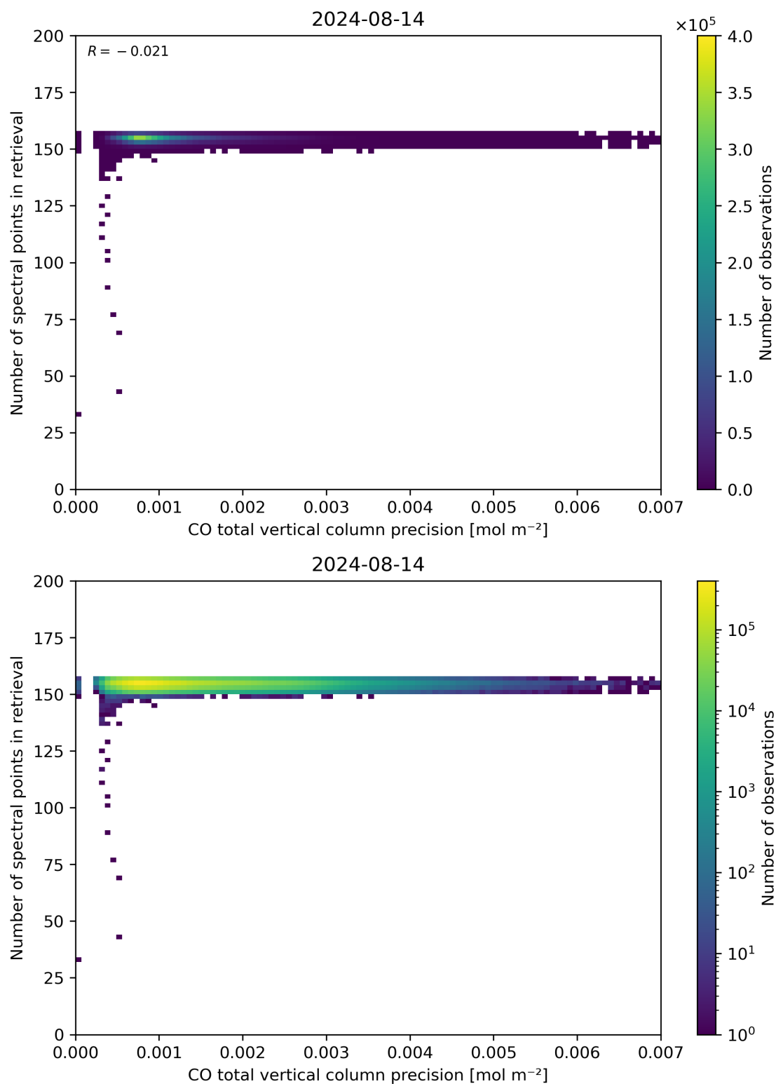
Figure 47: Scatter density plot of “CO total vertical column precision” against “Number of spectral points in retrieval” for 2024-08-13 to 2024-08-15.
