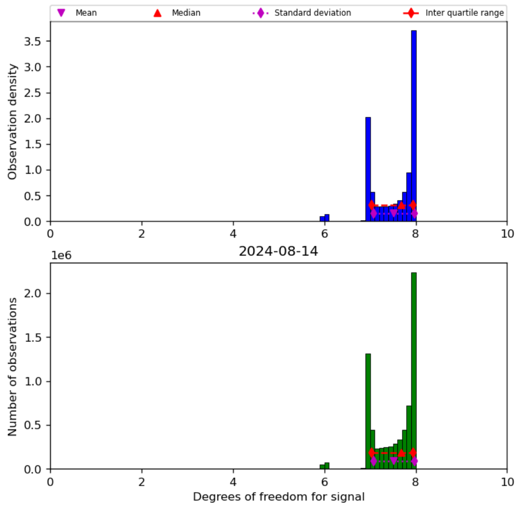
Figure 23: Histogram of “Degrees of freedom for signal” for 2024-08-13 to 2024-08-15
