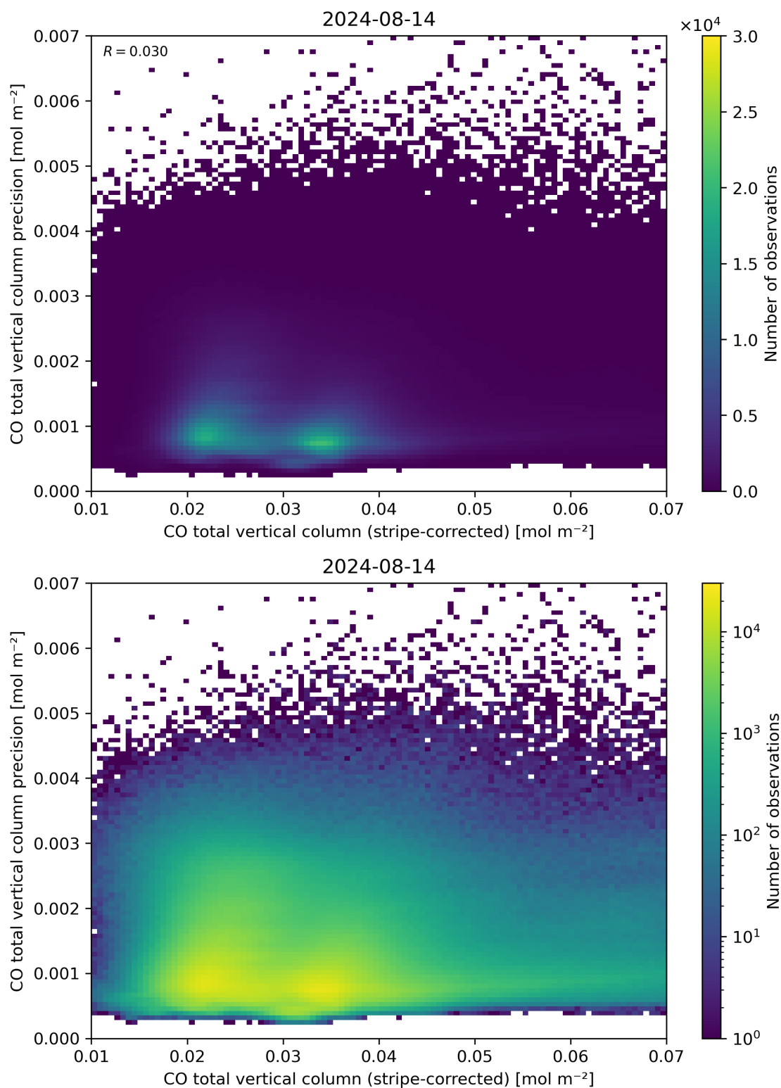
Figure 36: Scatter density plot of “CO total vertical column (stripe-corrected)” against “CO total vertical column precision” for 2024-08-13 to 2024-08-15.
