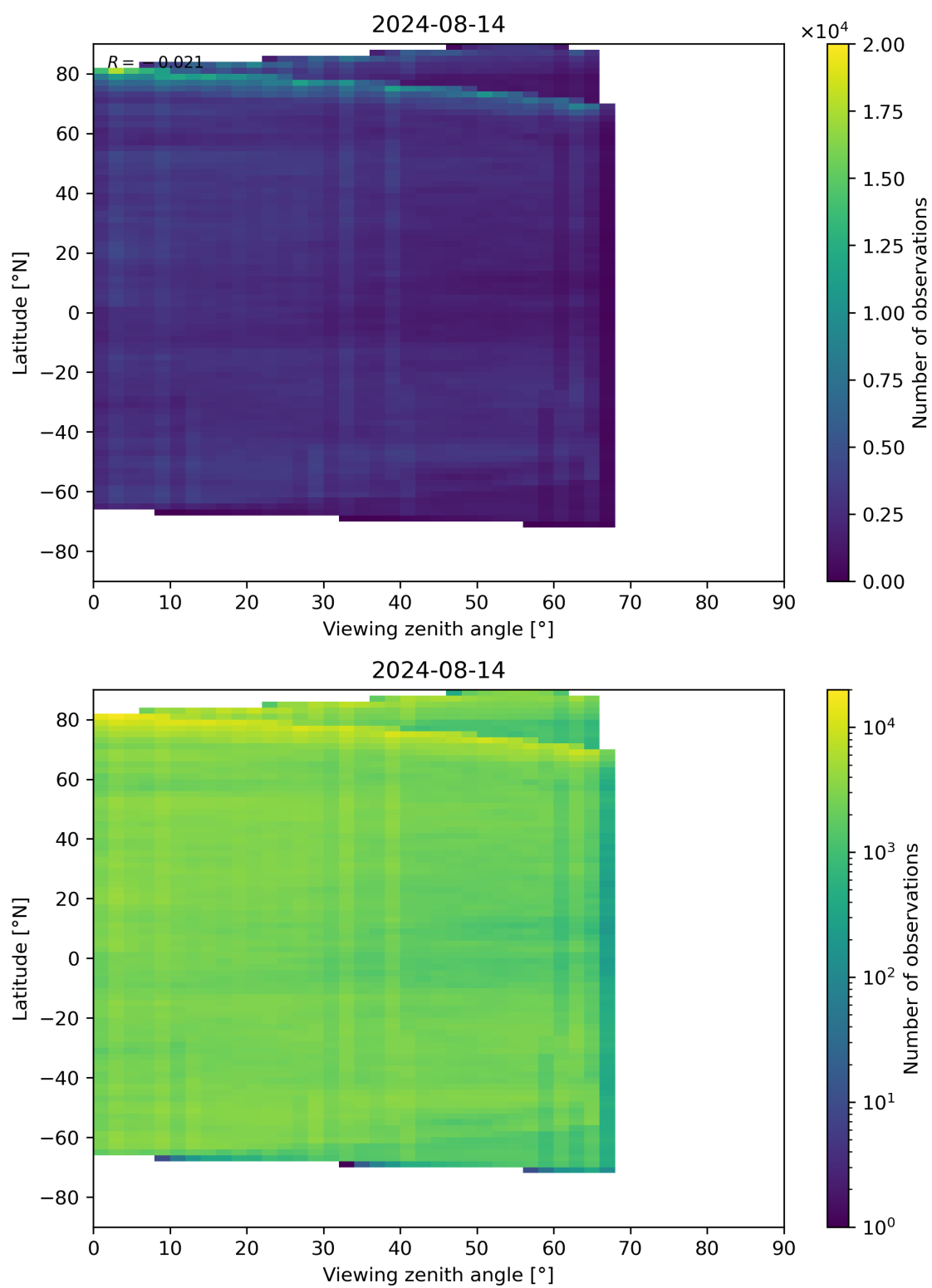
Figure 74: Scatter density plot of “Viewing zenith angle” against “Latitude” for 2024-08-13 to 2024-08-15.
