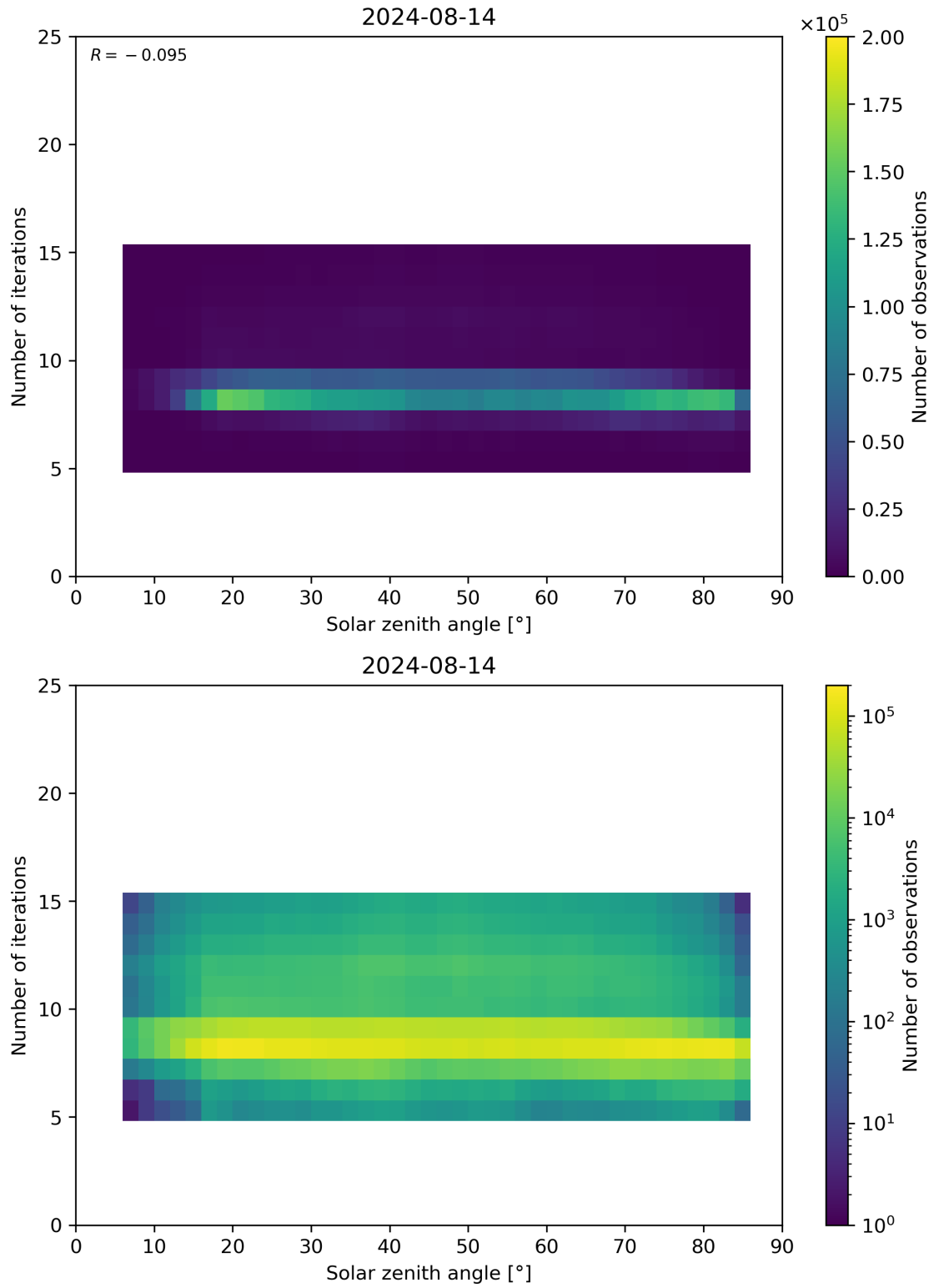
Figure 67: Scatter density plot of “Solar zenith angle” against “Number of iterations” for 2024-08-13 to 2024-08-15.
