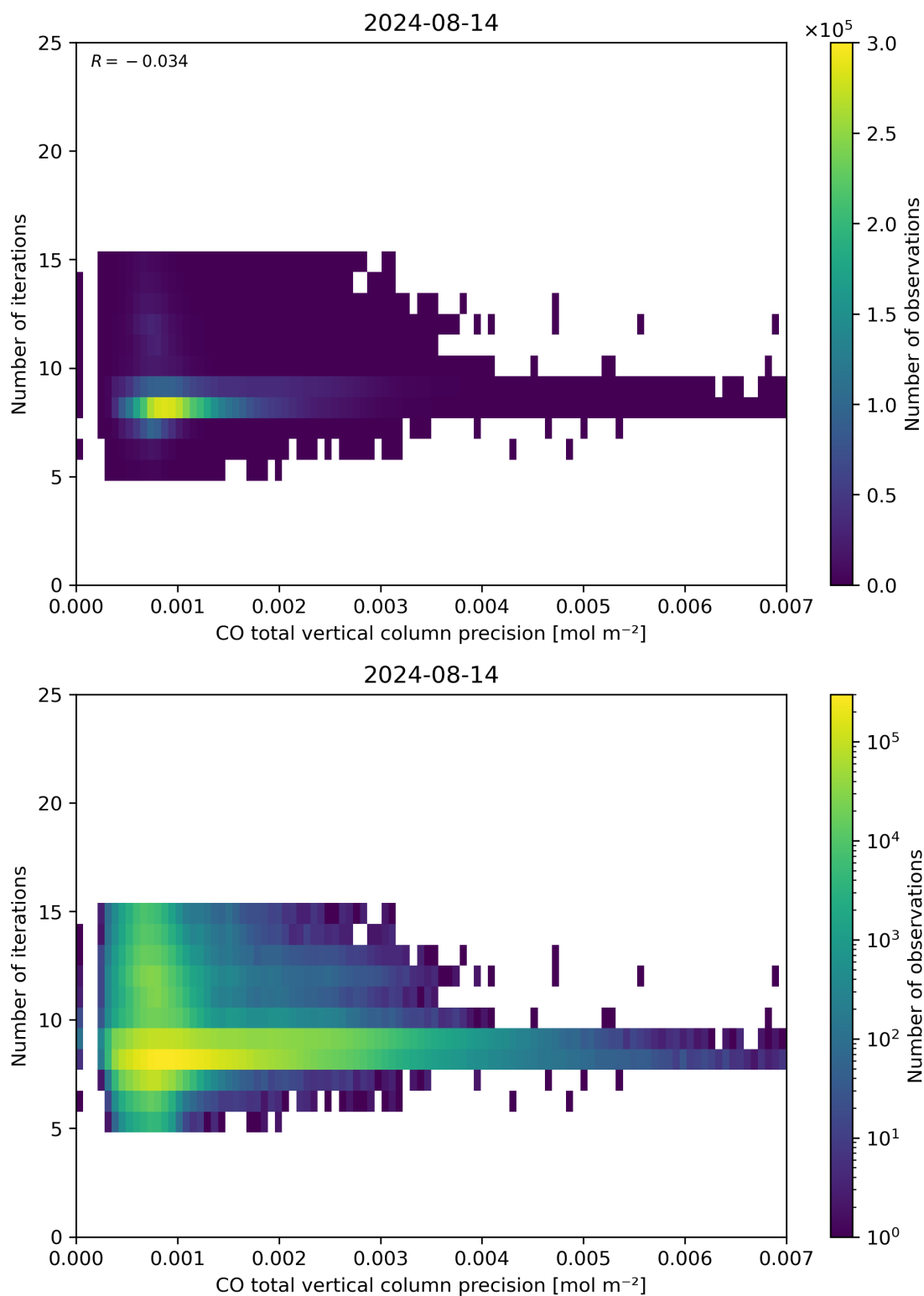
Figure 46: Scatter density plot of “CO total vertical column precision” against “Number of iterations” for 2024-08-13 to 2024-08-15.
