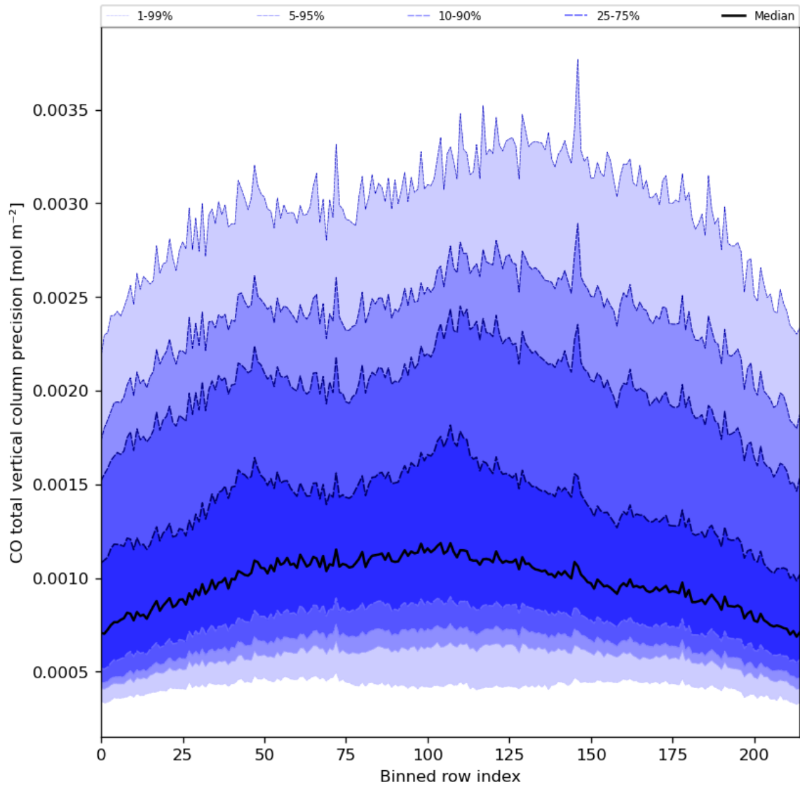
Figure 28: Along track statistics of “CO total vertical column precision” for 2024-08-13 to 2024-08-15
