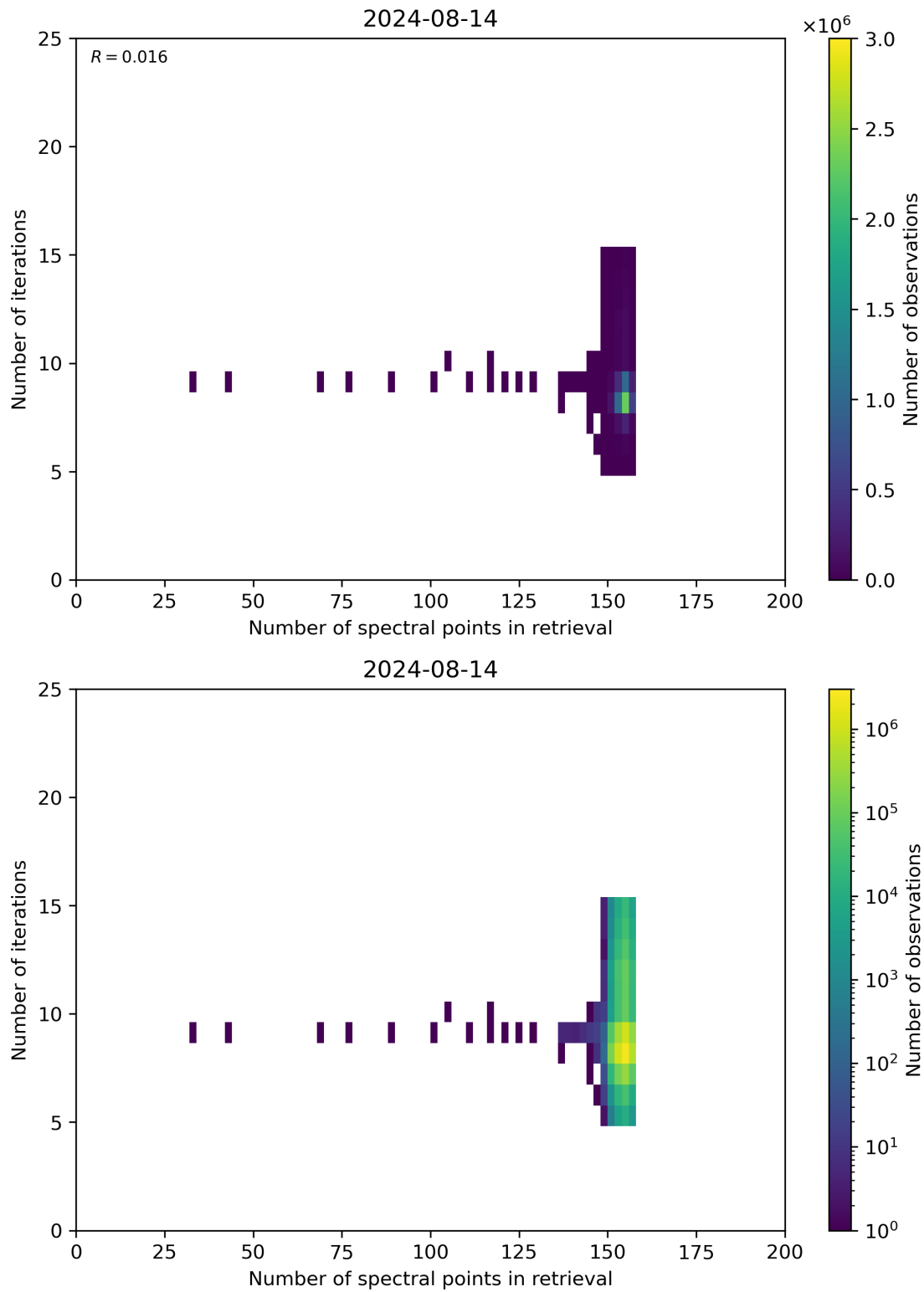
Figure 60: Scatter density plot of “Number of spectral points in retrieval” against “Number of iterations” for 2024-08-13 to 2024-08-15.
