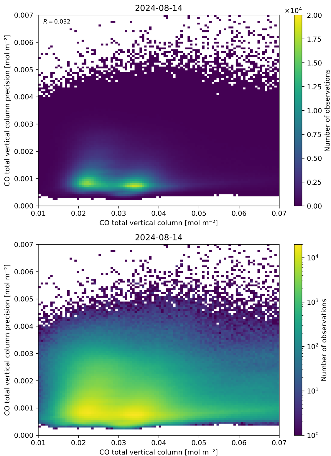
Figure 34: Scatter density plot of “CO total vertical column” against “CO total vertical column precision” for 2024-08-13 to 2024-08-15.
