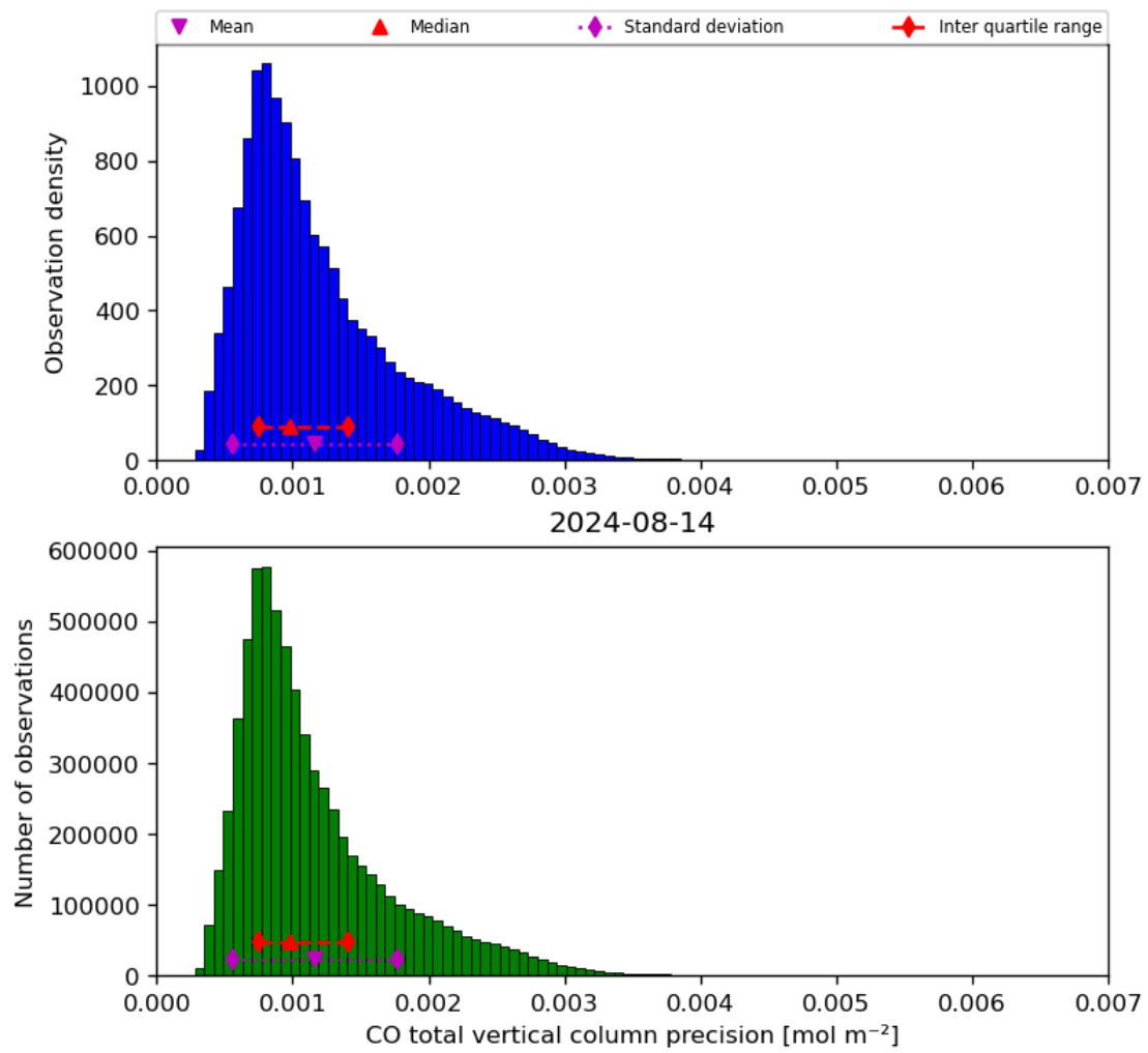
Figure 20: Histogram of “CO total vertical column precision” for 2024-08-13 to 2024-08-15
