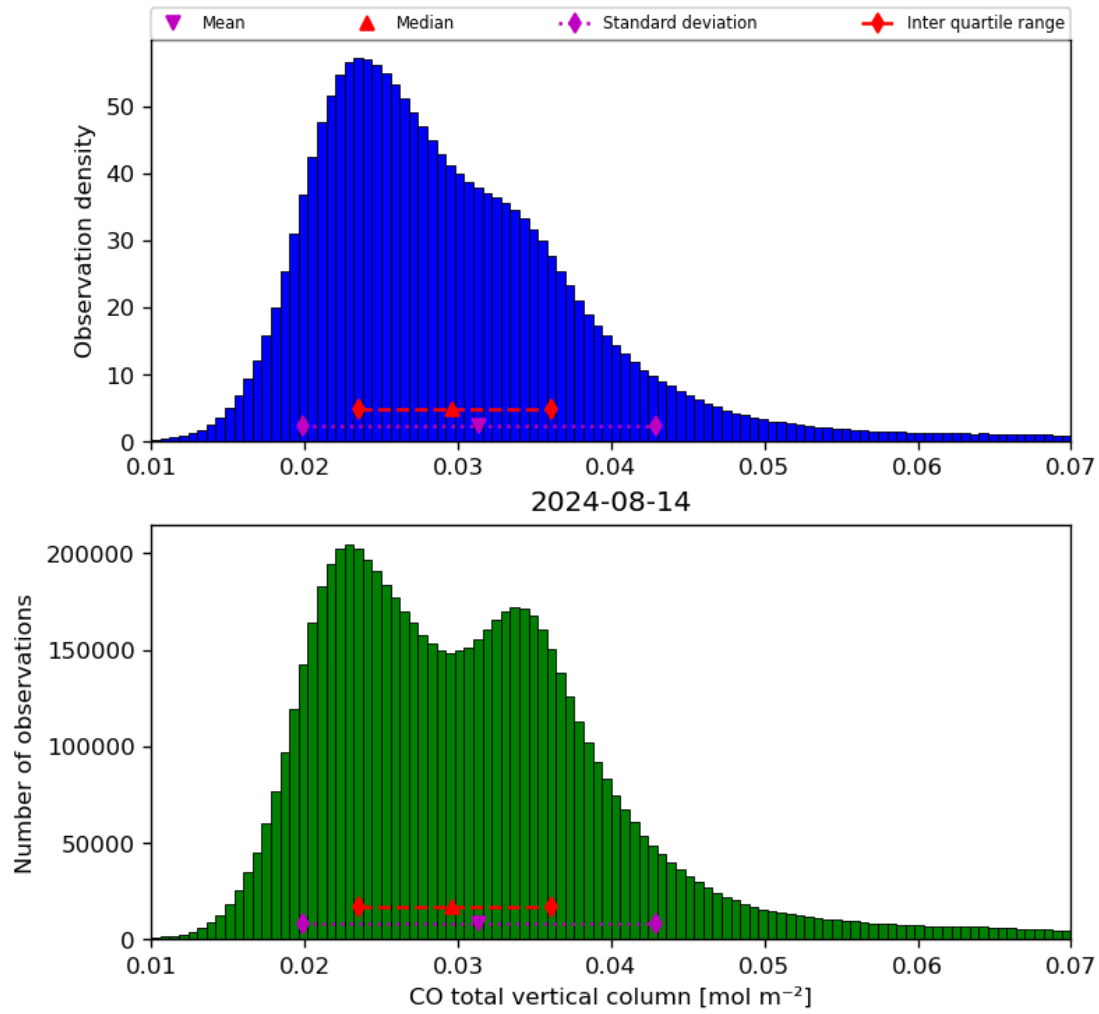
Figure 18: Histogram of “CO total vertical column” for 2024-08-13 to 2024-08-15
