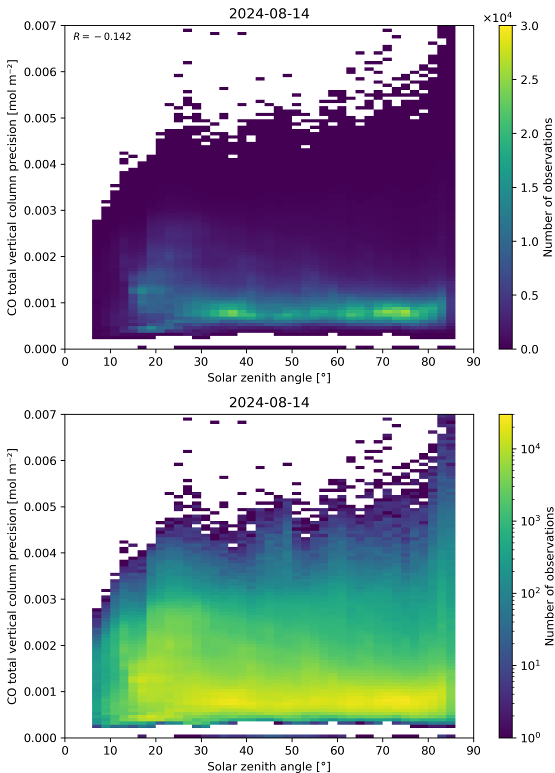
Figure 63: Scatter density plot of “Solar zenith angle” against “CO total vertical column precision” for 2024-08-13 to 2024-08-15.
