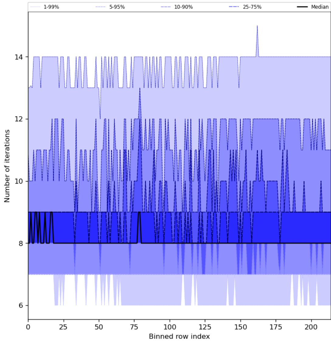
Figure 32: Along track statistics of “Number of iterations” for 2024-08-13 to 2024-08-15
