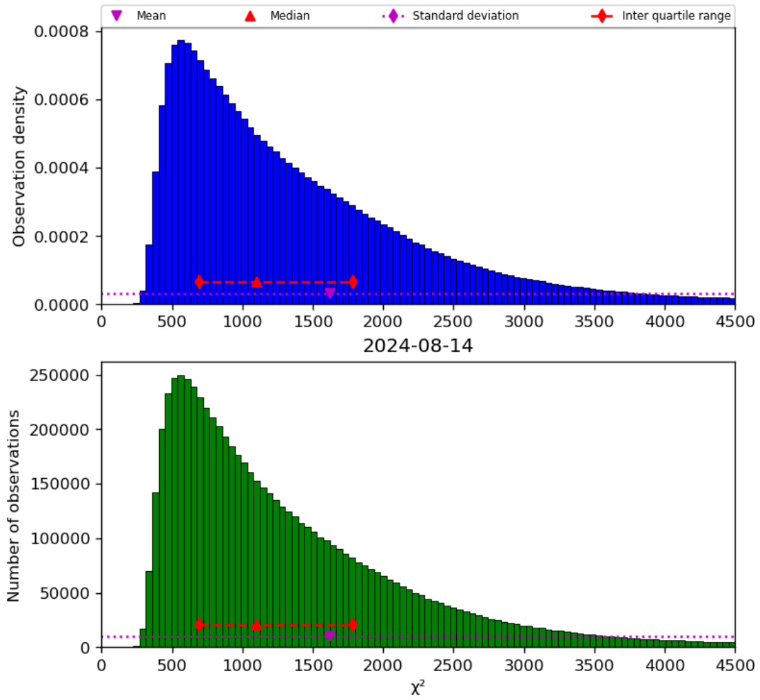
Figure 22: Histogram of “ \chi^2 ” for 2024-08-13 to 2024-08-15
