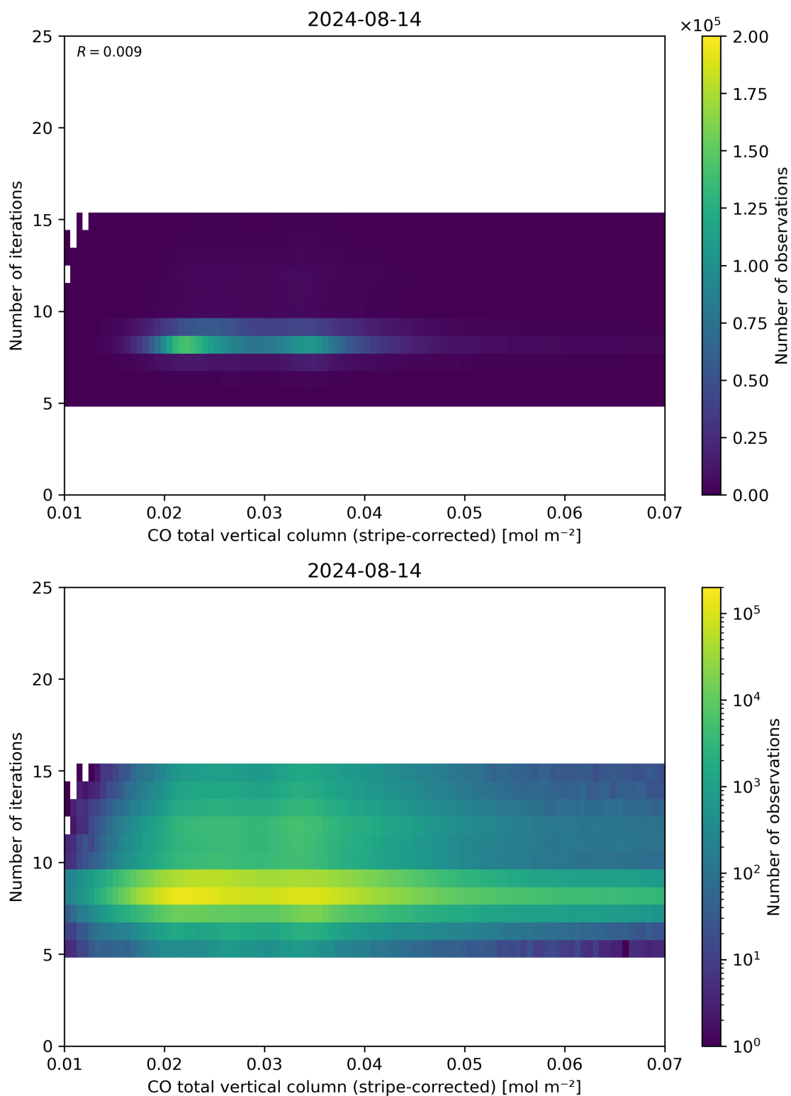
Figure 39: Scatter density plot of “CO total vertical column (stripe-corrected)” against “Number of iterations” for 2024-08-13 to 2024-08-15.
