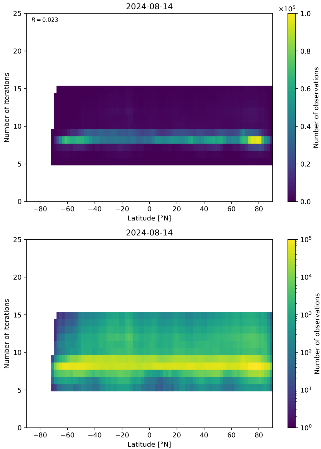
Figure 56: Scatter density plot of “Latitude” against “Number of iterations” for 2024-08-13 to 2024-08-15.
