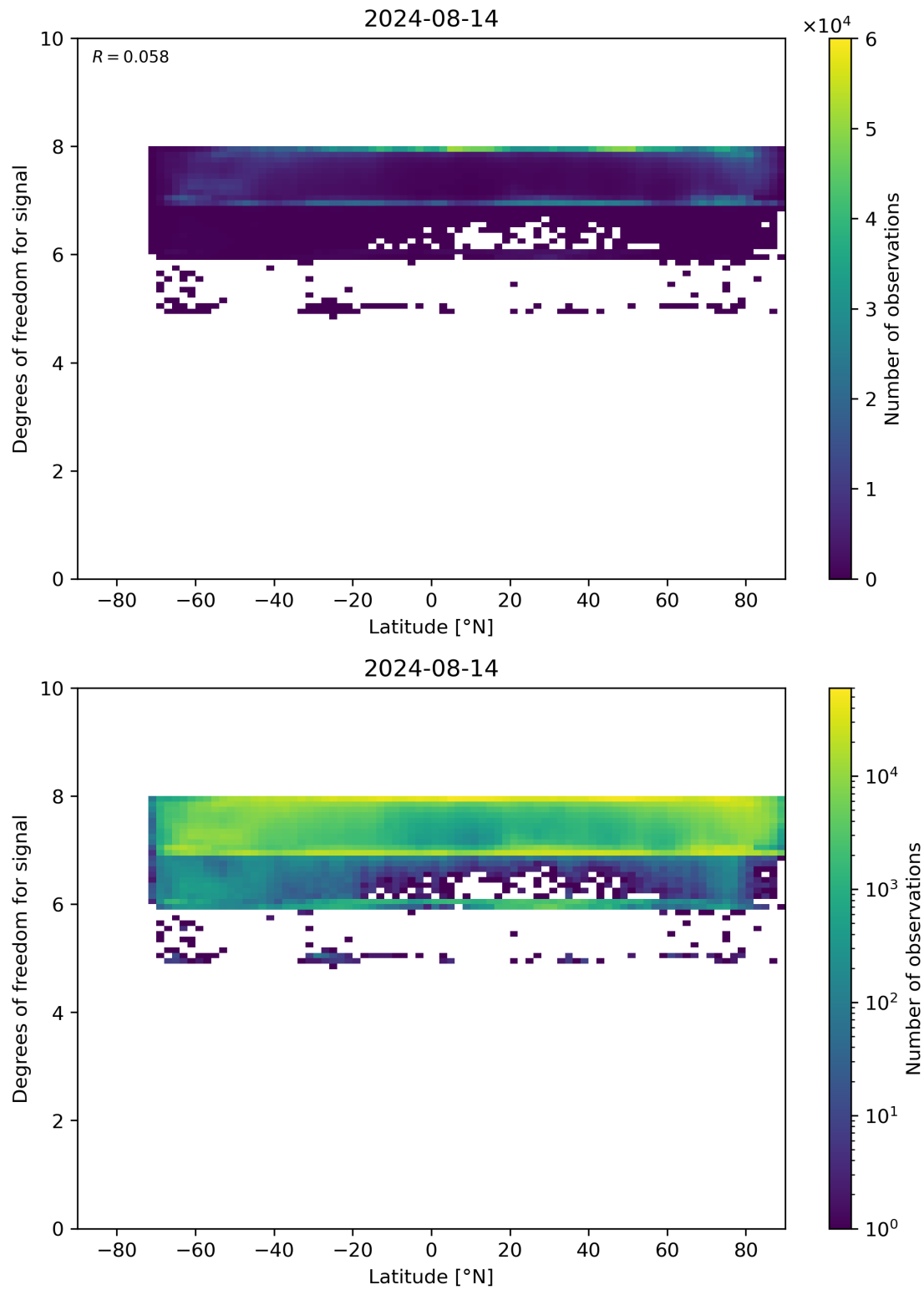
Figure 55: Scatter density plot of “Latitude” against “Degrees of freedom for signal” for 2024-08-13 to 2024-08-15.
