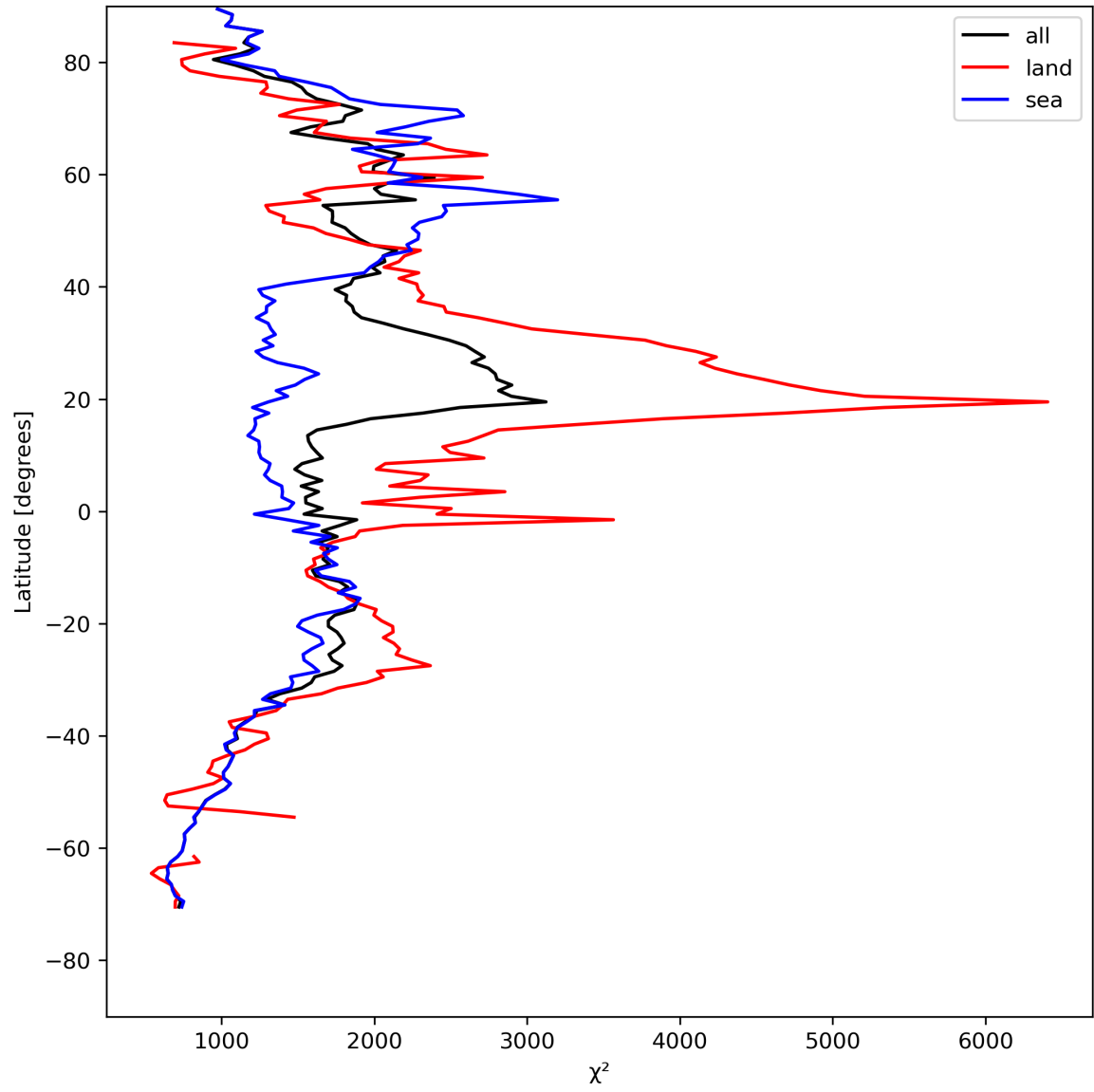
Figure 14: Zonal average of “ \chi^2 ” for 2024-08-13 to 2024-08-15.
