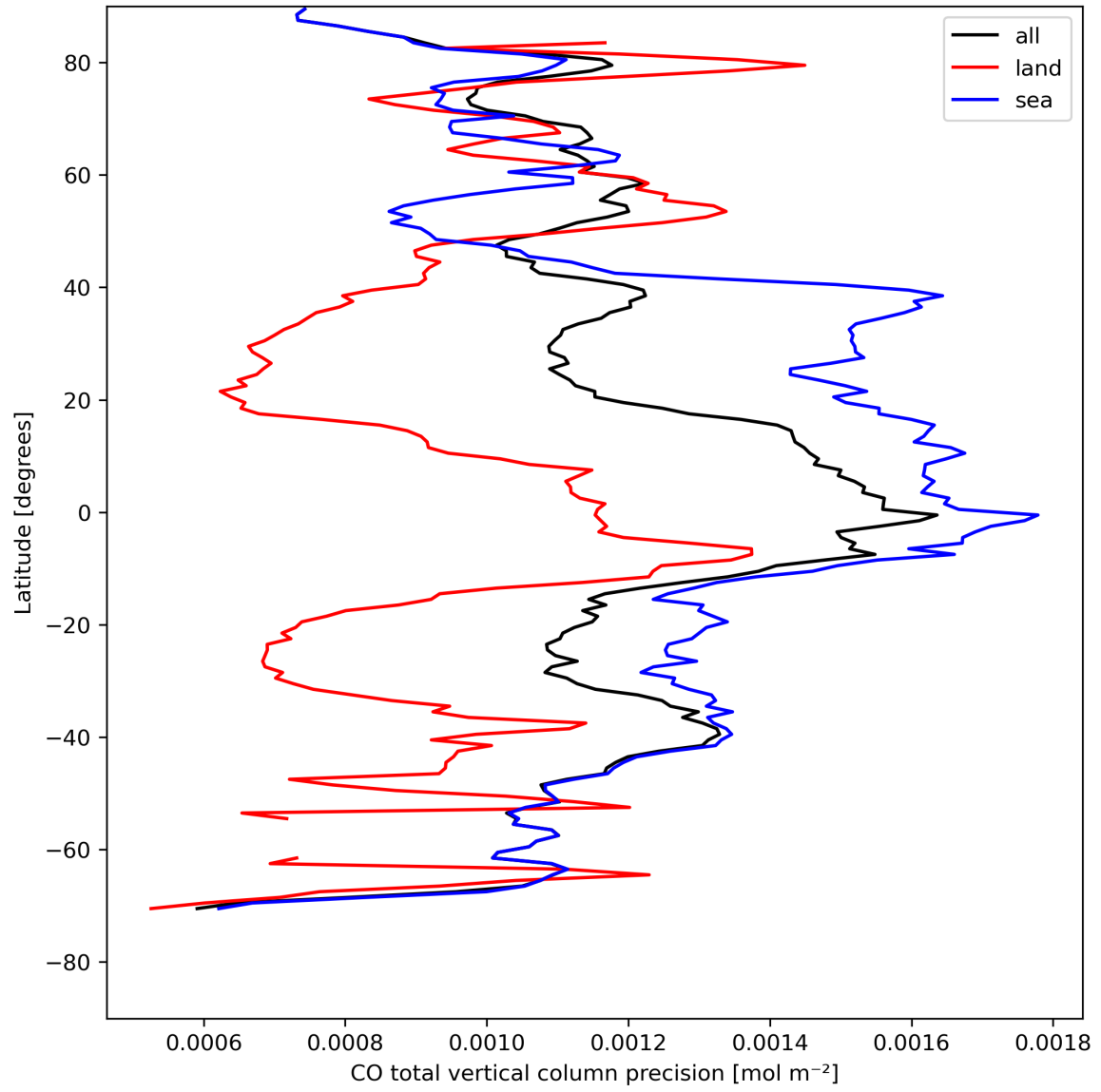
Figure 12: Zonal average of "CO total vertical column precision" for 2024-08-13 to 2024-08-15.
