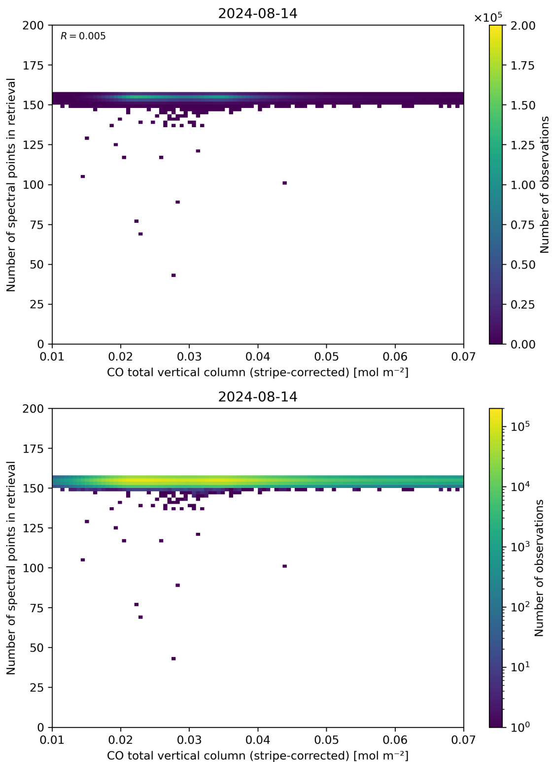
Figure 40: Scatter density plot of “CO total vertical column (stripe-corrected)” against “Number of spectral points in retrieval” for 2024-08-13 to 2024-08-15.
