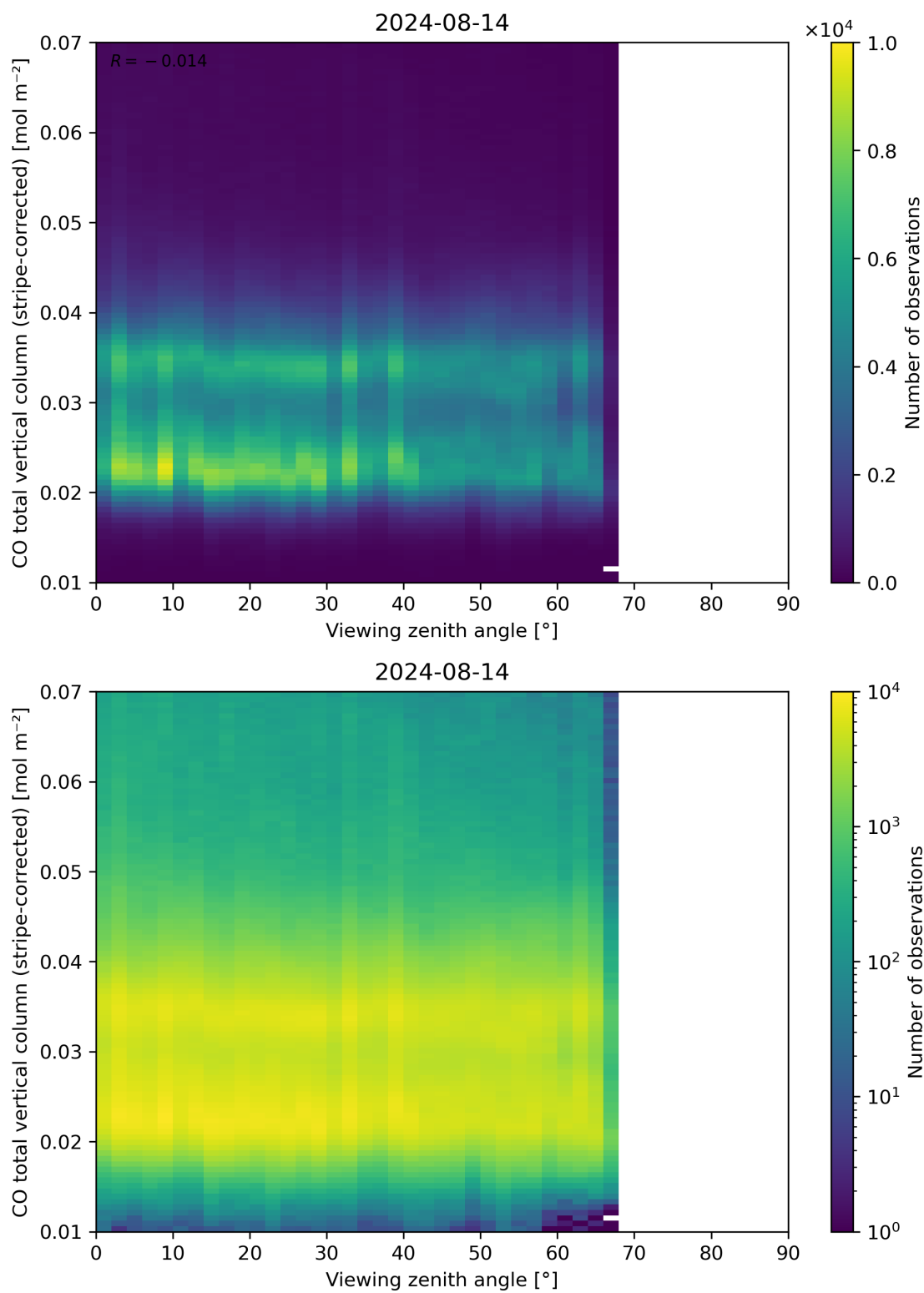
Figure 70: Scatter density plot of “Viewing zenith angle” against “CO total vertical column (stripe-corrected)” for 2024-08-13 to 2024-08-15.
