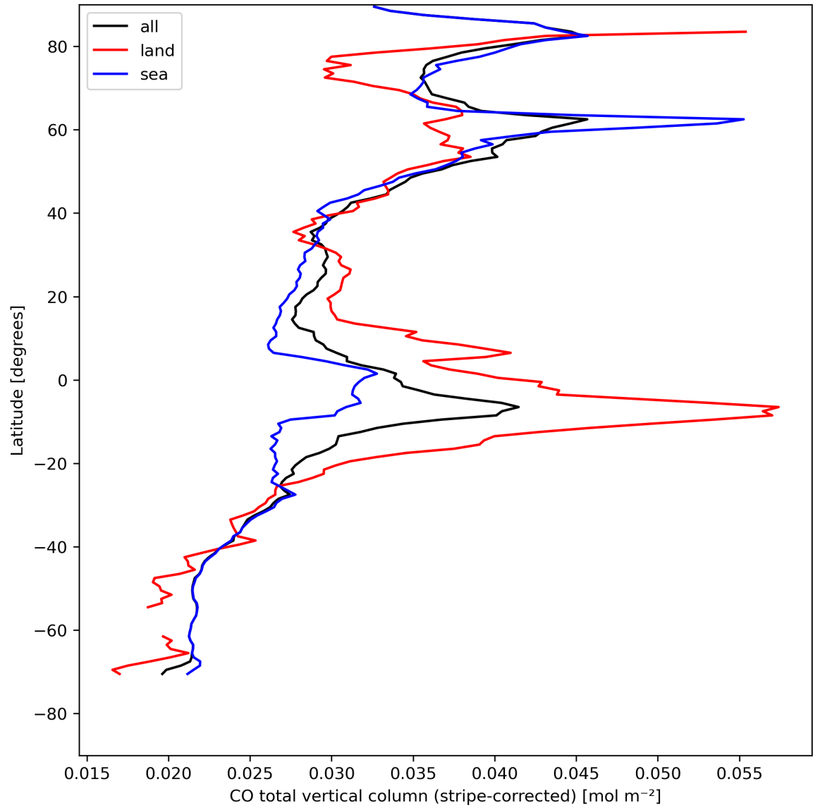
Figure 11: Zonal average of “CO total vertical column (stripe-corrected)” for 2024-08-13 to 2024-08-15.
