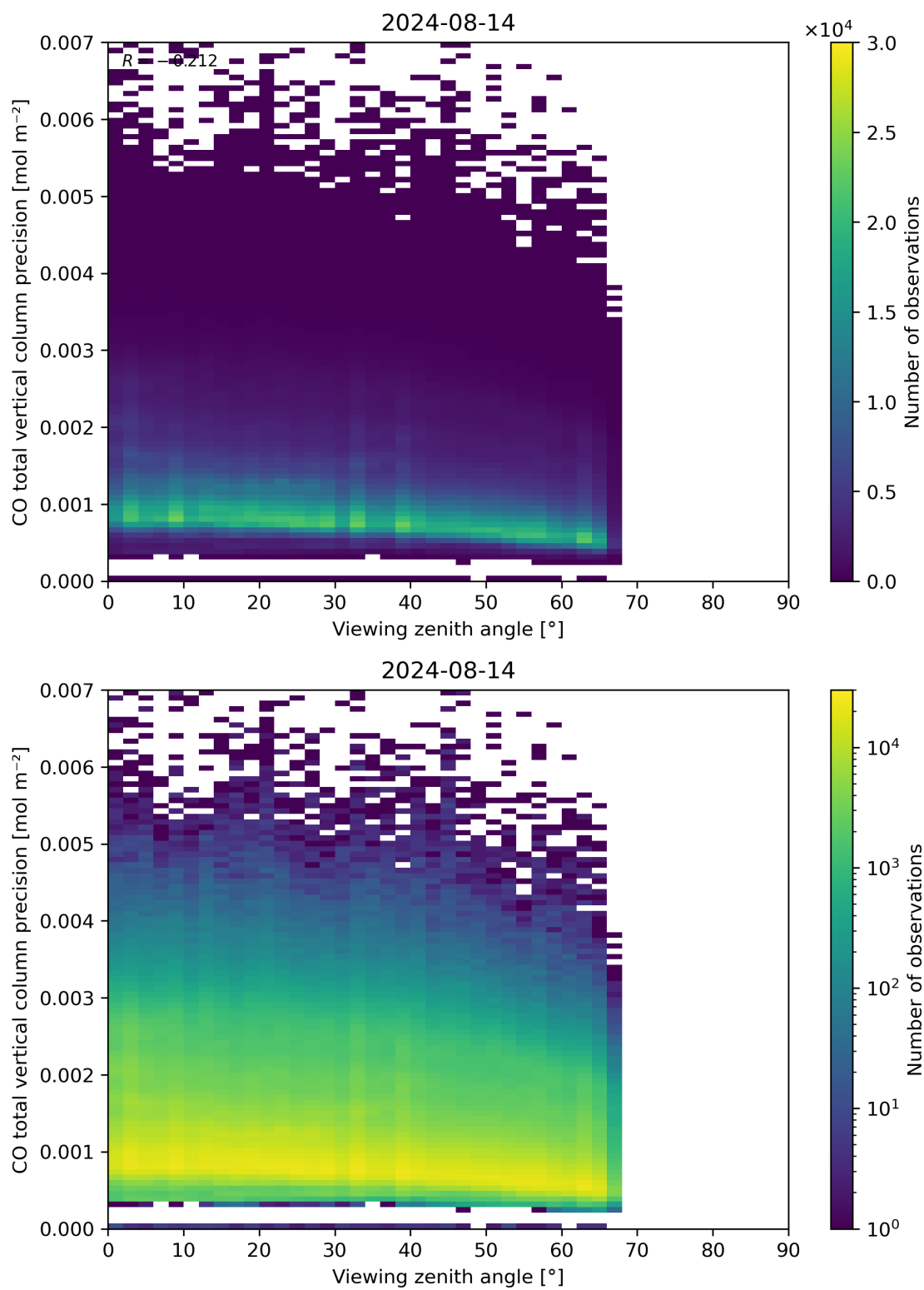
Figure 71: Scatter density plot of “Viewing zenith angle” against “CO total vertical column precision” for 2024-08-13 to 2024-08-15.
