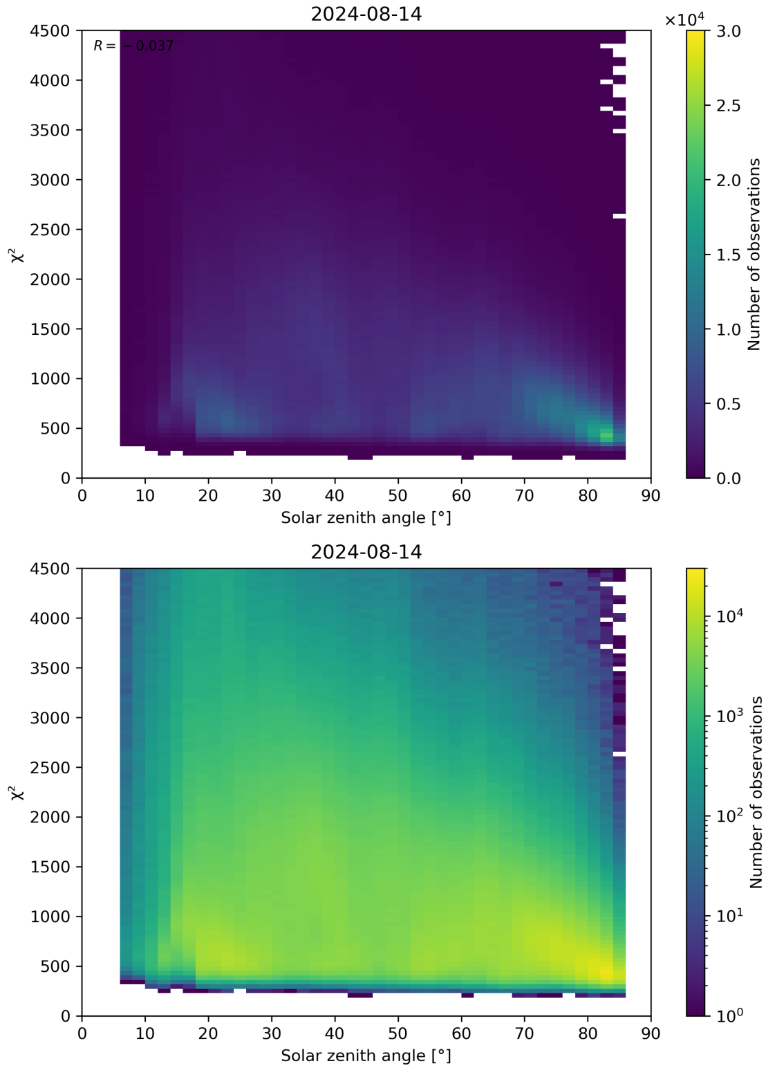
Figure 64: Scatter density plot of “Solar zenith angle” against “ \chi^2 ” for 2024-08-13 to 2024-08-15.
