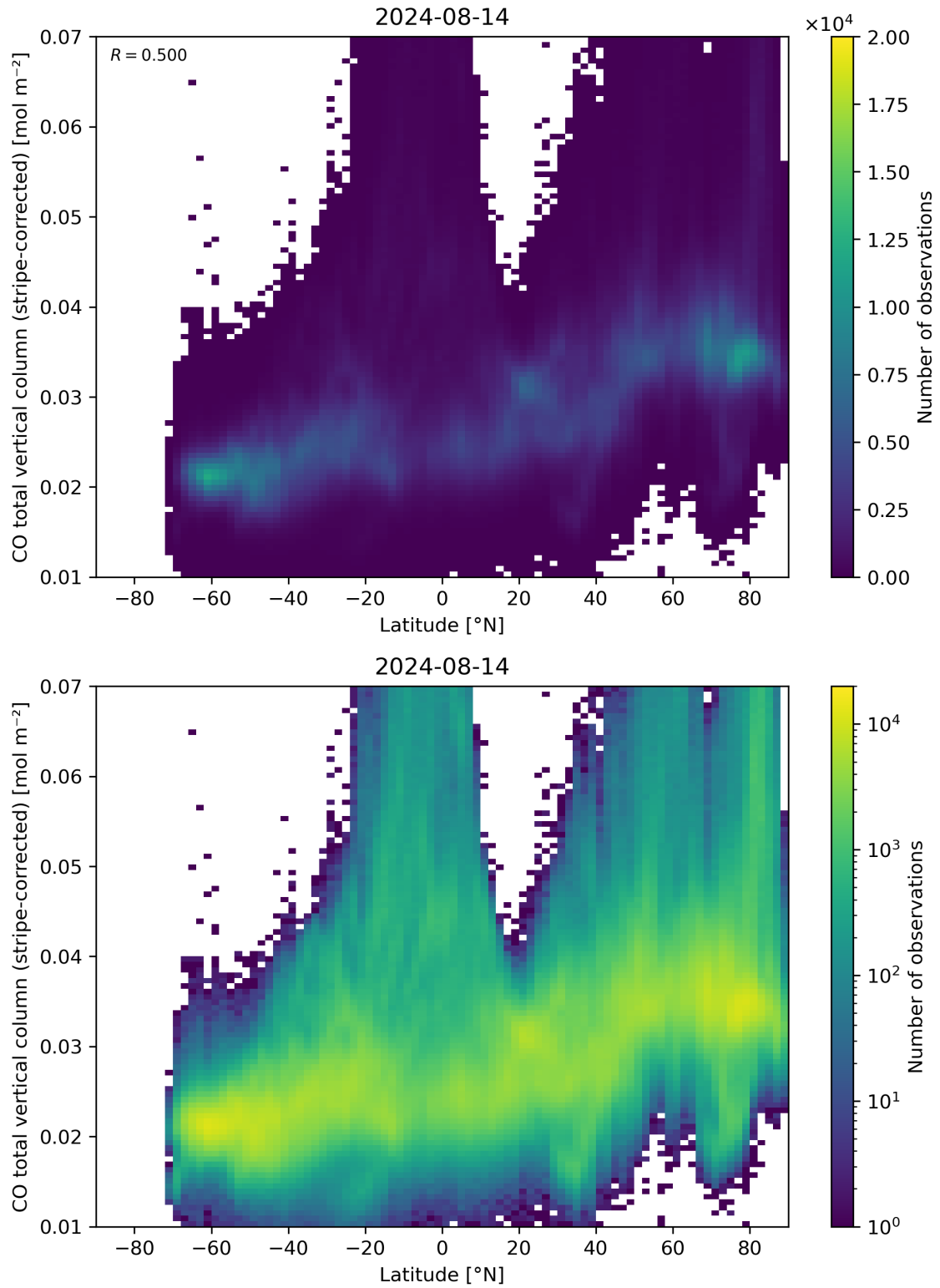
Figure 52: Scatter density plot of “Latitude” against “CO total vertical column (stripe-corrected)” for 2024-08-13 to 2024-08-15.
