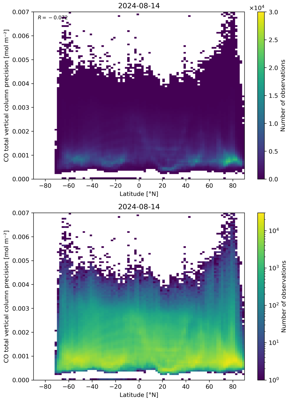
Figure 53: Scatter density plot of “Latitude” against “CO total vertical column precision” for 2024-08-13 to 2024-08-15.
