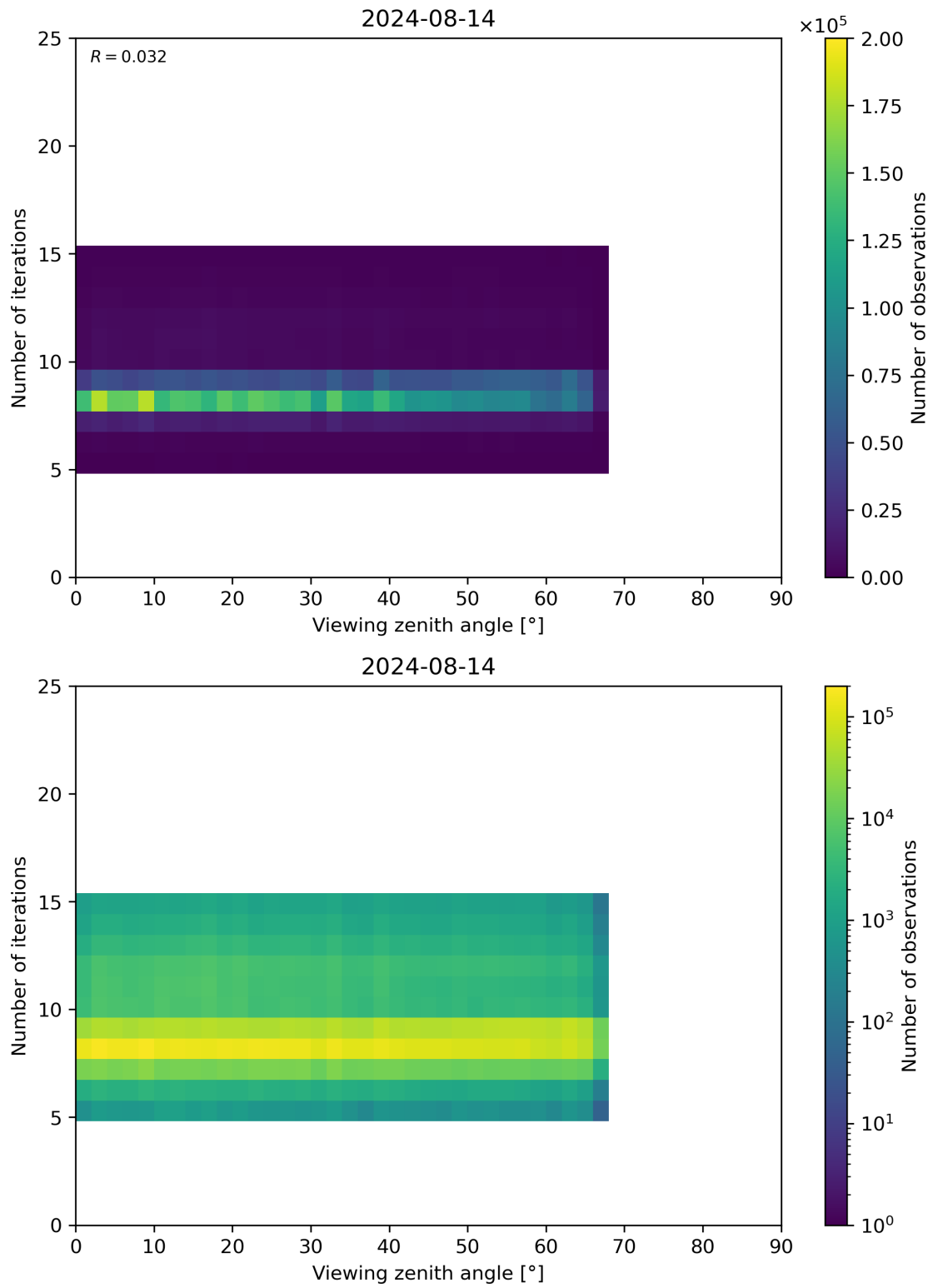
Figure 75: Scatter density plot of “Viewing zenith angle” against “Number of iterations” for 2024-08-13 to 2024-08-15.
