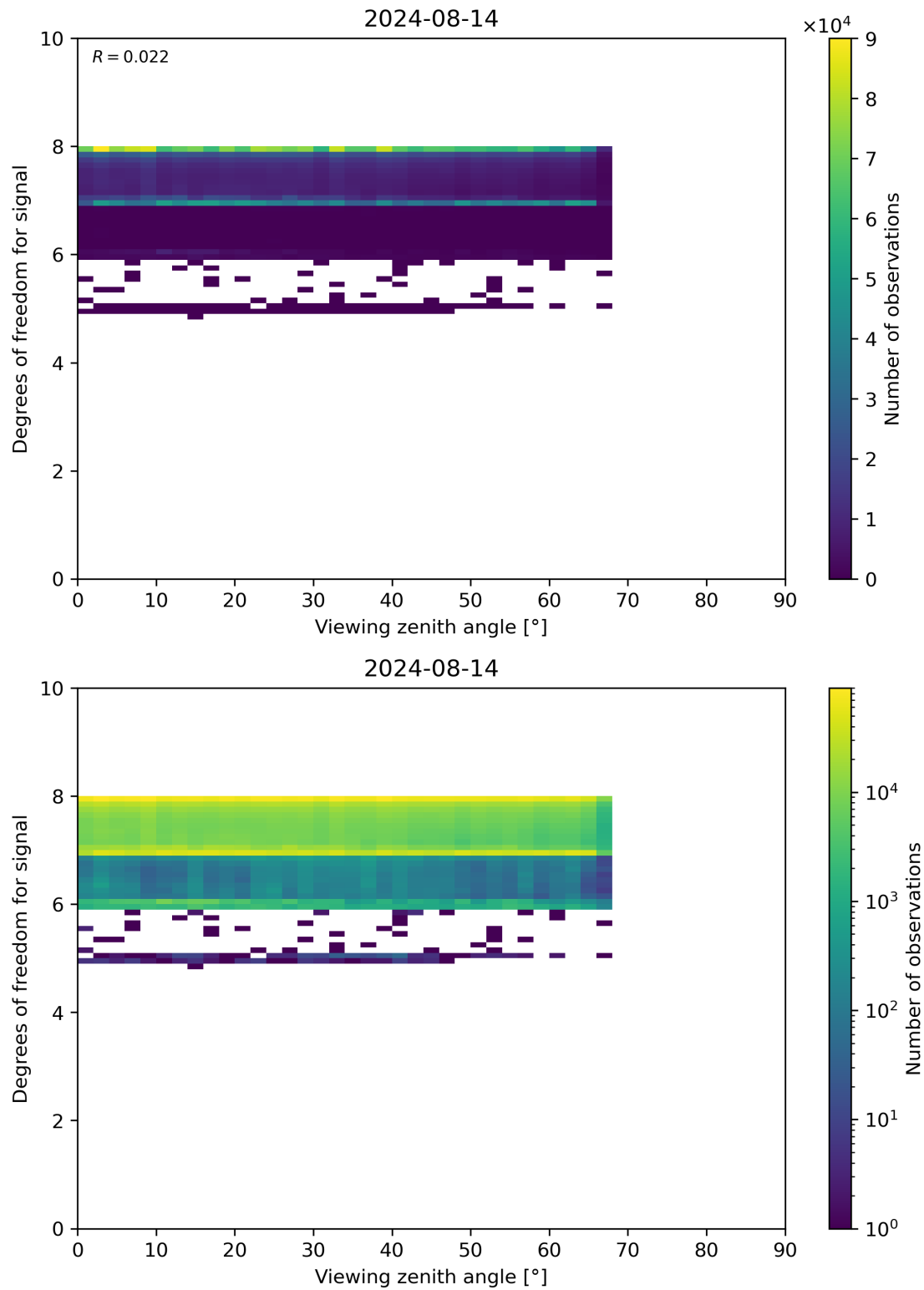
Figure 73: Scatter density plot of “Viewing zenith angle” against “Degrees of freedom for signal” for 2024-08-13 to 2024-08-15.
