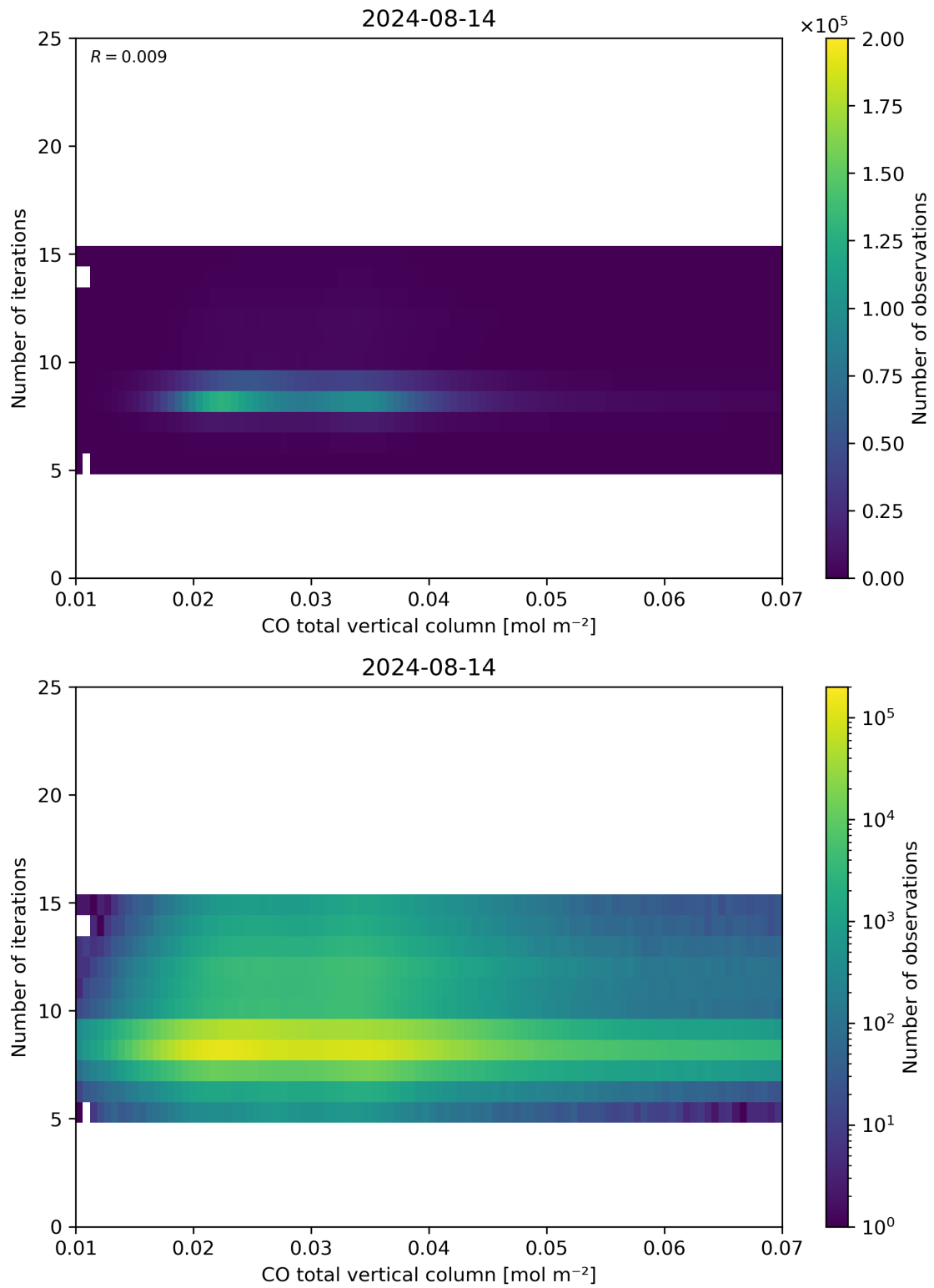
Figure 42: Scatter density plot of “CO total vertical column” against “Number of iterations” for 2024-08-13 to 2024-08-15.
