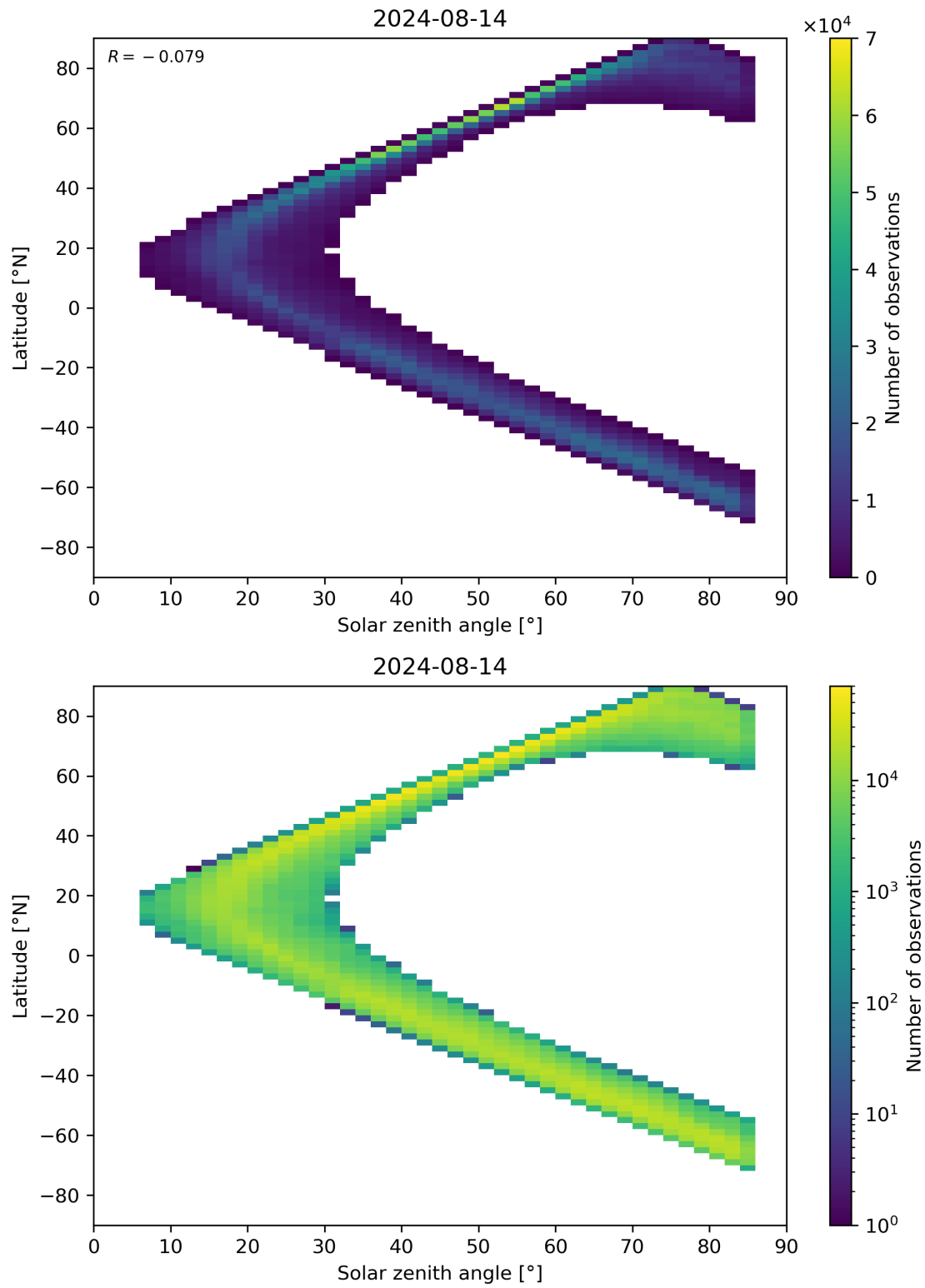
Figure 66: Scatter density plot of “Solar zenith angle” against “Latitude” for 2024-08-13 to 2024-08-15.
