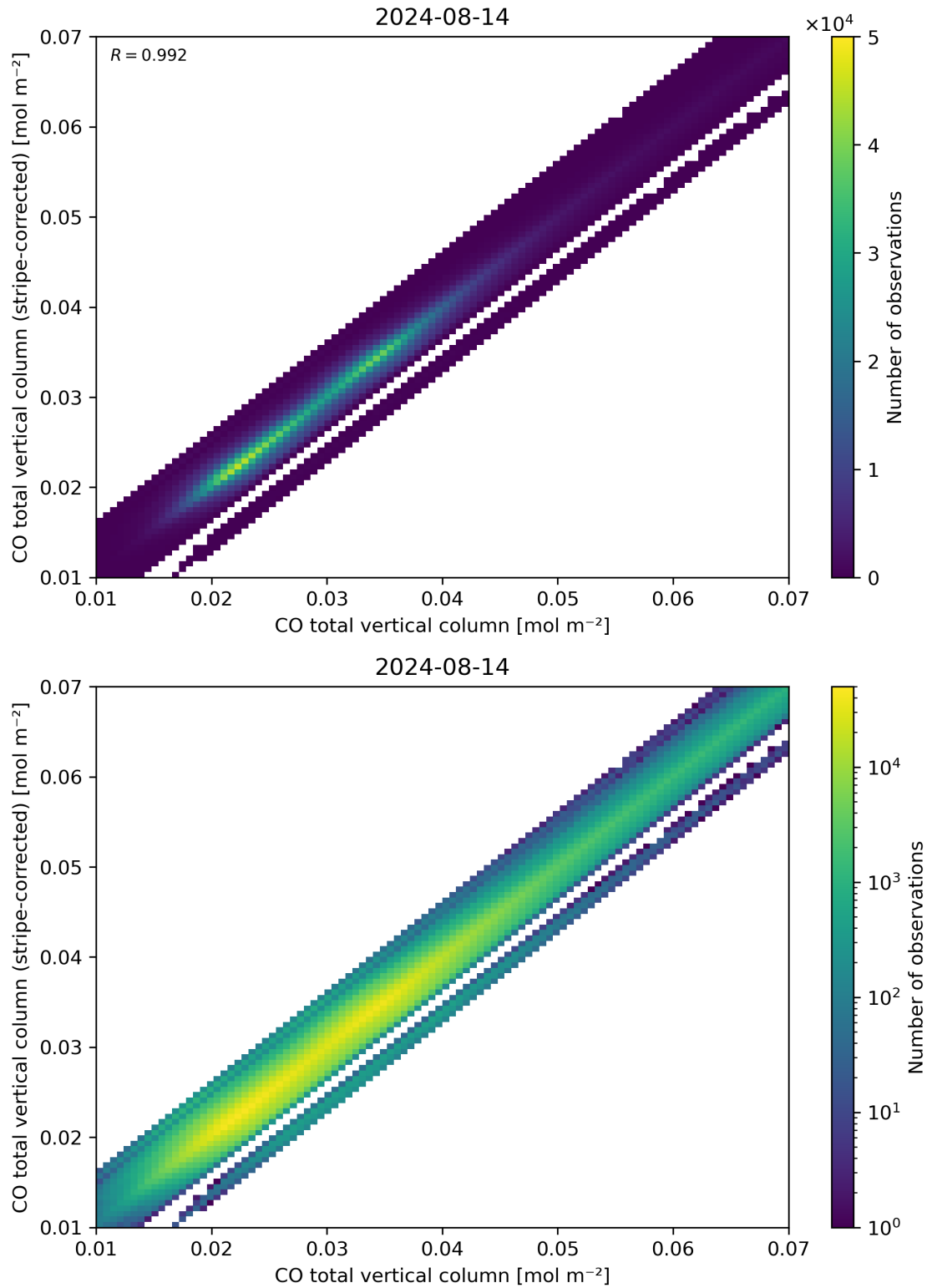
Figure 33: Scatter density plot of “CO total vertical column” against “CO total vertical column (stripe-corrected)” for 2024-08-13 to 2024-08-15.
