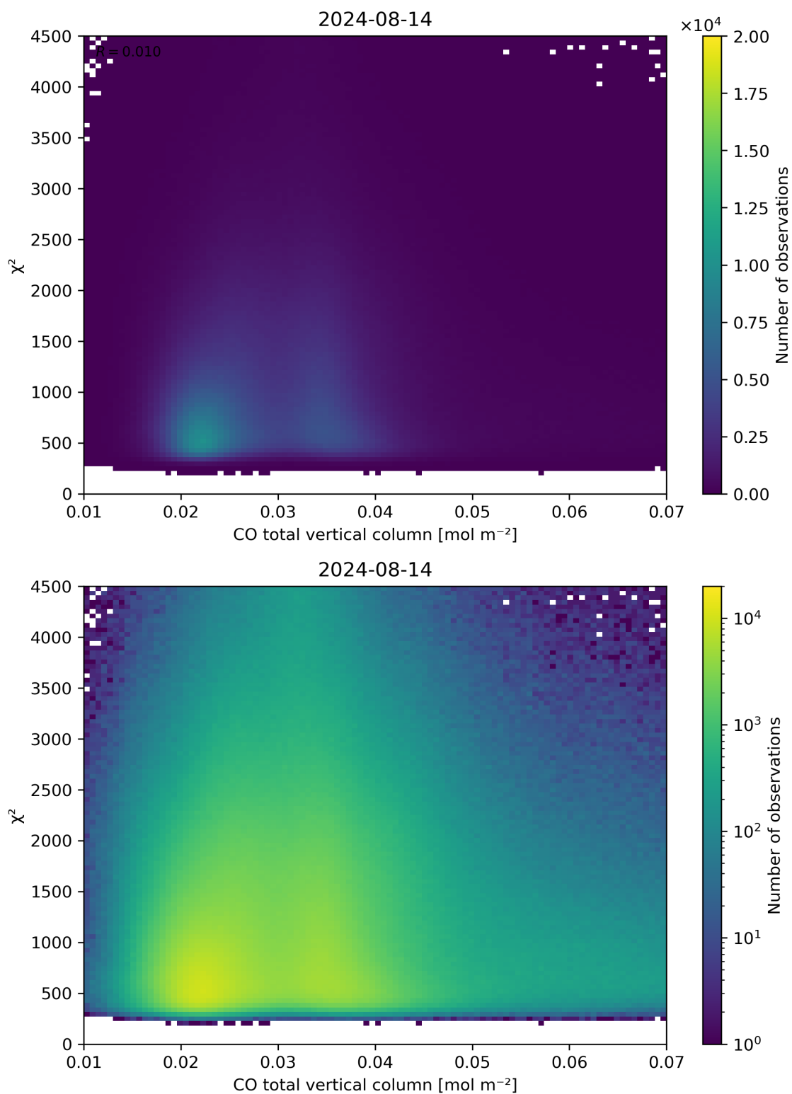
Figure 35: Scatter density plot of “CO total vertical column” against “ \chi^2 ” for 2024-08-13 to 2024-08-15.
