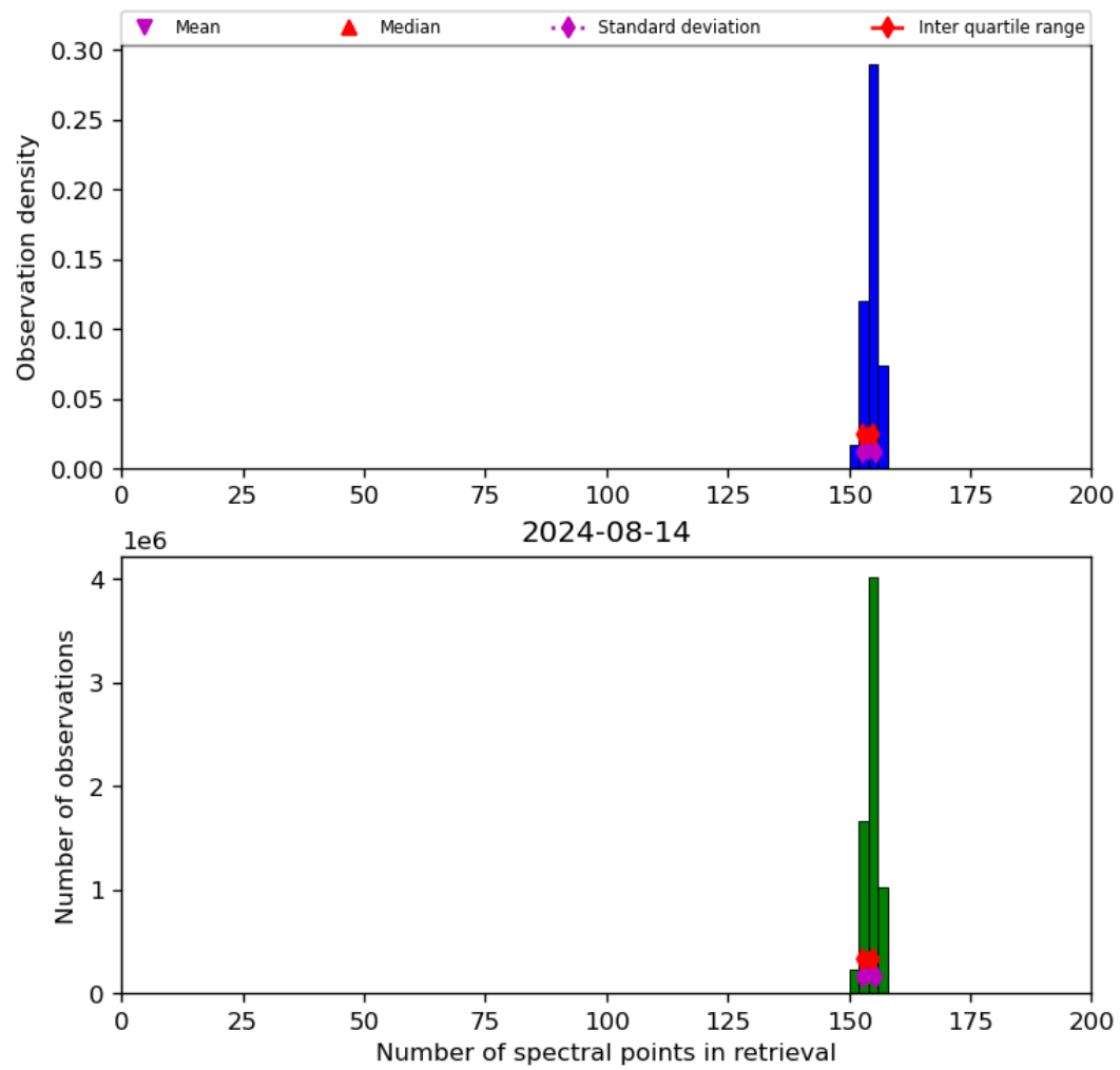
Figure 21: Histogram of “Number of spectral points in retrieval” for 2024-08-13 to 2024-08-15
