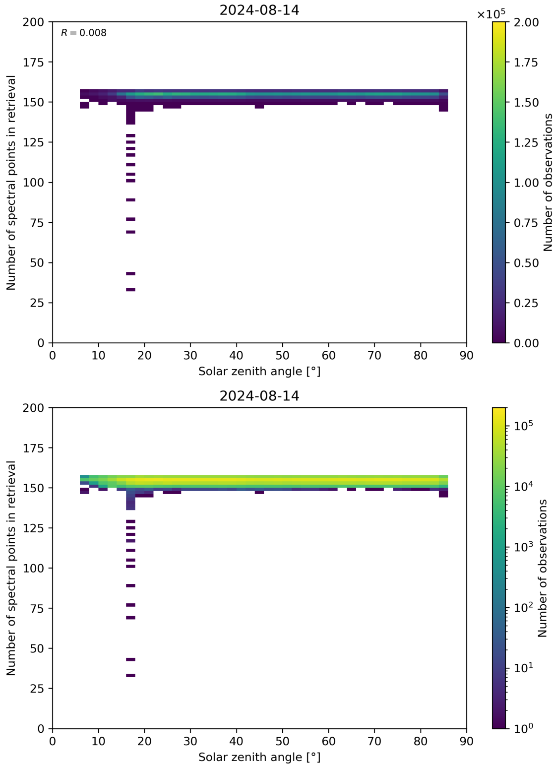
Figure 68: Scatter density plot of “Solar zenith angle” against “Number of spectral points in retrieval” for 2024-08-13 to 2024-08-15.
