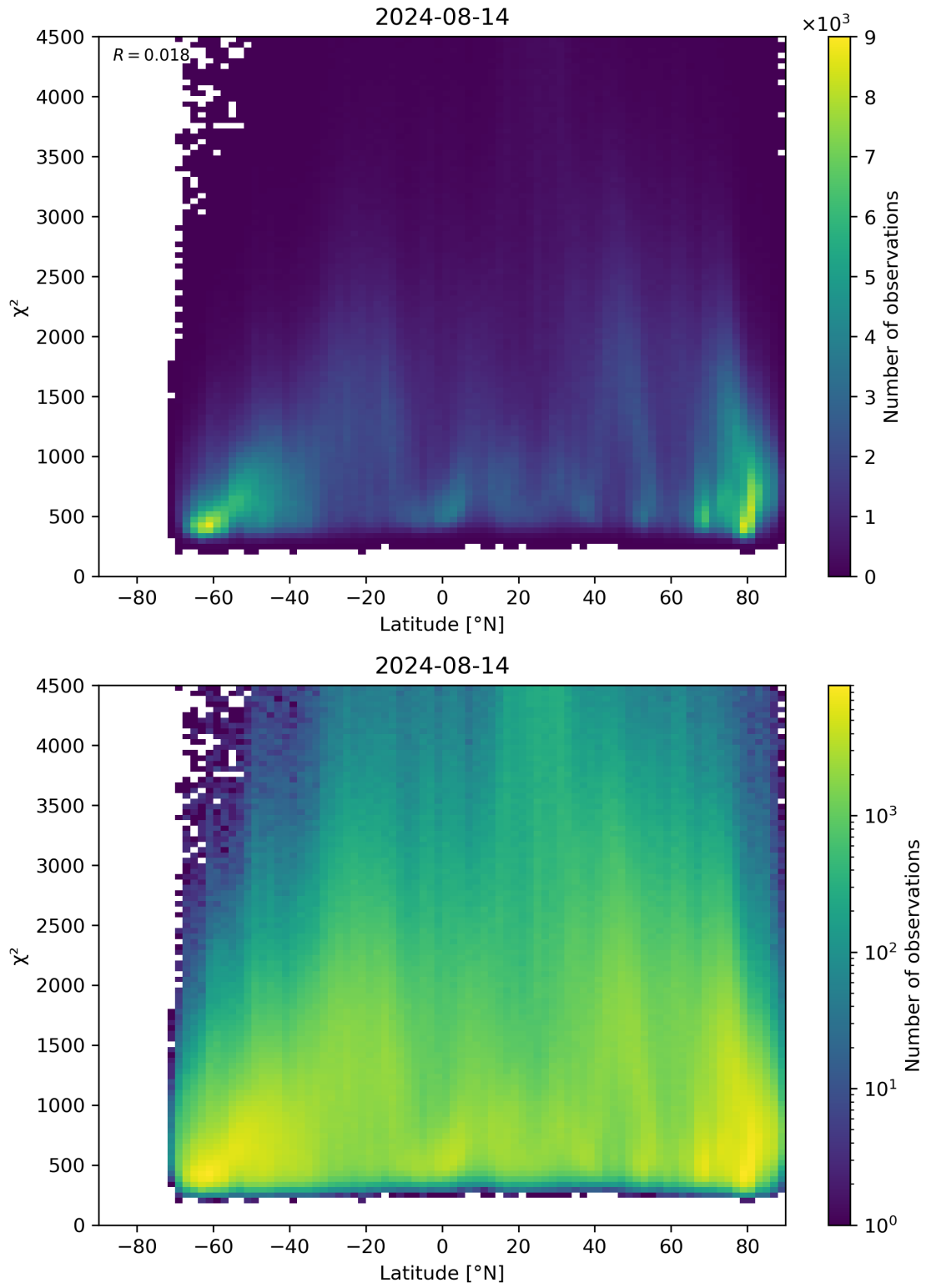
Figure 54: Scatter density plot of “Latitude” against “ \chi^2 ” for 2024-08-13 to 2024-08-15.
