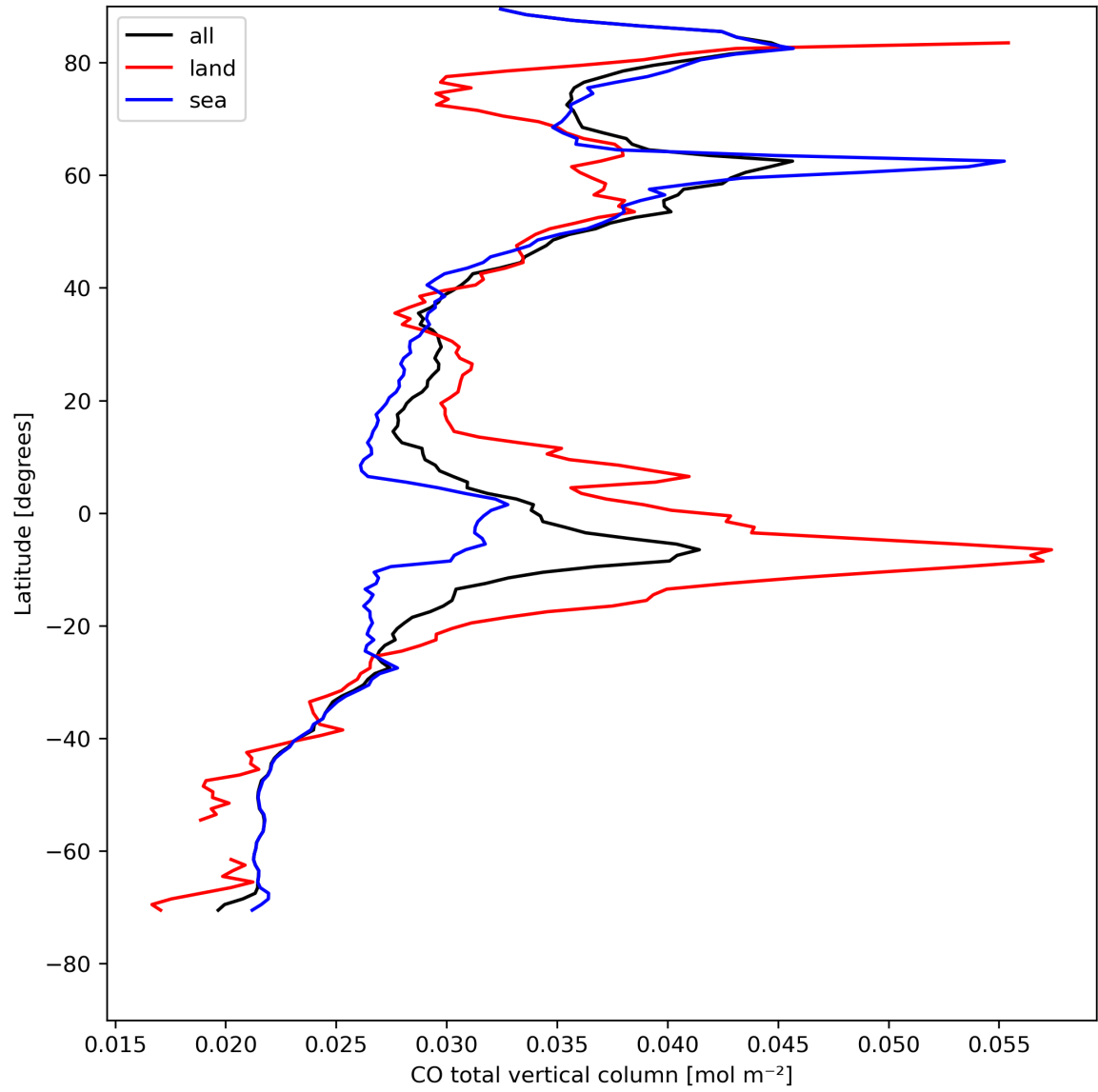
Figure 10: Zonal average of “CO total vertical column” for 2024-08-13 to 2024-08-15.
