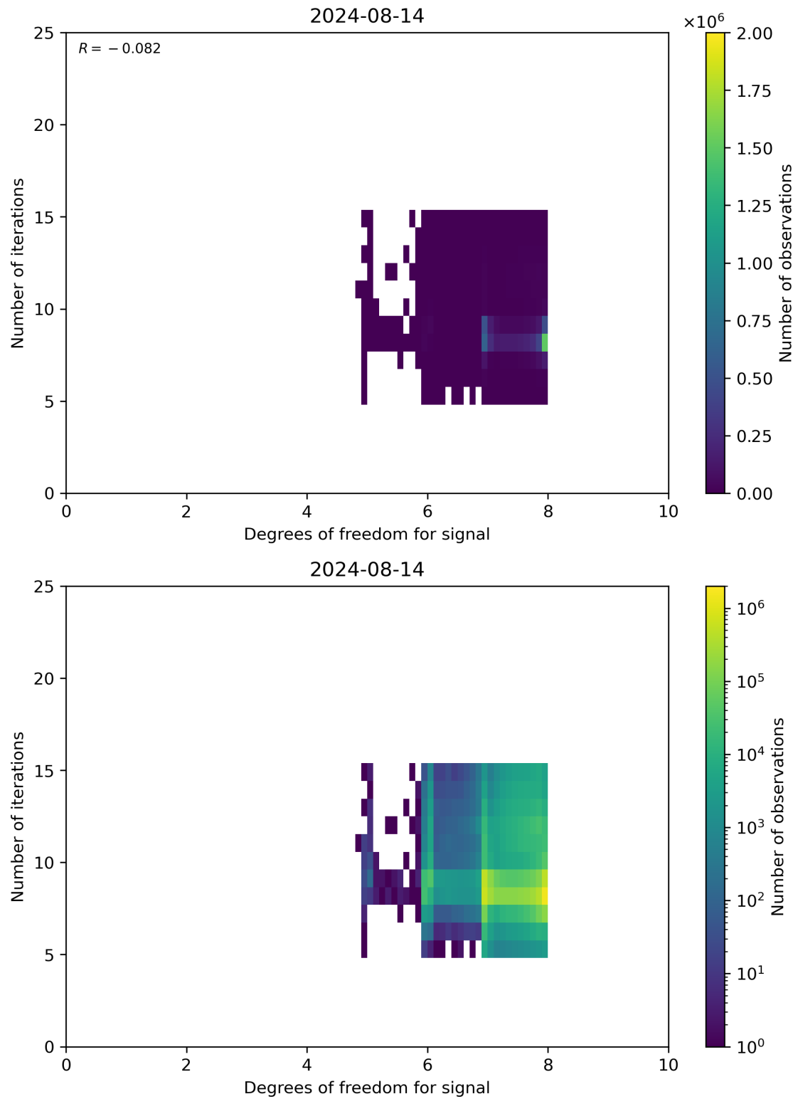
Figure 50: Scatter density plot of “Degrees of freedom for signal” against “Number of iterations” for 2024-08-13 to 2024-08-15.
