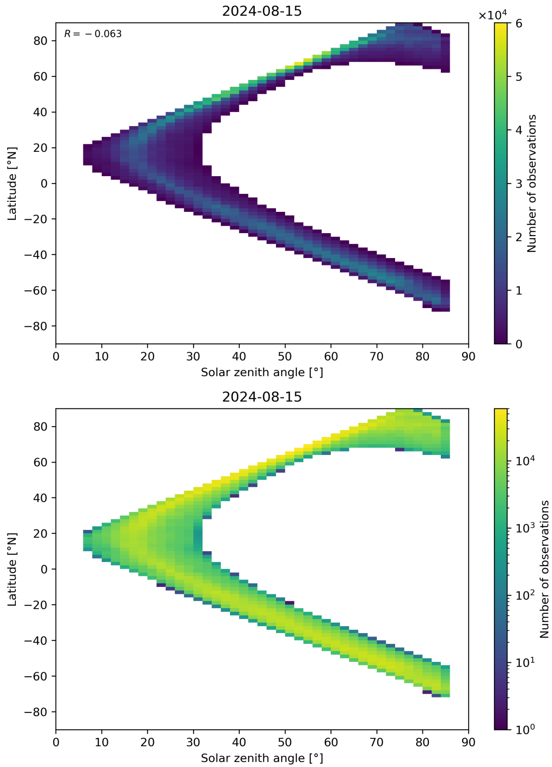
Figure 66: Scatter density plot of “Solar zenith angle” against “Latitude” for 2024-08-14 to 2024-08-16.
