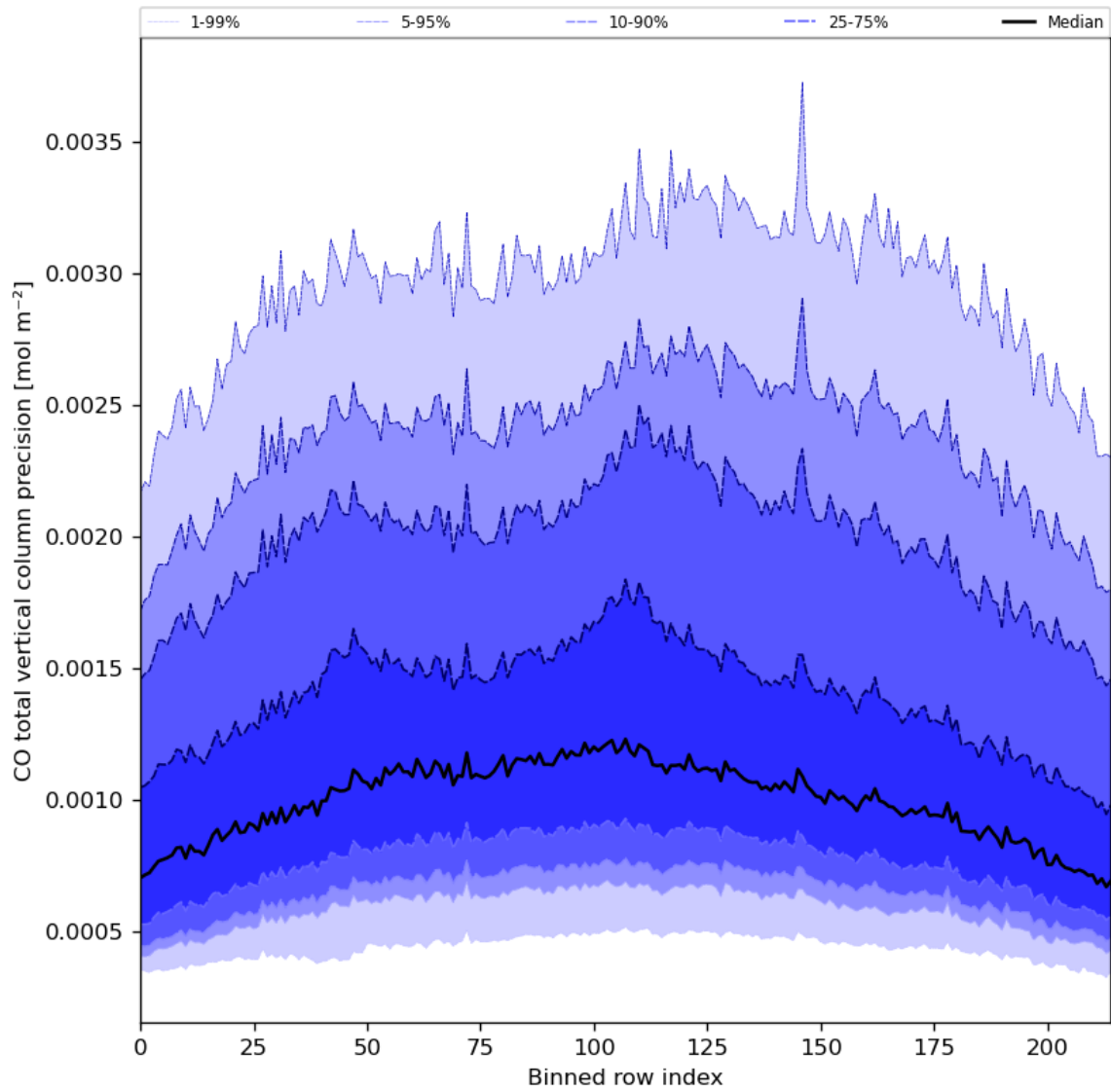
Figure 28: Along track statistics of “CO total vertical column precision” for 2024-08-14 to 2024-08-16
