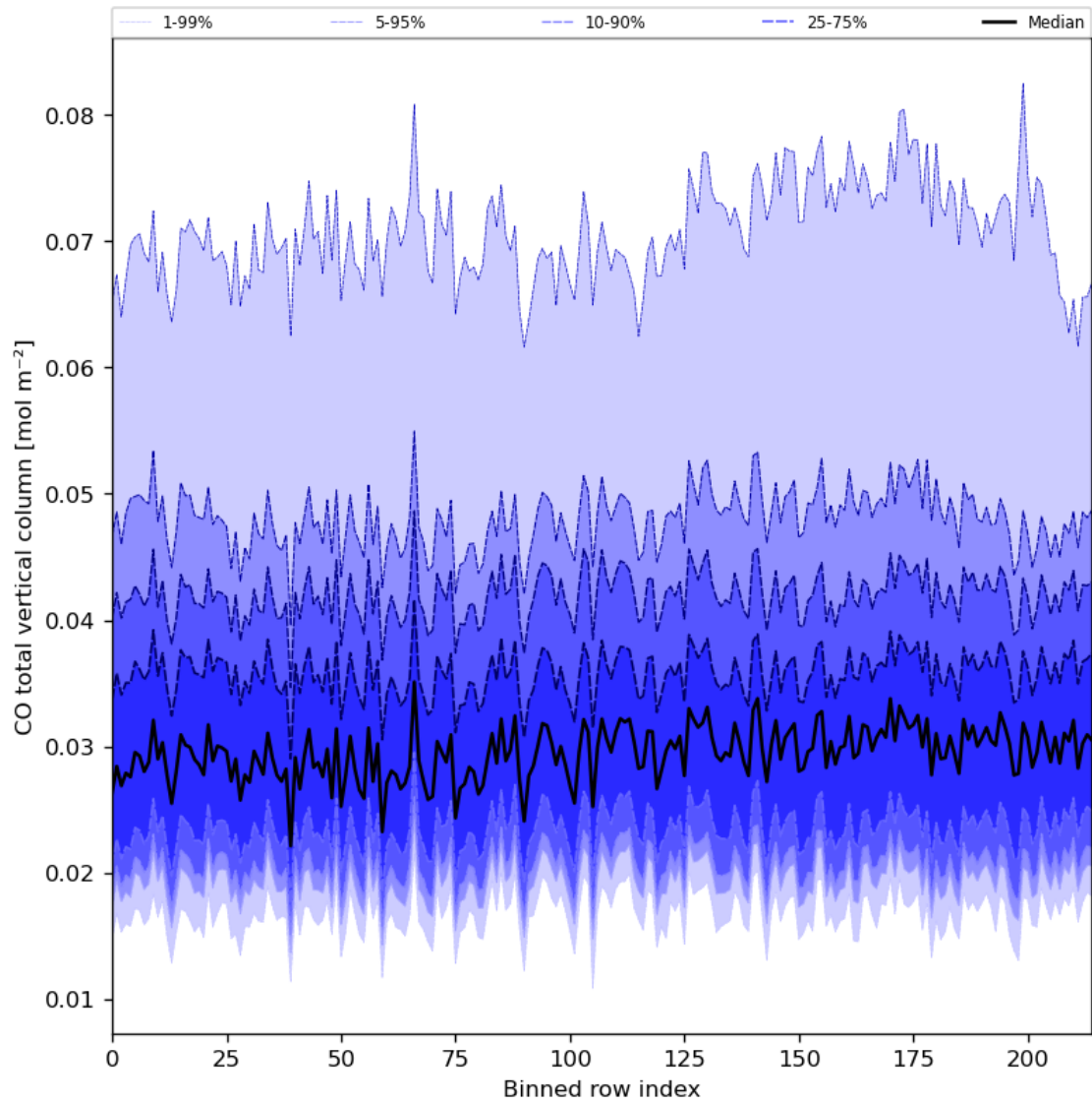
Figure 26: Along track statistics of “CO total vertical column” for 2024-08-14 to 2024-08-16
