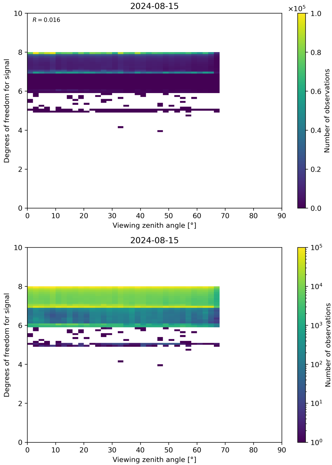
Figure 73: Scatter density plot of “Viewing zenith angle” against “Degrees of freedom for signal” for 2024-08-14 to 2024-08-16.
