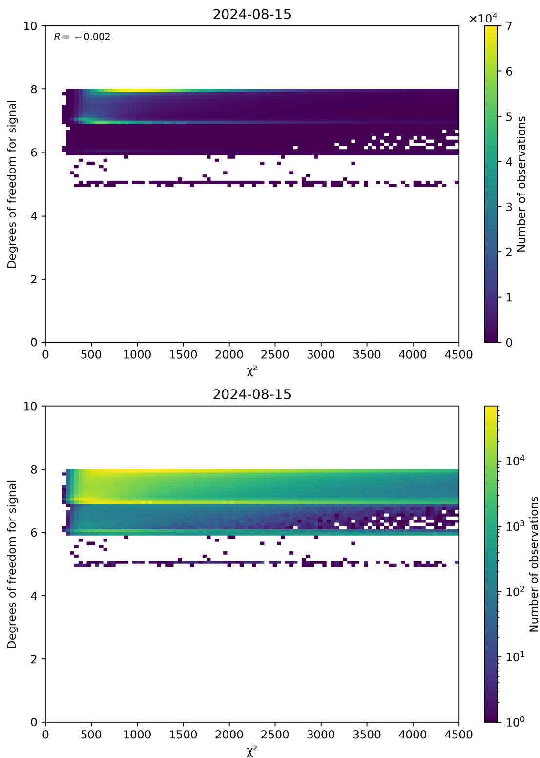
Figure 48: Scatter density plot of “ \chi^2 ” against “Degrees of freedom for signal” for 2024-08-14 to 2024-08-16.
