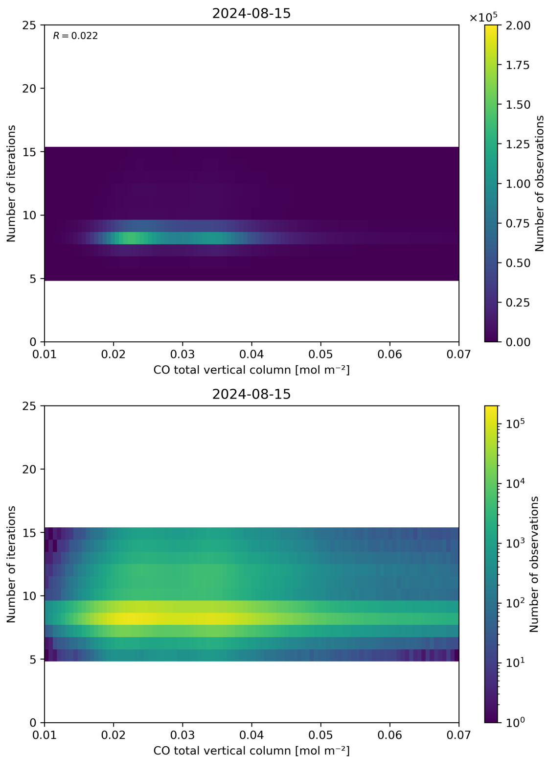
Figure 42: Scatter density plot of “CO total vertical column” against “Number of iterations” for 2024-08-14 to 2024-08-16.
