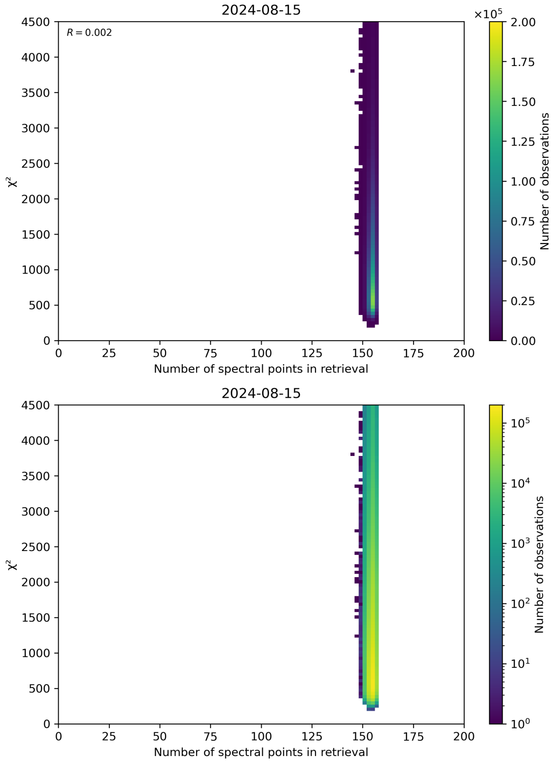
Figure 58: Scatter density plot of “Number of spectral points in retrieval” against “ \chi^2 ” for 2024-08-14 to 2024-08-16.
