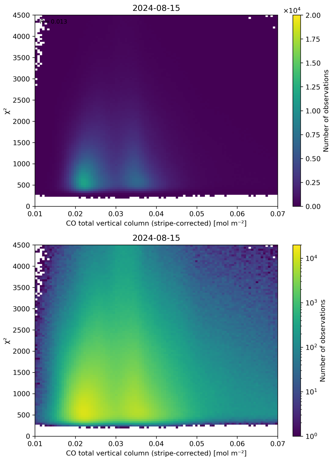
Figure 37: Scatter density plot of “CO total vertical column (stripe-corrected)” against “ \chi^2 ” for 2024-08-14 to 2024-08-16.
