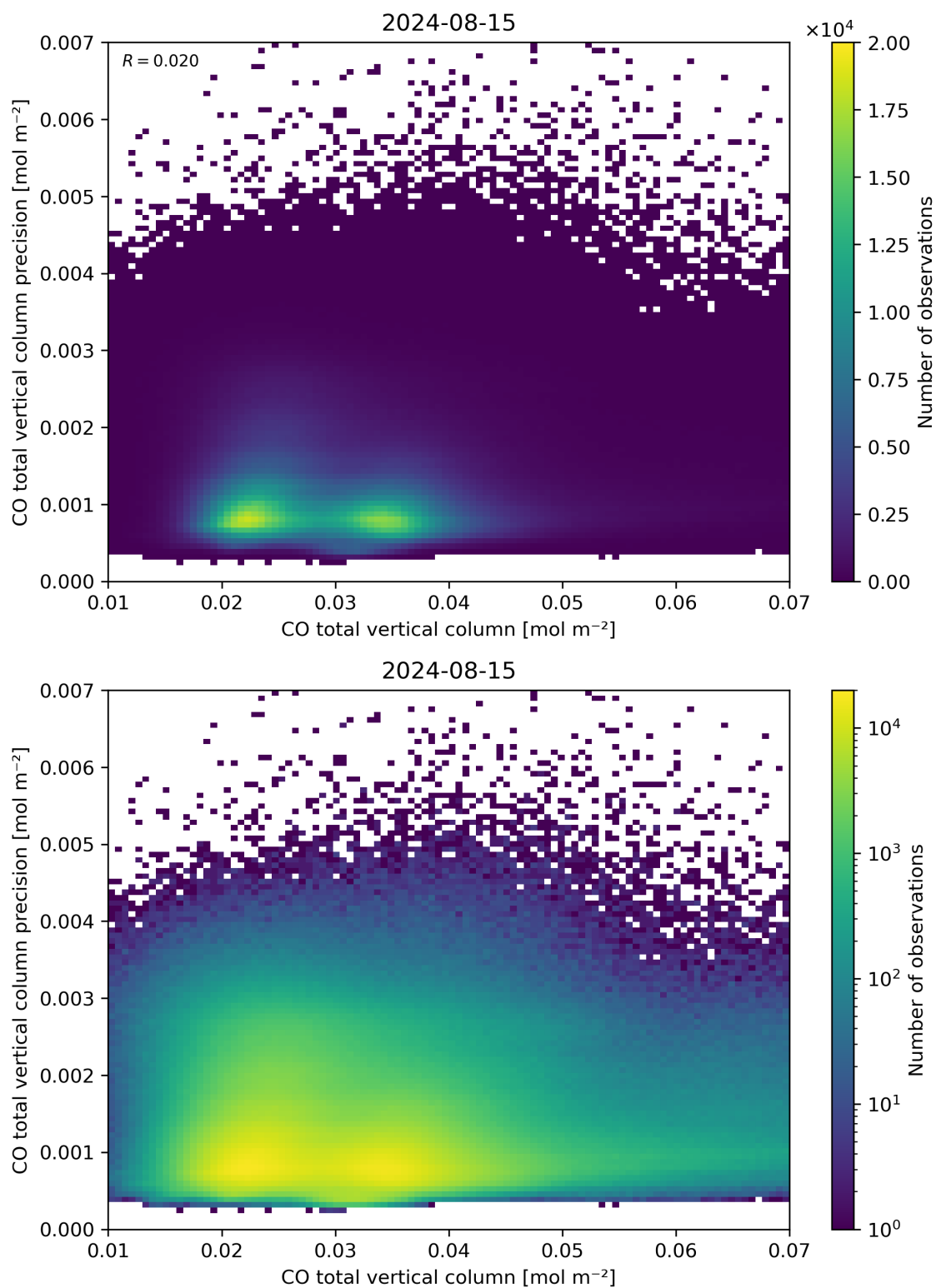
Figure 34: Scatter density plot of “CO total vertical column” against “CO total vertical column precision” for 2024-08-14 to 2024-08-16.
