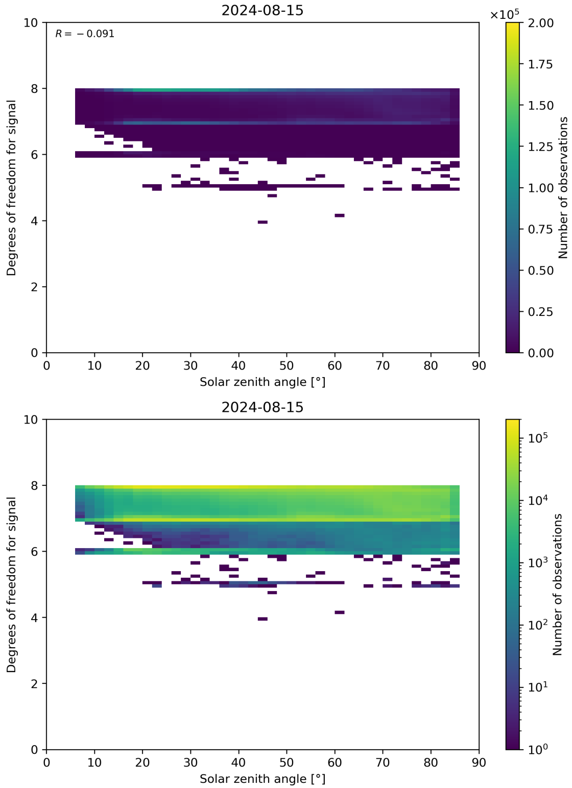
Figure 65: Scatter density plot of “Solar zenith angle” against “Degrees of freedom for signal” for 2024-08-14 to 2024-08-16.
