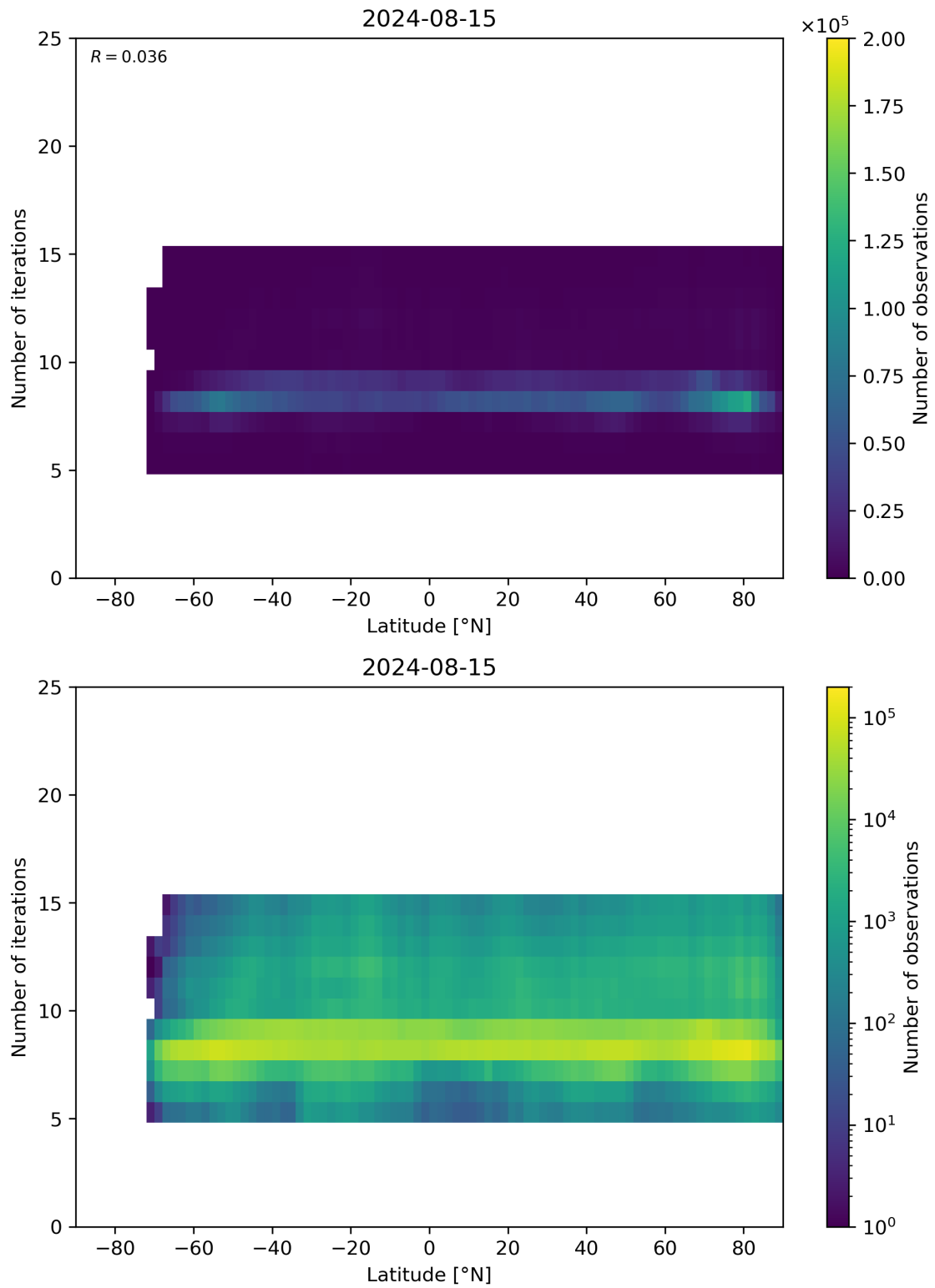
Figure 56: Scatter density plot of “Latitude” against “Number of iterations” for 2024-08-14 to 2024-08-16.
