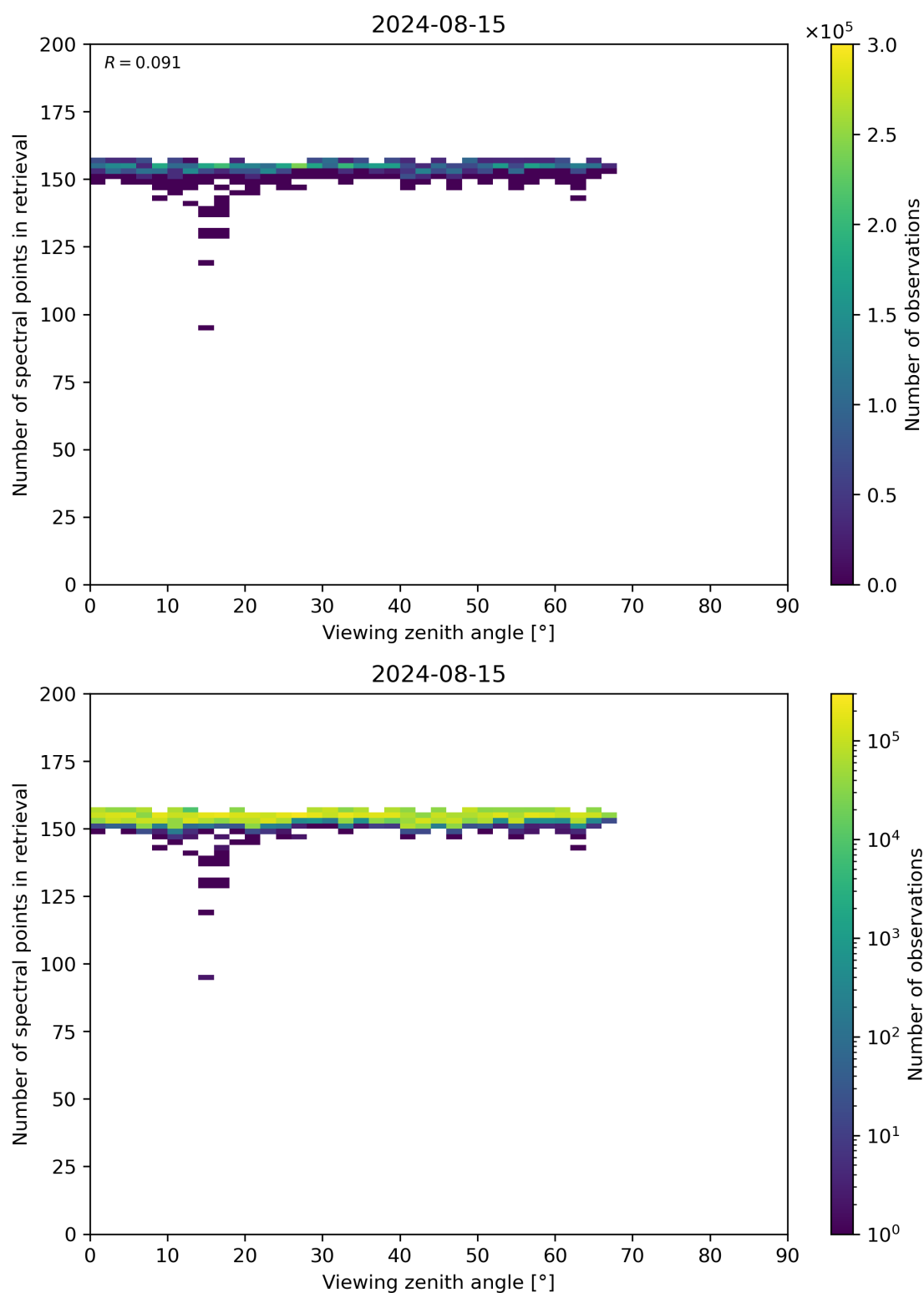
Figure 76: Scatter density plot of “Viewing zenith angle” against “Number of spectral points in retrieval” for 2024-08-14 to 2024-08-16.
