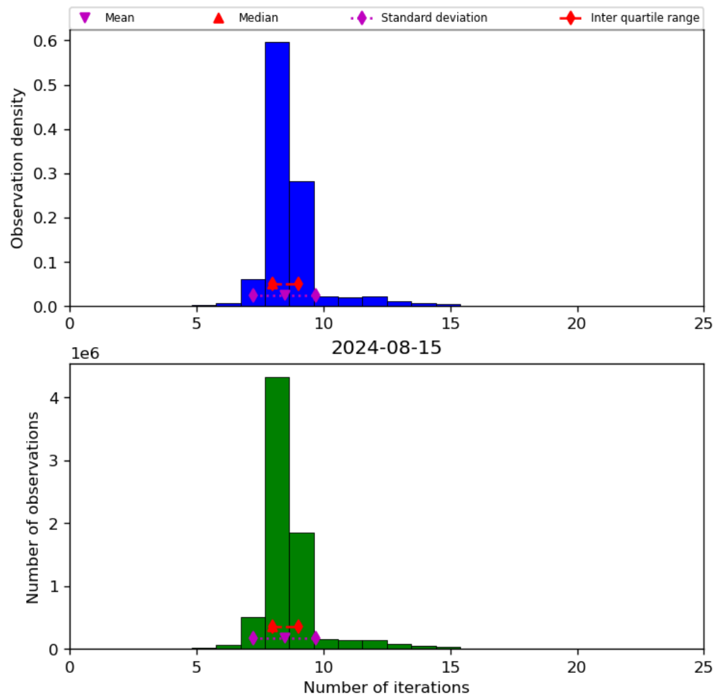
Figure 24: Histogram of “Number of iterations” for 2024-08-14 to 2024-08-16
