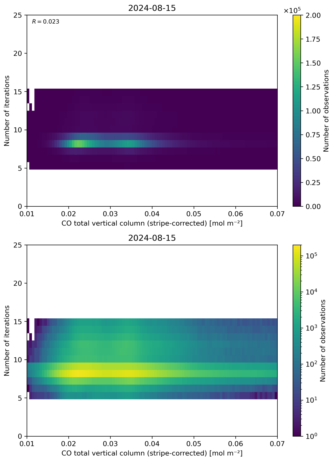
Figure 39: Scatter density plot of “CO total vertical column (stripe-corrected)” against “Number of iterations” for 2024-08-14 to 2024-08-16.
