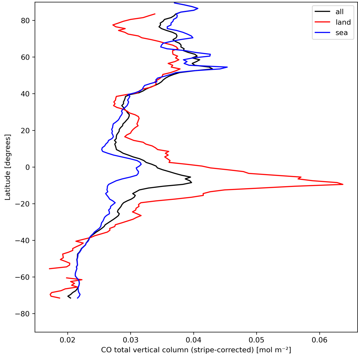
Figure 11: Zonal average of “CO total vertical column (stripe-corrected)” for 2024-08-14 to 2024-08-16.
