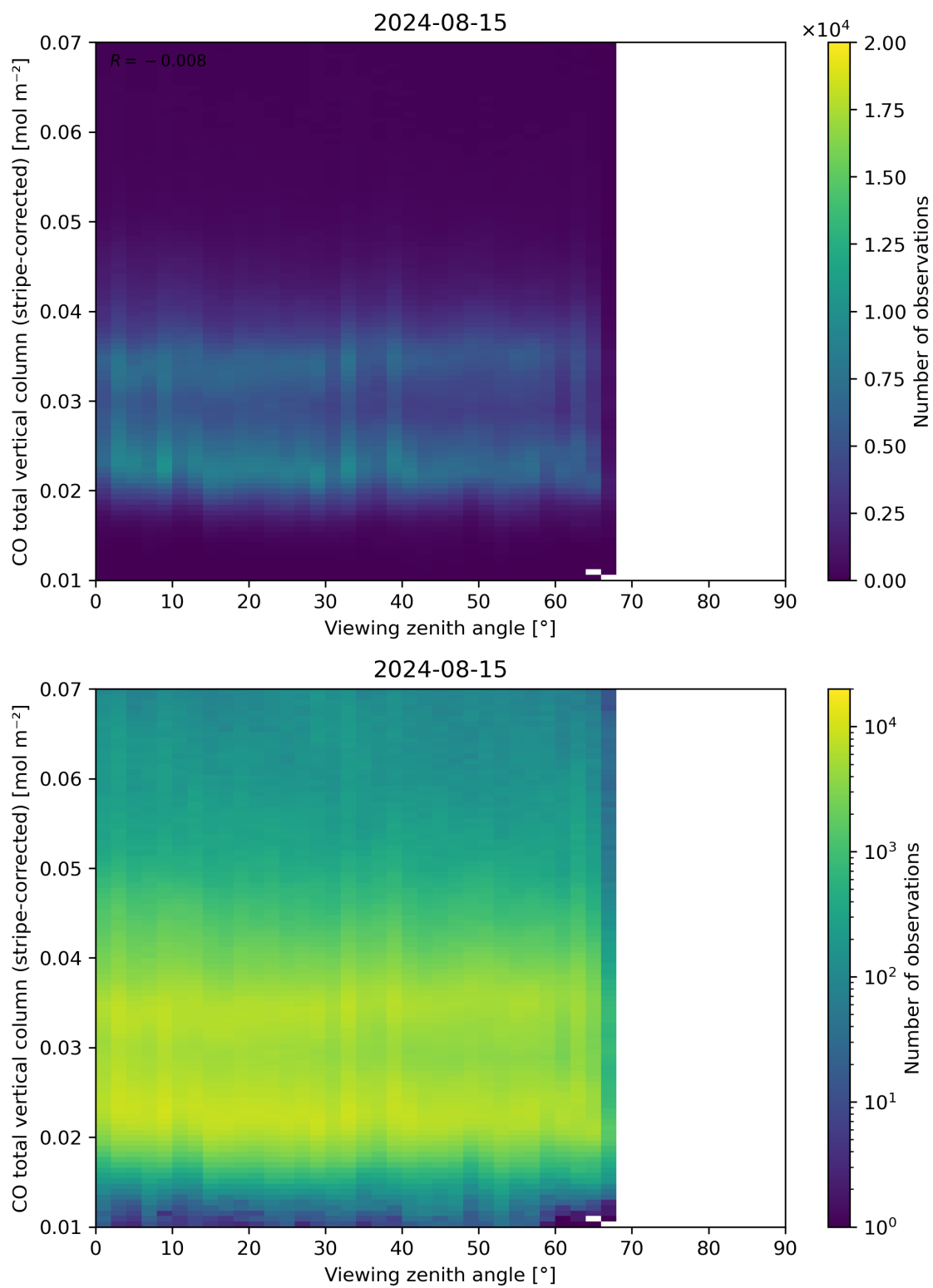
Figure 70: Scatter density plot of “Viewing zenith angle” against “CO total vertical column (stripe-corrected)” for 2024-08-14 to 2024-08-16.
