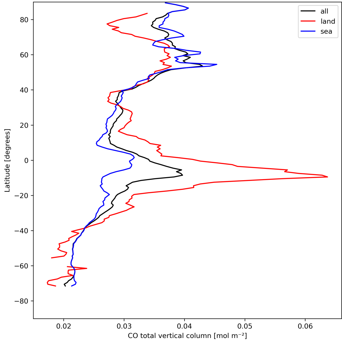
Figure 10: Zonal average of “CO total vertical column” for 2024-08-14 to 2024-08-16.
