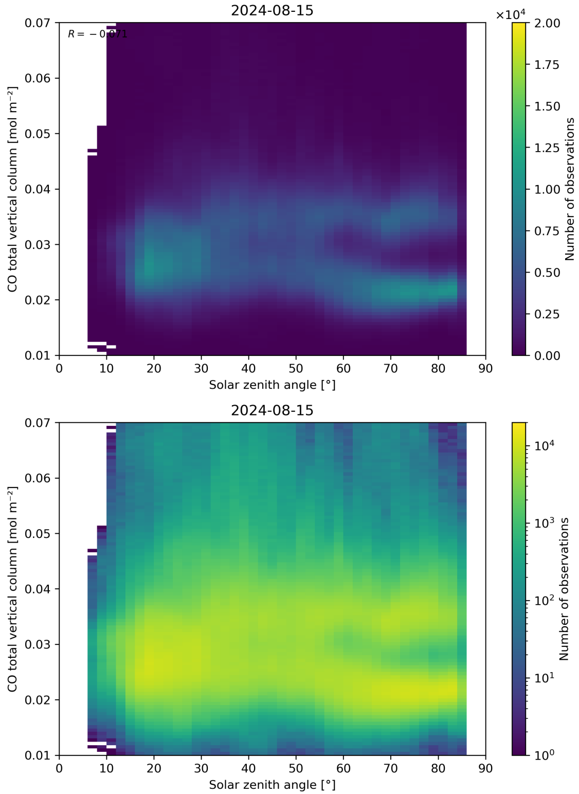
Figure 61: Scatter density plot of “Solar zenith angle” against “CO total vertical column” for 2024-08-14 to 2024-08-16.
