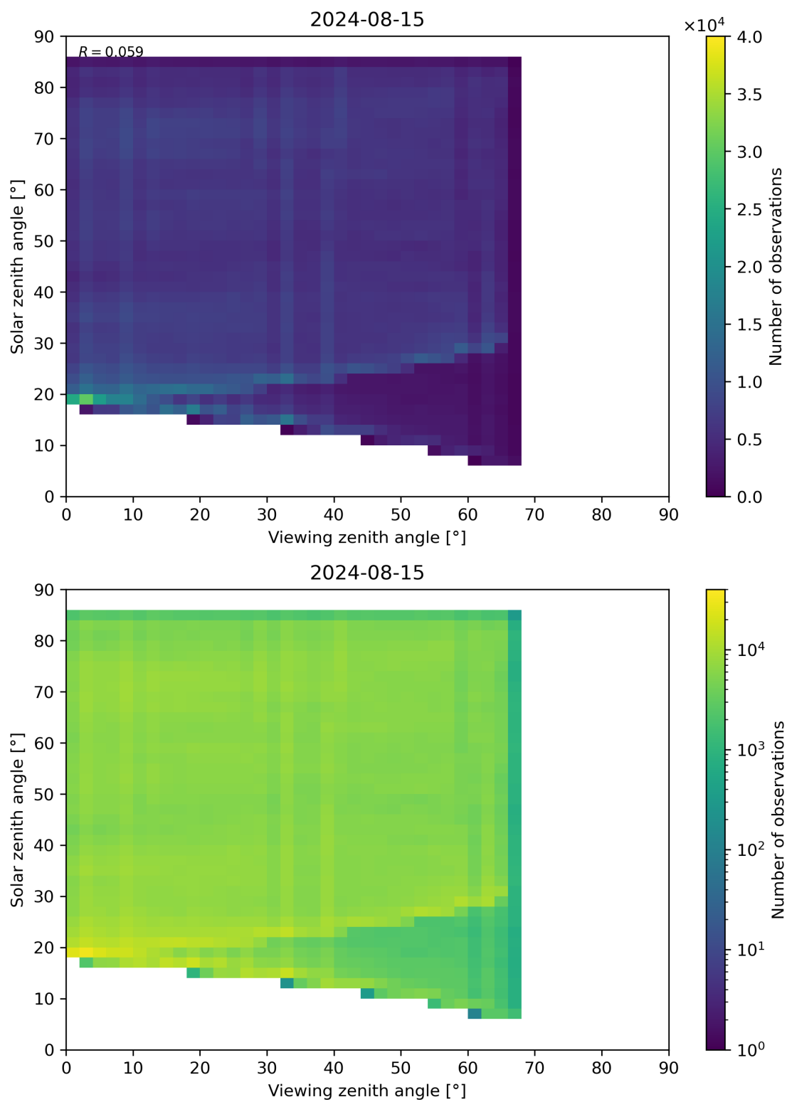
Figure 77: Scatter density plot of “Viewing zenith angle” against “Solar zenith angle” for 2024-08-14 to 2024-08-16.
