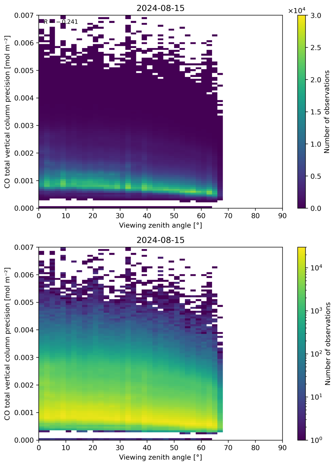
Figure 71: Scatter density plot of “Viewing zenith angle” against “CO total vertical column precision” for 2024-08-14 to 2024-08-16.
