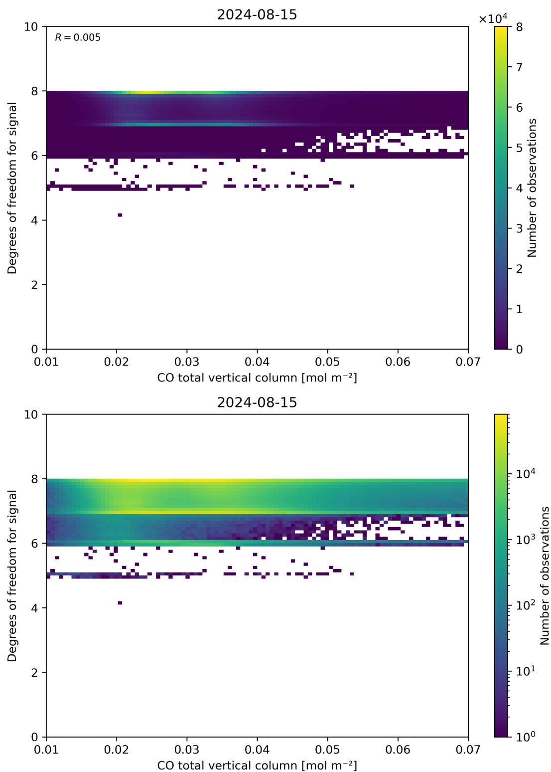
Figure 41: Scatter density plot of “CO total vertical column” against “Degrees of freedom for signal” for 2024-08-14 to 2024-08-16.
