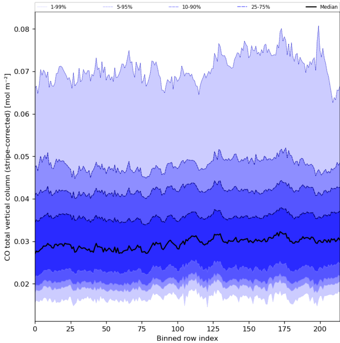
Figure 27: Along track statistics of “CO total vertical column (stripe-corrected)” for 2024-08-14 to 2024-08-16
