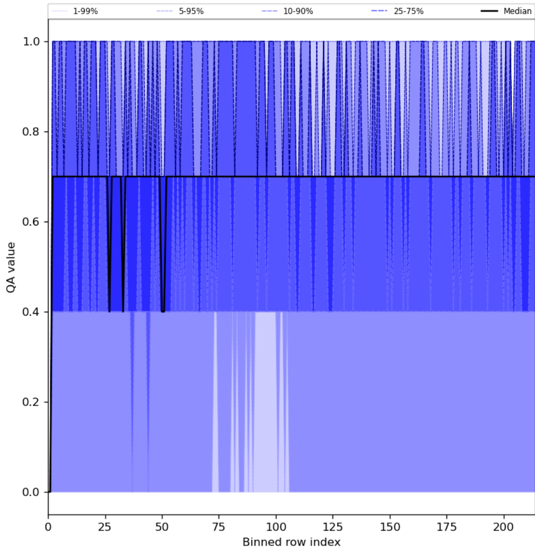
Figure 25: Along track statistics of “QA value” for 2024-08-14 to 2024-08-16
