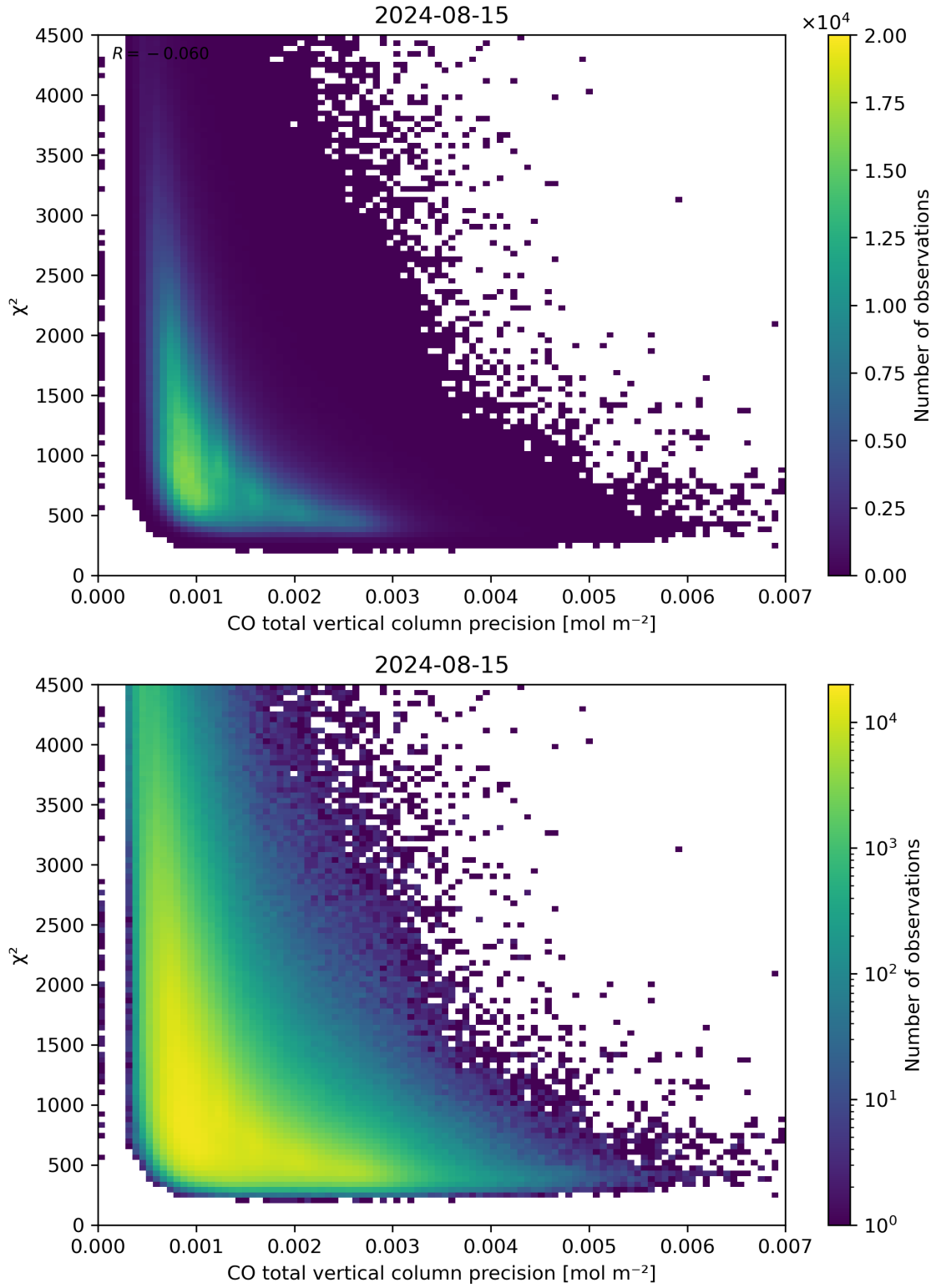
Figure 44: Scatter density plot of “CO total vertical column precision” against “ \chi^2 ” for 2024-08-14 to 2024-08-16.
