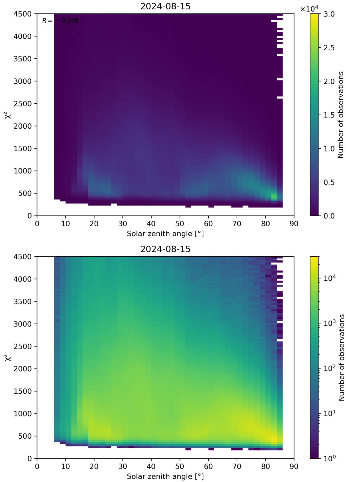
Figure 64: Scatter density plot of “Solar zenith angle” against “ \chi^2 ” for 2024-08-14 to 2024-08-16.
