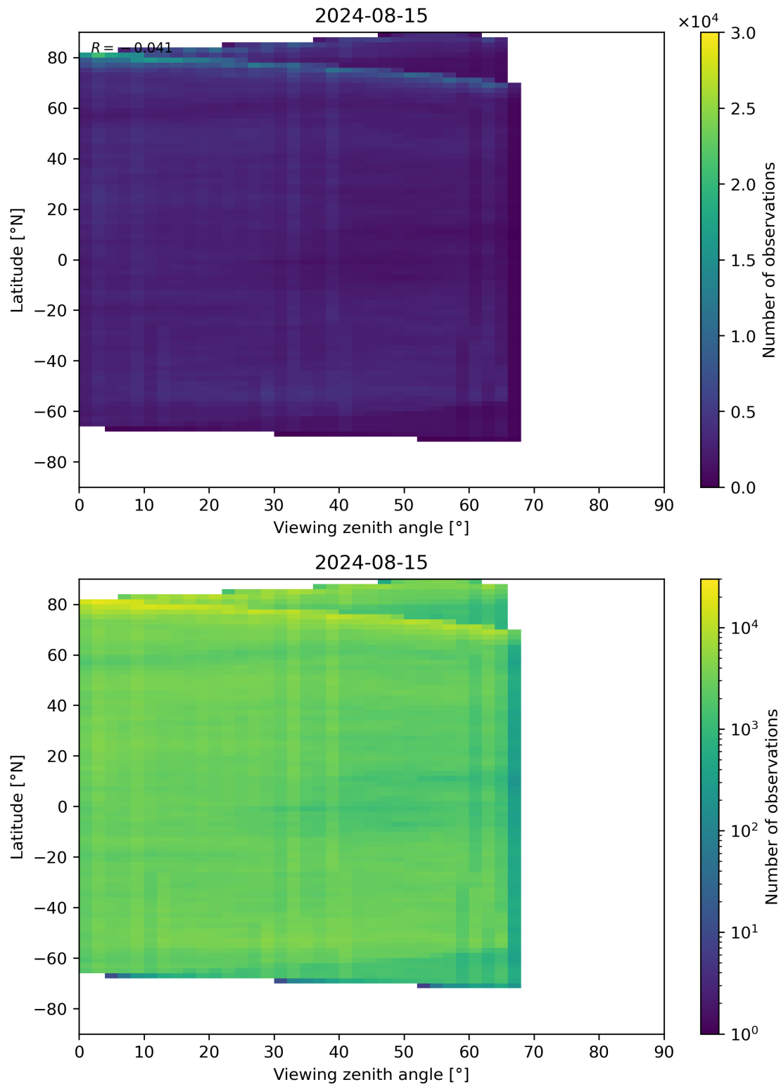
Figure 74: Scatter density plot of “Viewing zenith angle” against “Latitude” for 2024-08-14 to 2024-08-16.
