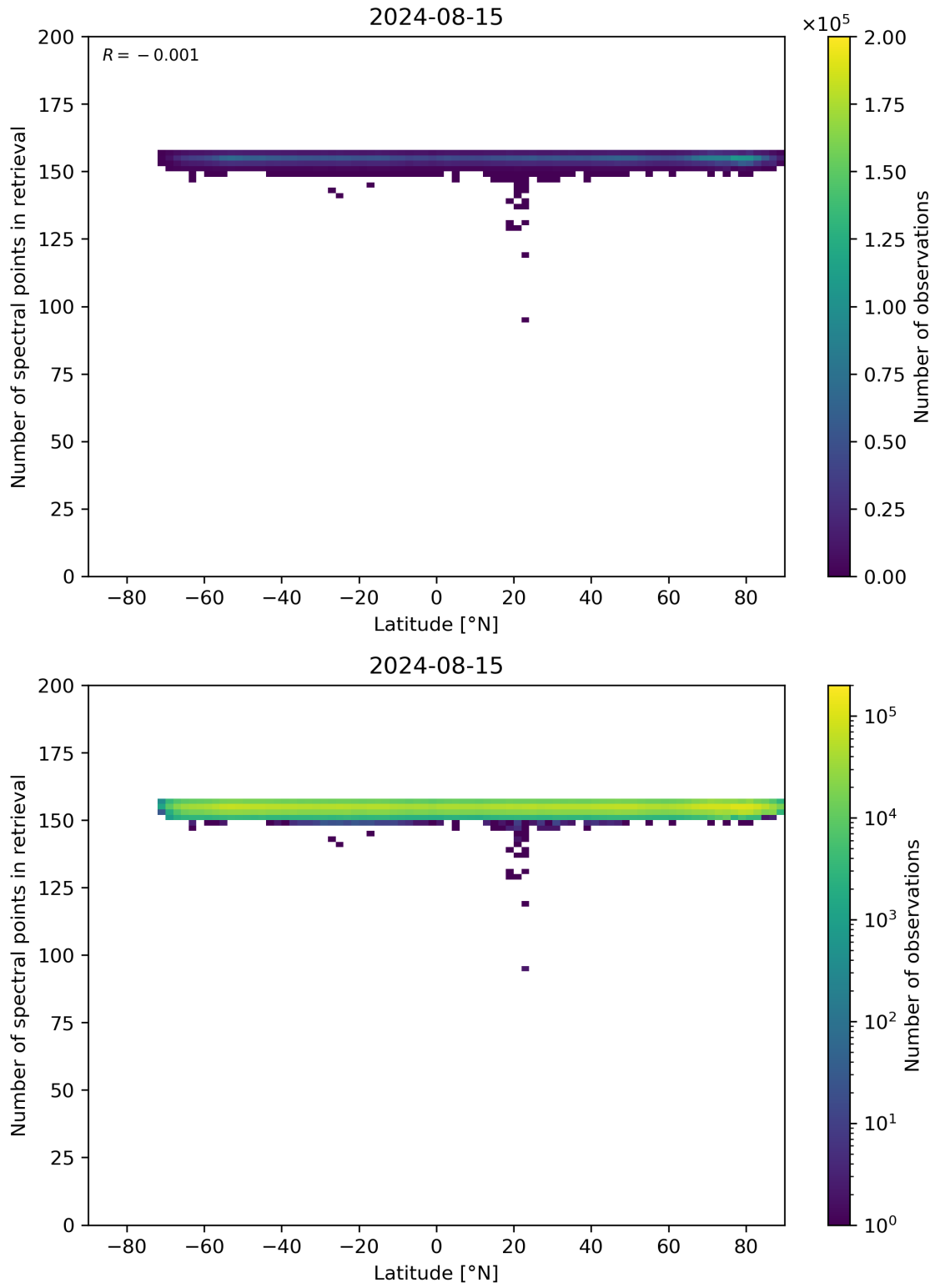
Figure 57: Scatter density plot of “Latitude” against “Number of spectral points in retrieval” for 2024-08-14 to 2024-08-16.
