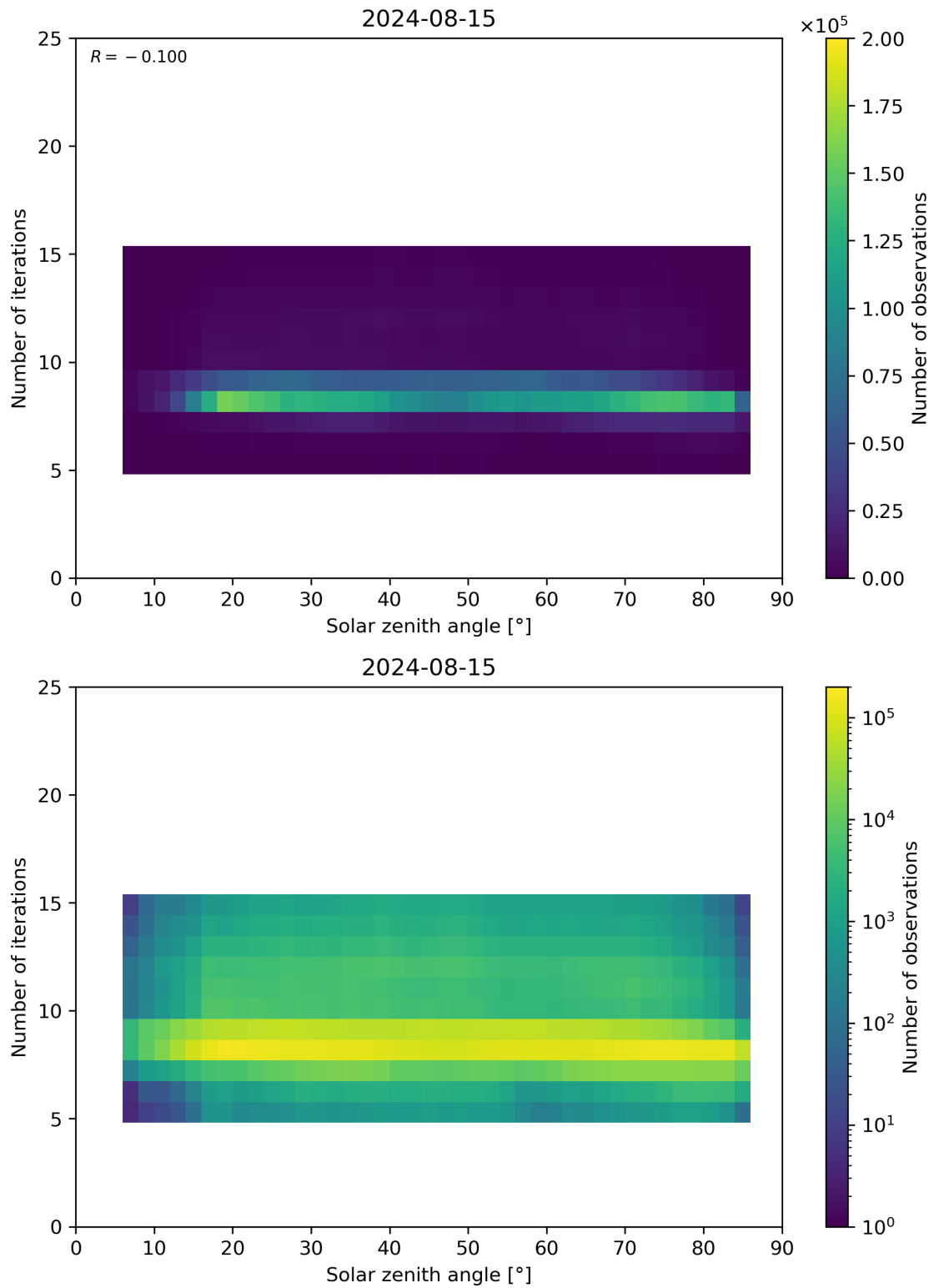
Figure 67: Scatter density plot of “Solar zenith angle” against “Number of iterations” for 2024-08-14 to 2024-08-16.
