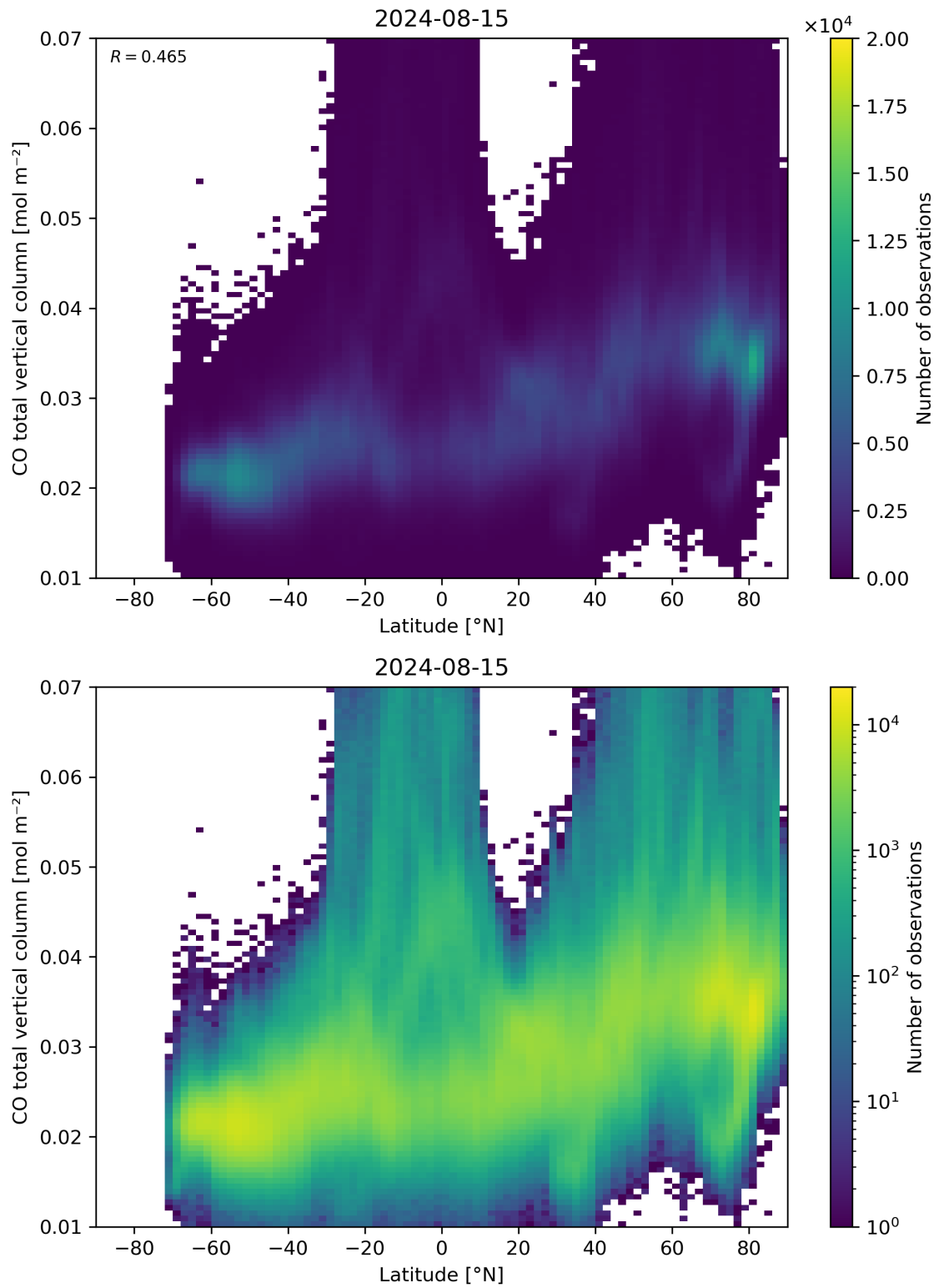
Figure 51: Scatter density plot of “Latitude” against “CO total vertical column” for 2024-08-14 to 2024-08-16.
