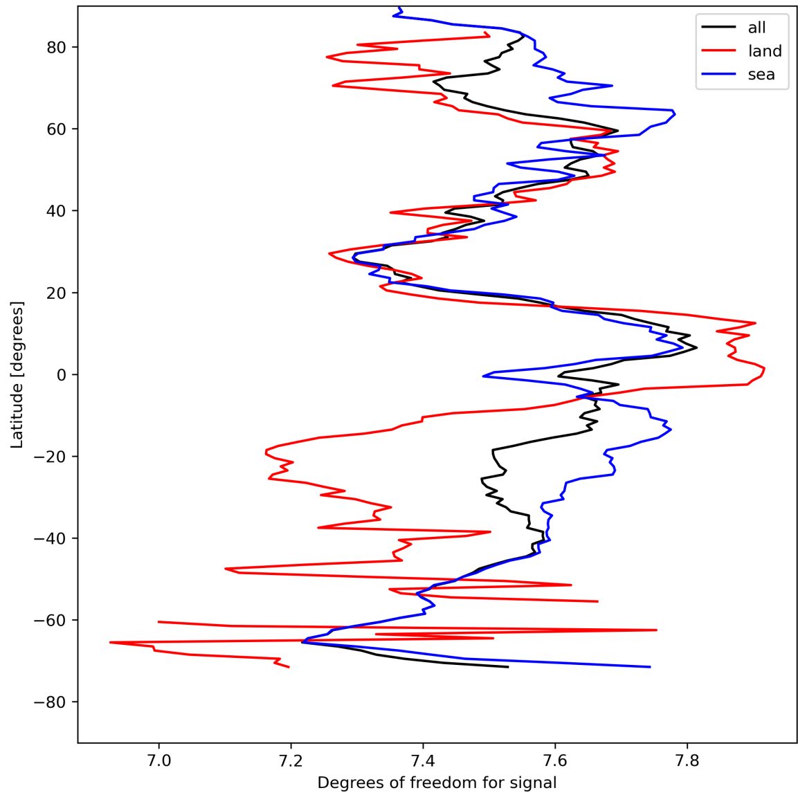
Figure 15: Zonal average of “Degrees of freedom for signal” for 2024-08-14 to 2024-08-16.
