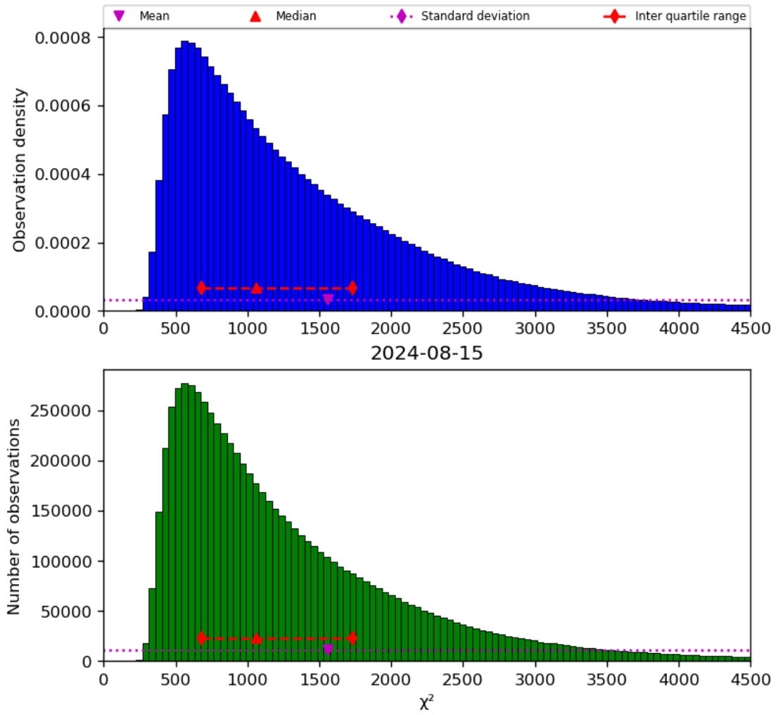
Figure 22: Histogram of “ \chi^2 ” for 2024-08-14 to 2024-08-16
