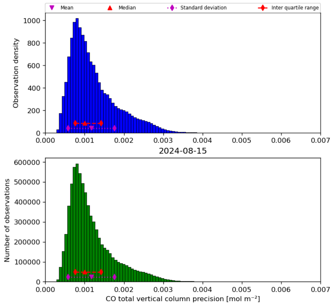
Figure 20: Histogram of “CO total vertical column precision” for 2024-08-14 to 2024-08-16
