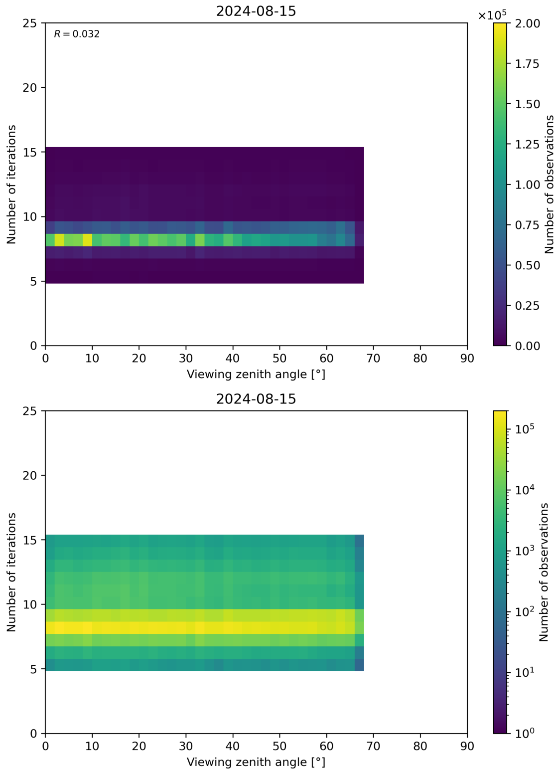
Figure 75: Scatter density plot of “Viewing zenith angle” against “Number of iterations” for 2024-08-14 to 2024-08-16.
