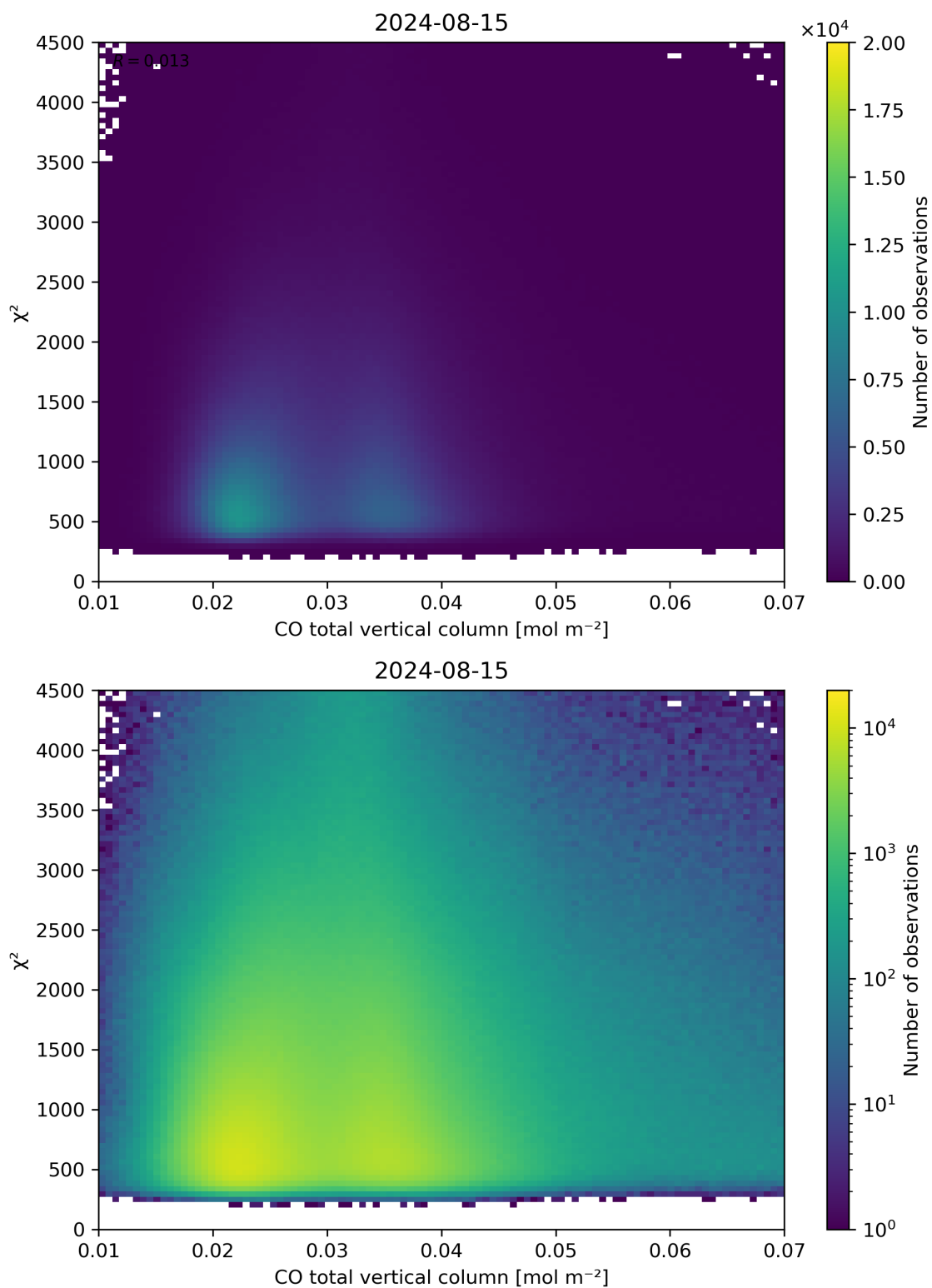
Figure 35: Scatter density plot of “CO total vertical column” against “ \chi^2 ” for 2024-08-14 to 2024-08-16.
