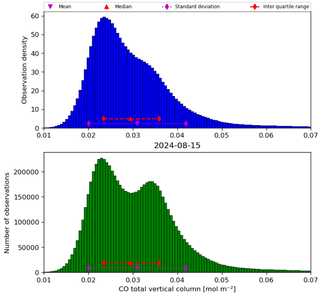
Figure 18: Histogram of “CO total vertical column” for 2024-08-14 to 2024-08-16
