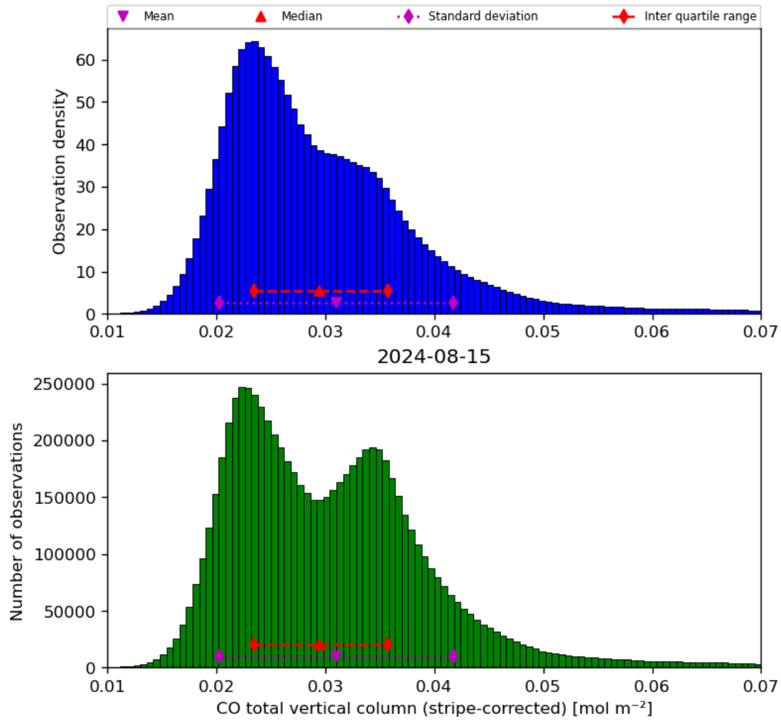
Figure 19: Histogram of “CO total vertical column (stripe-corrected)” for 2024-08-14 to 2024-08-16
