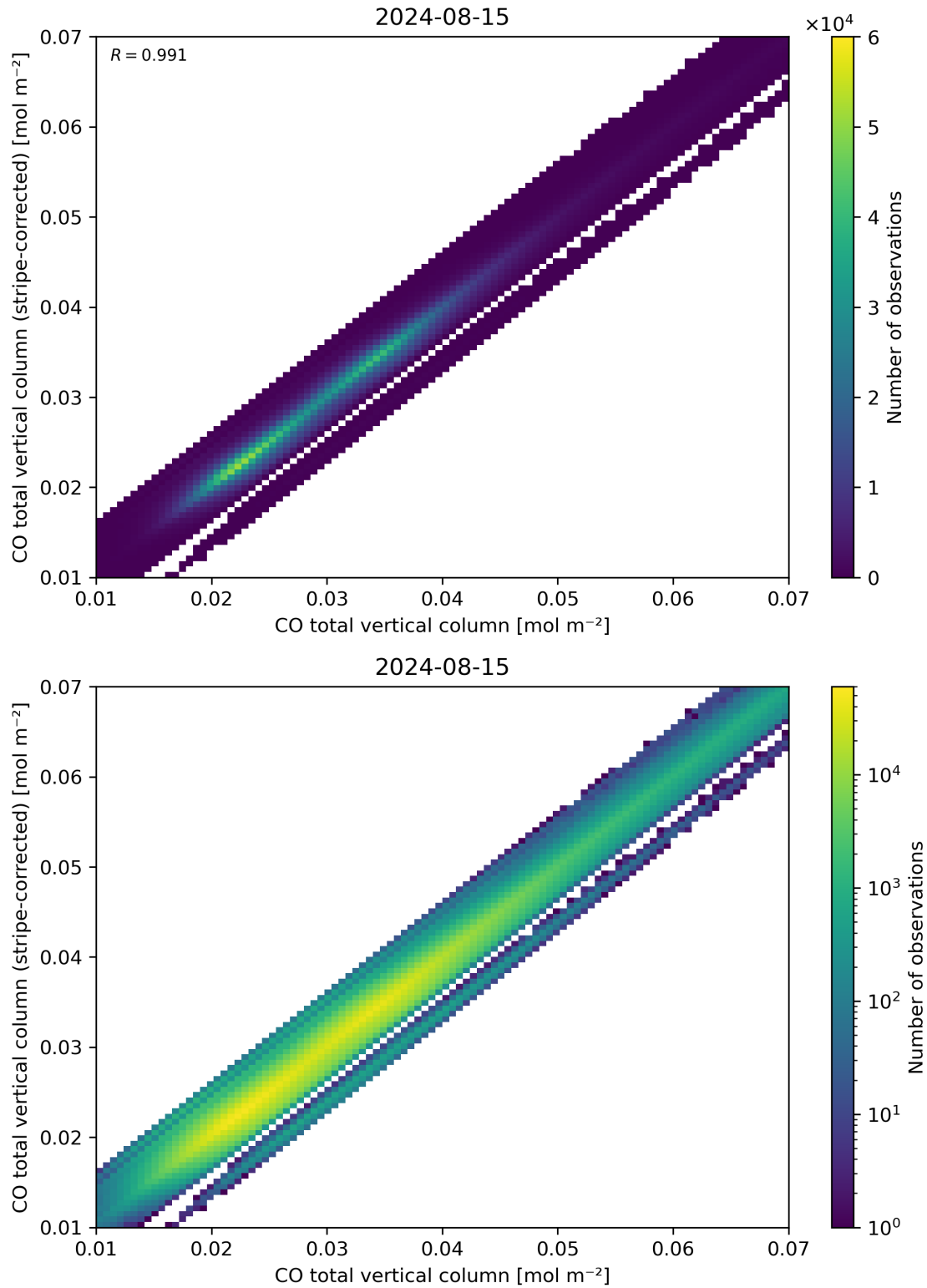
Figure 33: Scatter density plot of “CO total vertical column” against “CO total vertical column (stripe-corrected)” for 2024-08-14 to 2024-08-16.
