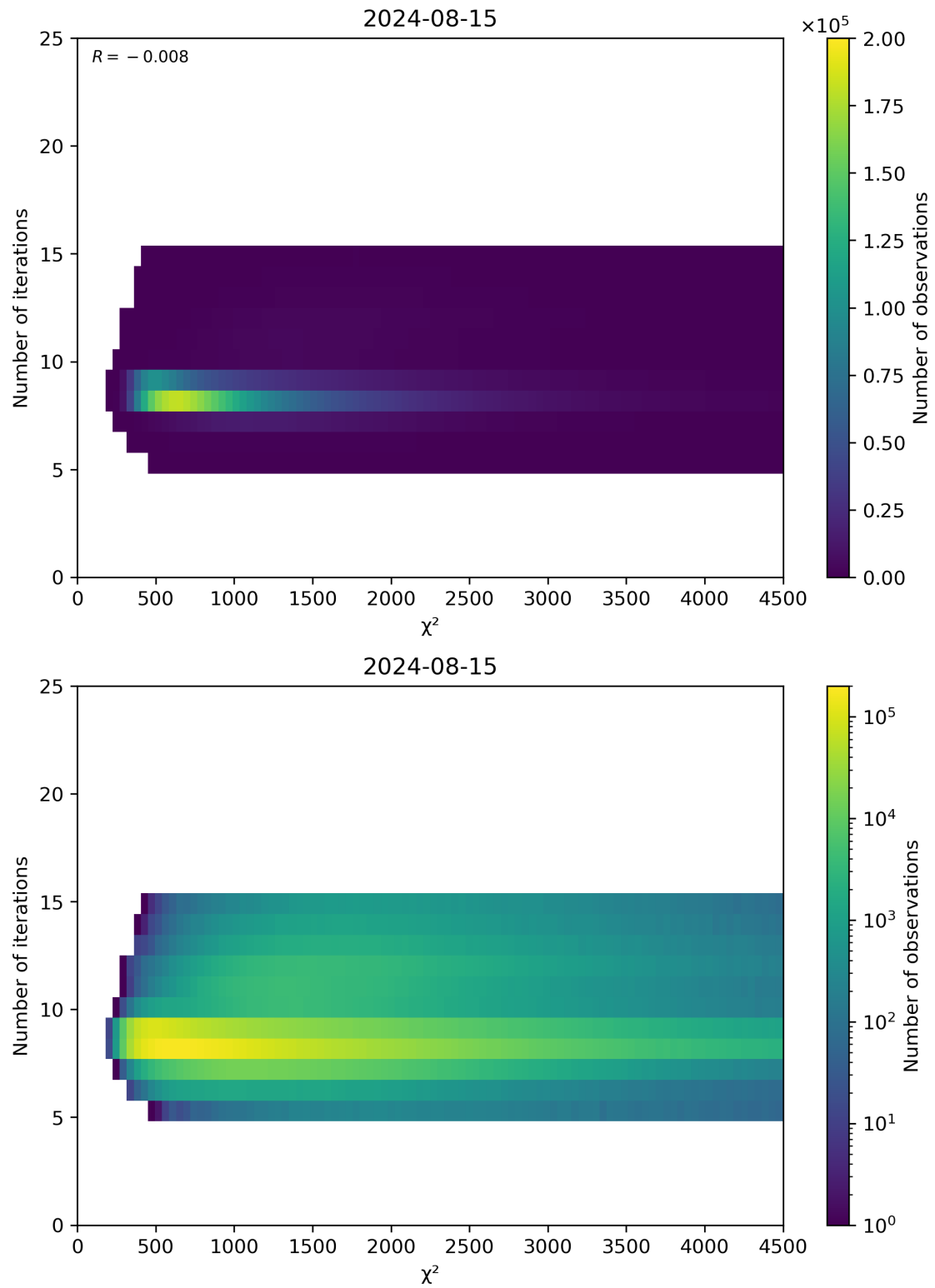
Figure 49: Scatter density plot of “ \chi^2 ” against “Number of iterations” for 2024-08-14 to 2024-08-16.
