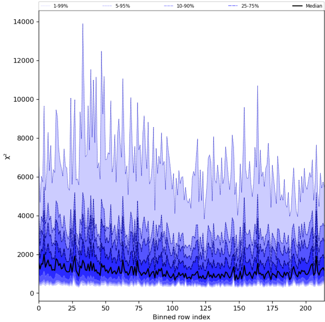
Figure 30: Along track statistics of “ \chi^2 ” for 2024-08-14 to 2024-08-16
