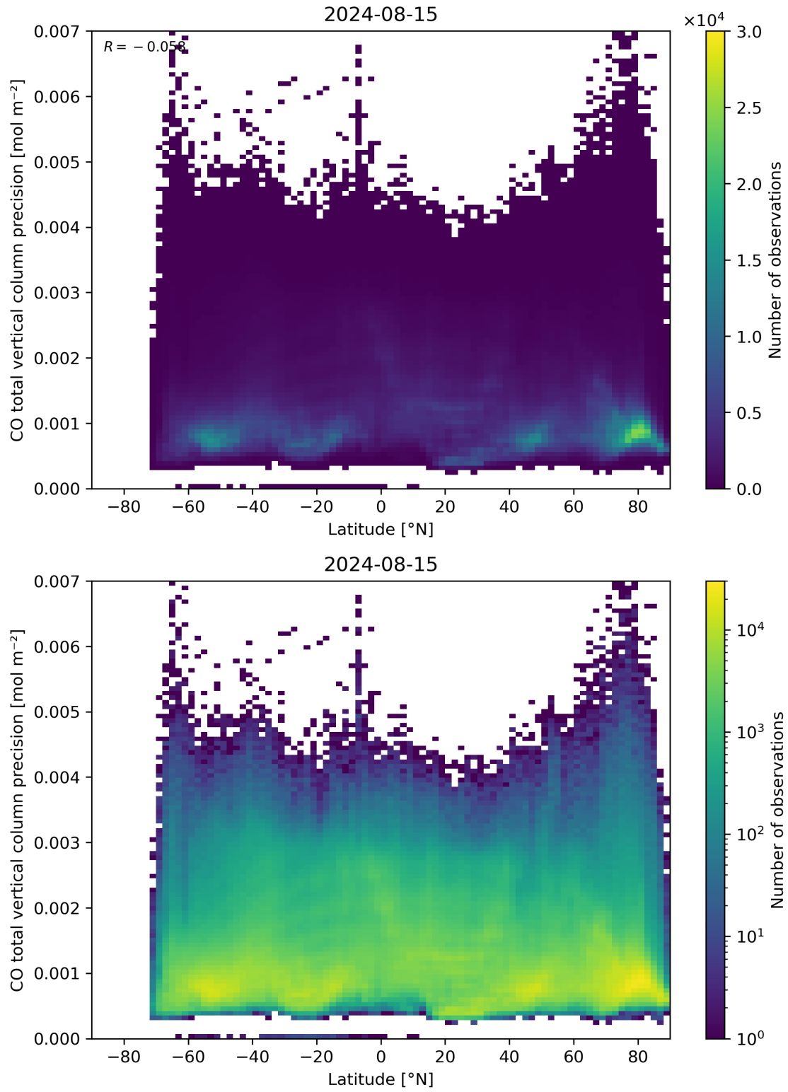
Figure 53: Scatter density plot of “Latitude” against “CO total vertical column precision” for 2024-08-14 to 2024-08-16.
