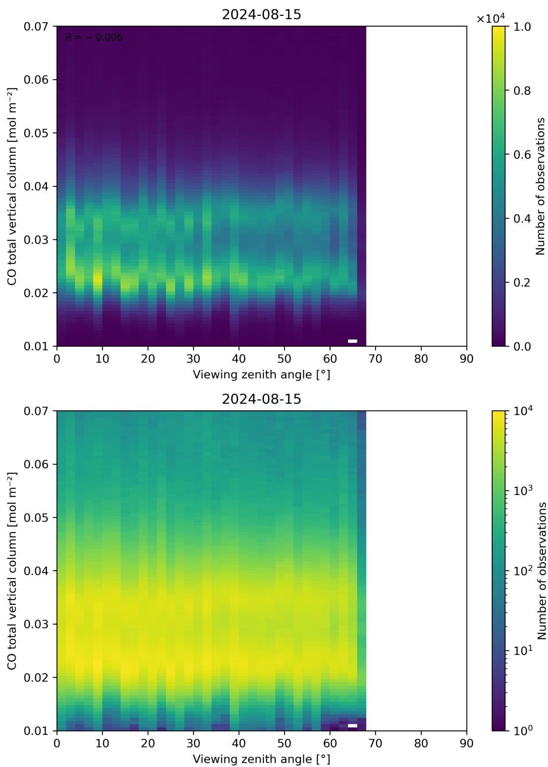
Figure 69: Scatter density plot of “Viewing zenith angle” against “CO total vertical column” for 2024-08-14 to 2024-08-16.
