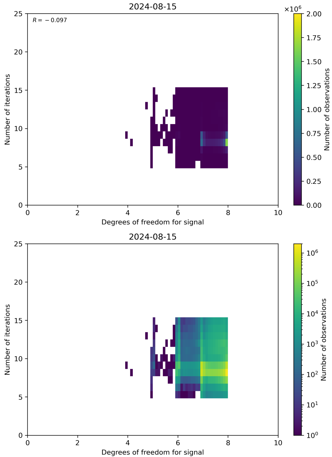
Figure 50: Scatter density plot of “Degrees of freedom for signal” against “Number of iterations” for 2024-08-14 to 2024-08-16.
