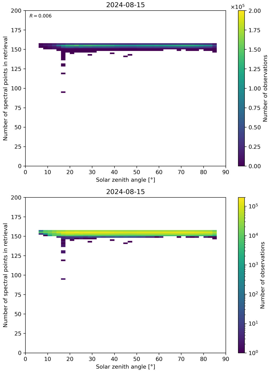
Figure 68: Scatter density plot of “Solar zenith angle” against “Number of spectral points in retrieval” for 2024-08-14 to 2024-08-16.
