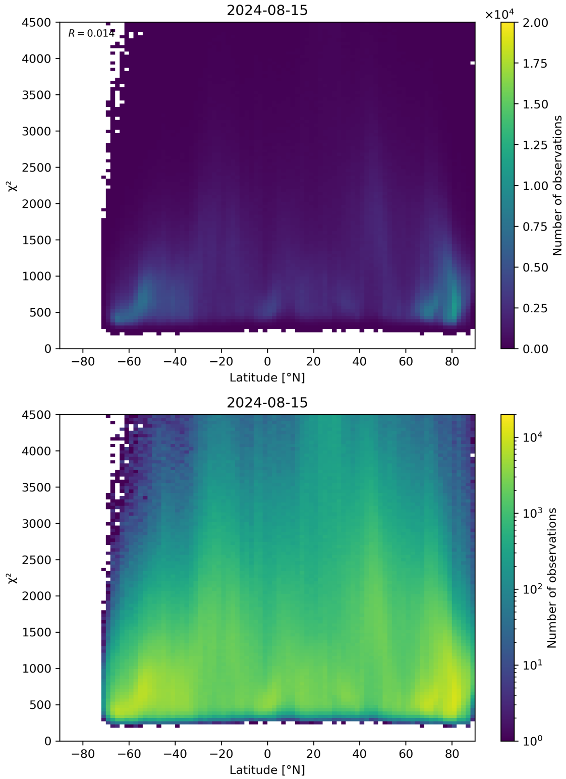
Figure 54: Scatter density plot of “Latitude” against “ \chi^2 ” for 2024-08-14 to 2024-08-16.
