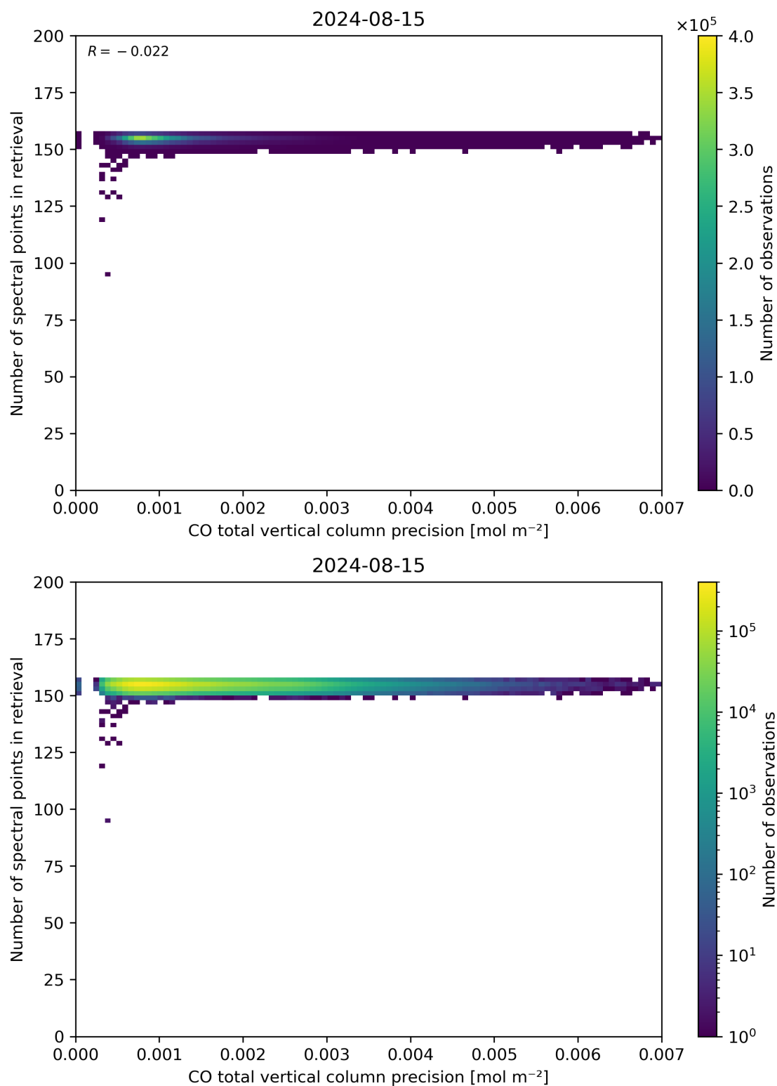
Figure 47: Scatter density plot of “CO total vertical column precision” against “Number of spectral points in retrieval” for 2024-08-14 to 2024-08-16.
