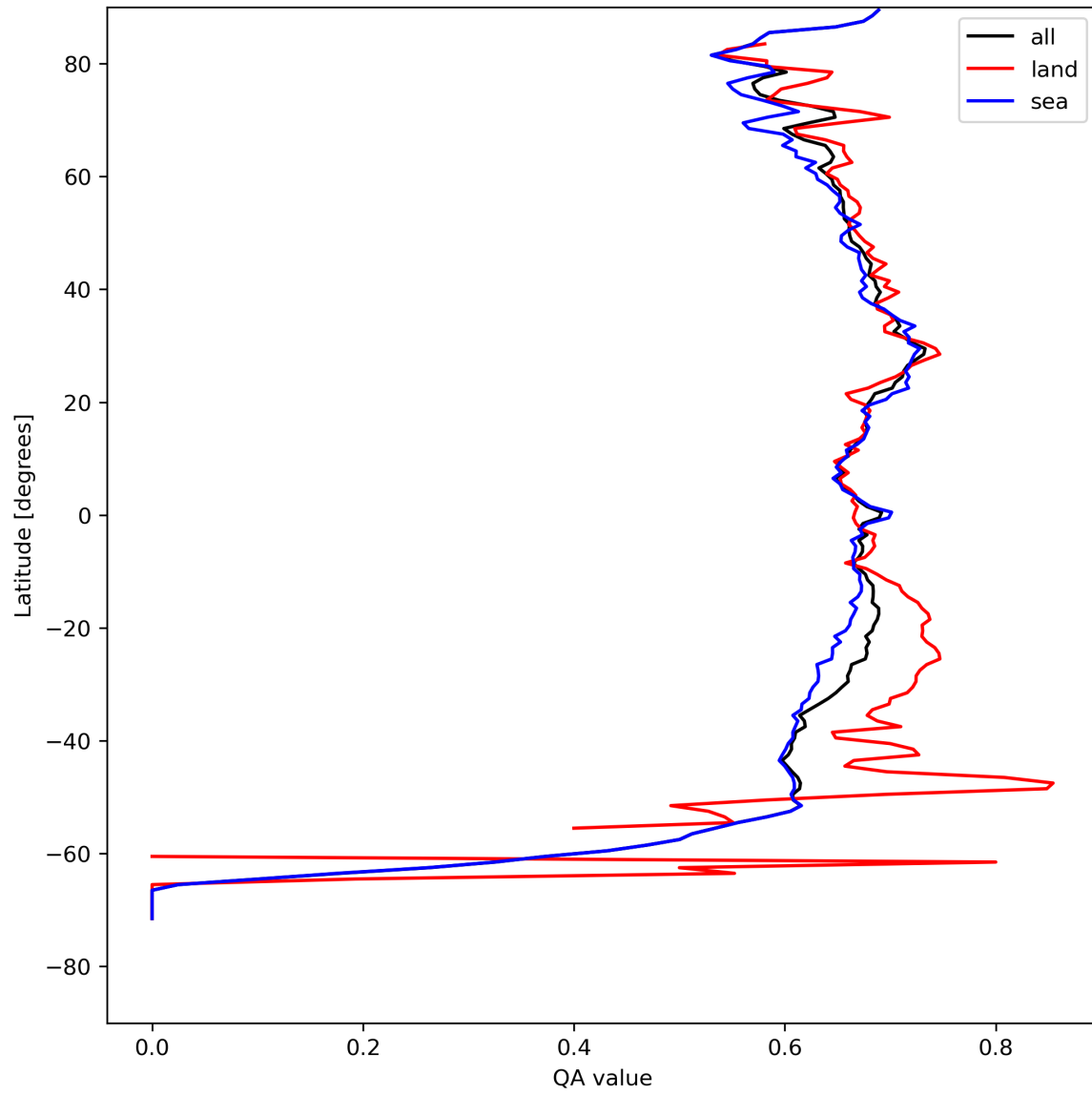
Figure 9: Zonal average of “QA value” for 2024-08-14 to 2024-08-16.
