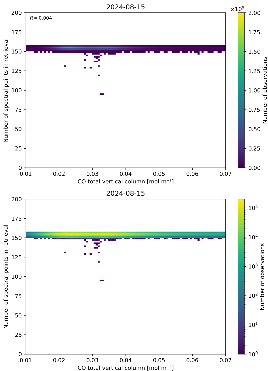
Figure 43: Scatter density plot of “CO total vertical column” against “Number of spectral points in retrieval” for 2024-08-14 to 2024-08-16.
