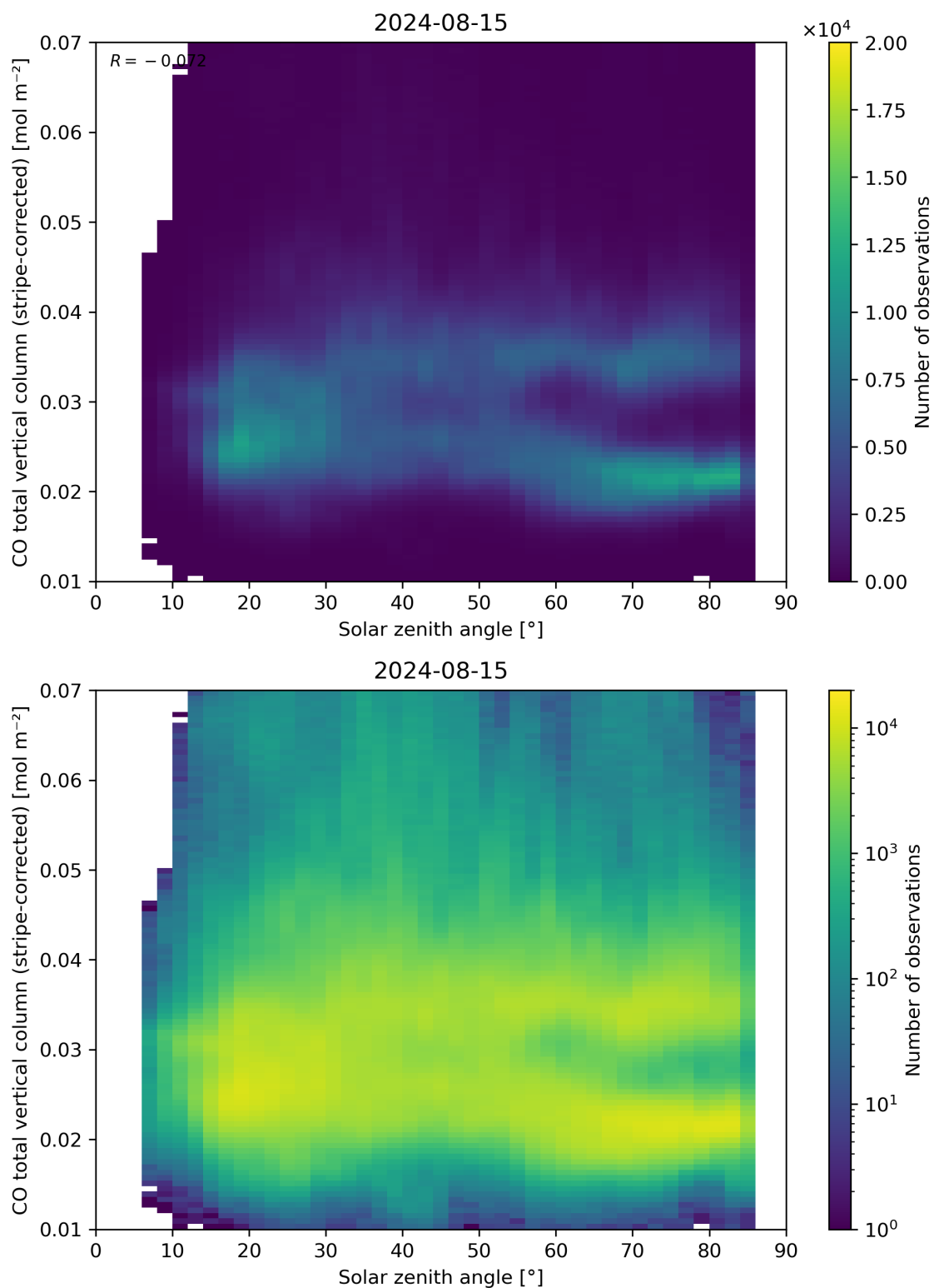
Figure 62: Scatter density plot of “Solar zenith angle” against “CO total vertical column (stripe-corrected)” for 2024-08-14 to 2024-08-16.
