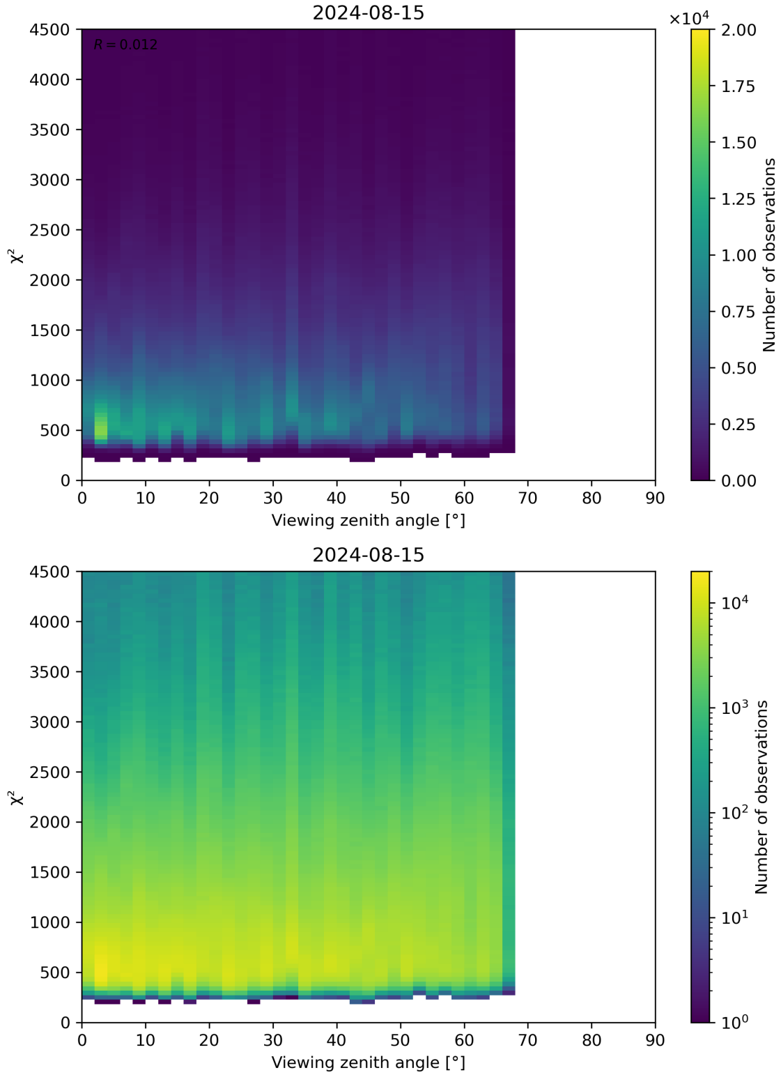
Figure 72: Scatter density plot of “Viewing zenith angle” against “ \chi^2 ” for 2024-08-14 to 2024-08-16.
