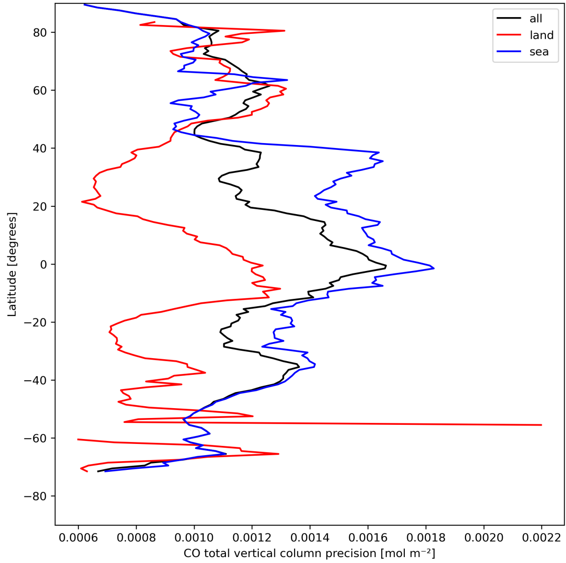
Figure 12: Zonal average of “CO total vertical column precision” for 2024-08-14 to 2024-08-16.
