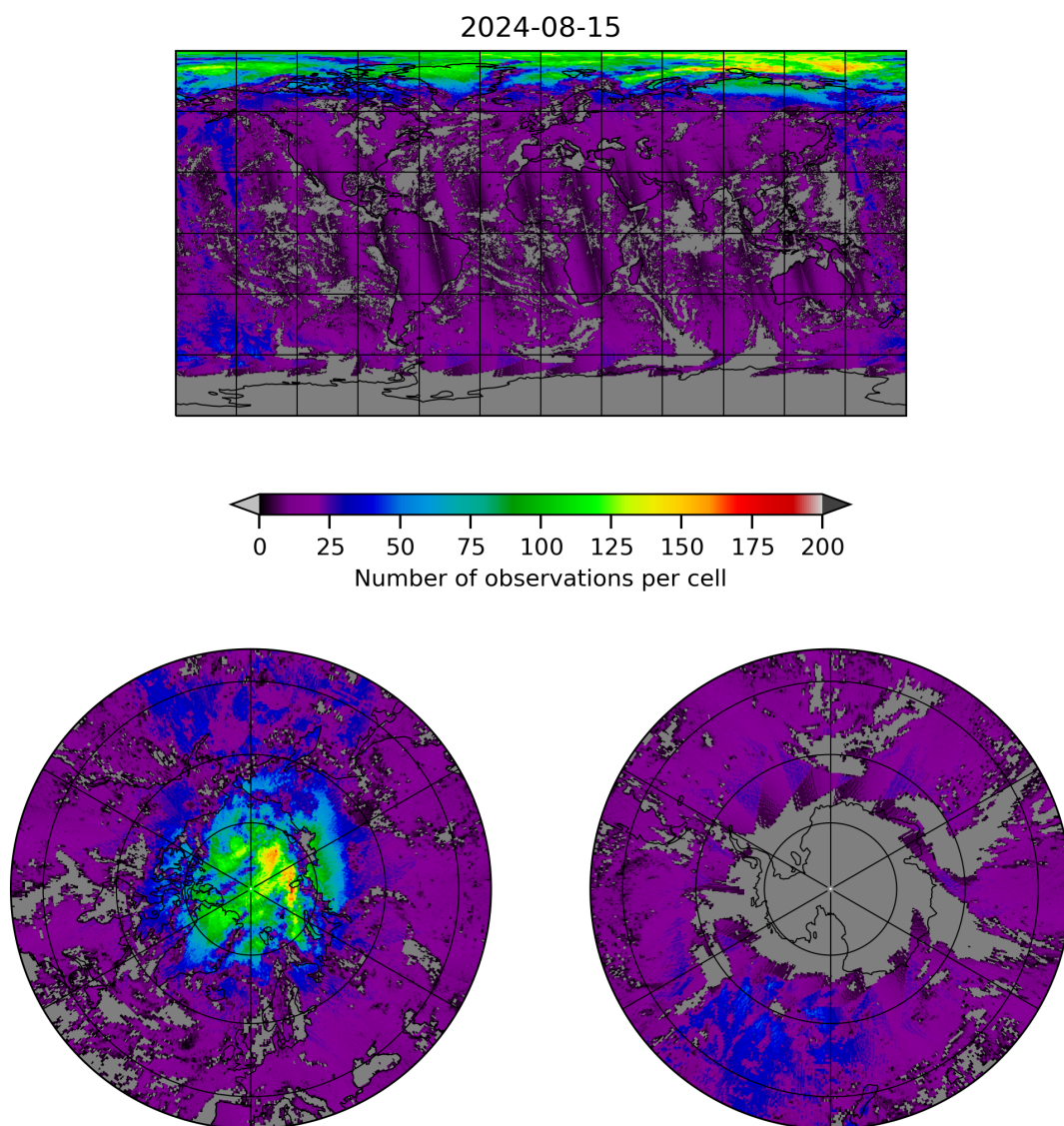
Figure 8: Map of the number of observations for 2024-08-14 to 2024-08-16
