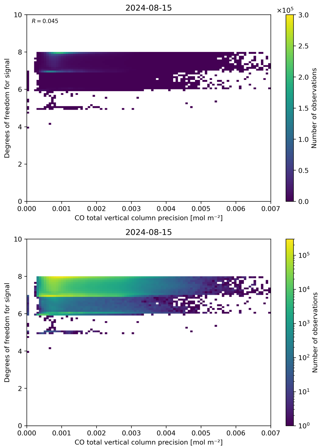
Figure 45: Scatter density plot of “CO total vertical column precision” against “Degrees of freedom for signal” for 2024-08-14 to 2024-08-16.
