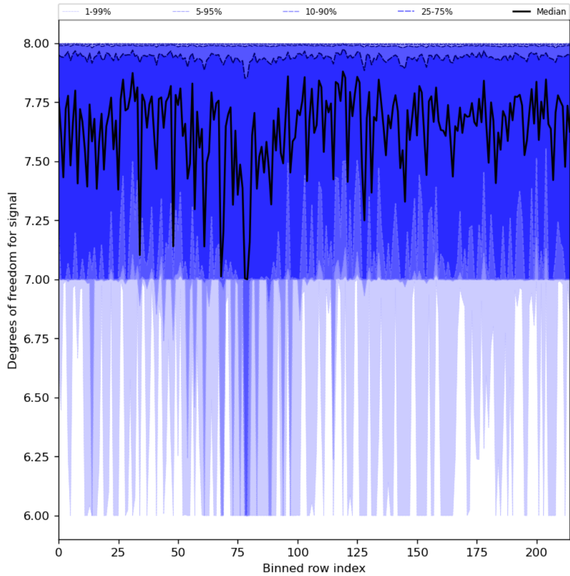
Figure 31: Along track statistics of “Degrees of freedom for signal” for 2024-08-14 to 2024-08-16
