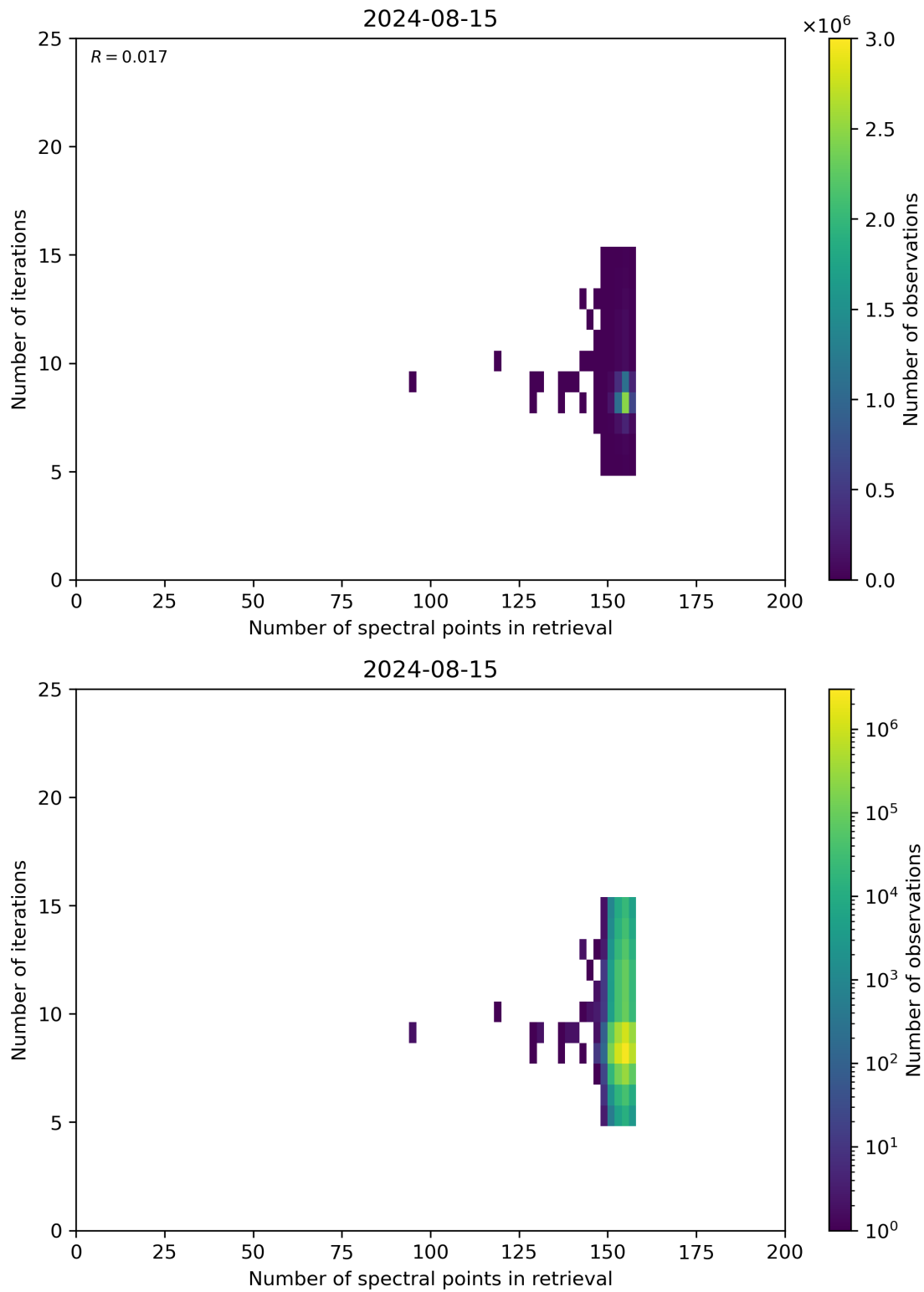
Figure 60: Scatter density plot of “Number of spectral points in retrieval” against “Number of iterations” for 2024-08-14 to 2024-08-16.
