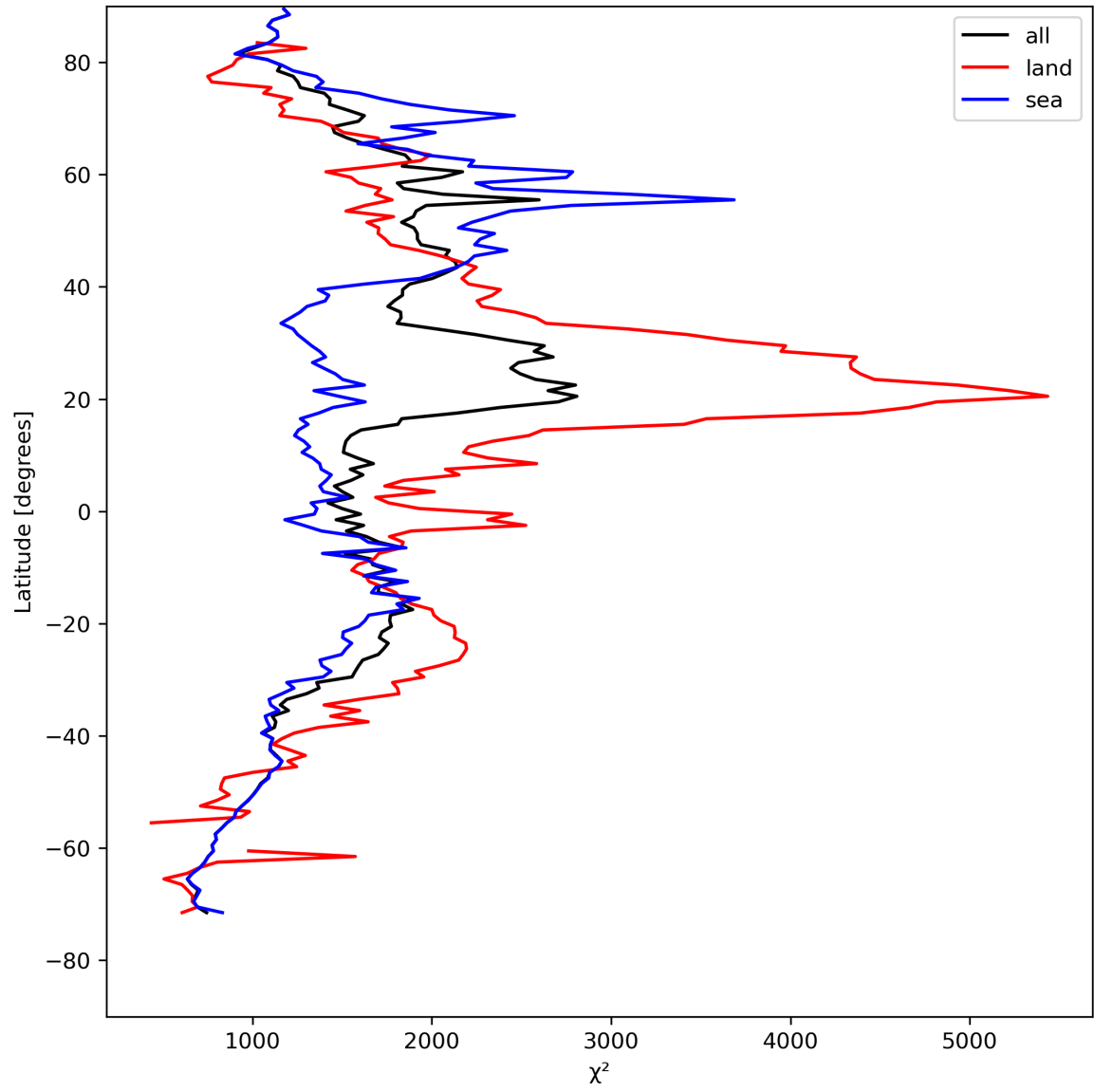
Figure 14: Zonal average of “ \chi^2 ” for 2024-08-14 to 2024-08-16.
