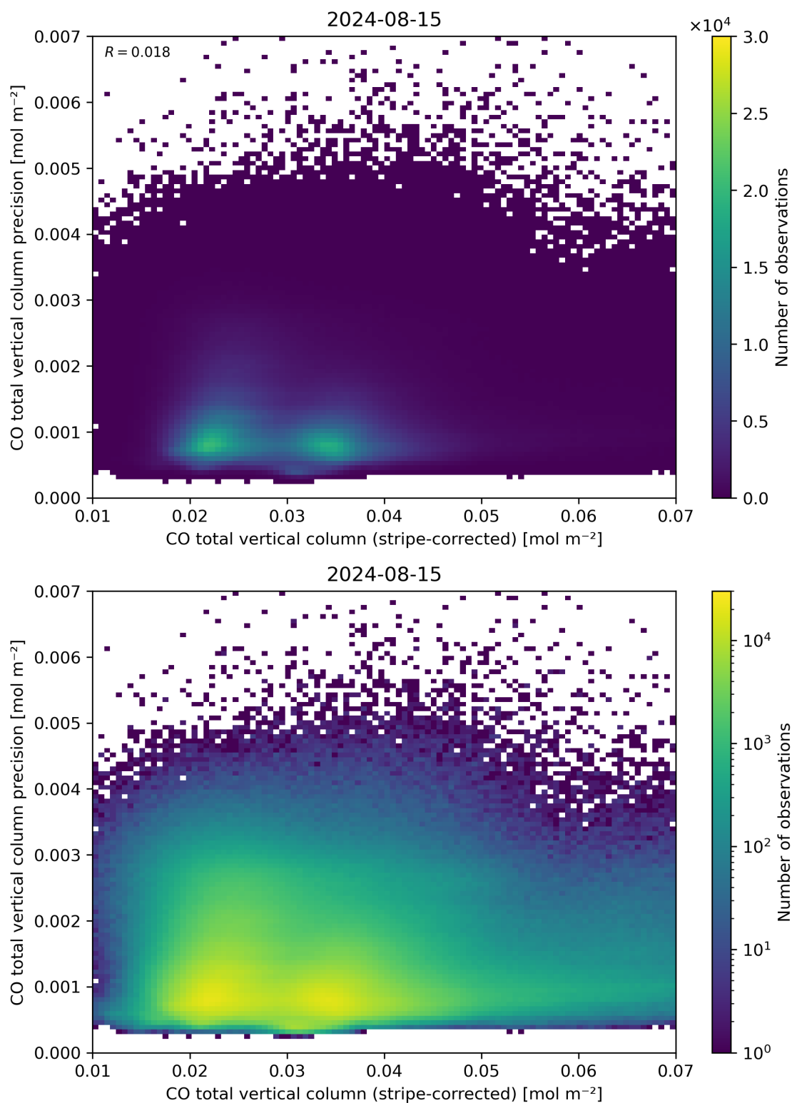
Figure 36: Scatter density plot of “CO total vertical column (stripe-corrected)” against “CO total vertical column precision” for 2024-08-14 to 2024-08-16.
