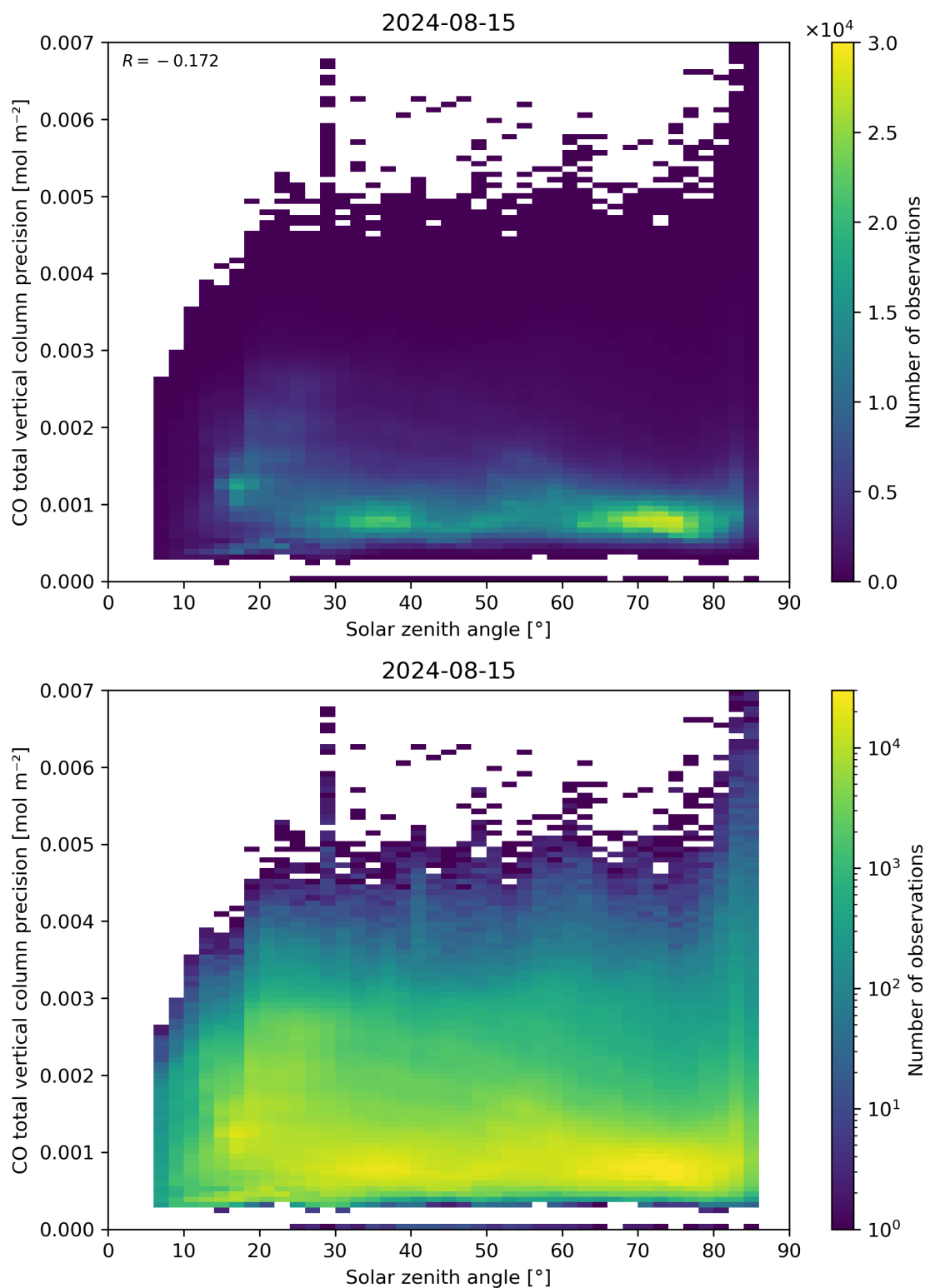
Figure 63: Scatter density plot of “Solar zenith angle” against “CO total vertical column precision” for 2024-08-14 to 2024-08-16.
