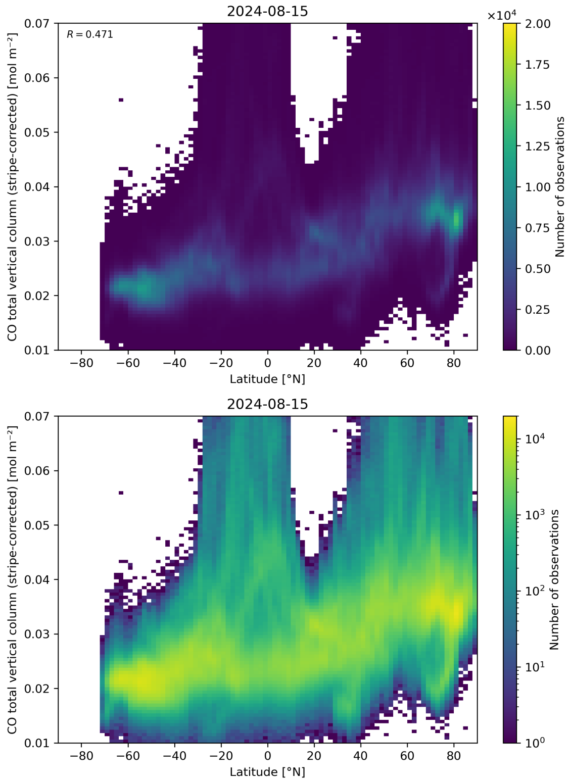
Figure 52: Scatter density plot of “Latitude” against “CO total vertical column (stripe-corrected)” for 2024-08-14 to 2024-08-16.
