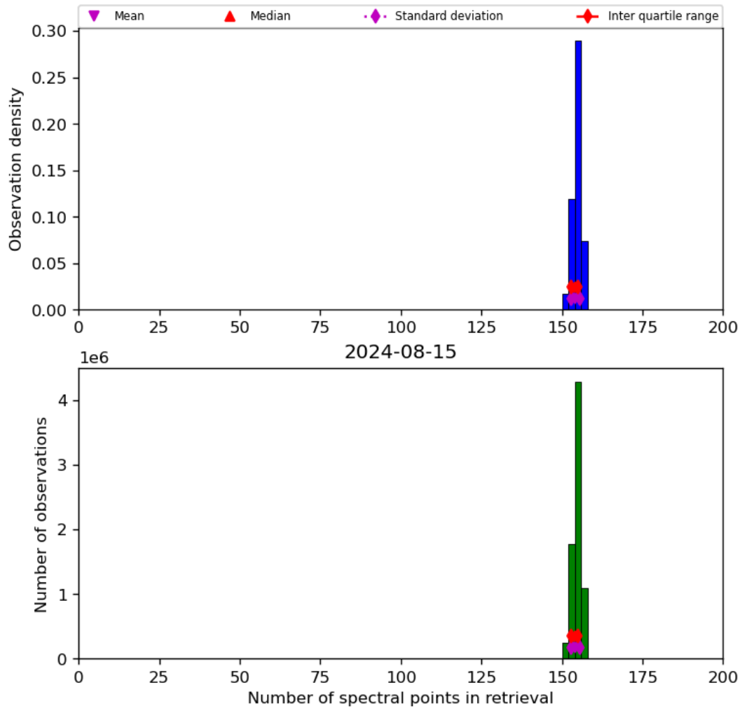
Figure 21: Histogram of “Number of spectral points in retrieval” for 2024-08-14 to 2024-08-16
