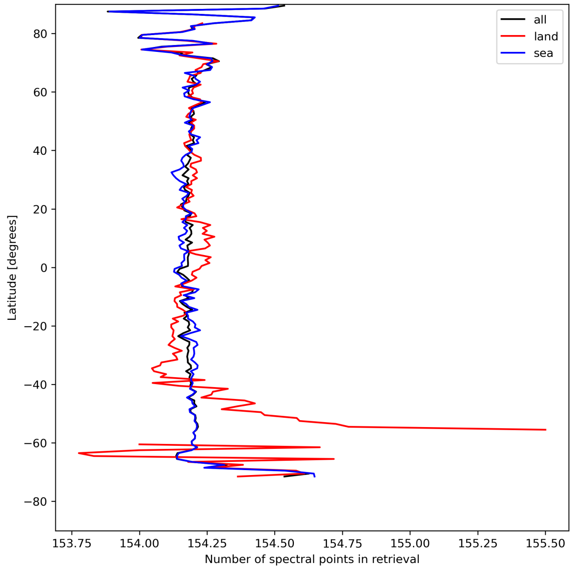
Figure 13: Zonal average of “Number of spectral points in retrieval” for 2024-08-14 to 2024-08-16.
