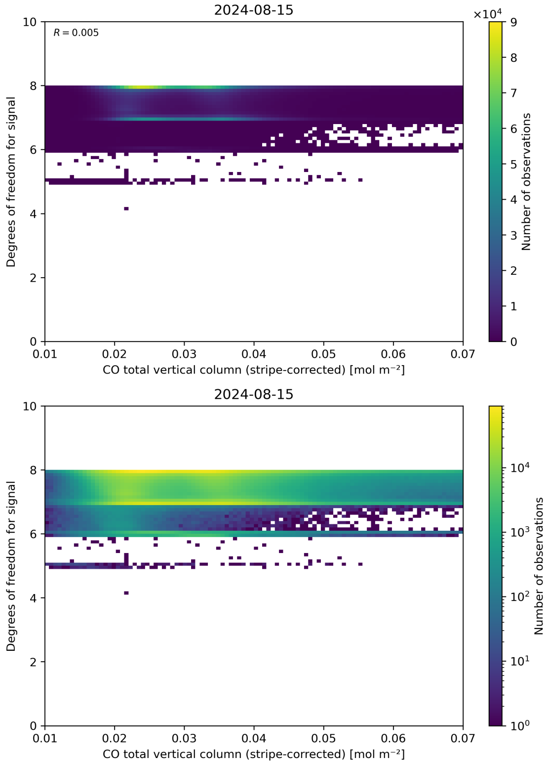
Figure 38: Scatter density plot of “CO total vertical column (stripe-corrected)” against “Degrees of freedom for signal” for 2024-08-14 to 2024-08-16.
