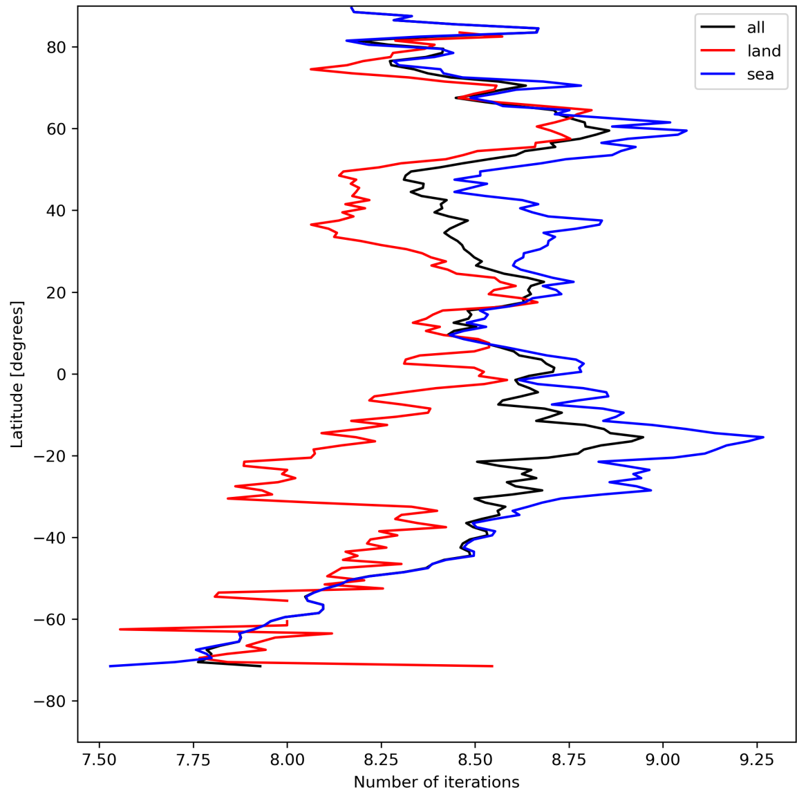
Figure 16: Zonal average of “Number of iterations” for 2024-08-14 to 2024-08-16.
