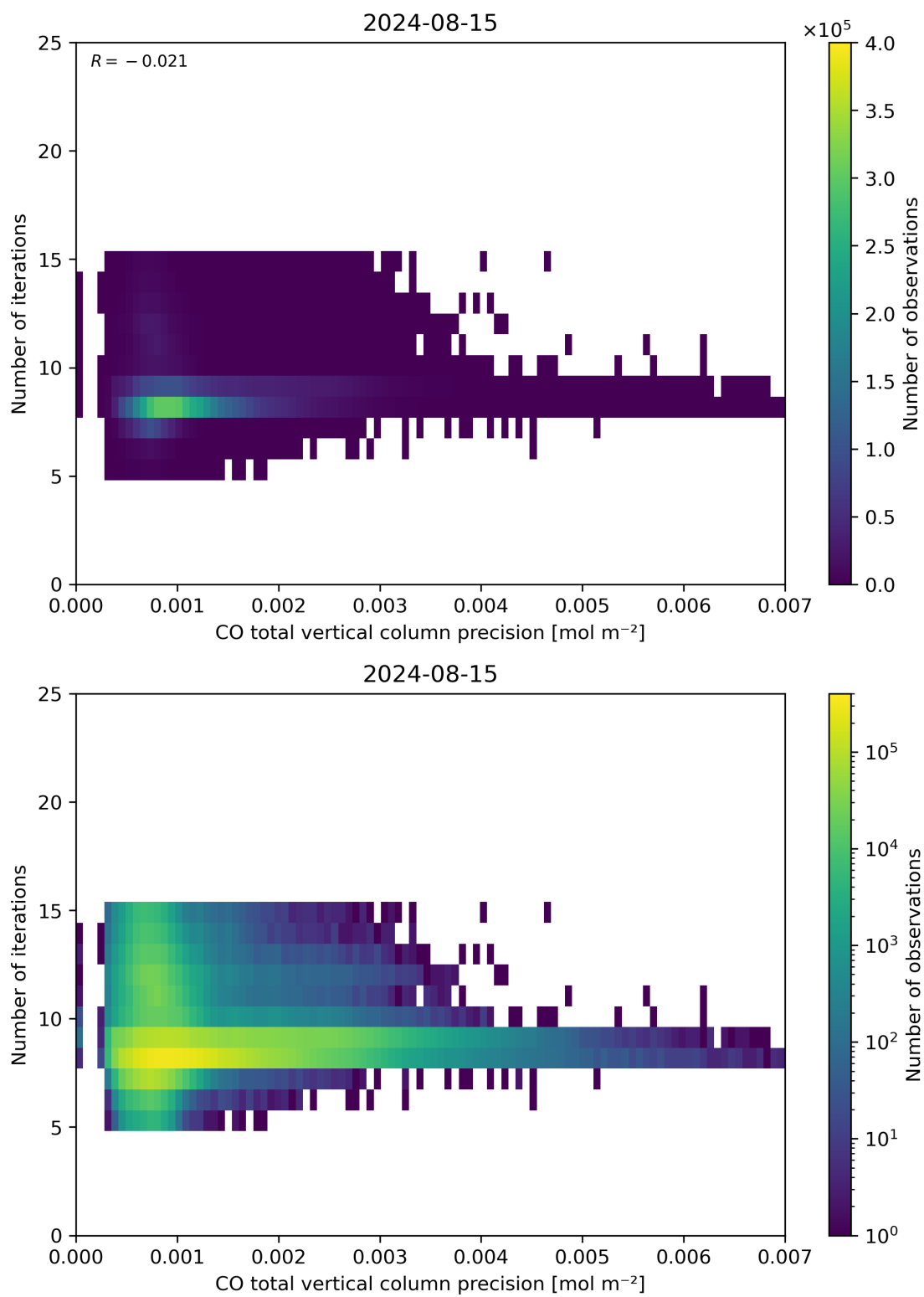
Figure 46: Scatter density plot of “CO total vertical column precision” against “Number of iterations” for 2024-08-14 to 2024-08-16.
