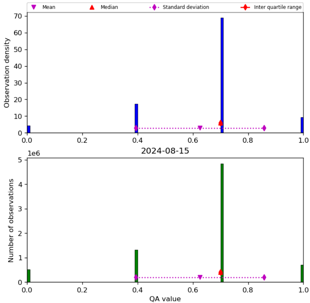
Figure 17: Histogram of “QA value” for 2024-08-14 to 2024-08-16
