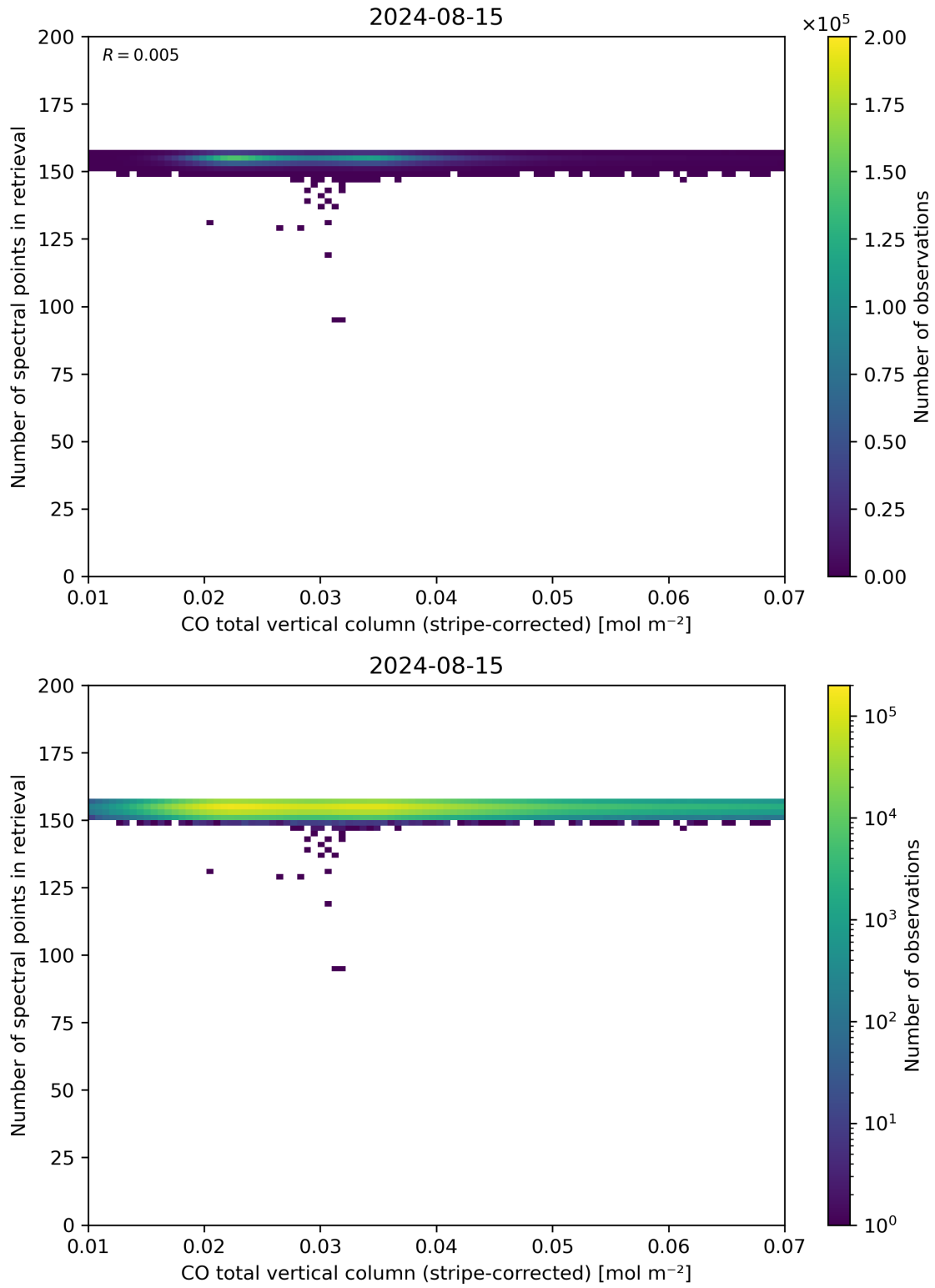
Figure 40: Scatter density plot of “CO total vertical column (stripe-corrected)” against “Number of spectral points in retrieval” for 2024-08-14 to 2024-08-16.
