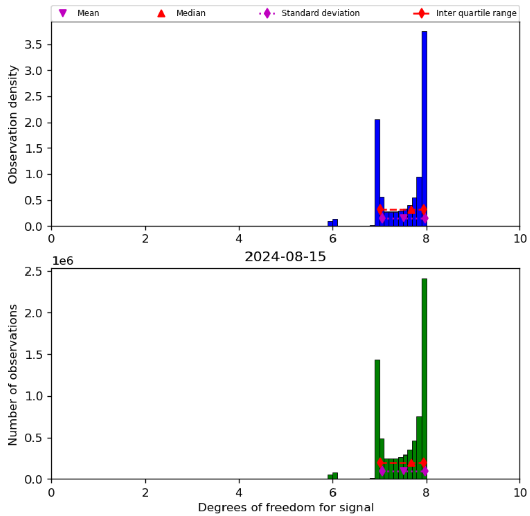
Figure 23: Histogram of “Degrees of freedom for signal” for 2024-08-14 to 2024-08-16
