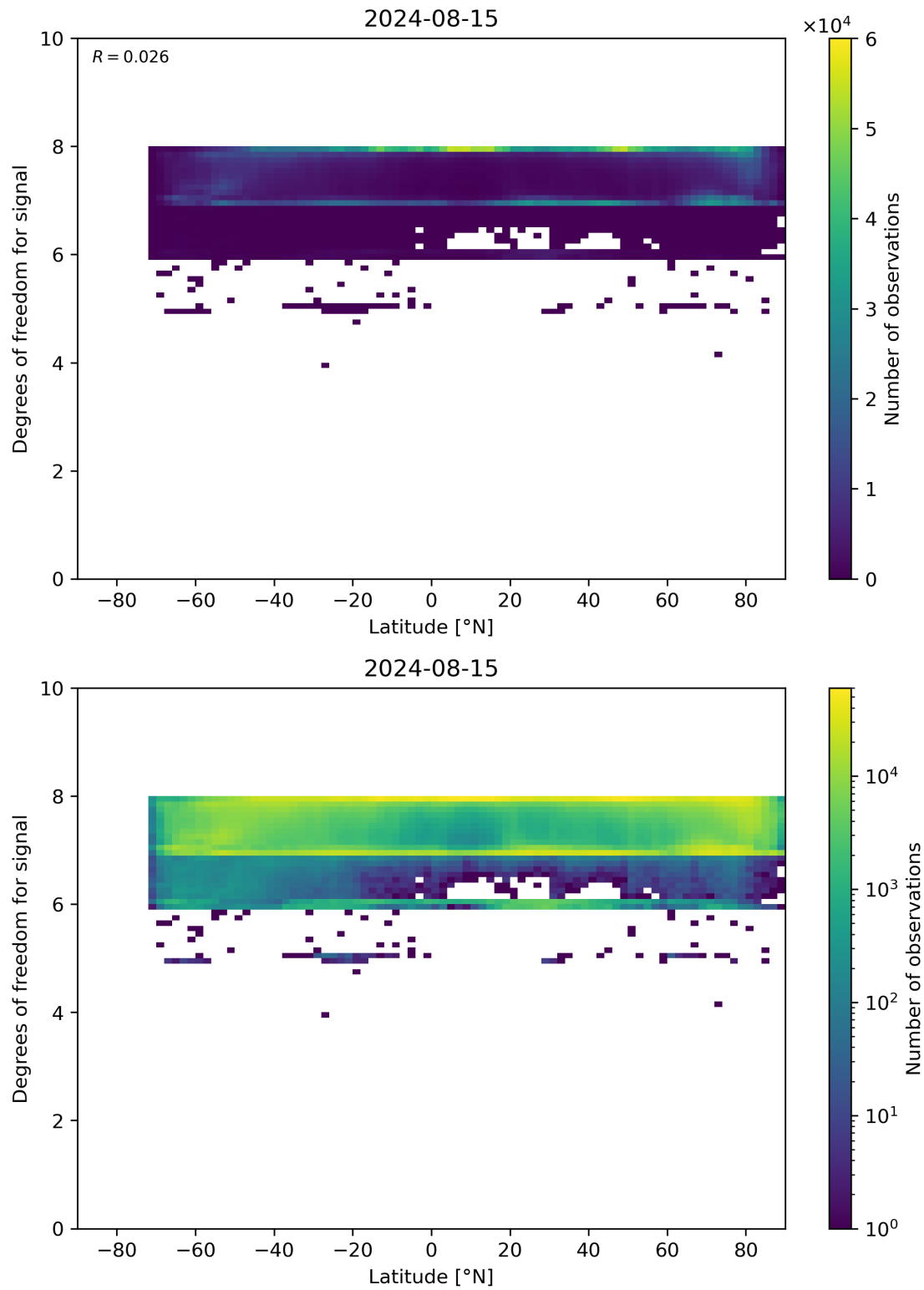
Figure 55: Scatter density plot of “Latitude” against “Degrees of freedom for signal” for 2024-08-14 to 2024-08-16.
