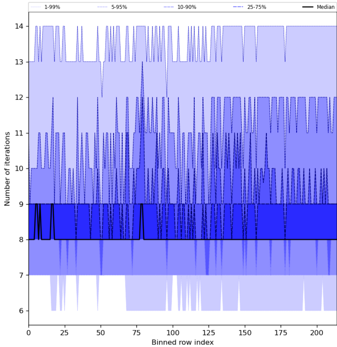
Figure 32: Along track statistics of “Number of iterations” for 2024-08-14 to 2024-08-16
