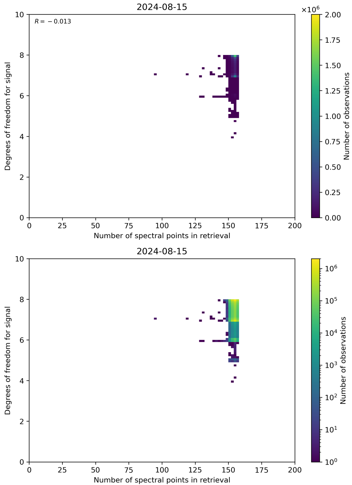
Figure 59: Scatter density plot of “Number of spectral points in retrieval” against “Degrees of freedom for signal” for 2024-08-14 to 2024-08-16.
