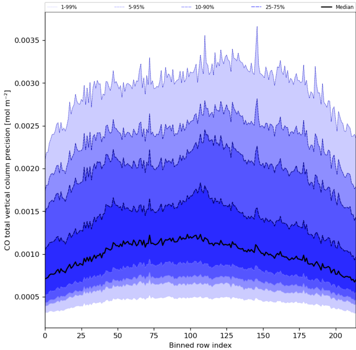
Figure 28: Along track statistics of “CO total vertical column precision” for 2024-08-16 to 2024-08-17
