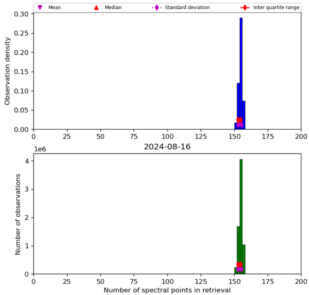
Figure 21: Histogram of “Number of spectral points in retrieval” for 2024-08-16 to 2024-08-17
