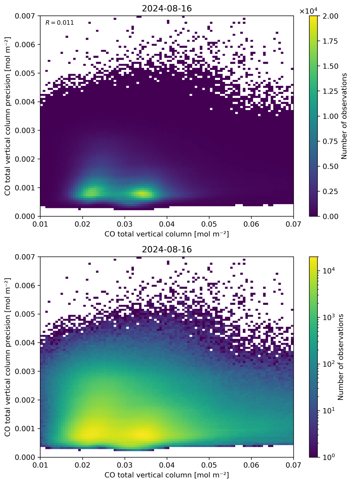
Figure 34: Scatter density plot of “CO total vertical column” against “CO total vertical column precision” for 2024-08-16 to 2024-08-17.
