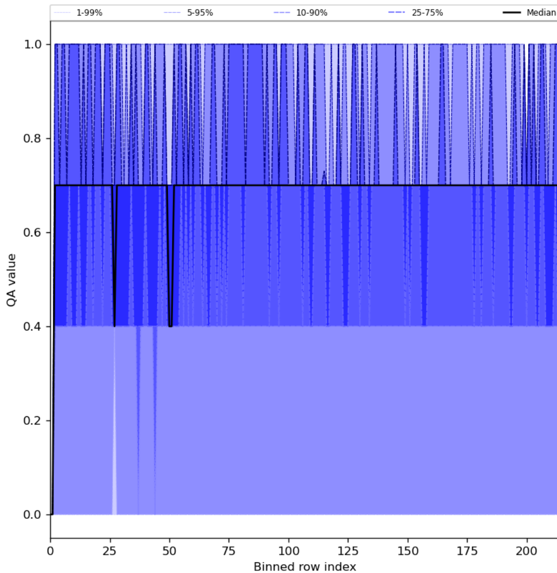
Figure 25: Along track statistics of “QA value” for 2024-08-16 to 2024-08-17
