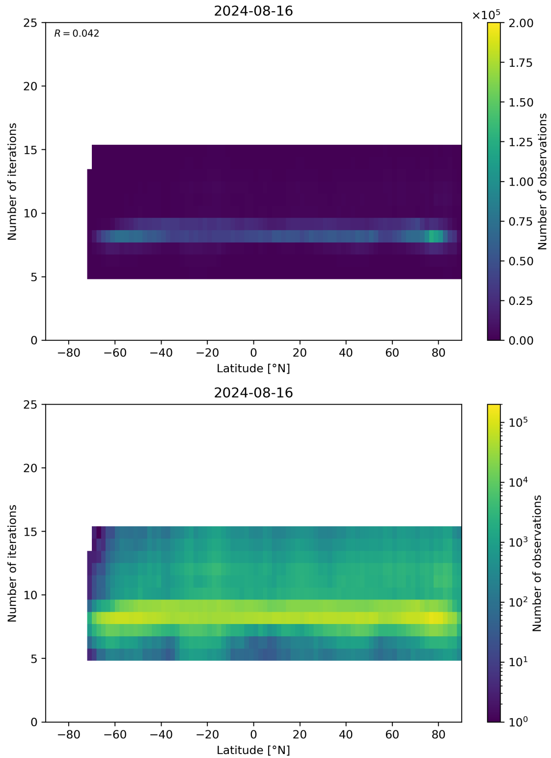
Figure 56: Scatter density plot of “Latitude” against “Number of iterations” for 2024-08-16 to 2024-08-17.
