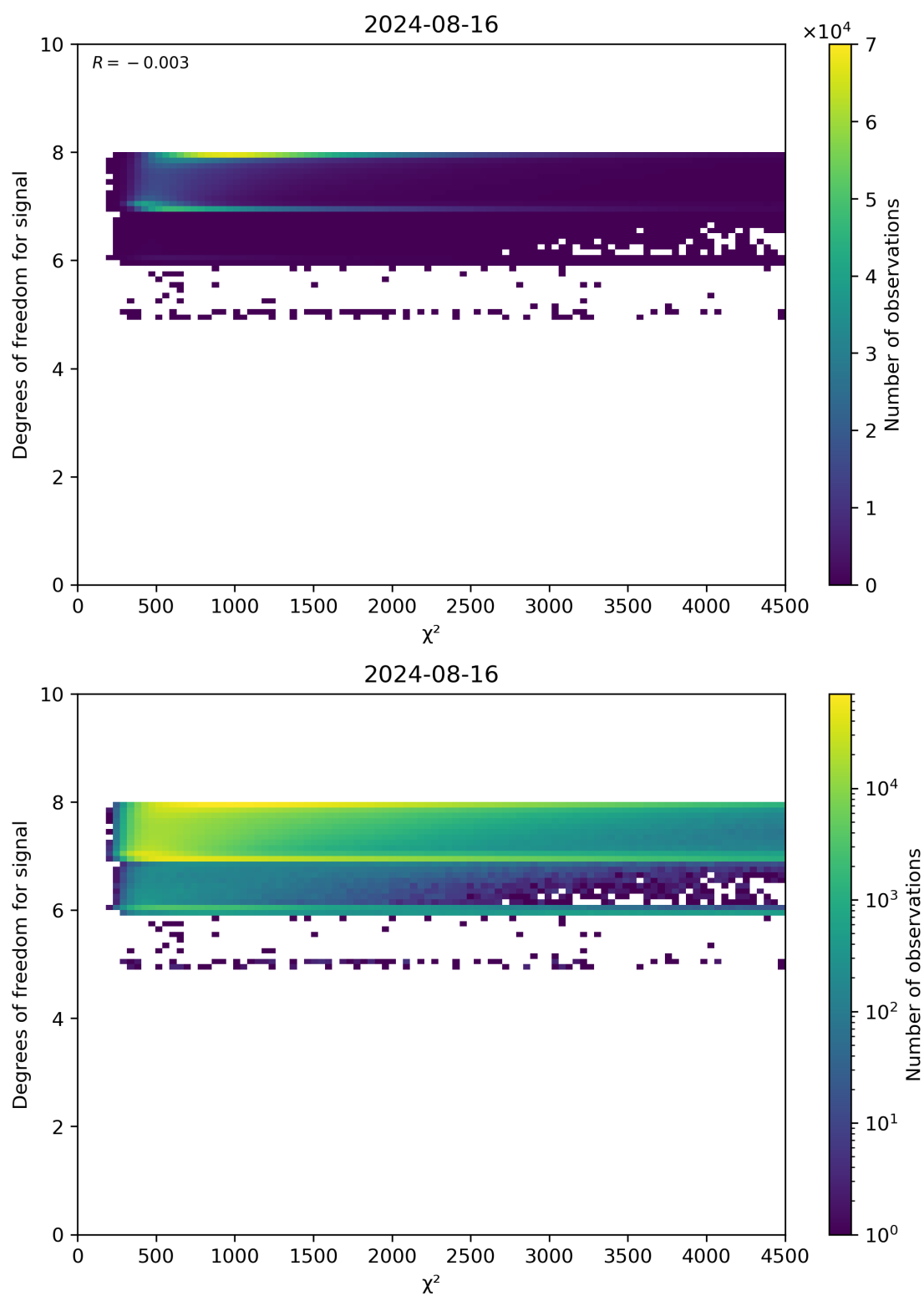
Figure 48: Scatter density plot of “ \chi^2 ” against “Degrees of freedom for signal” for 2024-08-16 to 2024-08-17.
