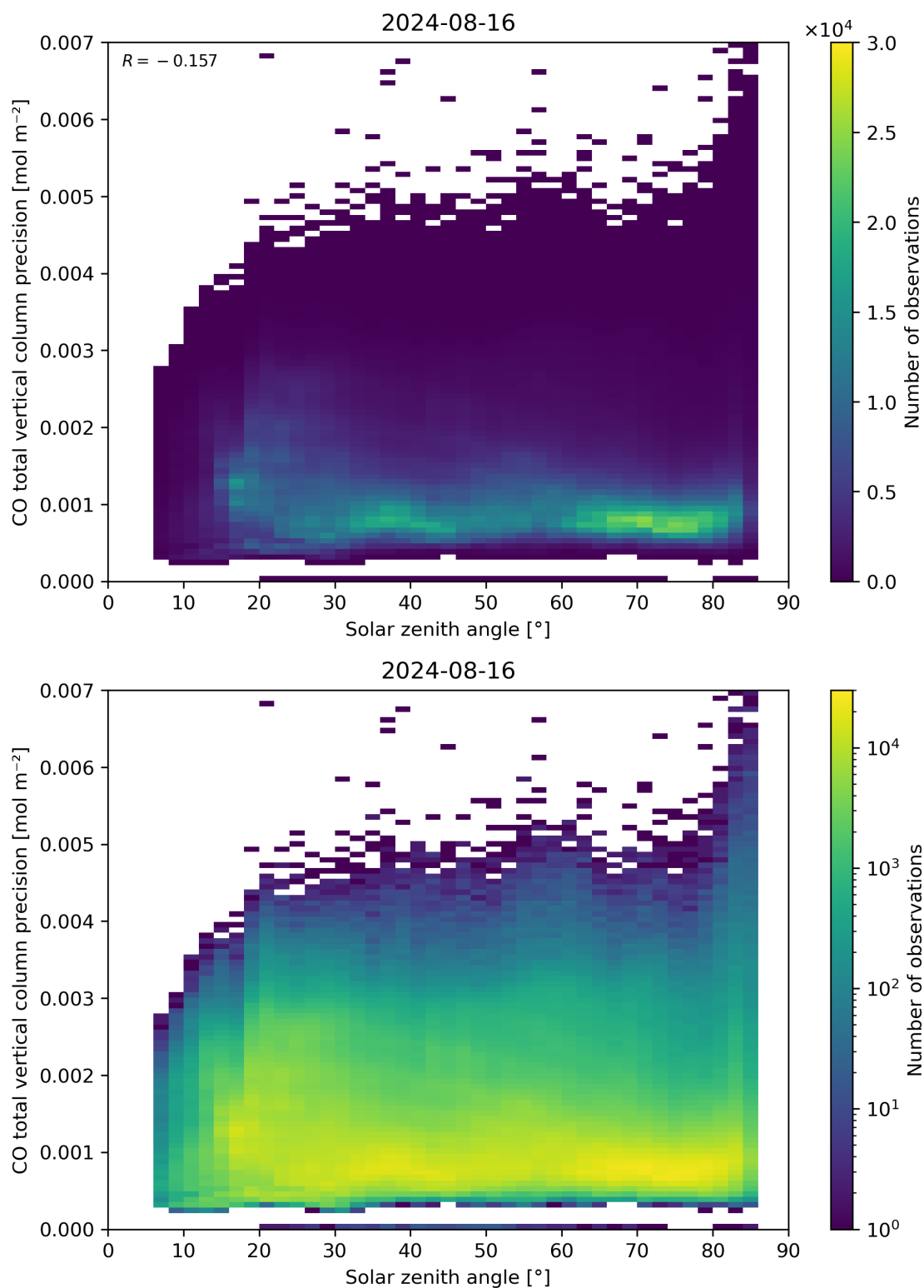
Figure 63: Scatter density plot of “Solar zenith angle” against “CO total vertical column precision” for 2024-08-16 to 2024-08-17.
