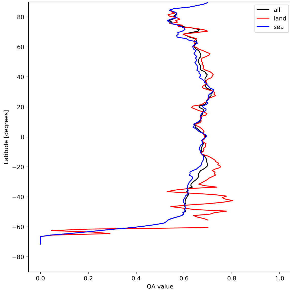
Figure 9: Zonal average of “QA value” for 2024-08-16 to 2024-08-17.
