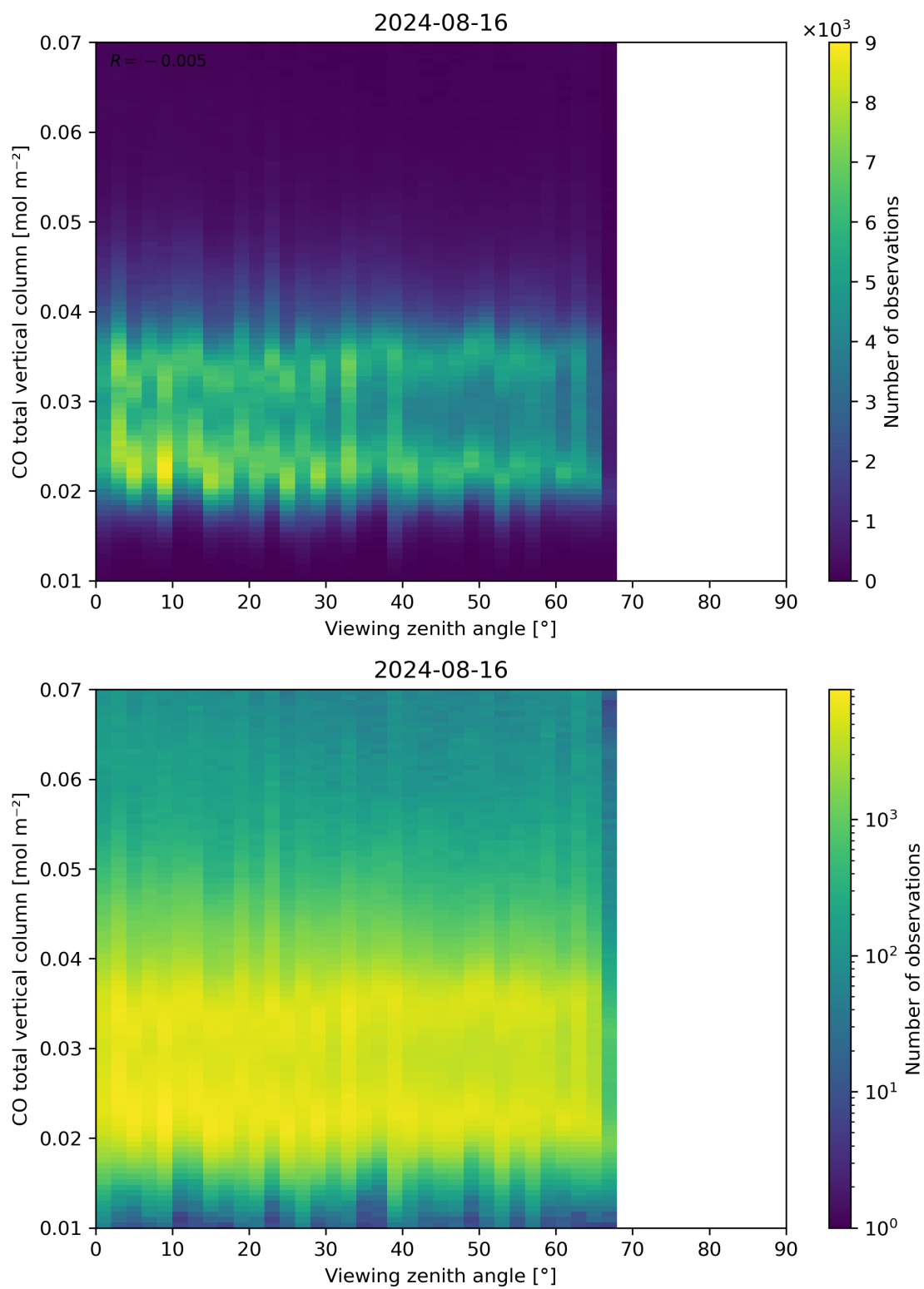
Figure 69: Scatter density plot of “Viewing zenith angle” against “CO total vertical column” for 2024-08-16 to 2024-08-17.
