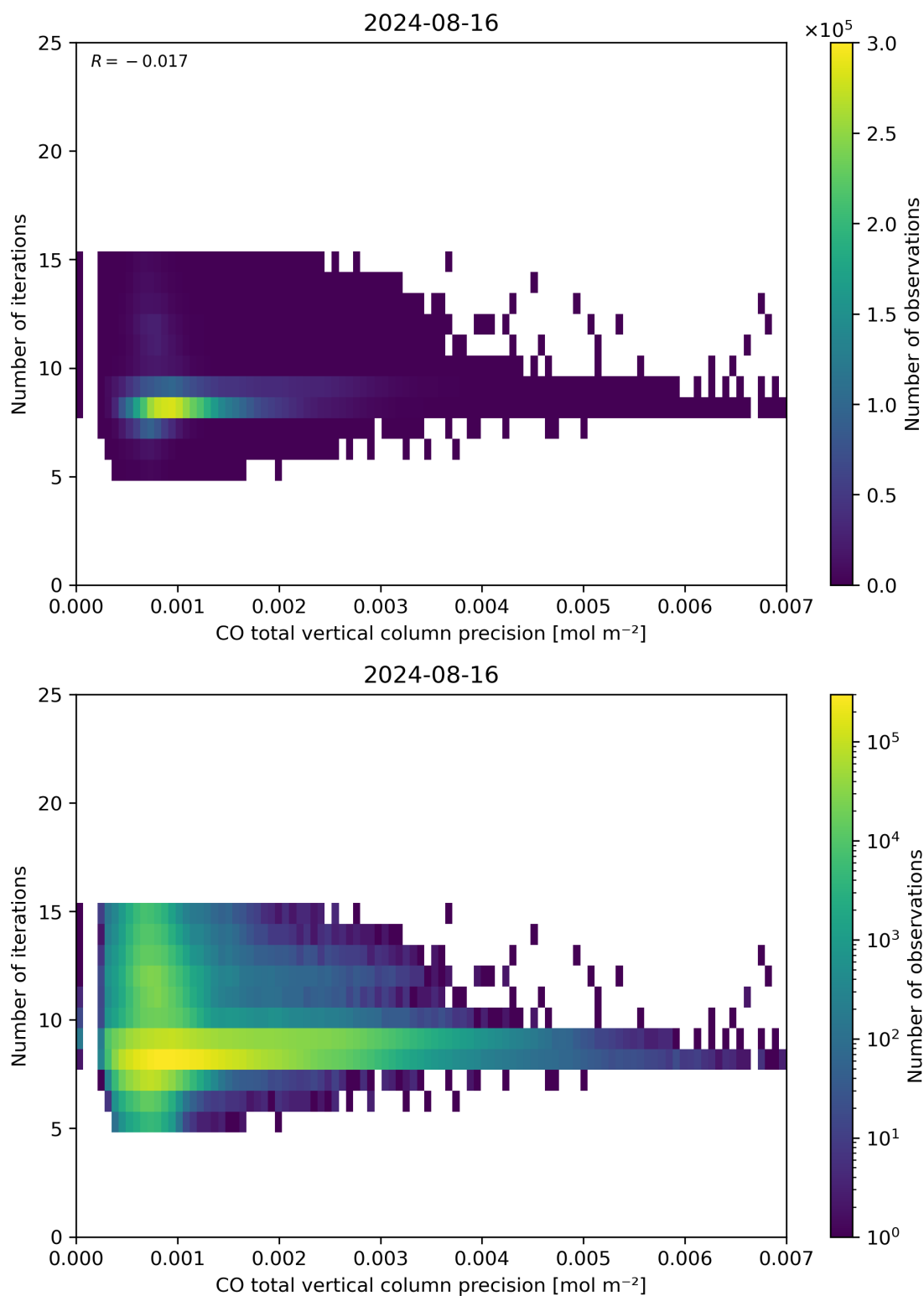
Figure 46: Scatter density plot of “CO total vertical column precision” against “Number of iterations” for 2024-08-16 to 2024-08-17.
