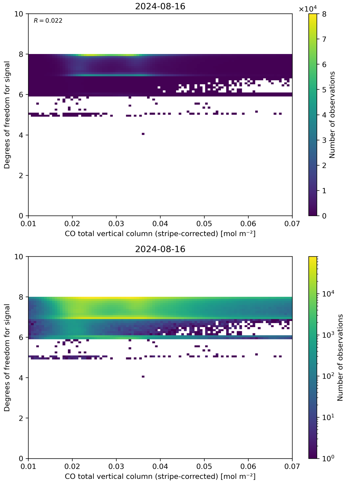
Figure 38: Scatter density plot of “CO total vertical column (stripe-corrected)” against “Degrees of freedom for signal” for 2024-08-16 to 2024-08-17.
