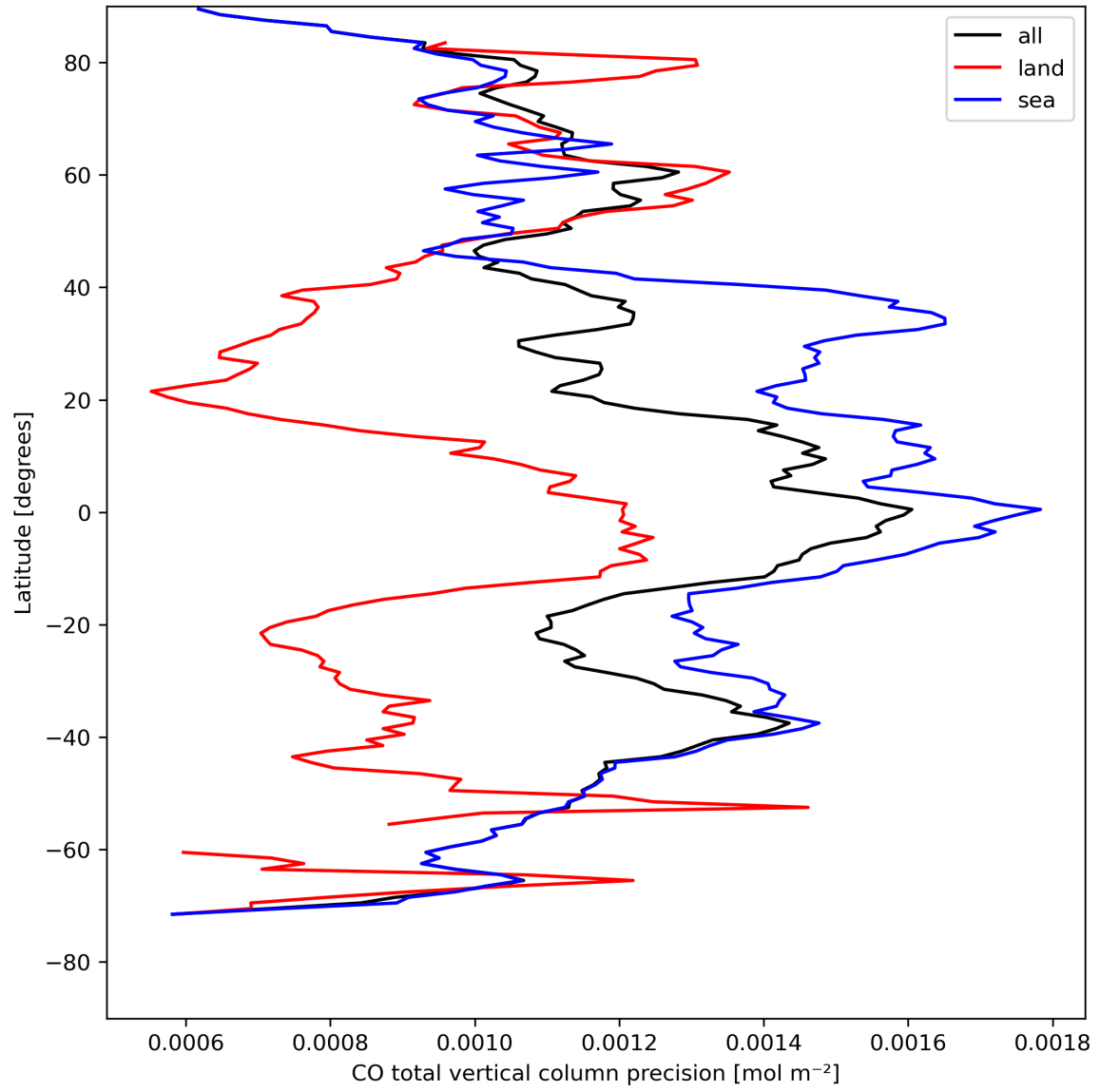
Figure 12: Zonal average of “CO total vertical column precision” for 2024-08-16 to 2024-08-17.
