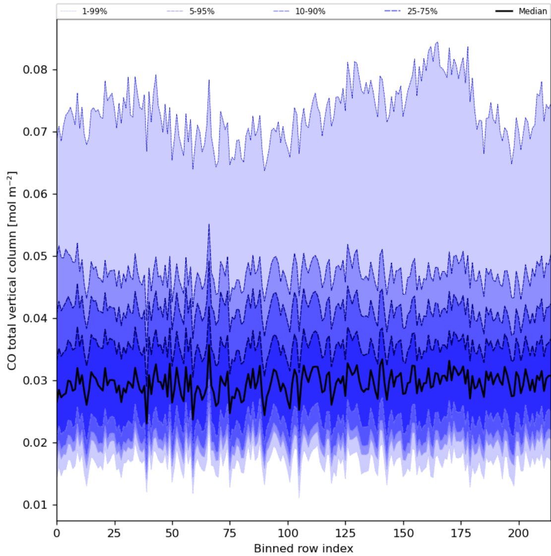
Figure 26: Along track statistics of “CO total vertical column” for 2024-08-16 to 2024-08-17
