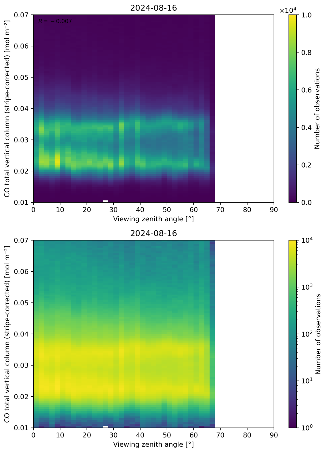
Figure 70: Scatter density plot of “Viewing zenith angle” against “CO total vertical column (stripe-corrected)” for 2024-08-16 to 2024-08-17.
