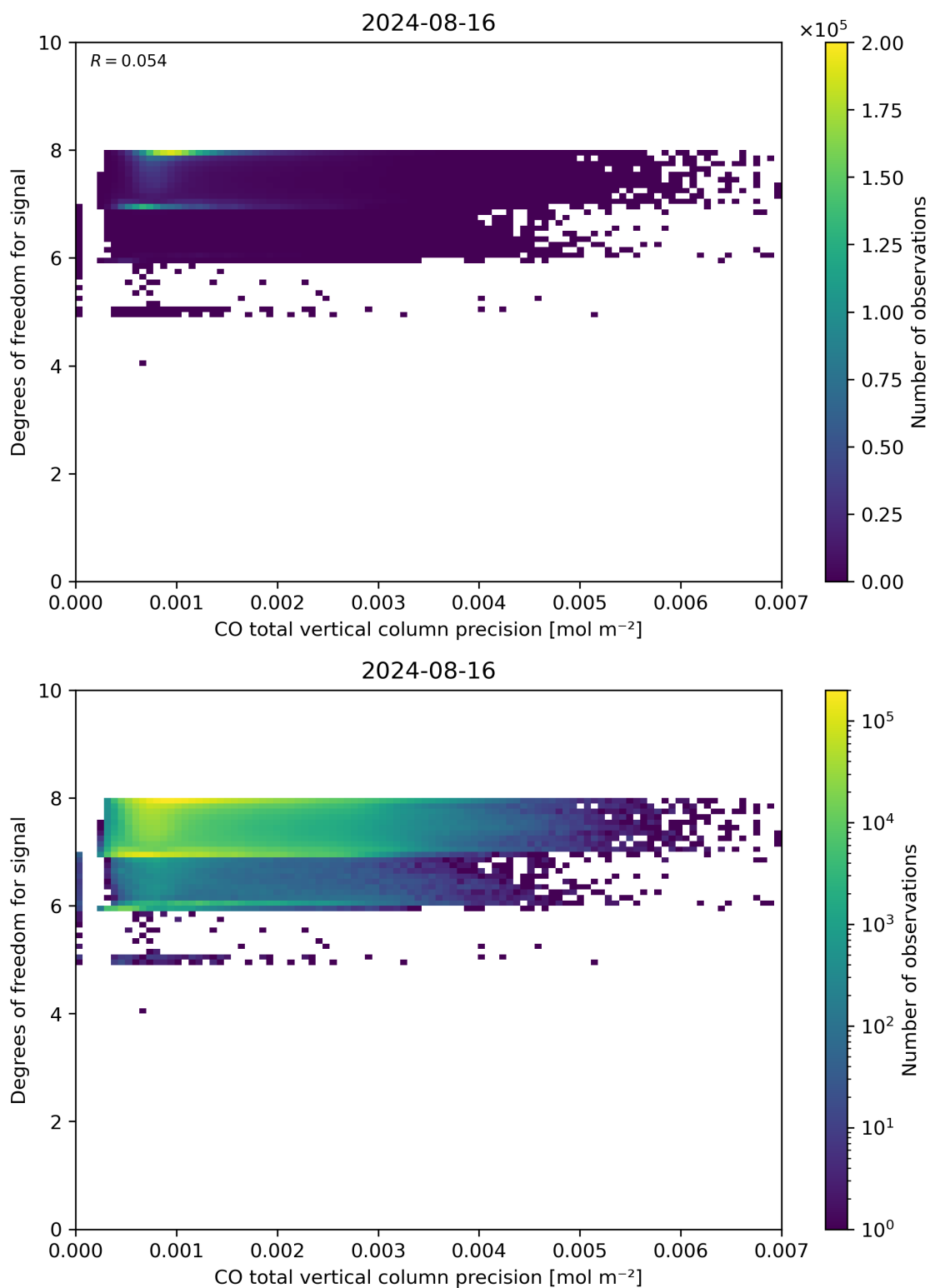
Figure 45: Scatter density plot of “CO total vertical column precision” against “Degrees of freedom for signal” for 2024-08-16 to 2024-08-17.
