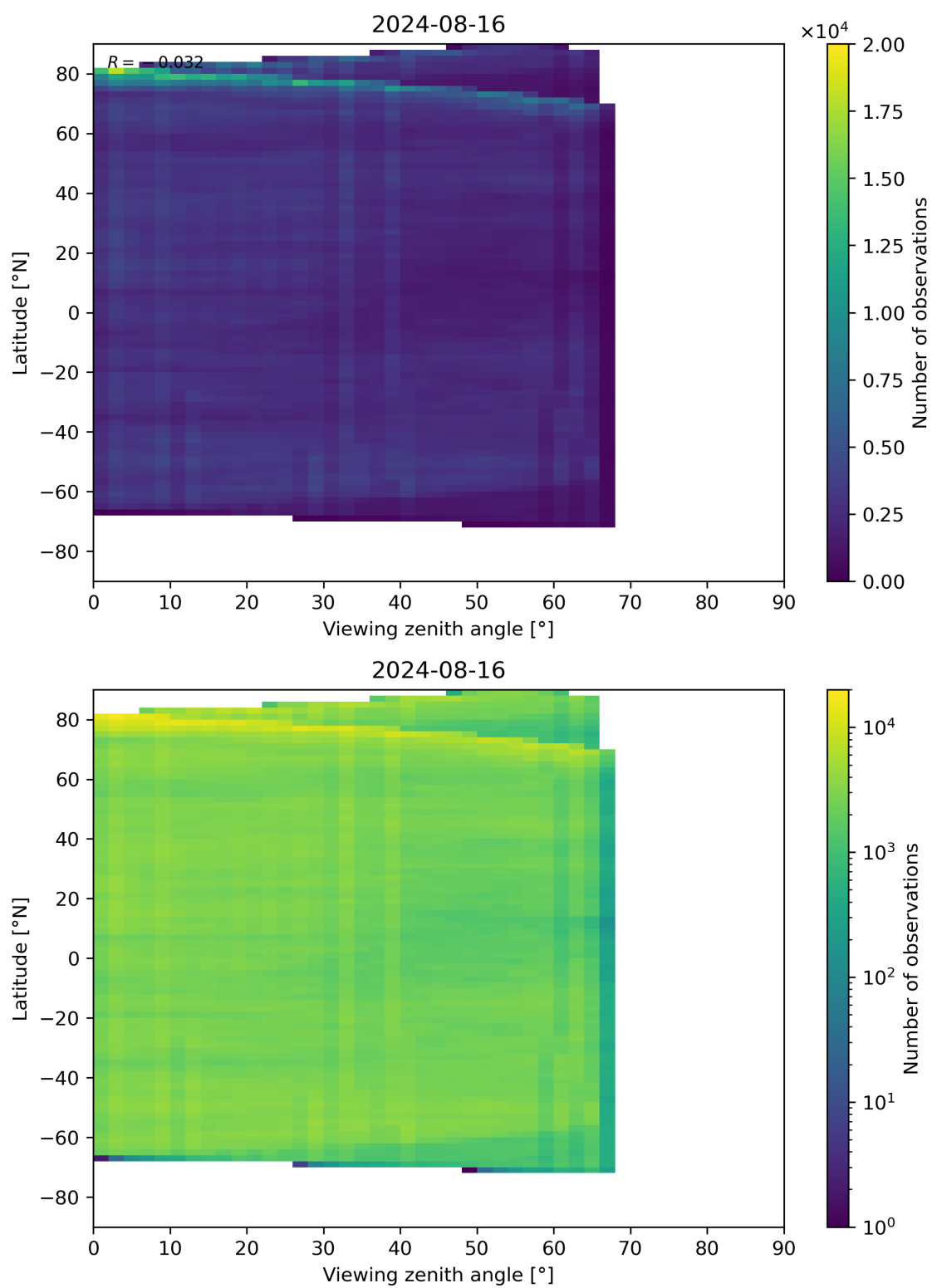
Figure 74: Scatter density plot of “Viewing zenith angle” against “Latitude” for 2024-08-16 to 2024-08-17.
