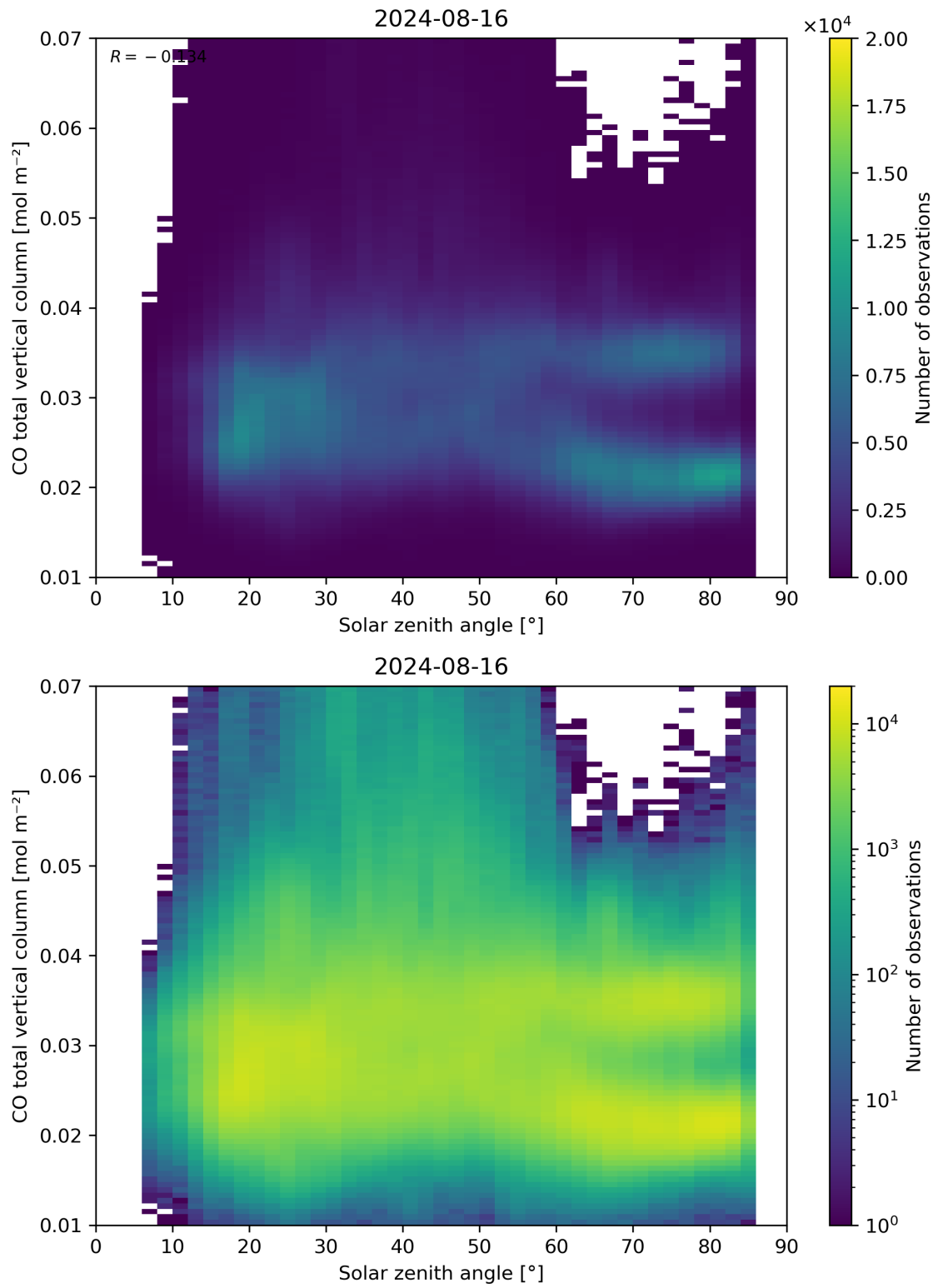
Figure 61: Scatter density plot of “Solar zenith angle” against “CO total vertical column” for 2024-08-16 to 2024-08-17.
