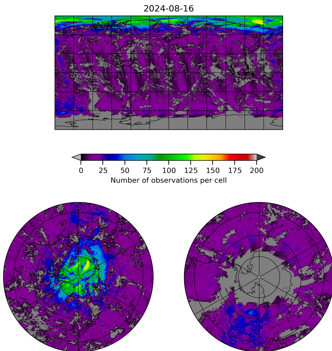
Figure 8: Map of the number of observations for 2024-08-16 to 2024-08-17
