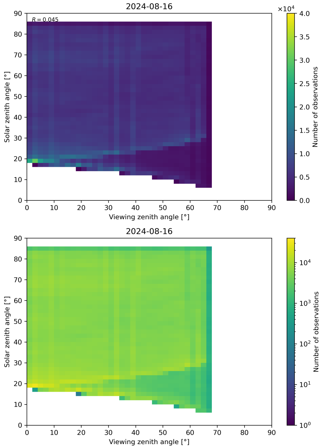
Figure 77: Scatter density plot of “Viewing zenith angle” against “Solar zenith angle” for 2024-08-16 to 2024-08-17.
