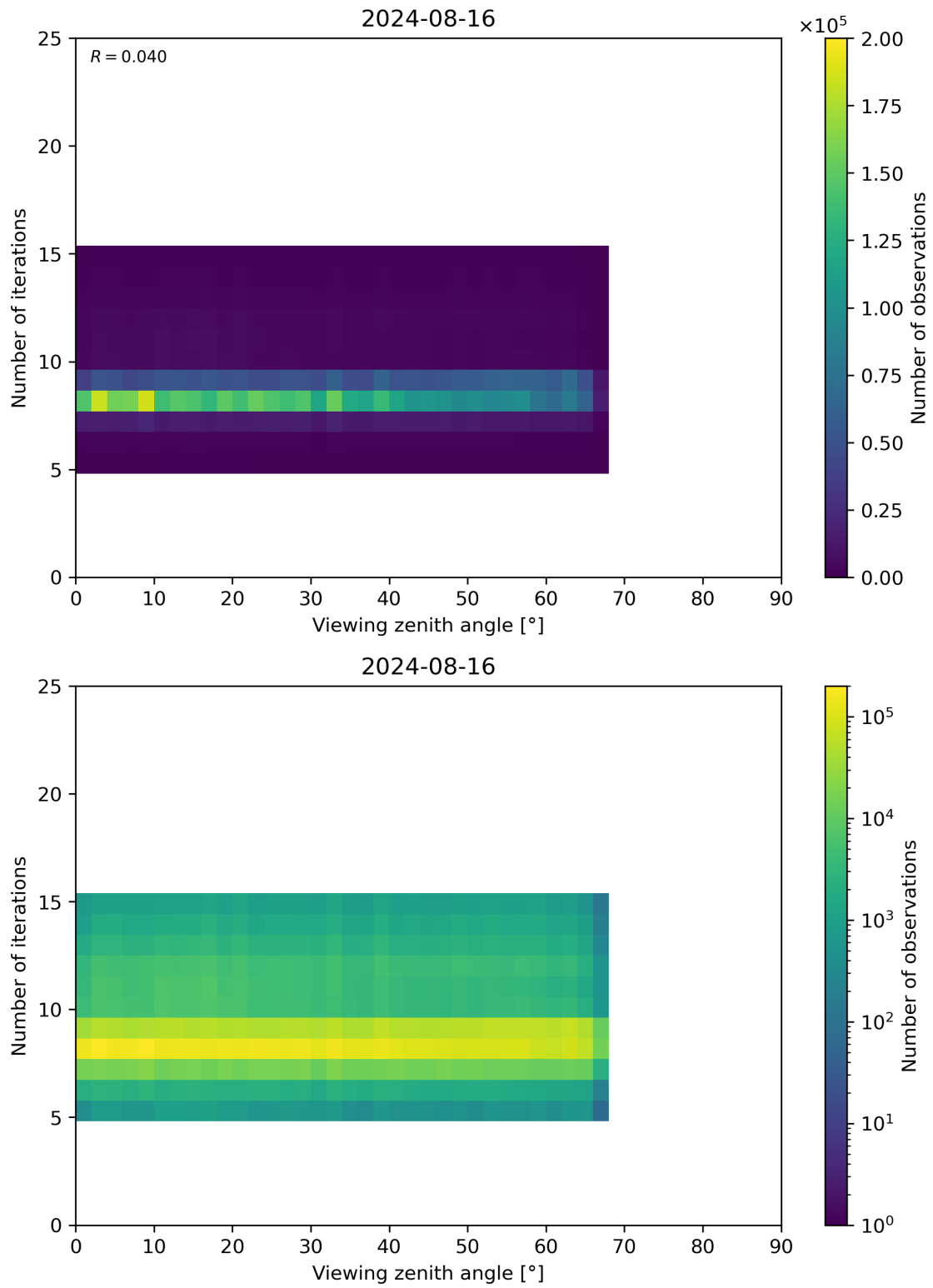
Figure 75: Scatter density plot of “Viewing zenith angle” against “Number of iterations” for 2024-08-16 to 2024-08-17.
