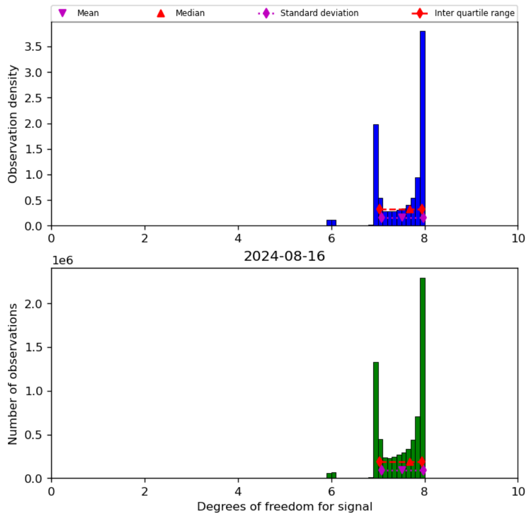
Figure 23: Histogram of “Degrees of freedom for signal” for 2024-08-16 to 2024-08-17
