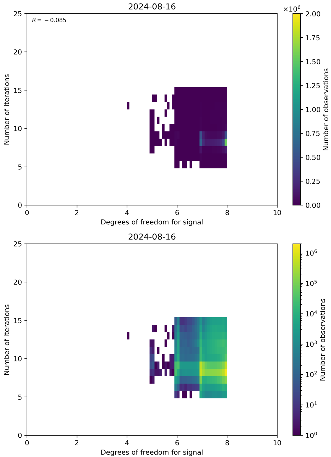
Figure 50: Scatter density plot of “Degrees of freedom for signal” against “Number of iterations” for 2024-08-16 to 2024-08-17.
