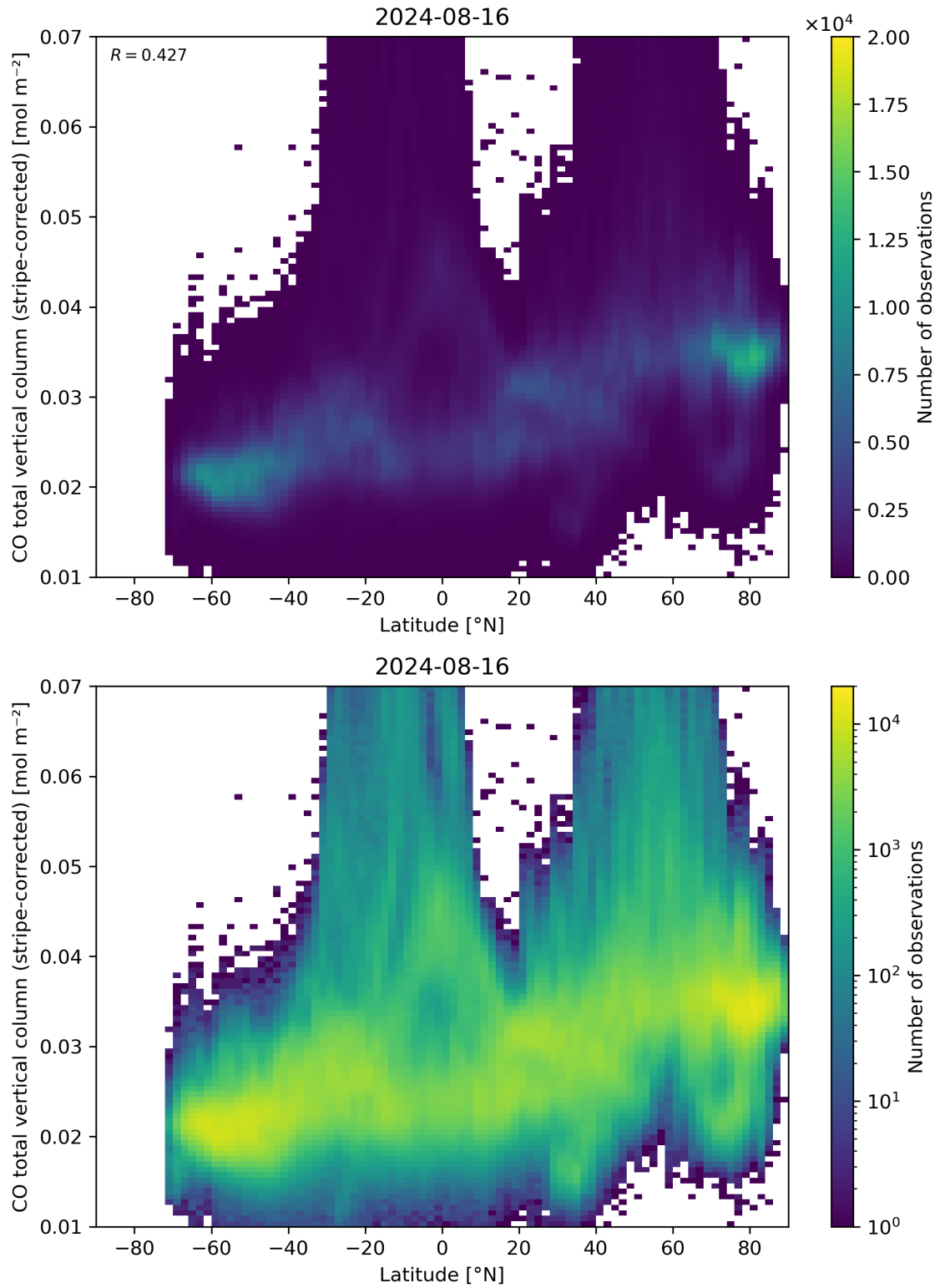
Figure 52: Scatter density plot of “Latitude” against “CO total vertical column (stripe-corrected)” for 2024-08-16 to 2024-08-17.
