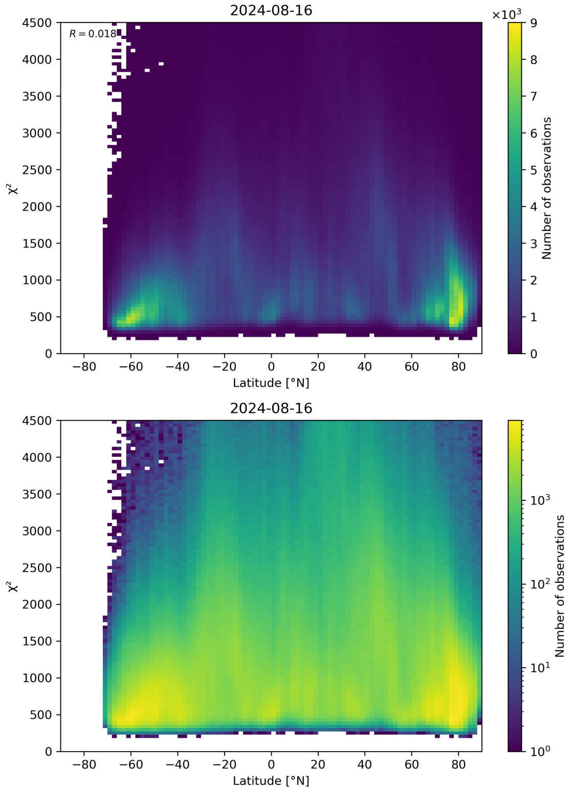
Figure 54: Scatter density plot of “Latitude” against “ \chi^2 ” for 2024-08-16 to 2024-08-17.
