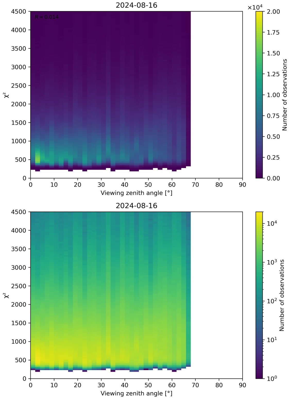
Figure 72: Scatter density plot of “Viewing zenith angle” against “ \chi^2 ” for 2024-08-16 to 2024-08-17.
