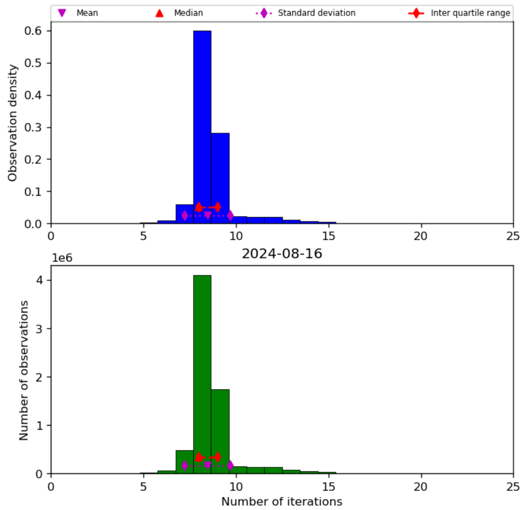
Figure 24: Histogram of “Number of iterations” for 2024-08-16 to 2024-08-17
