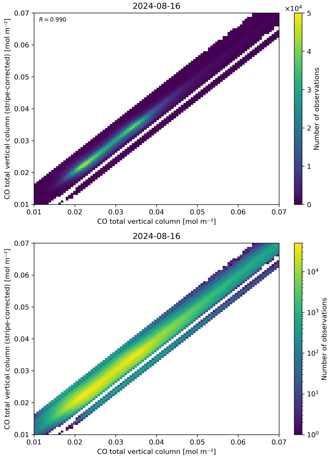
Figure 33: Scatter density plot of “CO total vertical column” against “CO total vertical column (stripe-corrected)” for 2024-08-16 to 2024-08-17.
