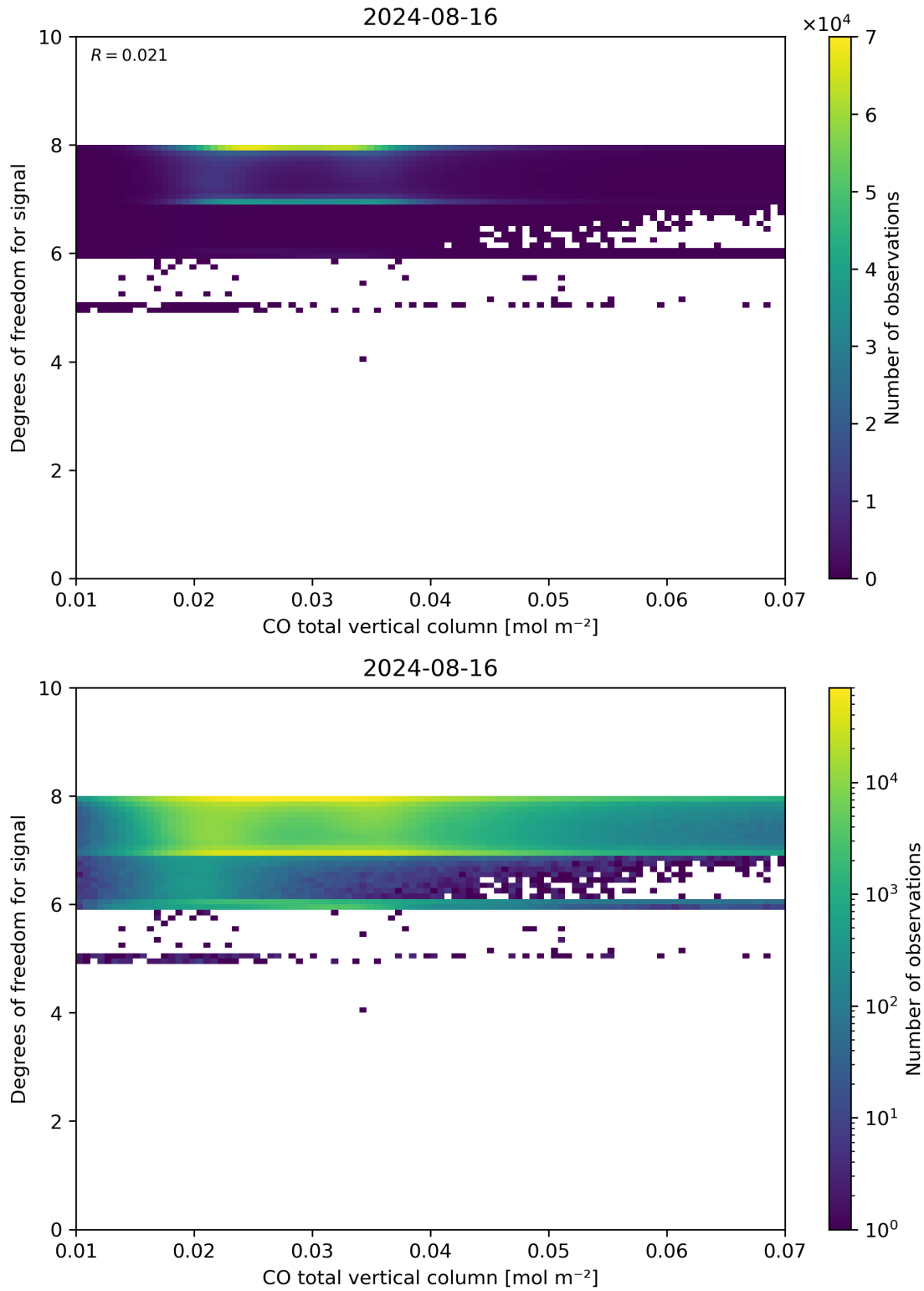
Figure 41: Scatter density plot of “CO total vertical column” against “Degrees of freedom for signal” for 2024-08-16 to 2024-08-17.
