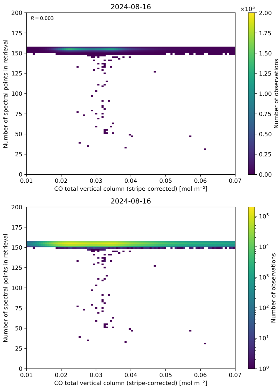
Figure 40: Scatter density plot of “CO total vertical column (stripe-corrected)” against “Number of spectral points in retrieval” for 2024-08-16 to 2024-08-17.
