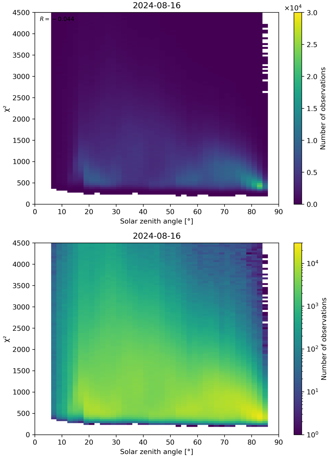
Figure 64: Scatter density plot of “Solar zenith angle” against “ \chi^2 ” for 2024-08-16 to 2024-08-17.
