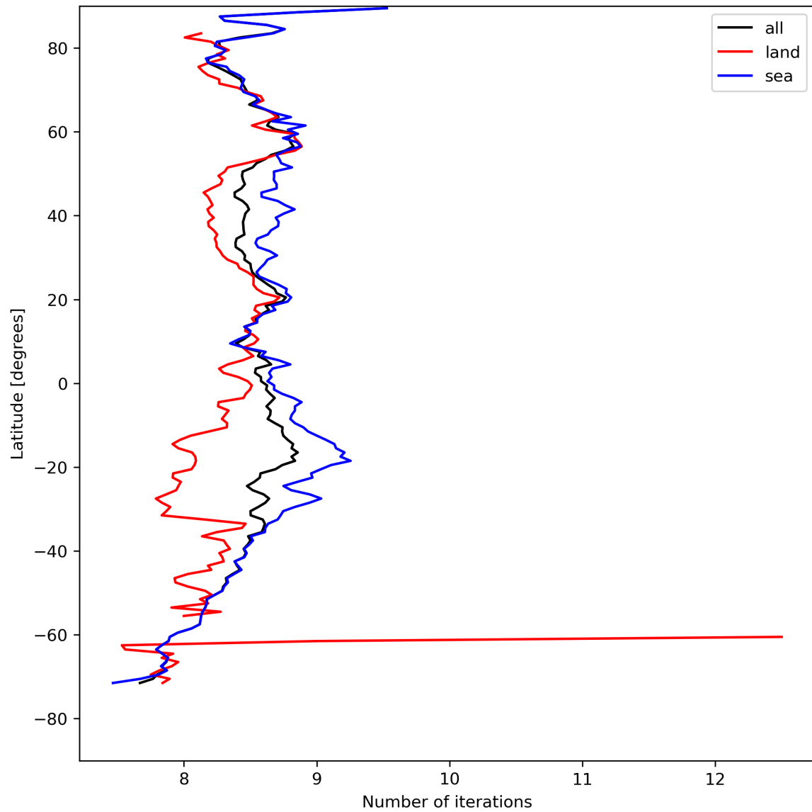
Figure 16: Zonal average of “Number of iterations” for 2024-08-16 to 2024-08-17.
