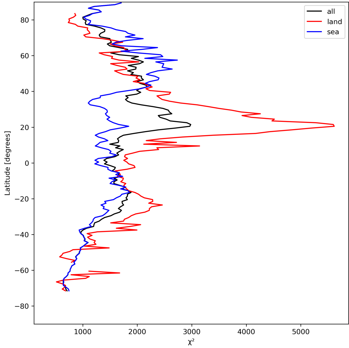
Figure 14: Zonal average of “ \chi^2 ” for 2024-08-16 to 2024-08-17.
