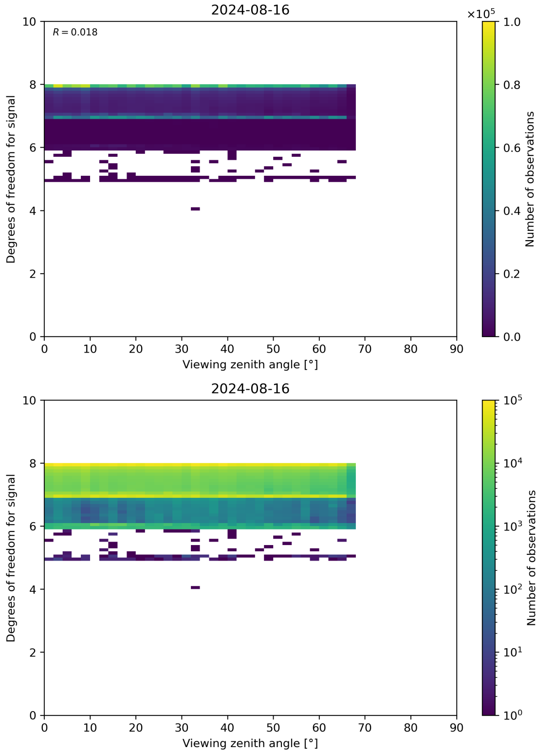
Figure 73: Scatter density plot of “Viewing zenith angle” against “Degrees of freedom for signal” for 2024-08-16 to 2024-08-17.
