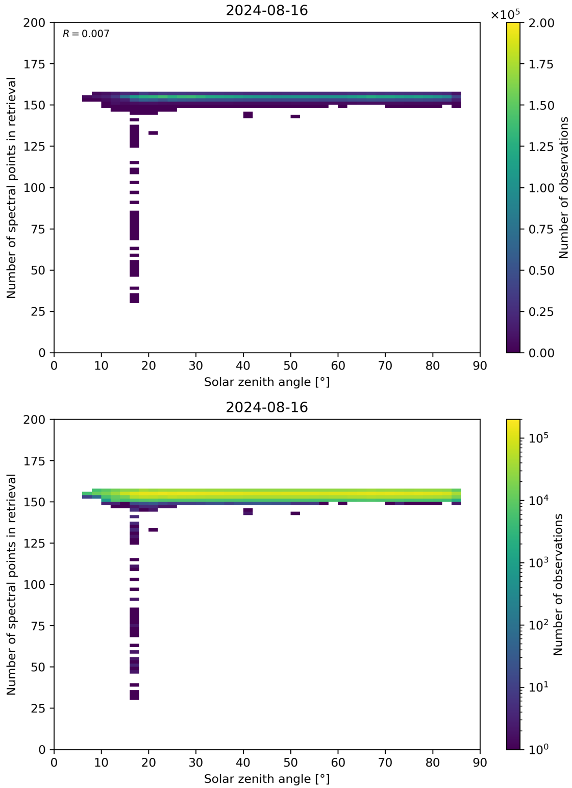
Figure 68: Scatter density plot of “Solar zenith angle” against “Number of spectral points in retrieval” for 2024-08-16 to 2024-08-17.
