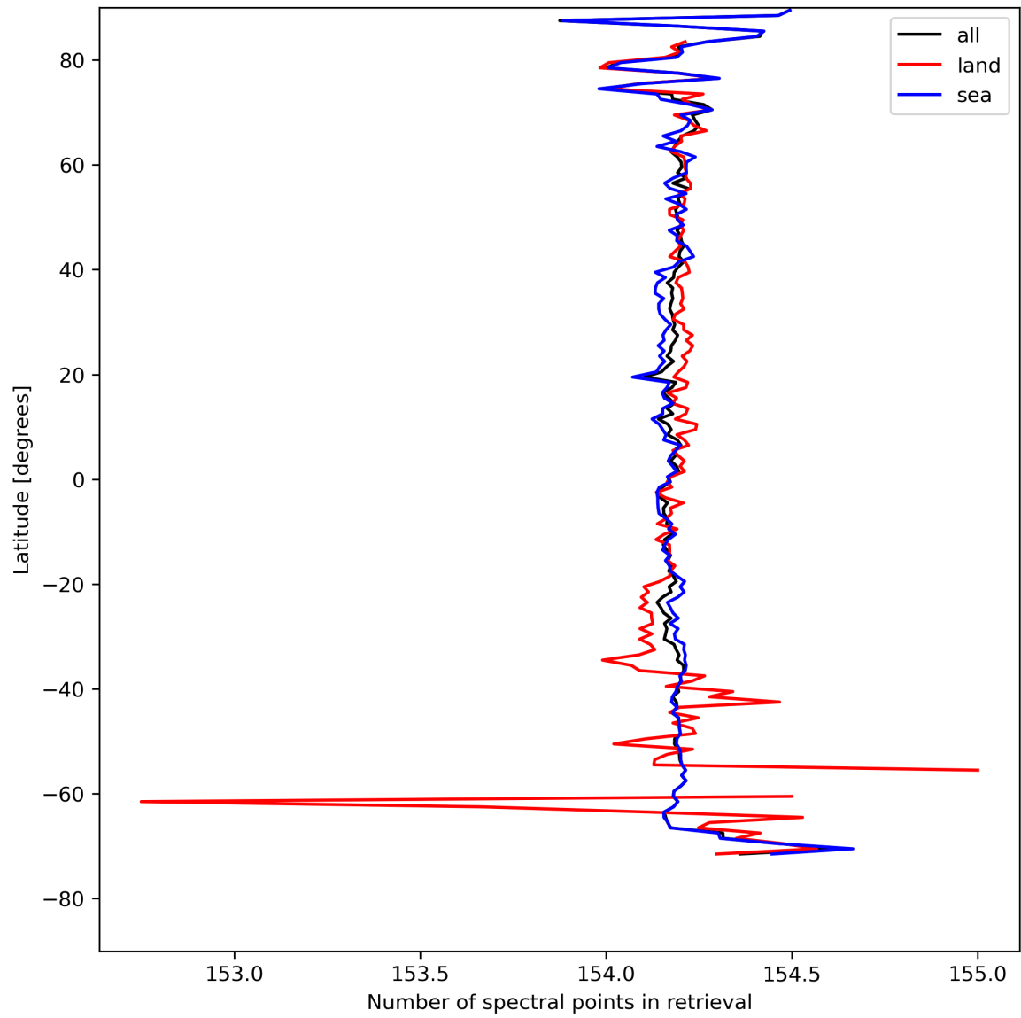
Figure 13: Zonal average of “Number of spectral points in retrieval” for 2024-08-16 to 2024-08-17.
