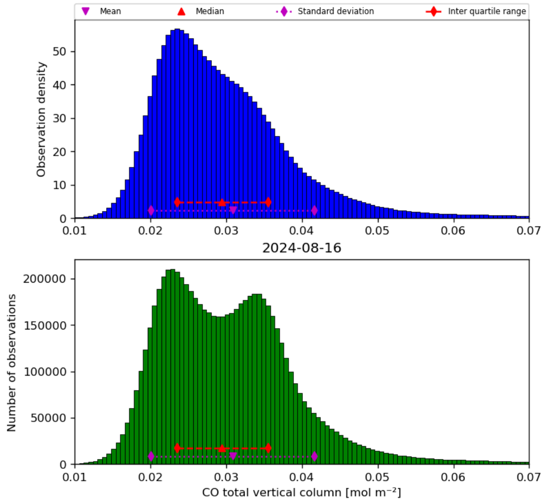
Figure 18: Histogram of “CO total vertical column” for 2024-08-16 to 2024-08-17
