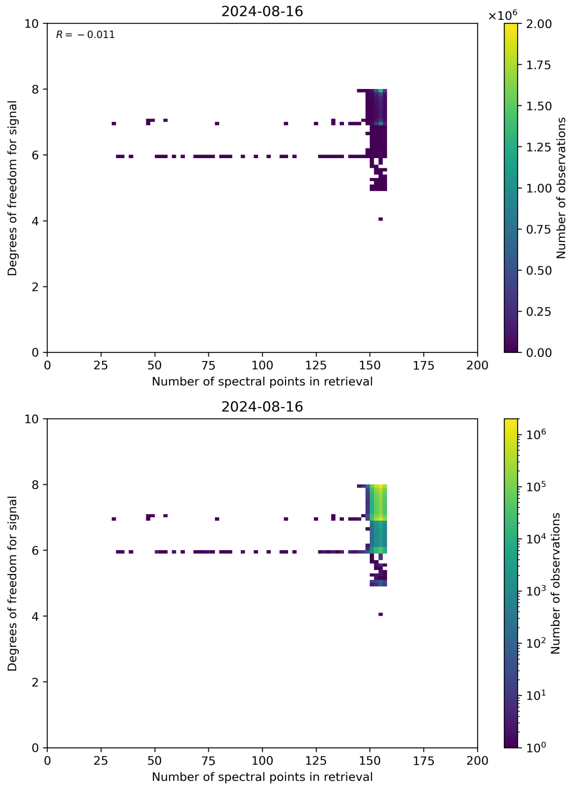
Figure 59: Scatter density plot of “Number of spectral points in retrieval” against “Degrees of freedom for signal” for 2024-08-16 to 2024-08-17.
