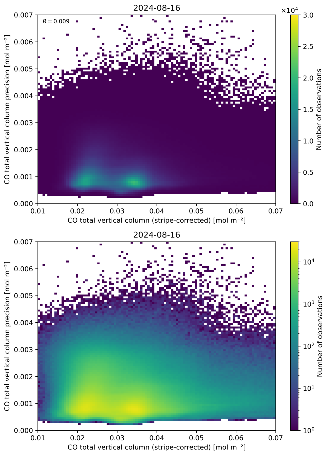
Figure 36: Scatter density plot of “CO total vertical column (stripe-corrected)” against “CO total vertical column precision” for 2024-08-16 to 2024-08-17.
