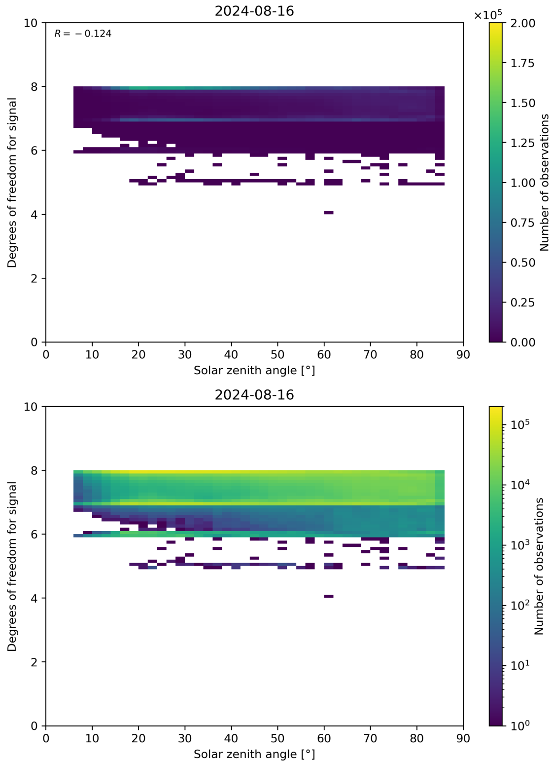
Figure 65: Scatter density plot of “Solar zenith angle” against “Degrees of freedom for signal” for 2024-08-16 to 2024-08-17.
