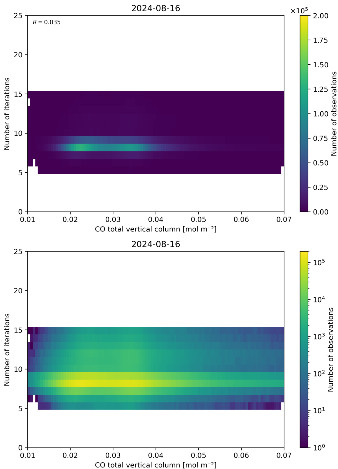
Figure 42: Scatter density plot of “CO total vertical column” against “Number of iterations” for 2024-08-16 to 2024-08-17.
