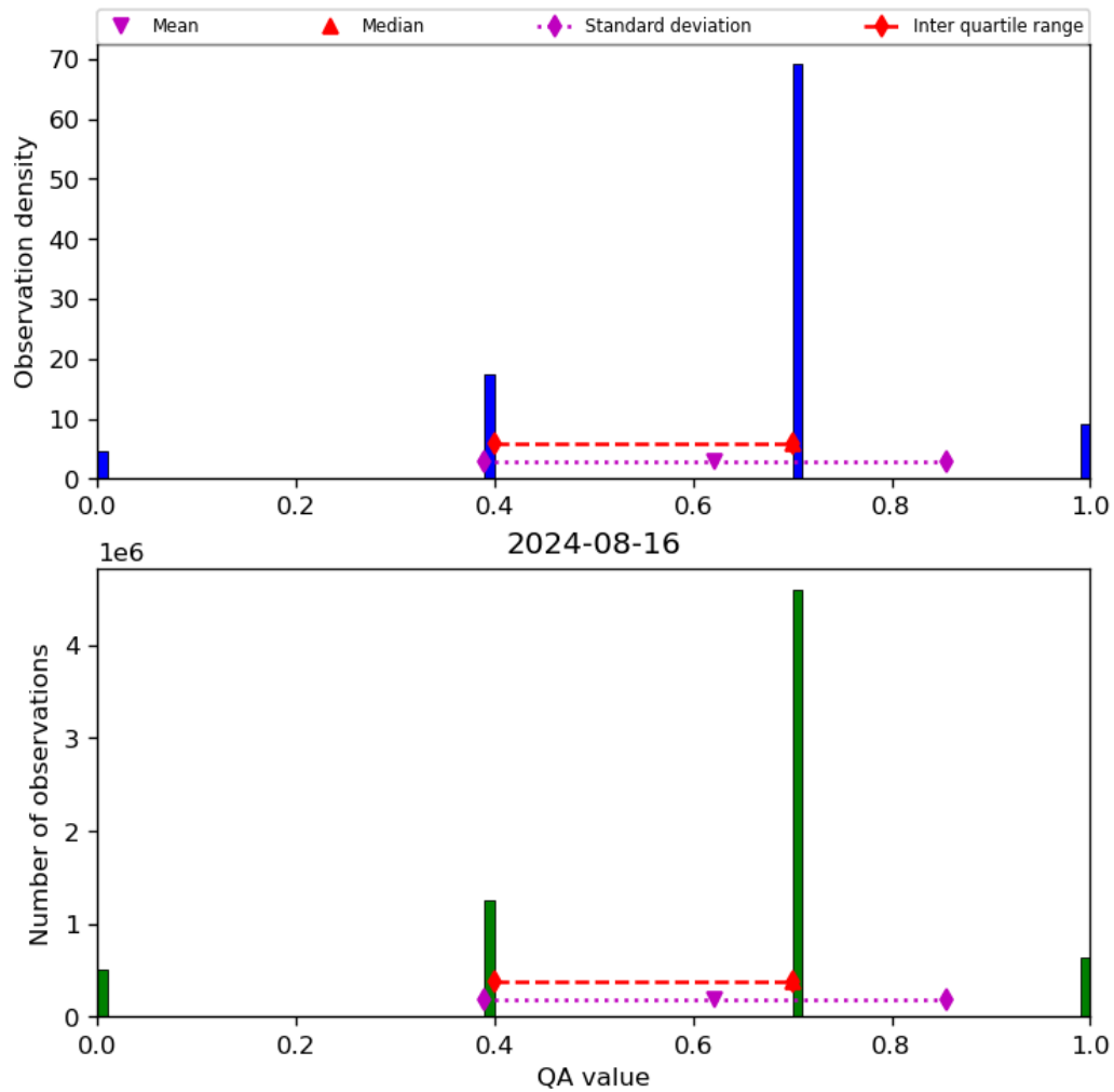
Figure 17: Histogram of “QA value” for 2024-08-16 to 2024-08-17
