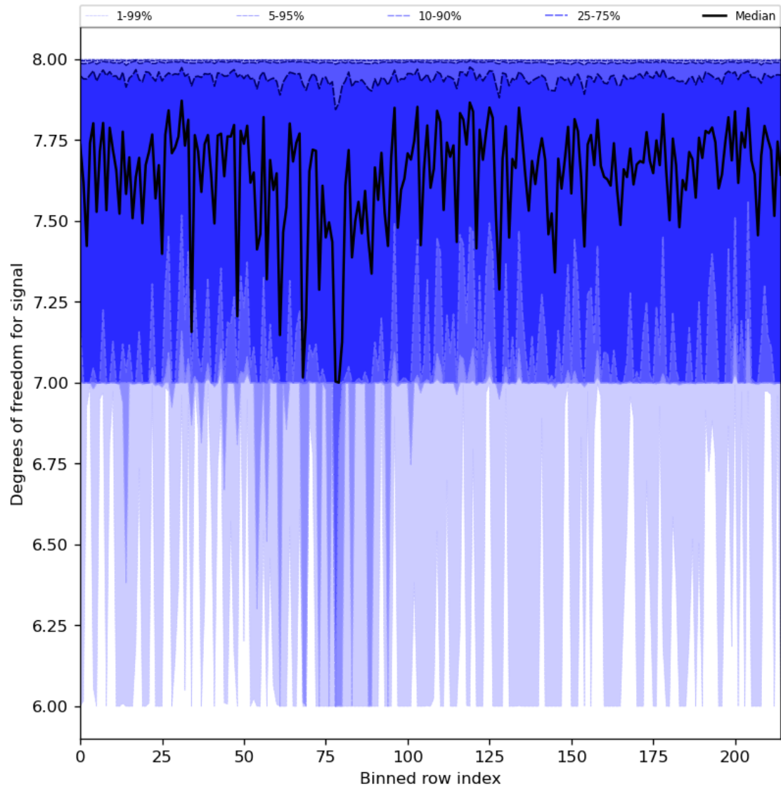
Figure 31: Along track statistics of “Degrees of freedom for signal” for 2024-08-16 to 2024-08-17
