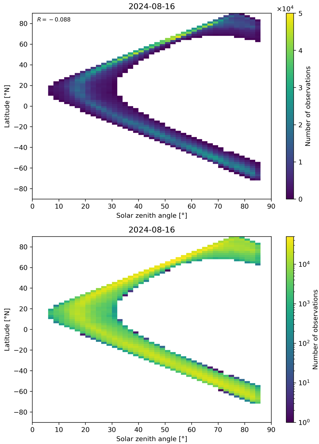
Figure 66: Scatter density plot of “Solar zenith angle” against “Latitude” for 2024-08-16 to 2024-08-17.
