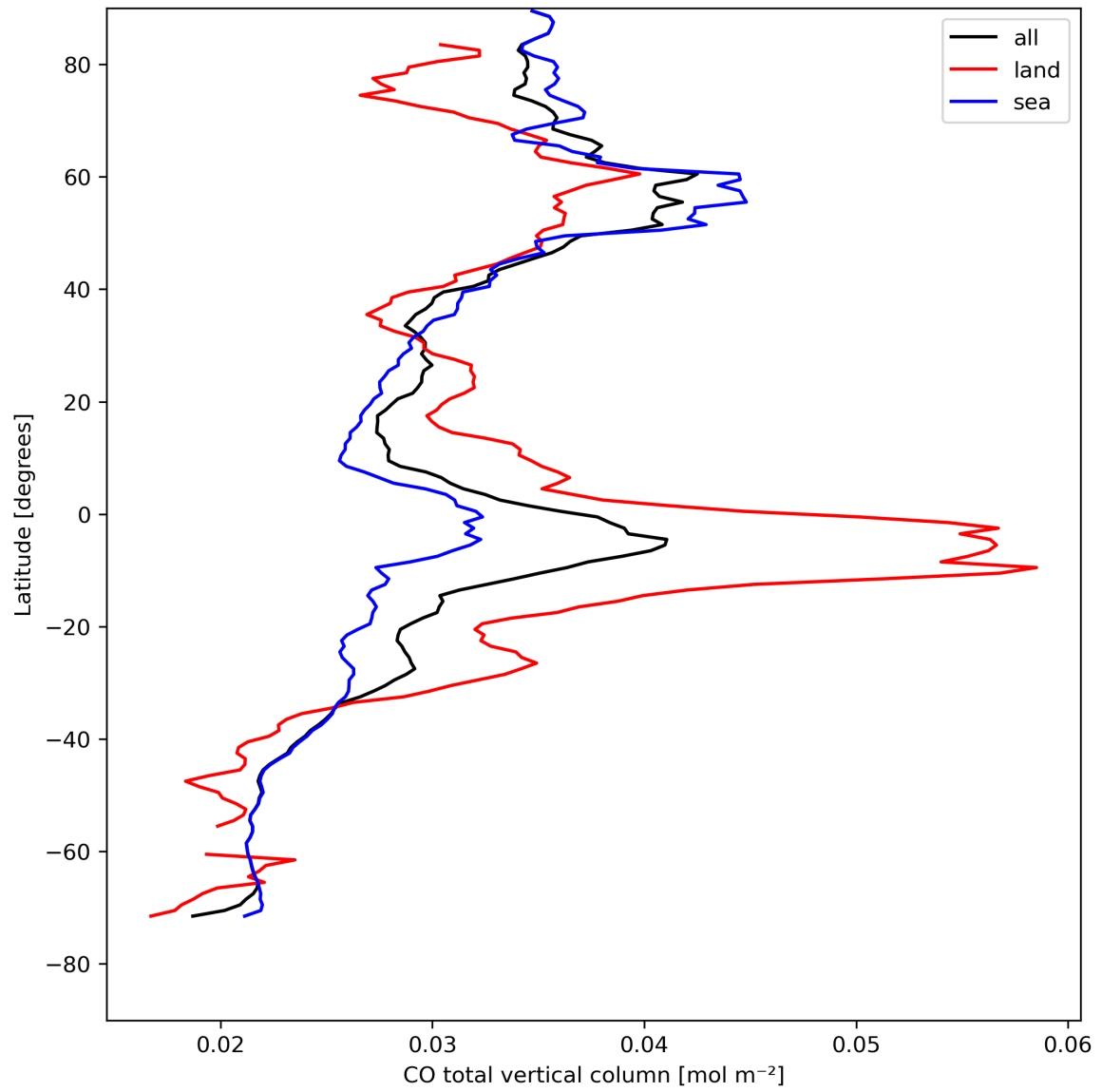
Figure 10: Zonal average of “CO total vertical column” for 2024-08-16 to 2024-08-17.
