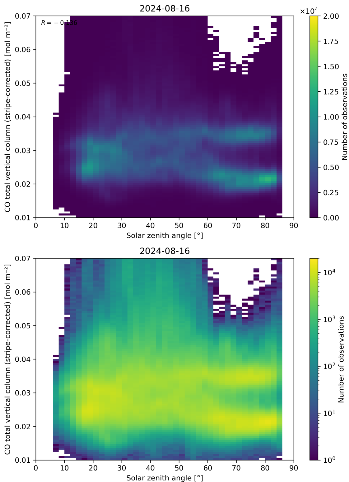
Figure 62: Scatter density plot of “Solar zenith angle” against “CO total vertical column (stripe-corrected)” for 2024-08-16 to 2024-08-17.
