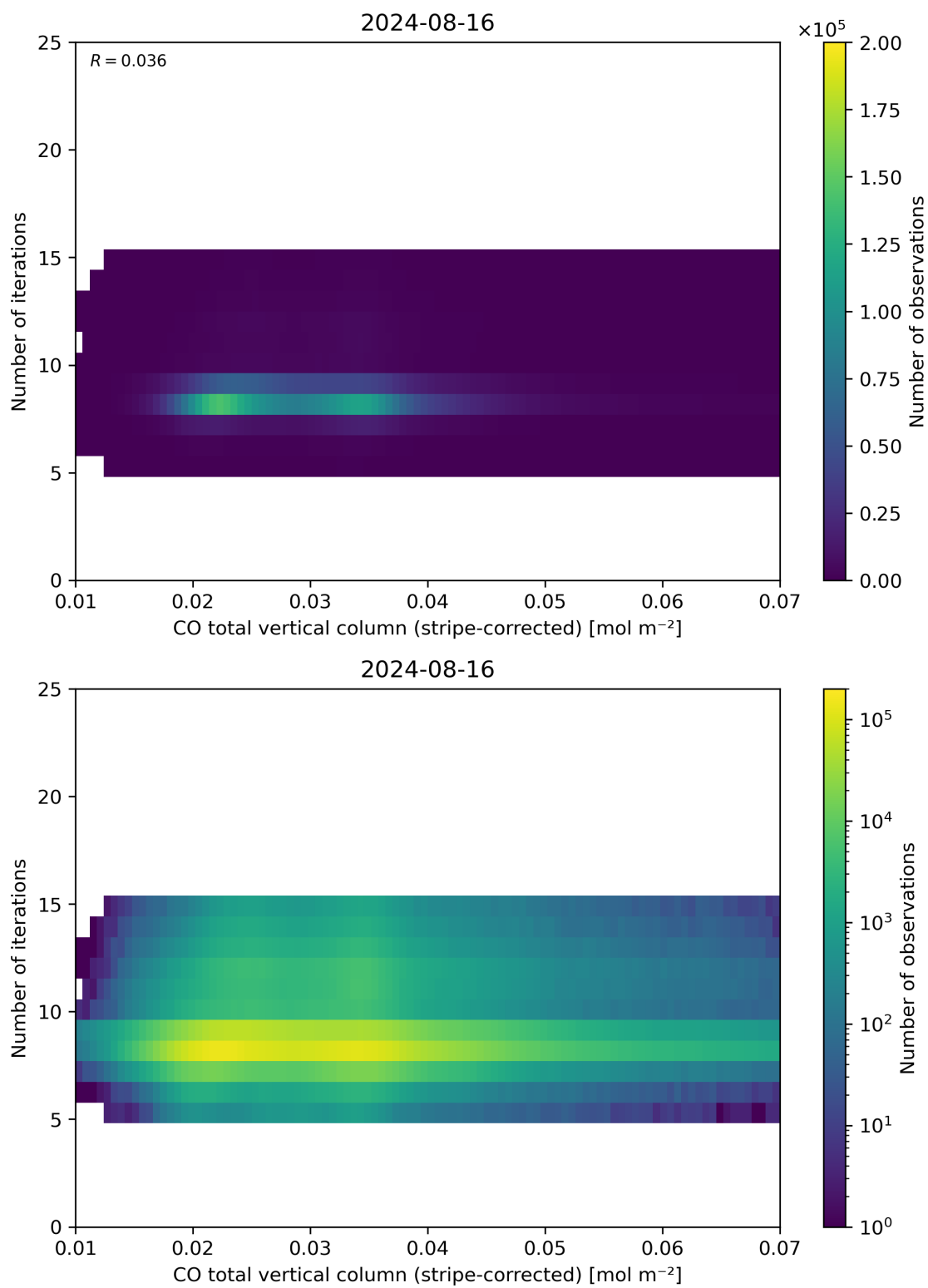
Figure 39: Scatter density plot of “CO total vertical column (stripe-corrected)” against “Number of iterations” for 2024-08-16 to 2024-08-17.
