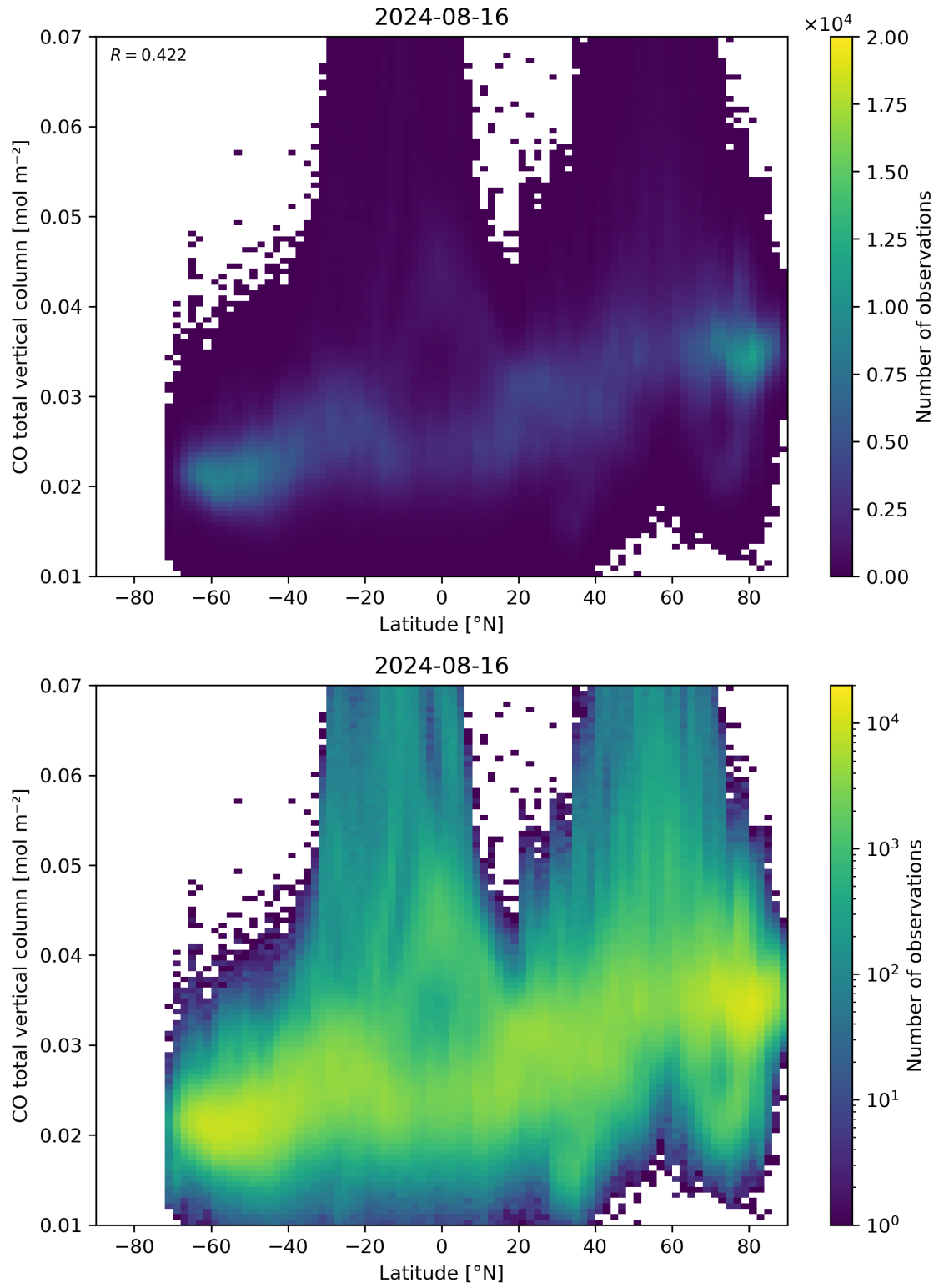
Figure 51: Scatter density plot of “Latitude” against “CO total vertical column” for 2024-08-16 to 2024-08-17.
