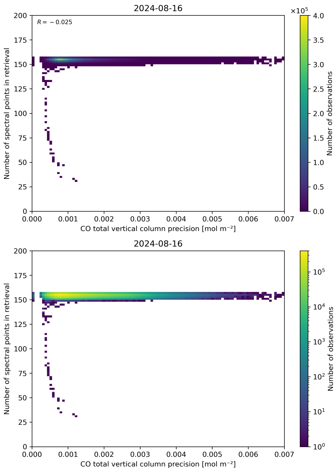
Figure 47: Scatter density plot of “CO total vertical column precision” against “Number of spectral points in retrieval” for 2024-08-16 to 2024-08-17.
