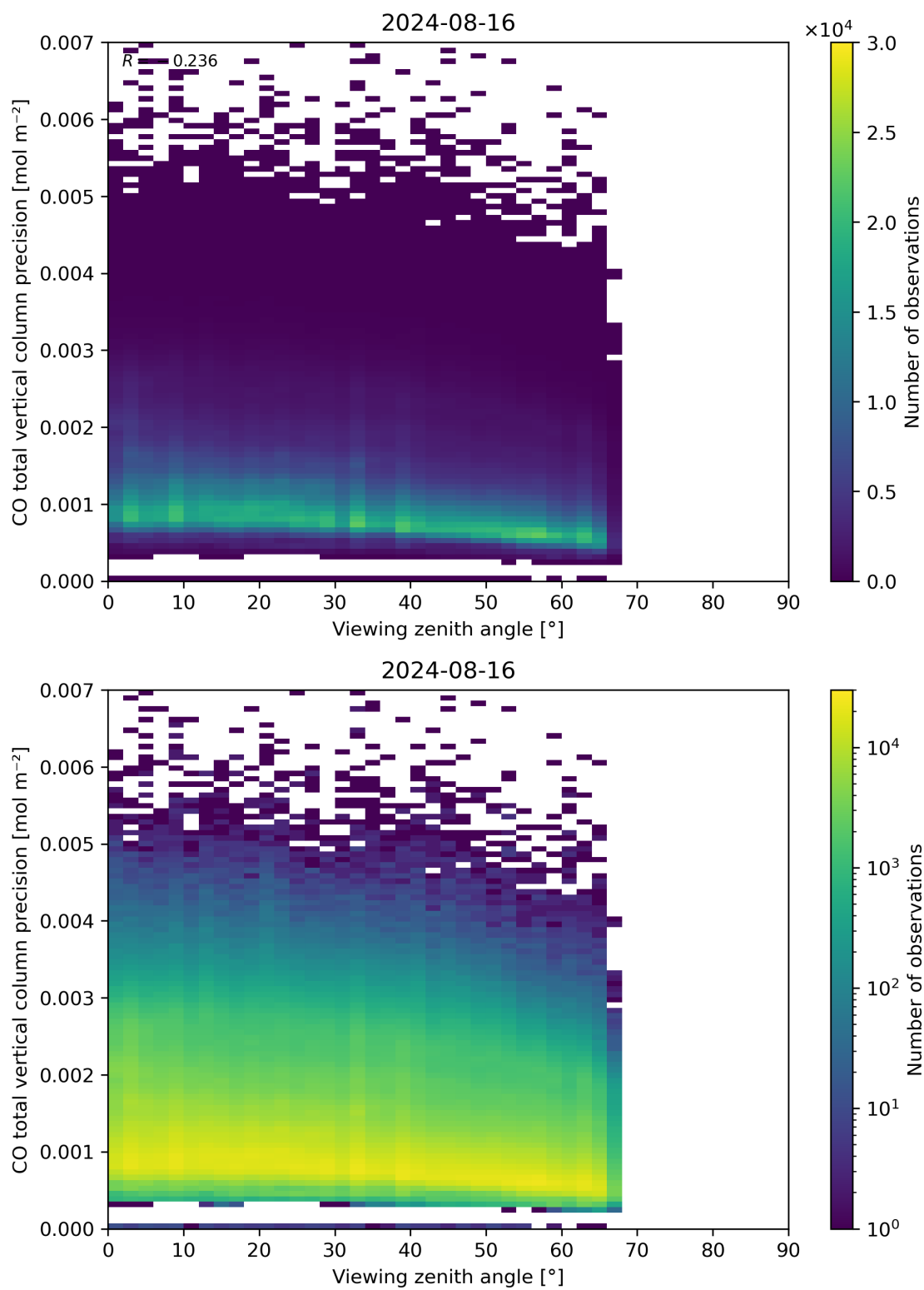
Figure 71: Scatter density plot of “Viewing zenith angle” against “CO total vertical column precision” for 2024-08-16 to 2024-08-17.
