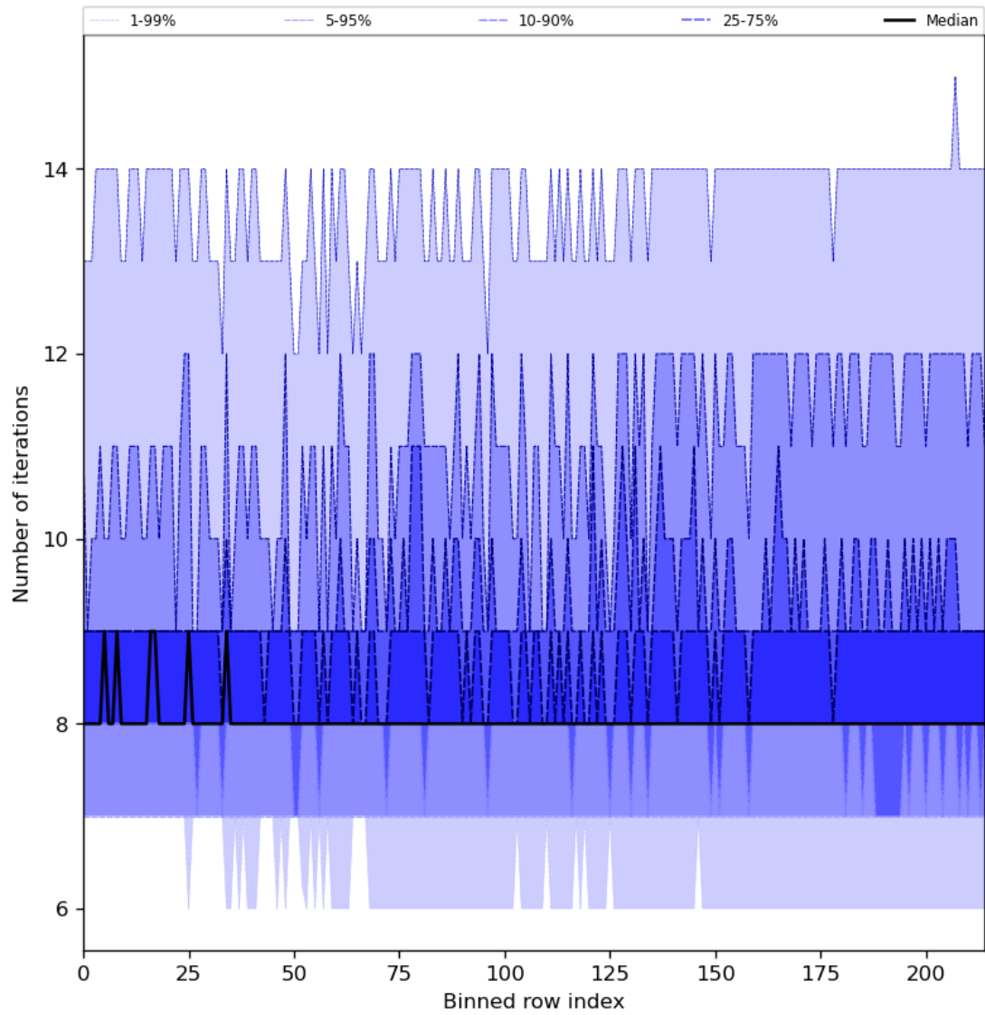
Figure 32: Along track statistics of “Number of iterations” for 2024-08-16 to 2024-08-17
