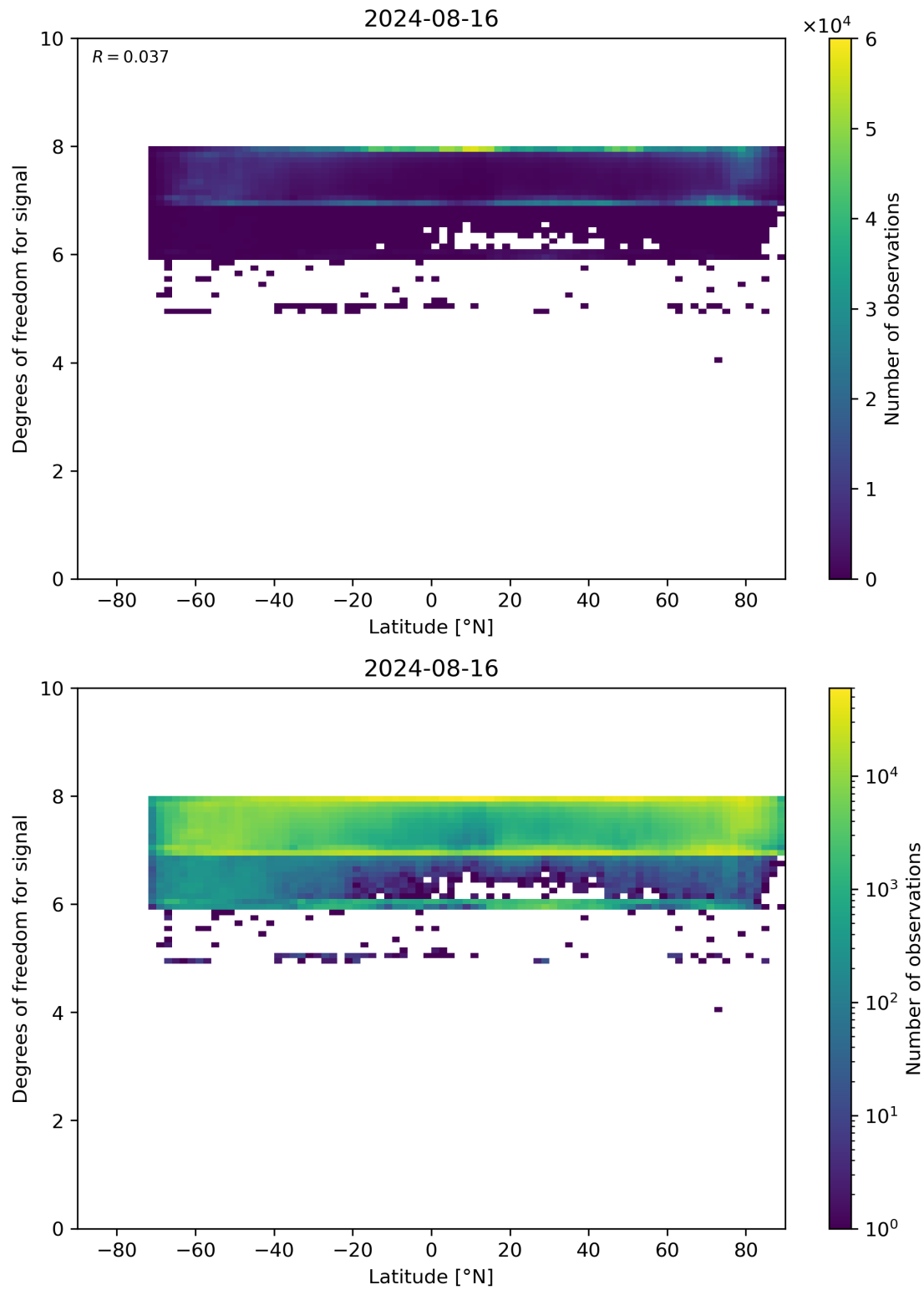
Figure 55: Scatter density plot of “Latitude” against “Degrees of freedom for signal” for 2024-08-16 to 2024-08-17.
