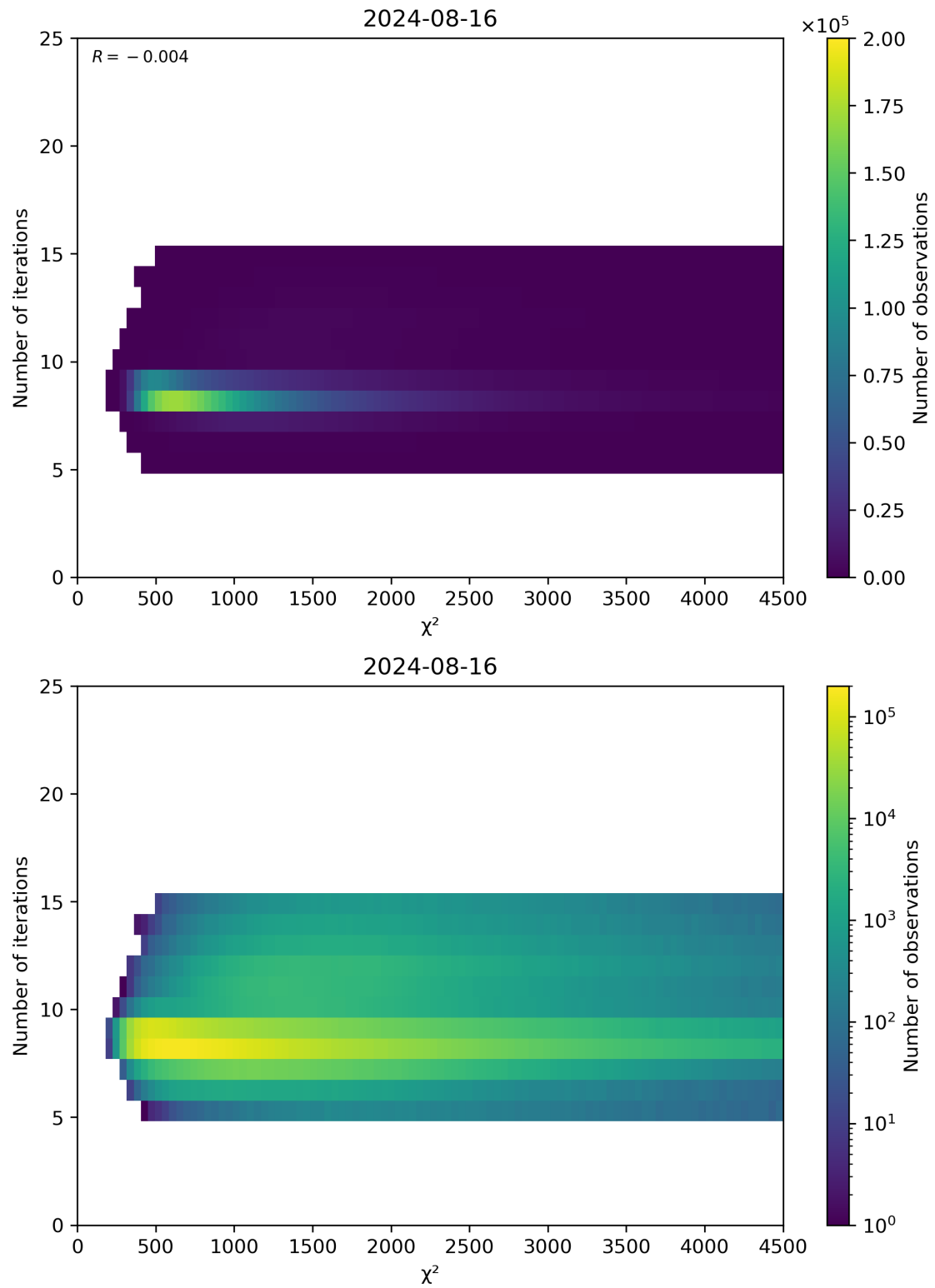
Figure 49: Scatter density plot of “ \chi^2 ” against “Number of iterations” for 2024-08-16 to 2024-08-17.
