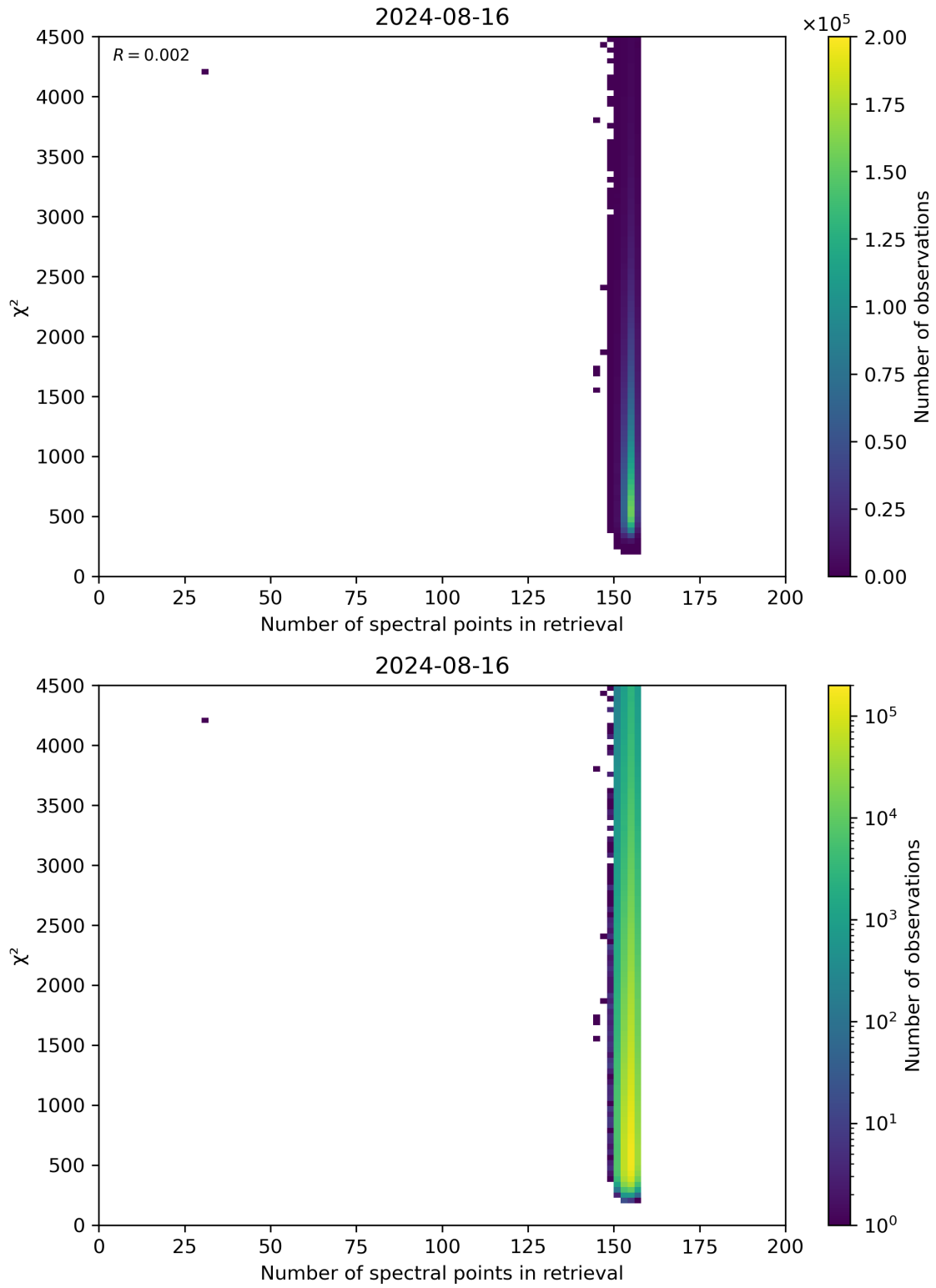
Figure 58: Scatter density plot of “Number of spectral points in retrieval” against “ \chi^2 ” for 2024-08-16 to 2024-08-17.
