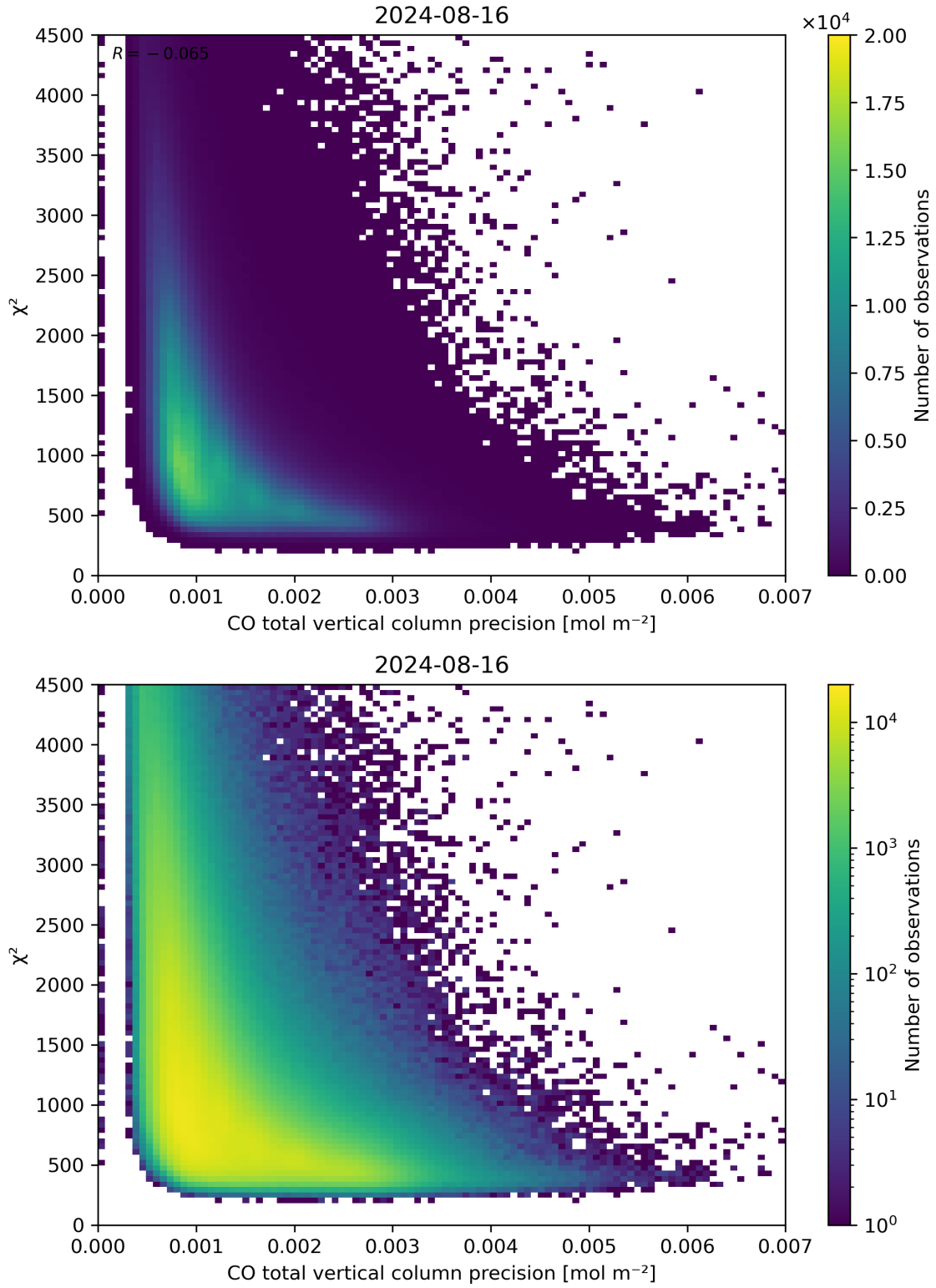
Figure 44: Scatter density plot of “CO total vertical column precision” against “ \chi^2 ” for 2024-08-16 to 2024-08-17.
