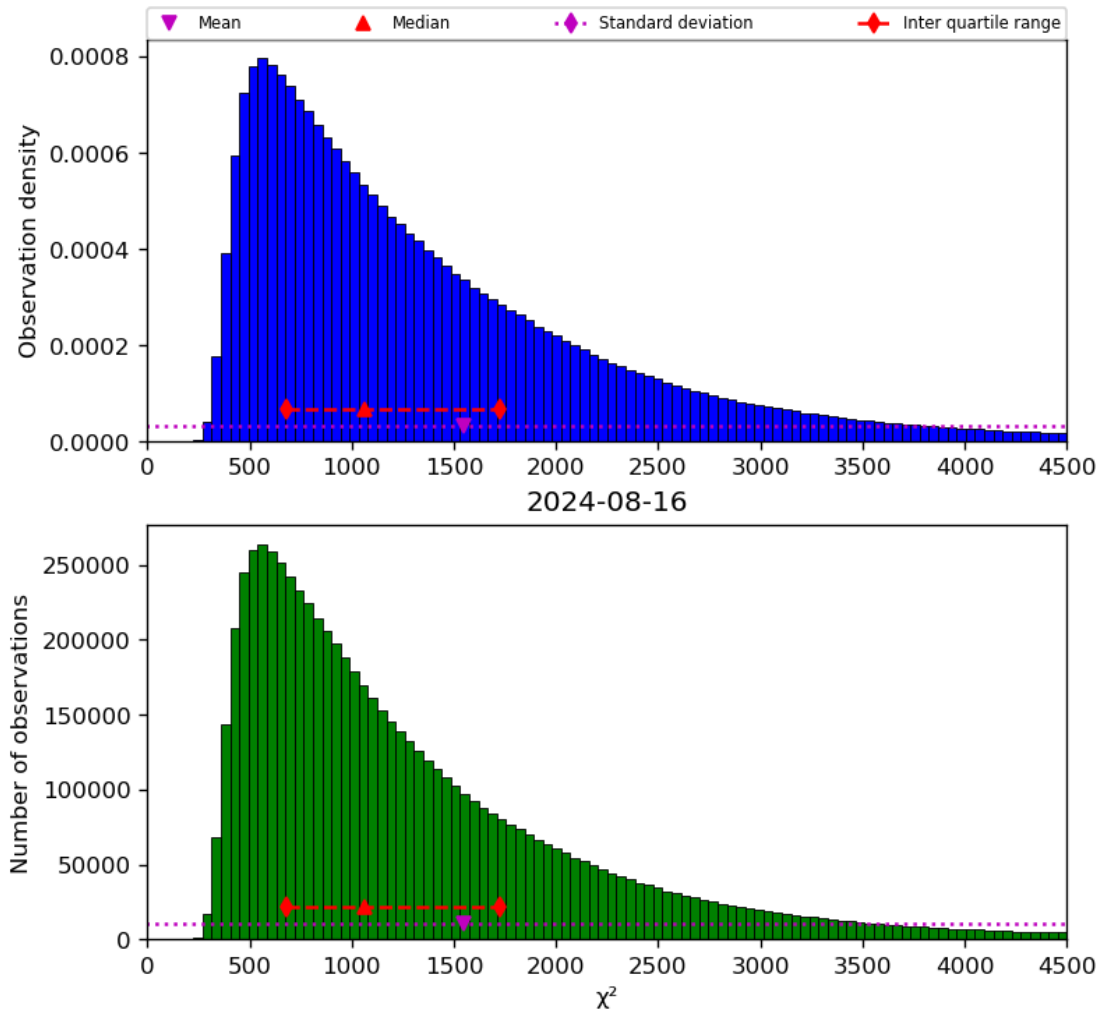
Figure 22: Histogram of “ \chi^2 ” for 2024-08-16 to 2024-08-17
