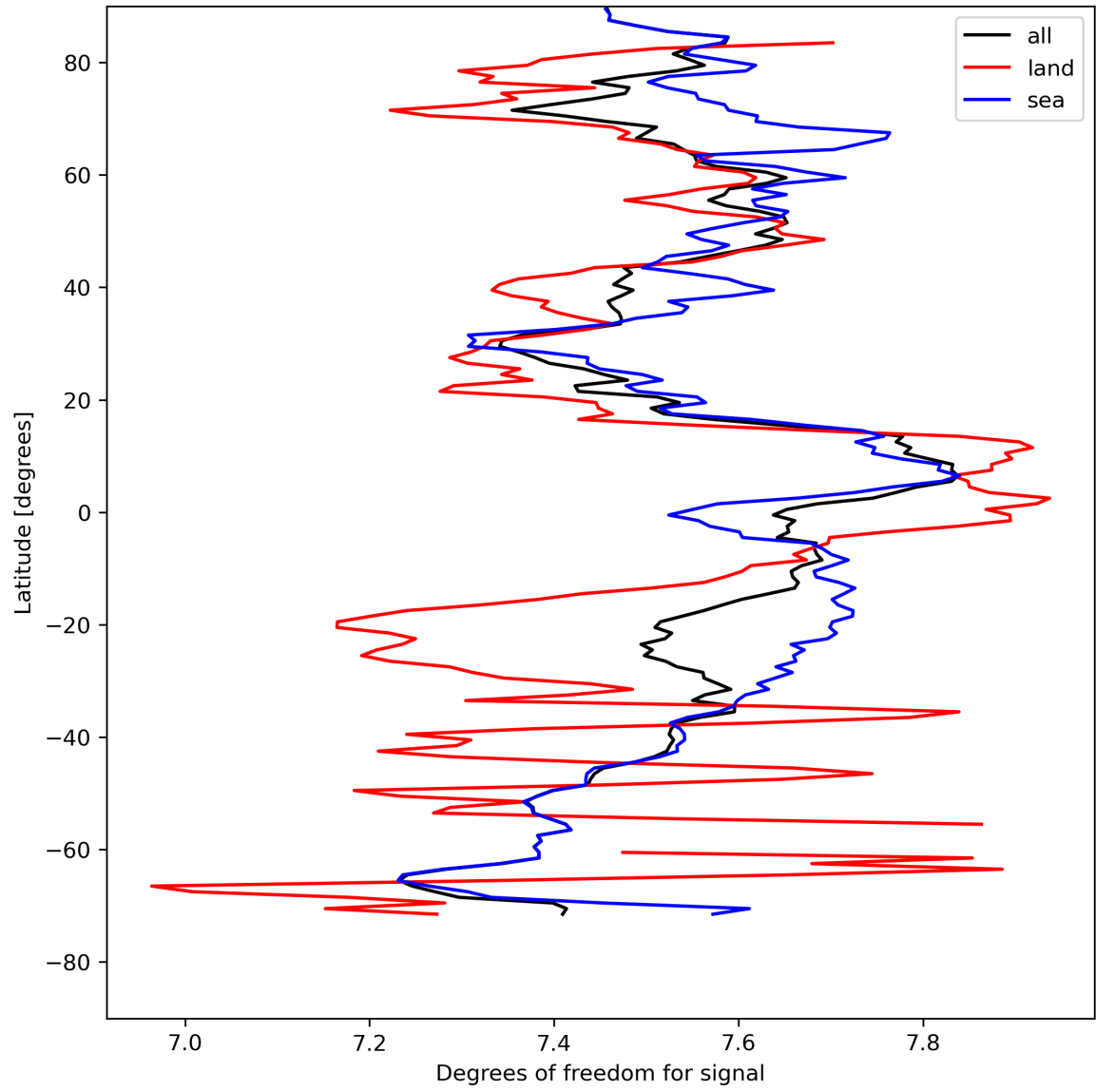
Figure 15: Zonal average of “Degrees of freedom for signal” for 2024-08-16 to 2024-08-17.
