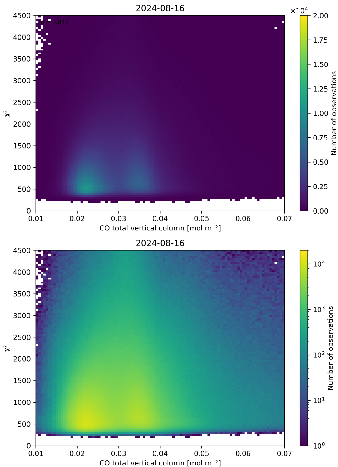
Figure 35: Scatter density plot of “CO total vertical column” against “ \chi^2 ” for 2024-08-16 to 2024-08-17.
