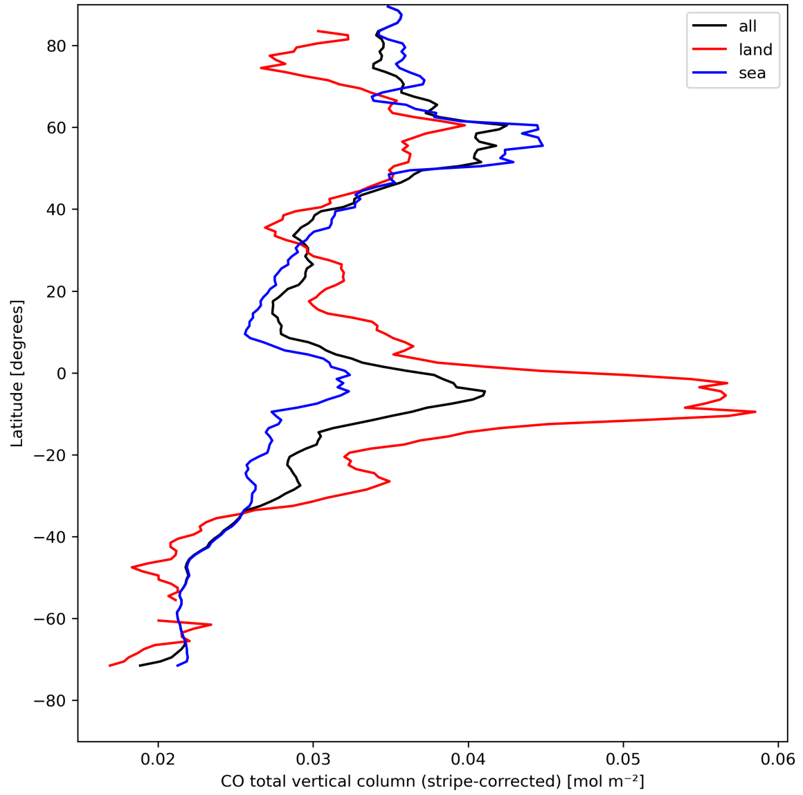
Figure 11: Zonal average of “CO total vertical column (stripe-corrected)” for 2024-08-16 to 2024-08-17.
