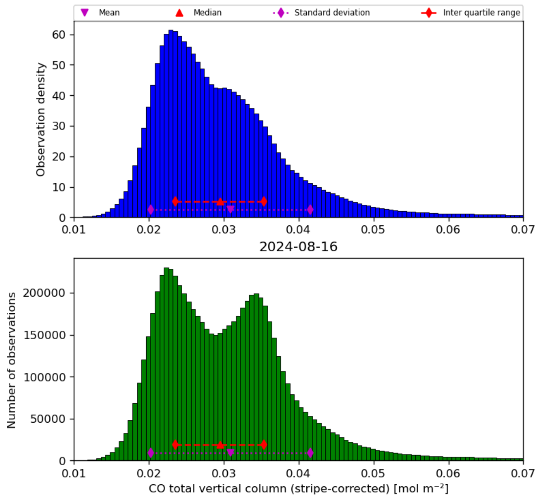
Figure 19: Histogram of “CO total vertical column (stripe-corrected)” for 2024-08-16 to 2024-08-17
