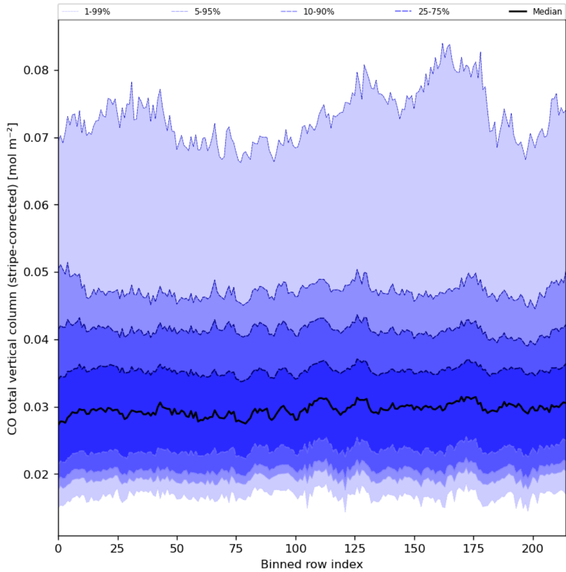
Figure 27: Along track statistics of “CO total vertical column (stripe-corrected)” for 2024-08-16 to 2024-08-17
