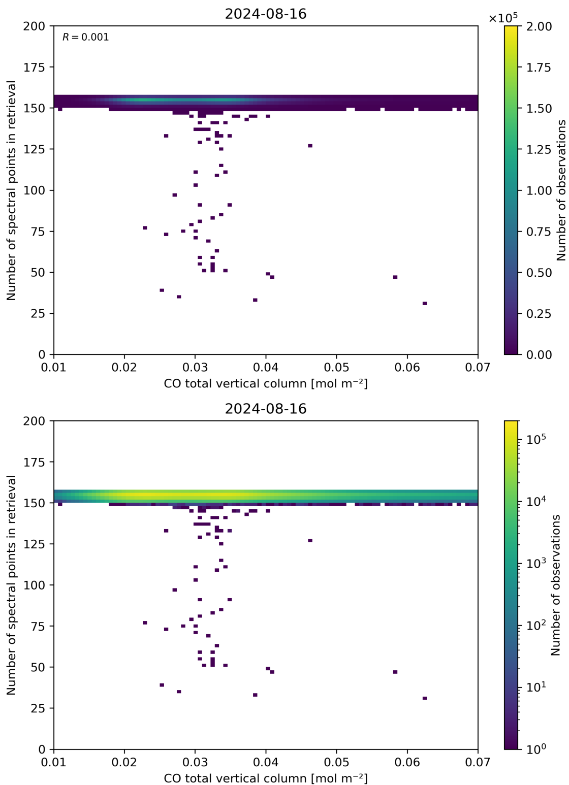
Figure 43: Scatter density plot of “CO total vertical column” against “Number of spectral points in retrieval” for 2024-08-16 to 2024-08-17.
