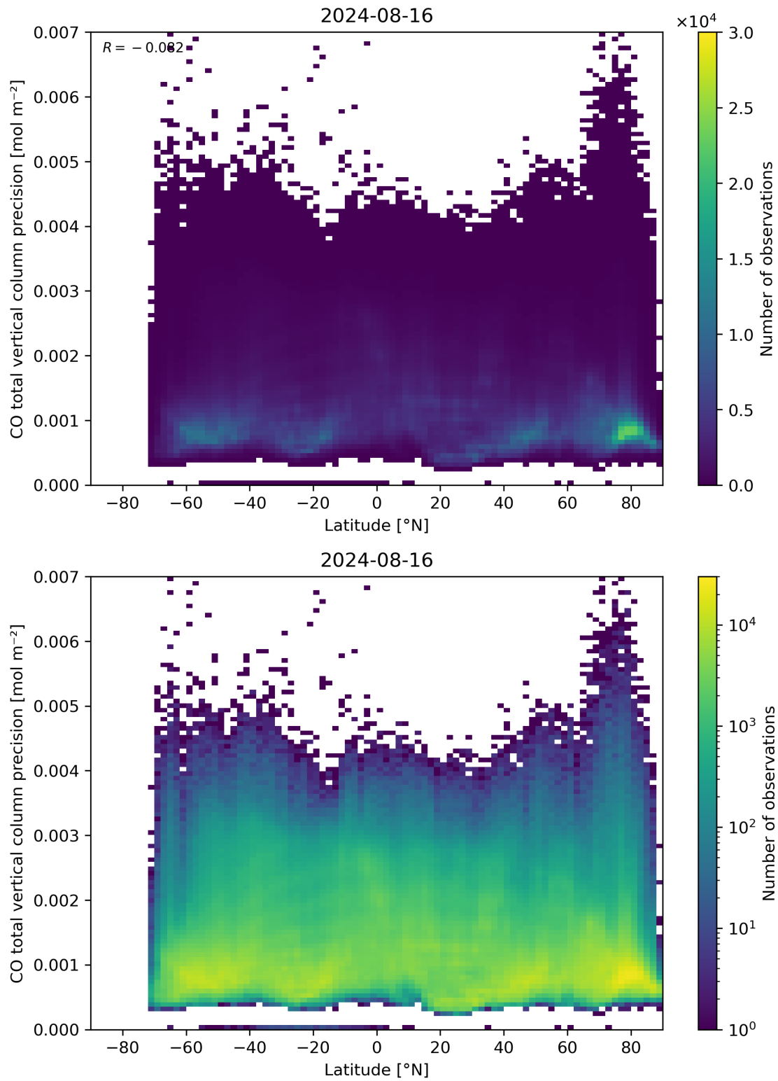
Figure 53: Scatter density plot of “Latitude” against “CO total vertical column precision” for 2024-08-16 to 2024-08-17.
