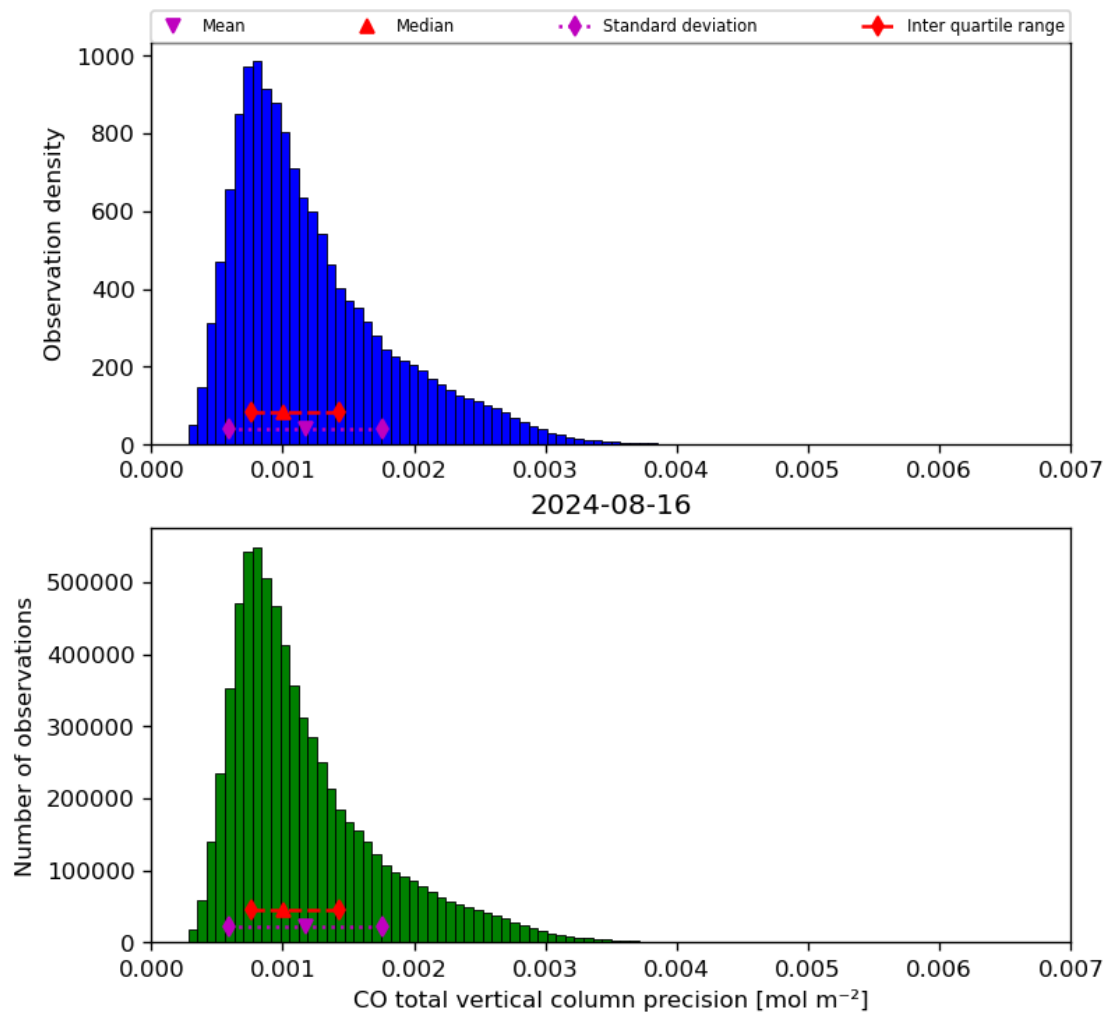
Figure 20: Histogram of “CO total vertical column precision” for 2024-08-16 to 2024-08-17
