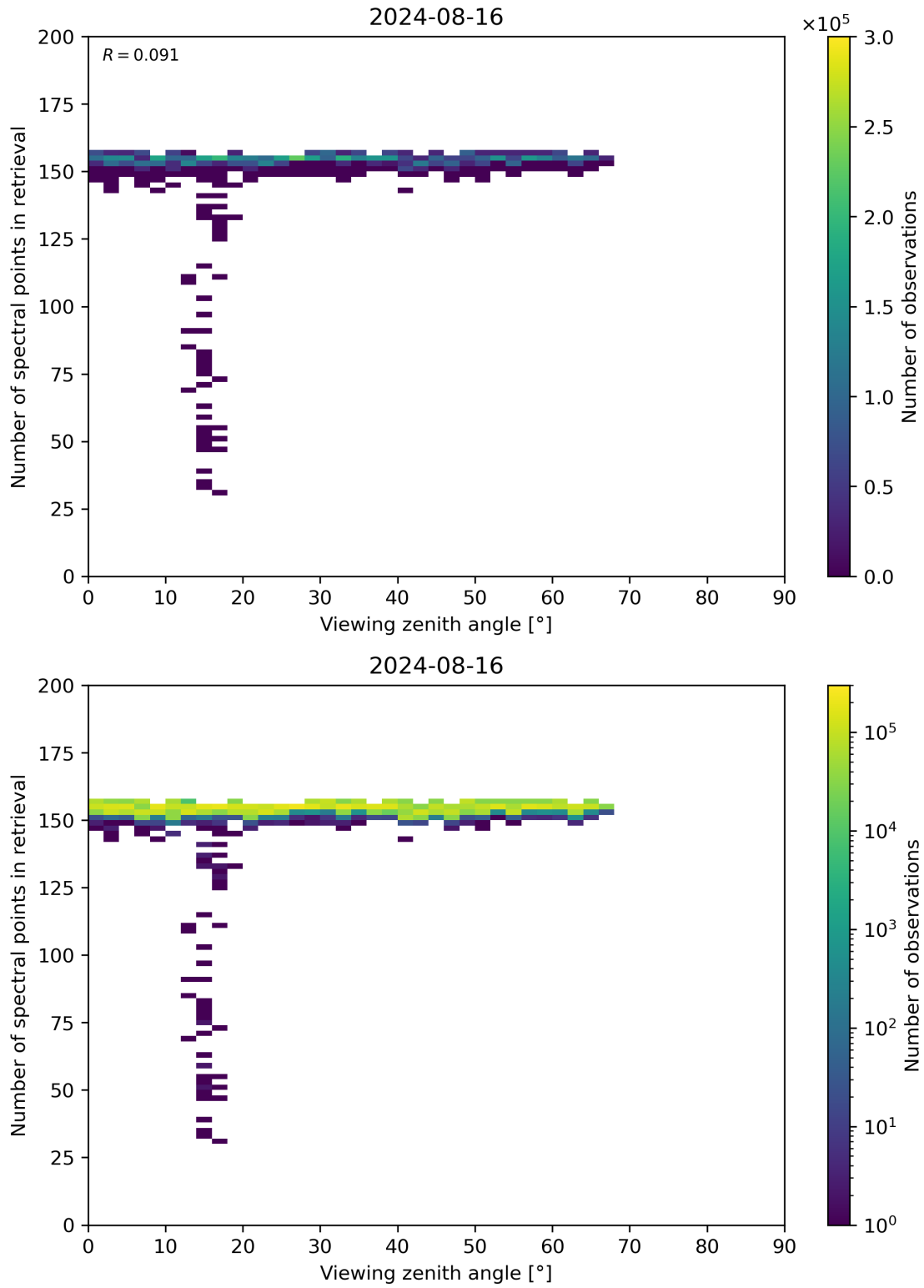
Figure 76: Scatter density plot of “Viewing zenith angle” against “Number of spectral points in retrieval” for 2024-08-16 to 2024-08-17.
