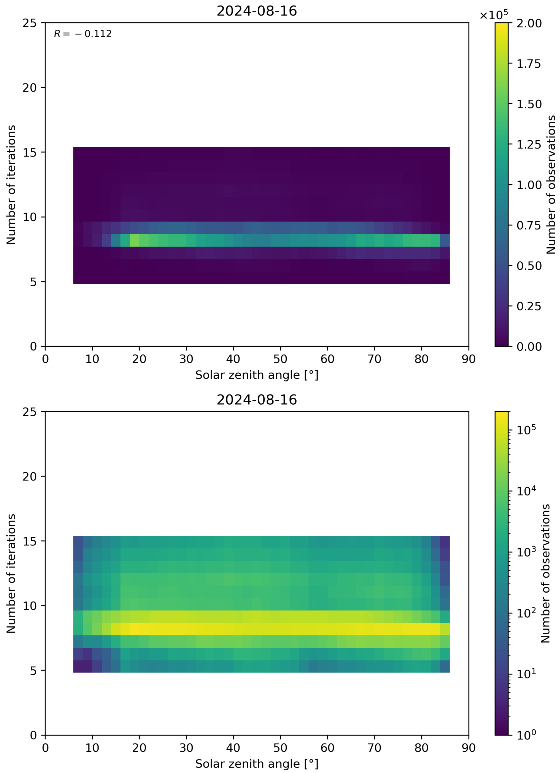
Figure 67: Scatter density plot of “Solar zenith angle” against “Number of iterations” for 2024-08-16 to 2024-08-17.
