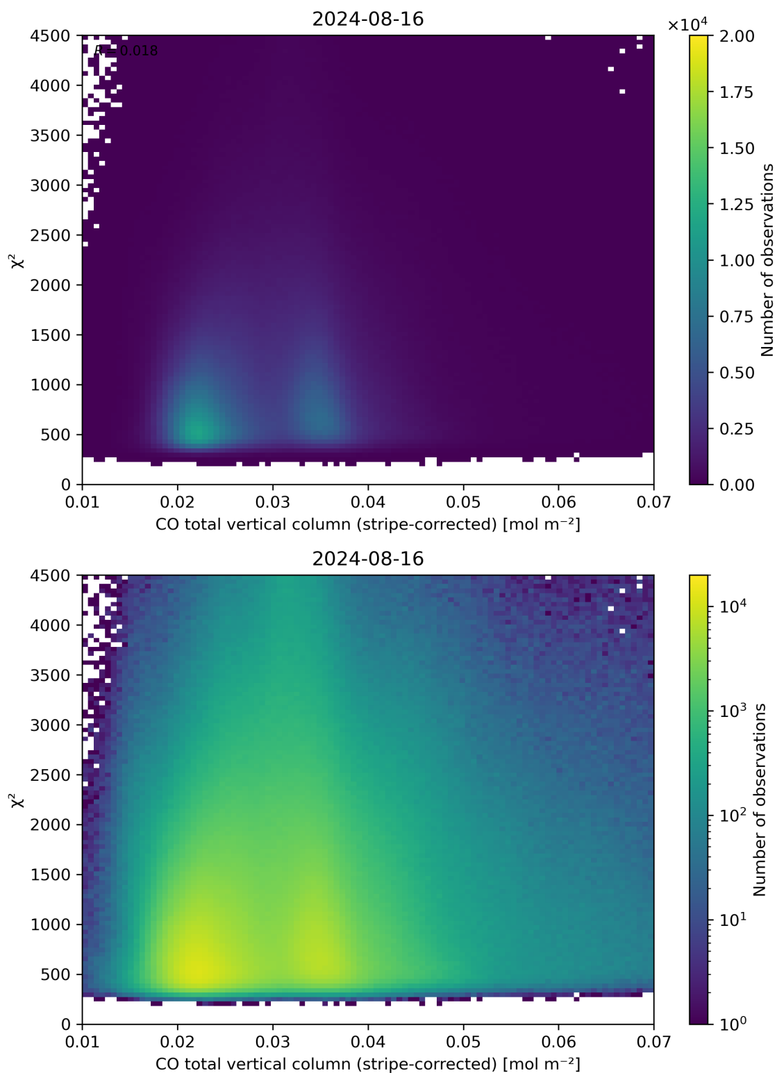
Figure 37: Scatter density plot of “CO total vertical column (stripe-corrected)” against “ \chi^2 ” for 2024-08-16 to 2024-08-17.
