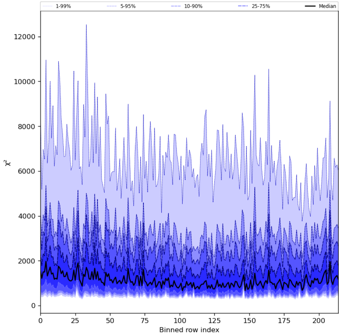
Figure 30: Along track statistics of “ \chi^2 ” for 2024-08-16 to 2024-08-17
