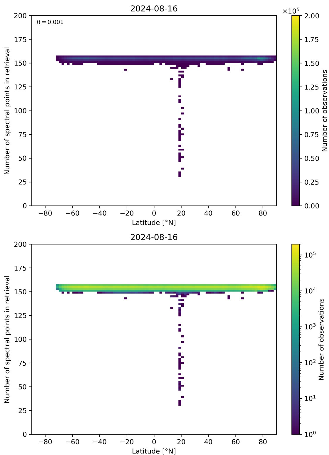
Figure 57: Scatter density plot of “Latitude” against “Number of spectral points in retrieval” for 2024-08-16 to 2024-08-17.
