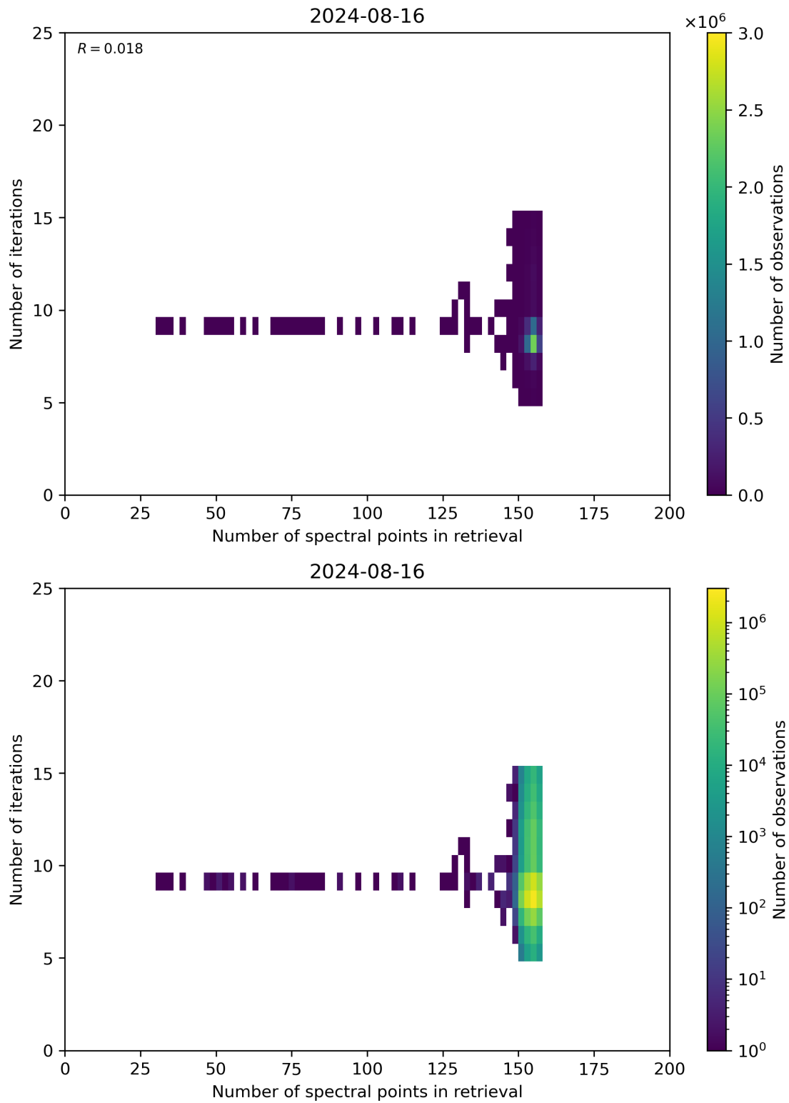
Figure 60: Scatter density plot of “Number of spectral points in retrieval” against “Number of iterations” for 2024-08-16 to 2024-08-17.
