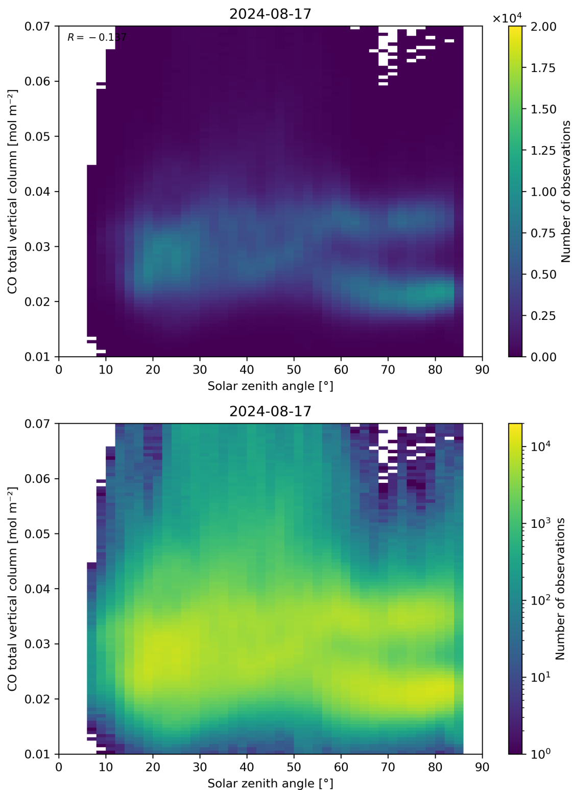
Figure 61: Scatter density plot of “Solar zenith angle” against “CO total vertical column” for 2024-08-16 to 2024-08-18.
