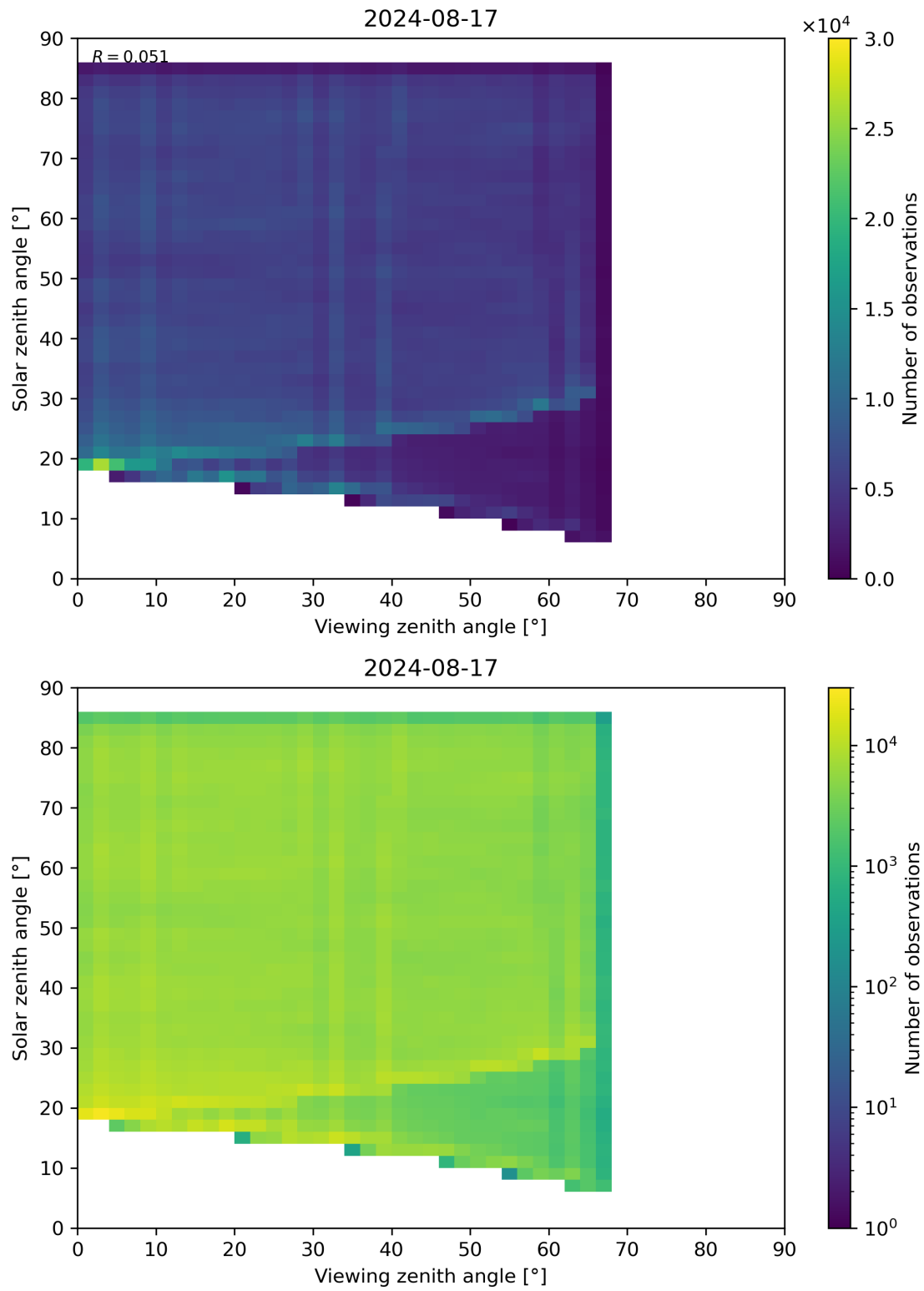
Figure 77: Scatter density plot of “Viewing zenith angle” against “Solar zenith angle” for 2024-08-16 to 2024-08-18.
