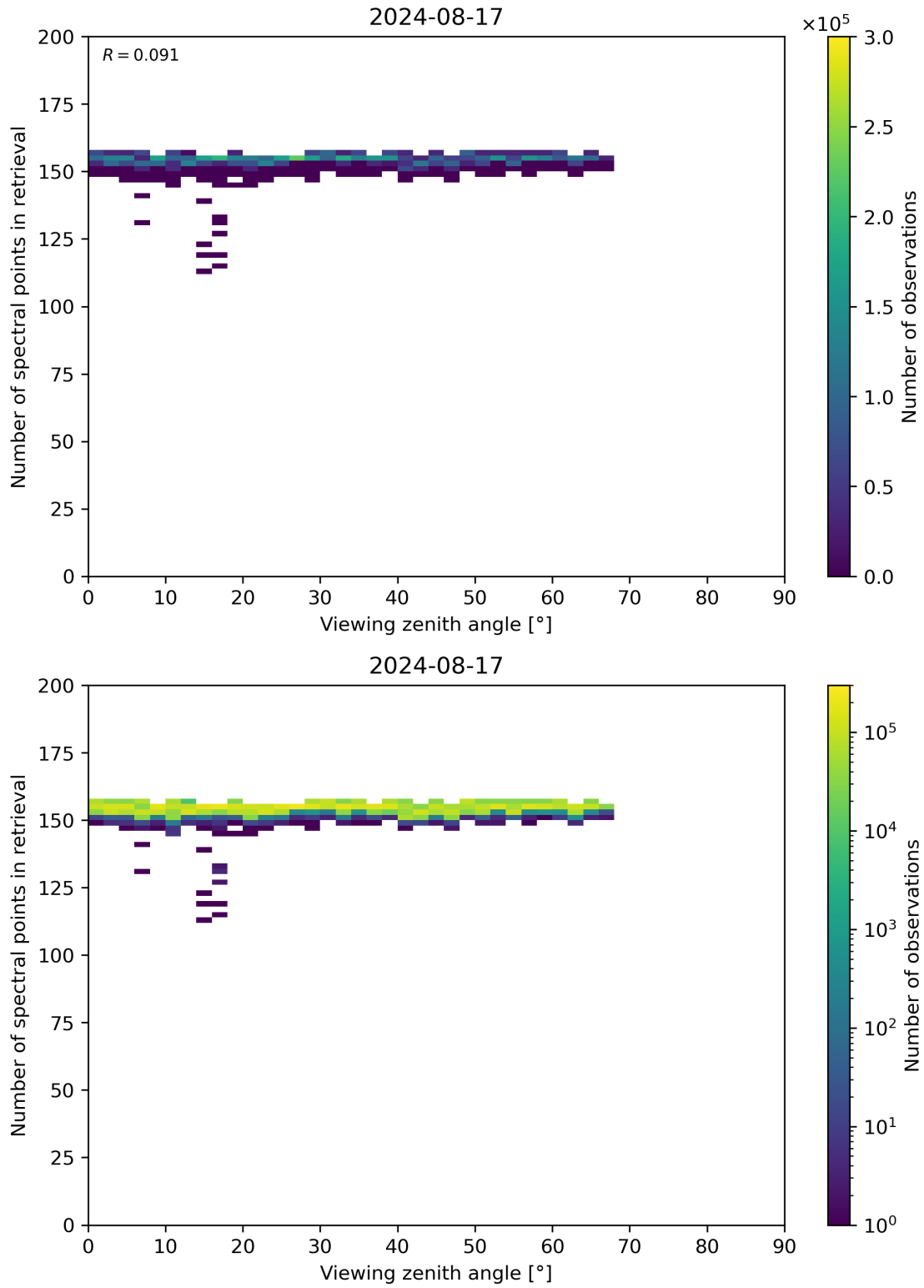
Figure 76: Scatter density plot of “Viewing zenith angle” against “Number of spectral points in retrieval” for 2024-08-16 to 2024-08-18.
