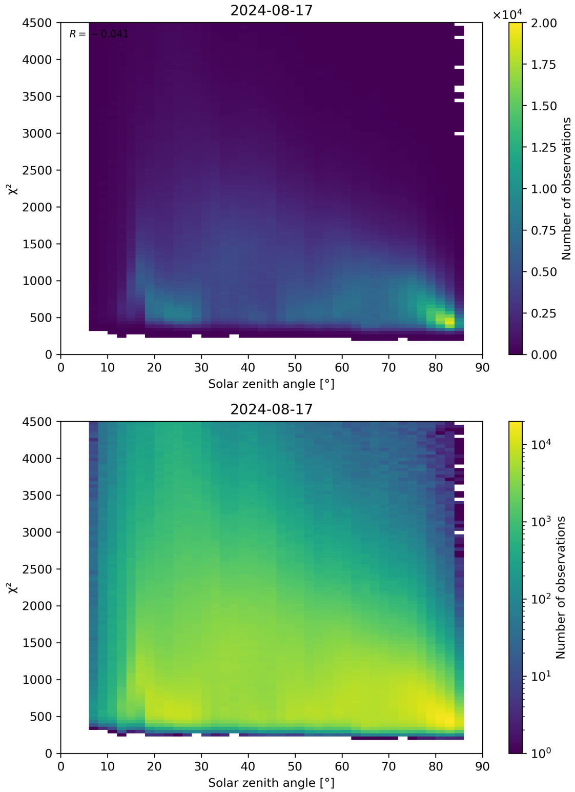
Figure 64: Scatter density plot of “Solar zenith angle” against “ \chi^2 ” for 2024-08-16 to 2024-08-18.
