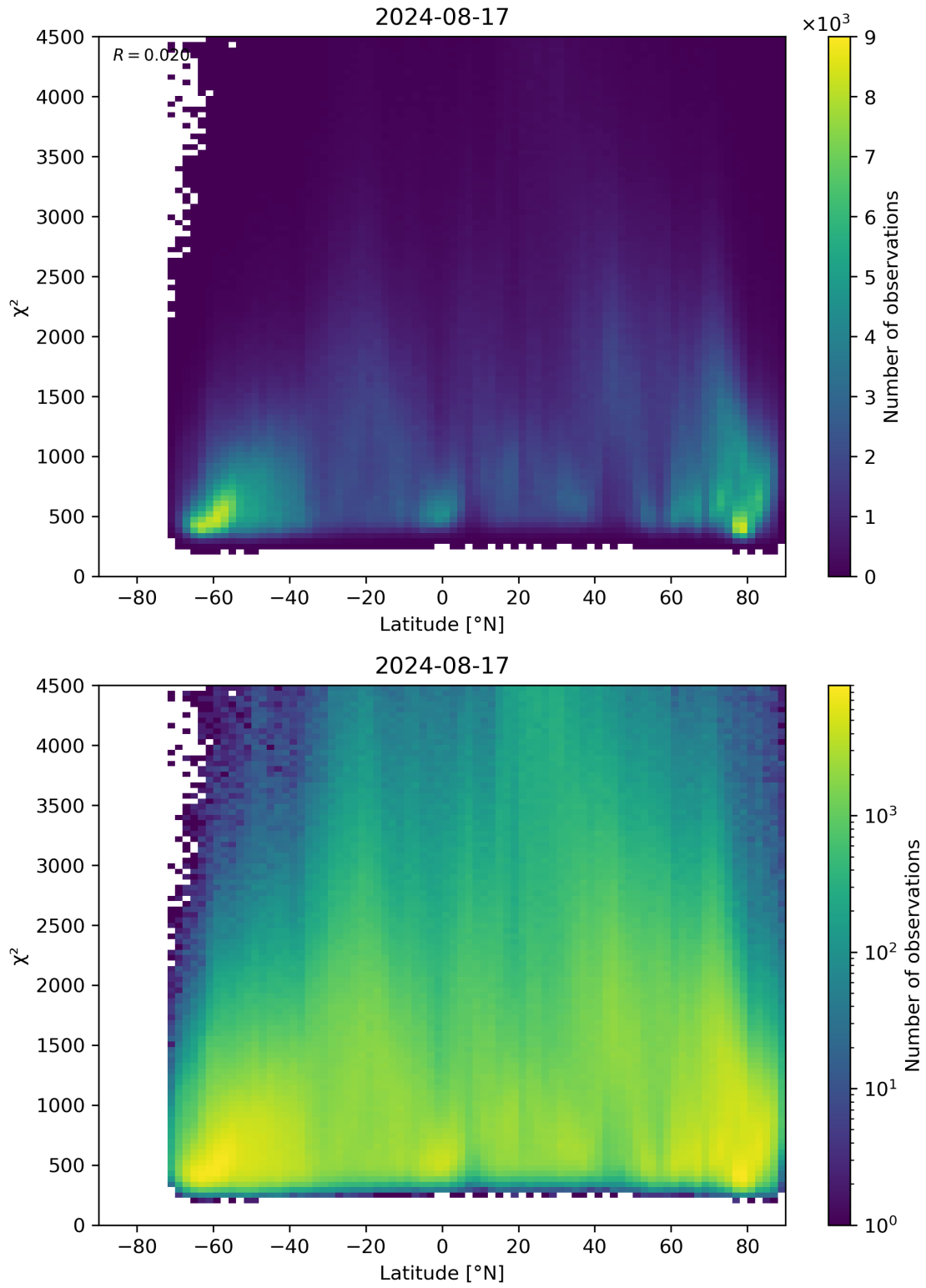
Figure 54: Scatter density plot of “Latitude” against “ \chi^2 ” for 2024-08-16 to 2024-08-18.
