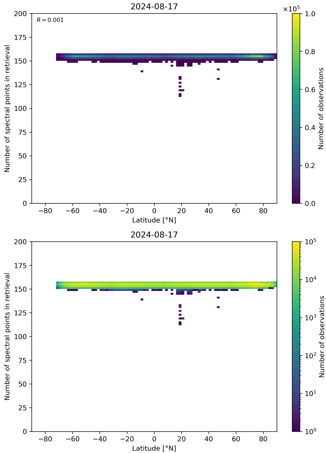
Figure 57: Scatter density plot of “Latitude” against “Number of spectral points in retrieval” for 2024-08-16 to 2024-08-18.
