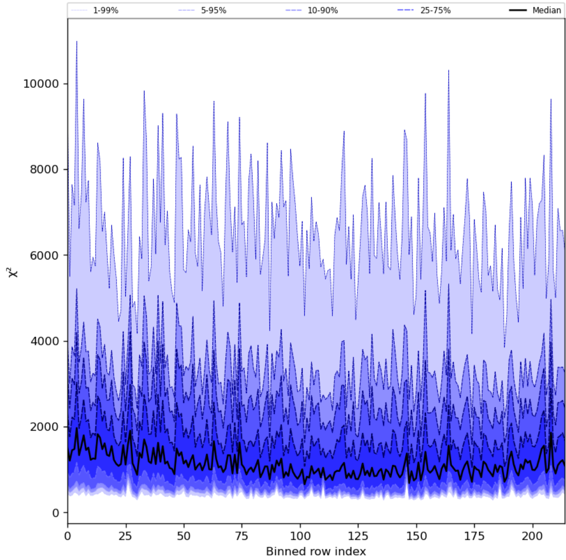
Figure 30: Along track statistics of “ \chi^2 ” for 2024-08-16 to 2024-08-18
