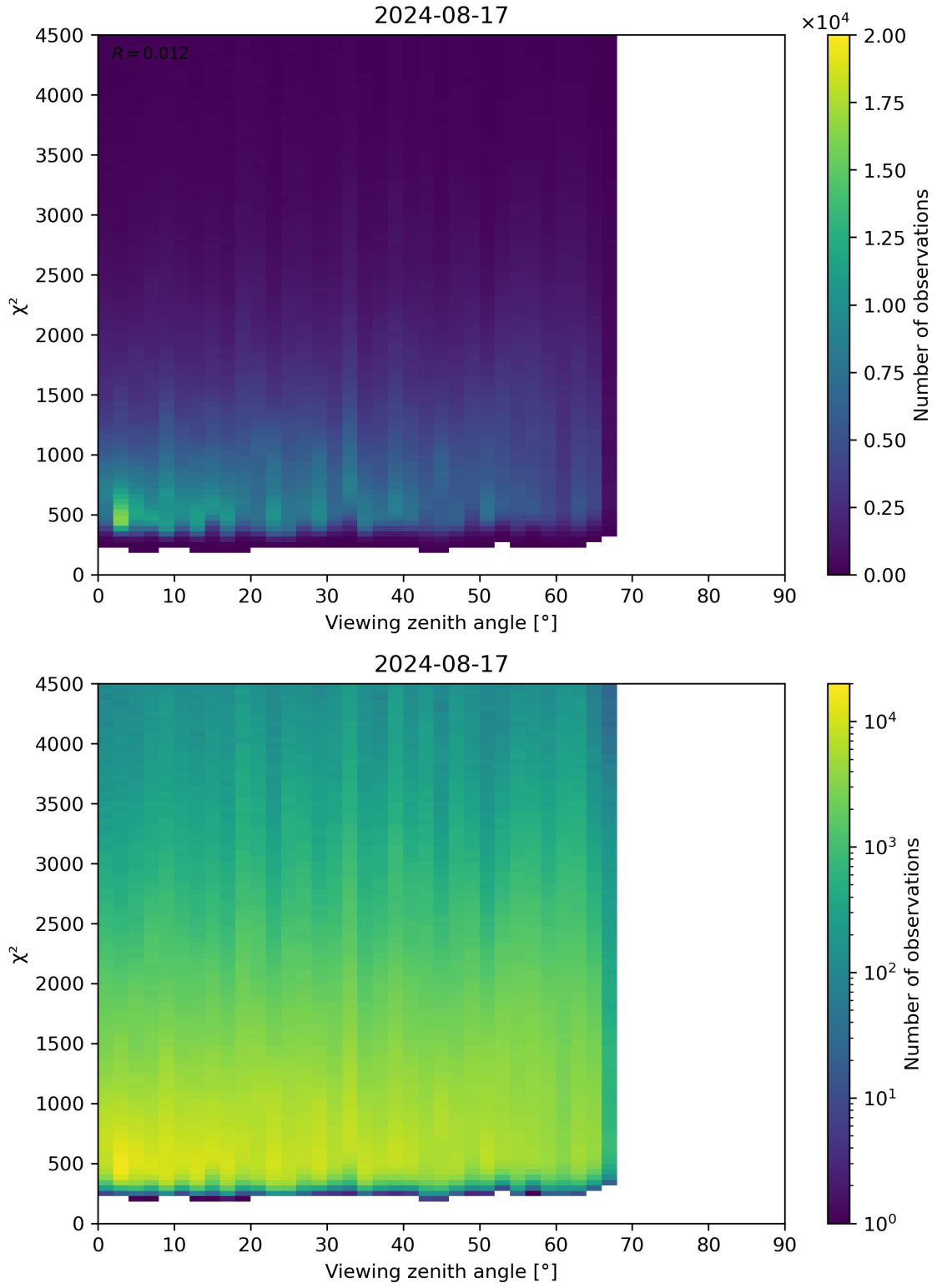
Figure 72: Scatter density plot of “Viewing zenith angle” against “ \chi^2 ” for 2024-08-16 to 2024-08-18.
