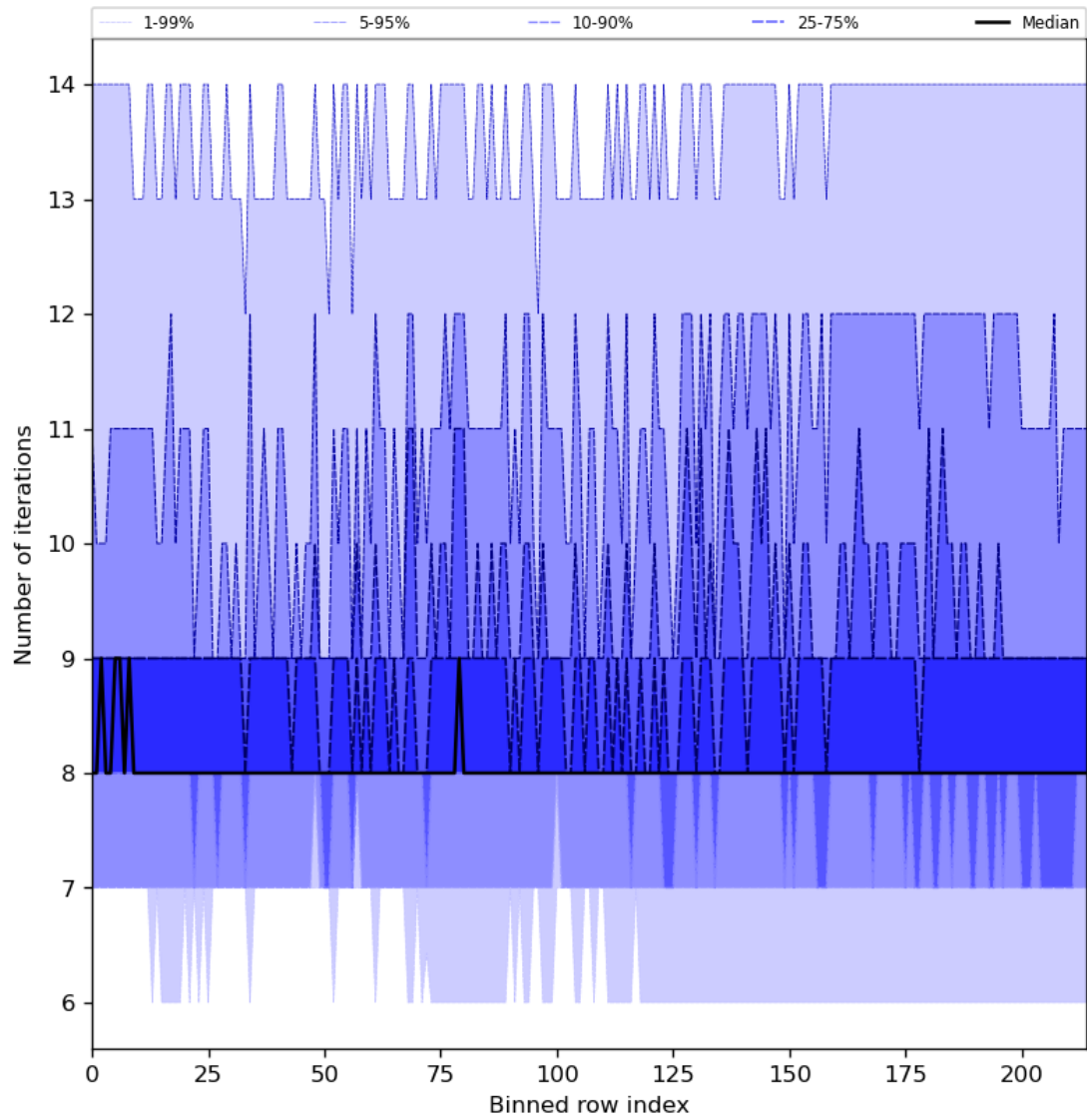
Figure 32: Along track statistics of “Number of iterations” for 2024-08-16 to 2024-08-18
