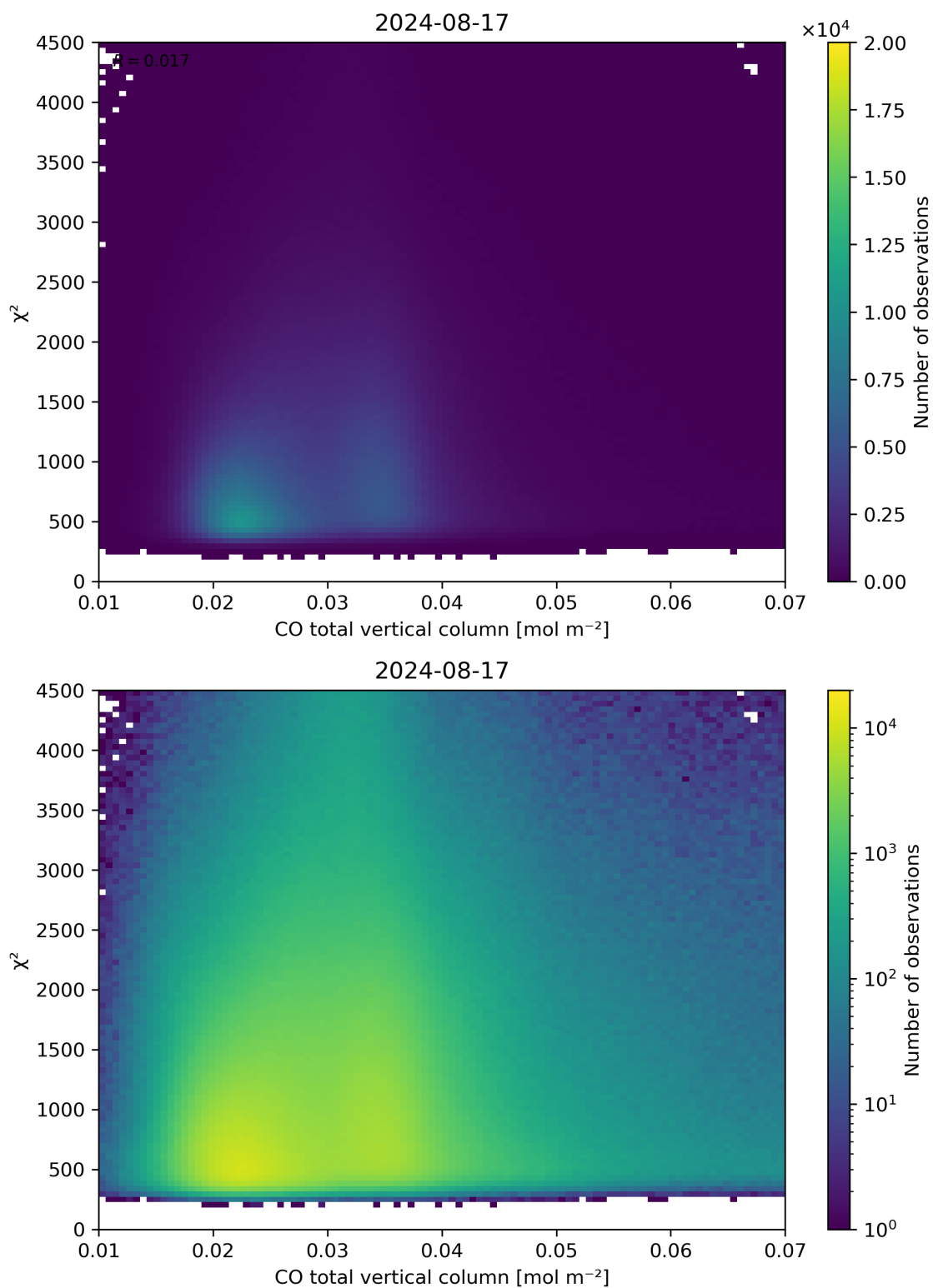
Figure 35: Scatter density plot of “CO total vertical column” against “ \chi^2 ” for 2024-08-16 to 2024-08-18.
