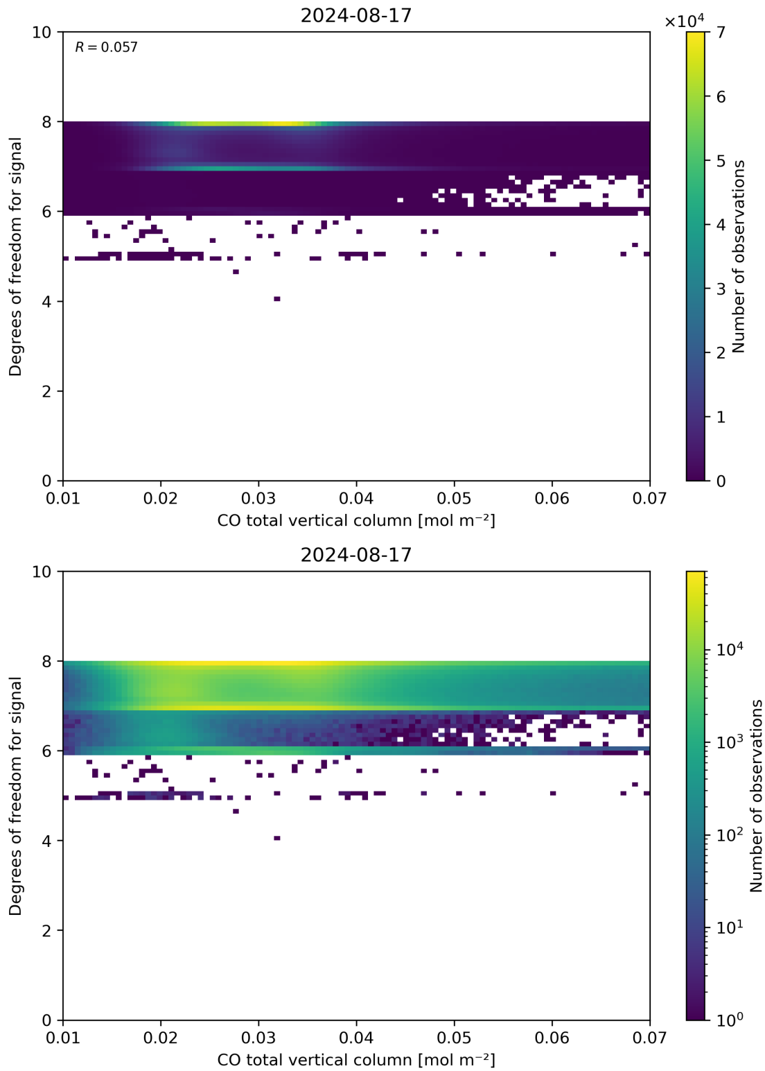
Figure 41: Scatter density plot of “CO total vertical column” against “Degrees of freedom for signal” for 2024-08-16 to 2024-08-18.
