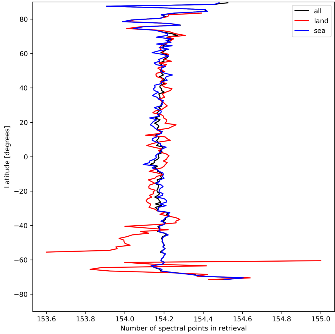
Figure 13: Zonal average of “Number of spectral points in retrieval” for 2024-08-16 to 2024-08-18.
