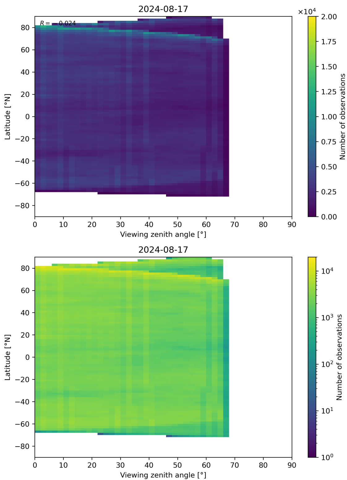
Figure 74: Scatter density plot of “Viewing zenith angle” against “Latitude” for 2024-08-16 to 2024-08-18.
