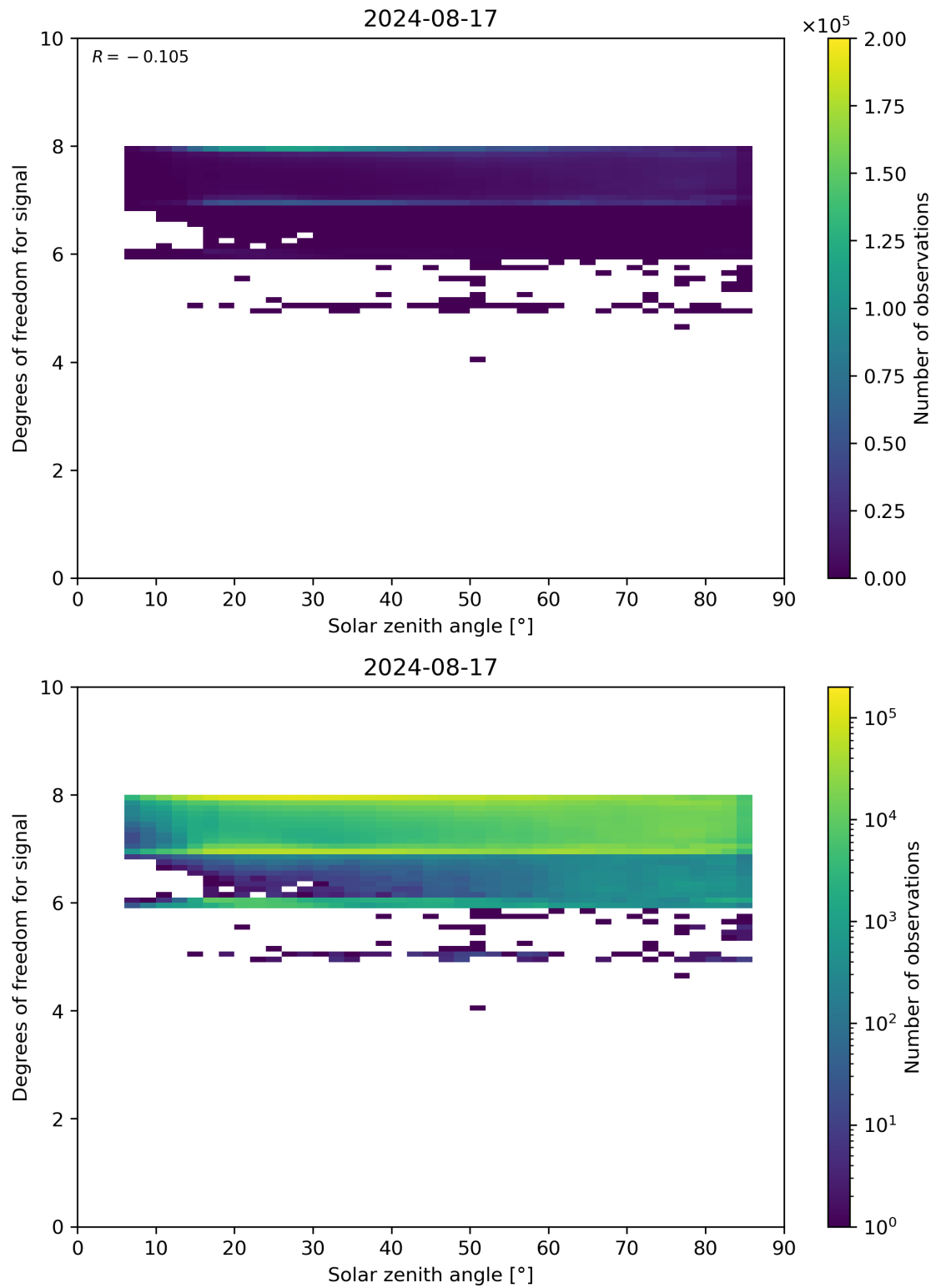
Figure 65: Scatter density plot of “Solar zenith angle” against “Degrees of freedom for signal” for 2024-08-16 to 2024-08-18.
