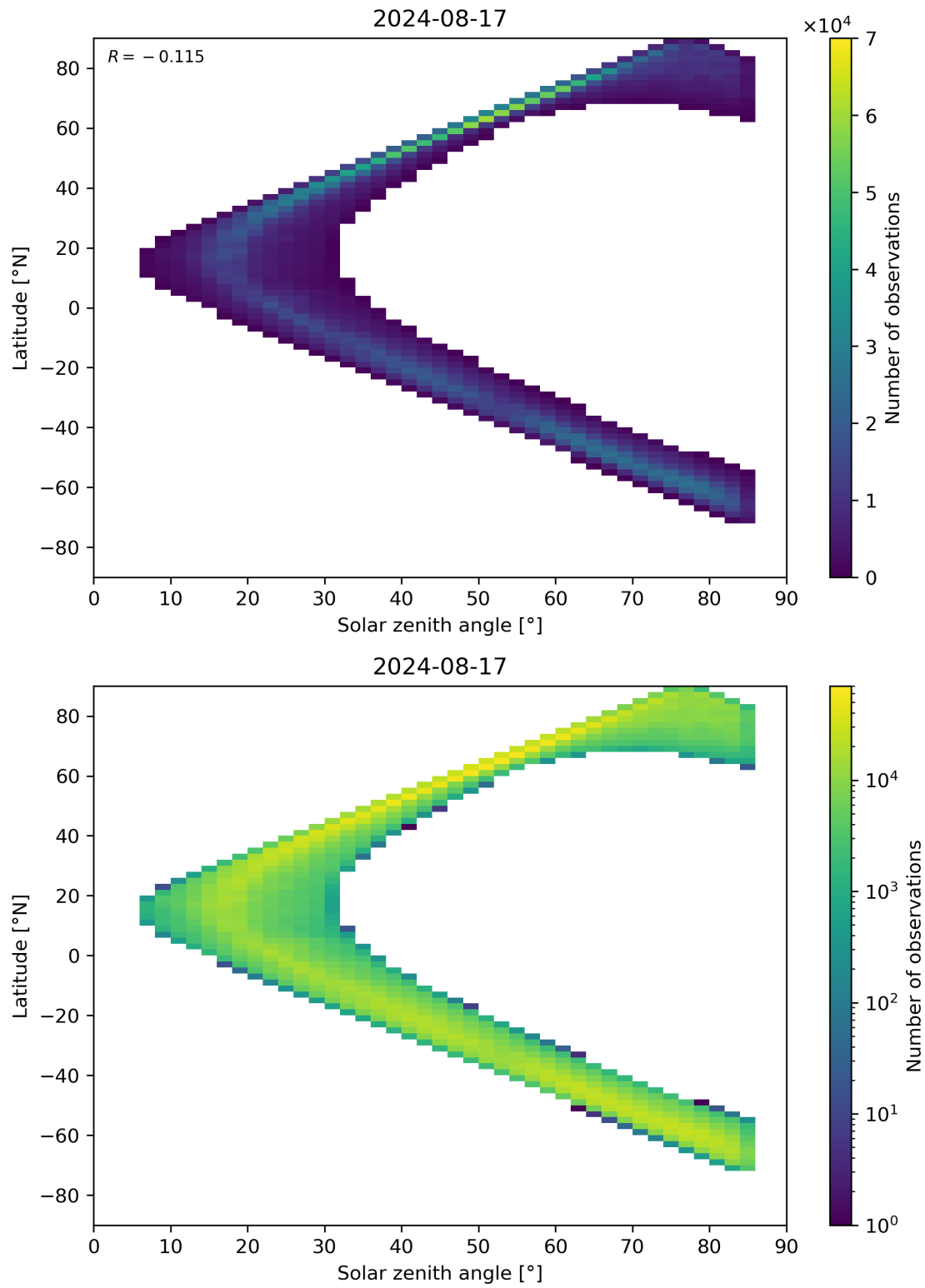
Figure 66: Scatter density plot of “Solar zenith angle” against “Latitude” for 2024-08-16 to 2024-08-18.
