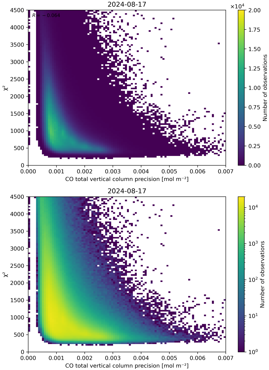
Figure 44: Scatter density plot of “CO total vertical column precision” against “ \chi^2 ” for 2024-08-16 to 2024-08-18.
