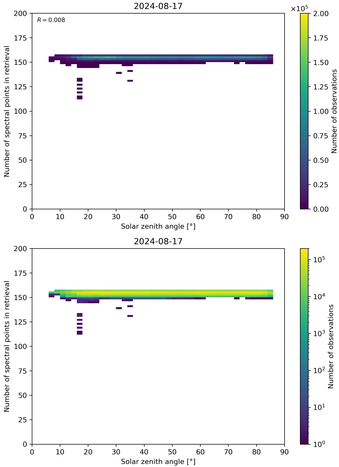
Figure 68: Scatter density plot of “Solar zenith angle” against “Number of spectral points in retrieval” for 2024-08-16 to 2024-08-18.
