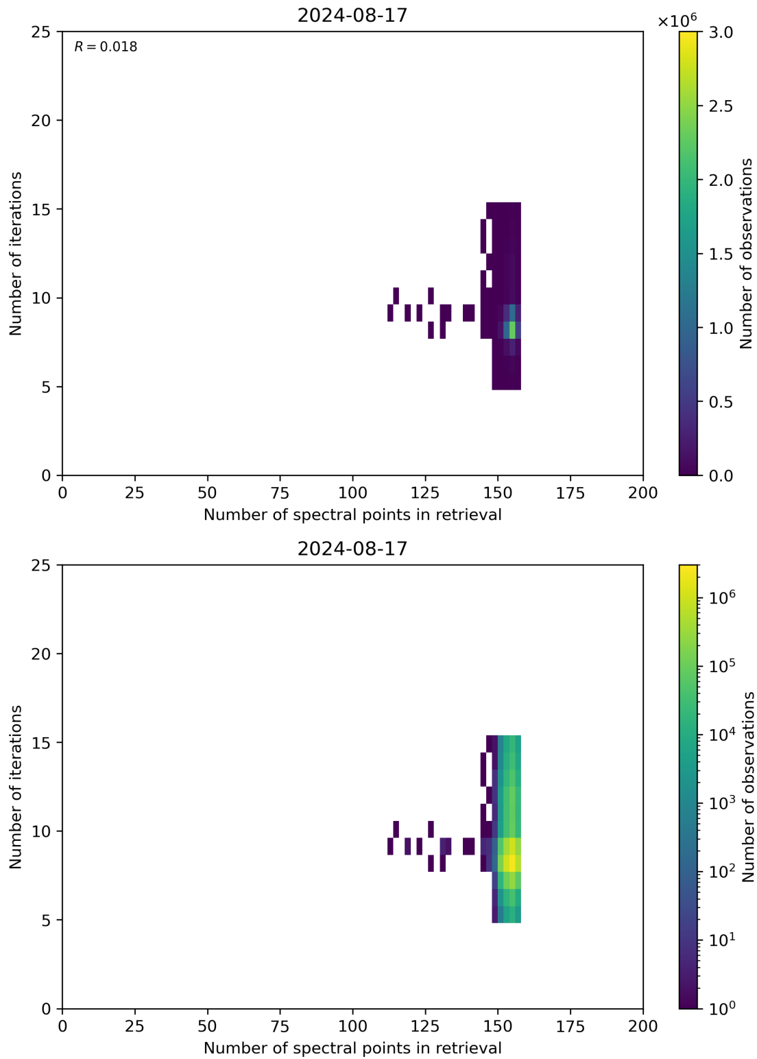
Figure 60: Scatter density plot of “Number of spectral points in retrieval” against “Number of iterations” for 2024-08-16 to 2024-08-18.
