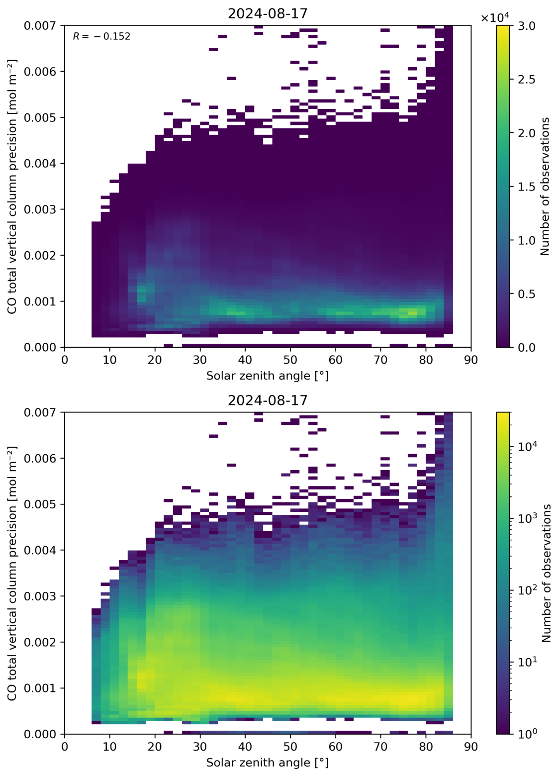
Figure 63: Scatter density plot of “Solar zenith angle” against “CO total vertical column precision” for 2024-08-16 to 2024-08-18.
