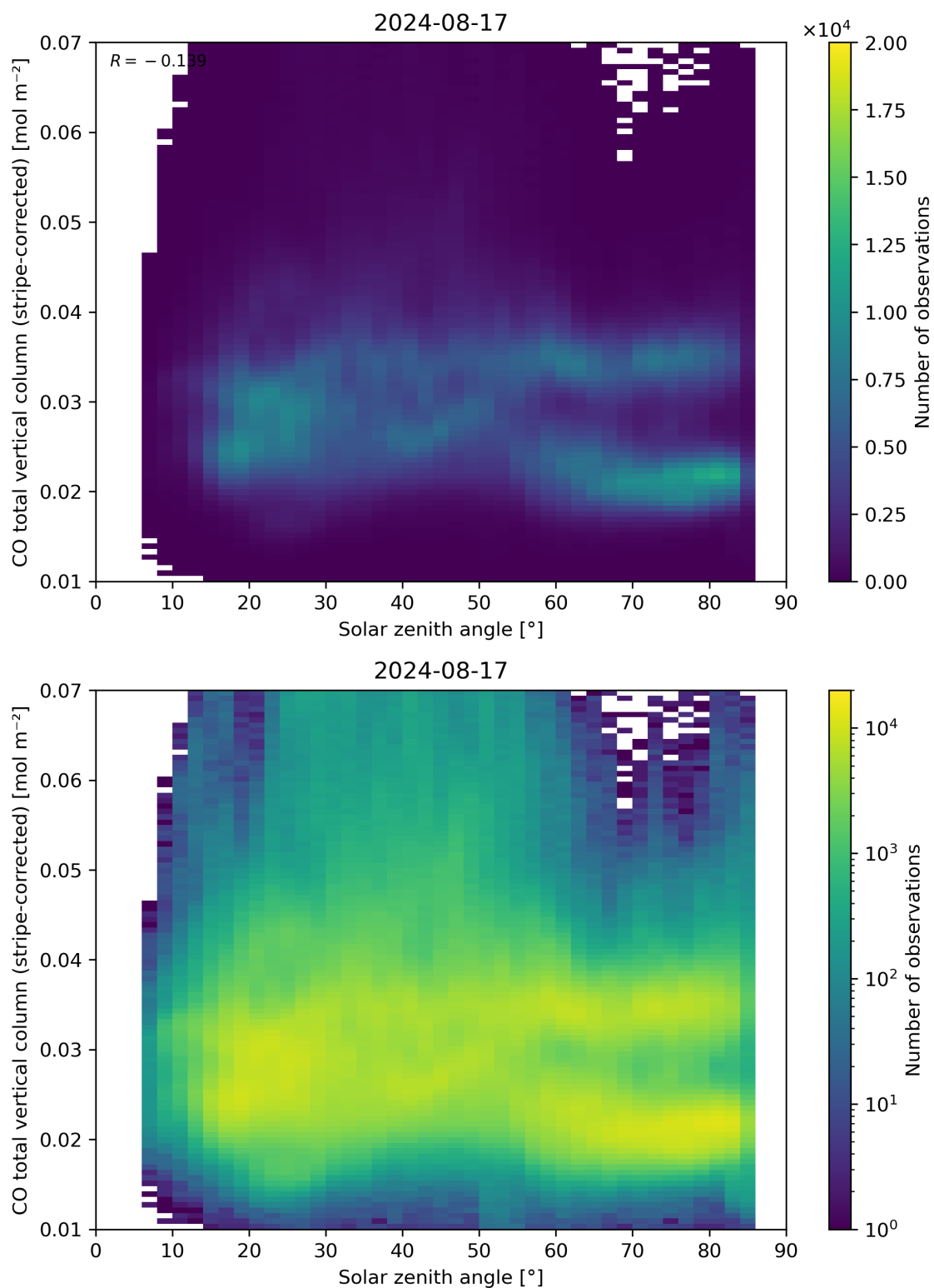
Figure 62: Scatter density plot of “Solar zenith angle” against “CO total vertical column (stripe-corrected)” for 2024-08-16 to 2024-08-18.
