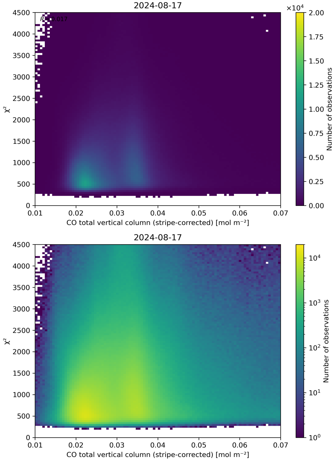
Figure 37: Scatter density plot of “CO total vertical column (stripe-corrected)” against “ \chi^2 ” for 2024-08-16 to 2024-08-18.
