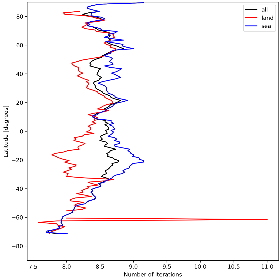
Figure 16: Zonal average of “Number of iterations” for 2024-08-16 to 2024-08-18.
