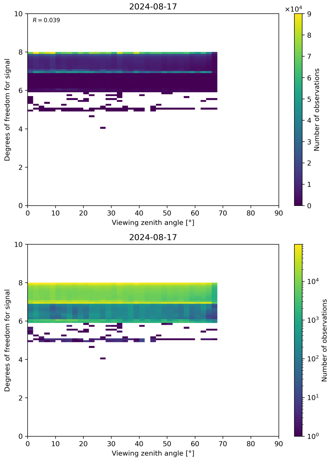
Figure 73: Scatter density plot of “Viewing zenith angle” against “Degrees of freedom for signal” for 2024-08-16 to 2024-08-18.
