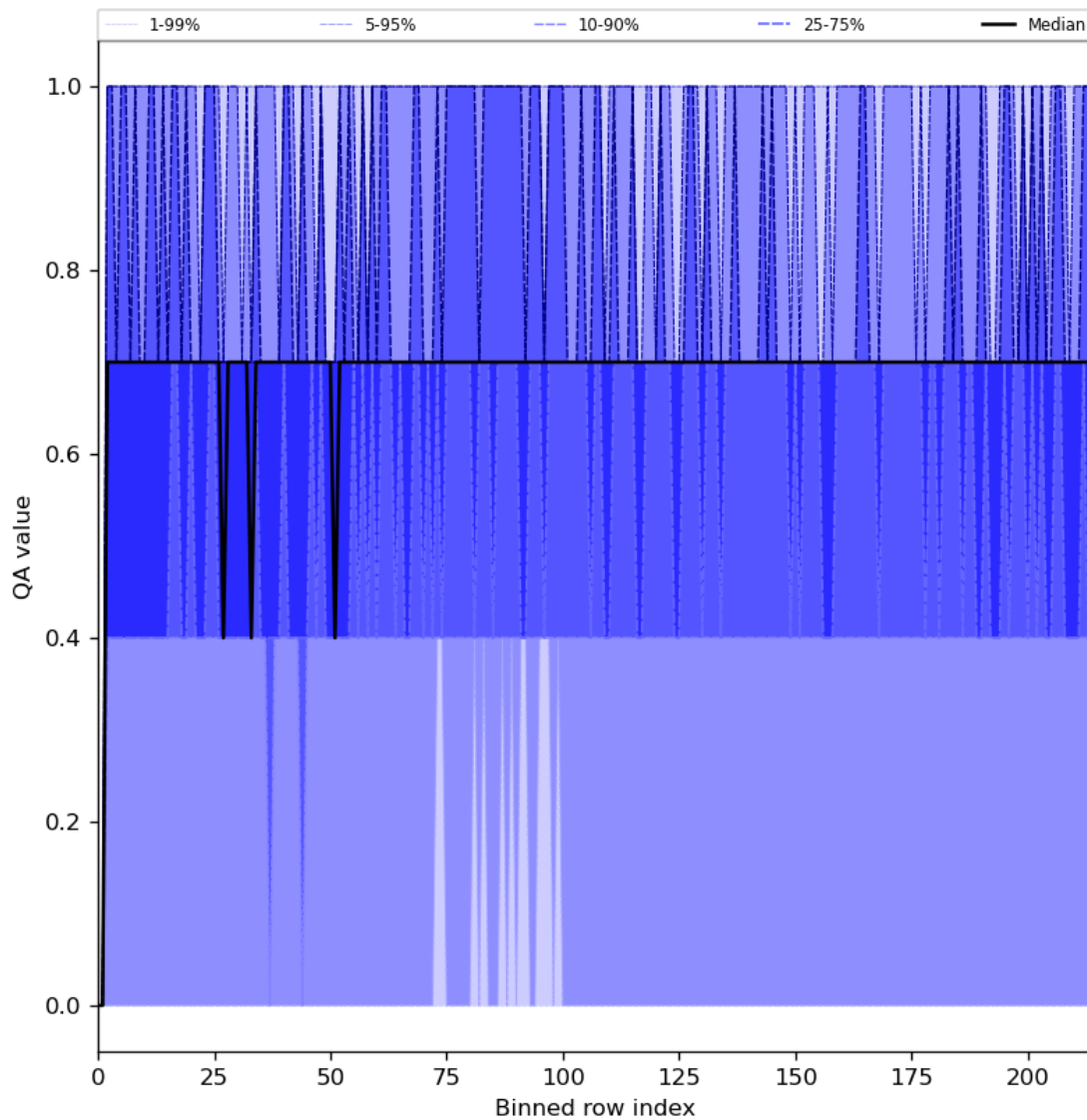
Figure 25: Along track statistics of “QA value” for 2024-08-16 to 2024-08-18
