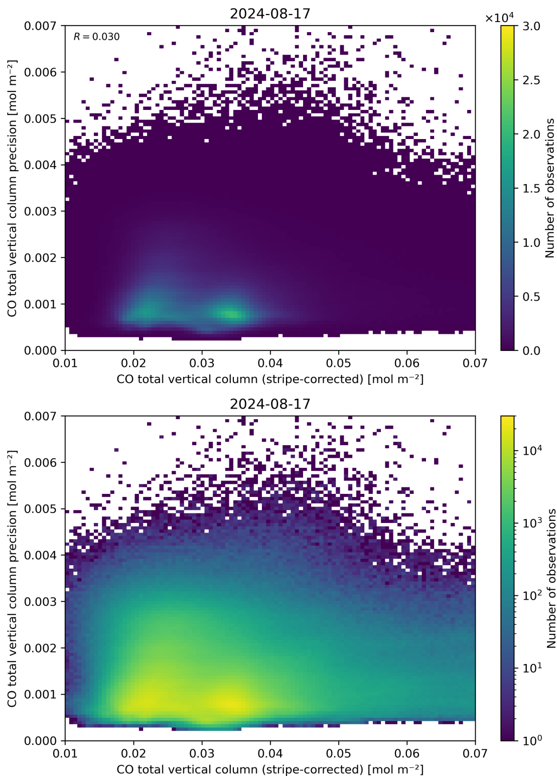
Figure 36: Scatter density plot of “CO total vertical column (stripe-corrected)” against “CO total vertical column precision” for 2024-08-16 to 2024-08-18.
