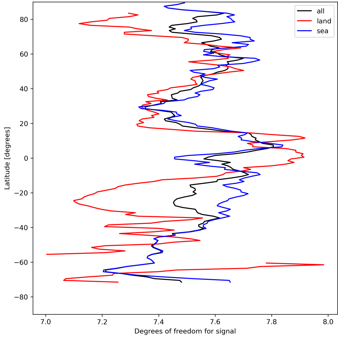
Figure 15: Zonal average of “Degrees of freedom for signal” for 2024-08-16 to 2024-08-18.
