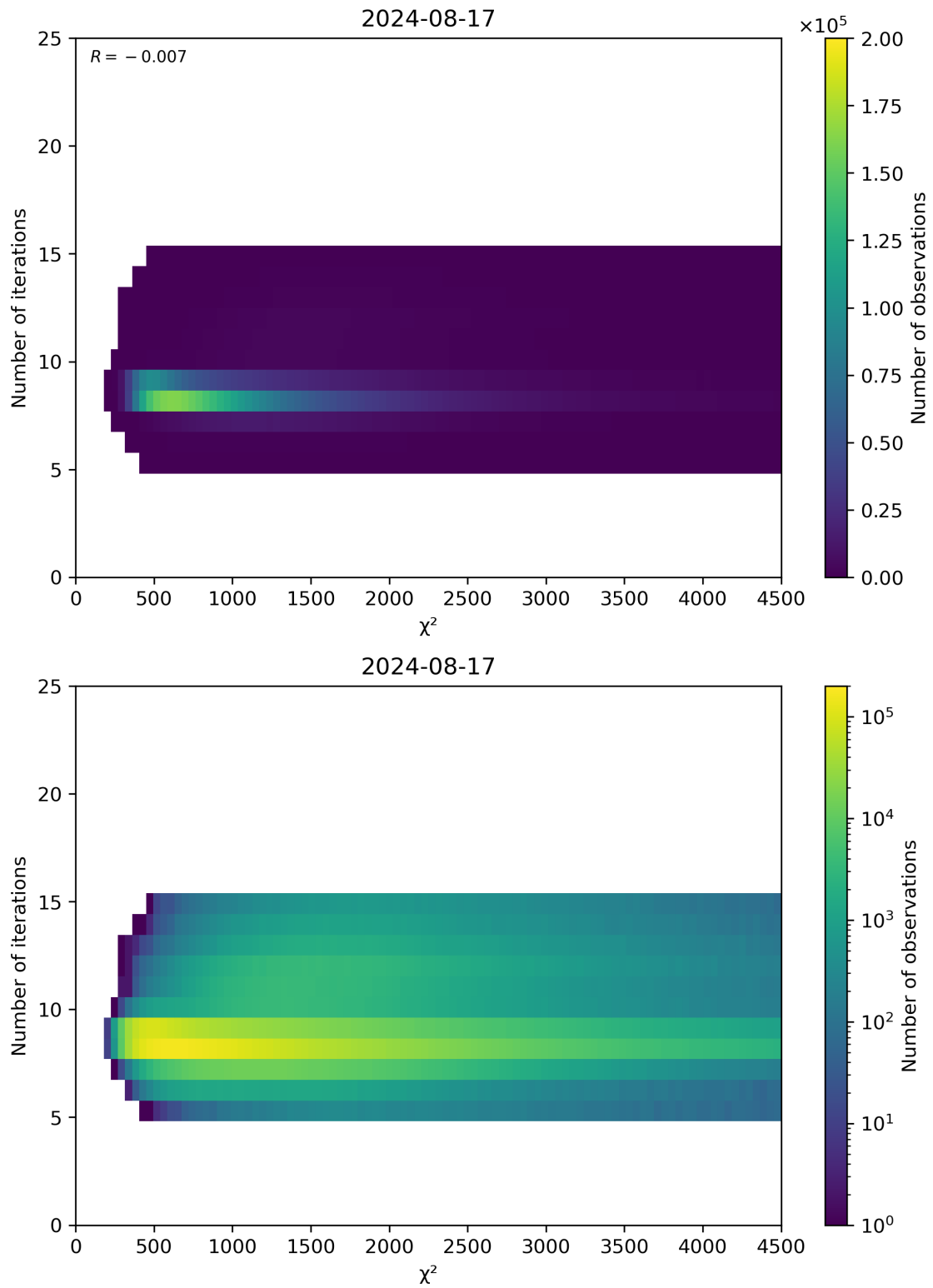
Figure 49: Scatter density plot of “ \chi^2 ” against “Number of iterations” for 2024-08-16 to 2024-08-18.
