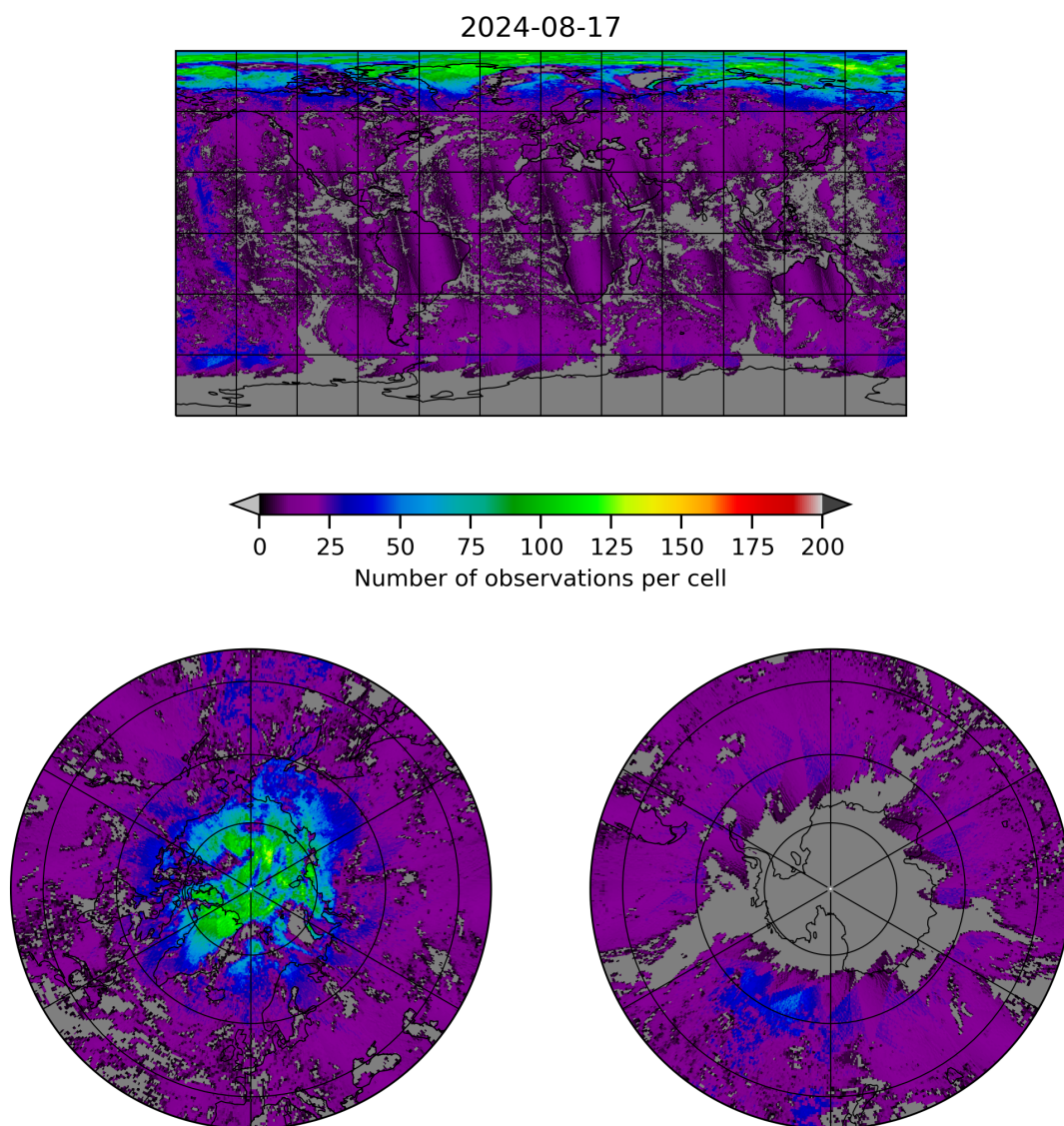
Figure 8: Map of the number of observations for 2024-08-16 to 2024-08-18
