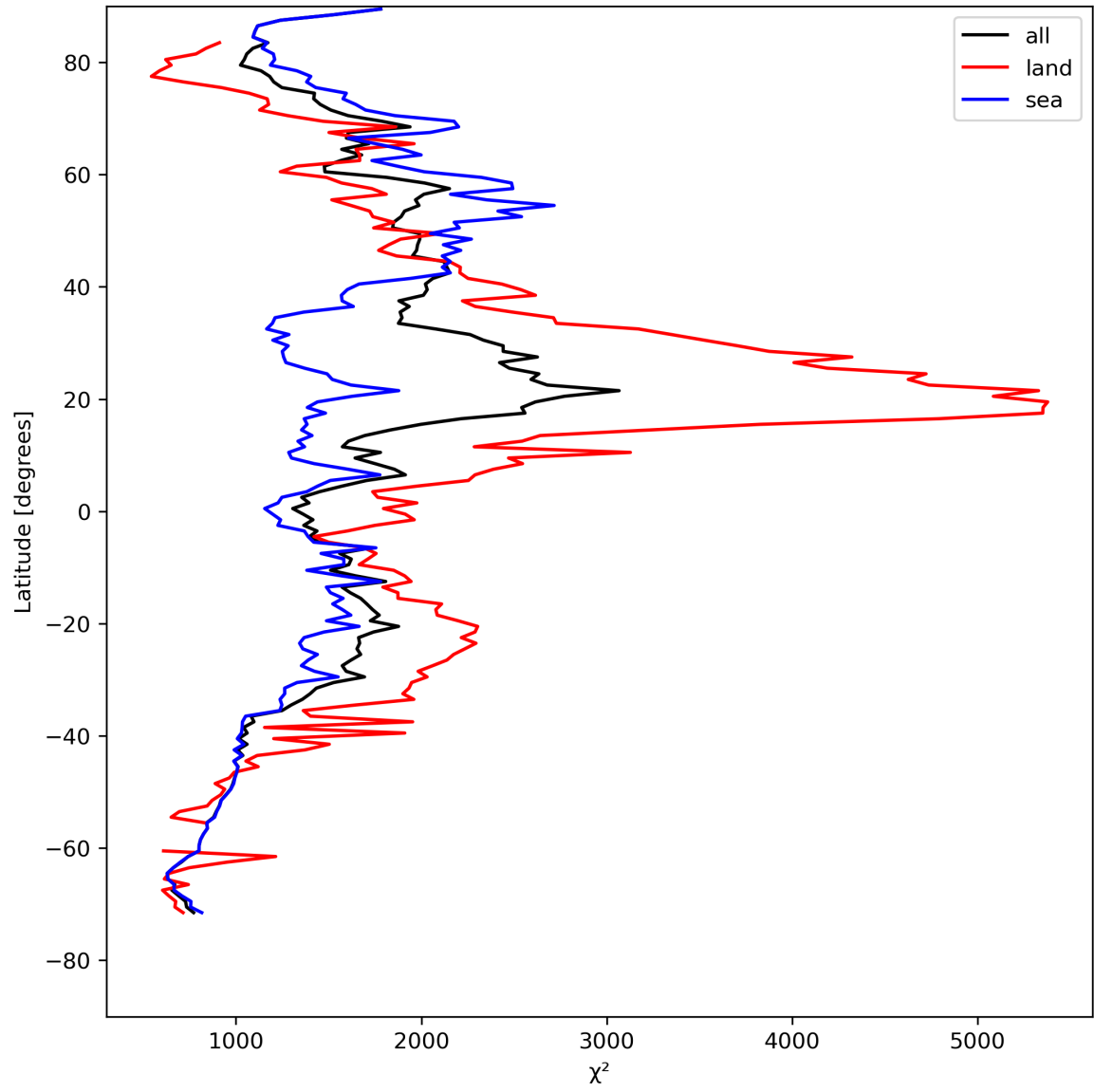
Figure 14: Zonal average of “ \chi^2 ” for 2024-08-16 to 2024-08-18.
