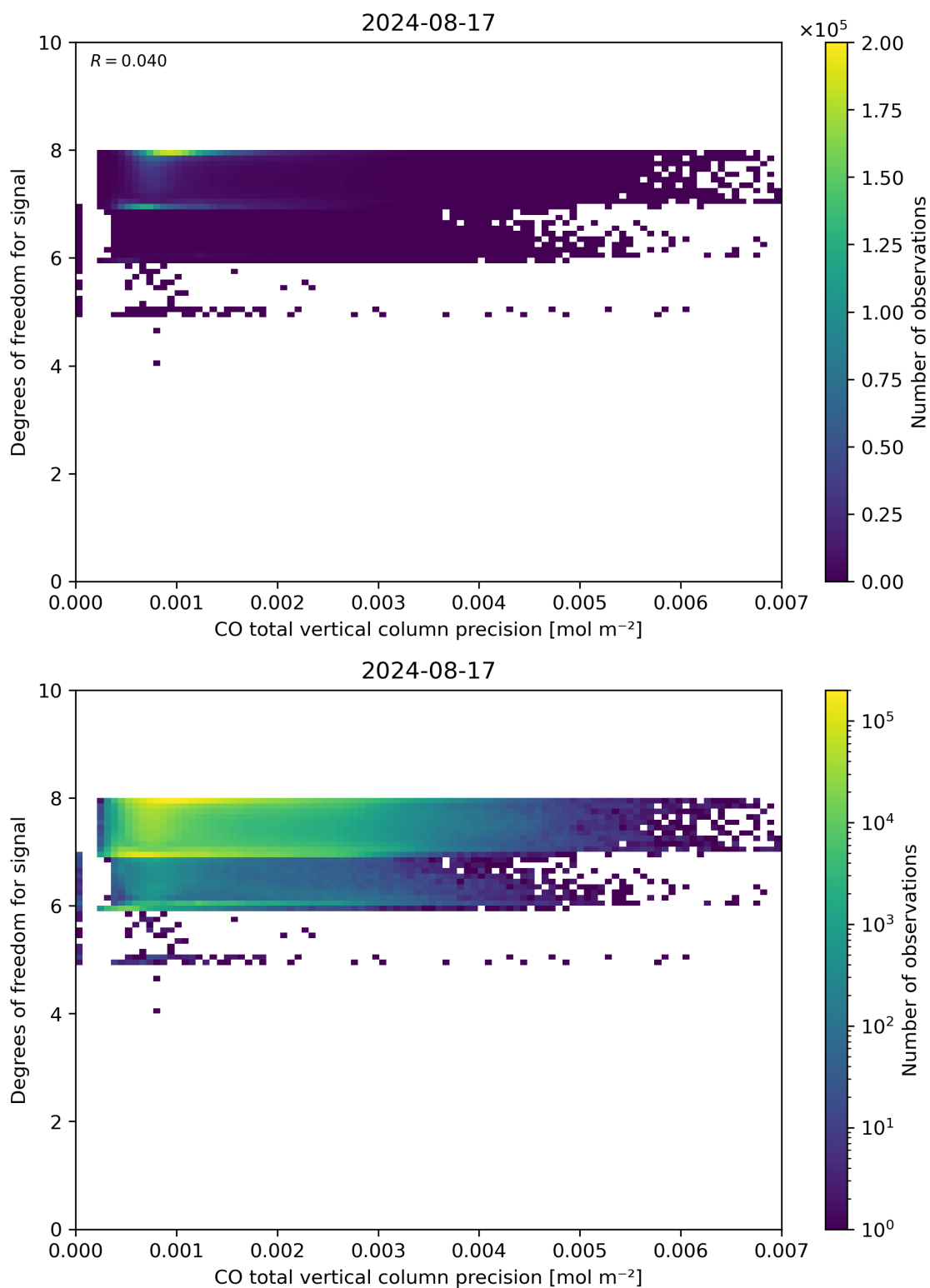
Figure 45: Scatter density plot of “CO total vertical column precision” against “Degrees of freedom for signal” for 2024-08-16 to 2024-08-18.
