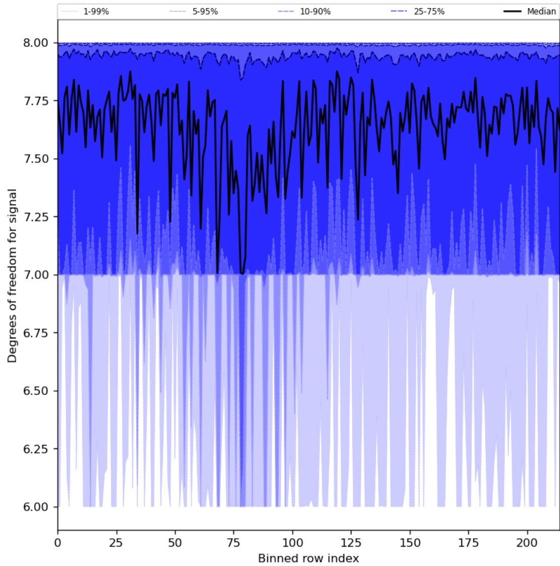
Figure 31: Along track statistics of “Degrees of freedom for signal” for 2024-08-16 to 2024-08-18
