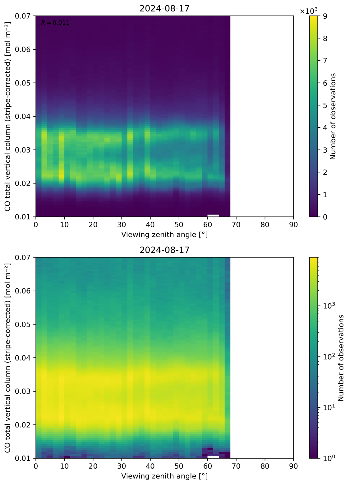
Figure 70: Scatter density plot of “Viewing zenith angle” against “CO total vertical column (stripe-corrected)” for 2024-08-16 to 2024-08-18.
