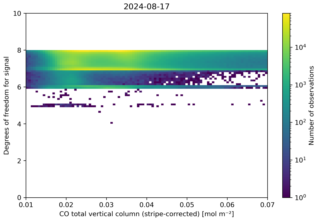
Figure 38: Scatter density plot of “CO total vertical column (stripe-corrected)” against “Degrees of freedom for signal” for 2024-08-16 to 2024-08-18.
