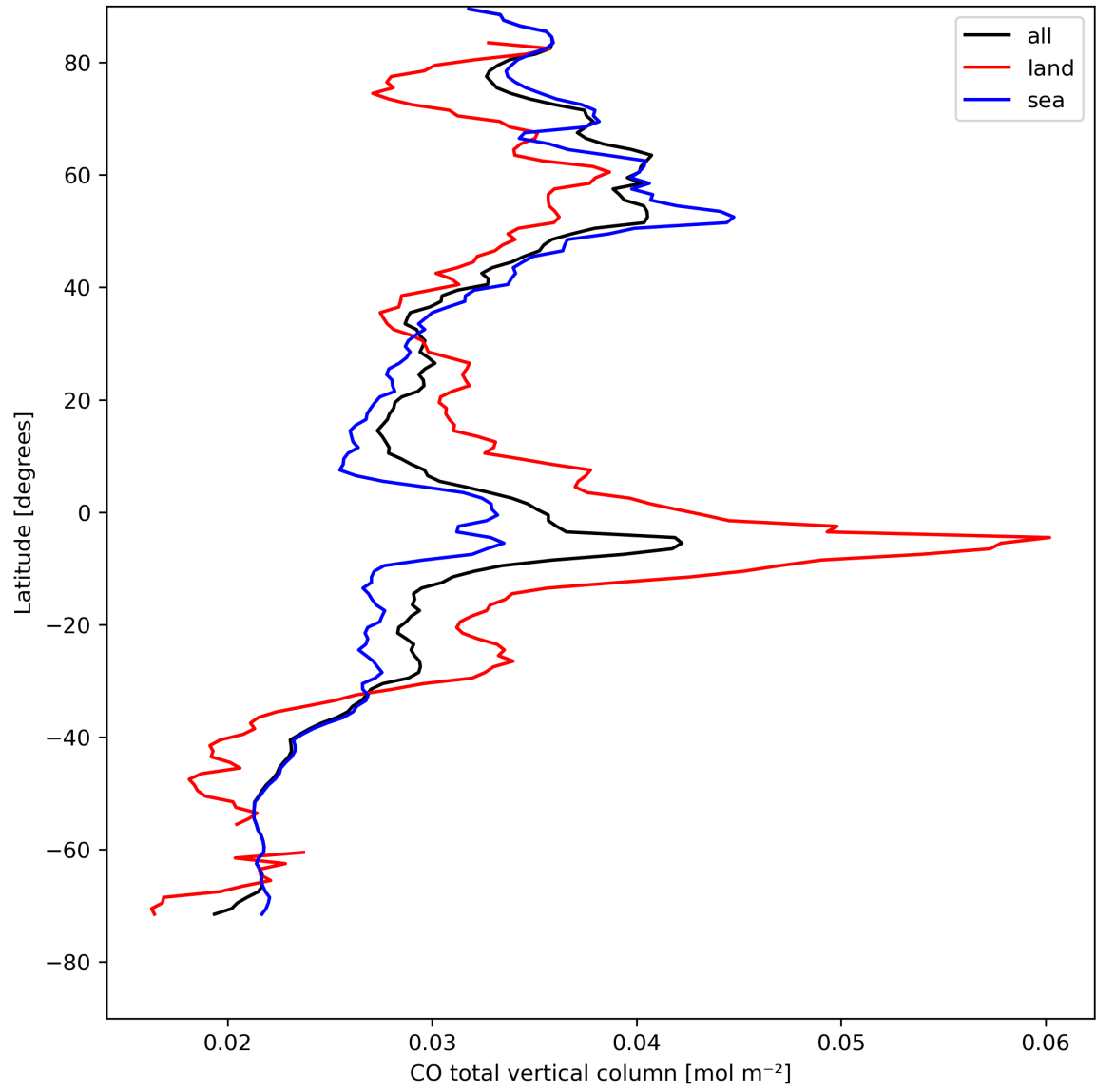
Figure 10: Zonal average of “CO total vertical column” for 2024-08-16 to 2024-08-18.
