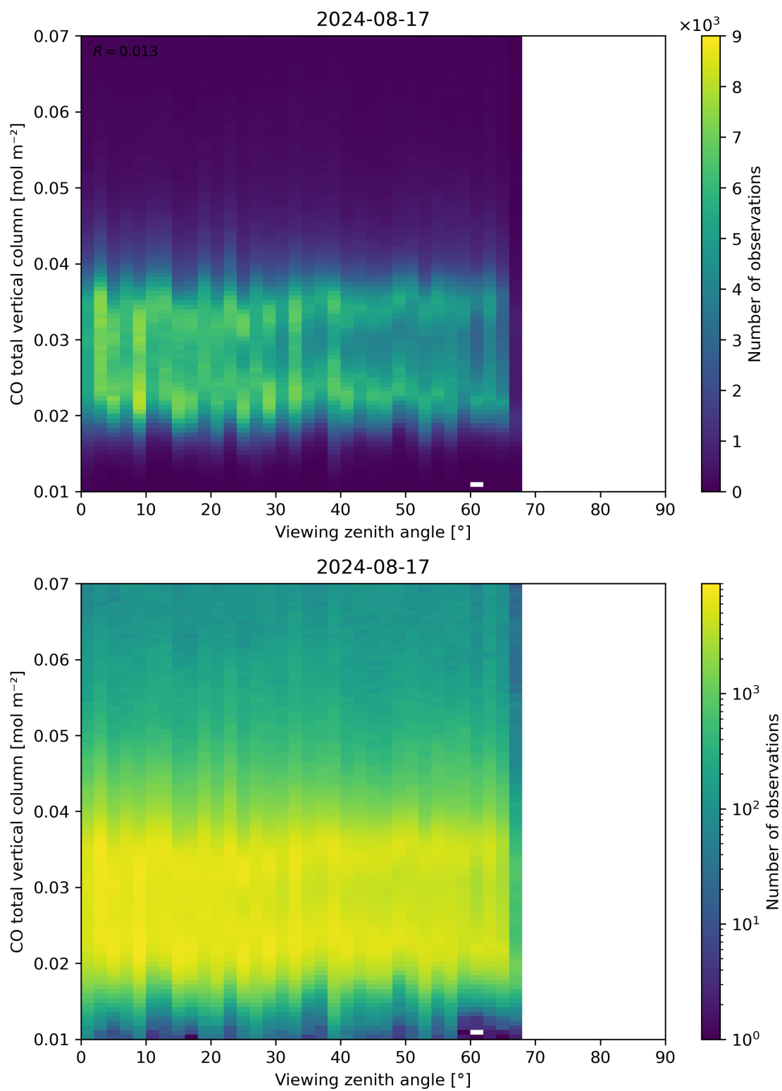
Figure 69: Scatter density plot of “Viewing zenith angle” against “CO total vertical column” for 2024-08-16 to 2024-08-18.
