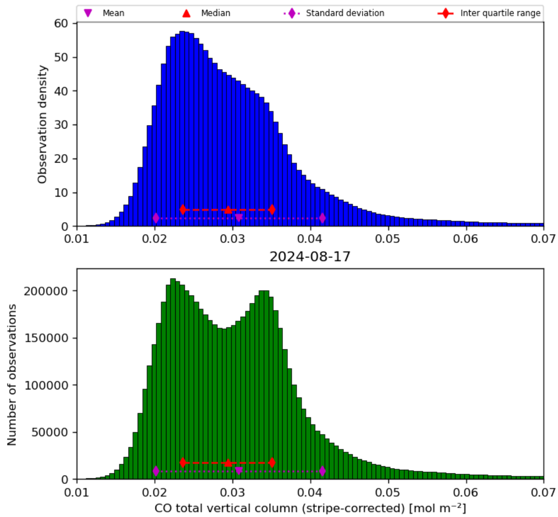
Figure 19: Histogram of “CO total vertical column (stripe-corrected)” for 2024-08-16 to 2024-08-18
