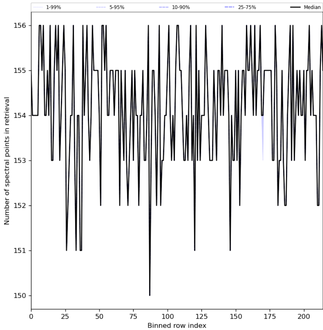
Figure 29: Along track statistics of “Number of spectral points in retrieval” for 2024-08-16 to 2024-08-18
