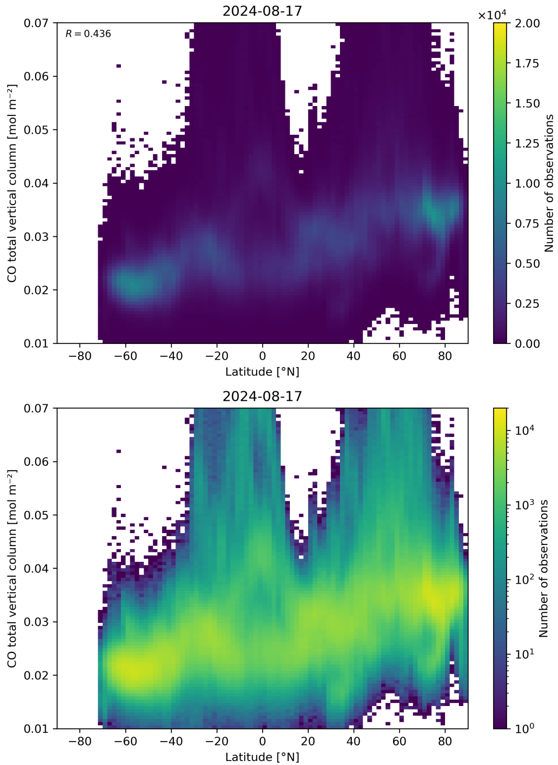
Figure 51: Scatter density plot of “Latitude” against “CO total vertical column” for 2024-08-16 to 2024-08-18.
