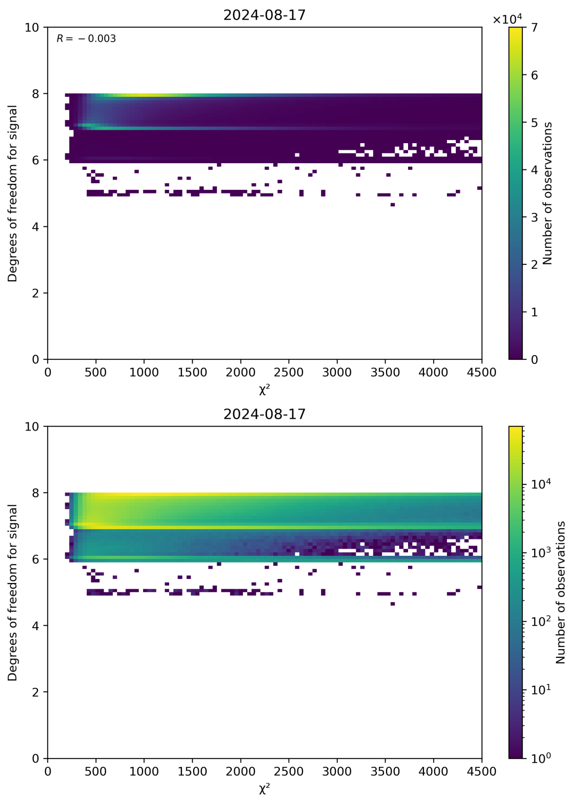
Figure 48: Scatter density plot of “ \chi^2 ” against “Degrees of freedom for signal” for 2024-08-16 to 2024-08-18.
