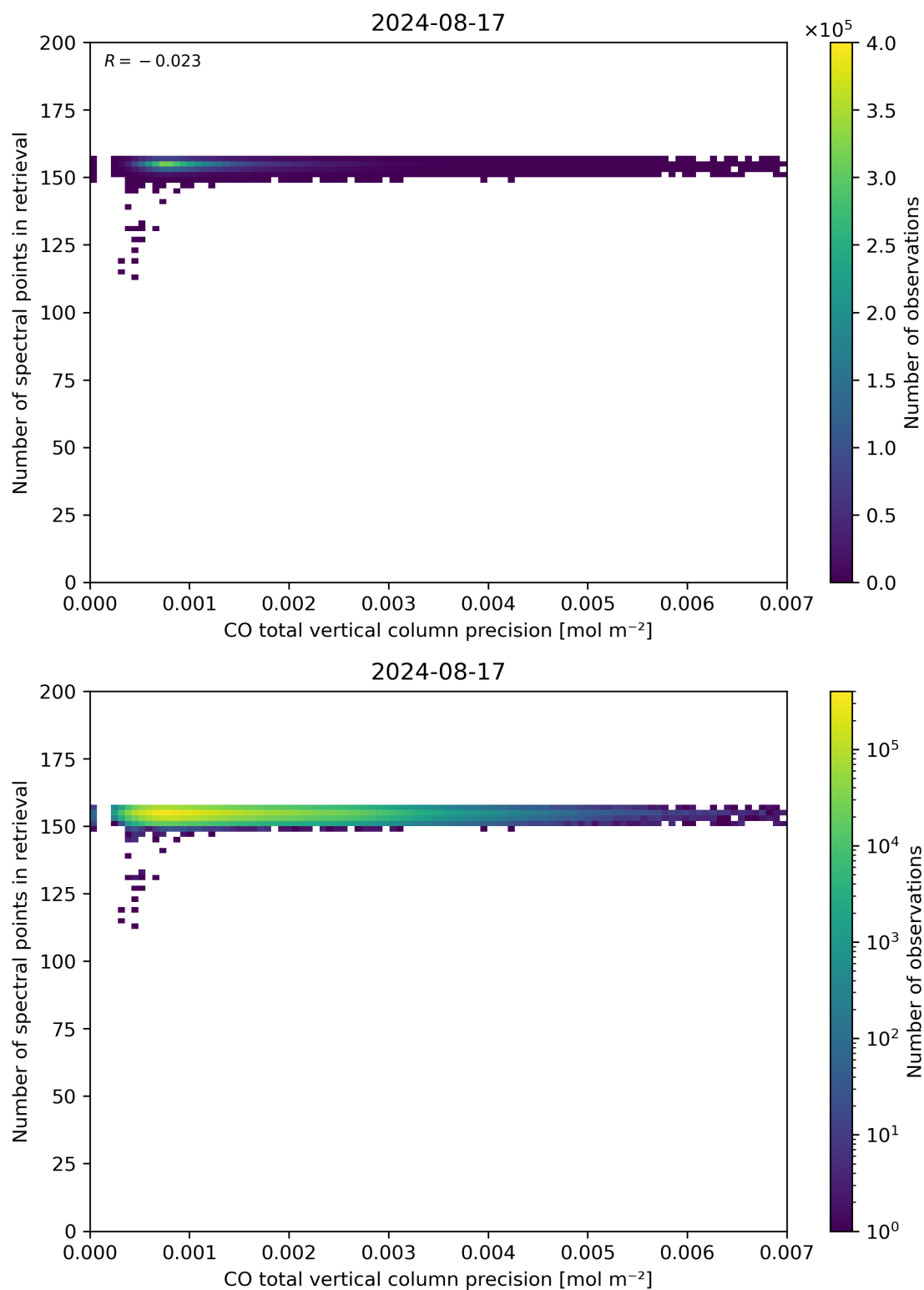
Figure 47: Scatter density plot of “CO total vertical column precision” against “Number of spectral points in retrieval” for 2024-08-16 to 2024-08-18.
