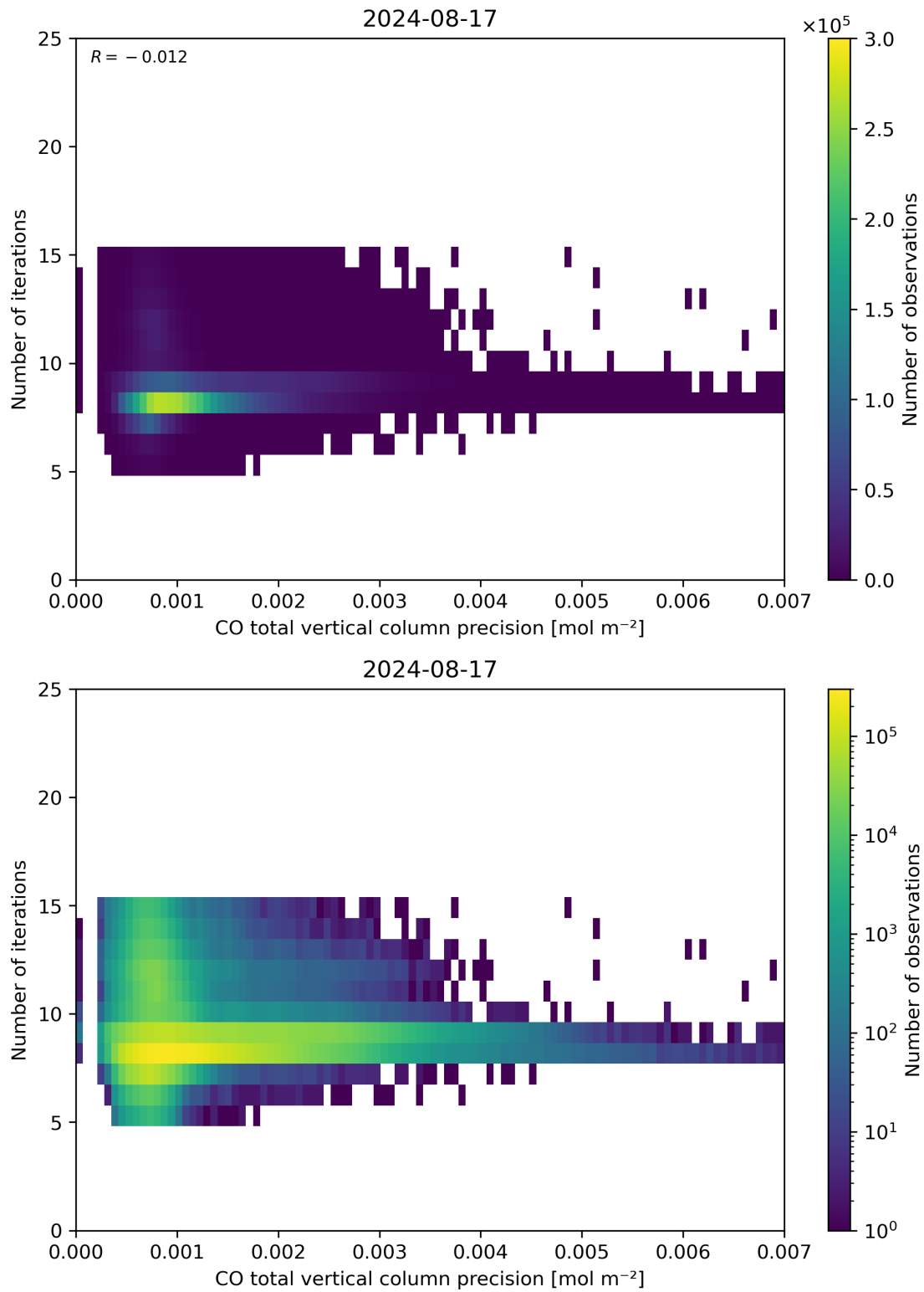
Figure 46: Scatter density plot of “CO total vertical column precision” against “Number of iterations” for 2024-08-16 to 2024-08-18.
