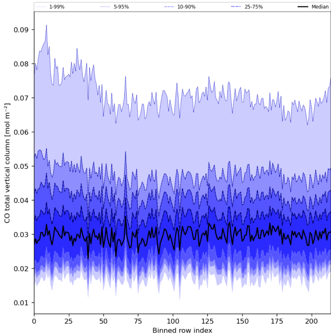
Figure 26: Along track statistics of “CO total vertical column” for 2024-08-16 to 2024-08-18
