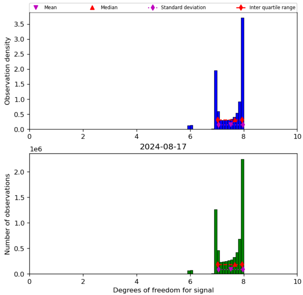
Figure 23: Histogram of “Degrees of freedom for signal” for 2024-08-16 to 2024-08-18
