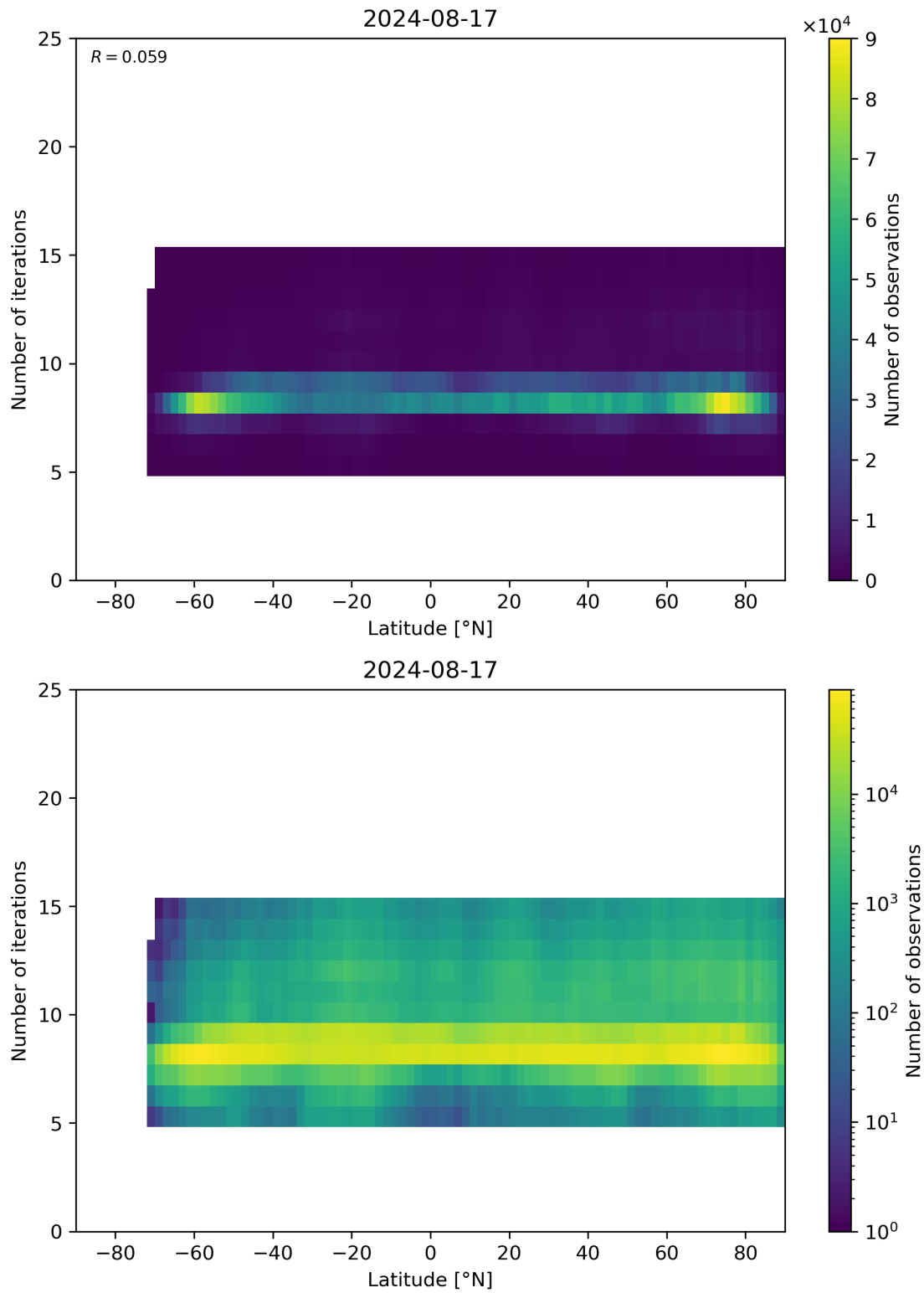
Figure 56: Scatter density plot of “Latitude” against “Number of iterations” for 2024-08-16 to 2024-08-18.
