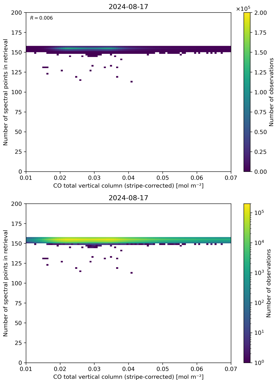
Figure 40: Scatter density plot of “CO total vertical column (stripe-corrected)” against “Number of spectral points in retrieval” for 2024-08-16 to 2024-08-18.
