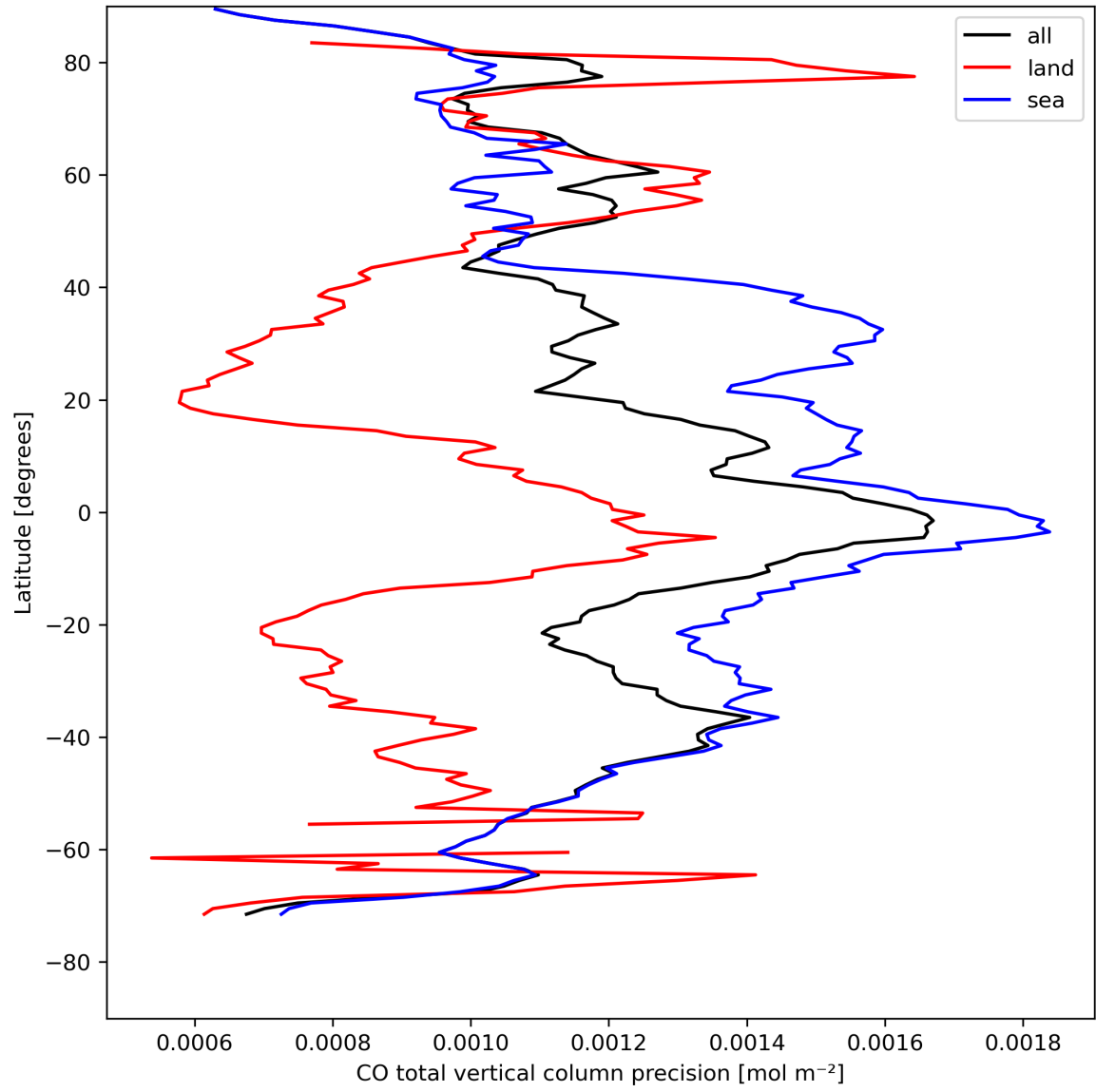
Figure 12: Zonal average of “CO total vertical column precision” for 2024-08-16 to 2024-08-18.
