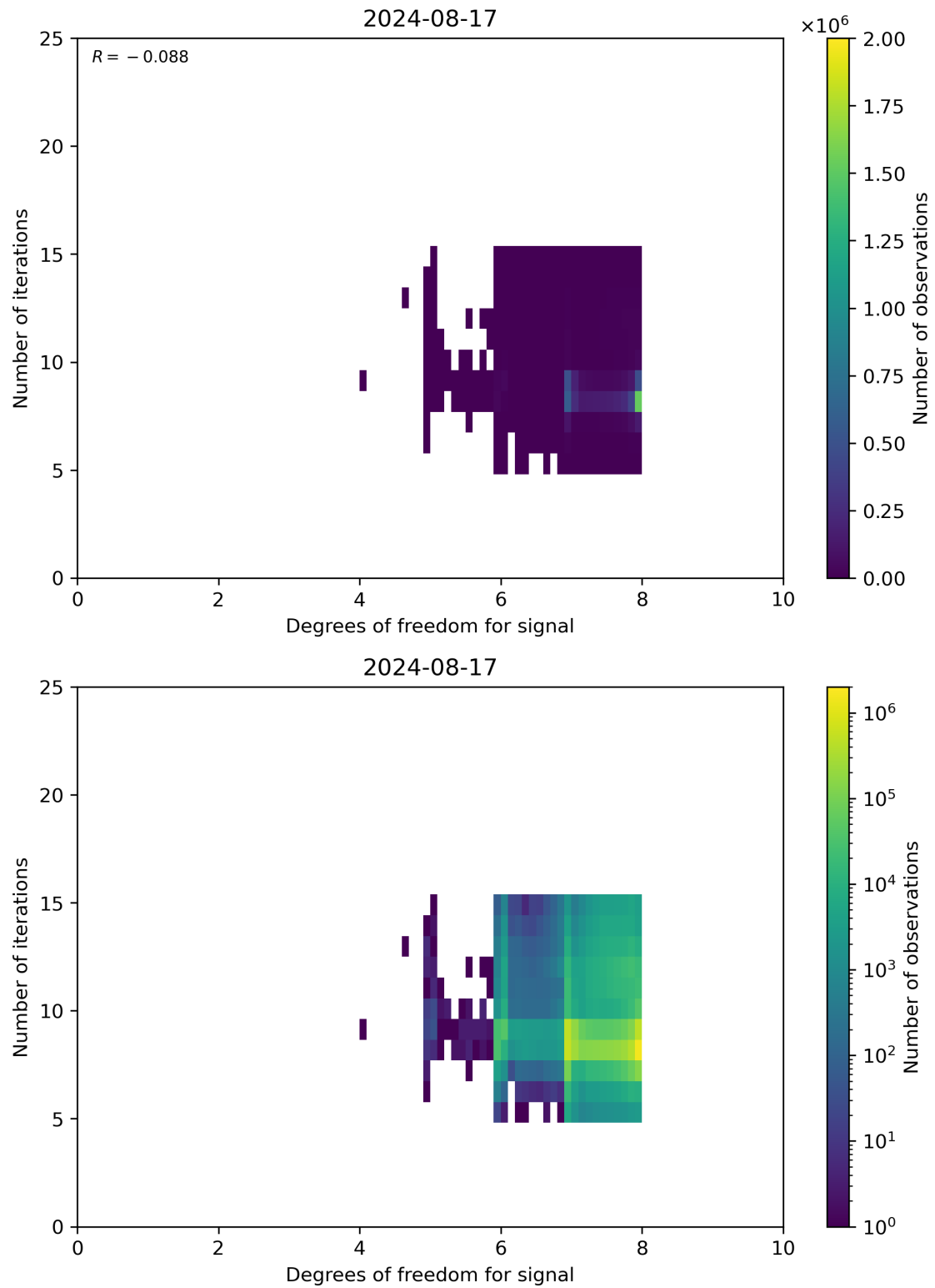
Figure 50: Scatter density plot of “Degrees of freedom for signal” against “Number of iterations” for 2024-08-16 to 2024-08-18.
