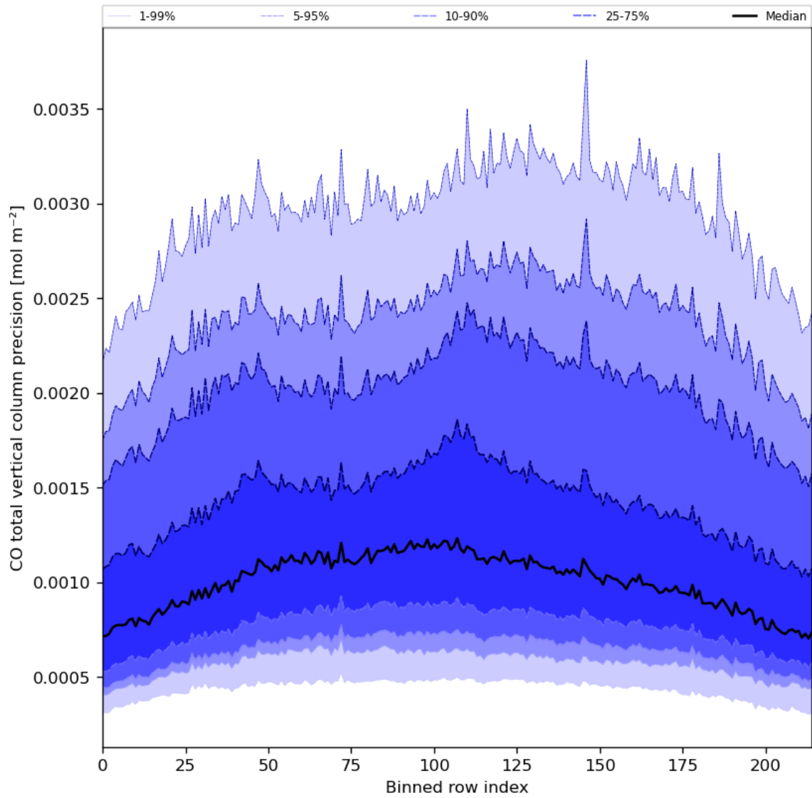
Figure 28: Along track statistics of “CO total vertical column precision” for 2024-08-16 to 2024-08-18
