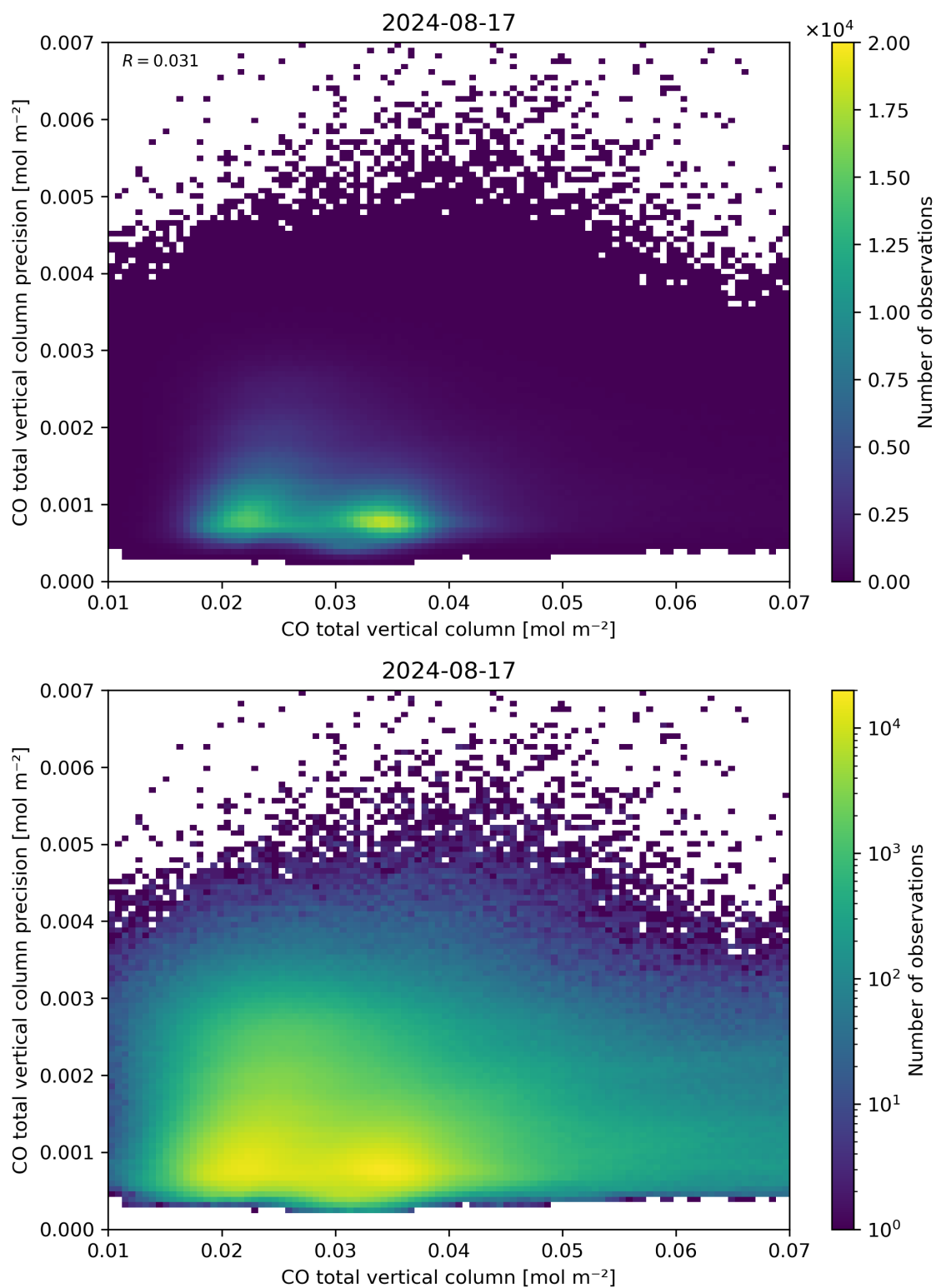
Figure 34: Scatter density plot of “CO total vertical column” against “CO total vertical column precision” for 2024-08-16 to 2024-08-18.
