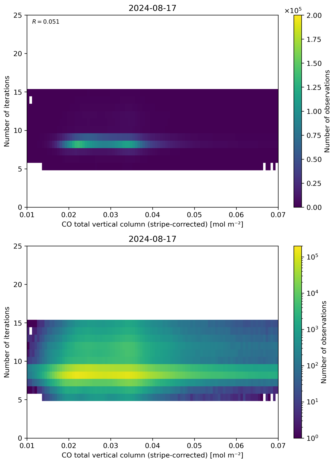
Figure 39: Scatter density plot of “CO total vertical column (stripe-corrected)” against “Number of iterations” for 2024-08-16 to 2024-08-18.
