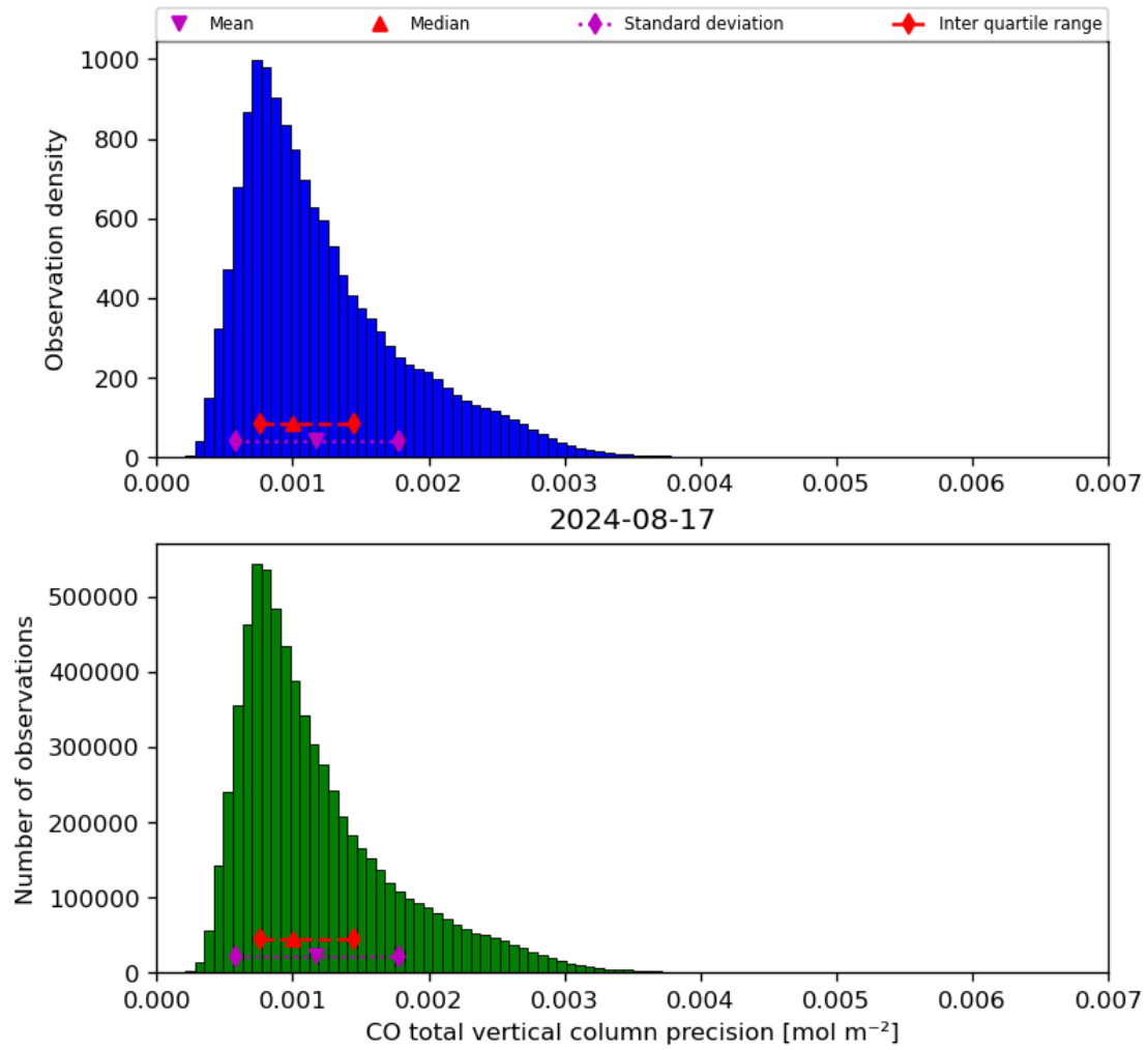
Figure 20: Histogram of “CO total vertical column precision” for 2024-08-16 to 2024-08-18
