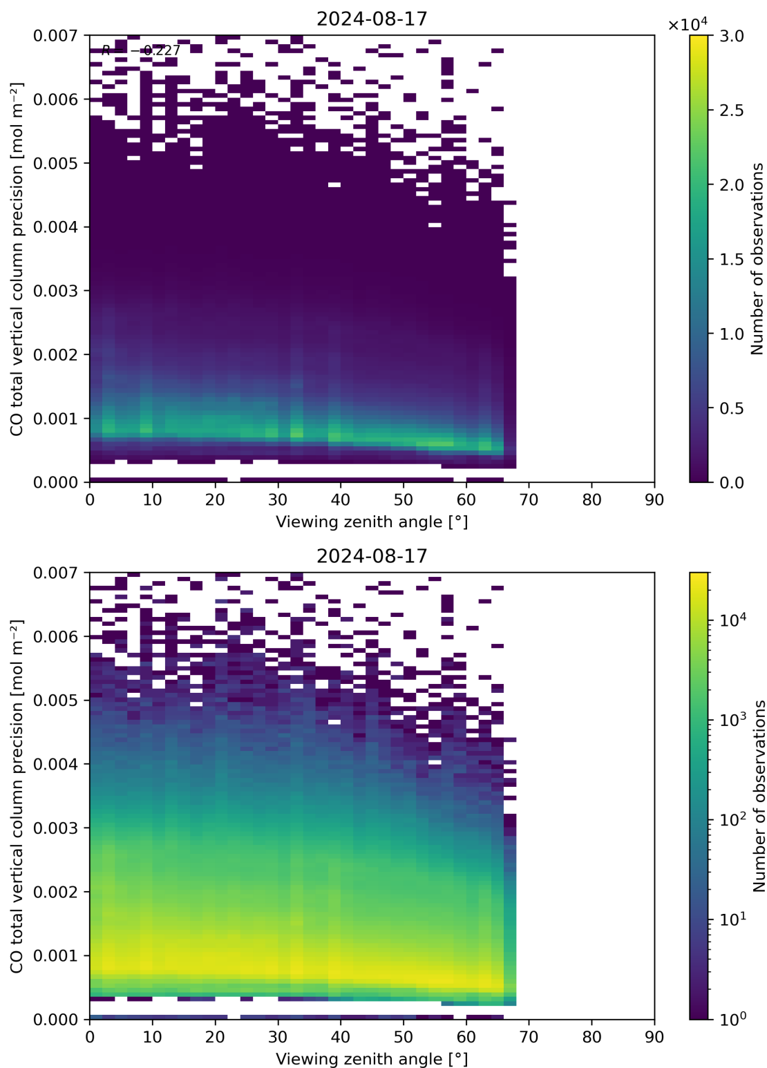
Figure 71: Scatter density plot of “Viewing zenith angle” against “CO total vertical column precision” for 2024-08-16 to 2024-08-18.
