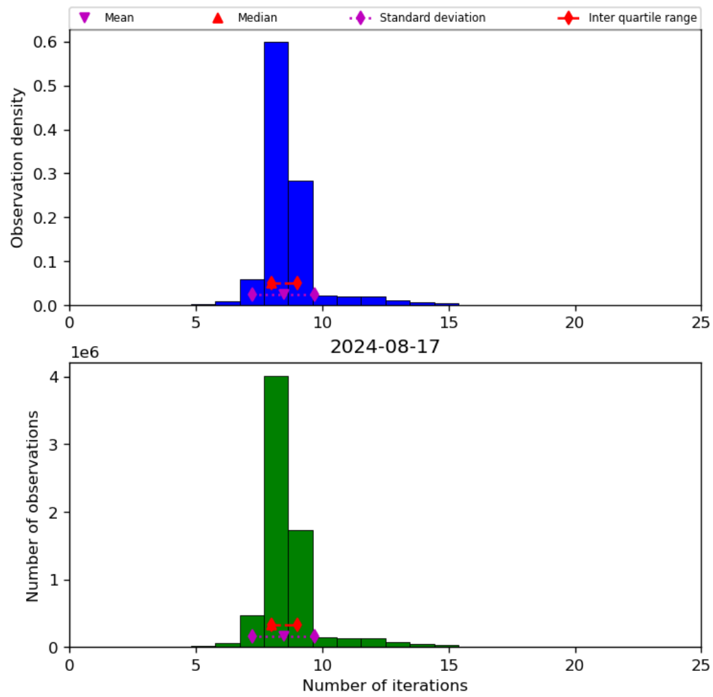
Figure 24: Histogram of “Number of iterations” for 2024-08-16 to 2024-08-18
