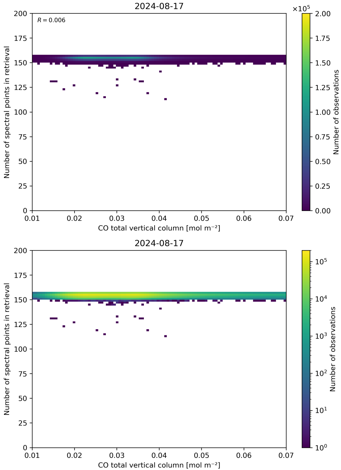
Figure 43: Scatter density plot of “CO total vertical column” against “Number of spectral points in retrieval” for 2024-08-16 to 2024-08-18.
