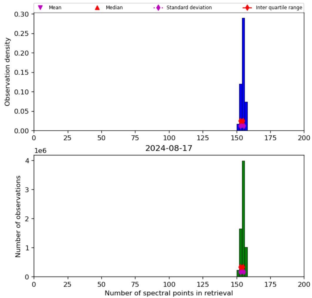
Figure 21: Histogram of “Number of spectral points in retrieval” for 2024-08-16 to 2024-08-18
