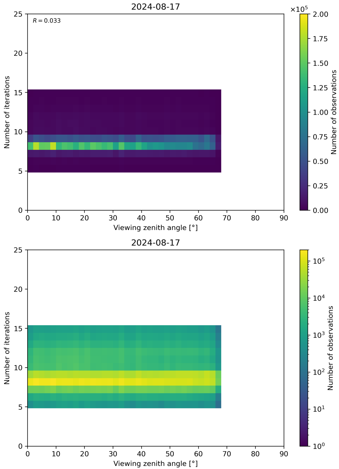
Figure 75: Scatter density plot of “Viewing zenith angle” against “Number of iterations” for 2024-08-16 to 2024-08-18.
