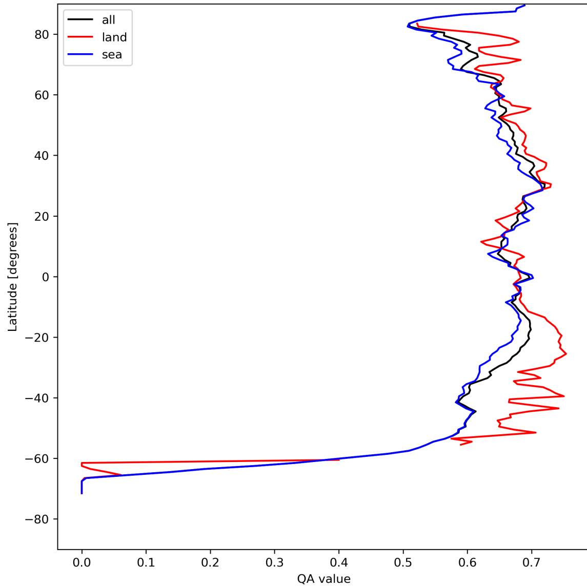
Figure 9: Zonal average of “QA value” for 2024-08-16 to 2024-08-18.
