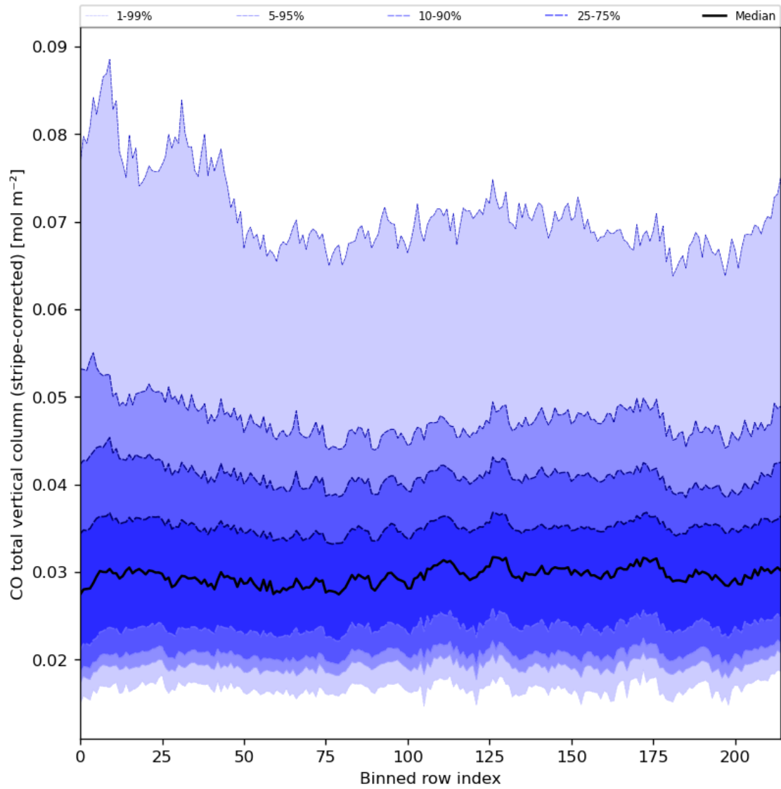
Figure 27: Along track statistics of “CO total vertical column (stripe-corrected)” for 2024-08-16 to 2024-08-18
