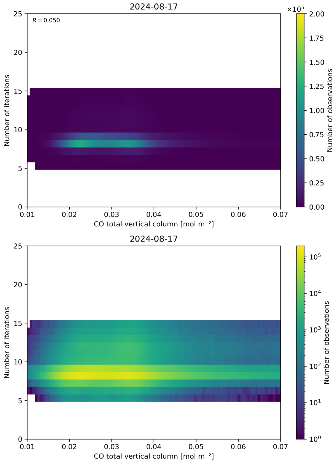
Figure 42: Scatter density plot of “CO total vertical column” against “Number of iterations” for 2024-08-16 to 2024-08-18.
