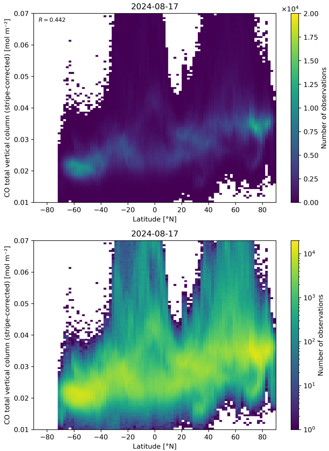
Figure 52: Scatter density plot of “Latitude” against “CO total vertical column (stripe-corrected)” for 2024-08-16 to 2024-08-18.
