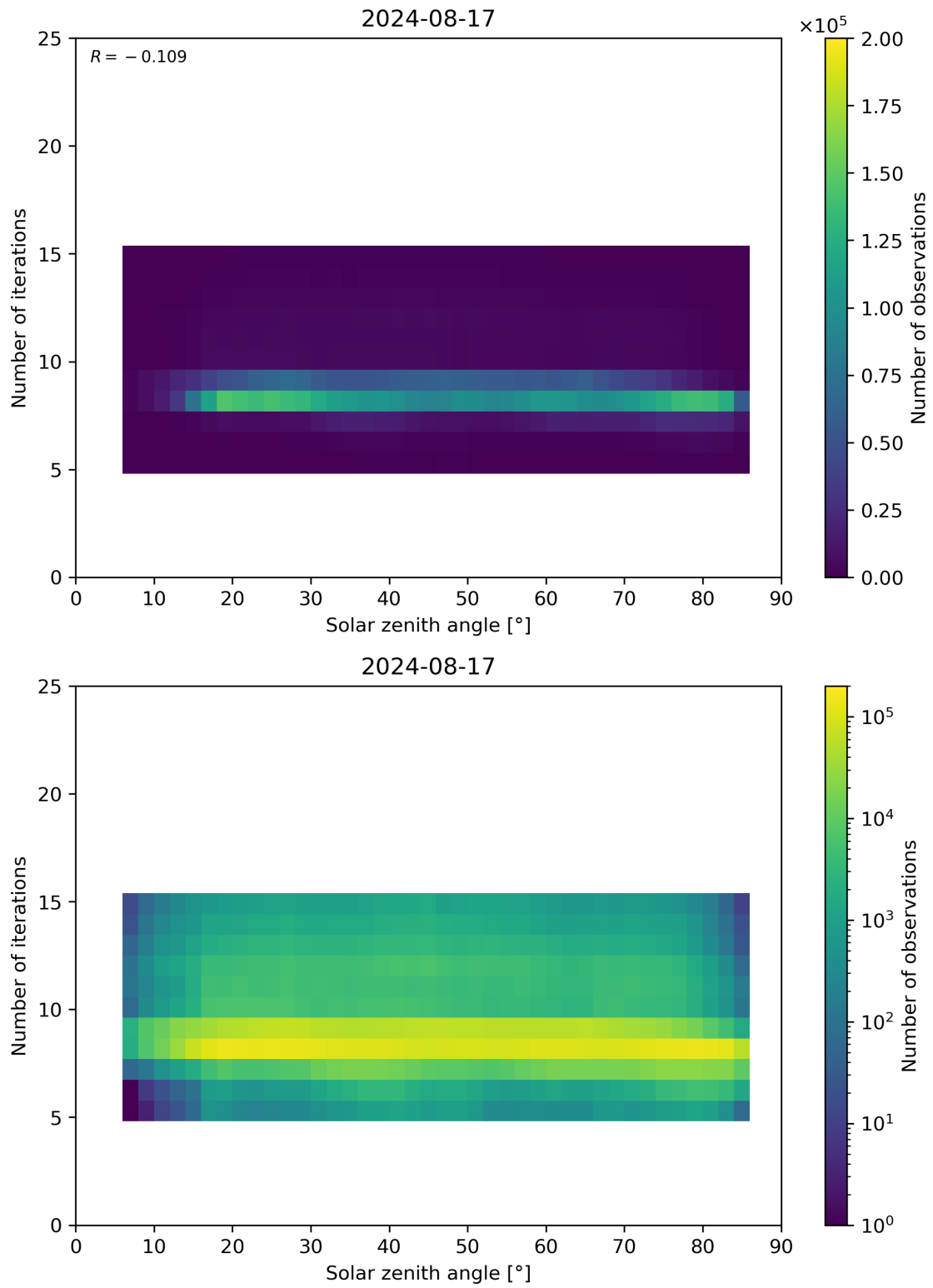
Figure 67: Scatter density plot of “Solar zenith angle” against “Number of iterations” for 2024-08-16 to 2024-08-18.
