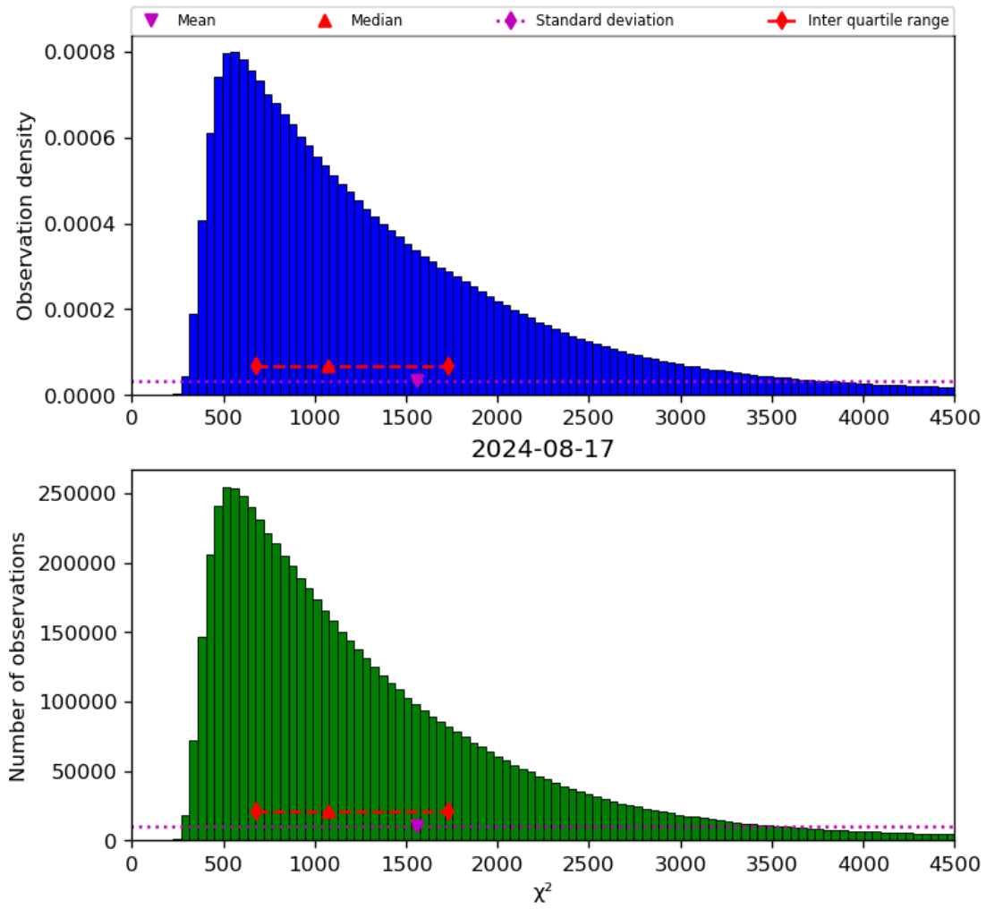
Figure 22: Histogram of “ \chi^2 ” for 2024-08-16 to 2024-08-18
