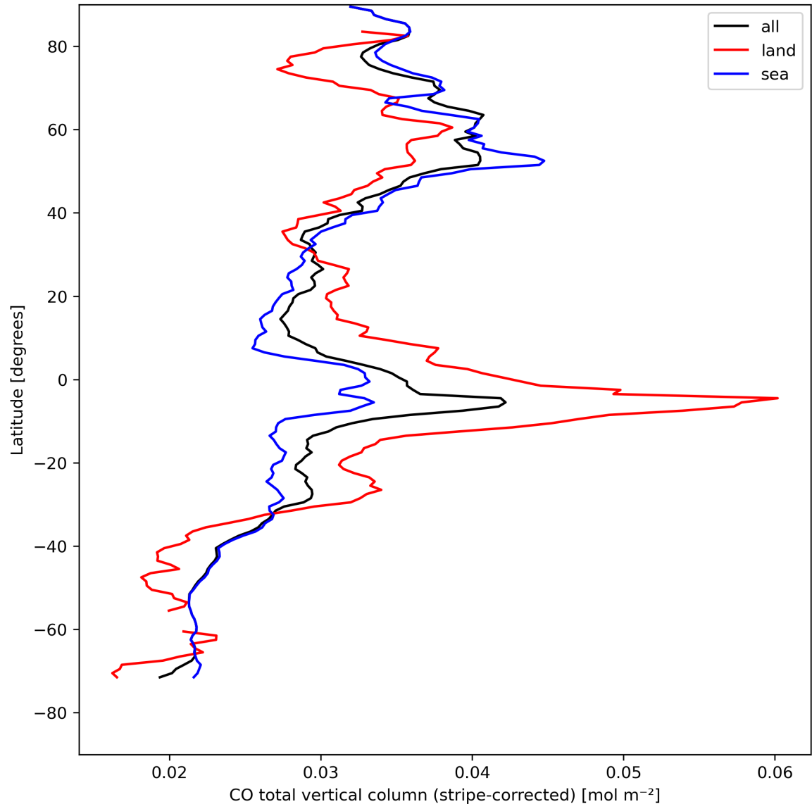
Figure 11: Zonal average of “CO total vertical column (stripe-corrected)” for 2024-08-16 to 2024-08-18.
