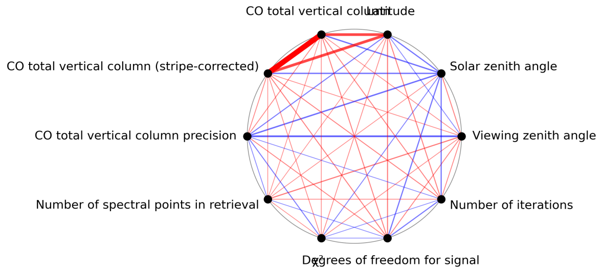
Figure 1: Map of correlation graph for 2024-08-16 to 2024-08-18.
