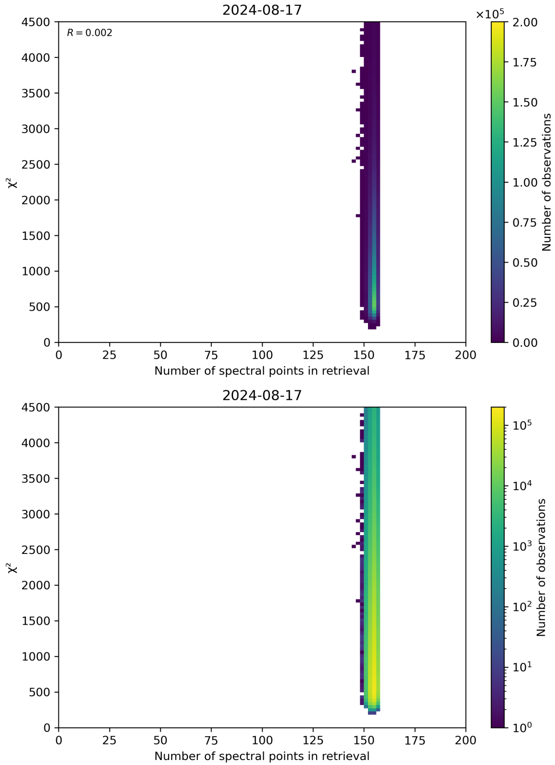
Figure 58: Scatter density plot of “Number of spectral points in retrieval” against “ \chi^2 ” for 2024-08-16 to 2024-08-18.
