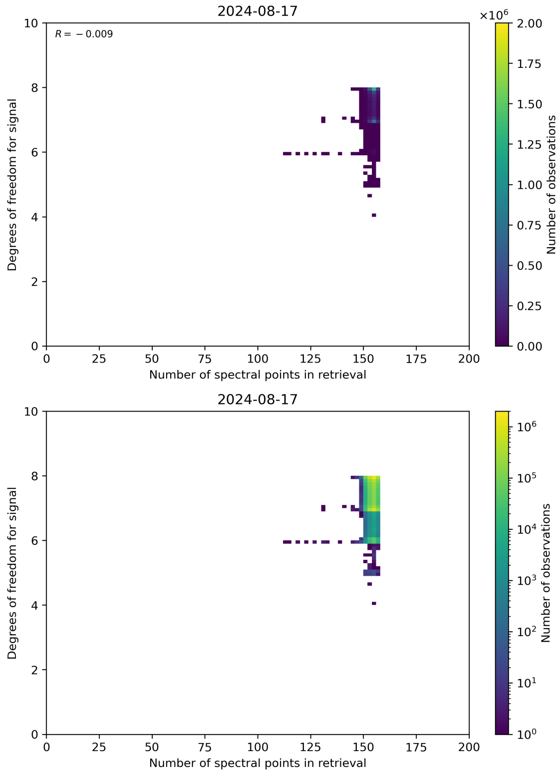
Figure 59: Scatter density plot of “Number of spectral points in retrieval” against “Degrees of freedom for signal” for 2024-08-16 to 2024-08-18.
