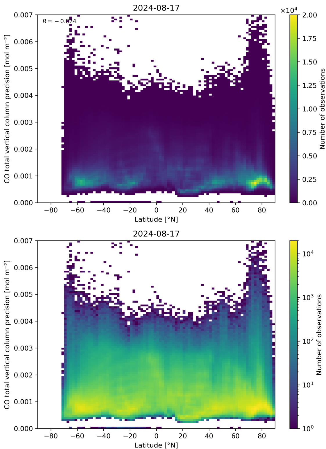
Figure 53: Scatter density plot of “Latitude” against “CO total vertical column precision” for 2024-08-16 to 2024-08-18.
