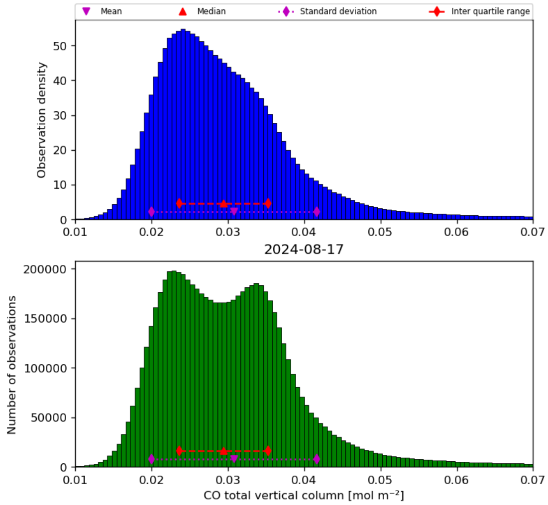
Figure 18: Histogram of “CO total vertical column” for 2024-08-16 to 2024-08-18
