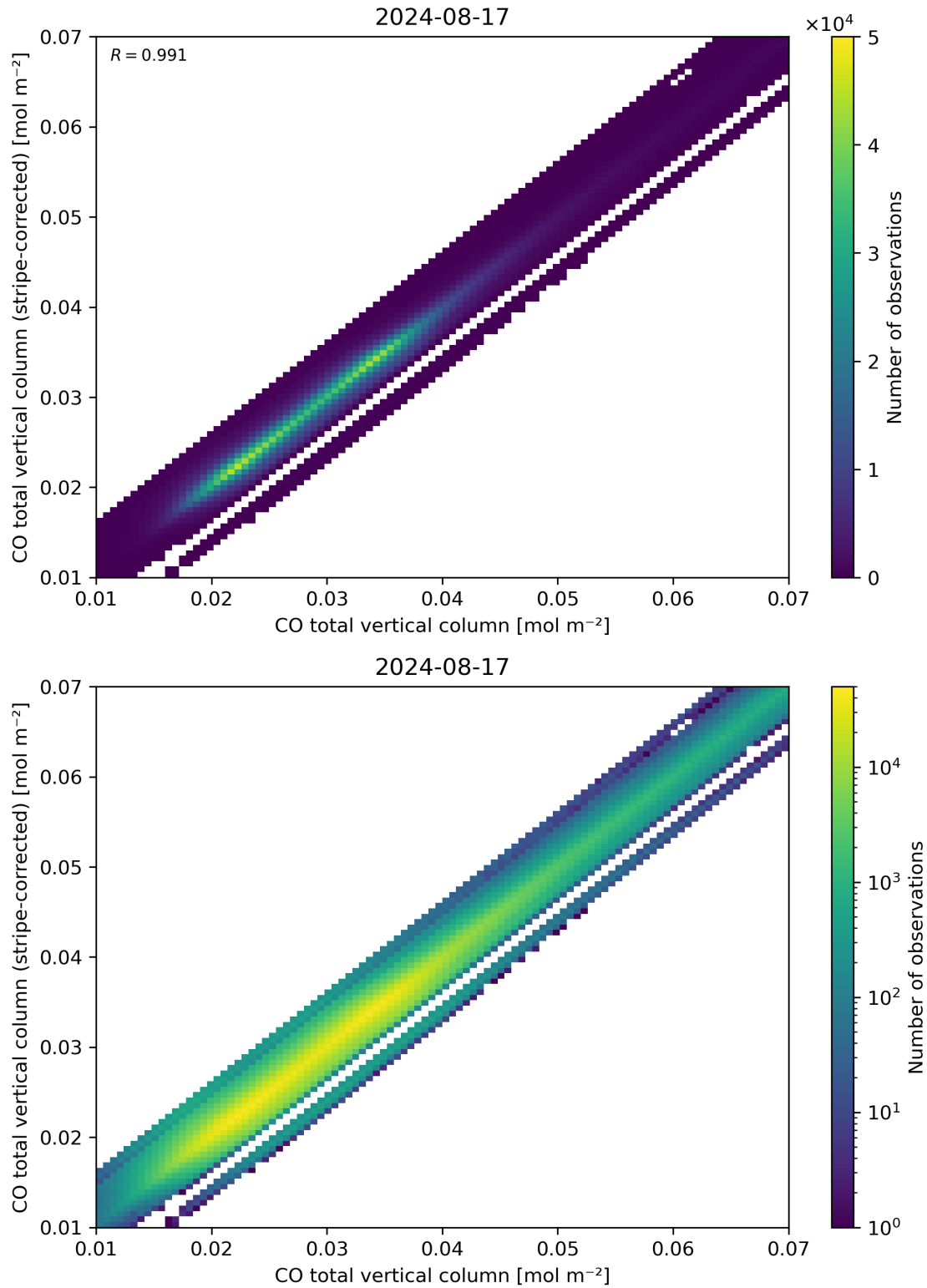
Figure 33: Scatter density plot of “CO total vertical column” against “CO total vertical column (stripe-corrected)” for 2024-08-16 to 2024-08-18.
