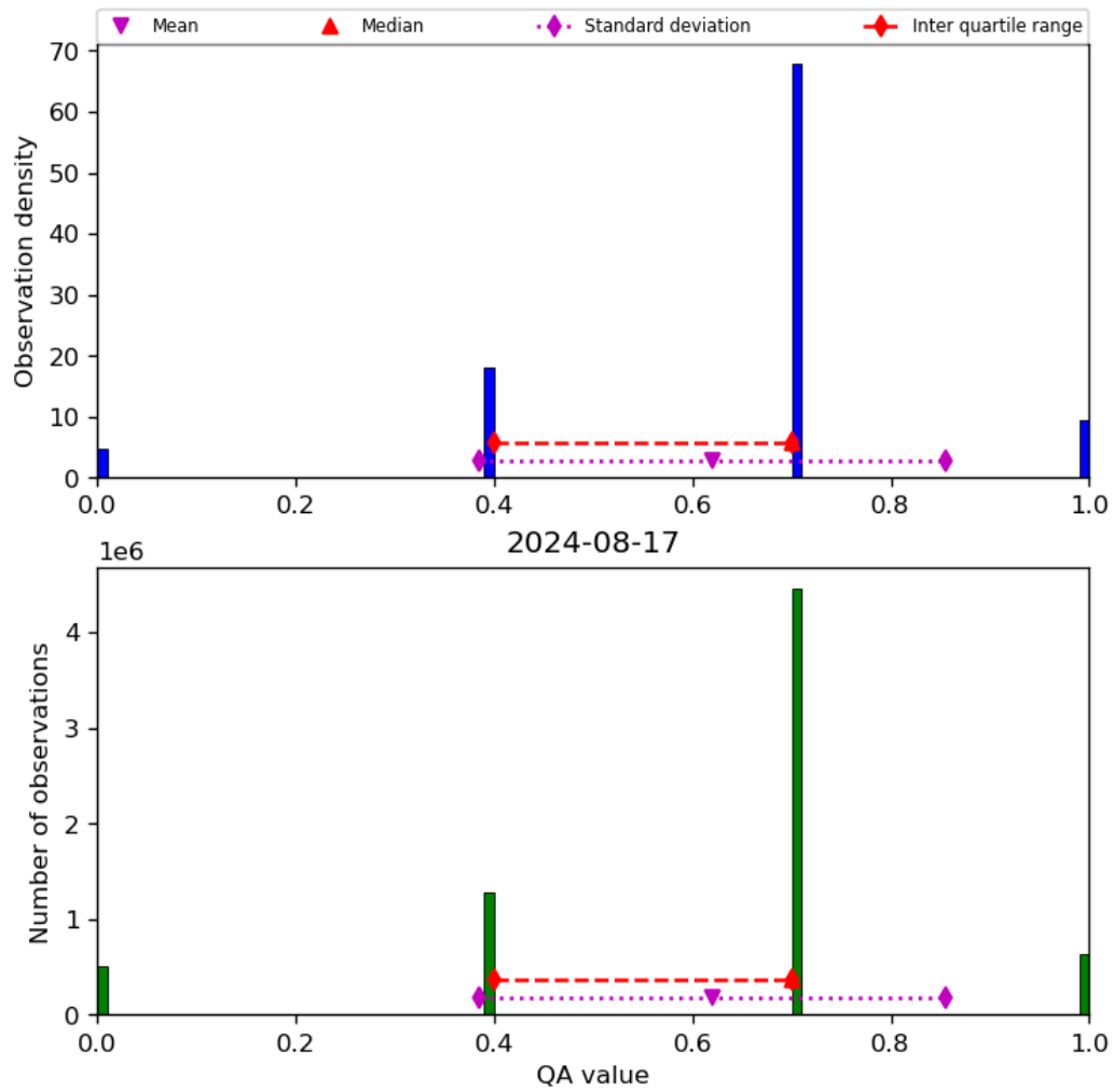
Figure 17: Histogram of “QA value” for 2024-08-16 to 2024-08-18
