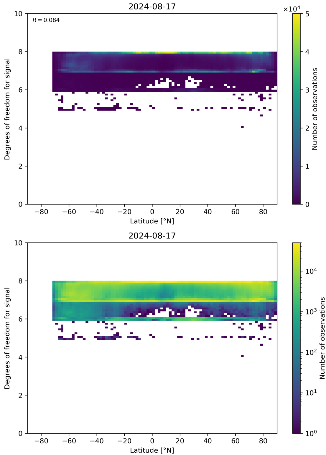
Figure 55: Scatter density plot of “Latitude” against “Degrees of freedom for signal” for 2024-08-16 to 2024-08-18.
