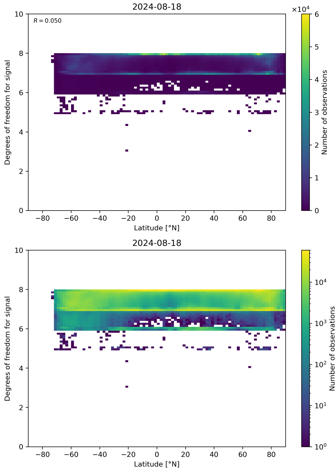
Figure 55: Scatter density plot of “Latitude” against “Degrees of freedom for signal” for 2024-08-17 to 2024-08-19.
