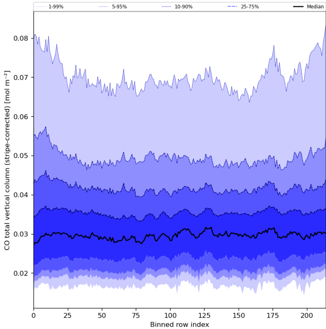
Figure 27: Along track statistics of “CO total vertical column (stripe-corrected)” for 2024-08-17 to 2024-08-19
