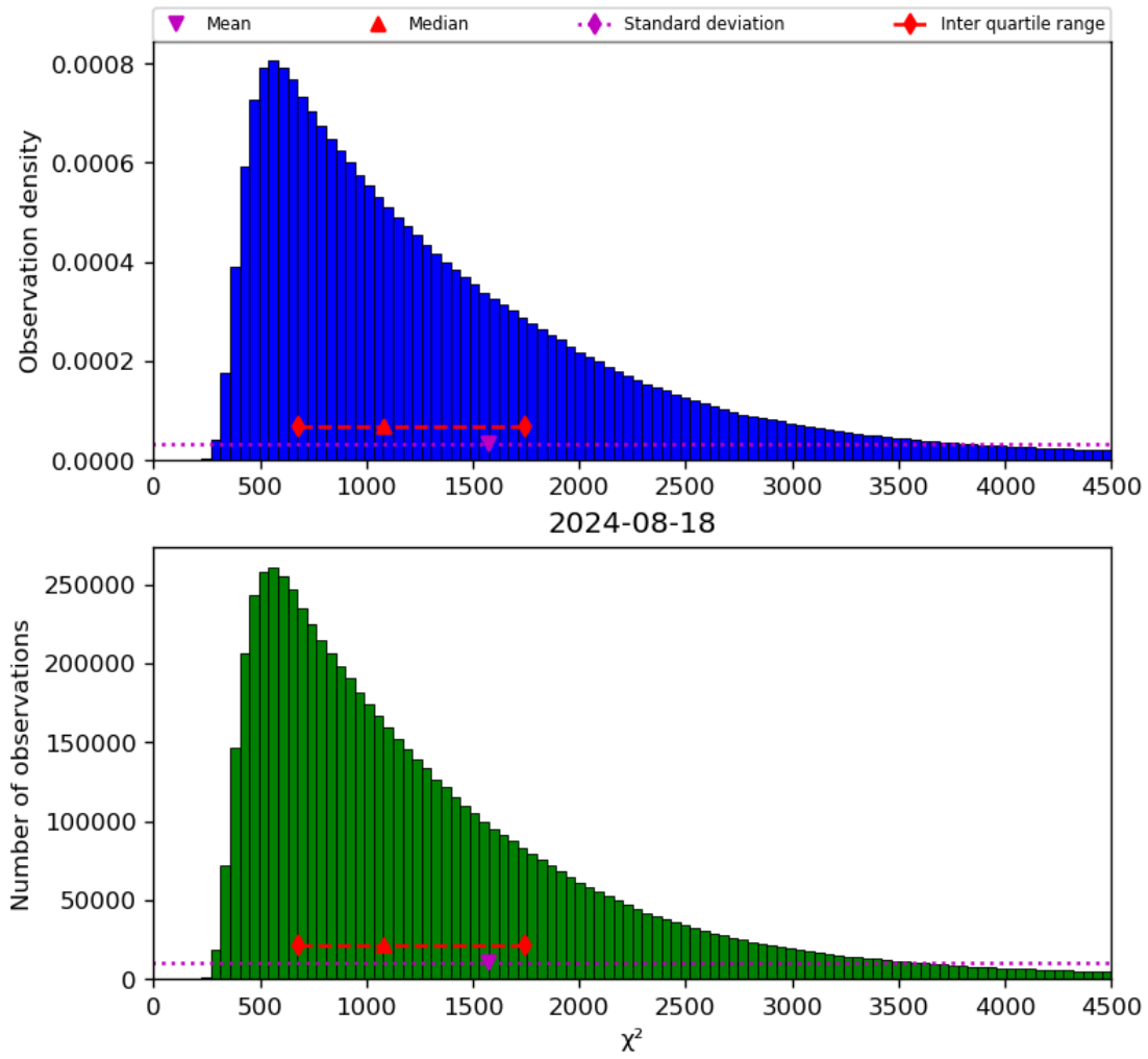
Figure 22: Histogram of “ \chi^2 ” for 2024-08-17 to 2024-08-19
