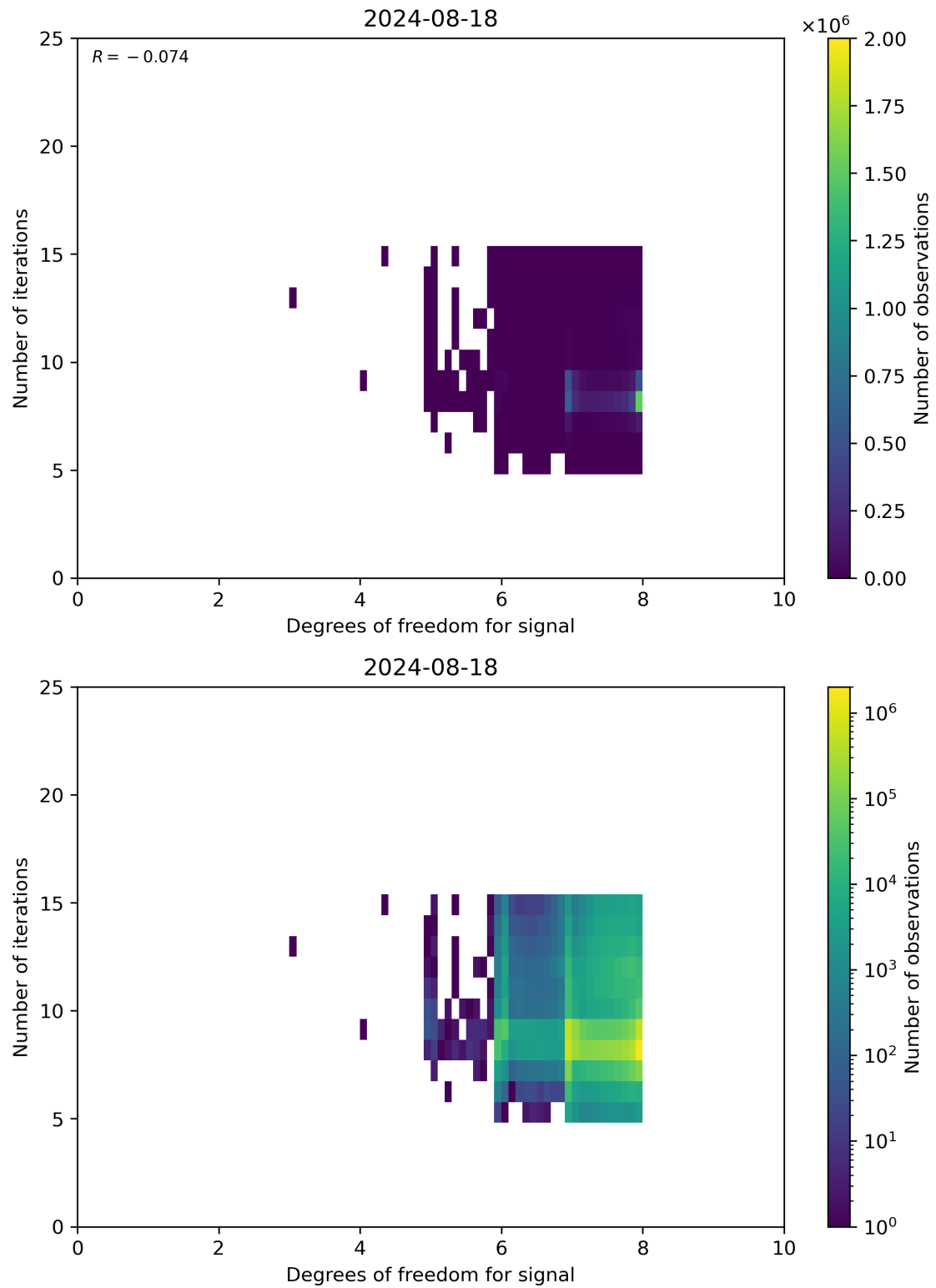
Figure 50: Scatter density plot of “Degrees of freedom for signal” against “Number of iterations” for 2024-08-17 to 2024-08-19.
