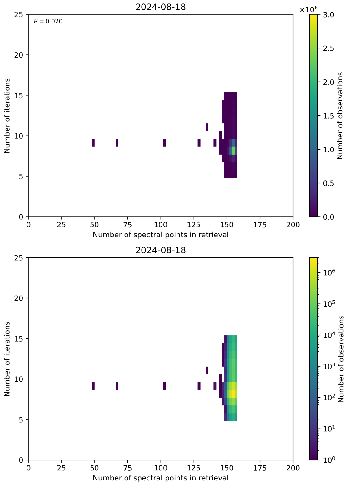
Figure 60: Scatter density plot of “Number of spectral points in retrieval” against “Number of iterations” for 2024-08-17 to 2024-08-19.
