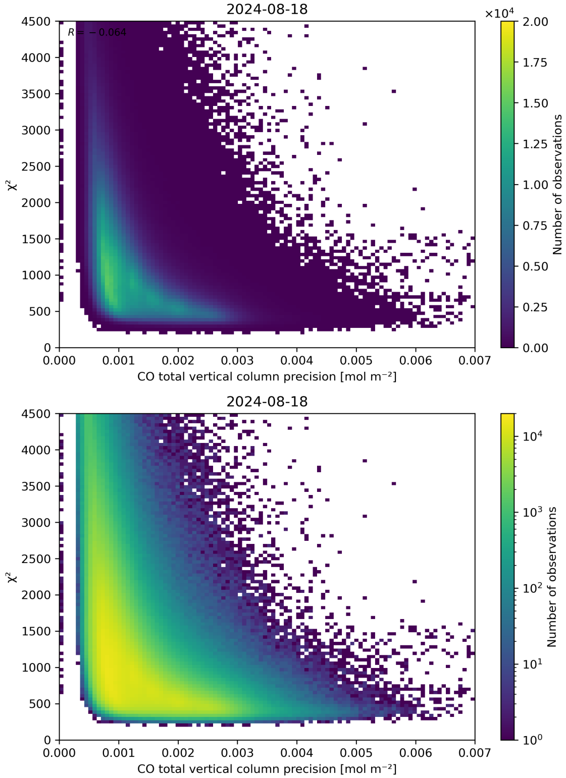
Figure 44: Scatter density plot of “CO total vertical column precision” against “ \chi^2 ” for 2024-08-17 to 2024-08-19.
