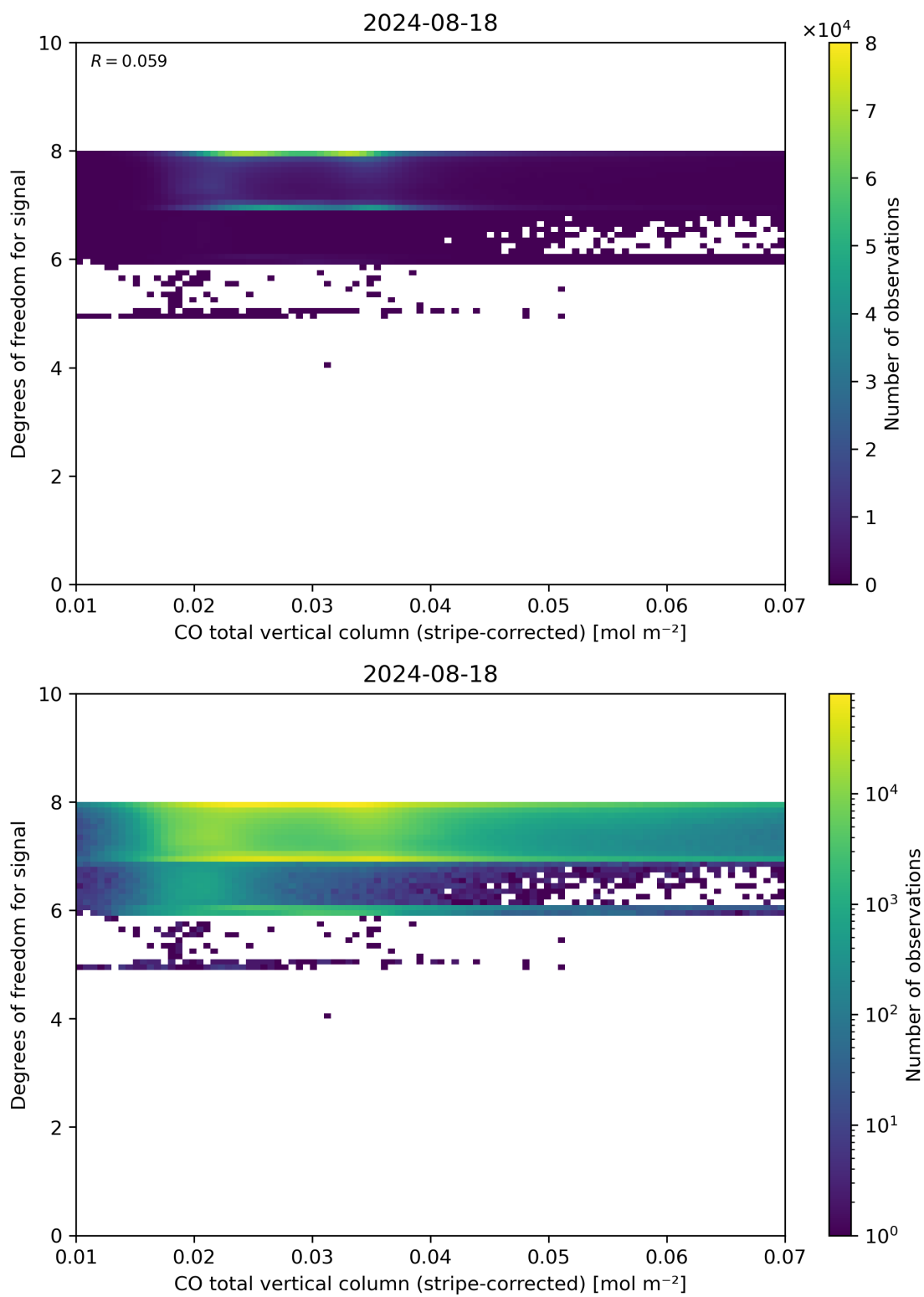
Figure 38: Scatter density plot of “CO total vertical column (stripe-corrected)” against “Degrees of freedom for signal” for 2024-08-17 to 2024-08-19.
