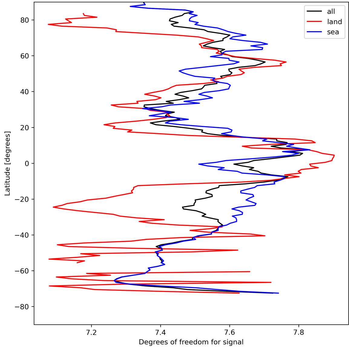
Figure 15: Zonal average of “Degrees of freedom for signal” for 2024-08-17 to 2024-08-19.
