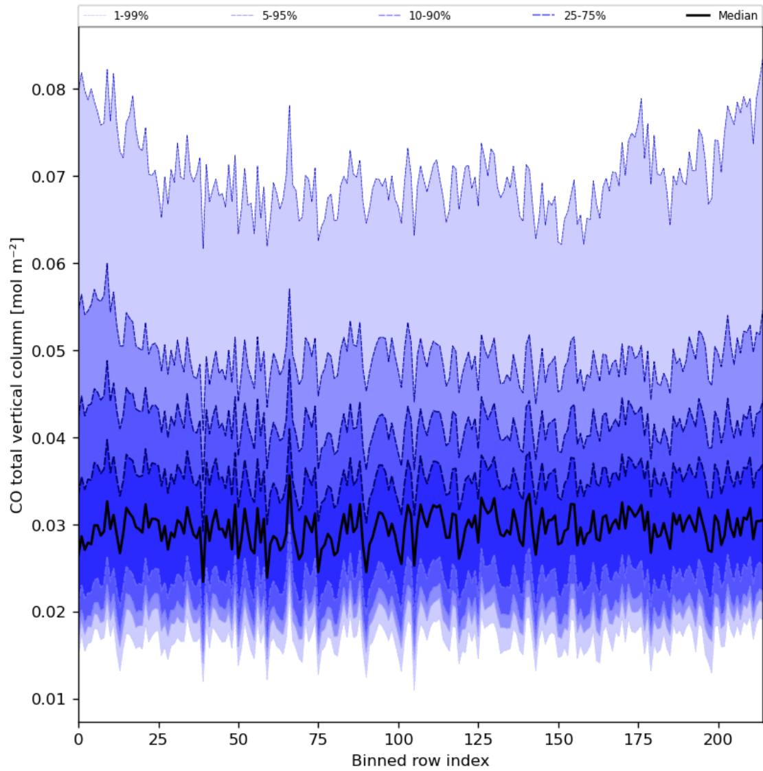
Figure 26: Along track statistics of “CO total vertical column” for 2024-08-17 to 2024-08-19
