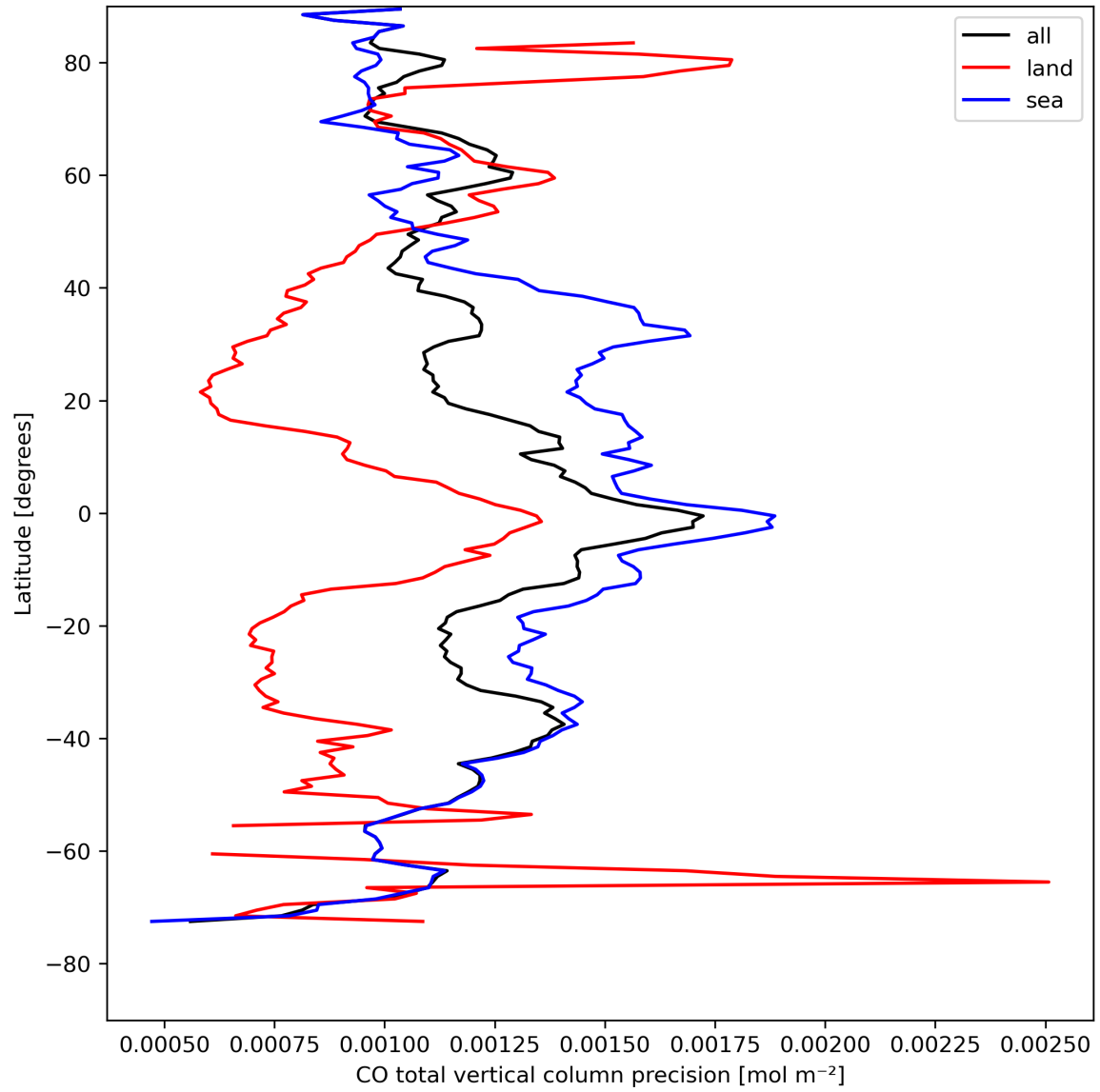
Figure 12: Zonal average of “CO total vertical column precision” for 2024-08-17 to 2024-08-19.
