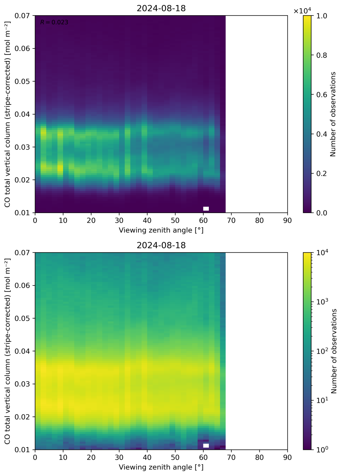
Figure 70: Scatter density plot of “Viewing zenith angle” against “CO total vertical column (stripe-corrected)” for 2024-08-17 to 2024-08-19.
