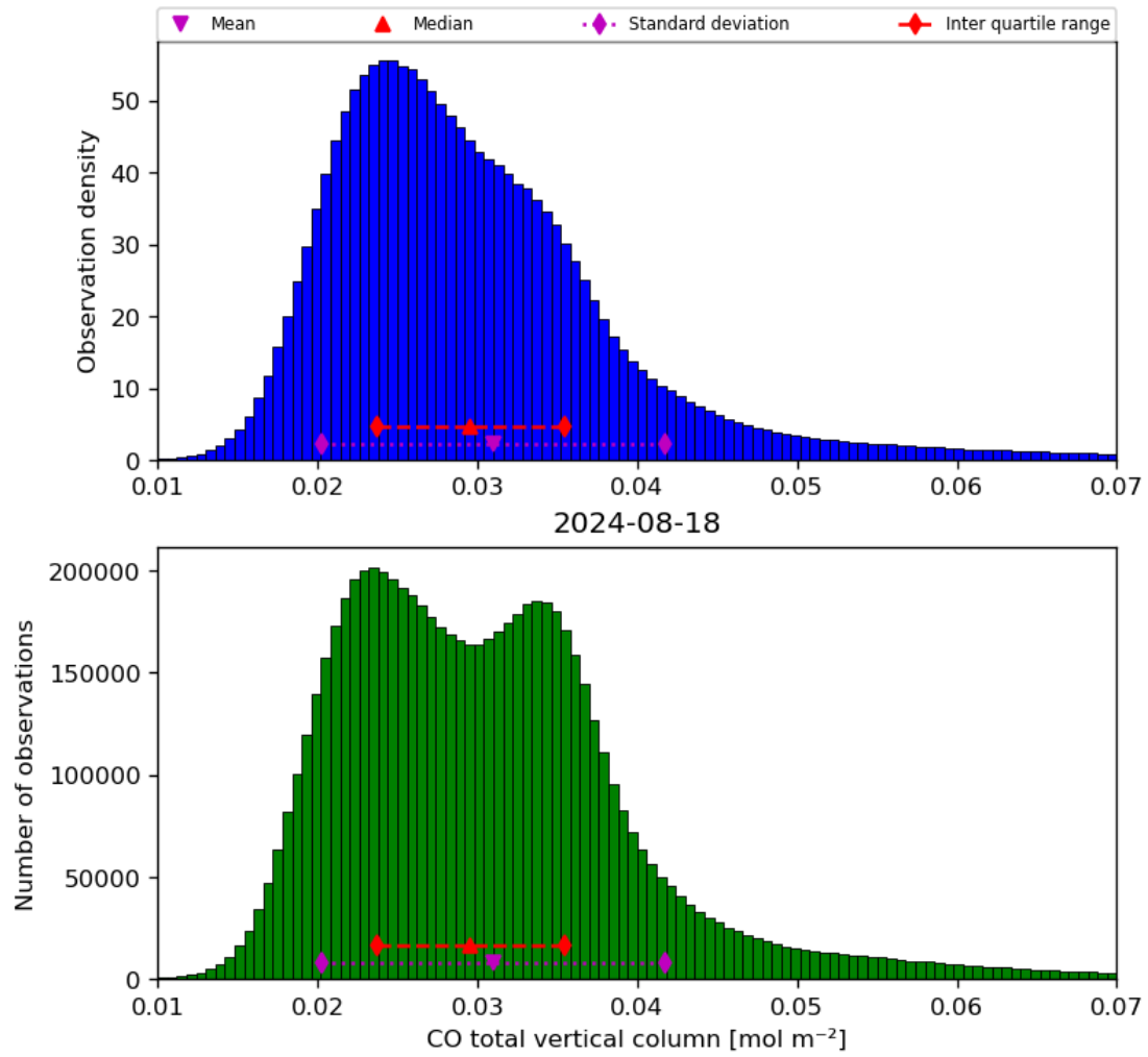
Figure 18: Histogram of “CO total vertical column” for 2024-08-17 to 2024-08-19
