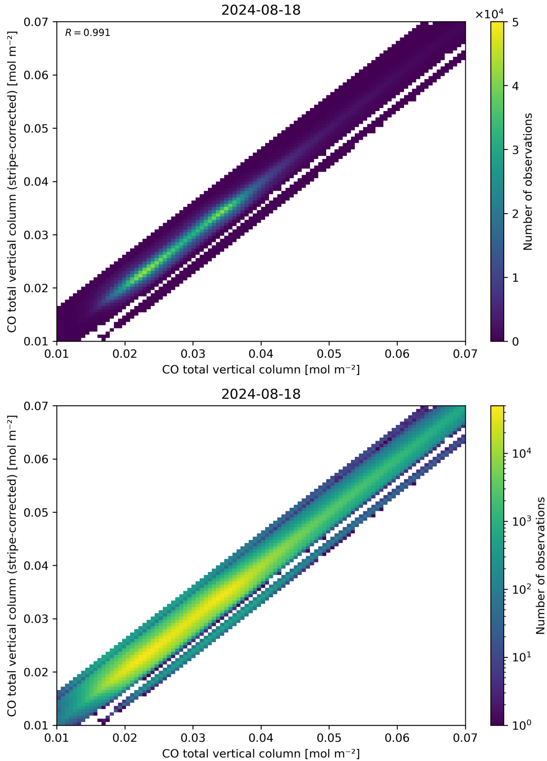
Figure 33: Scatter density plot of “CO total vertical column” against “CO total vertical column (stripe-corrected)” for 2024-08-17 to 2024-08-19.
