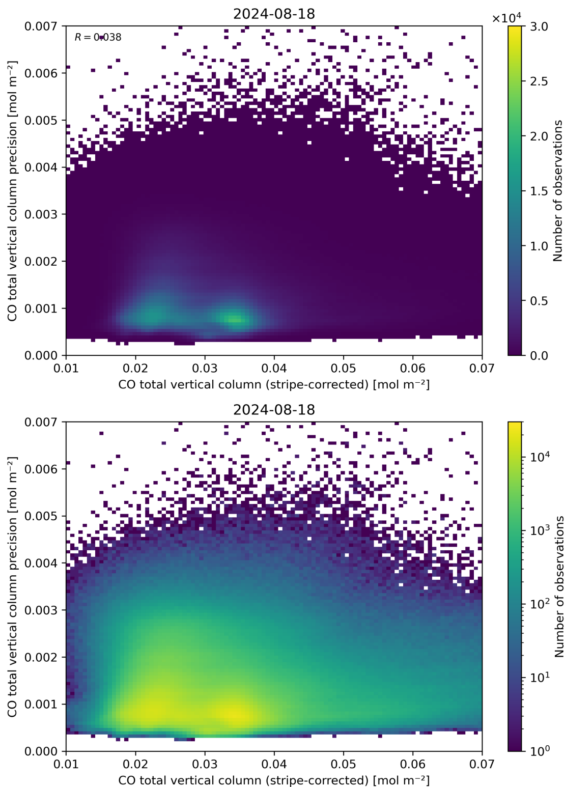
Figure 36: Scatter density plot of “CO total vertical column (stripe-corrected)” against “CO total vertical column precision” for 2024-08-17 to 2024-08-19.
