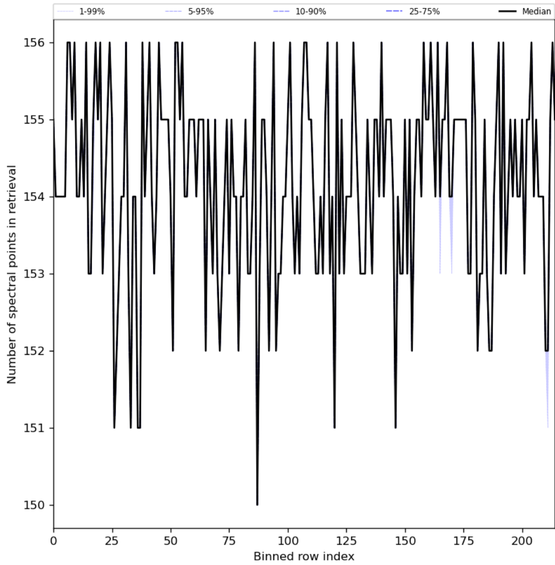
Figure 29: Along track statistics of “Number of spectral points in retrieval” for 2024-08-17 to 2024-08-19
