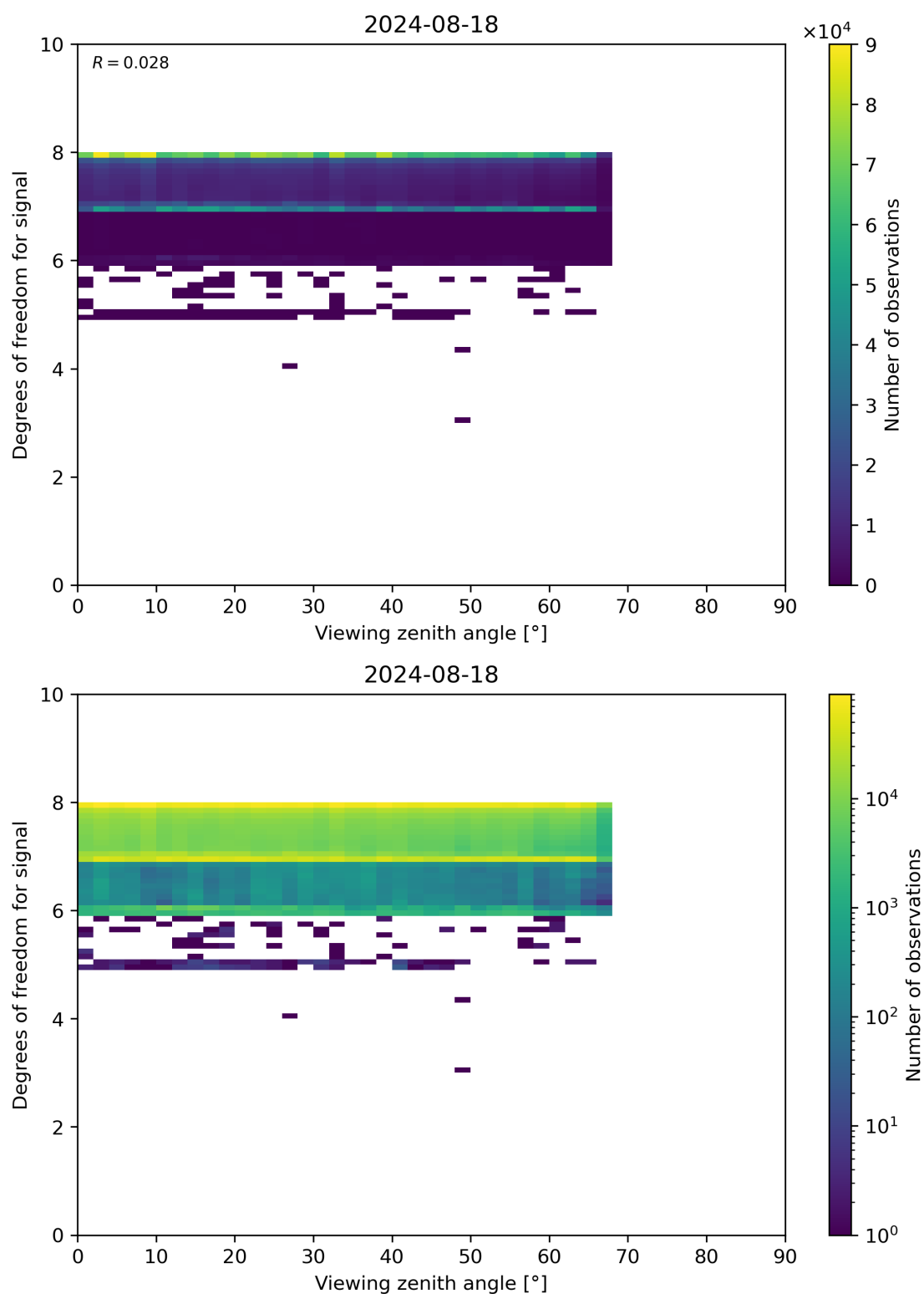
Figure 73: Scatter density plot of “Viewing zenith angle” against “Degrees of freedom for signal” for 2024-08-17 to 2024-08-19.
