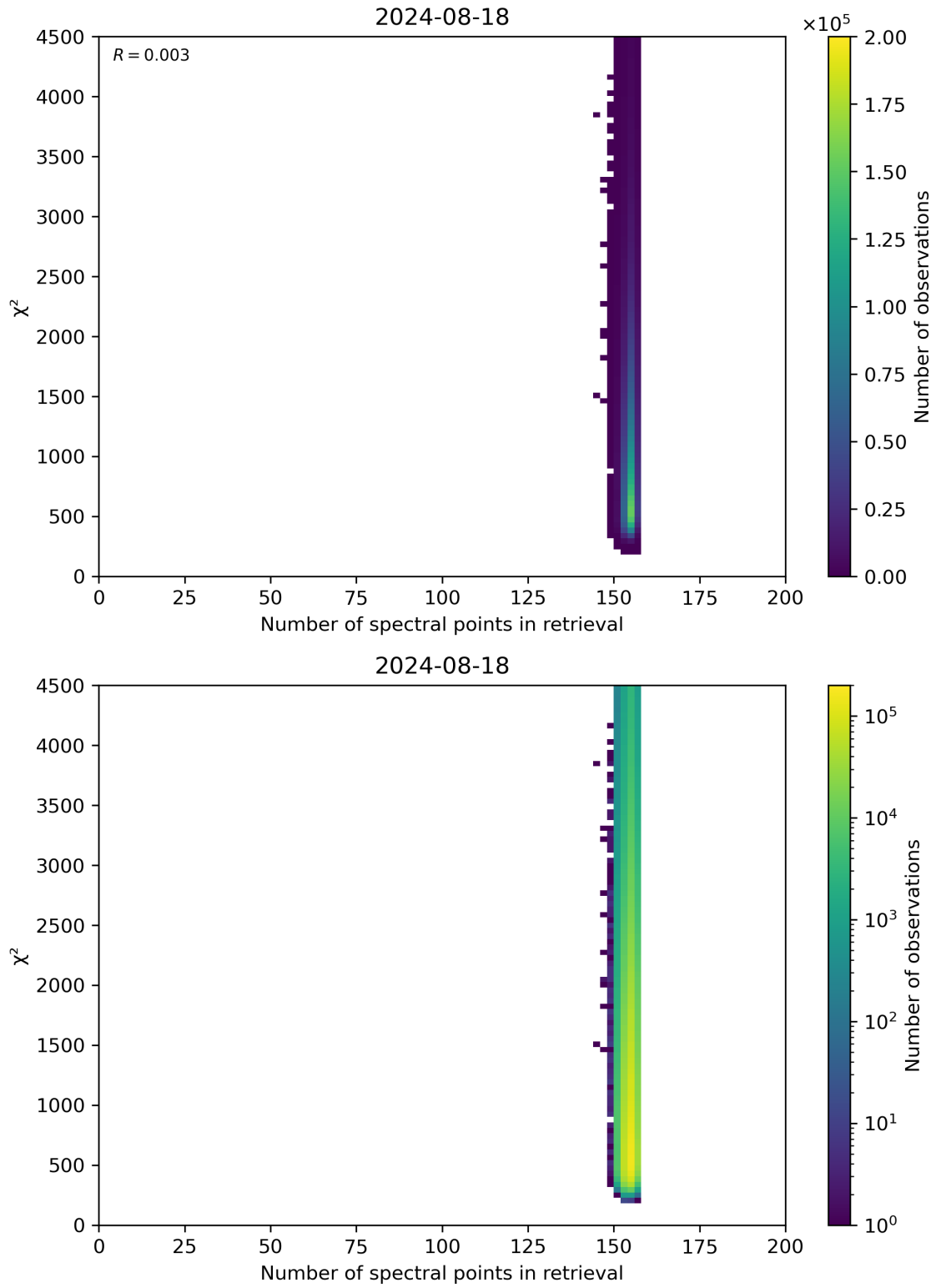
Figure 58: Scatter density plot of “Number of spectral points in retrieval” against “ \chi^2 ” for 2024-08-17 to 2024-08-19.
