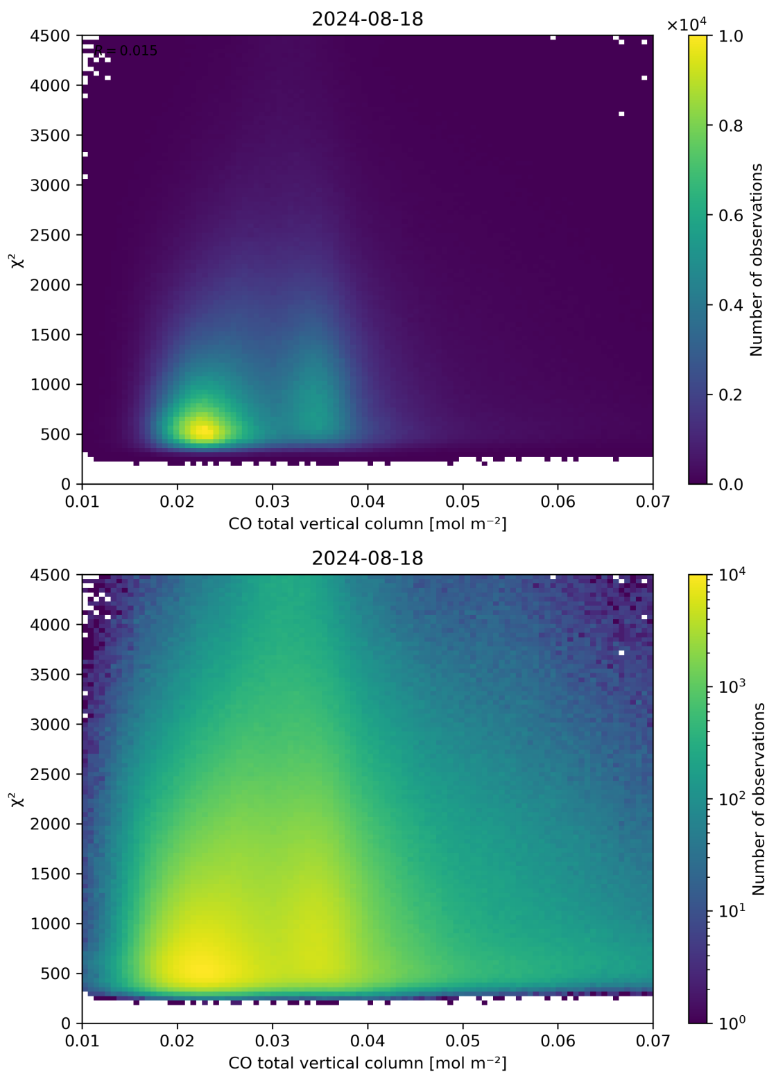
Figure 35: Scatter density plot of “CO total vertical column” against “ \chi^2 ” for 2024-08-17 to 2024-08-19.
