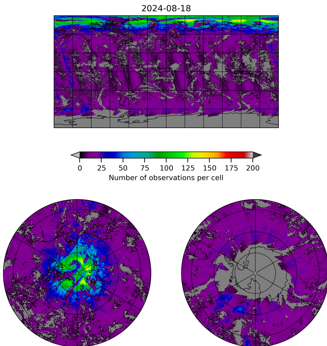
Figure 8: Map of the number of observations for 2024-08-17 to 2024-08-19
