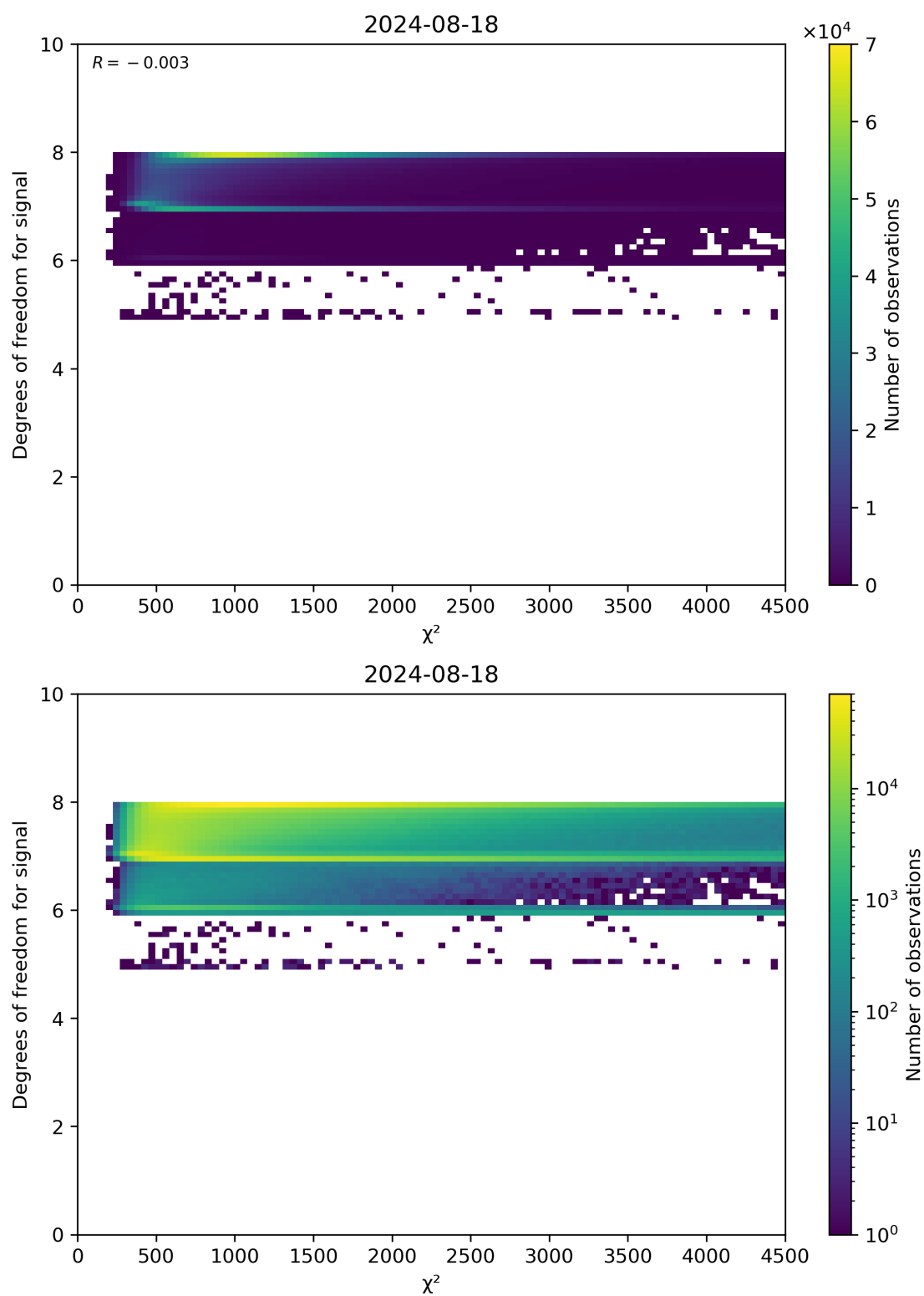
Figure 48: Scatter density plot of “ \chi^2 ” against “Degrees of freedom for signal” for 2024-08-17 to 2024-08-19.
