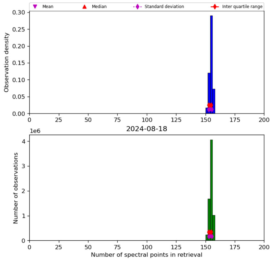
Figure 21: Histogram of “Number of spectral points in retrieval” for 2024-08-17 to 2024-08-19
