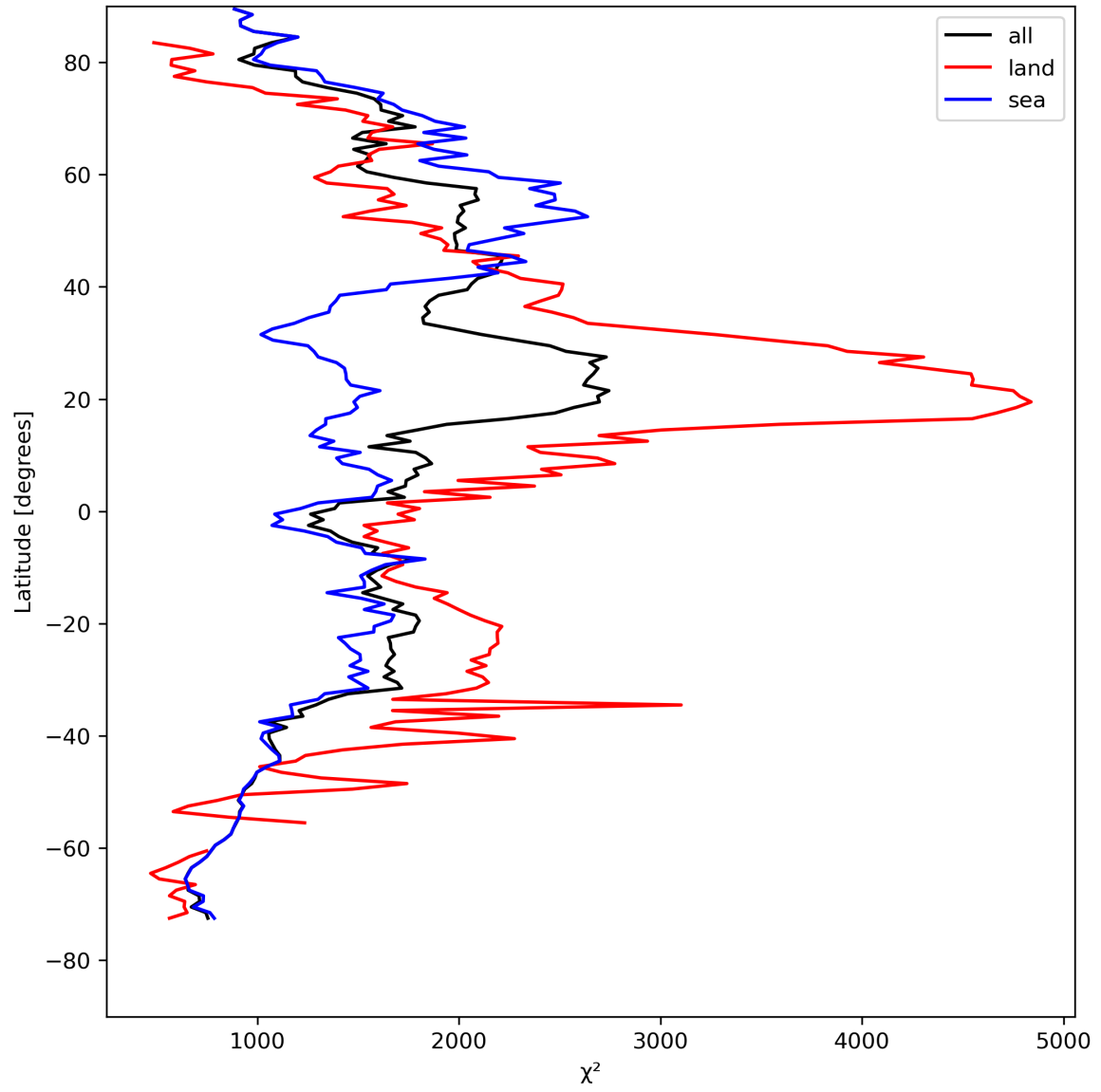
Figure 14: Zonal average of “ \chi^2 ” for 2024-08-17 to 2024-08-19.
