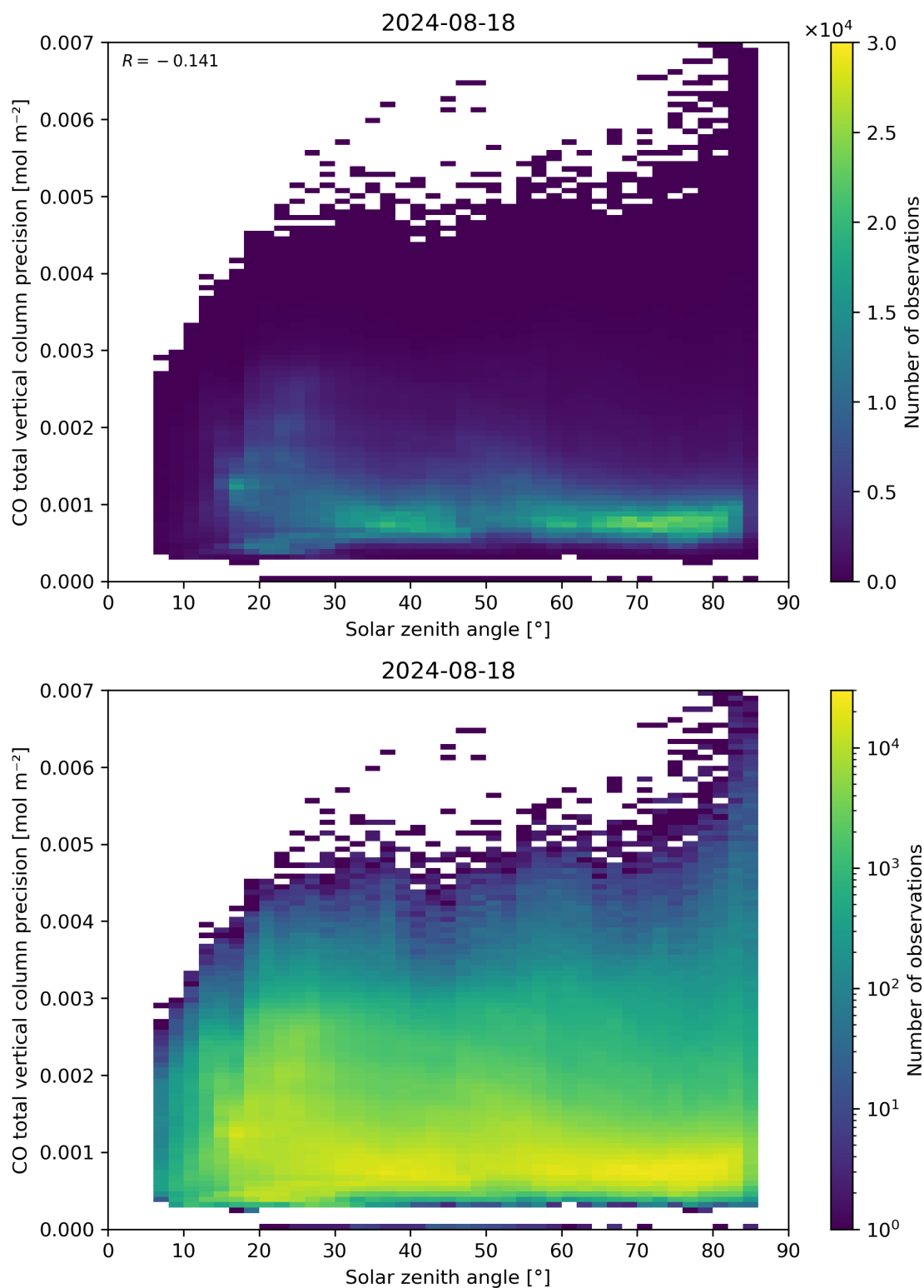
Figure 63: Scatter density plot of “Solar zenith angle” against “CO total vertical column precision” for 2024-08-17 to 2024-08-19.
