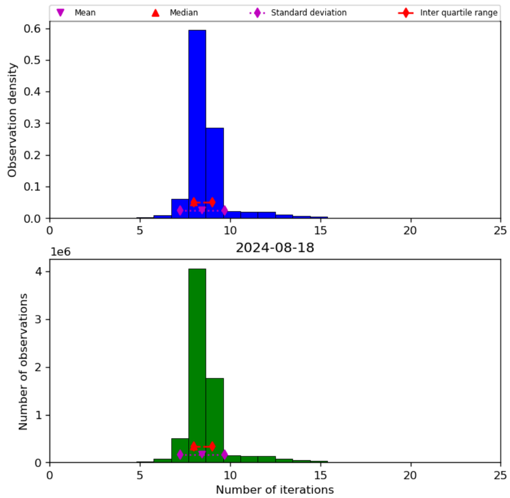
Figure 24: Histogram of “Number of iterations” for 2024-08-17 to 2024-08-19
