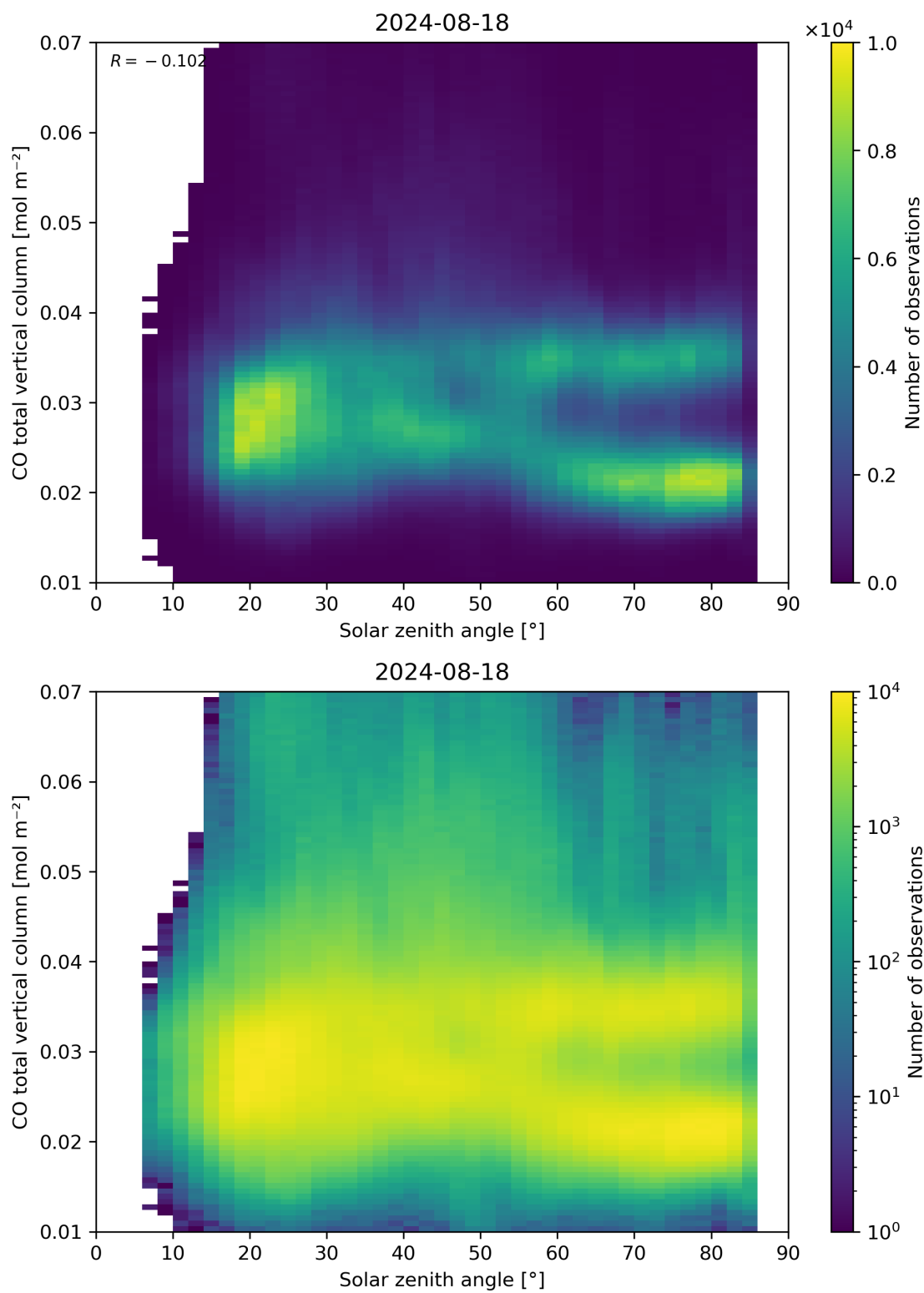
Figure 61: Scatter density plot of “Solar zenith angle” against “CO total vertical column” for 2024-08-17 to 2024-08-19.
