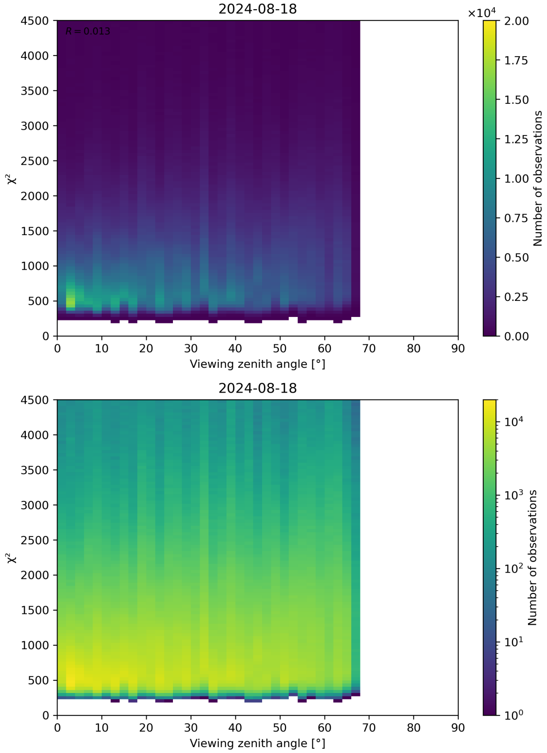
Figure 72: Scatter density plot of “Viewing zenith angle” against “ \chi^2 ” for 2024-08-17 to 2024-08-19.
