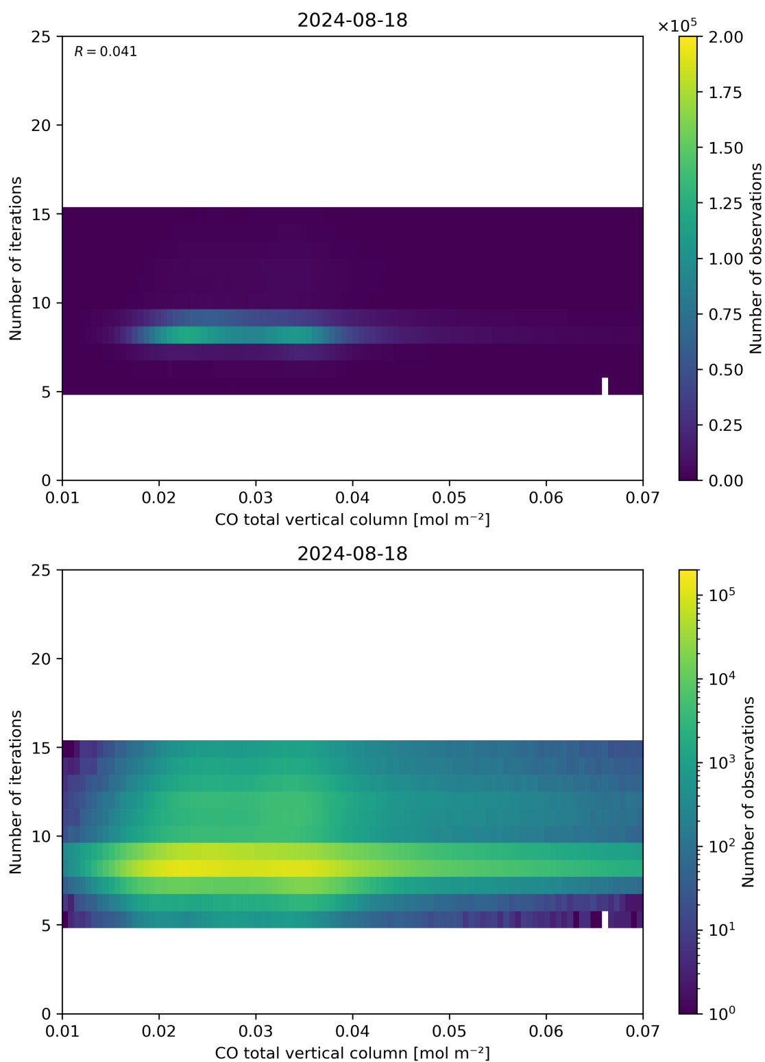
Figure 42: Scatter density plot of “CO total vertical column” against “Number of iterations” for 2024-08-17 to 2024-08-19.
