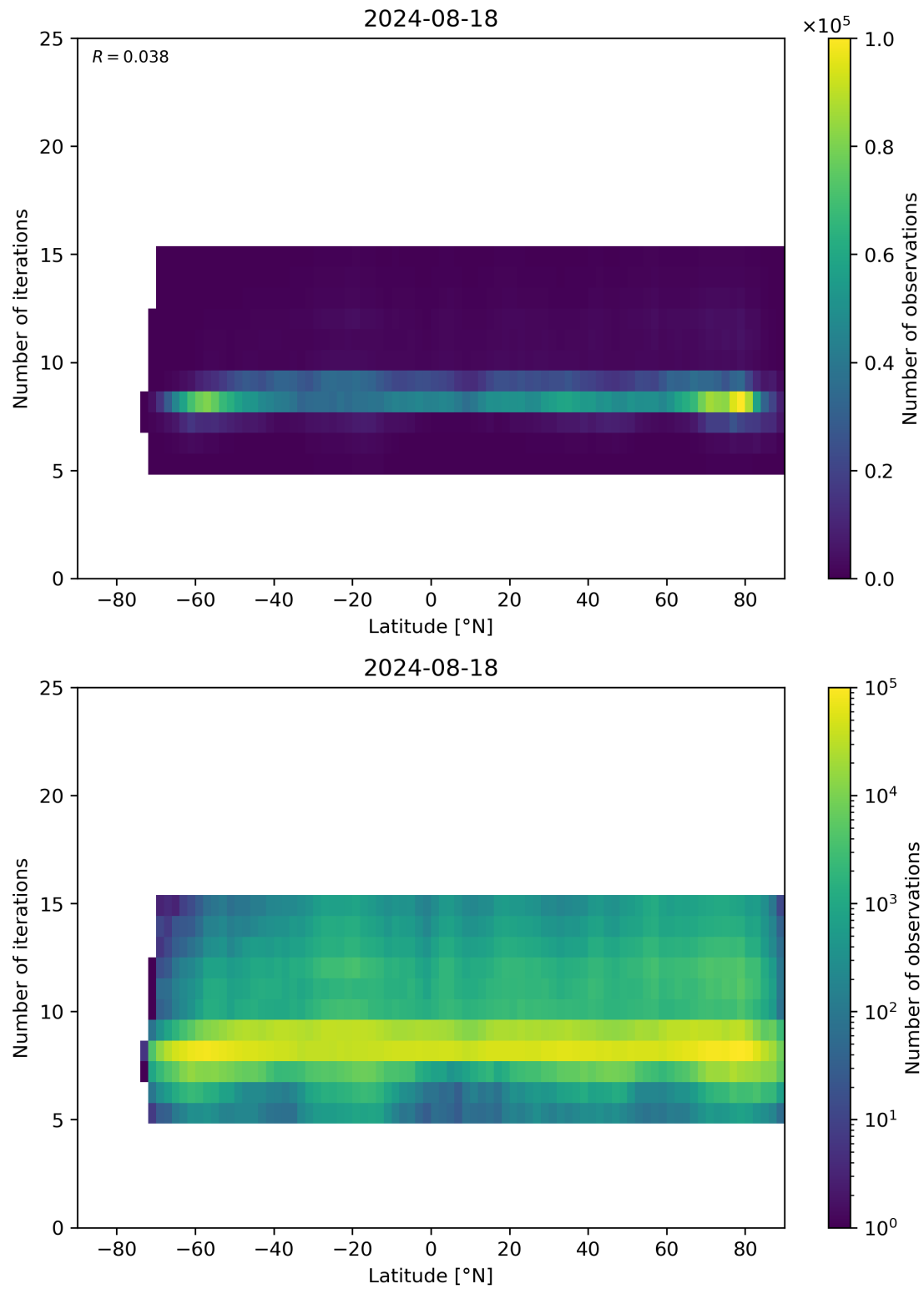
Figure 56: Scatter density plot of “Latitude” against “Number of iterations” for 2024-08-17 to 2024-08-19.
