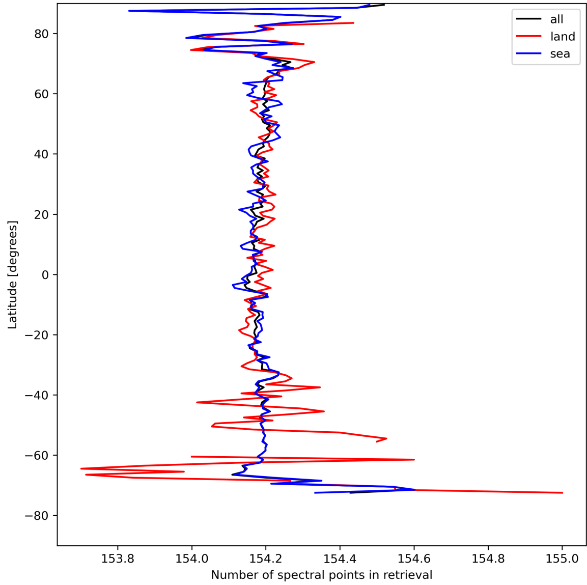
Figure 13: Zonal average of “Number of spectral points in retrieval” for 2024-08-17 to 2024-08-19.
