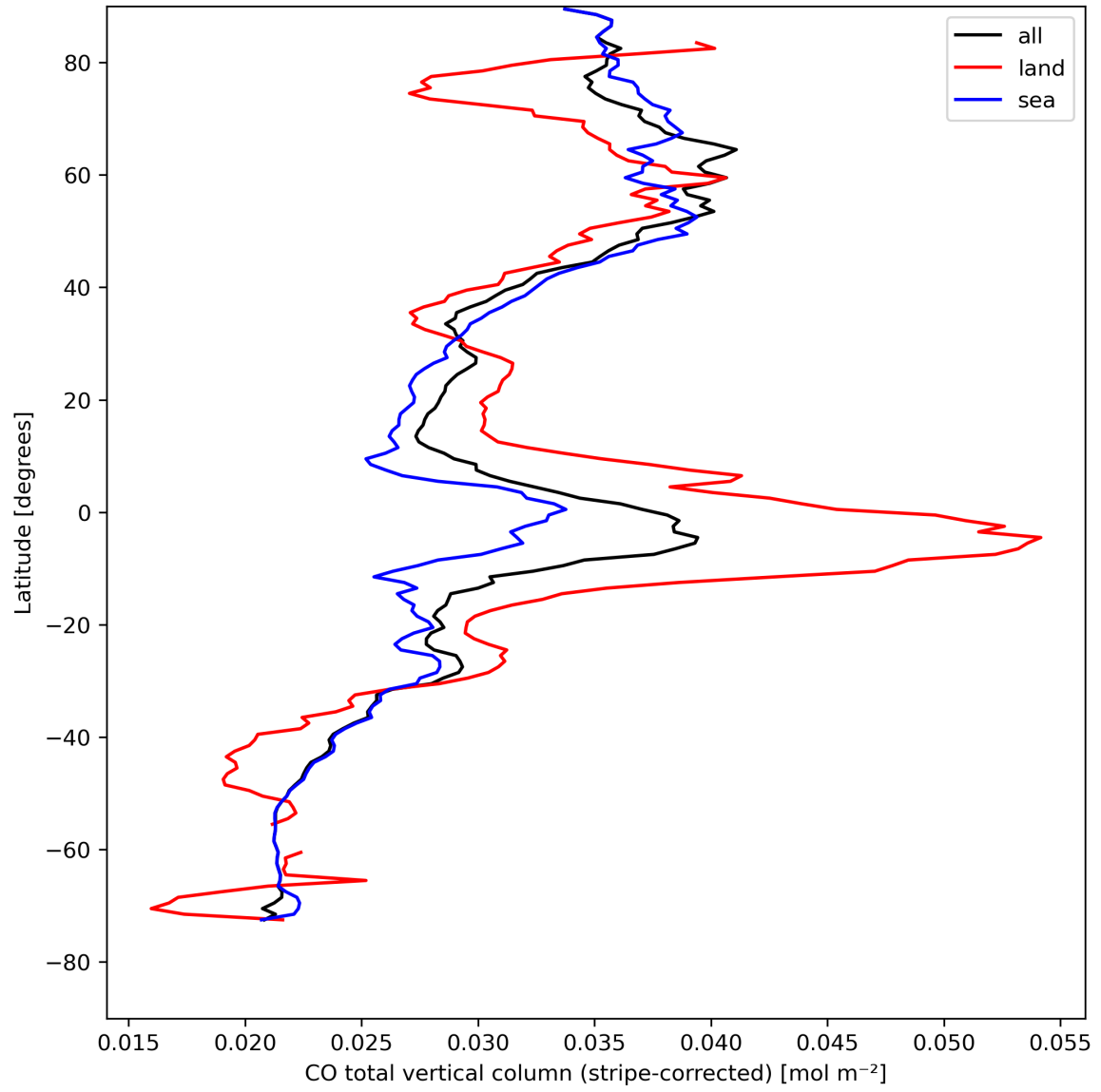
Figure 11: Zonal average of “CO total vertical column (stripe-corrected)” for 2024-08-17 to 2024-08-19.
