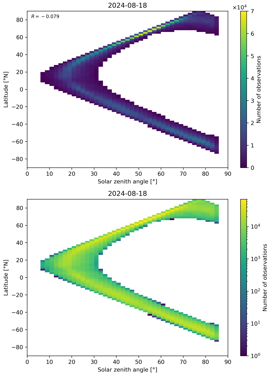
Figure 66: Scatter density plot of “Solar zenith angle” against “Latitude” for 2024-08-17 to 2024-08-19.
