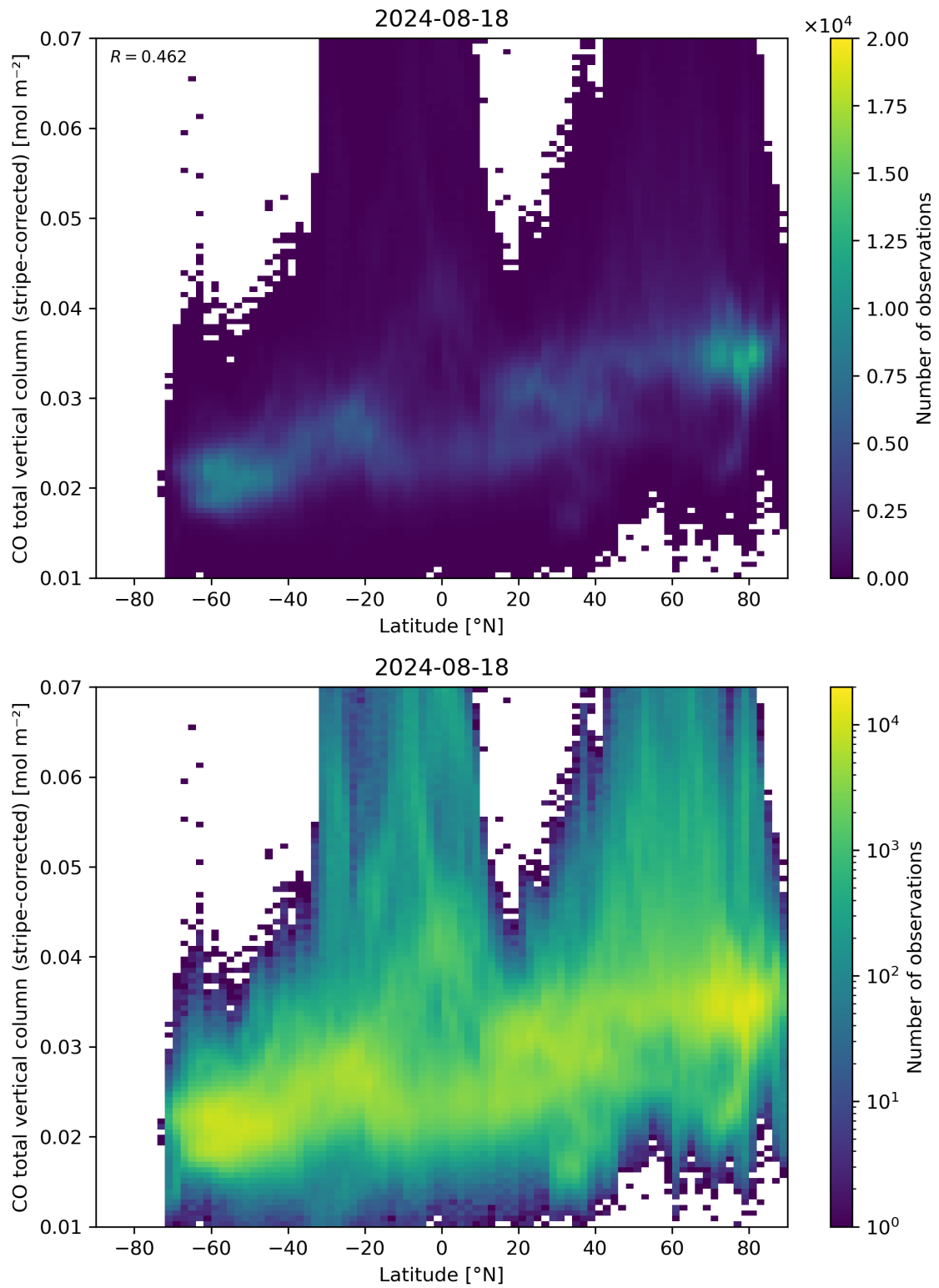
Figure 52: Scatter density plot of “Latitude” against “CO total vertical column (stripe-corrected)” for 2024-08-17 to 2024-08-19.
