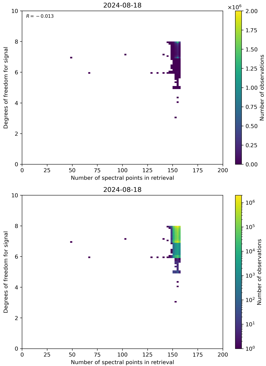
Figure 59: Scatter density plot of “Number of spectral points in retrieval” against “Degrees of freedom for signal” for 2024-08-17 to 2024-08-19.
