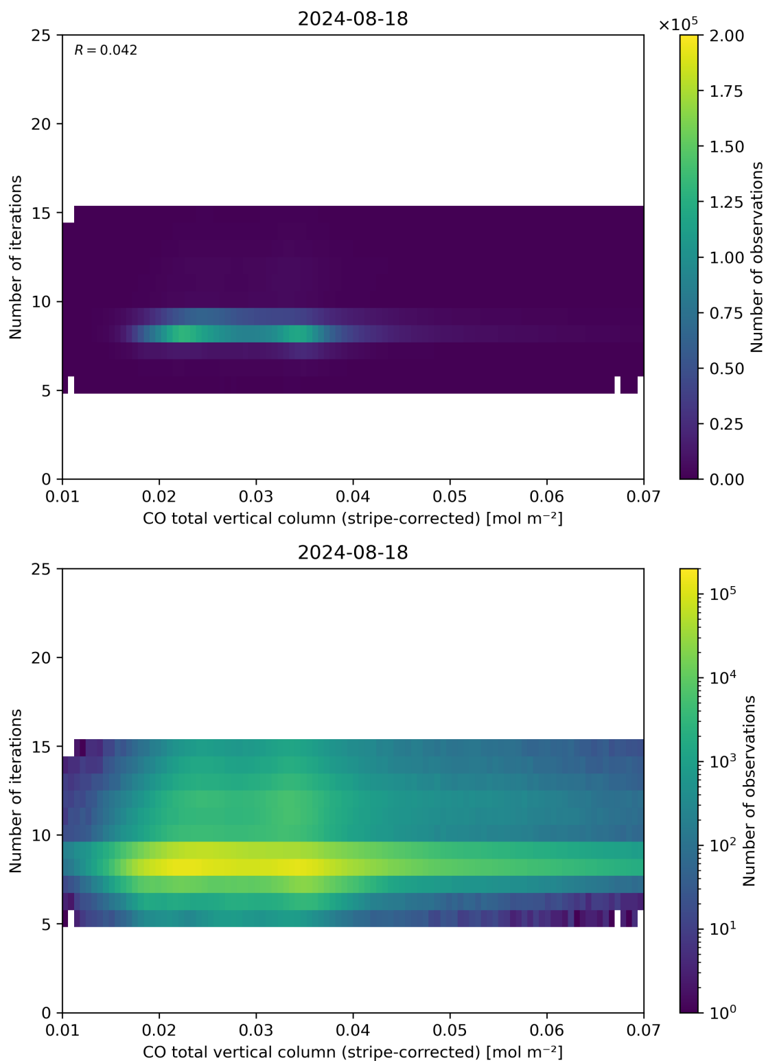
Figure 39: Scatter density plot of “CO total vertical column (stripe-corrected)” against “Number of iterations” for 2024-08-17 to 2024-08-19.
