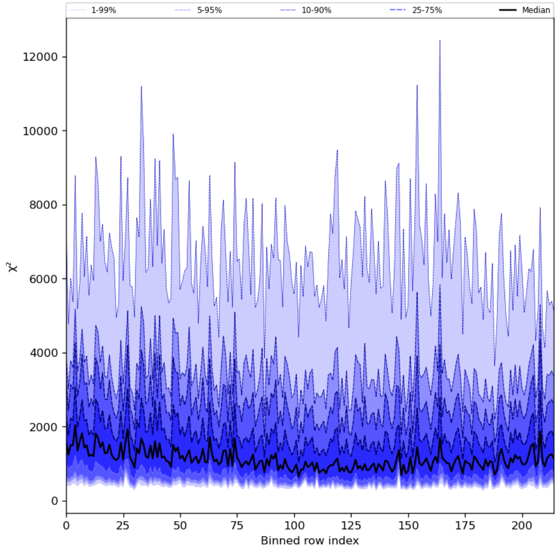
Figure 30: Along track statistics of “ \chi^2 ” for 2024-08-17 to 2024-08-19
