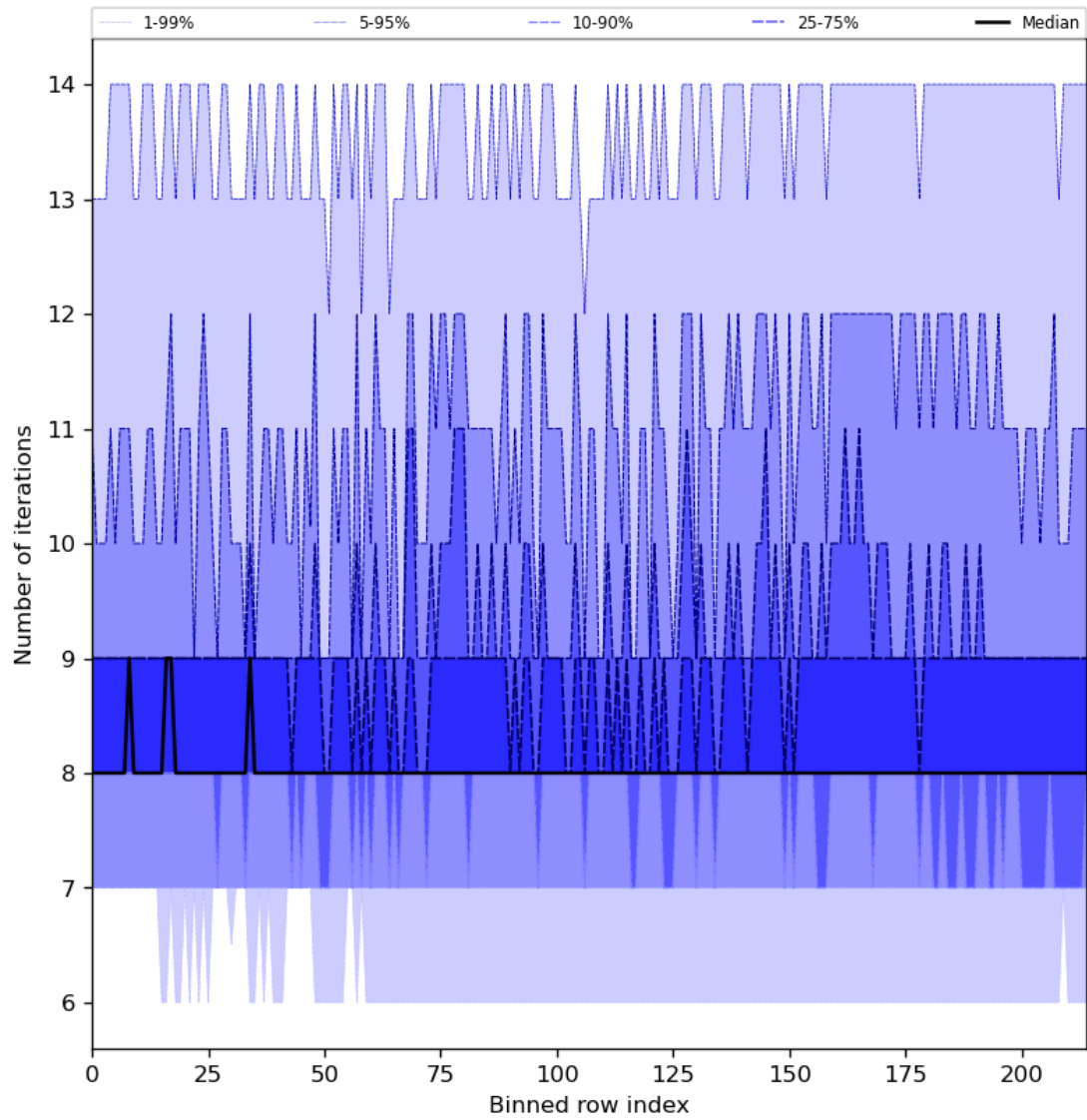
Figure 32: Along track statistics of “Number of iterations” for 2024-08-17 to 2024-08-19
