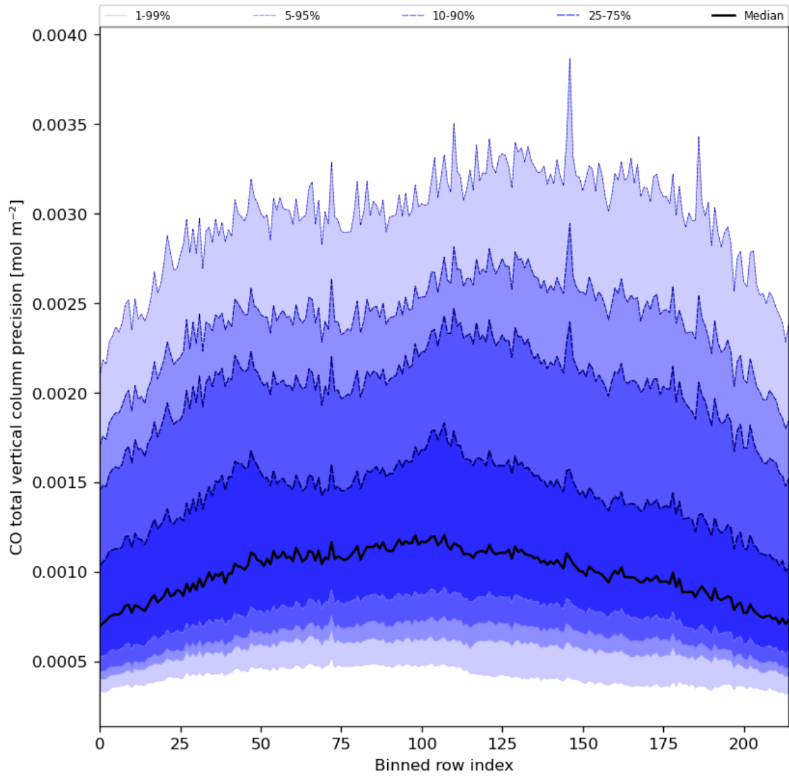
Figure 28: Along track statistics of “CO total vertical column precision” for 2024-08-17 to 2024-08-19
