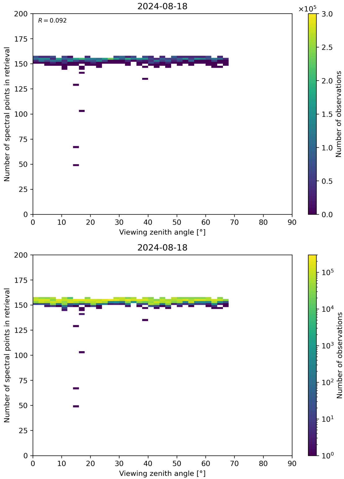
Figure 76: Scatter density plot of “Viewing zenith angle” against “Number of spectral points in retrieval” for 2024-08-17 to 2024-08-19.
