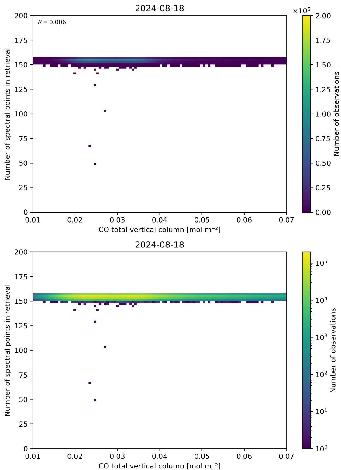
Figure 43: Scatter density plot of “CO total vertical column” against “Number of spectral points in retrieval” for 2024-08-17 to 2024-08-19.
