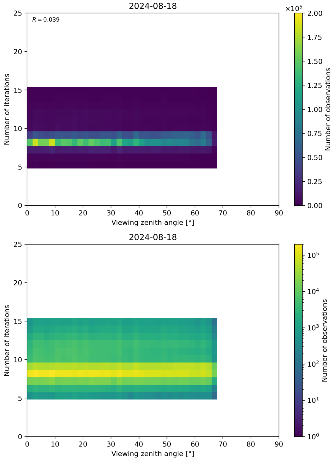
Figure 75: Scatter density plot of “Viewing zenith angle” against “Number of iterations” for 2024-08-17 to 2024-08-19.
