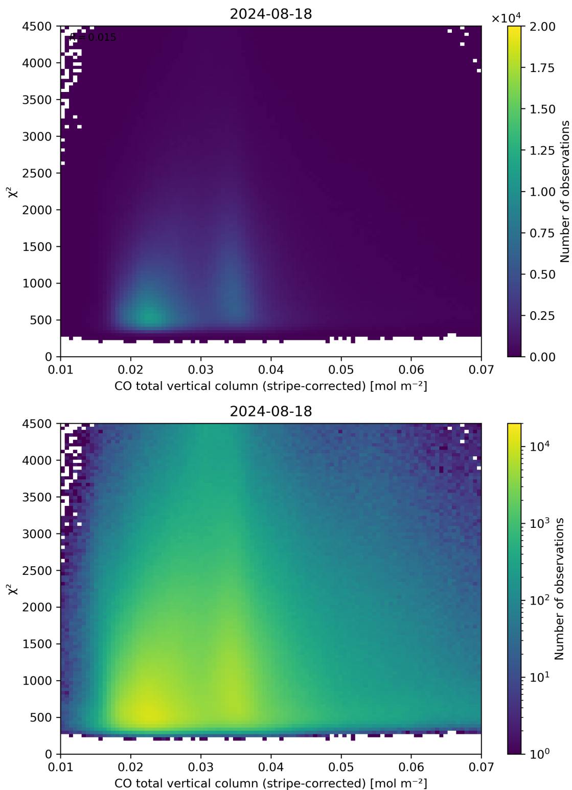
Figure 37: Scatter density plot of “CO total vertical column (stripe-corrected)” against “ \chi^2 ” for 2024-08-17 to 2024-08-19.
