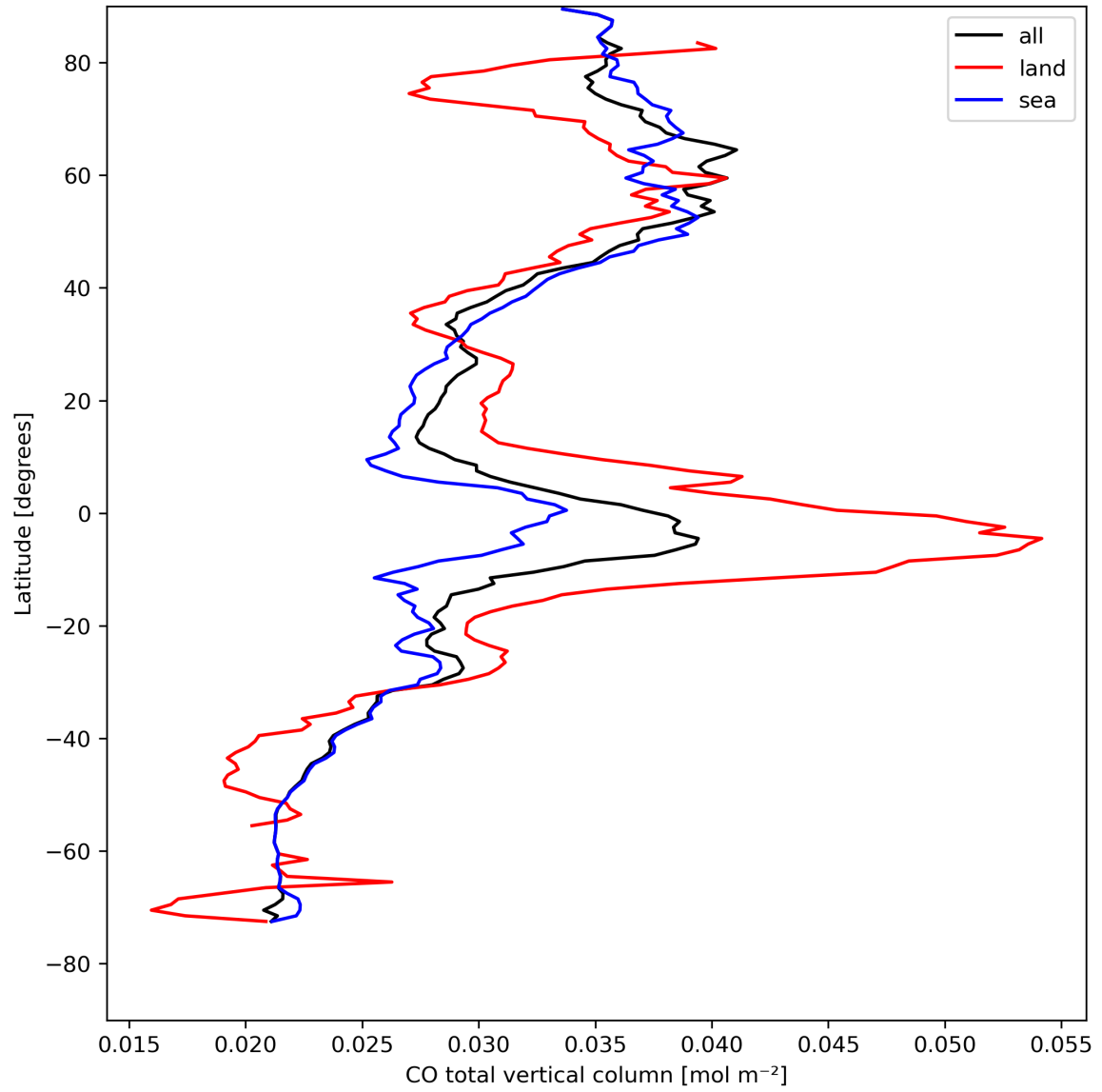
Figure 10: Zonal average of “CO total vertical column” for 2024-08-17 to 2024-08-19.
