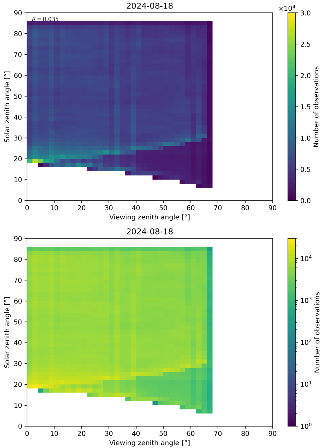
Figure 77: Scatter density plot of “Viewing zenith angle” against “Solar zenith angle” for 2024-08-17 to 2024-08-19.
