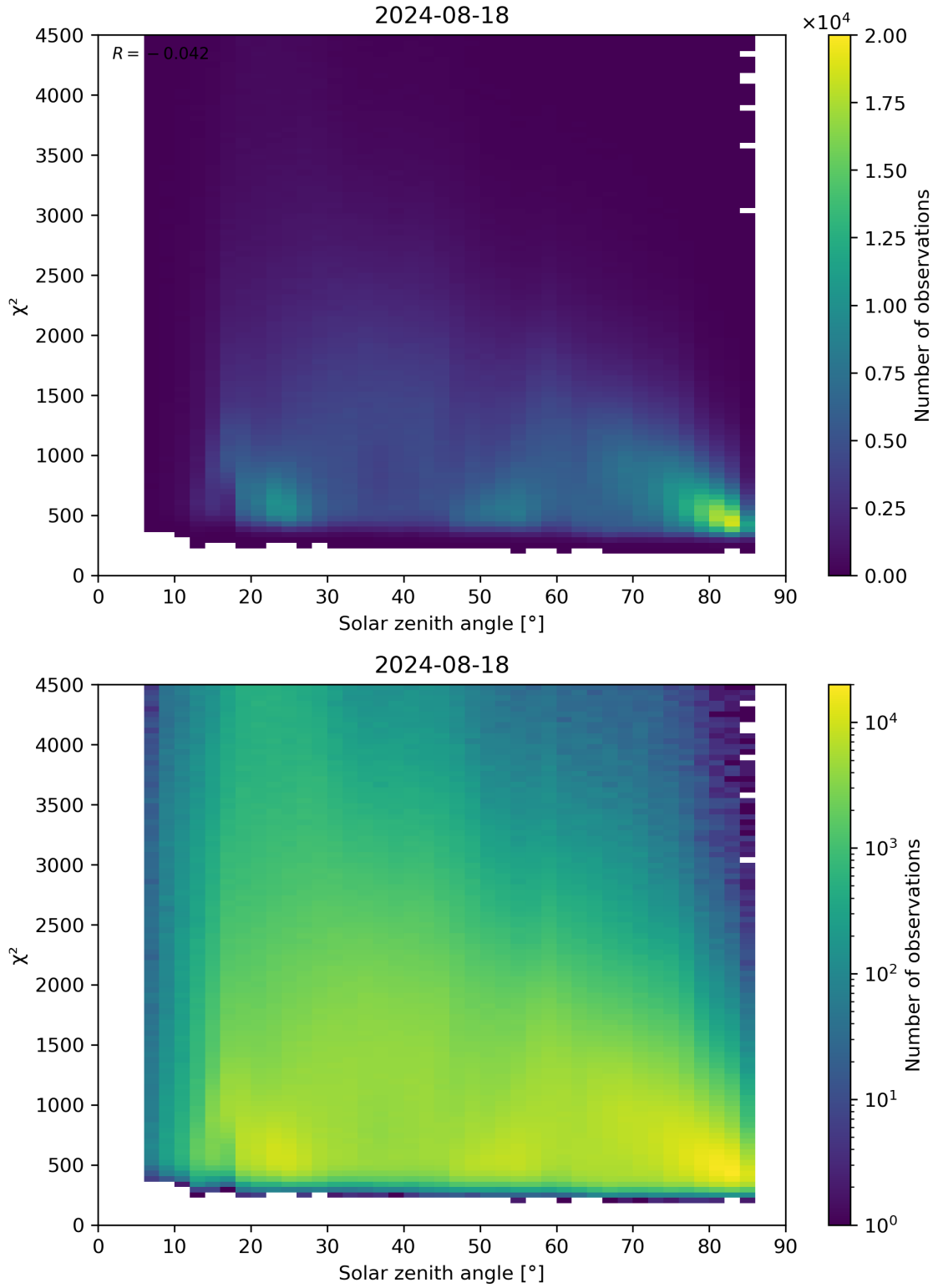
Figure 64: Scatter density plot of “Solar zenith angle” against “ \chi^2 ” for 2024-08-17 to 2024-08-19.
