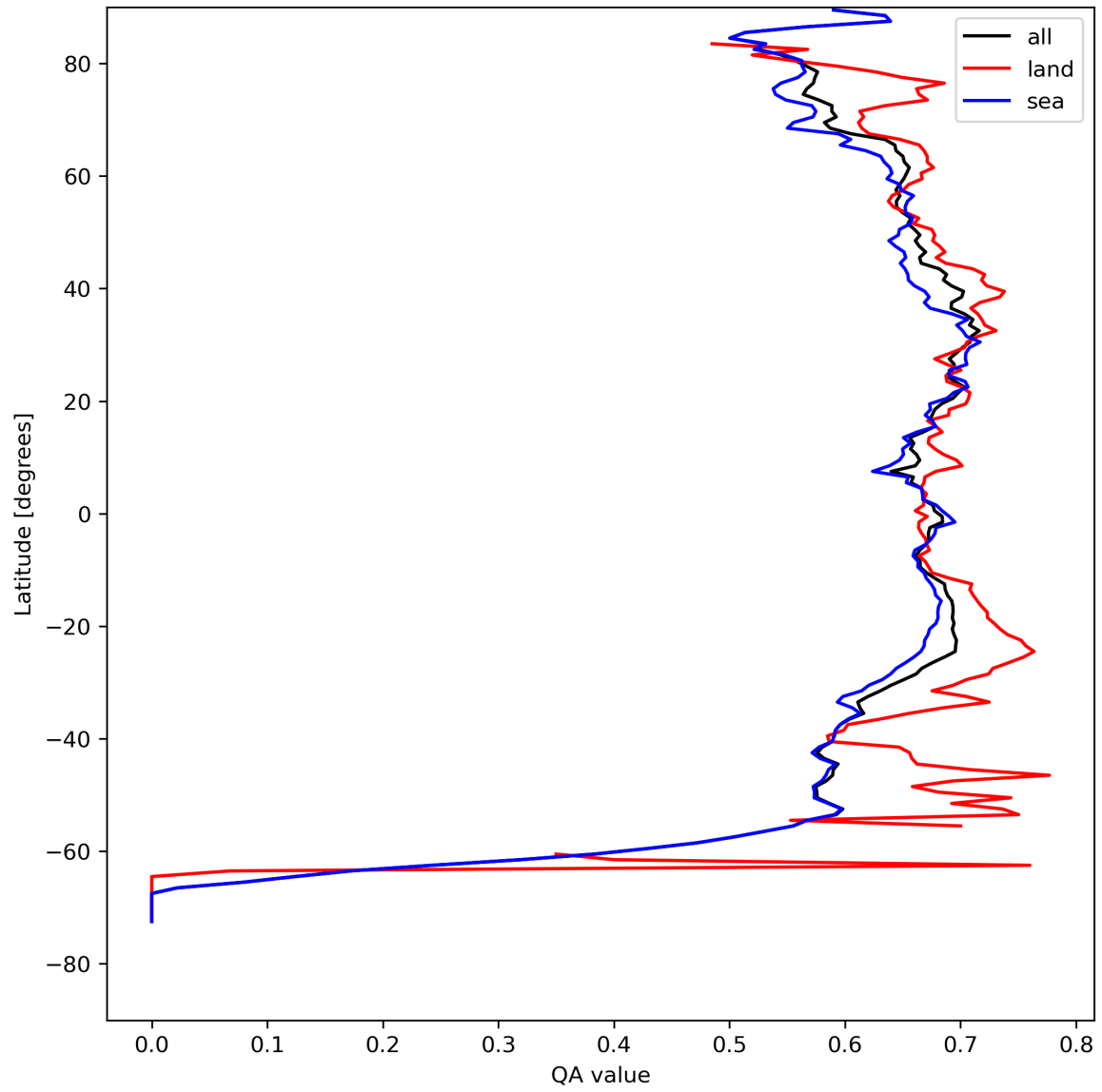
Figure 9: Zonal average of “QA value” for 2024-08-17 to 2024-08-19.
