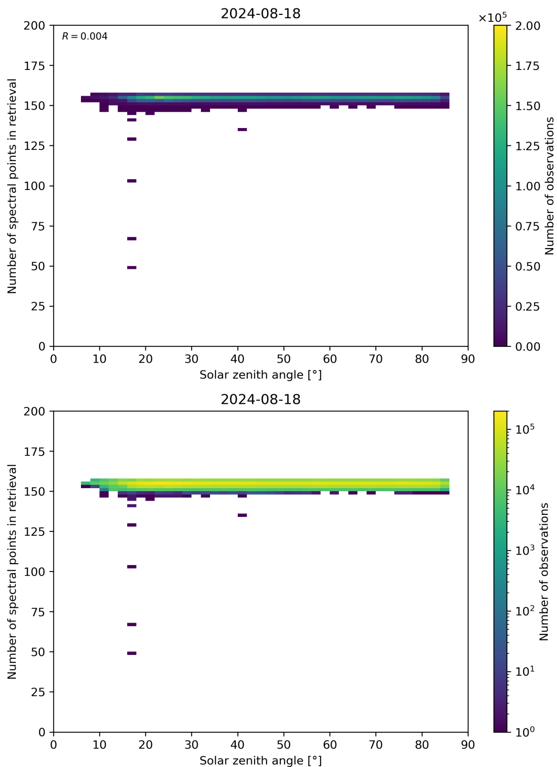
Figure 68: Scatter density plot of “Solar zenith angle” against “Number of spectral points in retrieval” for 2024-08-17 to 2024-08-19.
