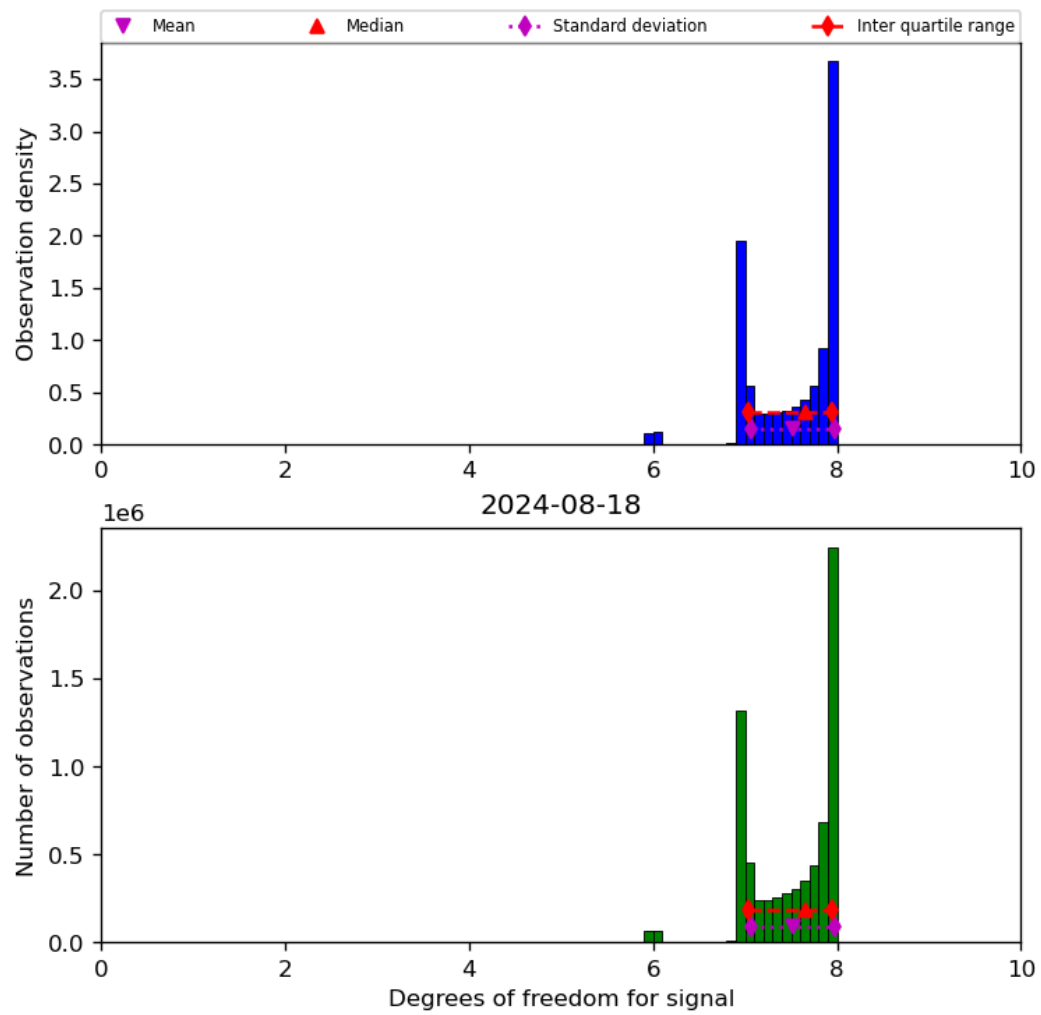
Figure 23: Histogram of “Degrees of freedom for signal” for 2024-08-17 to 2024-08-19
