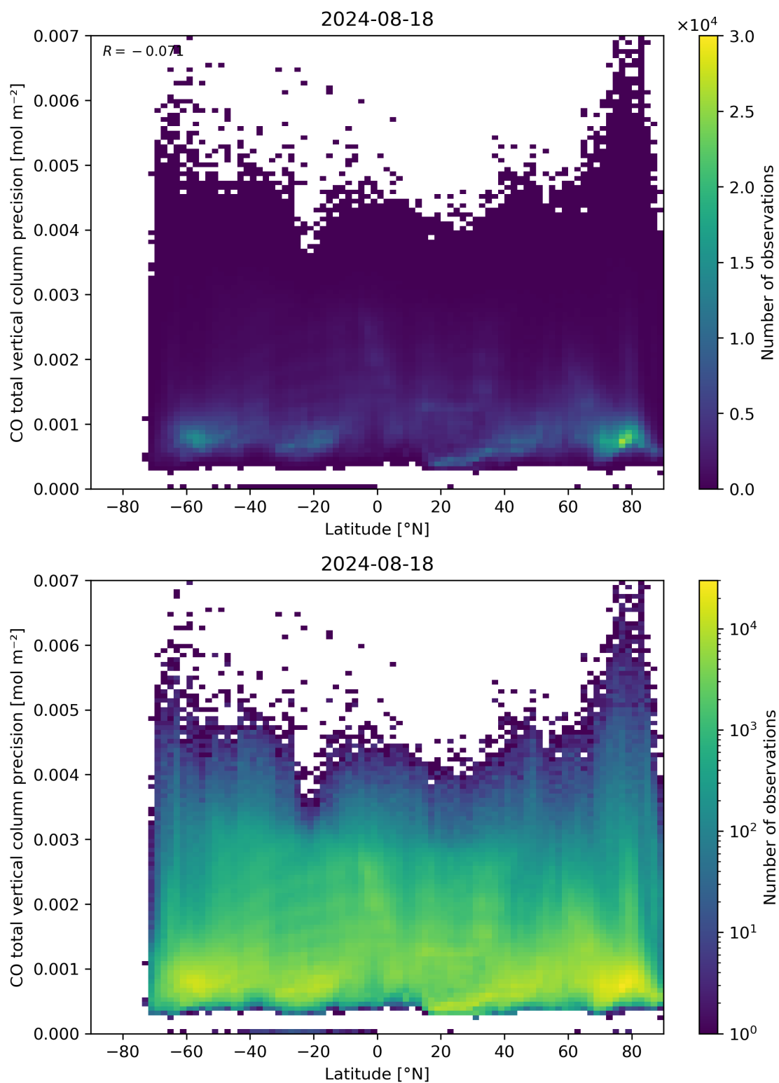
Figure 53: Scatter density plot of “Latitude” against “CO total vertical column precision” for 2024-08-17 to 2024-08-19.
