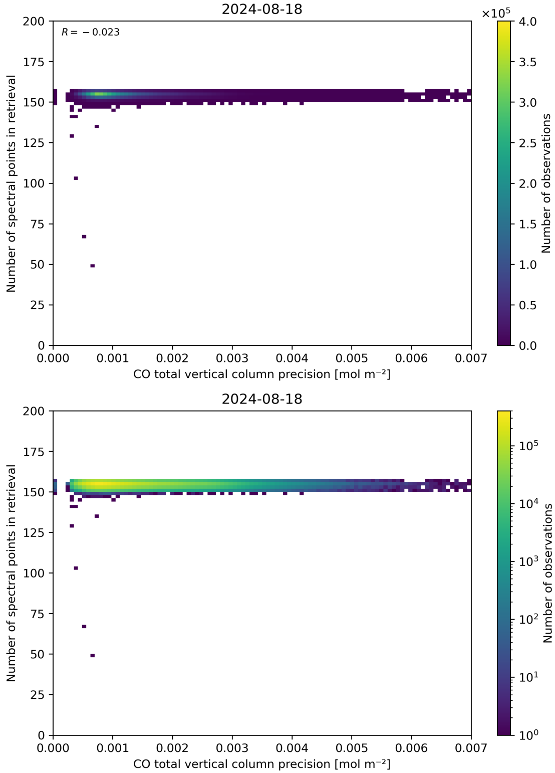
Figure 47: Scatter density plot of “CO total vertical column precision” against “Number of spectral points in retrieval” for 2024-08-17 to 2024-08-19.
