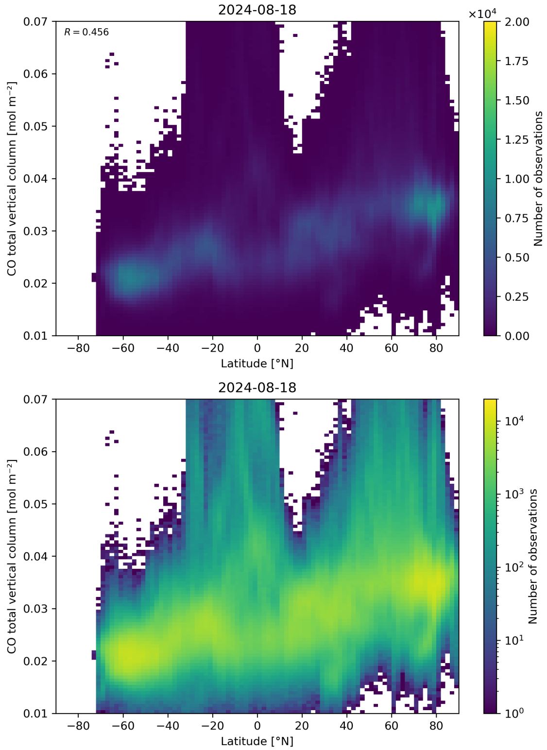
Figure 51: Scatter density plot of “Latitude” against “CO total vertical column” for 2024-08-17 to 2024-08-19.
