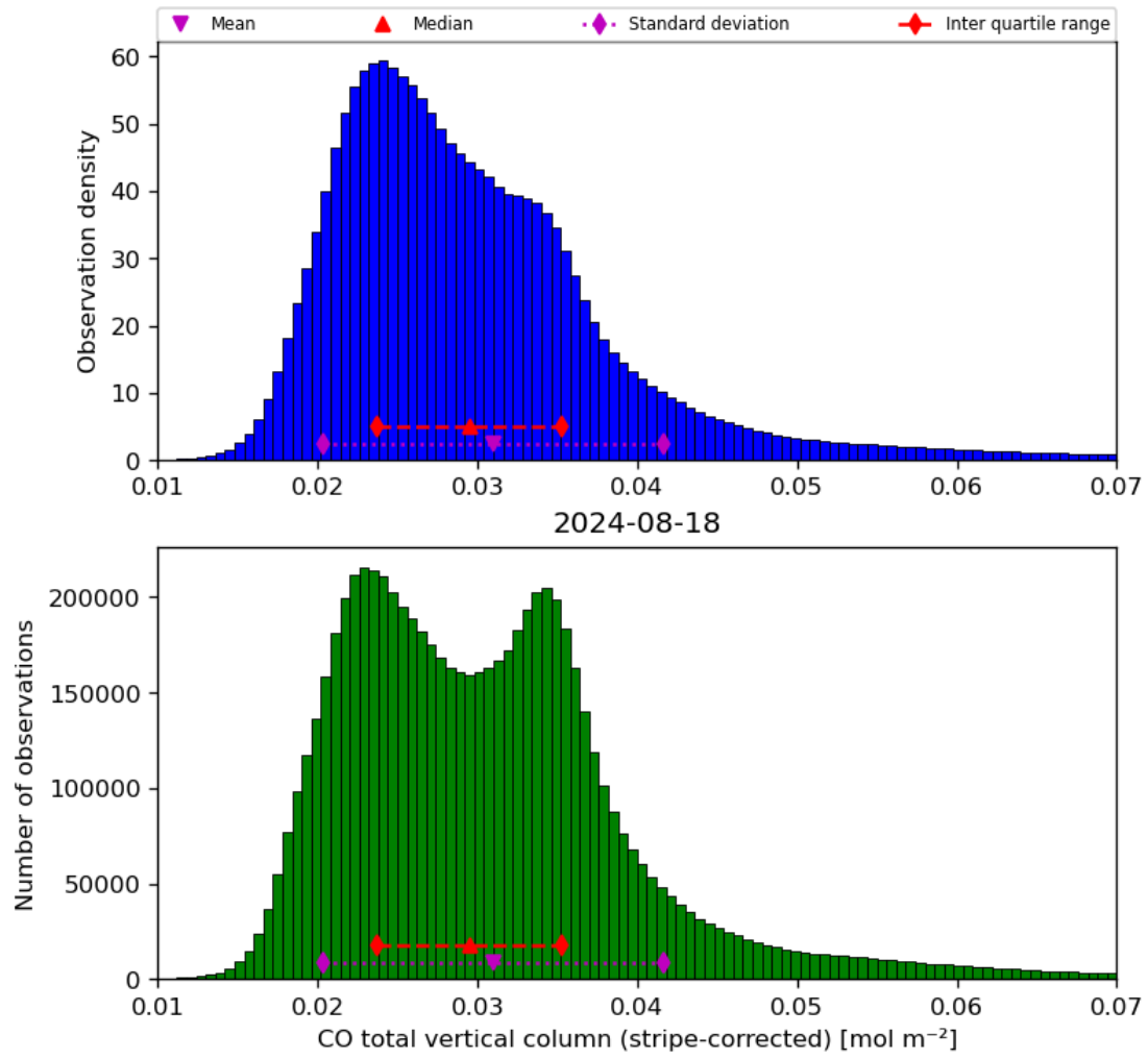
Figure 19: Histogram of “CO total vertical column (stripe-corrected)” for 2024-08-17 to 2024-08-19
