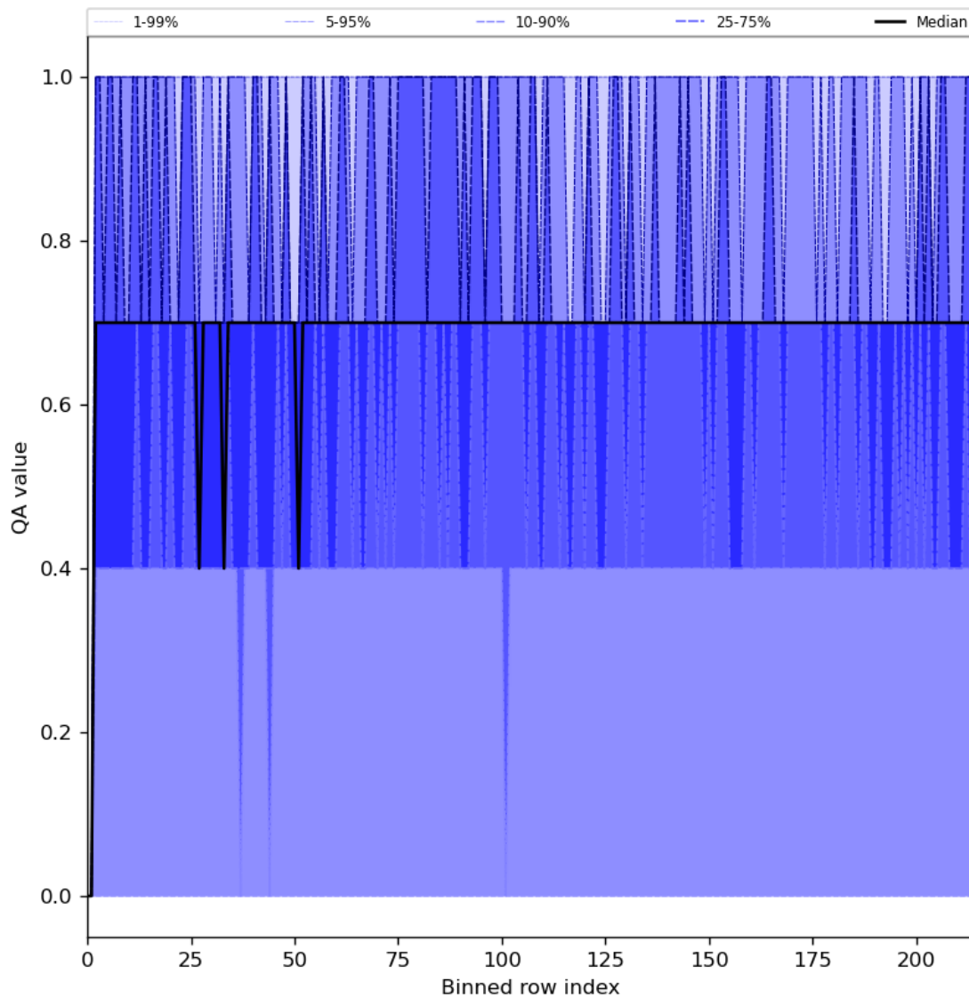
Figure 25: Along track statistics of “QA value” for 2024-08-17 to 2024-08-19
