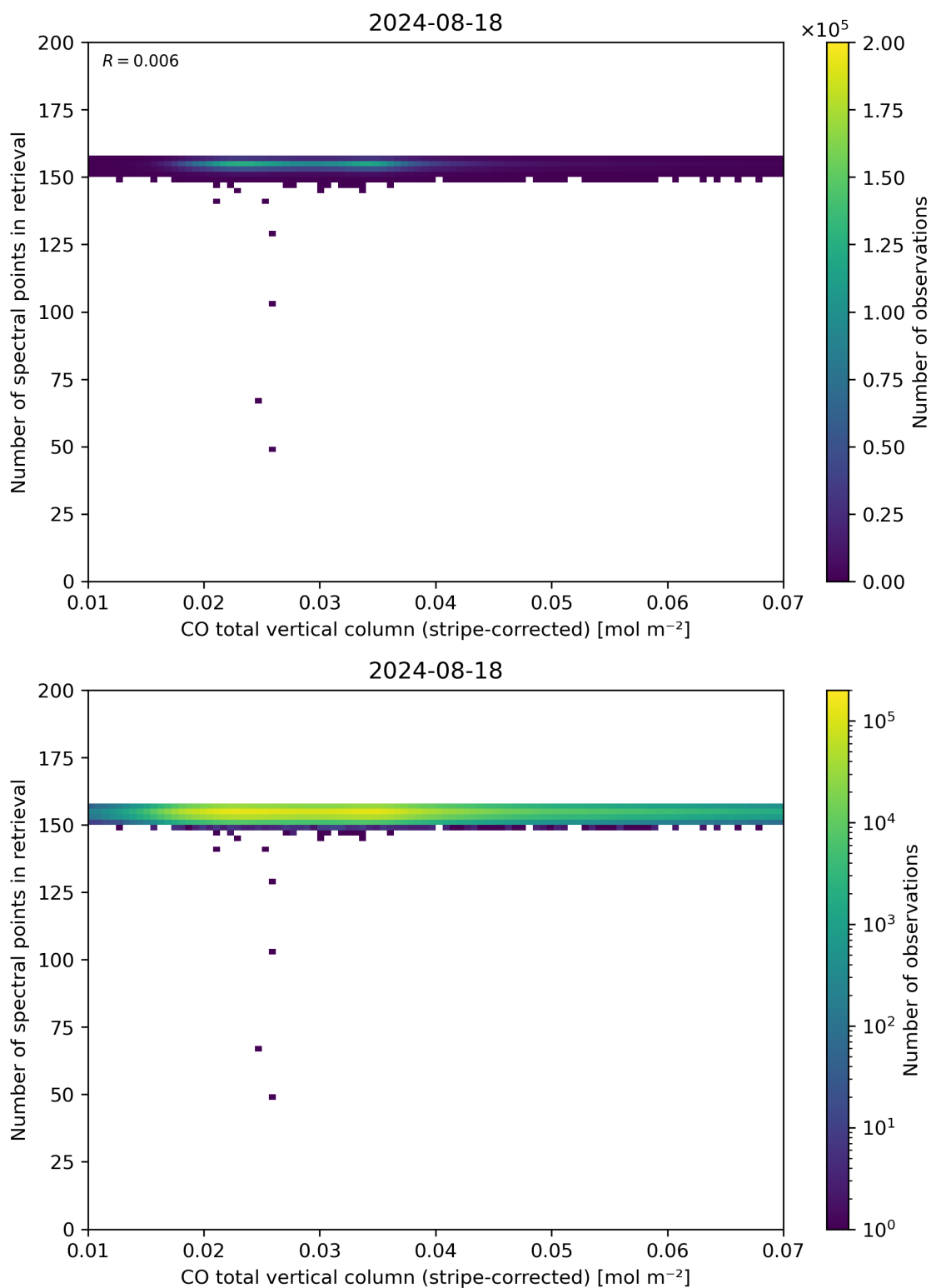
Figure 40: Scatter density plot of “CO total vertical column (stripe-corrected)” against “Number of spectral points in retrieval” for 2024-08-17 to 2024-08-19.
