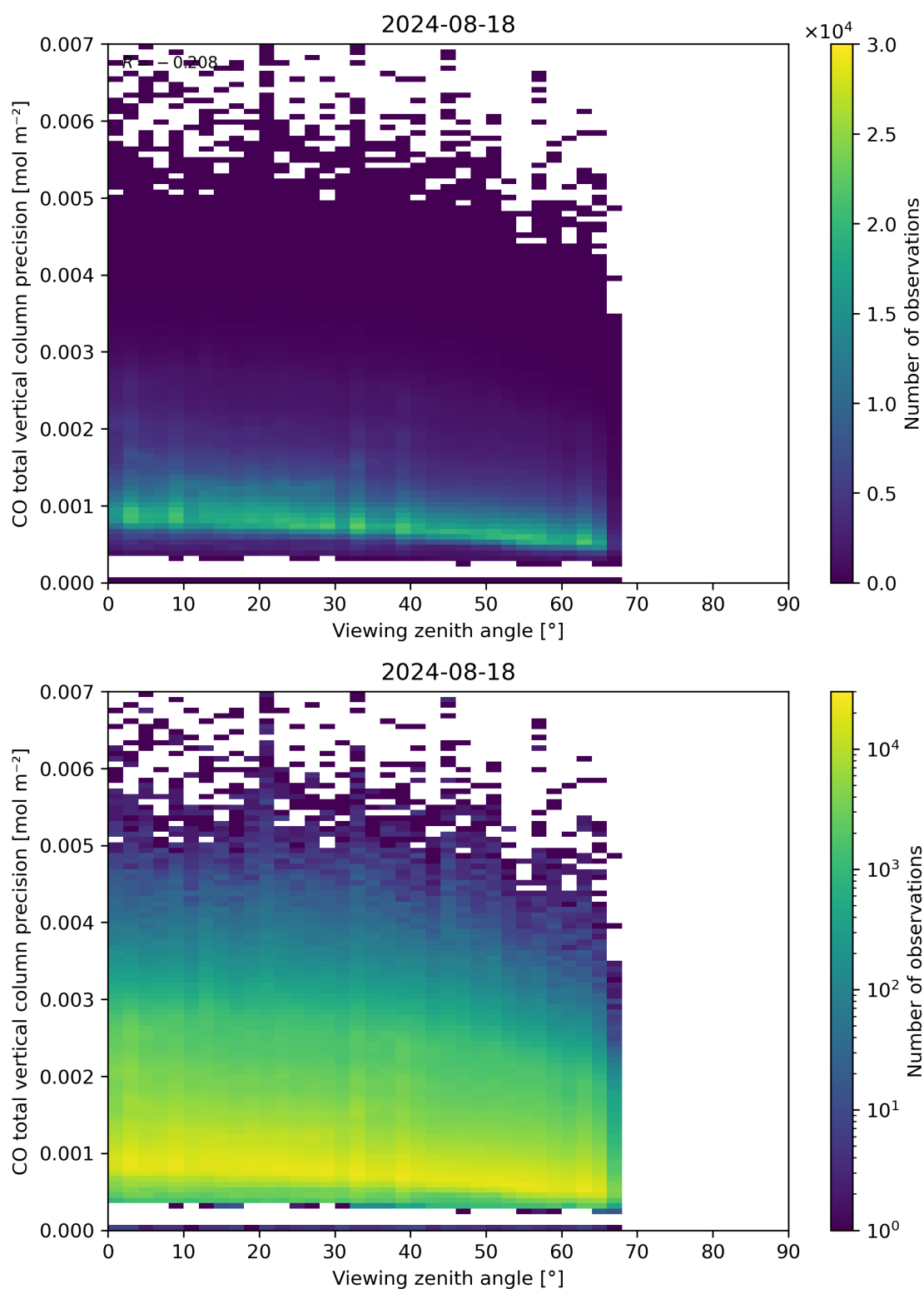
Figure 71: Scatter density plot of “Viewing zenith angle” against “CO total vertical column precision” for 2024-08-17 to 2024-08-19.
