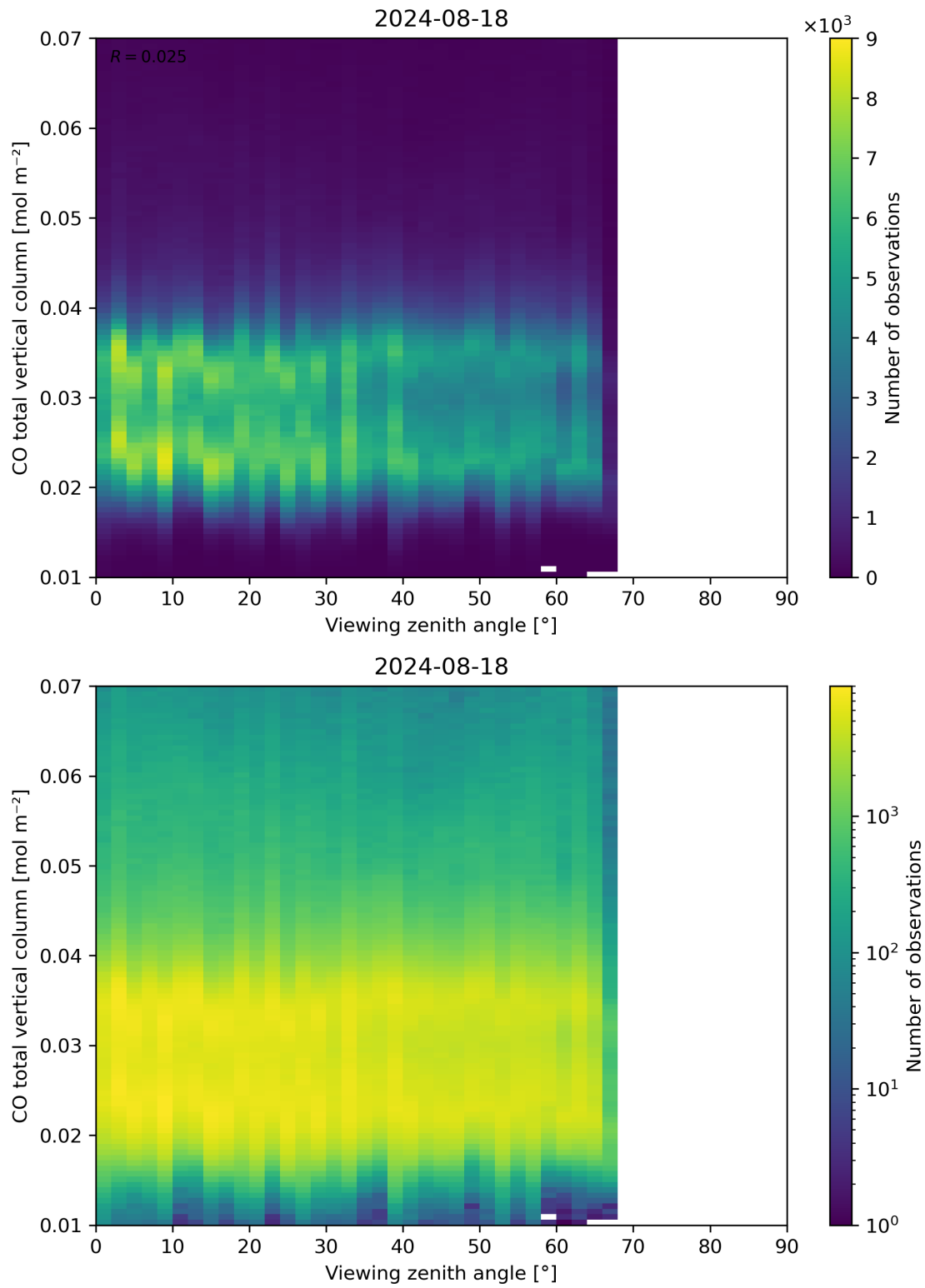
Figure 69: Scatter density plot of “Viewing zenith angle” against “CO total vertical column” for 2024-08-17 to 2024-08-19.
