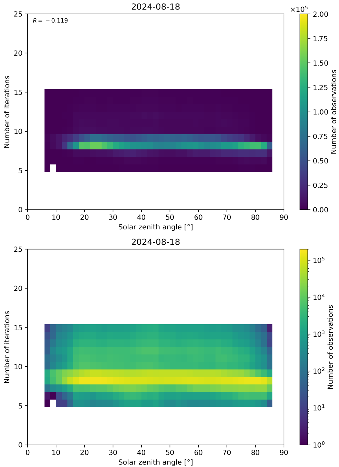
Figure 67: Scatter density plot of “Solar zenith angle” against “Number of iterations” for 2024-08-17 to 2024-08-19.
