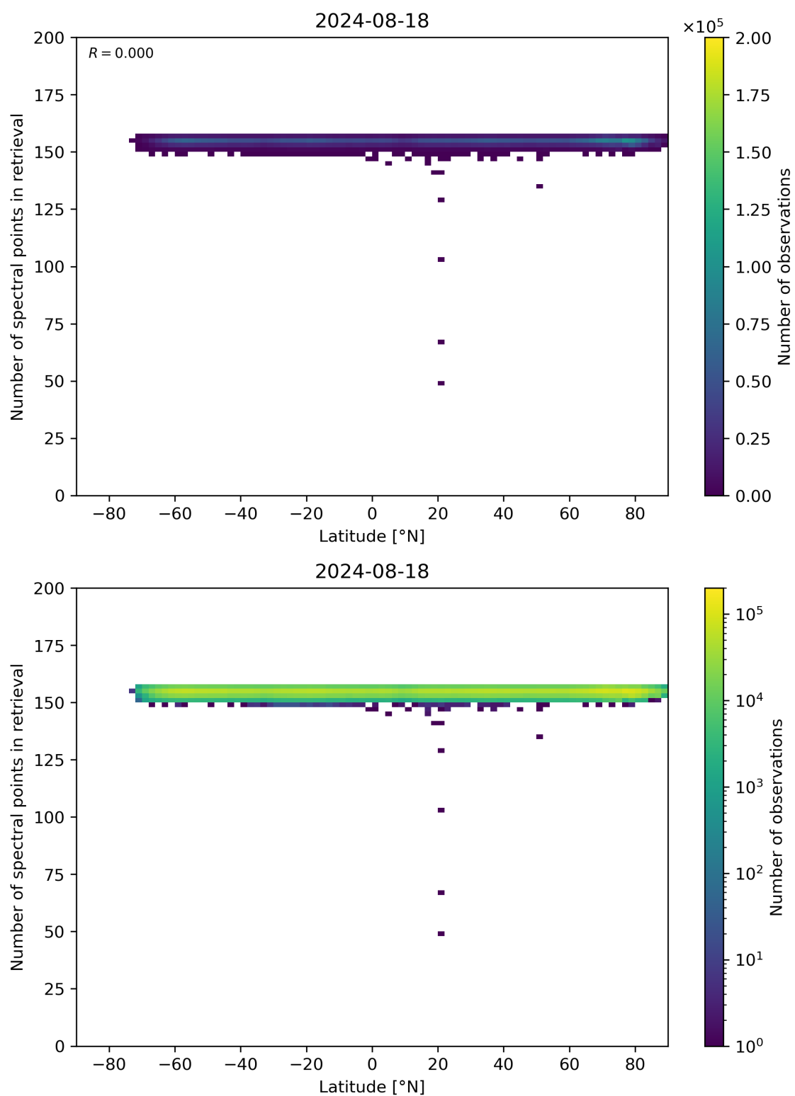
Figure 57: Scatter density plot of “Latitude” against “Number of spectral points in retrieval” for 2024-08-17 to 2024-08-19.
