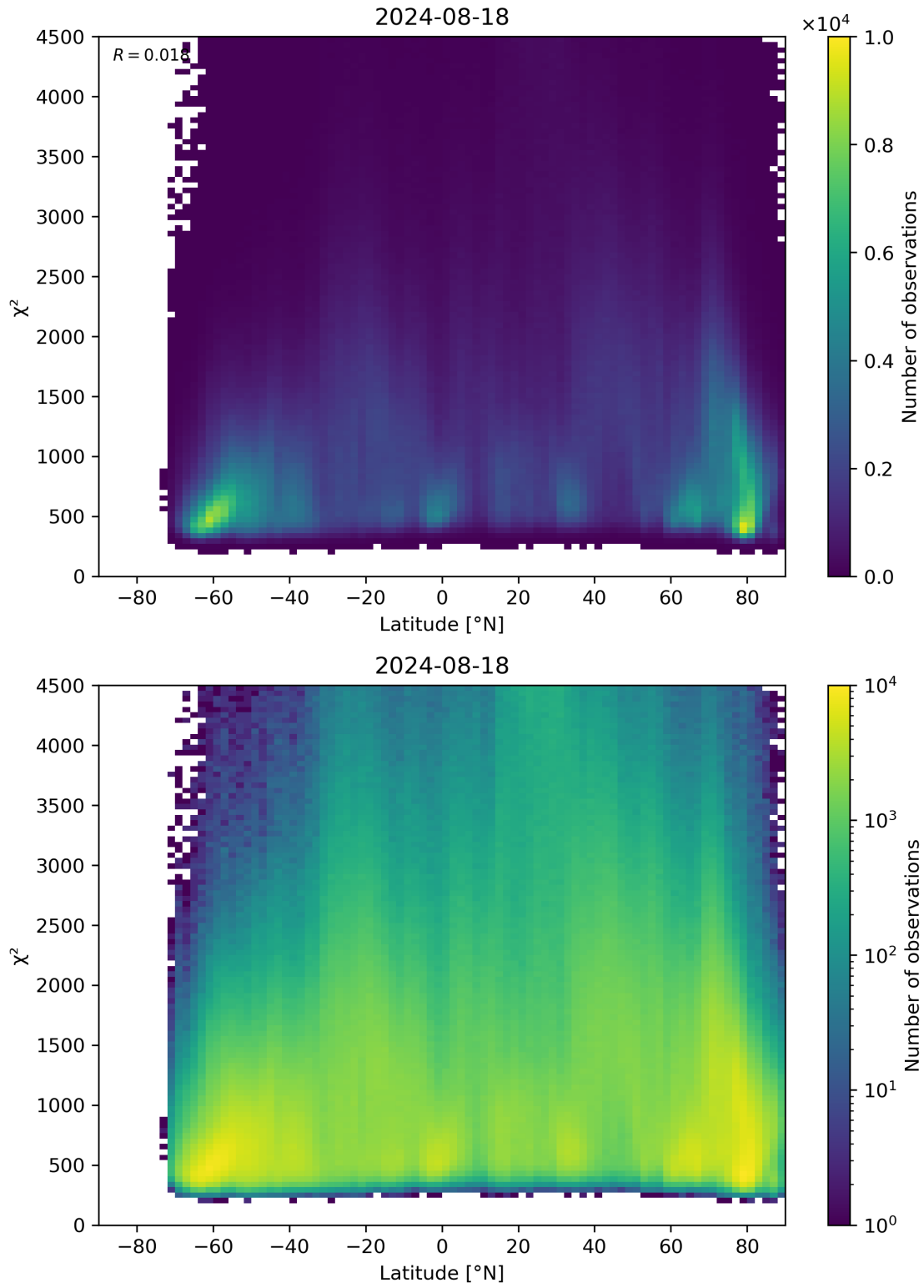
Figure 54: Scatter density plot of “Latitude” against “ \chi^2 ” for 2024-08-17 to 2024-08-19.
