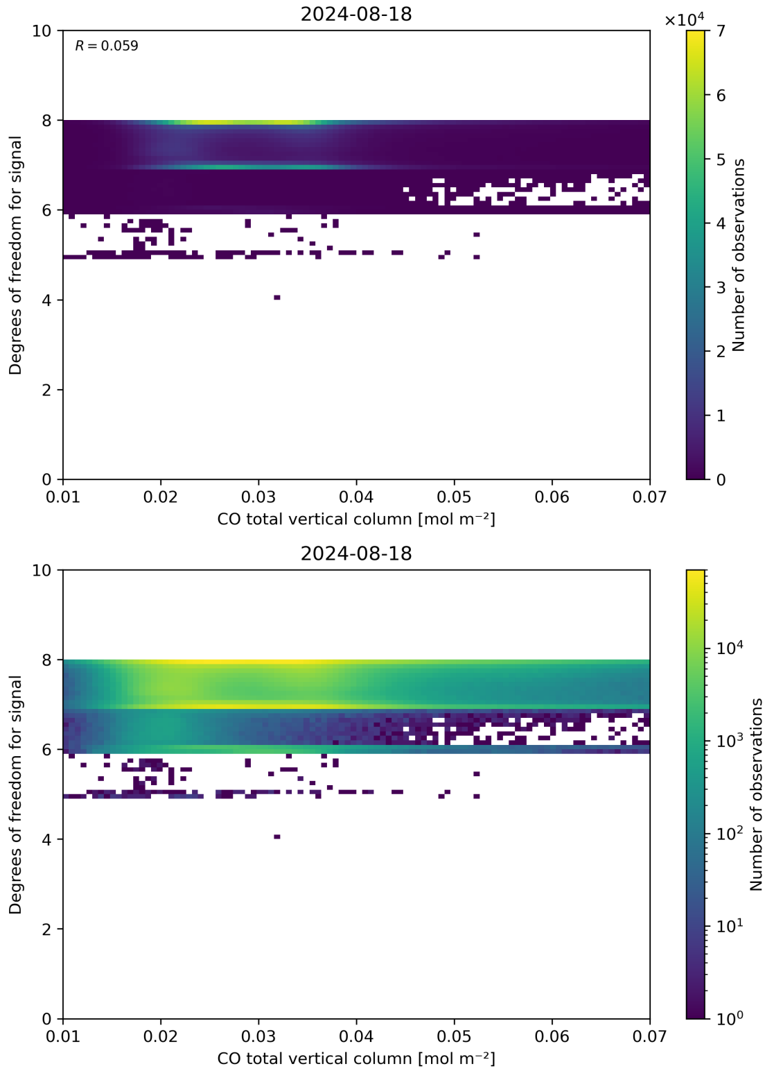
Figure 41: Scatter density plot of “CO total vertical column” against “Degrees of freedom for signal” for 2024-08-17 to 2024-08-19.
