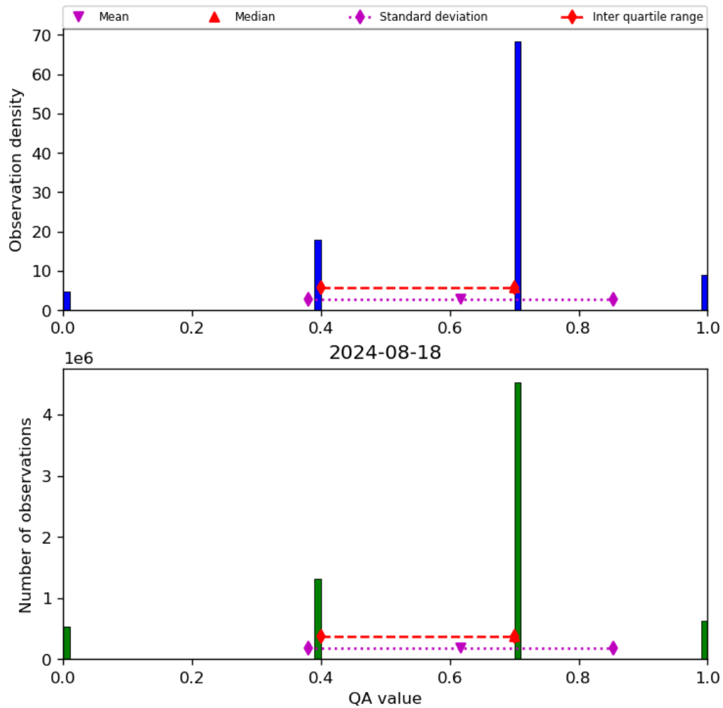
Figure 17: Histogram of “QA value” for 2024-08-17 to 2024-08-19
