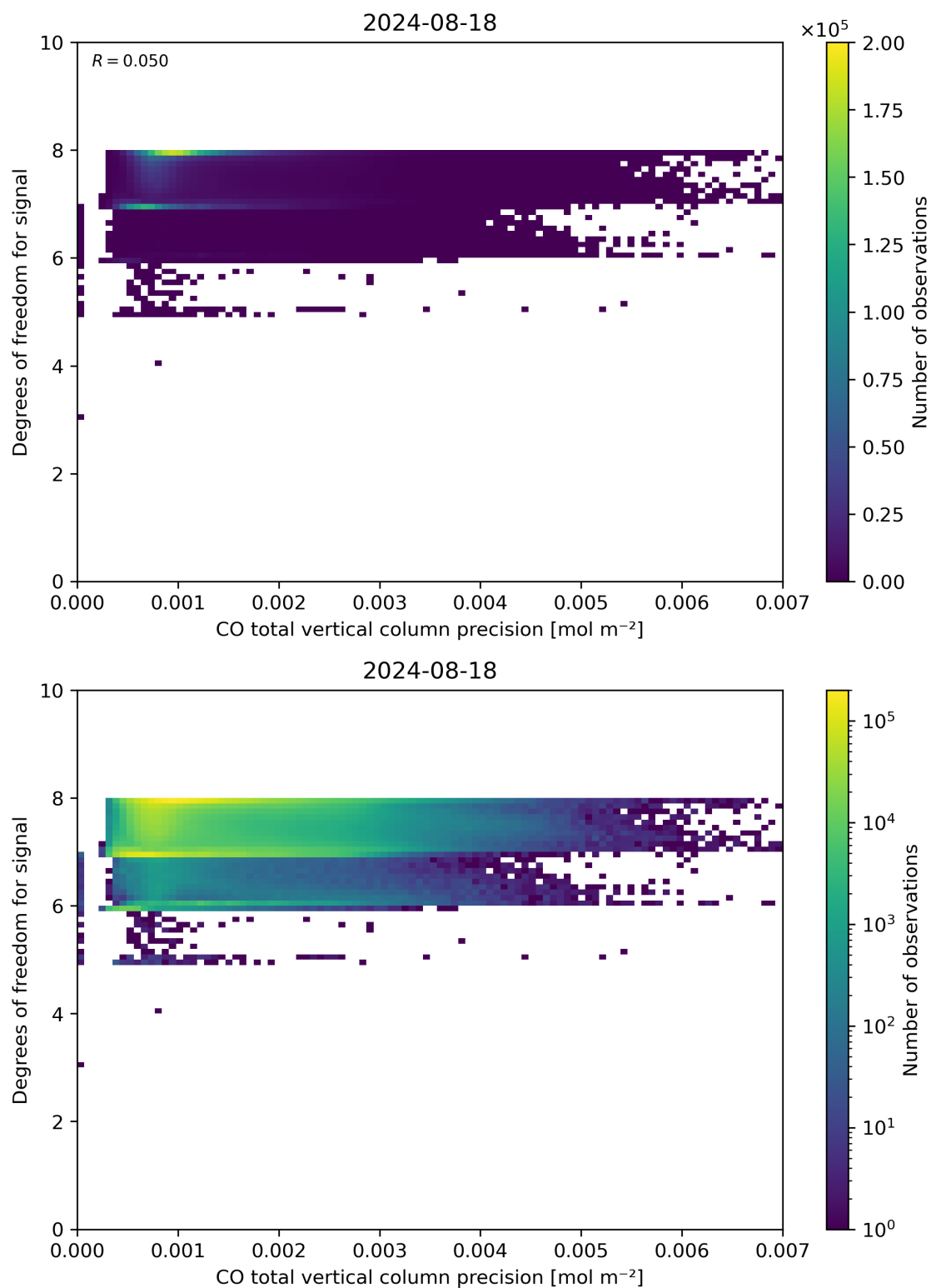
Figure 45: Scatter density plot of “CO total vertical column precision” against “Degrees of freedom for signal” for 2024-08-17 to 2024-08-19.
