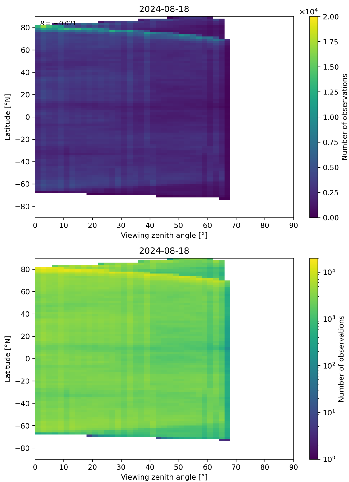
Figure 74: Scatter density plot of “Viewing zenith angle” against “Latitude” for 2024-08-17 to 2024-08-19.
