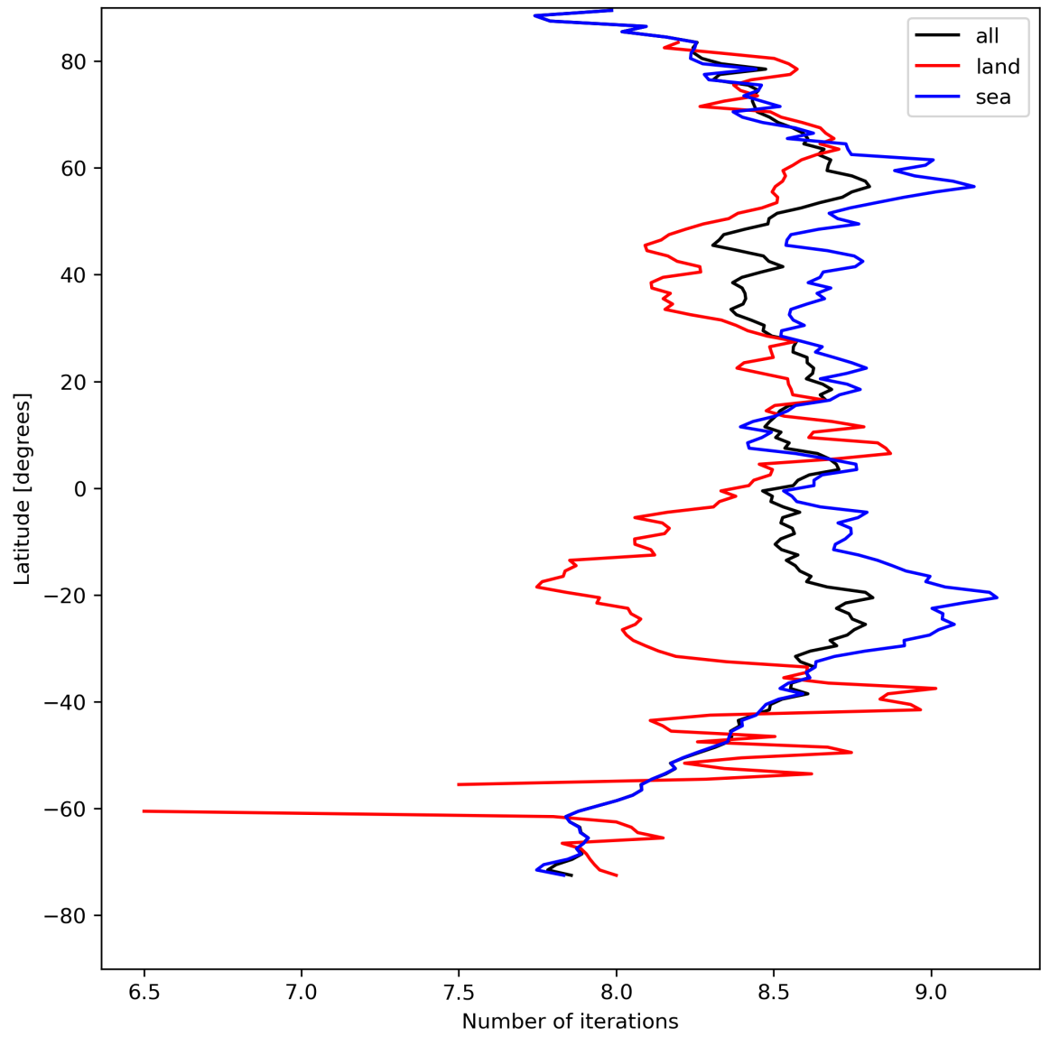
Figure 16: Zonal average of “Number of iterations” for 2024-08-17 to 2024-08-19.
