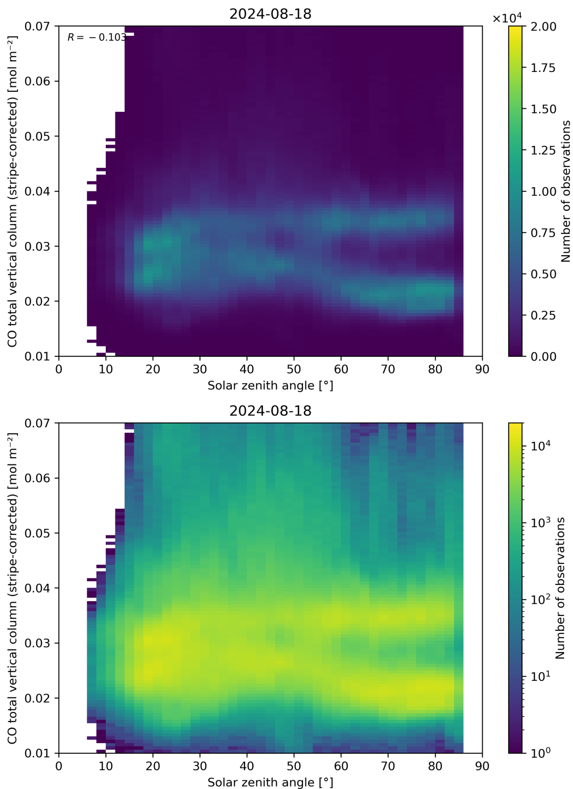
Figure 62: Scatter density plot of “Solar zenith angle” against “CO total vertical column (stripe-corrected)” for 2024-08-17 to 2024-08-19.
