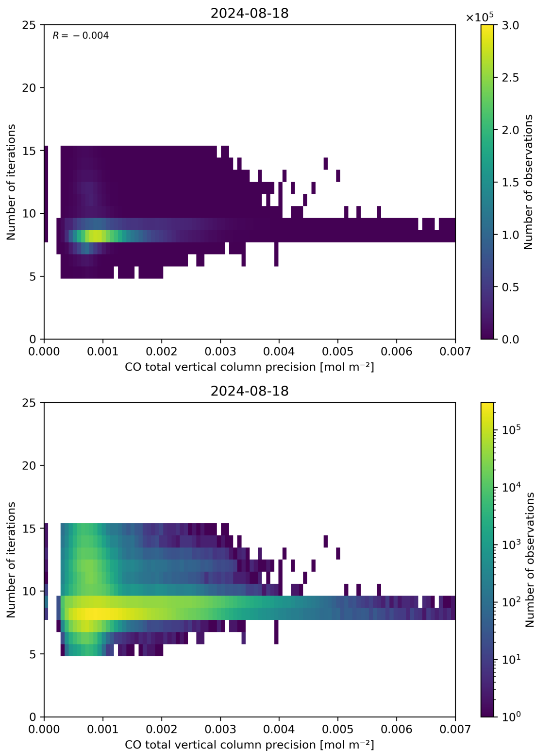
Figure 46: Scatter density plot of “CO total vertical column precision” against “Number of iterations” for 2024-08-17 to 2024-08-19.
