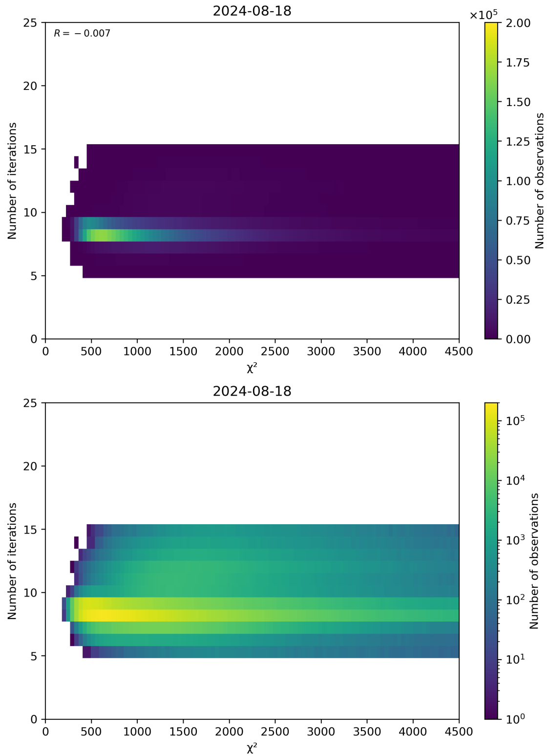
Figure 49: Scatter density plot of “ \chi^2 ” against “Number of iterations” for 2024-08-17 to 2024-08-19.
