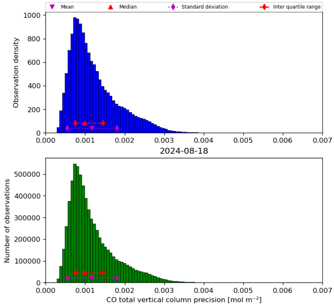
Figure 20: Histogram of “CO total vertical column precision” for 2024-08-17 to 2024-08-19
