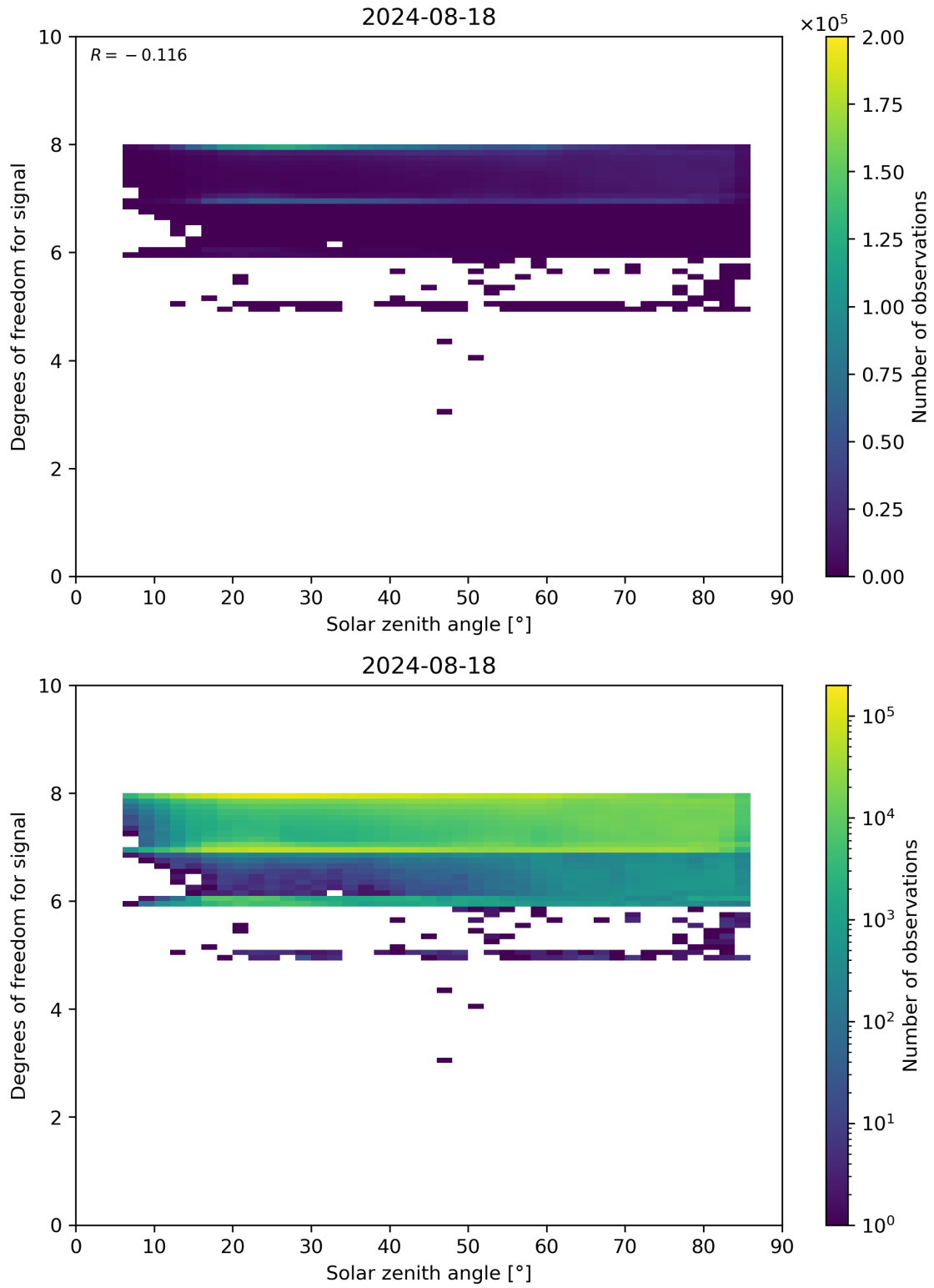
Figure 65: Scatter density plot of “Solar zenith angle” against “Degrees of freedom for signal” for 2024-08-17 to 2024-08-19.
