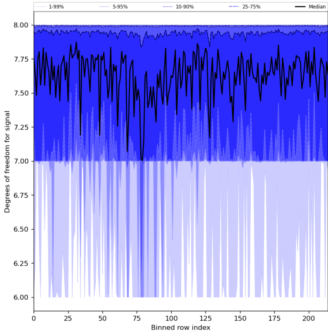
Figure 31: Along track statistics of “Degrees of freedom for signal” for 2024-08-17 to 2024-08-19
