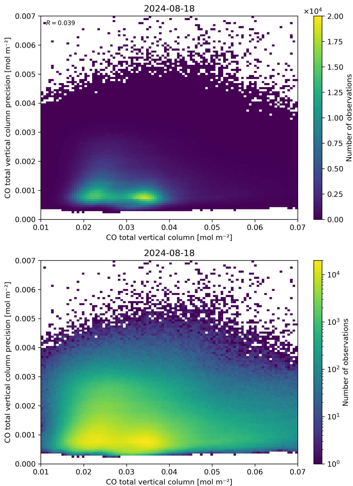
Figure 34: Scatter density plot of “CO total vertical column” against “CO total vertical column precision” for 2024-08-17 to 2024-08-19.
