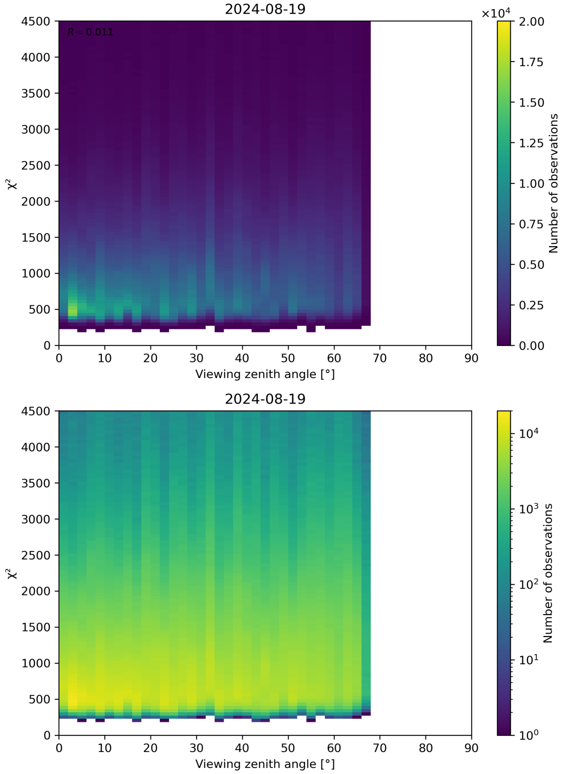
Figure 72: Scatter density plot of “Viewing zenith angle” against “ \chi^2 ” for 2024-08-18 to 2024-08-20.
