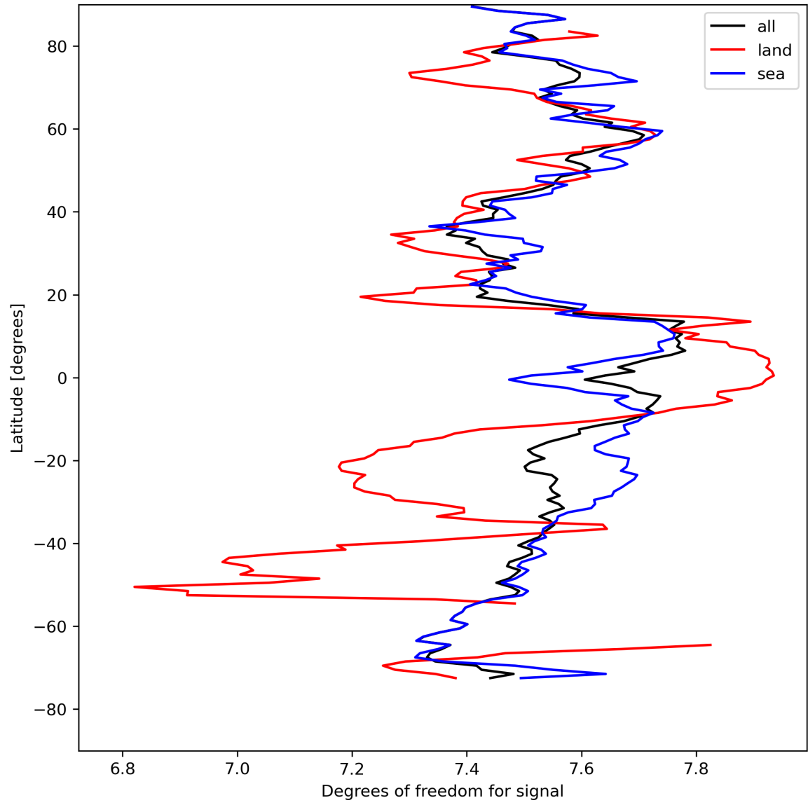
Figure 15: Zonal average of “Degrees of freedom for signal” for 2024-08-18 to 2024-08-20.
