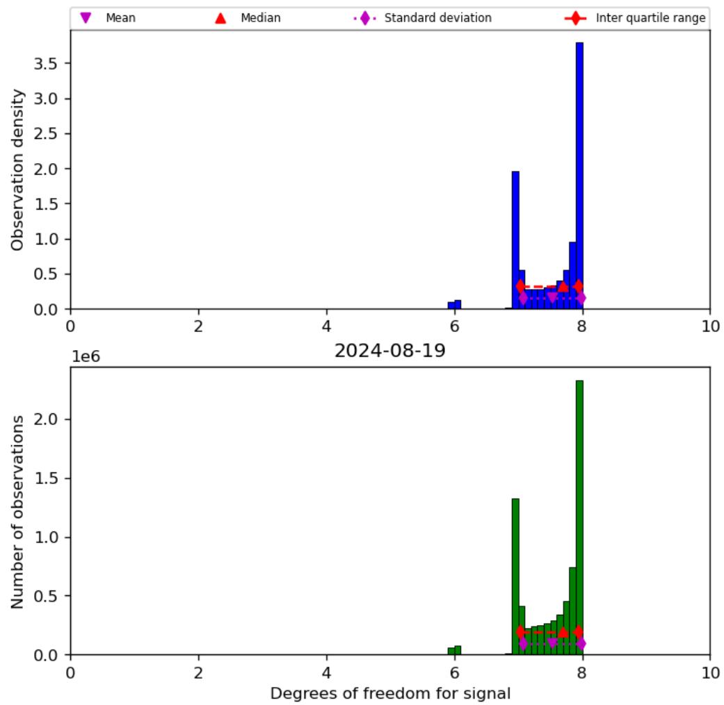
Figure 23: Histogram of “Degrees of freedom for signal” for 2024-08-18 to 2024-08-20
