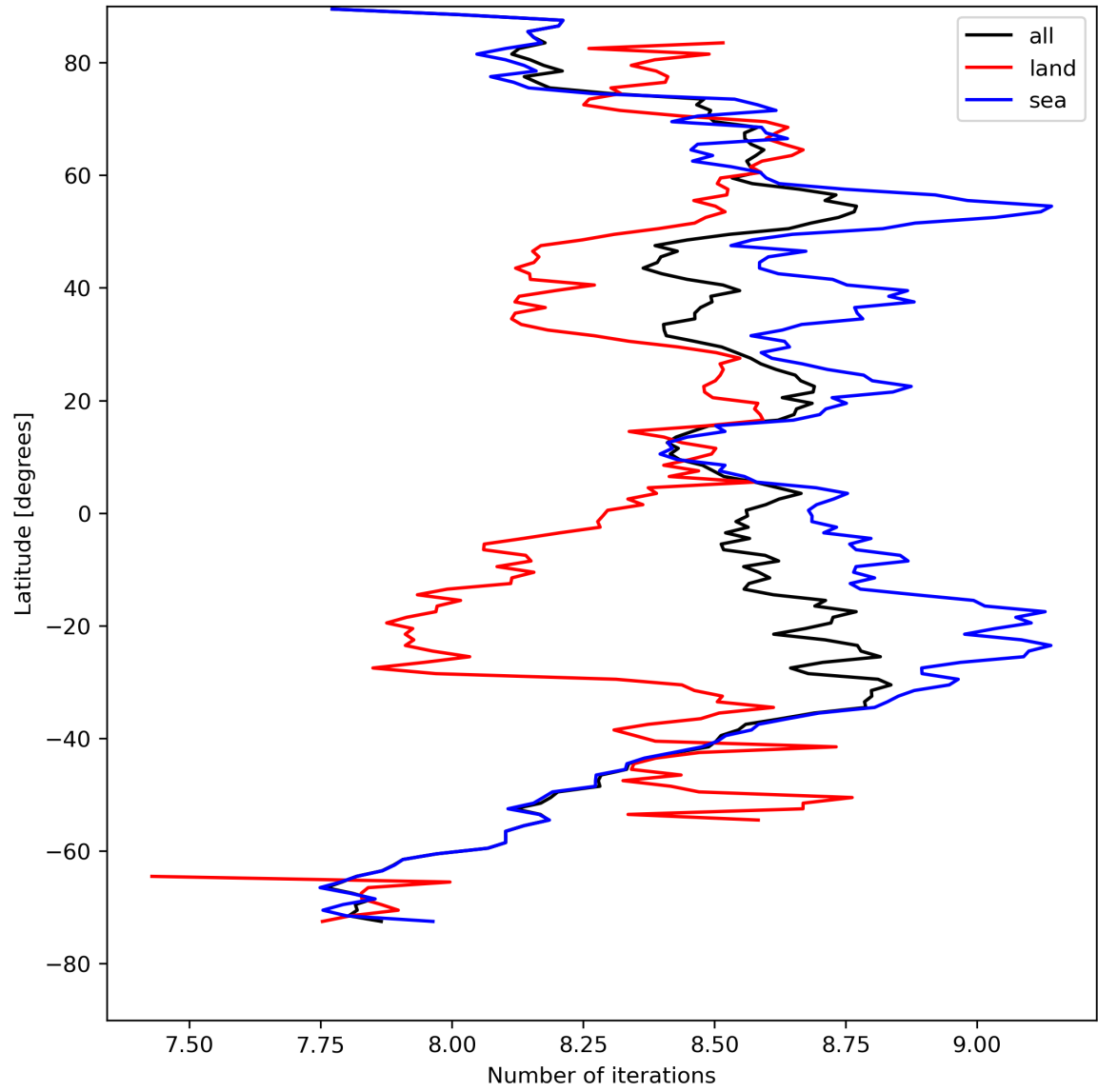
Figure 16: Zonal average of “Number of iterations” for 2024-08-18 to 2024-08-20.
