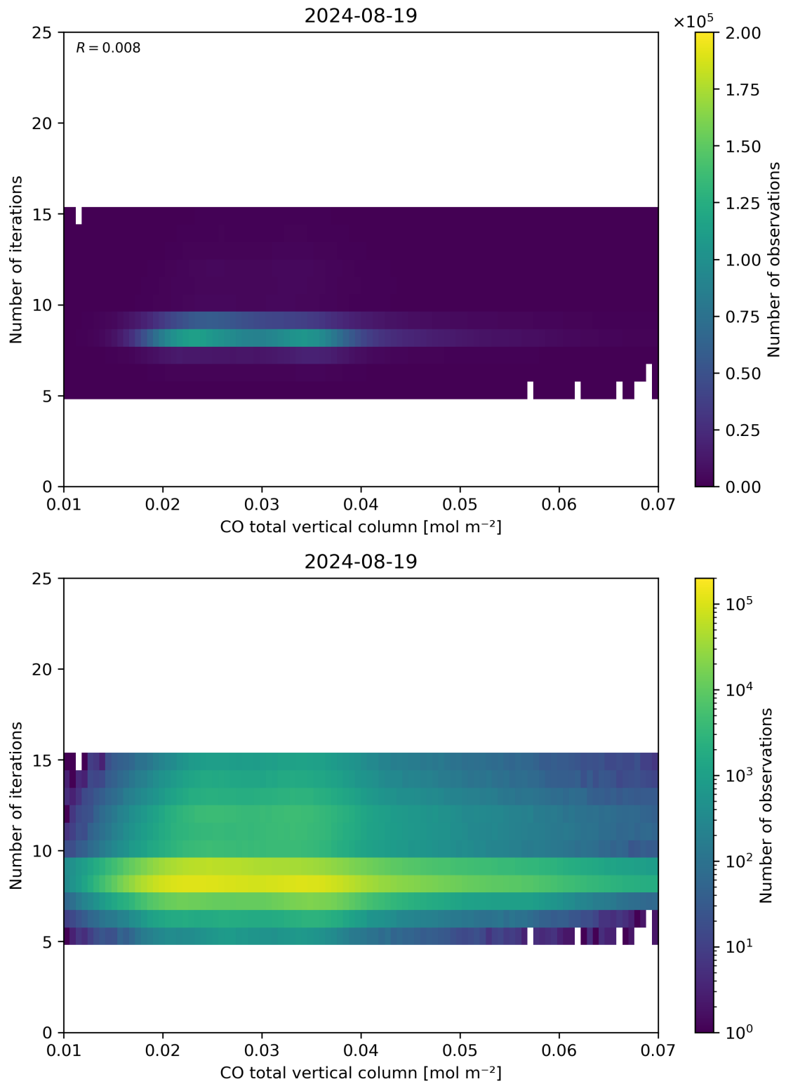
Figure 42: Scatter density plot of “CO total vertical column” against “Number of iterations” for 2024-08-18 to 2024-08-20.
