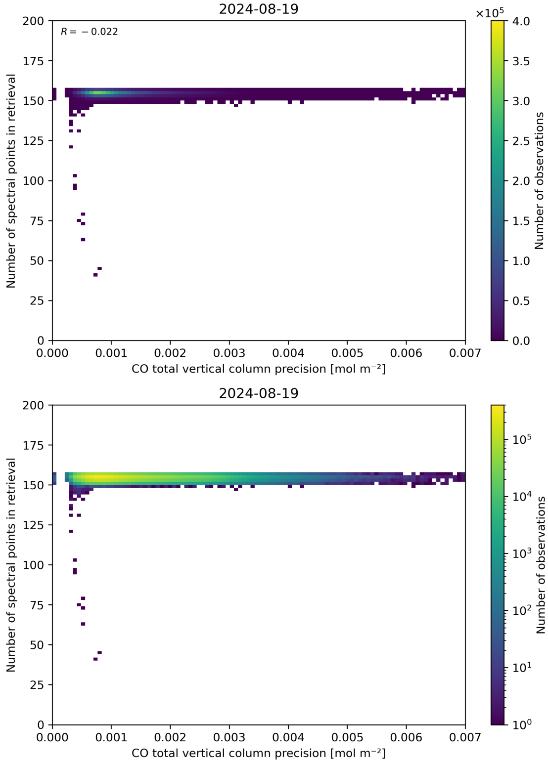
Figure 47: Scatter density plot of “CO total vertical column precision” against “Number of spectral points in retrieval” for 2024-08-18 to 2024-08-20.
