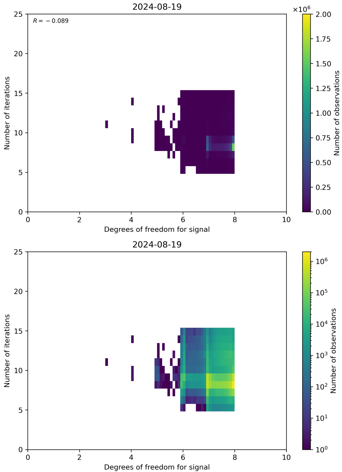
Figure 50: Scatter density plot of “Degrees of freedom for signal” against “Number of iterations” for 2024-08-18 to 2024-08-20.
