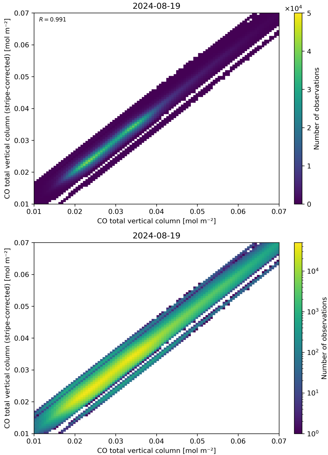
Figure 33: Scatter density plot of “CO total vertical column” against “CO total vertical column (stripe-corrected)” for 2024-08-18 to 2024-08-20.
