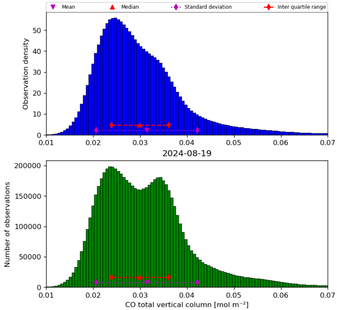
Figure 18: Histogram of “CO total vertical column” for 2024-08-18 to 2024-08-20
