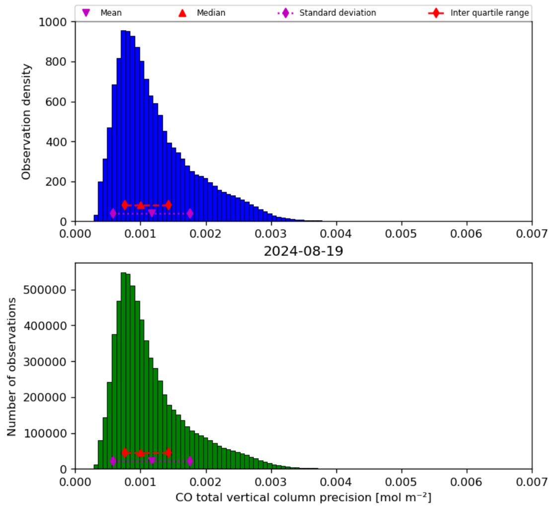
Figure 20: Histogram of “CO total vertical column precision” for 2024-08-18 to 2024-08-20
