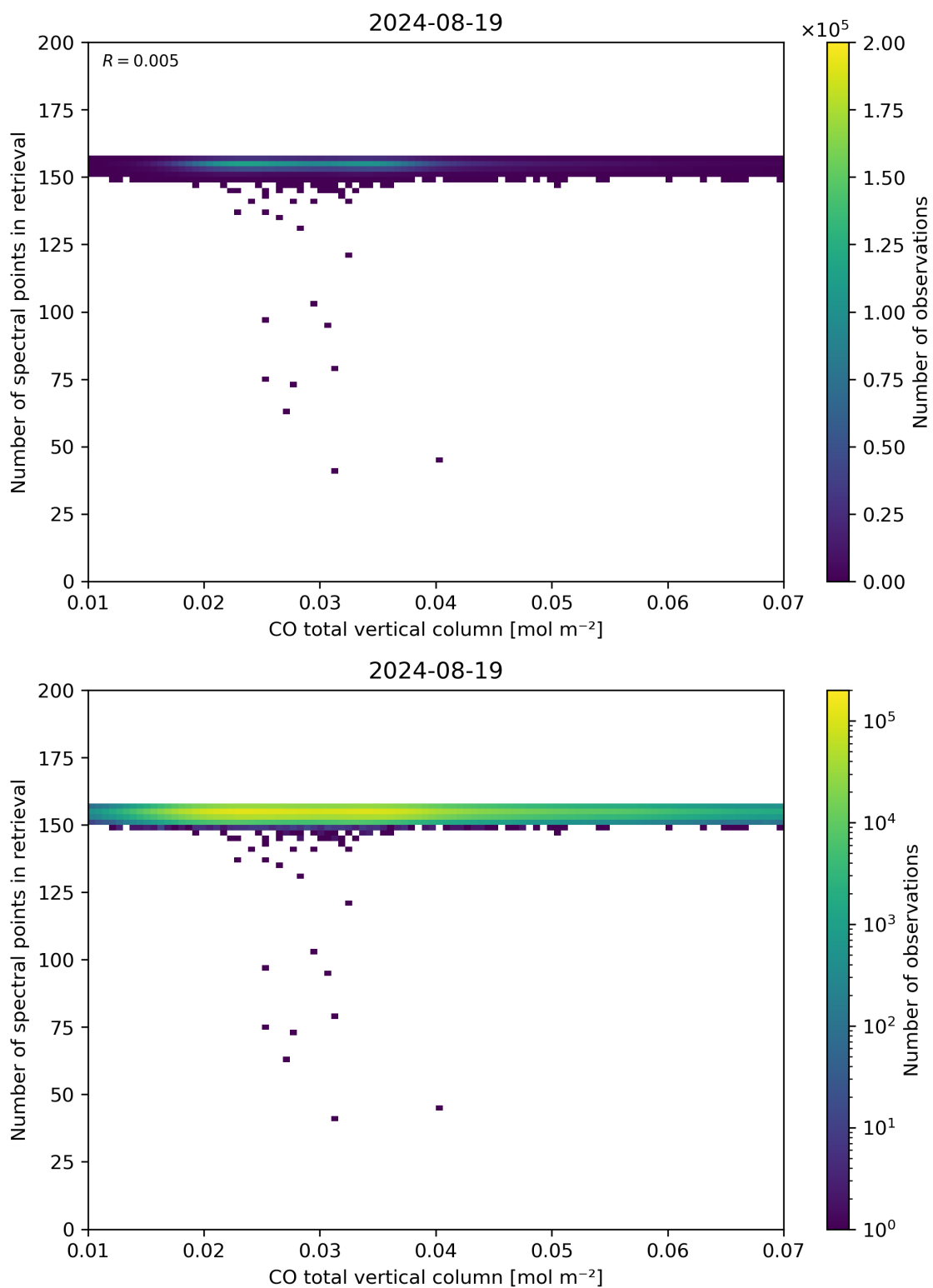
Figure 43: Scatter density plot of “CO total vertical column” against “Number of spectral points in retrieval” for 2024-08-18 to 2024-08-20.
