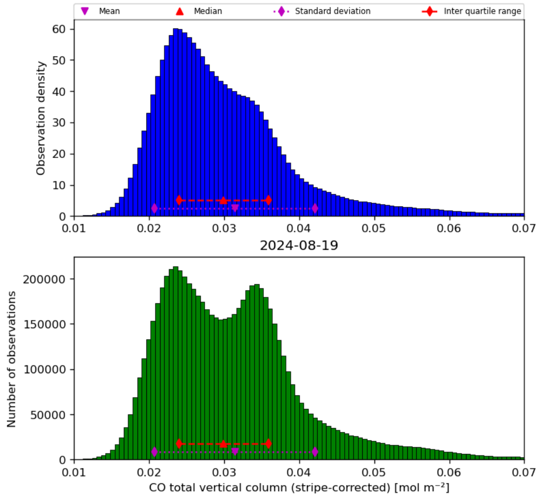
Figure 19: Histogram of “CO total vertical column (stripe-corrected)” for 2024-08-18 to 2024-08-20
