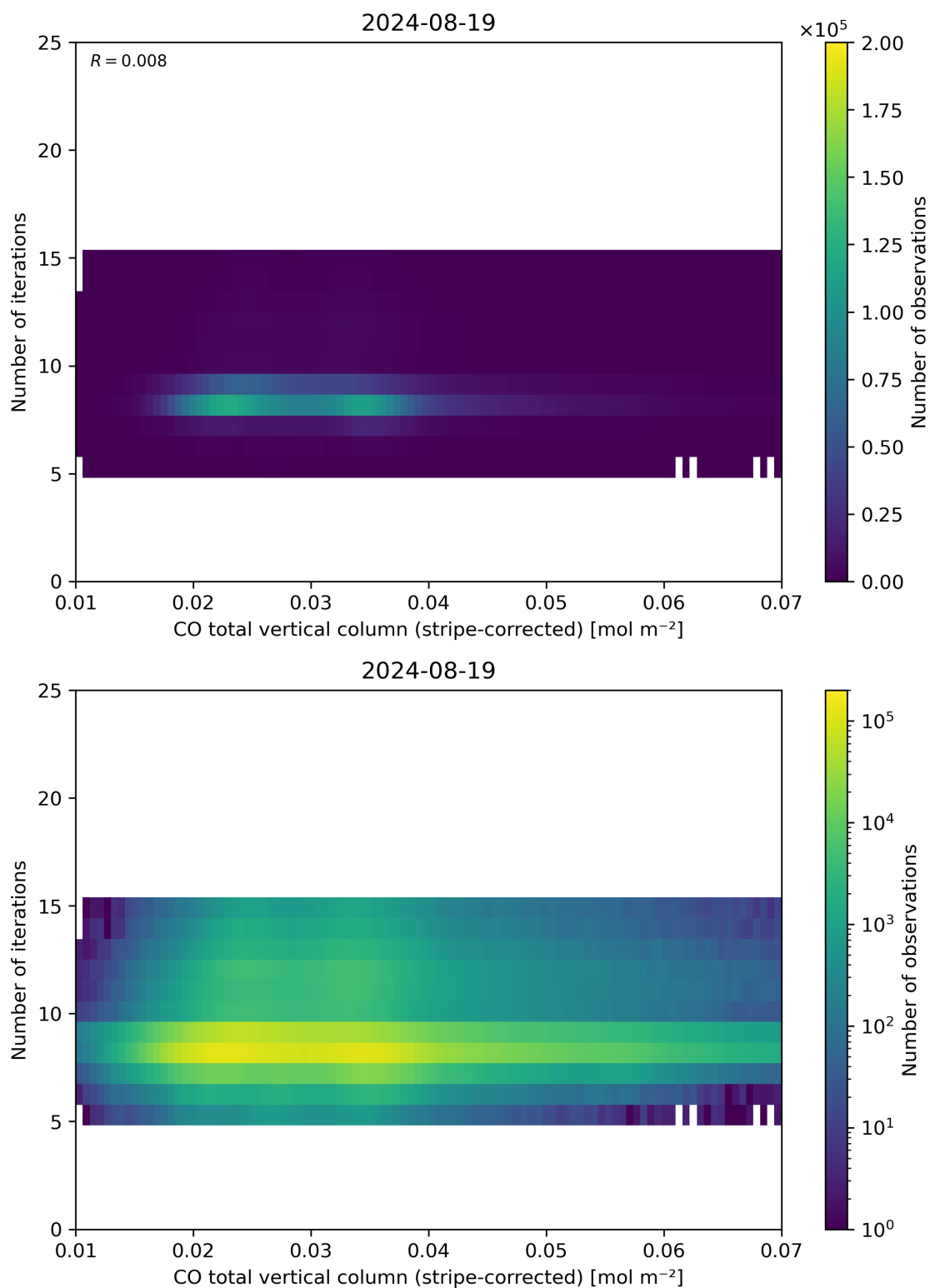
Figure 39: Scatter density plot of “CO total vertical column (stripe-corrected)” against “Number of iterations” for 2024-08-18 to 2024-08-20.
