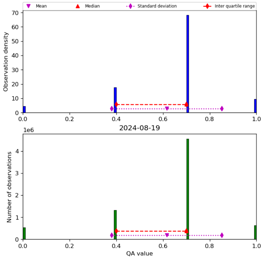
Figure 17: Histogram of “QA value” for 2024-08-18 to 2024-08-20
