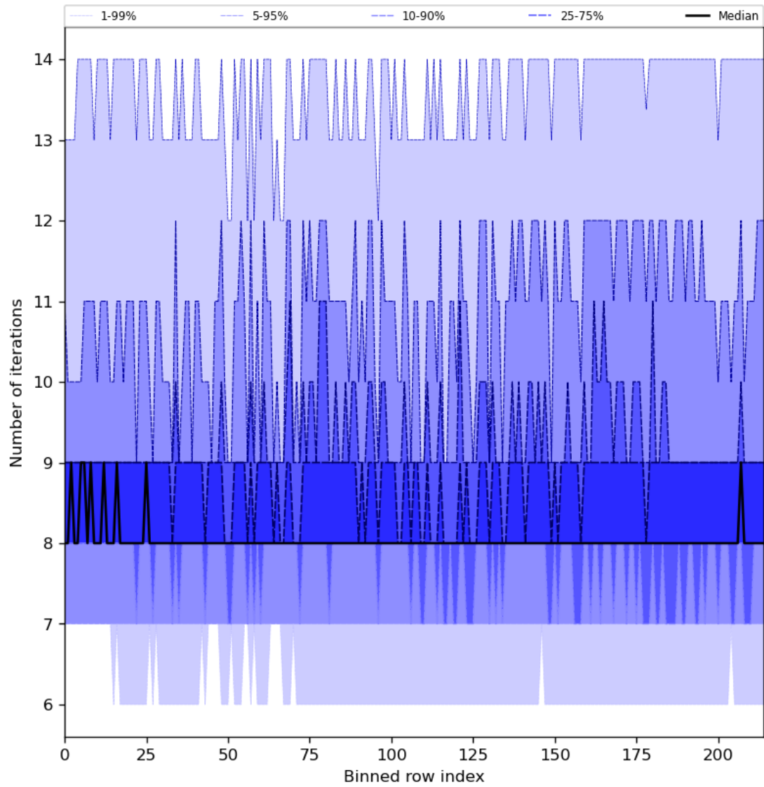
Figure 32: Along track statistics of “Number of iterations” for 2024-08-18 to 2024-08-20
