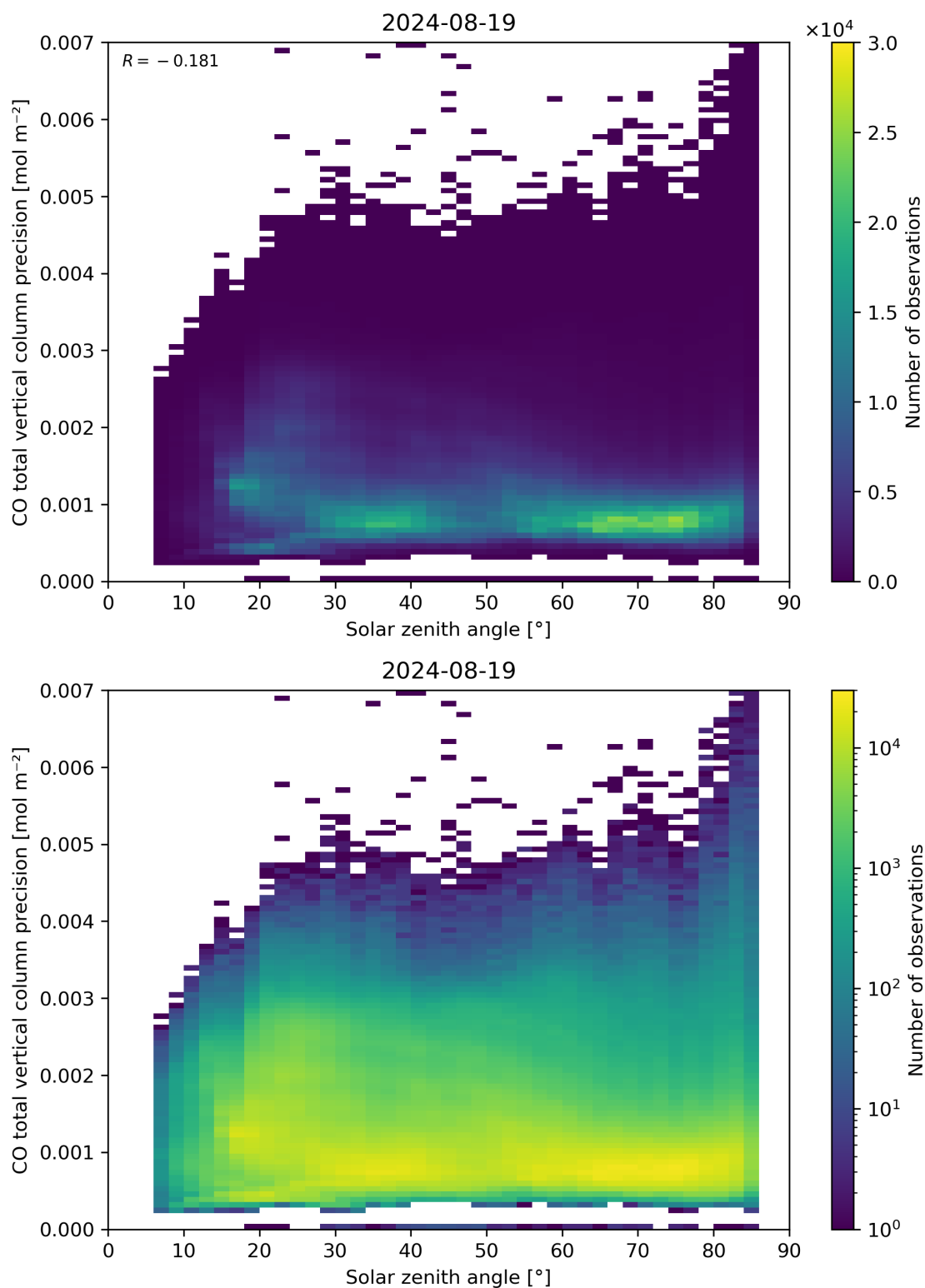
Figure 63: Scatter density plot of “Solar zenith angle” against “CO total vertical column precision” for 2024-08-18 to 2024-08-20.
