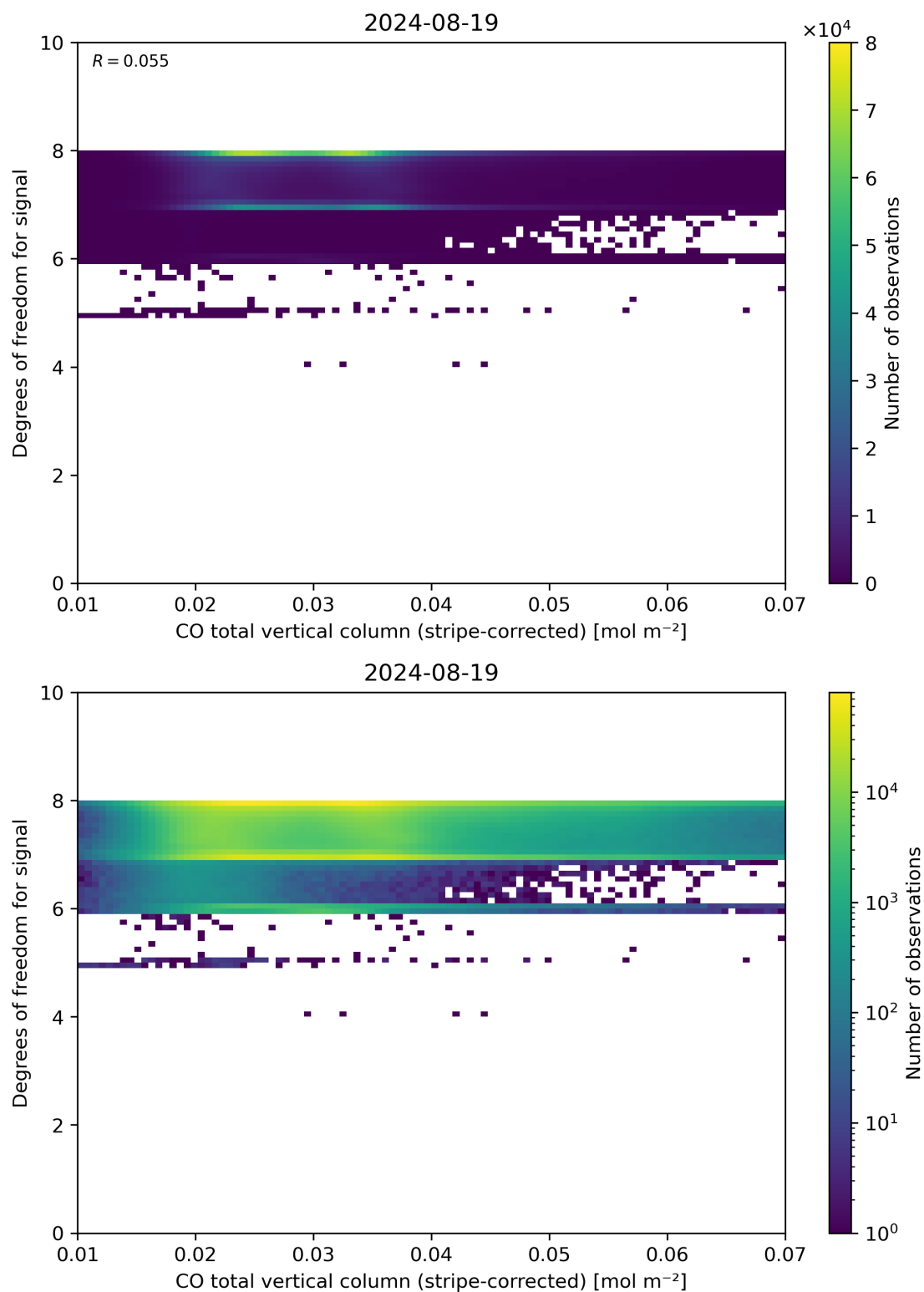
Figure 38: Scatter density plot of “CO total vertical column (stripe-corrected)” against “Degrees of freedom for signal” for 2024-08-18 to 2024-08-20.
