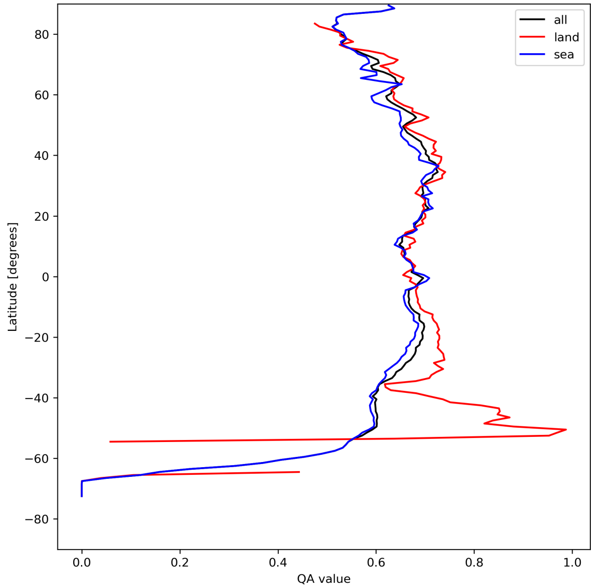
Figure 9: Zonal average of “QA value” for 2024-08-18 to 2024-08-20.
