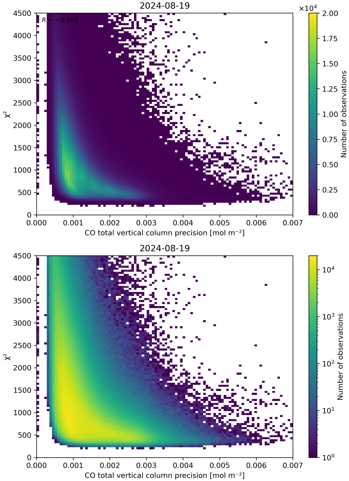
Figure 44: Scatter density plot of “CO total vertical column precision” against “ \chi^2 ” for 2024-08-18 to 2024-08-20.
