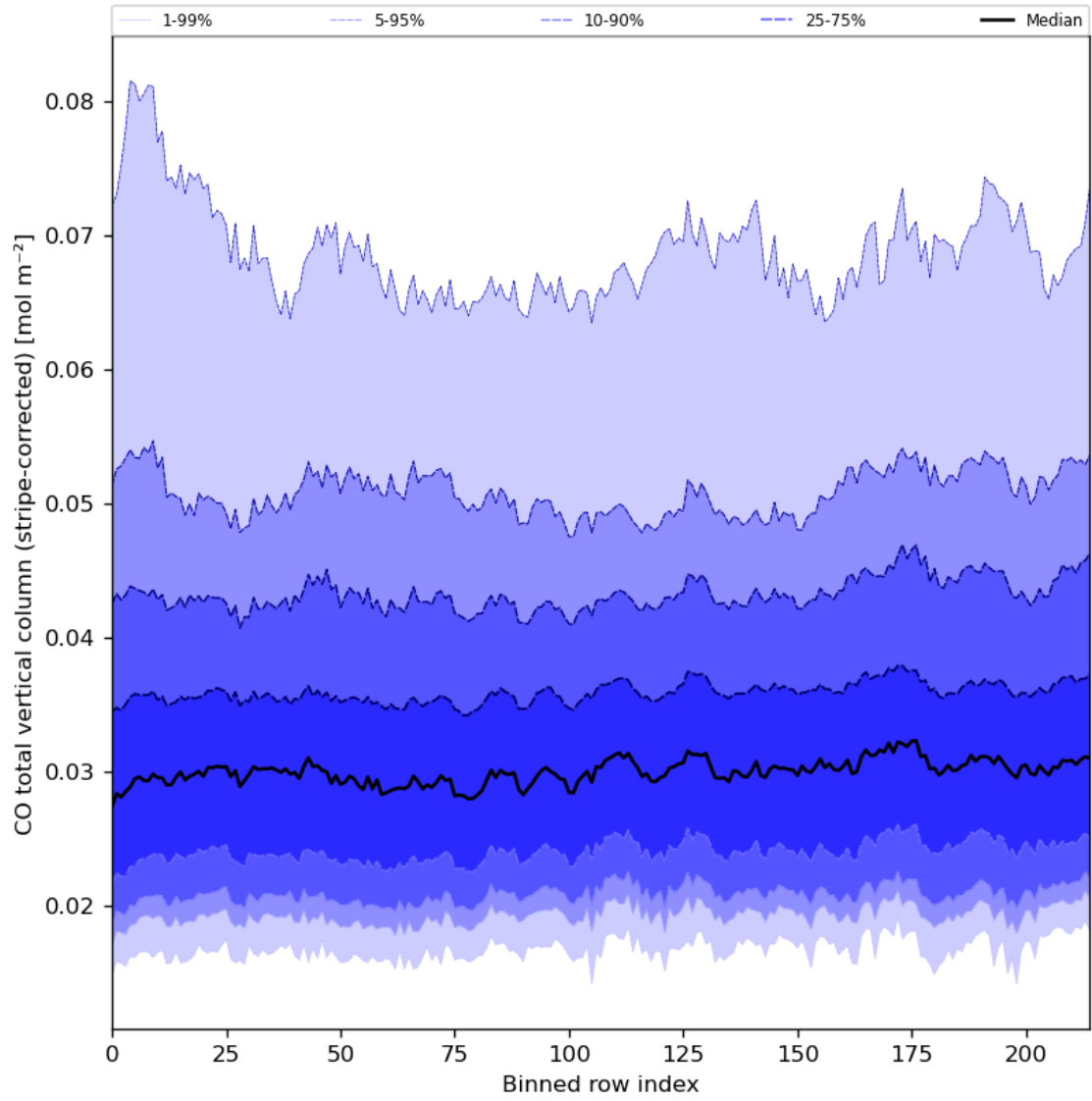
Figure 27: Along track statistics of “CO total vertical column (stripe-corrected)” for 2024-08-18 to 2024-08-20
