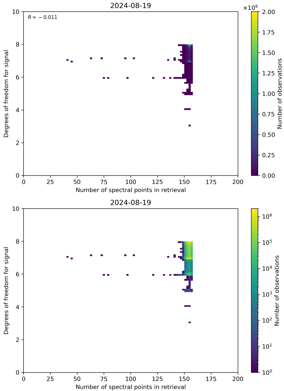
Figure 59: Scatter density plot of “Number of spectral points in retrieval” against “Degrees of freedom for signal” for 2024-08-18 to 2024-08-20.
