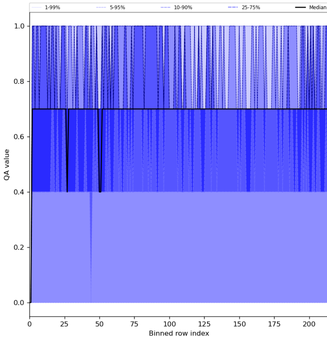
Figure 25: Along track statistics of “QA value” for 2024-08-18 to 2024-08-20
