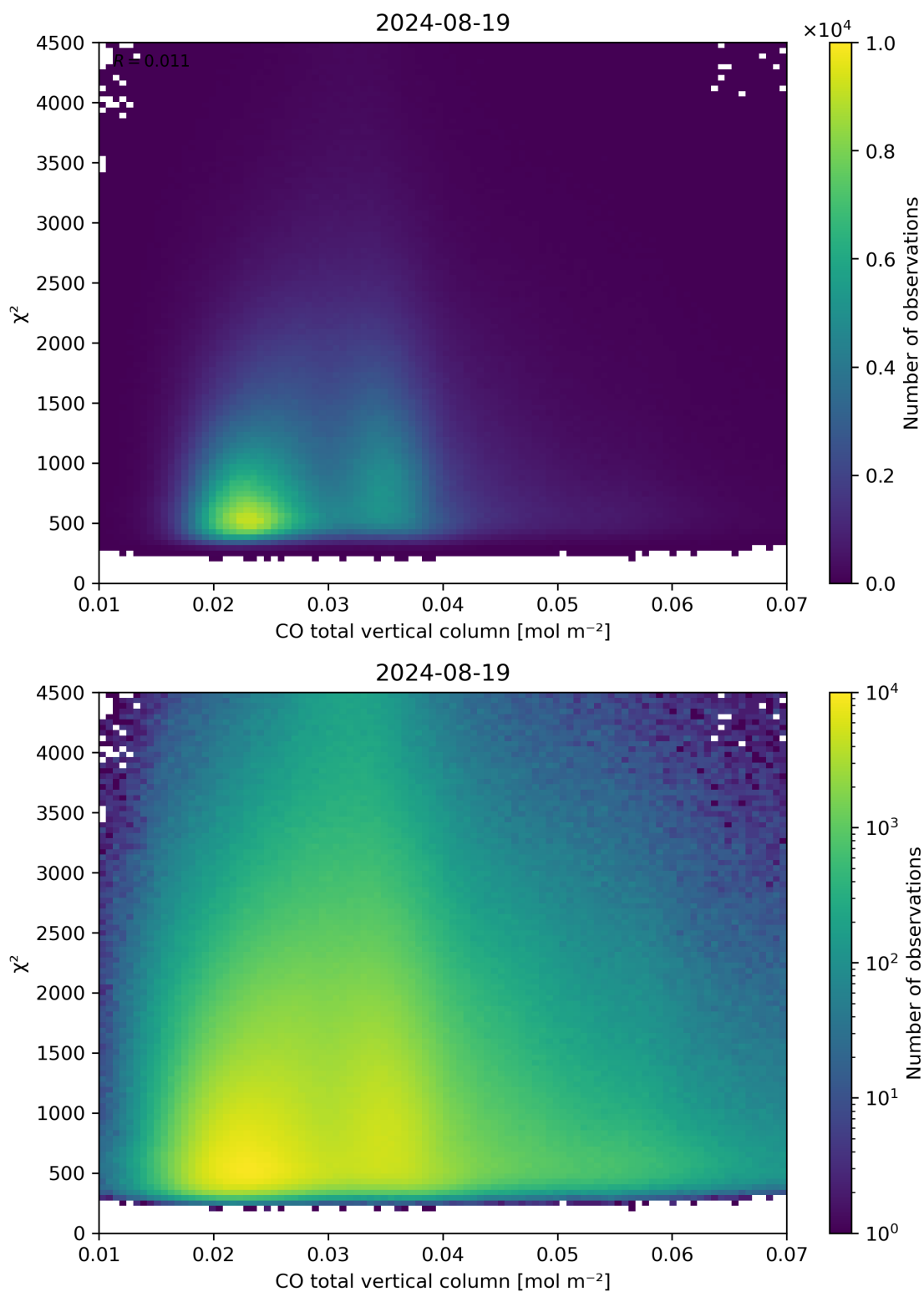
Figure 35: Scatter density plot of “CO total vertical column” against “ \chi^2 ” for 2024-08-18 to 2024-08-20.
