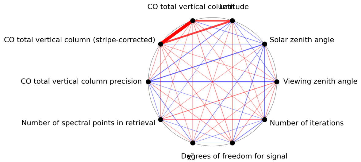
Figure 1: Map of correlation graph for 2024-08-18 to 2024-08-20.
