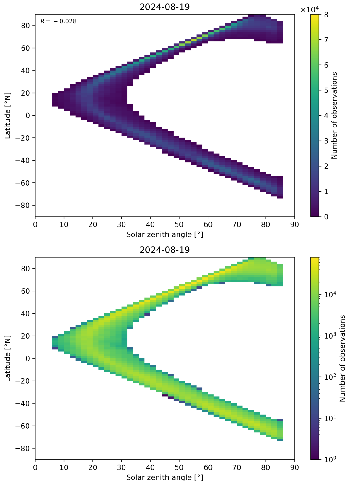
Figure 66: Scatter density plot of “Solar zenith angle” against “Latitude” for 2024-08-18 to 2024-08-20.
