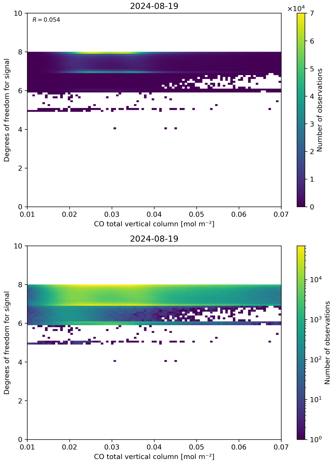
Figure 41: Scatter density plot of “CO total vertical column” against “Degrees of freedom for signal” for 2024-08-18 to 2024-08-20.
