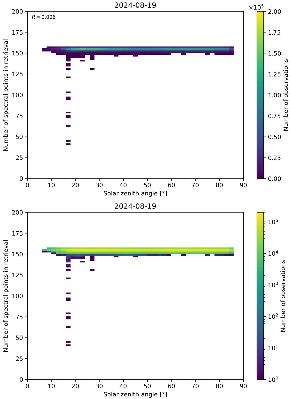
Figure 68: Scatter density plot of “Solar zenith angle” against “Number of spectral points in retrieval” for 2024-08-18 to 2024-08-20.
