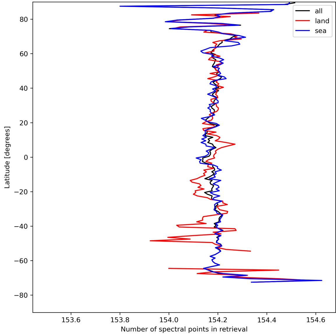
Figure 13: Zonal average of “Number of spectral points in retrieval” for 2024-08-18 to 2024-08-20.
