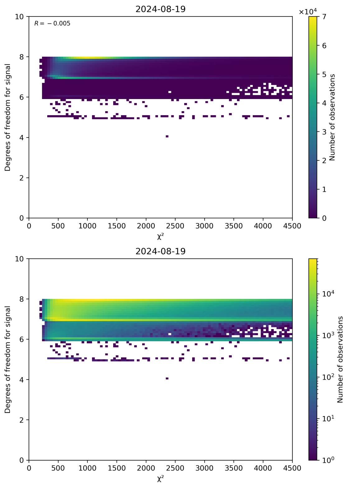
Figure 48: Scatter density plot of “ \chi^2 ” against “Degrees of freedom for signal” for 2024-08-18 to 2024-08-20.
