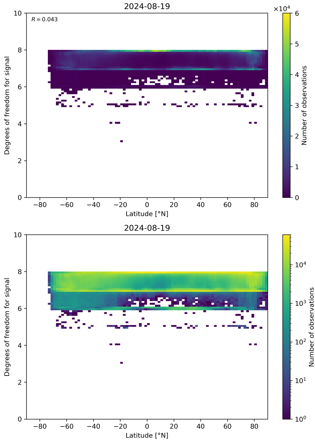
Figure 55: Scatter density plot of “Latitude” against “Degrees of freedom for signal” for 2024-08-18 to 2024-08-20.
