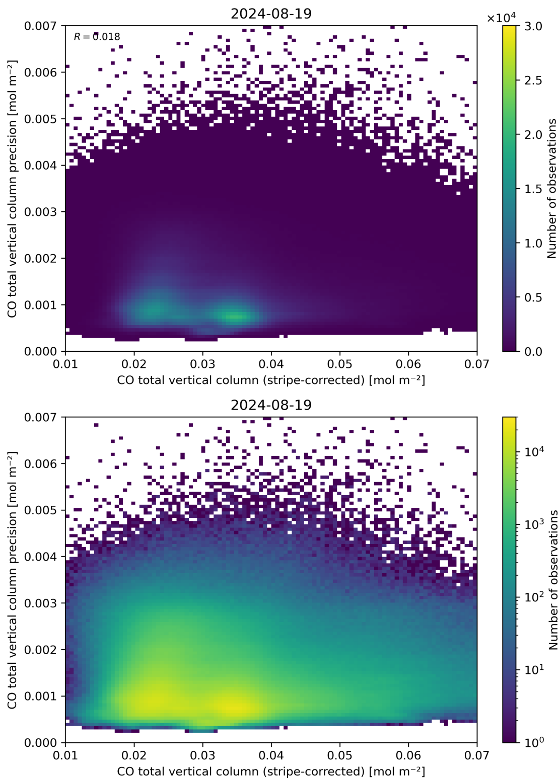
Figure 36: Scatter density plot of “CO total vertical column (stripe-corrected)” against “CO total vertical column precision” for 2024-08-18 to 2024-08-20.
