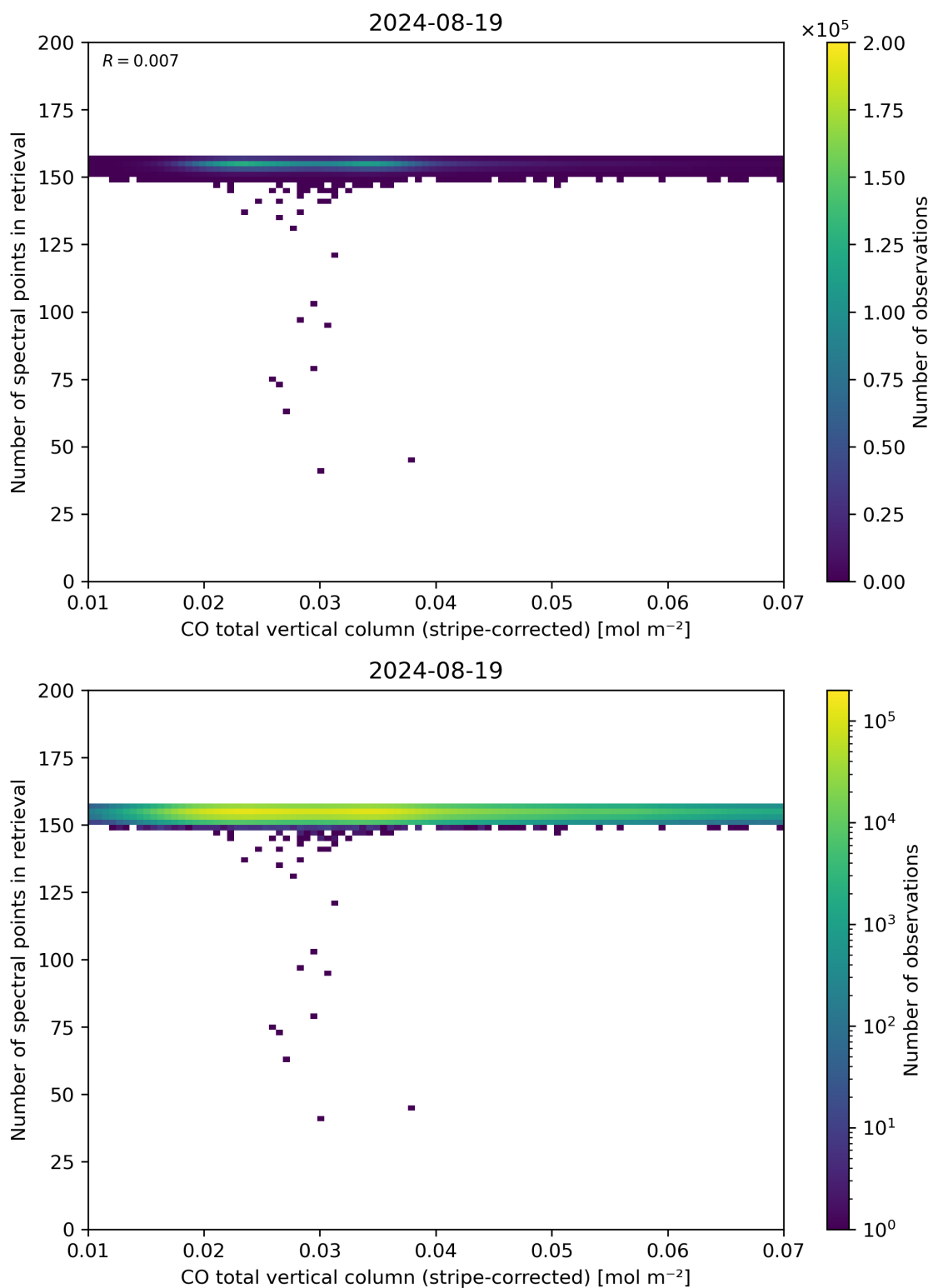
Figure 40: Scatter density plot of “CO total vertical column (stripe-corrected)” against “Number of spectral points in retrieval” for 2024-08-18 to 2024-08-20.
