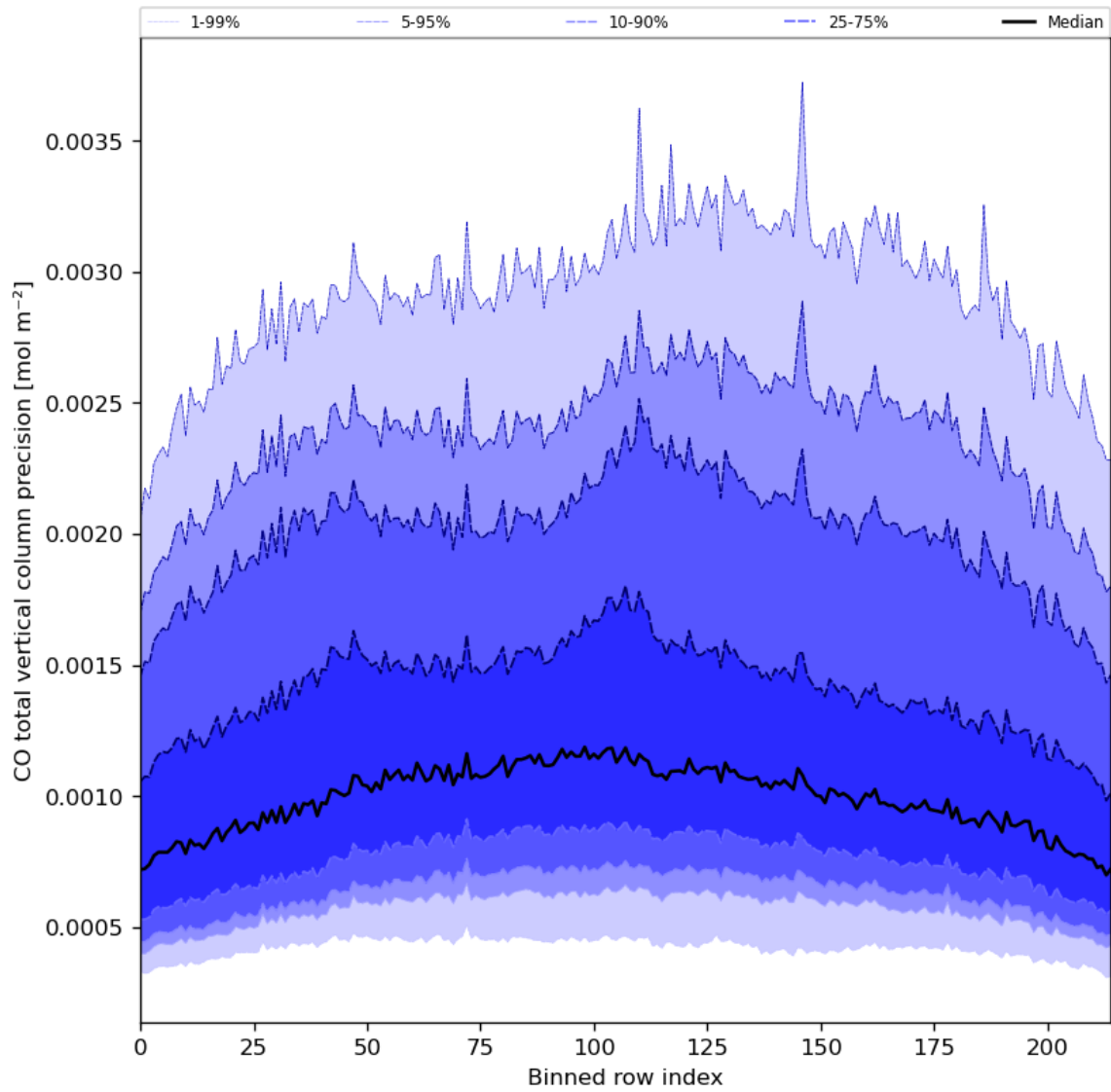
Figure 28: Along track statistics of “CO total vertical column precision” for 2024-08-18 to 2024-08-20
