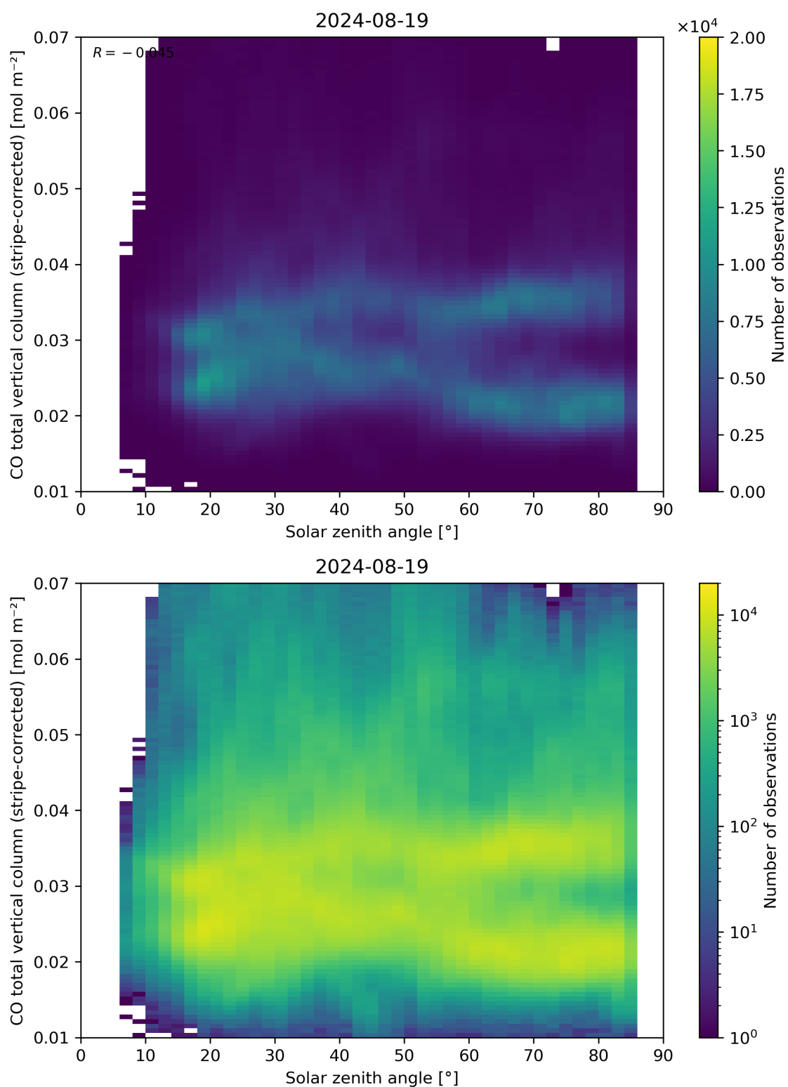
Figure 62: Scatter density plot of “Solar zenith angle” against “CO total vertical column (stripe-corrected)” for 2024-08-18 to 2024-08-20.
