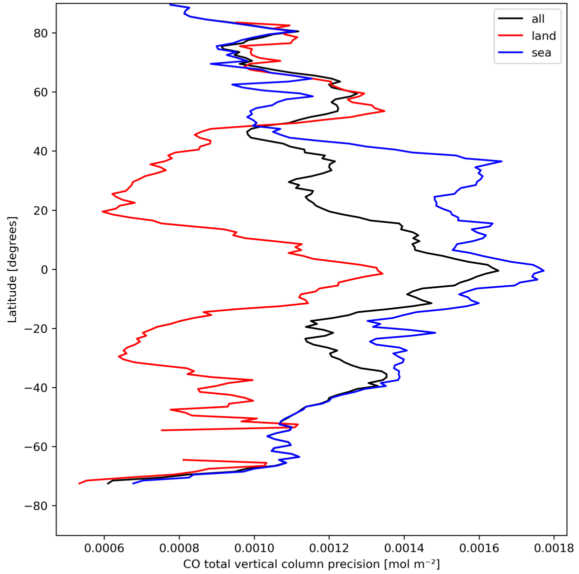
Figure 12: Zonal average of “CO total vertical column precision” for 2024-08-18 to 2024-08-20.
