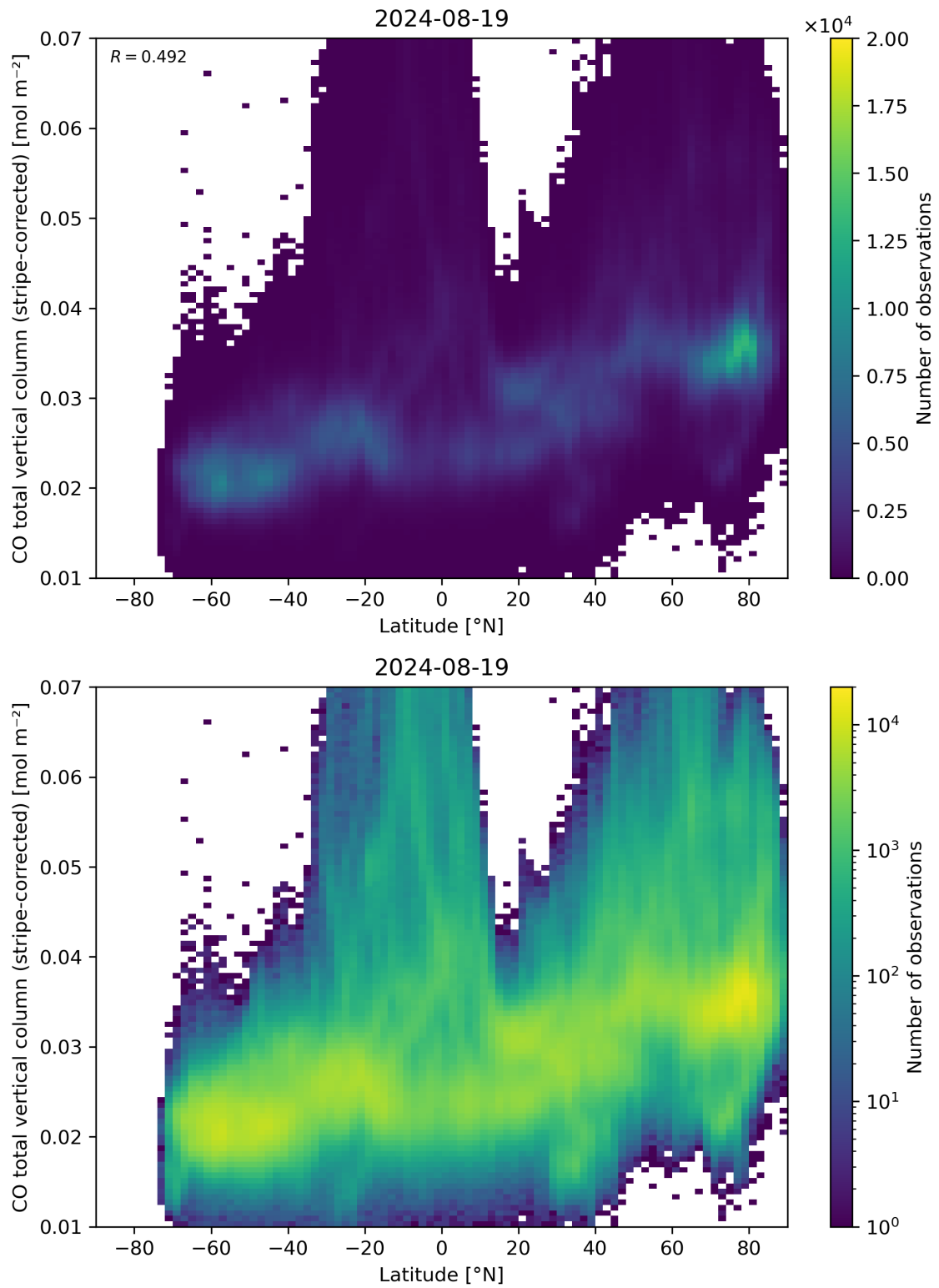
Figure 52: Scatter density plot of “Latitude” against “CO total vertical column (stripe-corrected)” for 2024-08-18 to 2024-08-20.
