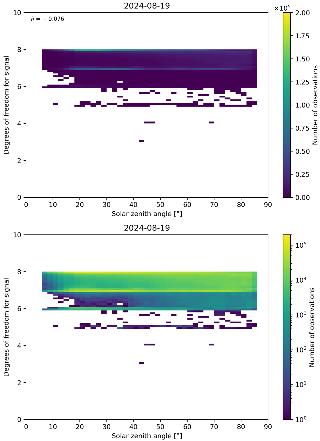
Figure 65: Scatter density plot of “Solar zenith angle” against “Degrees of freedom for signal” for 2024-08-18 to 2024-08-20.
