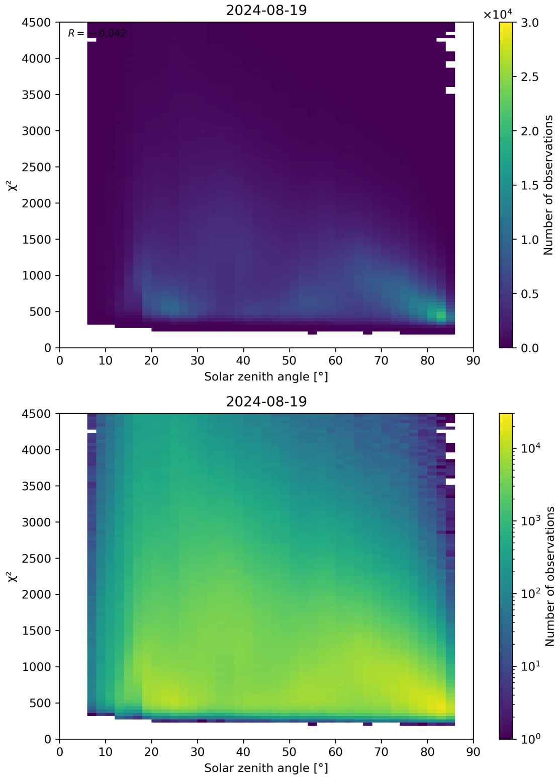
Figure 64: Scatter density plot of “Solar zenith angle” against “ \chi^2 ” for 2024-08-18 to 2024-08-20.
