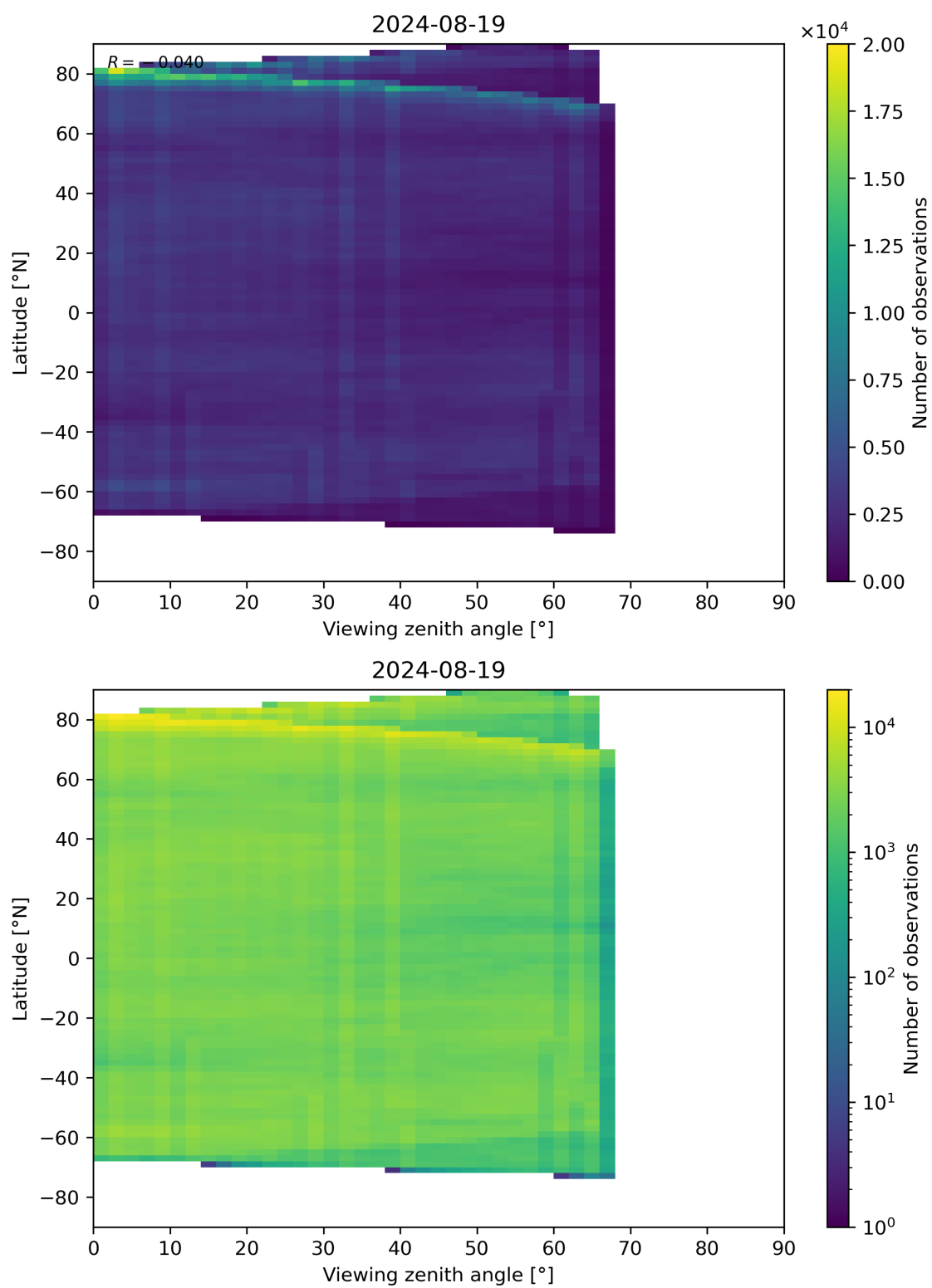
Figure 74: Scatter density plot of “Viewing zenith angle” against “Latitude” for 2024-08-18 to 2024-08-20.
