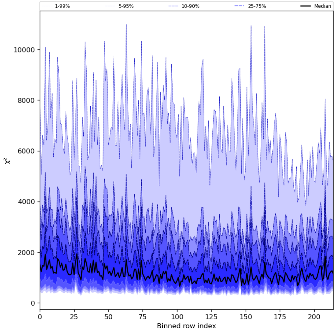
Figure 30: Along track statistics of “ \chi^2 ” for 2024-08-18 to 2024-08-20
