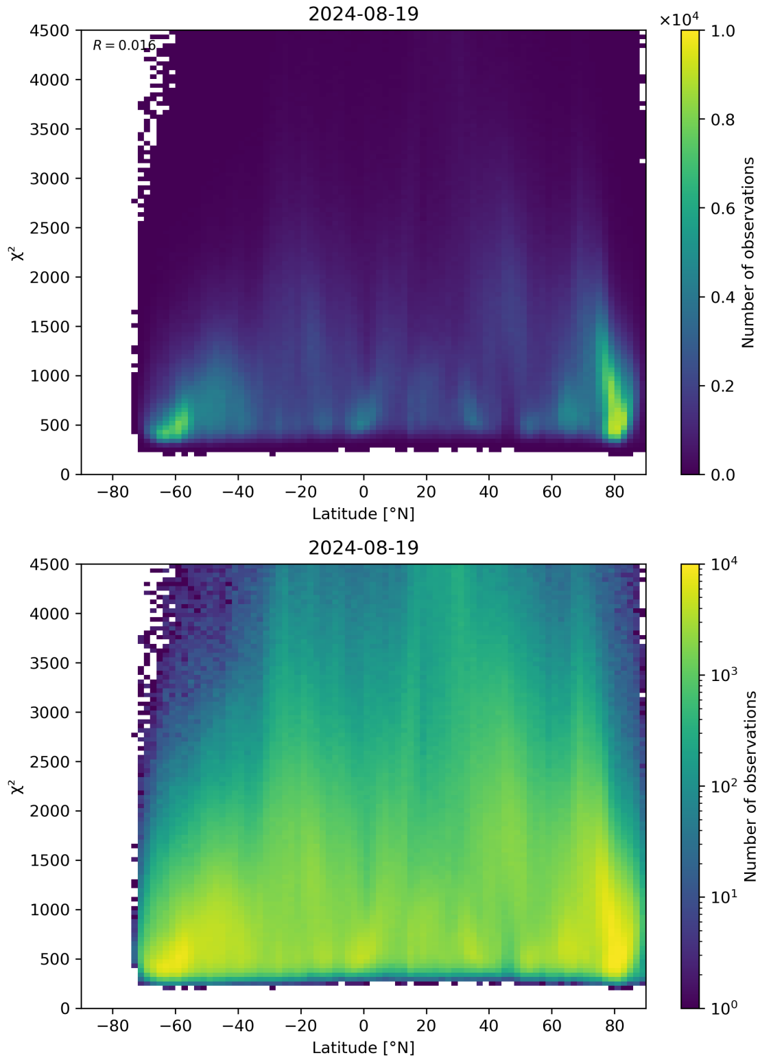
Figure 54: Scatter density plot of “Latitude” against “ \chi^2 ” for 2024-08-18 to 2024-08-20.
