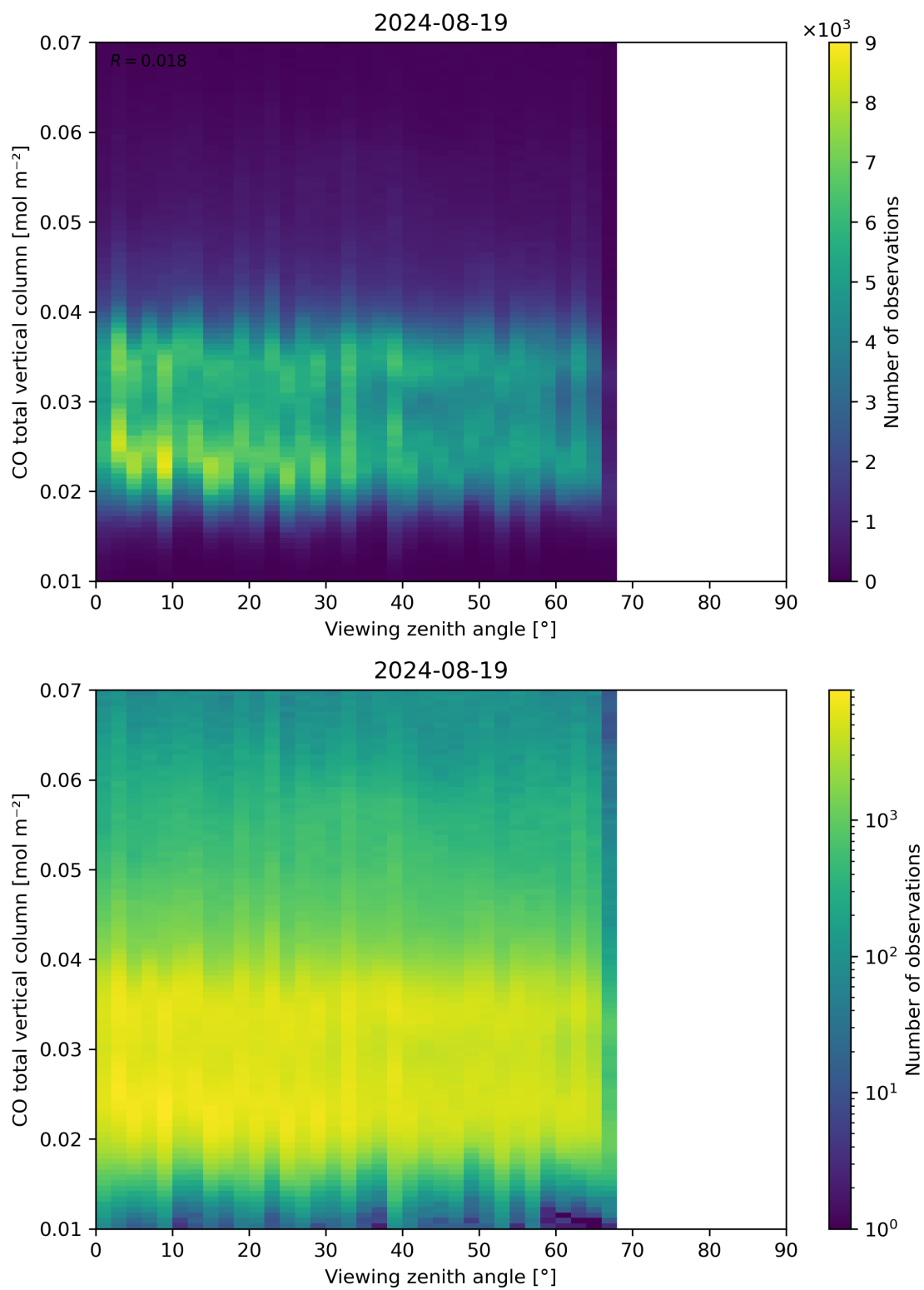
Figure 69: Scatter density plot of “Viewing zenith angle” against “CO total vertical column” for 2024-08-18 to 2024-08-20.
