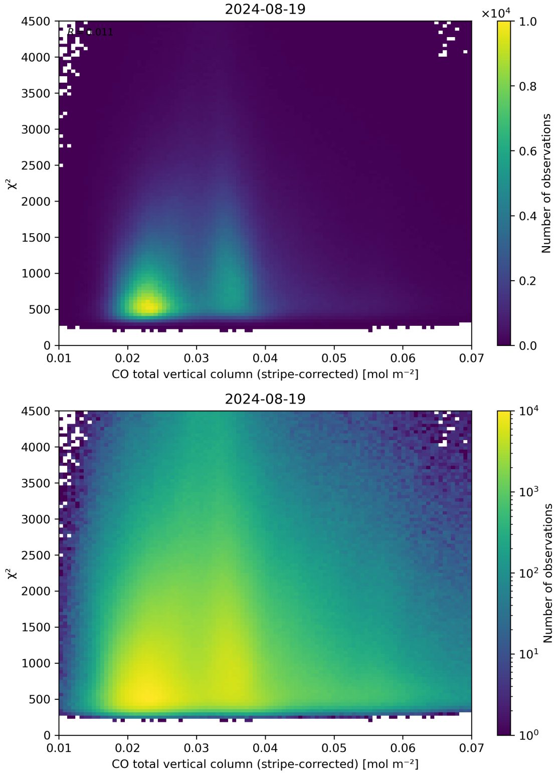
Figure 37: Scatter density plot of “CO total vertical column (stripe-corrected)” against “ \chi^2 ” for 2024-08-18 to 2024-08-20.
