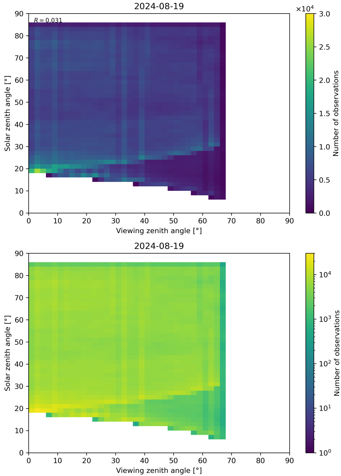
Figure 77: Scatter density plot of “Viewing zenith angle” against “Solar zenith angle” for 2024-08-18 to 2024-08-20.
