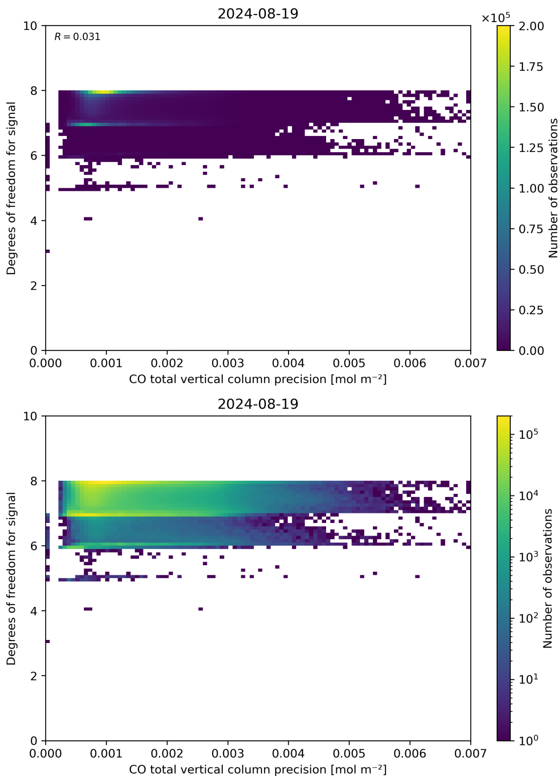
Figure 45: Scatter density plot of “CO total vertical column precision” against “Degrees of freedom for signal” for 2024-08-18 to 2024-08-20.
