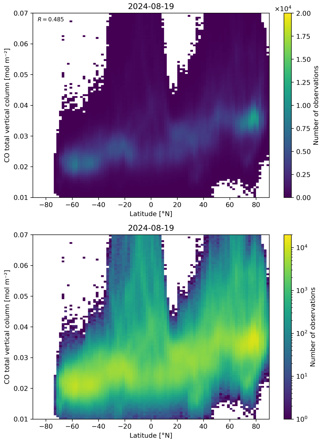
Figure 51: Scatter density plot of “Latitude” against “CO total vertical column” for 2024-08-18 to 2024-08-20.
