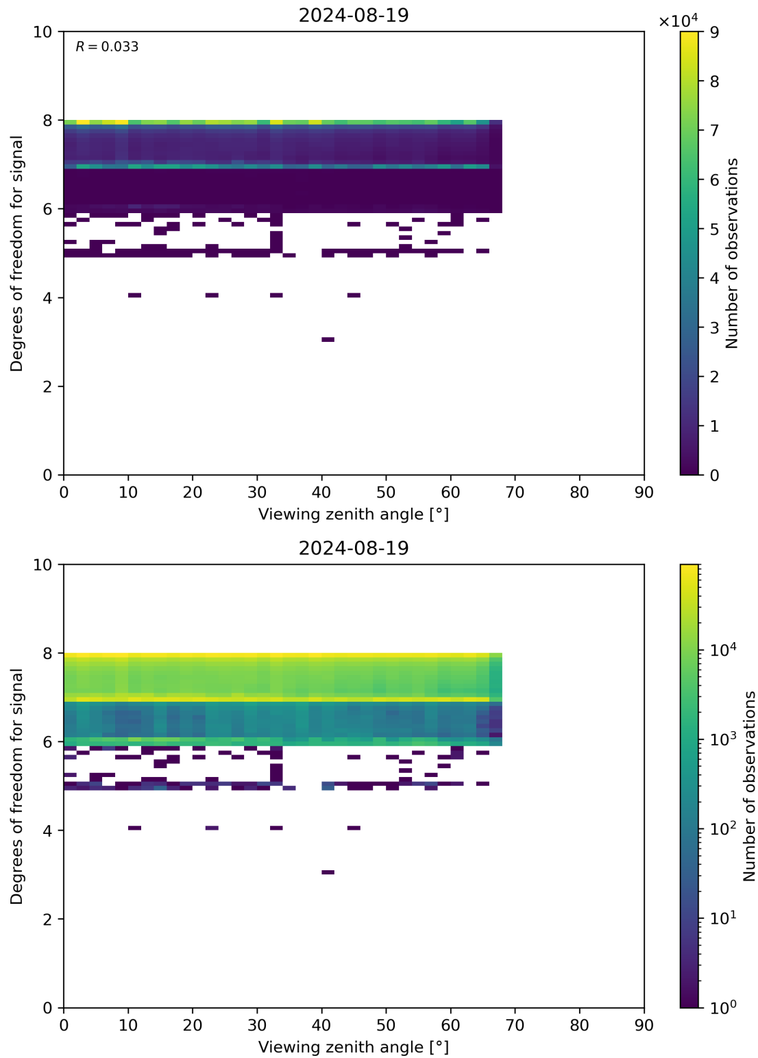
Figure 73: Scatter density plot of “Viewing zenith angle” against “Degrees of freedom for signal” for 2024-08-18 to 2024-08-20.
