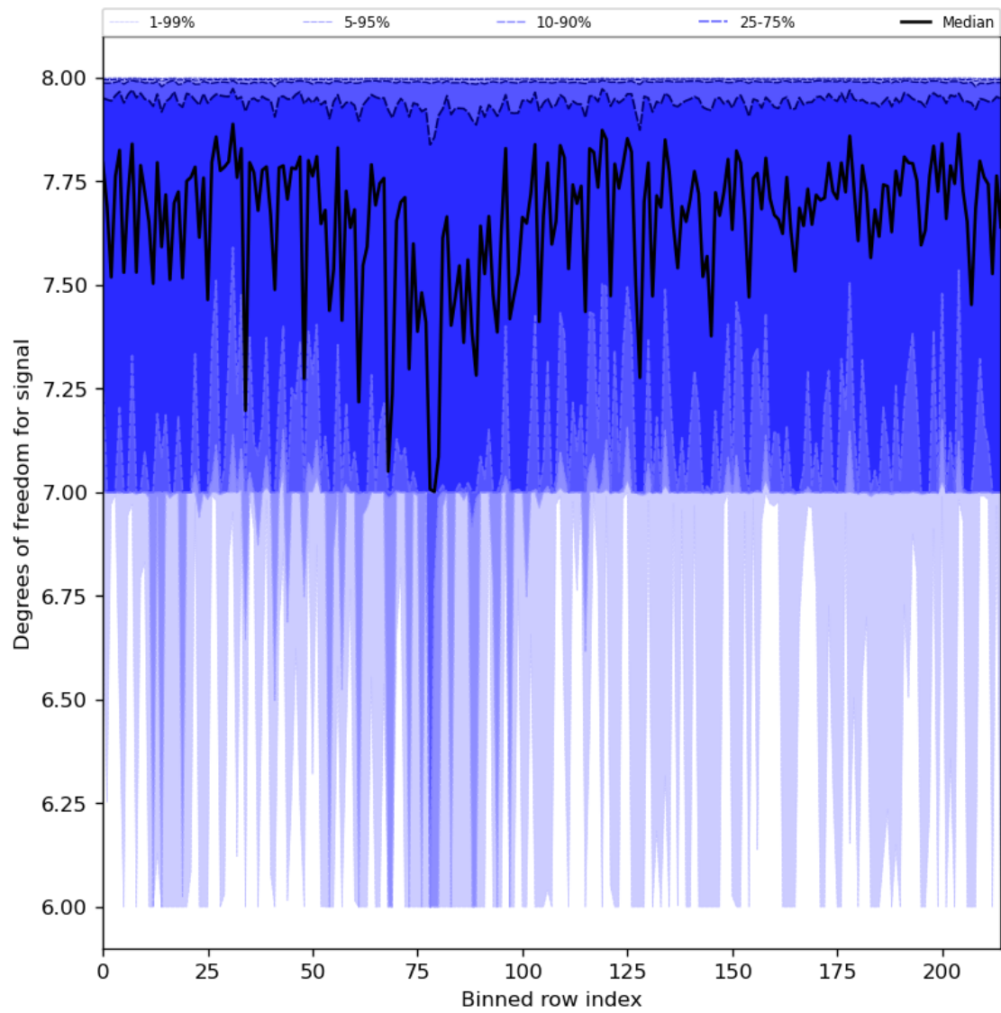
Figure 31: Along track statistics of “Degrees of freedom for signal” for 2024-08-18 to 2024-08-20
