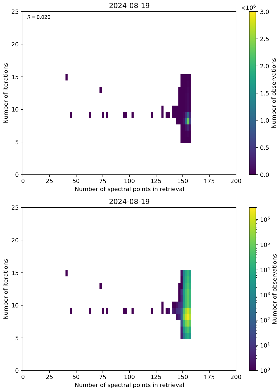
Figure 60: Scatter density plot of “Number of spectral points in retrieval” against “Number of iterations” for 2024-08-18 to 2024-08-20.
