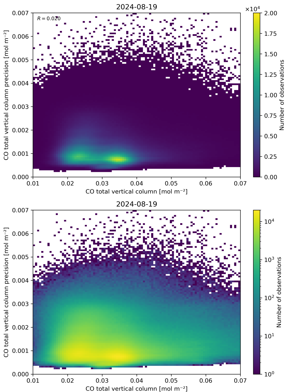
Figure 34: Scatter density plot of “CO total vertical column” against “CO total vertical column precision” for 2024-08-18 to 2024-08-20.
