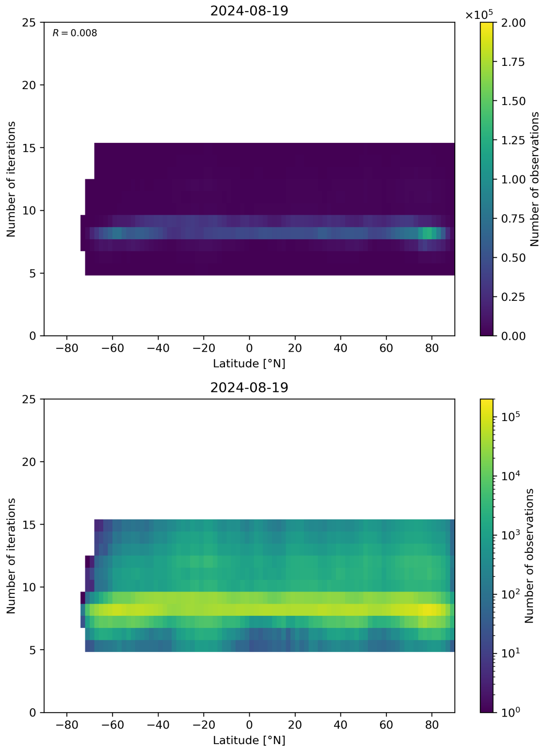
Figure 56: Scatter density plot of “Latitude” against “Number of iterations” for 2024-08-18 to 2024-08-20.
