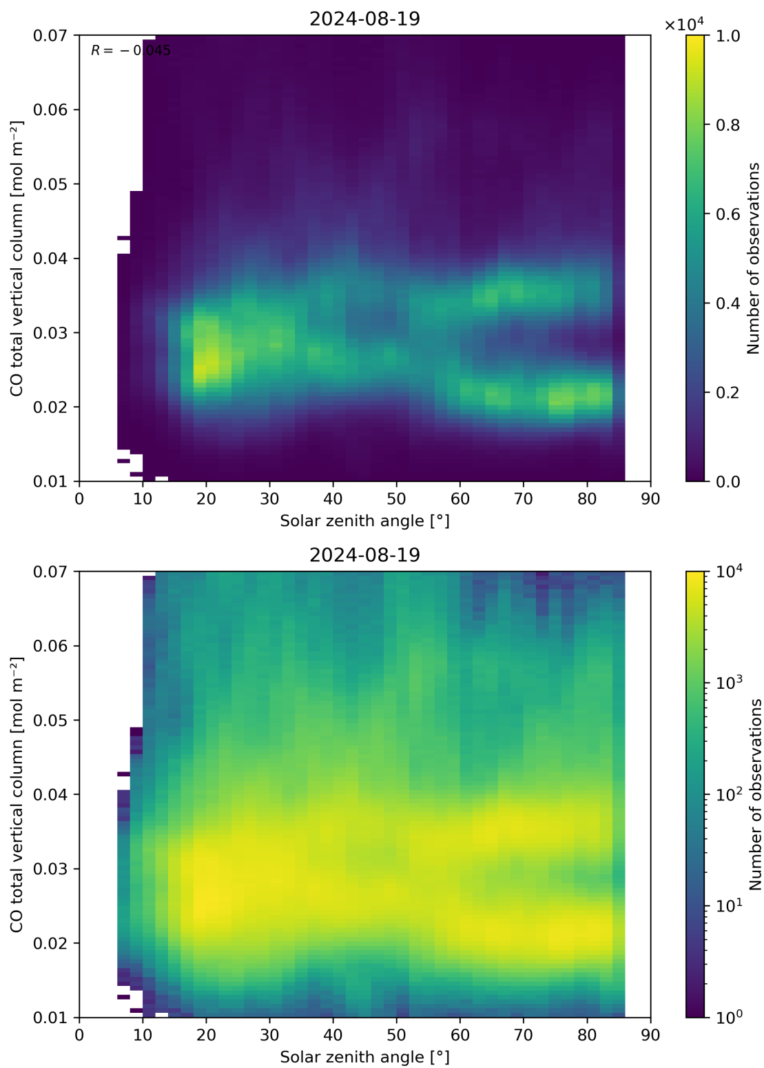
Figure 61: Scatter density plot of “Solar zenith angle” against “CO total vertical column” for 2024-08-18 to 2024-08-20.
