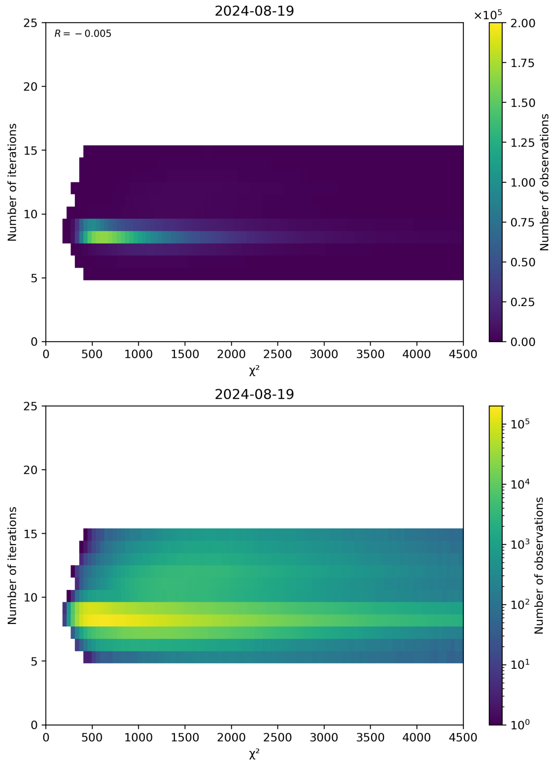
Figure 49: Scatter density plot of “ \chi^2 ” against “Number of iterations” for 2024-08-18 to 2024-08-20.
