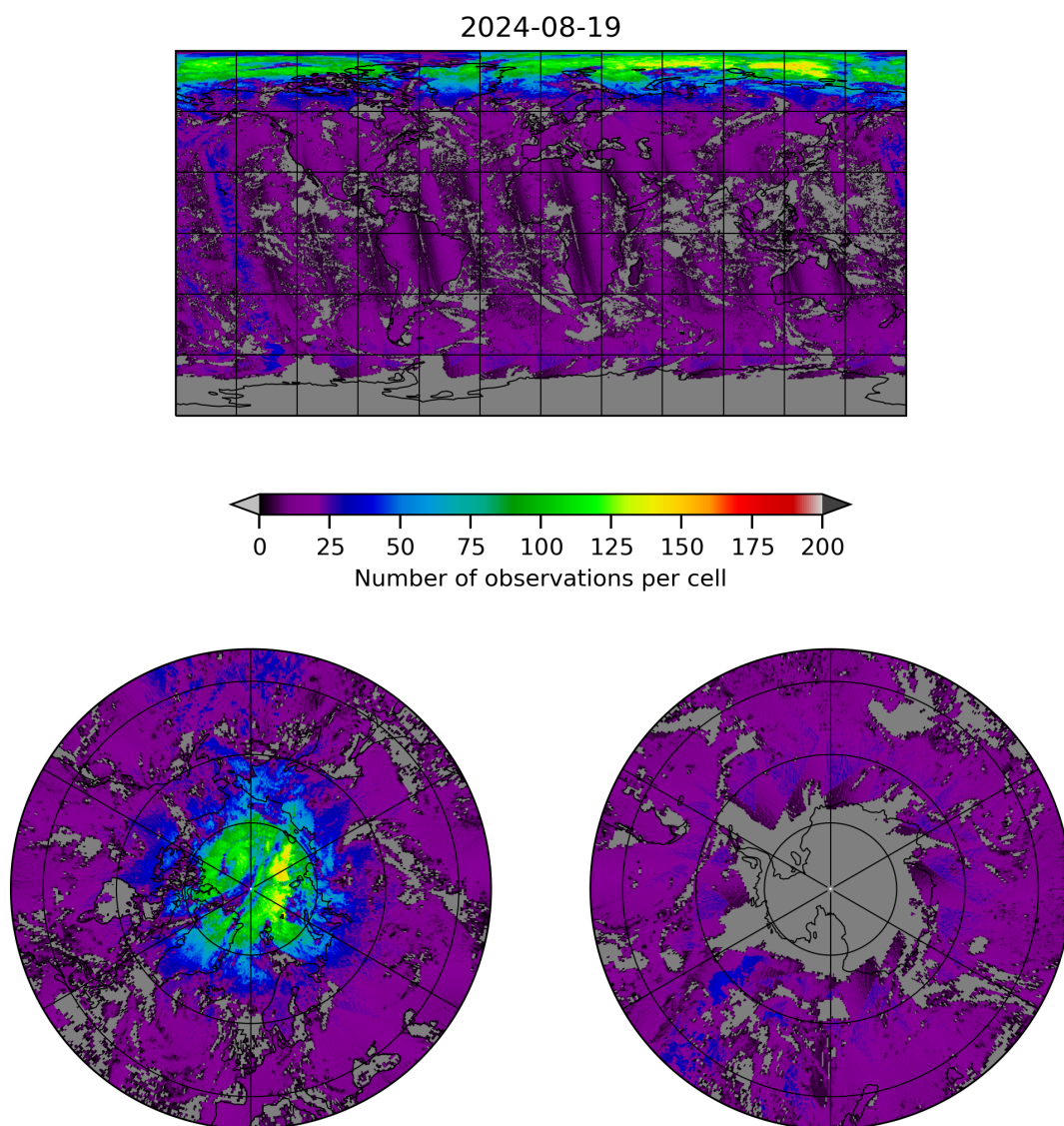
Figure 8: Map of the number of observations for 2024-08-18 to 2024-08-20
