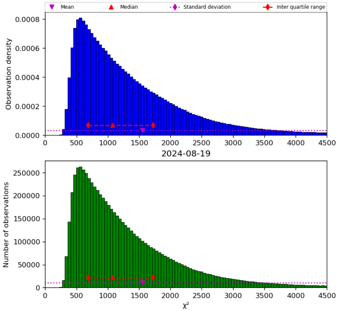
Figure 22: Histogram of “ \chi^2 ” for 2024-08-18 to 2024-08-20
