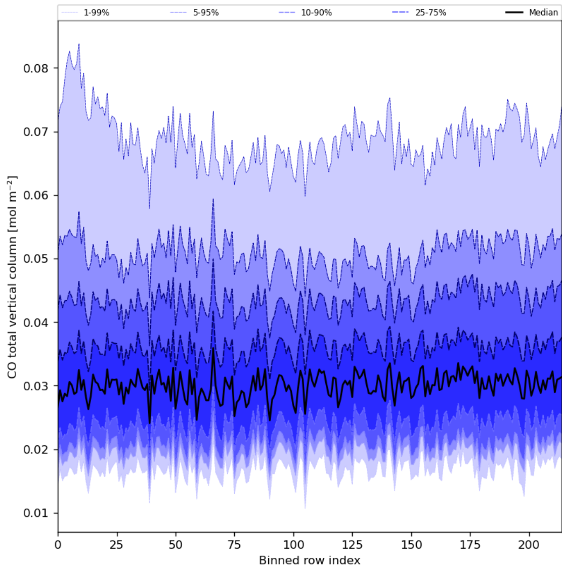
Figure 26: Along track statistics of “CO total vertical column” for 2024-08-18 to 2024-08-20
