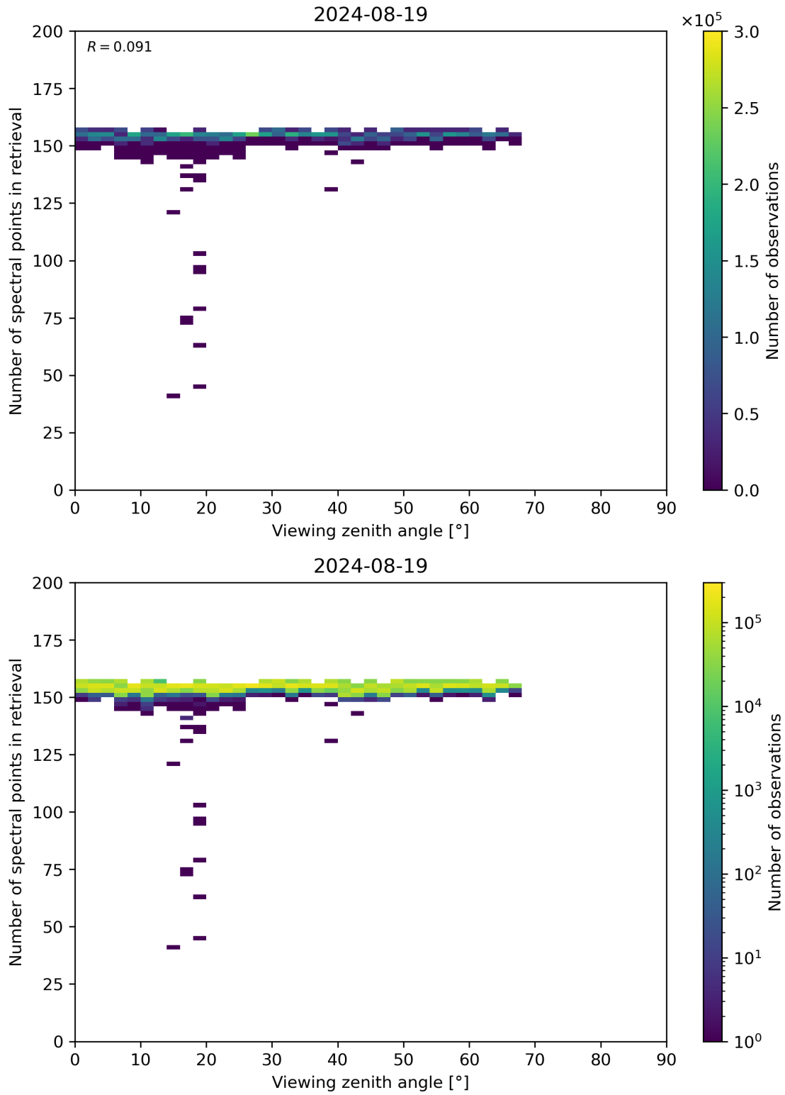
Figure 76: Scatter density plot of “Viewing zenith angle” against “Number of spectral points in retrieval” for 2024-08-18 to 2024-08-20.
