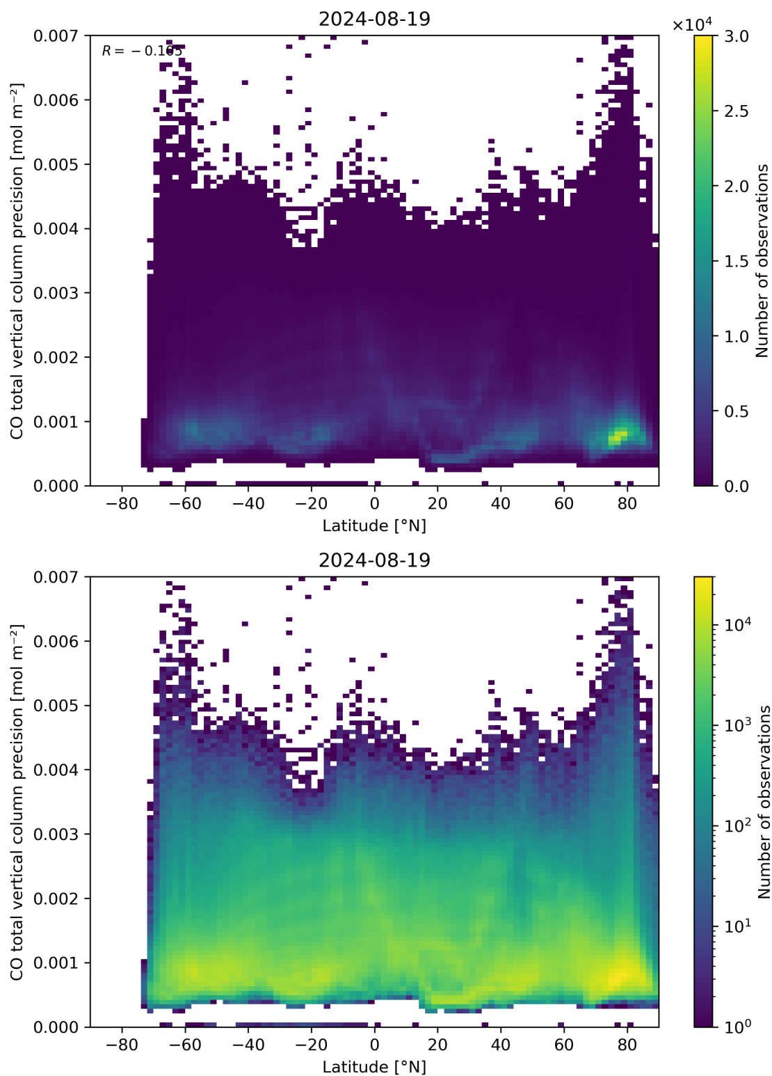
Figure 53: Scatter density plot of “Latitude” against “CO total vertical column precision” for 2024-08-18 to 2024-08-20.
