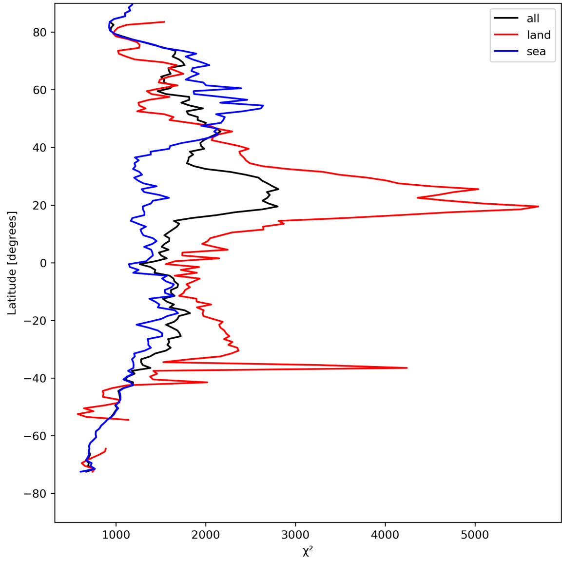
Figure 14: Zonal average of “ \chi^2 ” for 2024-08-18 to 2024-08-20.
