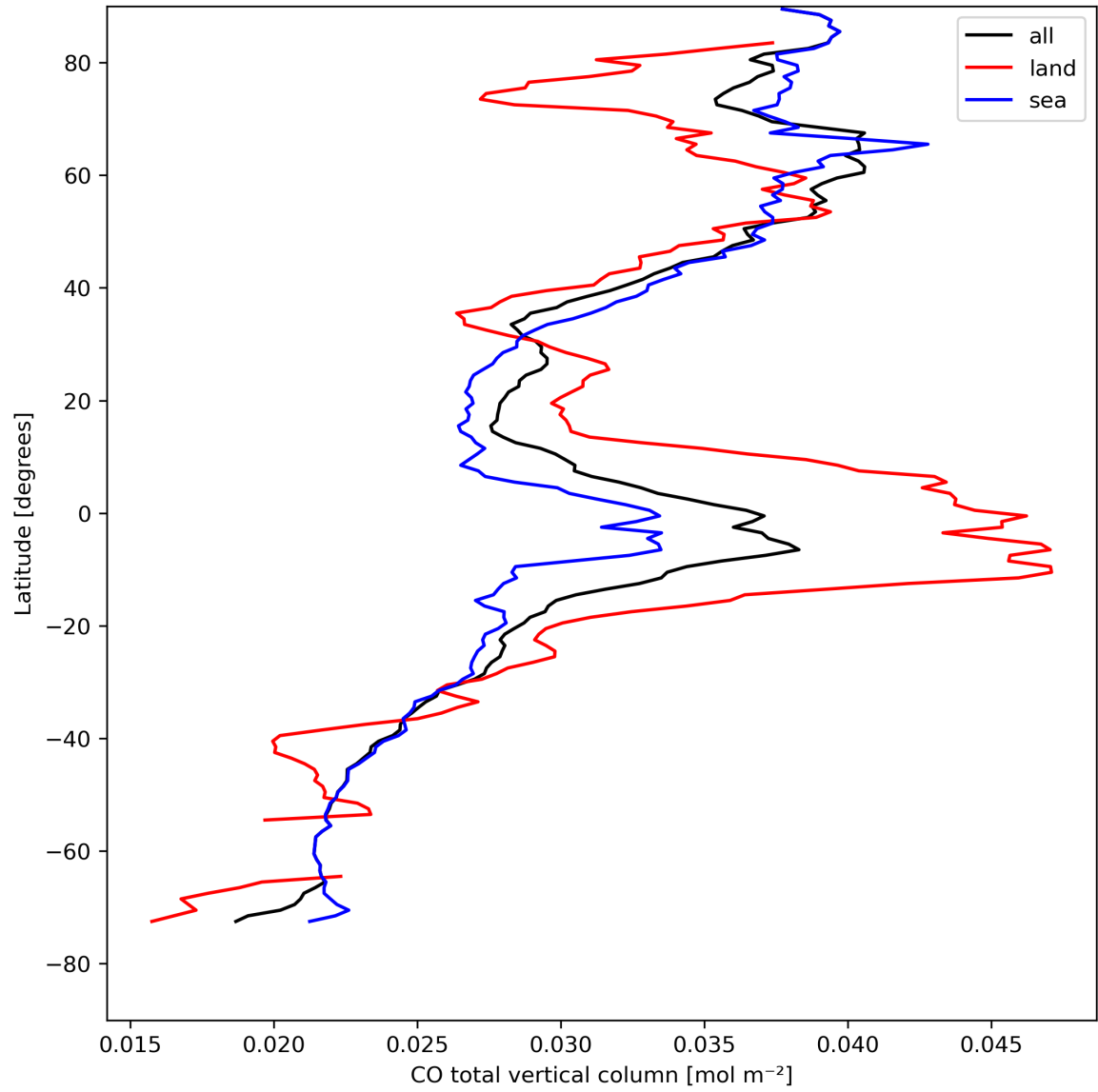
Figure 10: Zonal average of “CO total vertical column” for 2024-08-18 to 2024-08-20.
