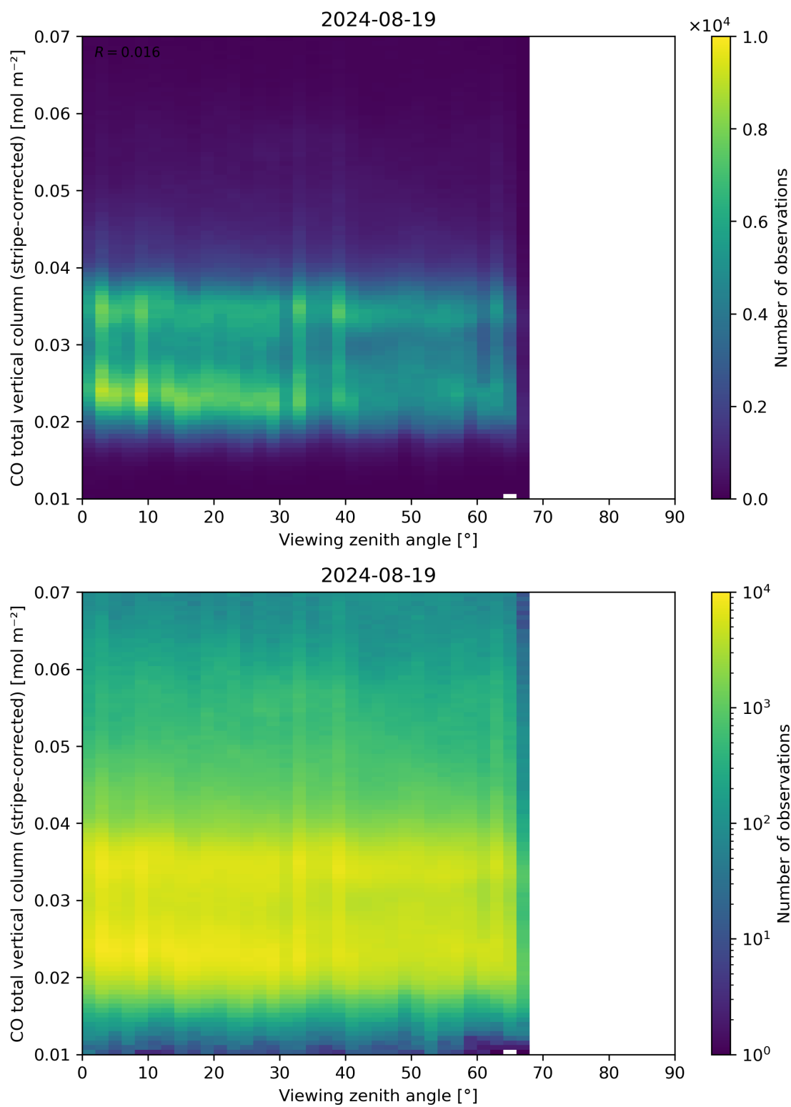
Figure 70: Scatter density plot of “Viewing zenith angle” against “CO total vertical column (stripe-corrected)” for 2024-08-18 to 2024-08-20.
