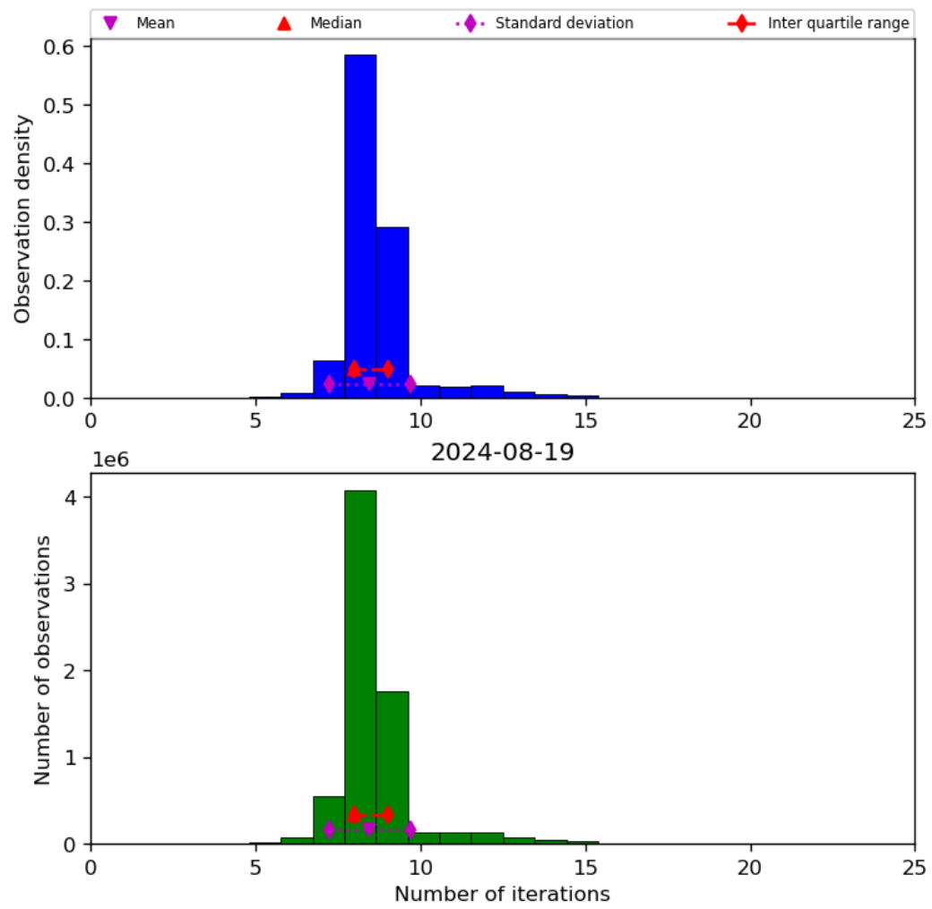
Figure 24: Histogram of “Number of iterations” for 2024-08-18 to 2024-08-20
