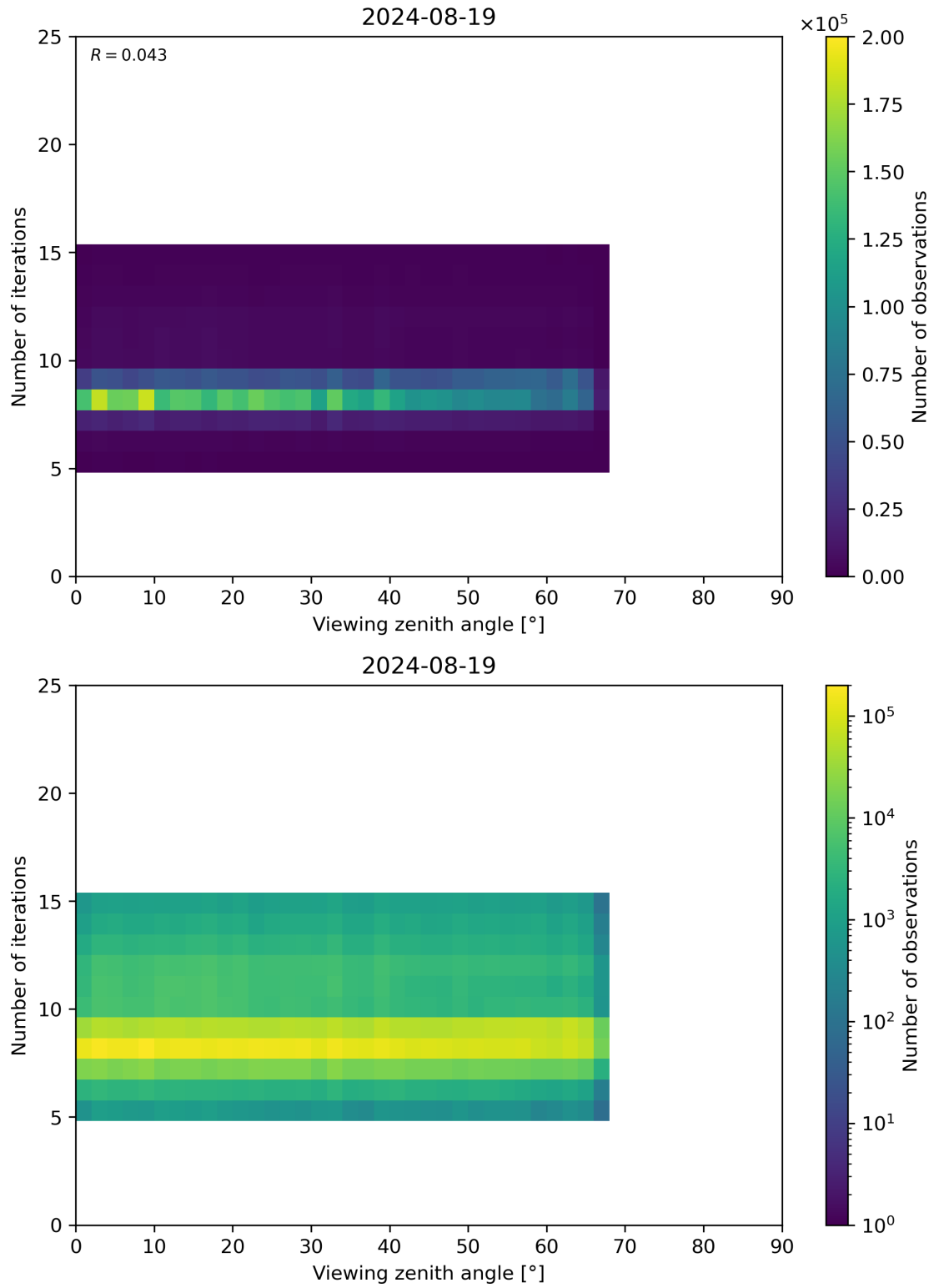
Figure 75: Scatter density plot of “Viewing zenith angle” against “Number of iterations” for 2024-08-18 to 2024-08-20.
