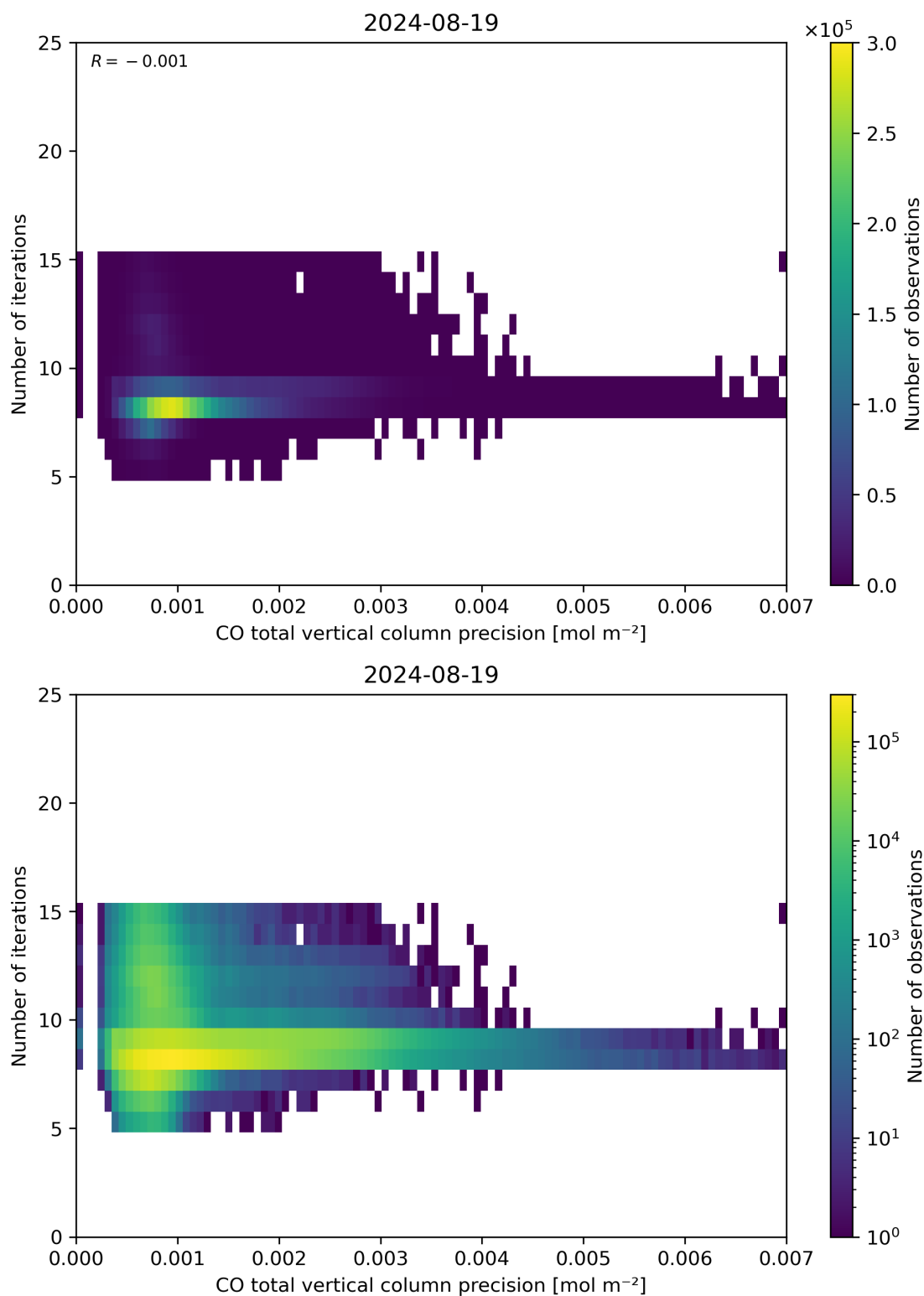
Figure 46: Scatter density plot of “CO total vertical column precision” against “Number of iterations” for 2024-08-18 to 2024-08-20.
