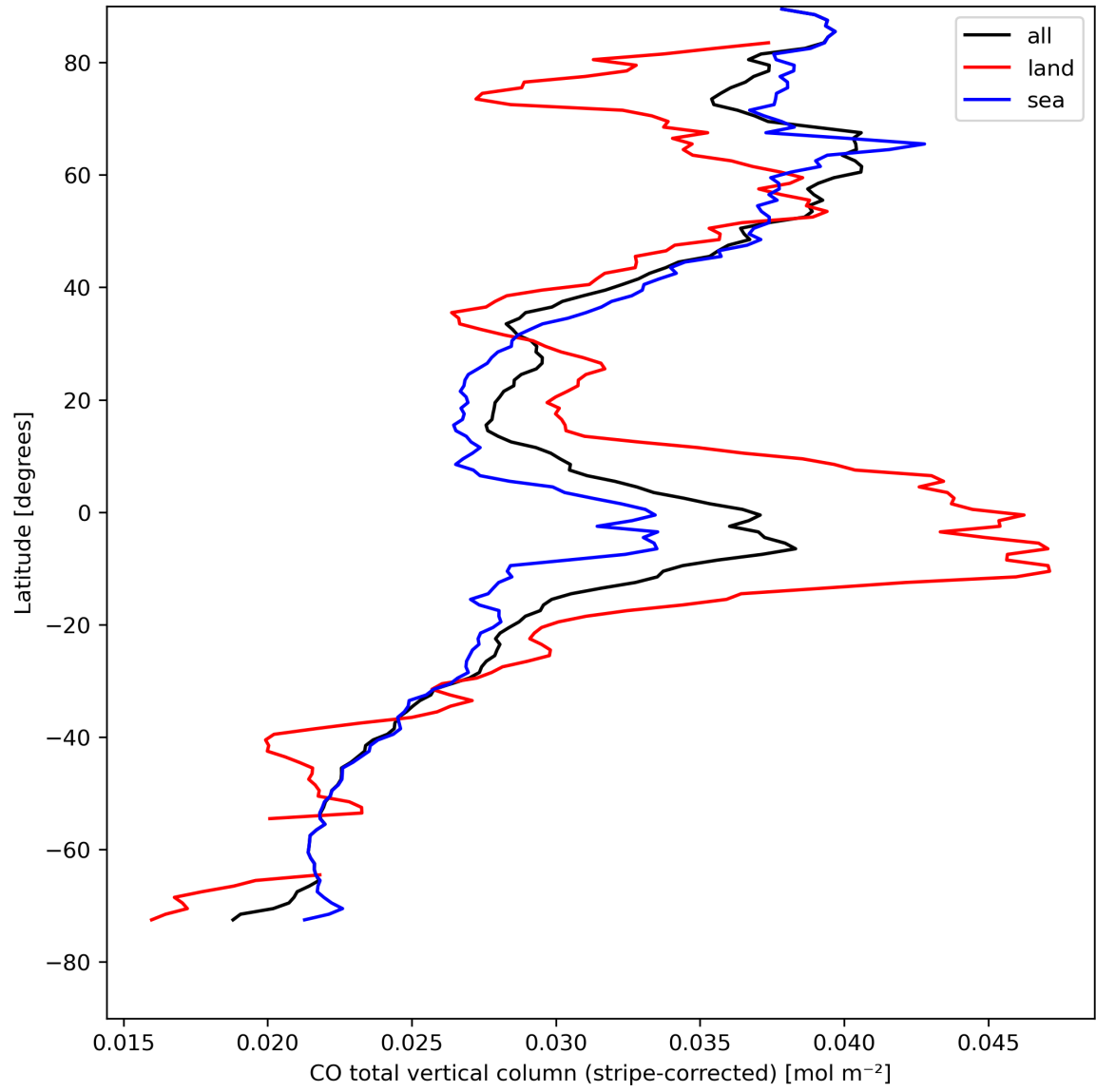
Figure 11: Zonal average of “CO total vertical column (stripe-corrected)” for 2024-08-18 to 2024-08-20.
