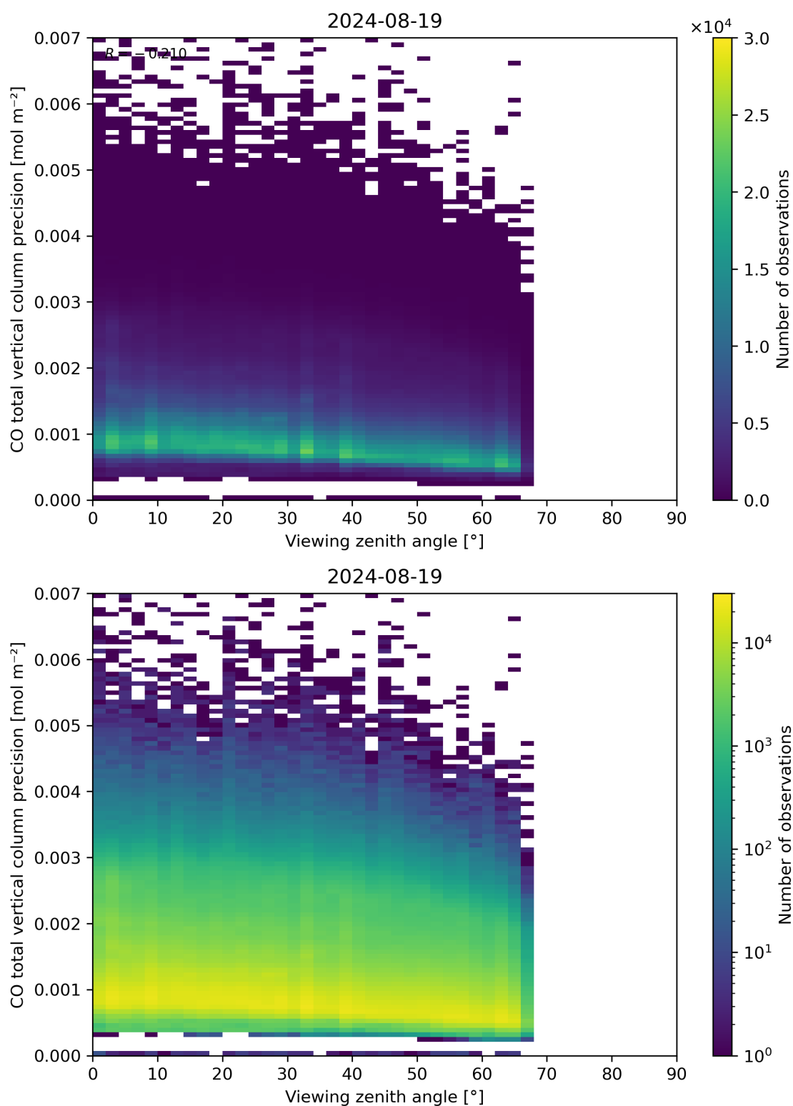
Figure 71: Scatter density plot of “Viewing zenith angle” against “CO total vertical column precision” for 2024-08-18 to 2024-08-20.
