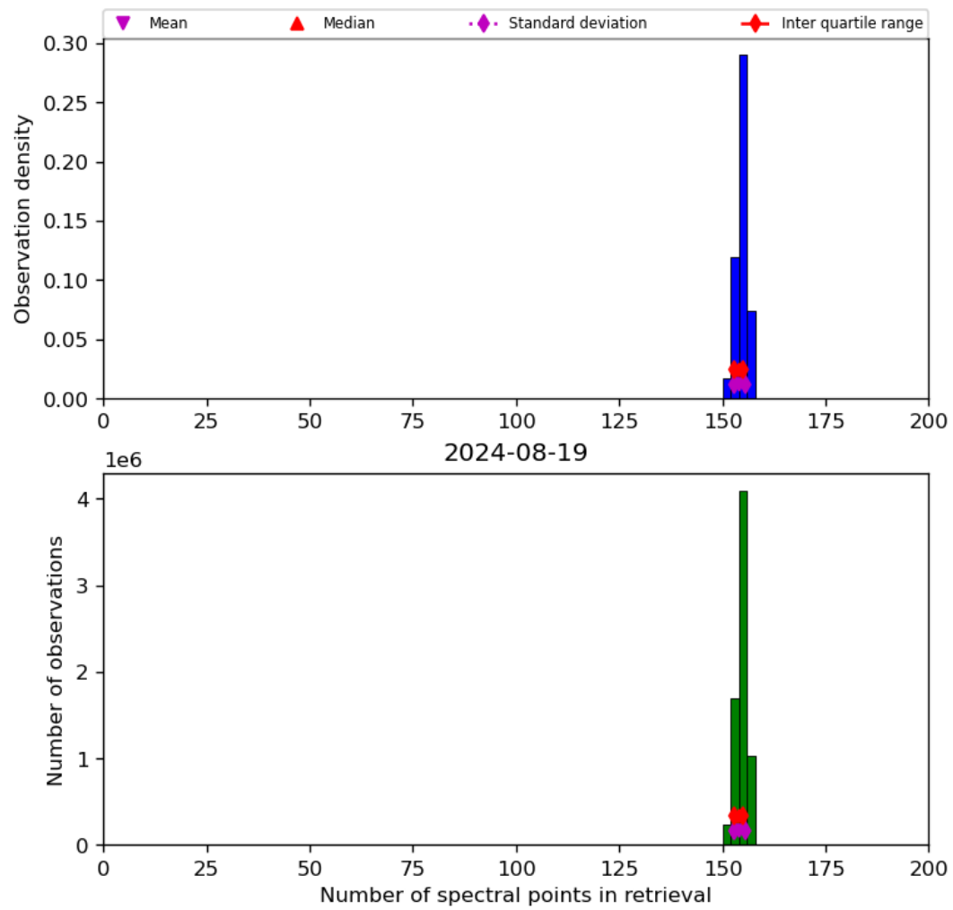
Figure 21: Histogram of “Number of spectral points in retrieval” for 2024-08-18 to 2024-08-20
