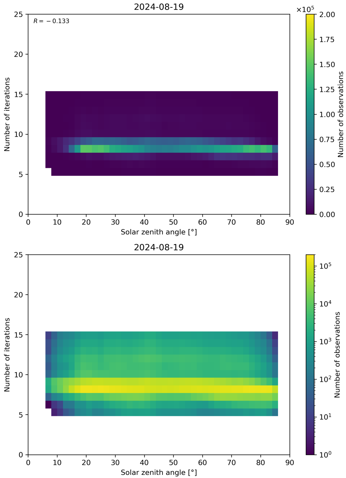
Figure 67: Scatter density plot of “Solar zenith angle” against “Number of iterations” for 2024-08-18 to 2024-08-20.
