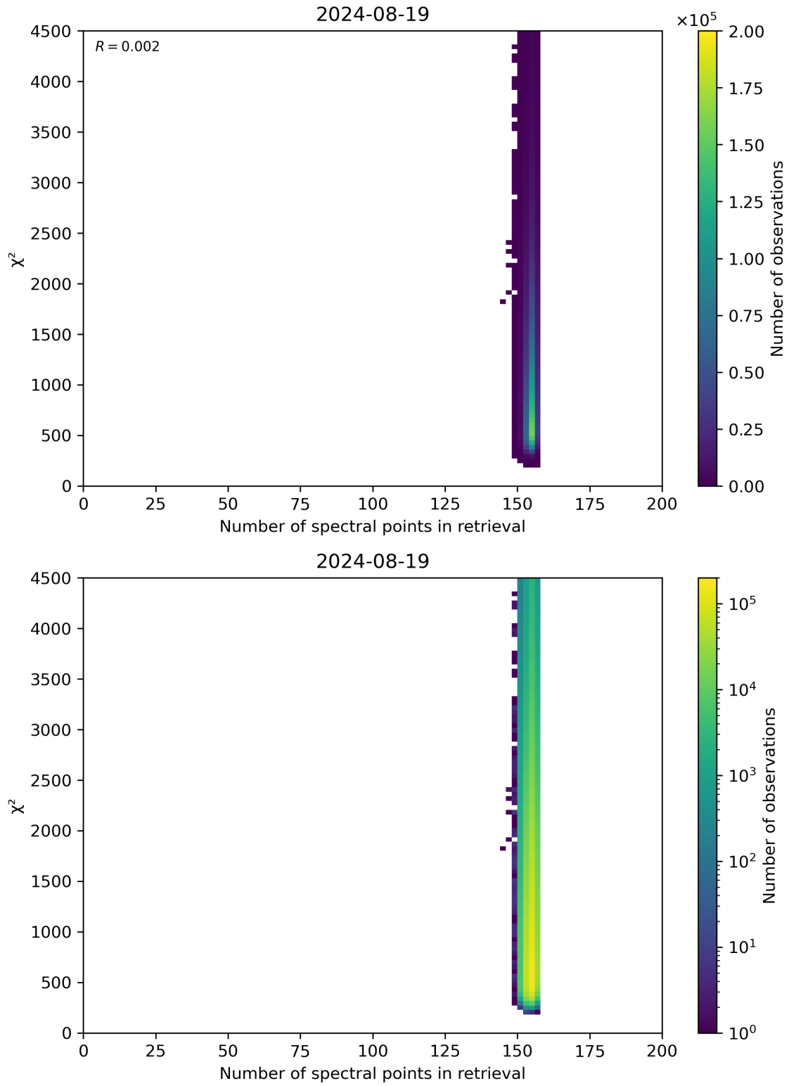
Figure 58: Scatter density plot of “Number of spectral points in retrieval” against “ \chi^2 ” for 2024-08-18 to 2024-08-20.
