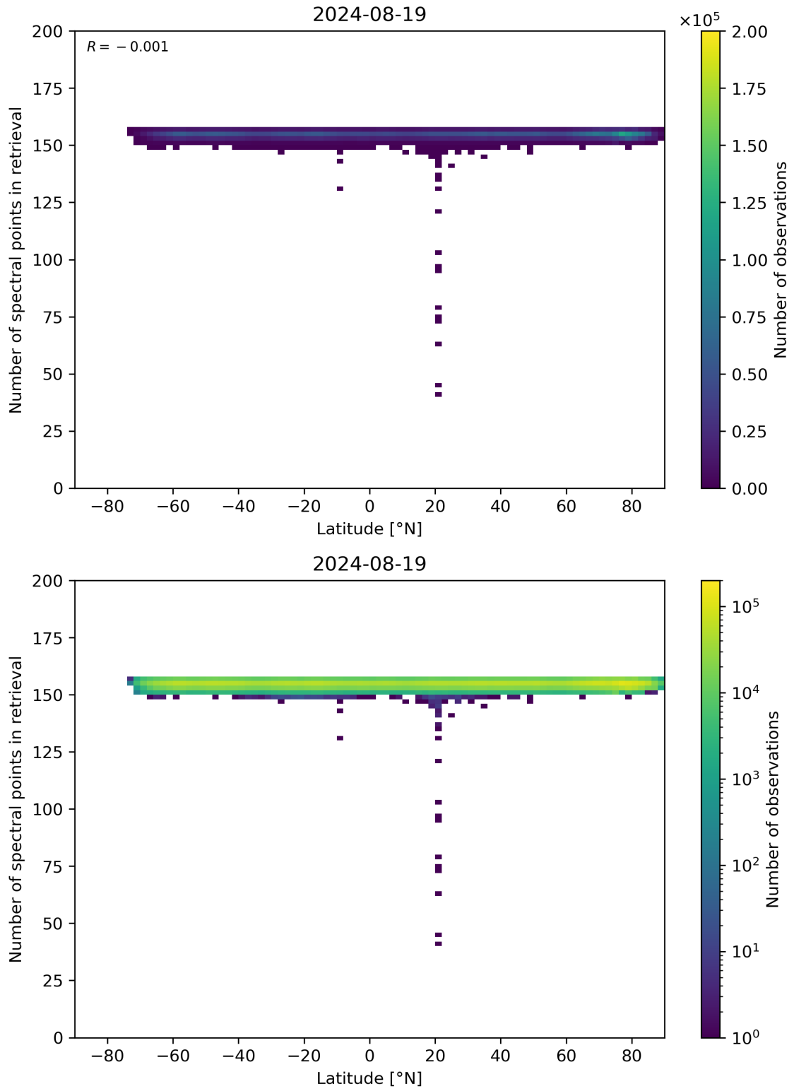
Figure 57: Scatter density plot of “Latitude” against “Number of spectral points in retrieval” for 2024-08-18 to 2024-08-20.
