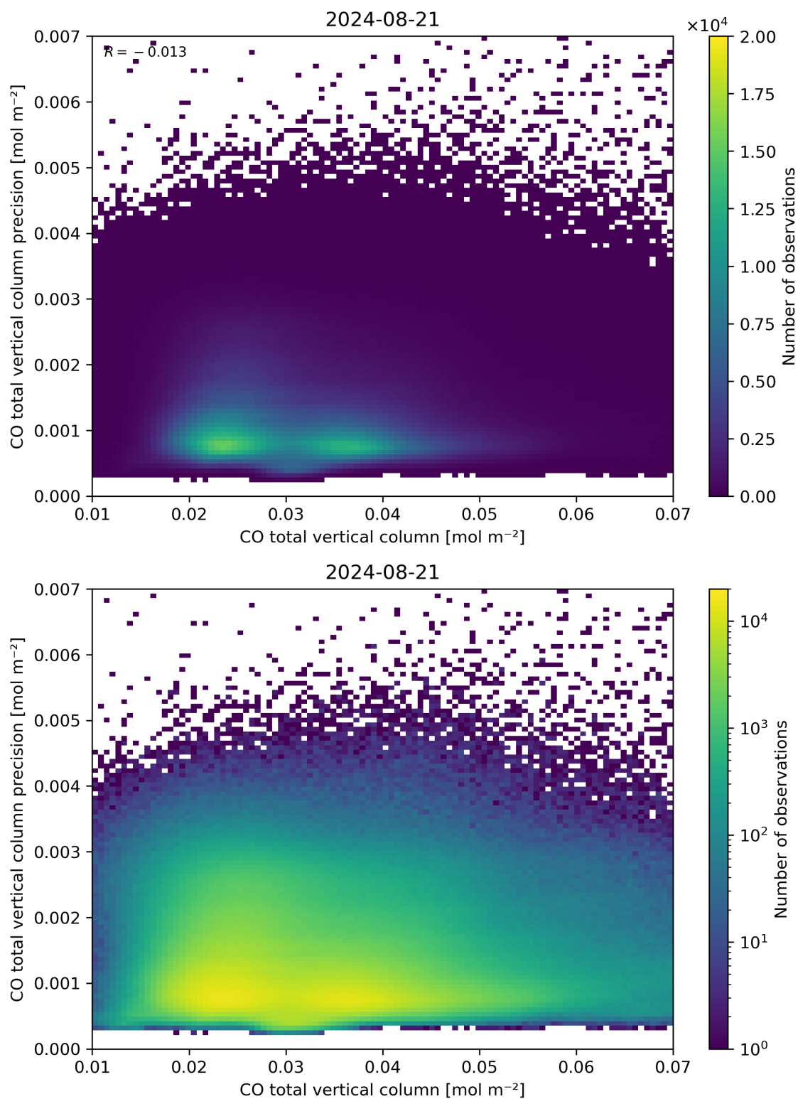
Figure 34: Scatter density plot of “CO total vertical column” against “CO total vertical column precision” for 2024-08-21 to 2024-08-22.
