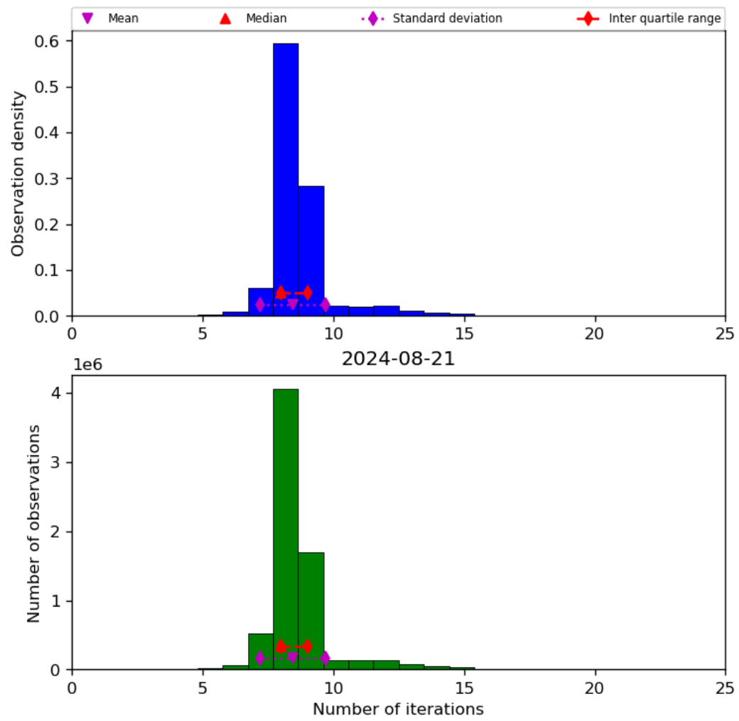
Figure 24: Histogram of “Number of iterations” for 2024-08-21 to 2024-08-22
