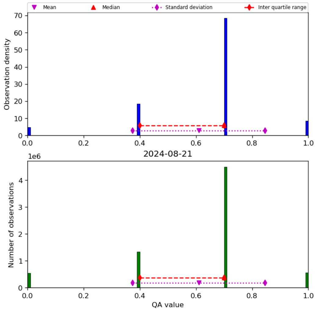
Figure 17: Histogram of “QA value” for 2024-08-21 to 2024-08-22
