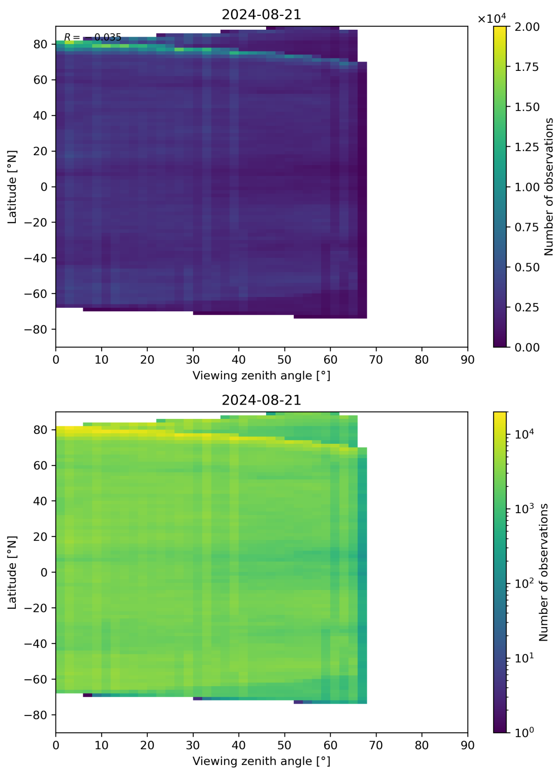
Figure 74: Scatter density plot of “Viewing zenith angle” against “Latitude” for 2024-08-21 to 2024-08-22.
