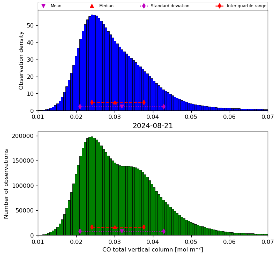
Figure 18: Histogram of “CO total vertical column” for 2024-08-21 to 2024-08-22
