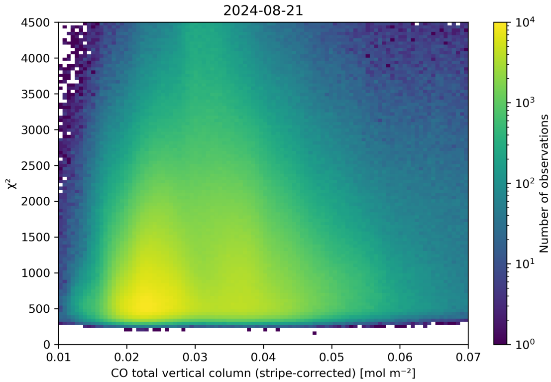
Figure 37: Scatter density plot of “CO total vertical column (stripe-corrected)” against “ \chi^2 ” for 2024-08-21 to 2024-08-22.
