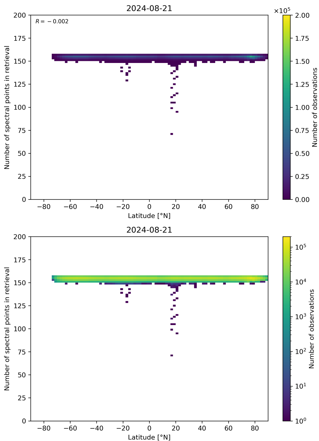
Figure 57: Scatter density plot of “Latitude” against “Number of spectral points in retrieval” for 2024-08-21 to 2024-08-22.
