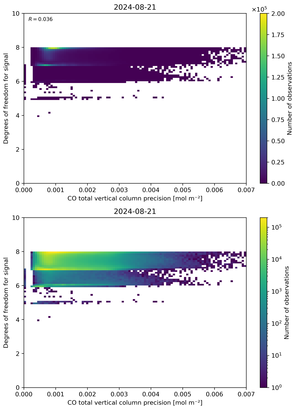
Figure 45: Scatter density plot of “CO total vertical column precision” against “Degrees of freedom for signal” for 2024-08-21 to 2024-08-22.
