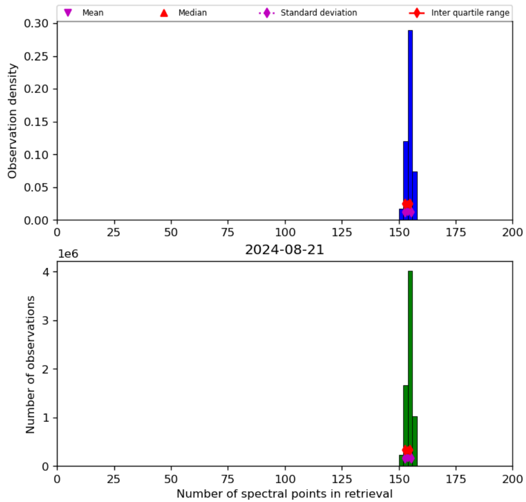
Figure 21: Histogram of “Number of spectral points in retrieval” for 2024-08-21 to 2024-08-22
