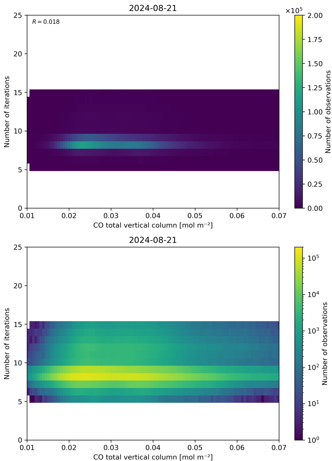
Figure 42: Scatter density plot of “CO total vertical column” against “Number of iterations” for 2024-08-21 to 2024-08-22.
