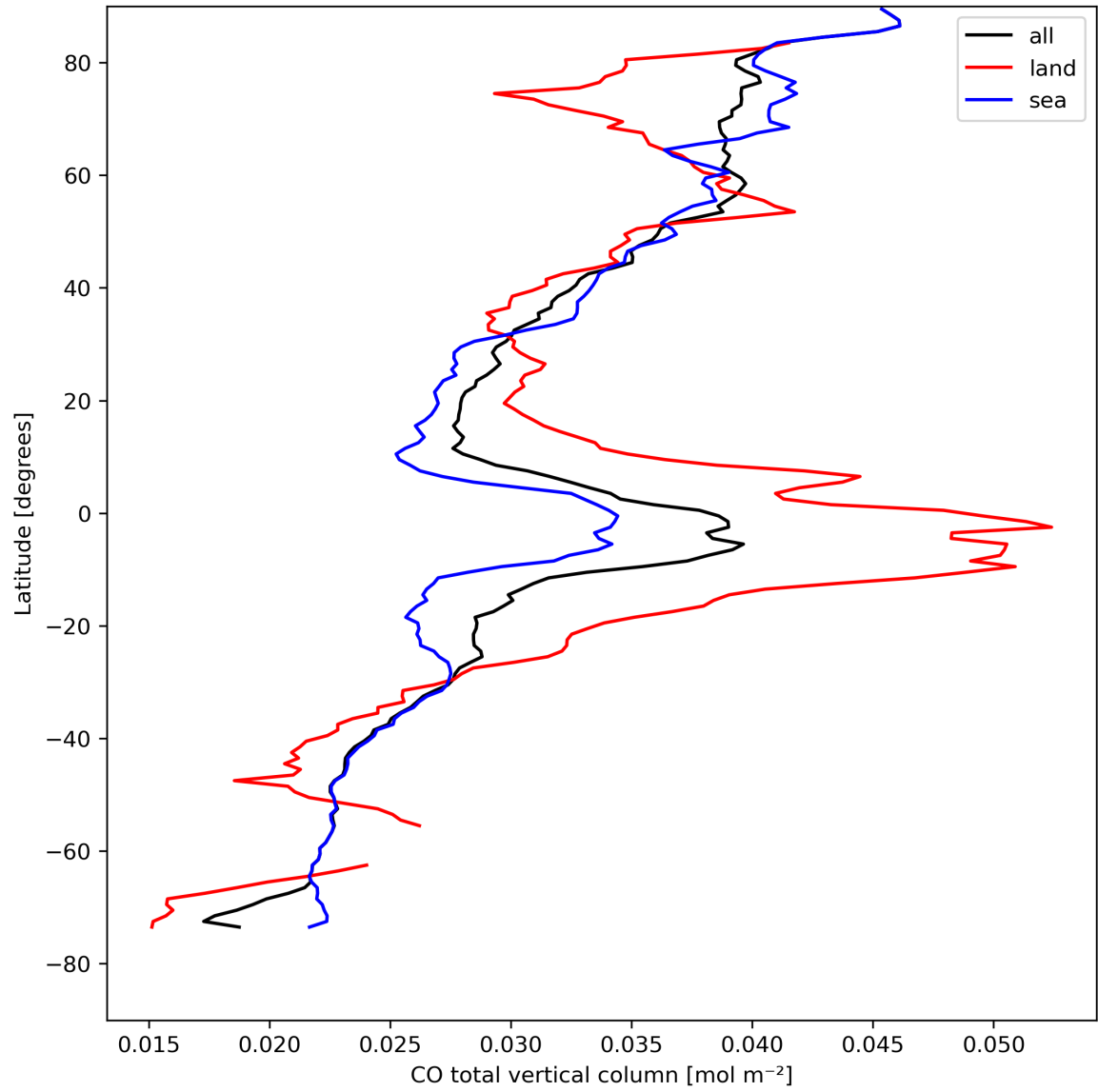
Figure 10: Zonal average of “CO total vertical column” for 2024-08-21 to 2024-08-22.
