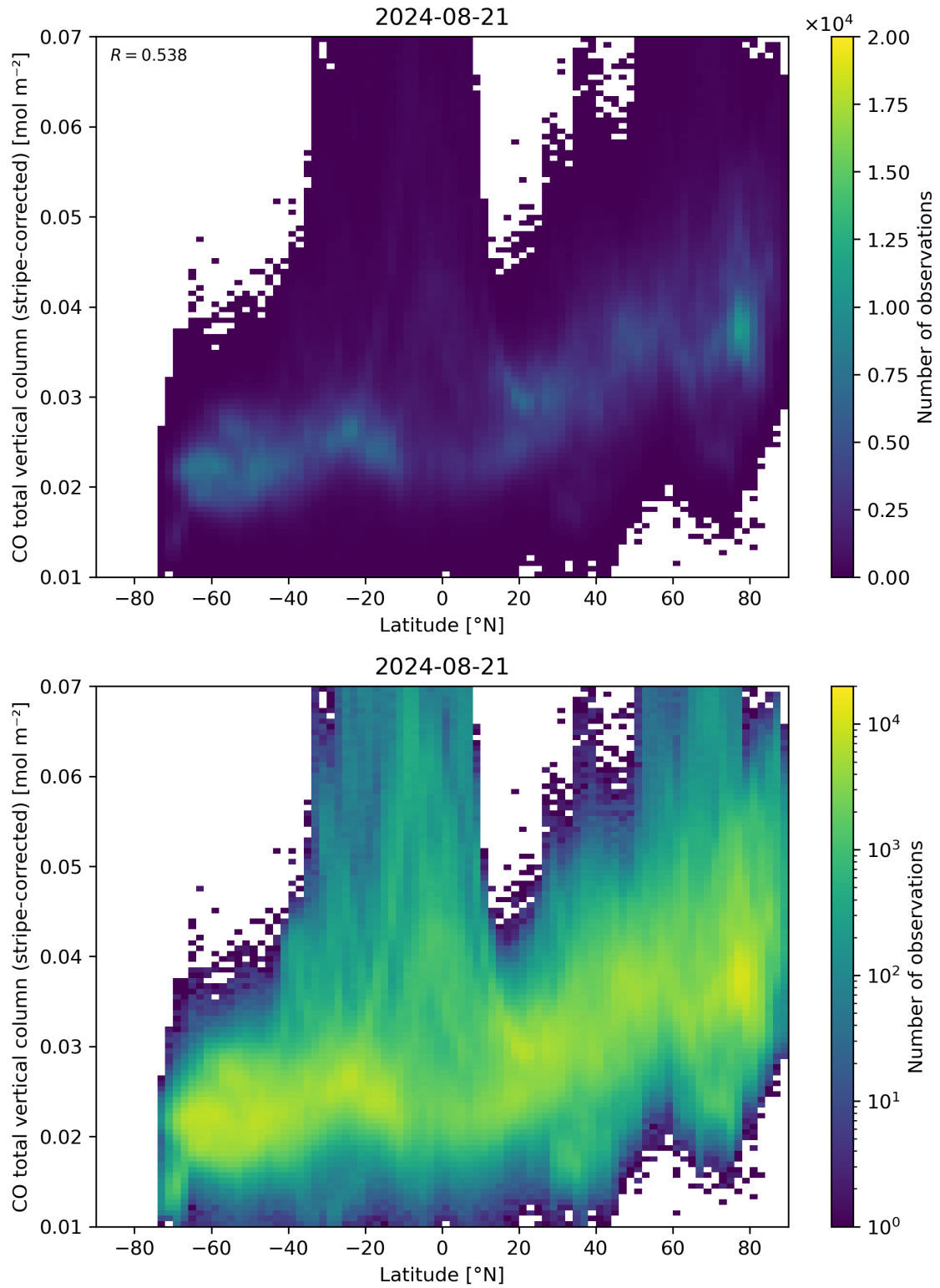
Figure 52: Scatter density plot of “Latitude” against “CO total vertical column (stripe-corrected)” for 2024-08-21 to 2024-08-22.
