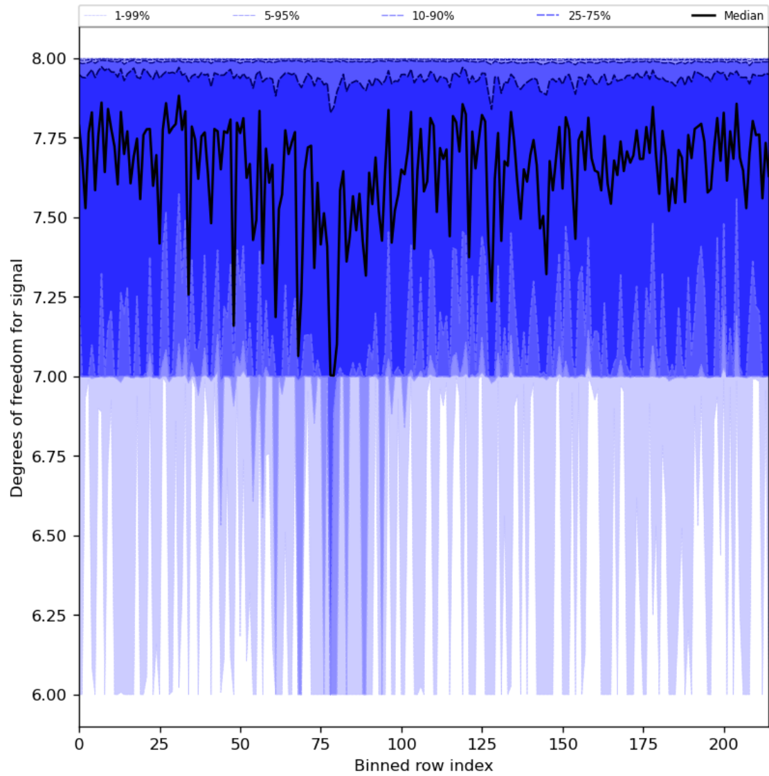
Figure 31: Along track statistics of “Degrees of freedom for signal” for 2024-08-21 to 2024-08-22
