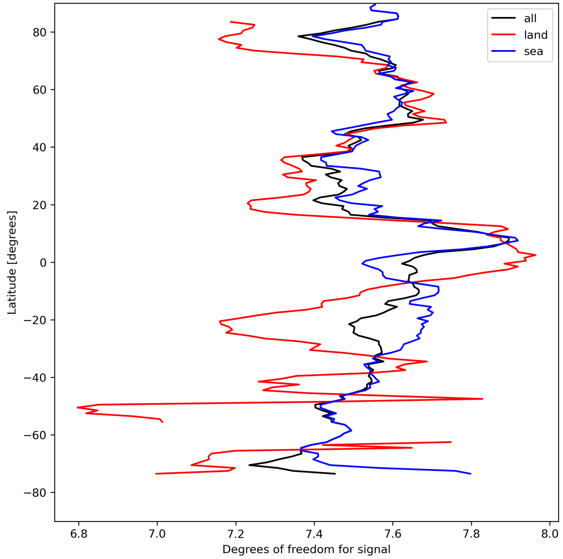
Figure 15: Zonal average of “Degrees of freedom for signal” for 2024-08-21 to 2024-08-22.
