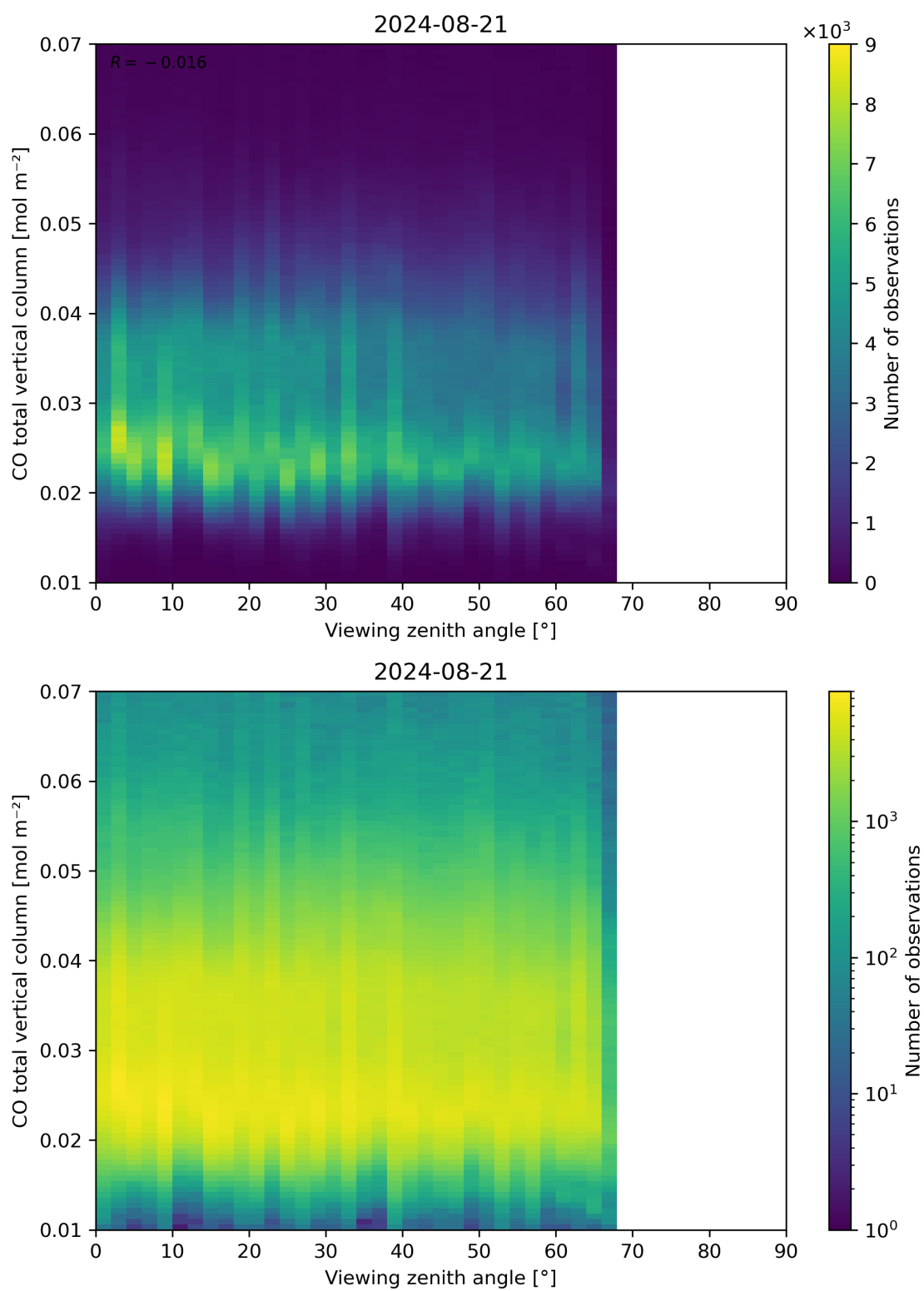
Figure 69: Scatter density plot of “Viewing zenith angle” against “CO total vertical column” for 2024-08-21 to 2024-08-22.
