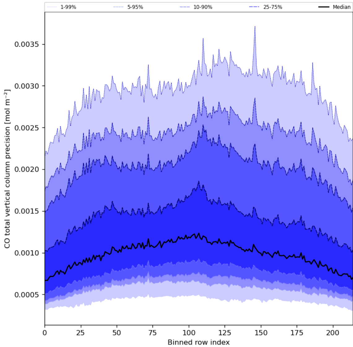
Figure 28: Along track statistics of “CO total vertical column precision” for 2024-08-21 to 2024-08-22
