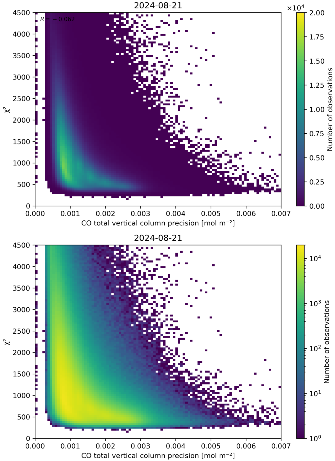
Figure 44: Scatter density plot of “CO total vertical column precision” against “ \chi^2 ” for 2024-08-21 to 2024-08-22.
