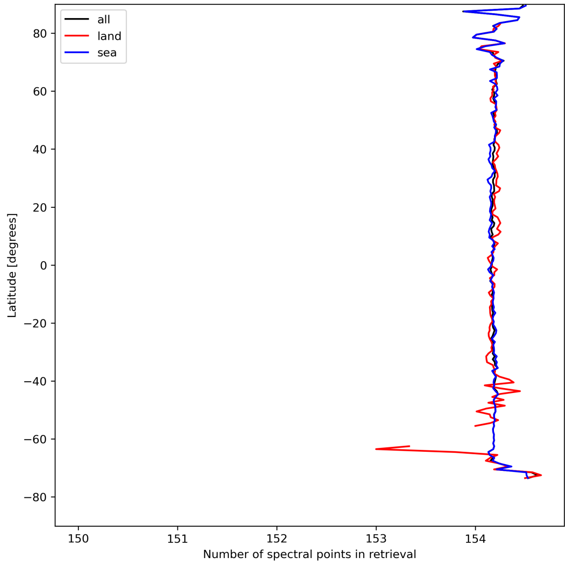
Figure 13: Zonal average of “Number of spectral points in retrieval” for 2024-08-21 to 2024-08-22.
