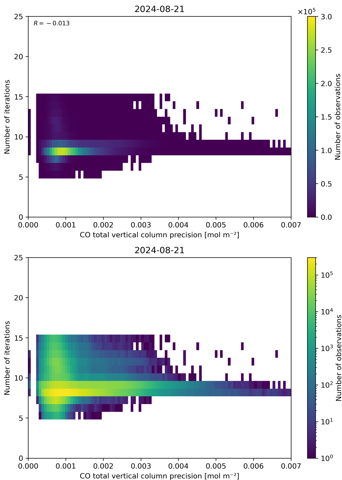
Figure 46: Scatter density plot of “CO total vertical column precision” against “Number of iterations” for 2024-08-21 to 2024-08-22.
