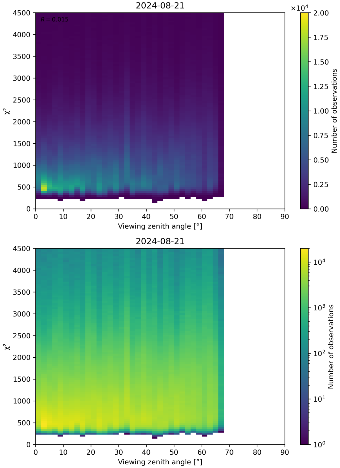
Figure 72: Scatter density plot of “Viewing zenith angle” against “ \chi^2 ” for 2024-08-21 to 2024-08-22.
