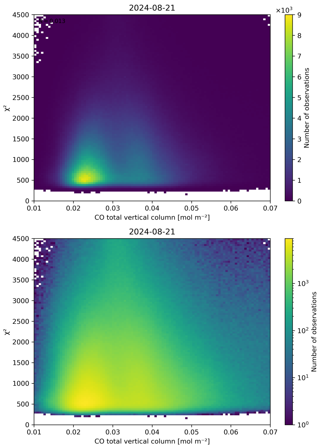
Figure 35: Scatter density plot of “CO total vertical column” against “ \chi^2 ” for 2024-08-21 to 2024-08-22.
