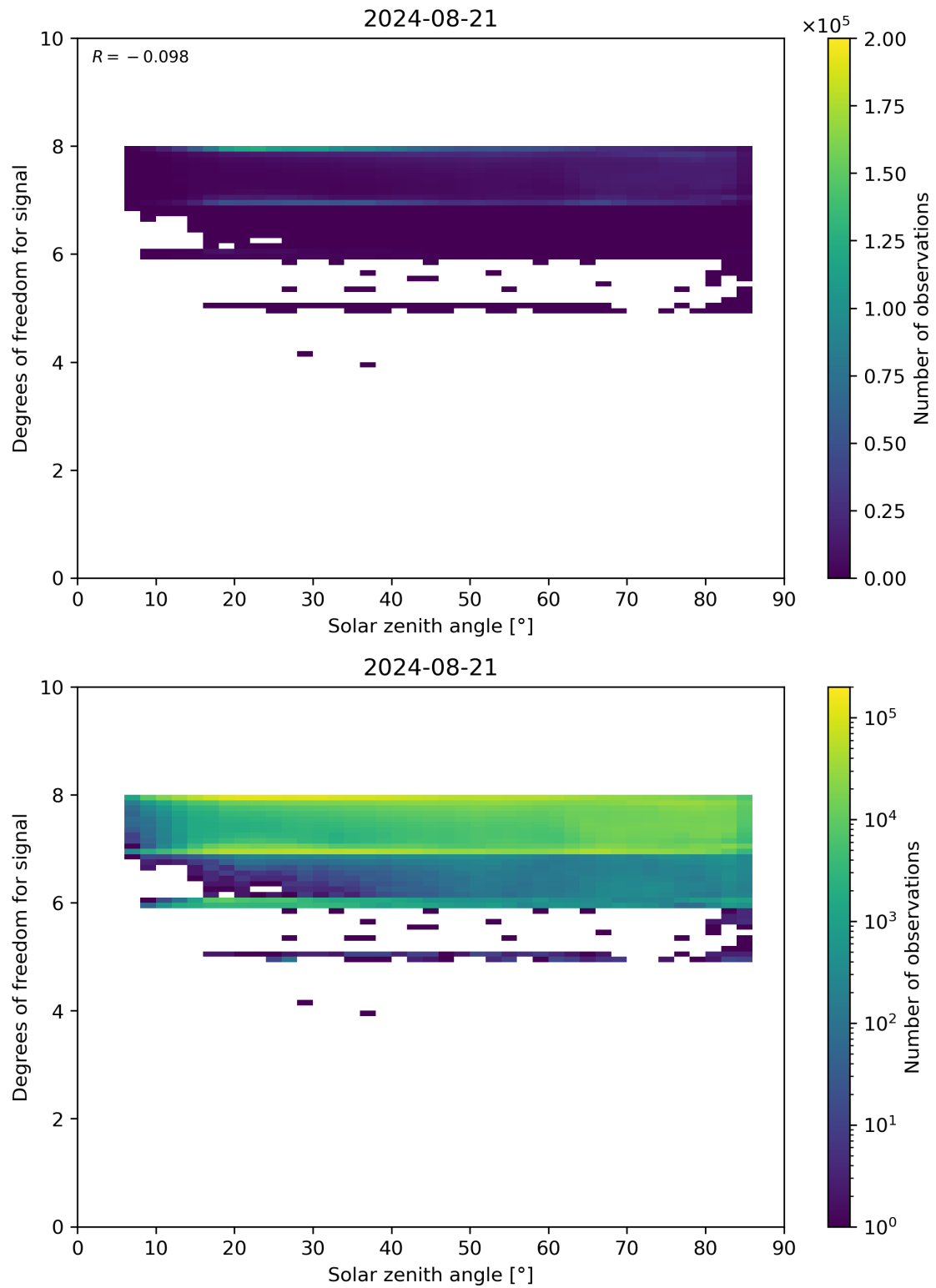
Figure 65: Scatter density plot of “Solar zenith angle” against “Degrees of freedom for signal” for 2024-08-21 to 2024-08-22.
