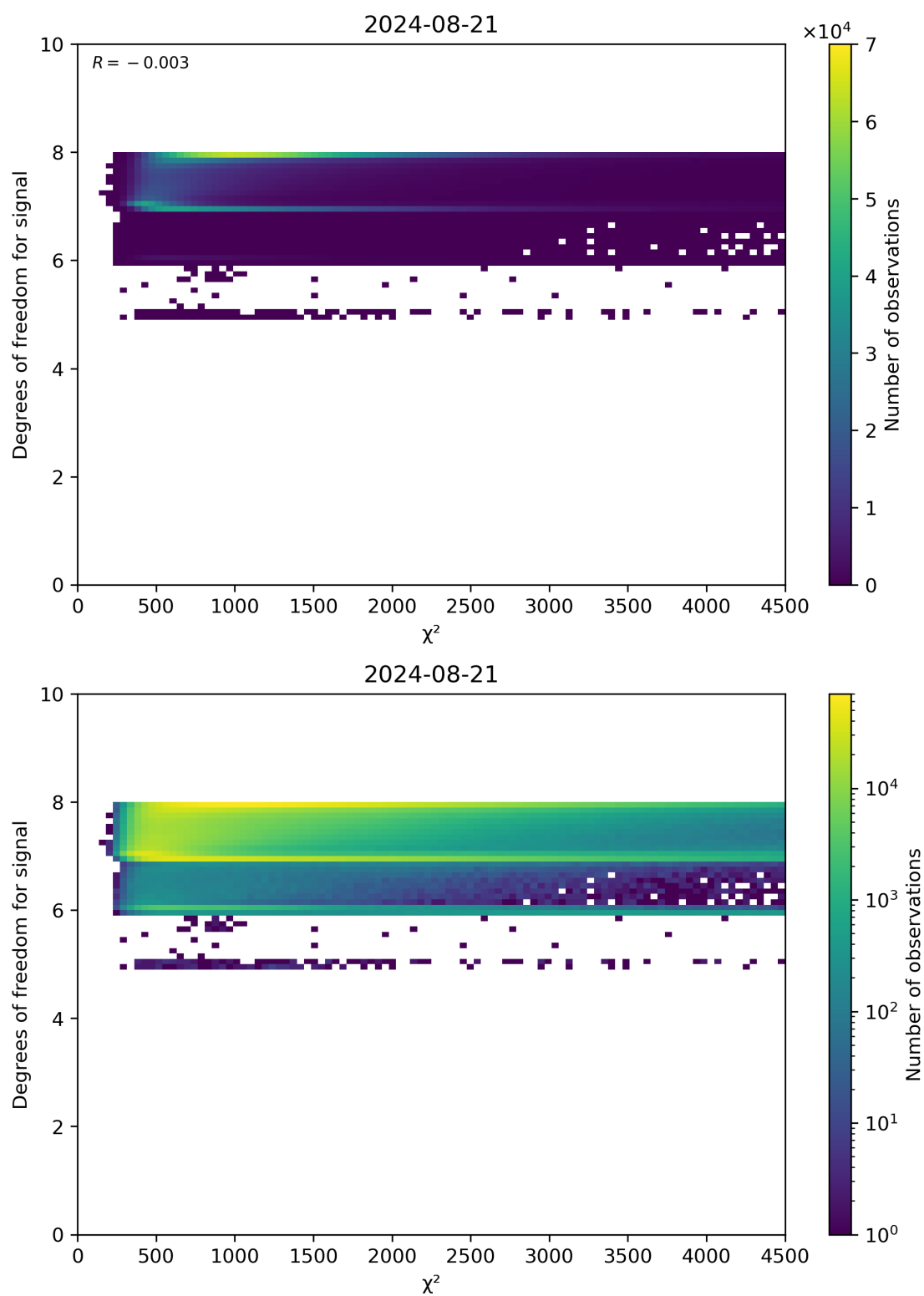
Figure 48: Scatter density plot of “ \chi^2 ” against “Degrees of freedom for signal” for 2024-08-21 to 2024-08-22.
