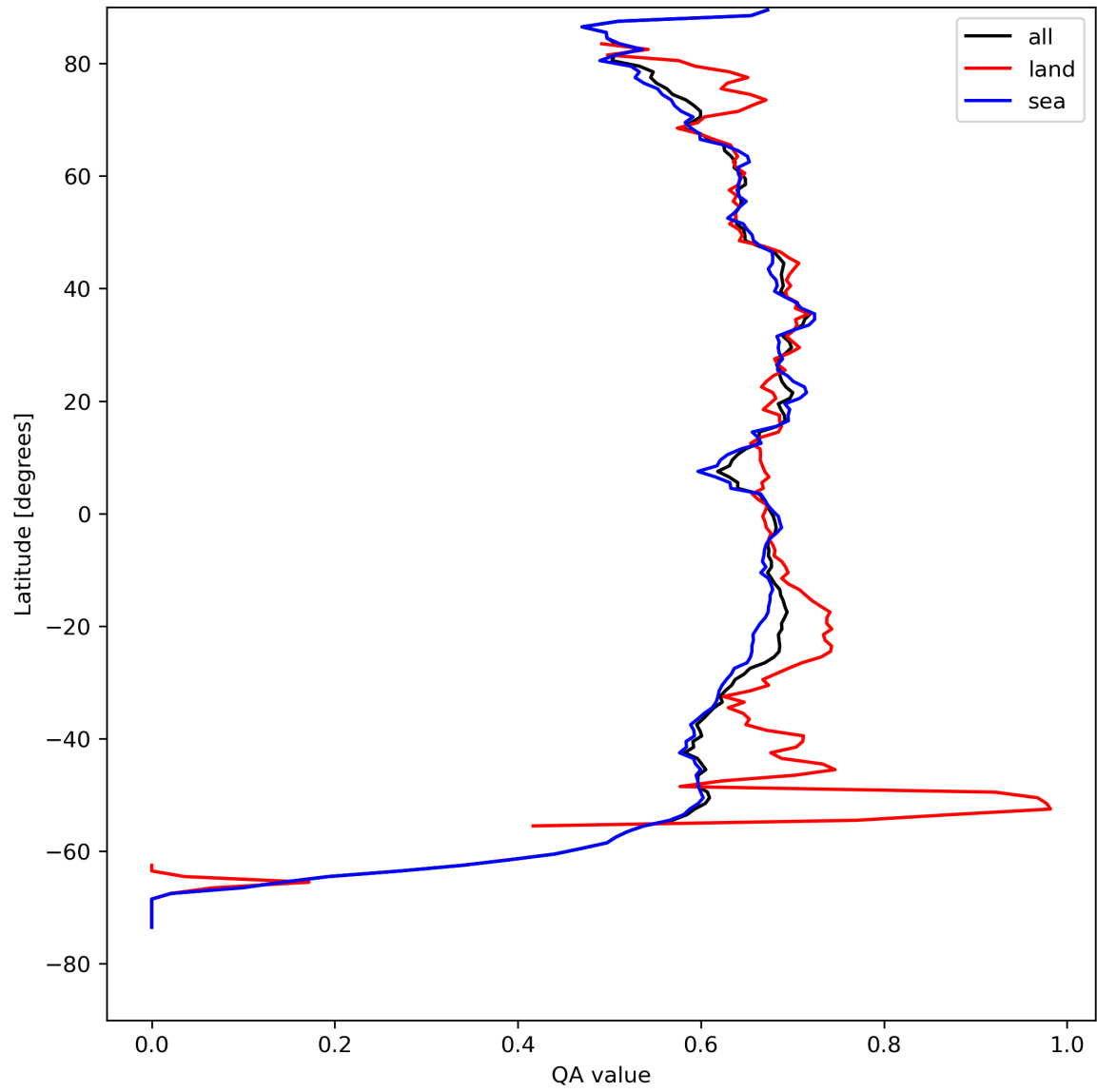
Figure 9: Zonal average of “QA value” for 2024-08-21 to 2024-08-22.
