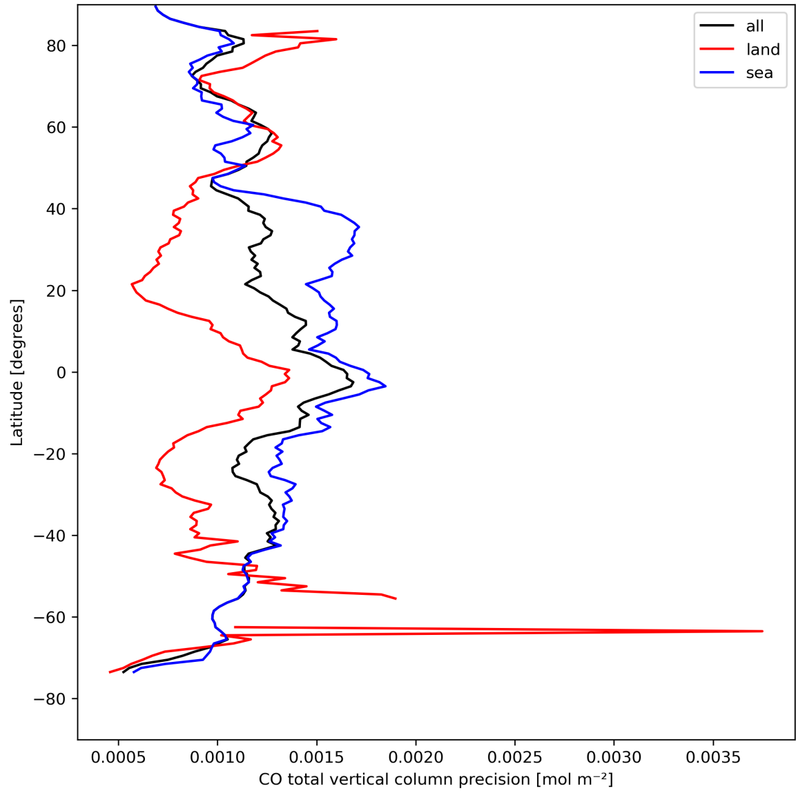
Figure 12: Zonal average of “CO total vertical column precision” for 2024-08-21 to 2024-08-22.
