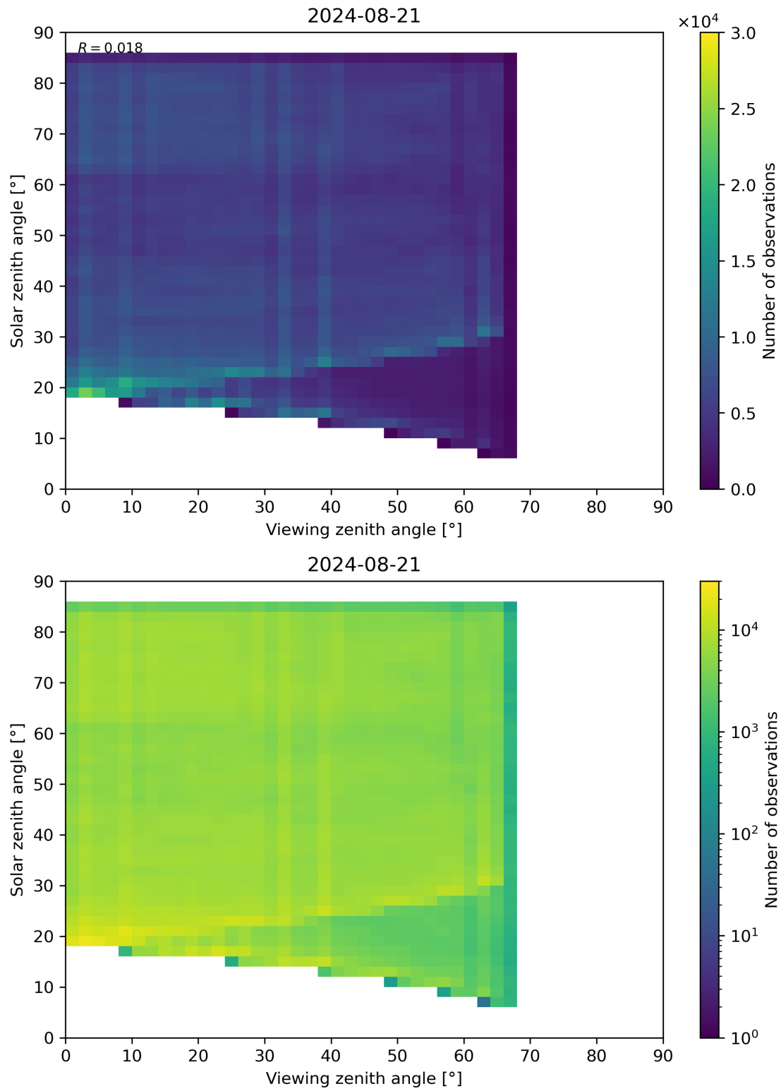
Figure 77: Scatter density plot of “Viewing zenith angle” against “Solar zenith angle” for 2024-08-21 to 2024-08-22.
