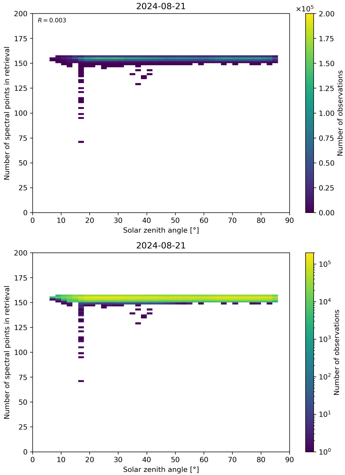
Figure 68: Scatter density plot of “Solar zenith angle” against “Number of spectral points in retrieval” for 2024-08-21 to 2024-08-22.
