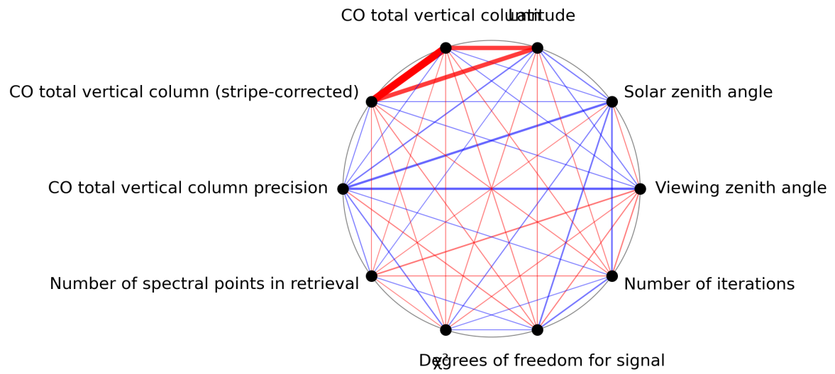
Figure 1: Map of correlation graph for 2024-08-21 to 2024-08-22.
