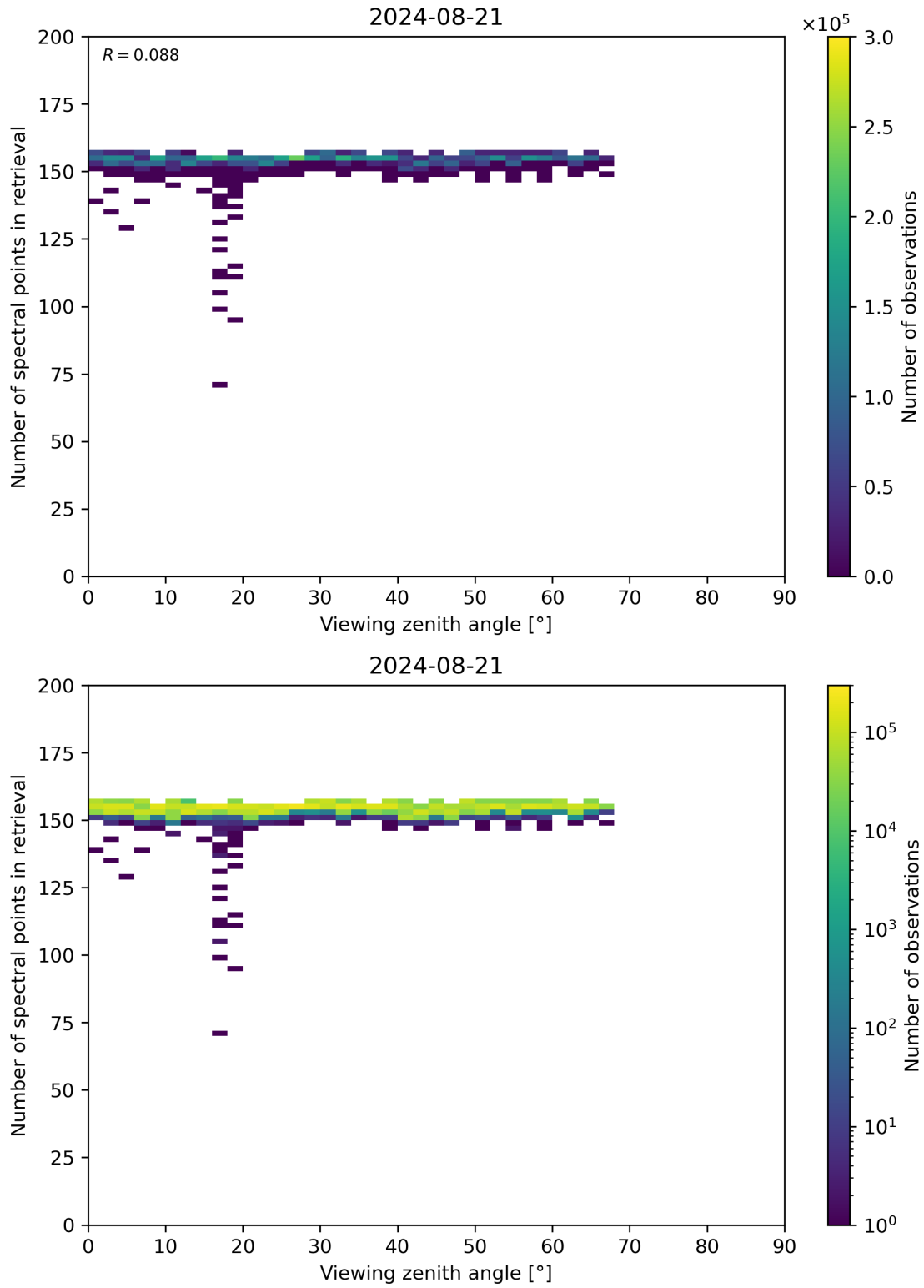
Figure 76: Scatter density plot of “Viewing zenith angle” against “Number of spectral points in retrieval” for 2024-08-21 to 2024-08-22.
