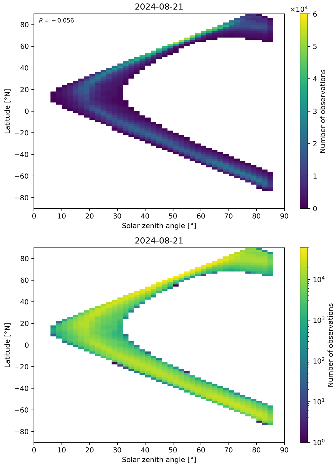
Figure 66: Scatter density plot of “Solar zenith angle” against “Latitude” for 2024-08-21 to 2024-08-22.
