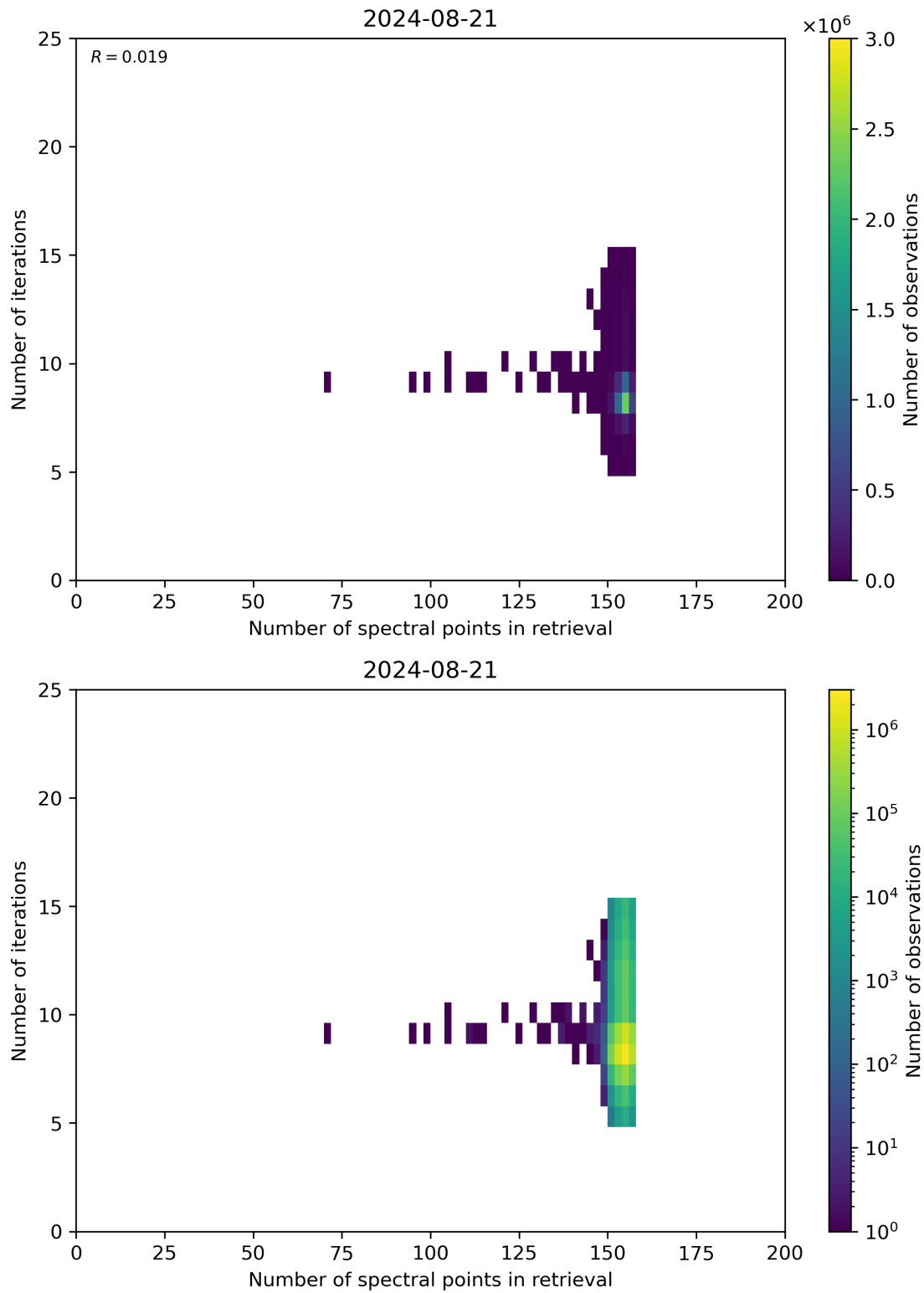
Figure 60: Scatter density plot of “Number of spectral points in retrieval” against “Number of iterations” for 2024-08-21 to 2024-08-22.
