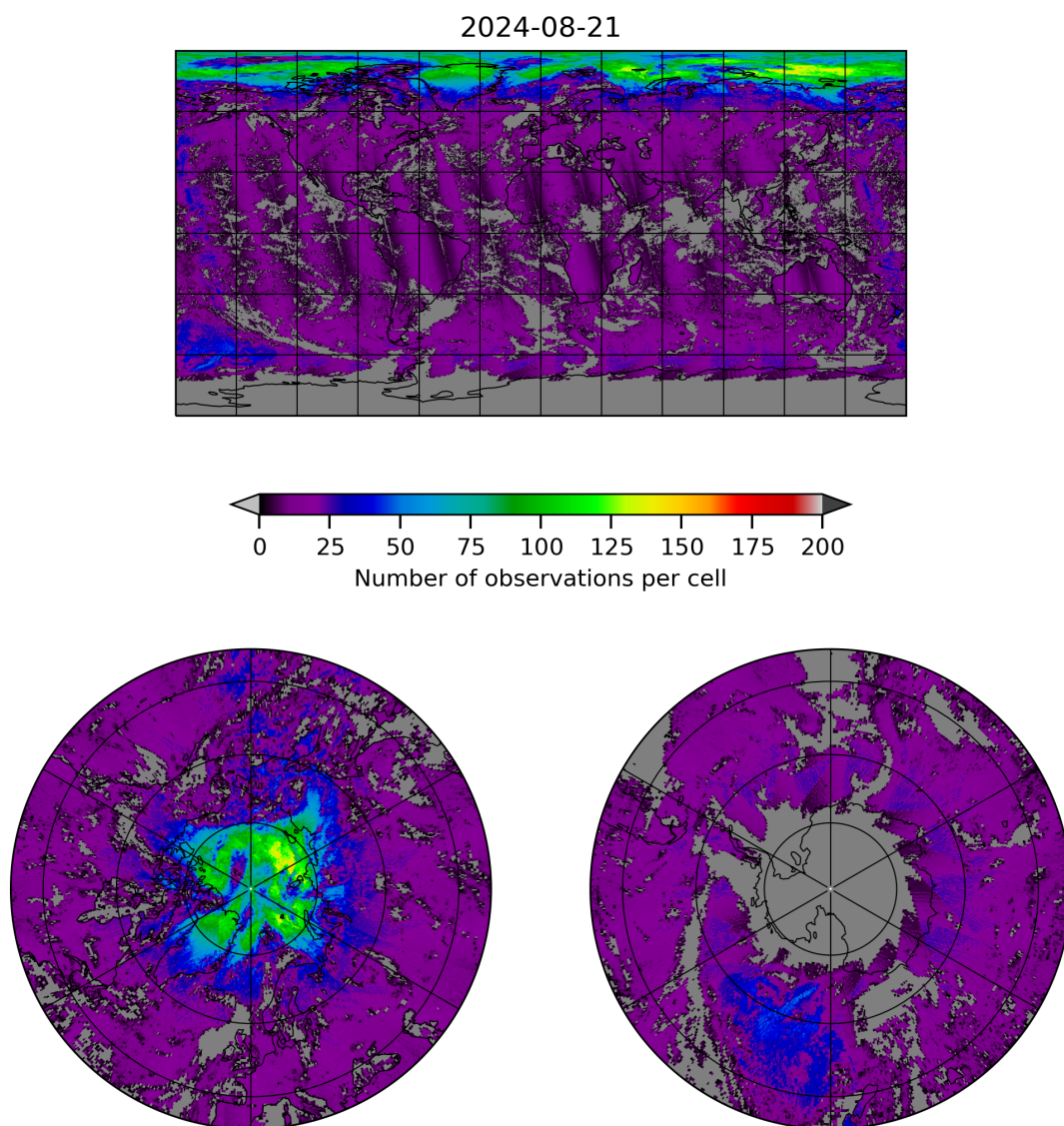
Figure 8: Map of the number of observations for 2024-08-21 to 2024-08-22
