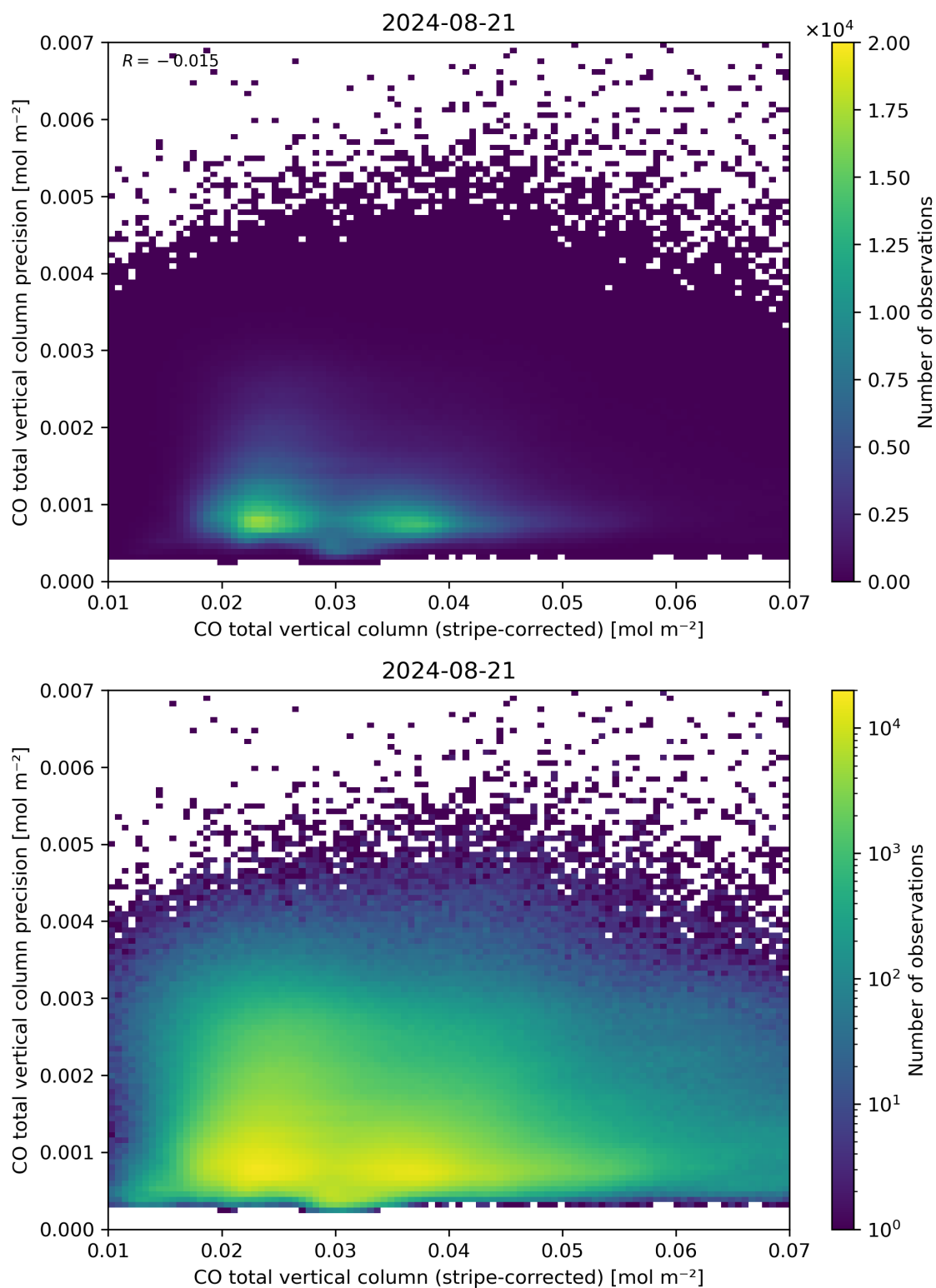
Figure 36: Scatter density plot of “CO total vertical column (stripe-corrected)” against “CO total vertical column precision” for 2024-08-21 to 2024-08-22.
