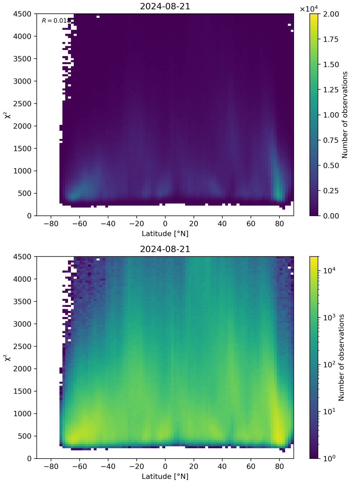
Figure 54: Scatter density plot of “Latitude” against “ \chi^2 ” for 2024-08-21 to 2024-08-22.
