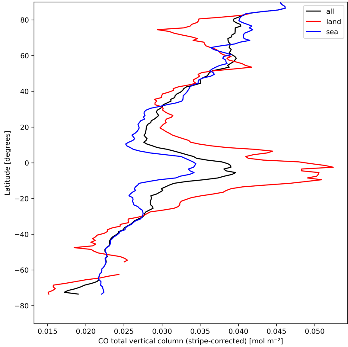
Figure 11: Zonal average of “CO total vertical column (stripe-corrected)” for 2024-08-21 to 2024-08-22.
