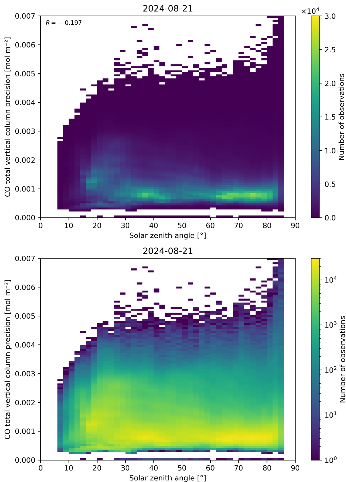
Figure 63: Scatter density plot of “Solar zenith angle” against “CO total vertical column precision” for 2024-08-21 to 2024-08-22.
