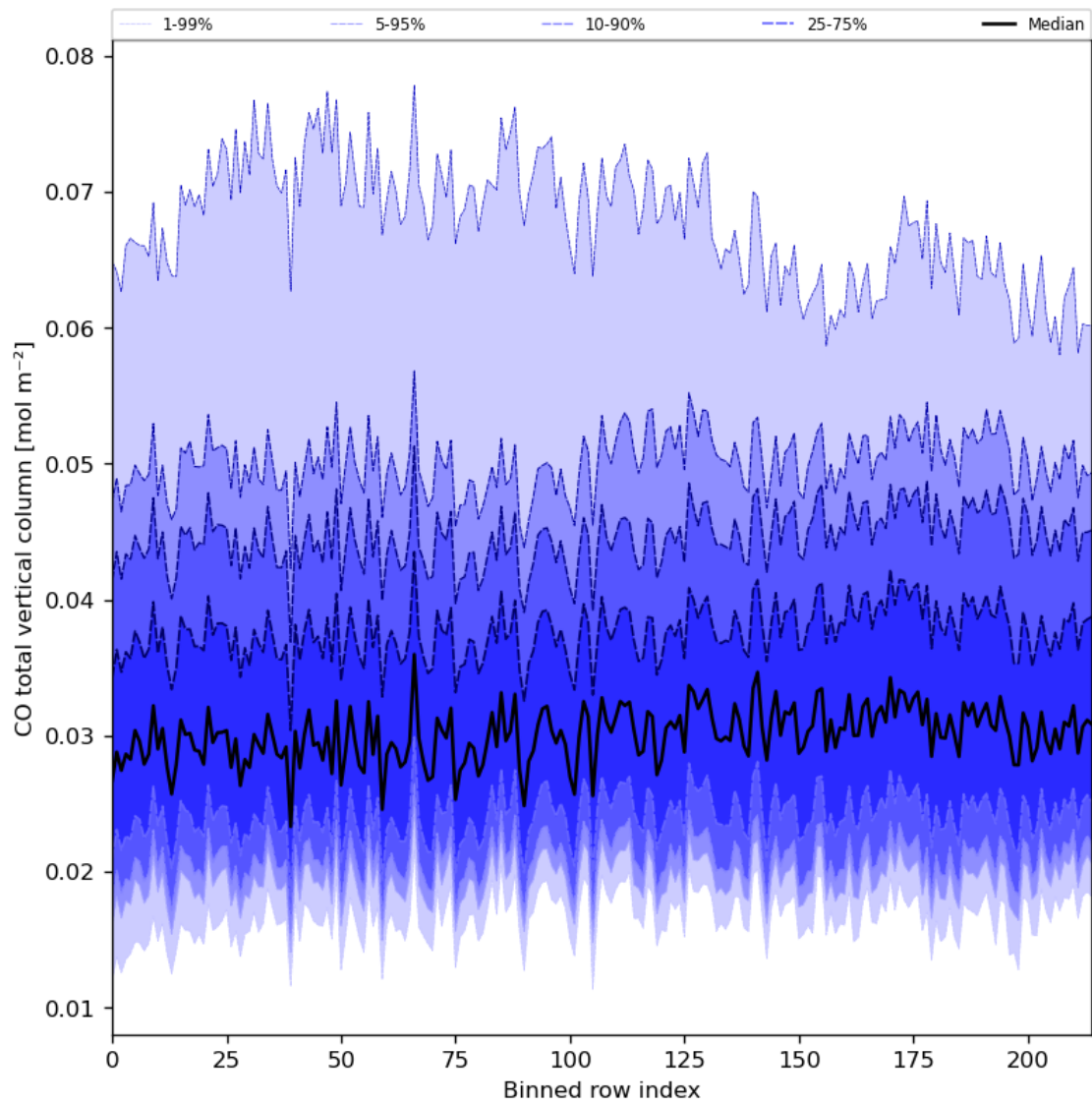
Figure 26: Along track statistics of “CO total vertical column” for 2024-08-21 to 2024-08-22
