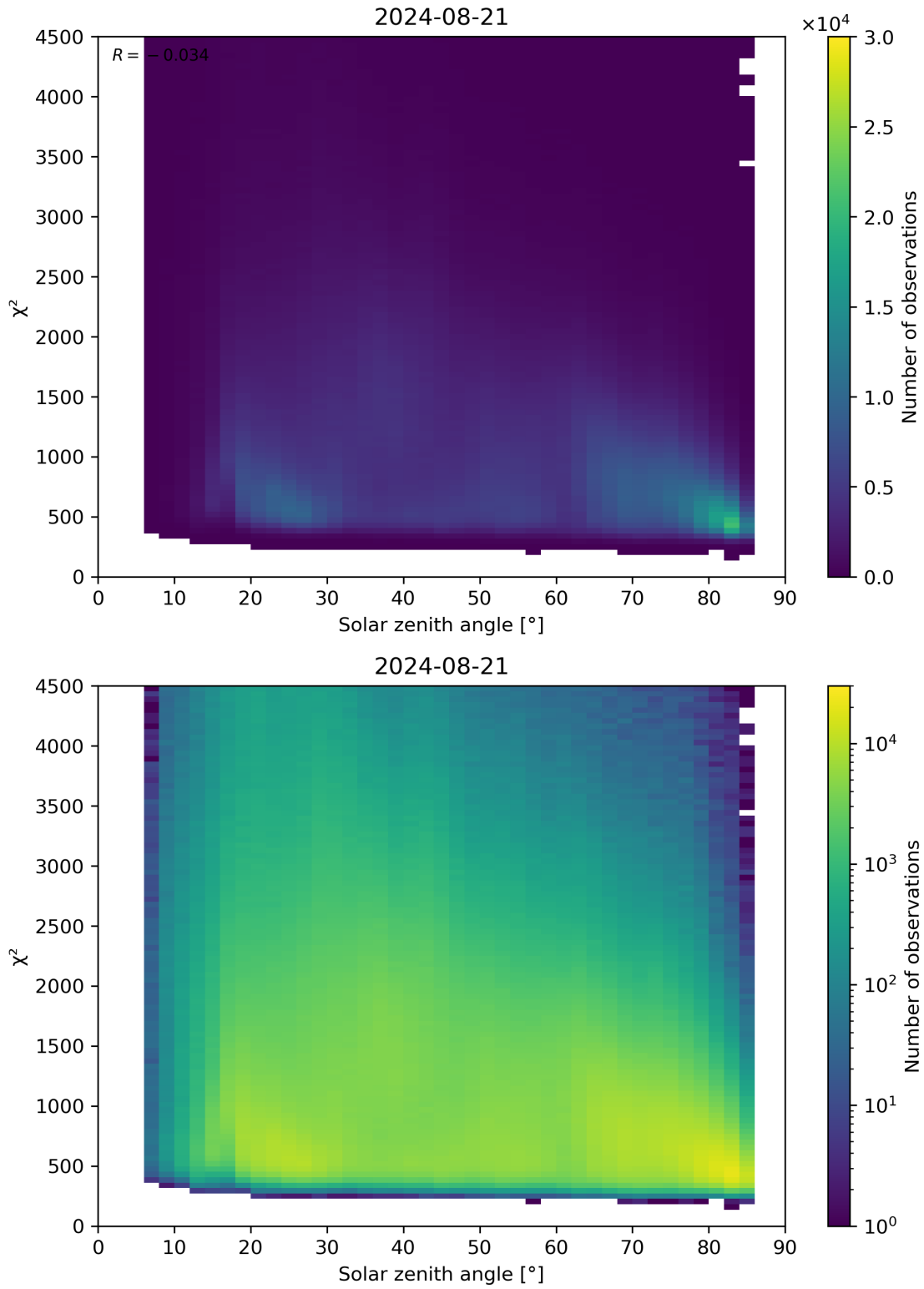
Figure 64: Scatter density plot of “Solar zenith angle” against “ \chi^2 ” for 2024-08-21 to 2024-08-22.
