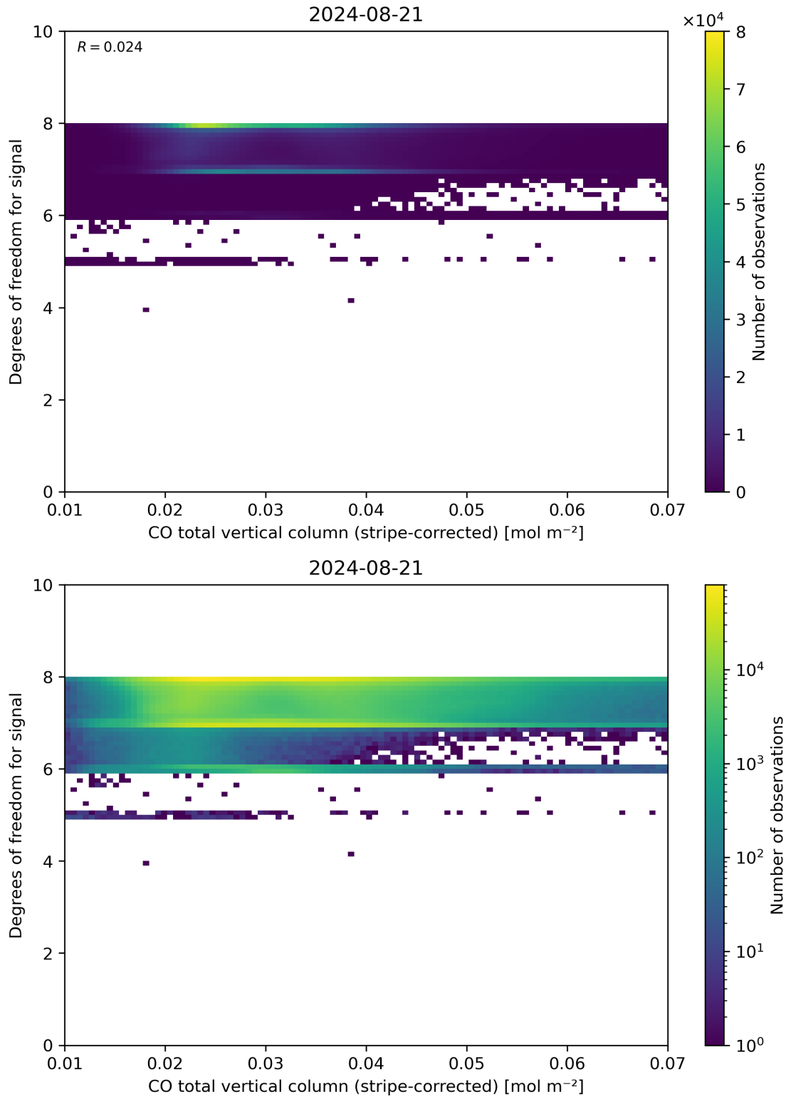
Figure 38: Scatter density plot of “CO total vertical column (stripe-corrected)” against “Degrees of freedom for signal” for 2024-08-21 to 2024-08-22.
