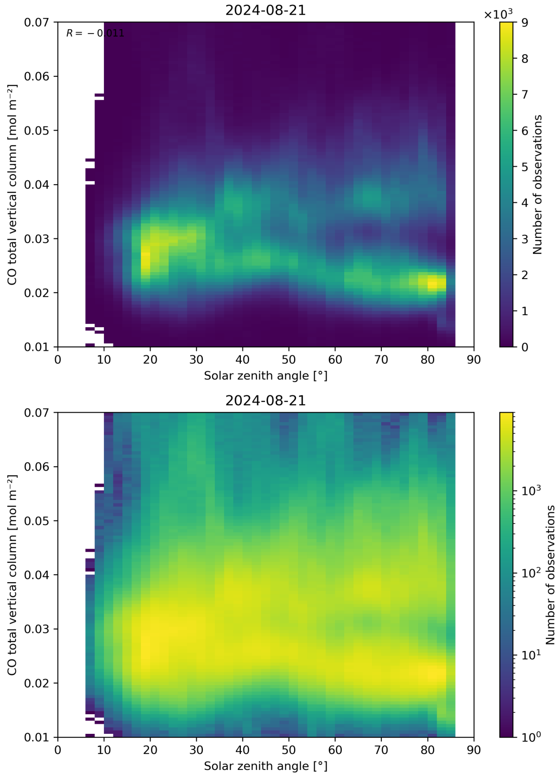
Figure 61: Scatter density plot of “Solar zenith angle” against “CO total vertical column” for 2024-08-21 to 2024-08-22.
