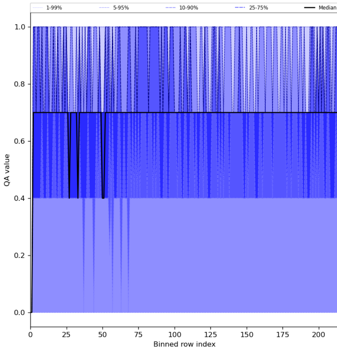
Figure 25: Along track statistics of “QA value” for 2024-08-21 to 2024-08-22
