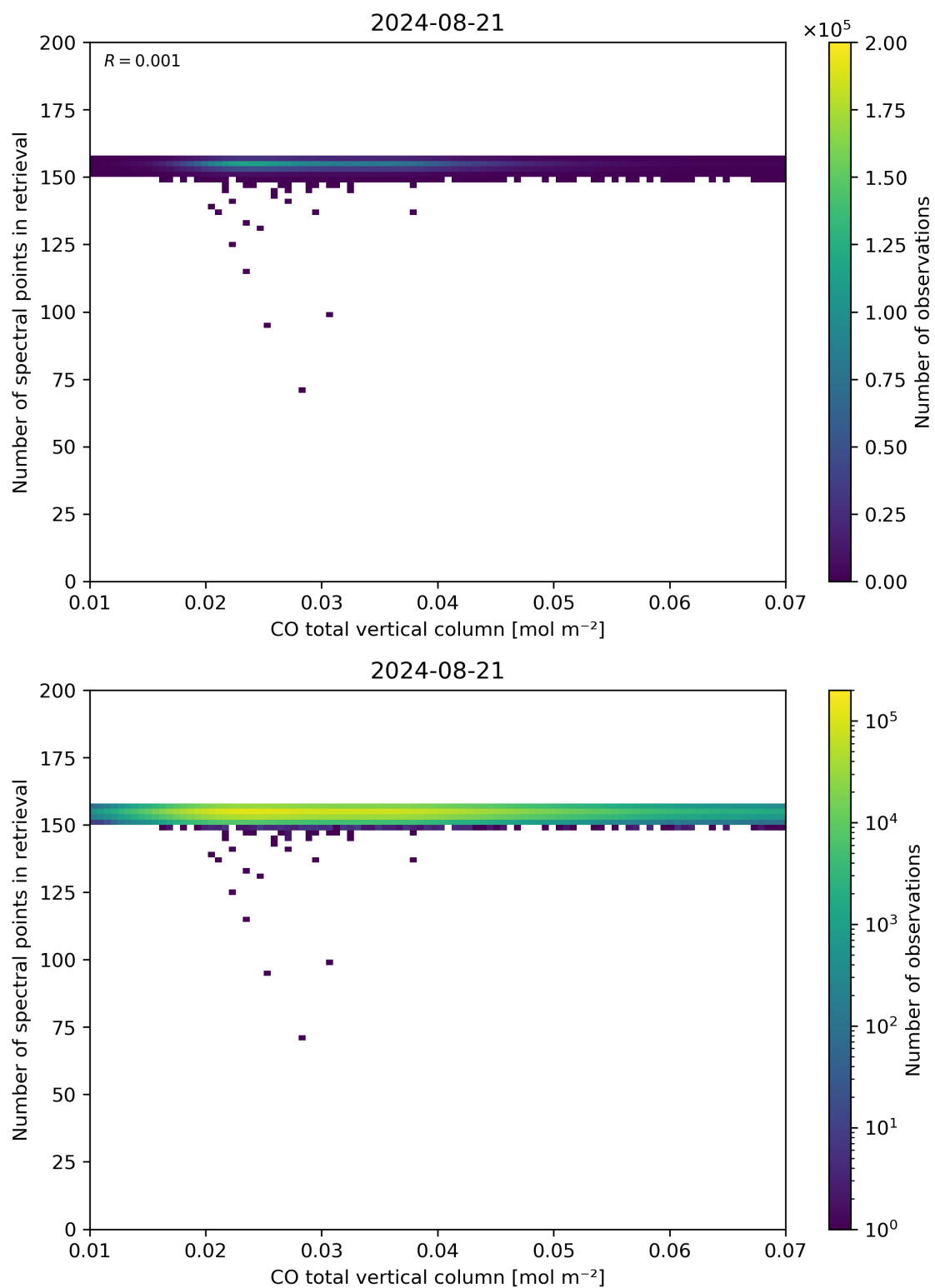
Figure 43: Scatter density plot of “CO total vertical column” against “Number of spectral points in retrieval” for 2024-08-21 to 2024-08-22.
