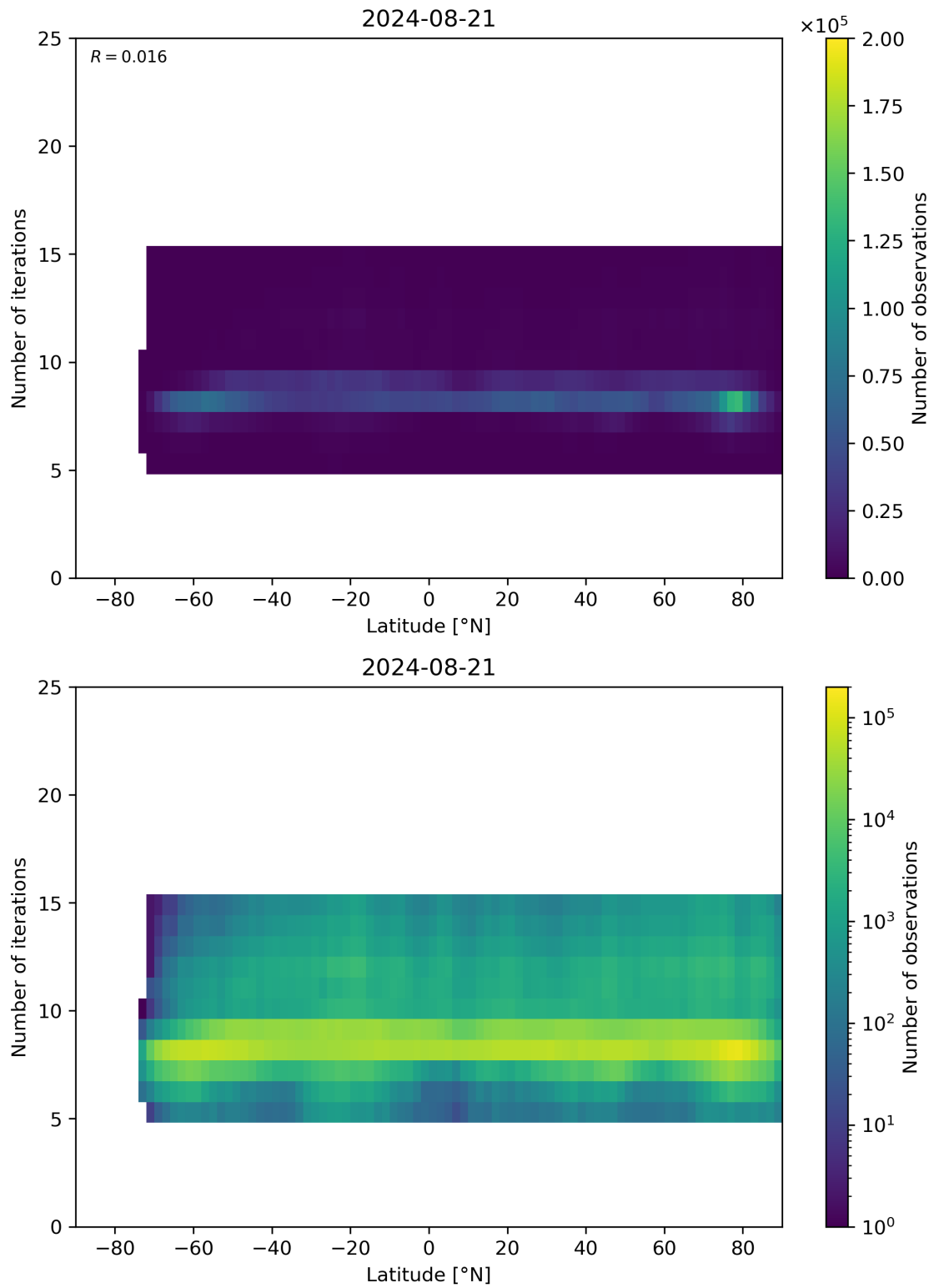
Figure 56: Scatter density plot of “Latitude” against “Number of iterations” for 2024-08-21 to 2024-08-22.
