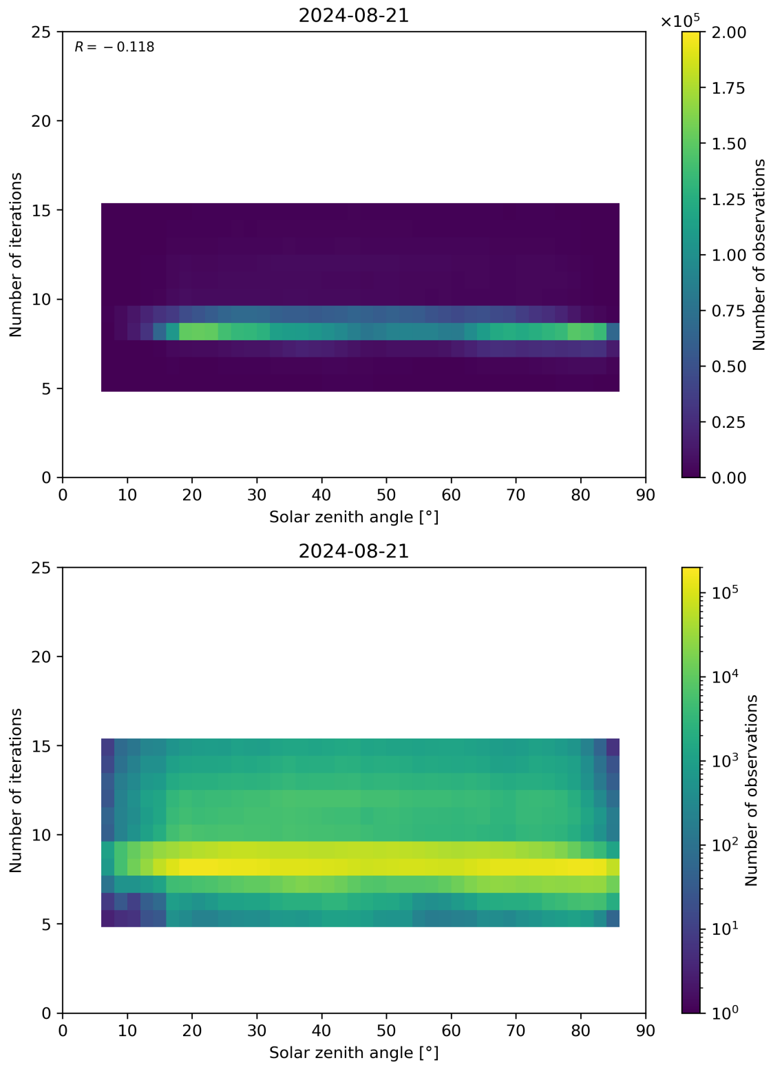
Figure 67: Scatter density plot of “Solar zenith angle” against “Number of iterations” for 2024-08-21 to 2024-08-22.
