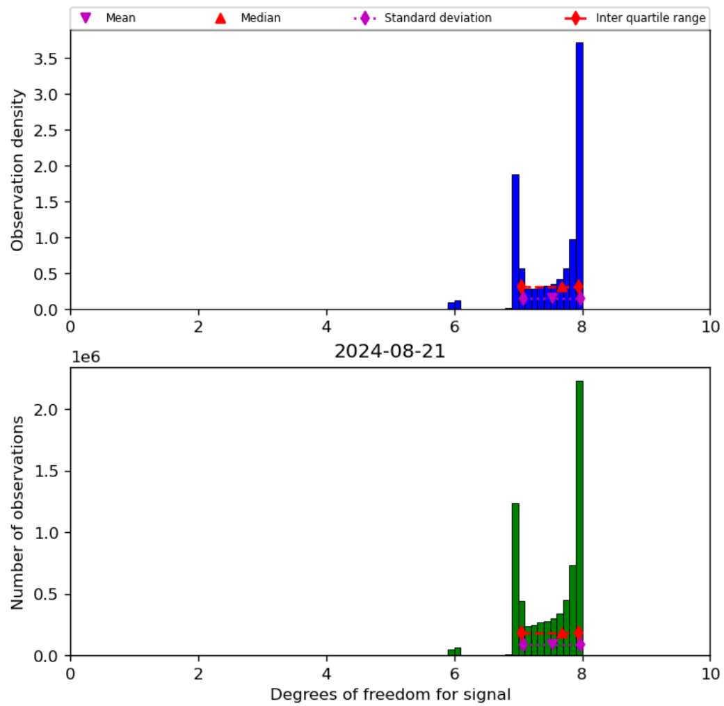
Figure 23: Histogram of “Degrees of freedom for signal” for 2024-08-21 to 2024-08-22
