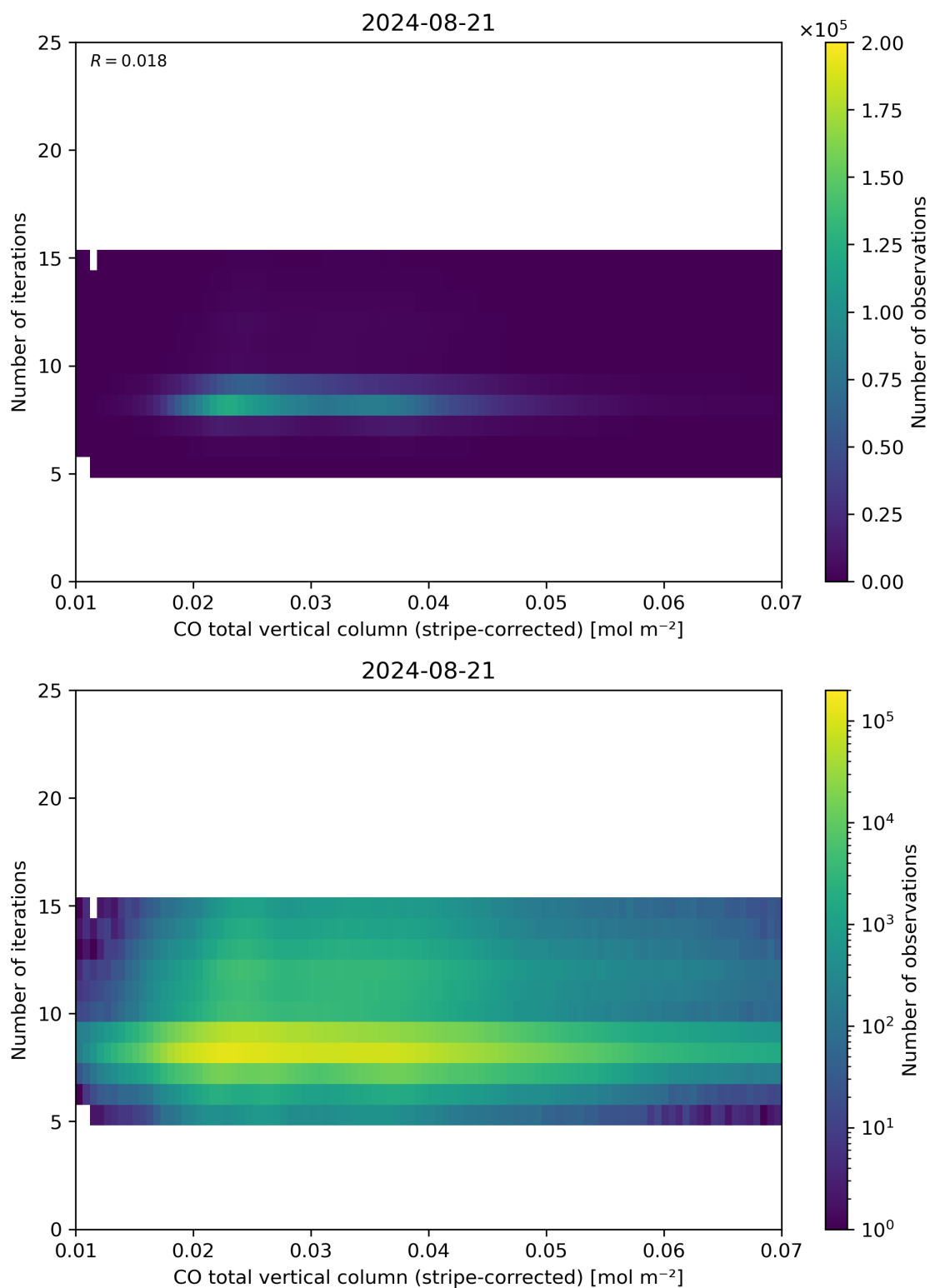
Figure 39: Scatter density plot of “CO total vertical column (stripe-corrected)” against “Number of iterations” for 2024-08-21 to 2024-08-22.
