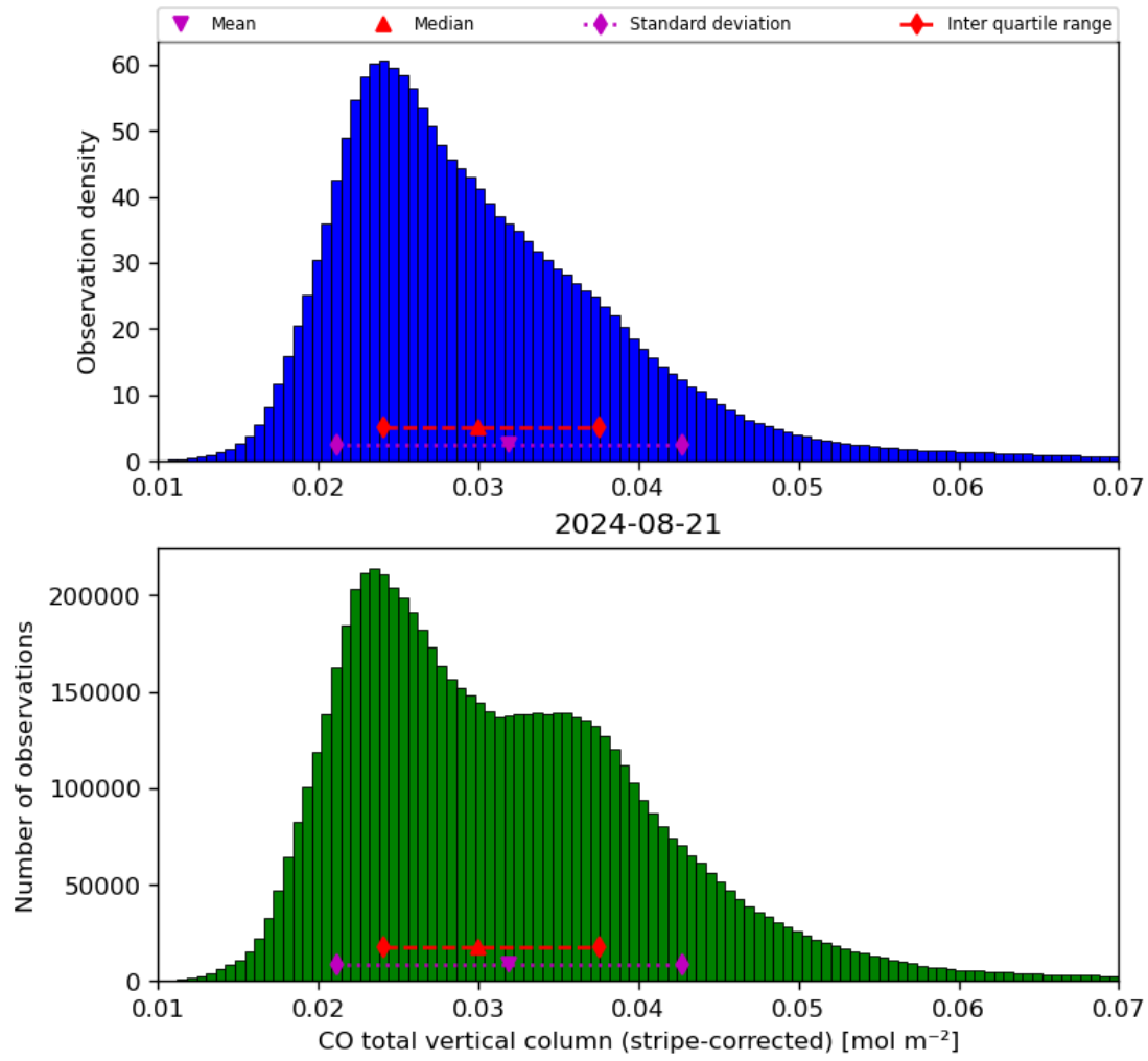
Figure 19: Histogram of “CO total vertical column (stripe-corrected)” for 2024-08-21 to 2024-08-22
