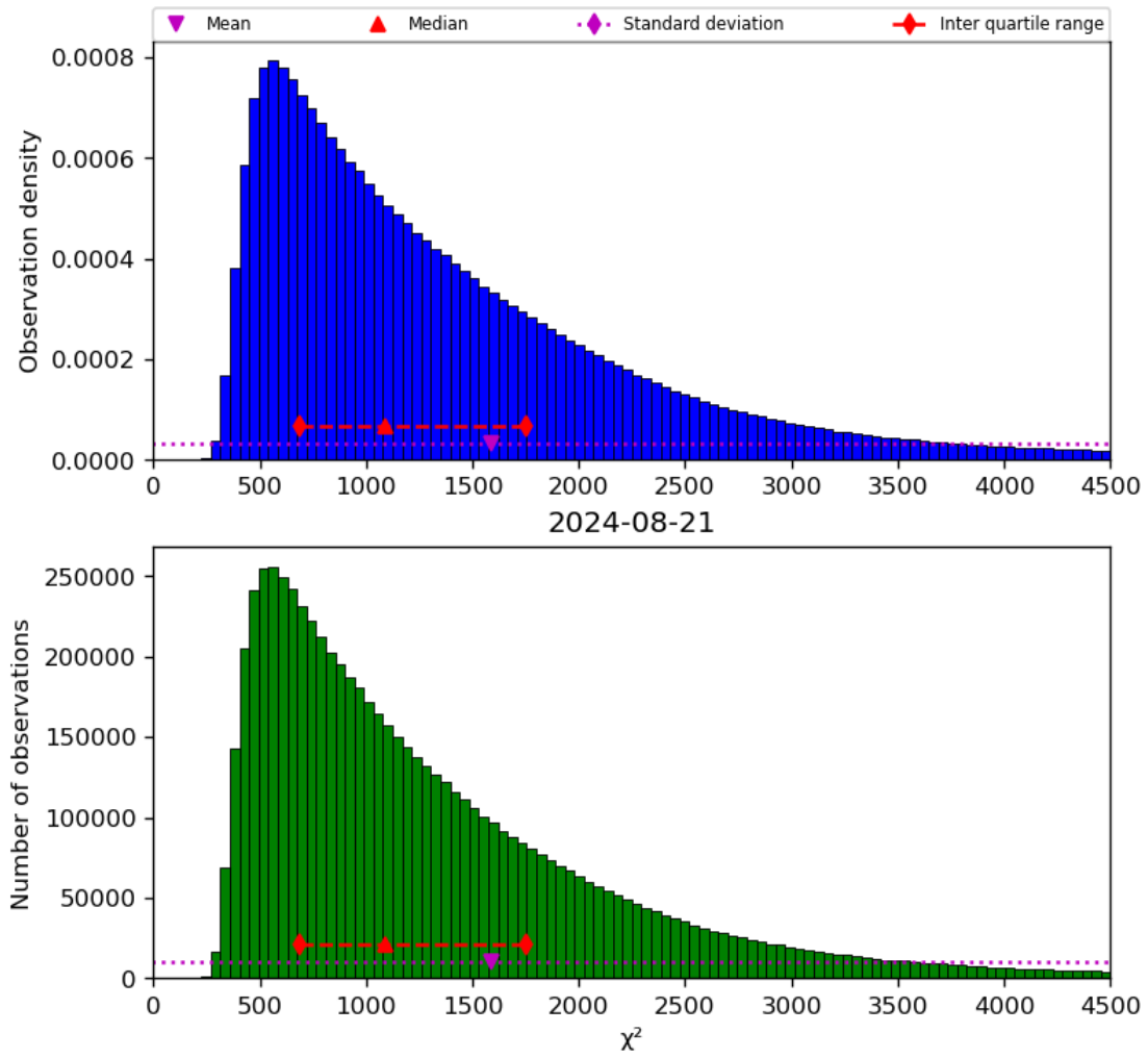
Figure 22: Histogram of “ \chi^2 ” for 2024-08-21 to 2024-08-22
