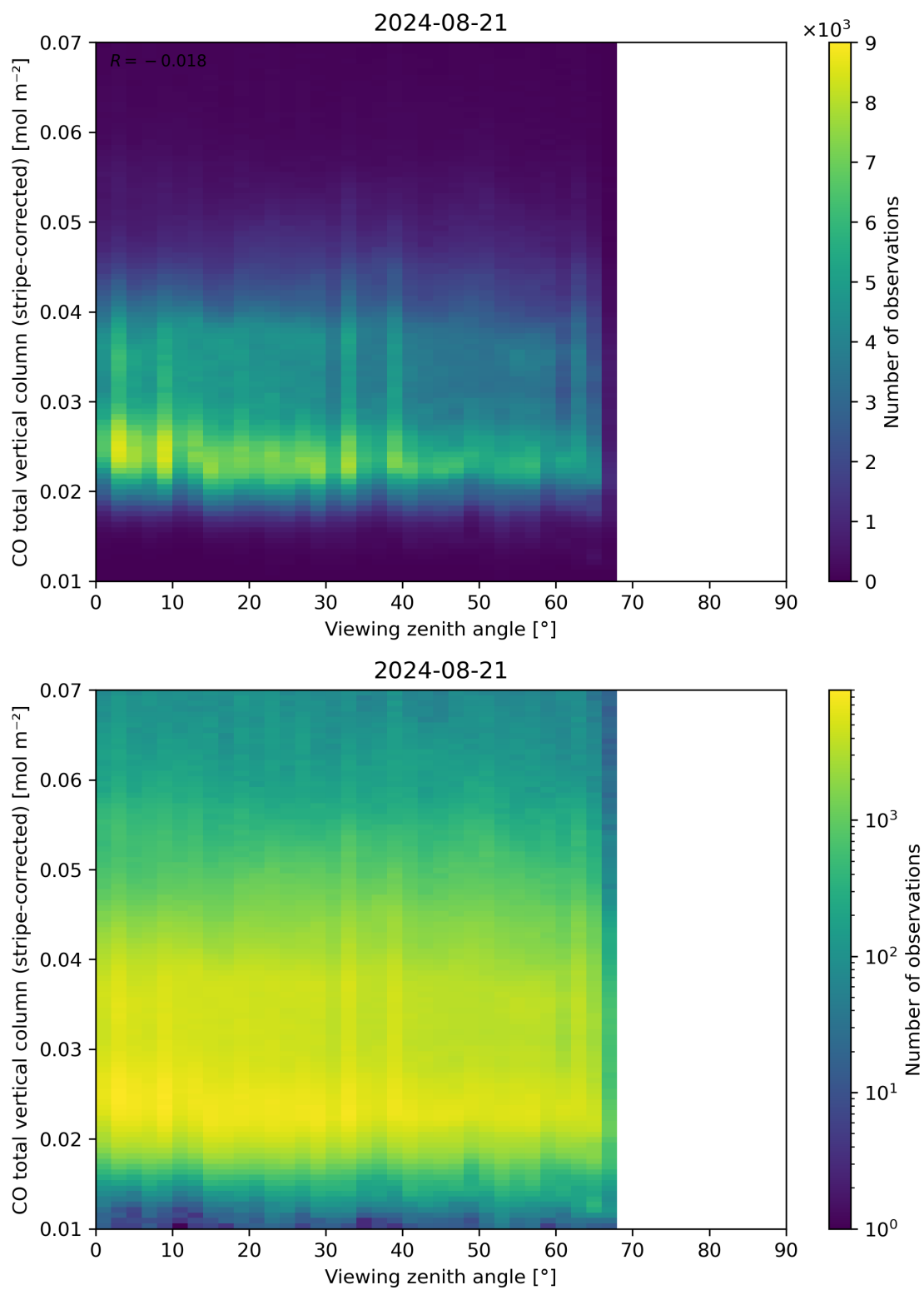
Figure 70: Scatter density plot of “Viewing zenith angle” against “CO total vertical column (stripe-corrected)” for 2024-08-21 to 2024-08-22.
