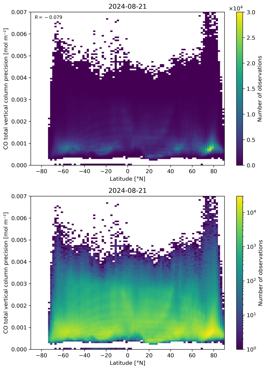
Figure 53: Scatter density plot of “Latitude” against “CO total vertical column precision” for 2024-08-21 to 2024-08-22.
