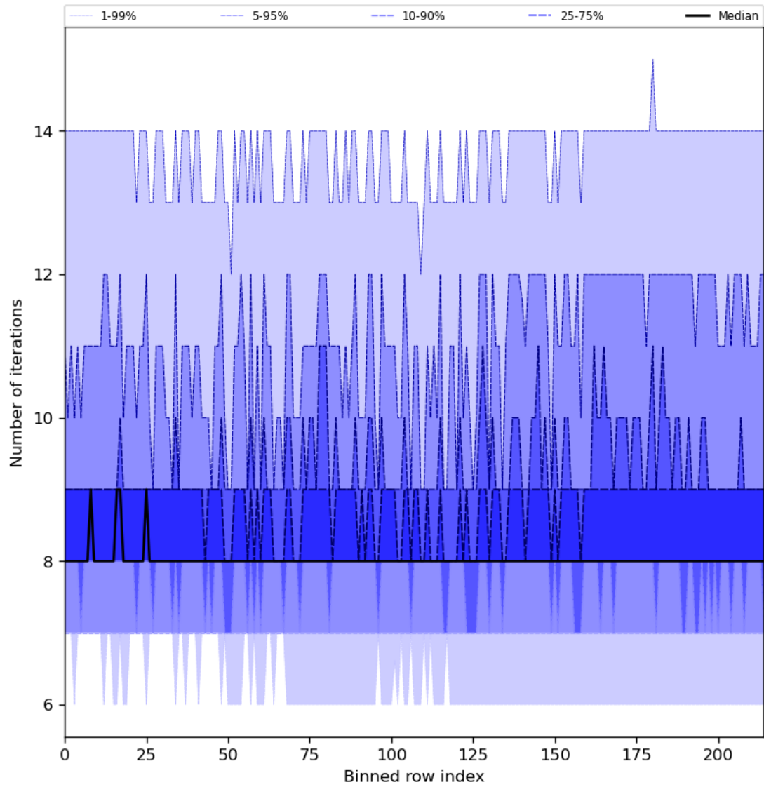
Figure 32: Along track statistics of “Number of iterations” for 2024-08-21 to 2024-08-22
