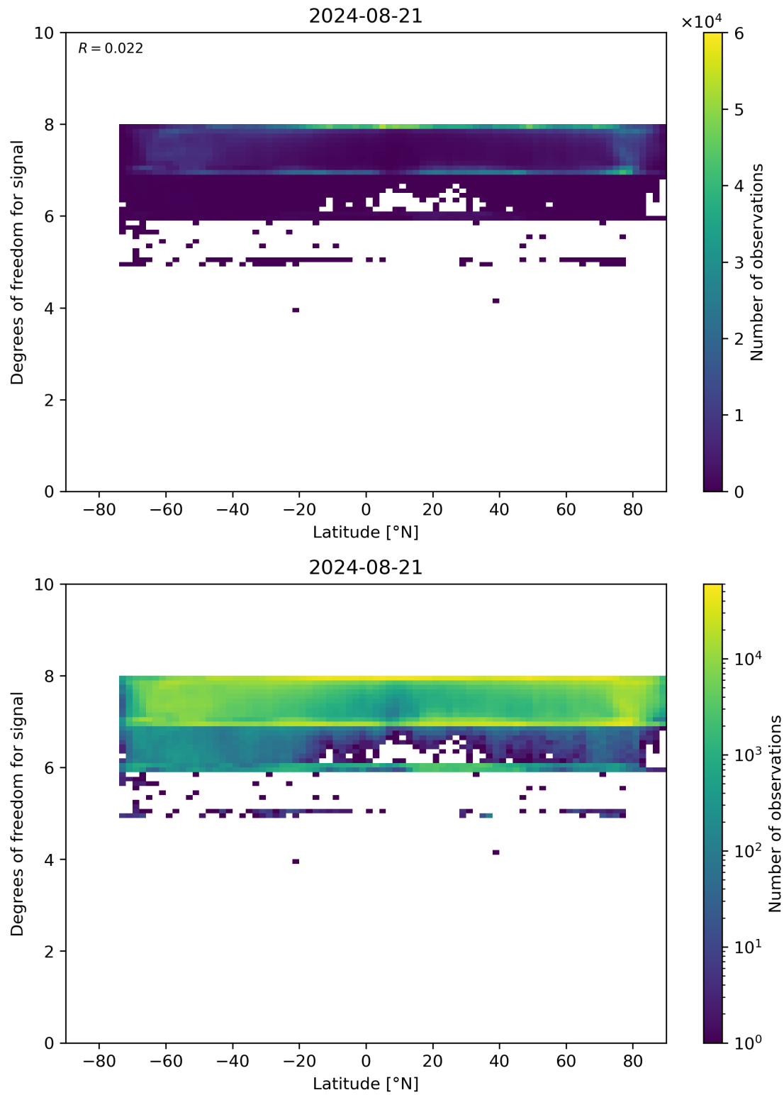
Figure 55: Scatter density plot of “Latitude” against “Degrees of freedom for signal” for 2024-08-21 to 2024-08-22.
