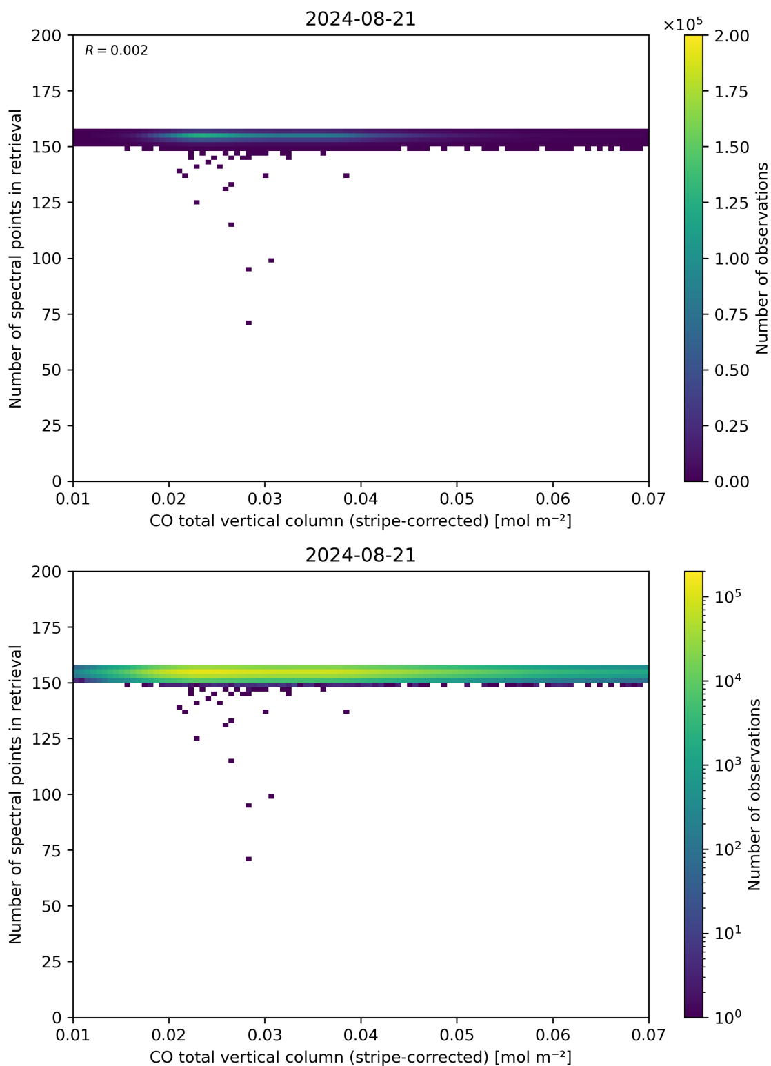
Figure 40: Scatter density plot of “CO total vertical column (stripe-corrected)” against “Number of spectral points in retrieval” for 2024-08-21 to 2024-08-22.
