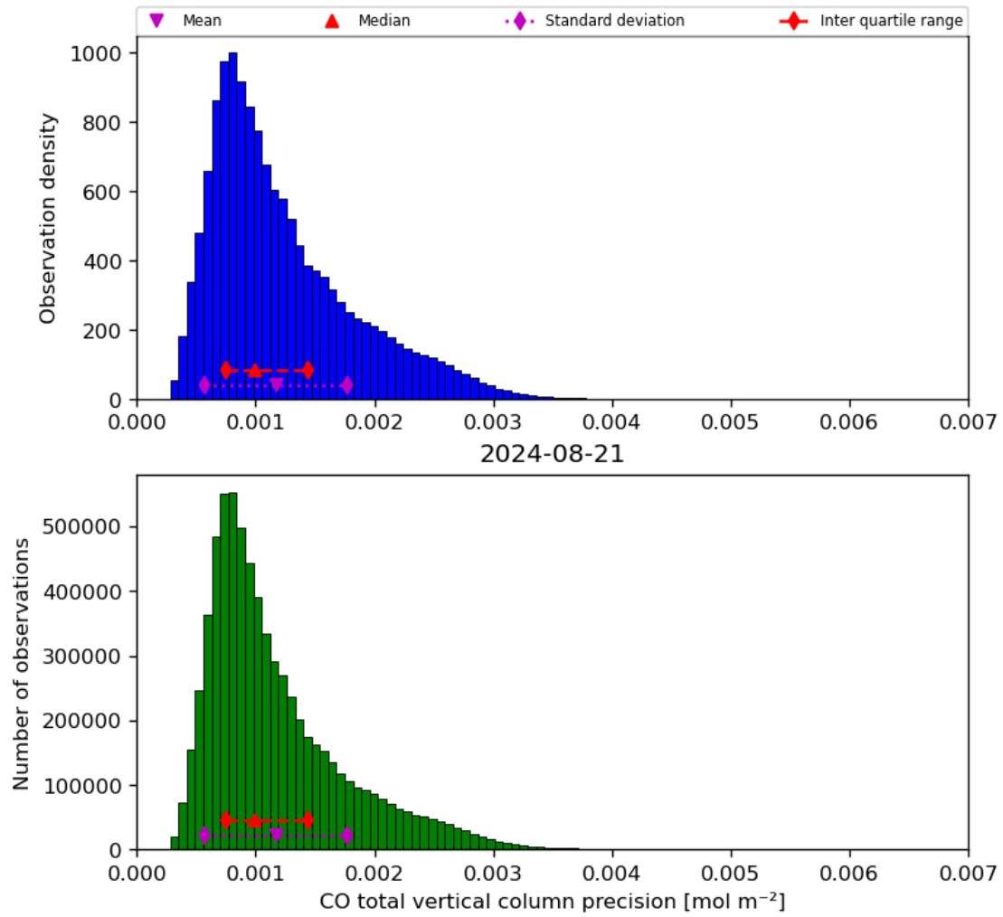
Figure 20: Histogram of “CO total vertical column precision” for 2024-08-21 to 2024-08-22
