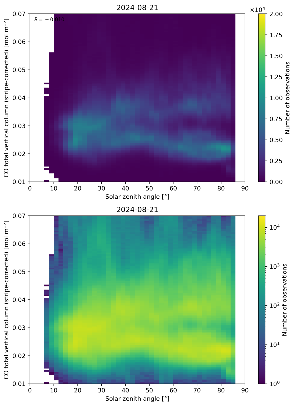
Figure 62: Scatter density plot of “Solar zenith angle” against “CO total vertical column (stripe-corrected)” for 2024-08-21 to 2024-08-22.
