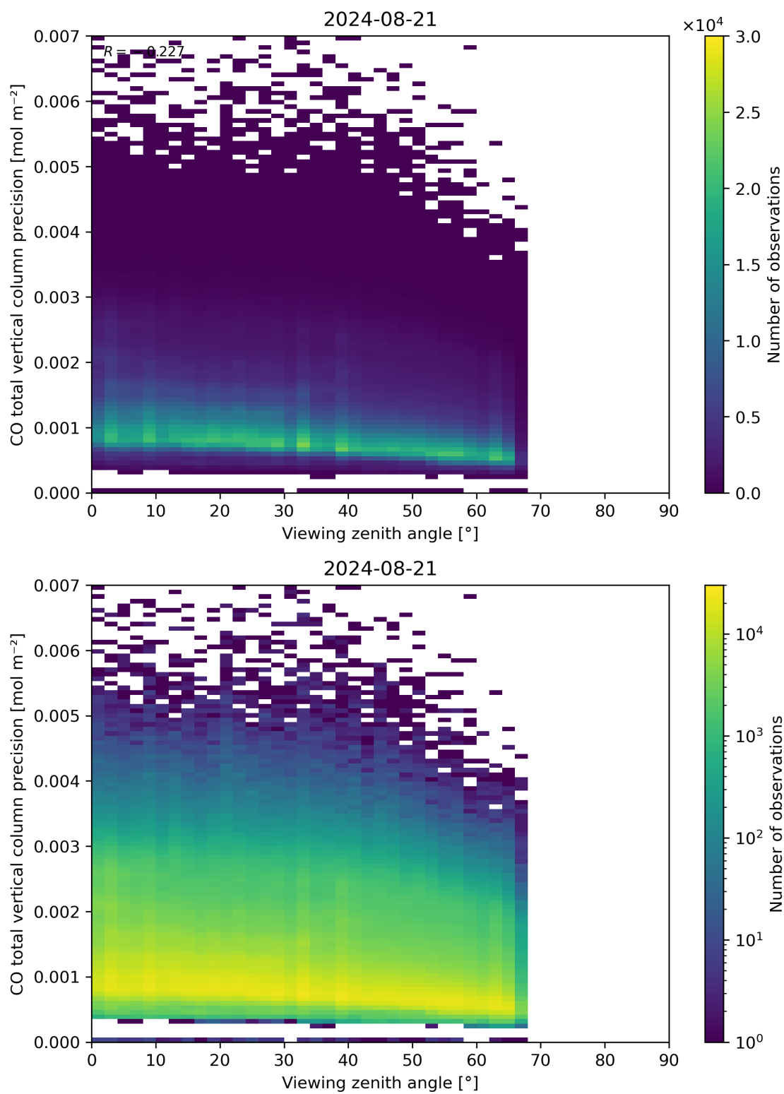
Figure 71: Scatter density plot of “Viewing zenith angle” against “CO total vertical column precision” for 2024-08-21 to 2024-08-22.
