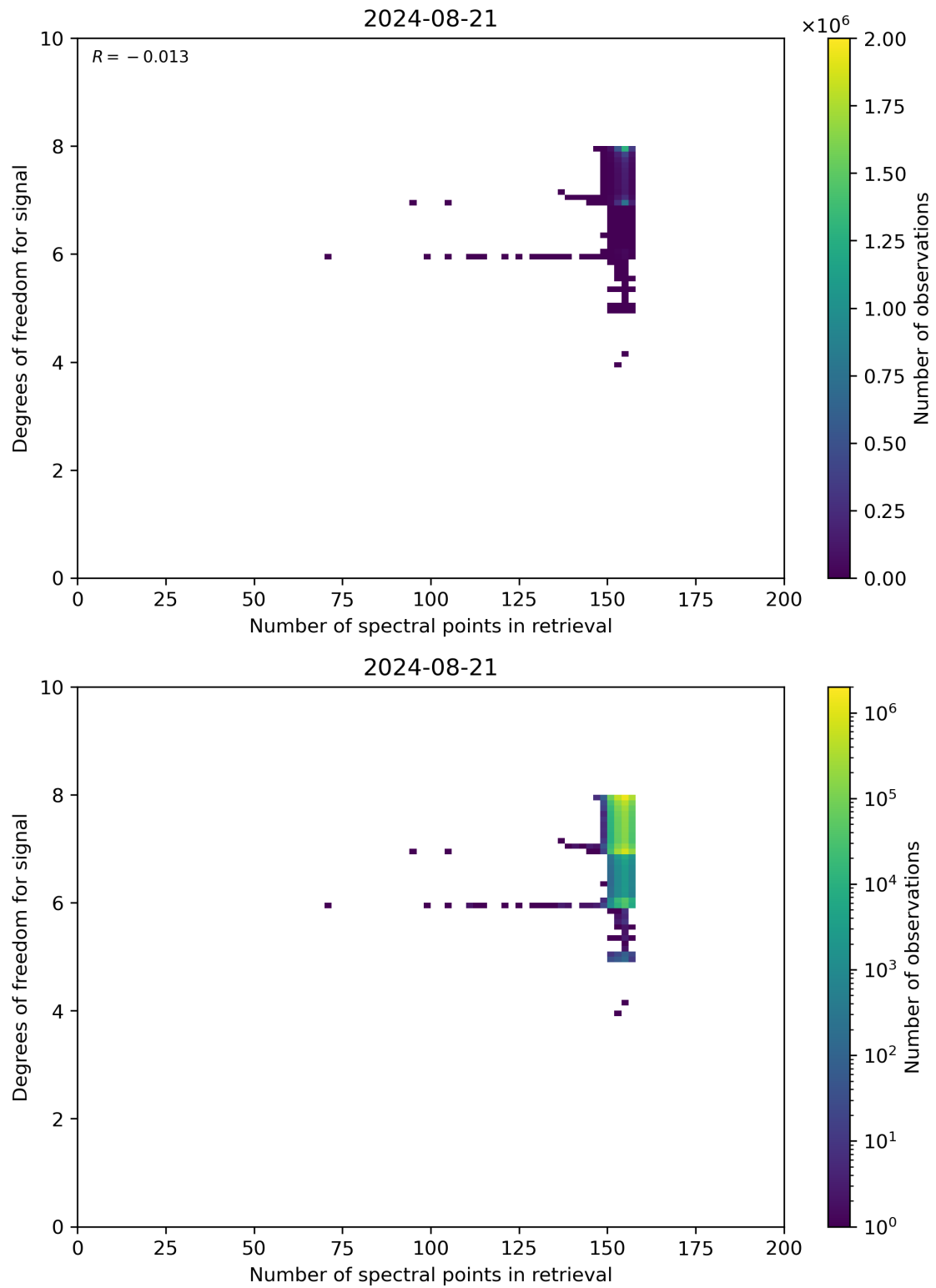
Figure 59: Scatter density plot of “Number of spectral points in retrieval” against “Degrees of freedom for signal” for 2024-08-21 to 2024-08-22.
