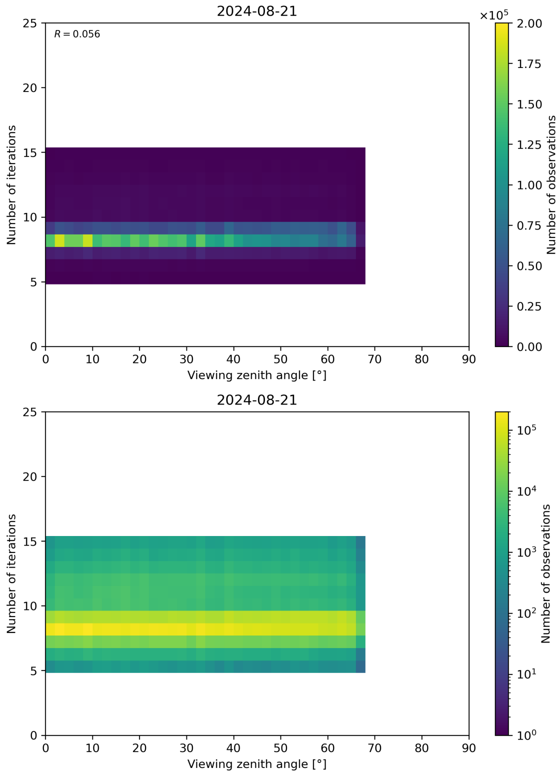
Figure 75: Scatter density plot of “Viewing zenith angle” against “Number of iterations” for 2024-08-21 to 2024-08-22.
