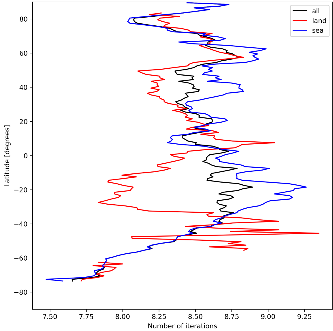
Figure 16: Zonal average of “Number of iterations” for 2024-08-21 to 2024-08-22.
