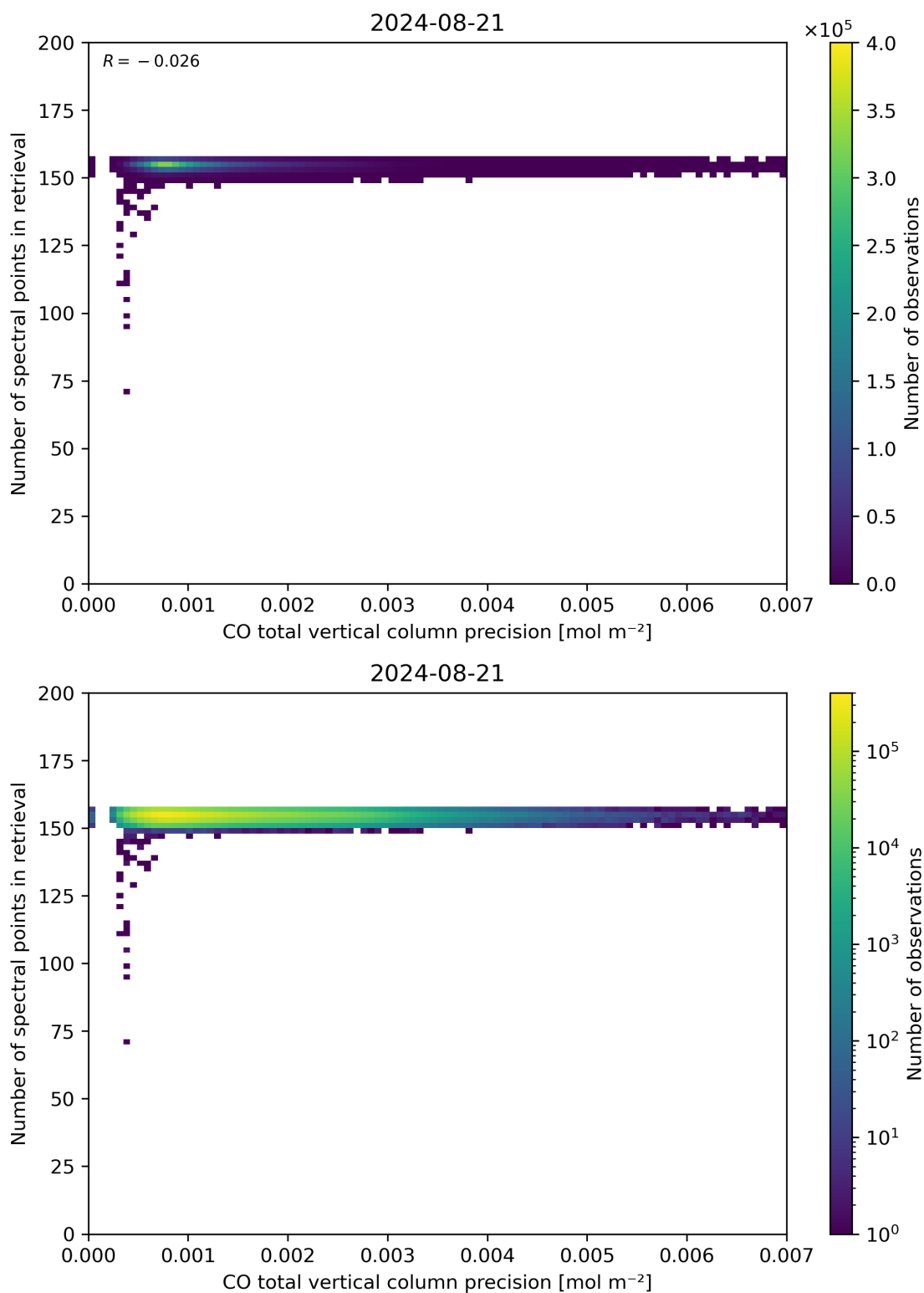
Figure 47: Scatter density plot of “CO total vertical column precision” against “Number of spectral points in retrieval” for 2024-08-21 to 2024-08-22.
