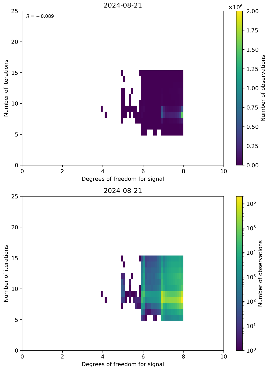
Figure 50: Scatter density plot of “Degrees of freedom for signal” against “Number of iterations” for 2024-08-21 to 2024-08-22.
