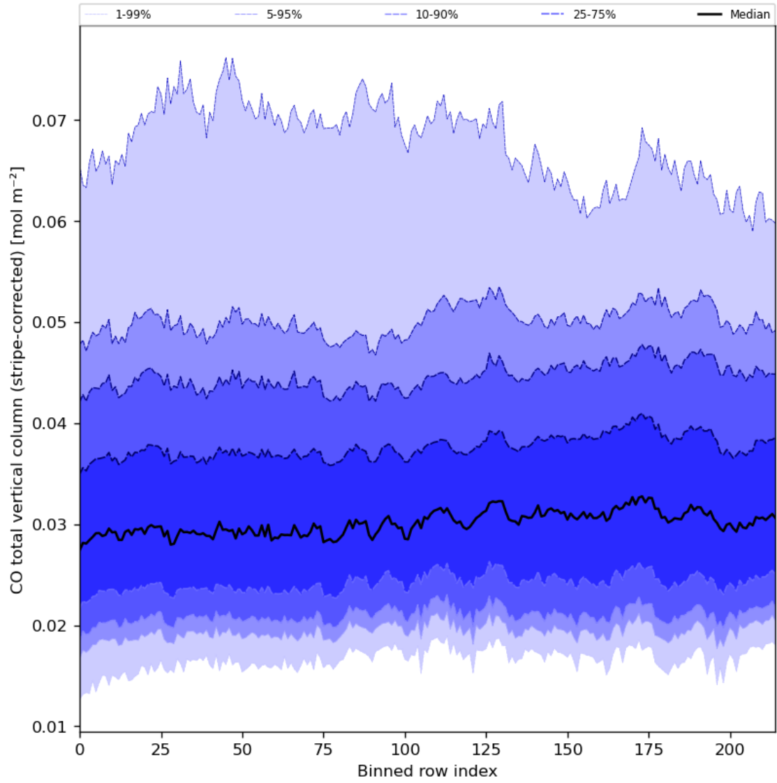
Figure 27: Along track statistics of “CO total vertical column (stripe-corrected)” for 2024-08-21 to 2024-08-22
