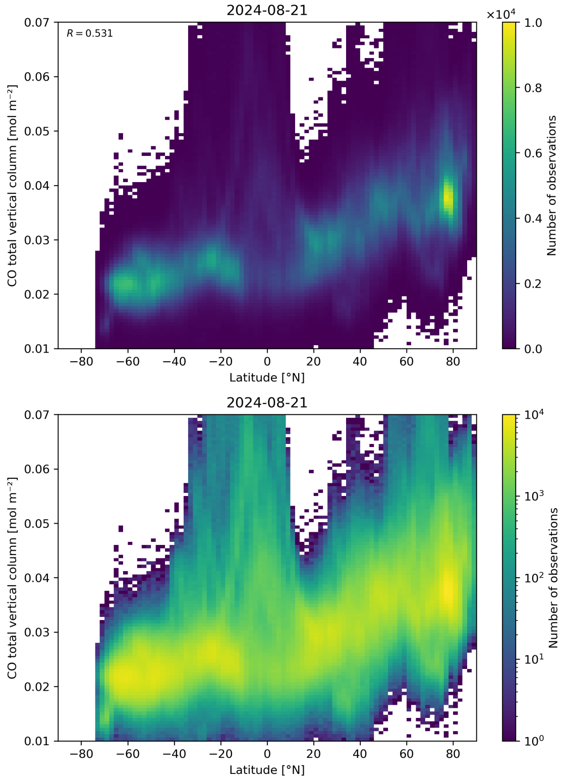
Figure 51: Scatter density plot of “Latitude” against “CO total vertical column” for 2024-08-21 to 2024-08-22.
