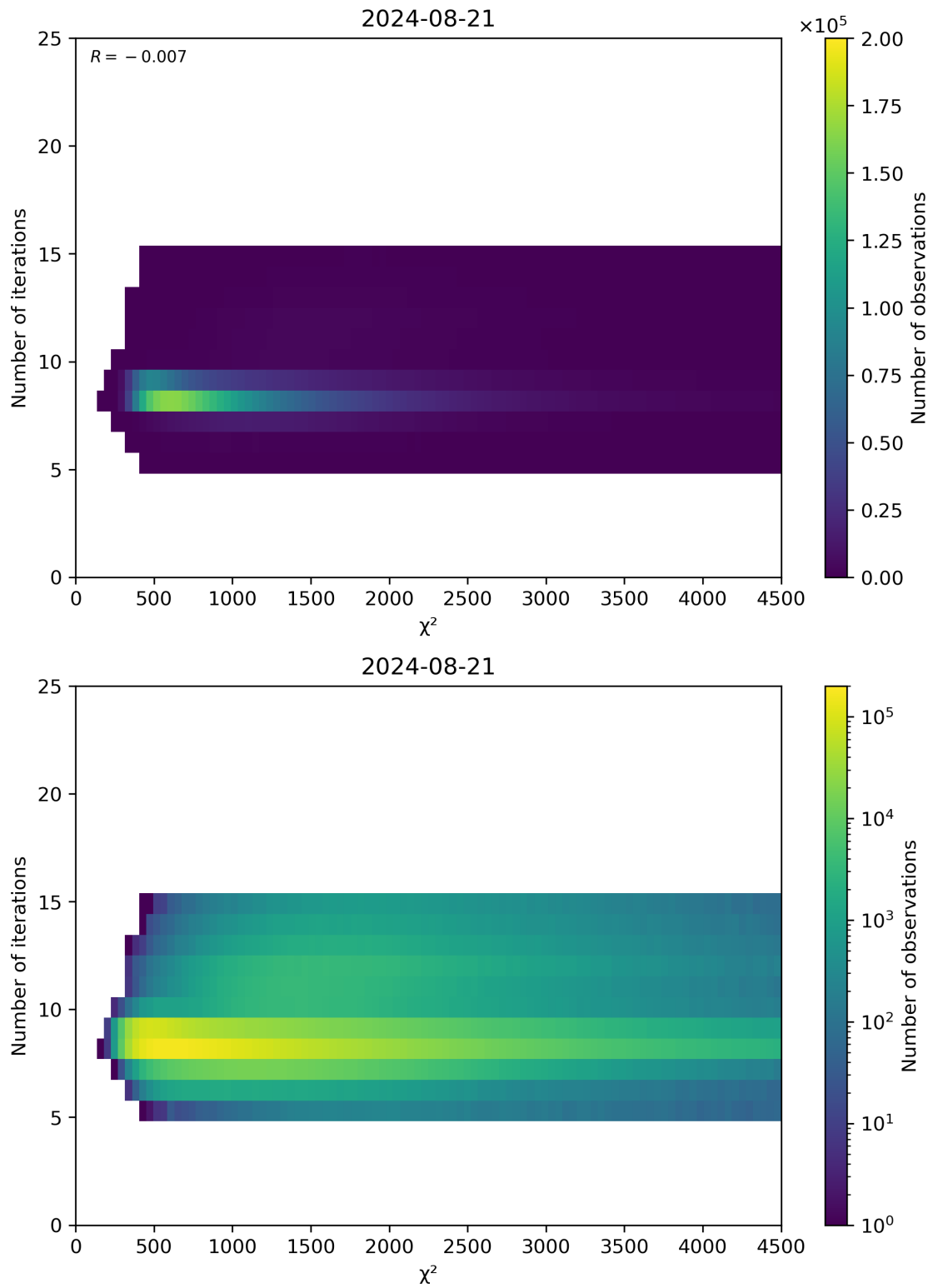
Figure 49: Scatter density plot of “ \chi^2 ” against “Number of iterations” for 2024-08-21 to 2024-08-22.
