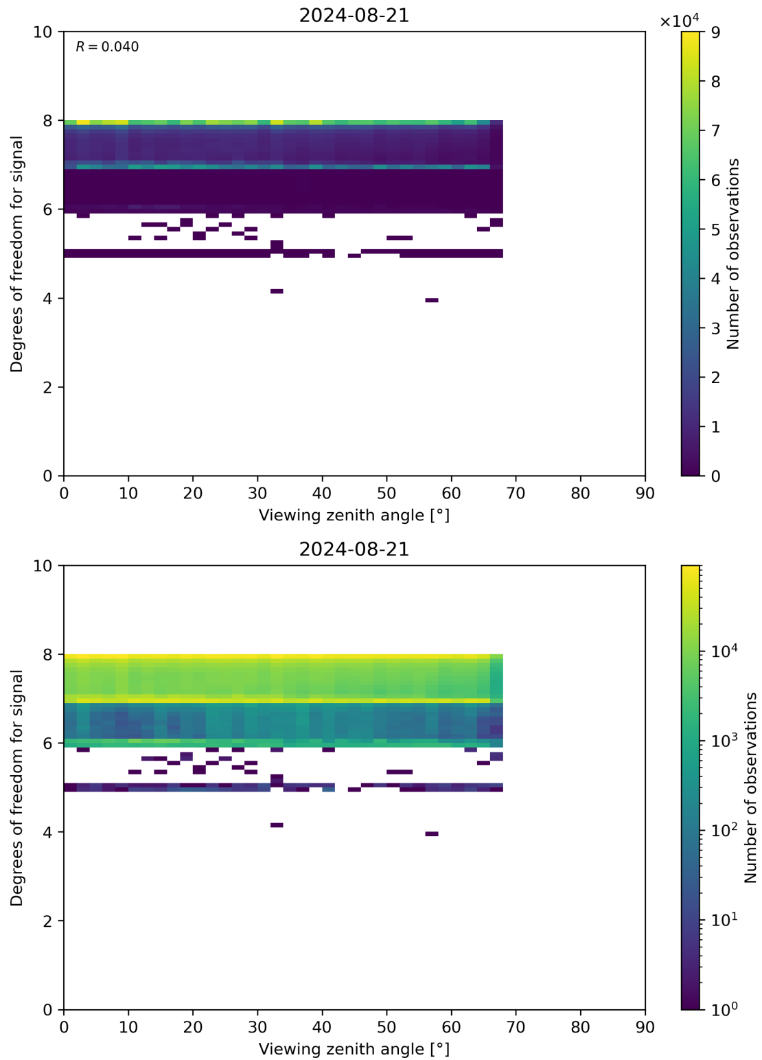
Figure 73: Scatter density plot of “Viewing zenith angle” against “Degrees of freedom for signal” for 2024-08-21 to 2024-08-22.
