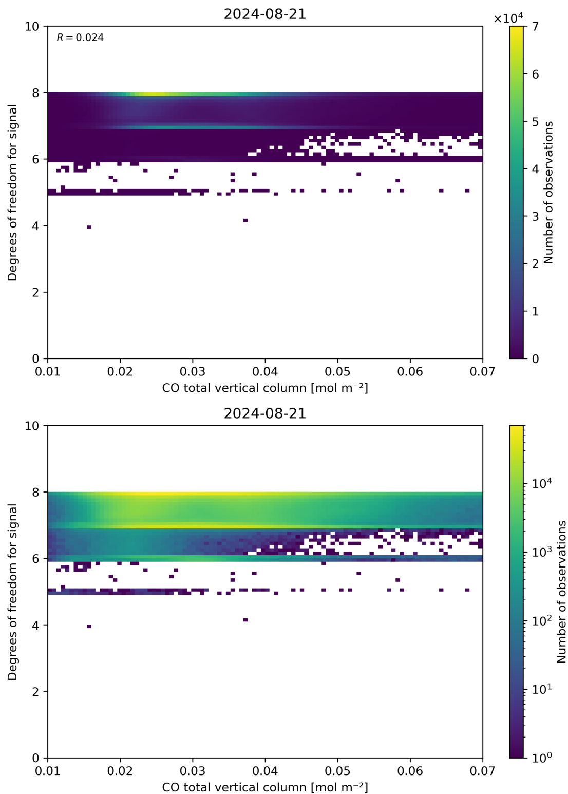
Figure 41: Scatter density plot of “CO total vertical column” against “Degrees of freedom for signal” for 2024-08-21 to 2024-08-22.
