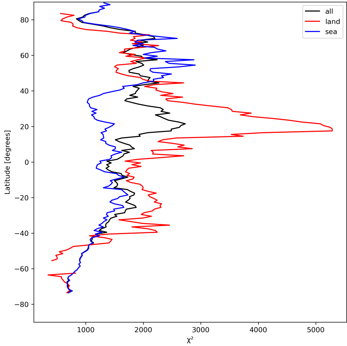
Figure 14: Zonal average of “ \chi^2 ” for 2024-08-21 to 2024-08-22.
