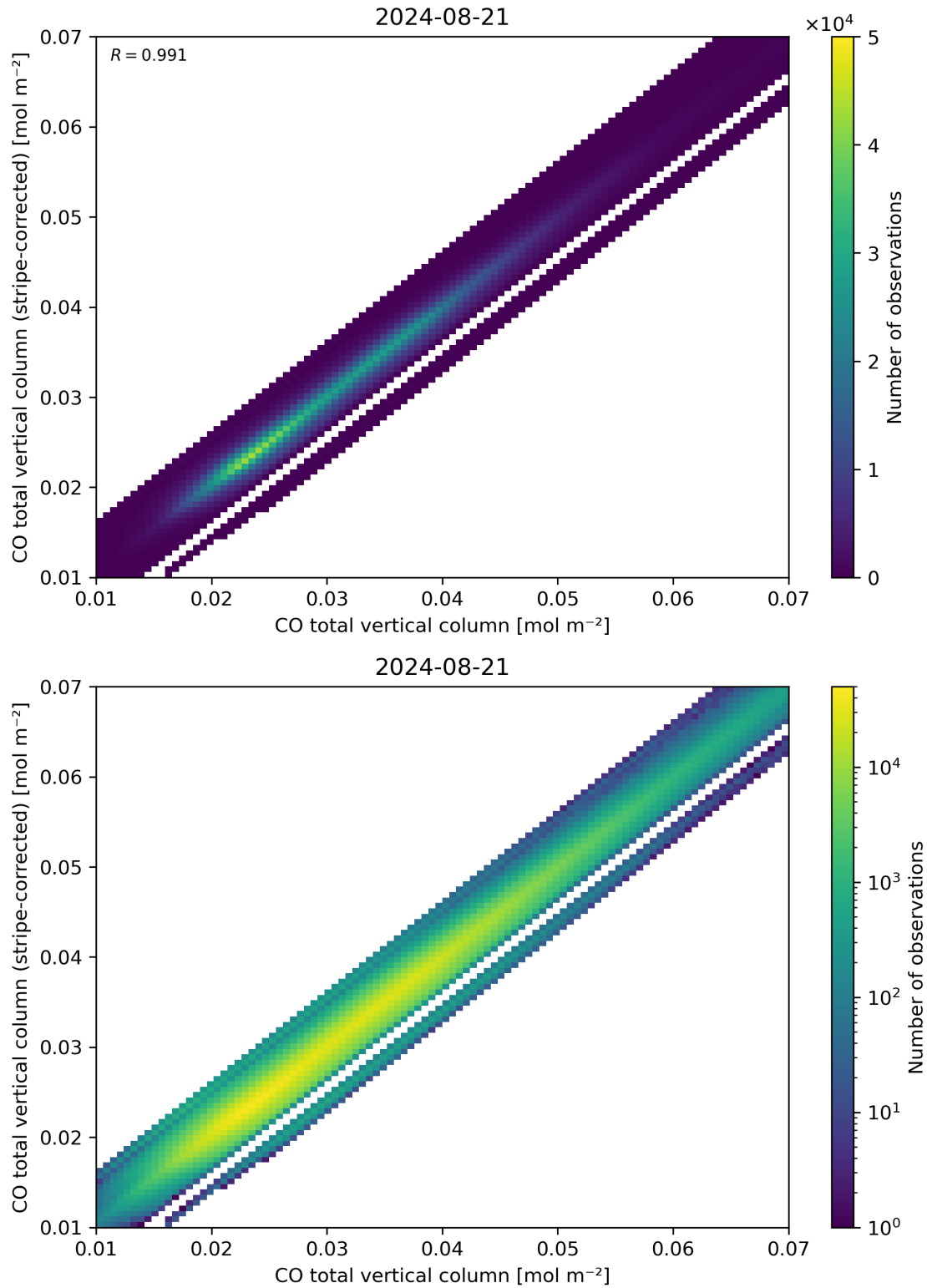
Figure 33: Scatter density plot of “CO total vertical column” against “CO total vertical column (stripe-corrected)” for 2024-08-21 to 2024-08-22.
