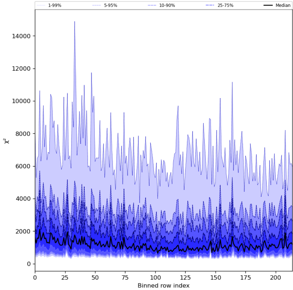
Figure 30: Along track statistics of “ \chi^2 ” for 2024-08-21 to 2024-08-22
