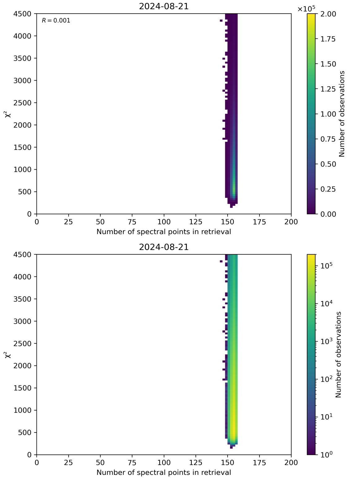
Figure 58: Scatter density plot of “Number of spectral points in retrieval” against “ \chi^2 ” for 2024-08-21 to 2024-08-22.
