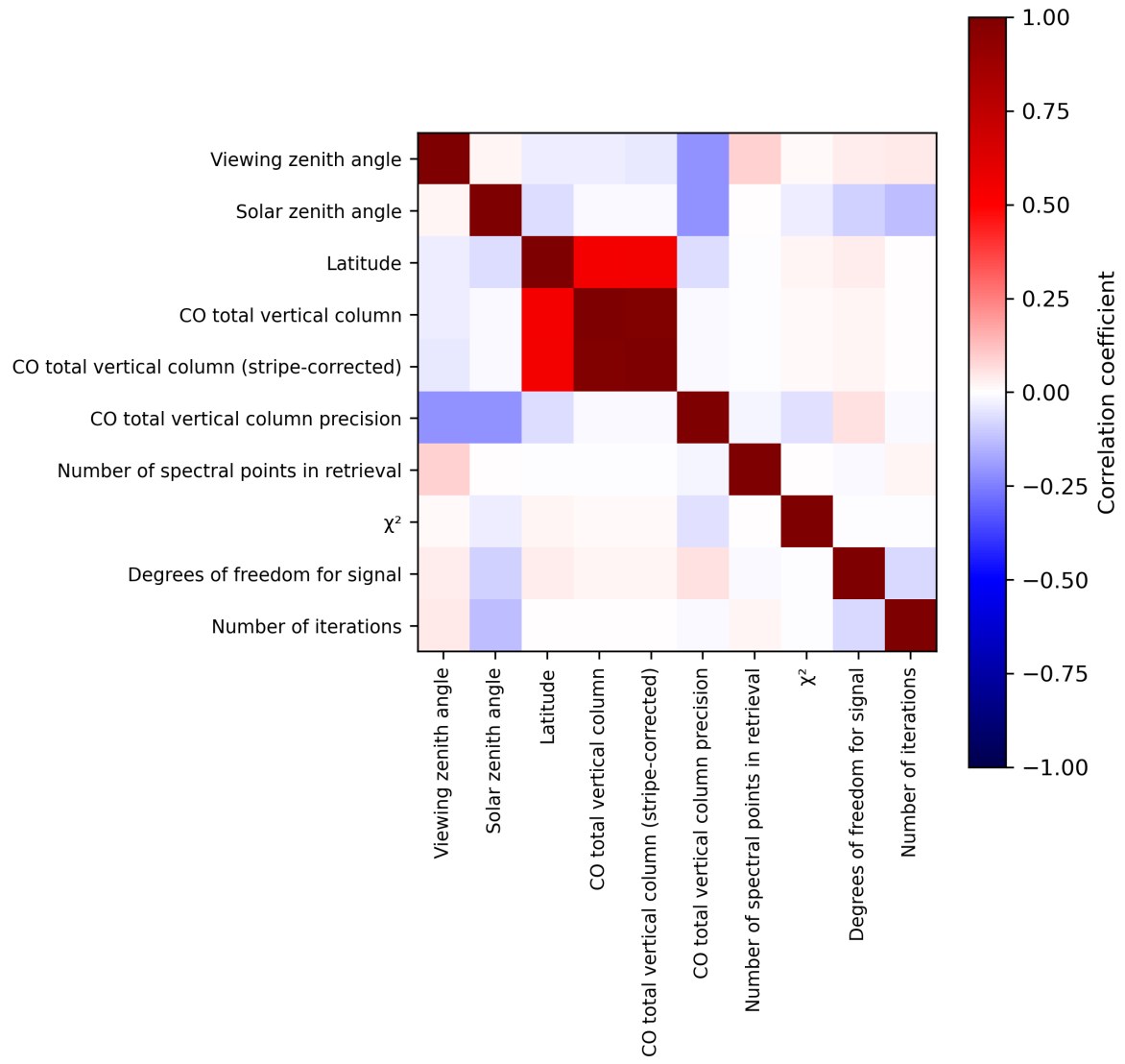
Figure 2: Map of correlation matrix for 2024-08-22 to 2024-08-23.
