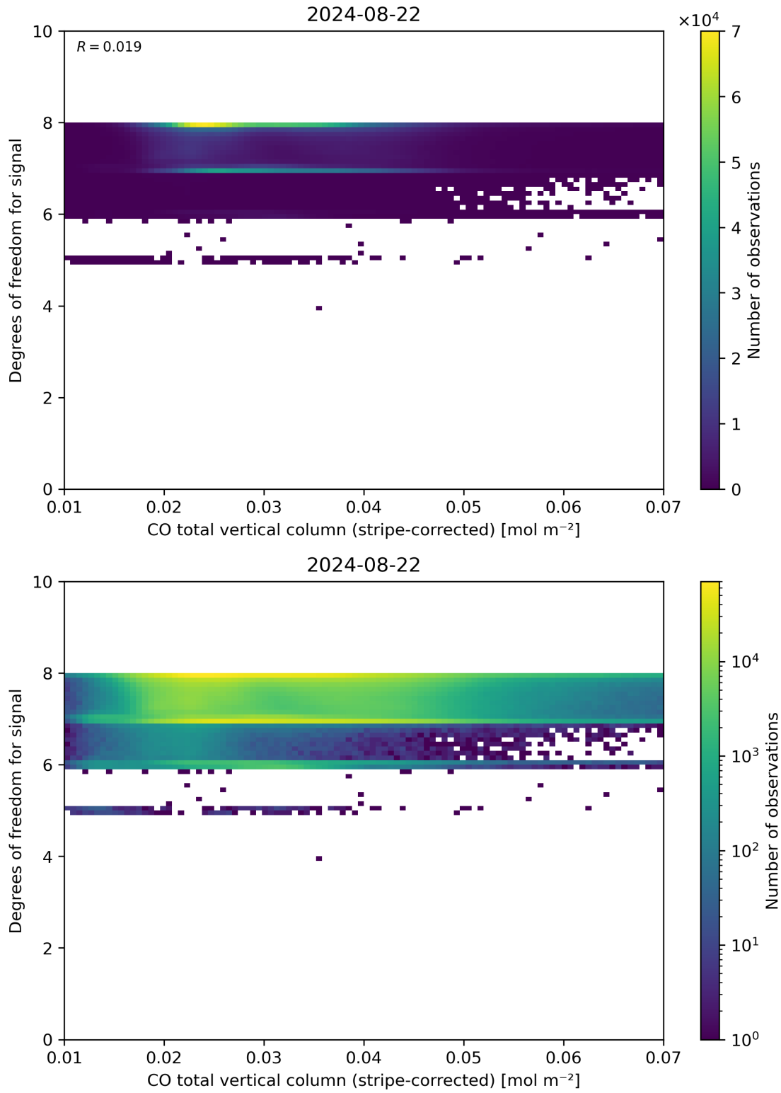
Figure 38: Scatter density plot of “CO total vertical column (stripe-corrected)” against “Degrees of freedom for signal” for 2024-08-22 to 2024-08-23.
