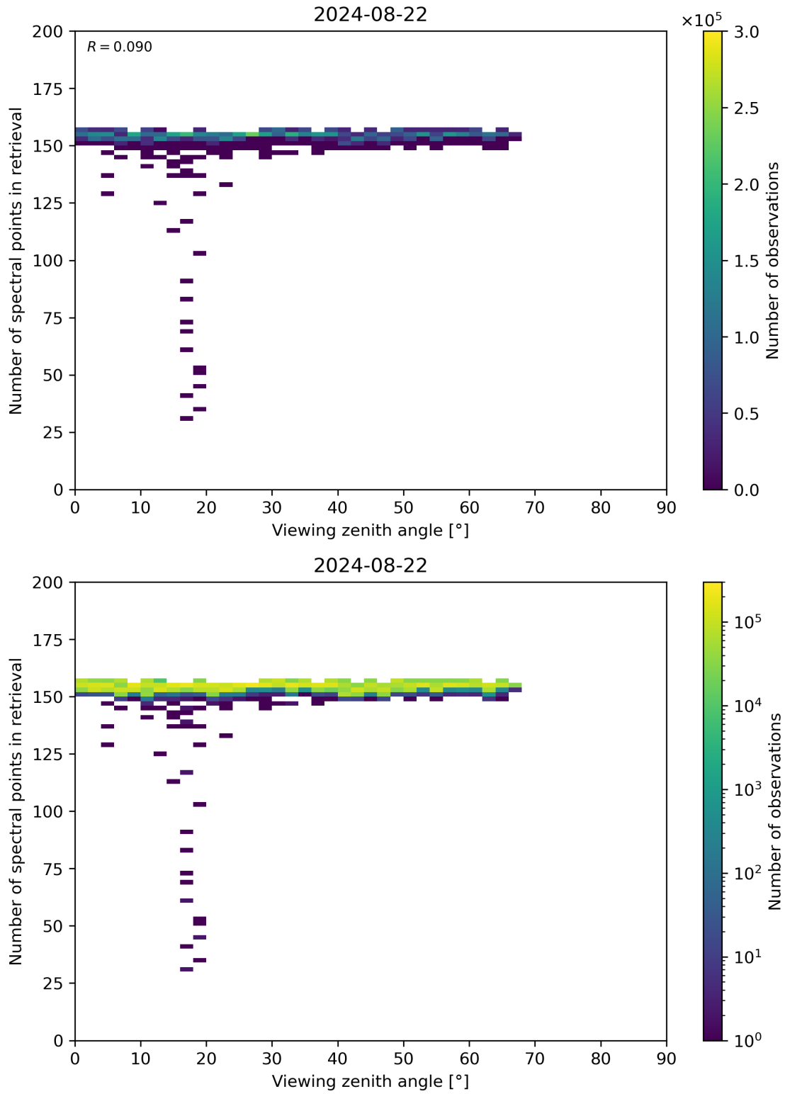
Figure 76: Scatter density plot of “Viewing zenith angle” against “Number of spectral points in retrieval” for 2024-08-22 to 2024-08-23.
