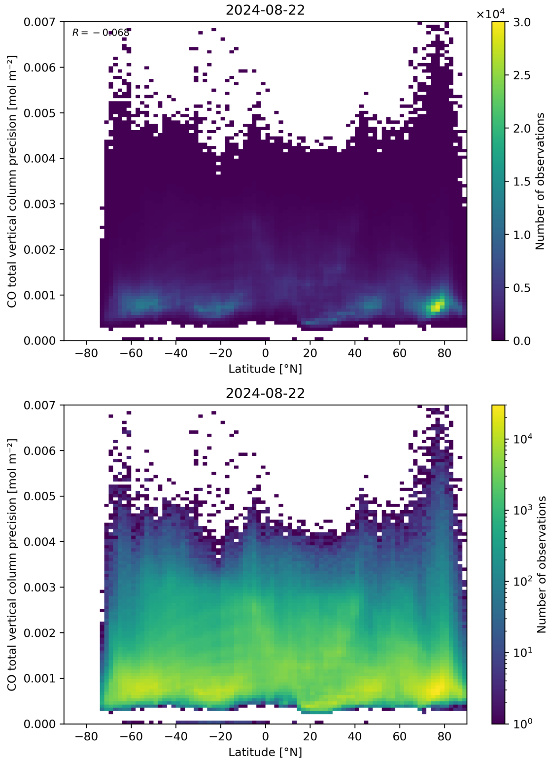
Figure 53: Scatter density plot of “Latitude” against “CO total vertical column precision” for 2024-08-22 to 2024-08-23.
