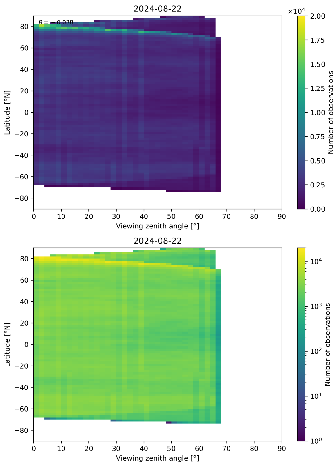
Figure 74: Scatter density plot of “Viewing zenith angle” against “Latitude” for 2024-08-22 to 2024-08-23.
