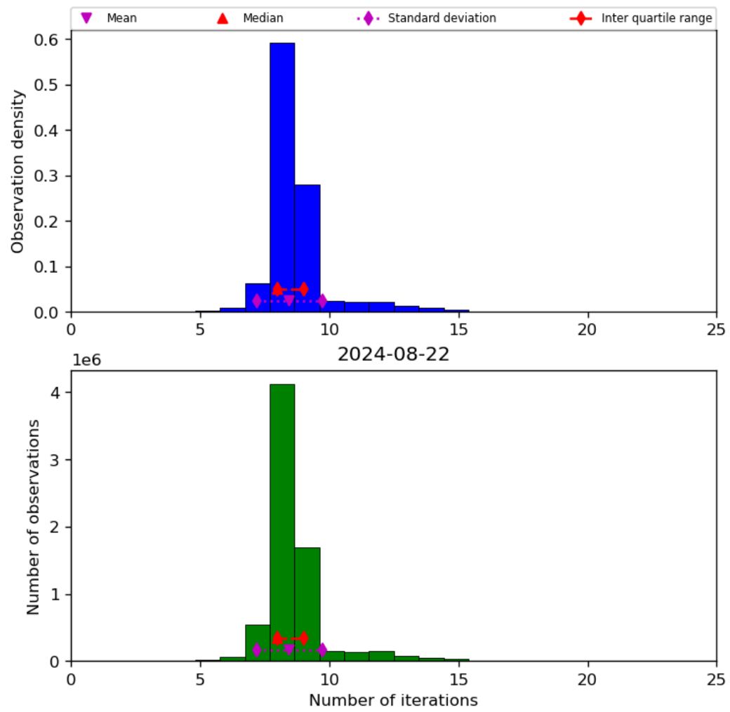
Figure 24: Histogram of “Number of iterations” for 2024-08-22 to 2024-08-23
