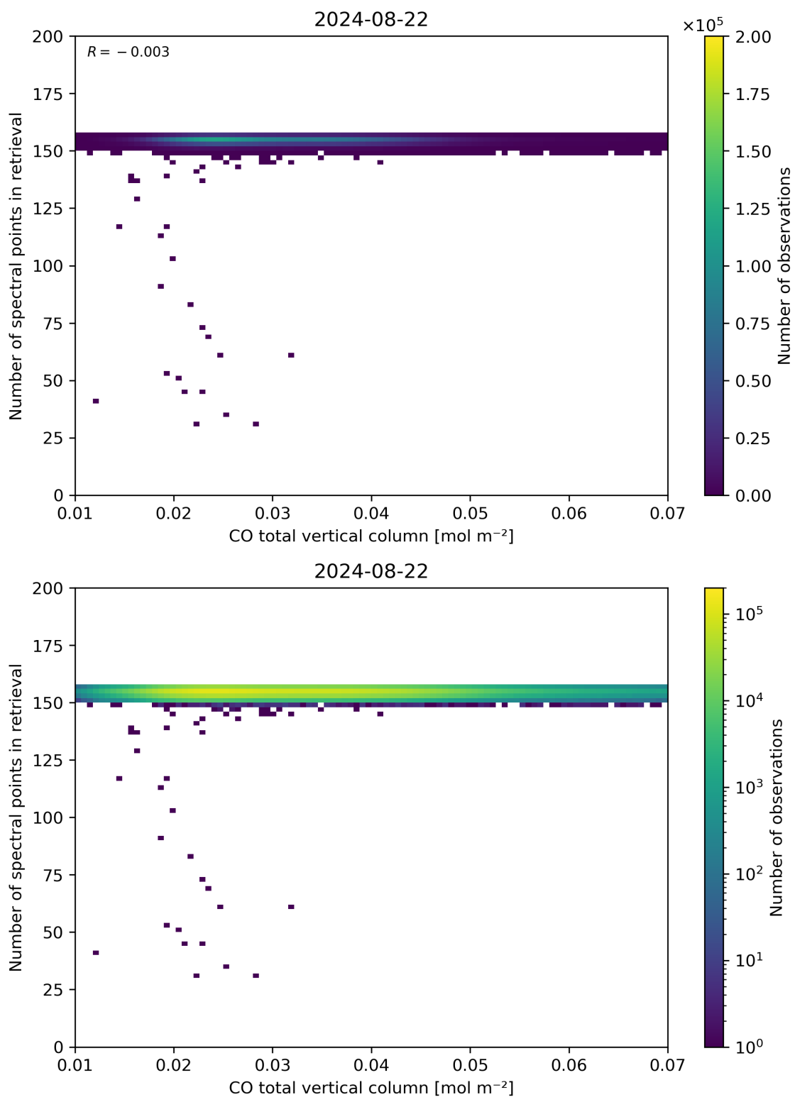
Figure 43: Scatter density plot of “CO total vertical column” against “Number of spectral points in retrieval” for 2024-08-22 to 2024-08-23.
