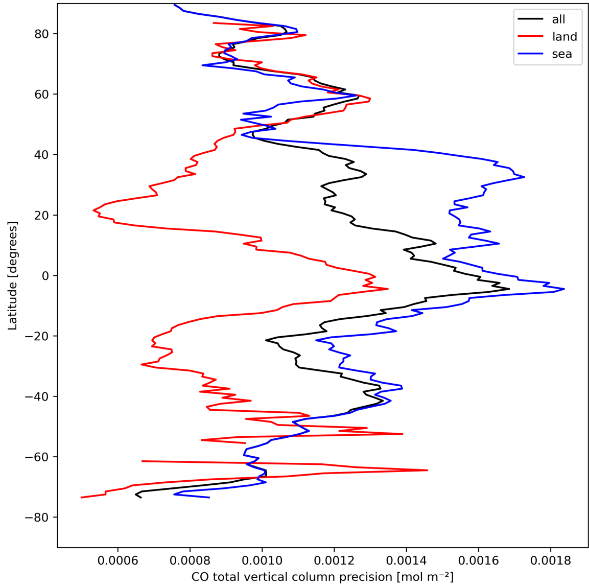
Figure 12: Zonal average of “CO total vertical column precision” for 2024-08-22 to 2024-08-23.
