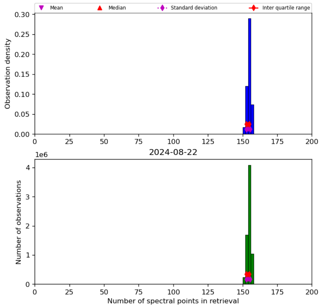
Figure 21: Histogram of “Number of spectral points in retrieval” for 2024-08-22 to 2024-08-23
