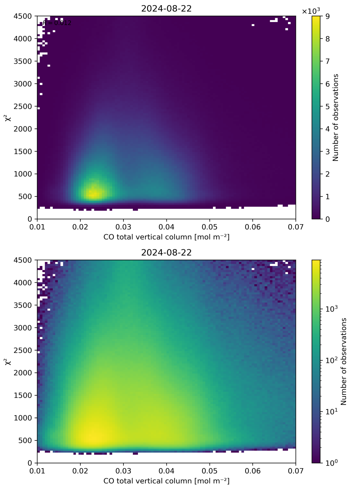
Figure 35: Scatter density plot of “CO total vertical column” against “ \chi^2 ” for 2024-08-22 to 2024-08-23.
