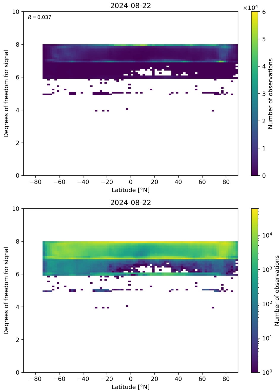
Figure 55: Scatter density plot of “Latitude” against “Degrees of freedom for signal” for 2024-08-22 to 2024-08-23.
