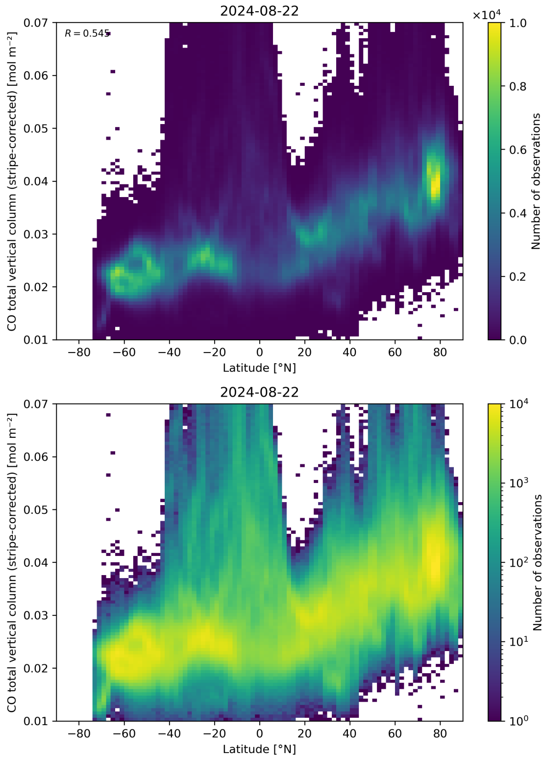
Figure 52: Scatter density plot of “Latitude” against “CO total vertical column (stripe-corrected)” for 2024-08-22 to 2024-08-23.
