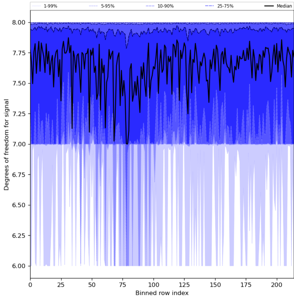
Figure 31: Along track statistics of “Degrees of freedom for signal” for 2024-08-22 to 2024-08-23
