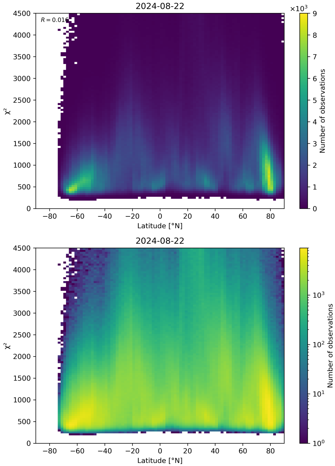
Figure 54: Scatter density plot of “Latitude” against “ \chi^2 ” for 2024-08-22 to 2024-08-23.
