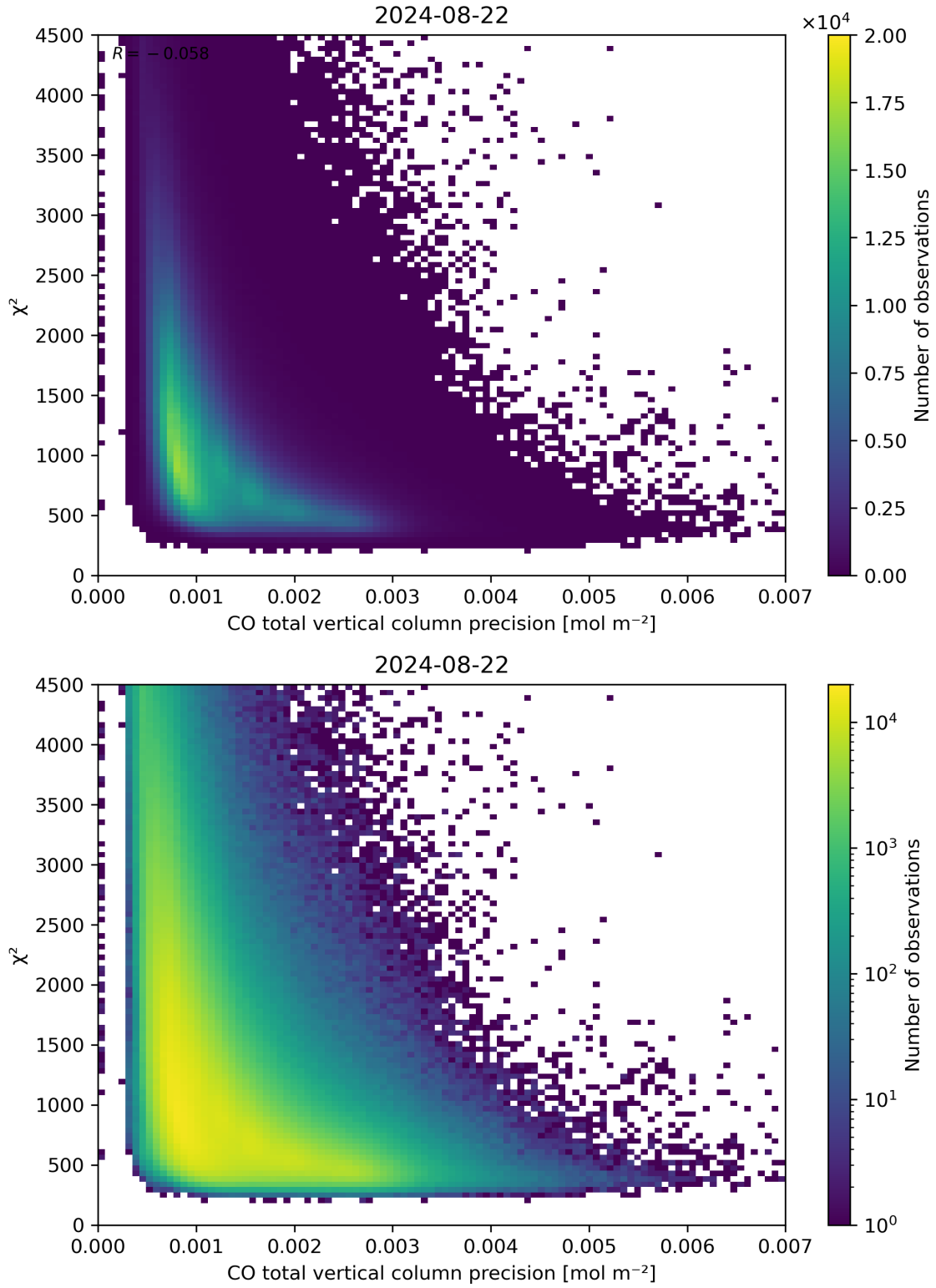
Figure 44: Scatter density plot of “CO total vertical column precision” against “ \chi^2 ” for 2024-08-22 to 2024-08-23.
