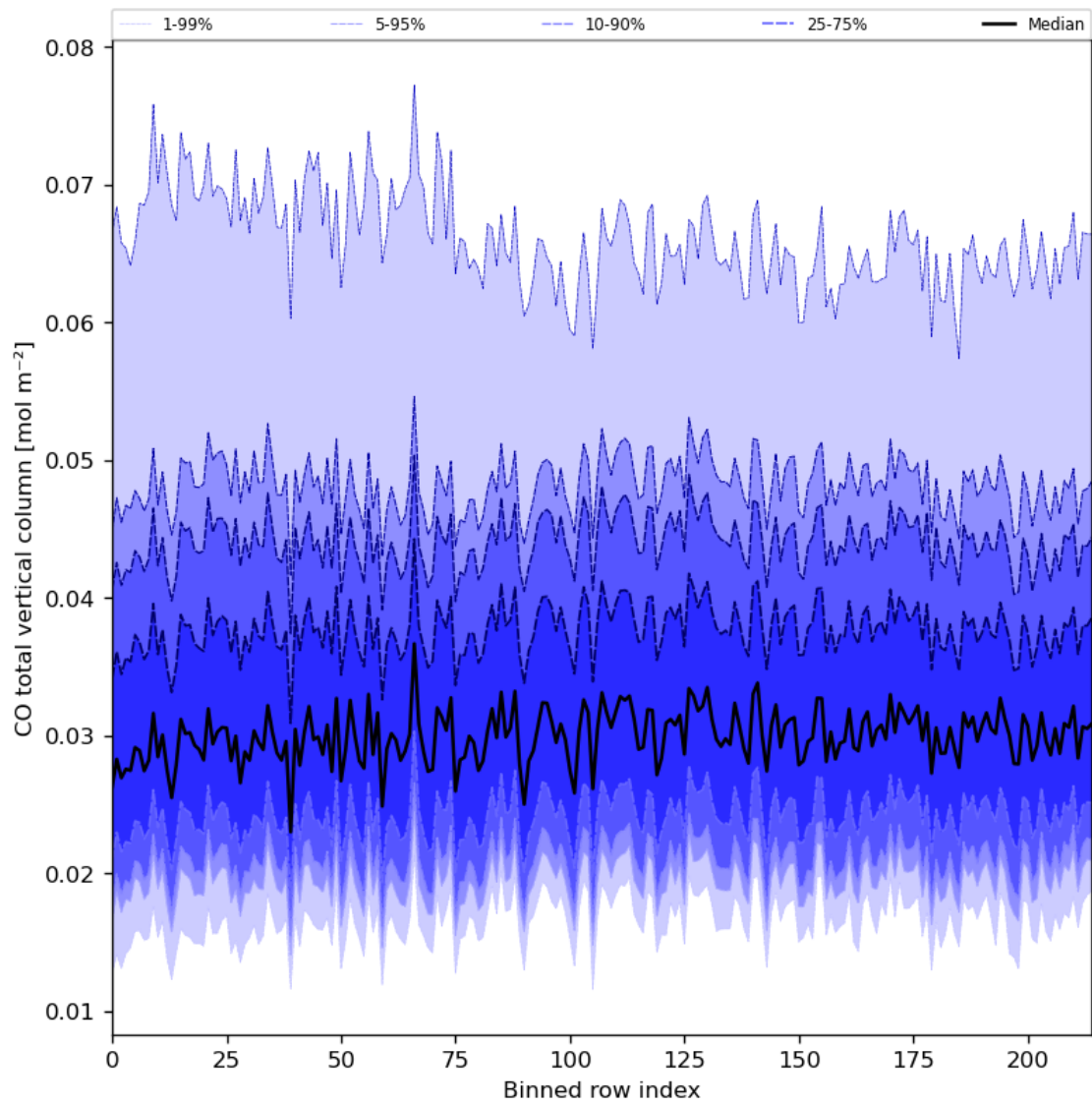
Figure 26: Along track statistics of “CO total vertical column” for 2024-08-22 to 2024-08-23
