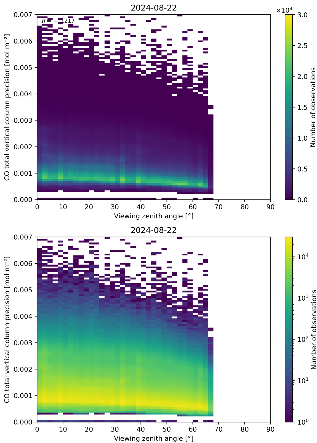
Figure 71: Scatter density plot of “Viewing zenith angle” against “CO total vertical column precision” for 2024-08-22 to 2024-08-23.
