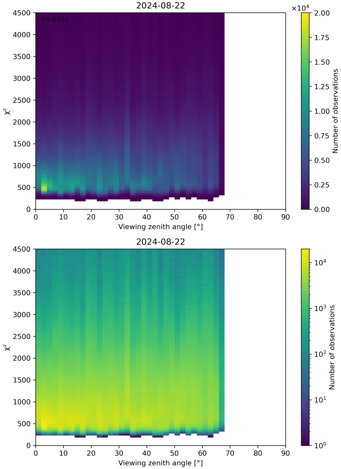
Figure 72: Scatter density plot of “Viewing zenith angle” against “ \chi^2 ” for 2024-08-22 to 2024-08-23.
