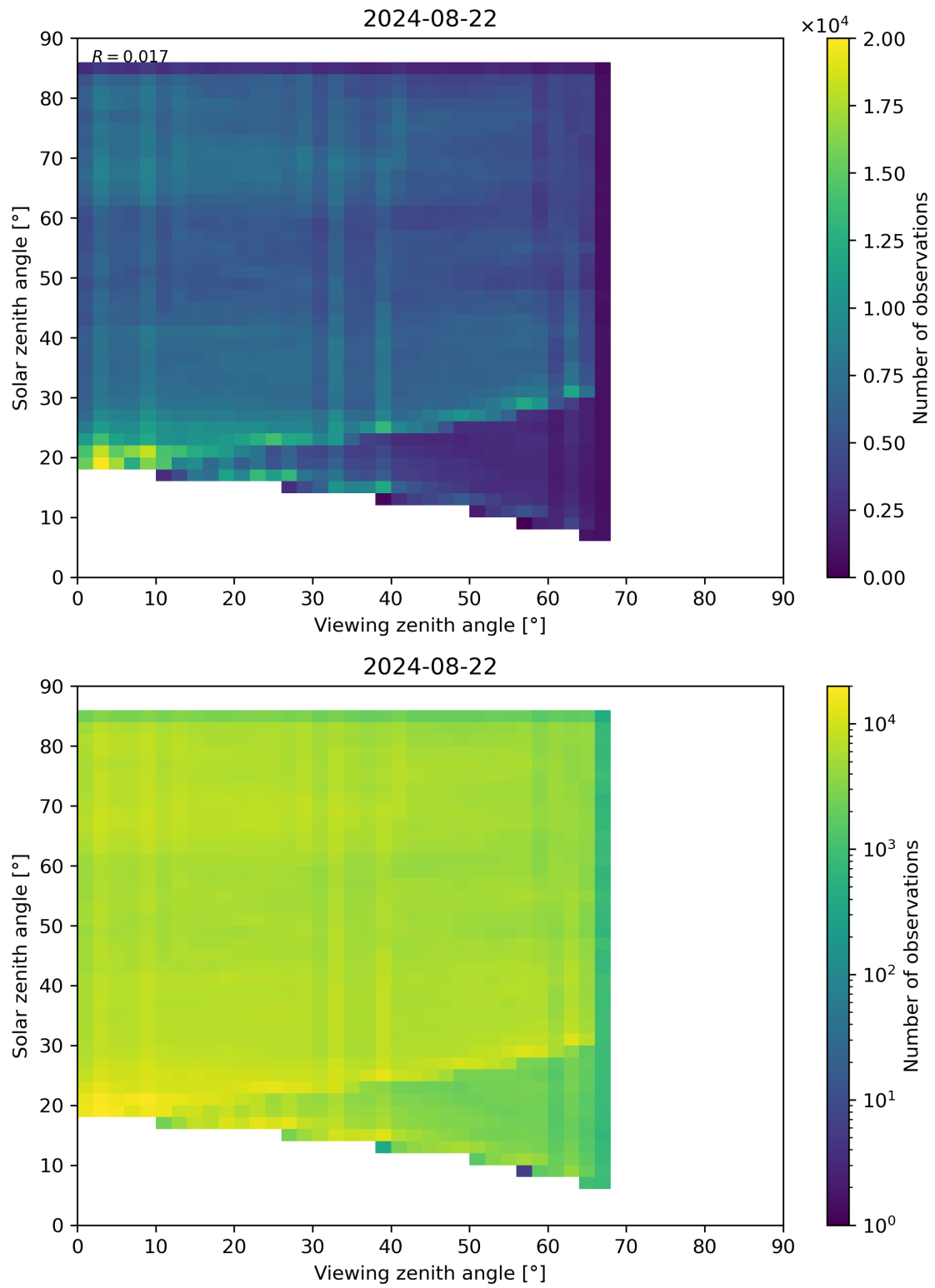
Figure 77: Scatter density plot of “Viewing zenith angle” against “Solar zenith angle” for 2024-08-22 to 2024-08-23.
