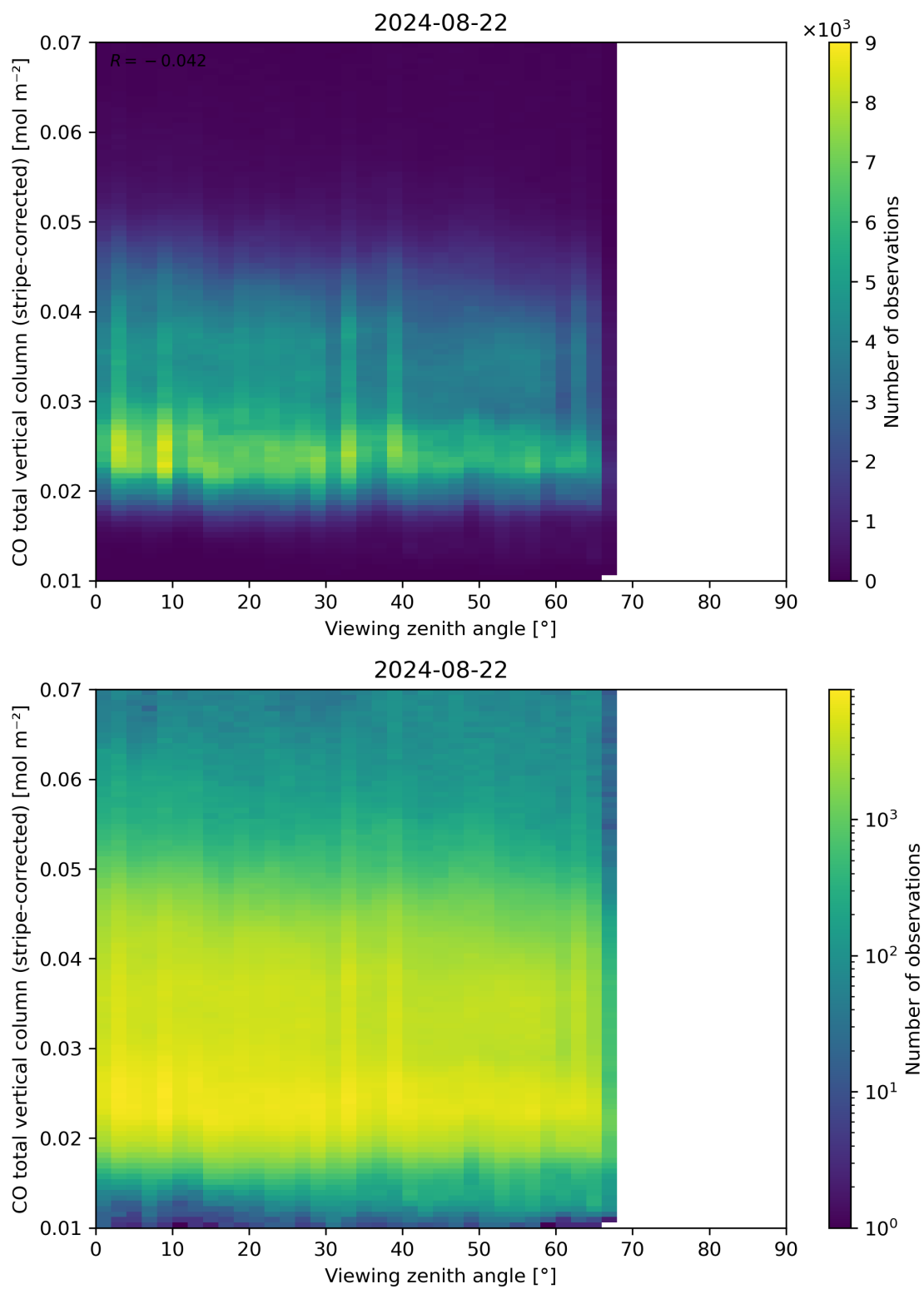
Figure 70: Scatter density plot of “Viewing zenith angle” against “CO total vertical column (stripe-corrected)” for 2024-08-22 to 2024-08-23.
