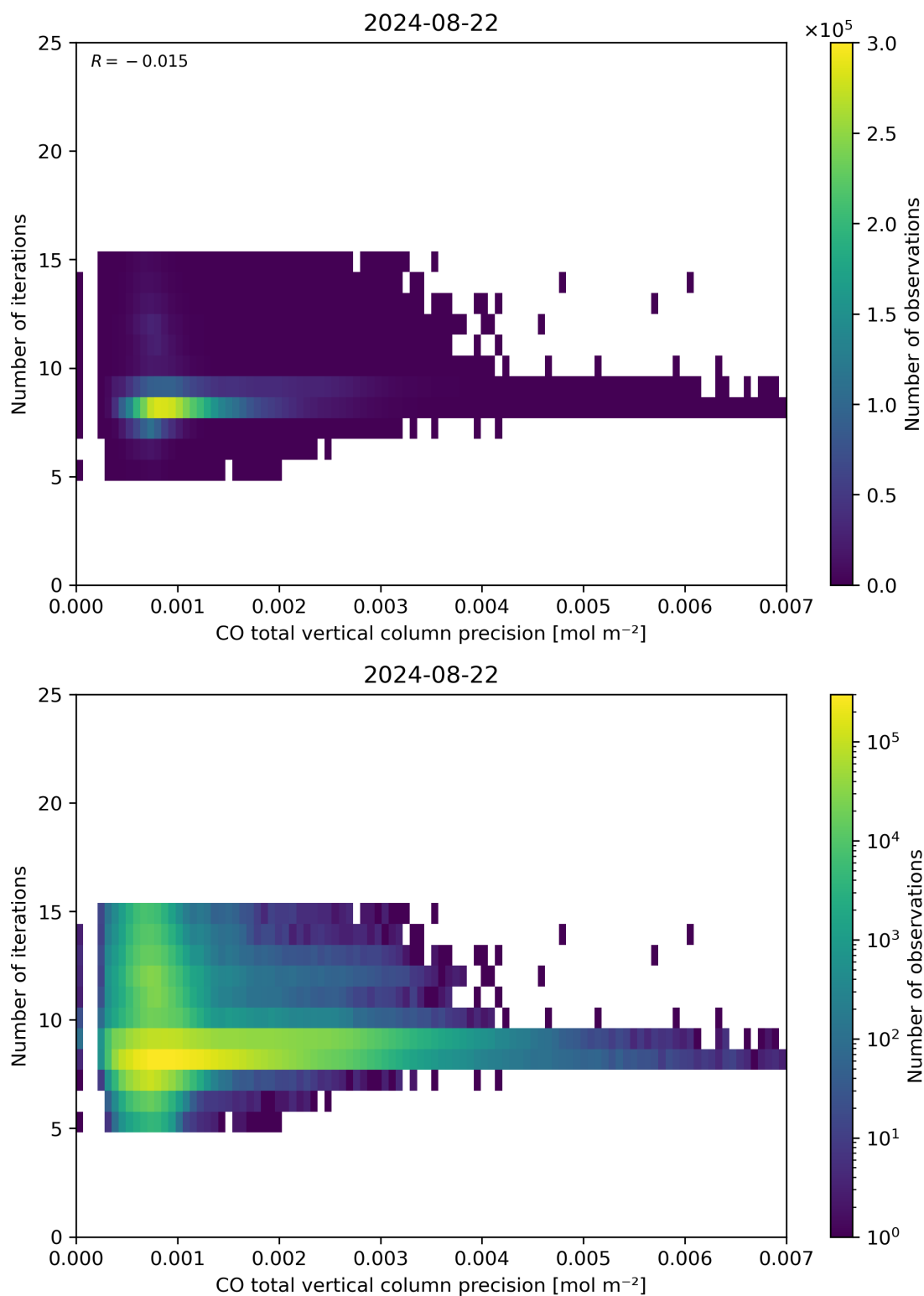
Figure 46: Scatter density plot of “CO total vertical column precision” against “Number of iterations” for 2024-08-22 to 2024-08-23.
