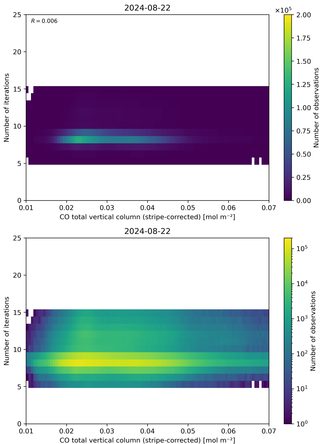
Figure 39: Scatter density plot of “CO total vertical column (stripe-corrected)” against “Number of iterations” for 2024-08-22 to 2024-08-23.
