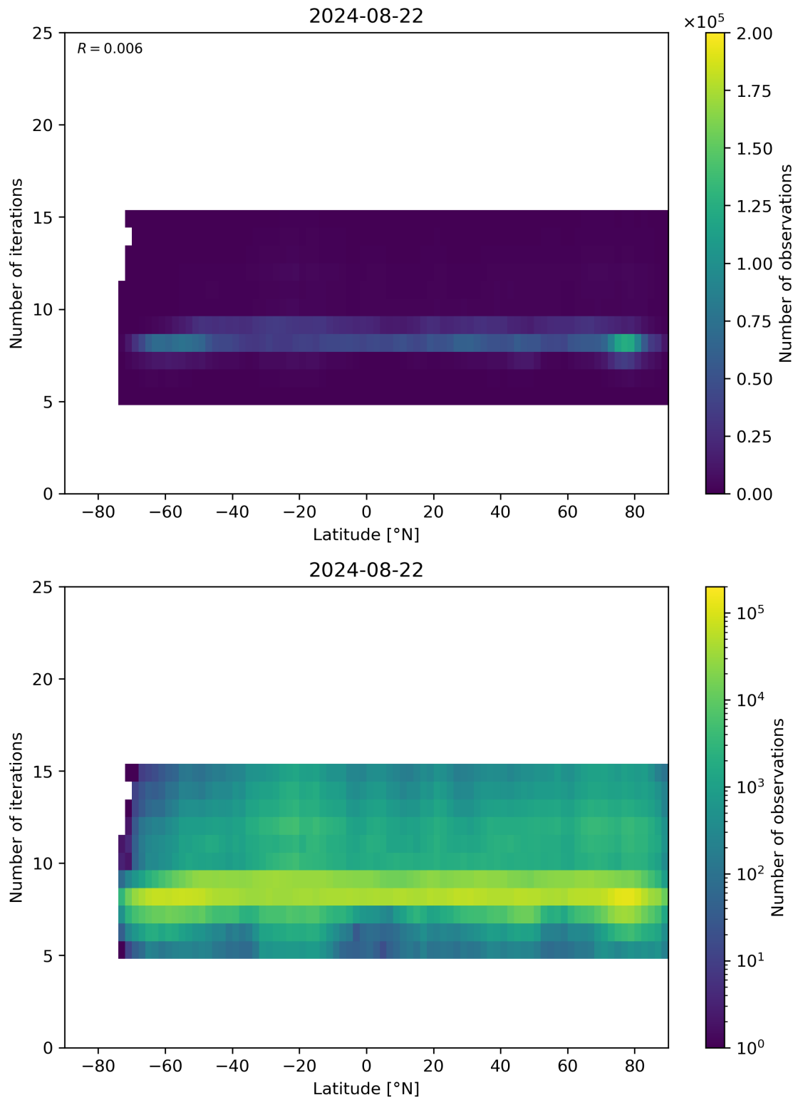
Figure 56: Scatter density plot of “Latitude” against “Number of iterations” for 2024-08-22 to 2024-08-23.
