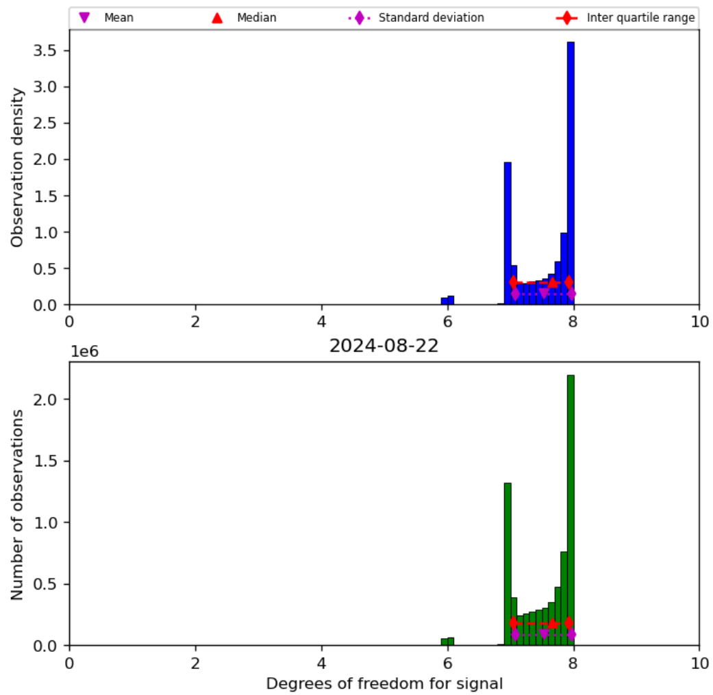
Figure 23: Histogram of “Degrees of freedom for signal” for 2024-08-22 to 2024-08-23
