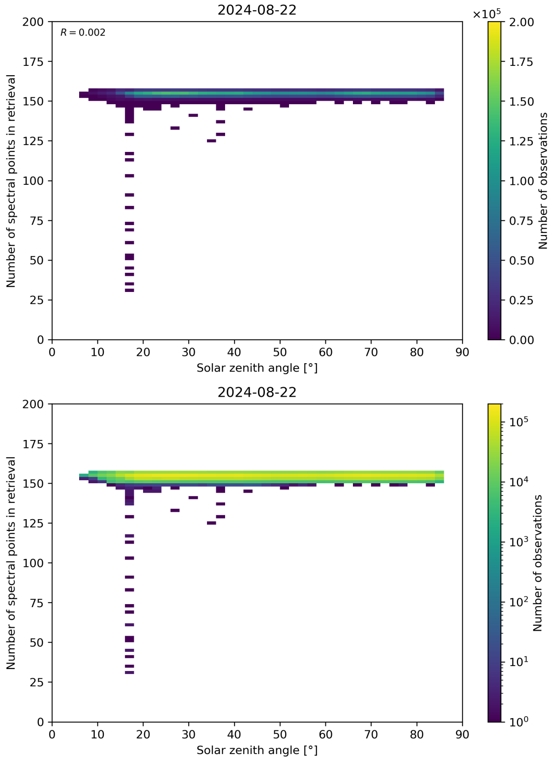
Figure 68: Scatter density plot of “Solar zenith angle” against “Number of spectral points in retrieval” for 2024-08-22 to 2024-08-23.
