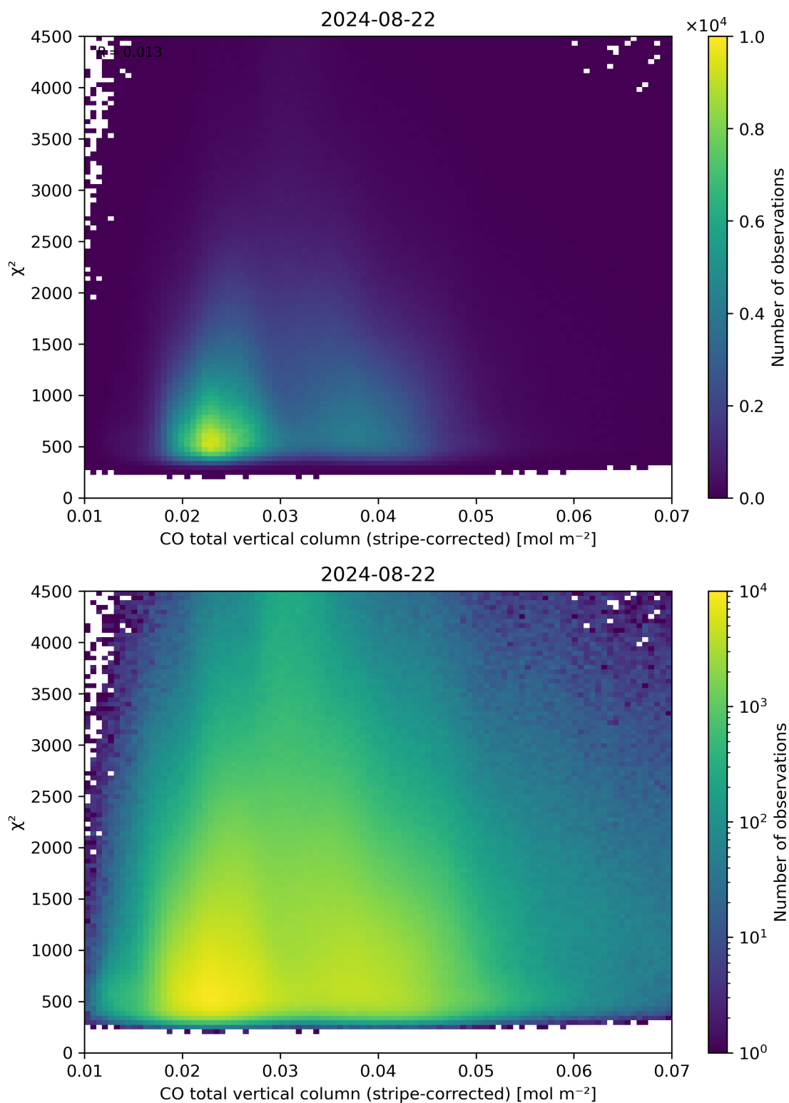
Figure 37: Scatter density plot of “CO total vertical column (stripe-corrected)” against “ \chi^2 ” for 2024-08-22 to 2024-08-23.
