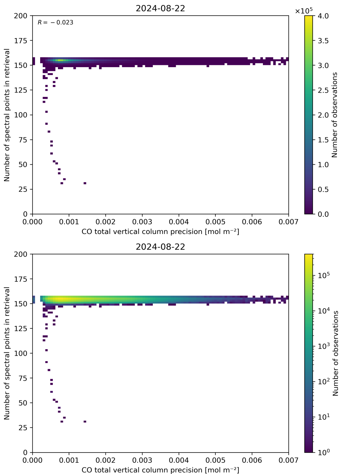
Figure 47: Scatter density plot of “CO total vertical column precision” against “Number of spectral points in retrieval” for 2024-08-22 to 2024-08-23.
