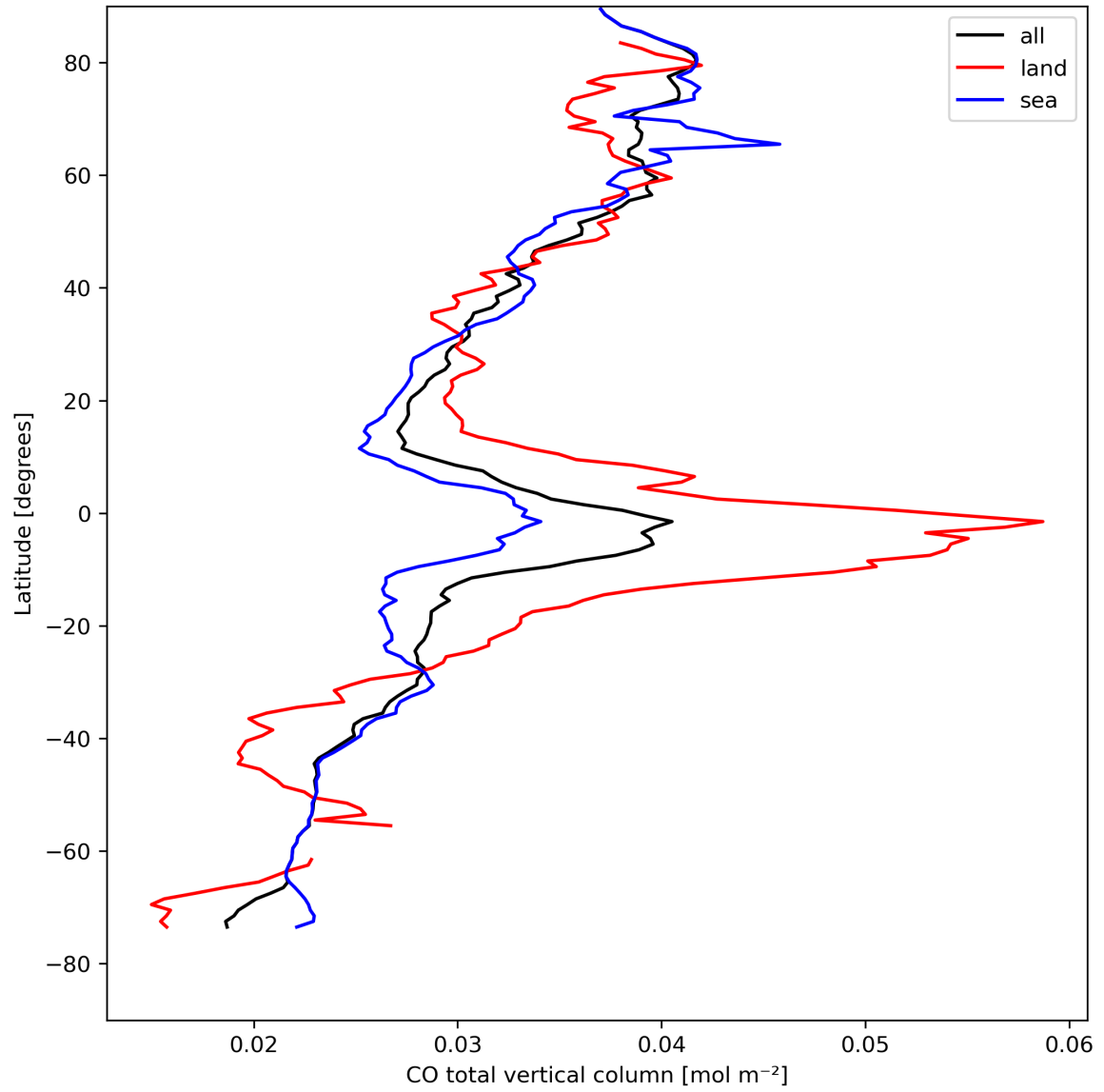
Figure 10: Zonal average of “CO total vertical column” for 2024-08-22 to 2024-08-23.
