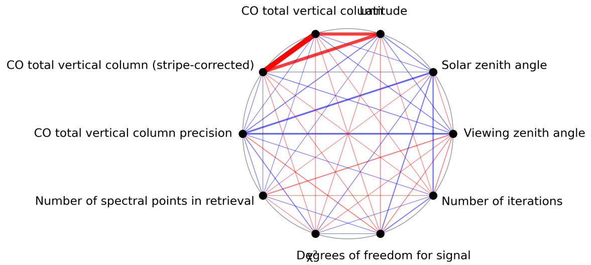
Figure 1: Map of correlation graph for 2024-08-22 to 2024-08-23.
