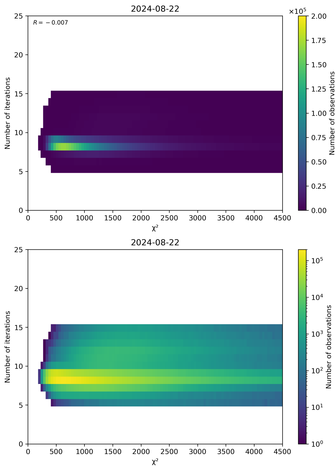
Figure 49: Scatter density plot of “ \chi^2 ” against “Number of iterations” for 2024-08-22 to 2024-08-23.
