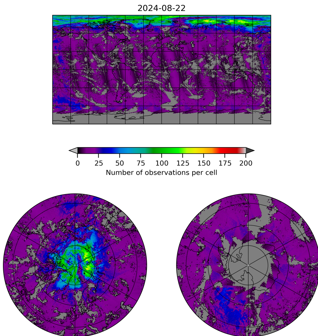
Figure 8: Map of the number of observations for 2024-08-22 to 2024-08-23
