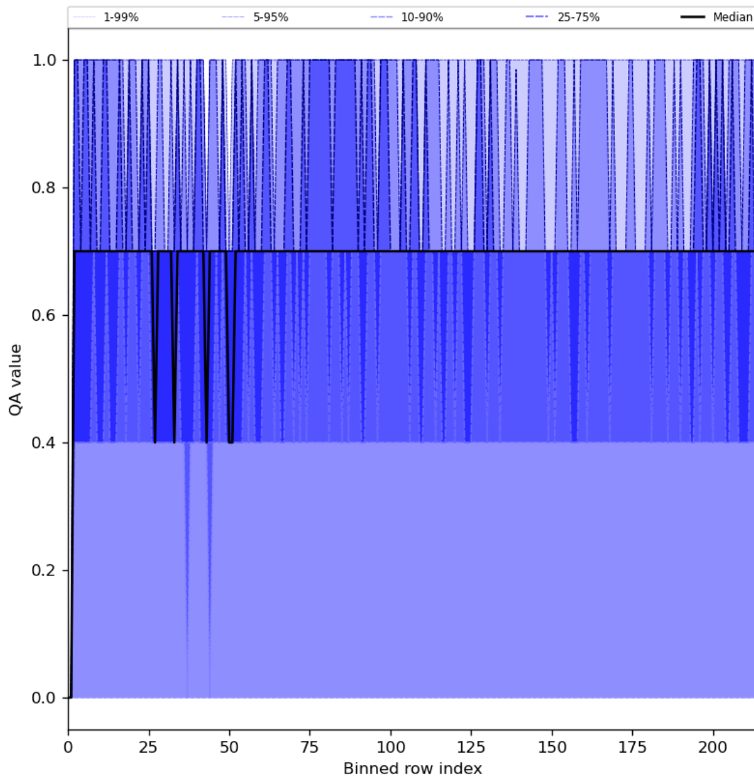
Figure 25: Along track statistics of “QA value” for 2024-08-22 to 2024-08-23
