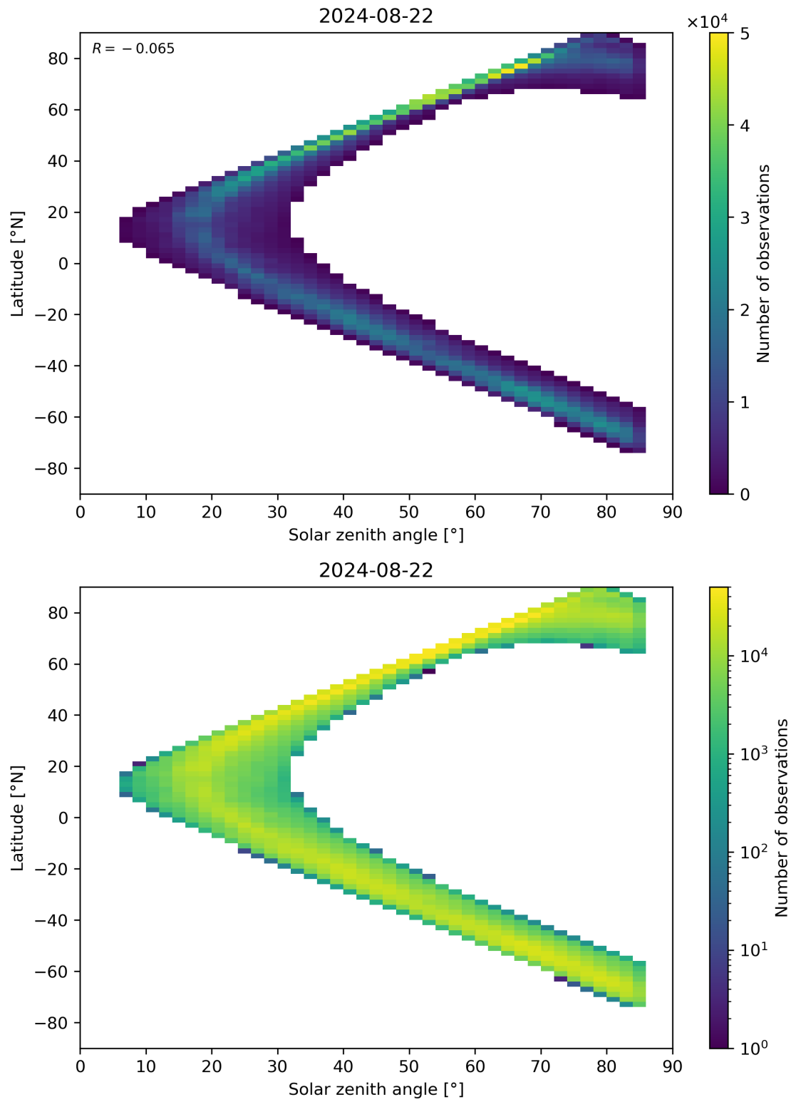
Figure 66: Scatter density plot of “Solar zenith angle” against “Latitude” for 2024-08-22 to 2024-08-23.
