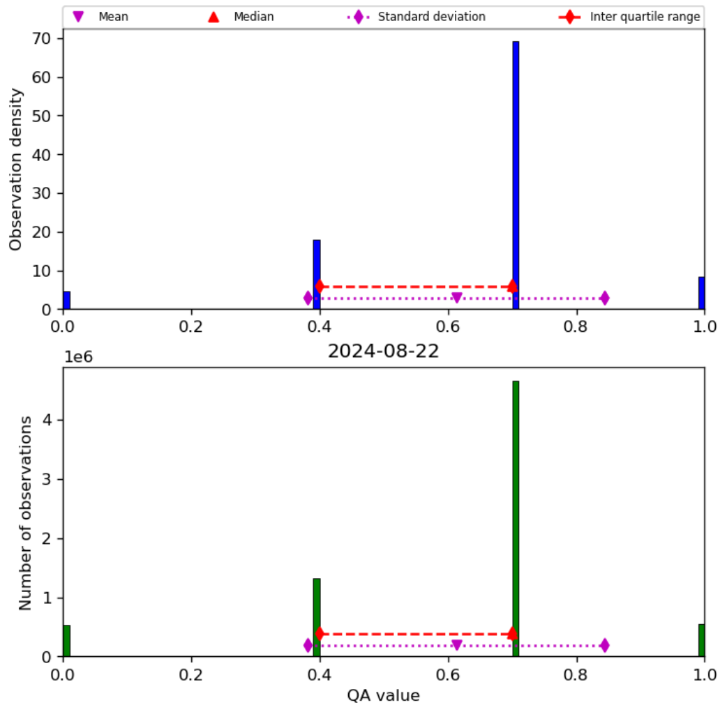
Figure 17: Histogram of “QA value” for 2024-08-22 to 2024-08-23
