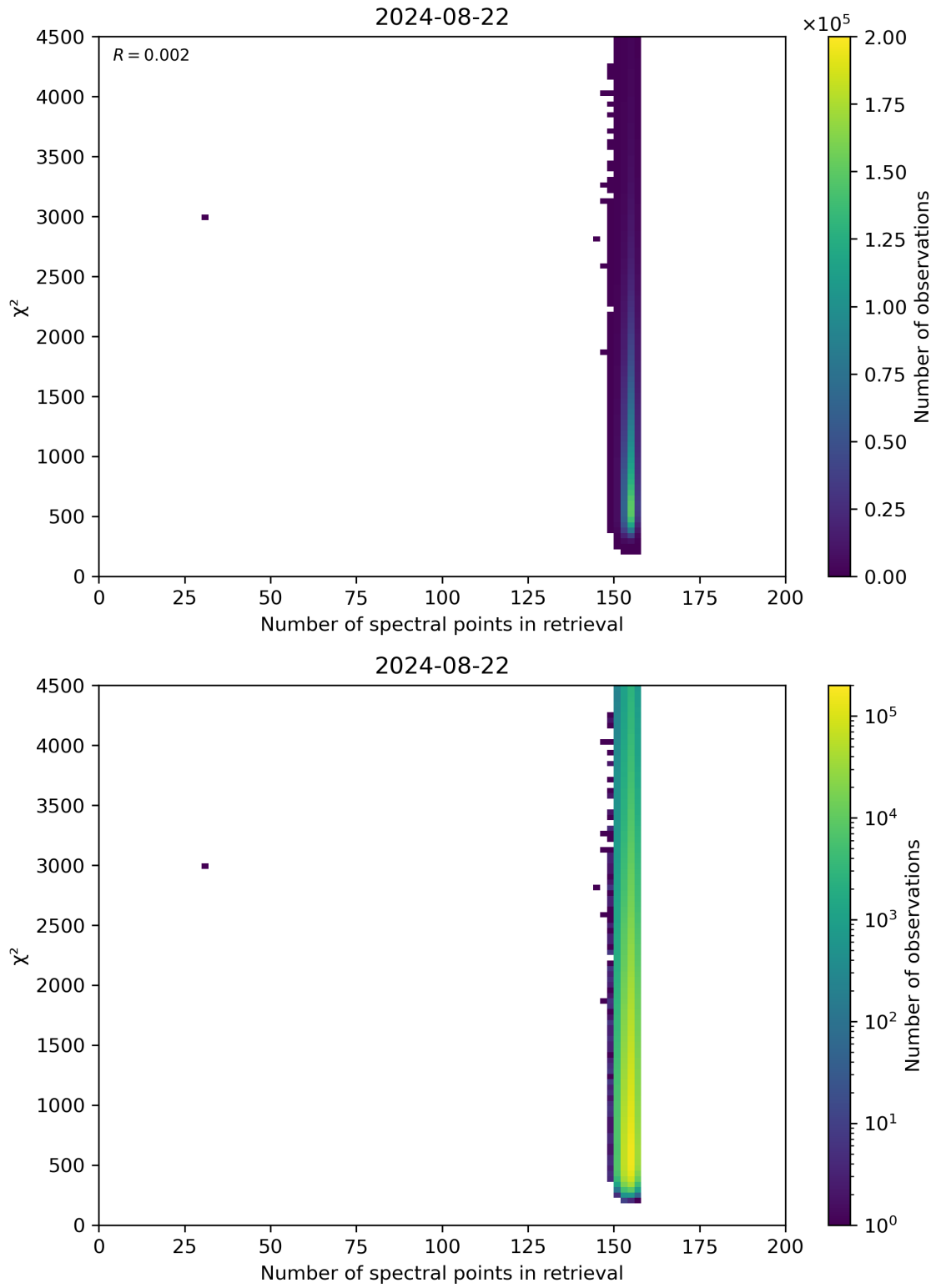
Figure 58: Scatter density plot of “Number of spectral points in retrieval” against “ \chi^2 ” for 2024-08-22 to 2024-08-23.
