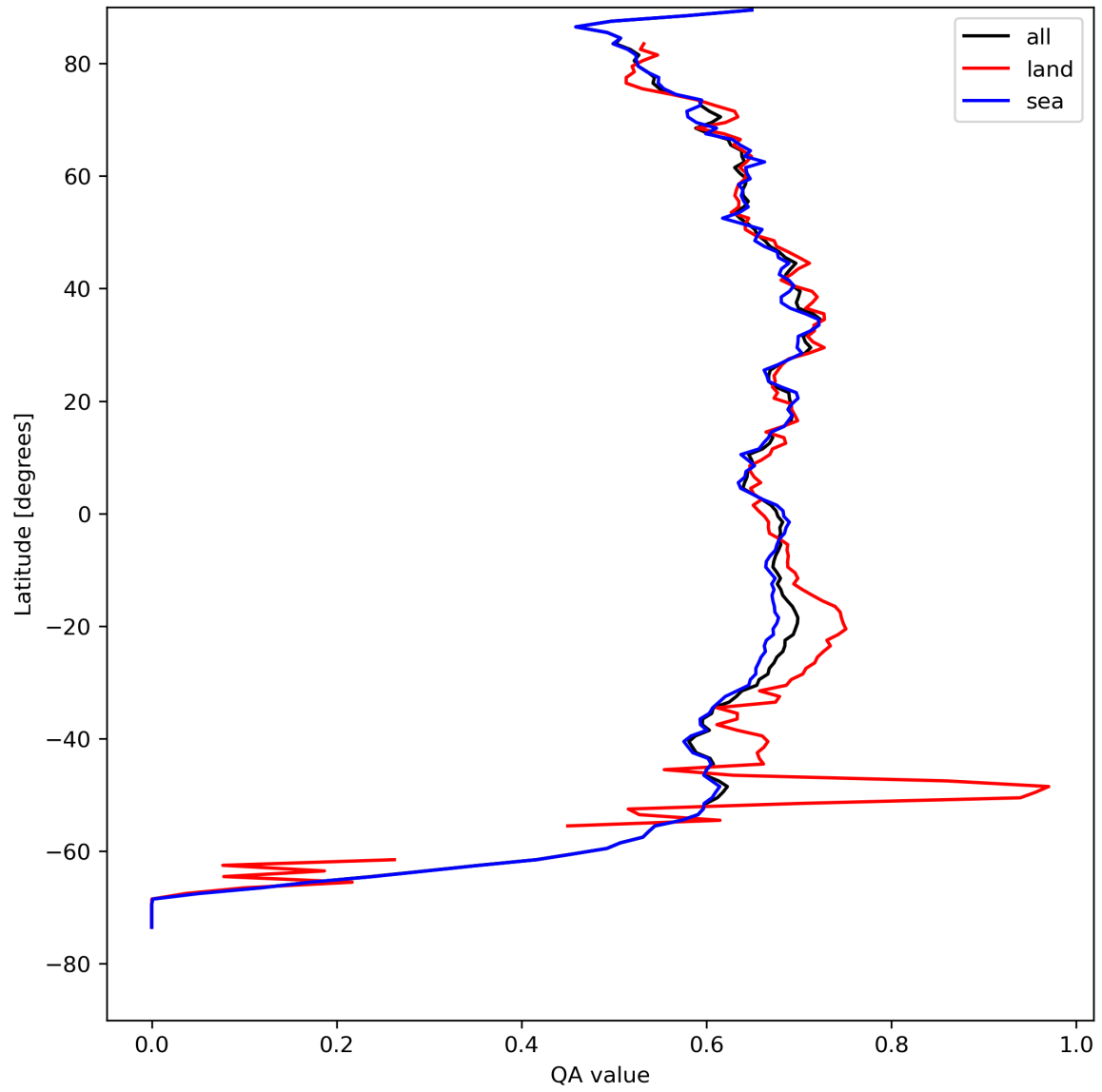
Figure 9: Zonal average of “QA value” for 2024-08-22 to 2024-08-23.
