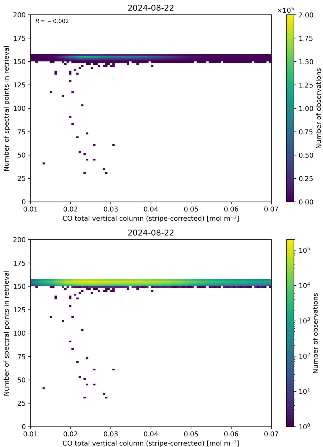
Figure 40: Scatter density plot of “CO total vertical column (stripe-corrected)” against “Number of spectral points in retrieval” for 2024-08-22 to 2024-08-23.
