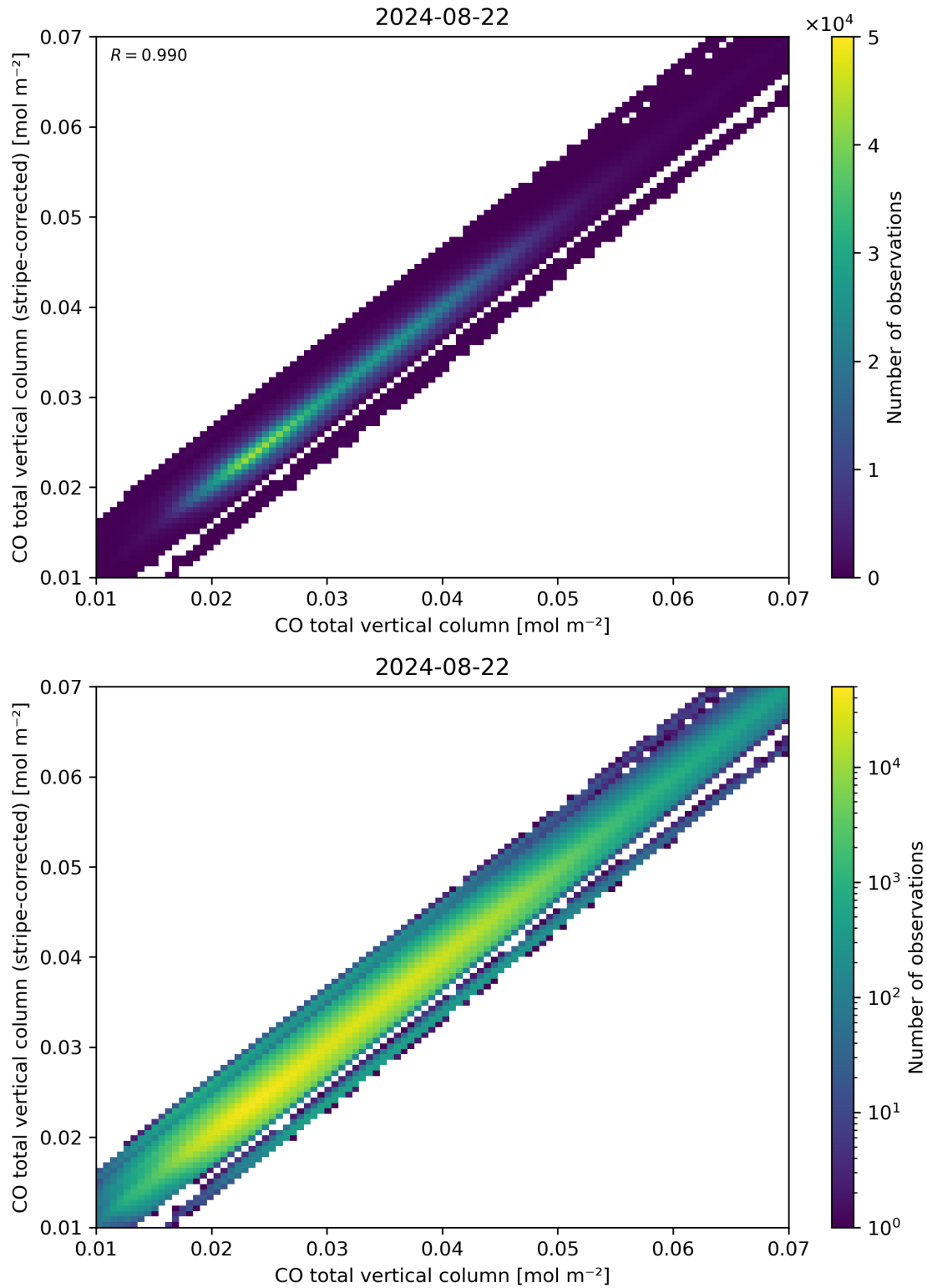
Figure 33: Scatter density plot of “CO total vertical column” against “CO total vertical column (stripe-corrected)” for 2024-08-22 to 2024-08-23.
