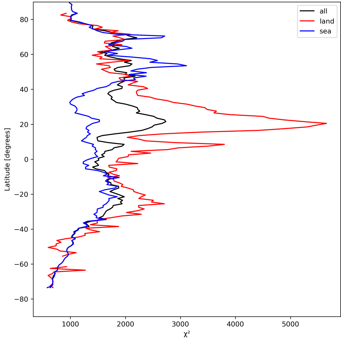
Figure 14: Zonal average of “ \chi^2 ” for 2024-08-22 to 2024-08-23.
