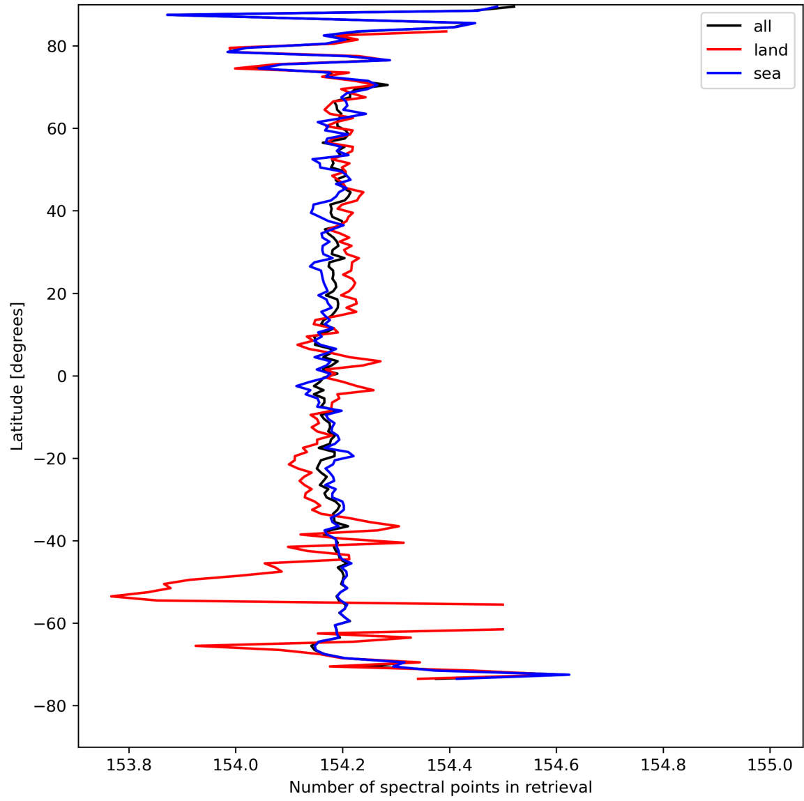
Figure 13: Zonal average of “Number of spectral points in retrieval” for 2024-08-22 to 2024-08-23.
