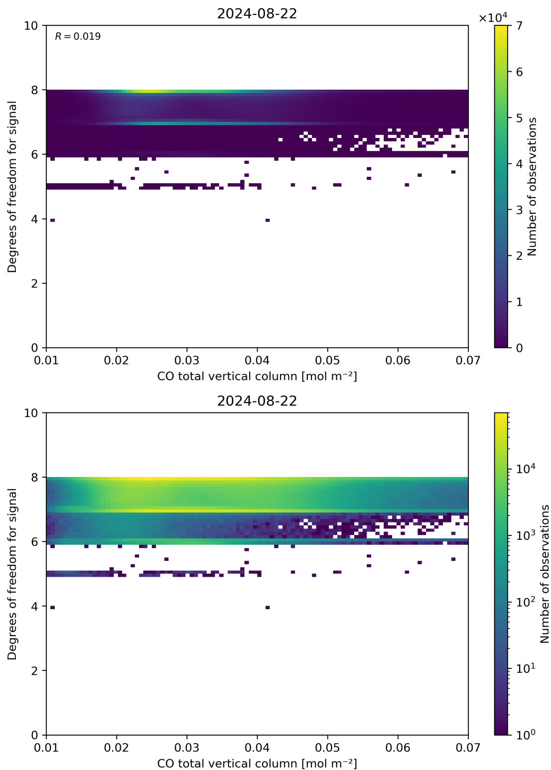
Figure 41: Scatter density plot of “CO total vertical column” against “Degrees of freedom for signal” for 2024-08-22 to 2024-08-23.
