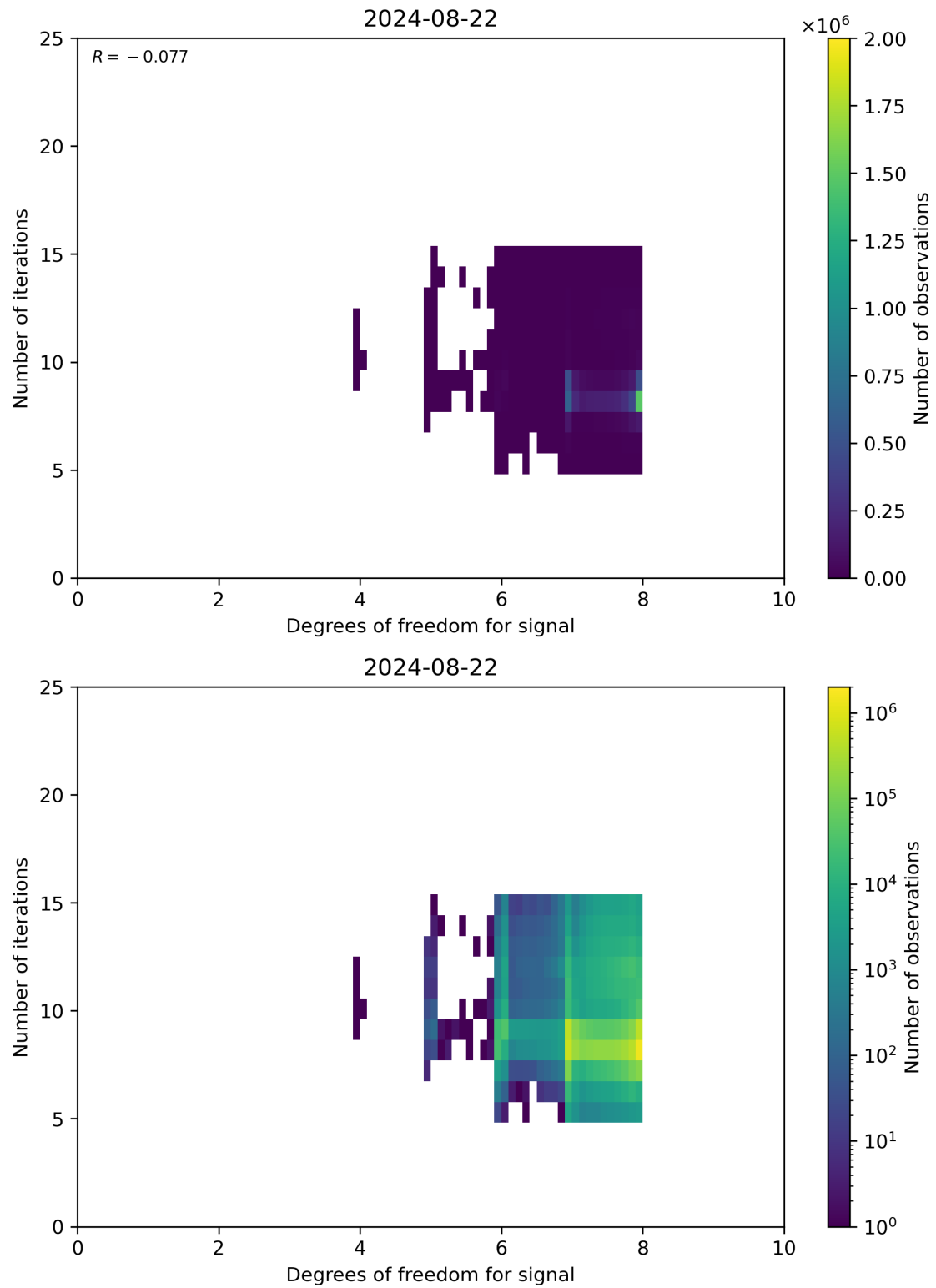
Figure 50: Scatter density plot of “Degrees of freedom for signal” against “Number of iterations” for 2024-08-22 to 2024-08-23.
