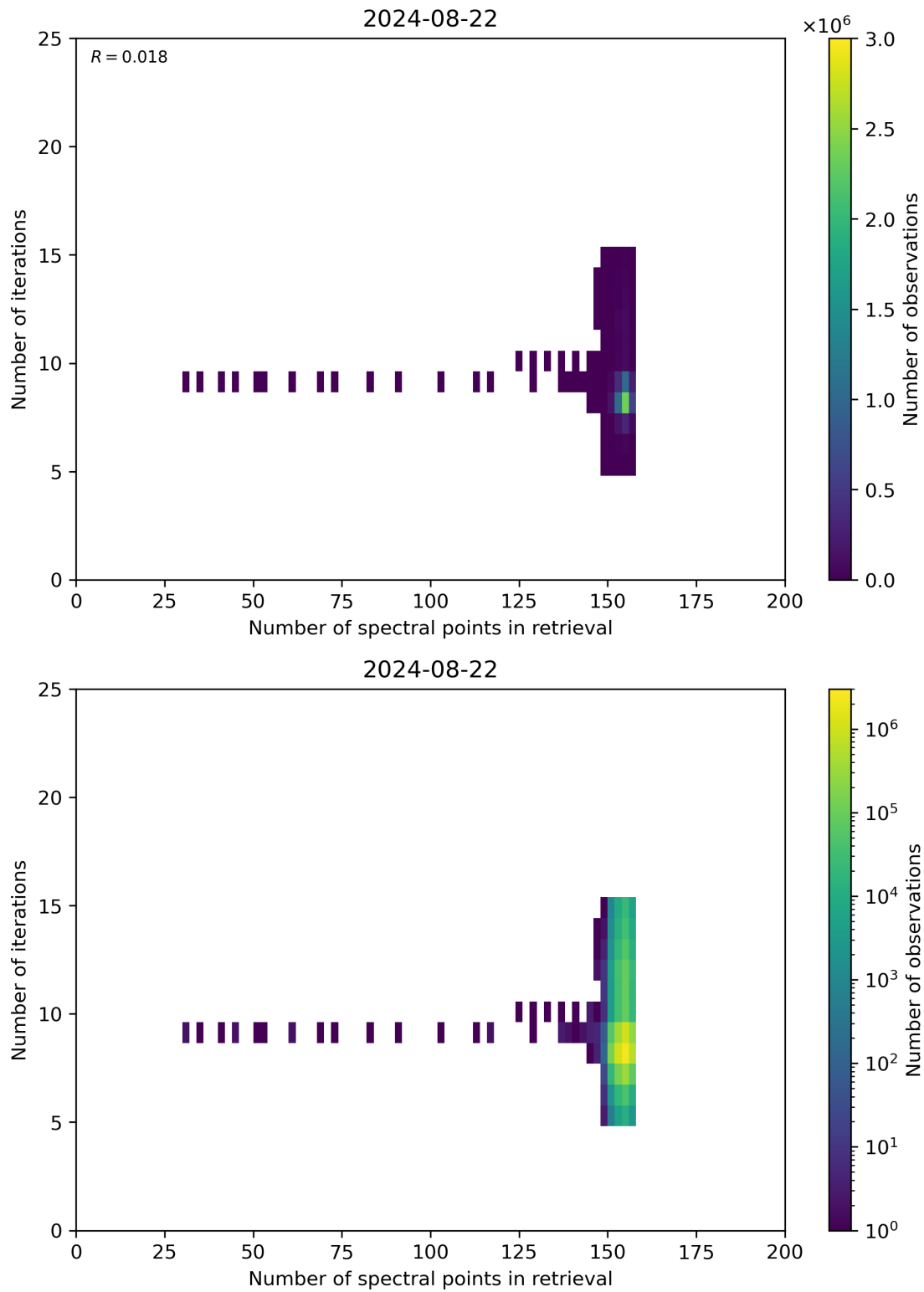
Figure 60: Scatter density plot of “Number of spectral points in retrieval” against “Number of iterations” for 2024-08-22 to 2024-08-23.
