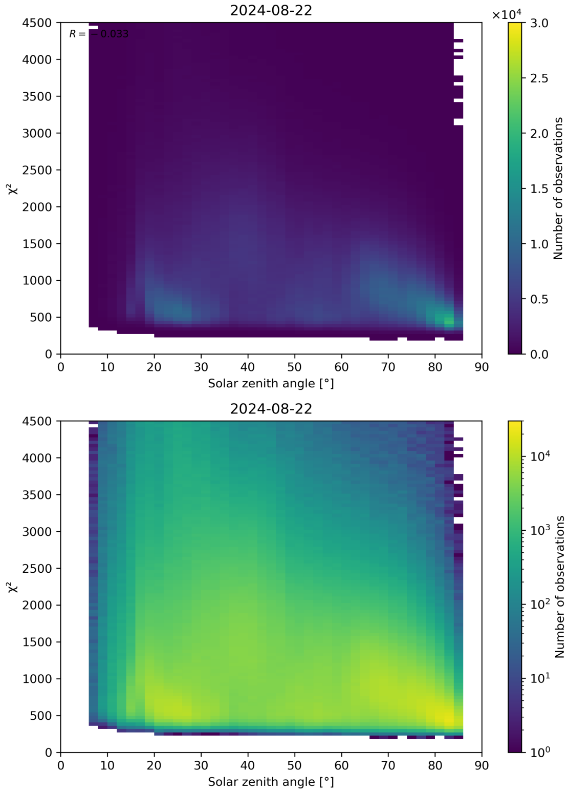
Figure 64: Scatter density plot of “Solar zenith angle” against “ \chi^2 ” for 2024-08-22 to 2024-08-23.
