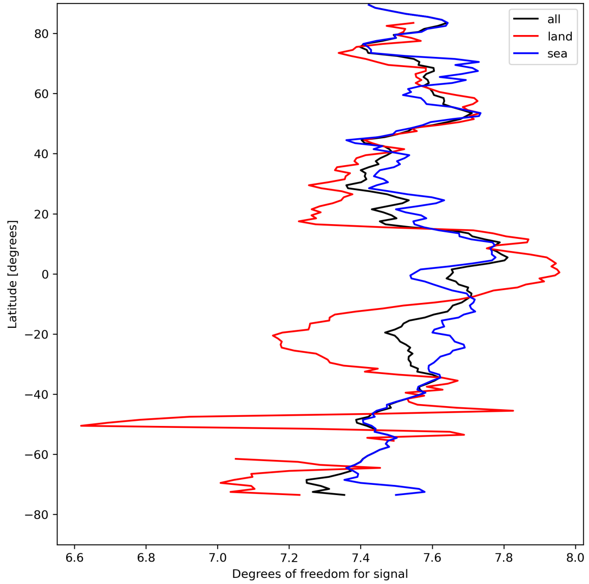
Figure 15: Zonal average of “Degrees of freedom for signal” for 2024-08-22 to 2024-08-23.
