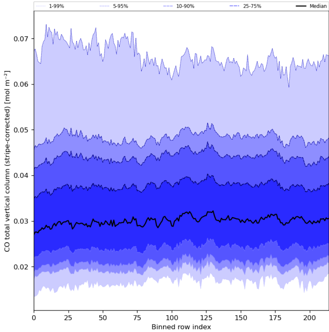
Figure 27: Along track statistics of “CO total vertical column (stripe-corrected)” for 2024-08-22 to 2024-08-23
