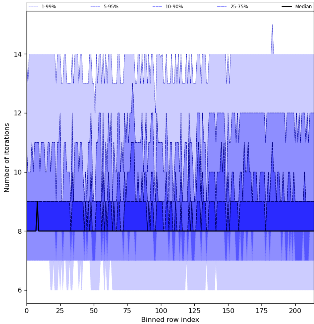
Figure 32: Along track statistics of “Number of iterations” for 2024-08-22 to 2024-08-23
