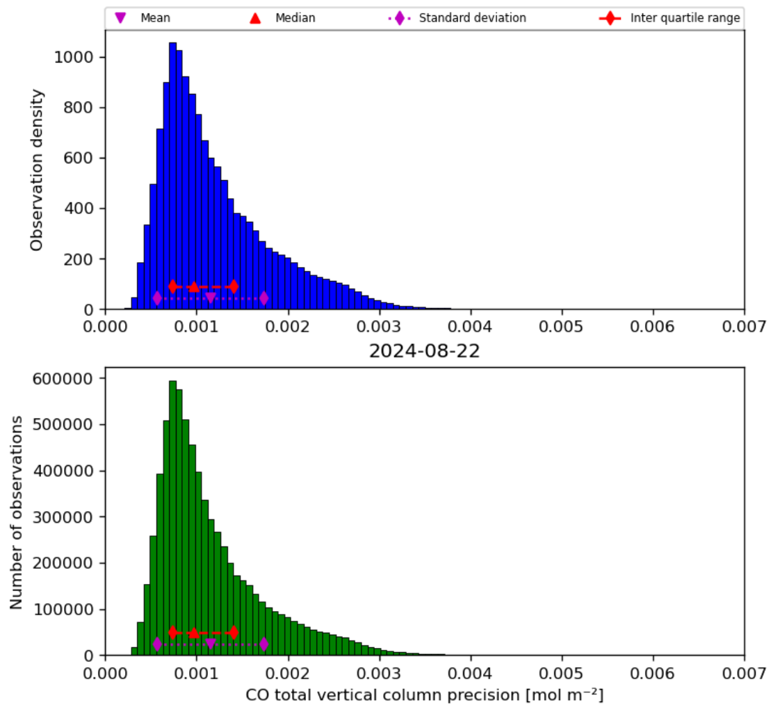
Figure 20: Histogram of “CO total vertical column precision” for 2024-08-22 to 2024-08-23
