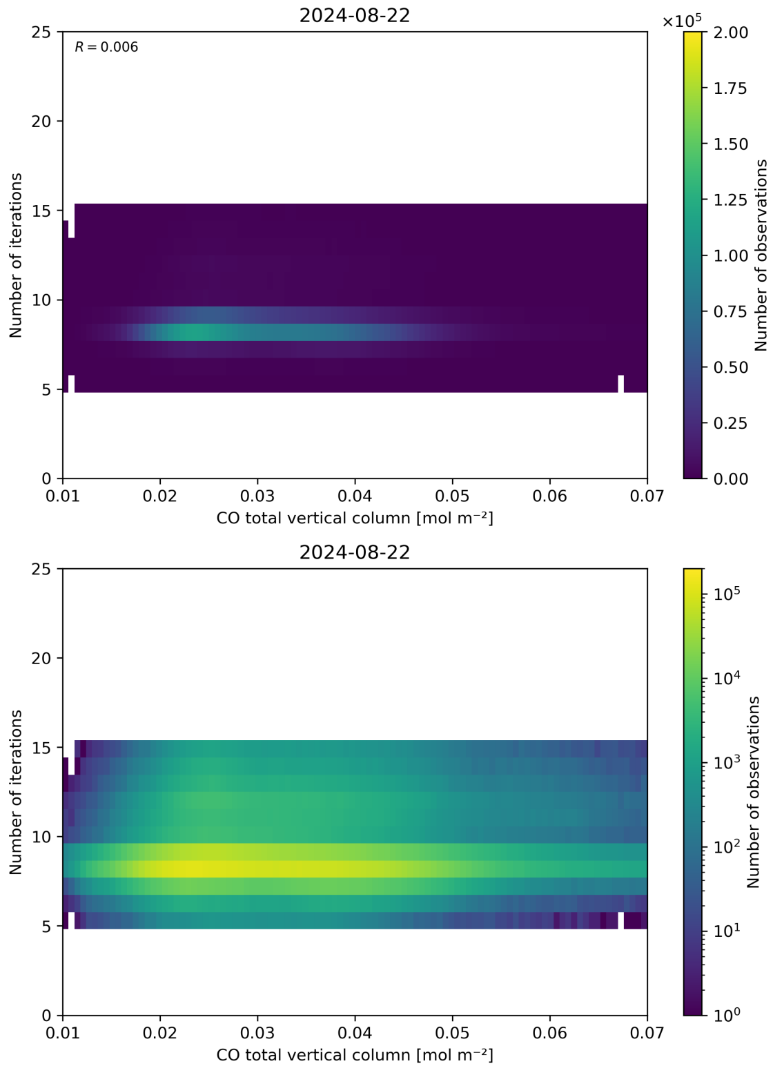
Figure 42: Scatter density plot of “CO total vertical column” against “Number of iterations” for 2024-08-22 to 2024-08-23.
