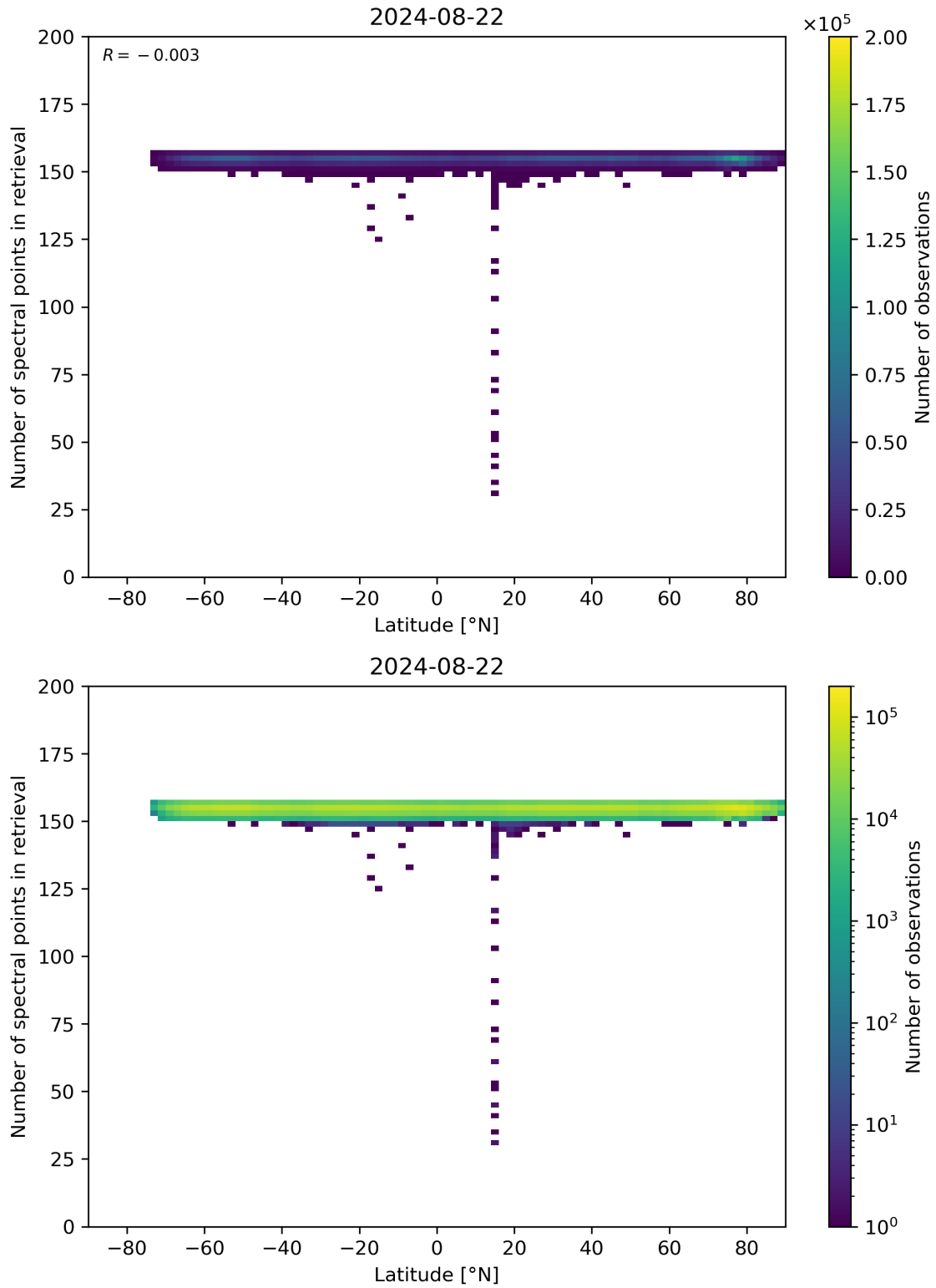
Figure 57: Scatter density plot of “Latitude” against “Number of spectral points in retrieval” for 2024-08-22 to 2024-08-23.
