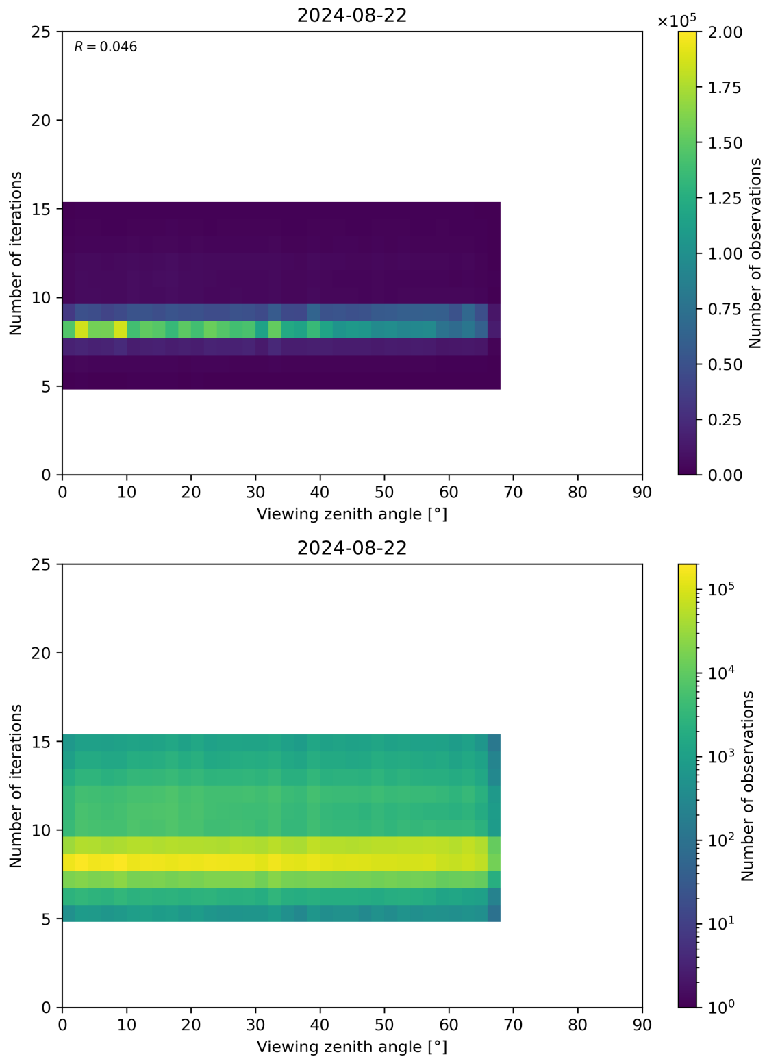
Figure 75: Scatter density plot of “Viewing zenith angle” against “Number of iterations” for 2024-08-22 to 2024-08-23.
