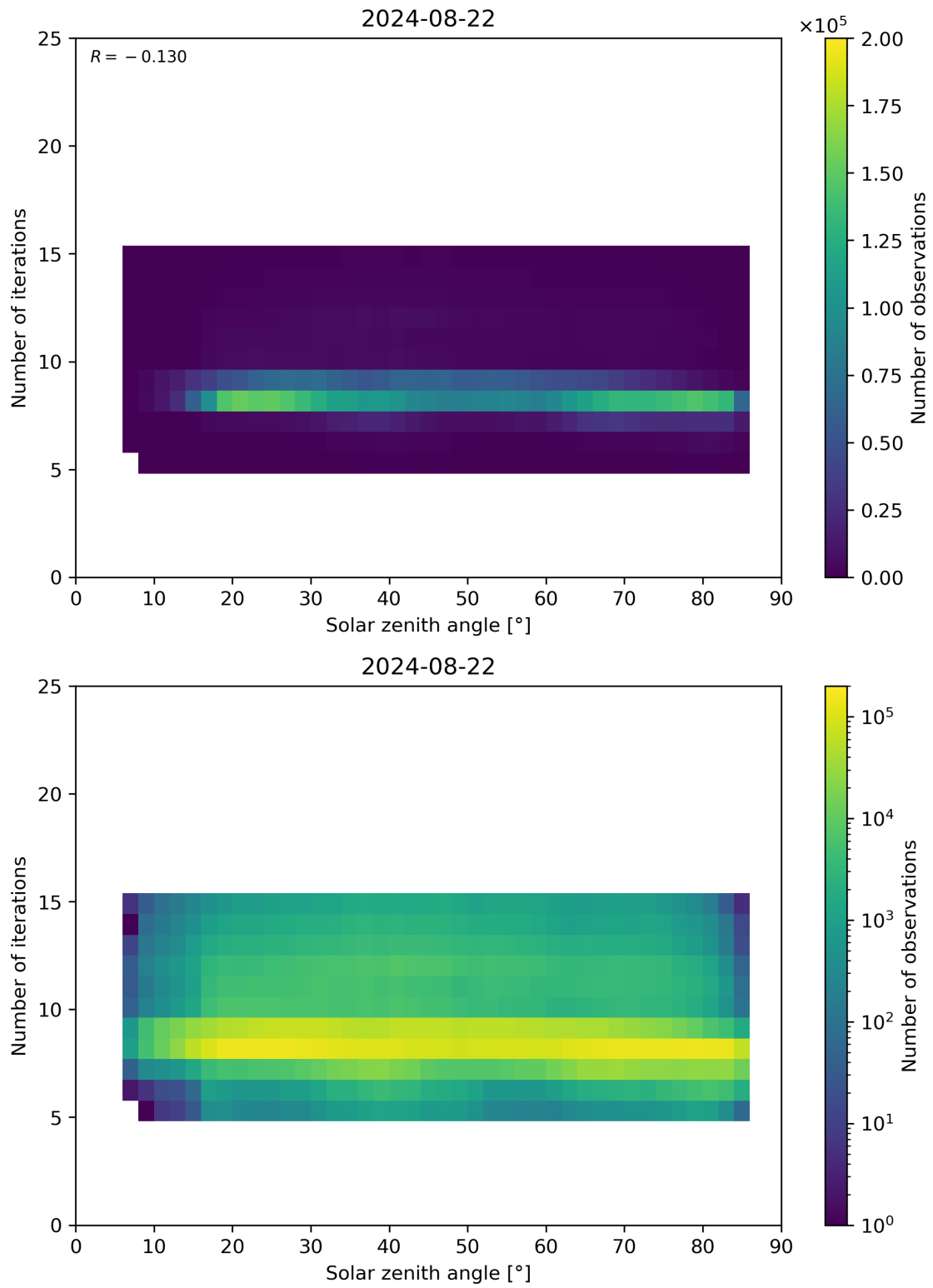
Figure 67: Scatter density plot of “Solar zenith angle” against “Number of iterations” for 2024-08-22 to 2024-08-23.
