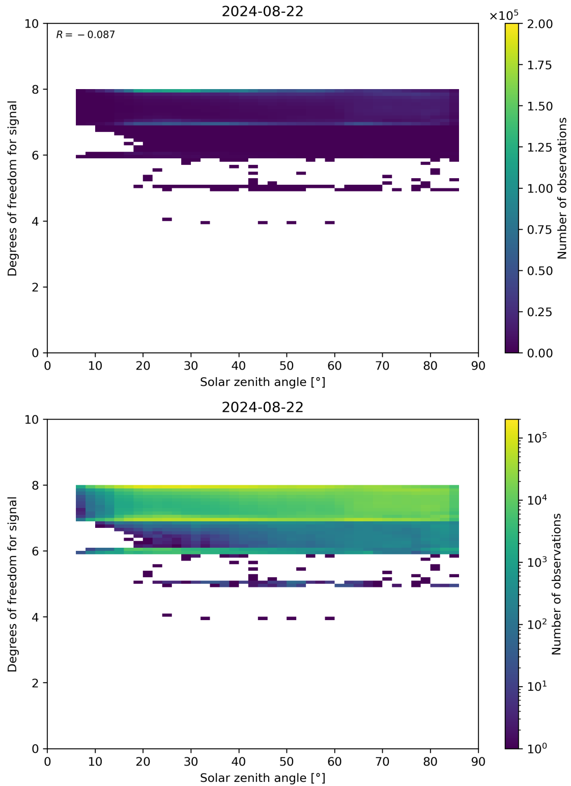
Figure 65: Scatter density plot of “Solar zenith angle” against “Degrees of freedom for signal” for 2024-08-22 to 2024-08-23.
