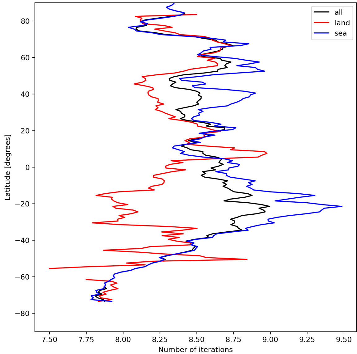
Figure 16: Zonal average of “Number of iterations” for 2024-08-22 to 2024-08-23.
