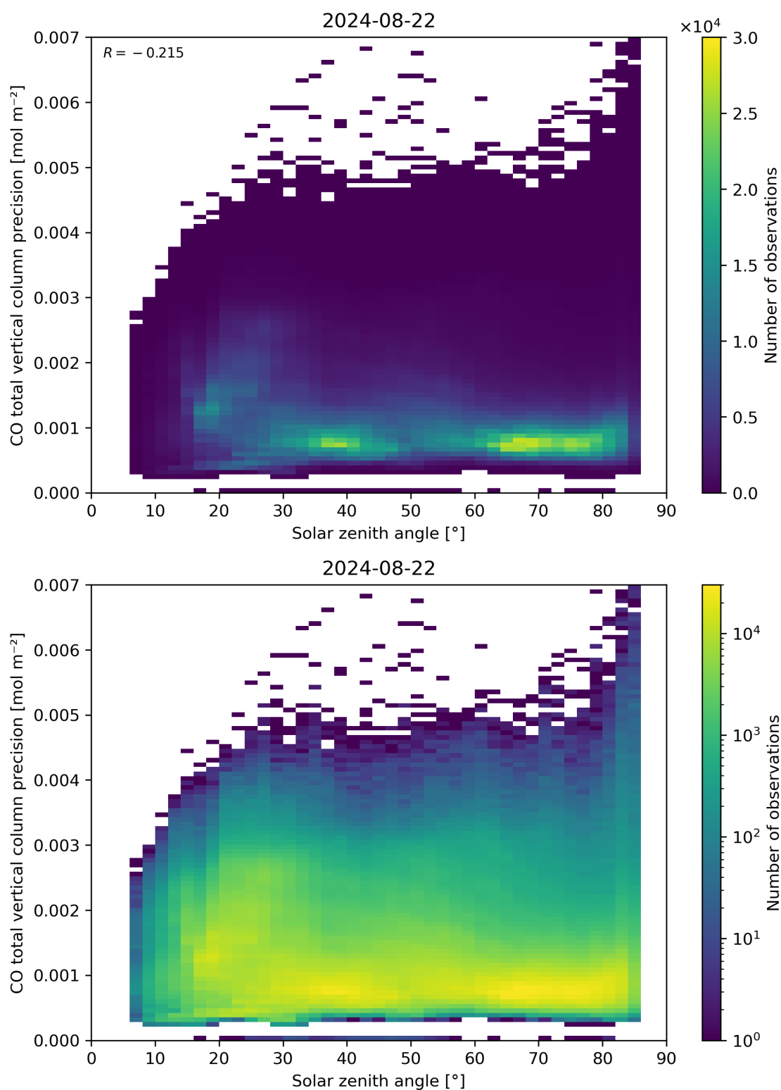
Figure 63: Scatter density plot of “Solar zenith angle” against “CO total vertical column precision” for 2024-08-22 to 2024-08-23.
