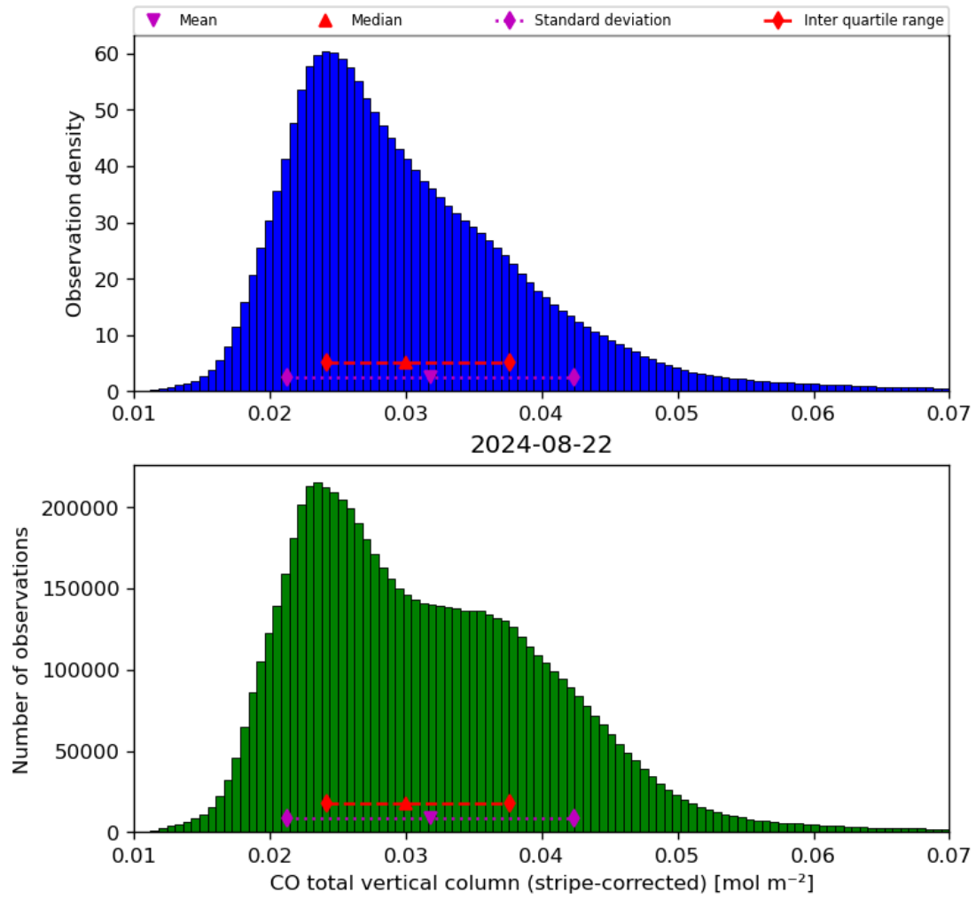
Figure 19: Histogram of “CO total vertical column (stripe-corrected)” for 2024-08-22 to 2024-08-23
