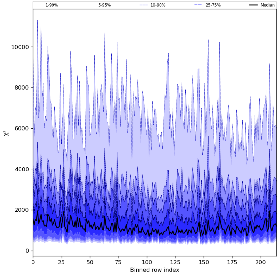
Figure 30: Along track statistics of “ \chi^2 ” for 2024-08-22 to 2024-08-23
