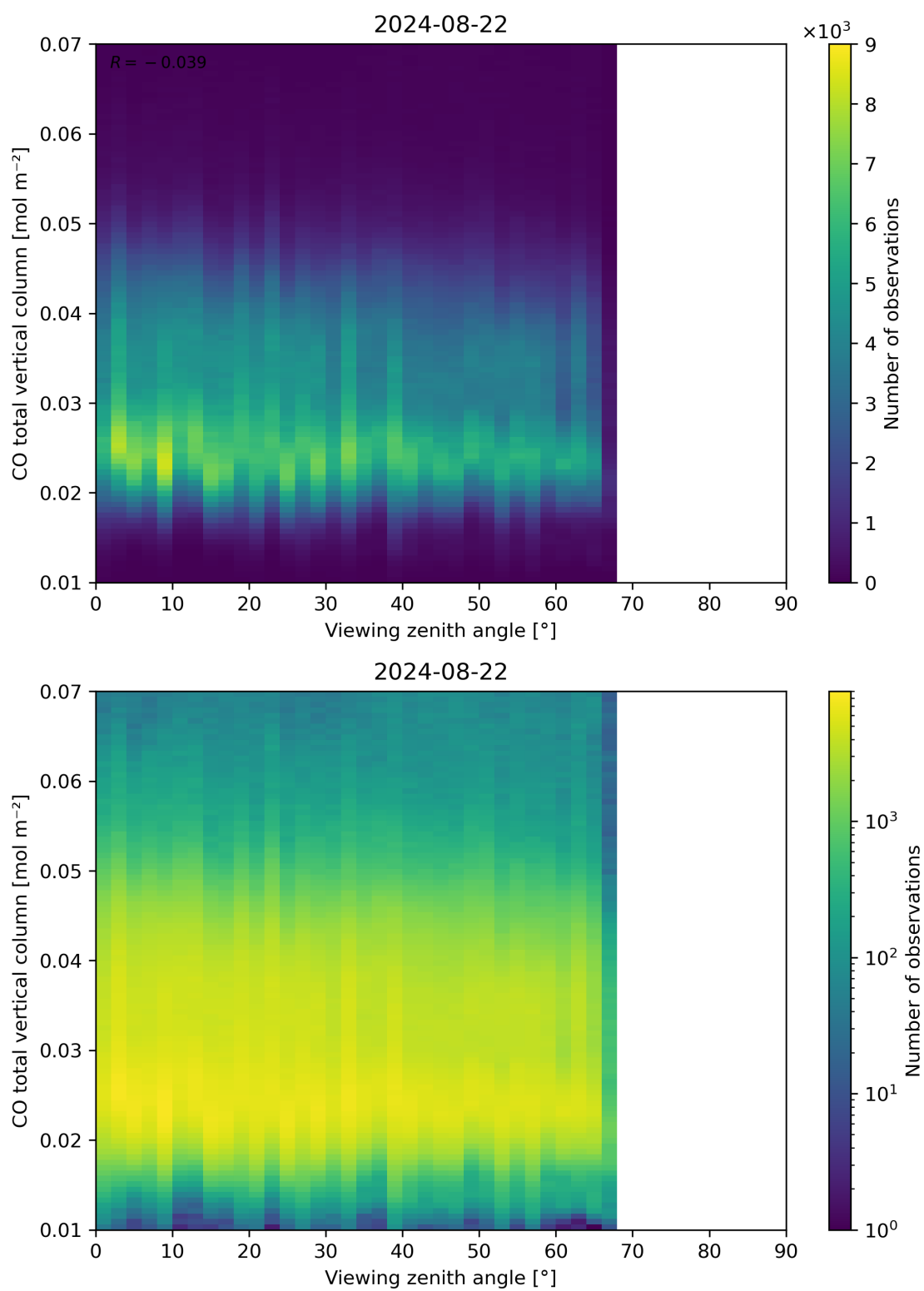
Figure 69: Scatter density plot of “Viewing zenith angle” against “CO total vertical column” for 2024-08-22 to 2024-08-23.
