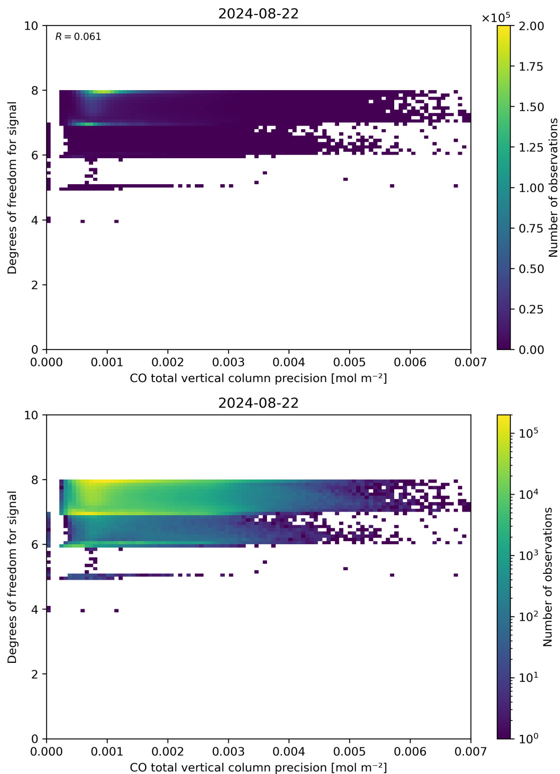
Figure 45: Scatter density plot of “CO total vertical column precision” against “Degrees of freedom for signal” for 2024-08-22 to 2024-08-23.
