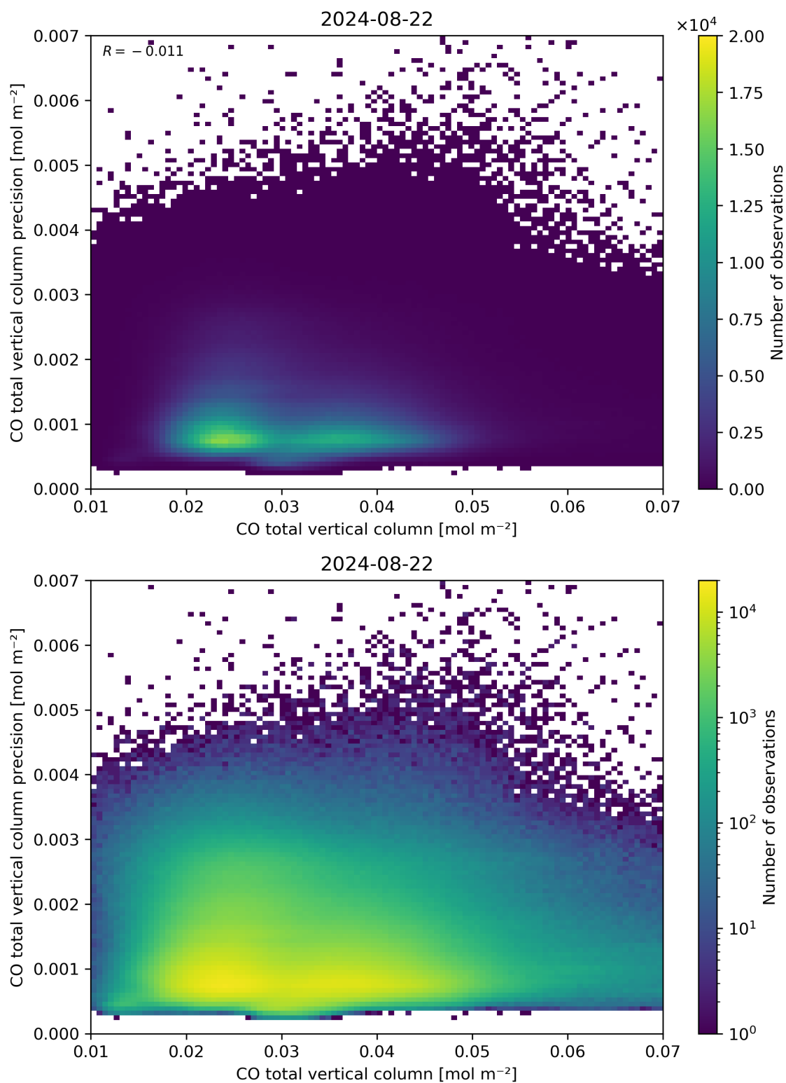
Figure 34: Scatter density plot of “CO total vertical column” against “CO total vertical column precision” for 2024-08-22 to 2024-08-23.
