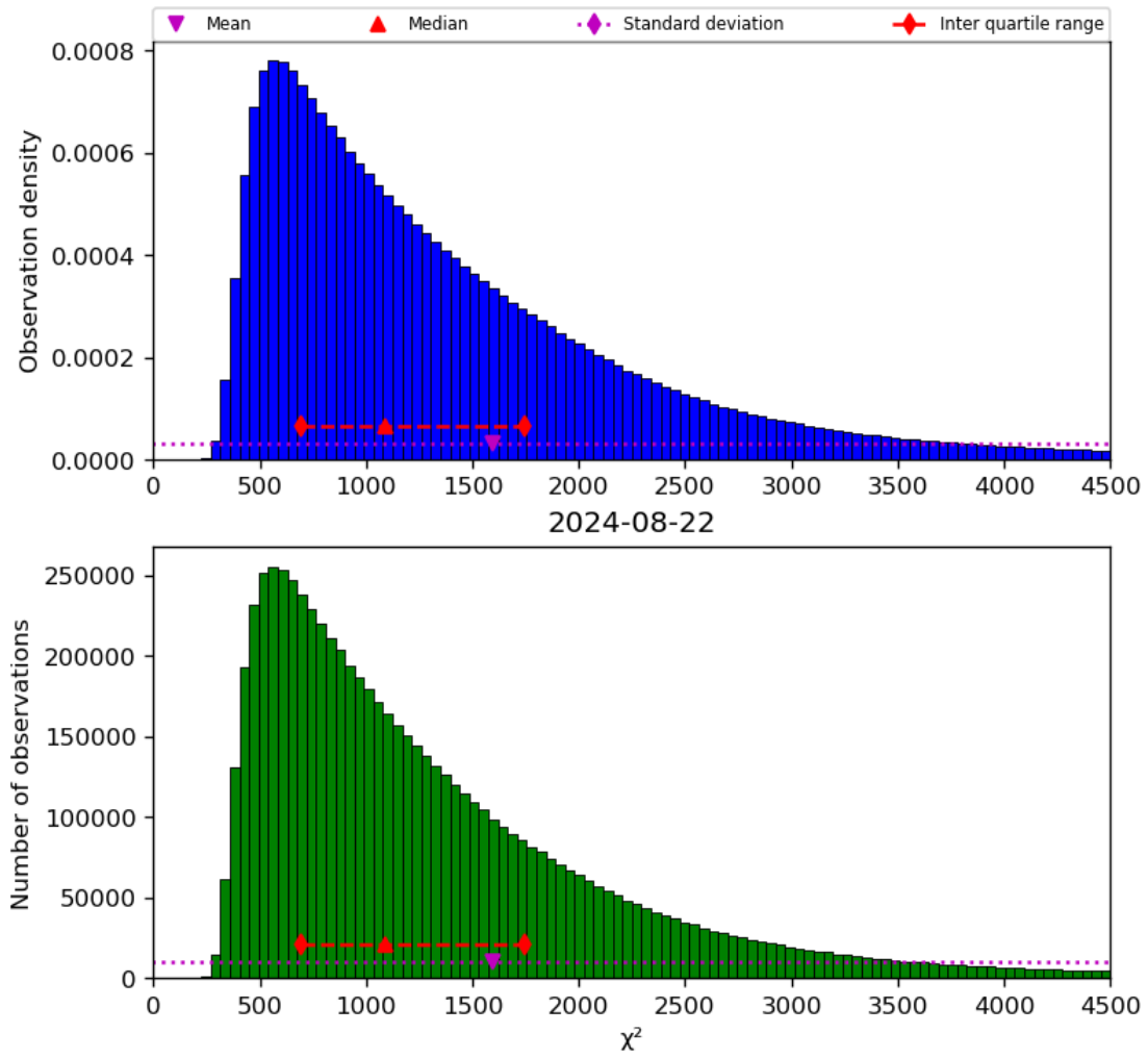
Figure 22: Histogram of “ \chi^2 ” for 2024-08-22 to 2024-08-23
