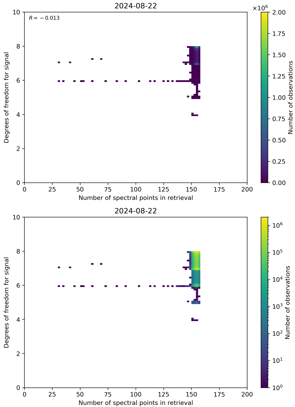
Figure 59: Scatter density plot of “Number of spectral points in retrieval” against “Degrees of freedom for signal” for 2024-08-22 to 2024-08-23.
