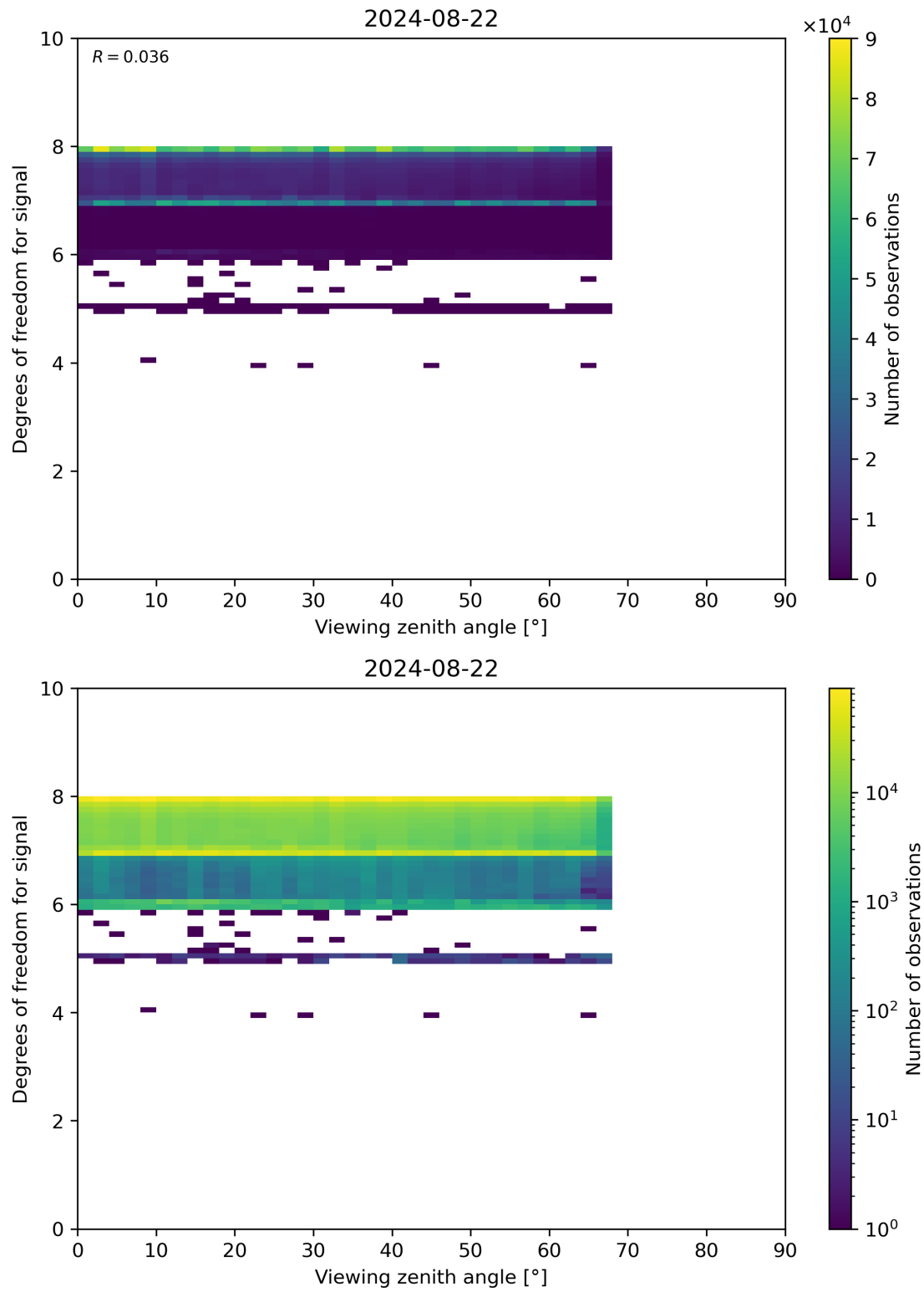
Figure 73: Scatter density plot of “Viewing zenith angle” against “Degrees of freedom for signal” for 2024-08-22 to 2024-08-23.
