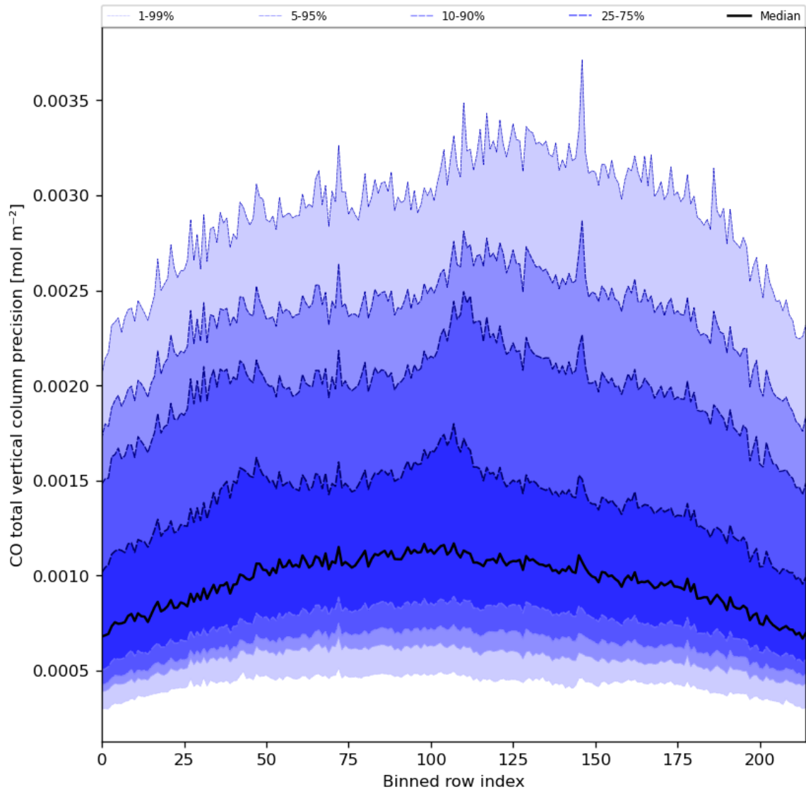
Figure 28: Along track statistics of “CO total vertical column precision” for 2024-08-22 to 2024-08-23
