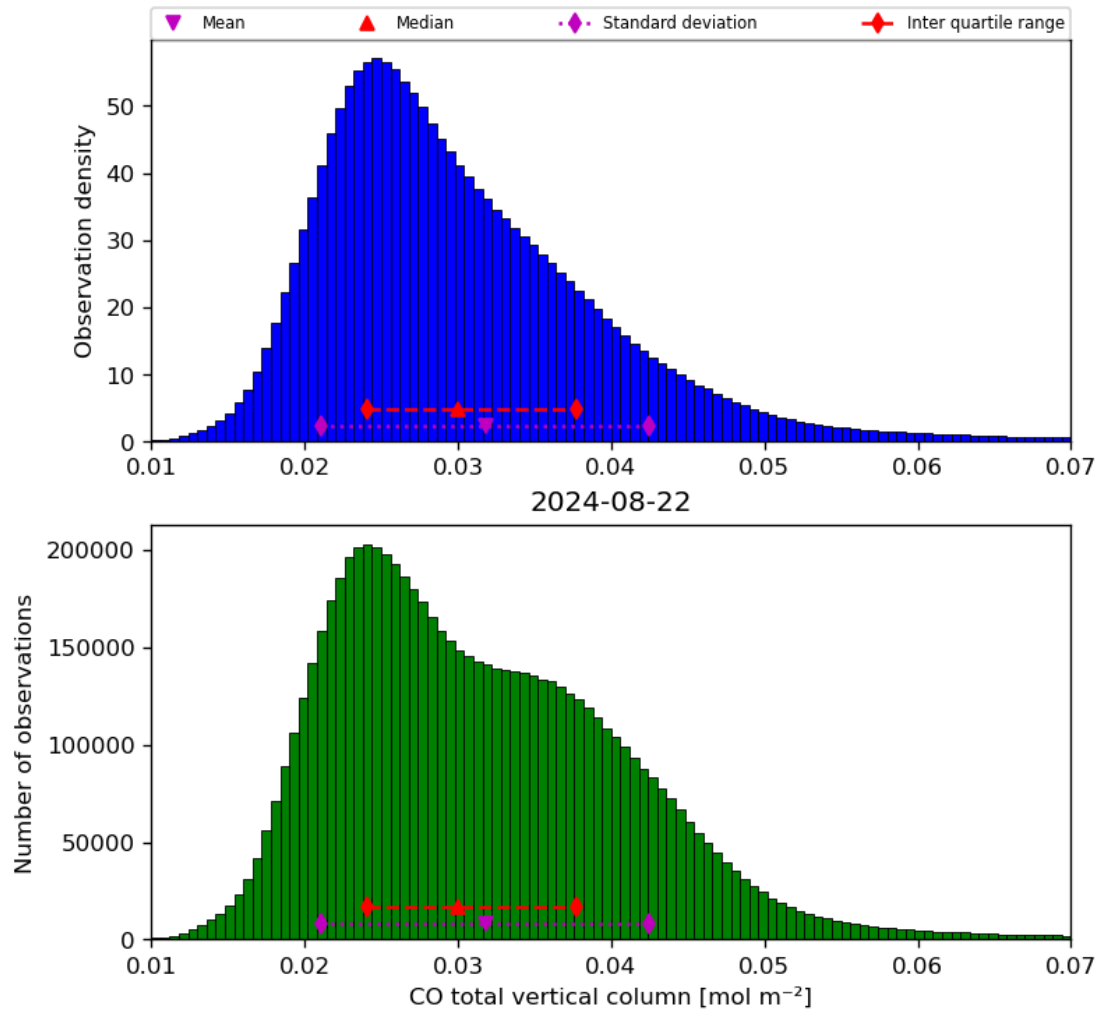
Figure 18: Histogram of “CO total vertical column” for 2024-08-22 to 2024-08-23
