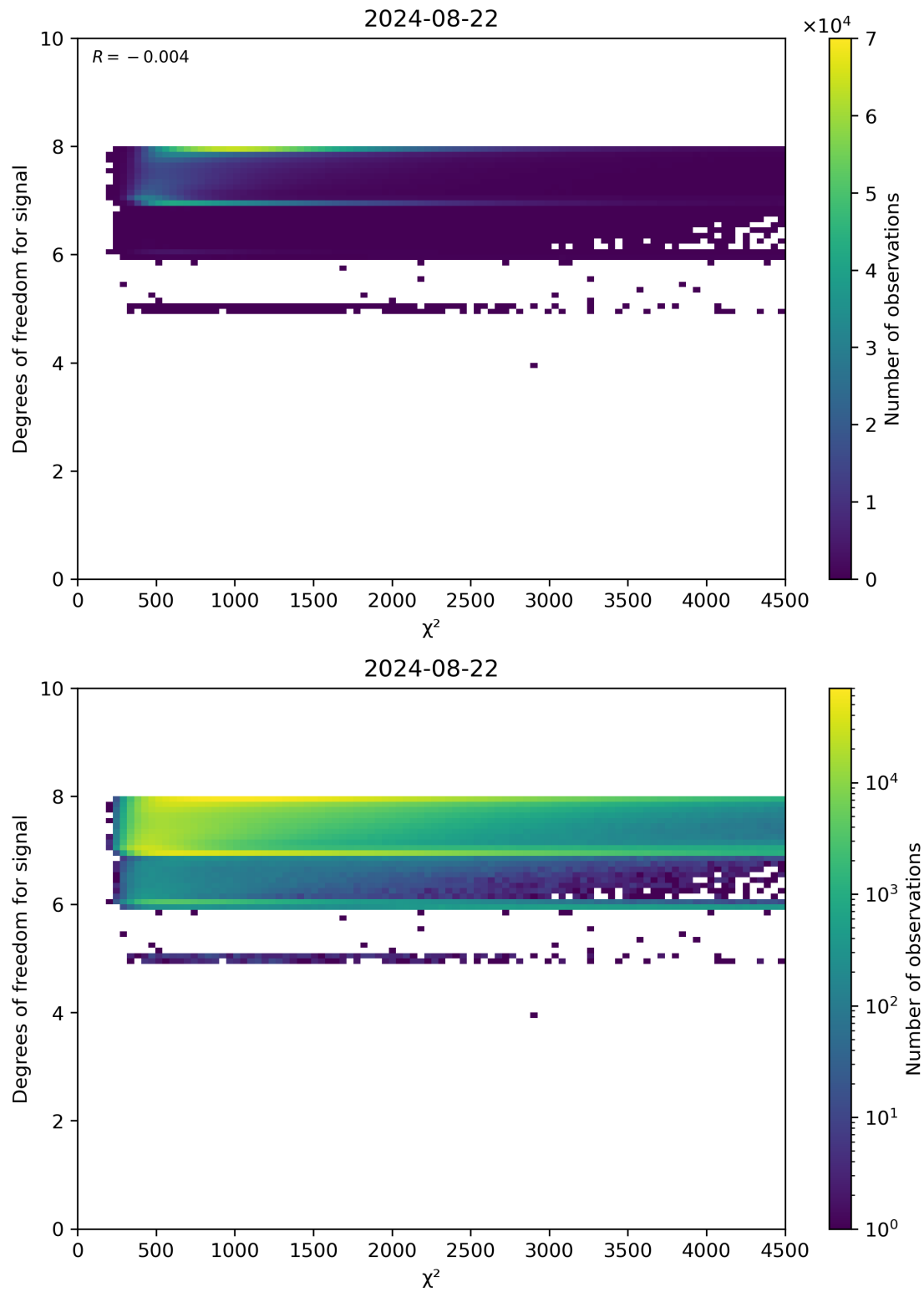
Figure 48: Scatter density plot of “ \chi^2 ” against “Degrees of freedom for signal” for 2024-08-22 to 2024-08-23.
