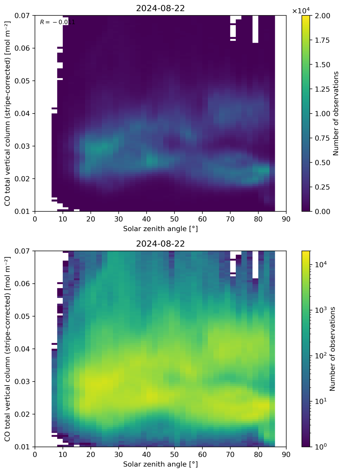
Figure 62: Scatter density plot of “Solar zenith angle” against “CO total vertical column (stripe-corrected)” for 2024-08-22 to 2024-08-23.
