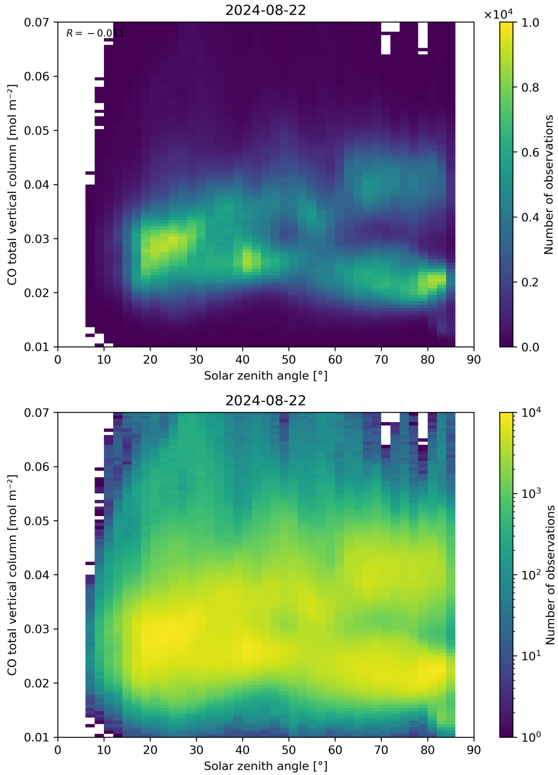
Figure 61: Scatter density plot of “Solar zenith angle” against “CO total vertical column” for 2024-08-22 to 2024-08-23.
