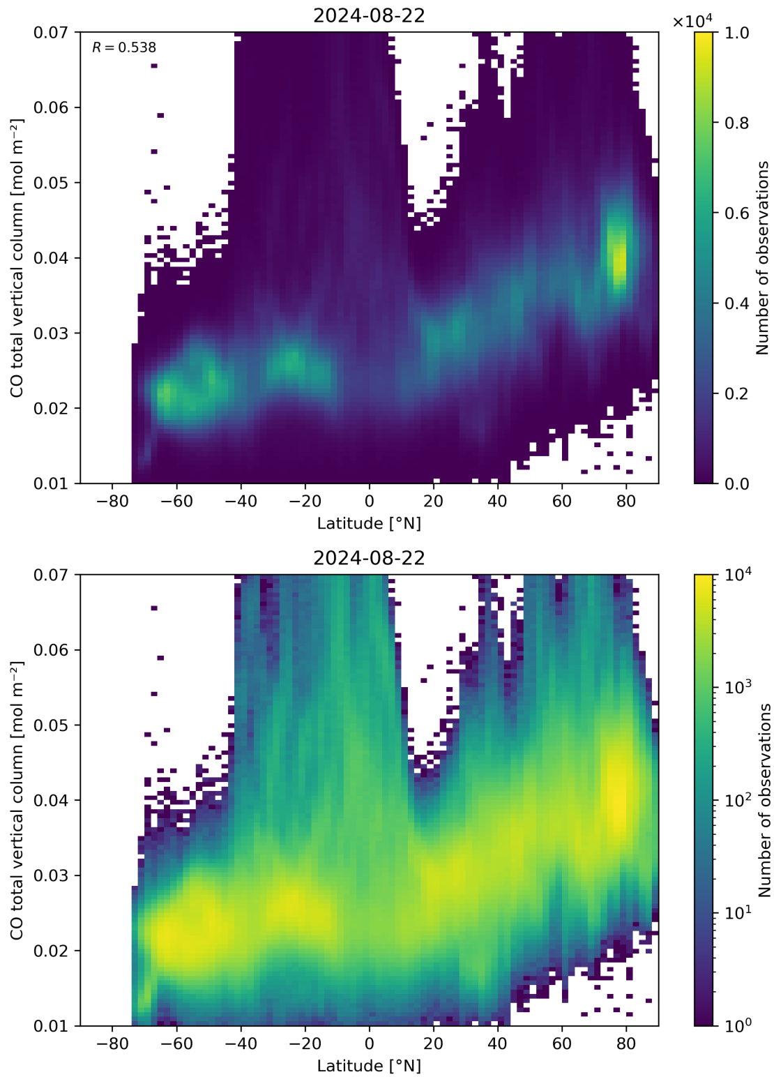
Figure 51: Scatter density plot of “Latitude” against “CO total vertical column” for 2024-08-22 to 2024-08-23.
