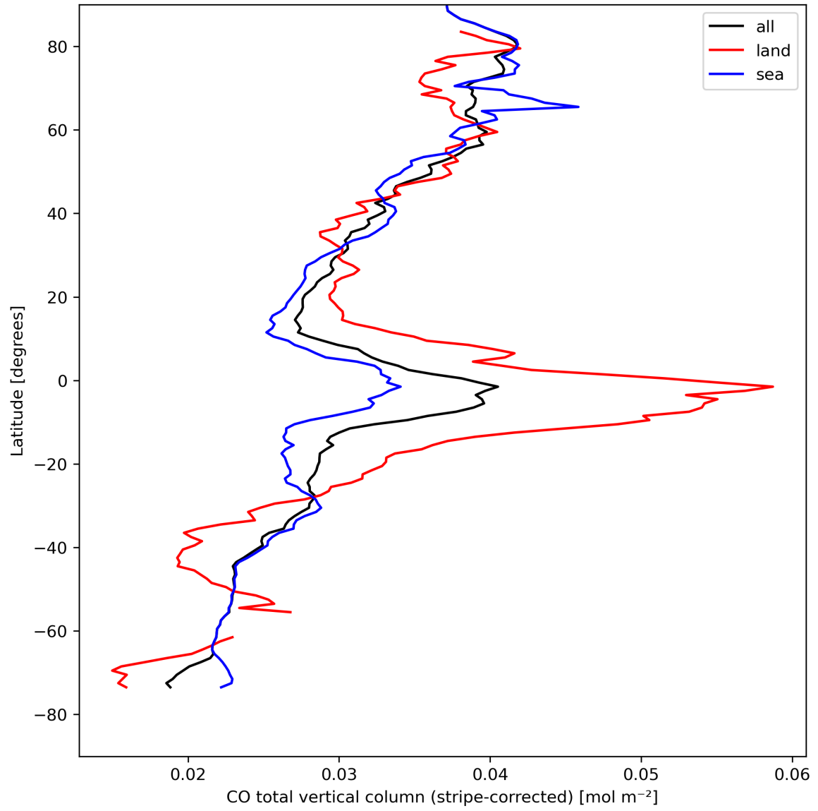
Figure 11: Zonal average of “CO total vertical column (stripe-corrected)” for 2024-08-22 to 2024-08-23.
