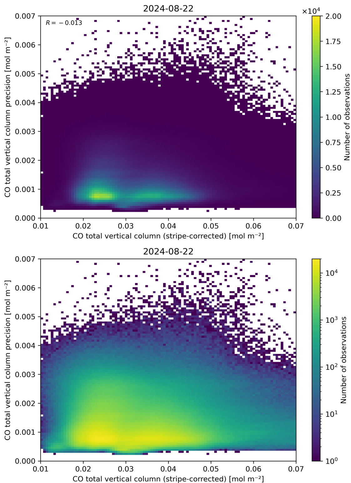
Figure 36: Scatter density plot of “CO total vertical column (stripe-corrected)” against “CO total vertical column precision” for 2024-08-22 to 2024-08-23.
