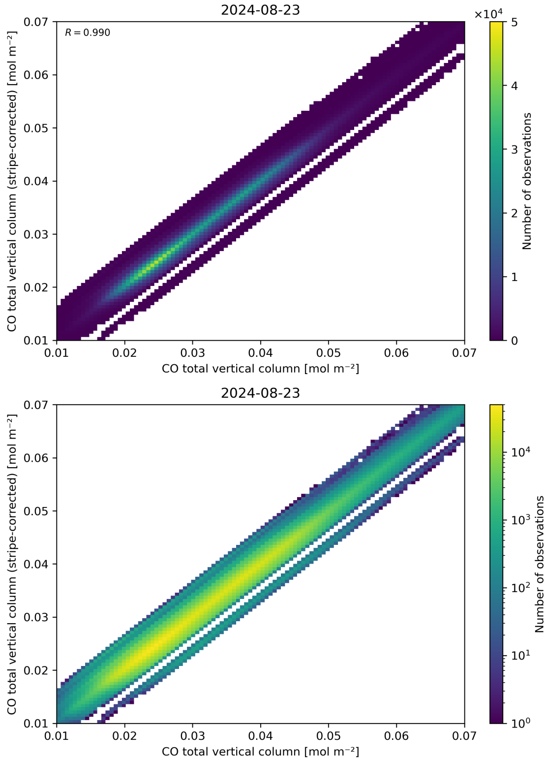
Figure 33: Scatter density plot of “CO total vertical column” against “CO total vertical column (stripe-corrected)” for 2024-08-22 to 2024-08-24.
