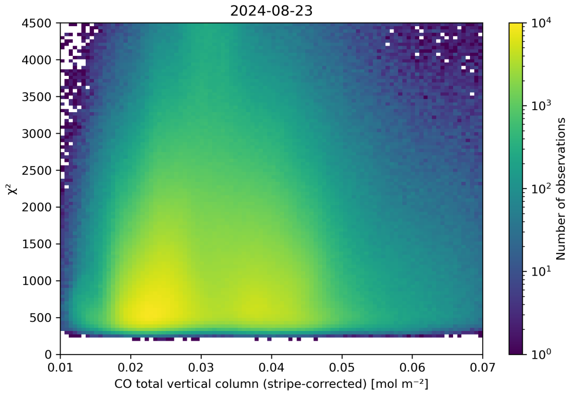
Figure 37: Scatter density plot of “CO total vertical column (stripe-corrected)” against “ \chi^2 ” for 2024-08-22 to 2024-08-24.
