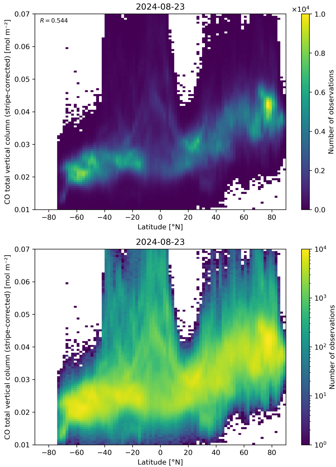
Figure 52: Scatter density plot of “Latitude” against “CO total vertical column (stripe-corrected)” for 2024-08-22 to 2024-08-24.
