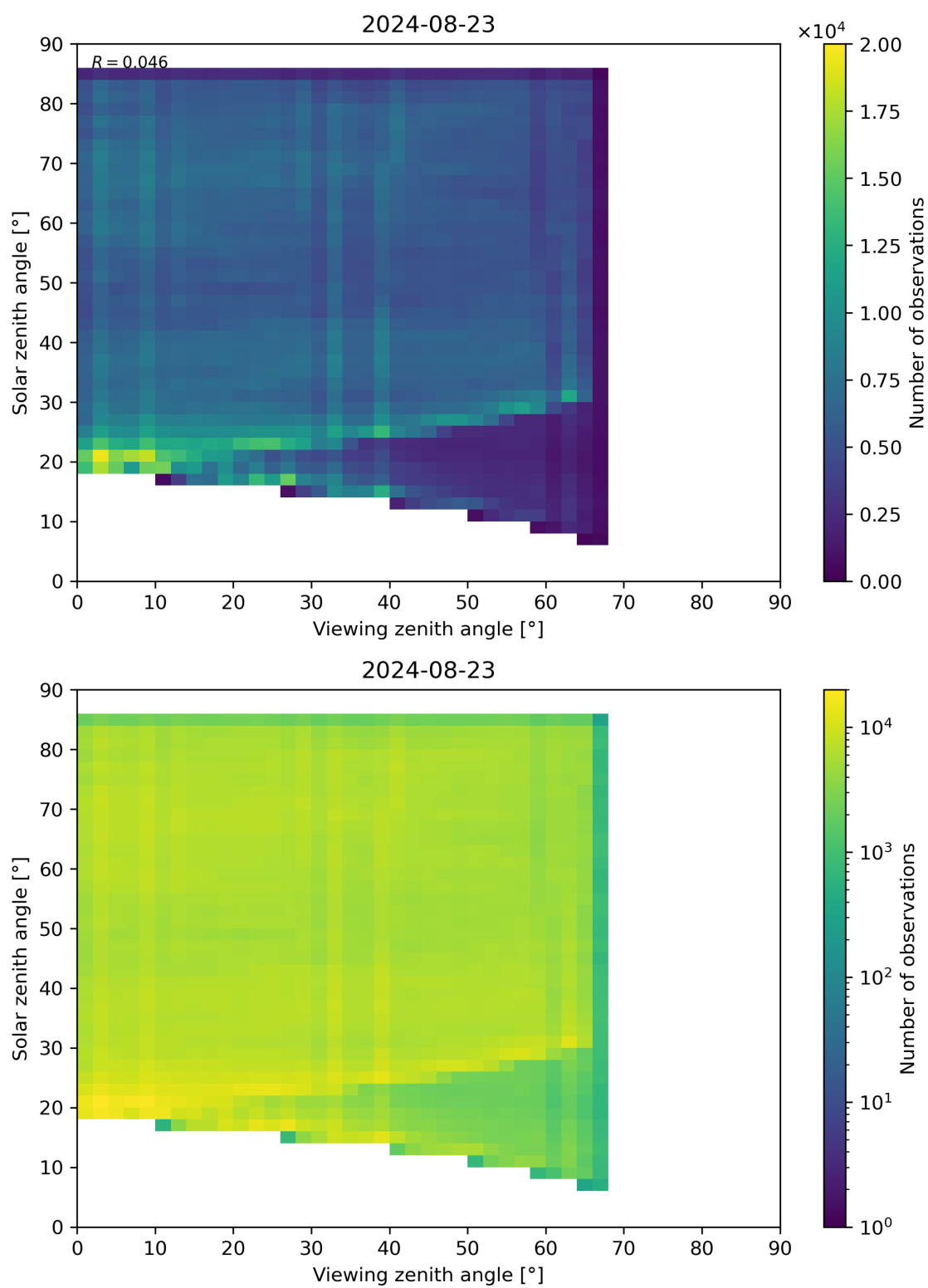
Figure 77: Scatter density plot of “Viewing zenith angle” against “Solar zenith angle” for 2024-08-22 to 2024-08-24.
