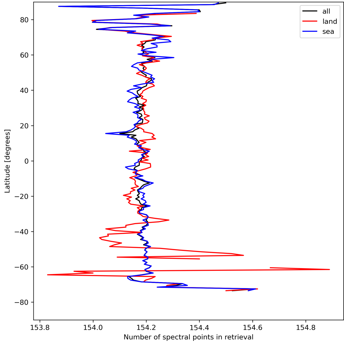
Figure 13: Zonal average of “Number of spectral points in retrieval” for 2024-08-22 to 2024-08-24.
