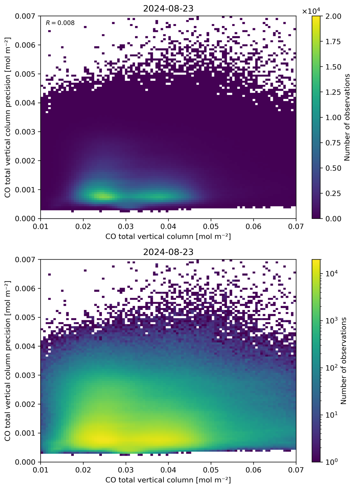
Figure 34: Scatter density plot of “CO total vertical column” against “CO total vertical column precision” for 2024-08-22 to 2024-08-24.
