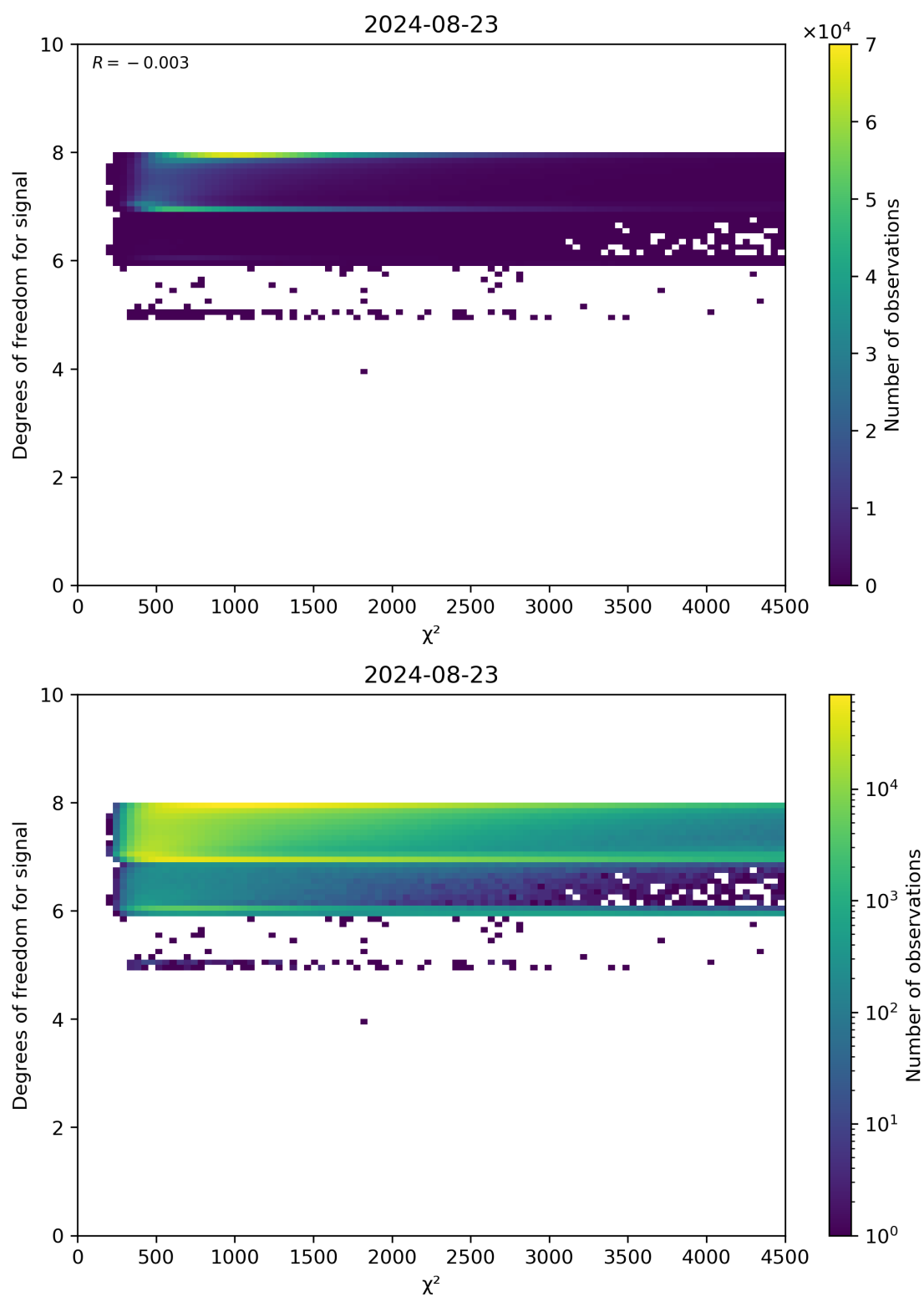
Figure 48: Scatter density plot of “ \chi^2 ” against “Degrees of freedom for signal” for 2024-08-22 to 2024-08-24.
