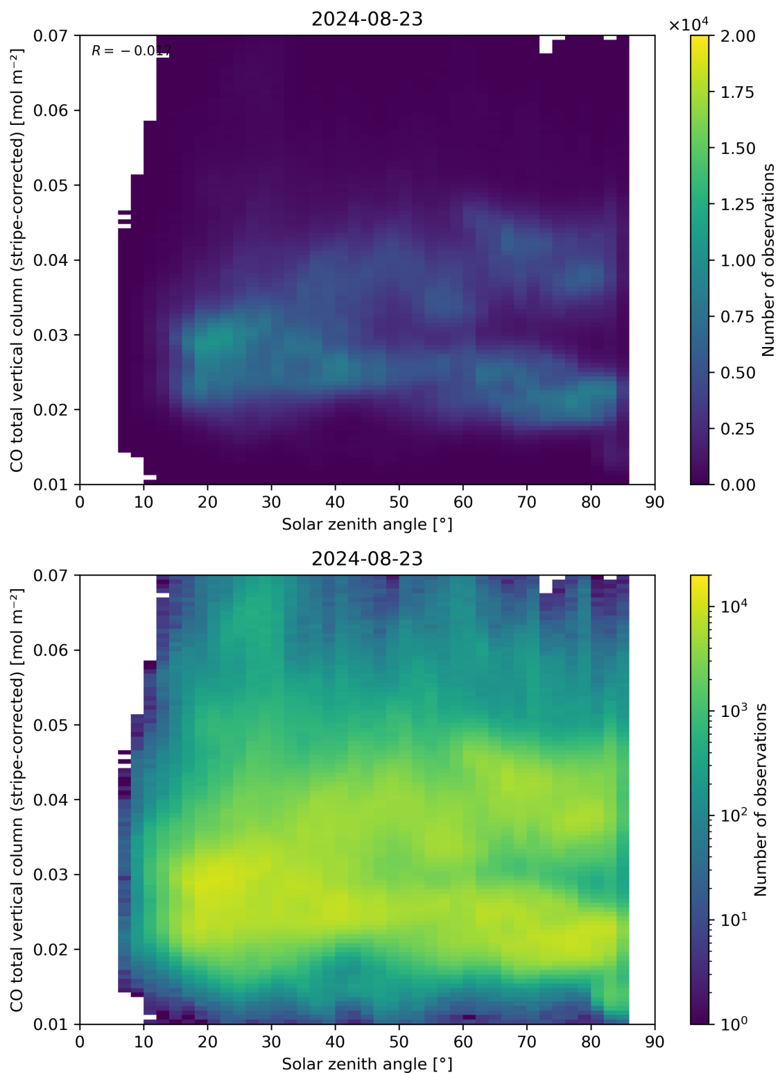
Figure 62: Scatter density plot of “Solar zenith angle” against “CO total vertical column (stripe-corrected)” for 2024-08-22 to 2024-08-24.
