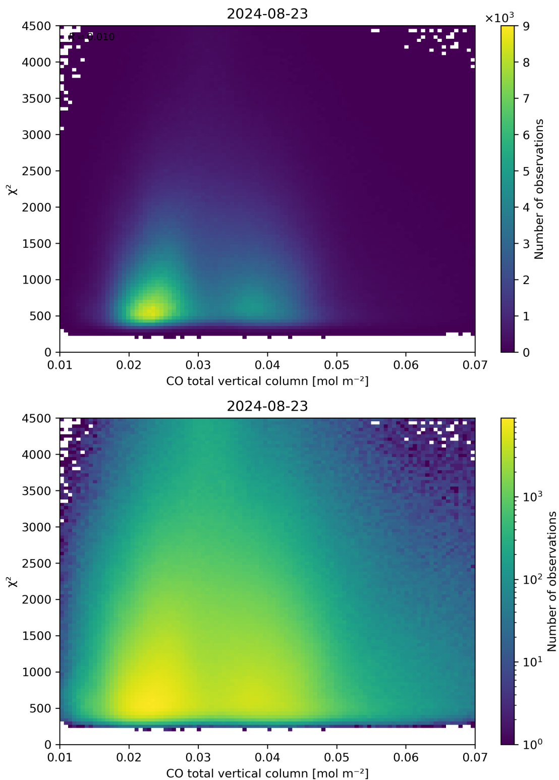
Figure 35: Scatter density plot of “CO total vertical column” against “ \chi^2 ” for 2024-08-22 to 2024-08-24.
