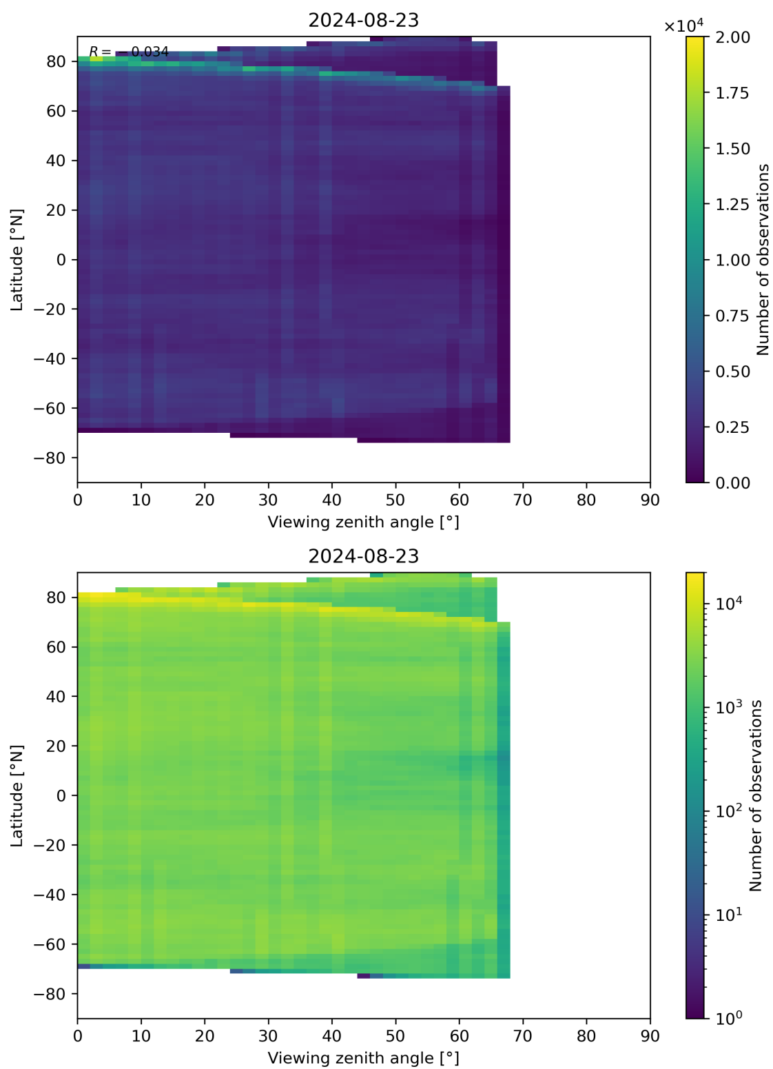
Figure 74: Scatter density plot of “Viewing zenith angle” against “Latitude” for 2024-08-22 to 2024-08-24.
