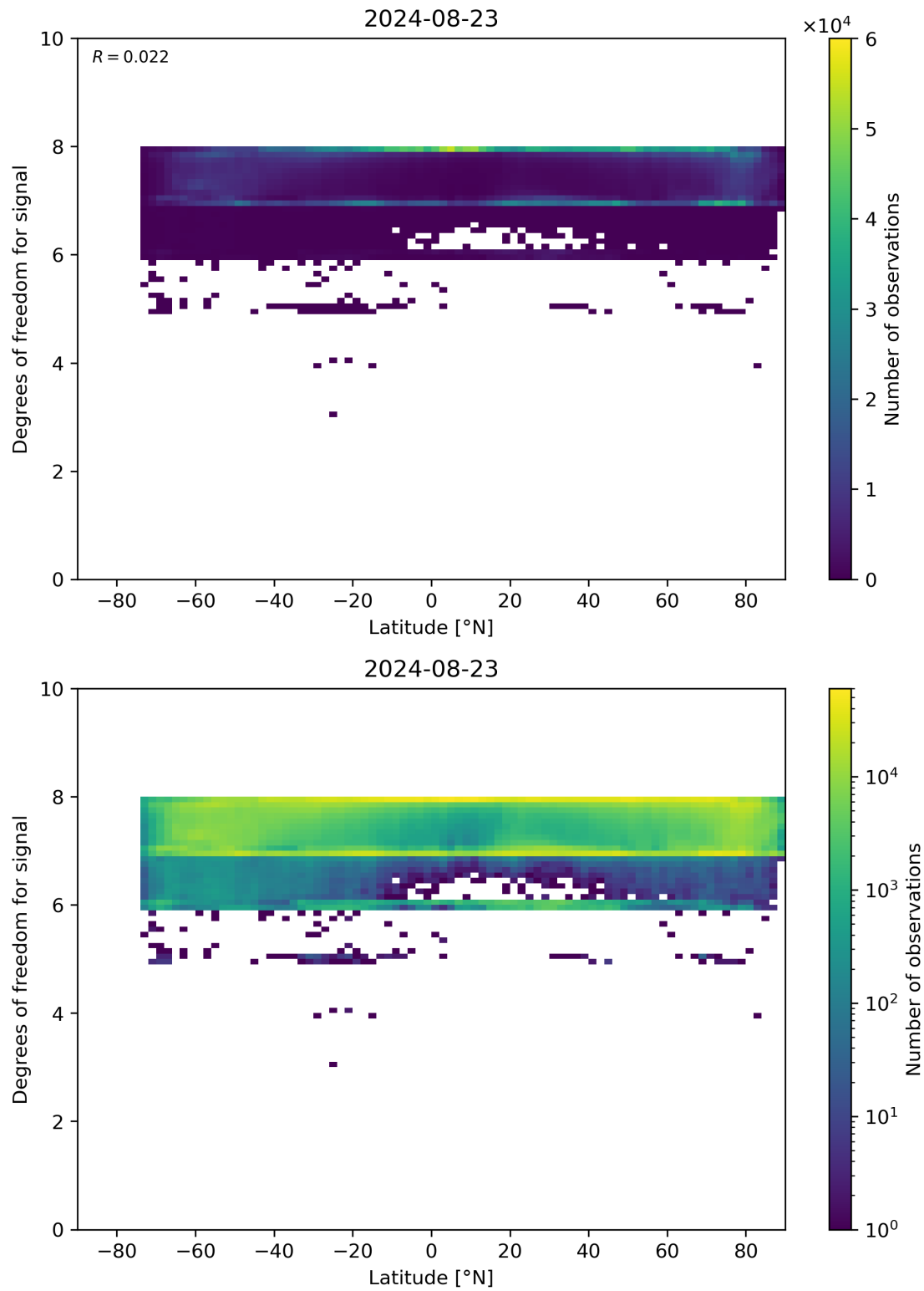
Figure 55: Scatter density plot of “Latitude” against “Degrees of freedom for signal” for 2024-08-22 to 2024-08-24.
