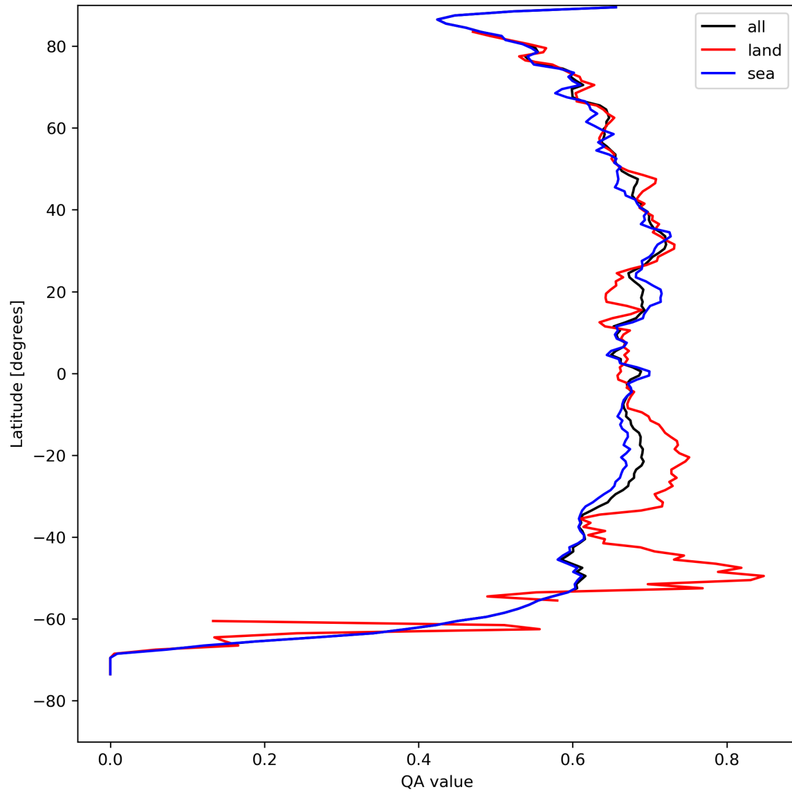
Figure 9: Zonal average of “QA value” for 2024-08-22 to 2024-08-24.
