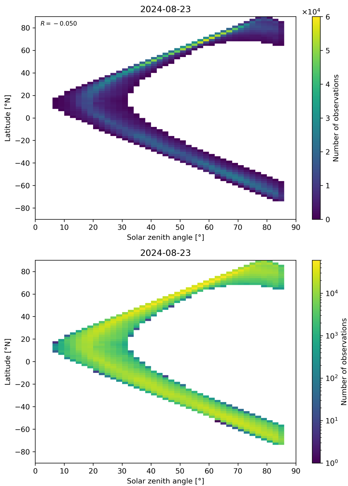
Figure 66: Scatter density plot of “Solar zenith angle” against “Latitude” for 2024-08-22 to 2024-08-24.
