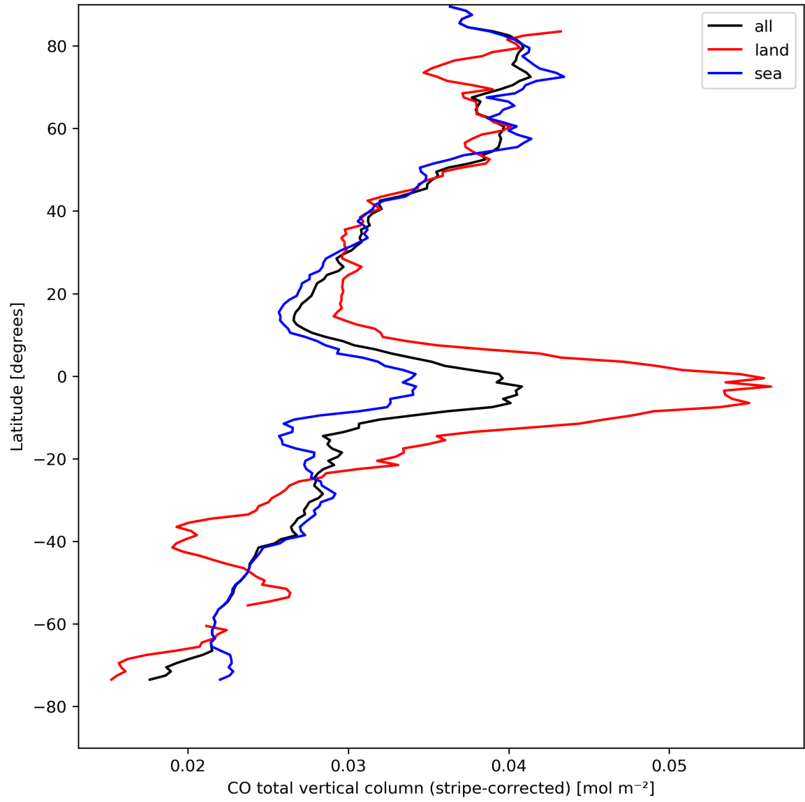
Figure 11: Zonal average of “CO total vertical column (stripe-corrected)” for 2024-08-22 to 2024-08-24.
