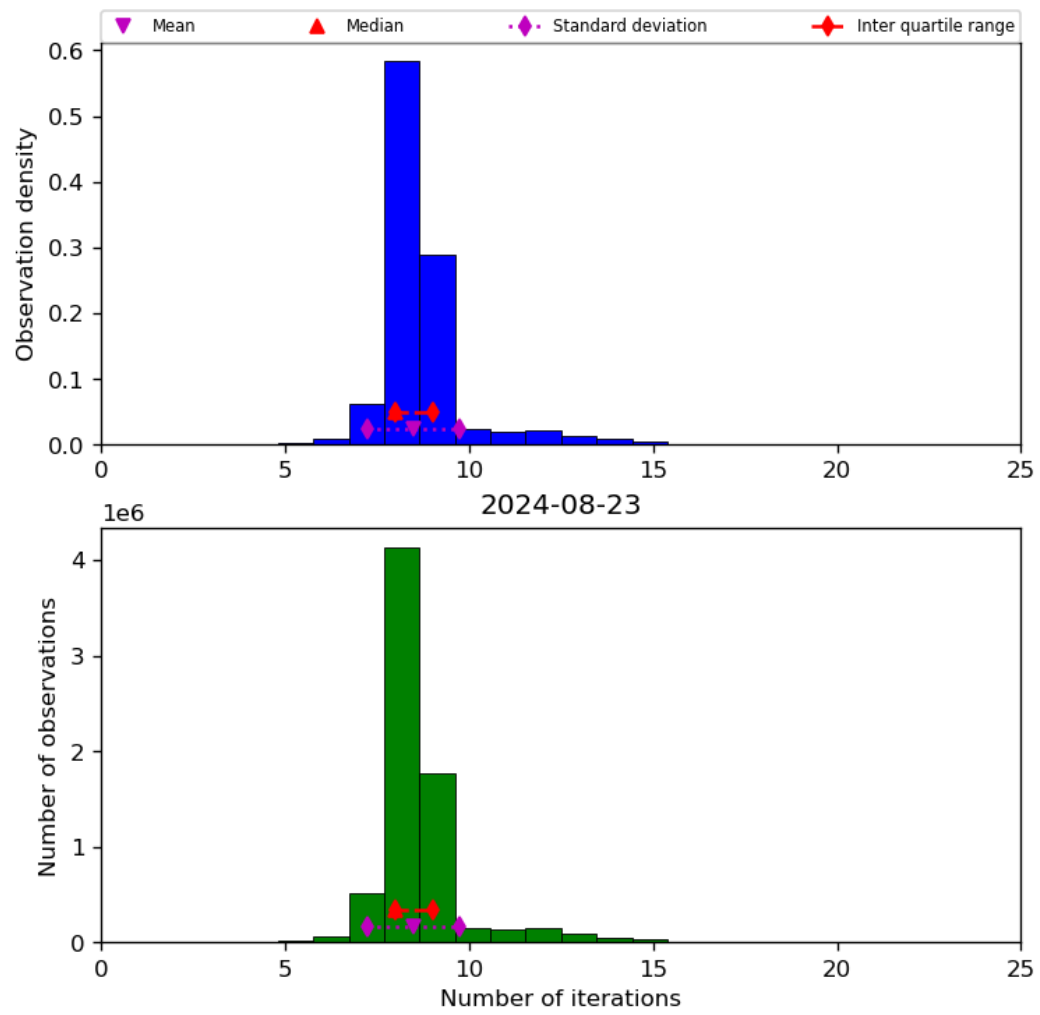
Figure 24: Histogram of “Number of iterations” for 2024-08-22 to 2024-08-24
