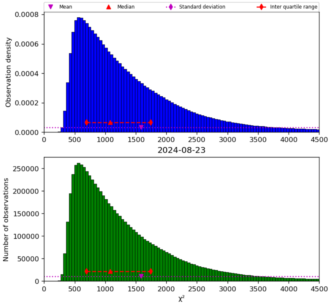
Figure 22: Histogram of “ \chi^2 ” for 2024-08-22 to 2024-08-24
