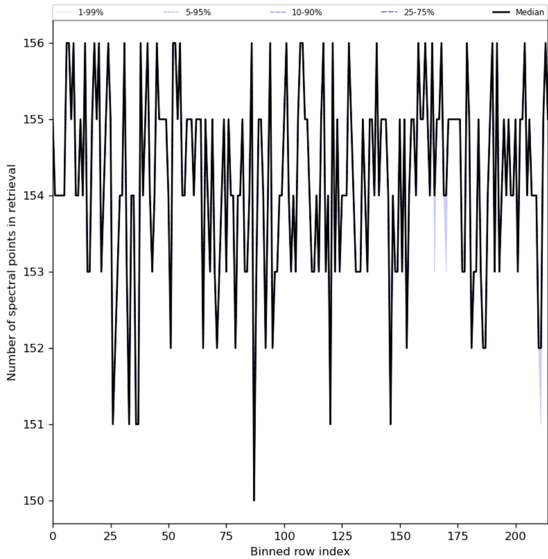
Figure 29: Along track statistics of “Number of spectral points in retrieval” for 2024-08-22 to 2024-08-24
