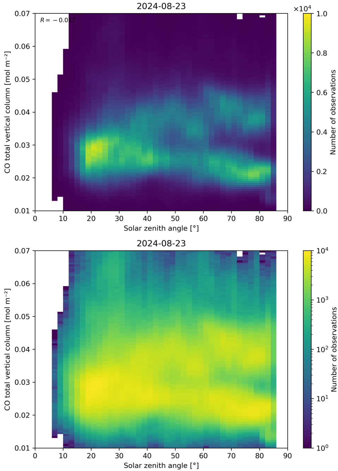
Figure 61: Scatter density plot of “Solar zenith angle” against “CO total vertical column” for 2024-08-22 to 2024-08-24.
