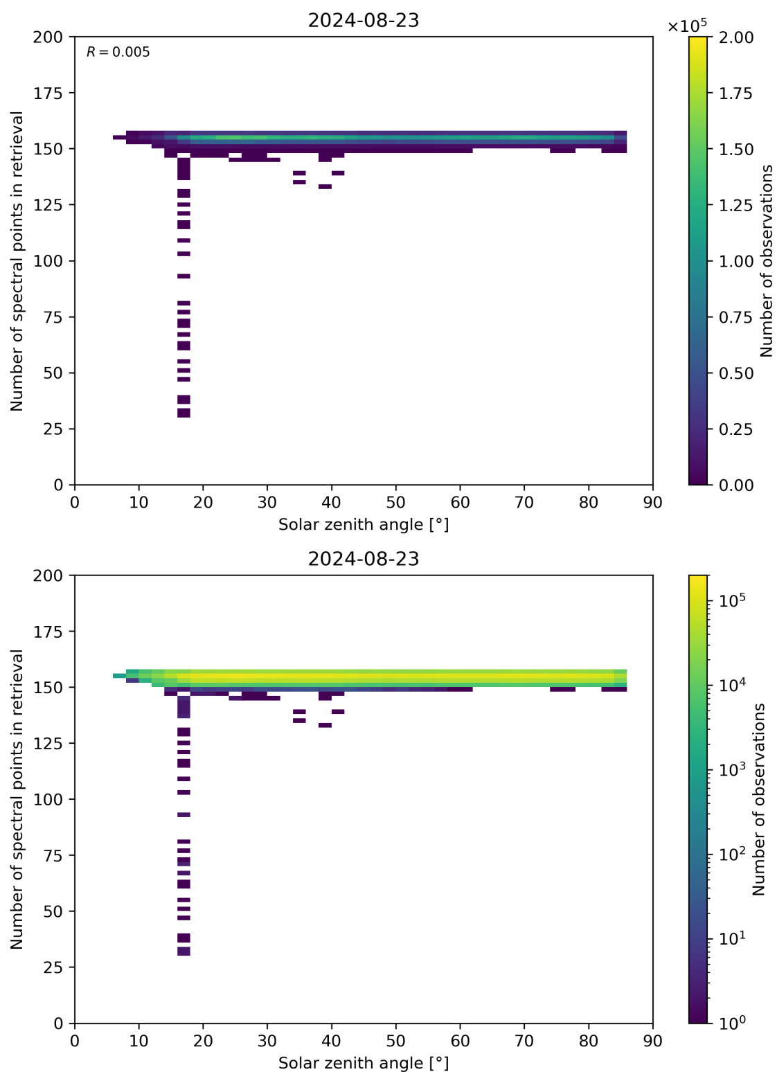
Figure 68: Scatter density plot of “Solar zenith angle” against “Number of spectral points in retrieval” for 2024-08-22 to 2024-08-24.
