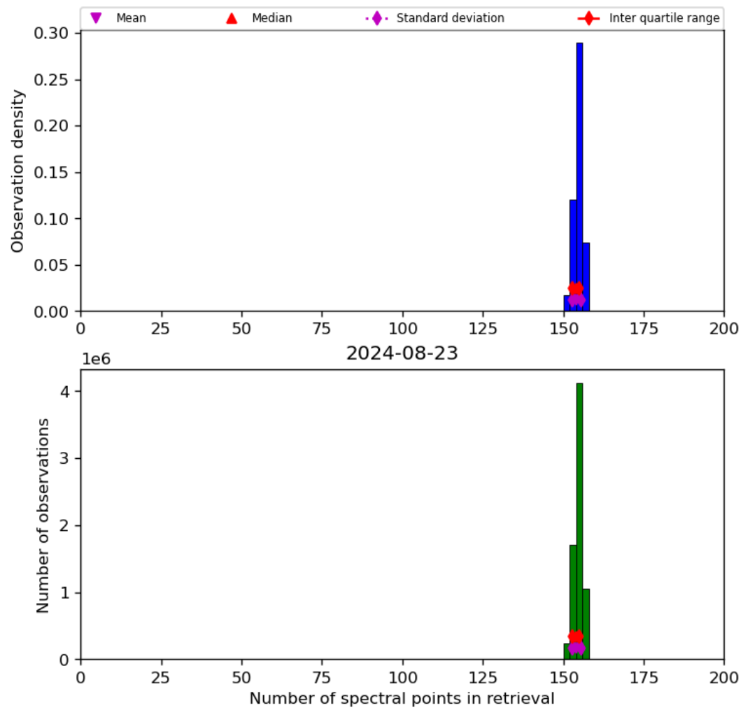
Figure 21: Histogram of “Number of spectral points in retrieval” for 2024-08-22 to 2024-08-24
