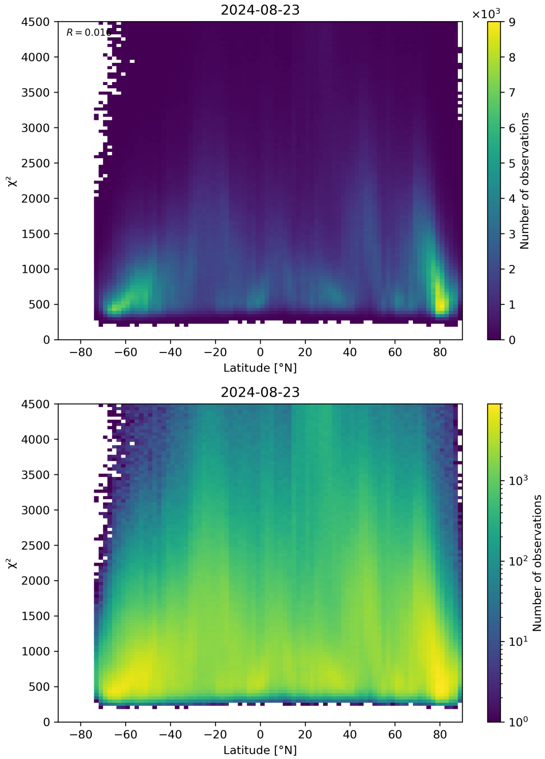
Figure 54: Scatter density plot of “Latitude” against “ \chi^2 ” for 2024-08-22 to 2024-08-24.
