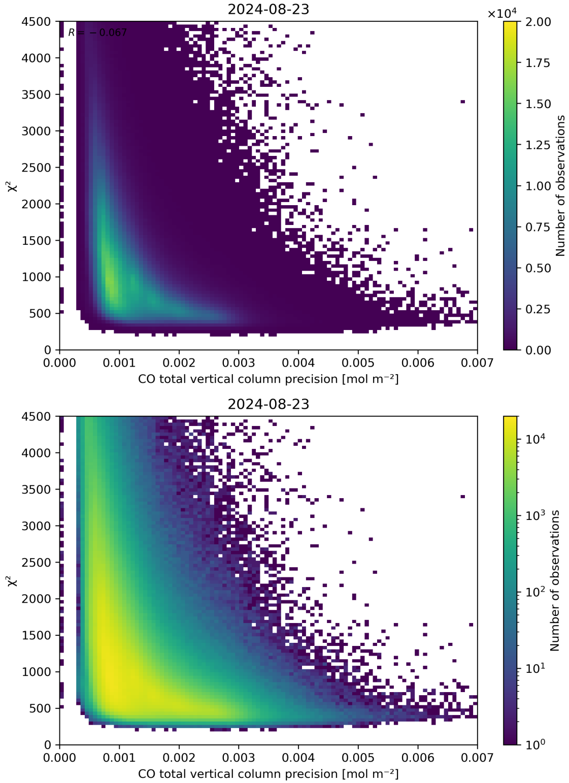
Figure 44: Scatter density plot of “CO total vertical column precision” against “ \chi^2 ” for 2024-08-22 to 2024-08-24.
