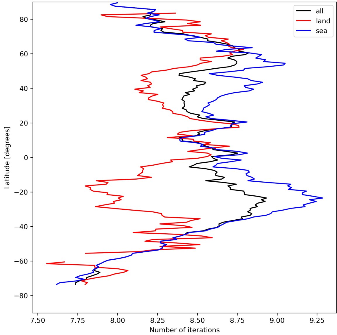
Figure 16: Zonal average of “Number of iterations” for 2024-08-22 to 2024-08-24.
