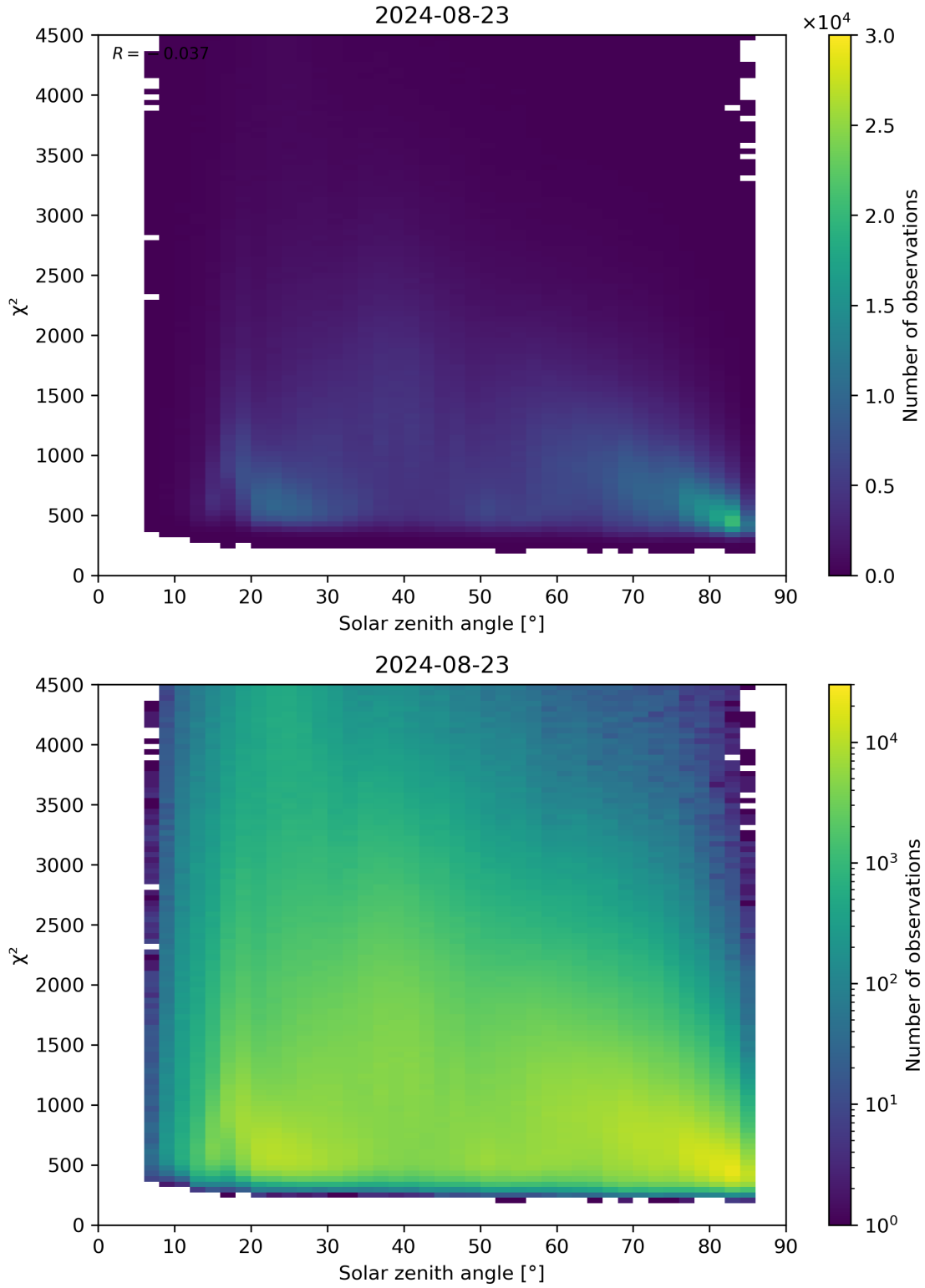
Figure 64: Scatter density plot of “Solar zenith angle” against “ \chi^2 ” for 2024-08-22 to 2024-08-24.
