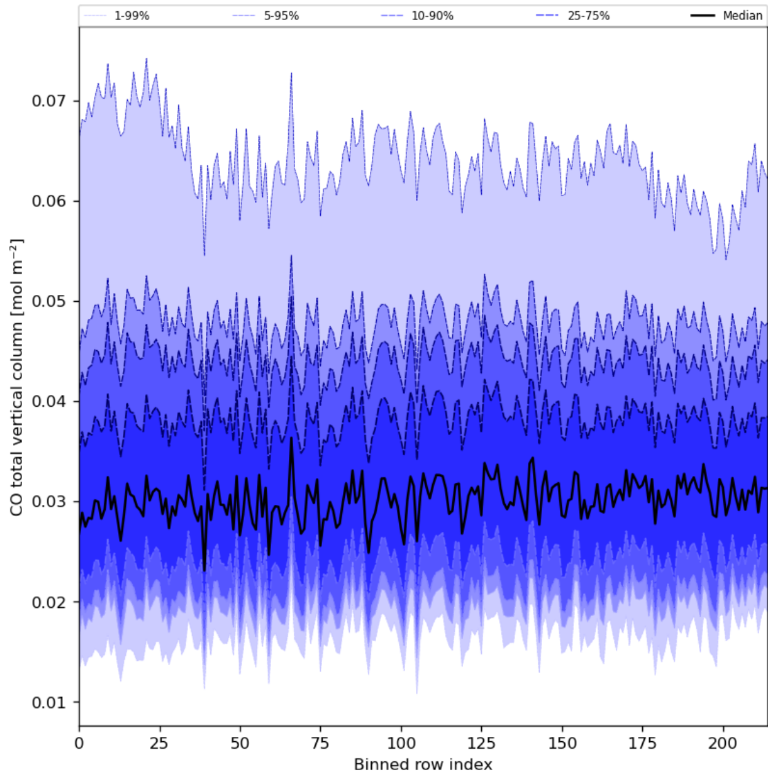
Figure 26: Along track statistics of “CO total vertical column” for 2024-08-22 to 2024-08-24
