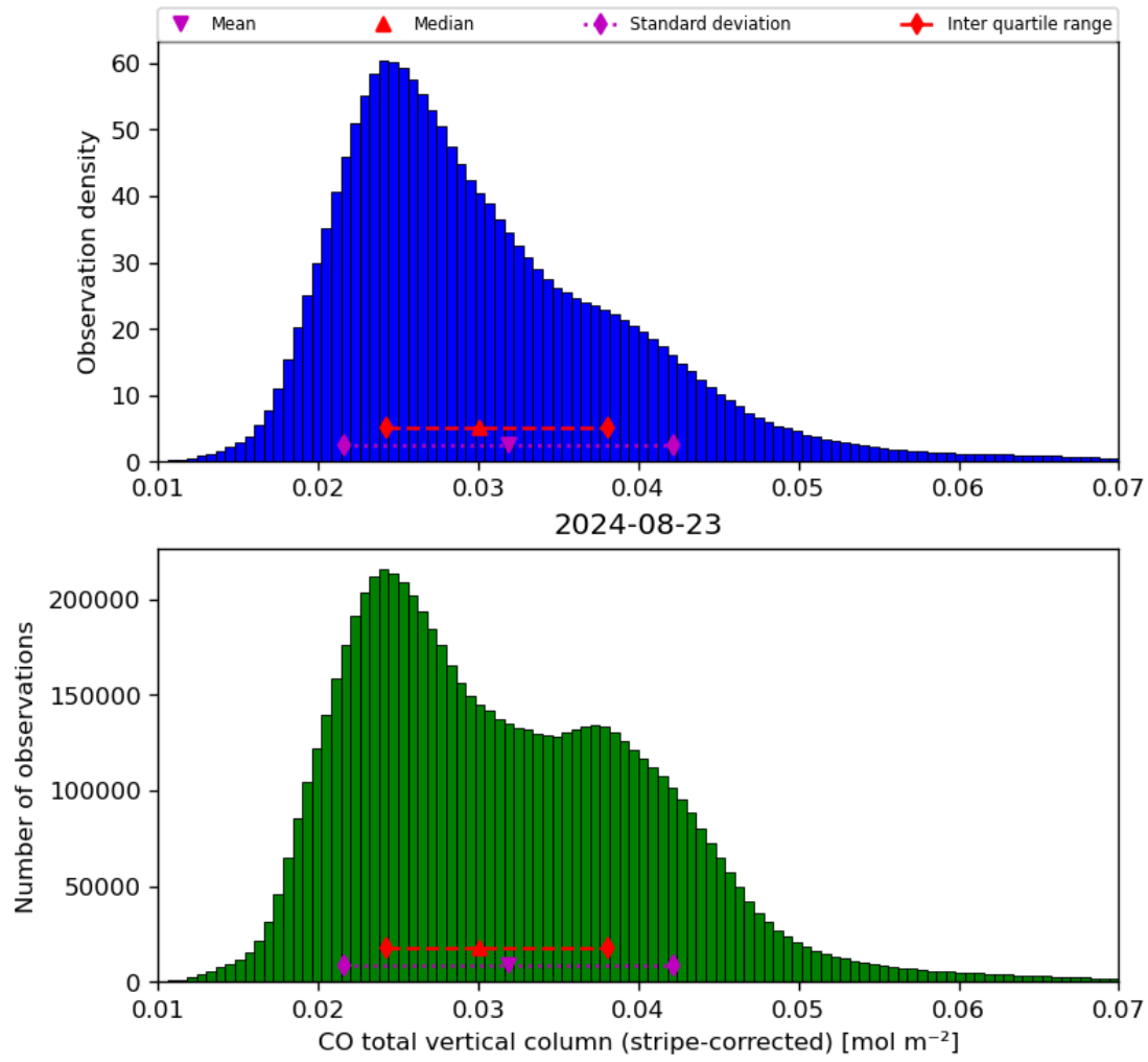
Figure 19: Histogram of “CO total vertical column (stripe-corrected)” for 2024-08-22 to 2024-08-24
