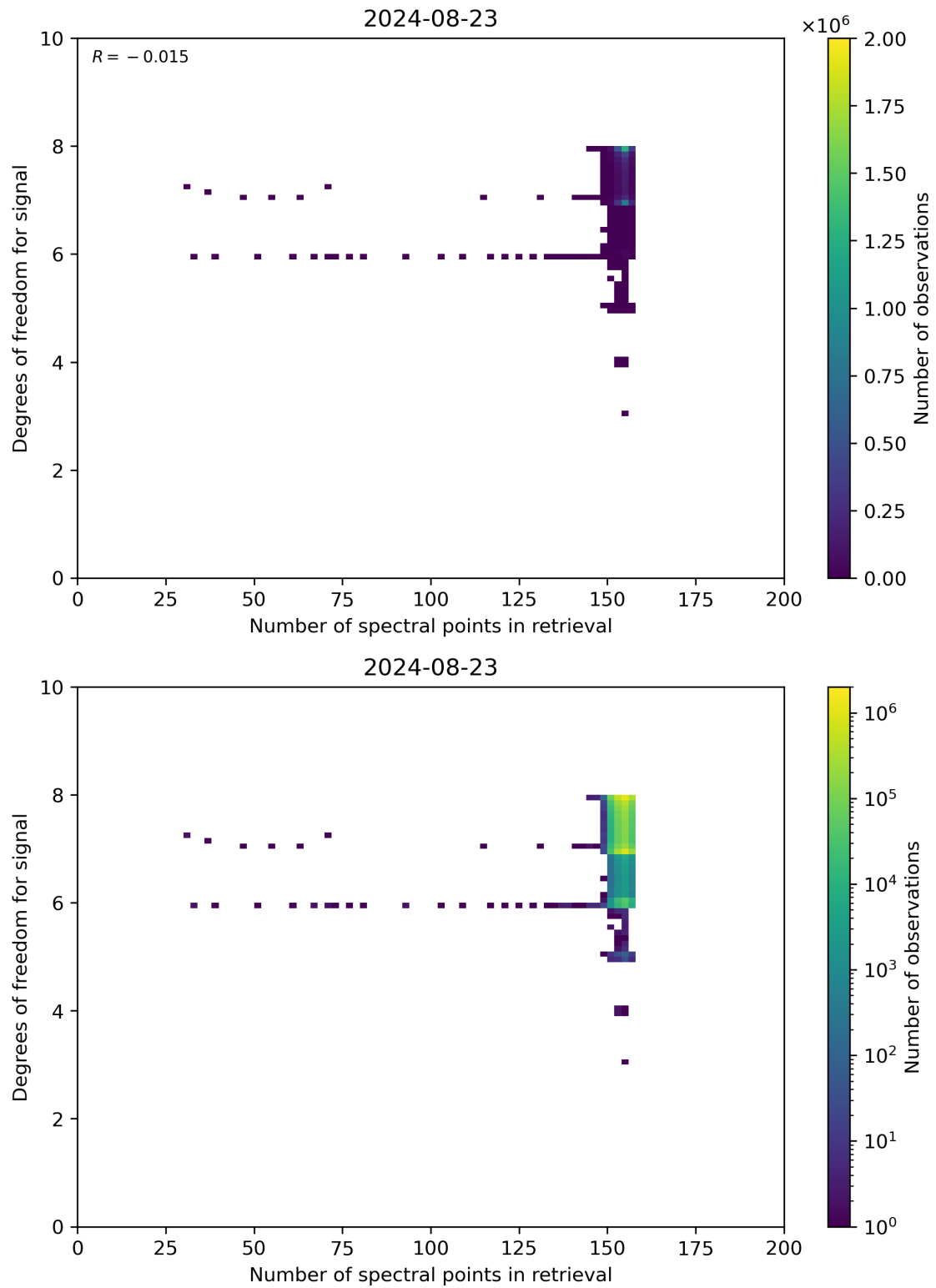
Figure 59: Scatter density plot of “Number of spectral points in retrieval” against “Degrees of freedom for signal” for 2024-08-22 to 2024-08-24.
