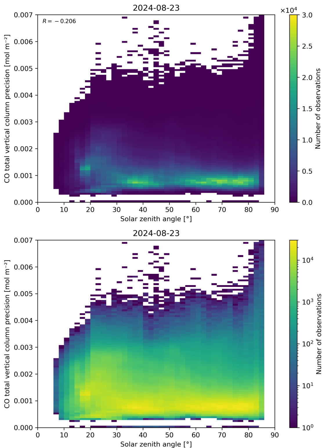
Figure 63: Scatter density plot of “Solar zenith angle” against “CO total vertical column precision” for 2024-08-22 to 2024-08-24.
