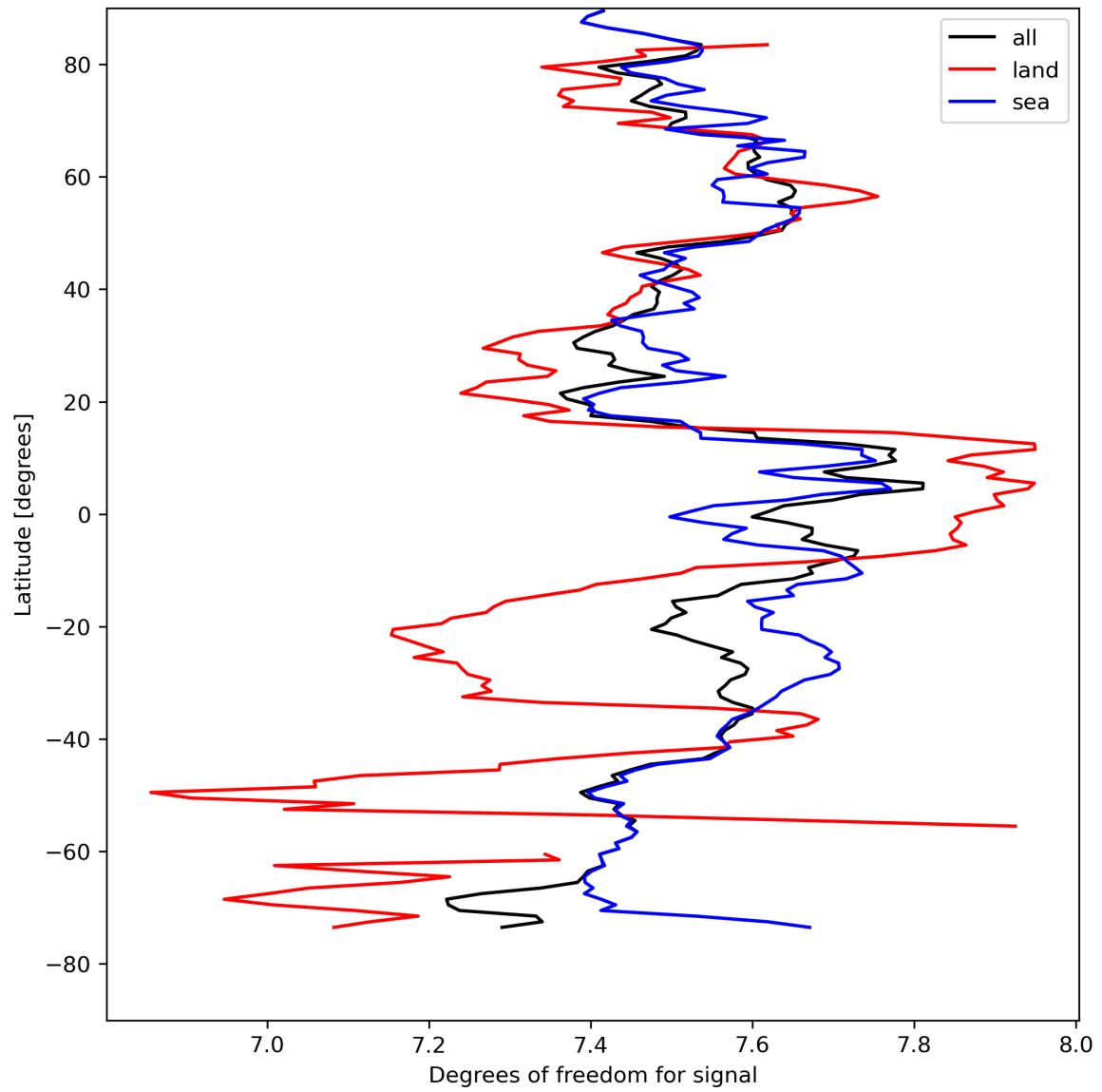
Figure 15: Zonal average of “Degrees of freedom for signal” for 2024-08-22 to 2024-08-24.
