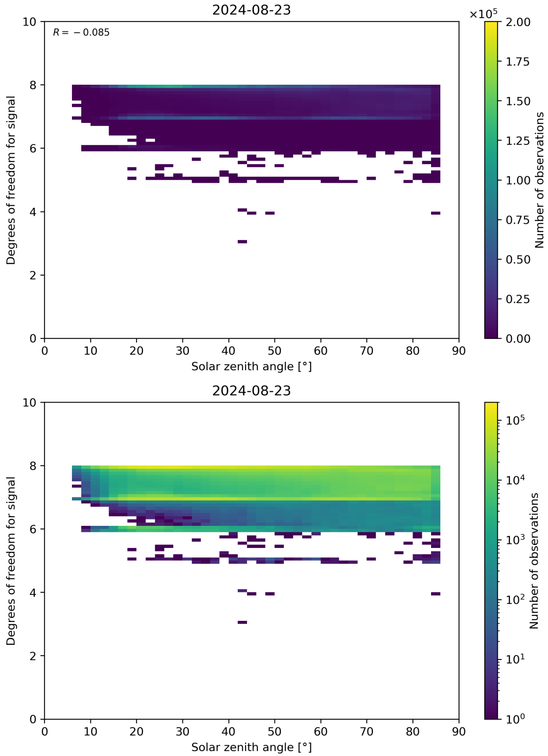
Figure 65: Scatter density plot of “Solar zenith angle” against “Degrees of freedom for signal” for 2024-08-22 to 2024-08-24.
