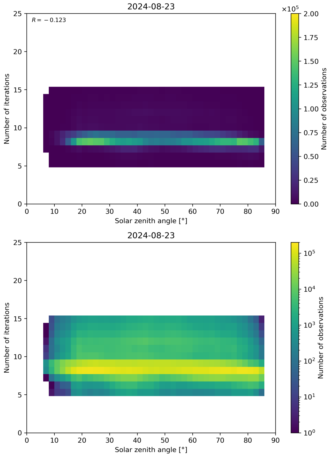
Figure 67: Scatter density plot of “Solar zenith angle” against “Number of iterations” for 2024-08-22 to 2024-08-24.
