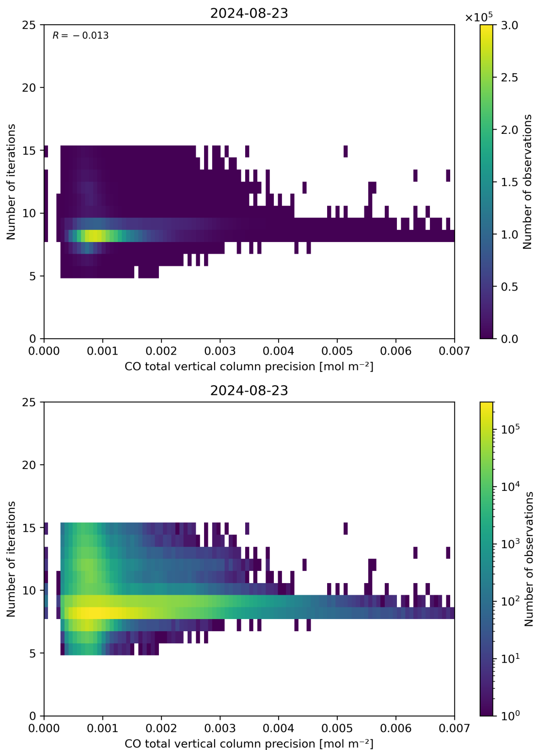
Figure 46: Scatter density plot of “CO total vertical column precision” against “Number of iterations” for 2024-08-22 to 2024-08-24.
