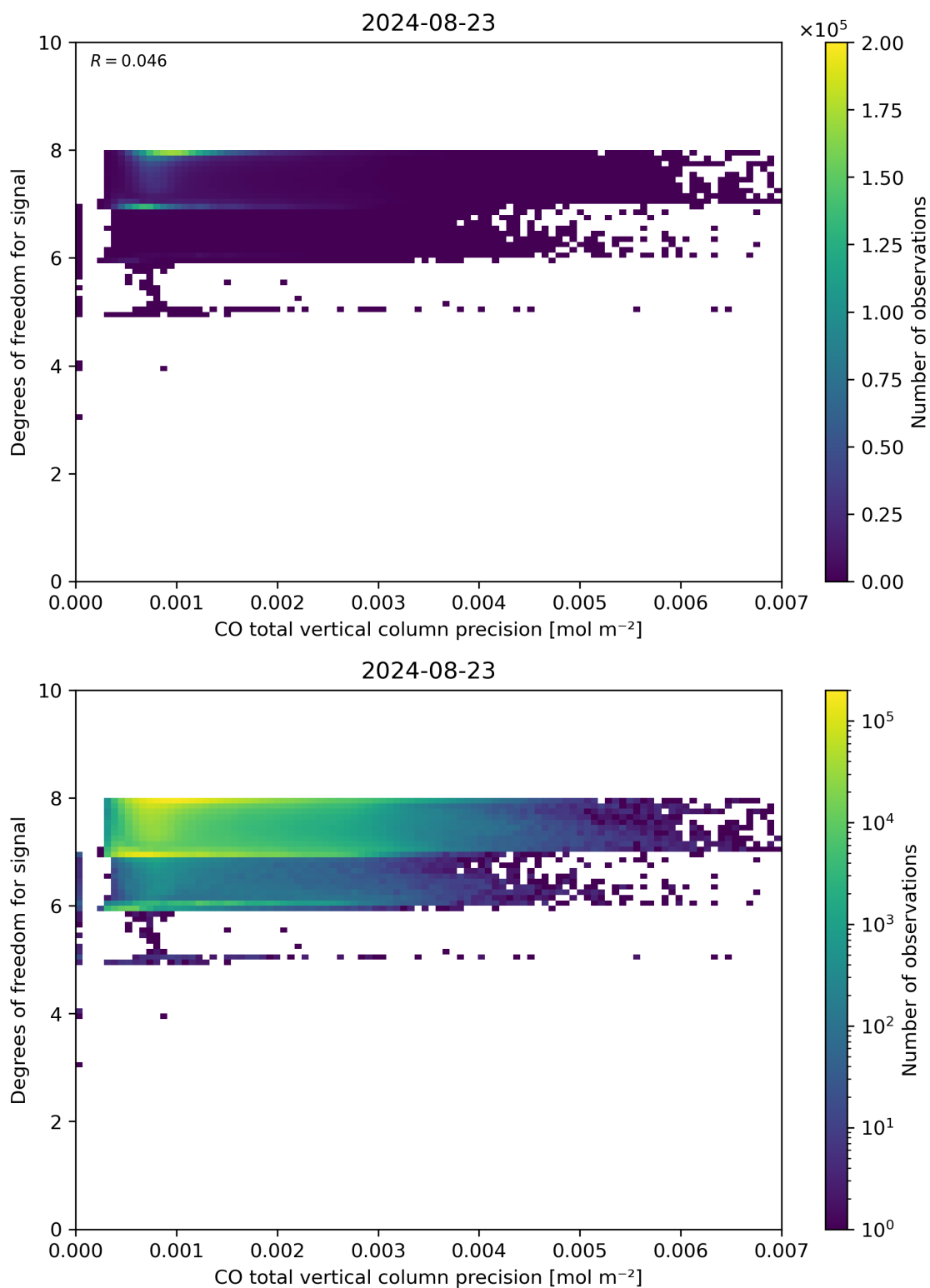
Figure 45: Scatter density plot of “CO total vertical column precision” against “Degrees of freedom for signal” for 2024-08-22 to 2024-08-24.
