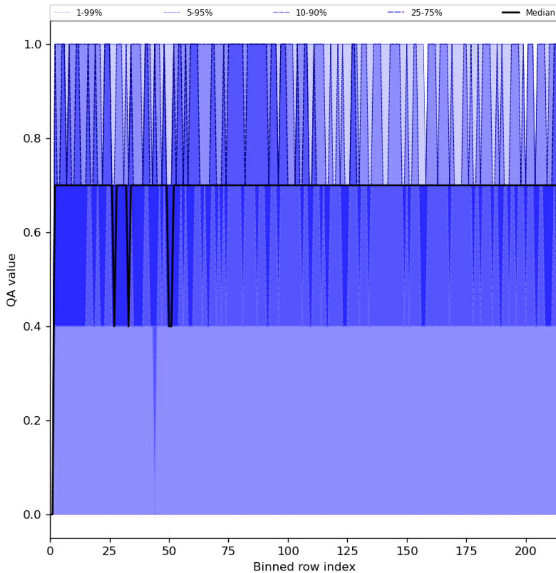
Figure 25: Along track statistics of “QA value” for 2024-08-22 to 2024-08-24
