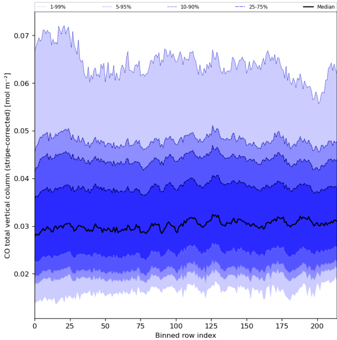
Figure 27: Along track statistics of “CO total vertical column (stripe-corrected)” for 2024-08-22 to 2024-08-24
