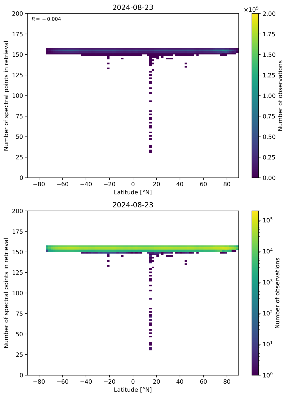
Figure 57: Scatter density plot of “Latitude” against “Number of spectral points in retrieval” for 2024-08-22 to 2024-08-24.
