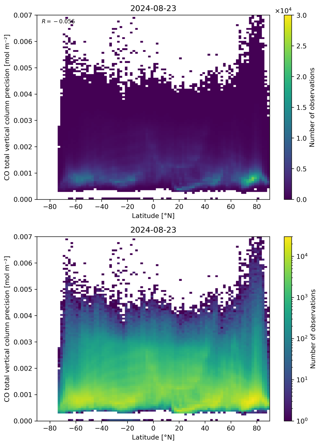
Figure 53: Scatter density plot of “Latitude” against “CO total vertical column precision” for 2024-08-22 to 2024-08-24.
