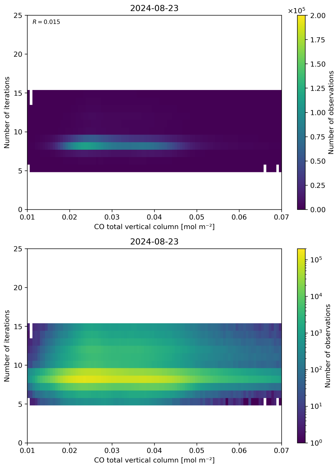
Figure 42: Scatter density plot of “CO total vertical column” against “Number of iterations” for 2024-08-22 to 2024-08-24.
