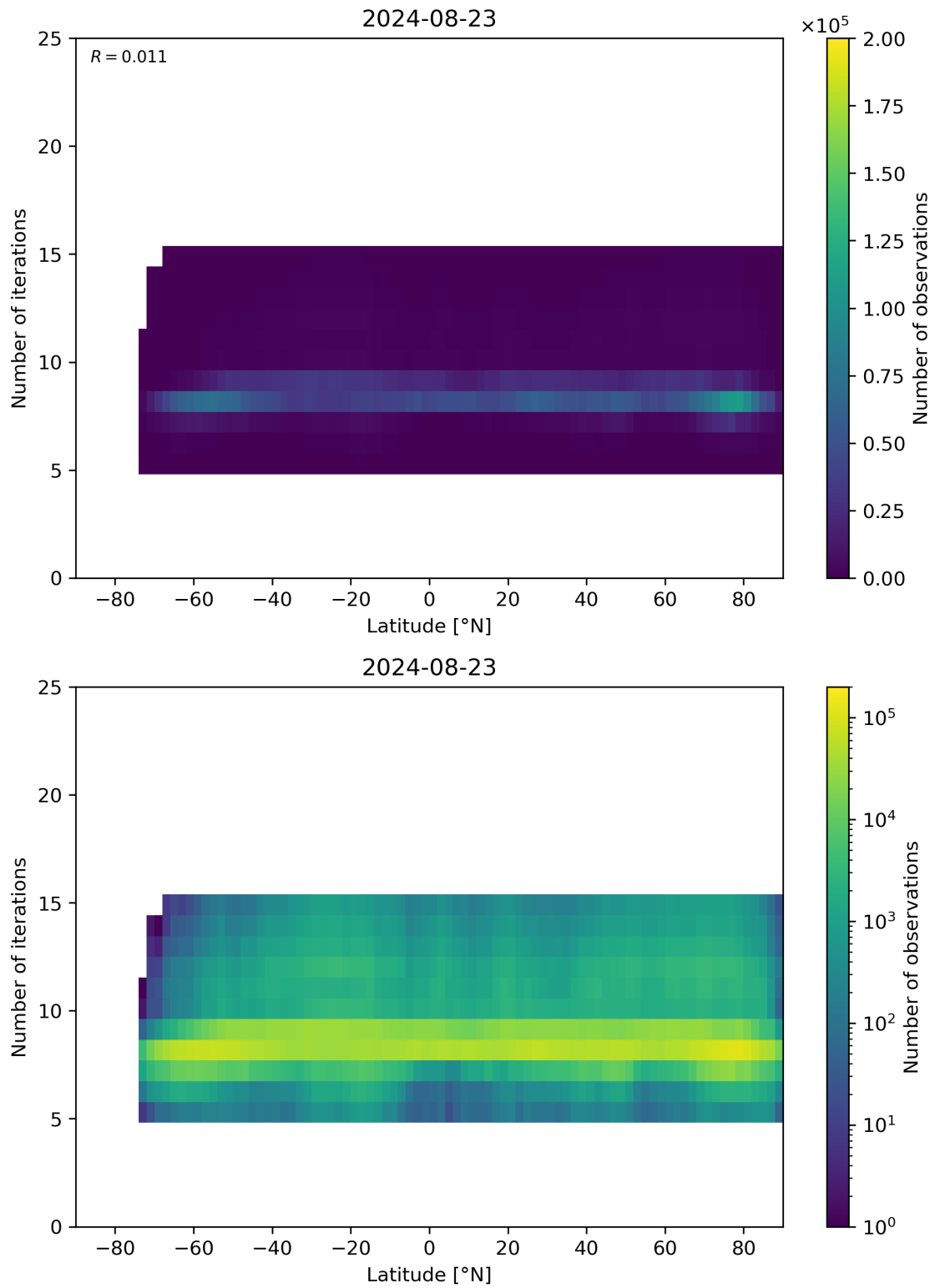
Figure 56: Scatter density plot of “Latitude” against “Number of iterations” for 2024-08-22 to 2024-08-24.
