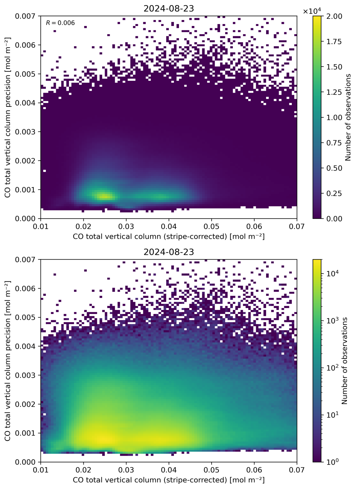
Figure 36: Scatter density plot of “CO total vertical column (stripe-corrected)” against “CO total vertical column precision” for 2024-08-22 to 2024-08-24.
