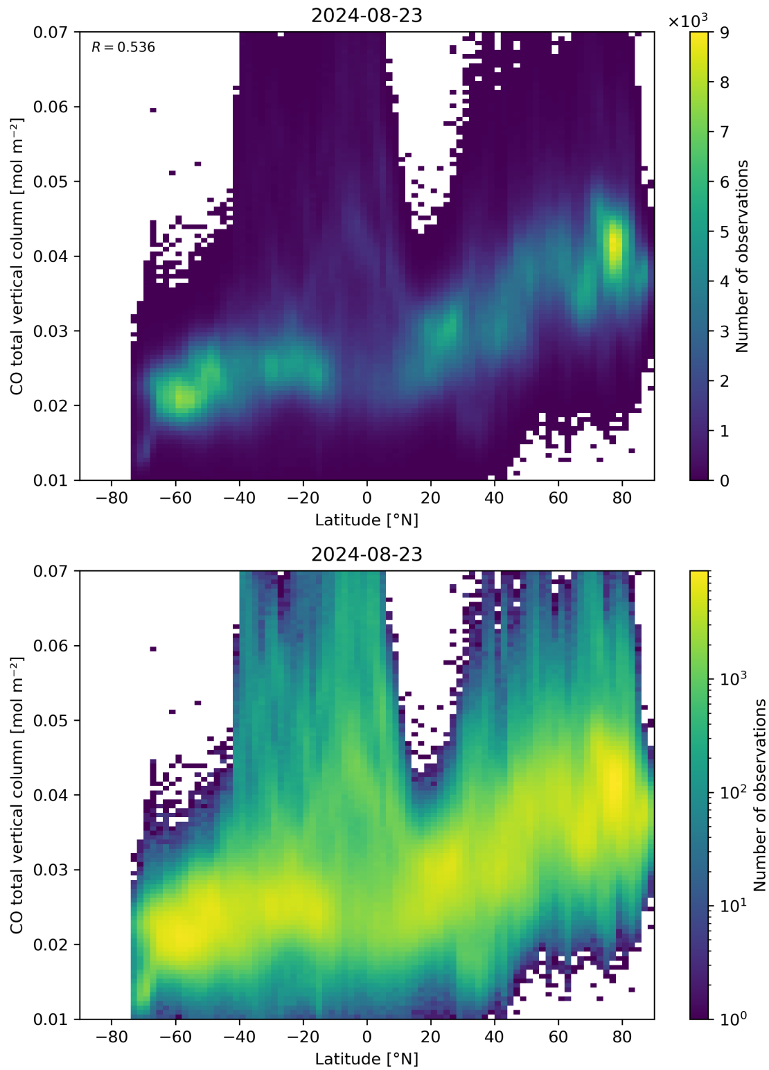
Figure 51: Scatter density plot of “Latitude” against “CO total vertical column” for 2024-08-22 to 2024-08-24.
