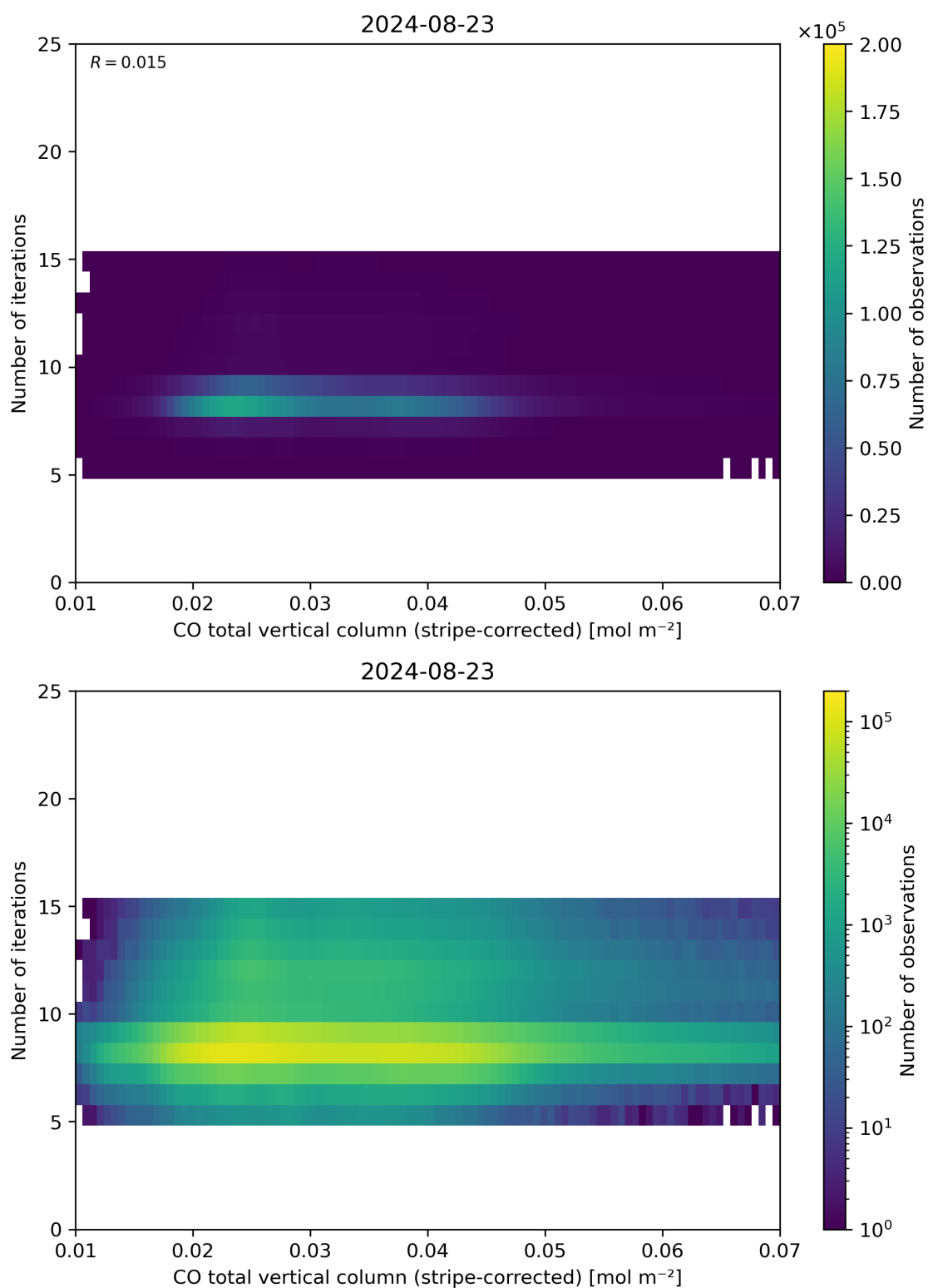
Figure 39: Scatter density plot of “CO total vertical column (stripe-corrected)” against “Number of iterations” for 2024-08-22 to 2024-08-24.
