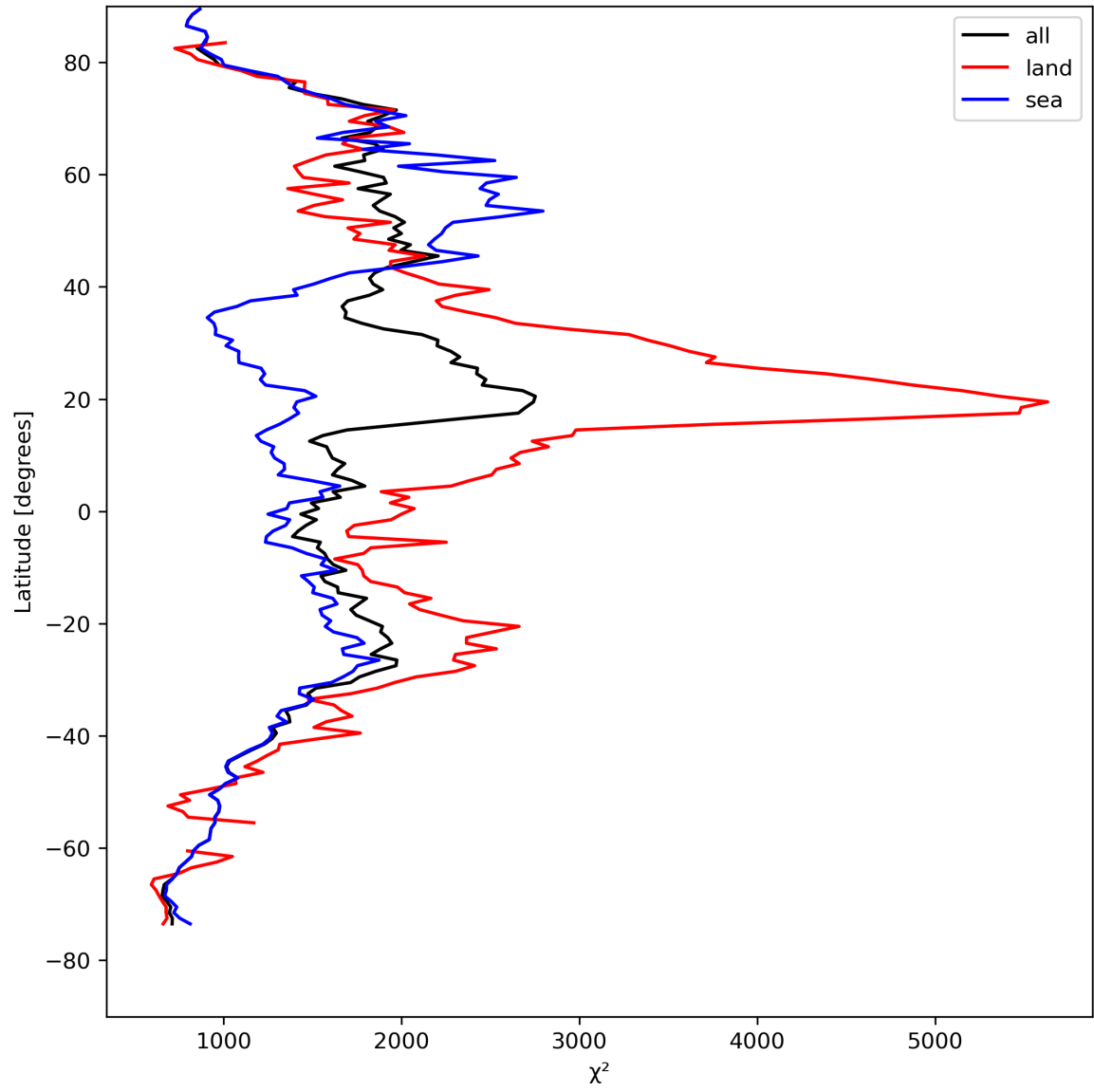
Figure 14: Zonal average of “ \chi^2 ” for 2024-08-22 to 2024-08-24.
