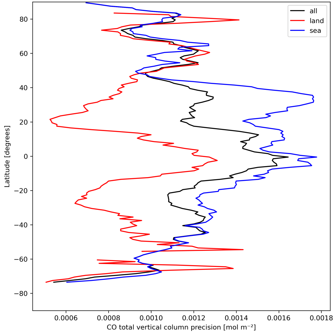
Figure 12: Zonal average of “CO total vertical column precision” for 2024-08-22 to 2024-08-24.
