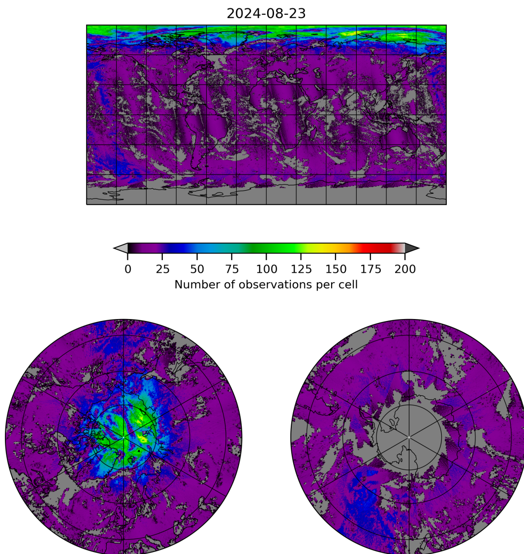
Figure 8: Map of the number of observations for 2024-08-22 to 2024-08-24
