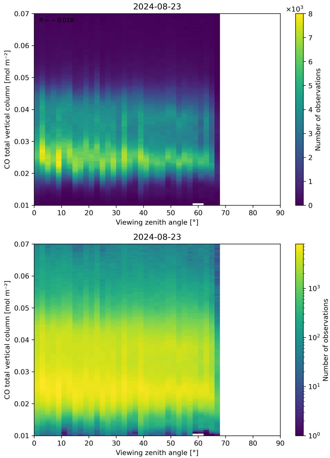
Figure 69: Scatter density plot of “Viewing zenith angle” against “CO total vertical column” for 2024-08-22 to 2024-08-24.
