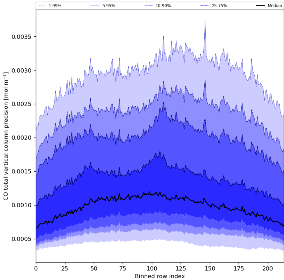
Figure 28: Along track statistics of “CO total vertical column precision” for 2024-08-22 to 2024-08-24
