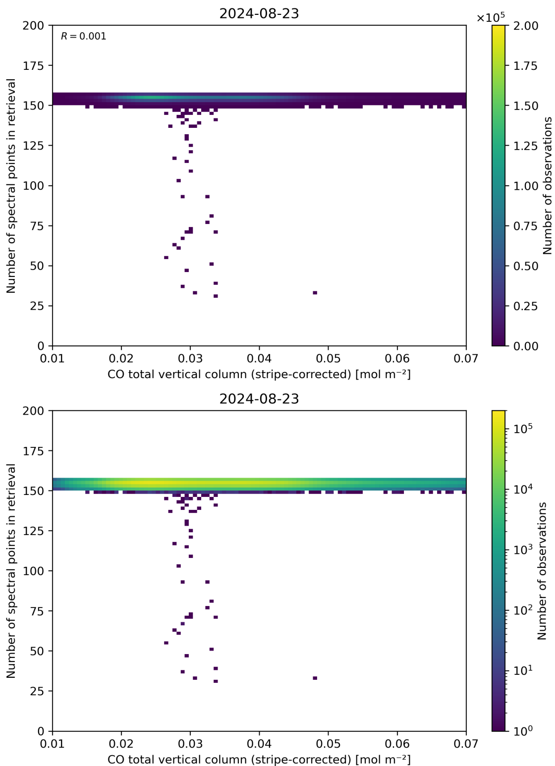
Figure 40: Scatter density plot of “CO total vertical column (stripe-corrected)” against “Number of spectral points in retrieval” for 2024-08-22 to 2024-08-24.
