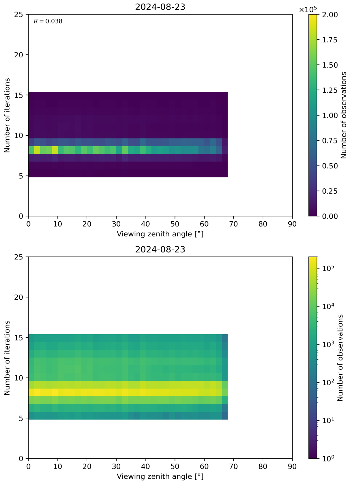
Figure 75: Scatter density plot of “Viewing zenith angle” against “Number of iterations” for 2024-08-22 to 2024-08-24.
