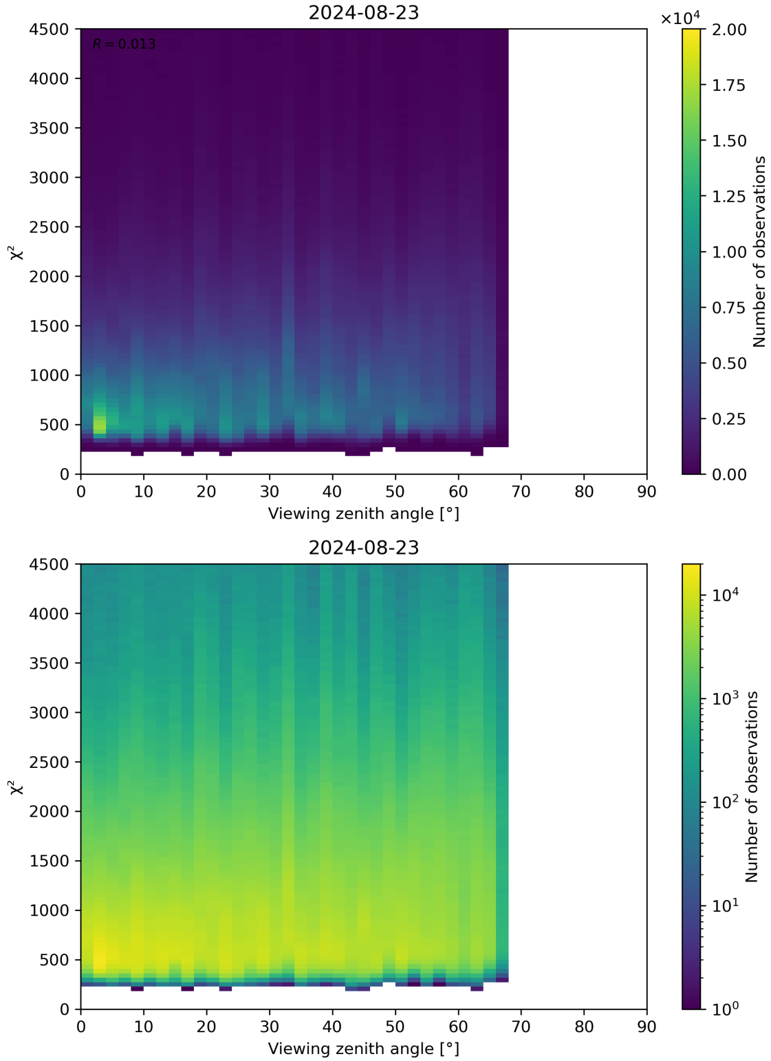
Figure 72: Scatter density plot of “Viewing zenith angle” against “ \chi^2 ” for 2024-08-22 to 2024-08-24.
