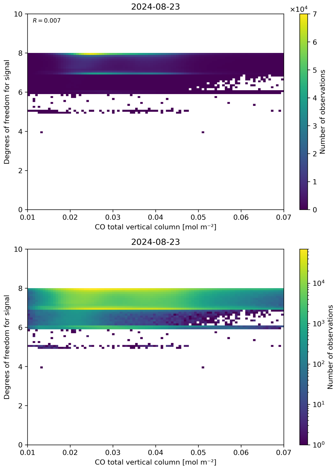
Figure 41: Scatter density plot of “CO total vertical column” against “Degrees of freedom for signal” for 2024-08-22 to 2024-08-24.
