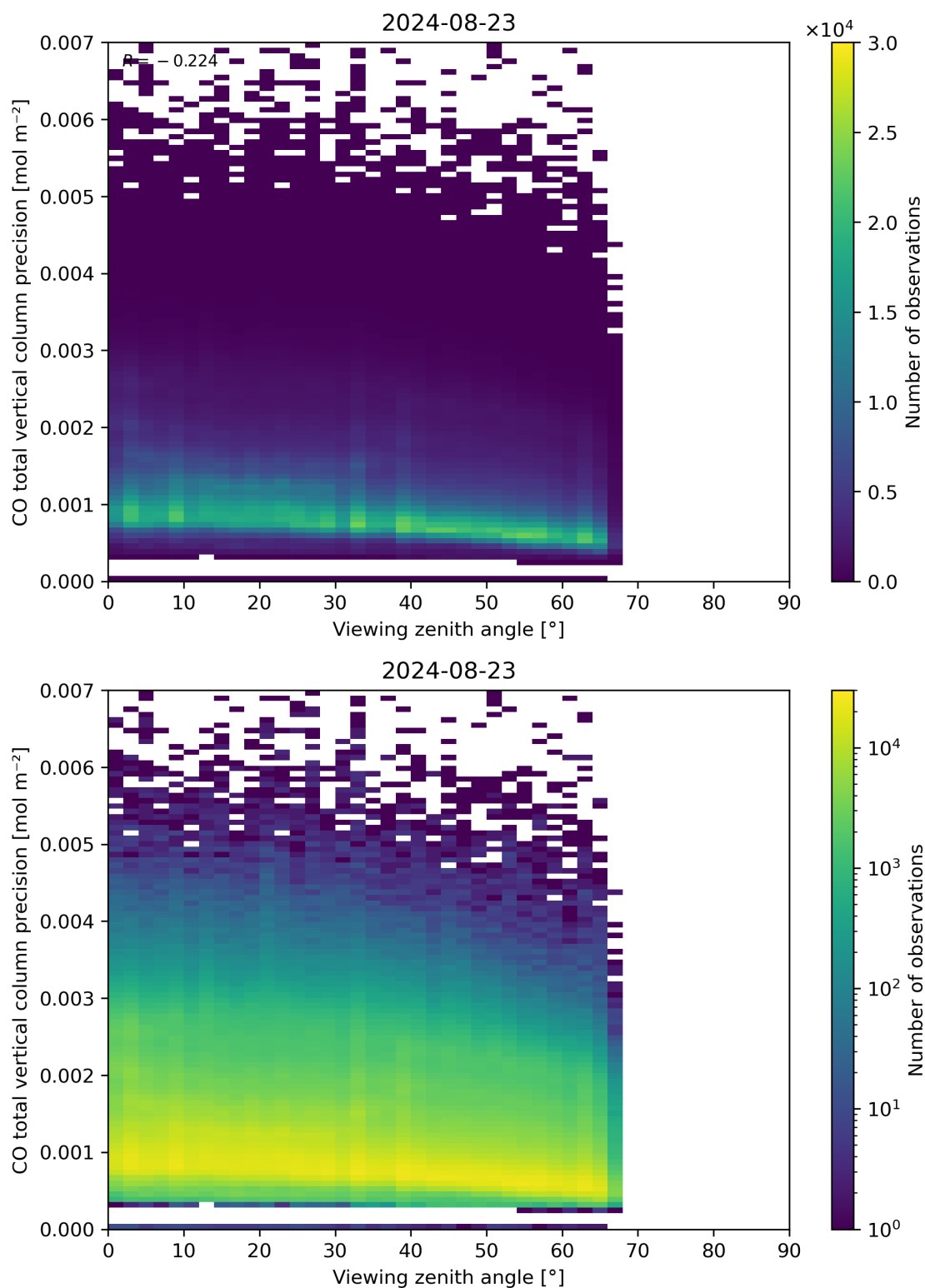
Figure 71: Scatter density plot of “Viewing zenith angle” against “CO total vertical column precision” for 2024-08-22 to 2024-08-24.
