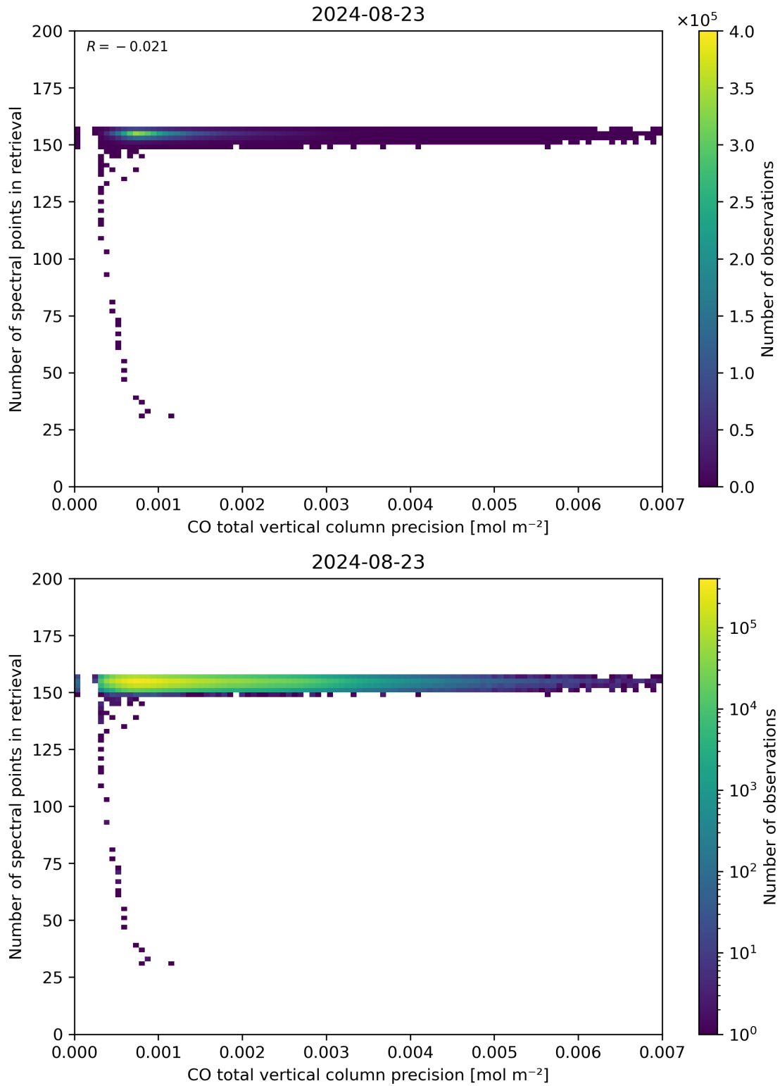
Figure 47: Scatter density plot of “CO total vertical column precision” against “Number of spectral points in retrieval” for 2024-08-22 to 2024-08-24.
