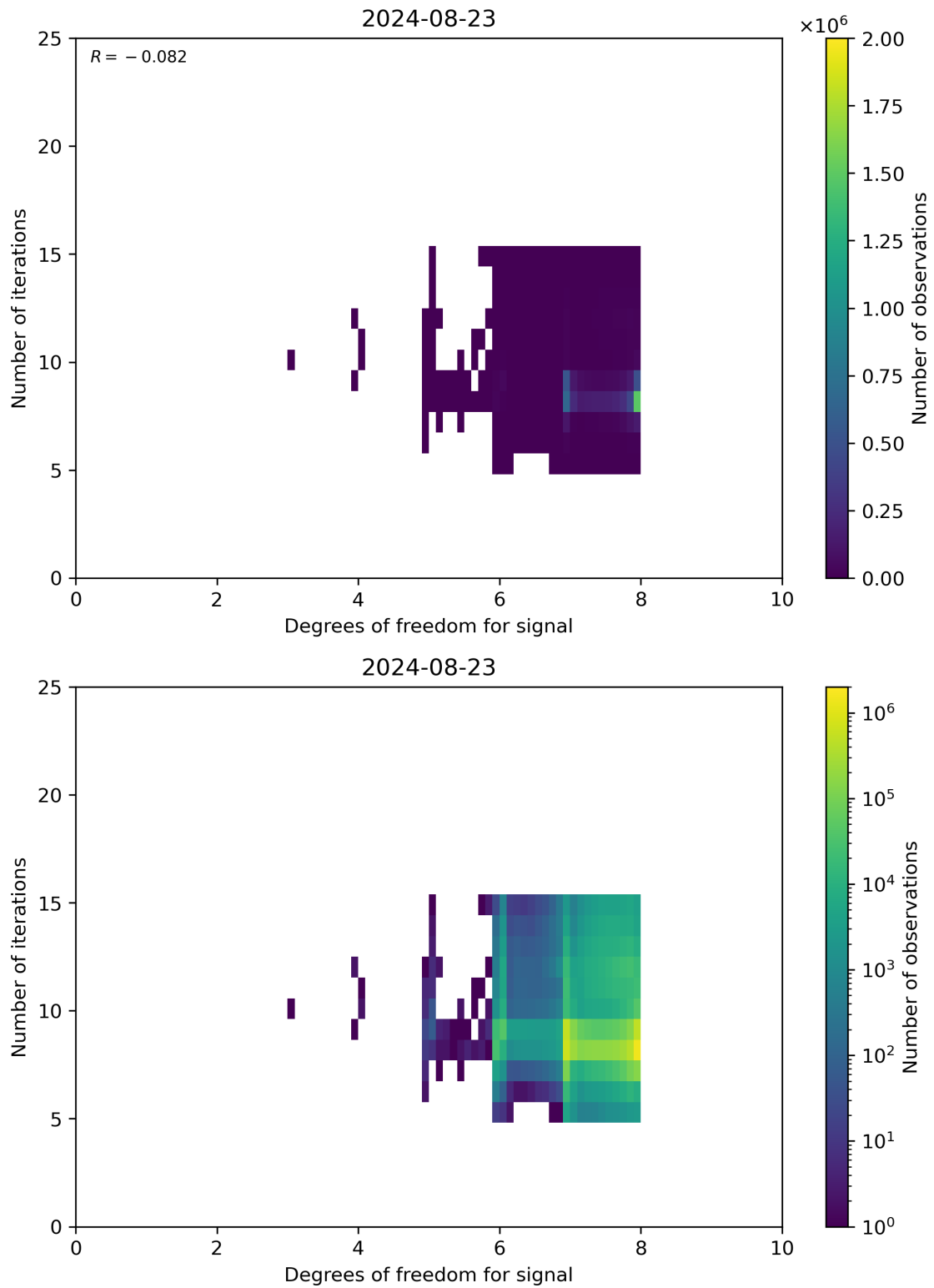
Figure 50: Scatter density plot of “Degrees of freedom for signal” against “Number of iterations” for 2024-08-22 to 2024-08-24.
