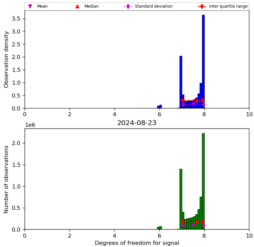
Figure 23: Histogram of “Degrees of freedom for signal” for 2024-08-22 to 2024-08-24
