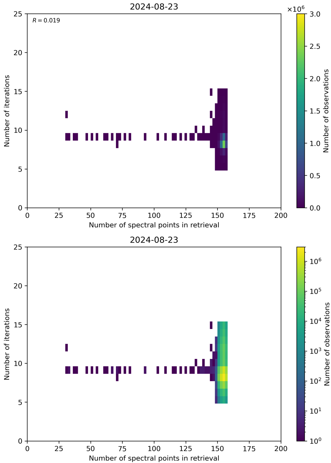
Figure 60: Scatter density plot of “Number of spectral points in retrieval” against “Number of iterations” for 2024-08-22 to 2024-08-24.
