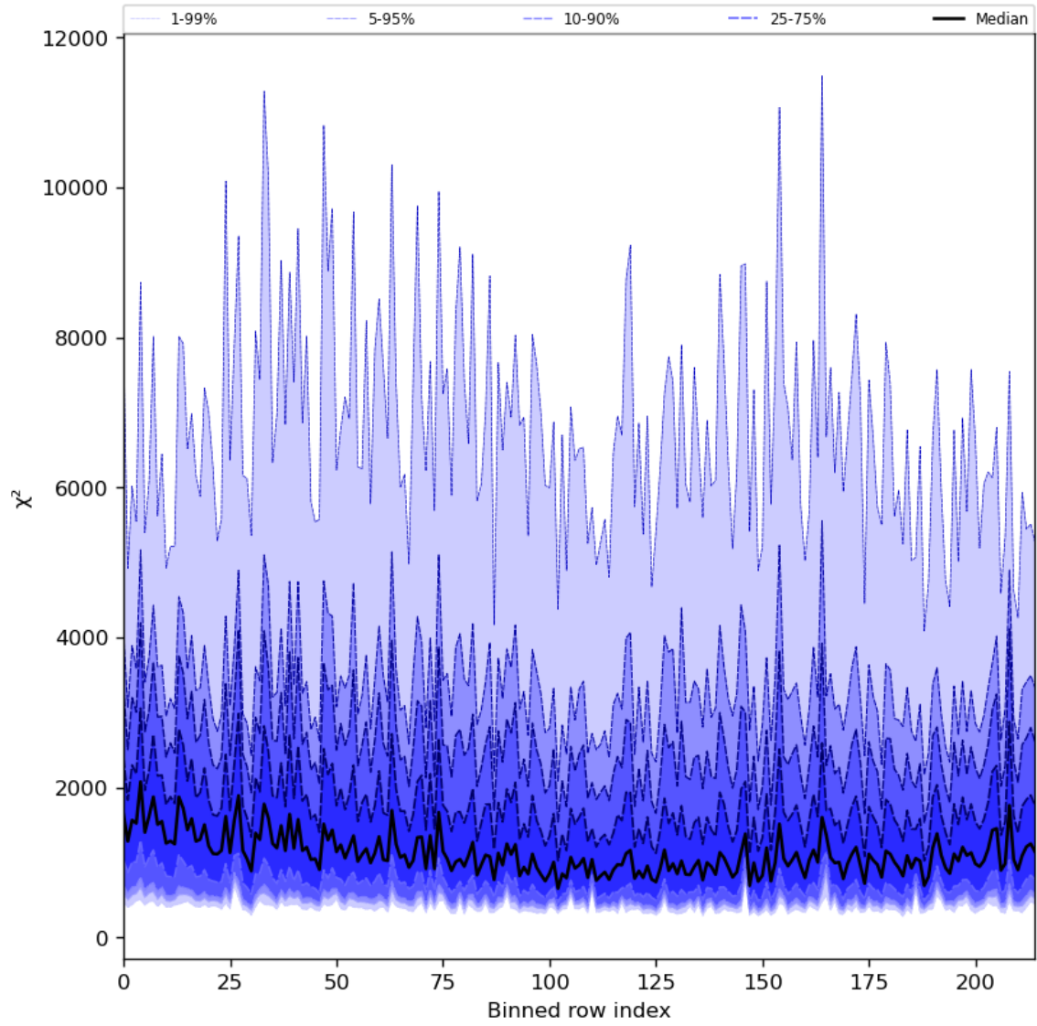
Figure 30: Along track statistics of “ \chi^2 ” for 2024-08-22 to 2024-08-24
