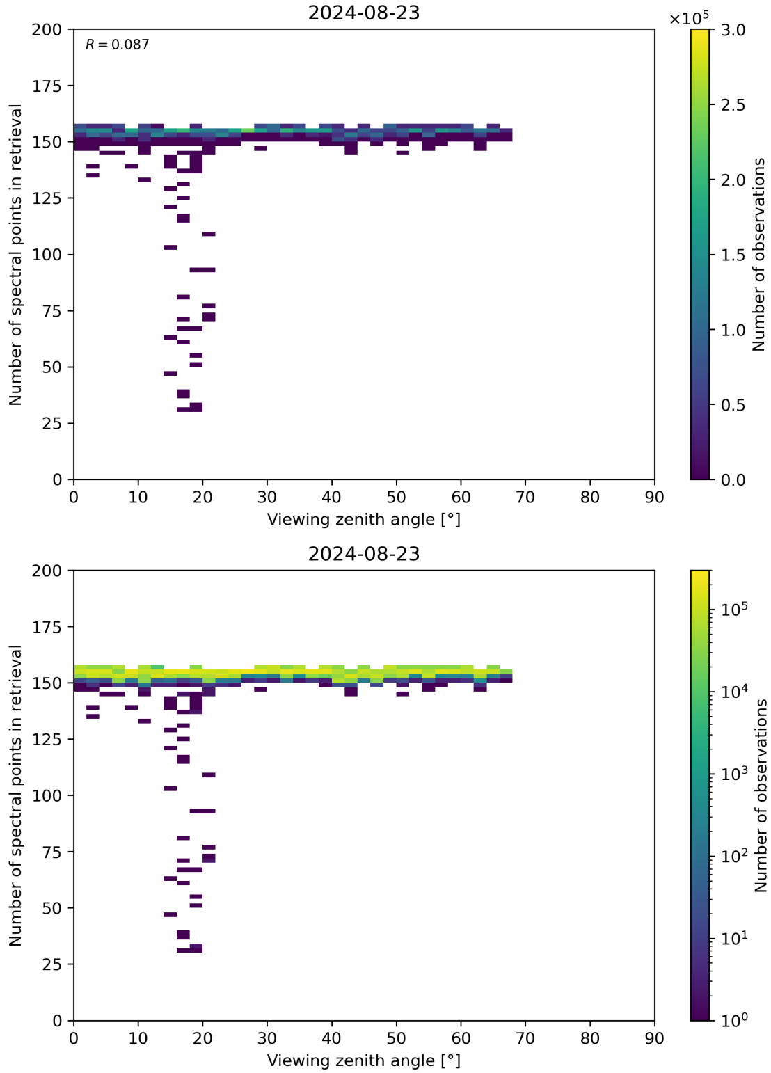
Figure 76: Scatter density plot of “Viewing zenith angle” against “Number of spectral points in retrieval” for 2024-08-22 to 2024-08-24.
