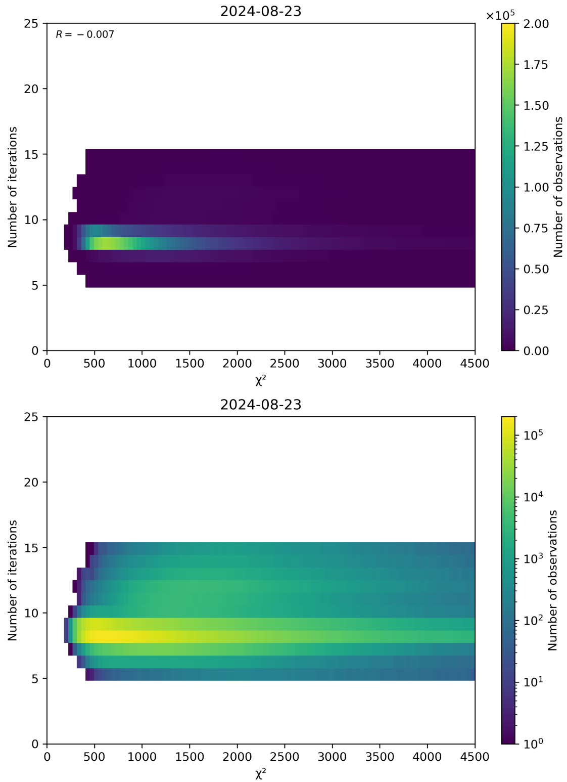
Figure 49: Scatter density plot of “ \chi^2 ” against “Number of iterations” for 2024-08-22 to 2024-08-24.
