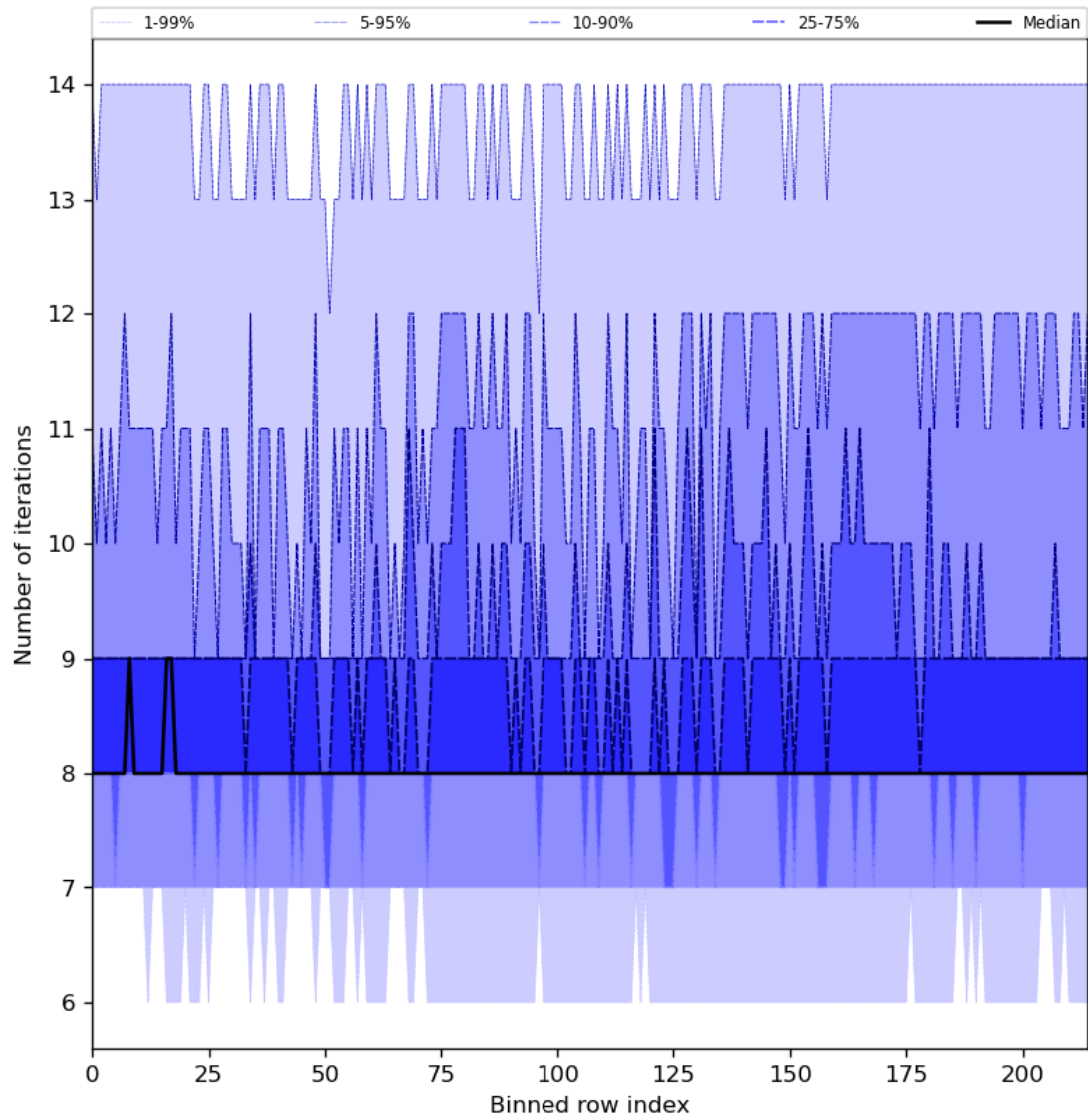
Figure 32: Along track statistics of “Number of iterations” for 2024-08-22 to 2024-08-24
