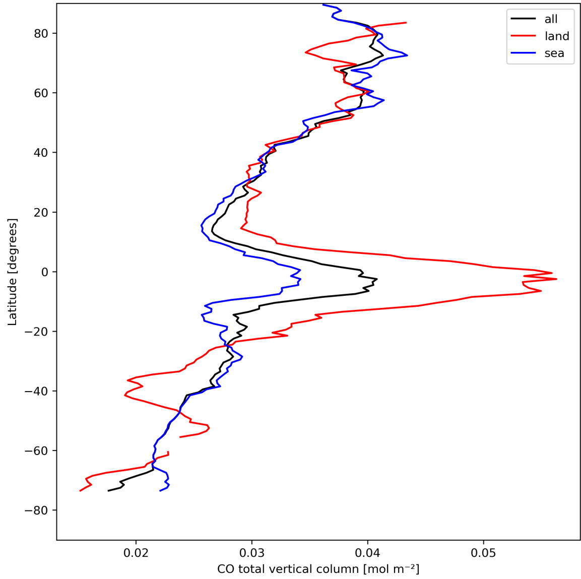
Figure 10: Zonal average of “CO total vertical column” for 2024-08-22 to 2024-08-24.
