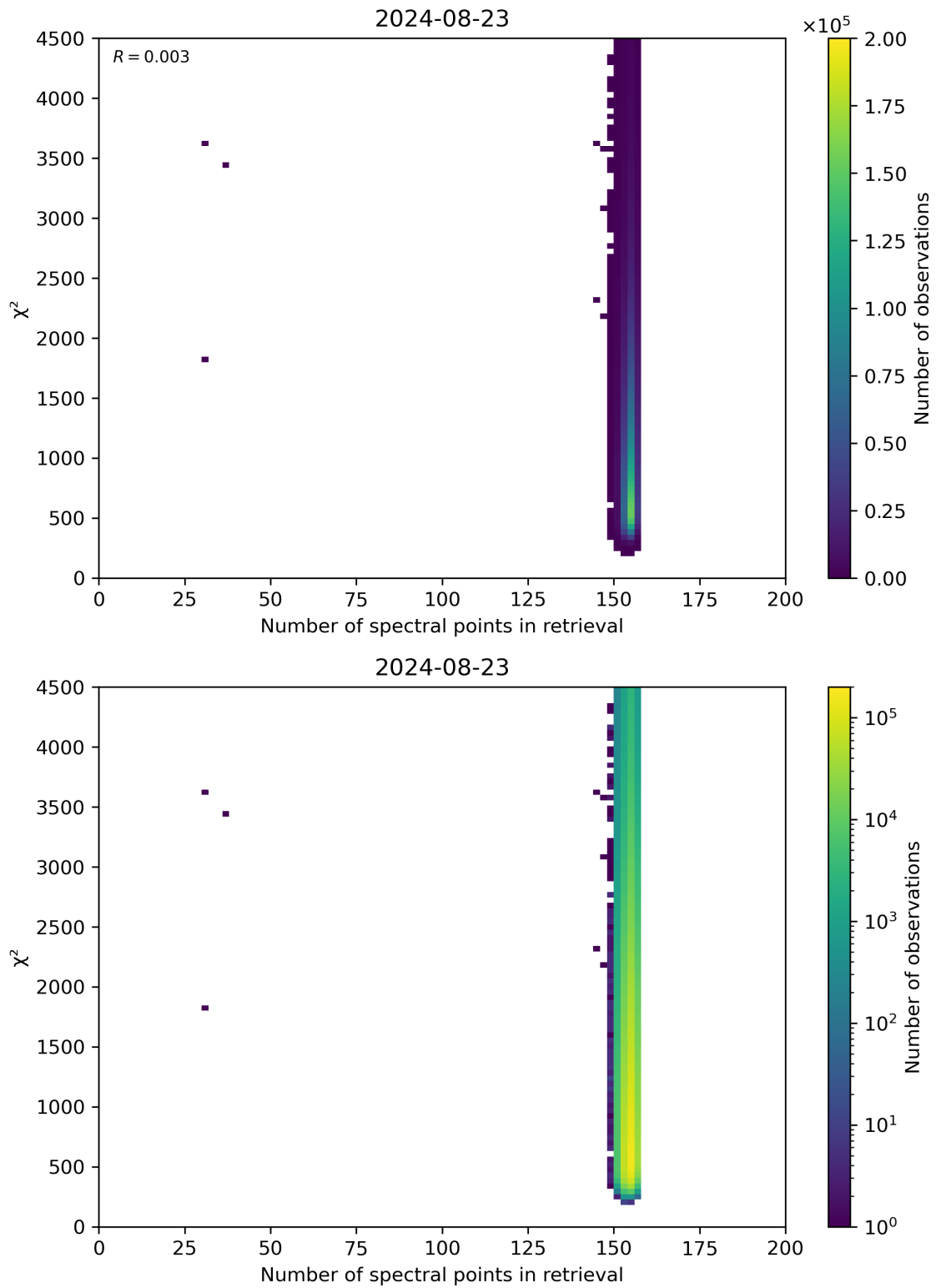
Figure 58: Scatter density plot of “Number of spectral points in retrieval” against “ \chi^2 ” for 2024-08-22 to 2024-08-24.
