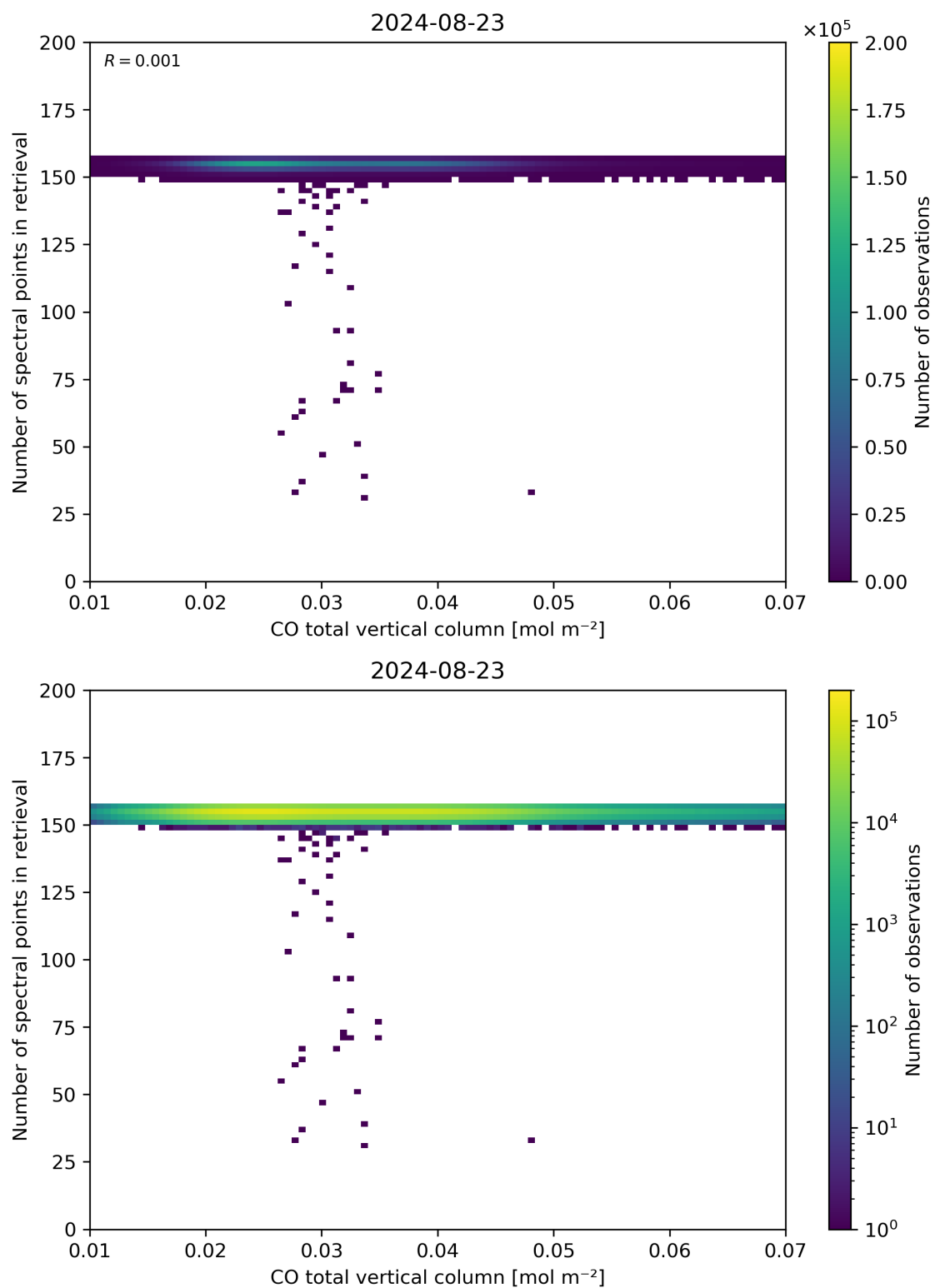
Figure 43: Scatter density plot of “CO total vertical column” against “Number of spectral points in retrieval” for 2024-08-22 to 2024-08-24.
