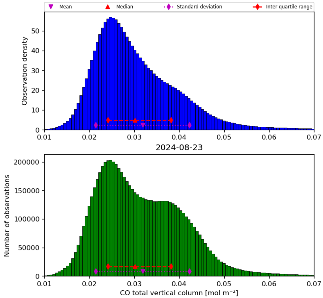
Figure 18: Histogram of “CO total vertical column” for 2024-08-22 to 2024-08-24
