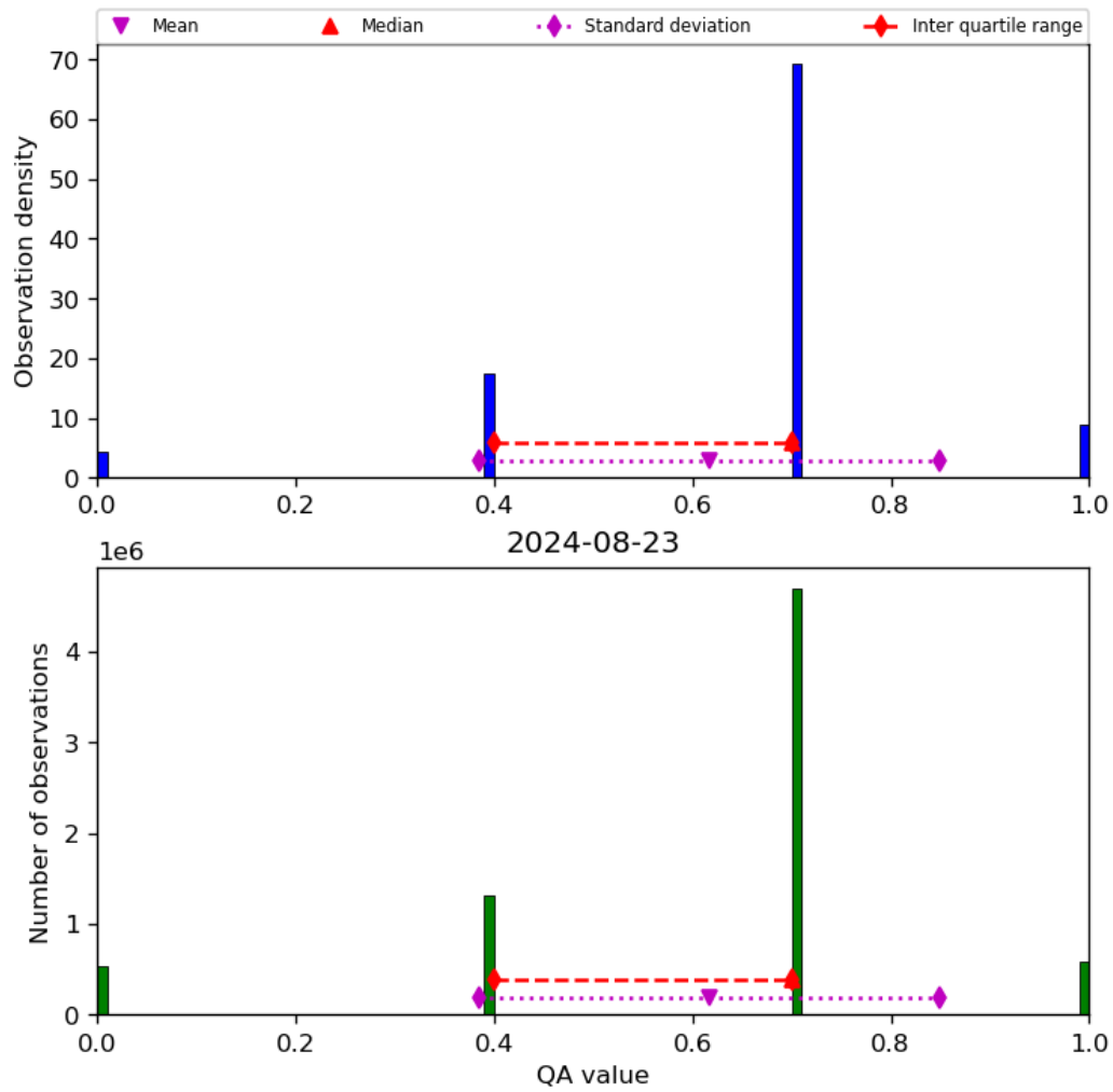
Figure 17: Histogram of “QA value” for 2024-08-22 to 2024-08-24
