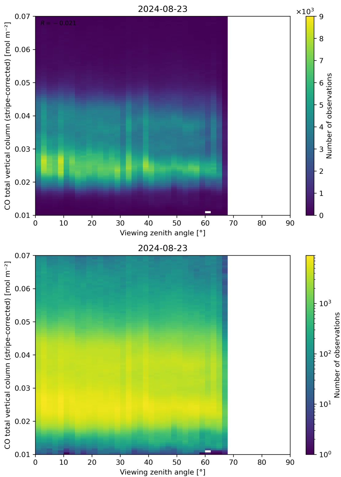
Figure 70: Scatter density plot of “Viewing zenith angle” against “CO total vertical column (stripe-corrected)” for 2024-08-22 to 2024-08-24.
