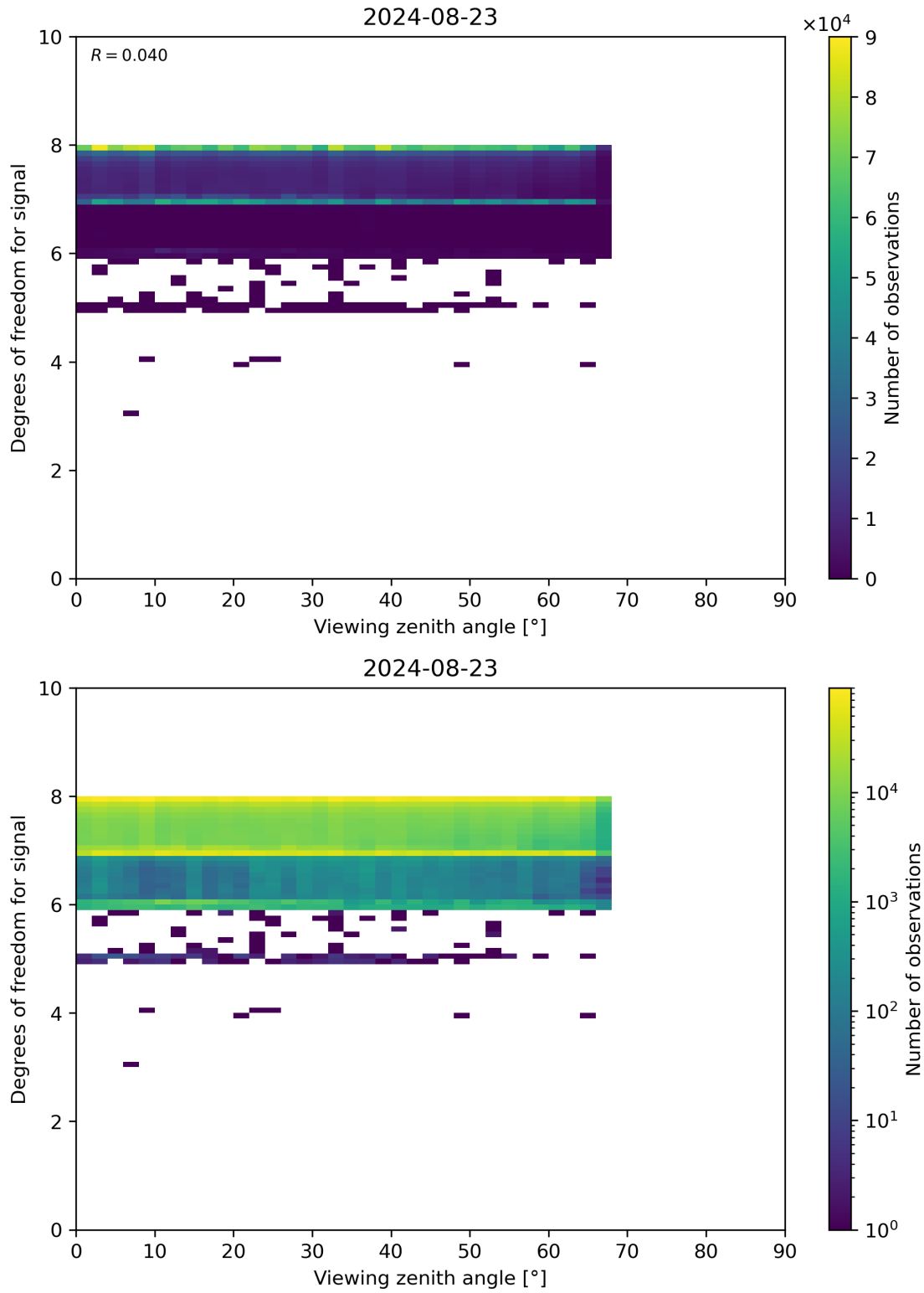
Figure 73: Scatter density plot of “Viewing zenith angle” against “Degrees of freedom for signal” for 2024-08-22 to 2024-08-24.
