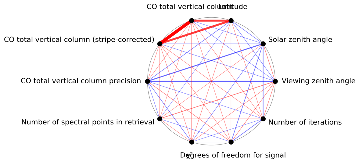
Figure 1: Map of correlation graph for 2024-08-22 to 2024-08-24.
