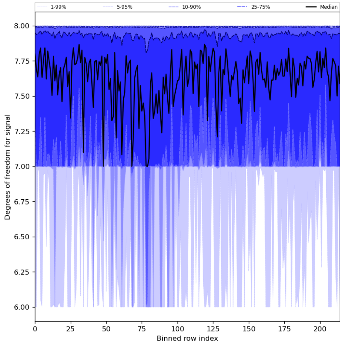
Figure 31: Along track statistics of “Degrees of freedom for signal” for 2024-08-22 to 2024-08-24
