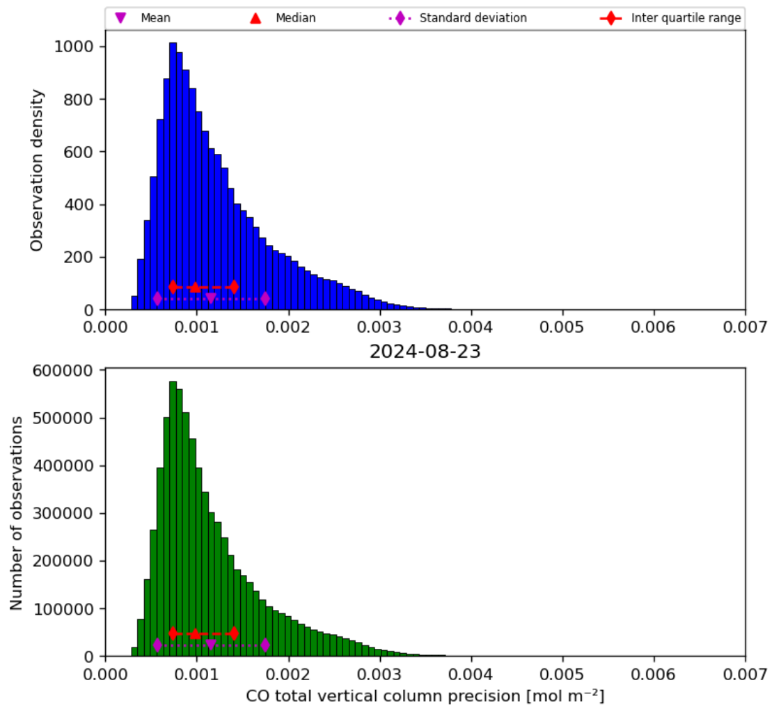
Figure 20: Histogram of “CO total vertical column precision” for 2024-08-22 to 2024-08-24
