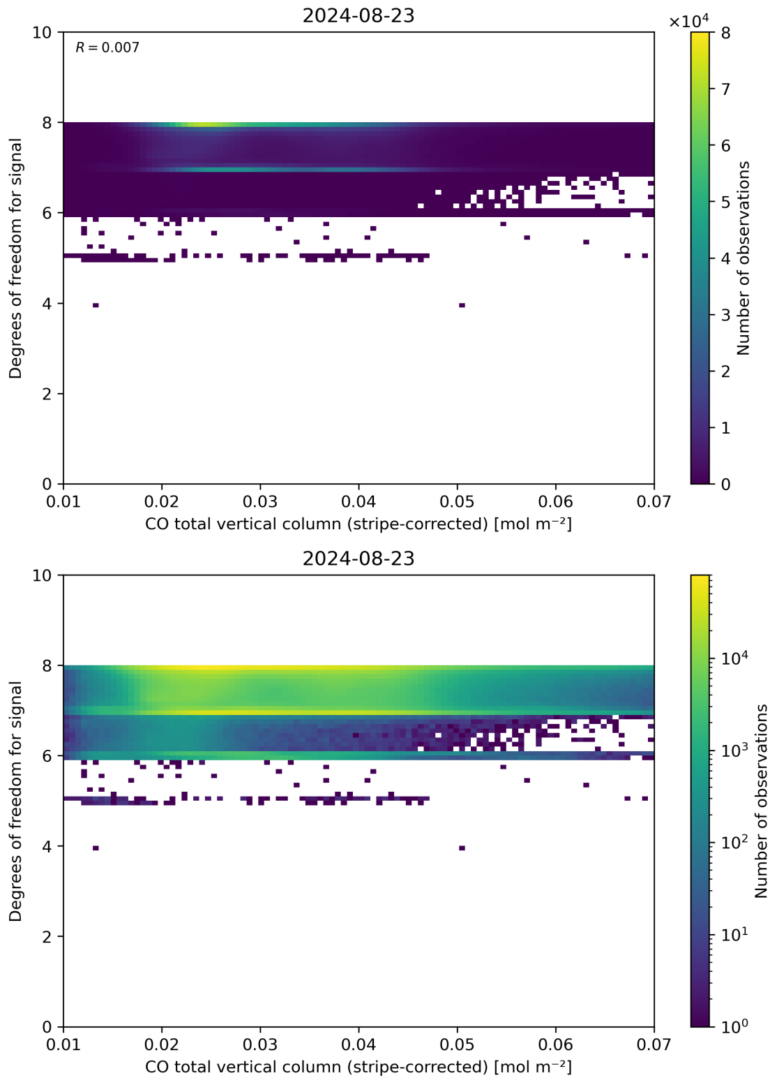
Figure 38: Scatter density plot of “CO total vertical column (stripe-corrected)” against “Degrees of freedom for signal” for 2024-08-22 to 2024-08-24.
