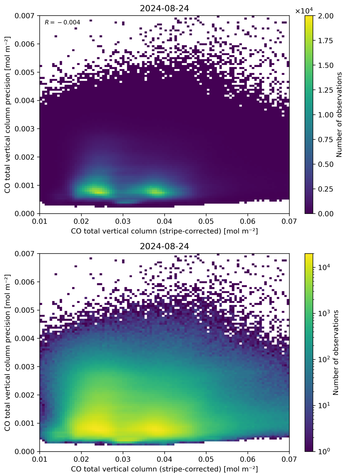
Figure 36: Scatter density plot of “CO total vertical column (stripe-corrected)” against “CO total vertical column precision” for 2024-08-23 to 2024-08-25.
