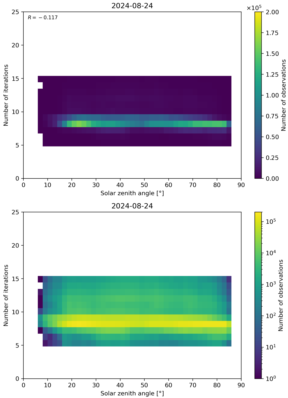
Figure 67: Scatter density plot of “Solar zenith angle” against “Number of iterations” for 2024-08-23 to 2024-08-25.
