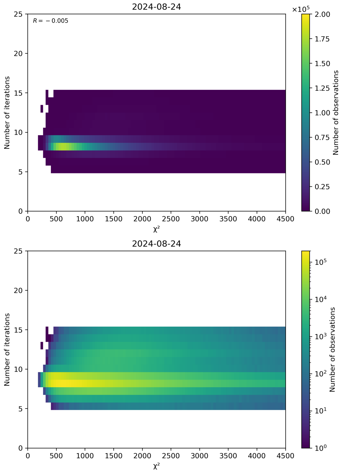
Figure 49: Scatter density plot of “ \chi^2 ” against “Number of iterations” for 2024-08-23 to 2024-08-25.
