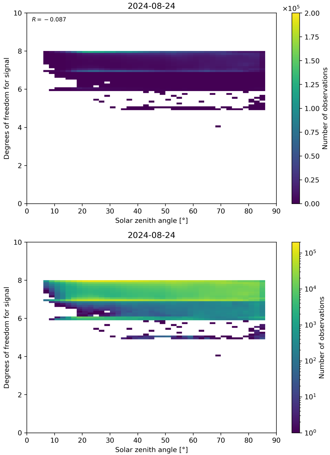
Figure 65: Scatter density plot of “Solar zenith angle” against “Degrees of freedom for signal” for 2024-08-23 to 2024-08-25.
