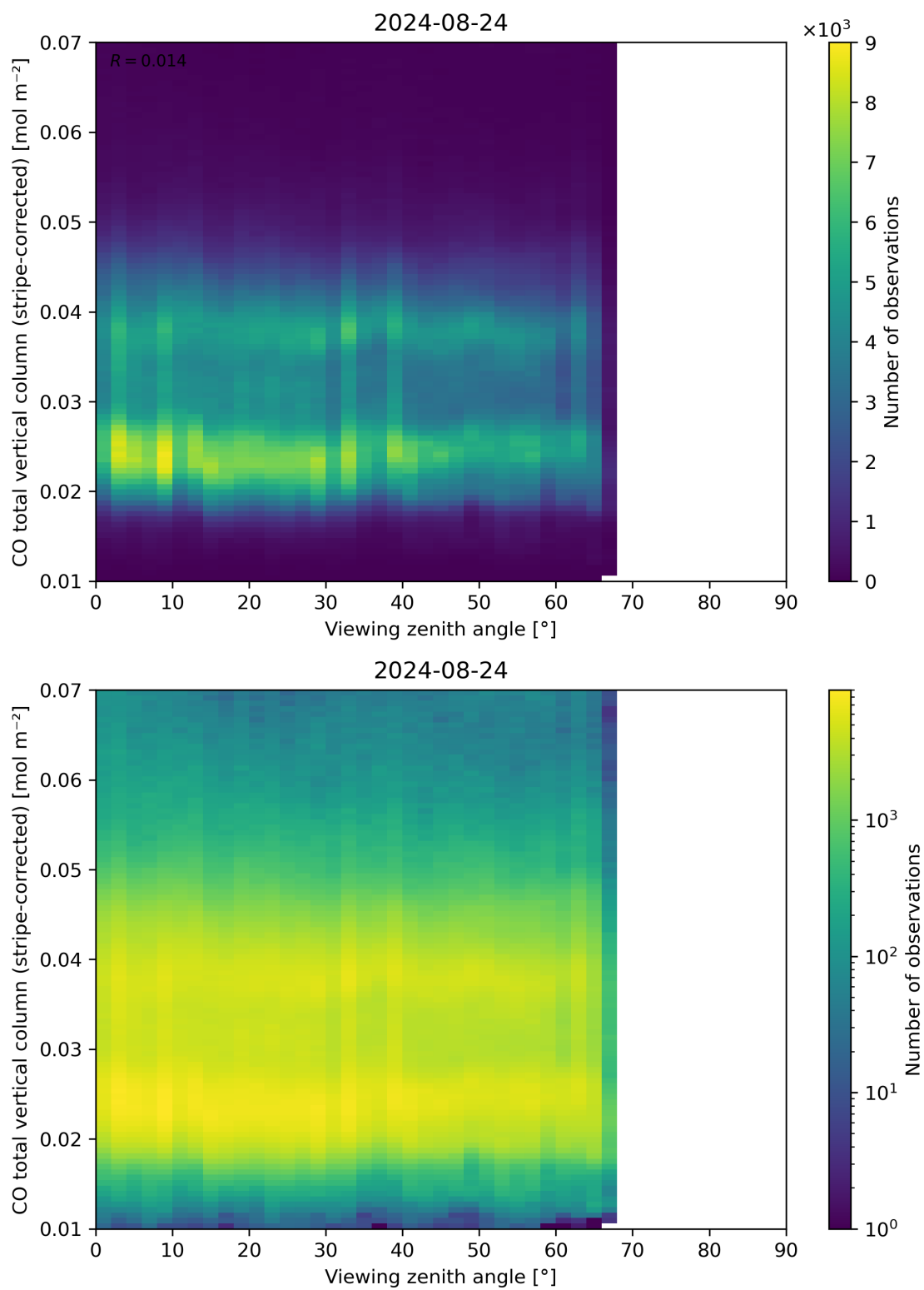
Figure 70: Scatter density plot of “Viewing zenith angle” against “CO total vertical column (stripe-corrected)” for 2024-08-23 to 2024-08-25.
