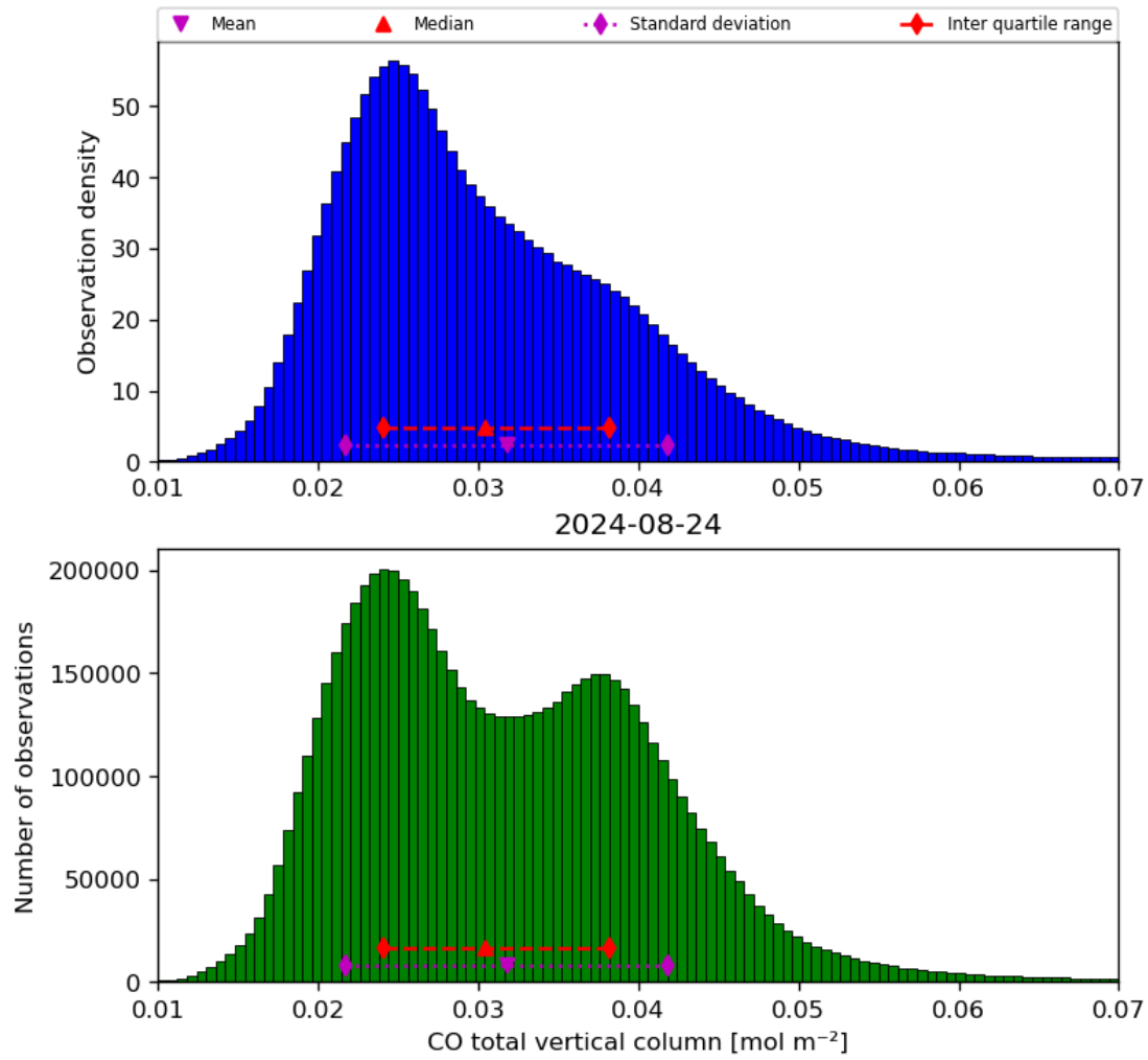
Figure 18: Histogram of “CO total vertical column” for 2024-08-23 to 2024-08-25
