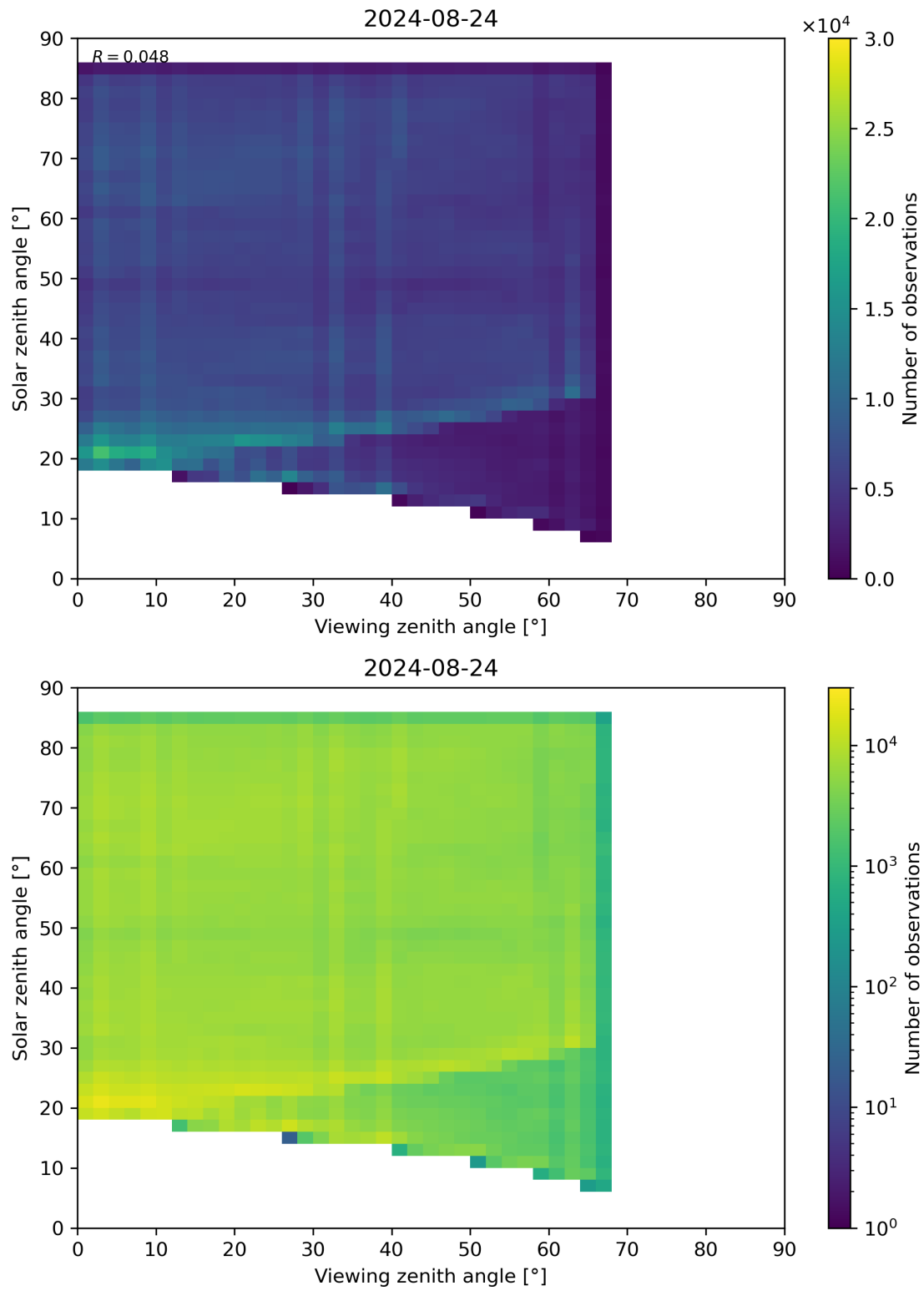
Figure 77: Scatter density plot of “Viewing zenith angle” against “Solar zenith angle” for 2024-08-23 to 2024-08-25.
