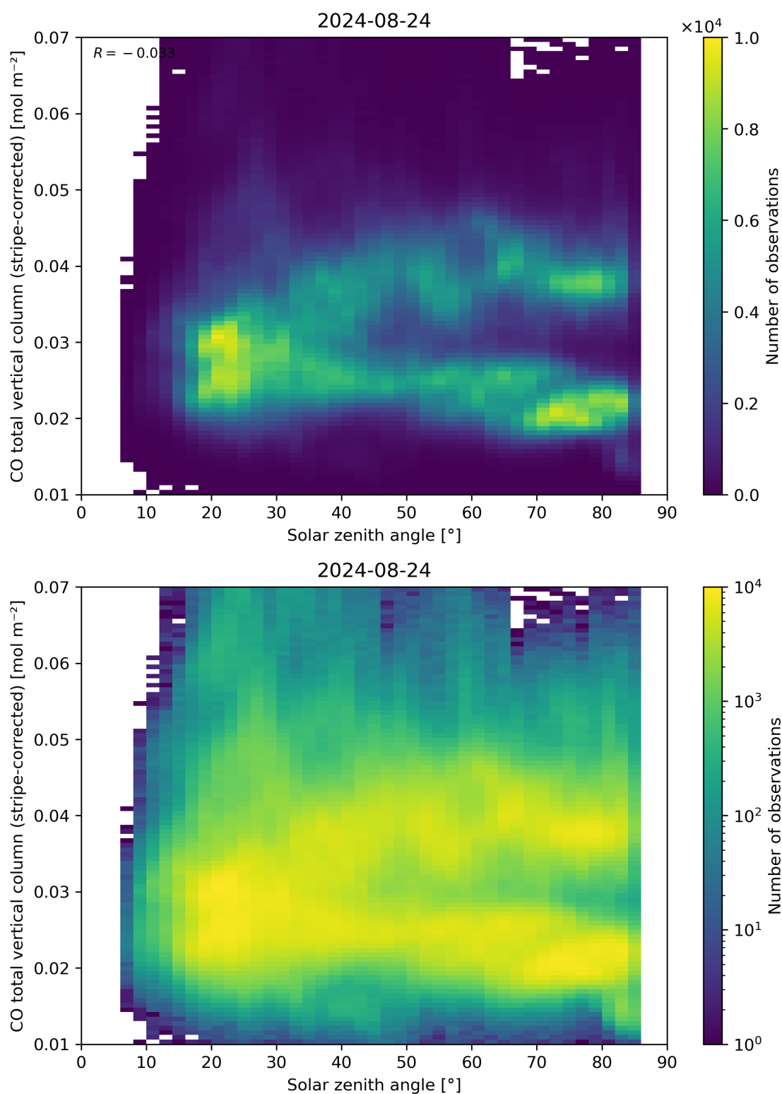
Figure 62: Scatter density plot of “Solar zenith angle” against “CO total vertical column (stripe-corrected)” for 2024-08-23 to 2024-08-25.
