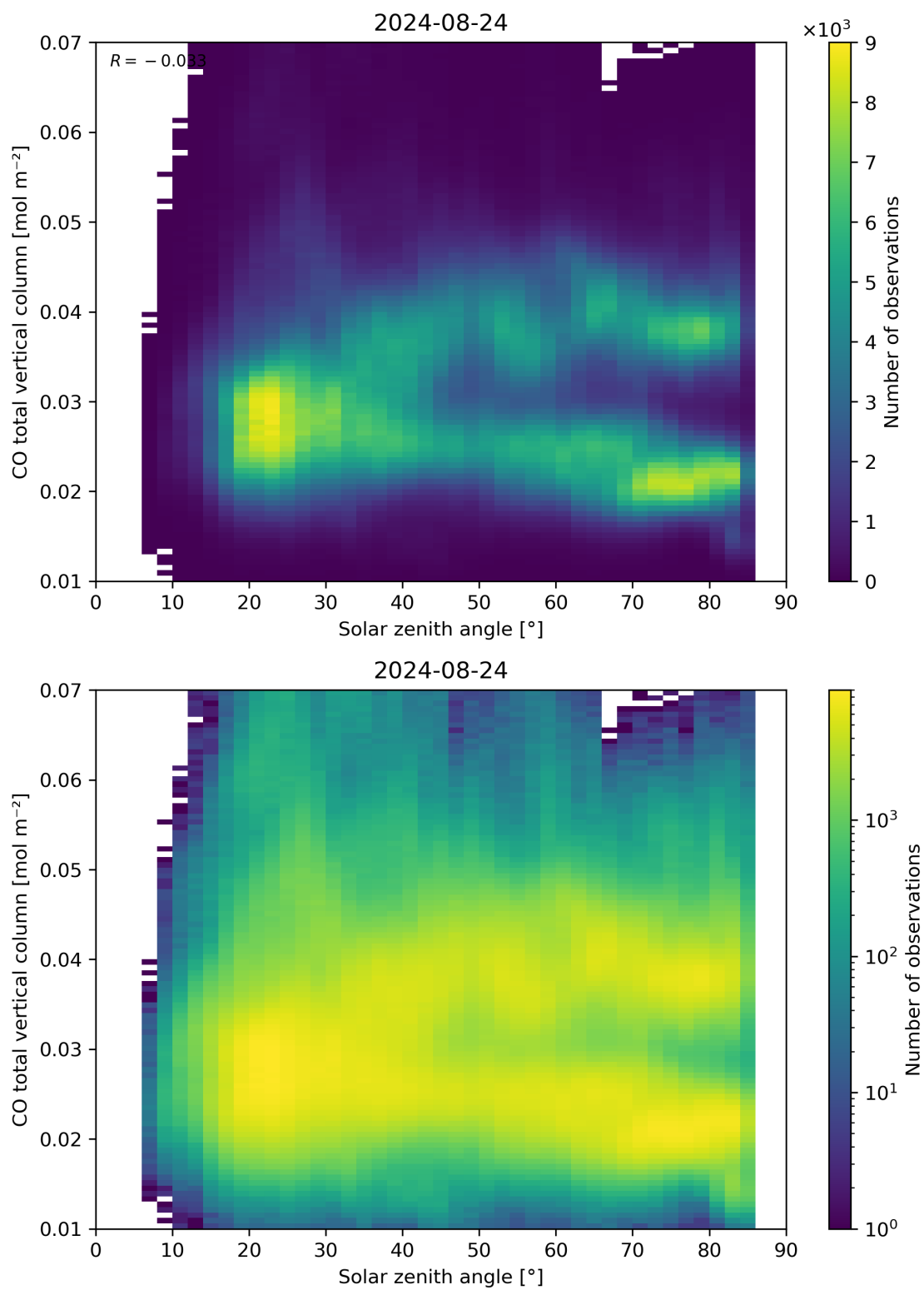
Figure 61: Scatter density plot of “Solar zenith angle” against “CO total vertical column” for 2024-08-23 to 2024-08-25.
