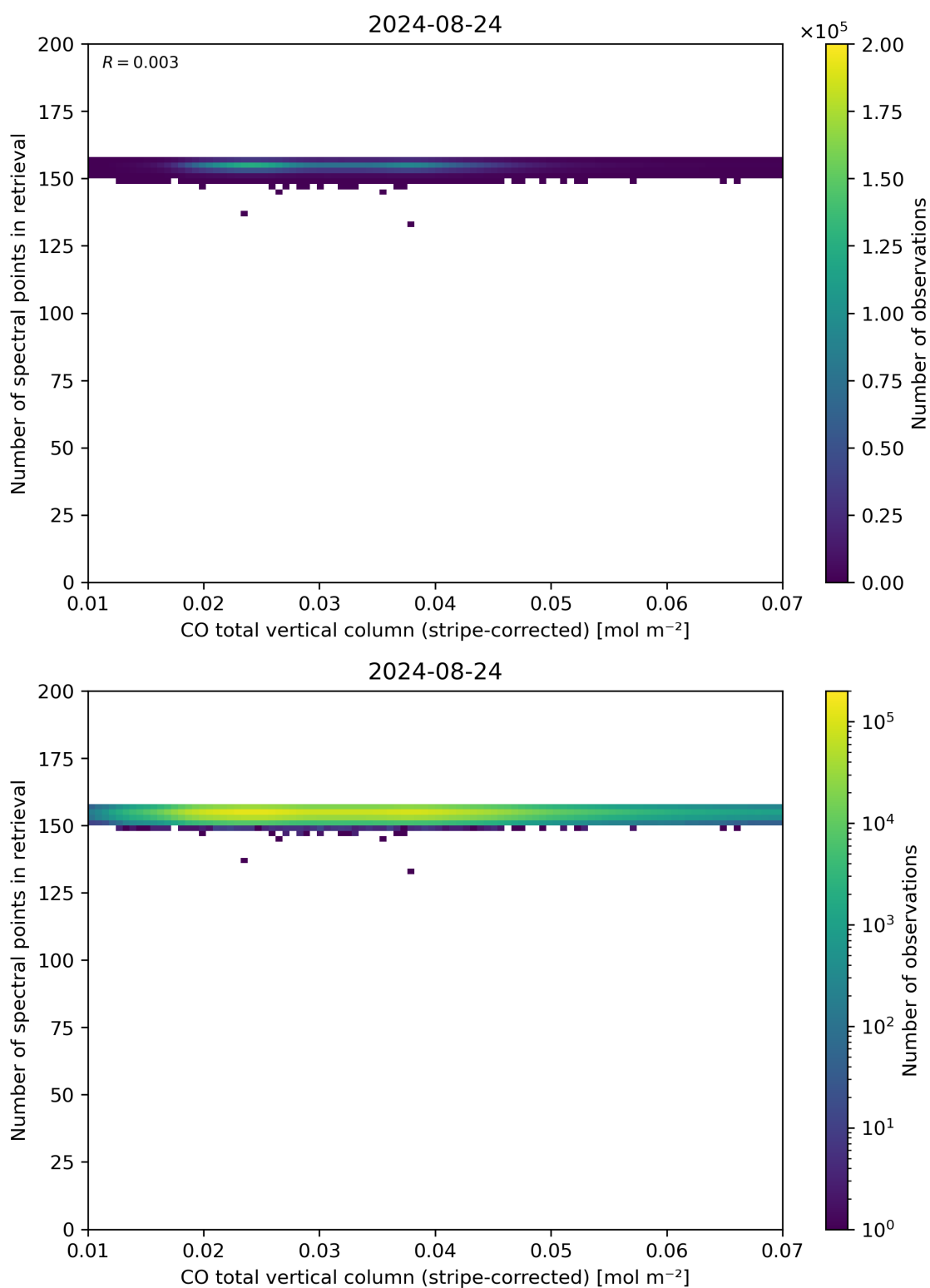
Figure 40: Scatter density plot of “CO total vertical column (stripe-corrected)” against “Number of spectral points in retrieval” for 2024-08-23 to 2024-08-25.
