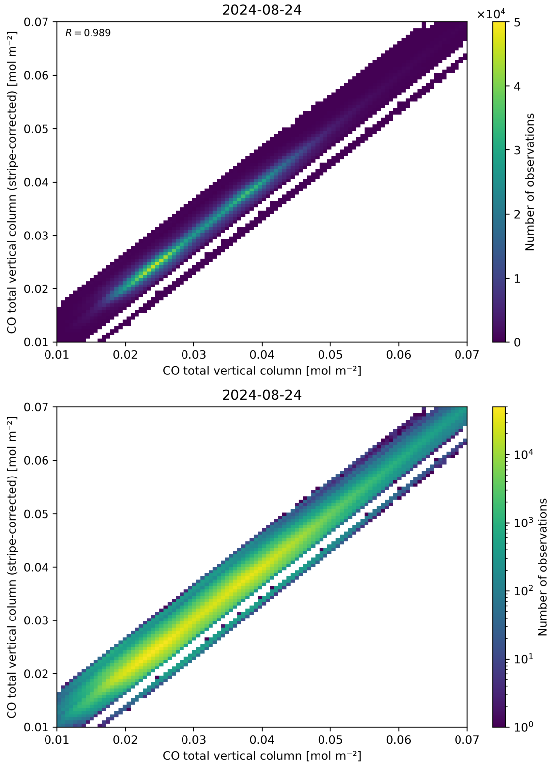
Figure 33: Scatter density plot of “CO total vertical column” against “CO total vertical column (stripe-corrected)” for 2024-08-23 to 2024-08-25.
