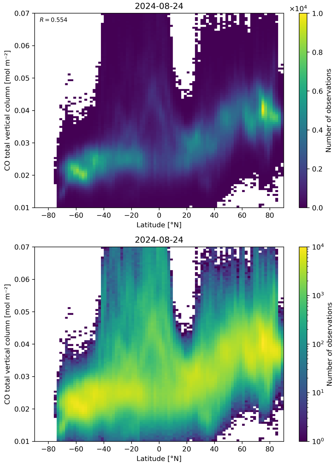
Figure 51: Scatter density plot of “Latitude” against “CO total vertical column” for 2024-08-23 to 2024-08-25.
