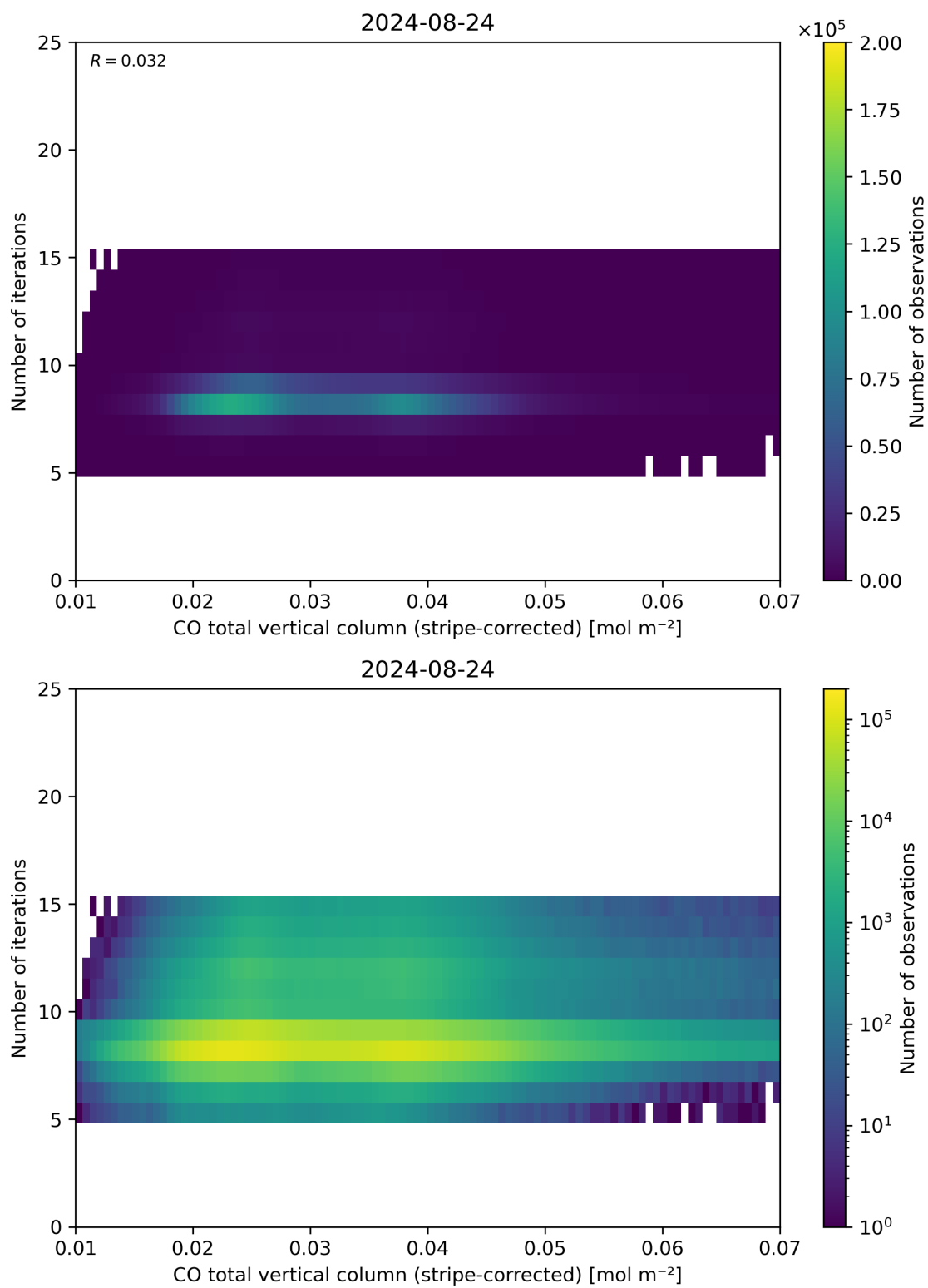
Figure 39: Scatter density plot of “CO total vertical column (stripe-corrected)” against “Number of iterations” for 2024-08-23 to 2024-08-25.
