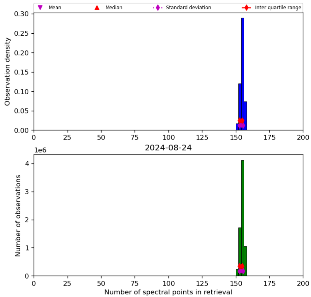
Figure 21: Histogram of “Number of spectral points in retrieval” for 2024-08-23 to 2024-08-25
