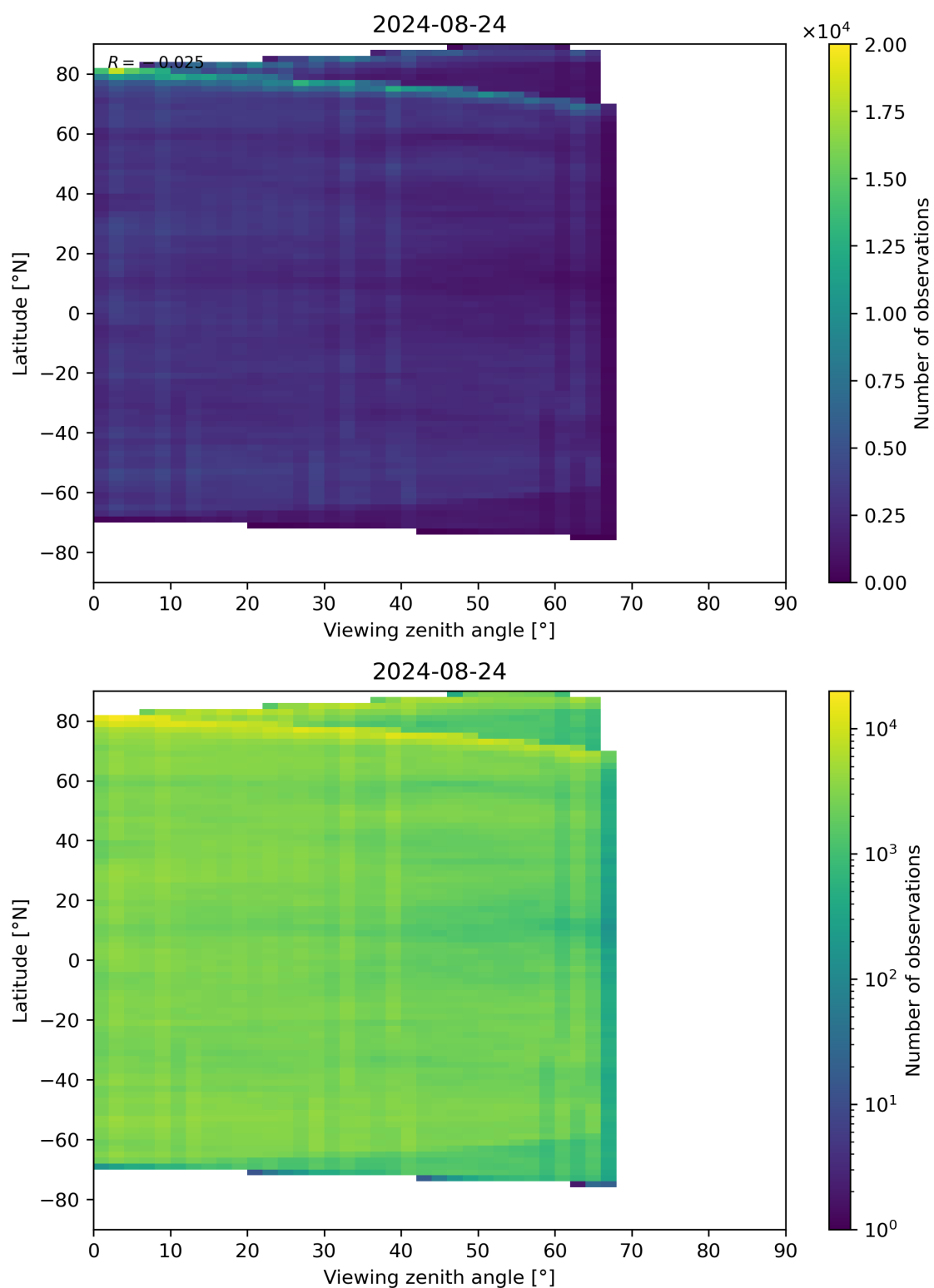
Figure 74: Scatter density plot of “Viewing zenith angle” against “Latitude” for 2024-08-23 to 2024-08-25.
