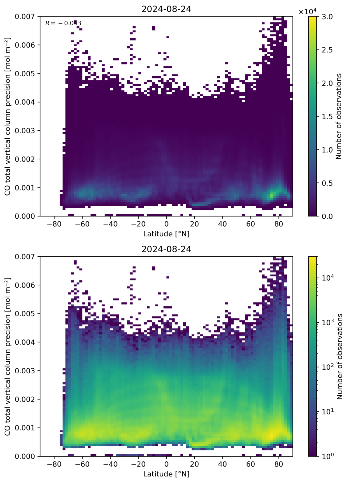
Figure 53: Scatter density plot of “Latitude” against “CO total vertical column precision” for 2024-08-23 to 2024-08-25.
