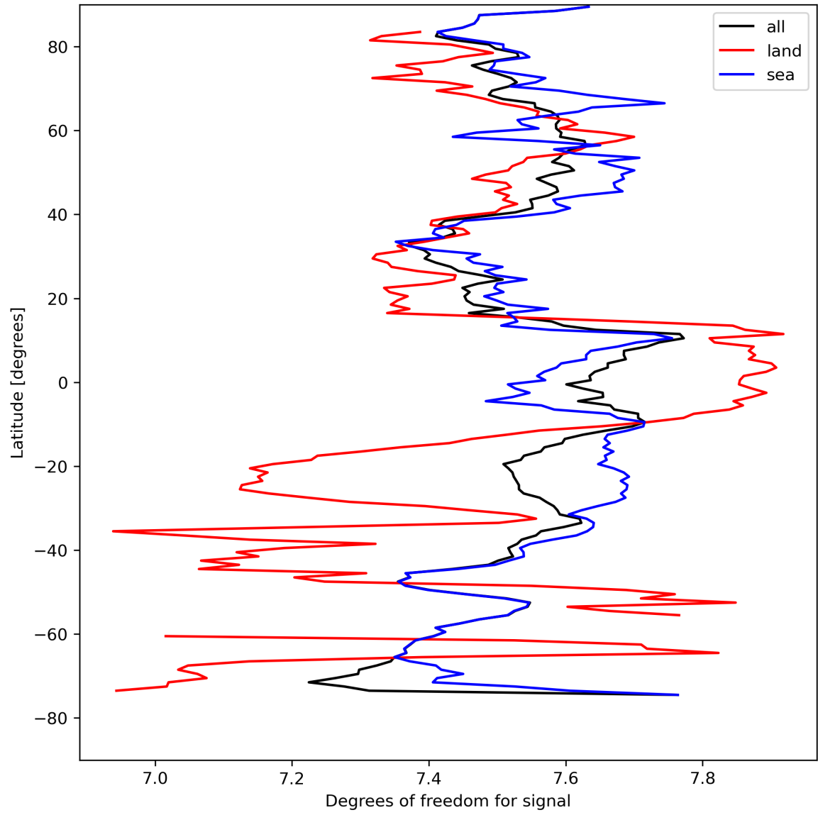
Figure 15: Zonal average of “Degrees of freedom for signal” for 2024-08-23 to 2024-08-25.
