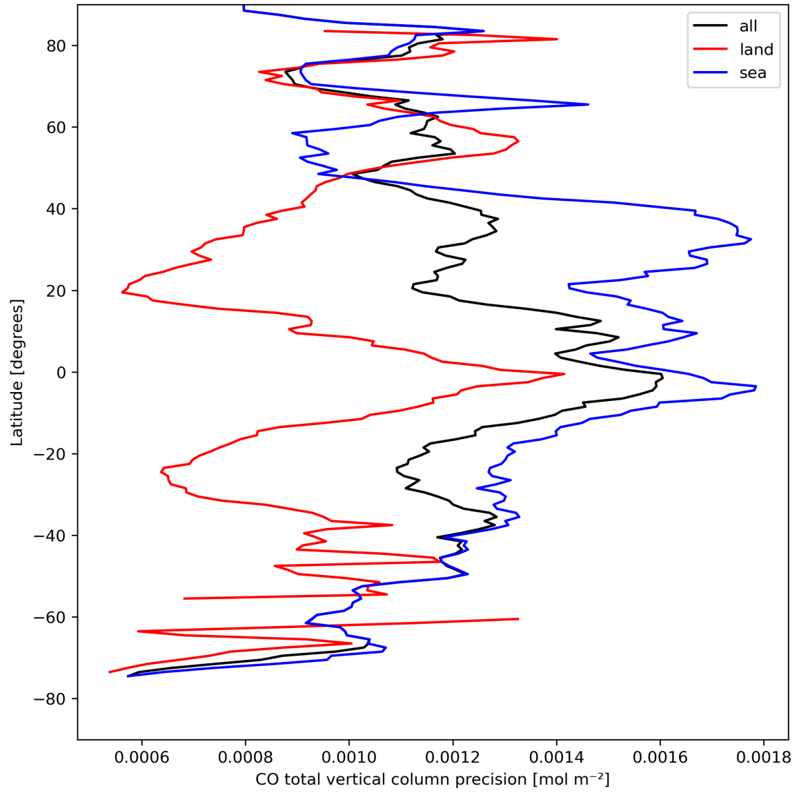
Figure 12: Zonal average of "CO total vertical column precision" for 2024-08-23 to 2024-08-25.
