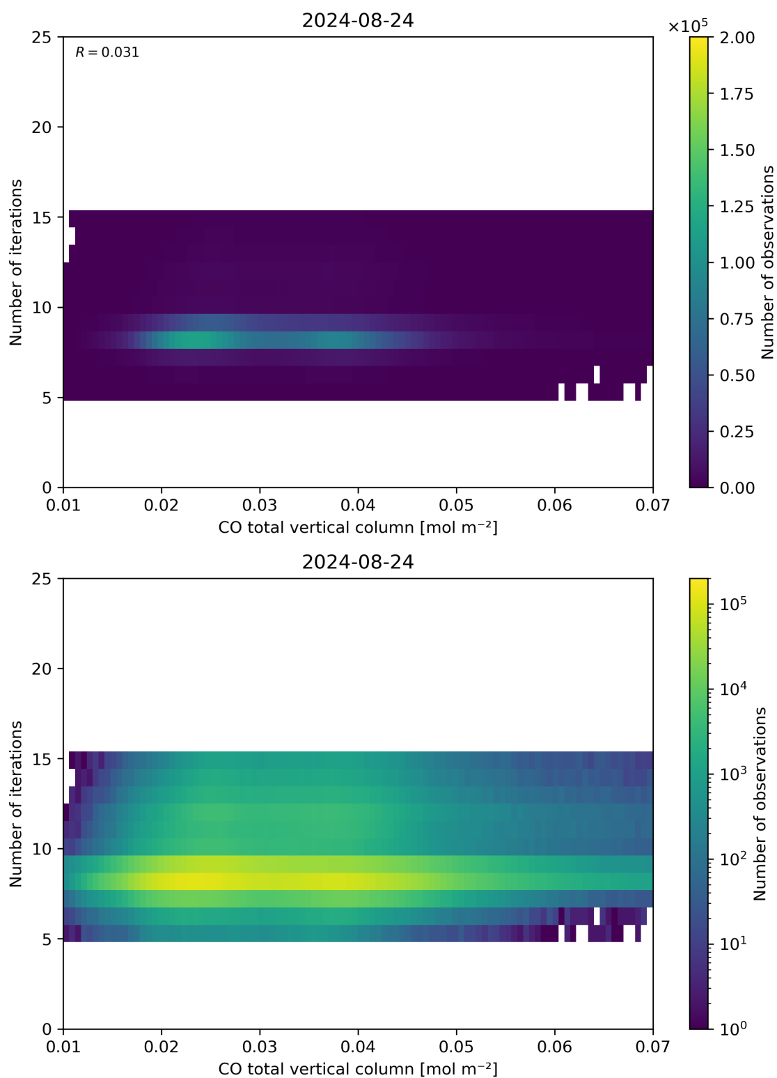
Figure 42: Scatter density plot of “CO total vertical column” against “Number of iterations” for 2024-08-23 to 2024-08-25.
