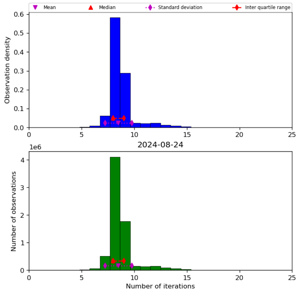
Figure 24: Histogram of “Number of iterations” for 2024-08-23 to 2024-08-25
