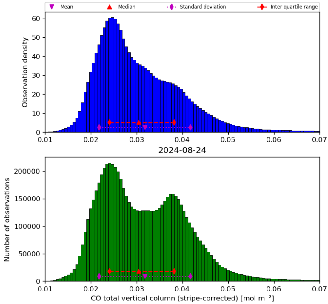
Figure 19: Histogram of “CO total vertical column (stripe-corrected)” for 2024-08-23 to 2024-08-25
