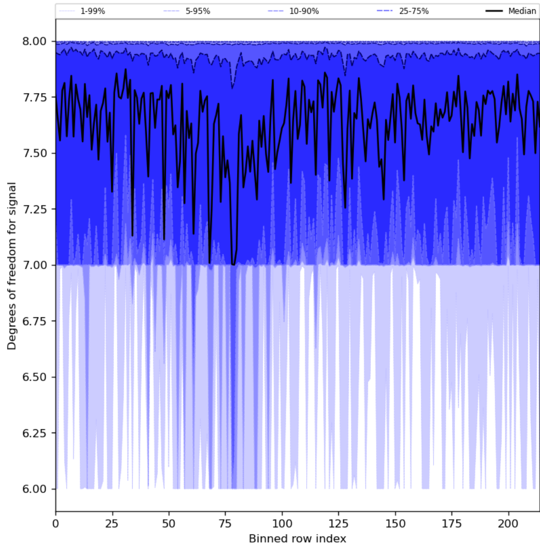
Figure 31: Along track statistics of “Degrees of freedom for signal” for 2024-08-23 to 2024-08-25
