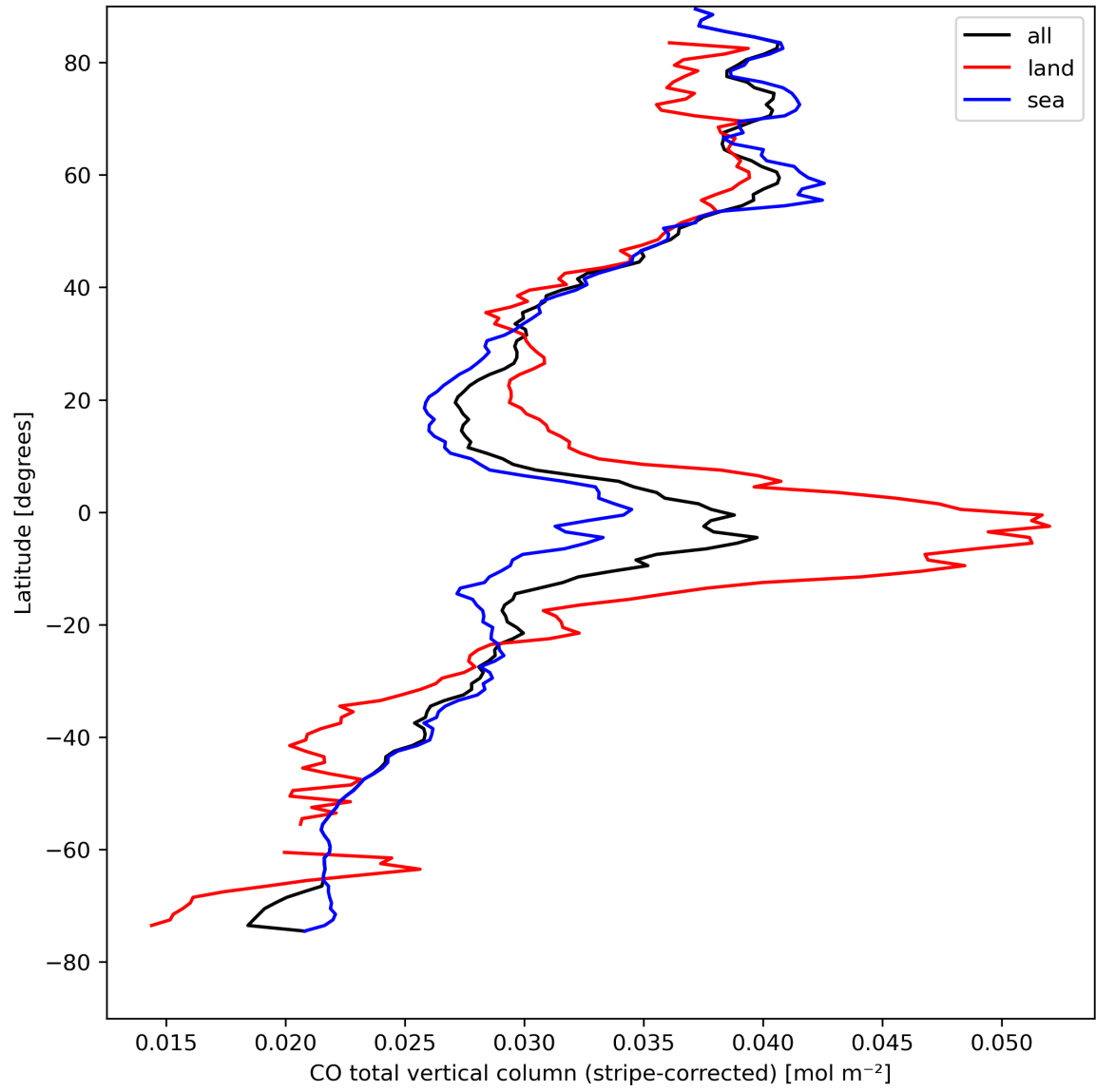
Figure 11: Zonal average of “CO total vertical column (stripe-corrected)” for 2024-08-23 to 2024-08-25.
