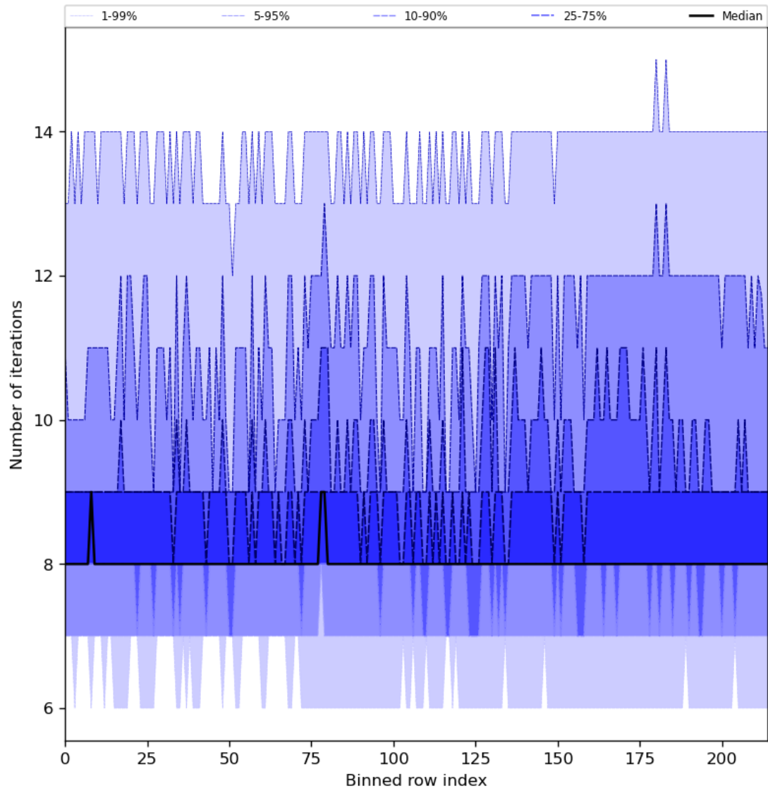
Figure 32: Along track statistics of “Number of iterations” for 2024-08-23 to 2024-08-25
