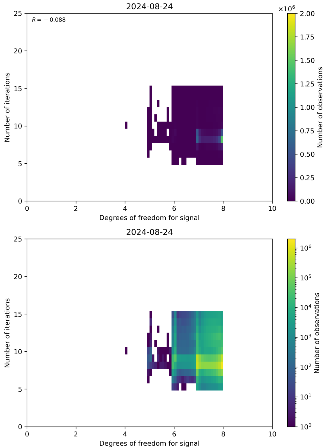
Figure 50: Scatter density plot of “Degrees of freedom for signal” against “Number of iterations” for 2024-08-23 to 2024-08-25.
