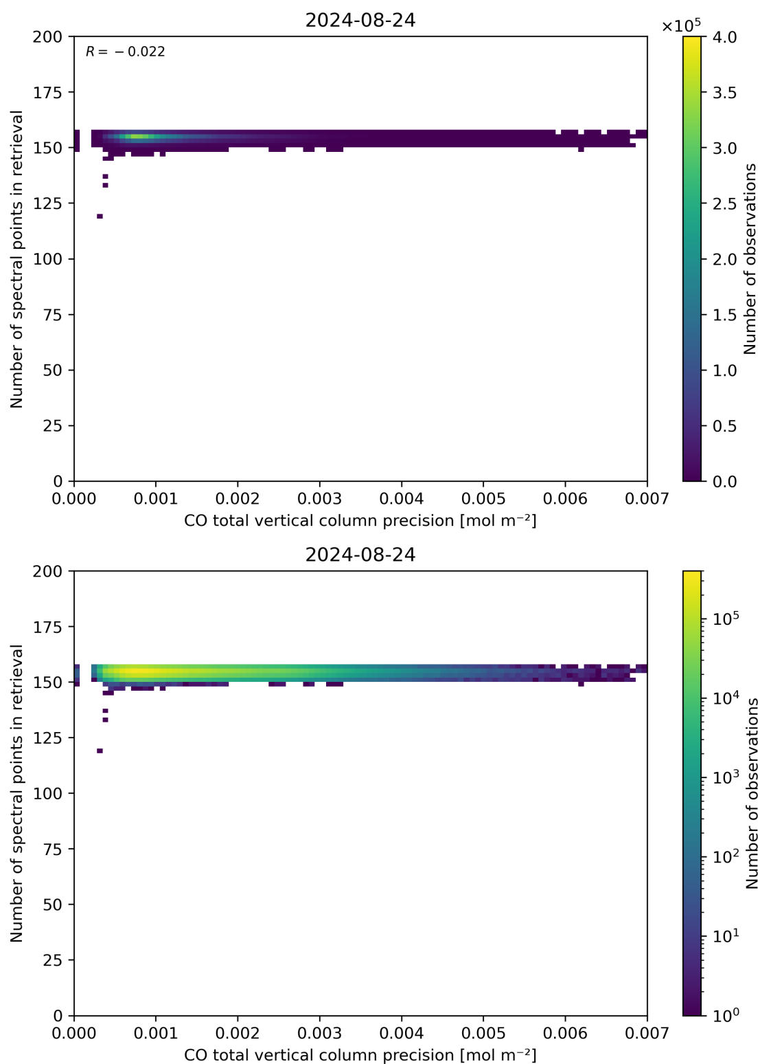
Figure 47: Scatter density plot of “CO total vertical column precision” against “Number of spectral points in retrieval” for 2024-08-23 to 2024-08-25.
