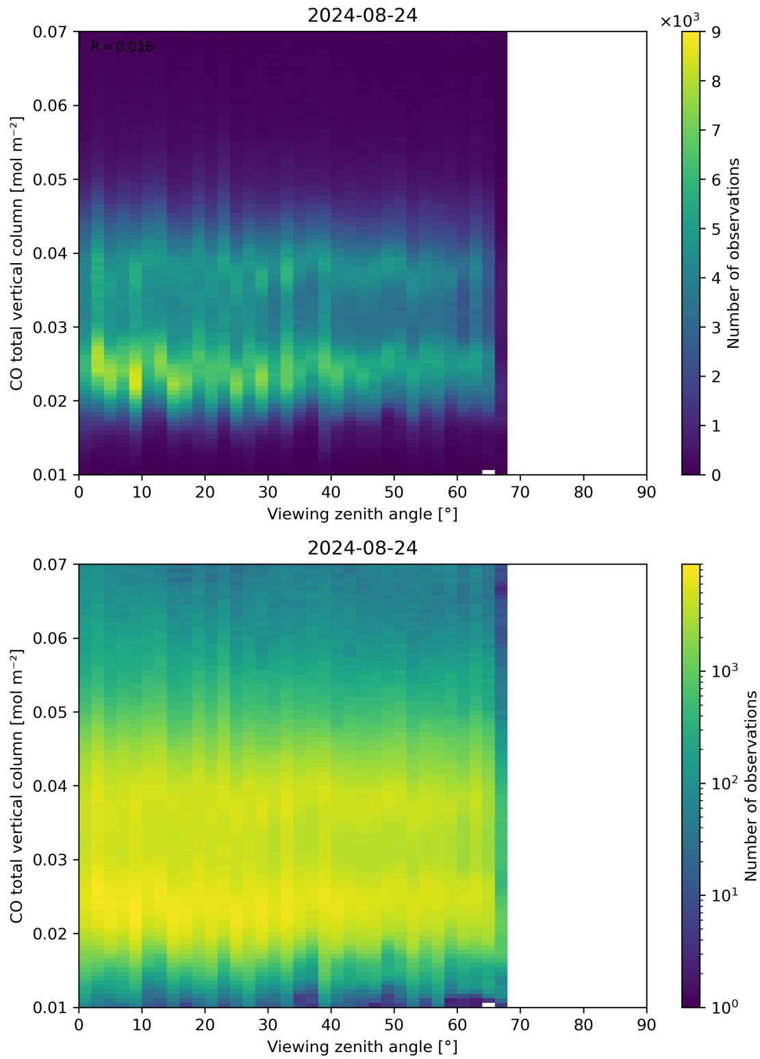
Figure 69: Scatter density plot of “Viewing zenith angle” against “CO total vertical column” for 2024-08-23 to 2024-08-25.
