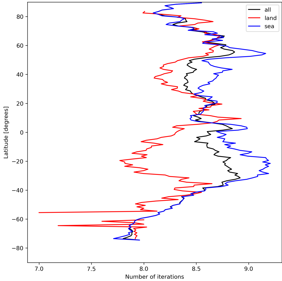
Figure 16: Zonal average of “Number of iterations” for 2024-08-23 to 2024-08-25.
