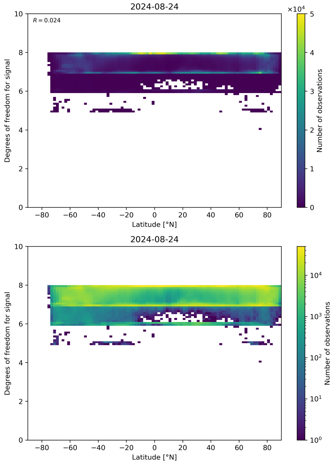
Figure 55: Scatter density plot of “Latitude” against “Degrees of freedom for signal” for 2024-08-23 to 2024-08-25.
