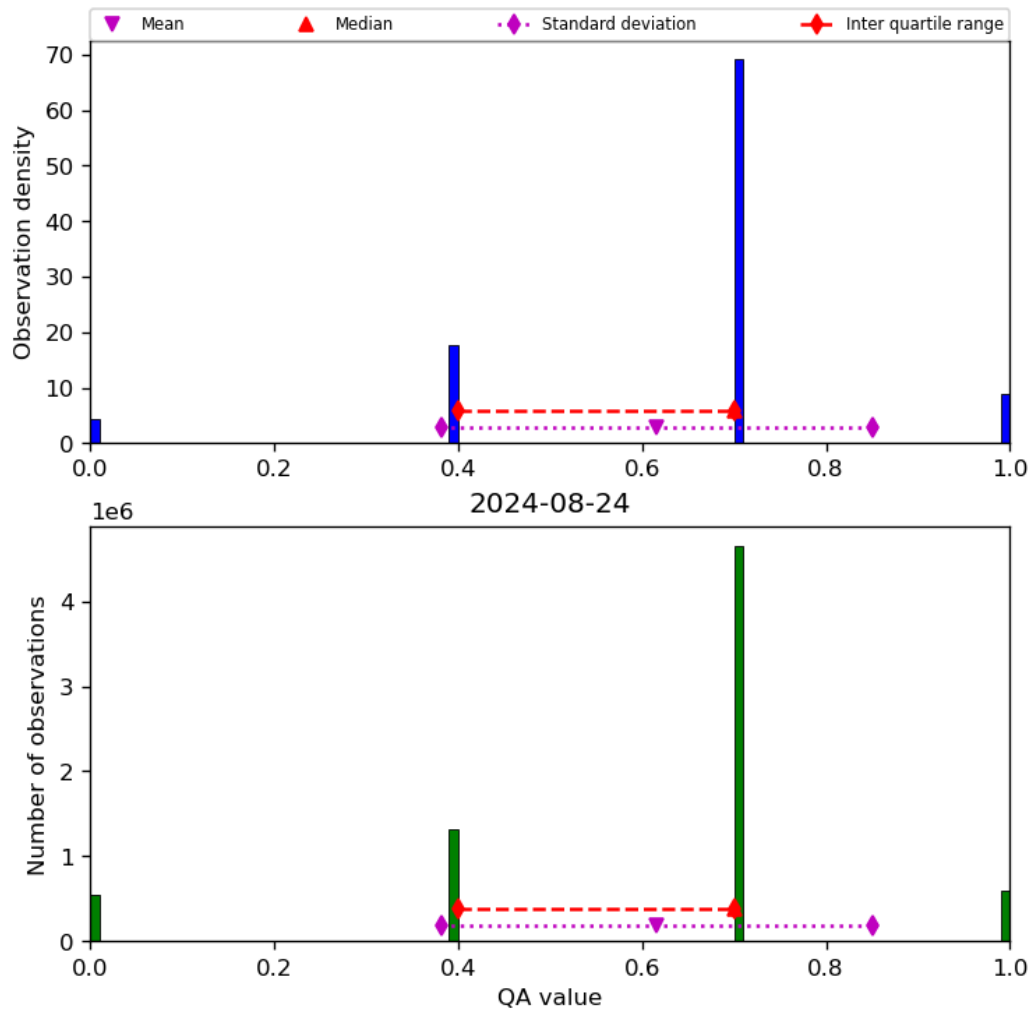
Figure 17: Histogram of “QA value” for 2024-08-23 to 2024-08-25
