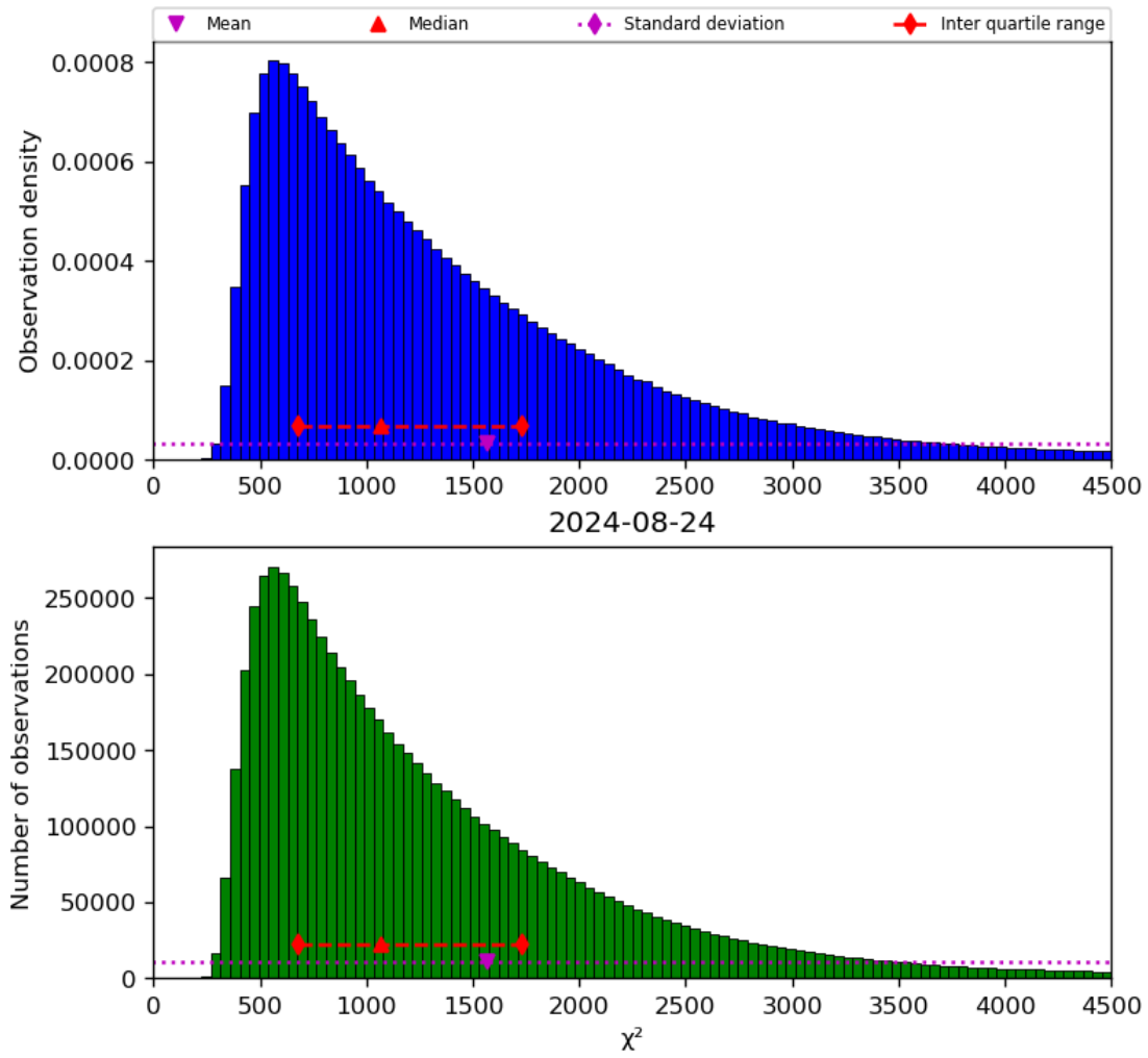
Figure 22: Histogram of “ \chi^2 ” for 2024-08-23 to 2024-08-25
