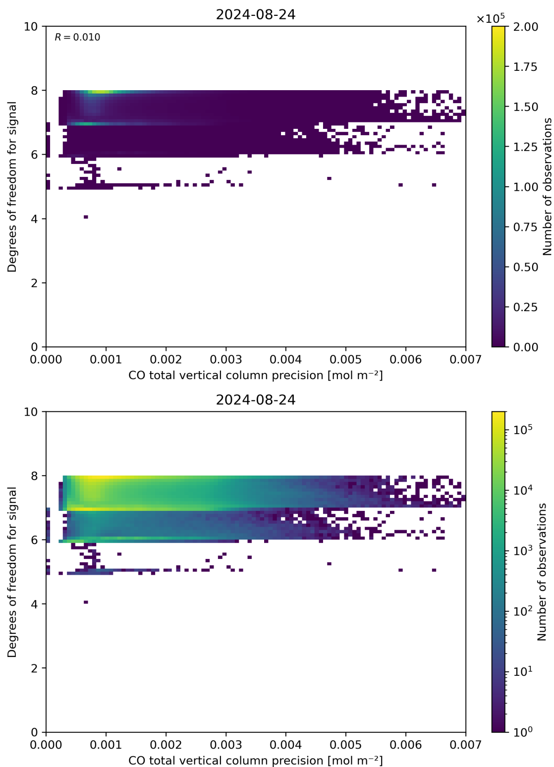
Figure 45: Scatter density plot of “CO total vertical column precision” against “Degrees of freedom for signal” for 2024-08-23 to 2024-08-25.
