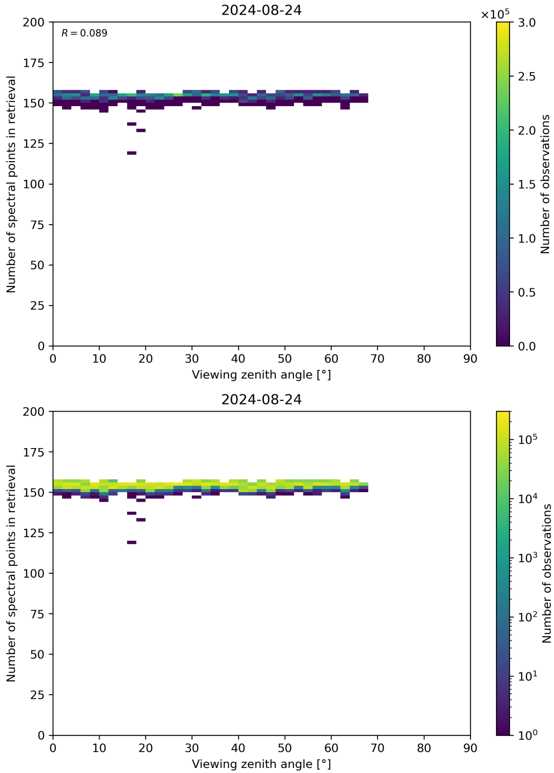
Figure 76: Scatter density plot of “Viewing zenith angle” against “Number of spectral points in retrieval” for 2024-08-23 to 2024-08-25.
