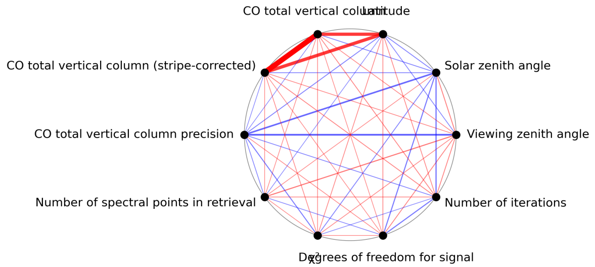
Figure 1: Map of correlation graph for 2024-08-23 to 2024-08-25.
