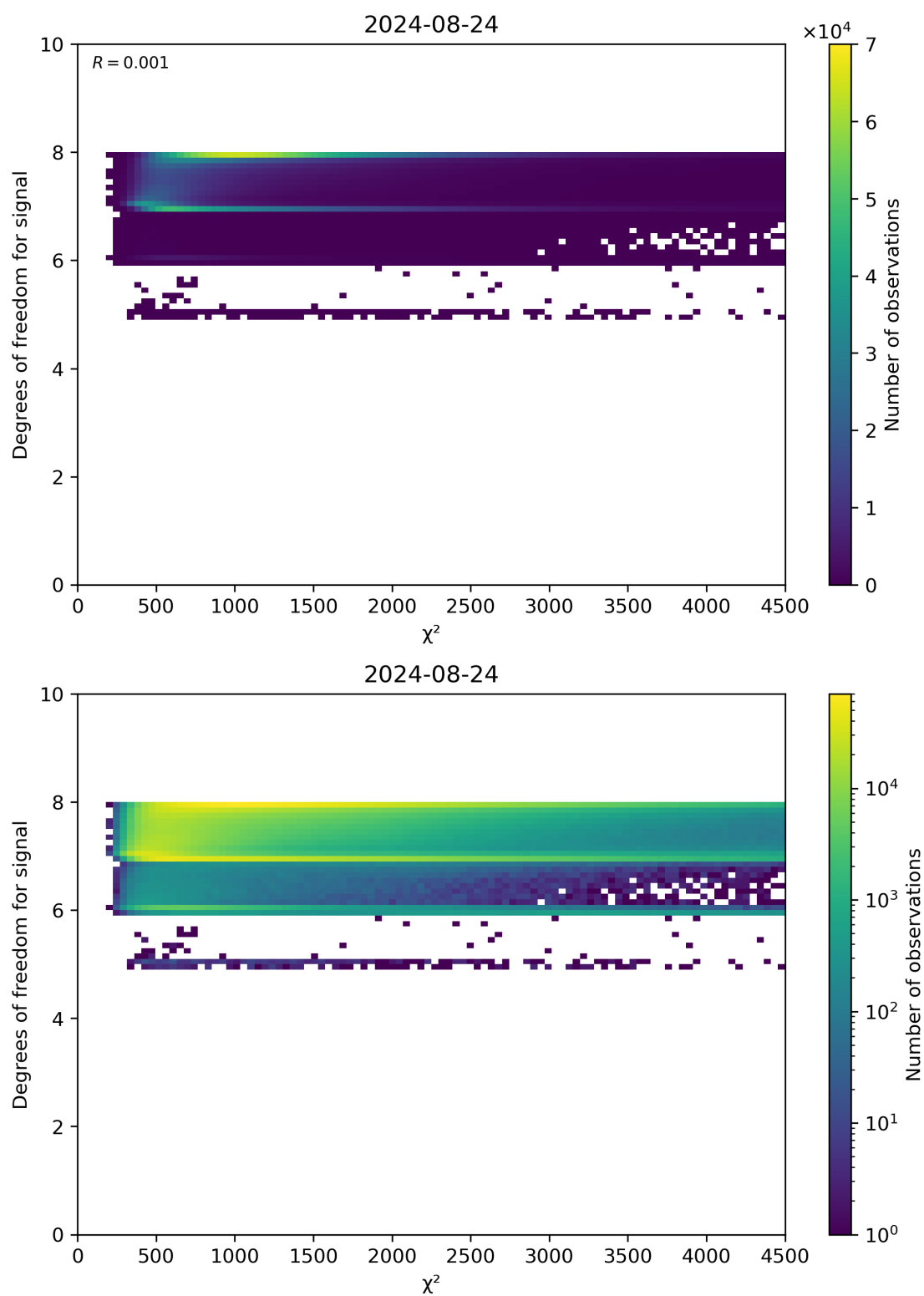
Figure 48: Scatter density plot of “ \chi^2 ” against “Degrees of freedom for signal” for 2024-08-23 to 2024-08-25.
