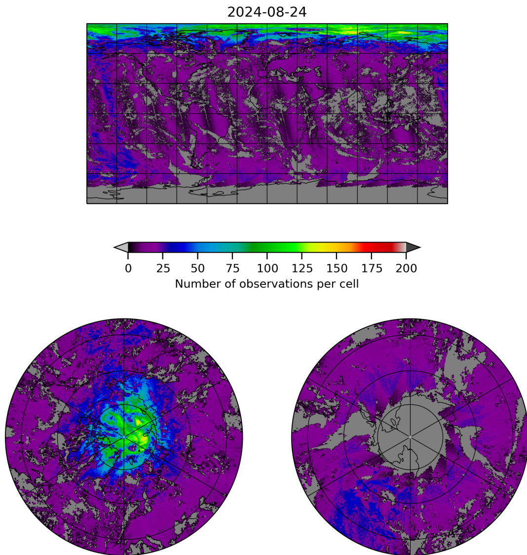
Figure 8: Map of the number of observations for 2024-08-23 to 2024-08-25
