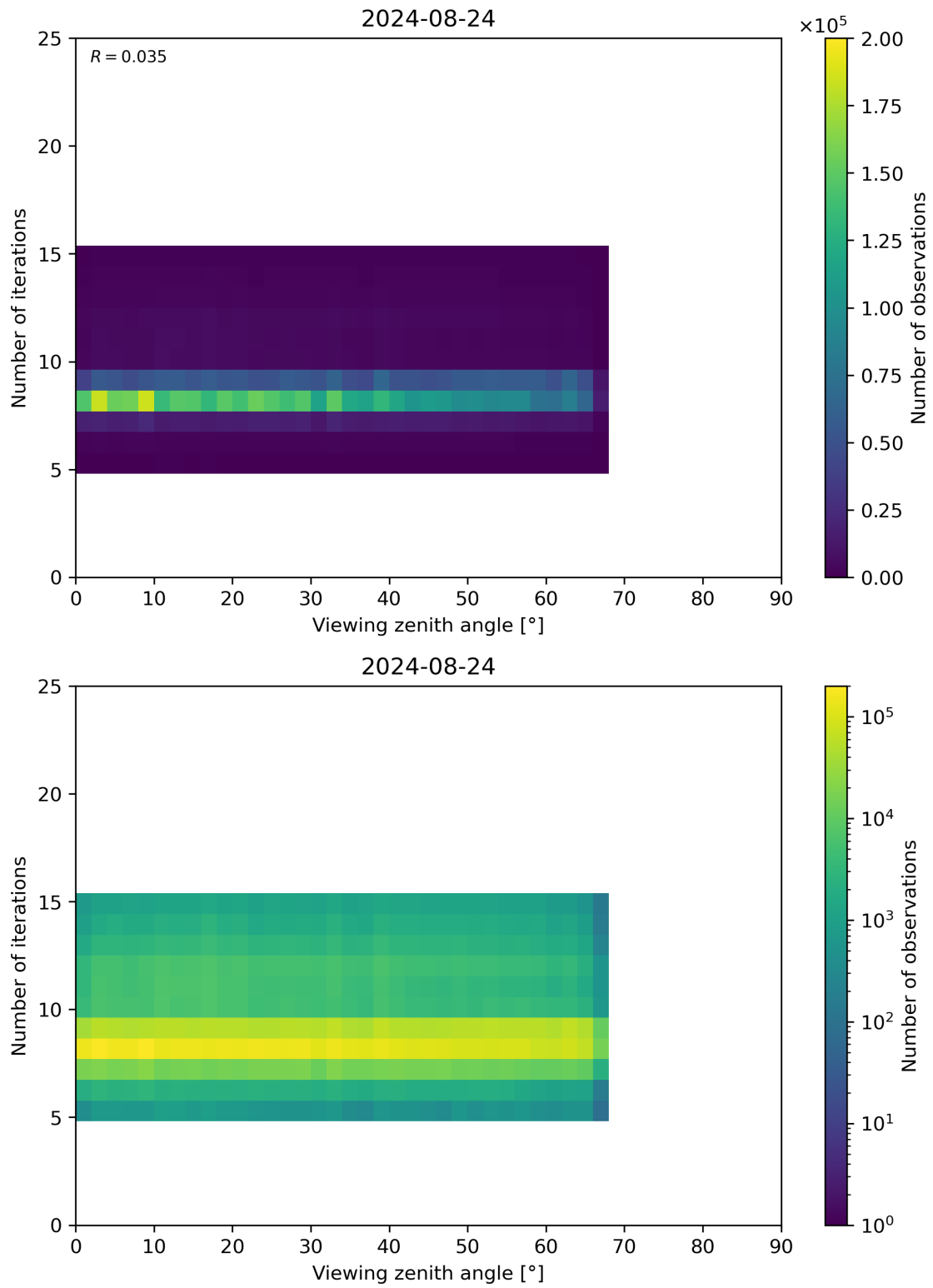
Figure 75: Scatter density plot of “Viewing zenith angle” against “Number of iterations” for 2024-08-23 to 2024-08-25.
