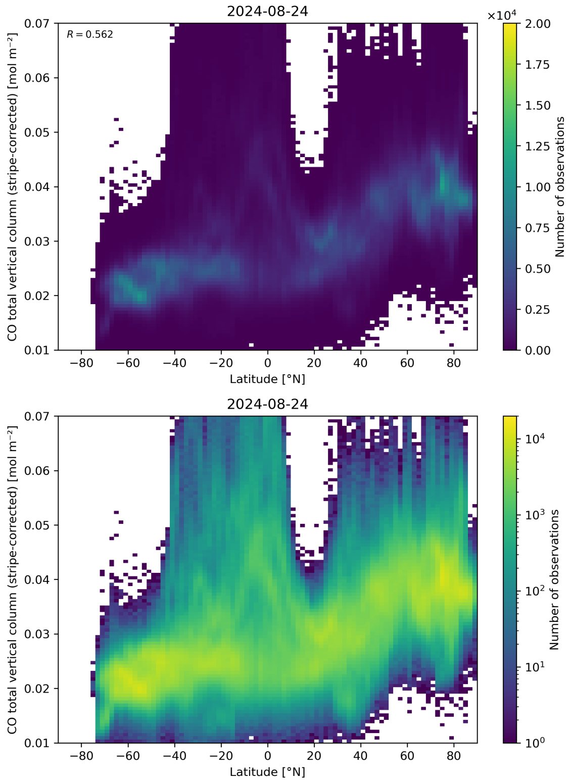
Figure 52: Scatter density plot of “Latitude” against “CO total vertical column (stripe-corrected)” for 2024-08-23 to 2024-08-25.
