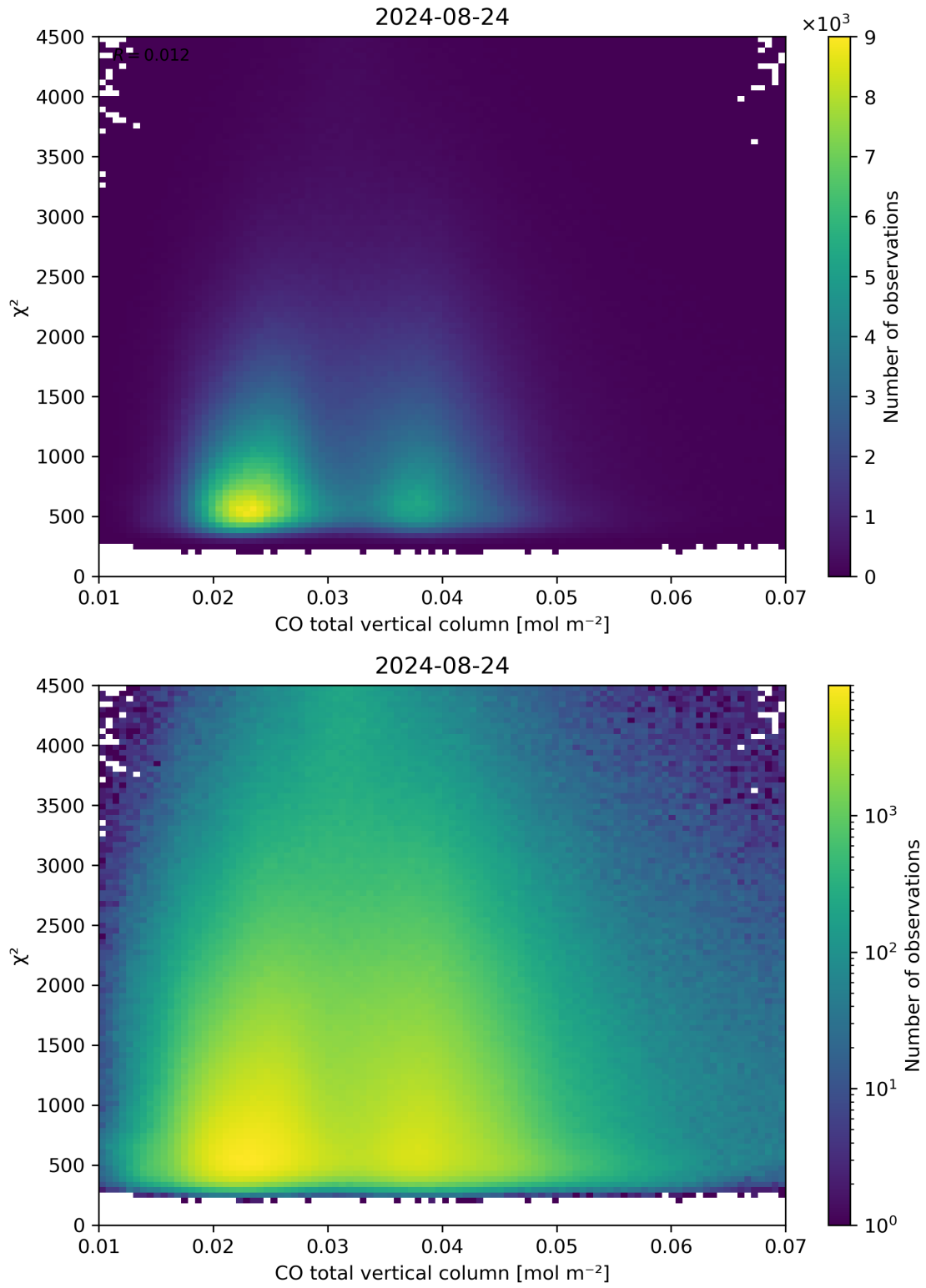
Figure 35: Scatter density plot of “CO total vertical column” against “ \chi^2 ” for 2024-08-23 to 2024-08-25.
