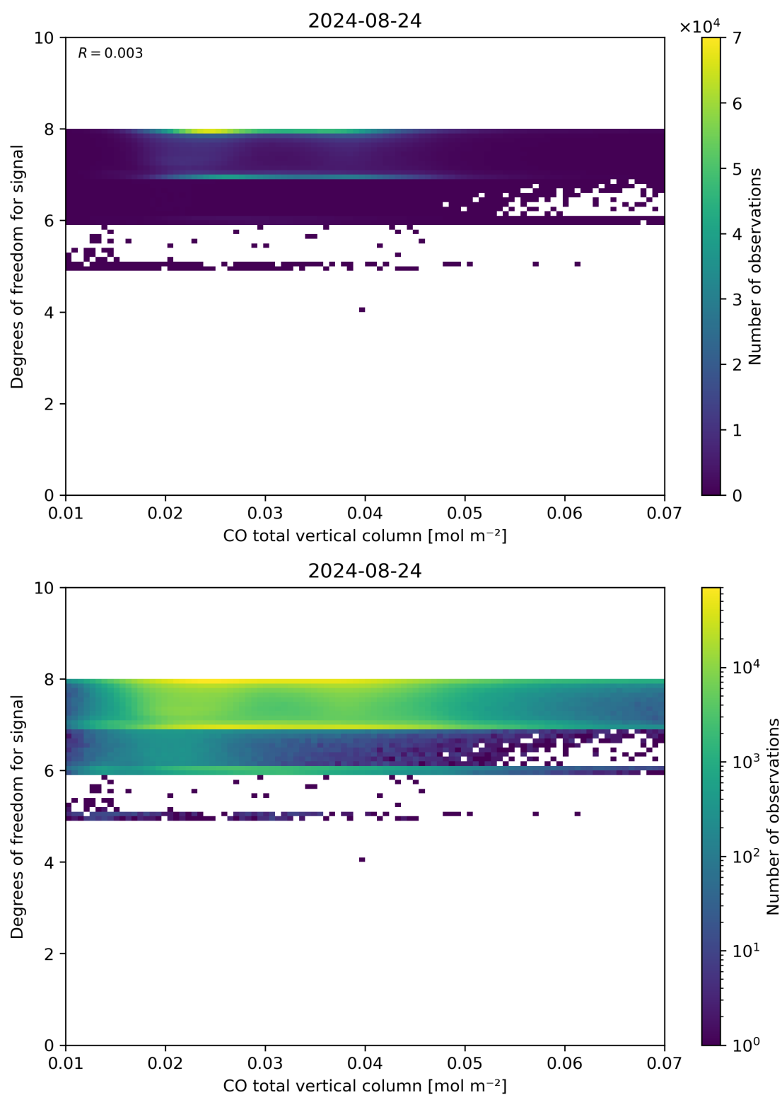
Figure 41: Scatter density plot of “CO total vertical column” against “Degrees of freedom for signal” for 2024-08-23 to 2024-08-25.
