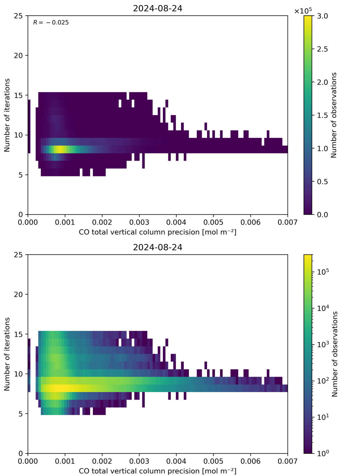
Figure 46: Scatter density plot of “CO total vertical column precision” against “Number of iterations” for 2024-08-23 to 2024-08-25.
