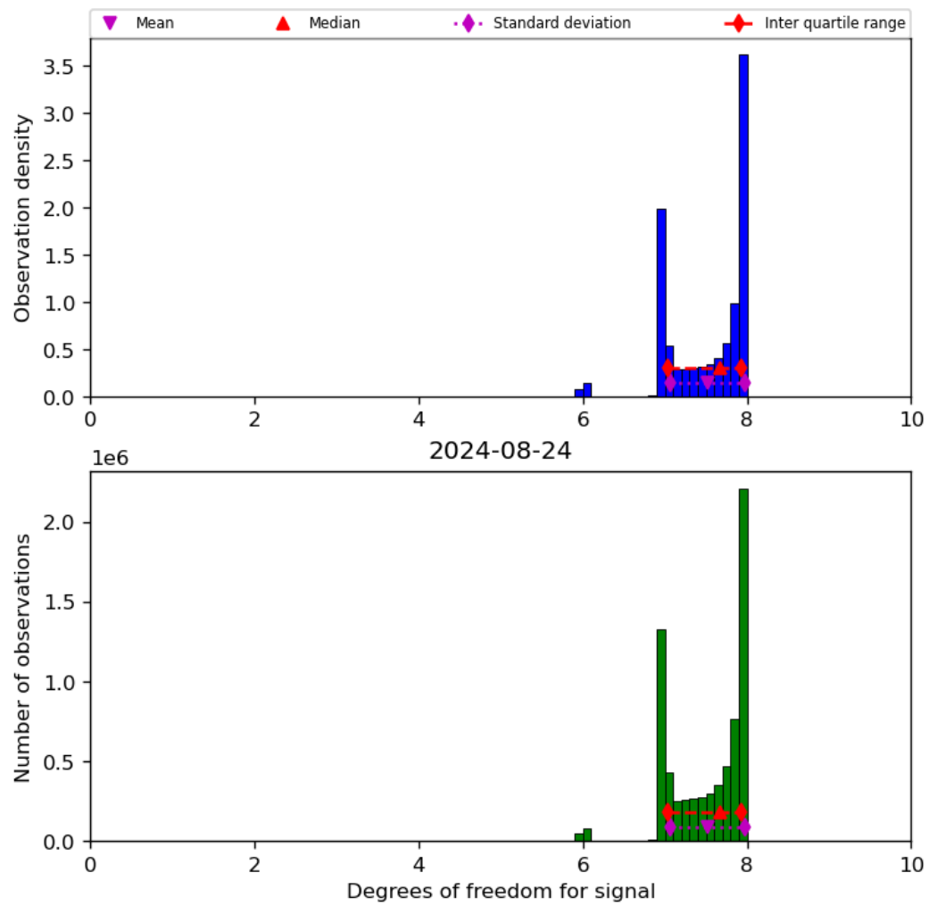
Figure 23: Histogram of “Degrees of freedom for signal” for 2024-08-23 to 2024-08-25
