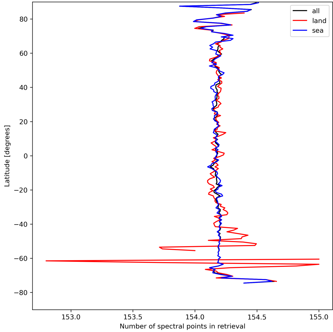
Figure 13: Zonal average of “Number of spectral points in retrieval” for 2024-08-23 to 2024-08-25.
