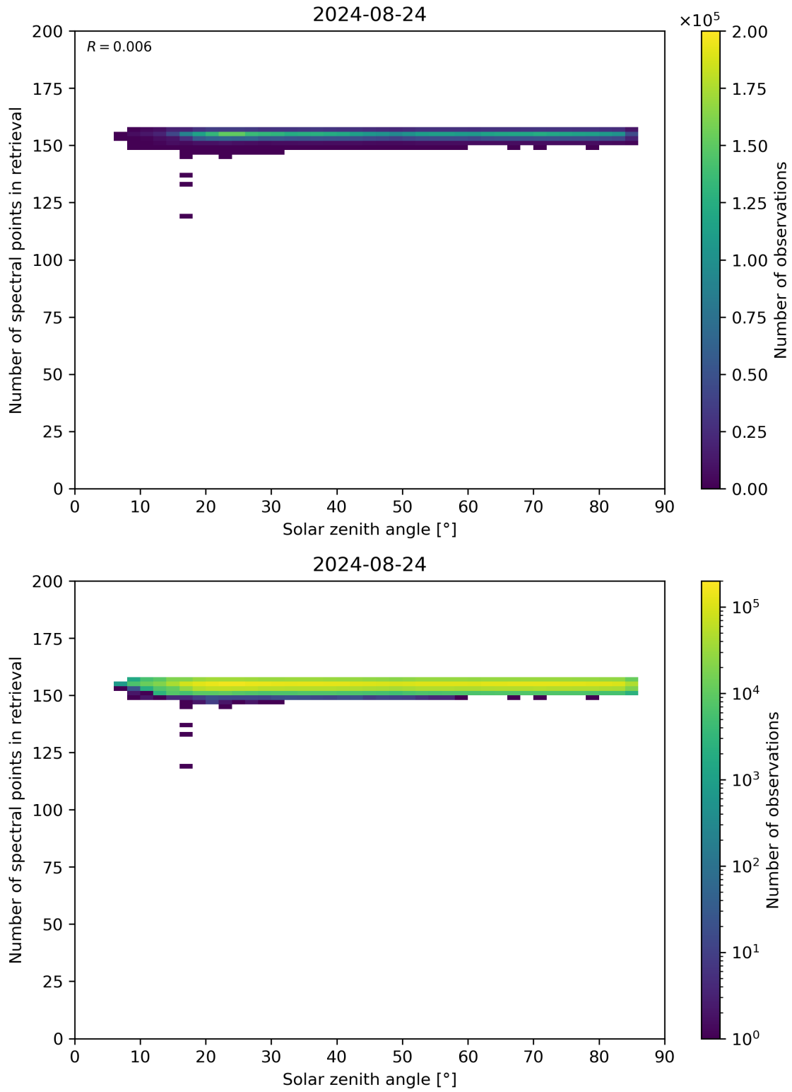
Figure 68: Scatter density plot of “Solar zenith angle” against “Number of spectral points in retrieval” for 2024-08-23 to 2024-08-25.
