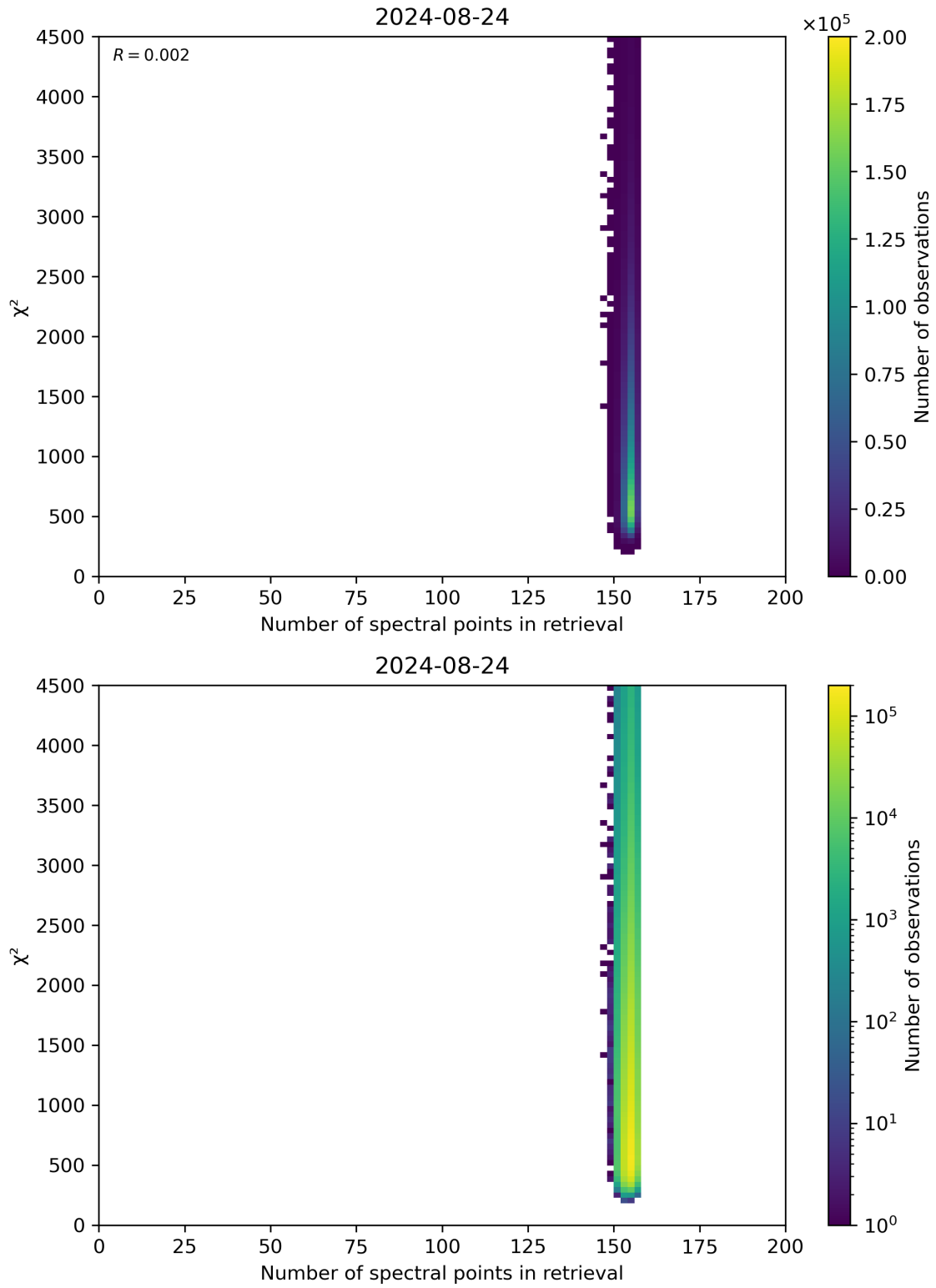
Figure 58: Scatter density plot of “Number of spectral points in retrieval” against “ \chi^2 ” for 2024-08-23 to 2024-08-25.
