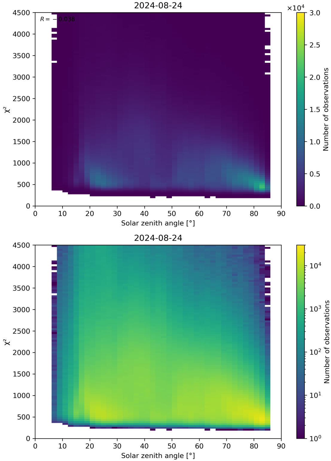
Figure 64: Scatter density plot of “Solar zenith angle” against “ \chi^2 ” for 2024-08-23 to 2024-08-25.
