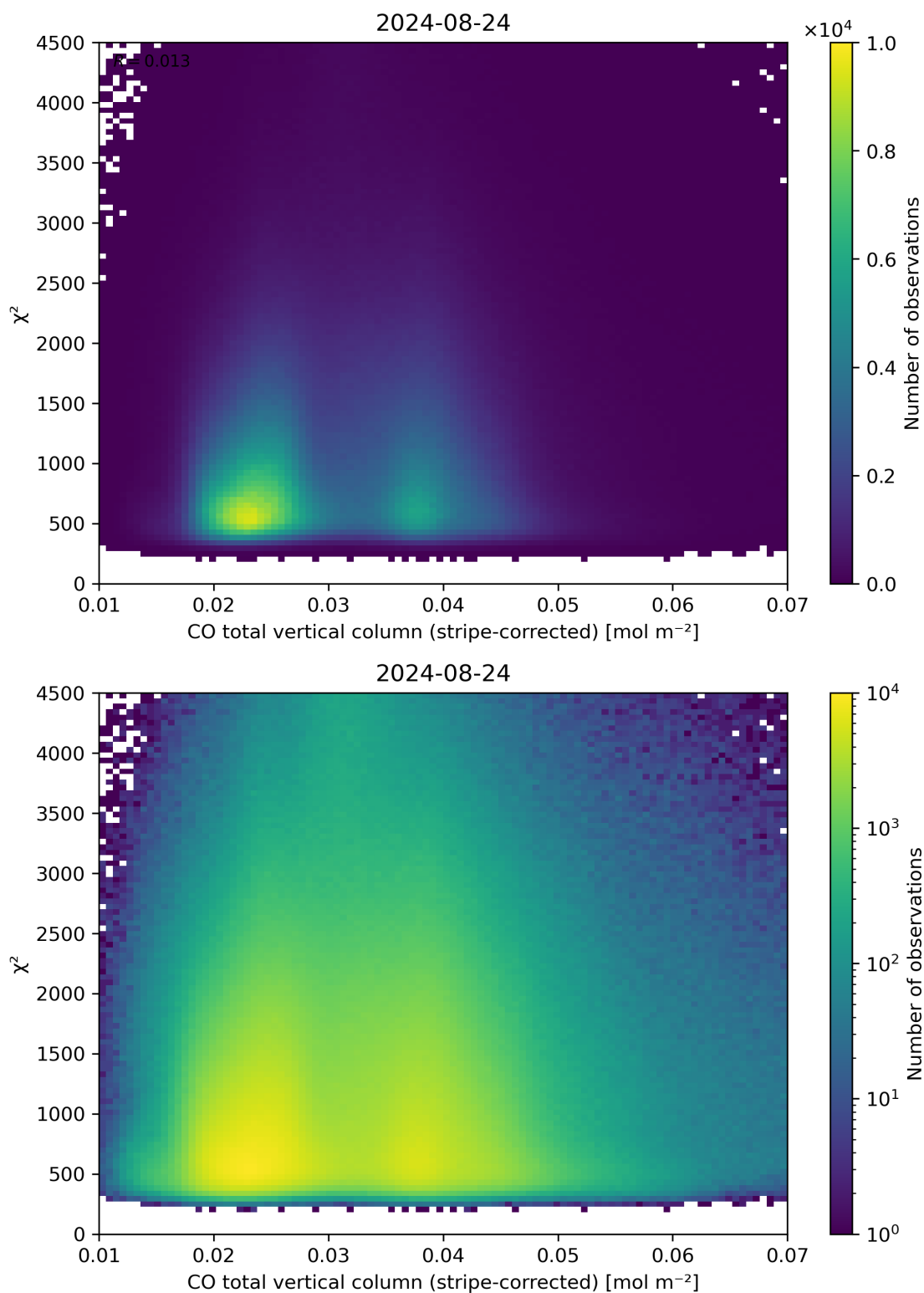
Figure 37: Scatter density plot of “CO total vertical column (stripe-corrected)” against “ \chi^2 ” for 2024-08-23 to 2024-08-25.
