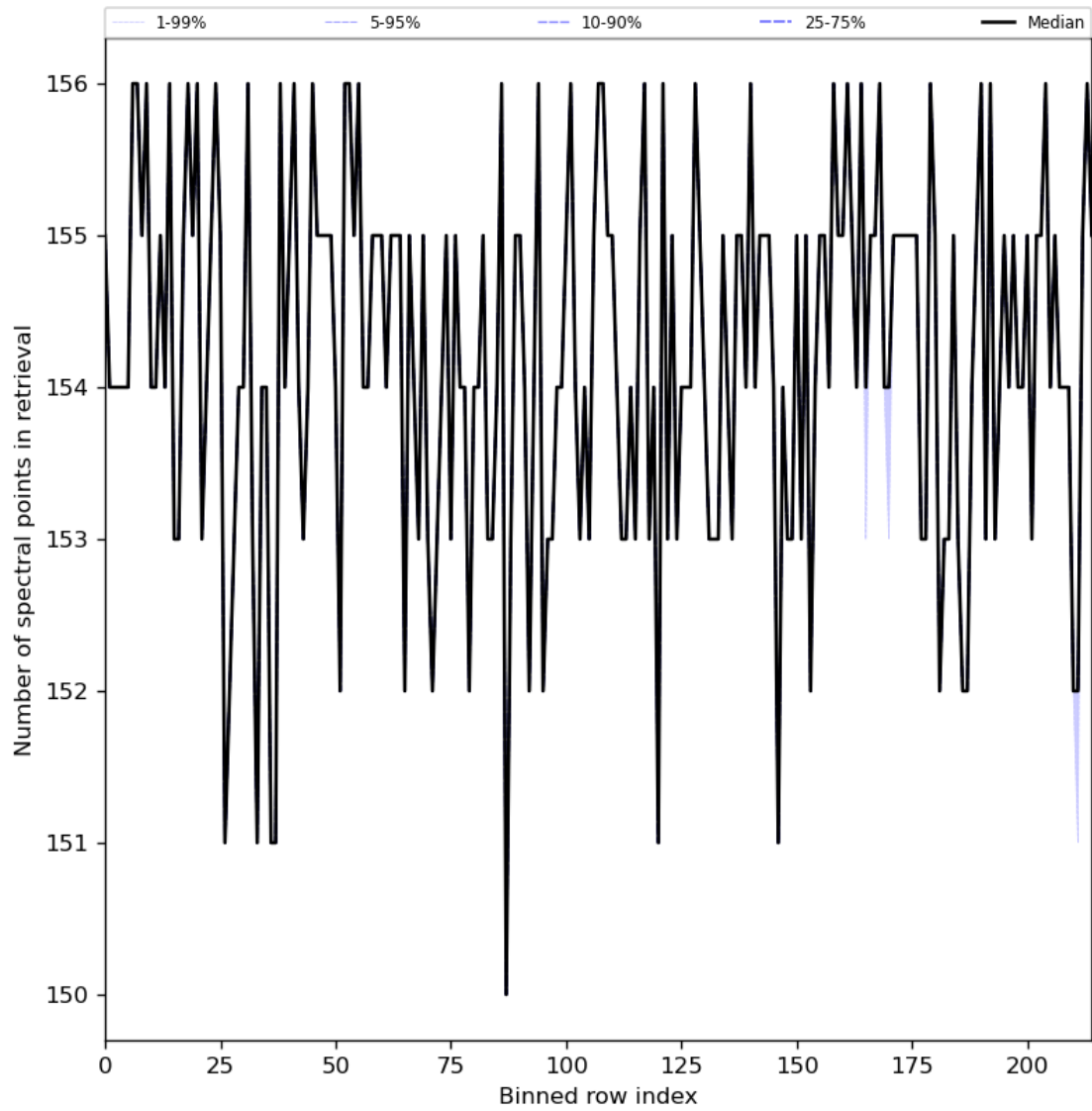
Figure 29: Along track statistics of “Number of spectral points in retrieval” for 2024-08-23 to 2024-08-25
