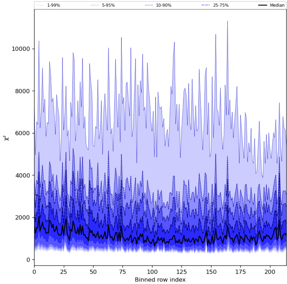
Figure 30: Along track statistics of “ \chi^2 ” for 2024-08-23 to 2024-08-25
