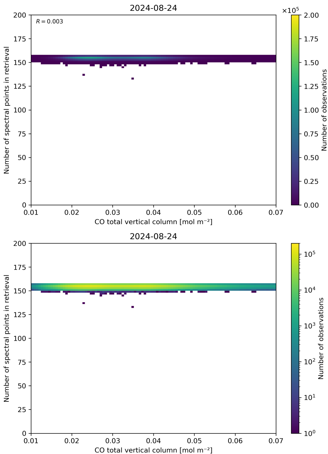
Figure 43: Scatter density plot of “CO total vertical column” against “Number of spectral points in retrieval” for 2024-08-23 to 2024-08-25.
