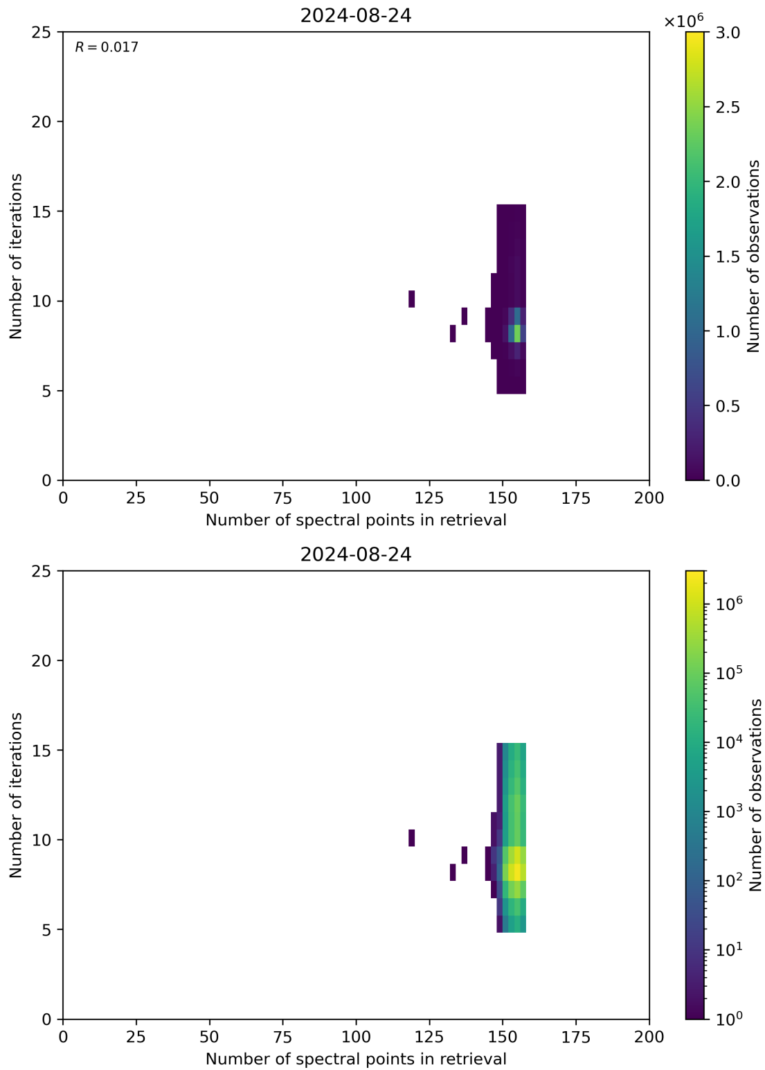
Figure 60: Scatter density plot of “Number of spectral points in retrieval” against “Number of iterations” for 2024-08-23 to 2024-08-25.
