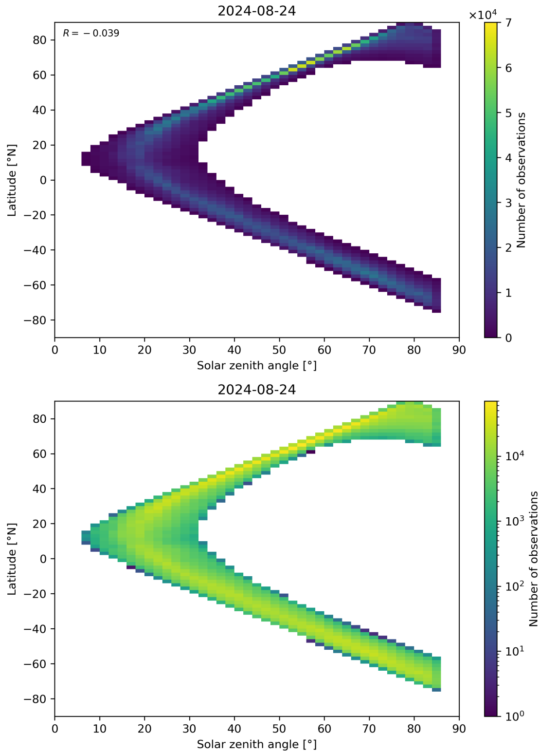
Figure 66: Scatter density plot of “Solar zenith angle” against “Latitude” for 2024-08-23 to 2024-08-25.
