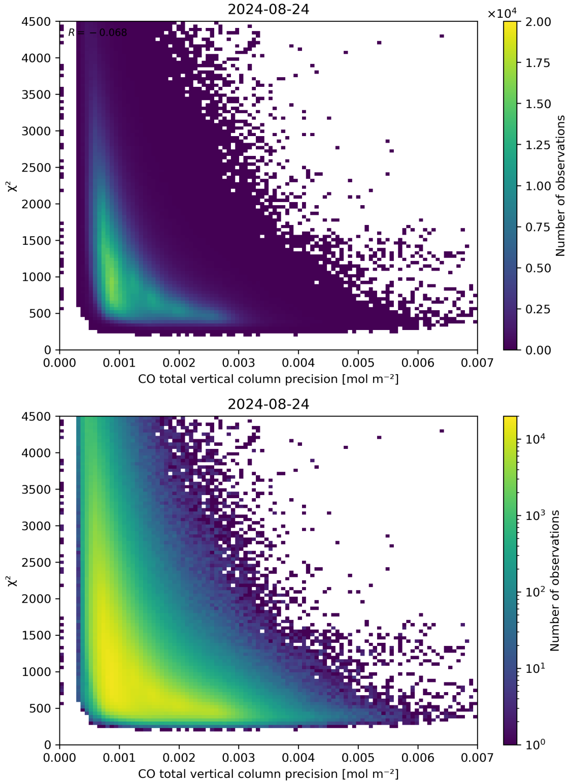
Figure 44: Scatter density plot of “CO total vertical column precision” against “ \chi^2 ” for 2024-08-23 to 2024-08-25.
