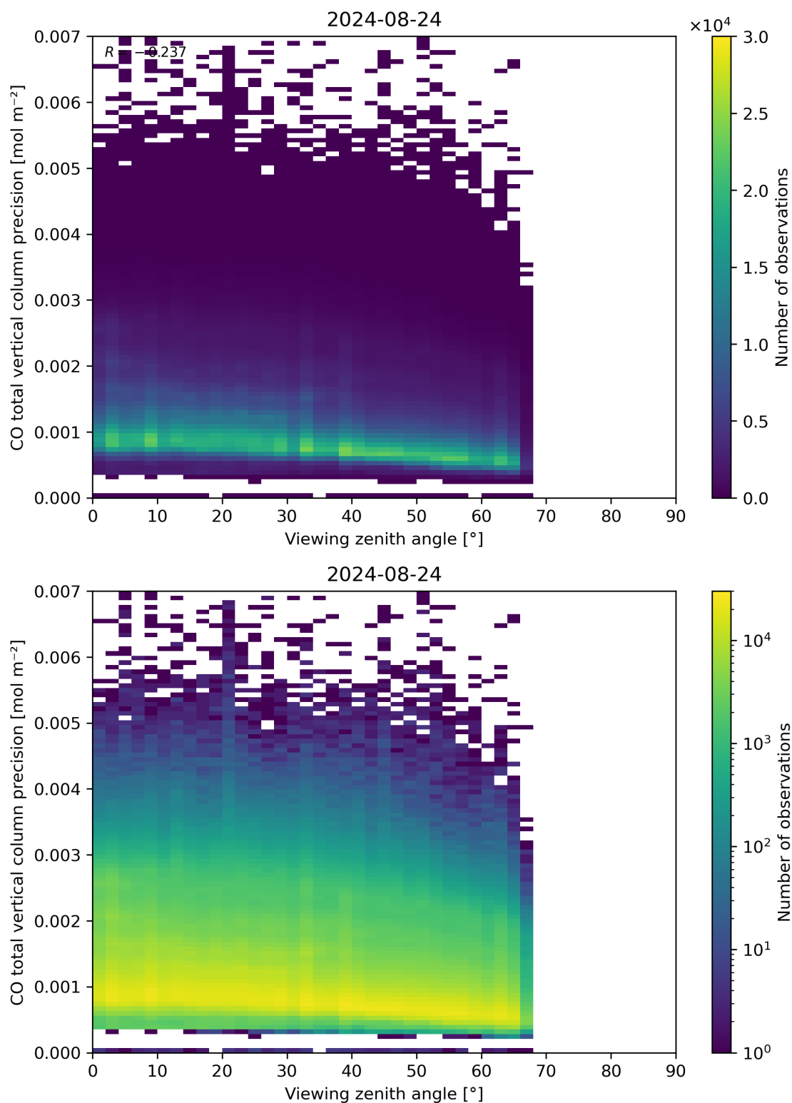
Figure 71: Scatter density plot of “Viewing zenith angle” against “CO total vertical column precision” for 2024-08-23 to 2024-08-25.
