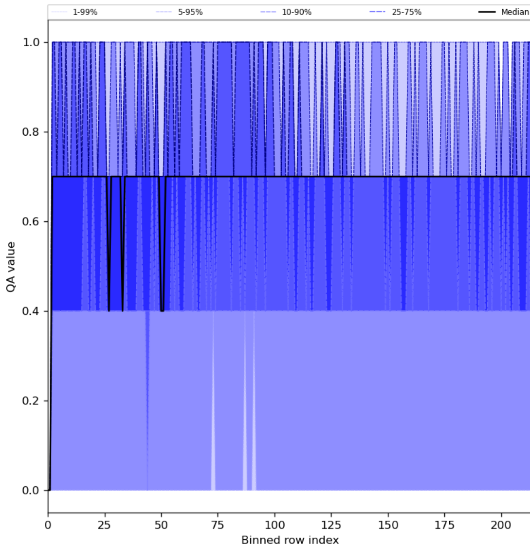
Figure 25: Along track statistics of “QA value” for 2024-08-23 to 2024-08-25
