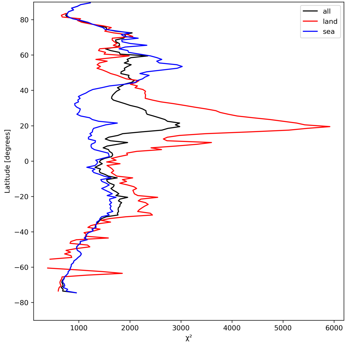
Figure 14: Zonal average of “ \chi^2 ” for 2024-08-23 to 2024-08-25.
