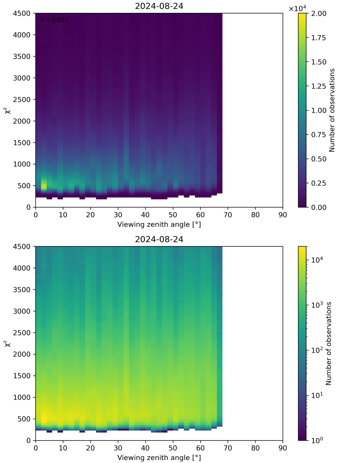
Figure 72: Scatter density plot of “Viewing zenith angle” against “ \chi^2 ” for 2024-08-23 to 2024-08-25.
