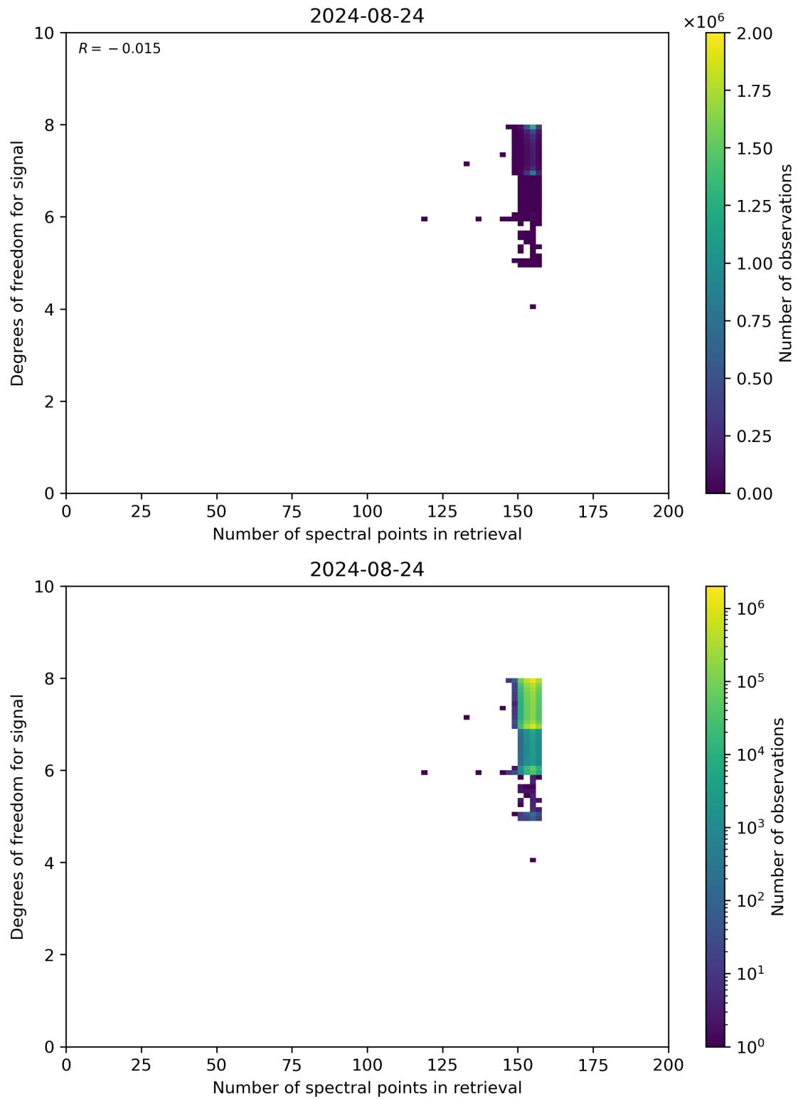
Figure 59: Scatter density plot of “Number of spectral points in retrieval” against “Degrees of freedom for signal” for 2024-08-23 to 2024-08-25.
