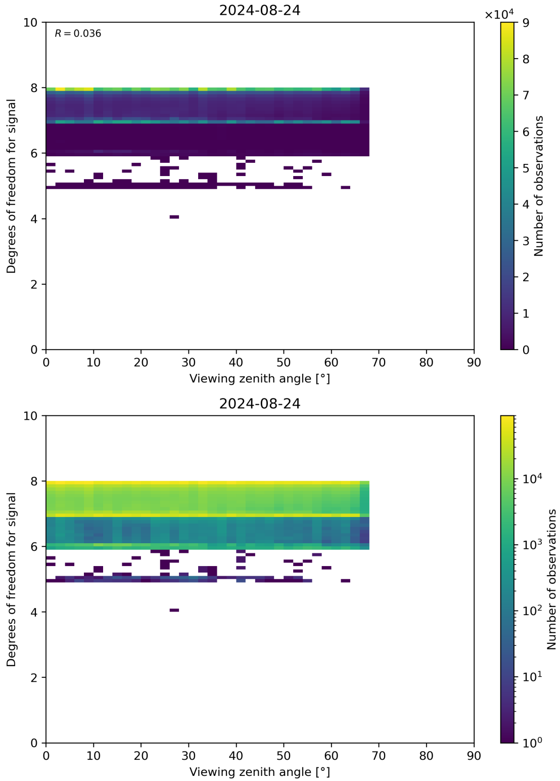
Figure 73: Scatter density plot of “Viewing zenith angle” against “Degrees of freedom for signal” for 2024-08-23 to 2024-08-25.
