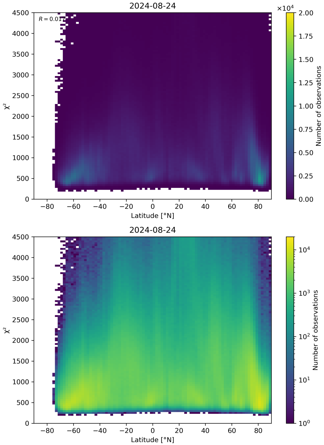
Figure 54: Scatter density plot of “Latitude” against “ \chi^2 ” for 2024-08-23 to 2024-08-25.
