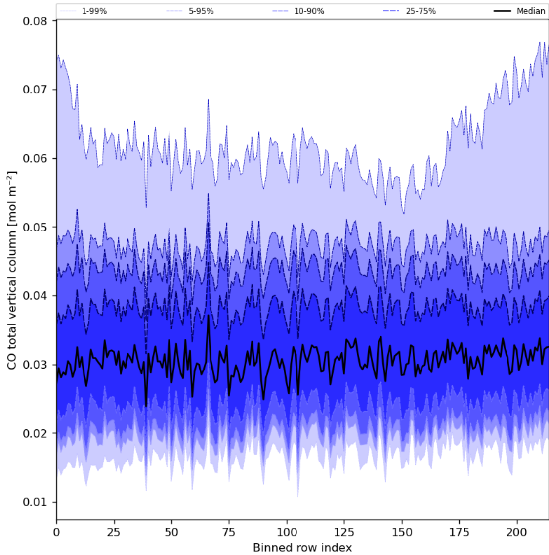
Figure 26: Along track statistics of “CO total vertical column” for 2024-08-23 to 2024-08-25
