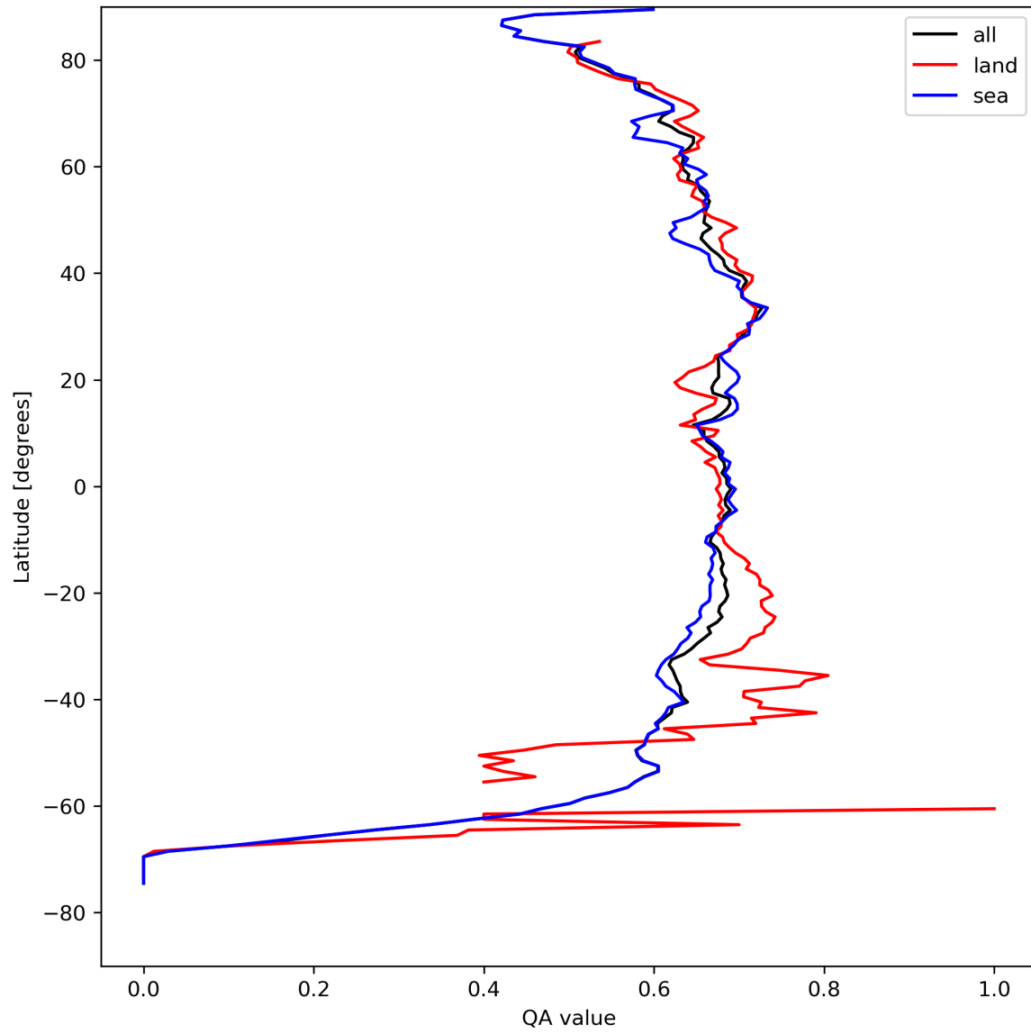
Figure 9: Zonal average of “QA value” for 2024-08-23 to 2024-08-25.
