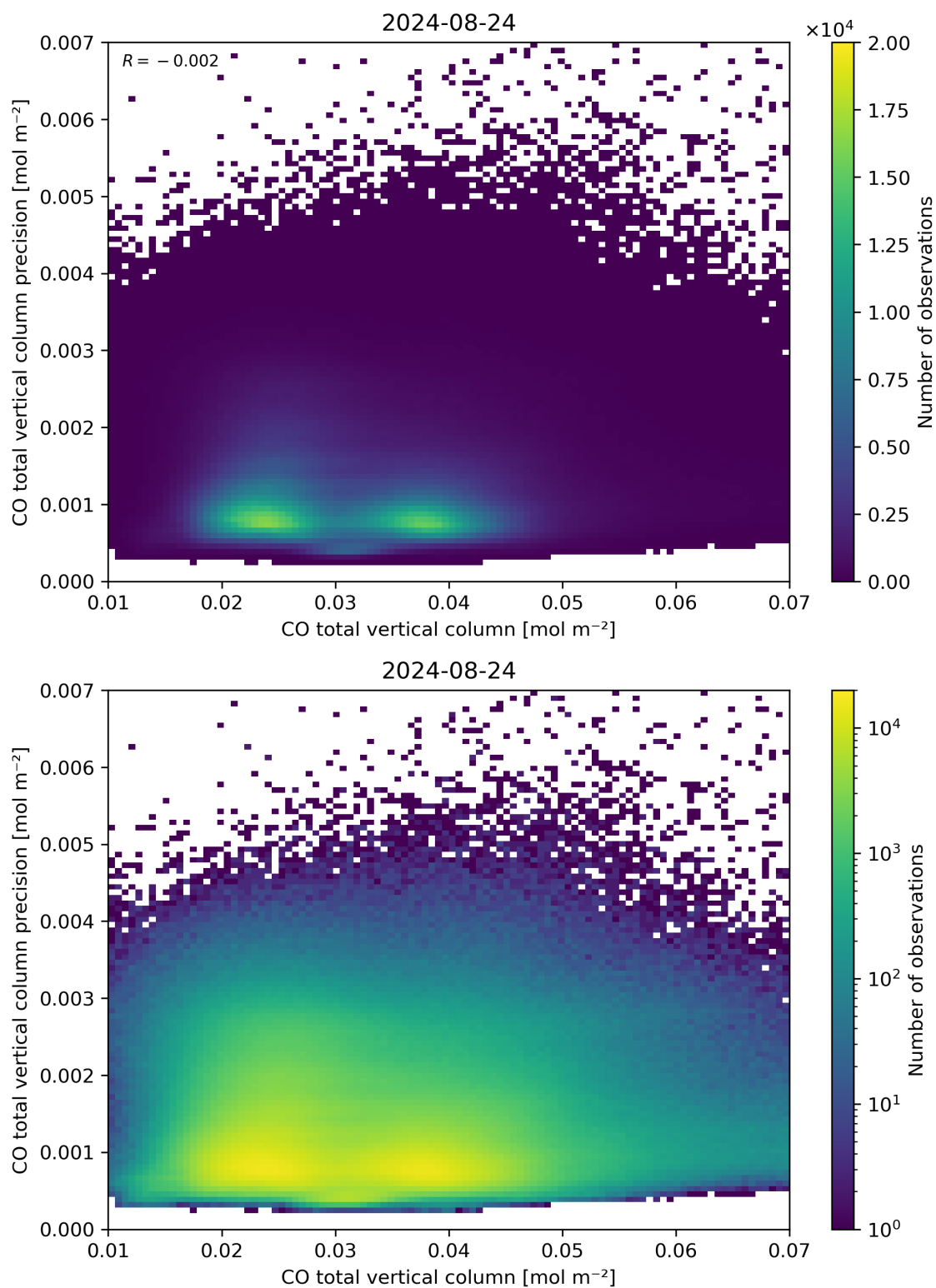
Figure 34: Scatter density plot of “CO total vertical column” against “CO total vertical column precision” for 2024-08-23 to 2024-08-25.
