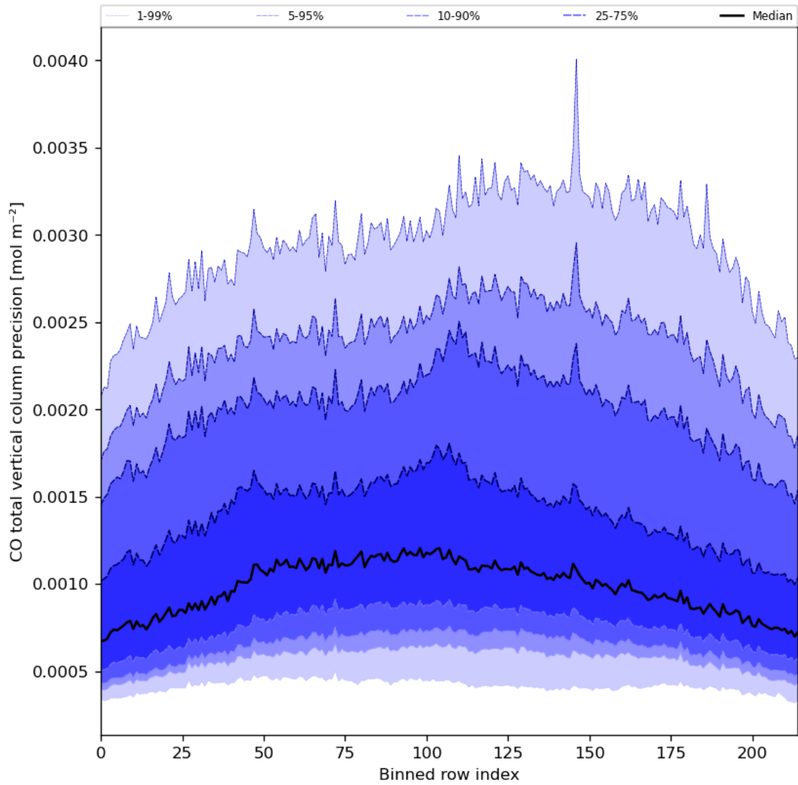
Figure 28: Along track statistics of “CO total vertical column precision” for 2024-08-23 to 2024-08-25
