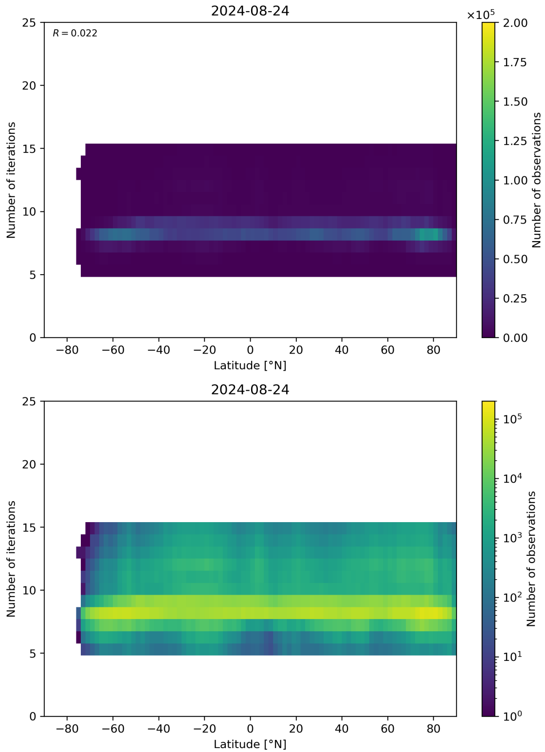
Figure 56: Scatter density plot of “Latitude” against “Number of iterations” for 2024-08-23 to 2024-08-25.
