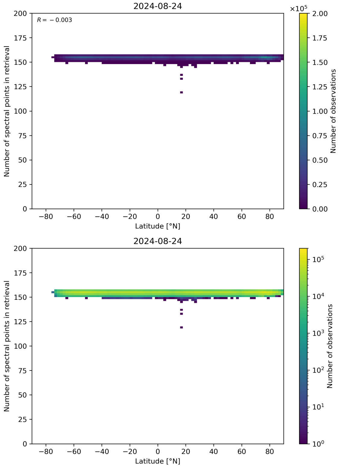
Figure 57: Scatter density plot of “Latitude” against “Number of spectral points in retrieval” for 2024-08-23 to 2024-08-25.
