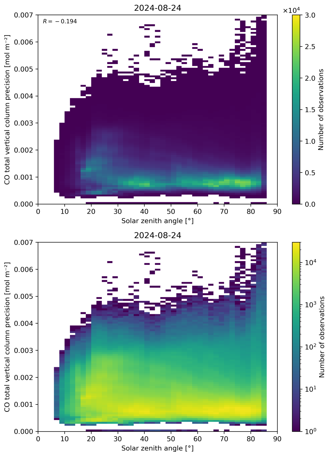
Figure 63: Scatter density plot of “Solar zenith angle” against “CO total vertical column precision” for 2024-08-23 to 2024-08-25.
