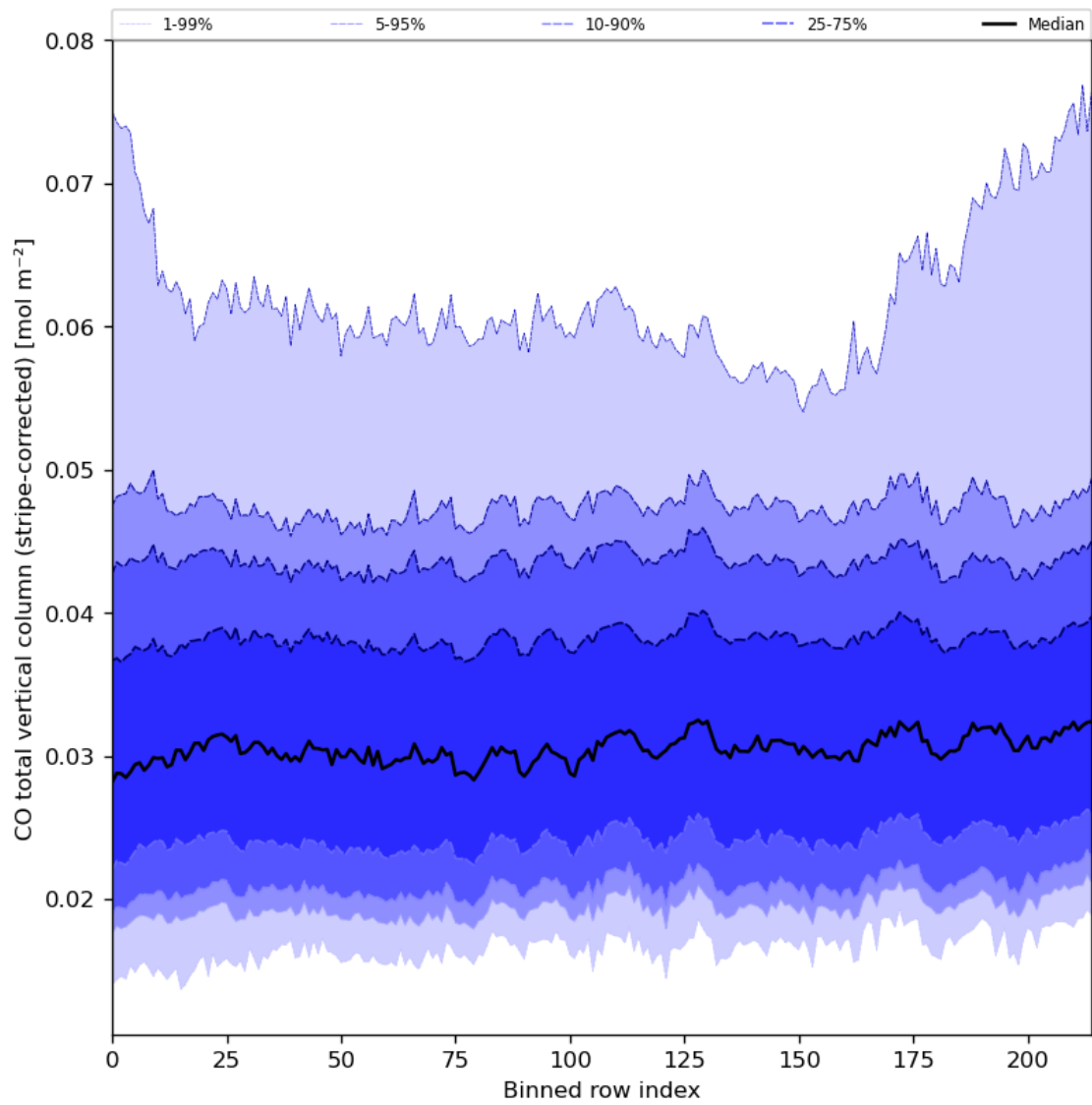
Figure 27: Along track statistics of “CO total vertical column (stripe-corrected)” for 2024-08-23 to 2024-08-25
