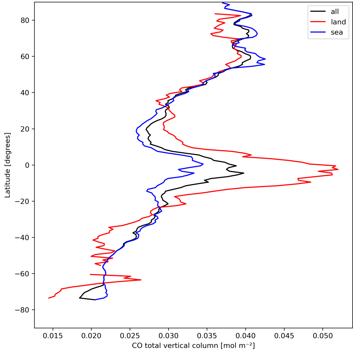
Figure 10: Zonal average of “CO total vertical column” for 2024-08-23 to 2024-08-25.
