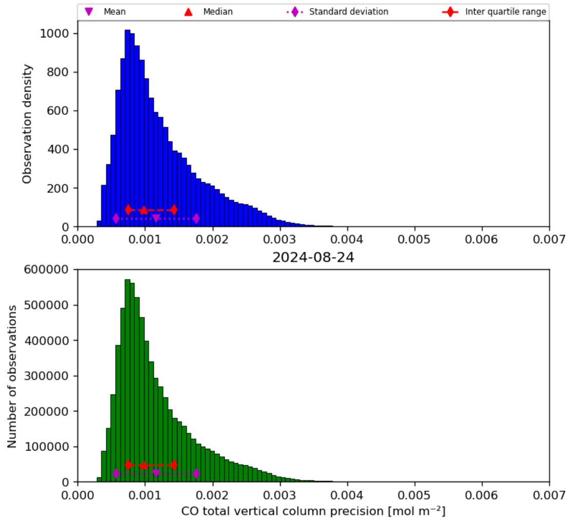
Figure 20: Histogram of “CO total vertical column precision” for 2024-08-23 to 2024-08-25
