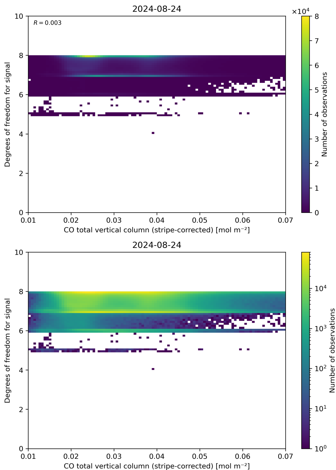
Figure 38: Scatter density plot of “CO total vertical column (stripe-corrected)” against “Degrees of freedom for signal” for 2024-08-23 to 2024-08-25.
