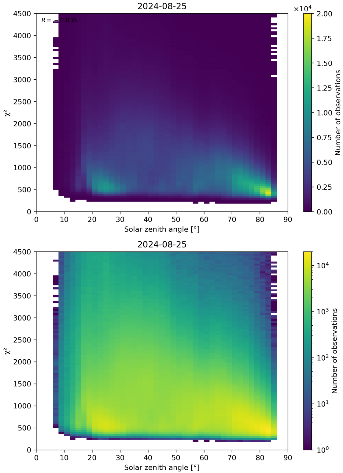
Figure 64: Scatter density plot of “Solar zenith angle” against “ \chi^2 ” for 2024-08-24 to 2024-08-26.
