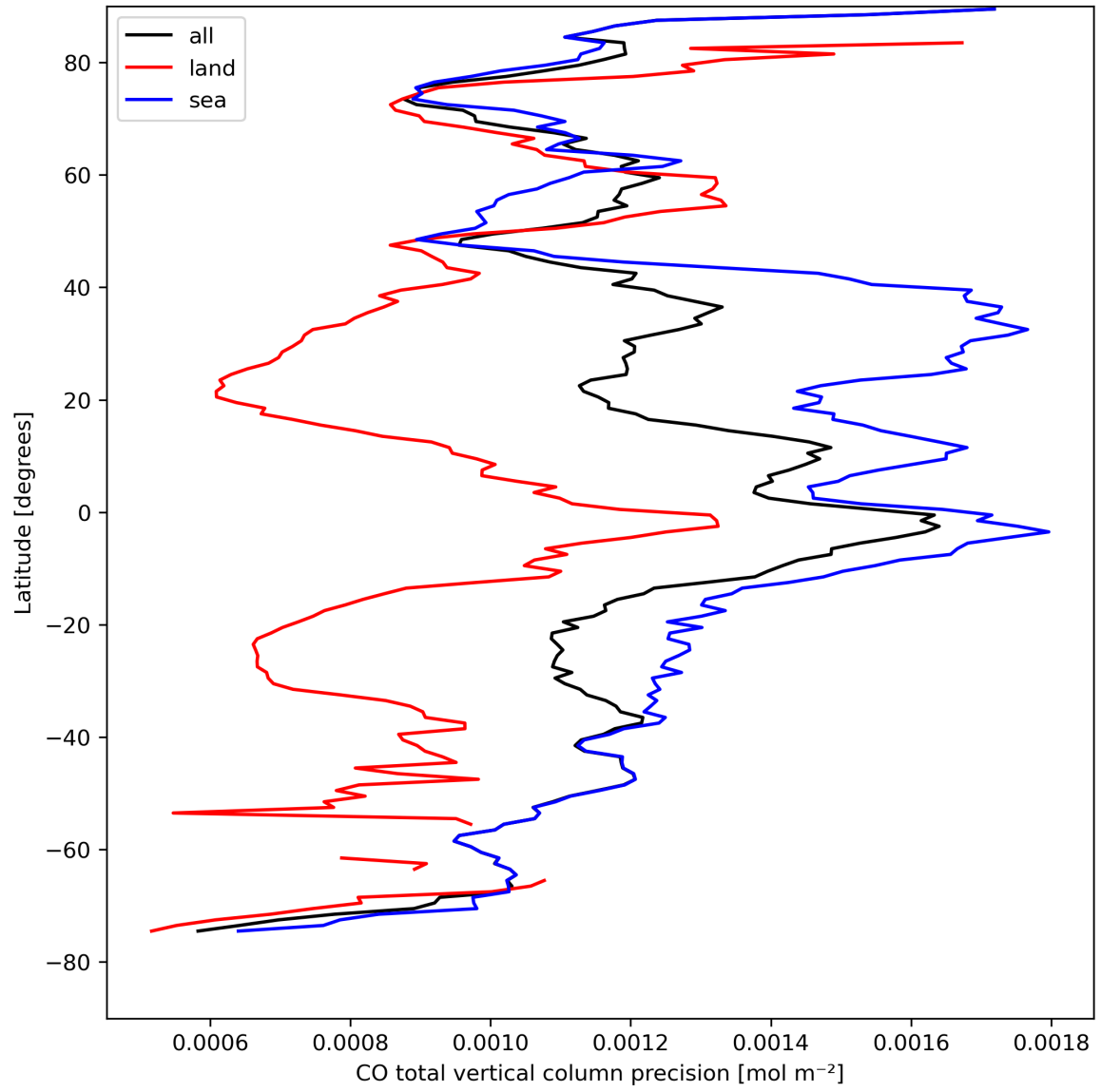
Figure 12: Zonal average of “CO total vertical column precision” for 2024-08-24 to 2024-08-26.
