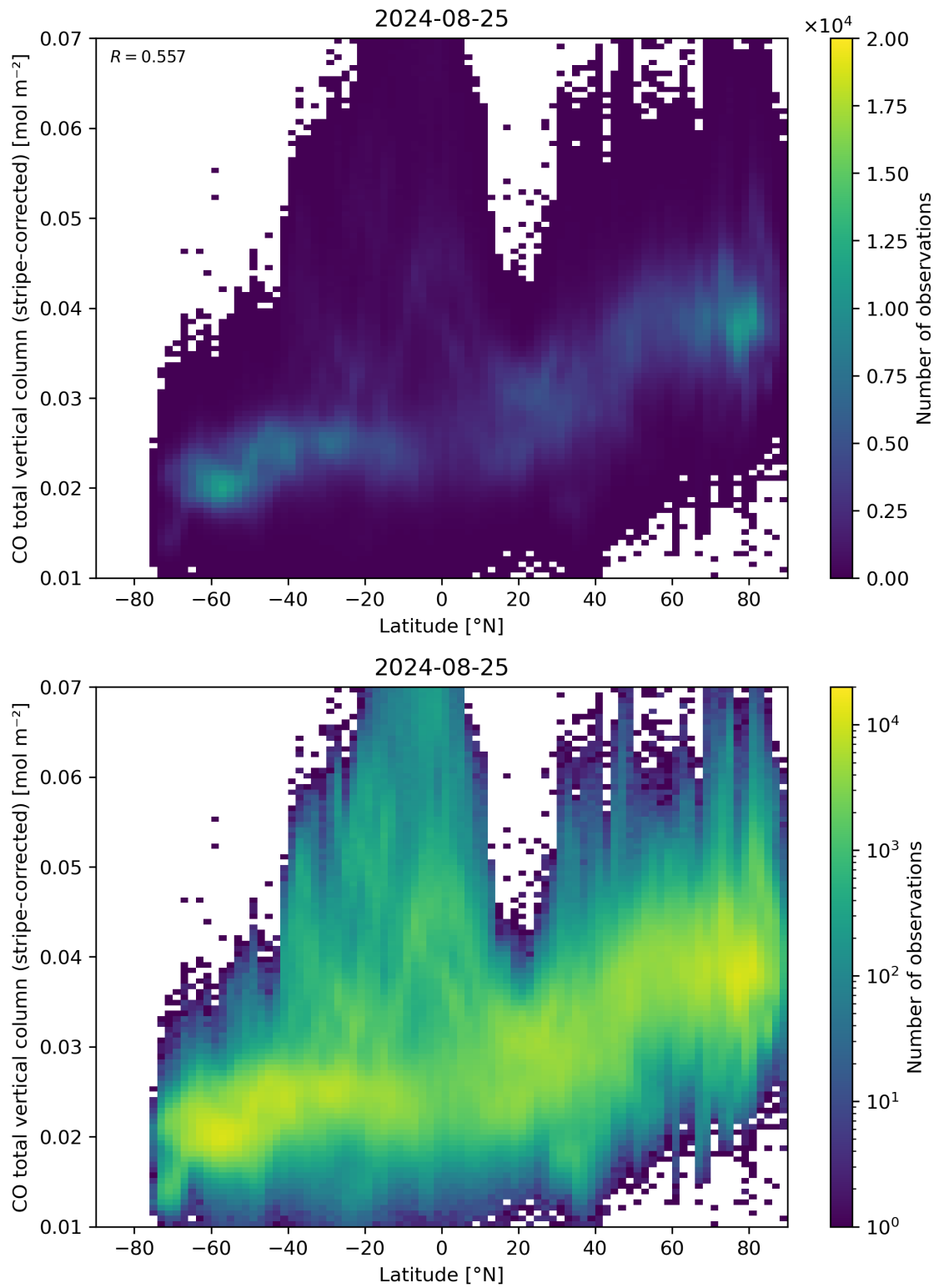
Figure 52: Scatter density plot of “Latitude” against “CO total vertical column (stripe-corrected)” for 2024-08-24 to 2024-08-26.
