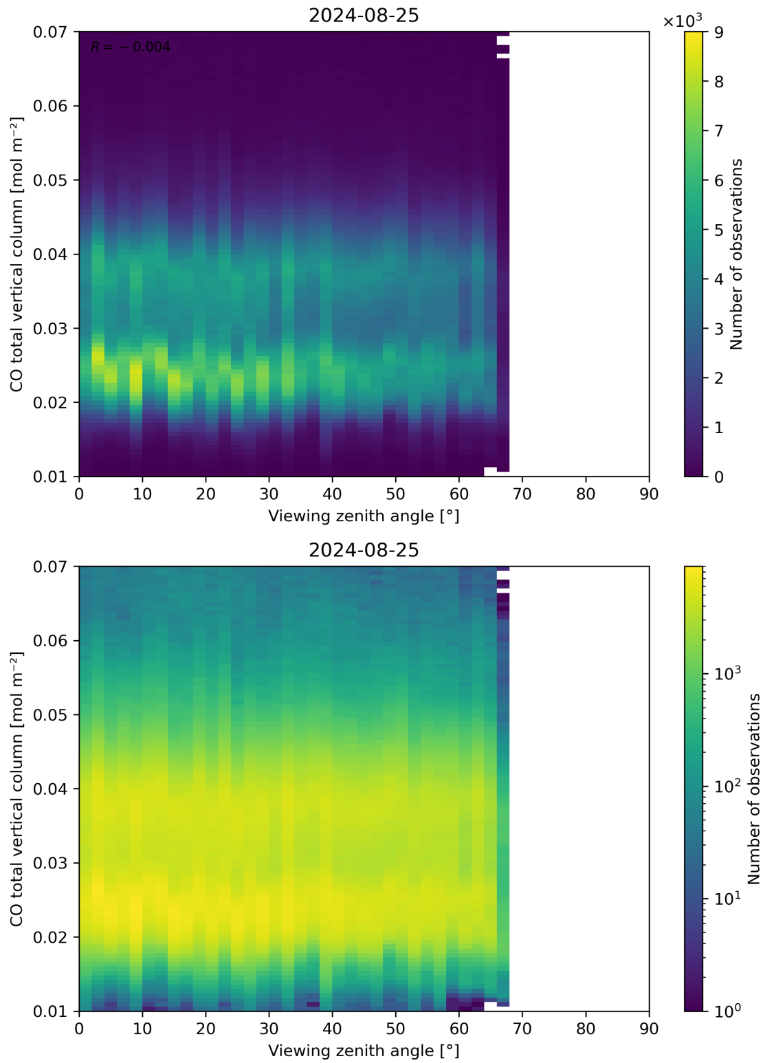
Figure 69: Scatter density plot of “Viewing zenith angle” against “CO total vertical column” for 2024-08-24 to 2024-08-26.
