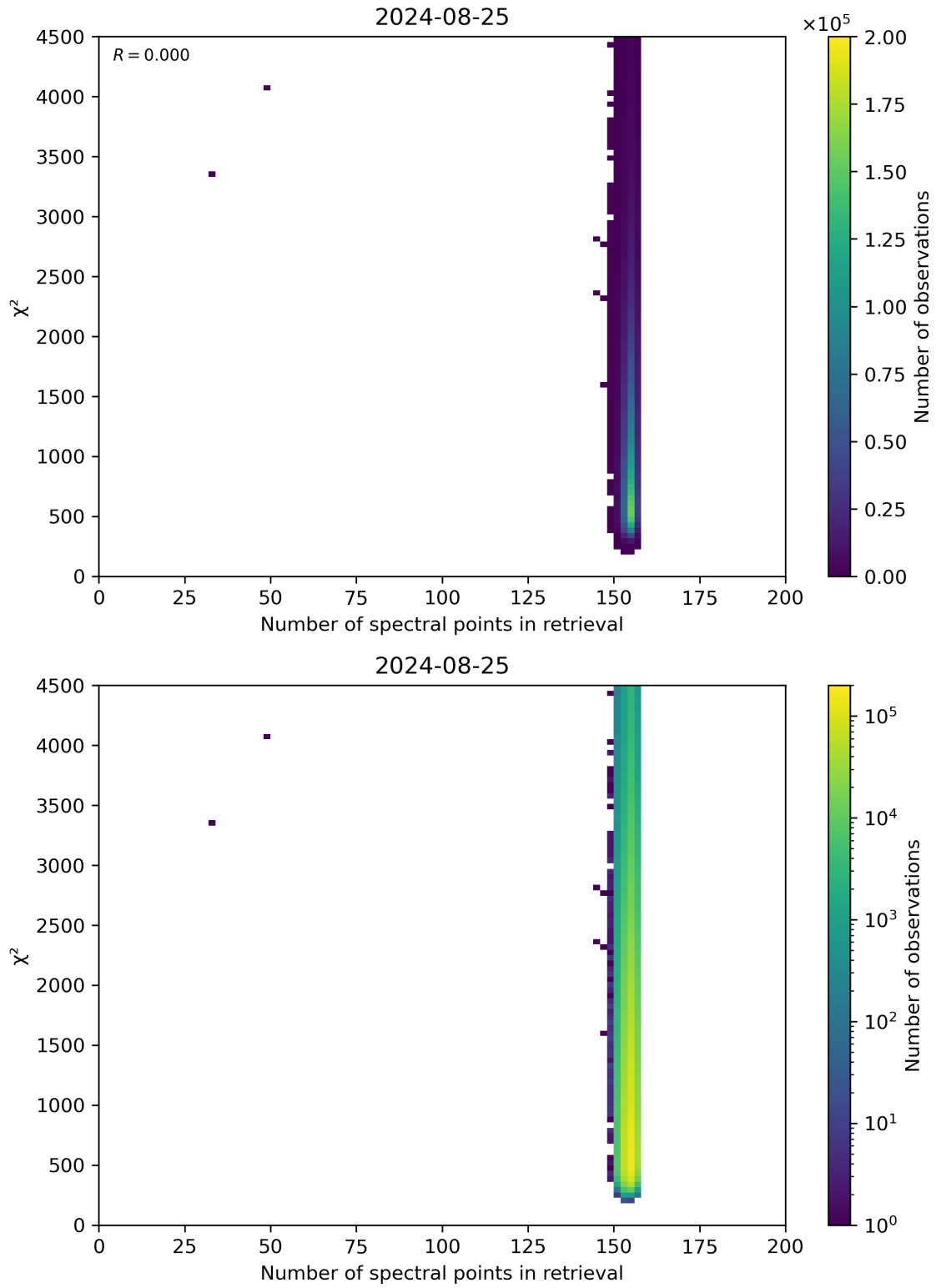
Figure 58: Scatter density plot of “Number of spectral points in retrieval” against “ \chi^2 ” for 2024-08-24 to 2024-08-26.
