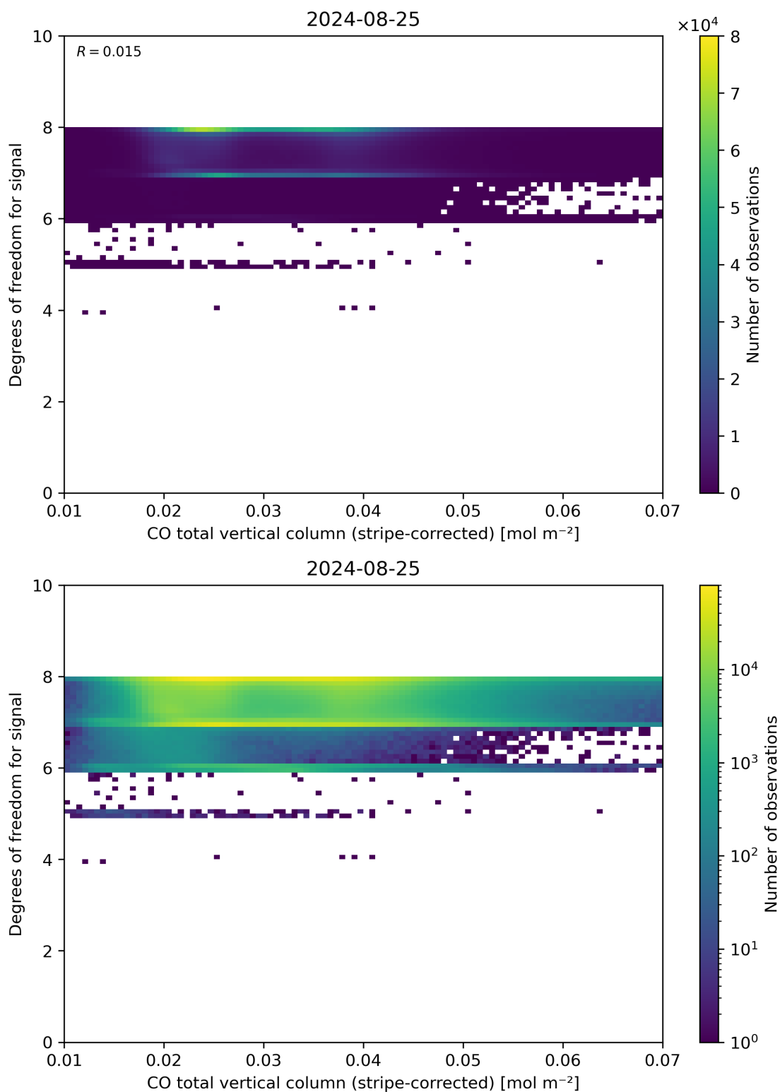
Figure 38: Scatter density plot of “CO total vertical column (stripe-corrected)” against “Degrees of freedom for signal” for 2024-08-24 to 2024-08-26.
