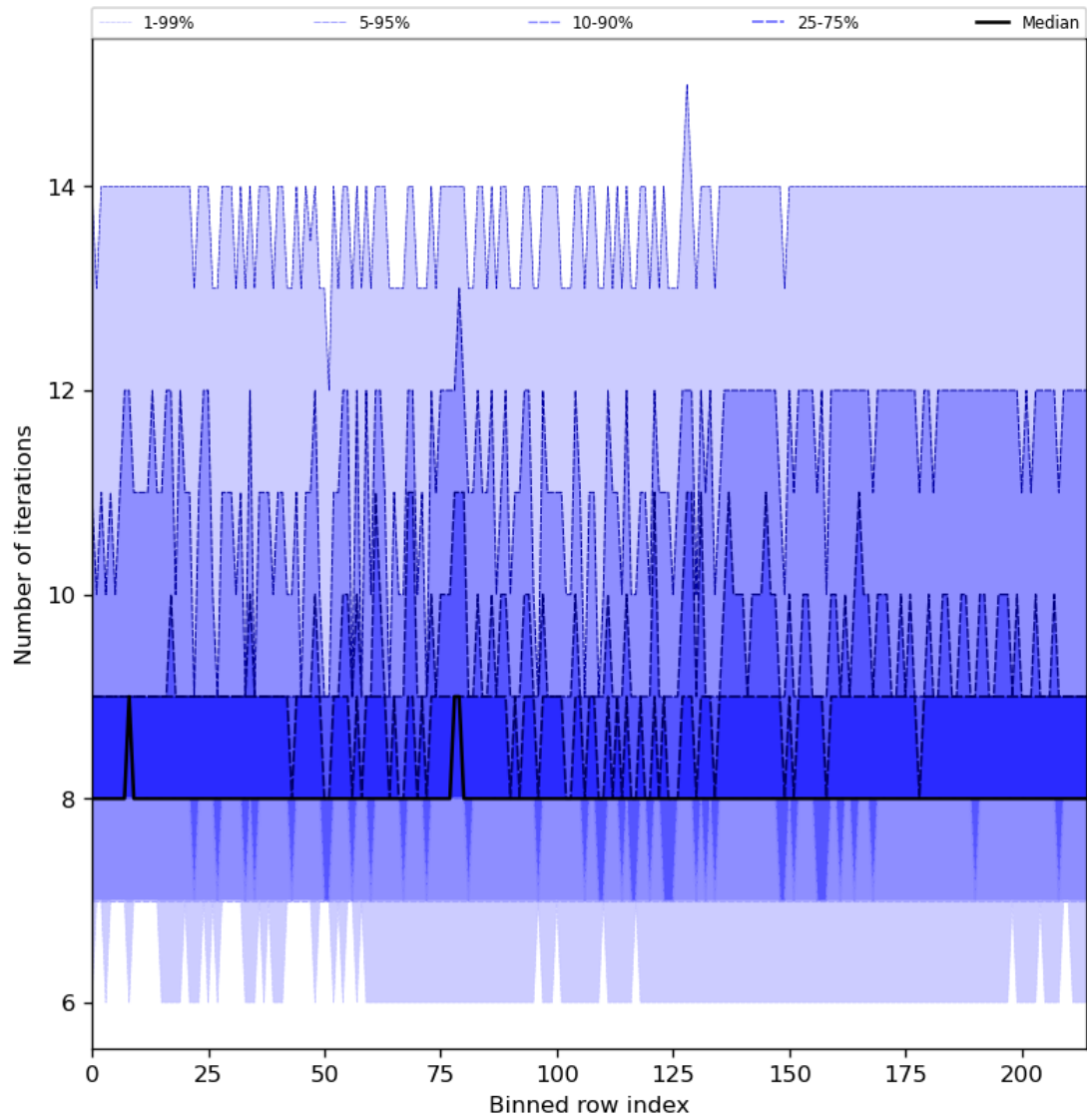
Figure 32: Along track statistics of “Number of iterations” for 2024-08-24 to 2024-08-26
