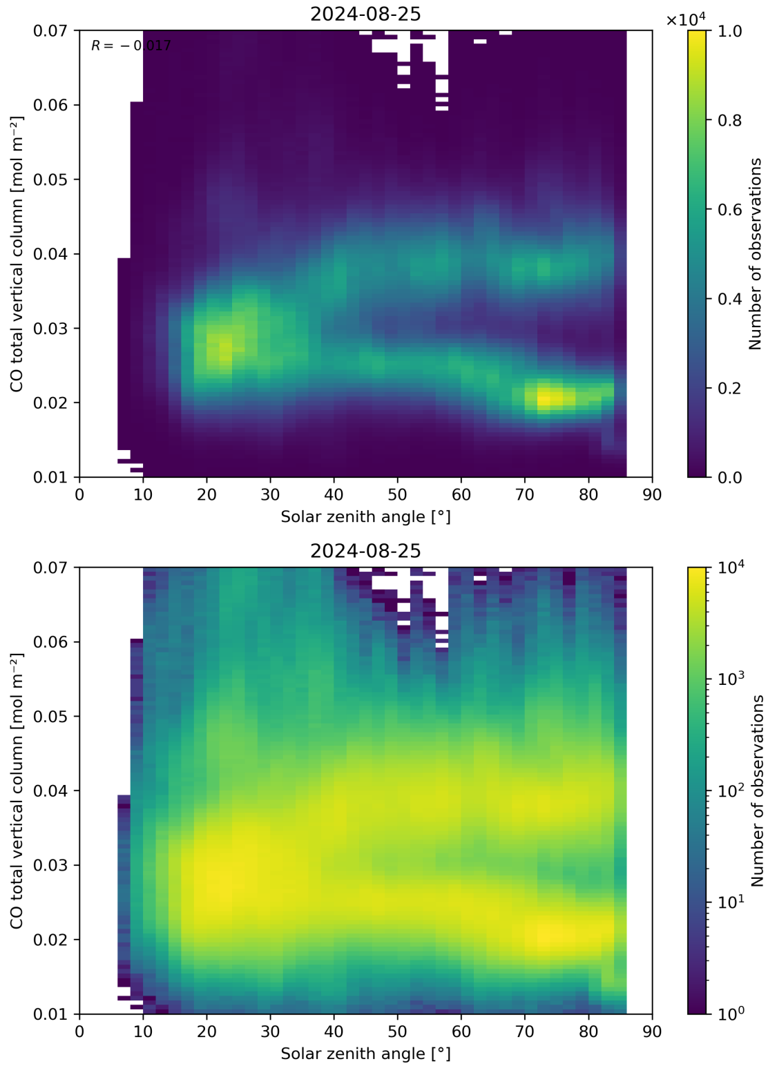
Figure 61: Scatter density plot of “Solar zenith angle” against “CO total vertical column” for 2024-08-24 to 2024-08-26.
