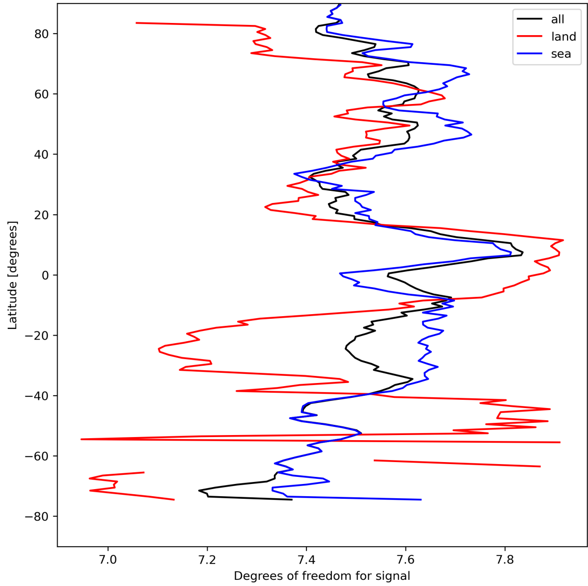
Figure 15: Zonal average of “Degrees of freedom for signal” for 2024-08-24 to 2024-08-26.
