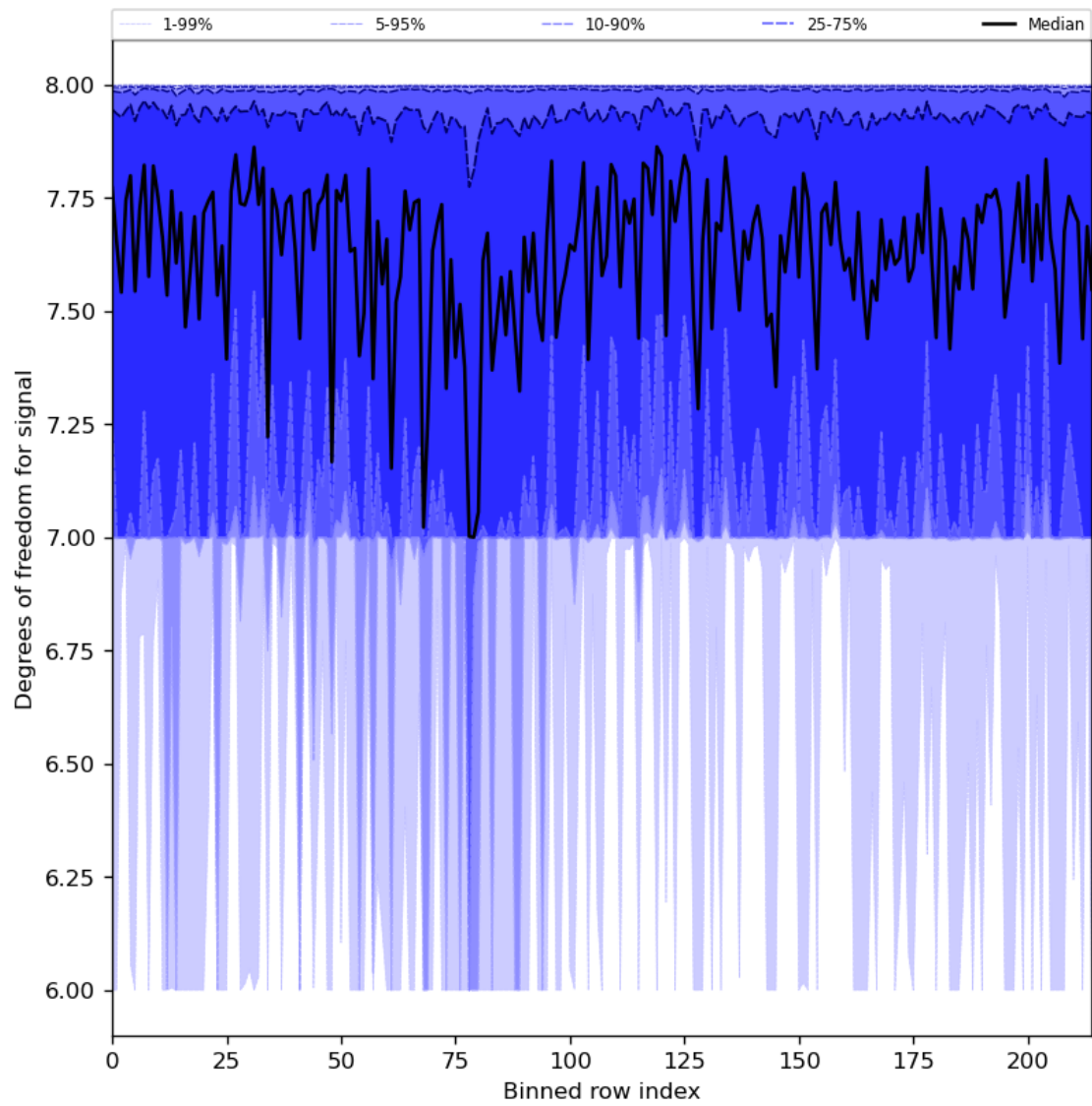
Figure 31: Along track statistics of “Degrees of freedom for signal” for 2024-08-24 to 2024-08-26
