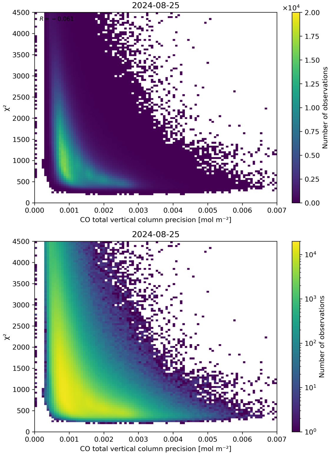
Figure 44: Scatter density plot of “CO total vertical column precision” against “ \chi^2 ” for 2024-08-24 to 2024-08-26.
