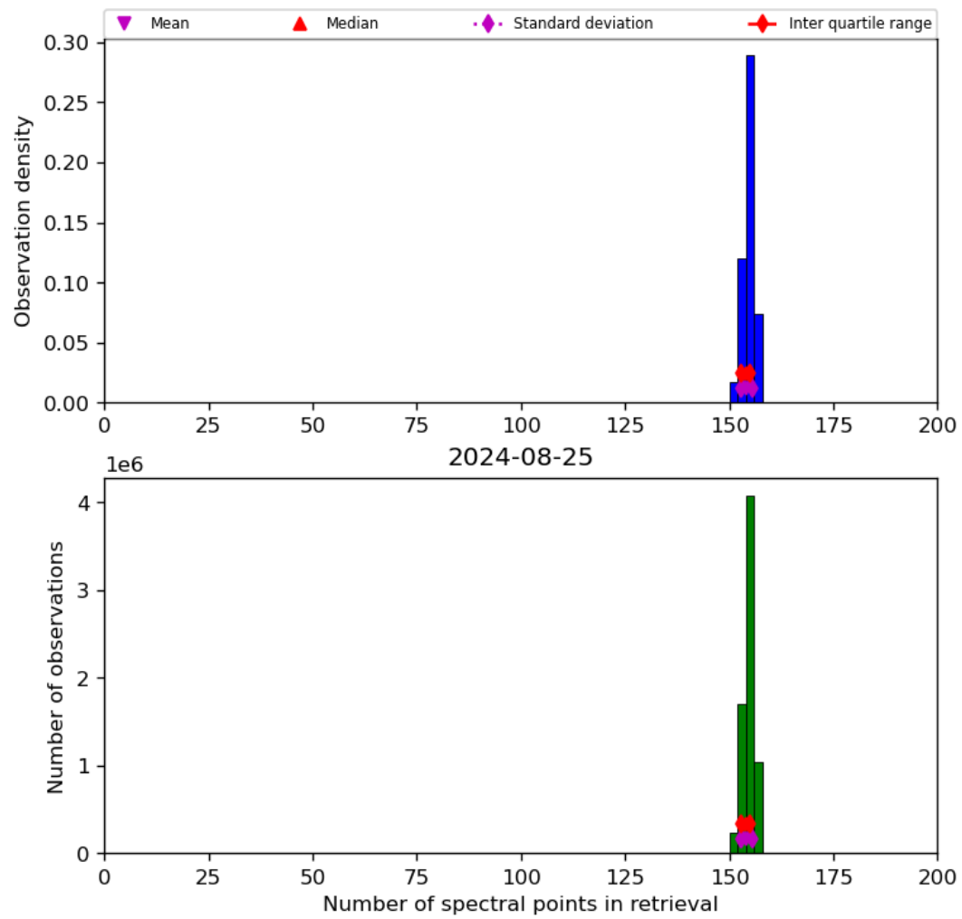
Figure 21: Histogram of “Number of spectral points in retrieval” for 2024-08-24 to 2024-08-26
