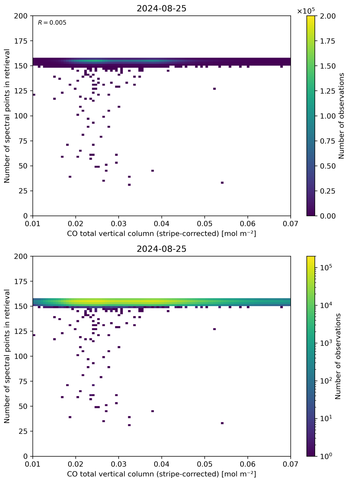
Figure 40: Scatter density plot of “CO total vertical column (stripe-corrected)” against “Number of spectral points in retrieval” for 2024-08-24 to 2024-08-26.
