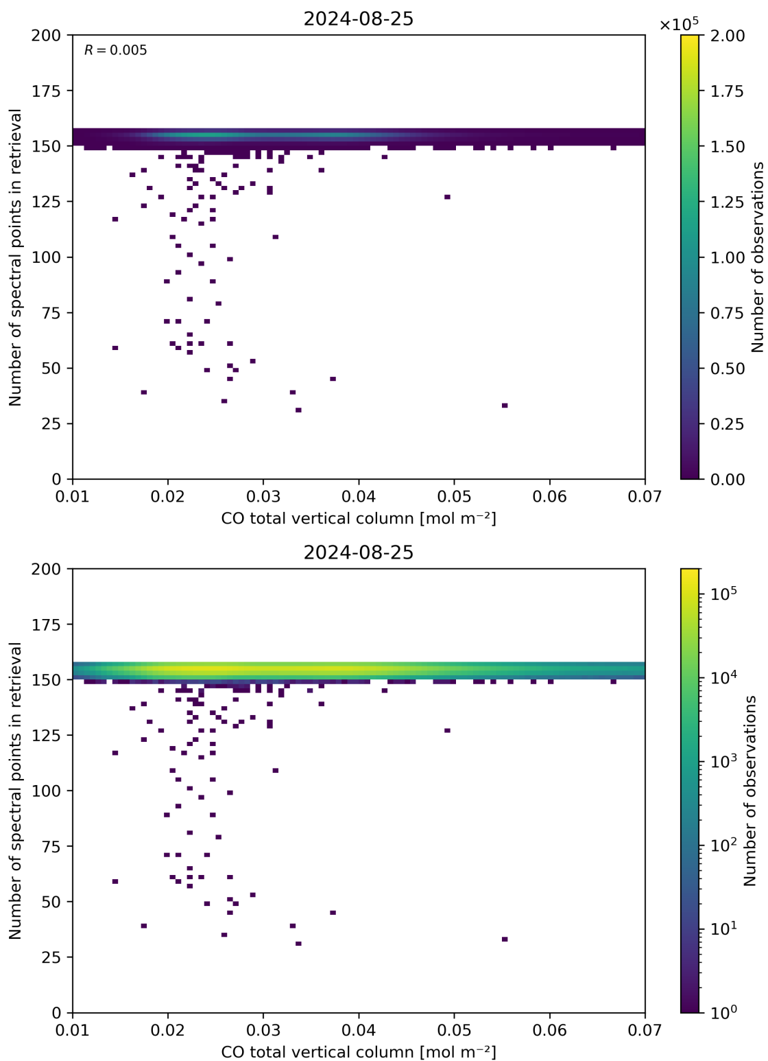
Figure 43: Scatter density plot of “CO total vertical column” against “Number of spectral points in retrieval” for 2024-08-24 to 2024-08-26.
