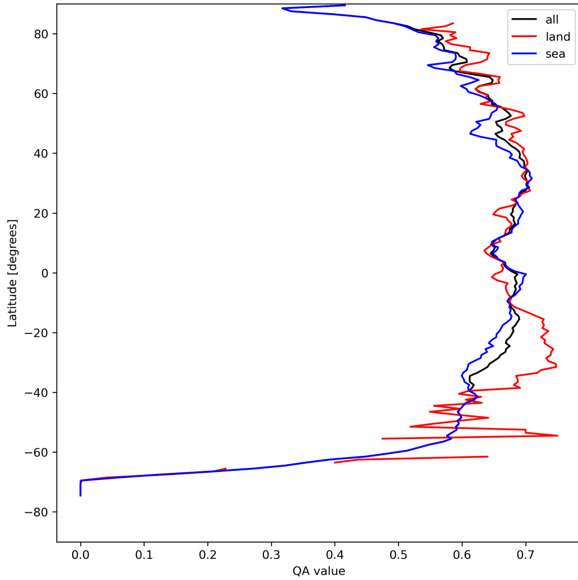
Figure 9: Zonal average of “QA value” for 2024-08-24 to 2024-08-26.
