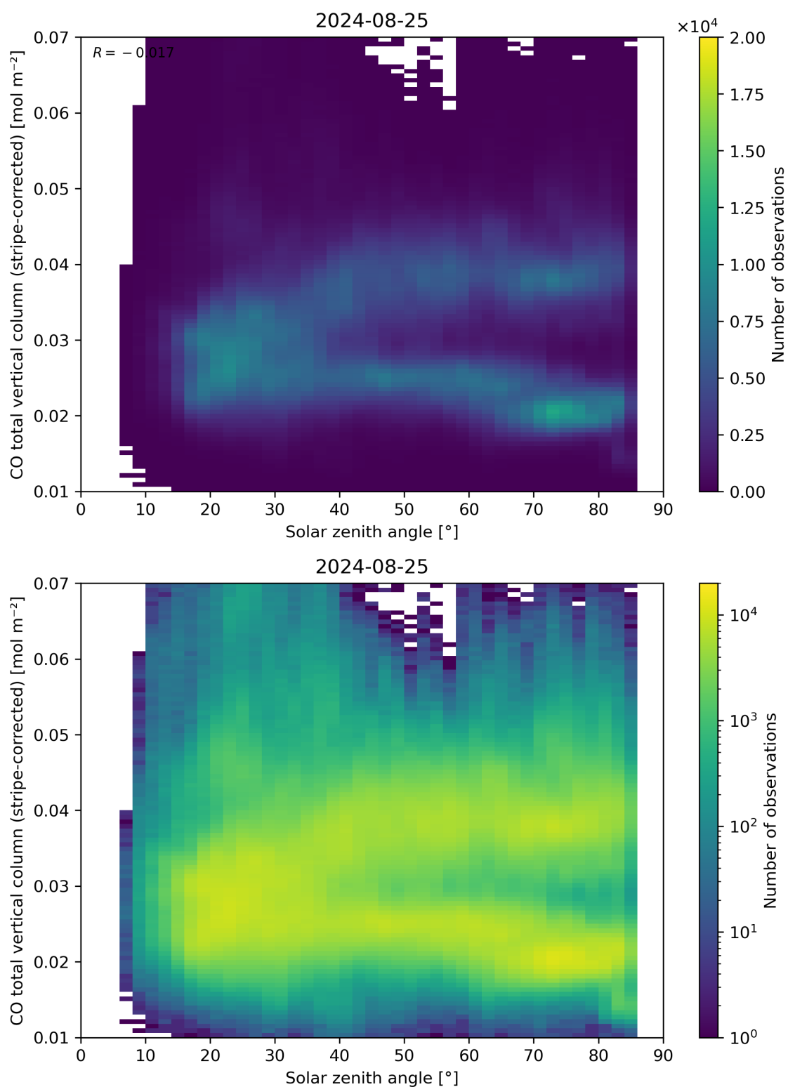
Figure 62: Scatter density plot of “Solar zenith angle” against “CO total vertical column (stripe-corrected)” for 2024-08-24 to 2024-08-26.
