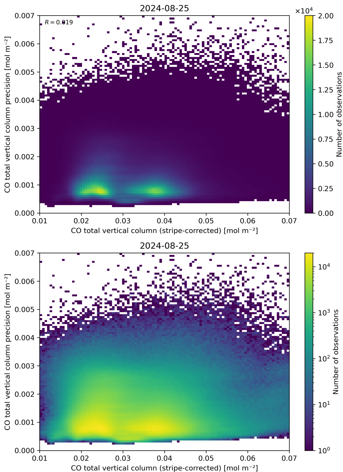
Figure 36: Scatter density plot of “CO total vertical column (stripe-corrected)” against “CO total vertical column precision” for 2024-08-24 to 2024-08-26.
