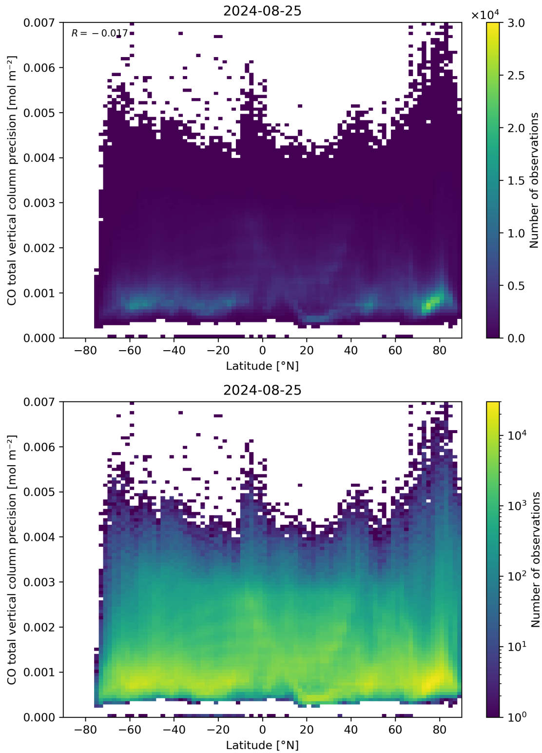
Figure 53: Scatter density plot of “Latitude” against “CO total vertical column precision” for 2024-08-24 to 2024-08-26.
