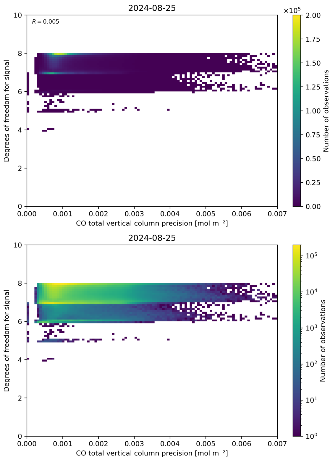
Figure 45: Scatter density plot of “CO total vertical column precision” against “Degrees of freedom for signal” for 2024-08-24 to 2024-08-26.
