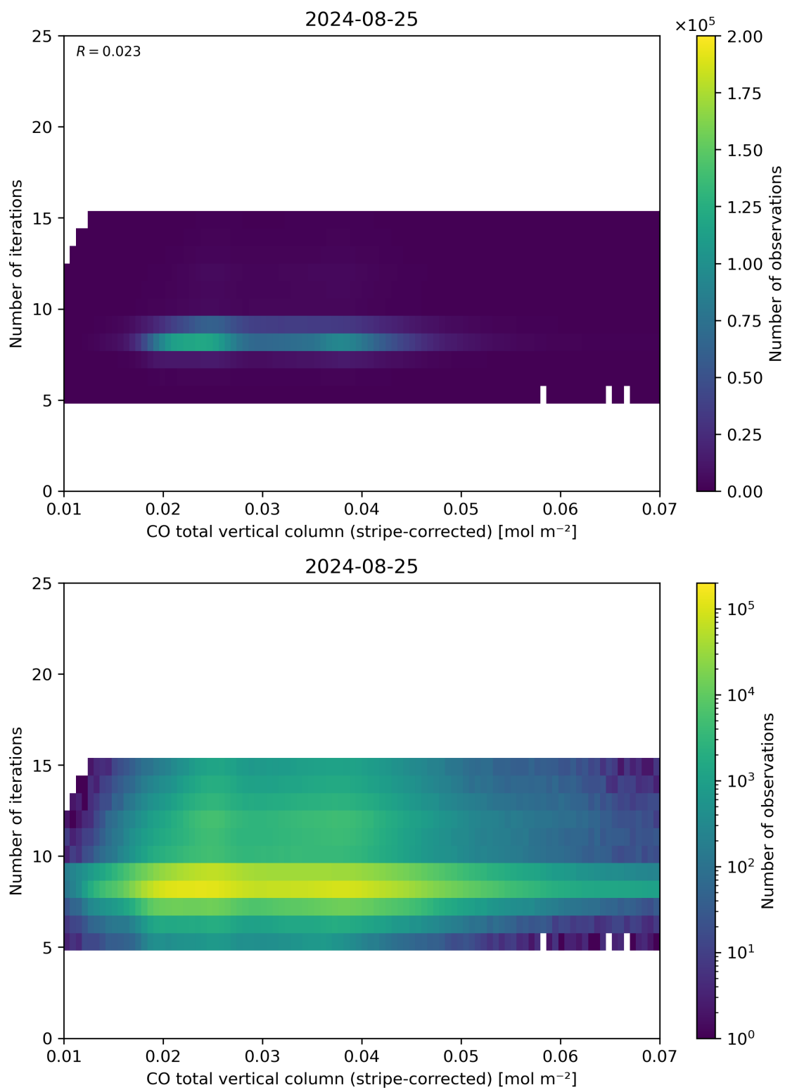
Figure 39: Scatter density plot of “CO total vertical column (stripe-corrected)” against “Number of iterations” for 2024-08-24 to 2024-08-26.
