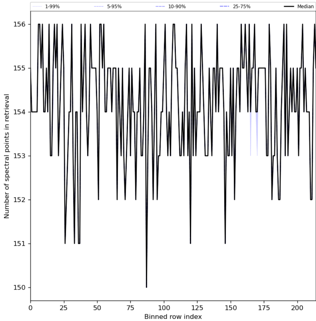
Figure 29: Along track statistics of “Number of spectral points in retrieval” for 2024-08-24 to 2024-08-26
