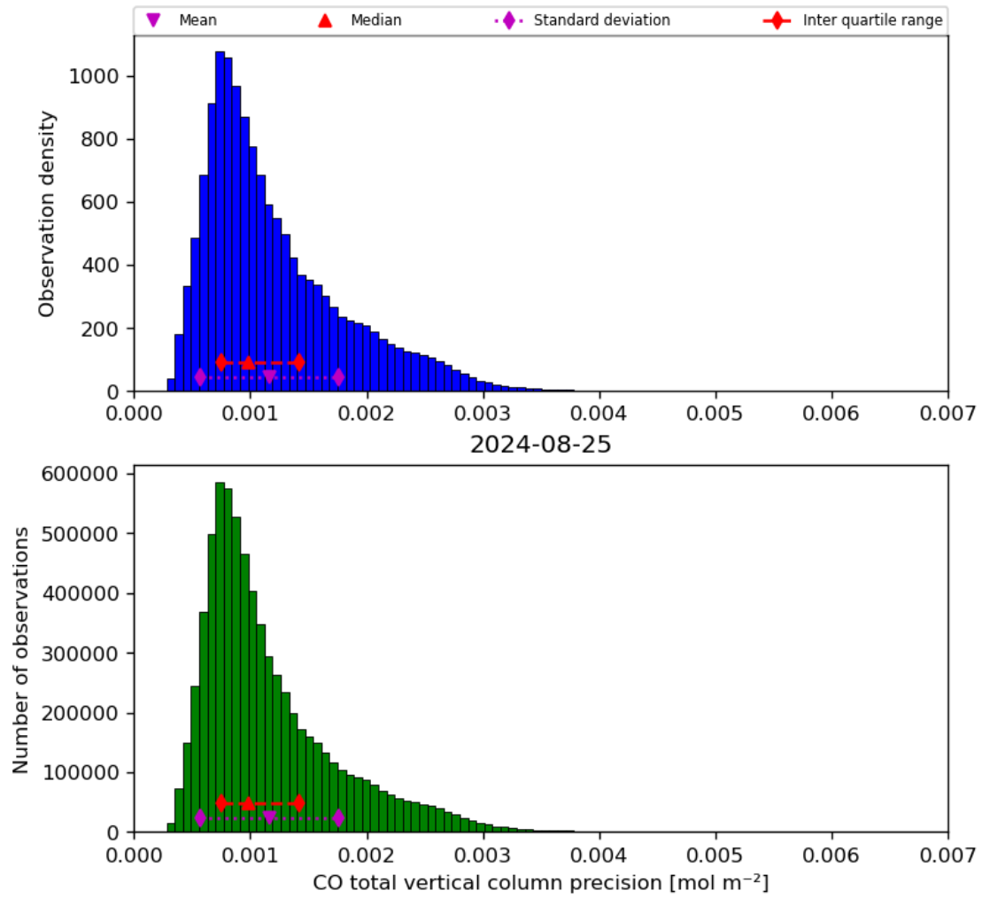
Figure 20: Histogram of “CO total vertical column precision” for 2024-08-24 to 2024-08-26
