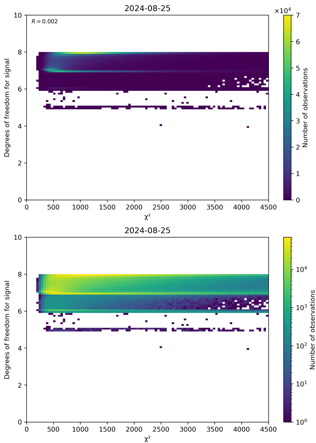
Figure 48: Scatter density plot of “ \chi^2 ” against “Degrees of freedom for signal” for 2024-08-24 to 2024-08-26.
