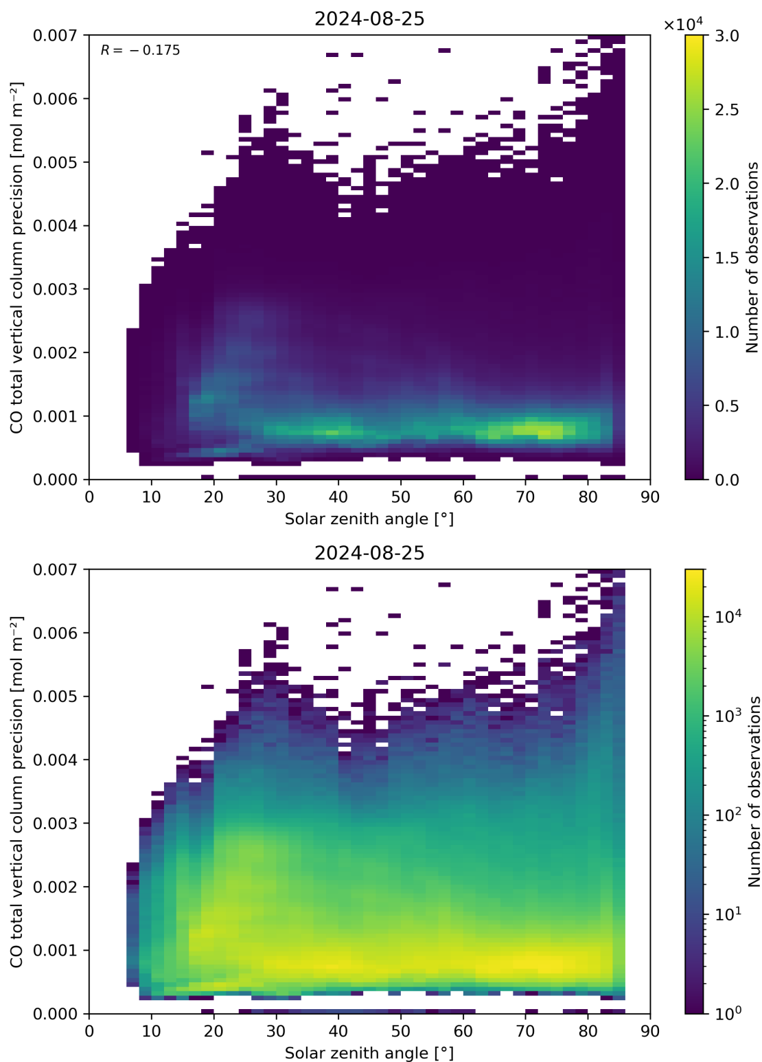
Figure 63: Scatter density plot of “Solar zenith angle” against “CO total vertical column precision” for 2024-08-24 to 2024-08-26.
