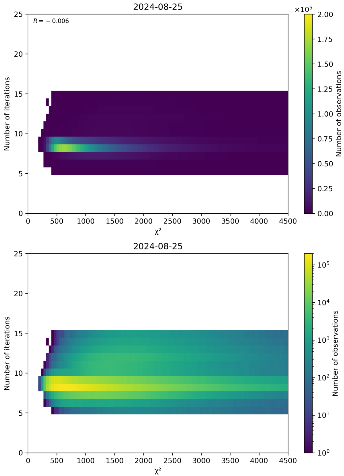
Figure 49: Scatter density plot of “ \chi^2 ” against “Number of iterations” for 2024-08-24 to 2024-08-26.
