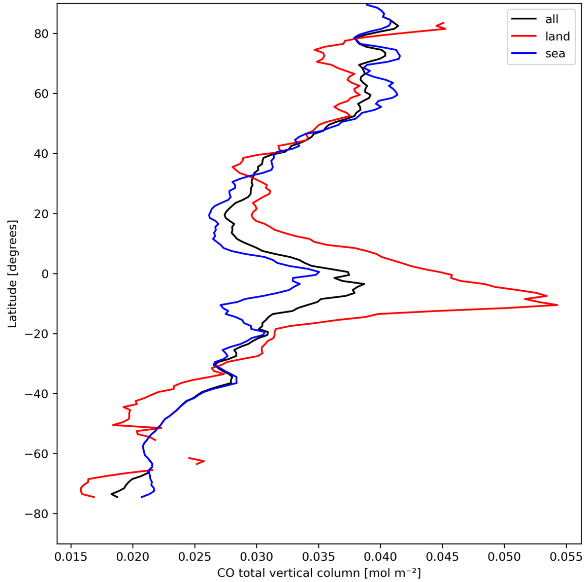
Figure 10: Zonal average of “CO total vertical column” for 2024-08-24 to 2024-08-26.
