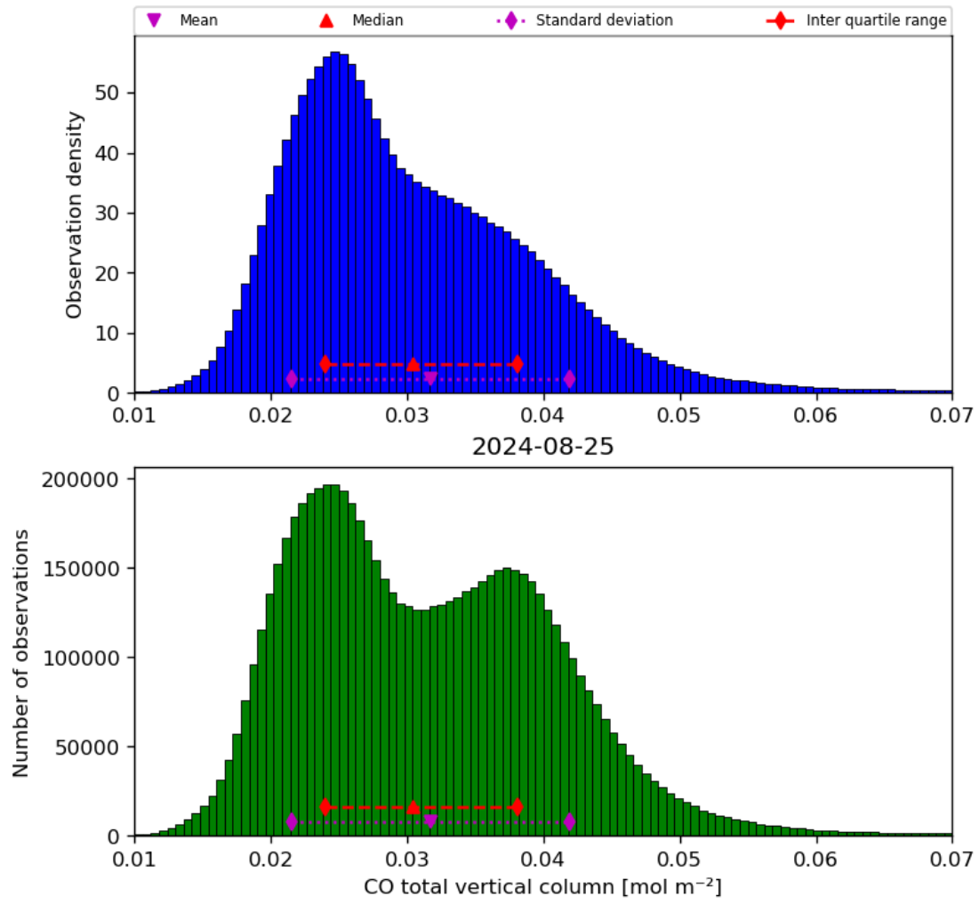
Figure 18: Histogram of “CO total vertical column” for 2024-08-24 to 2024-08-26
