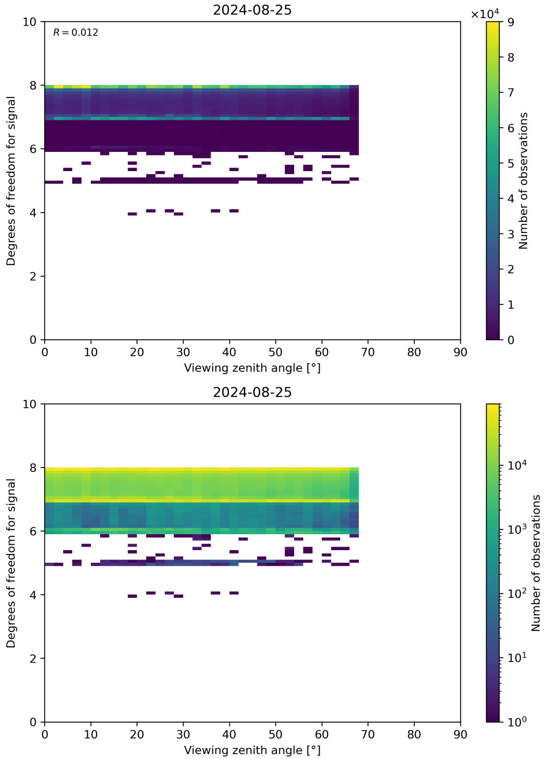
Figure 73: Scatter density plot of “Viewing zenith angle” against “Degrees of freedom for signal” for 2024-08-24 to 2024-08-26.
