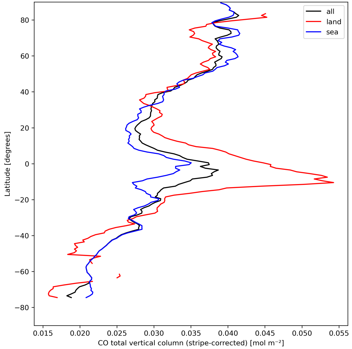
Figure 11: Zonal average of “CO total vertical column (stripe-corrected)” for 2024-08-24 to 2024-08-26.
