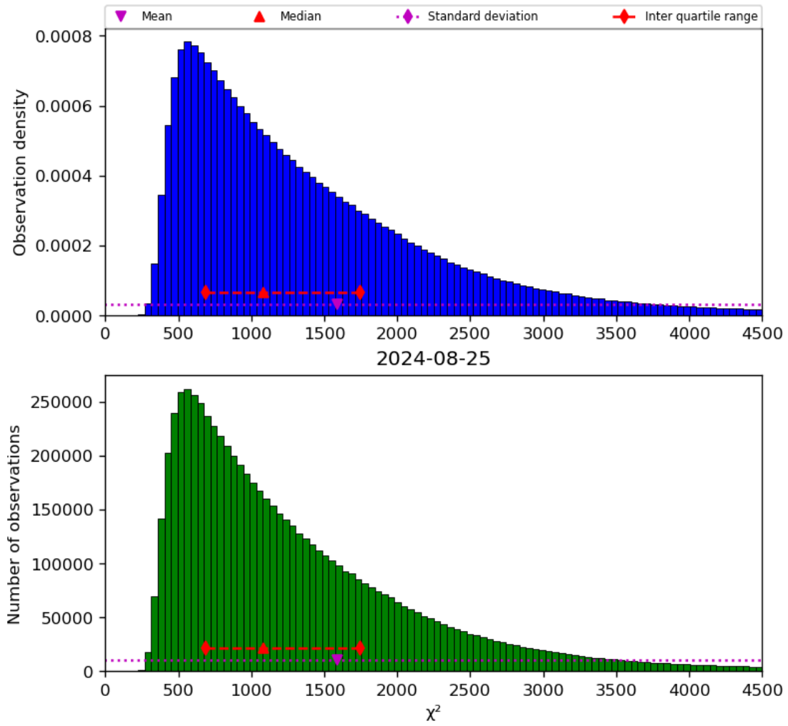
Figure 22: Histogram of “ \chi^2 ” for 2024-08-24 to 2024-08-26
