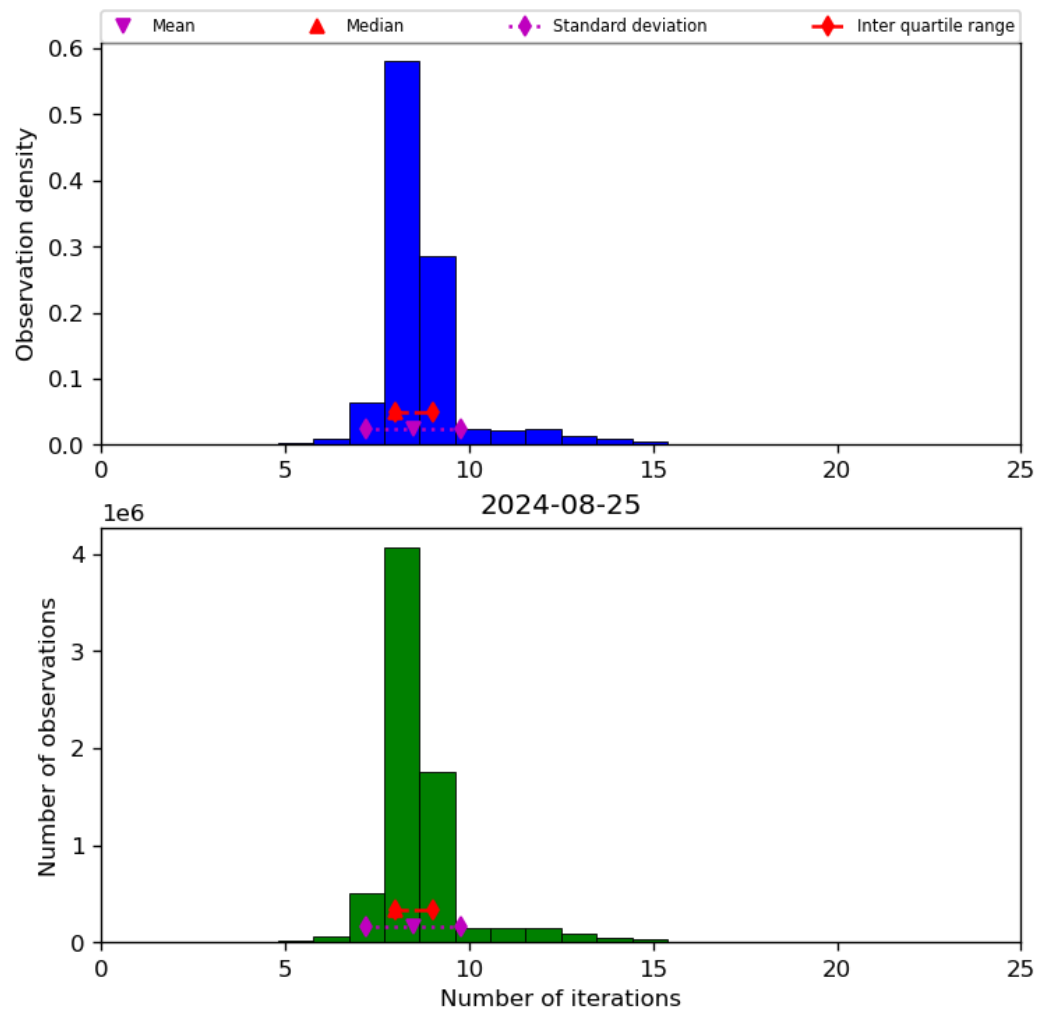
Figure 24: Histogram of “Number of iterations” for 2024-08-24 to 2024-08-26
