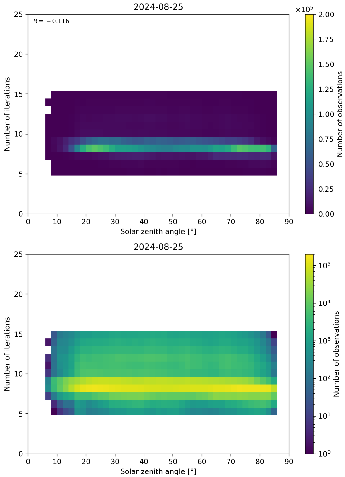
Figure 67: Scatter density plot of “Solar zenith angle” against “Number of iterations” for 2024-08-24 to 2024-08-26.
