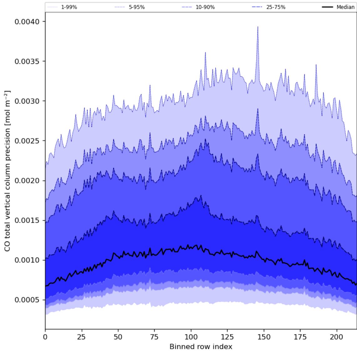
Figure 28: Along track statistics of “CO total vertical column precision” for 2024-08-24 to 2024-08-26
