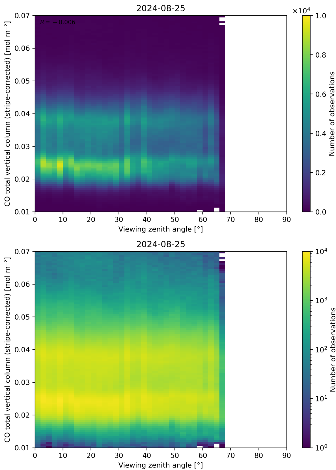
Figure 70: Scatter density plot of “Viewing zenith angle” against “CO total vertical column (stripe-corrected)” for 2024-08-24 to 2024-08-26.
