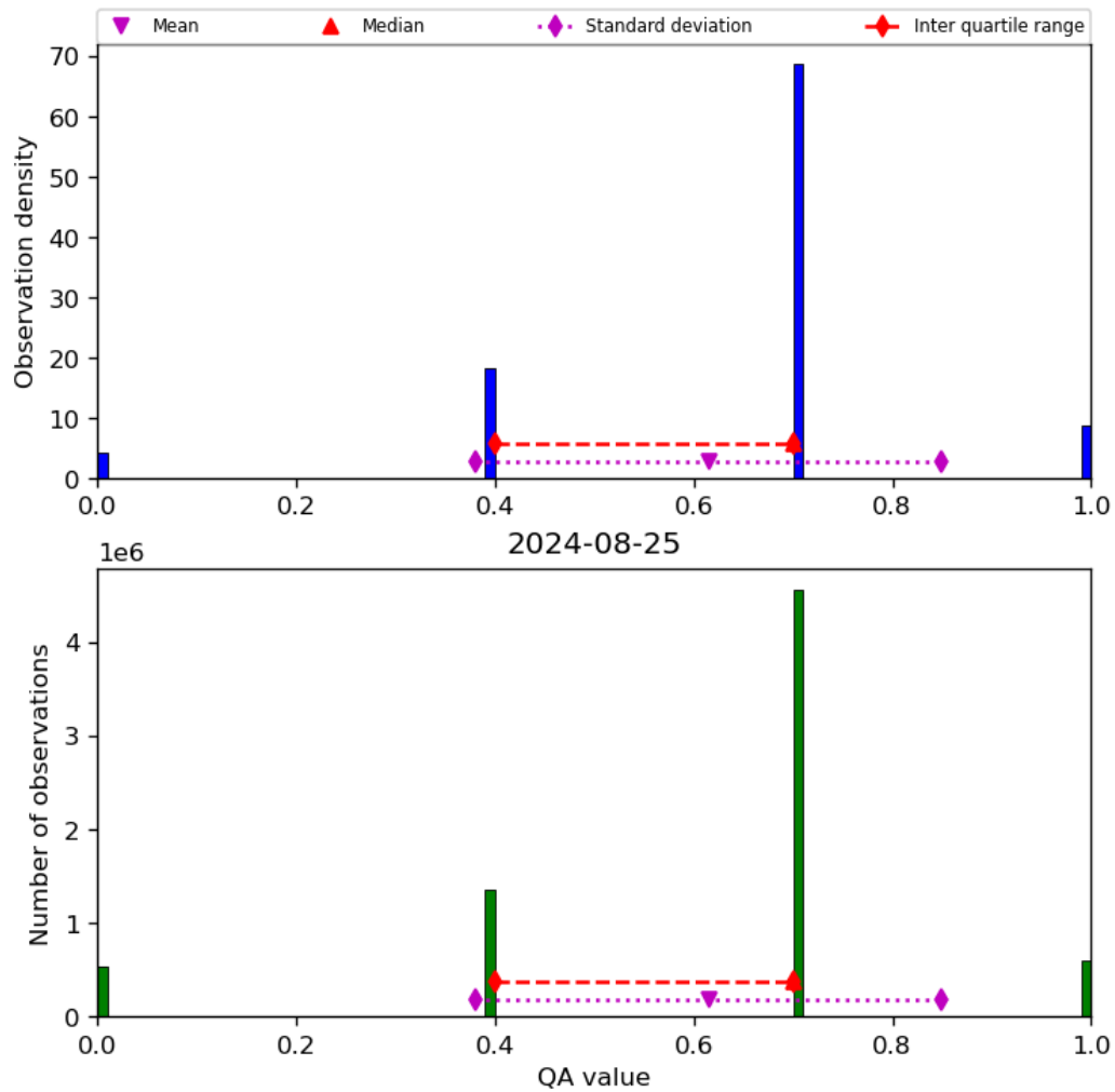
Figure 17: Histogram of “QA value” for 2024-08-24 to 2024-08-26
