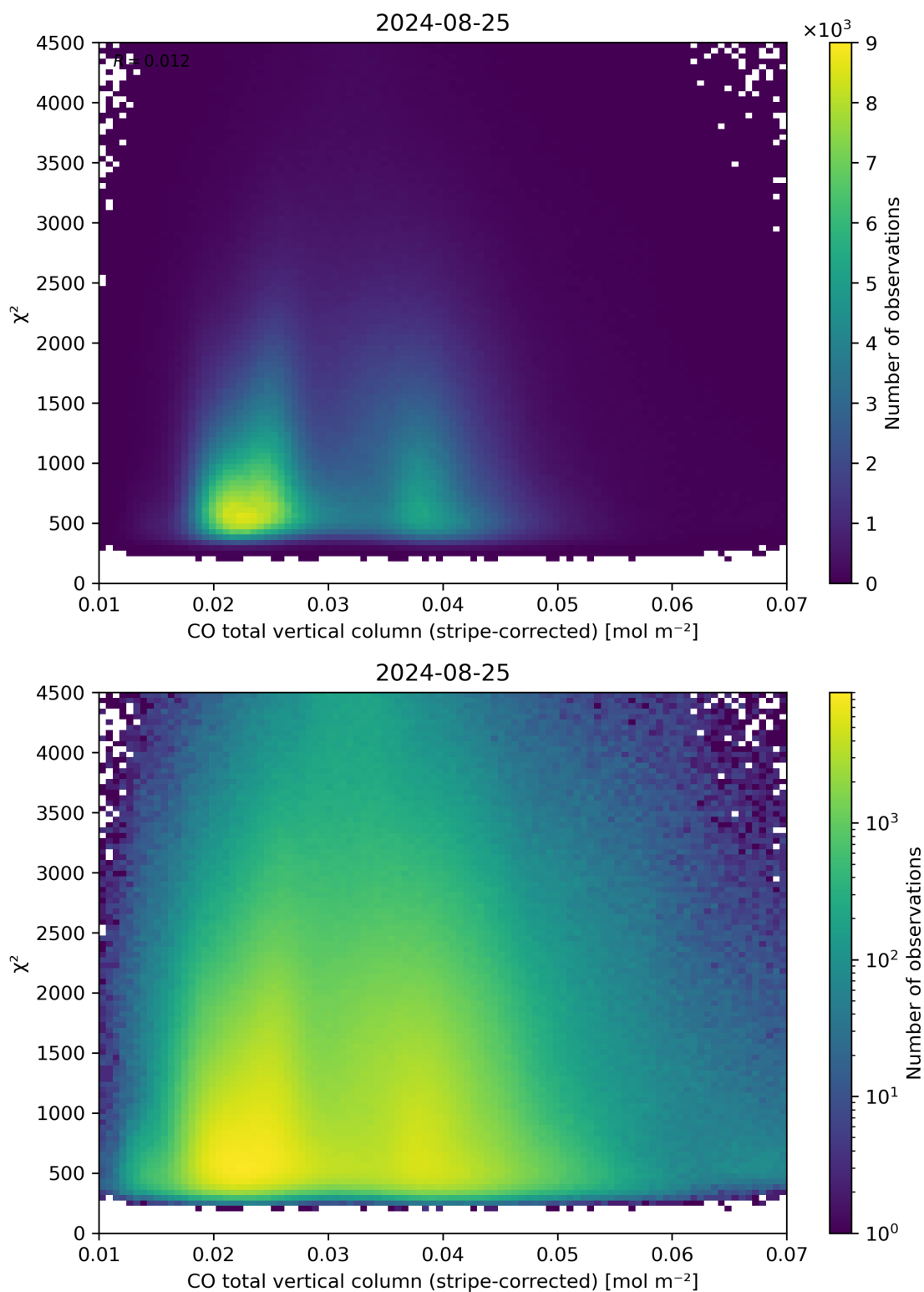
Figure 37: Scatter density plot of “CO total vertical column (stripe-corrected)” against “ \chi^2 ” for 2024-08-24 to 2024-08-26.
