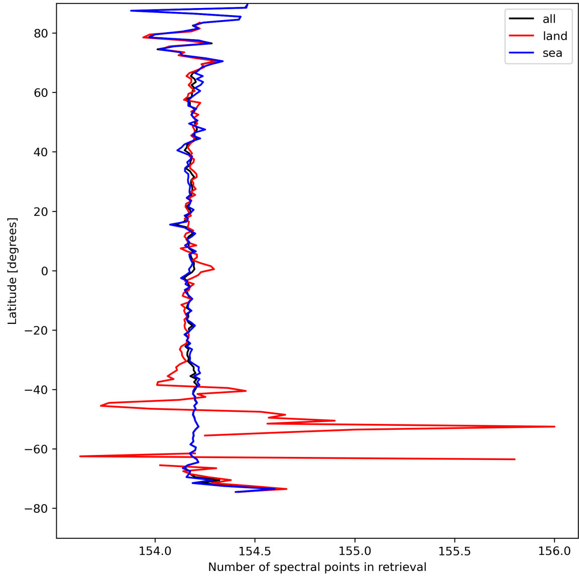
Figure 13: Zonal average of “Number of spectral points in retrieval” for 2024-08-24 to 2024-08-26.
