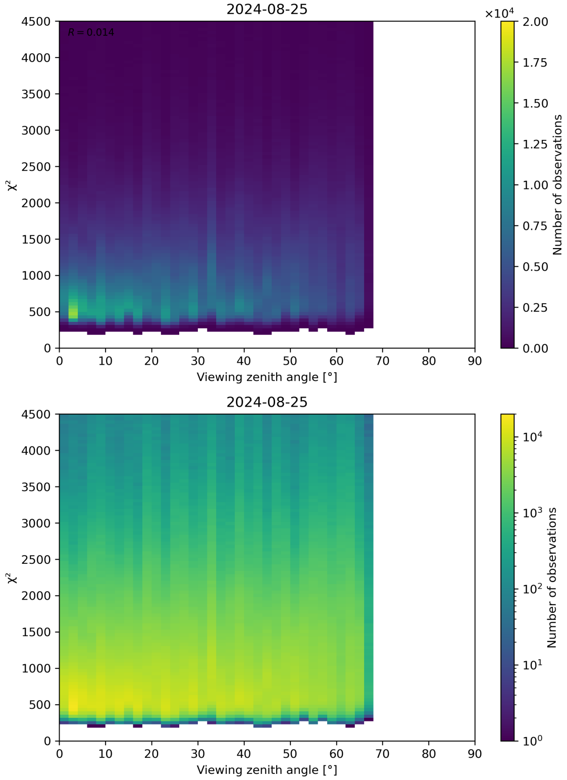
Figure 72: Scatter density plot of “Viewing zenith angle” against “ \chi^2 ” for 2024-08-24 to 2024-08-26.
