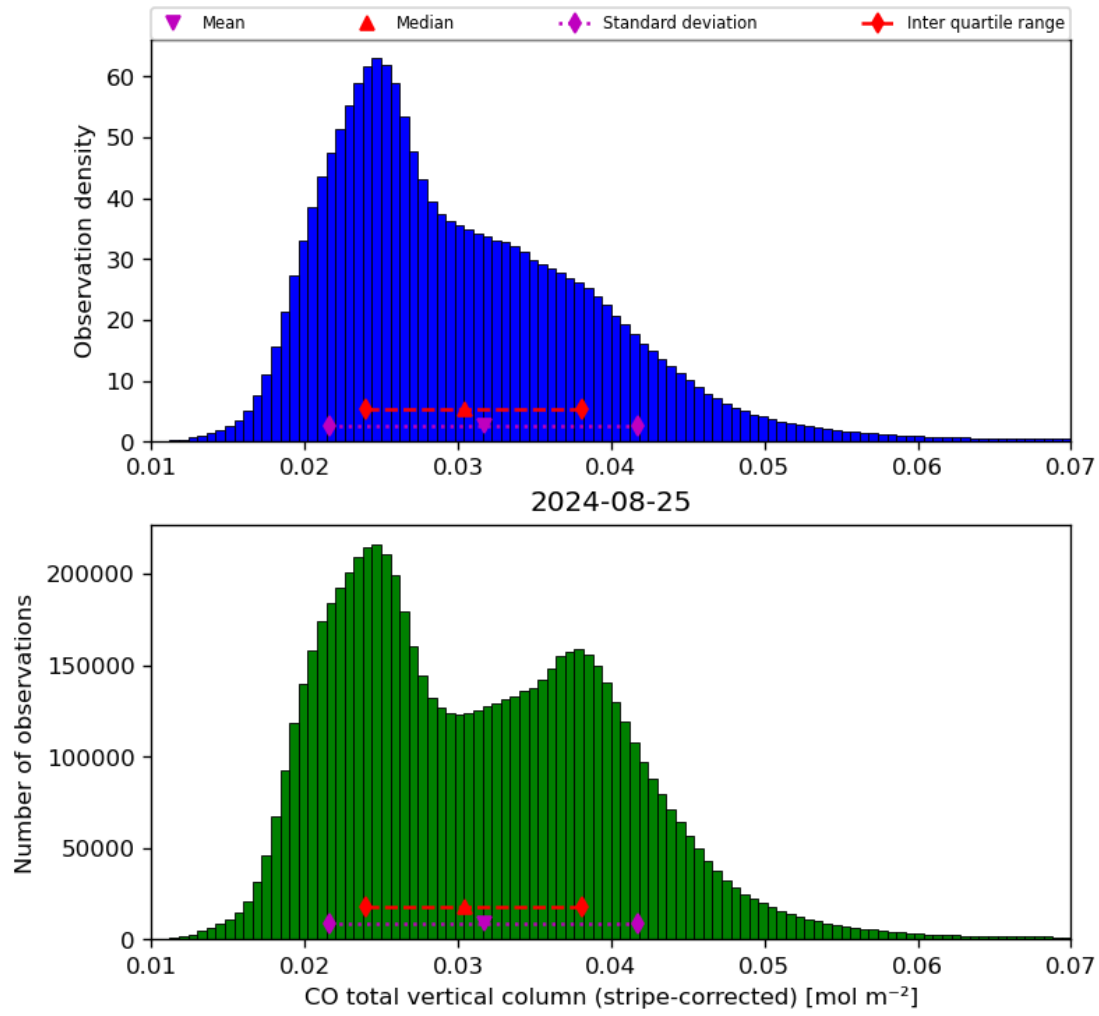
Figure 19: Histogram of “CO total vertical column (stripe-corrected)” for 2024-08-24 to 2024-08-26
