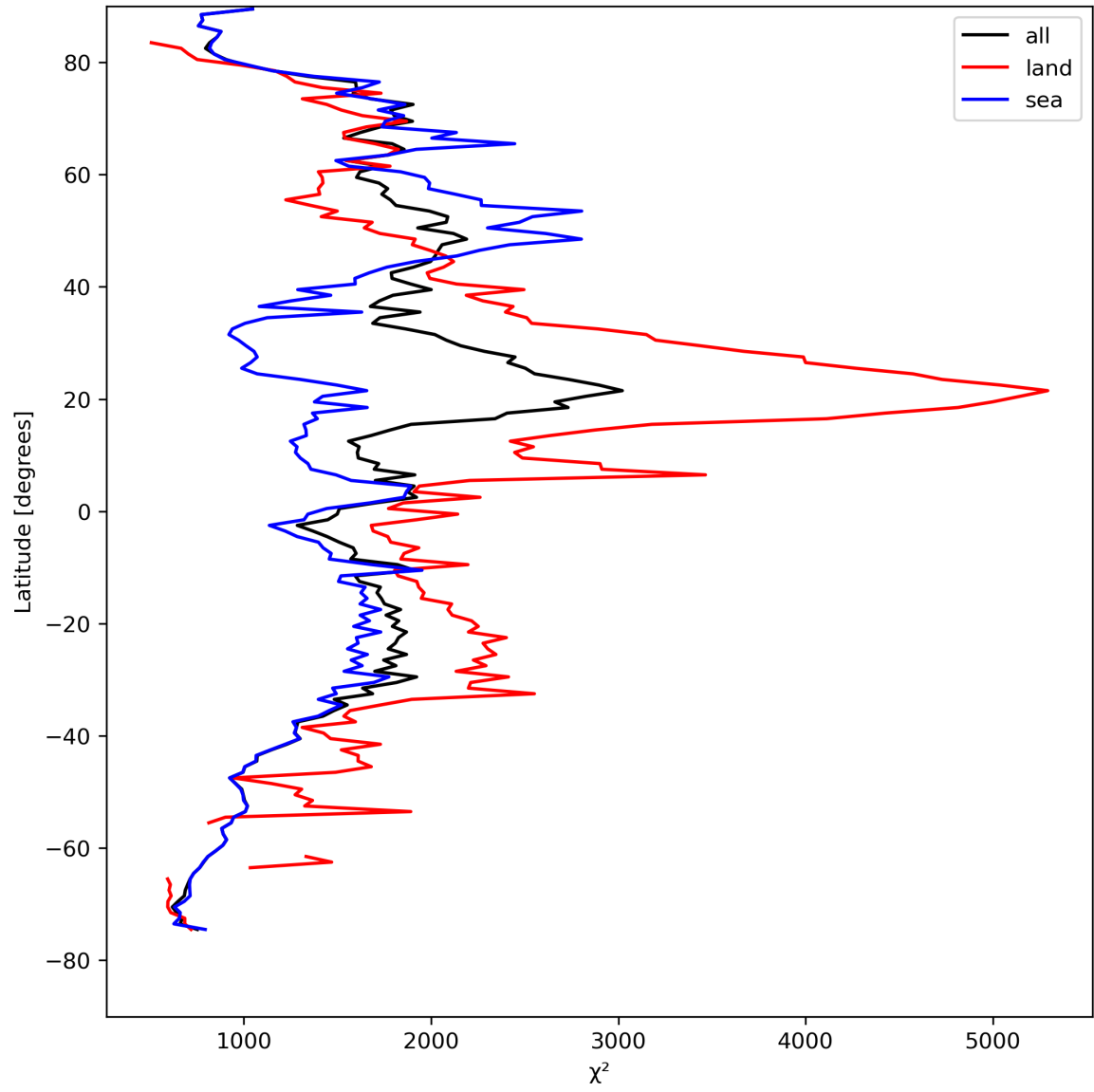
Figure 14: Zonal average of “ \chi^2 ” for 2024-08-24 to 2024-08-26.
