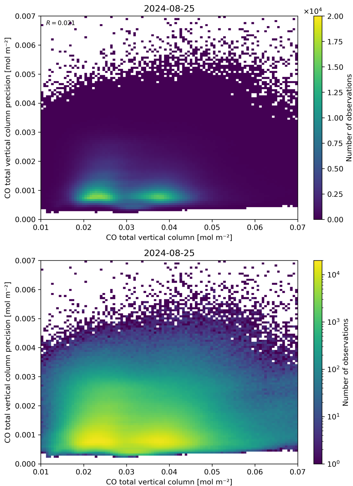
Figure 34: Scatter density plot of “CO total vertical column” against “CO total vertical column precision” for 2024-08-24 to 2024-08-26.
