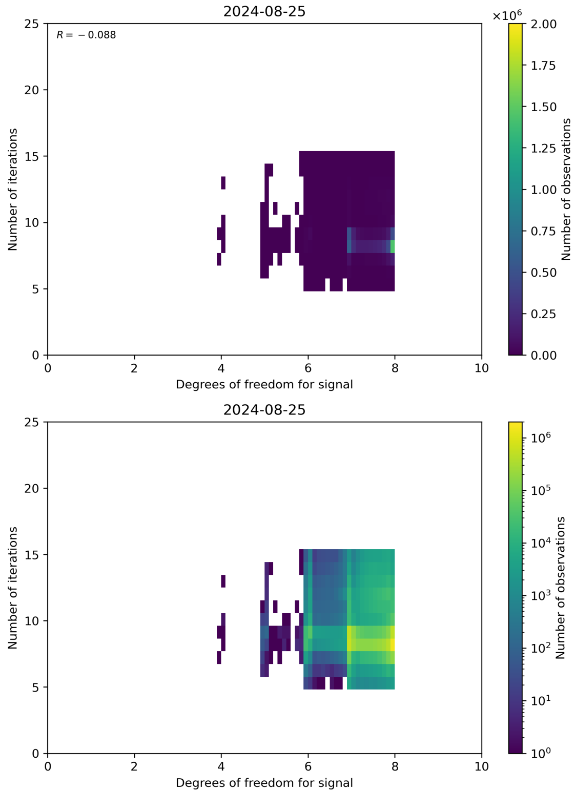
Figure 50: Scatter density plot of “Degrees of freedom for signal” against “Number of iterations” for 2024-08-24 to 2024-08-26.
