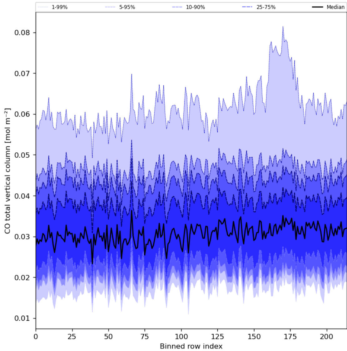
Figure 26: Along track statistics of “CO total vertical column” for 2024-08-24 to 2024-08-26
