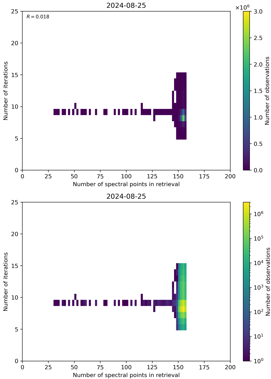
Figure 60: Scatter density plot of “Number of spectral points in retrieval” against “Number of iterations” for 2024-08-24 to 2024-08-26.
