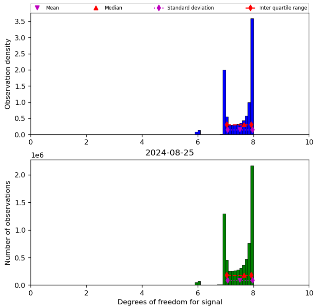
Figure 23: Histogram of “Degrees of freedom for signal” for 2024-08-24 to 2024-08-26
