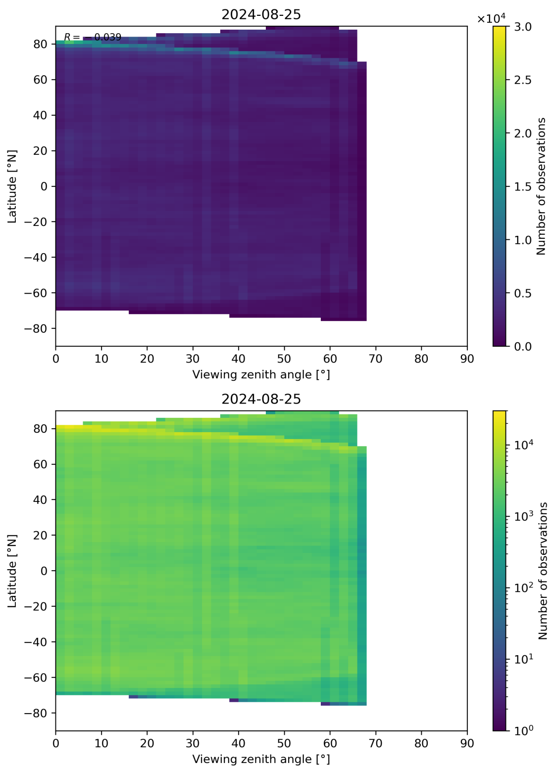
Figure 74: Scatter density plot of “Viewing zenith angle” against “Latitude” for 2024-08-24 to 2024-08-26.
