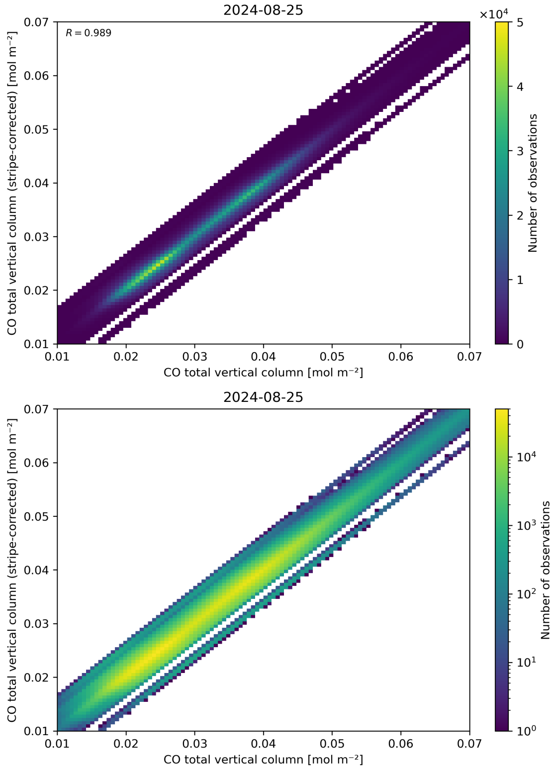
Figure 33: Scatter density plot of “CO total vertical column” against “CO total vertical column (stripe-corrected)” for 2024-08-24 to 2024-08-26.
