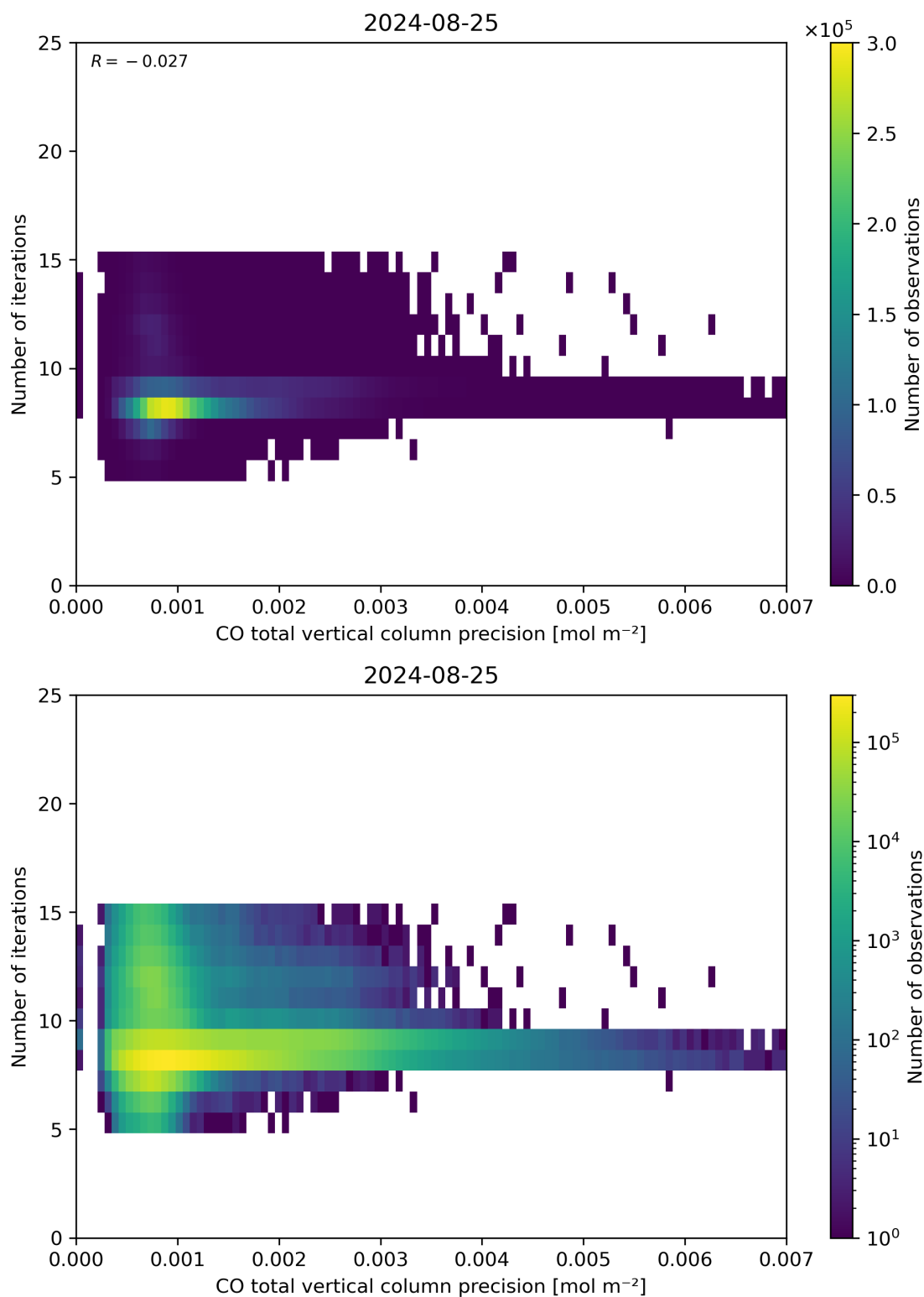
Figure 46: Scatter density plot of “CO total vertical column precision” against “Number of iterations” for 2024-08-24 to 2024-08-26.
