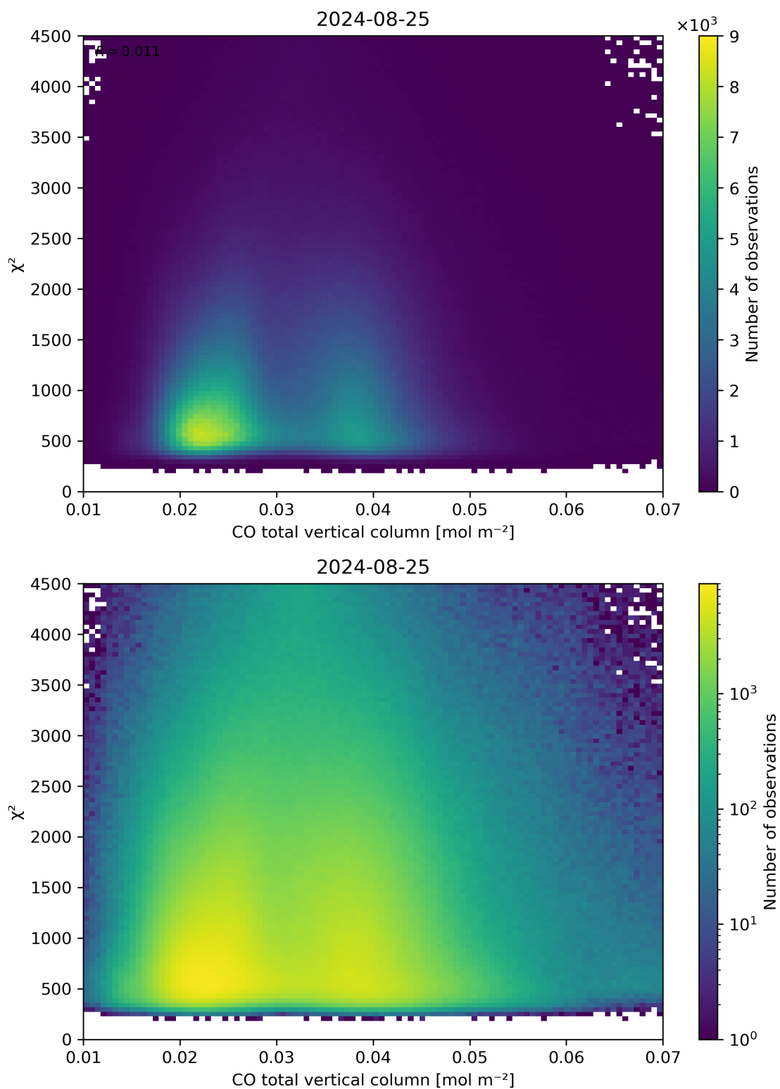
Figure 35: Scatter density plot of “CO total vertical column” against “ \chi^2 ” for 2024-08-24 to 2024-08-26.
