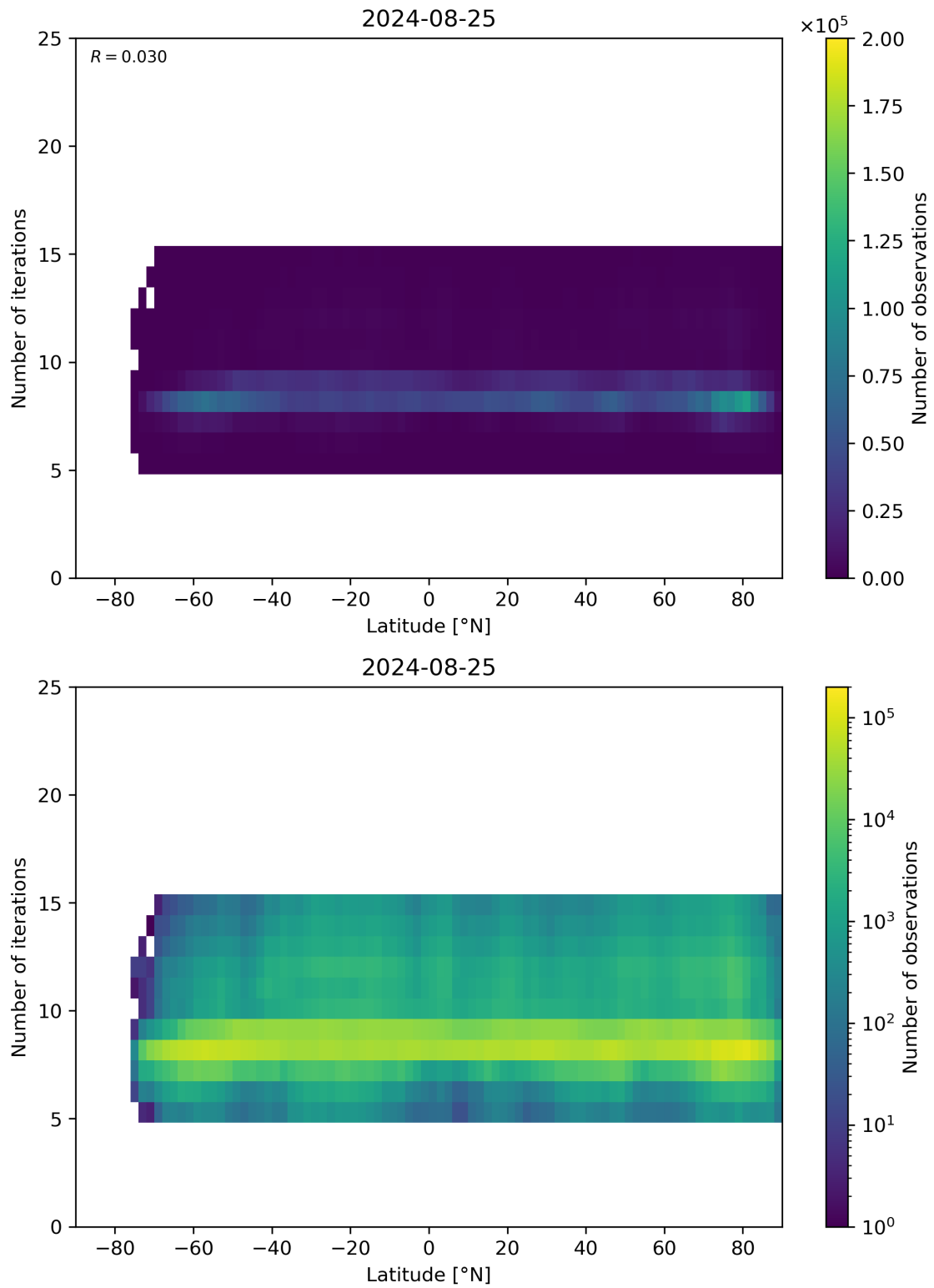
Figure 56: Scatter density plot of “Latitude” against “Number of iterations” for 2024-08-24 to 2024-08-26.
