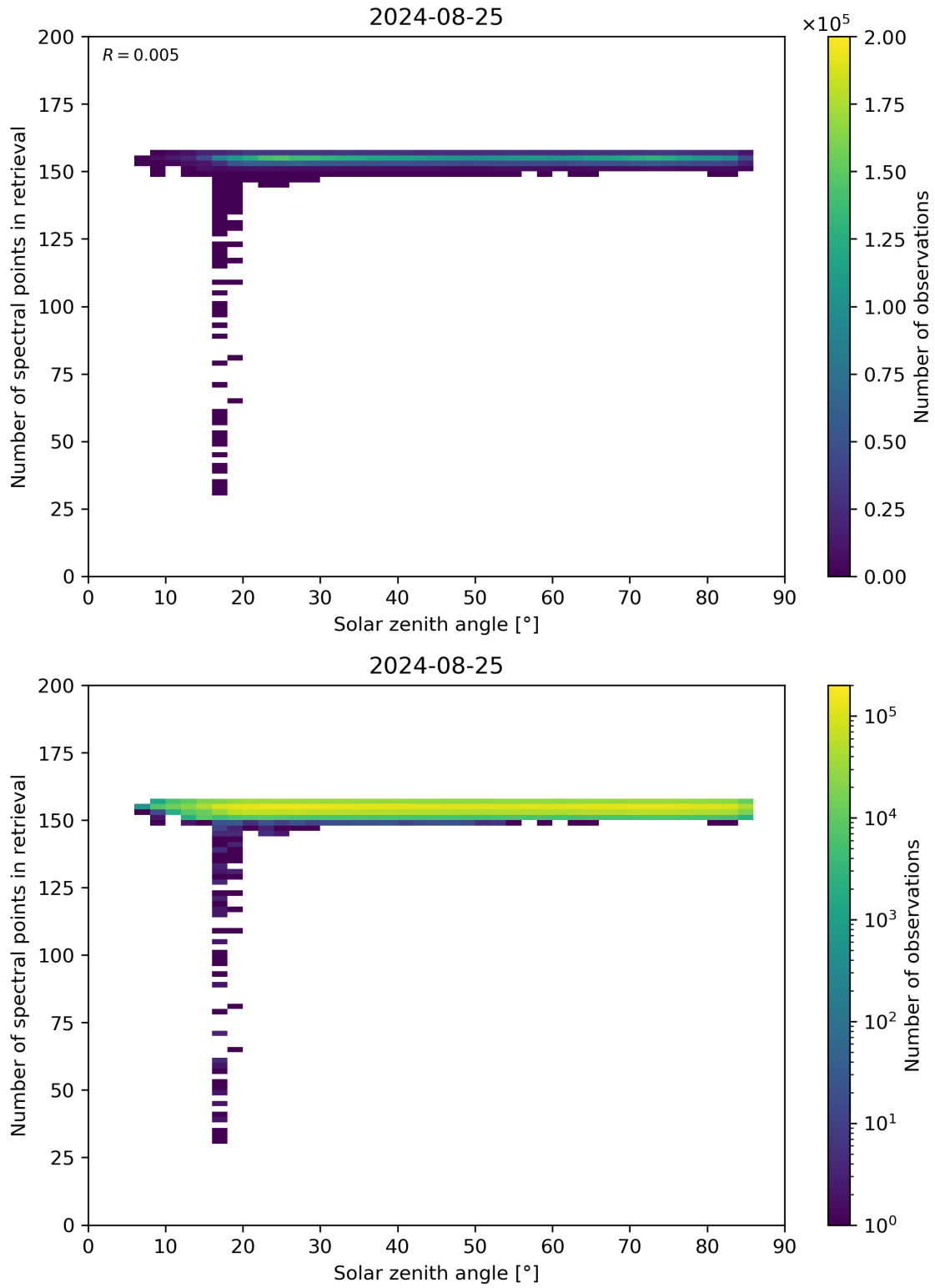
Figure 68: Scatter density plot of “Solar zenith angle” against “Number of spectral points in retrieval” for 2024-08-24 to 2024-08-26.
