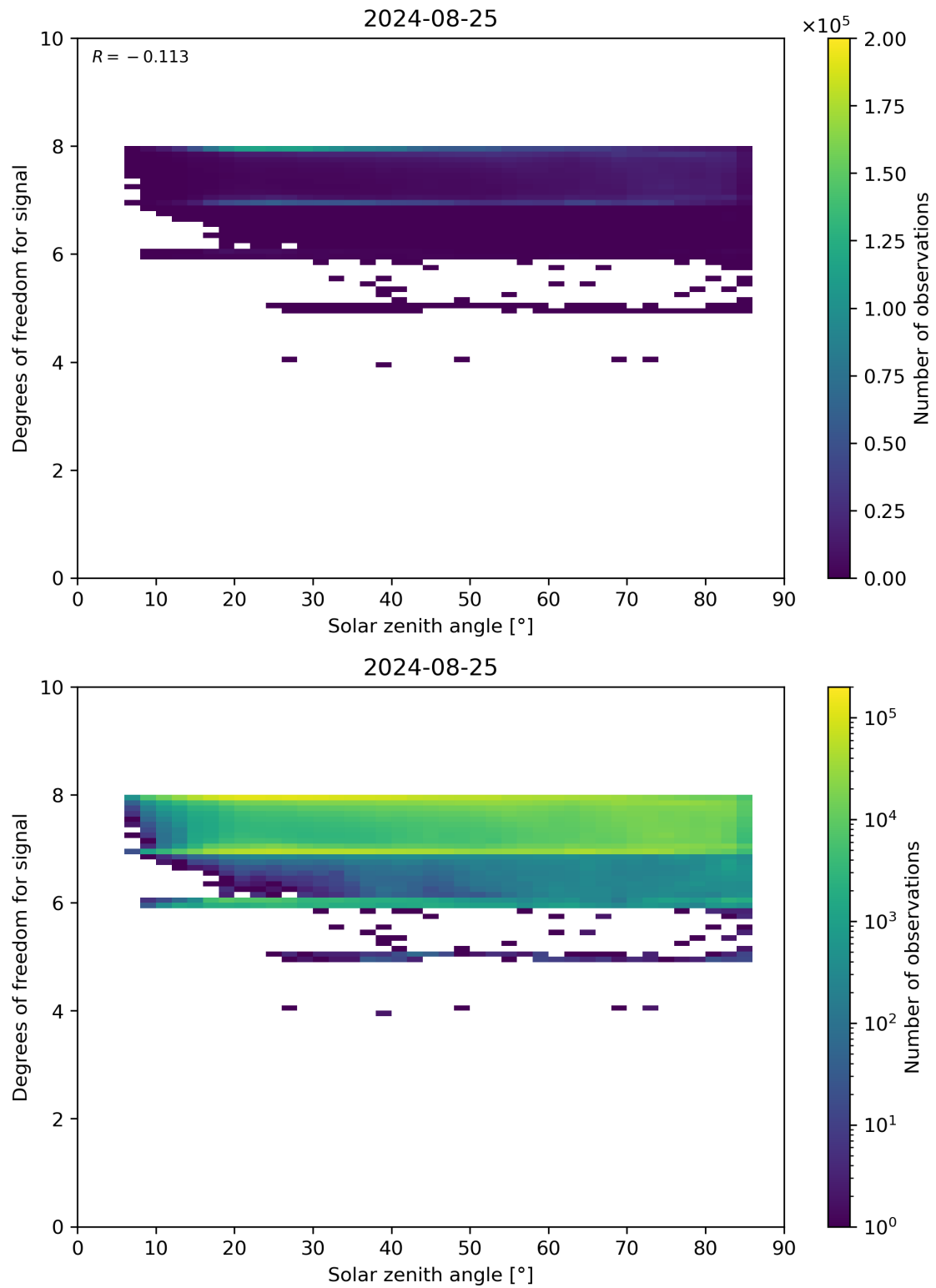
Figure 65: Scatter density plot of “Solar zenith angle” against “Degrees of freedom for signal” for 2024-08-24 to 2024-08-26.
