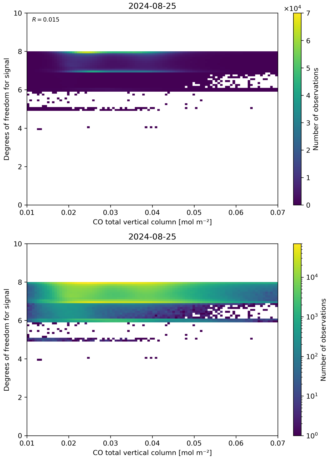
Figure 41: Scatter density plot of “CO total vertical column” against “Degrees of freedom for signal” for 2024-08-24 to 2024-08-26.
