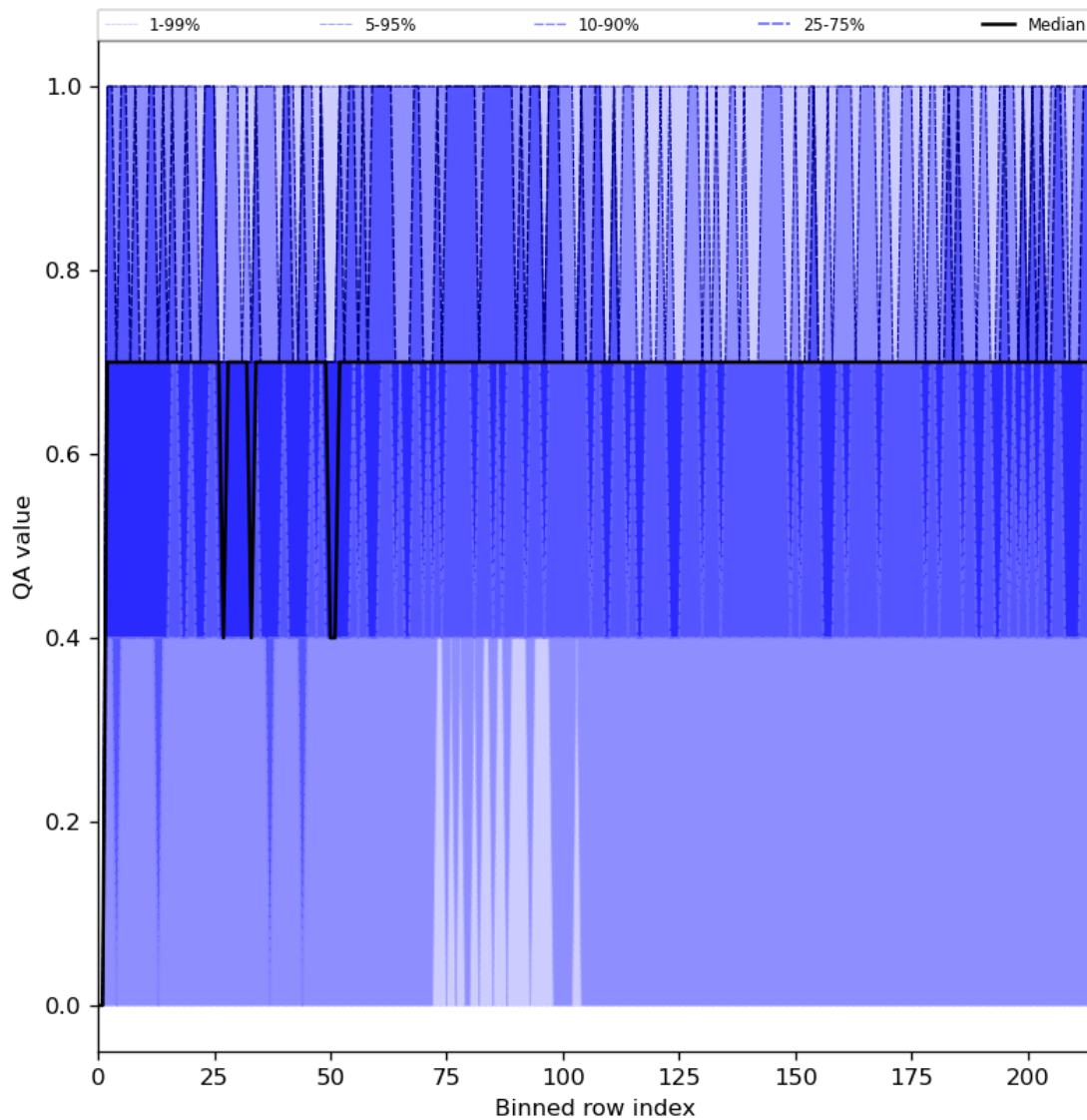
Figure 25: Along track statistics of “QA value” for 2024-08-24 to 2024-08-26
