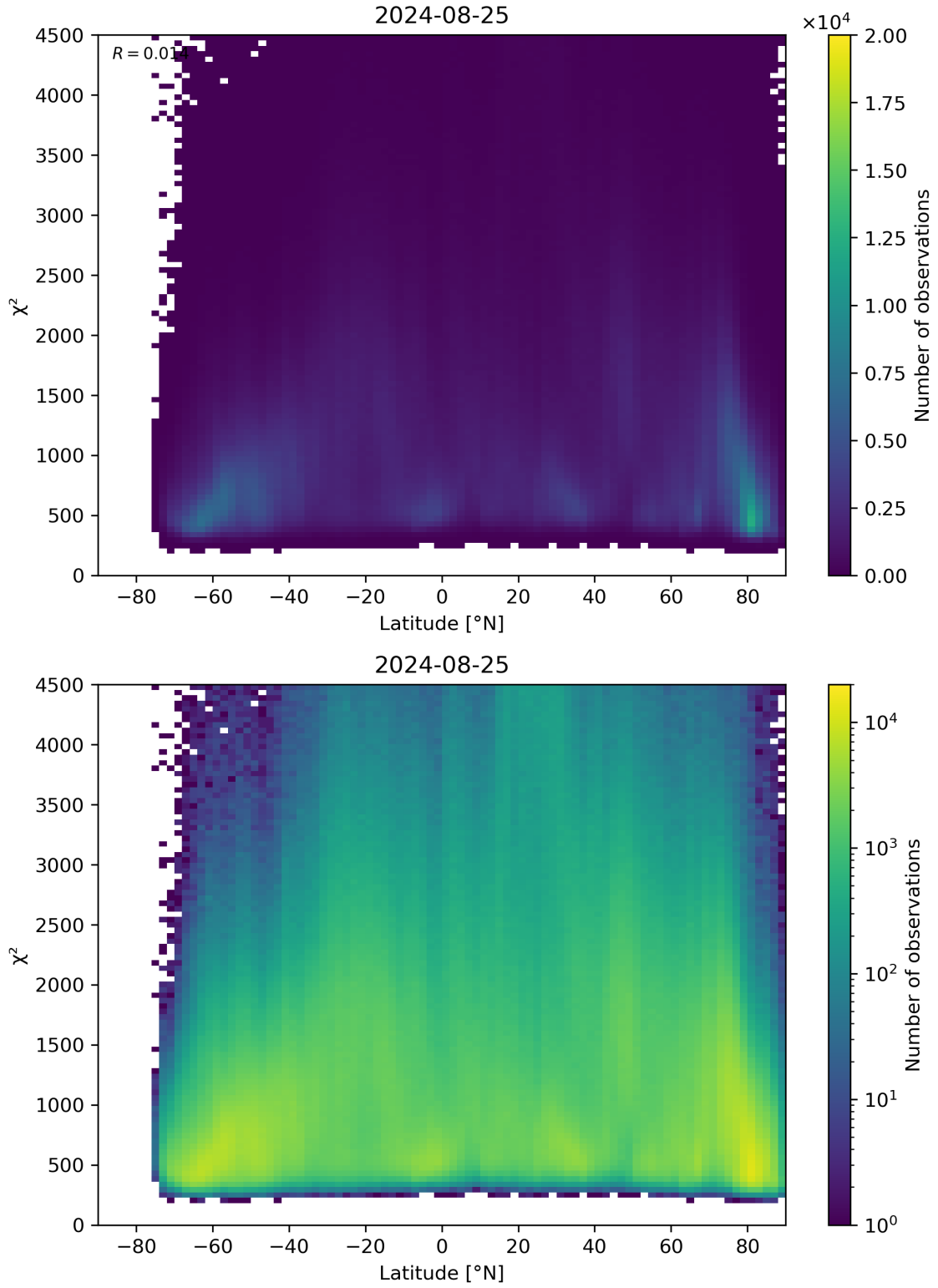
Figure 54: Scatter density plot of “Latitude” against “ \chi^2 ” for 2024-08-24 to 2024-08-26.
