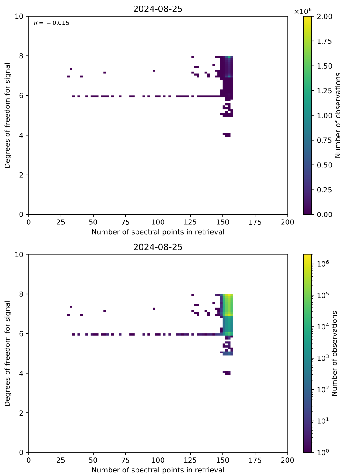
Figure 59: Scatter density plot of “Number of spectral points in retrieval” against “Degrees of freedom for signal” for 2024-08-24 to 2024-08-26.
