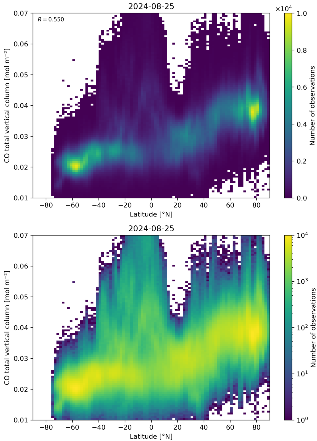
Figure 51: Scatter density plot of “Latitude” against “CO total vertical column” for 2024-08-24 to 2024-08-26.
