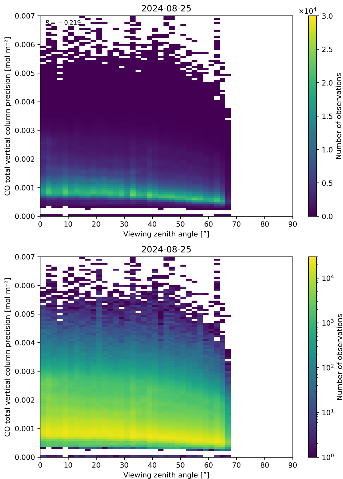
Figure 71: Scatter density plot of “Viewing zenith angle” against “CO total vertical column precision” for 2024-08-24 to 2024-08-26.
