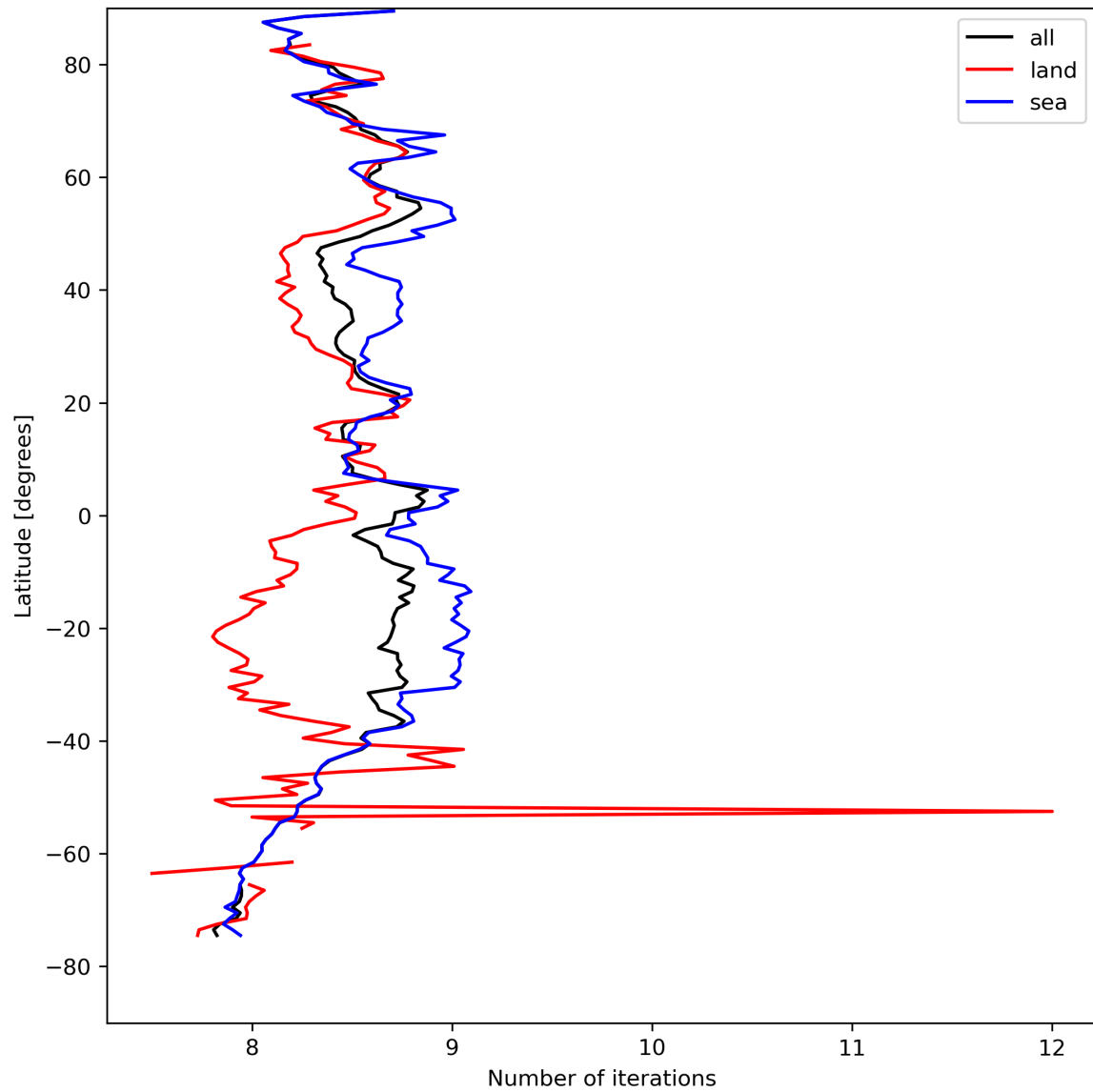
Figure 16: Zonal average of “Number of iterations” for 2024-08-24 to 2024-08-26.
