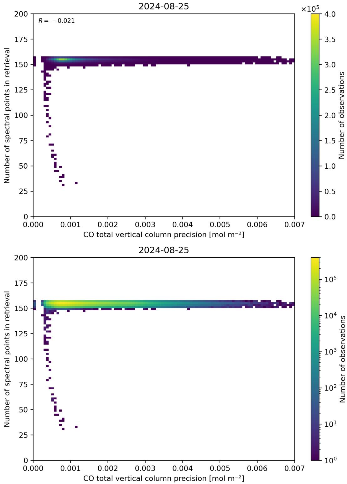
Figure 47: Scatter density plot of “CO total vertical column precision” against “Number of spectral points in retrieval” for 2024-08-24 to 2024-08-26.
