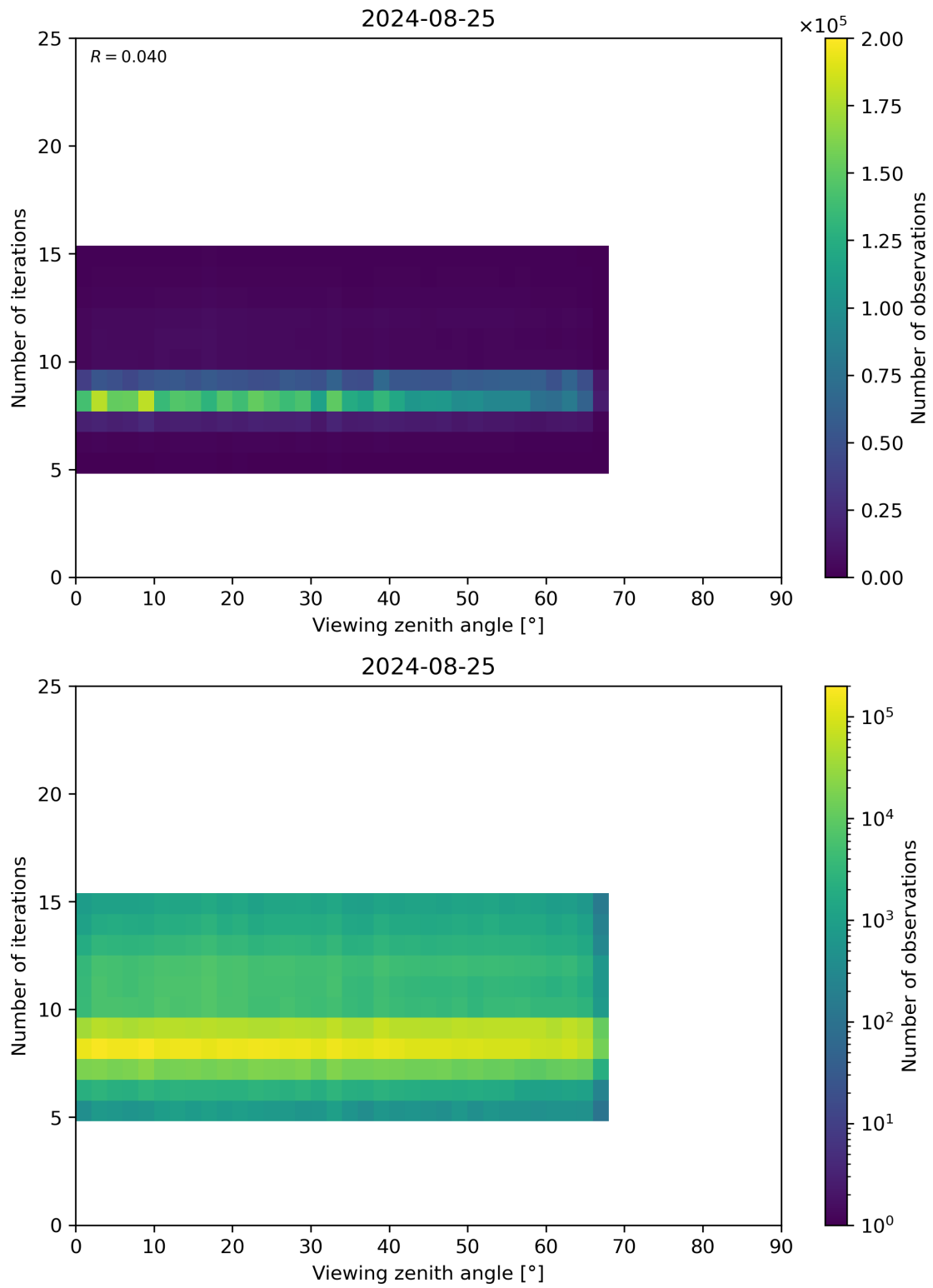
Figure 75: Scatter density plot of “Viewing zenith angle” against “Number of iterations” for 2024-08-24 to 2024-08-26.
