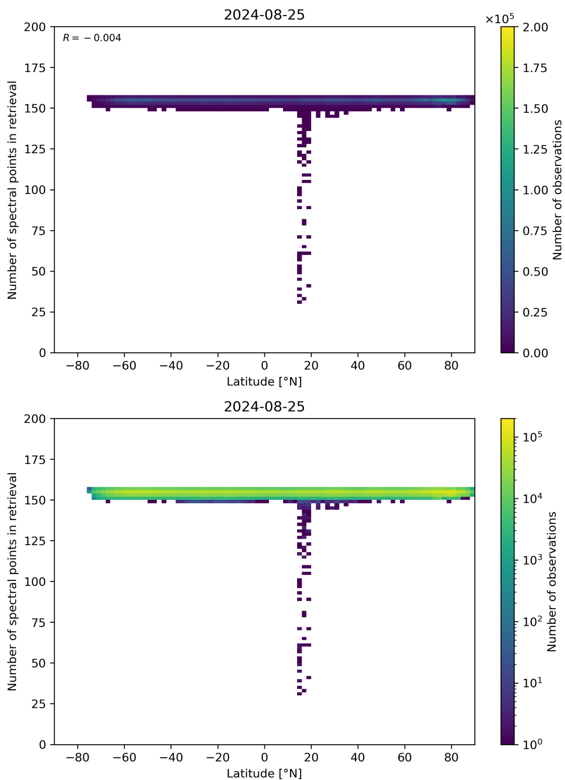
Figure 57: Scatter density plot of “Latitude” against “Number of spectral points in retrieval” for 2024-08-24 to 2024-08-26.
