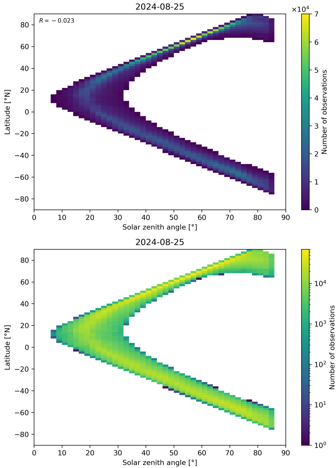
Figure 66: Scatter density plot of “Solar zenith angle” against “Latitude” for 2024-08-24 to 2024-08-26.
