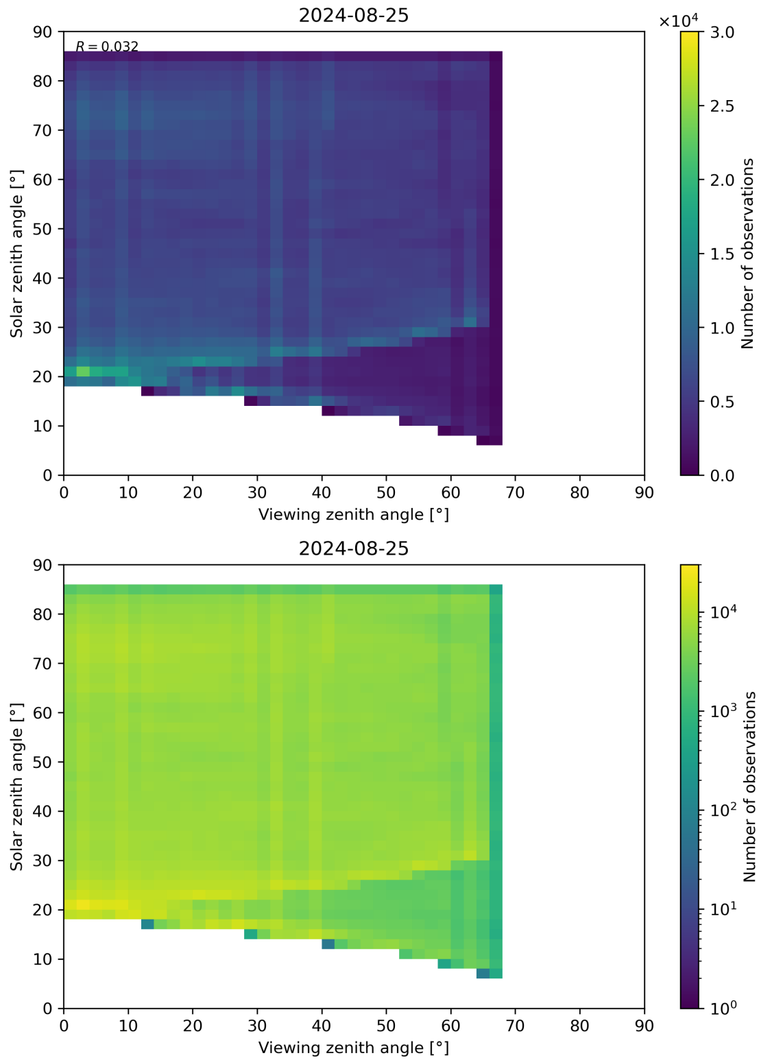
Figure 77: Scatter density plot of “Viewing zenith angle” against “Solar zenith angle” for 2024-08-24 to 2024-08-26.
