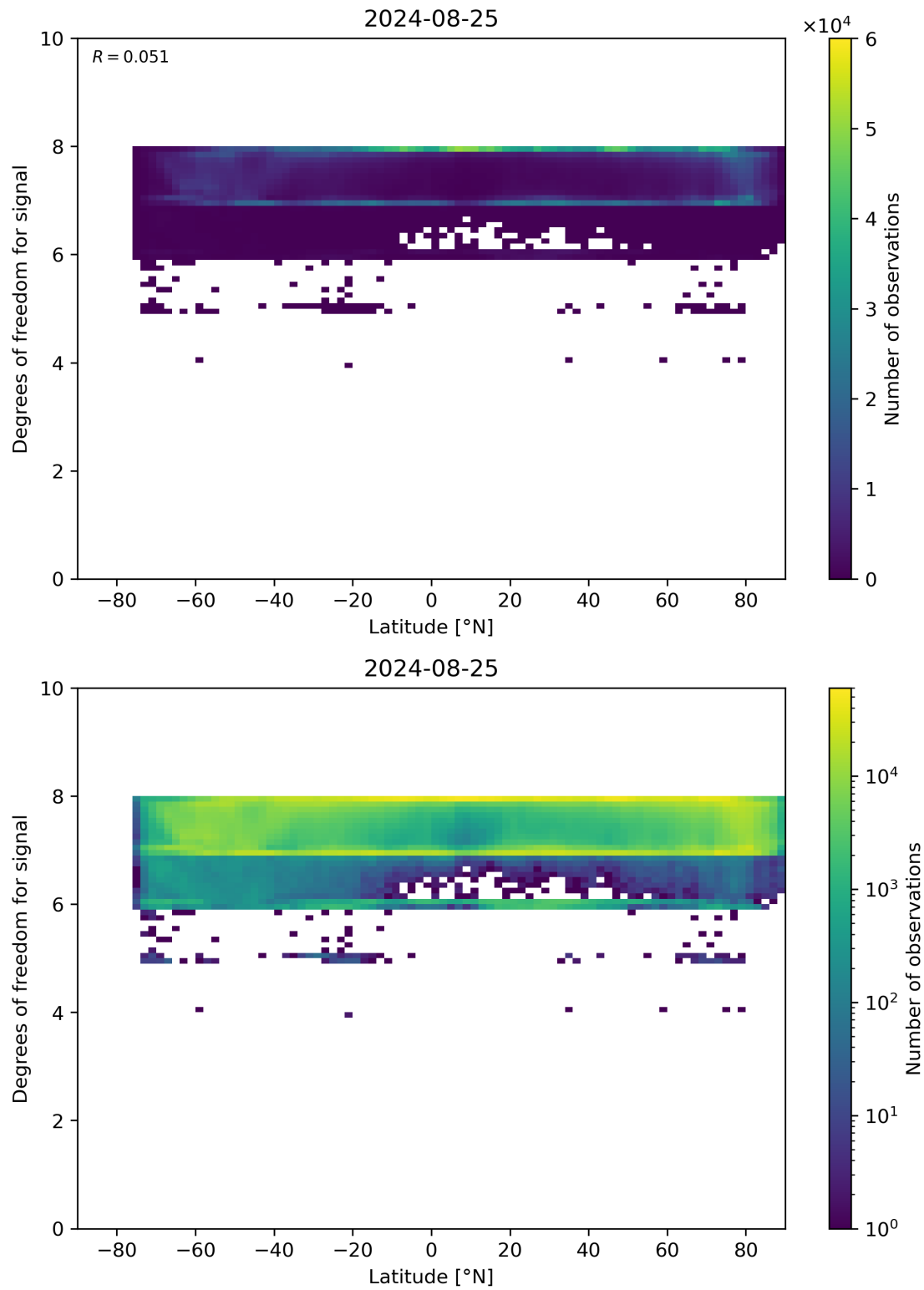
Figure 55: Scatter density plot of “Latitude” against “Degrees of freedom for signal” for 2024-08-24 to 2024-08-26.
