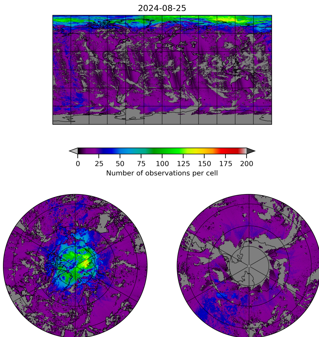
Figure 8: Map of the number of observations for 2024-08-24 to 2024-08-26
