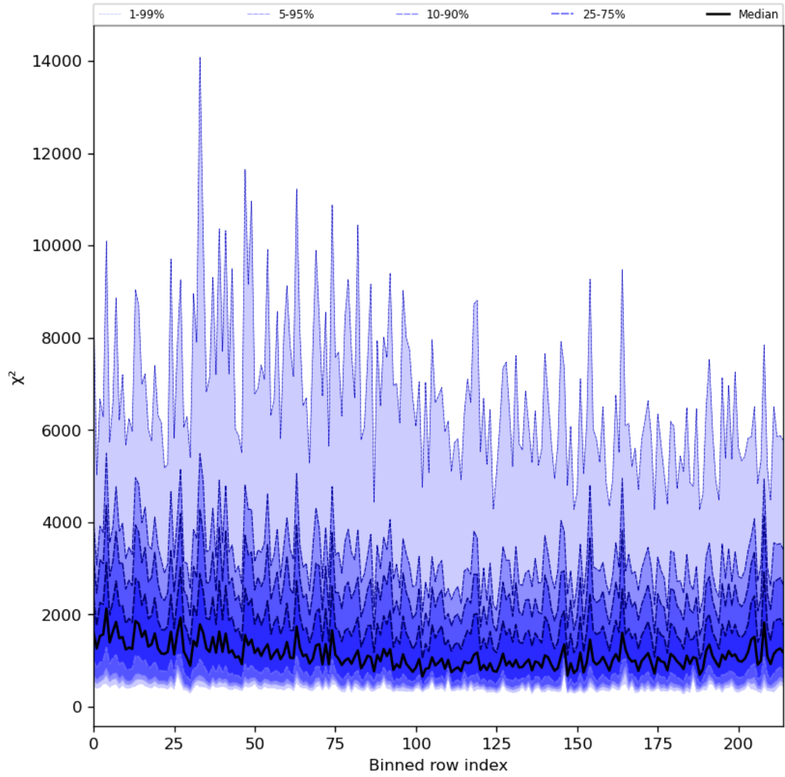
Figure 30: Along track statistics of “ \chi^2 ” for 2024-08-24 to 2024-08-26
