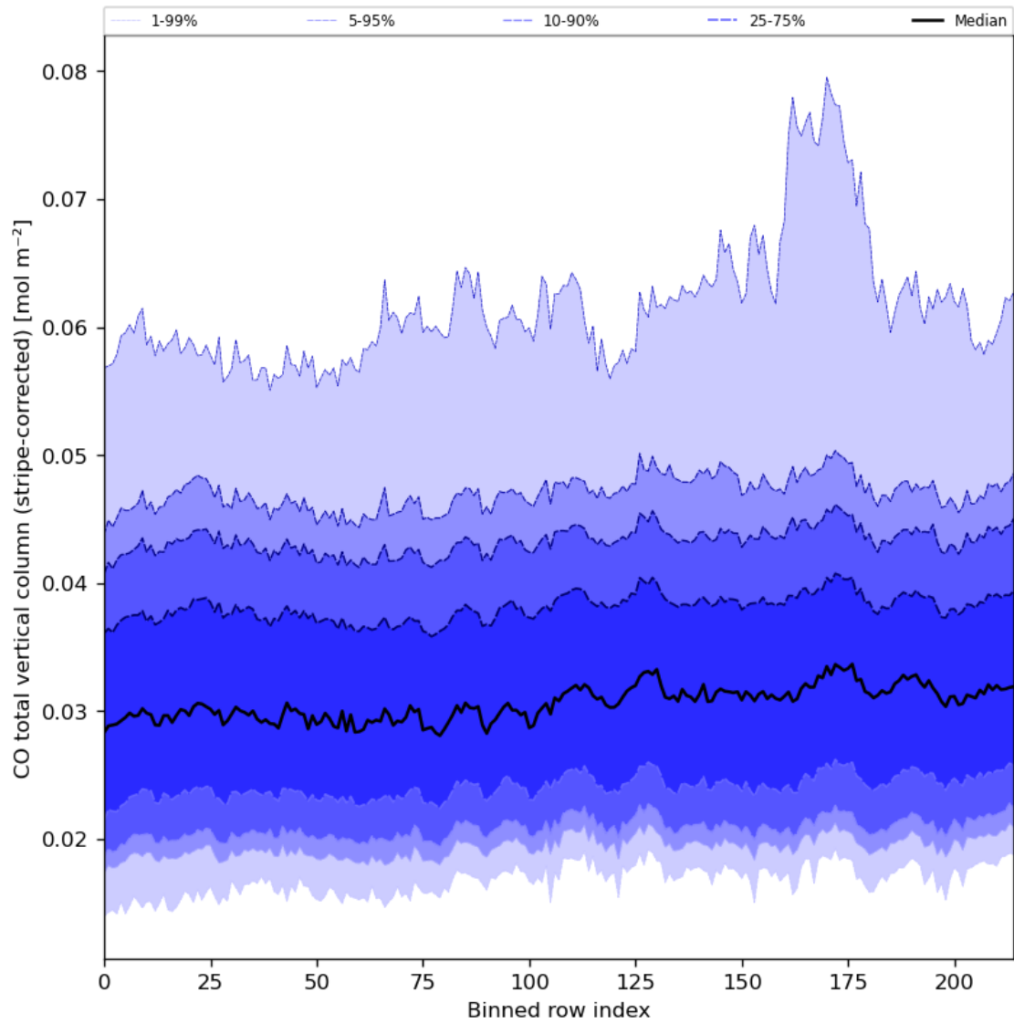
Figure 27: Along track statistics of “CO total vertical column (stripe-corrected)” for 2024-08-24 to 2024-08-26
