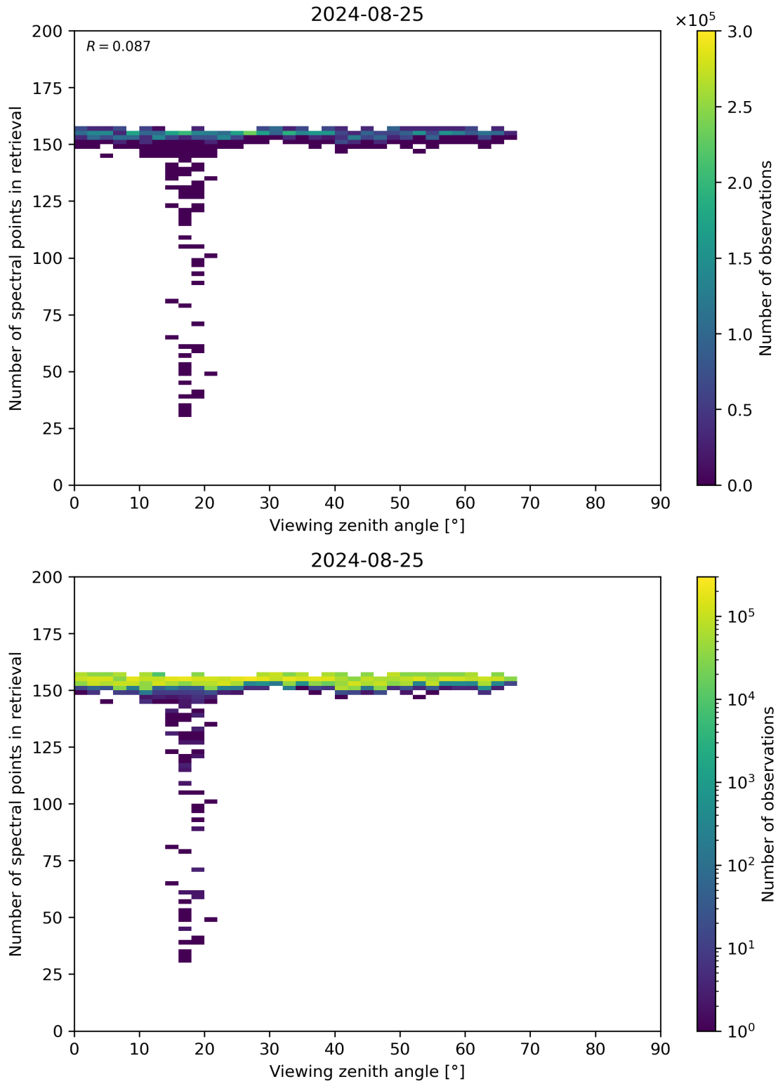
Figure 76: Scatter density plot of “Viewing zenith angle” against “Number of spectral points in retrieval” for 2024-08-24 to 2024-08-26.
