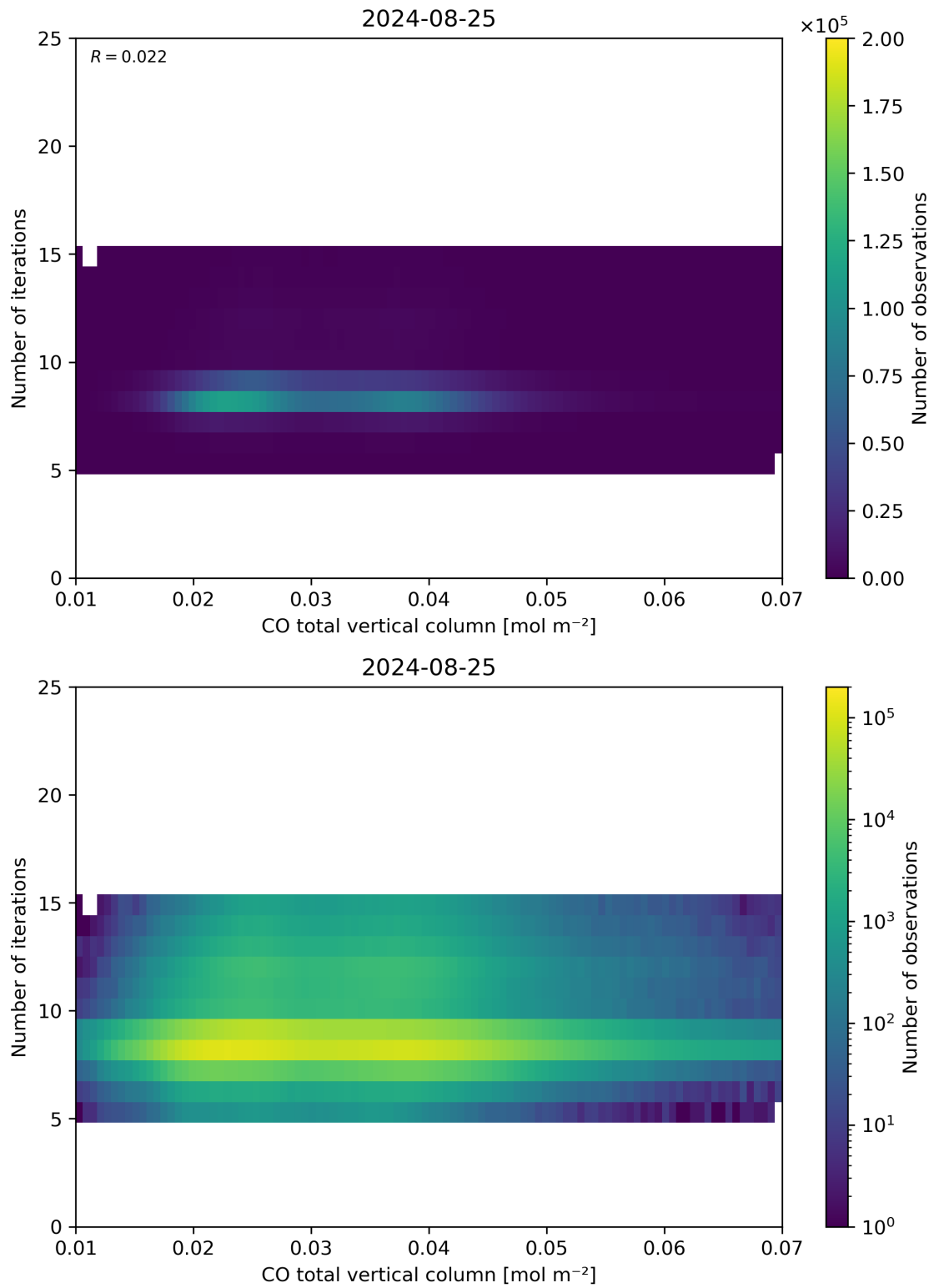
Figure 42: Scatter density plot of “CO total vertical column” against “Number of iterations” for 2024-08-24 to 2024-08-26.
