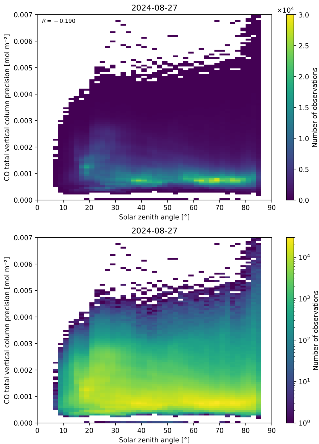
Figure 63: Scatter density plot of “Solar zenith angle” against “CO total vertical column precision” for 2024-08-27 to 2024-08-28.
