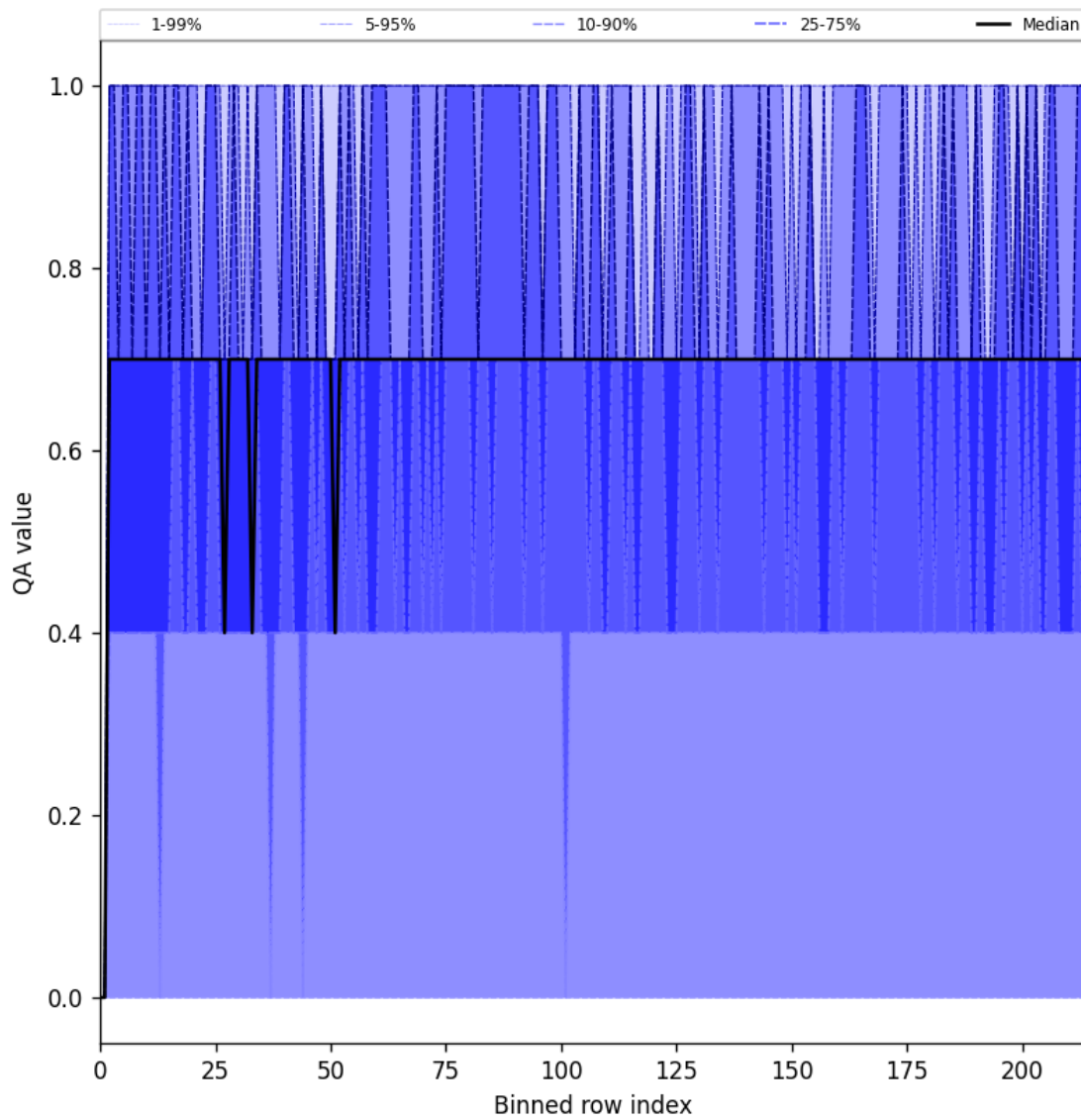
Figure 25: Along track statistics of “QA value” for 2024-08-27 to 2024-08-28
