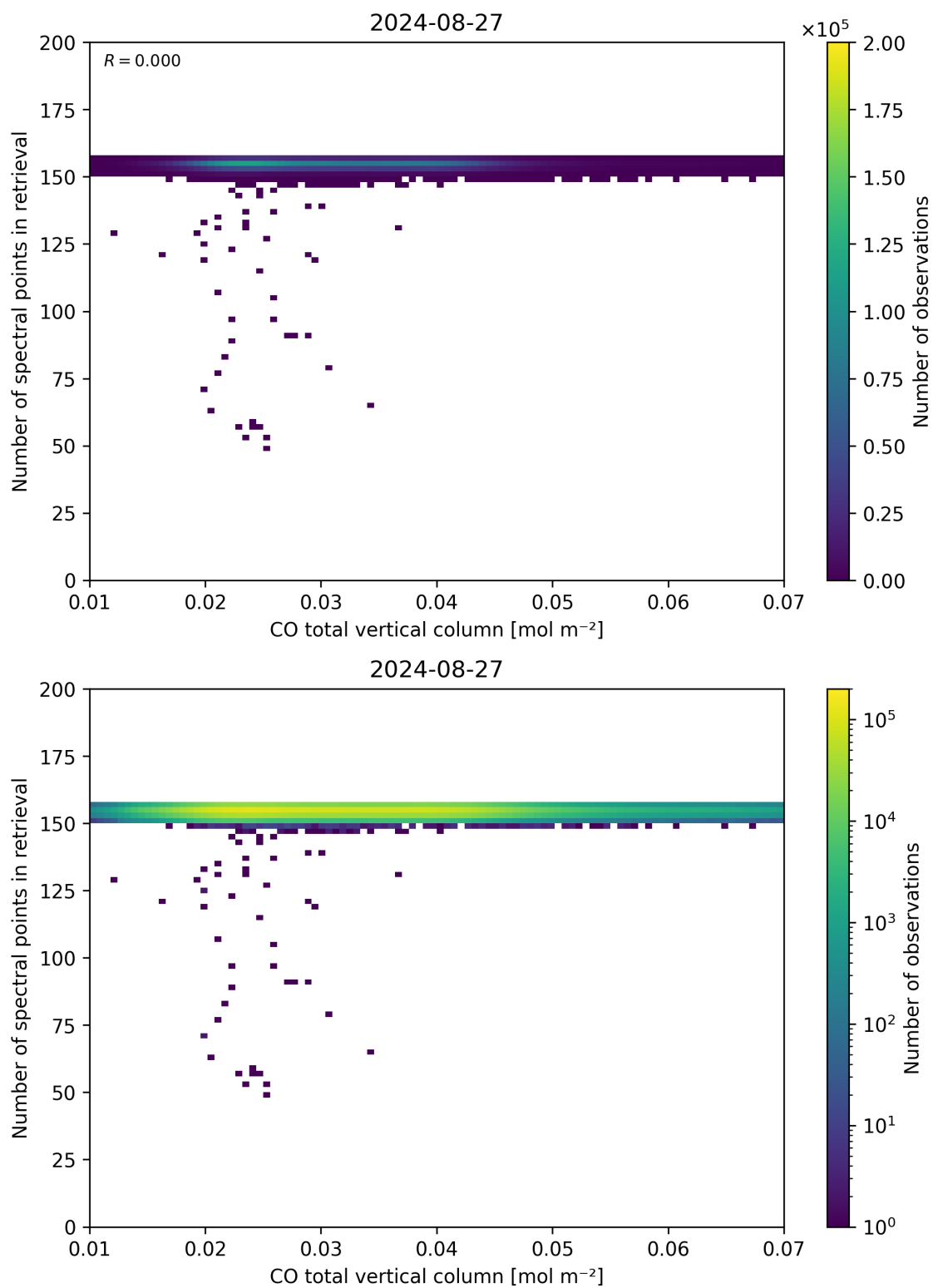
Figure 43: Scatter density plot of “CO total vertical column” against “Number of spectral points in retrieval” for 2024-08-27 to 2024-08-28.
