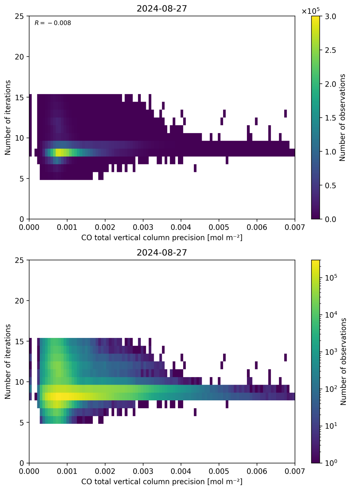
Figure 46: Scatter density plot of “CO total vertical column precision” against “Number of iterations” for 2024-08-27 to 2024-08-28.
