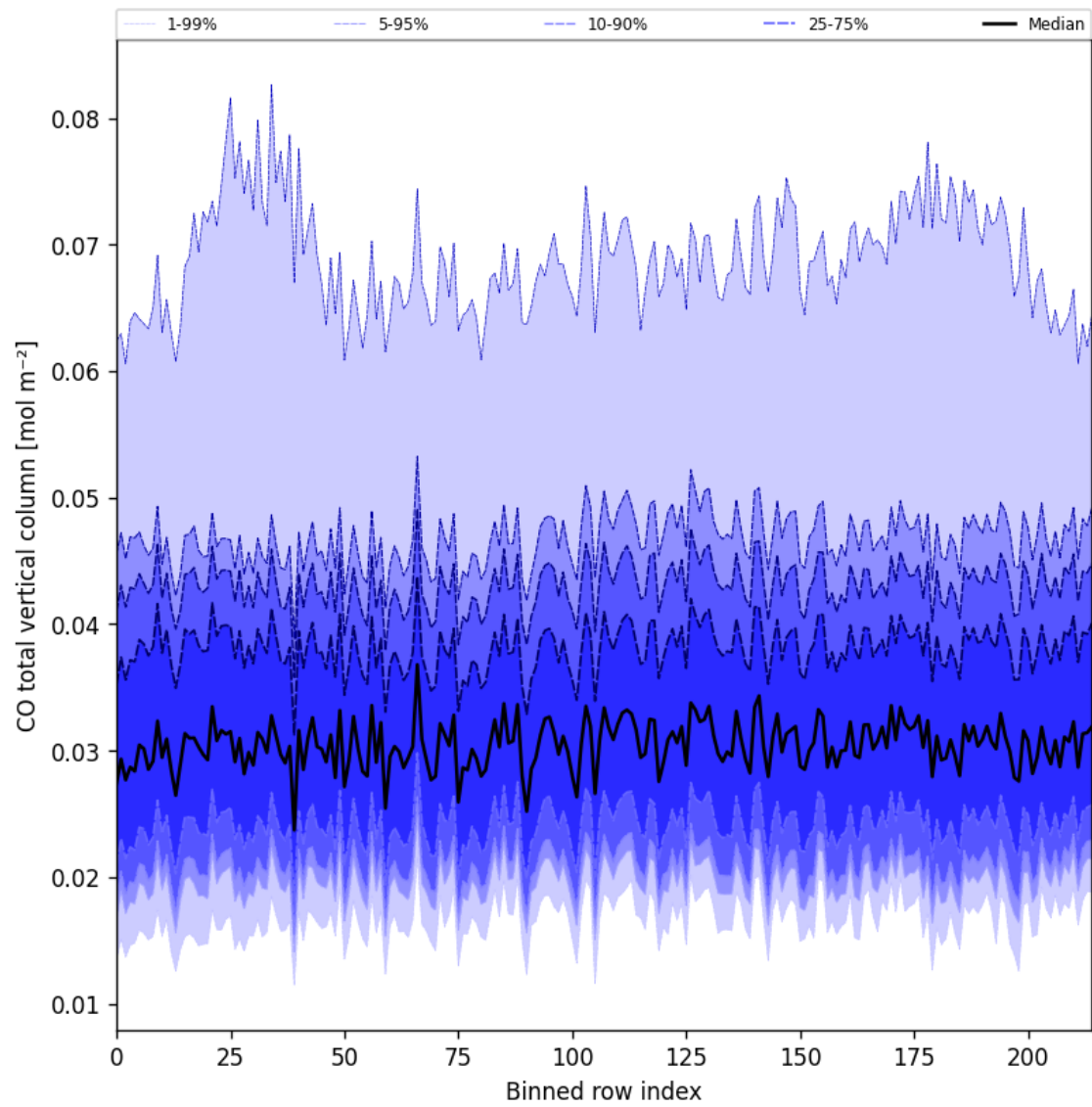
Figure 26: Along track statistics of “CO total vertical column” for 2024-08-27 to 2024-08-28
