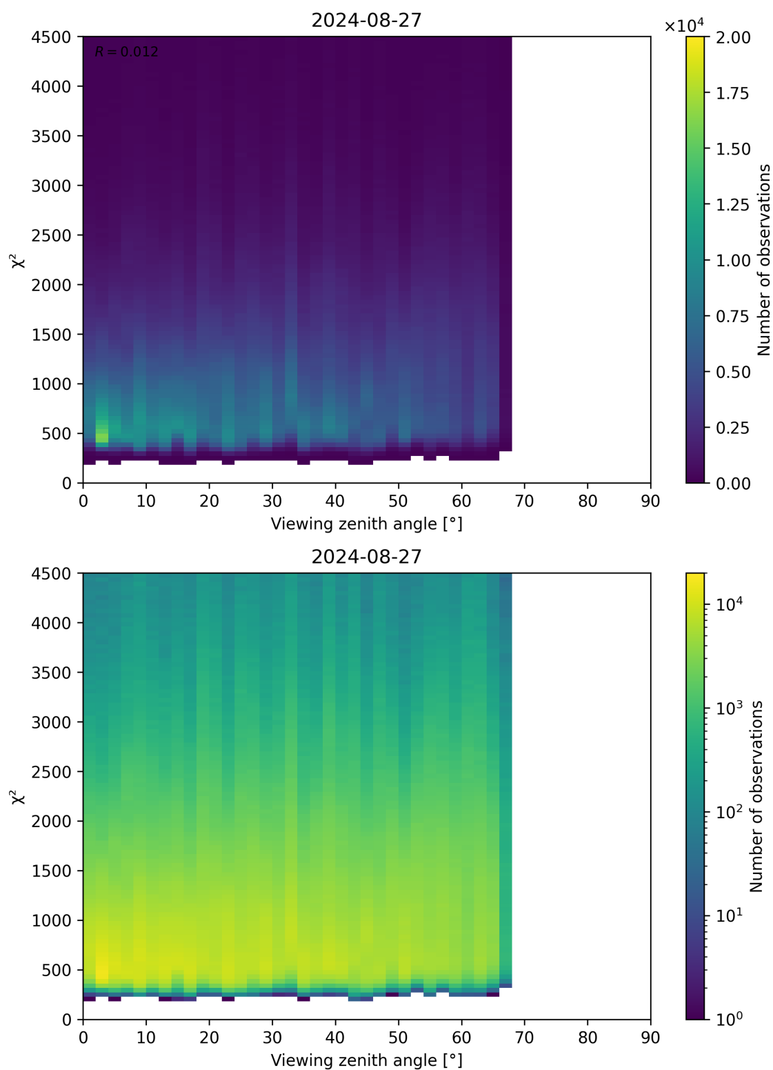
Figure 72: Scatter density plot of “Viewing zenith angle” against “ \chi^2 ” for 2024-08-27 to 2024-08-28.
