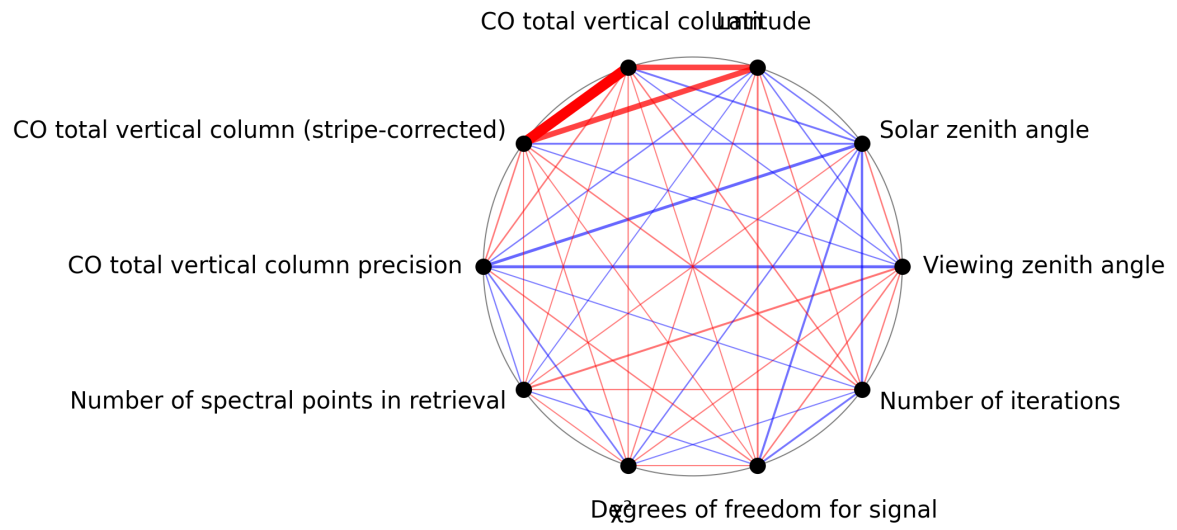
Figure 1: Map of correlation graph for 2024-08-27 to 2024-08-28.
