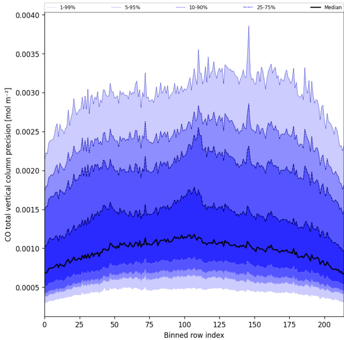
Figure 28: Along track statistics of “CO total vertical column precision” for 2024-08-27 to 2024-08-28
