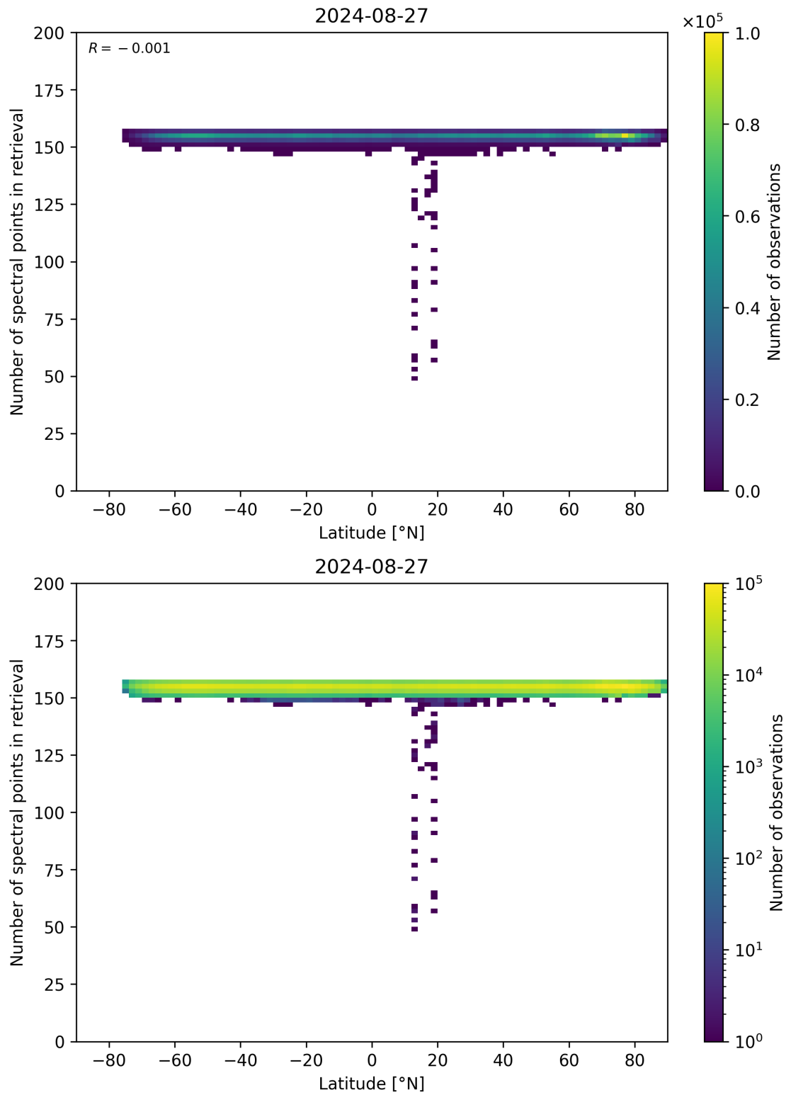
Figure 57: Scatter density plot of “Latitude” against “Number of spectral points in retrieval” for 2024-08-27 to 2024-08-28.
