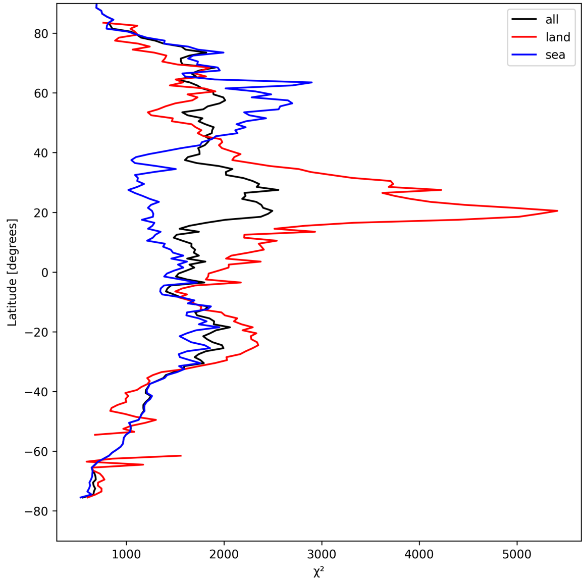
Figure 14: Zonal average of “ \chi^2 ” for 2024-08-27 to 2024-08-28.
