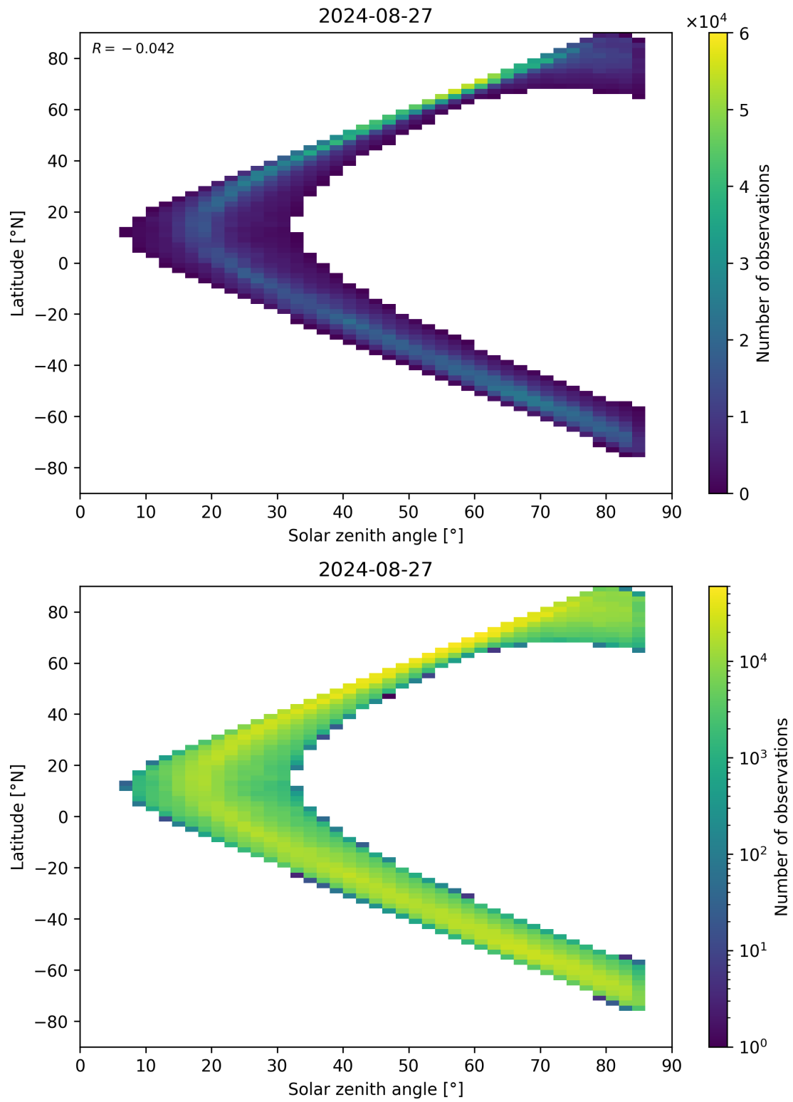
Figure 66: Scatter density plot of “Solar zenith angle” against “Latitude” for 2024-08-27 to 2024-08-28.
