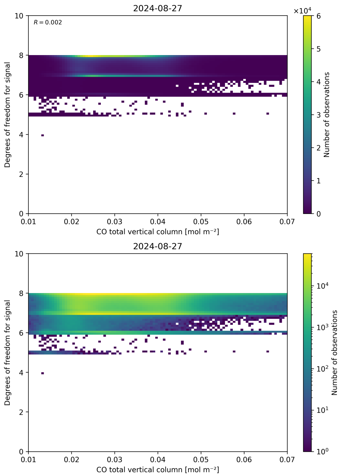
Figure 41: Scatter density plot of “CO total vertical column” against “Degrees of freedom for signal” for 2024-08-27 to 2024-08-28.
