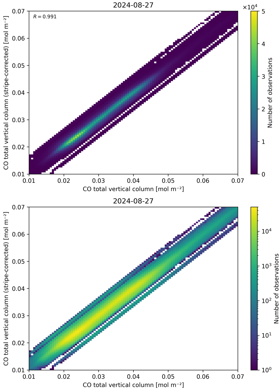
Figure 33: Scatter density plot of “CO total vertical column” against “CO total vertical column (stripe-corrected)” for 2024-08-27 to 2024-08-28.
