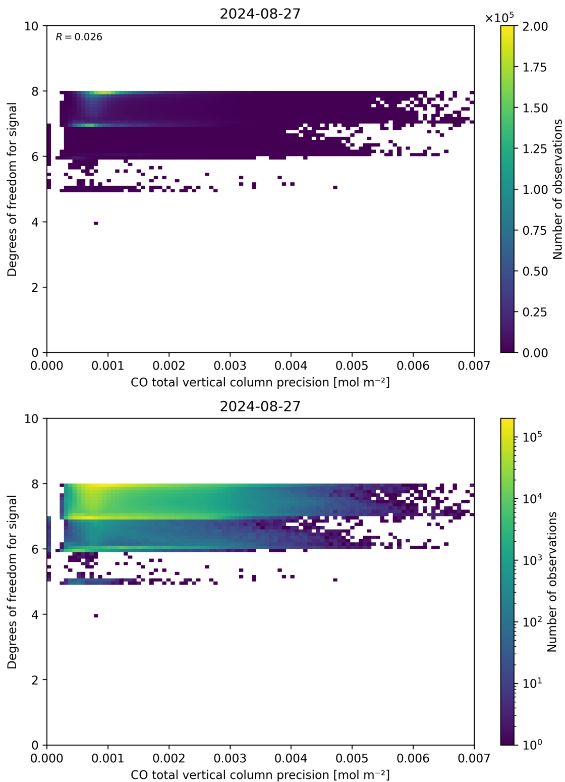
Figure 45: Scatter density plot of “CO total vertical column precision” against “Degrees of freedom for signal” for 2024-08-27 to 2024-08-28.
