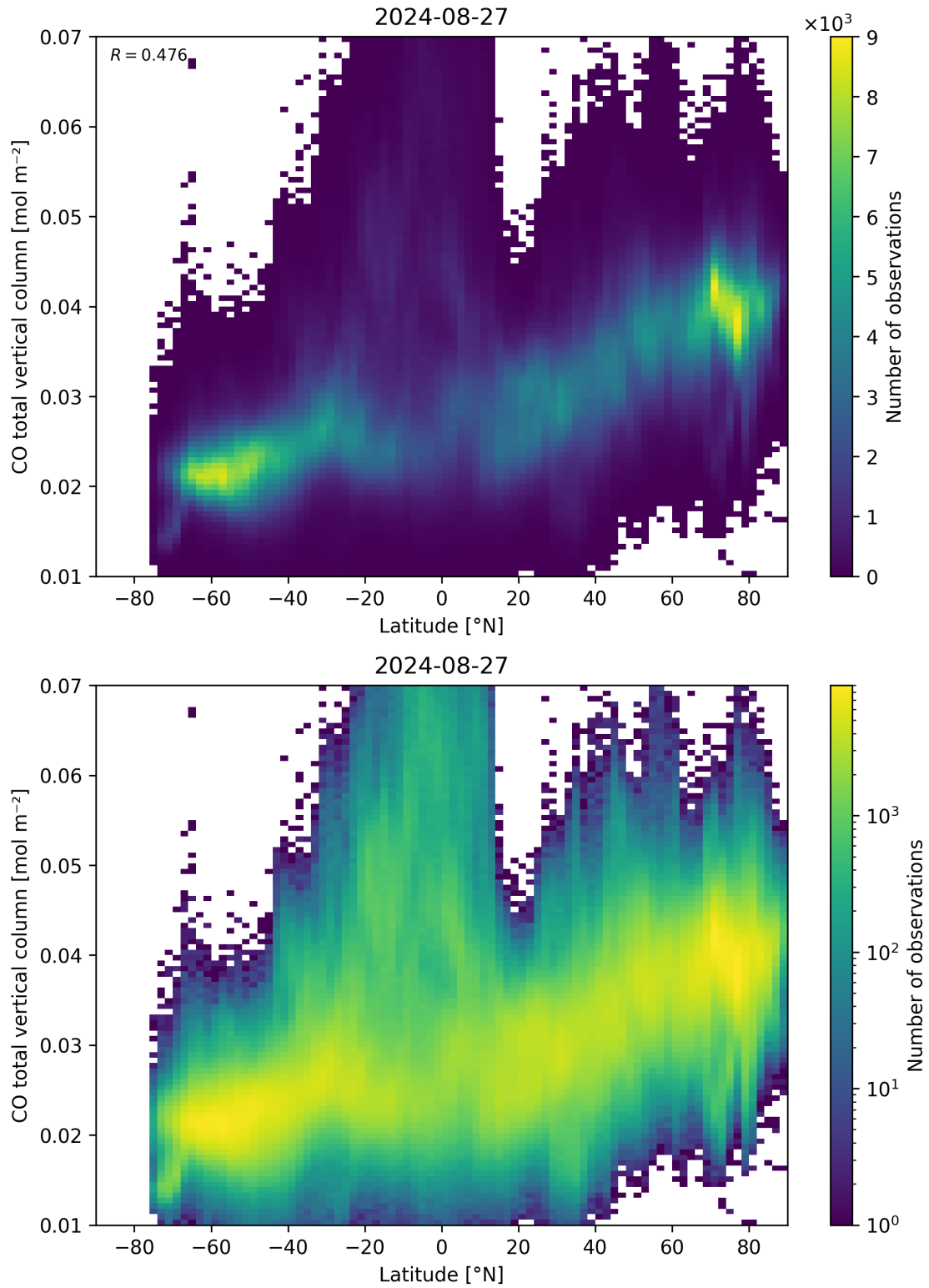
Figure 51: Scatter density plot of “Latitude” against “CO total vertical column” for 2024-08-27 to 2024-08-28.
