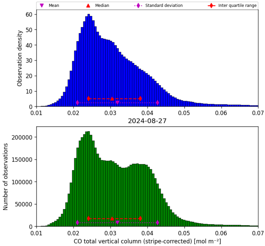
Figure 19: Histogram of “CO total vertical column (stripe-corrected)” for 2024-08-27 to 2024-08-28
