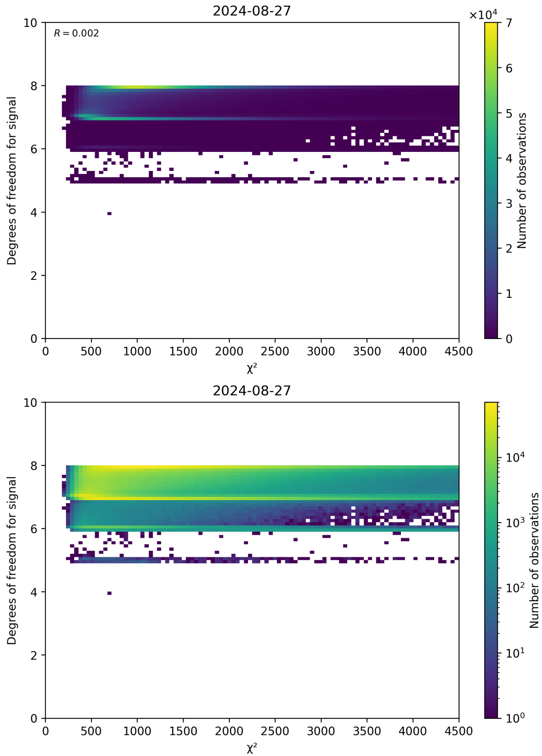
Figure 48: Scatter density plot of “ \chi^2 ” against “Degrees of freedom for signal” for 2024-08-27 to 2024-08-28.
