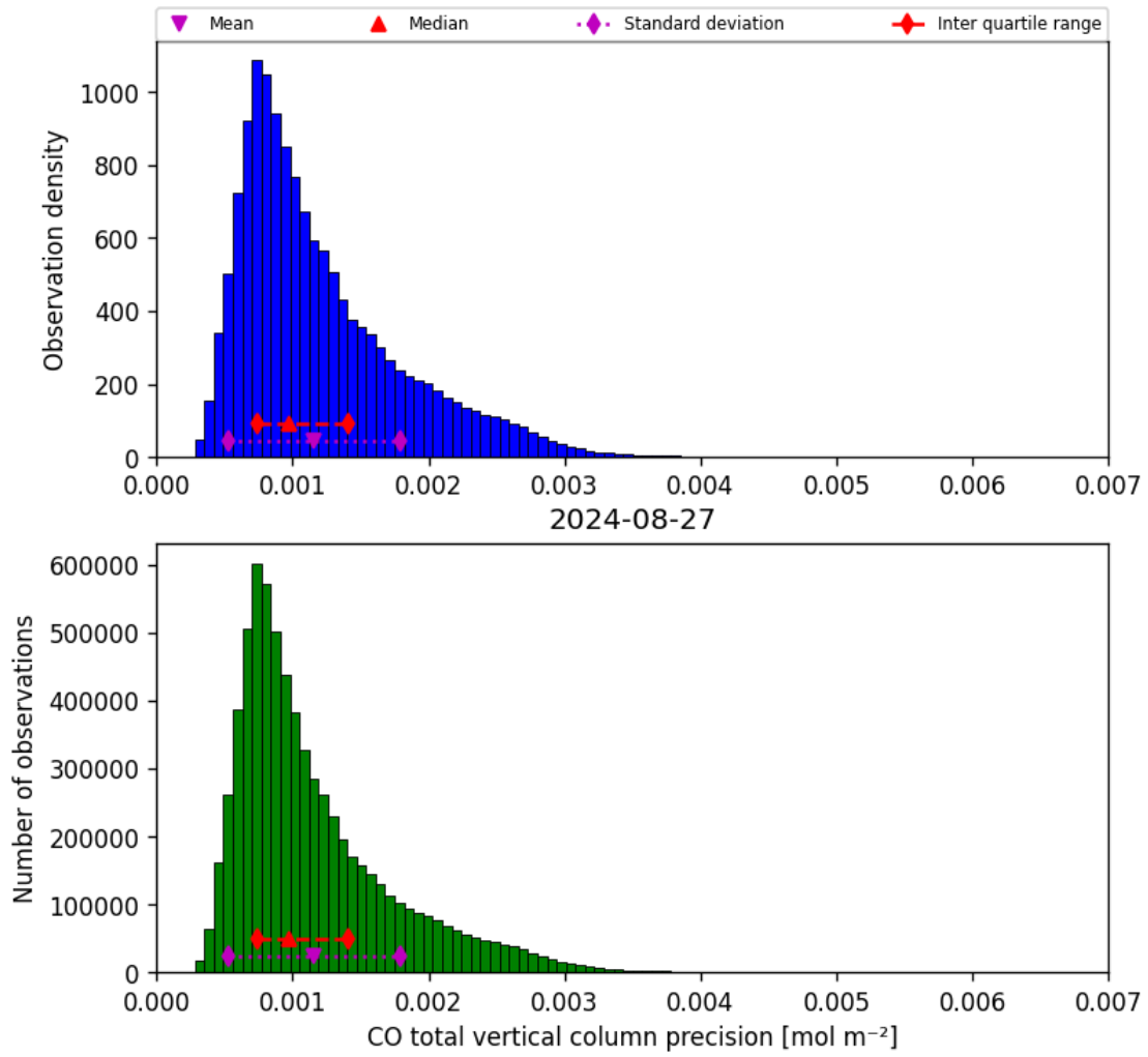
Figure 20: Histogram of “CO total vertical column precision” for 2024-08-27 to 2024-08-28
