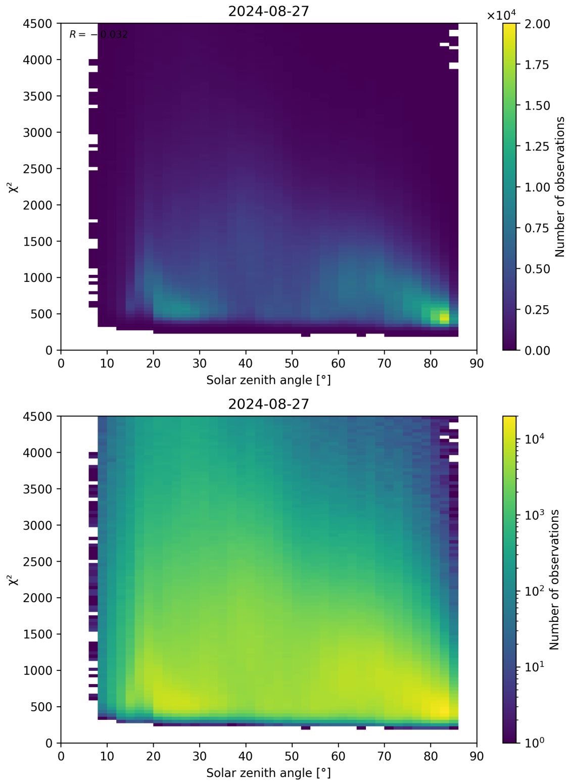
Figure 64: Scatter density plot of “Solar zenith angle” against “ \chi^2 ” for 2024-08-27 to 2024-08-28.
