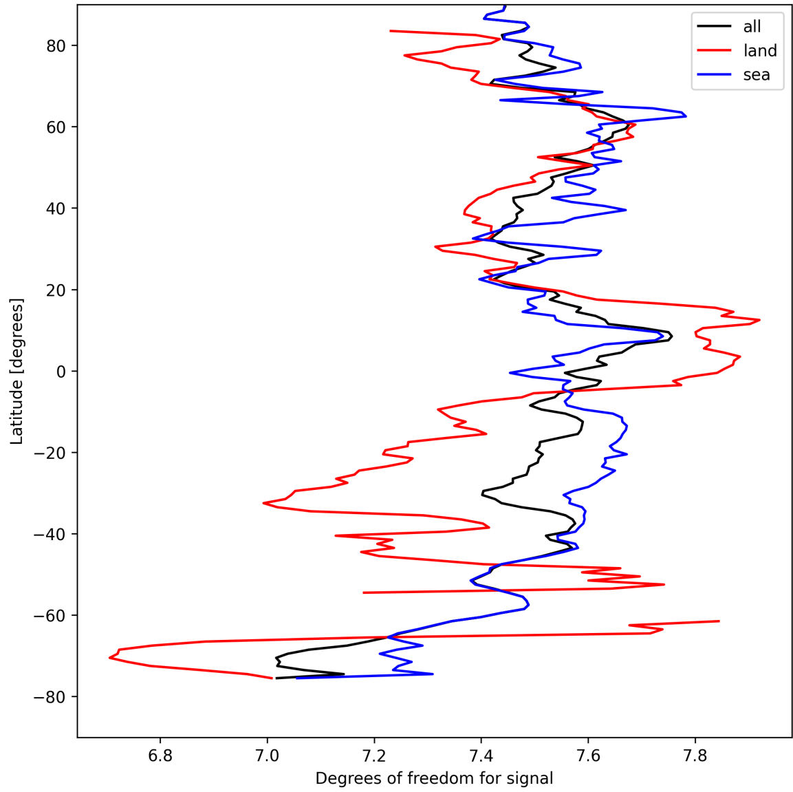
Figure 15: Zonal average of “Degrees of freedom for signal” for 2024-08-27 to 2024-08-28.
