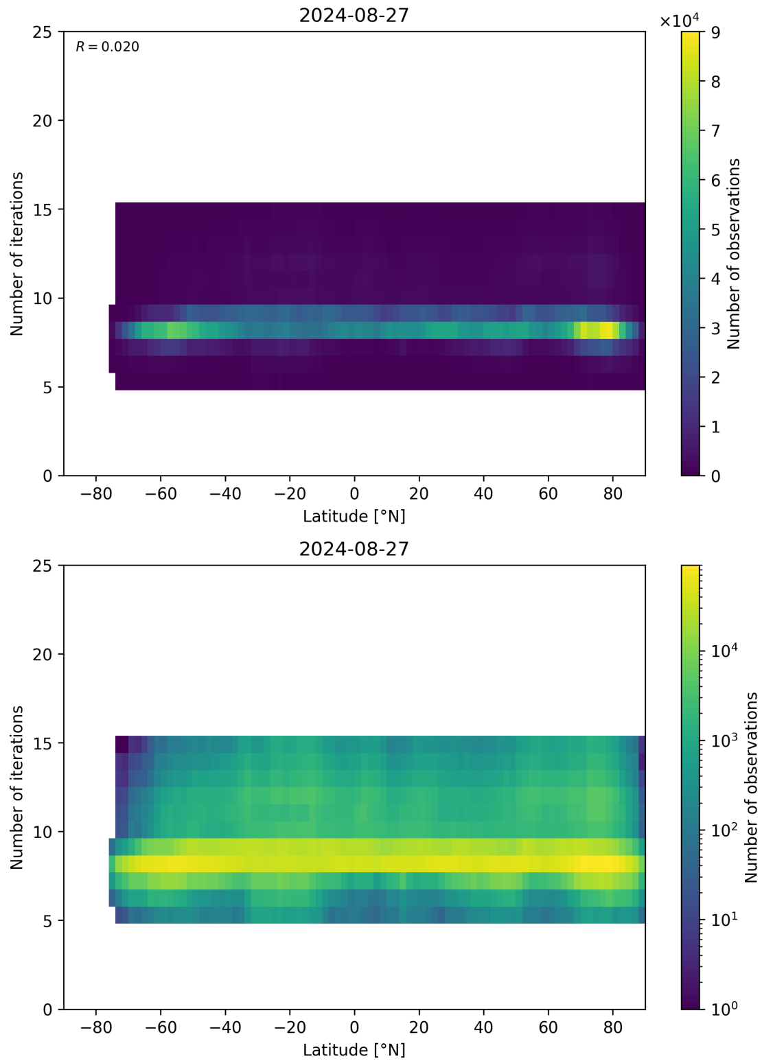
Figure 56: Scatter density plot of “Latitude” against “Number of iterations” for 2024-08-27 to 2024-08-28.
