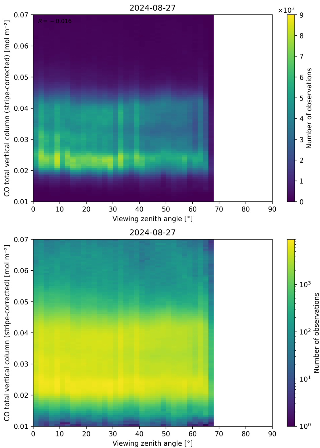
Figure 70: Scatter density plot of “Viewing zenith angle” against “CO total vertical column (stripe-corrected)” for 2024-08-27 to 2024-08-28.
