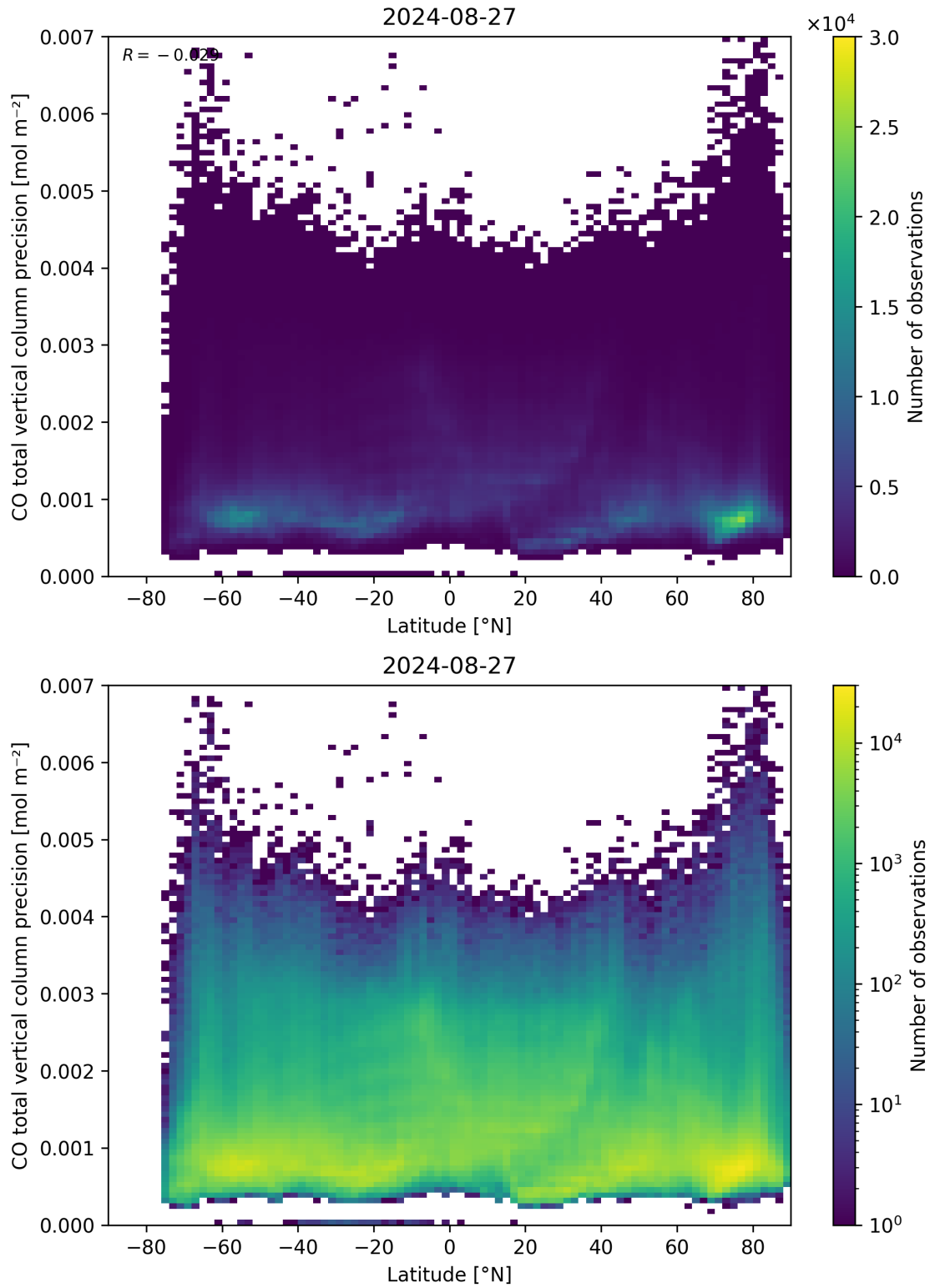
Figure 53: Scatter density plot of “Latitude” against “CO total vertical column precision” for 2024-08-27 to 2024-08-28.
