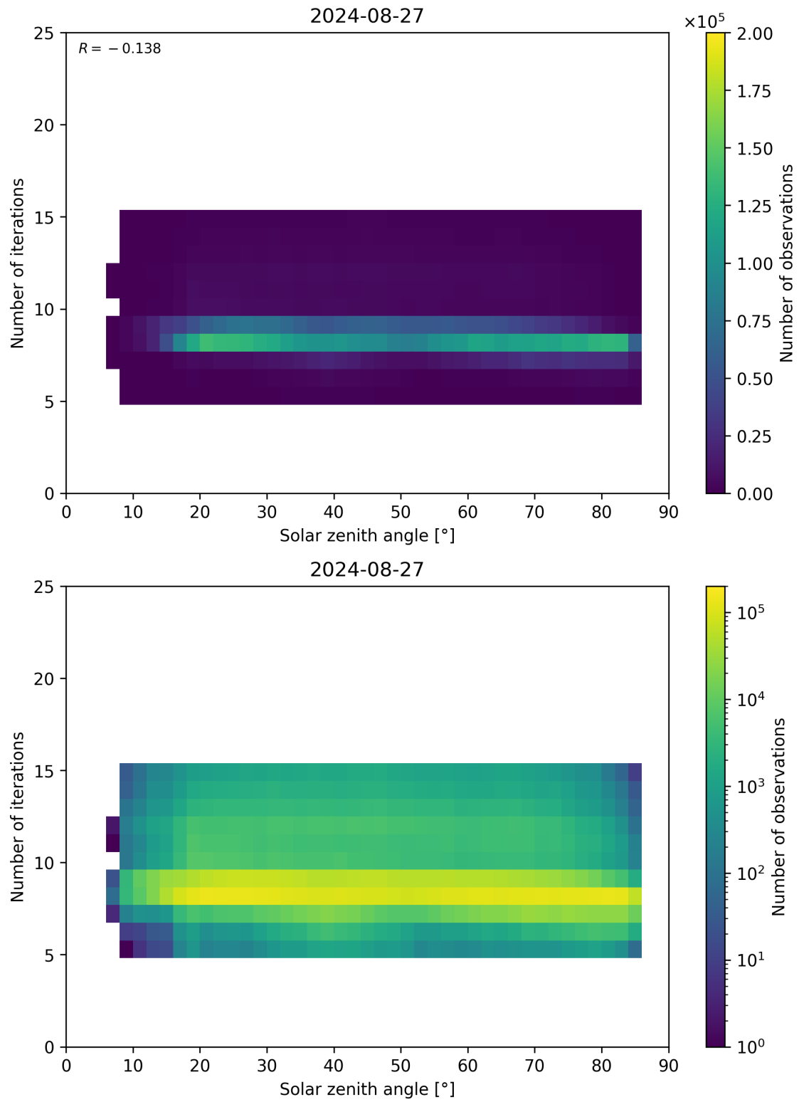
Figure 67: Scatter density plot of “Solar zenith angle” against “Number of iterations” for 2024-08-27 to 2024-08-28.
