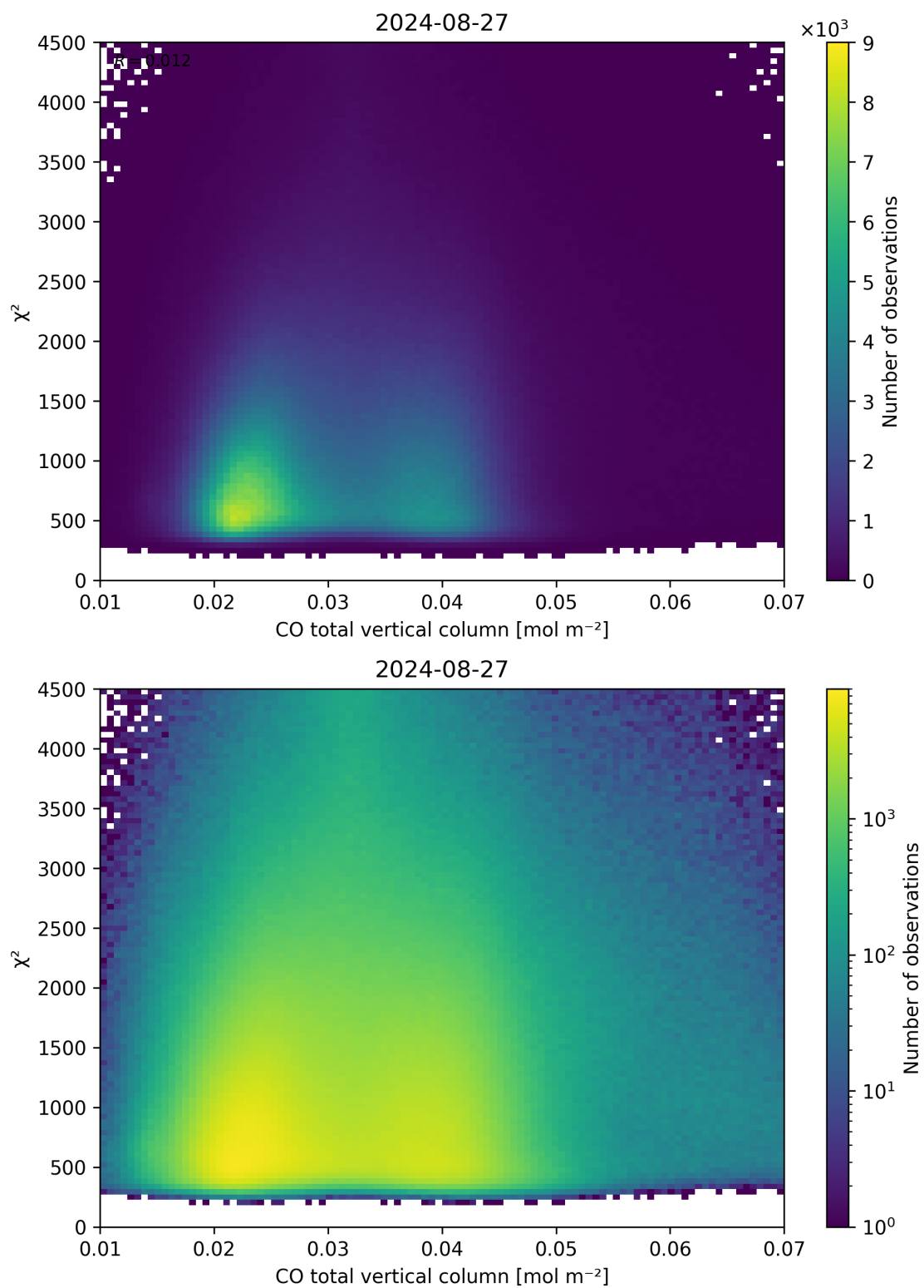
Figure 35: Scatter density plot of “CO total vertical column” against “ \chi^2 ” for 2024-08-27 to 2024-08-28.
