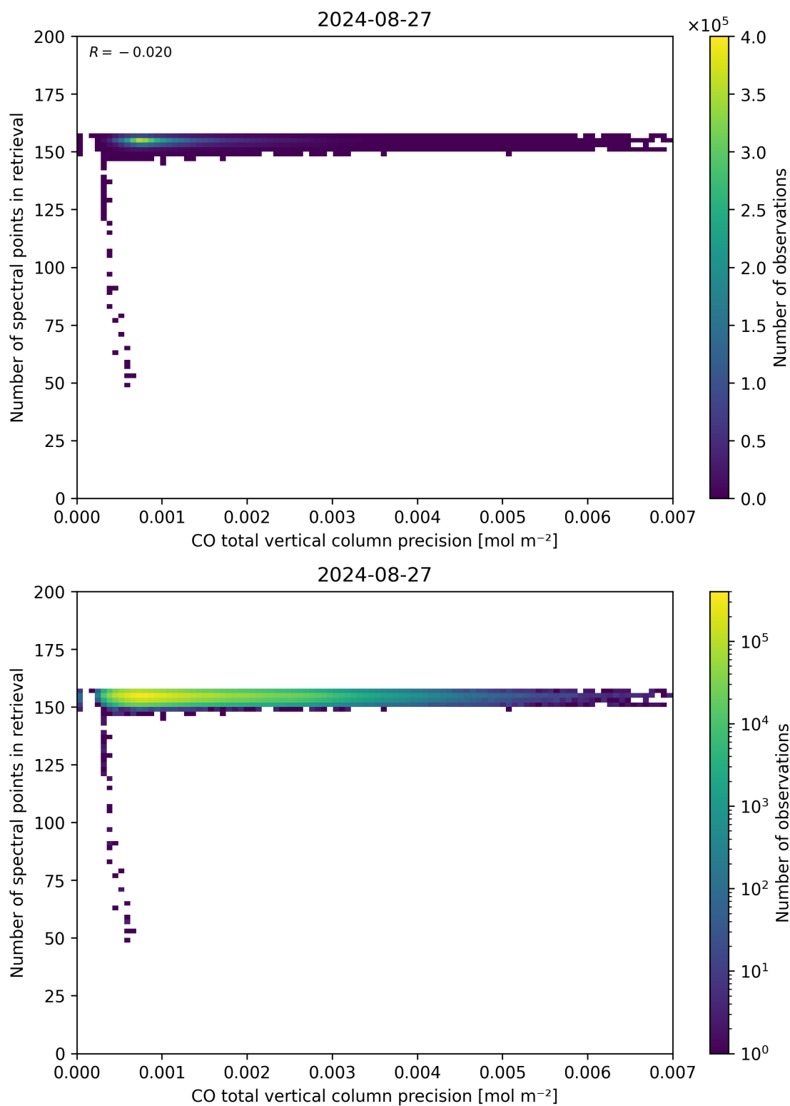
Figure 47: Scatter density plot of “CO total vertical column precision” against “Number of spectral points in retrieval” for 2024-08-27 to 2024-08-28.
