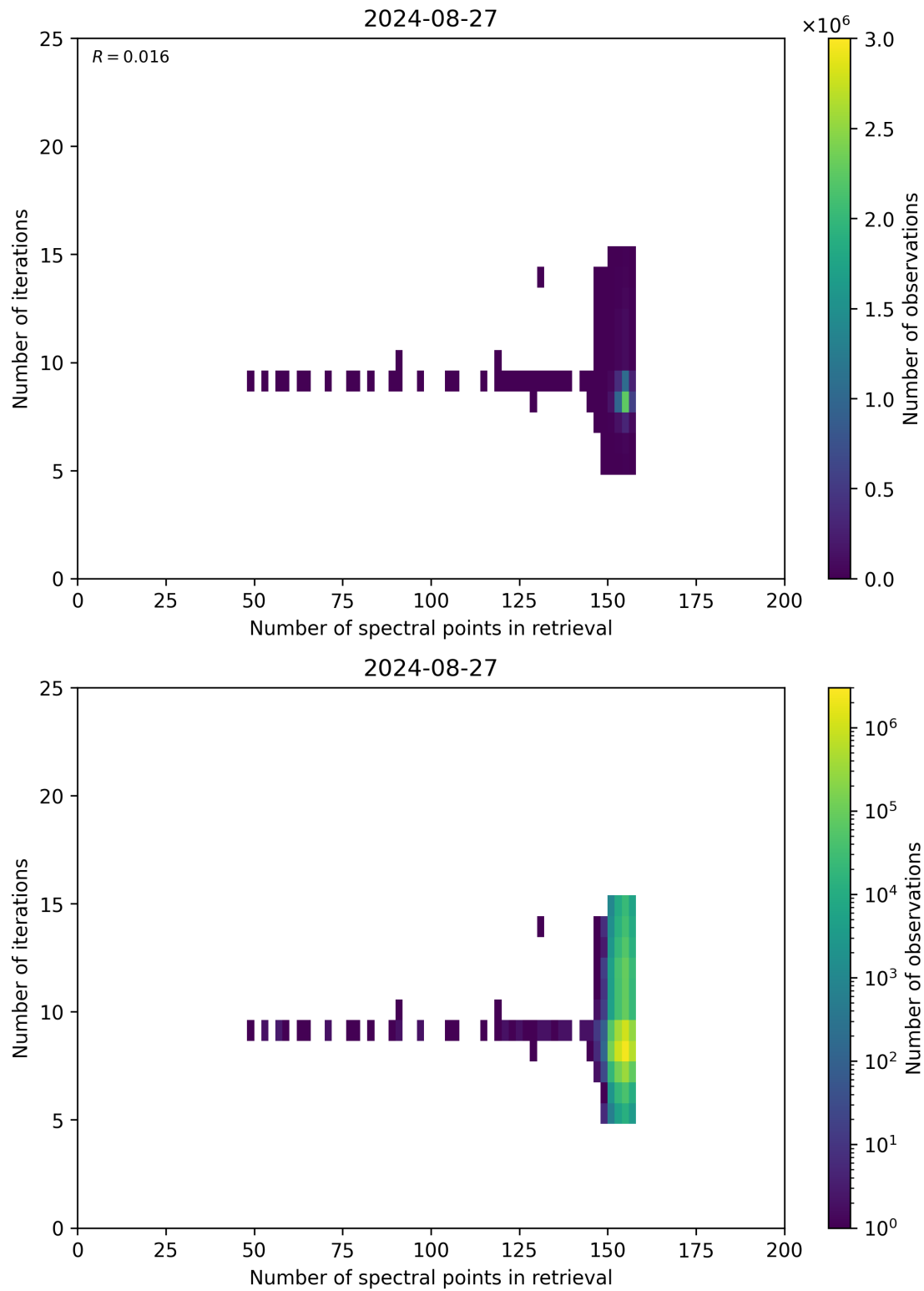
Figure 60: Scatter density plot of “Number of spectral points in retrieval” against “Number of iterations” for 2024-08-27 to 2024-08-28.
