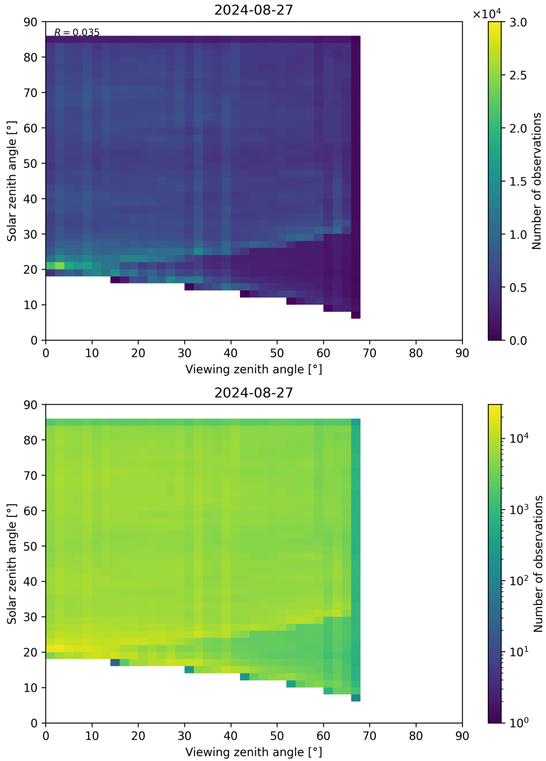
Figure 77: Scatter density plot of “Viewing zenith angle” against “Solar zenith angle” for 2024-08-27 to 2024-08-28.
