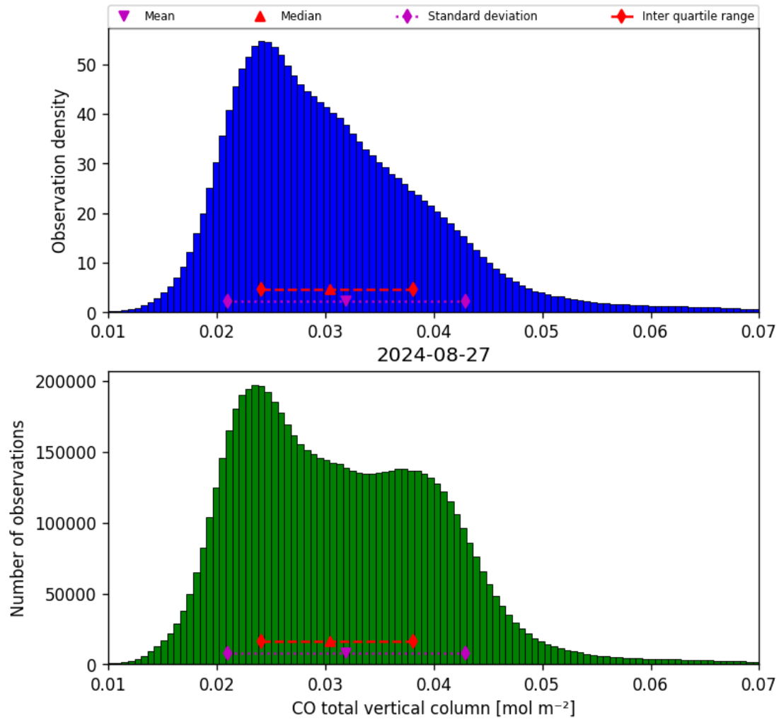
Figure 18: Histogram of “CO total vertical column” for 2024-08-27 to 2024-08-28
