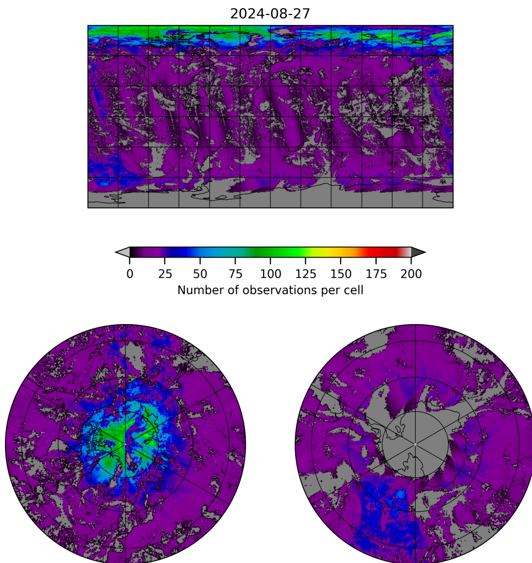
Figure 8: Map of the number of observations for 2024-08-27 to 2024-08-28
