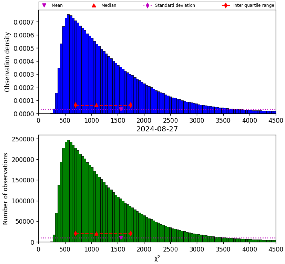
Figure 22: Histogram of “ \chi^2 ” for 2024-08-27 to 2024-08-28
