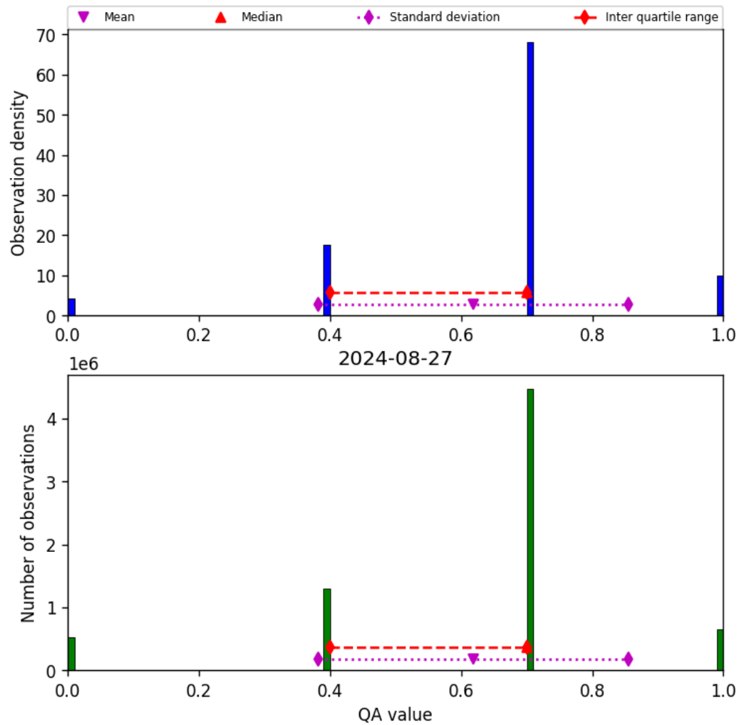
Figure 17: Histogram of “QA value” for 2024-08-27 to 2024-08-28
