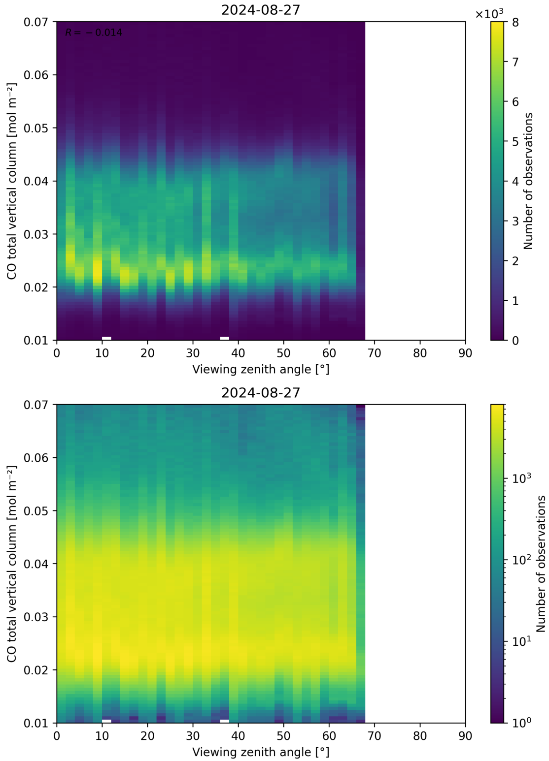
Figure 69: Scatter density plot of “Viewing zenith angle” against “CO total vertical column” for 2024-08-27 to 2024-08-28.
