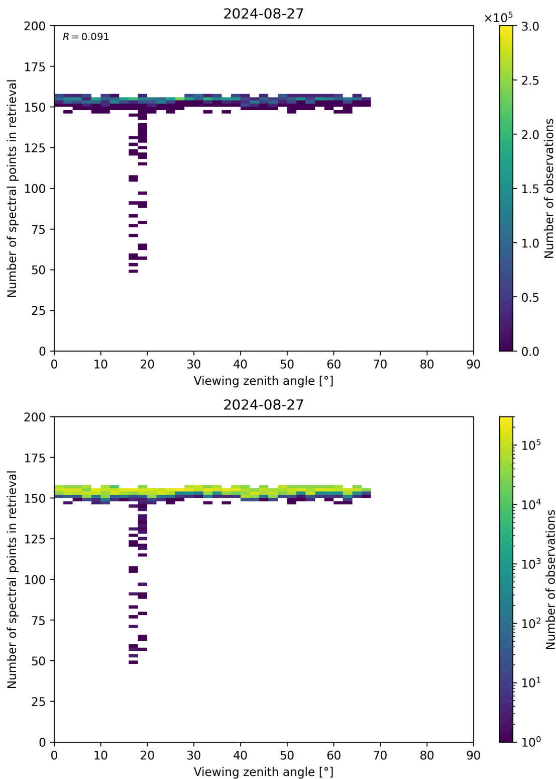
Figure 76: Scatter density plot of “Viewing zenith angle” against “Number of spectral points in retrieval” for 2024-08-27 to 2024-08-28.
