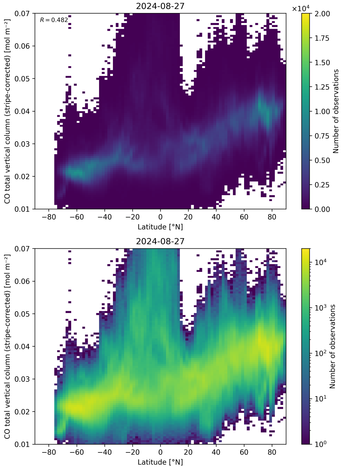
Figure 52: Scatter density plot of “Latitude” against “CO total vertical column (stripe-corrected)” for 2024-08-27 to 2024-08-28.
