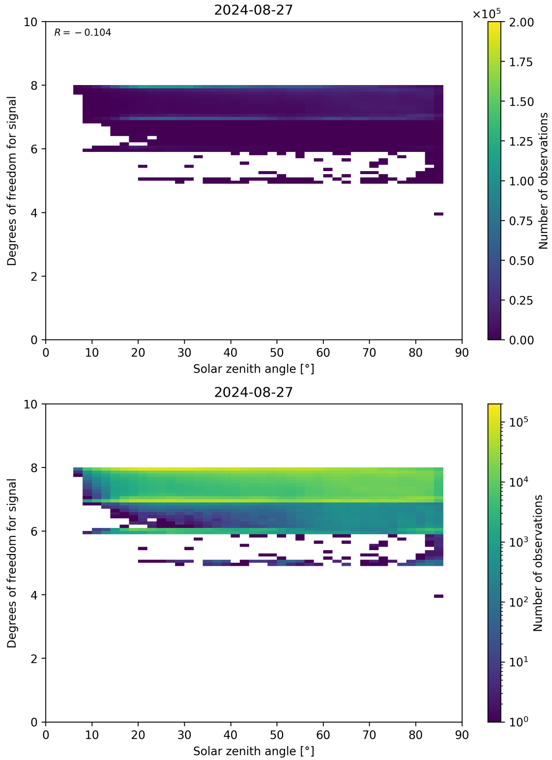
Figure 65: Scatter density plot of “Solar zenith angle” against “Degrees of freedom for signal” for 2024-08-27 to 2024-08-28.
