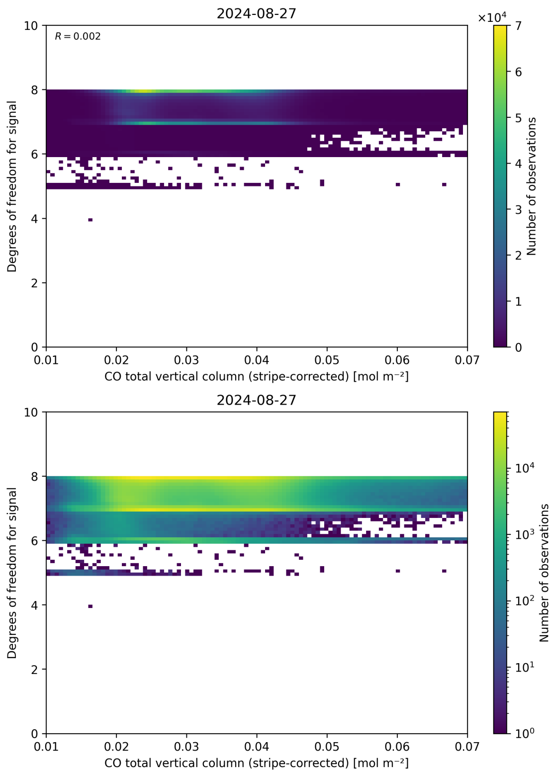
Figure 38: Scatter density plot of “CO total vertical column (stripe-corrected)” against “Degrees of freedom for signal” for 2024-08-27 to 2024-08-28.
