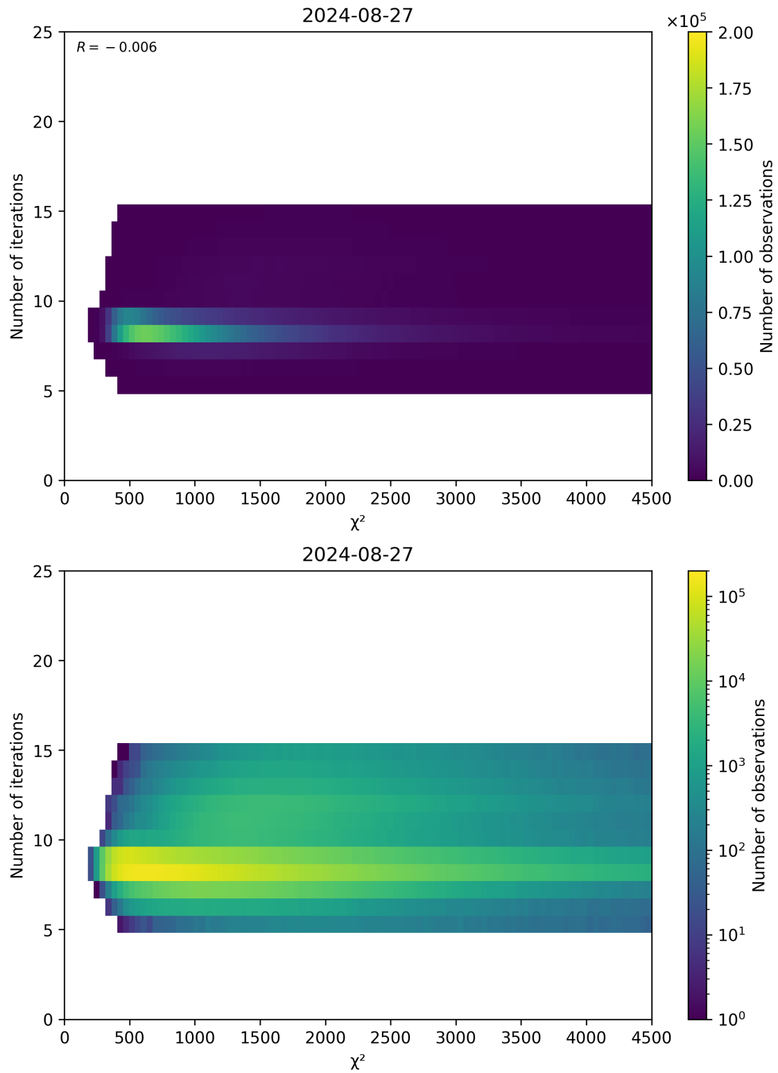
Figure 49: Scatter density plot of “ \chi^2 ” against “Number of iterations” for 2024-08-27 to 2024-08-28.
