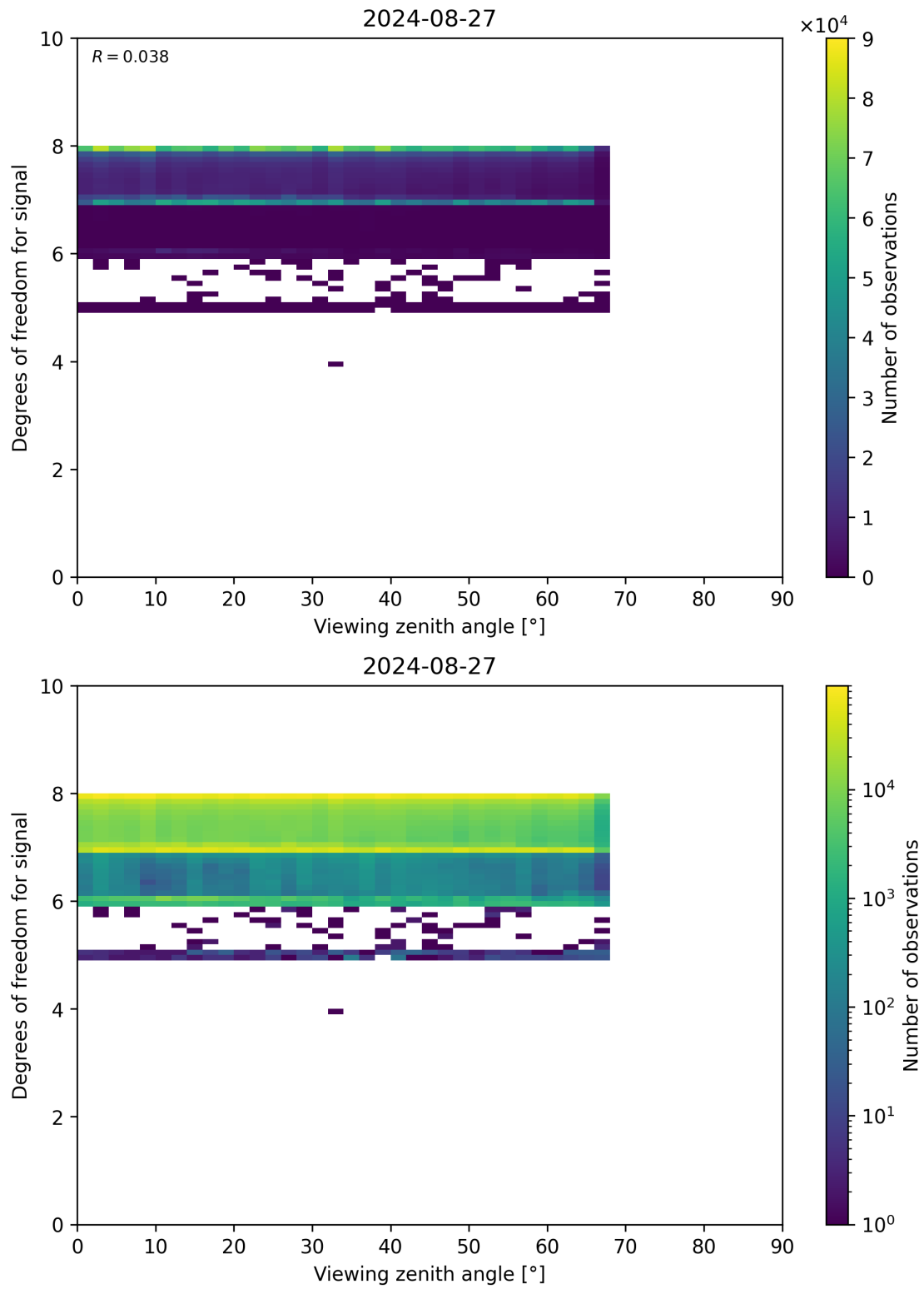
Figure 73: Scatter density plot of “Viewing zenith angle” against “Degrees of freedom for signal” for 2024-08-27 to 2024-08-28.
