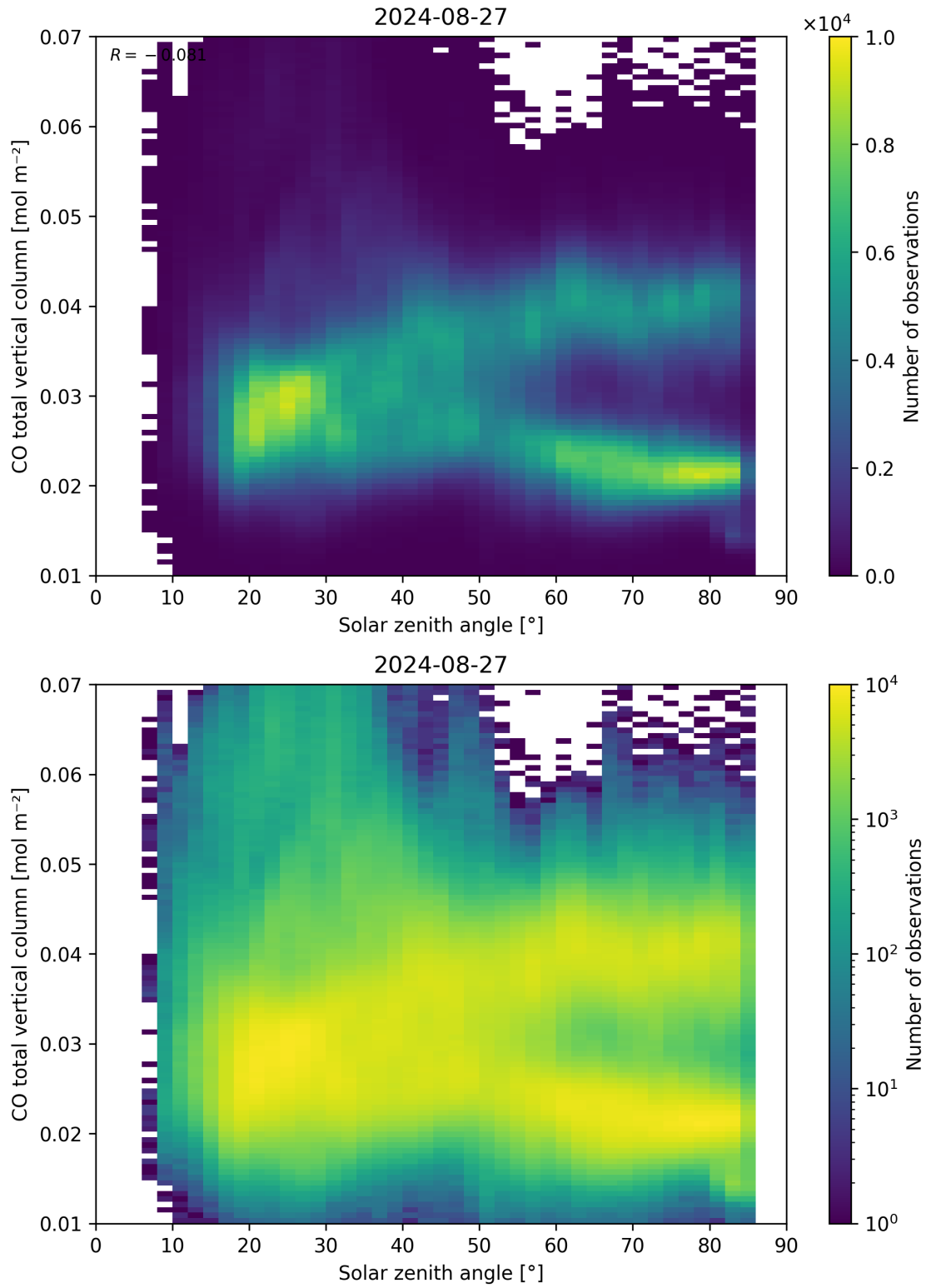
Figure 61: Scatter density plot of “Solar zenith angle” against “CO total vertical column” for 2024-08-27 to 2024-08-28.
