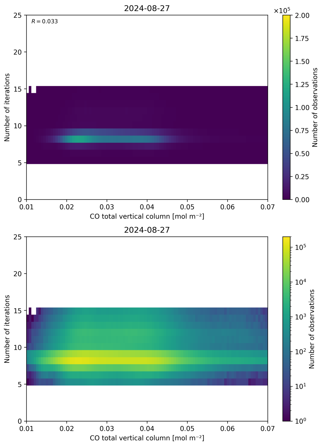
Figure 42: Scatter density plot of “CO total vertical column” against “Number of iterations” for 2024-08-27 to 2024-08-28.
