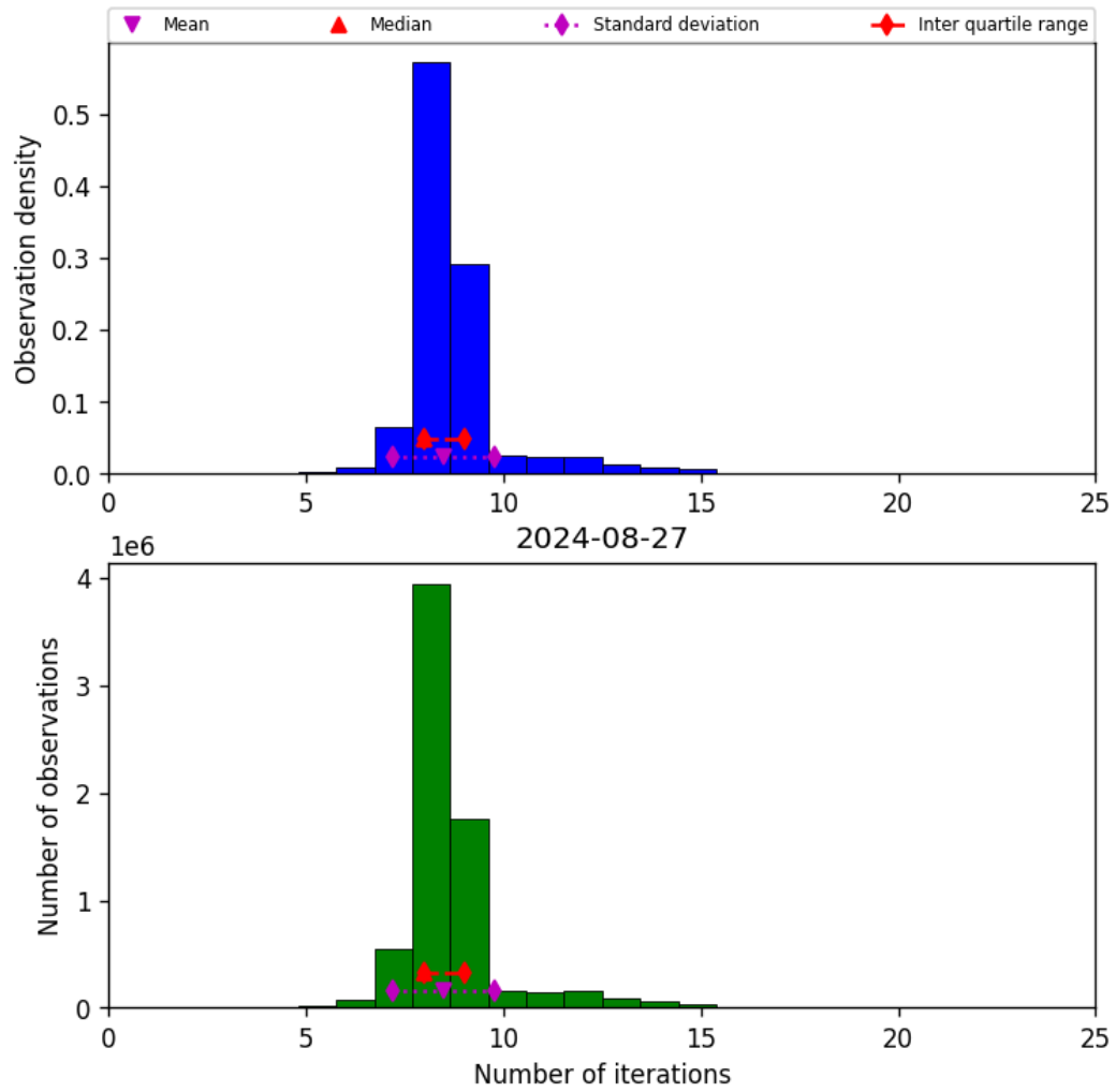
Figure 24: Histogram of “Number of iterations” for 2024-08-27 to 2024-08-28
