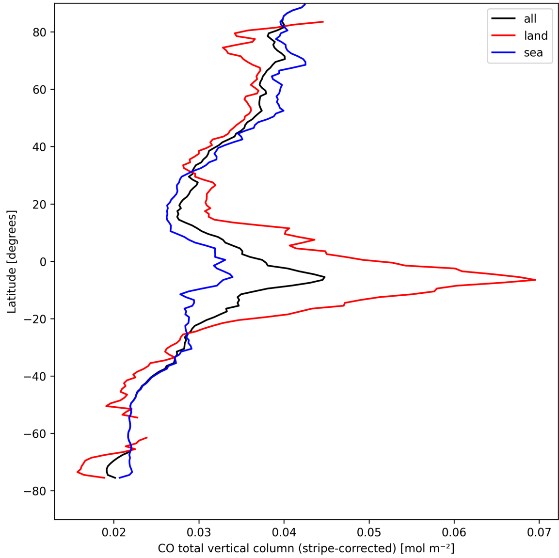
Figure 11: Zonal average of “CO total vertical column (stripe-corrected)” for 2024-08-27 to 2024-08-28.
