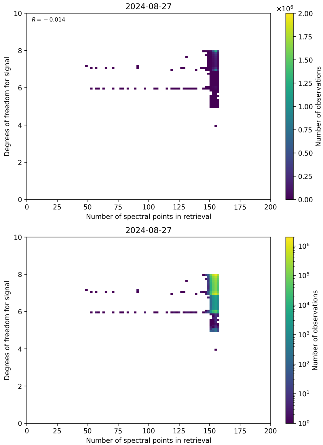
Figure 59: Scatter density plot of “Number of spectral points in retrieval” against “Degrees of freedom for signal” for 2024-08-27 to 2024-08-28.
