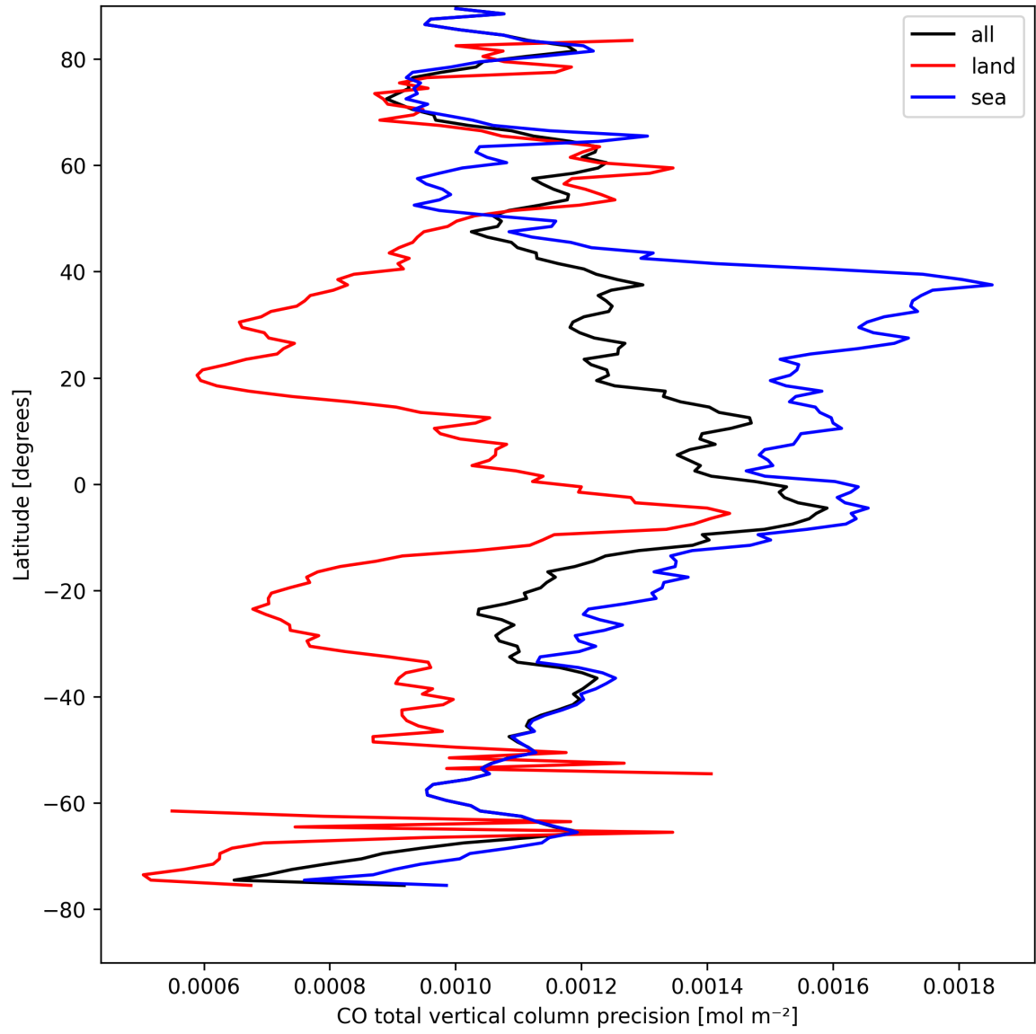
Figure 12: Zonal average of “CO total vertical column precision” for 2024-08-27 to 2024-08-28.
