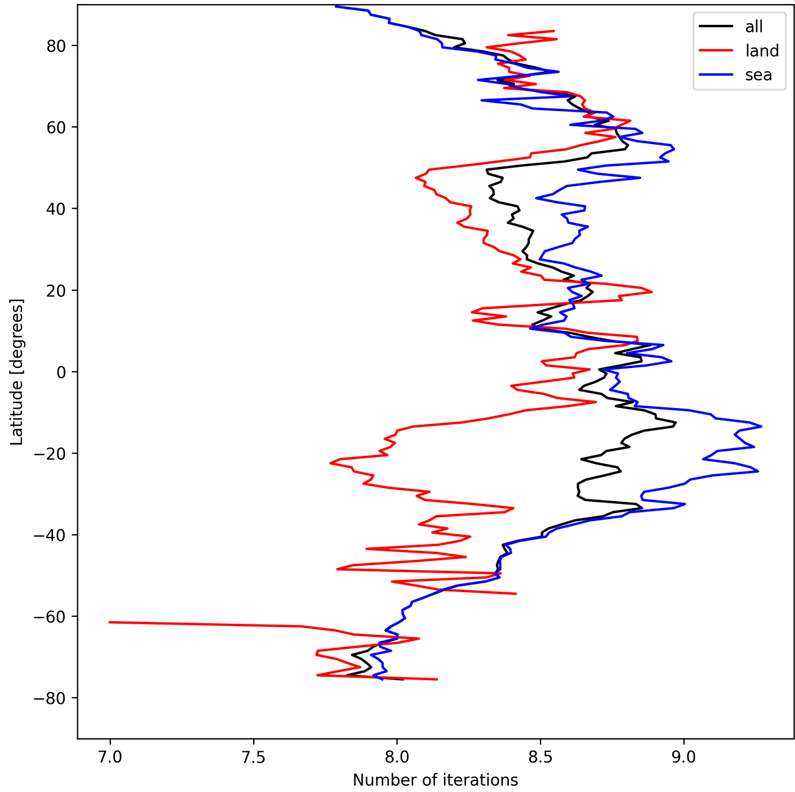
Figure 16: Zonal average of “Number of iterations” for 2024-08-27 to 2024-08-28.
