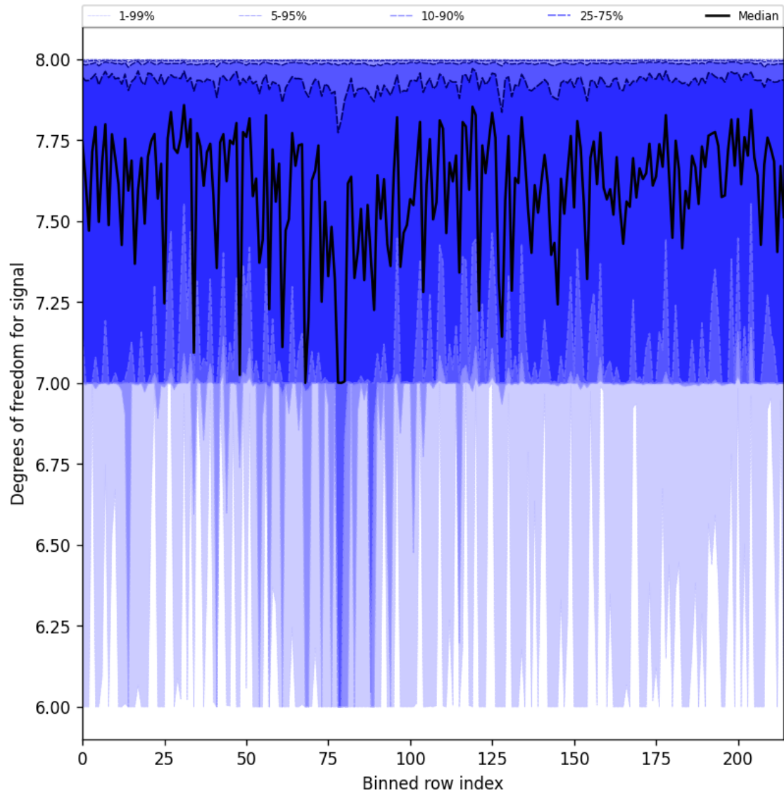
Figure 31: Along track statistics of “Degrees of freedom for signal” for 2024-08-27 to 2024-08-28
