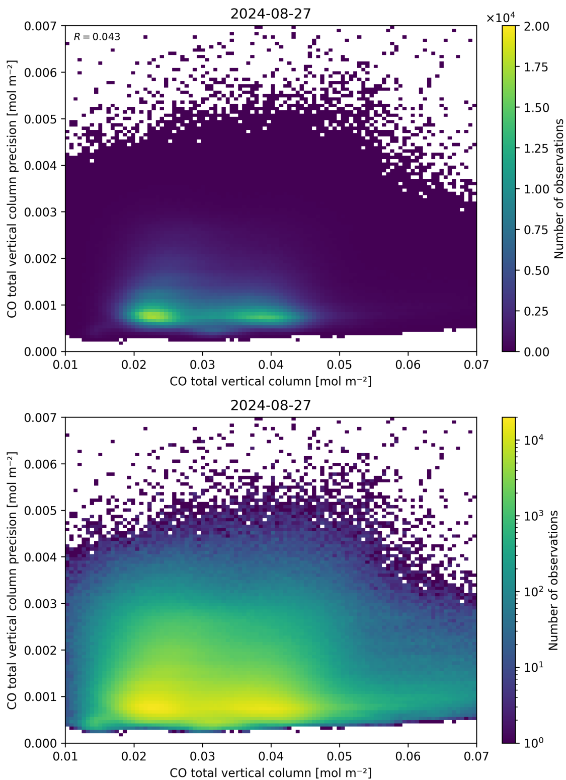
Figure 34: Scatter density plot of “CO total vertical column” against “CO total vertical column precision” for 2024-08-27 to 2024-08-28.
