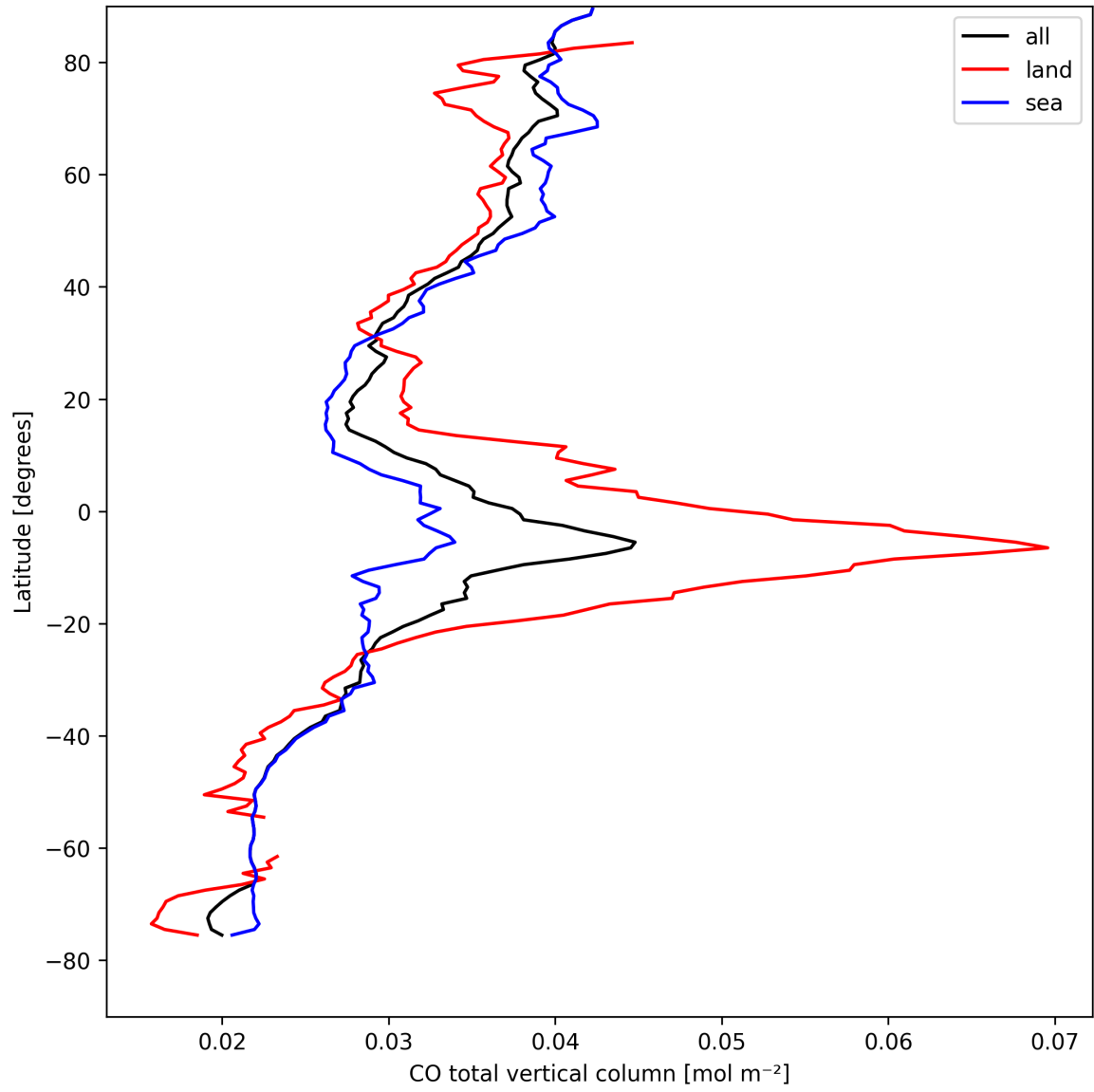
Figure 10: Zonal average of “CO total vertical column” for 2024-08-27 to 2024-08-28.
