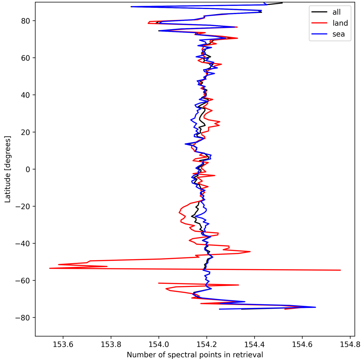
Figure 13: Zonal average of “Number of spectral points in retrieval” for 2024-08-27 to 2024-08-28.
