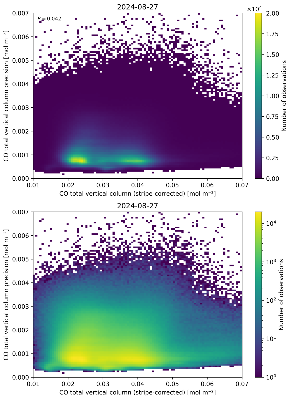
Figure 36: Scatter density plot of “CO total vertical column (stripe-corrected)” against “CO total vertical column precision” for 2024-08-27 to 2024-08-28.
