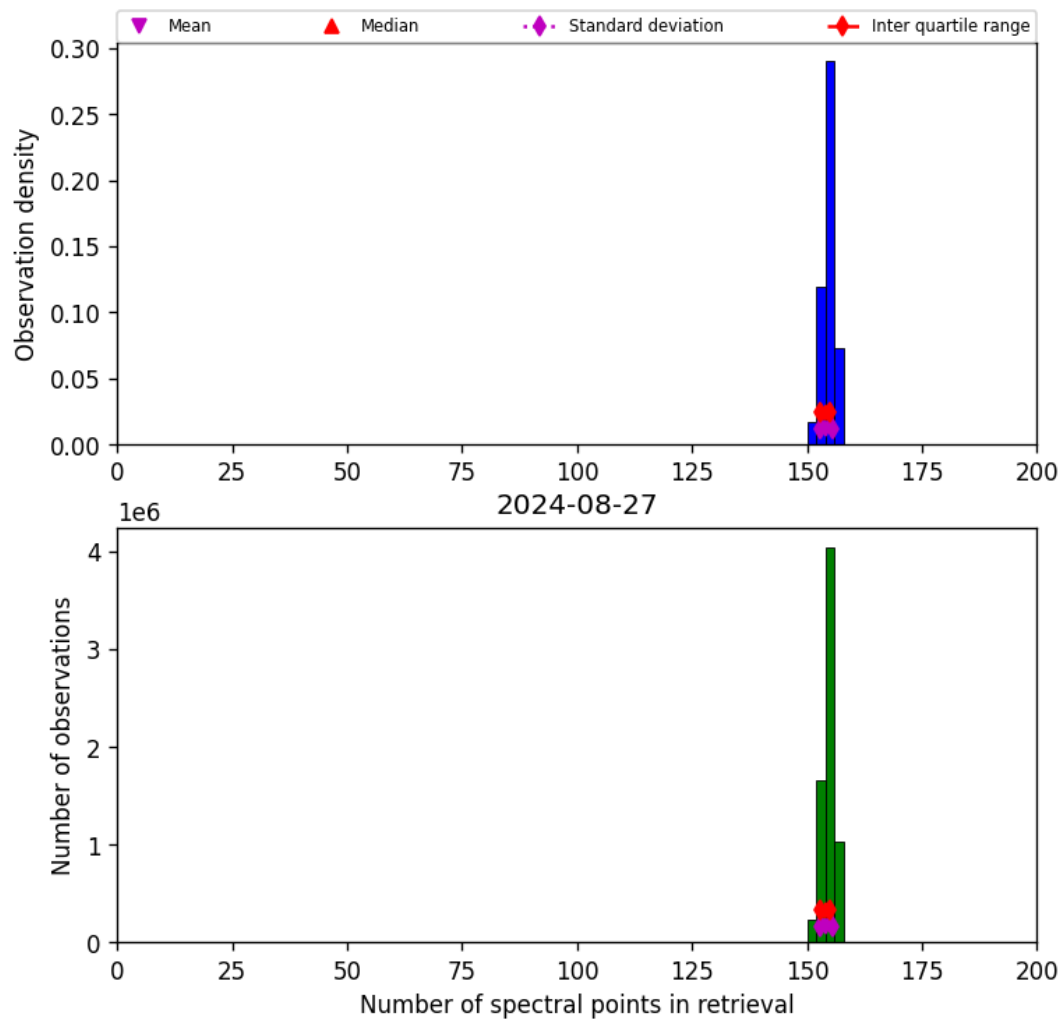
Figure 21: Histogram of “Number of spectral points in retrieval” for 2024-08-27 to 2024-08-28
