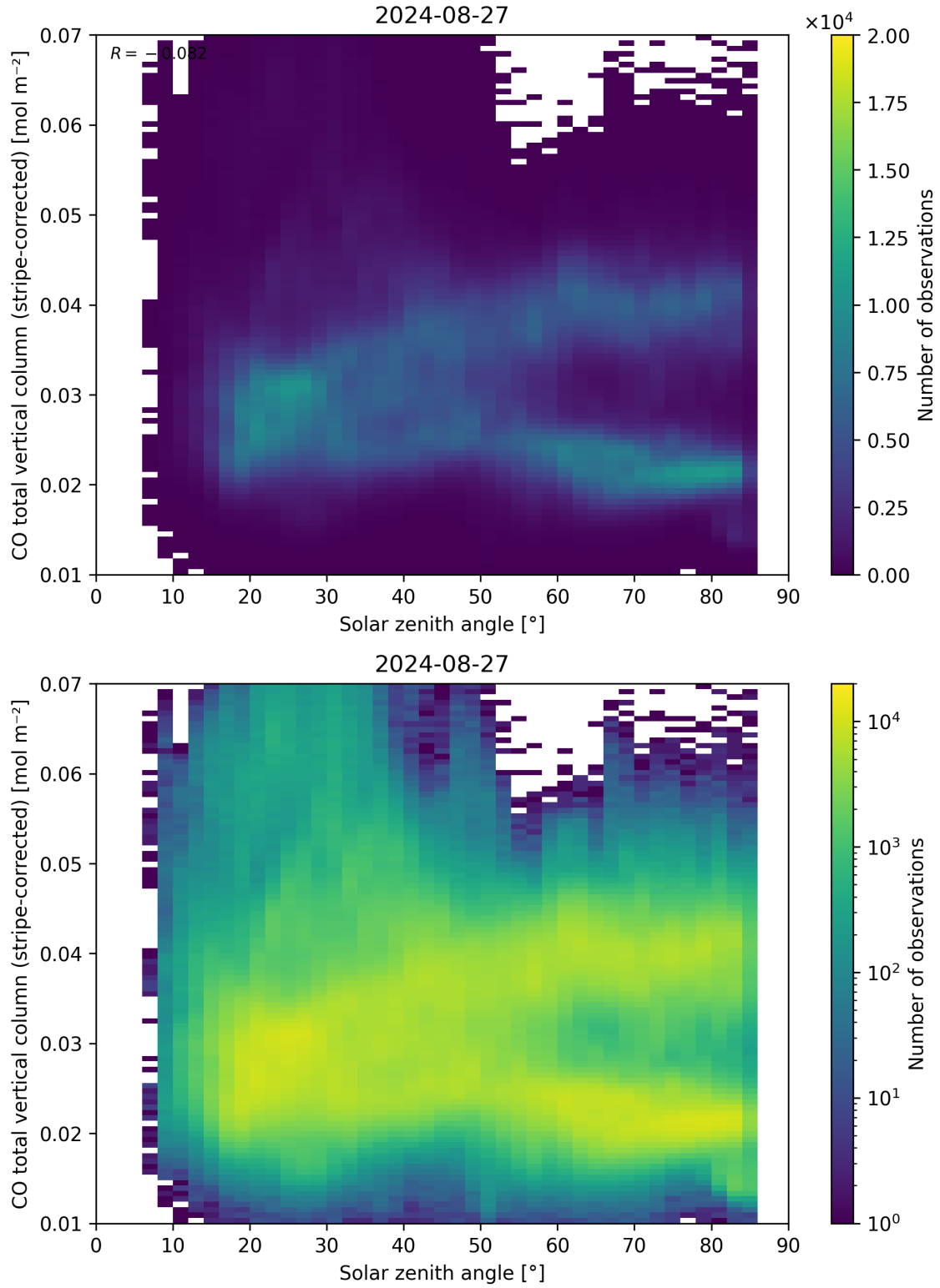
Figure 62: Scatter density plot of “Solar zenith angle” against “CO total vertical column (stripe-corrected)” for 2024-08-27 to 2024-08-28.
