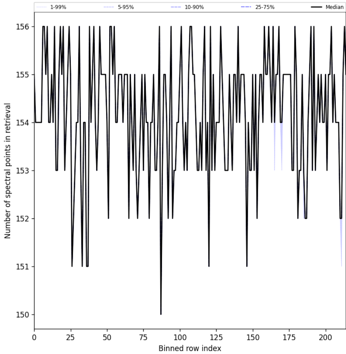
Figure 29: Along track statistics of “Number of spectral points in retrieval” for 2024-08-27 to 2024-08-28
