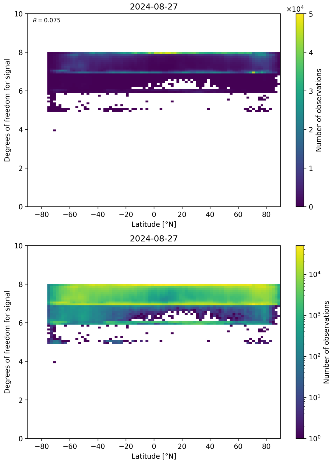
Figure 55: Scatter density plot of “Latitude” against “Degrees of freedom for signal” for 2024-08-27 to 2024-08-28.
