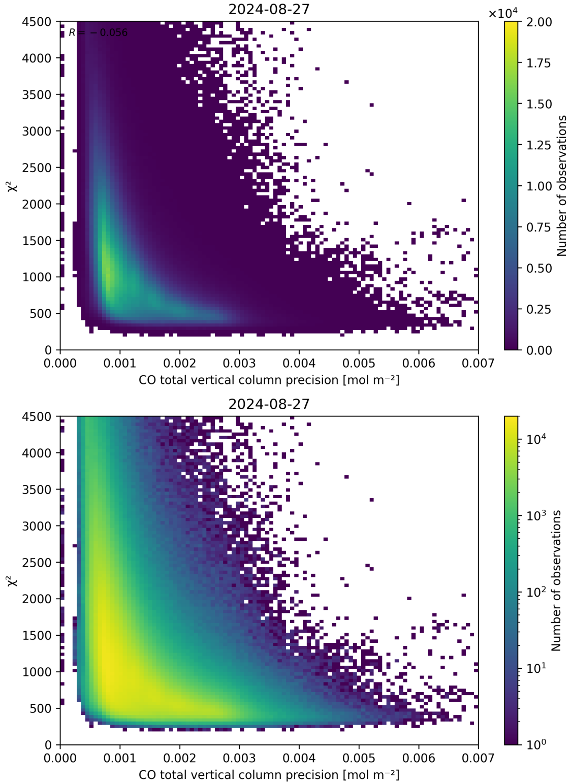
Figure 44: Scatter density plot of “CO total vertical column precision” against “ \chi^2 ” for 2024-08-27 to 2024-08-28.
