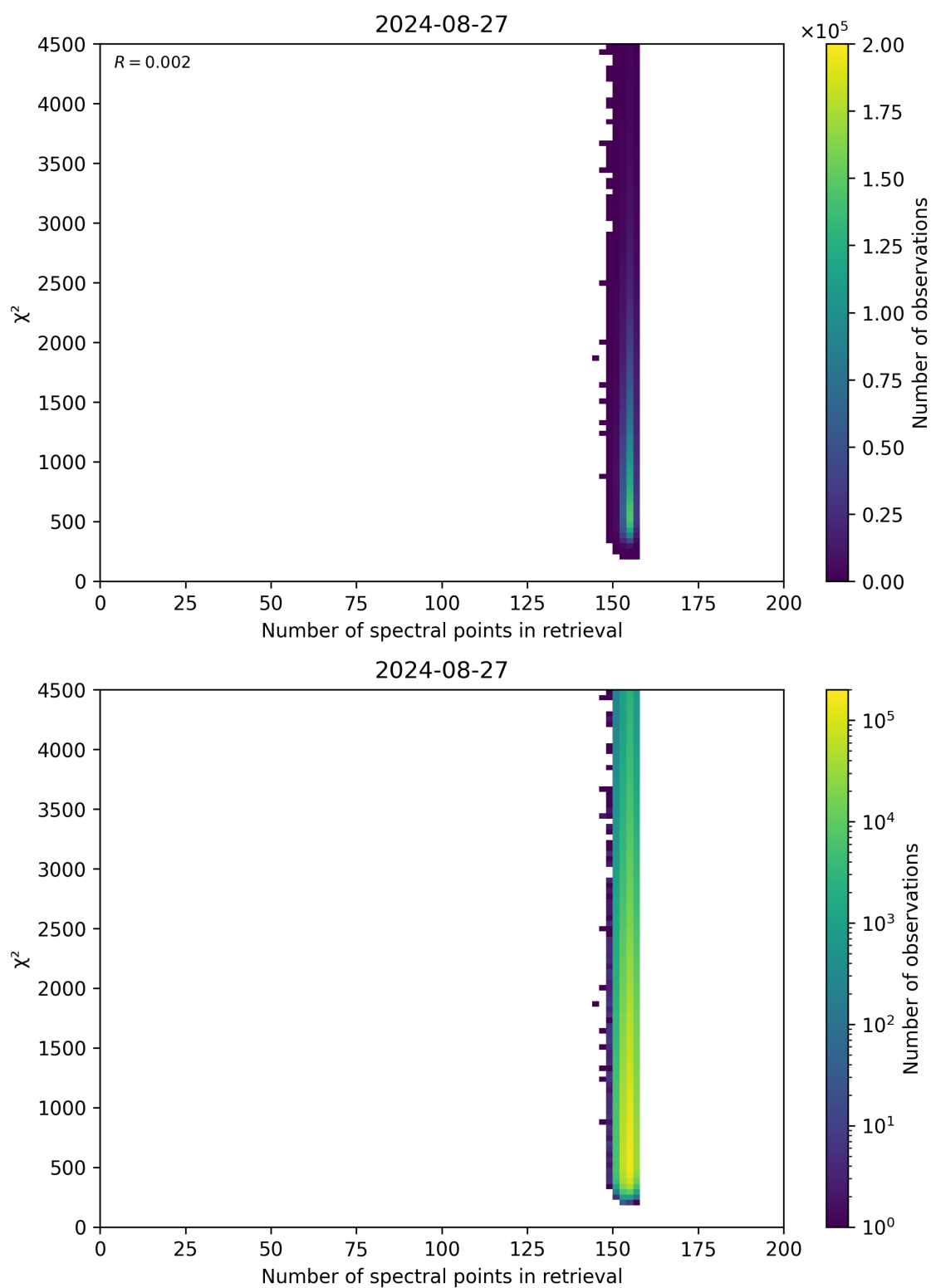
Figure 58: Scatter density plot of “Number of spectral points in retrieval” against “ \chi^2 ” for 2024-08-27 to 2024-08-28.
