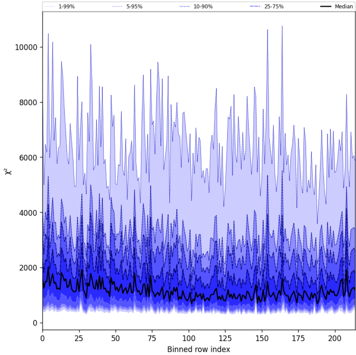
Figure 30: Along track statistics of “ \chi^2 ” for 2024-08-27 to 2024-08-28
