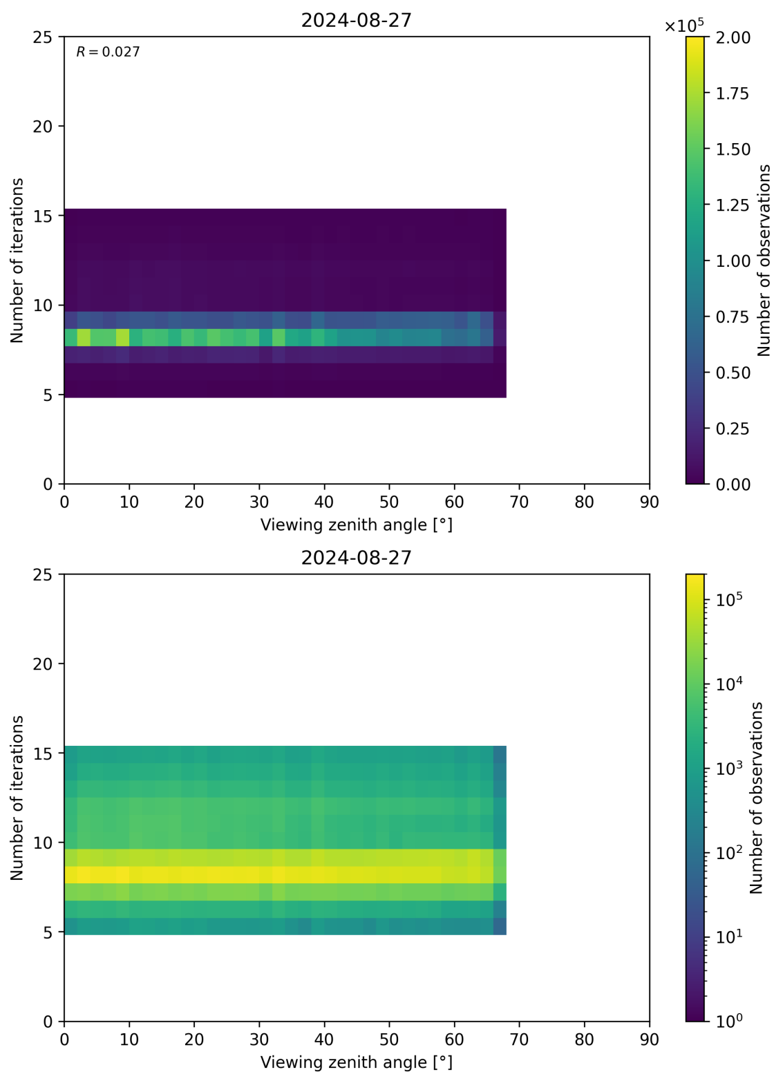
Figure 75: Scatter density plot of “Viewing zenith angle” against “Number of iterations” for 2024-08-27 to 2024-08-28.
