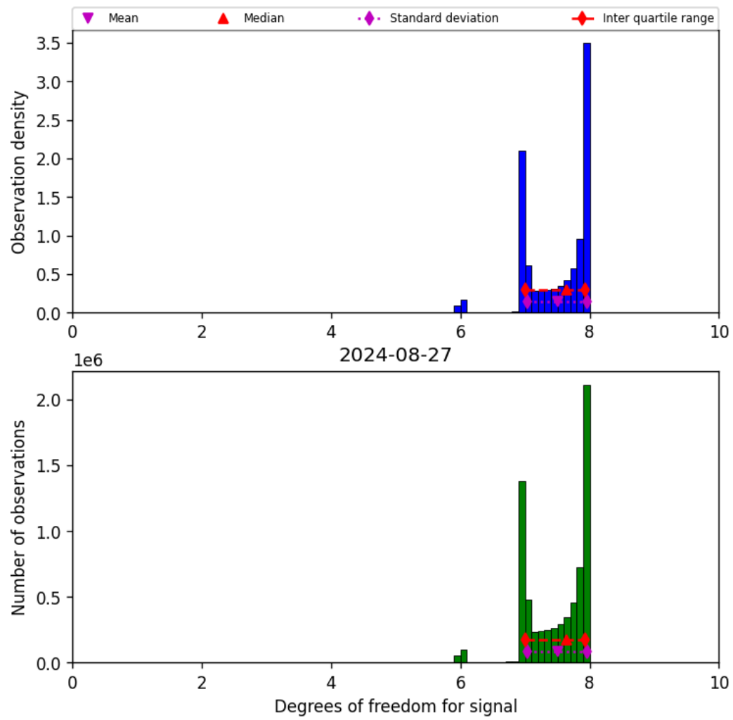
Figure 23: Histogram of “Degrees of freedom for signal” for 2024-08-27 to 2024-08-28
