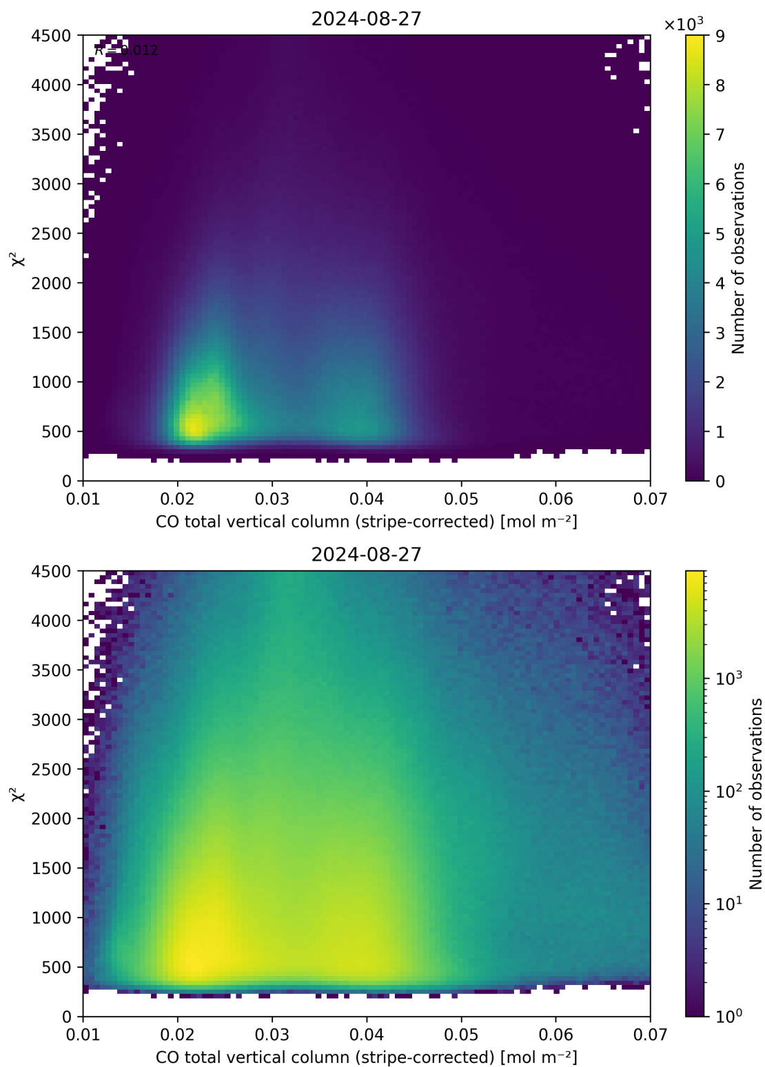
Figure 37: Scatter density plot of “CO total vertical column (stripe-corrected)” against “ \chi^2 ” for 2024-08-27 to 2024-08-28.
