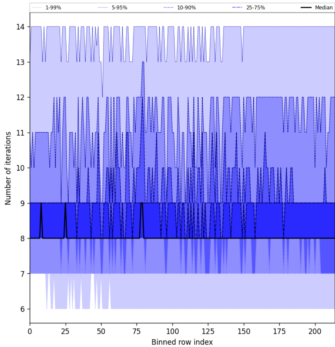
Figure 32: Along track statistics of “Number of iterations” for 2024-08-27 to 2024-08-28
