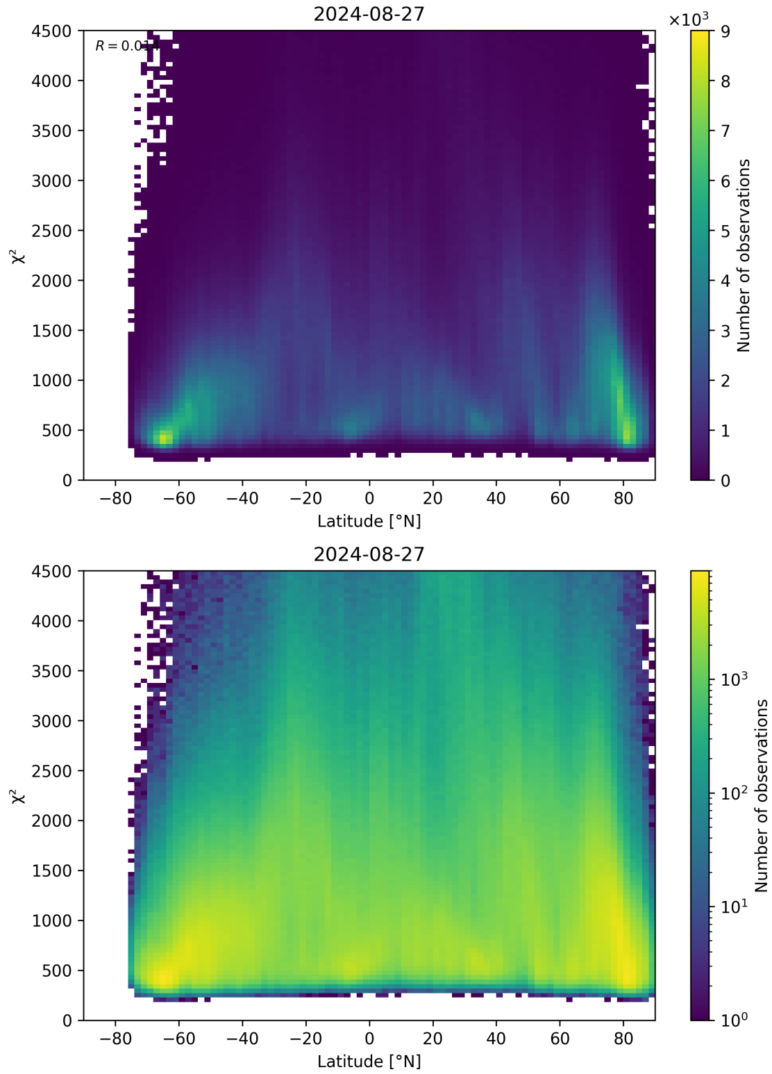
Figure 54: Scatter density plot of “Latitude” against “ \chi^2 ” for 2024-08-27 to 2024-08-28.
