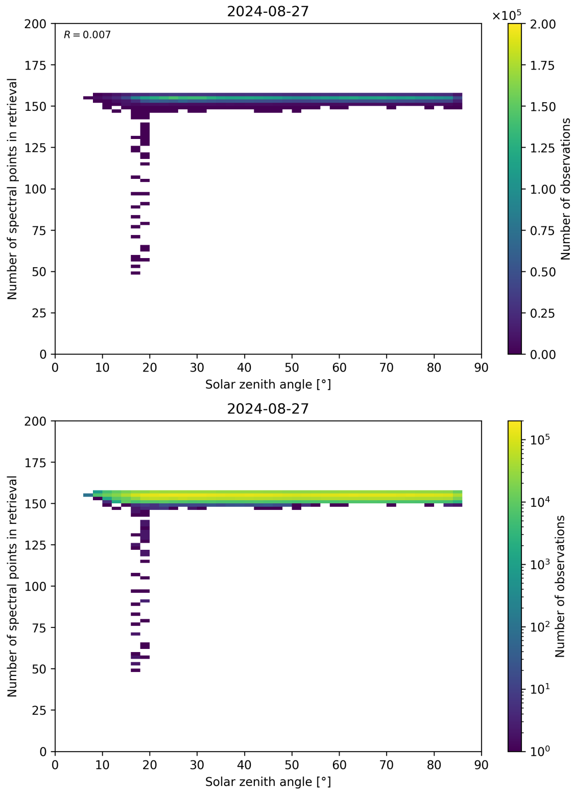
Figure 68: Scatter density plot of “Solar zenith angle” against “Number of spectral points in retrieval” for 2024-08-27 to 2024-08-28.
