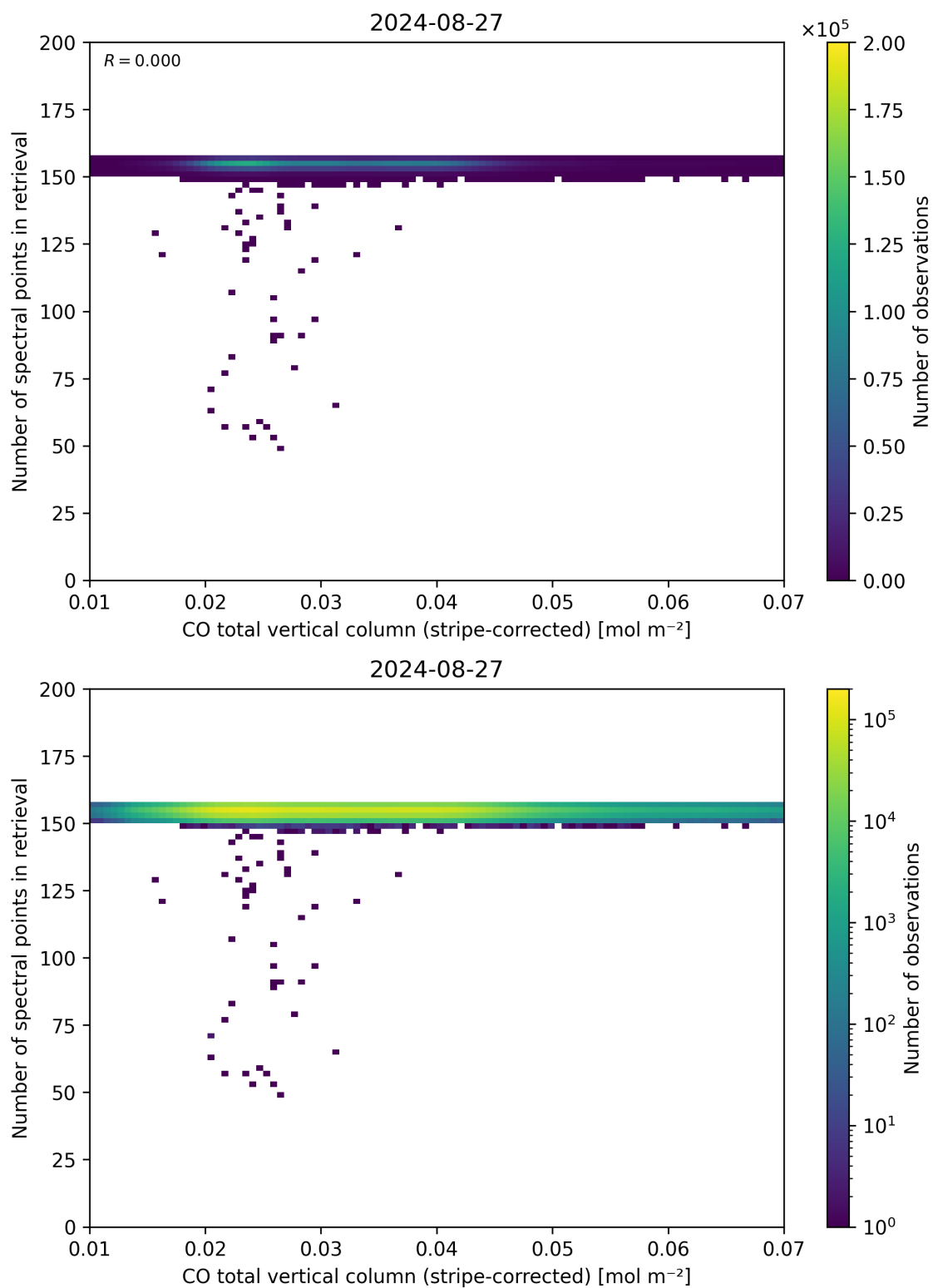
Figure 40: Scatter density plot of “CO total vertical column (stripe-corrected)” against “Number of spectral points in retrieval” for 2024-08-27 to 2024-08-28.
