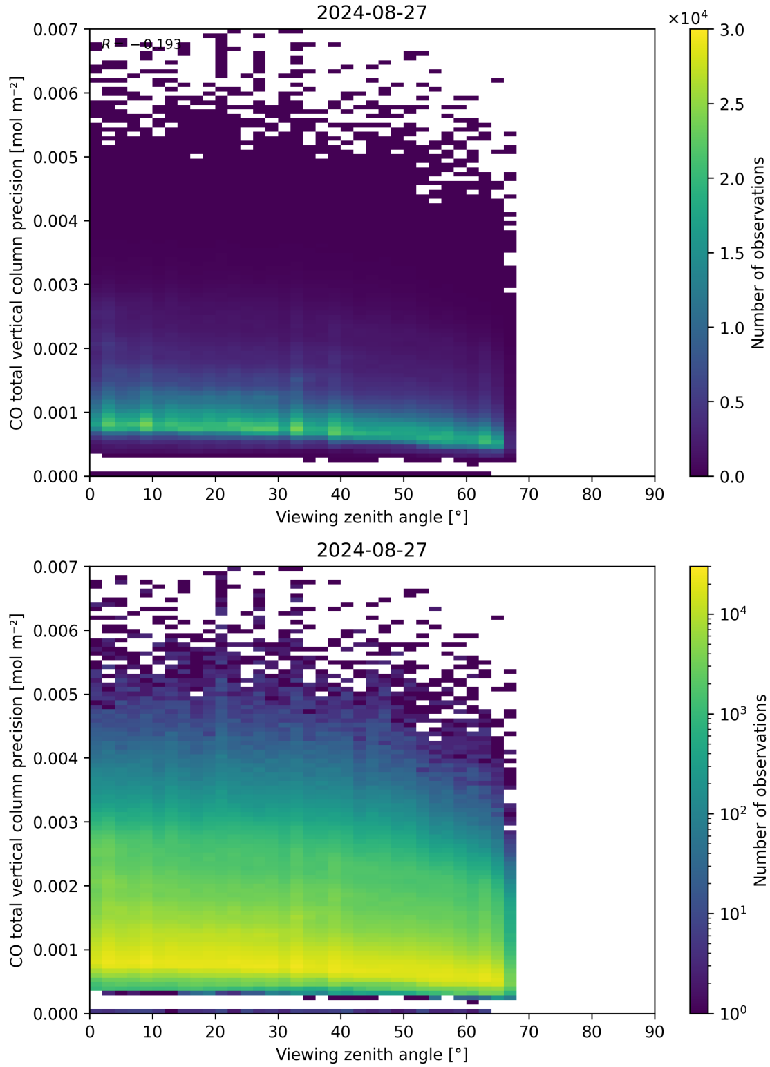
Figure 71: Scatter density plot of “Viewing zenith angle” against “CO total vertical column precision” for 2024-08-27 to 2024-08-28.
