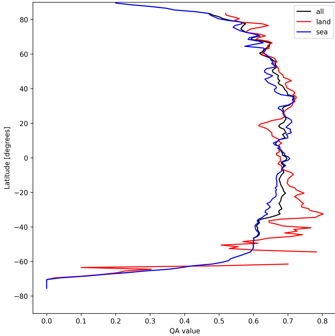
Figure 9: Zonal average of “QA value” for 2024-08-27 to 2024-08-28.
