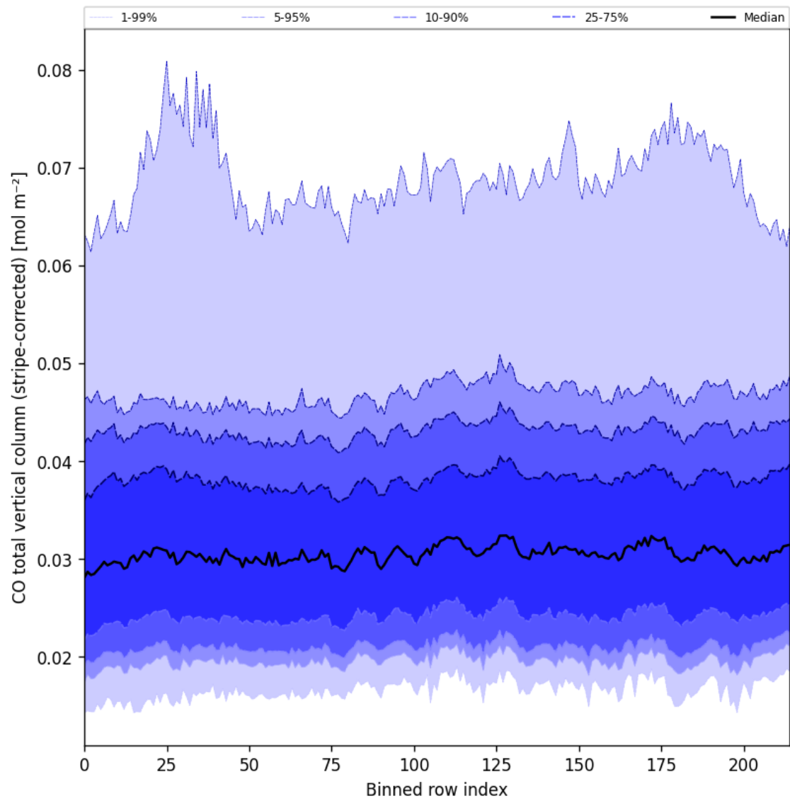
Figure 27: Along track statistics of “CO total vertical column (stripe-corrected)” for 2024-08-27 to 2024-08-28
