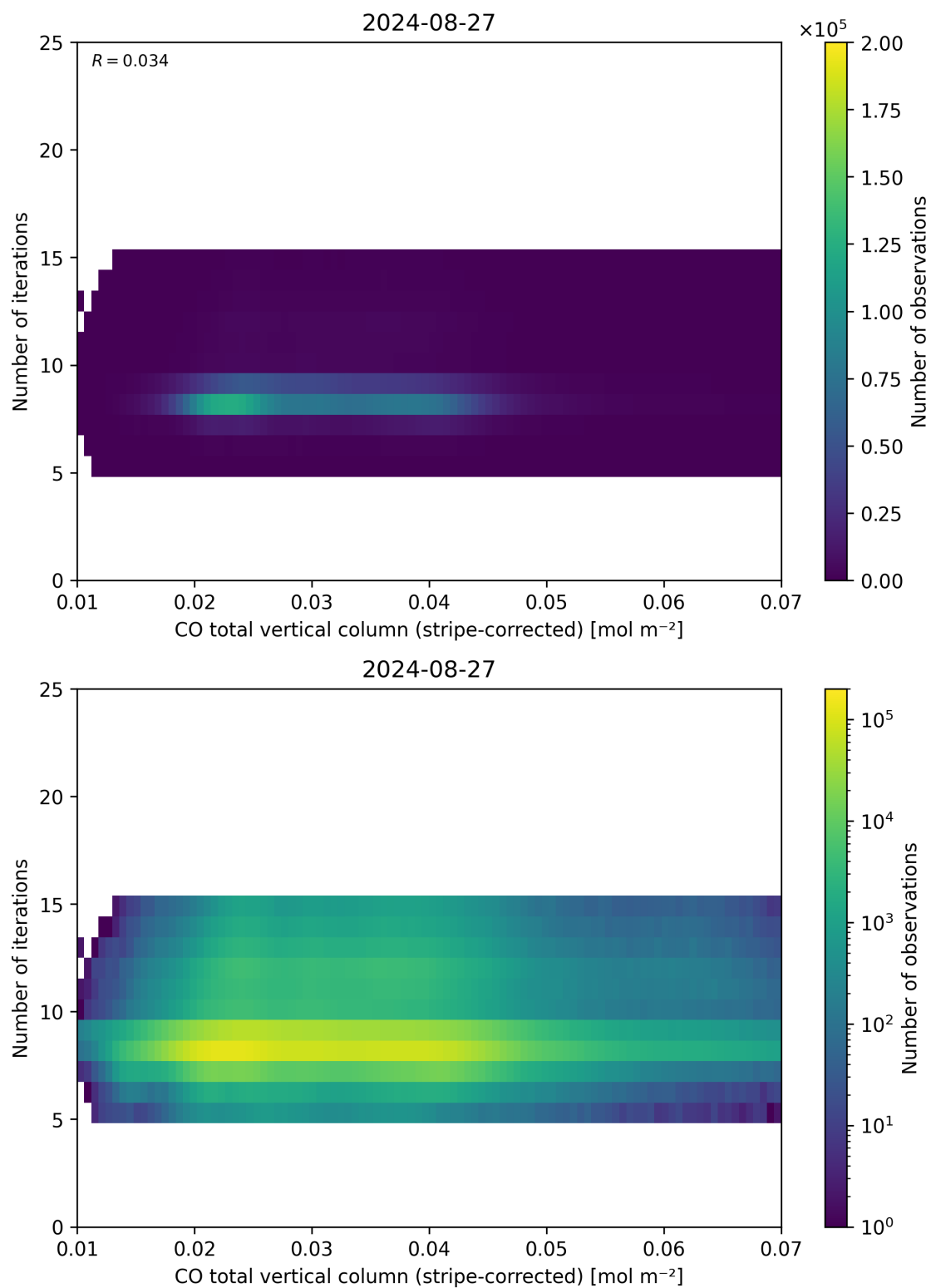
Figure 39: Scatter density plot of “CO total vertical column (stripe-corrected)” against “Number of iterations” for 2024-08-27 to 2024-08-28.
