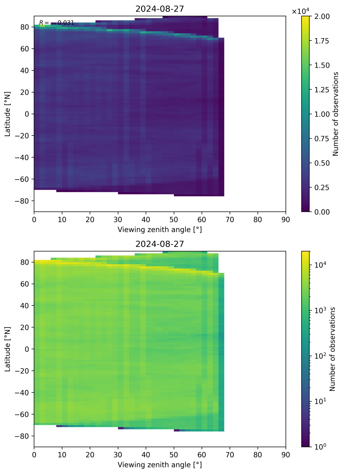
Figure 74: Scatter density plot of “Viewing zenith angle” against “Latitude” for 2024-08-27 to 2024-08-28.
