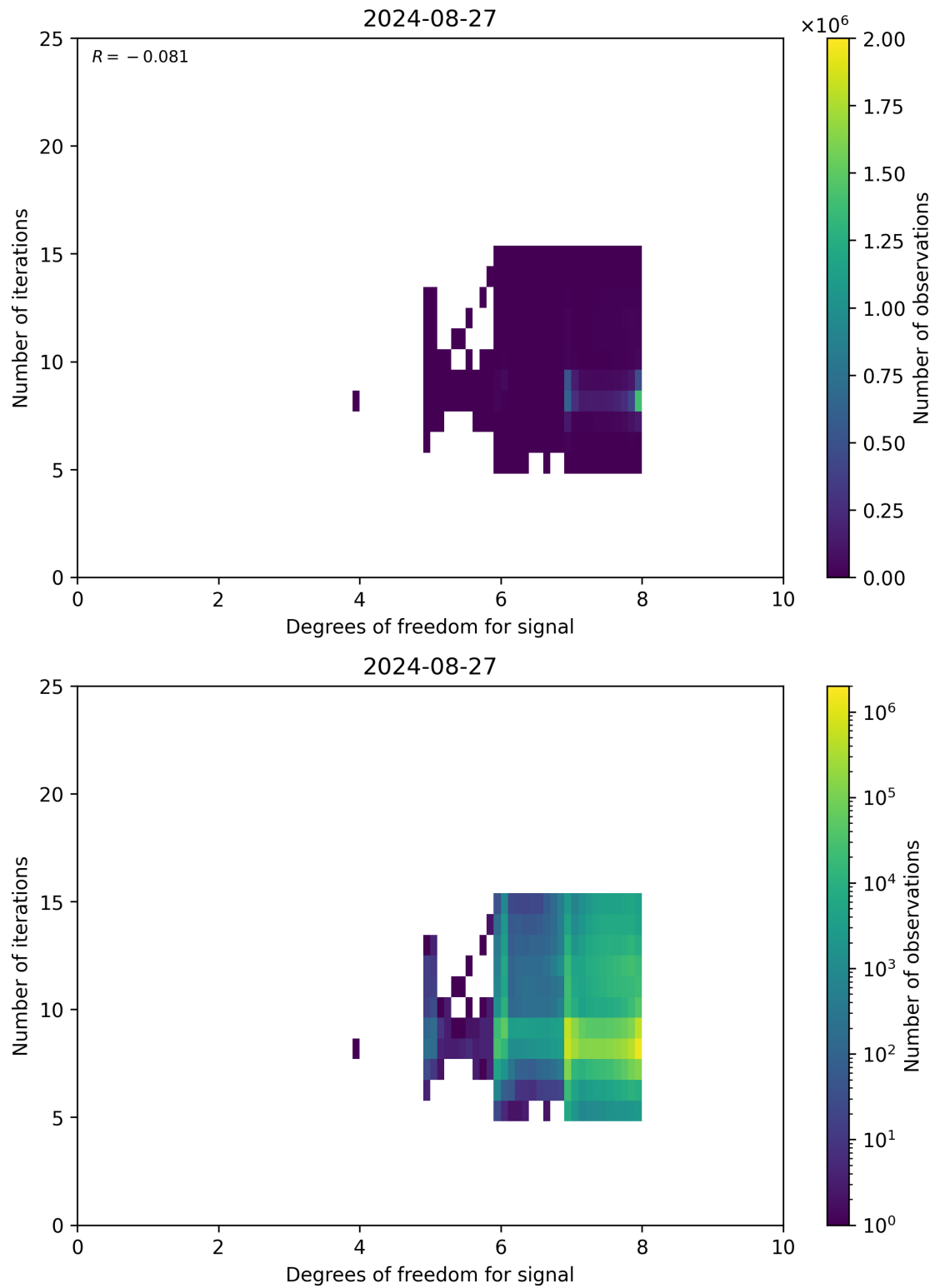
Figure 50: Scatter density plot of “Degrees of freedom for signal” against “Number of iterations” for 2024-08-27 to 2024-08-28.
