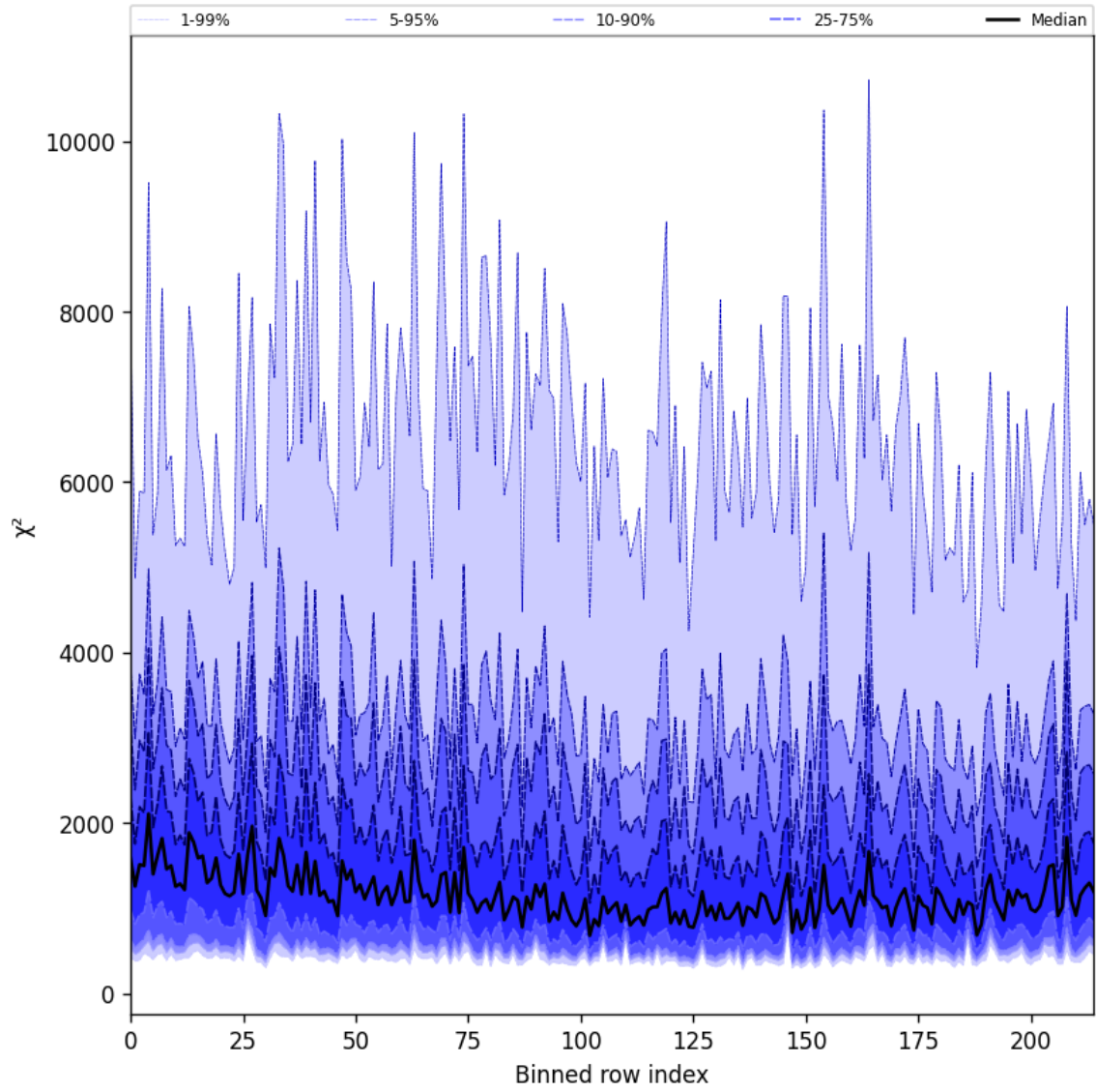
Figure 30: Along track statistics of “ \chi^2 ” for 2024-08-27 to 2024-08-29
