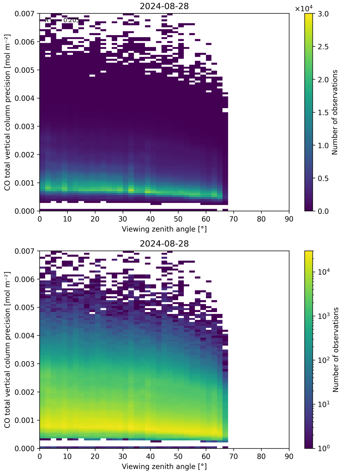
Figure 71: Scatter density plot of “Viewing zenith angle” against “CO total vertical column precision” for 2024-08-27 to 2024-08-29.
