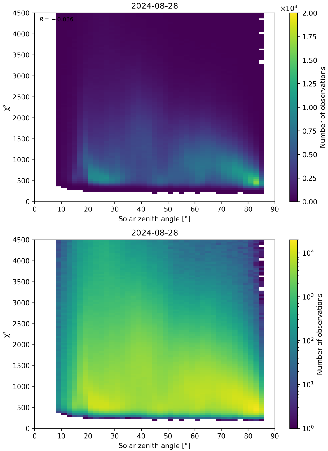
Figure 64: Scatter density plot of “Solar zenith angle” against “ \chi^2 ” for 2024-08-27 to 2024-08-29.
