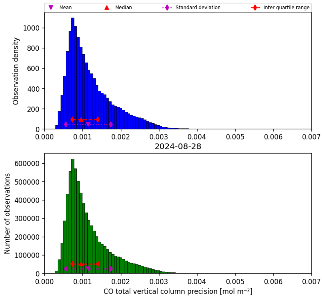
Figure 20: Histogram of “CO total vertical column precision” for 2024-08-27 to 2024-08-29
