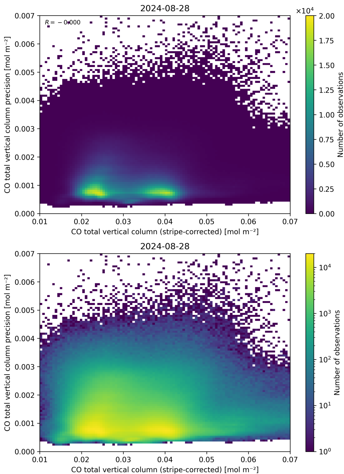
Figure 36: Scatter density plot of “CO total vertical column (stripe-corrected)” against “CO total vertical column precision” for 2024-08-27 to 2024-08-29.
