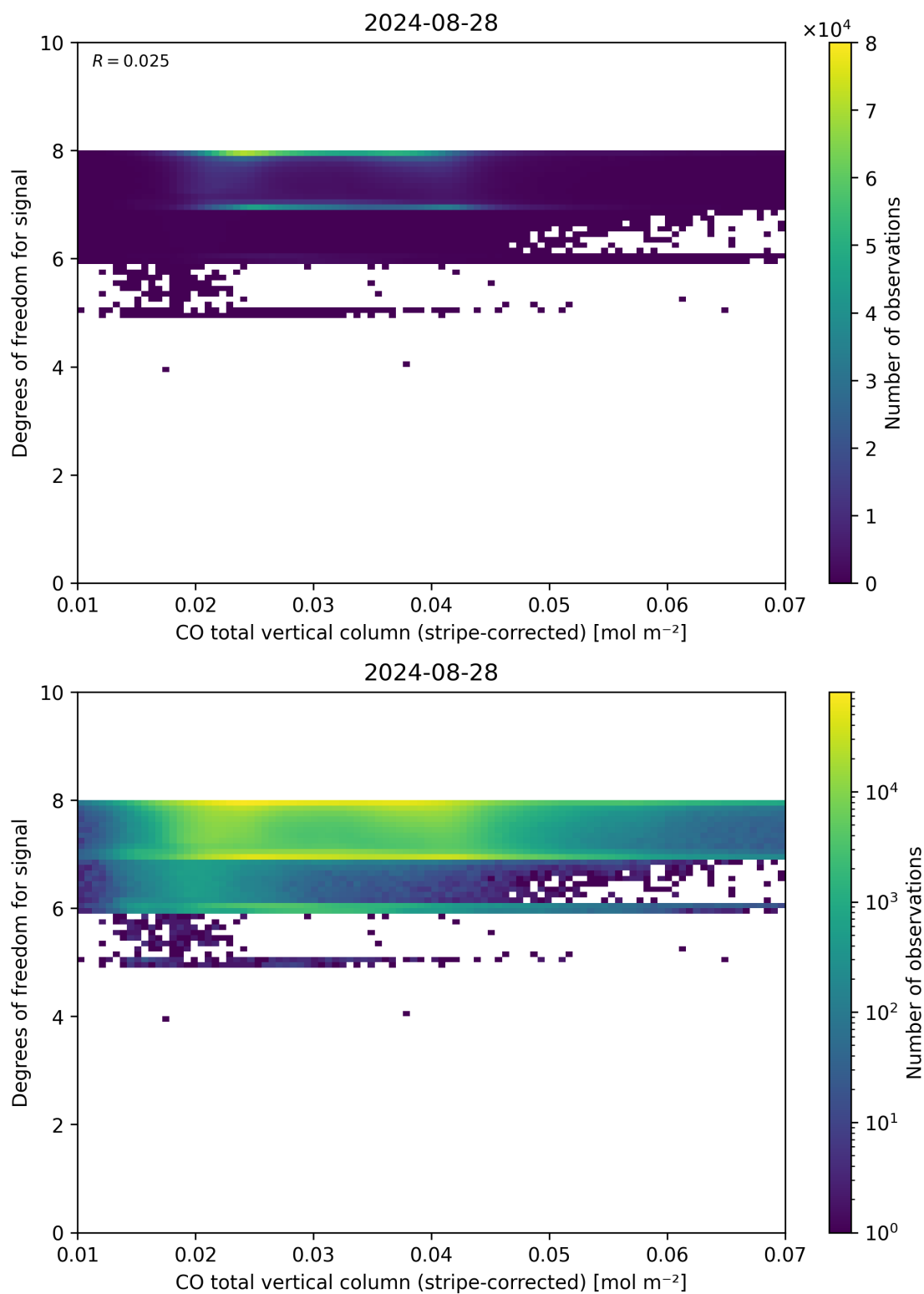
Figure 38: Scatter density plot of “CO total vertical column (stripe-corrected)” against “Degrees of freedom for signal” for 2024-08-27 to 2024-08-29.
