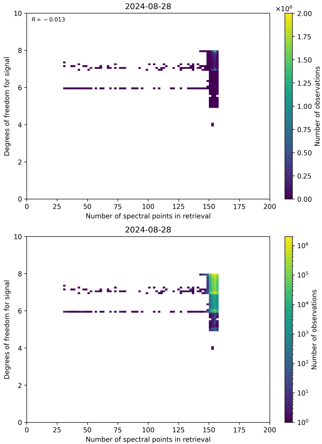
Figure 59: Scatter density plot of “Number of spectral points in retrieval” against “Degrees of freedom for signal” for 2024-08-27 to 2024-08-29.
