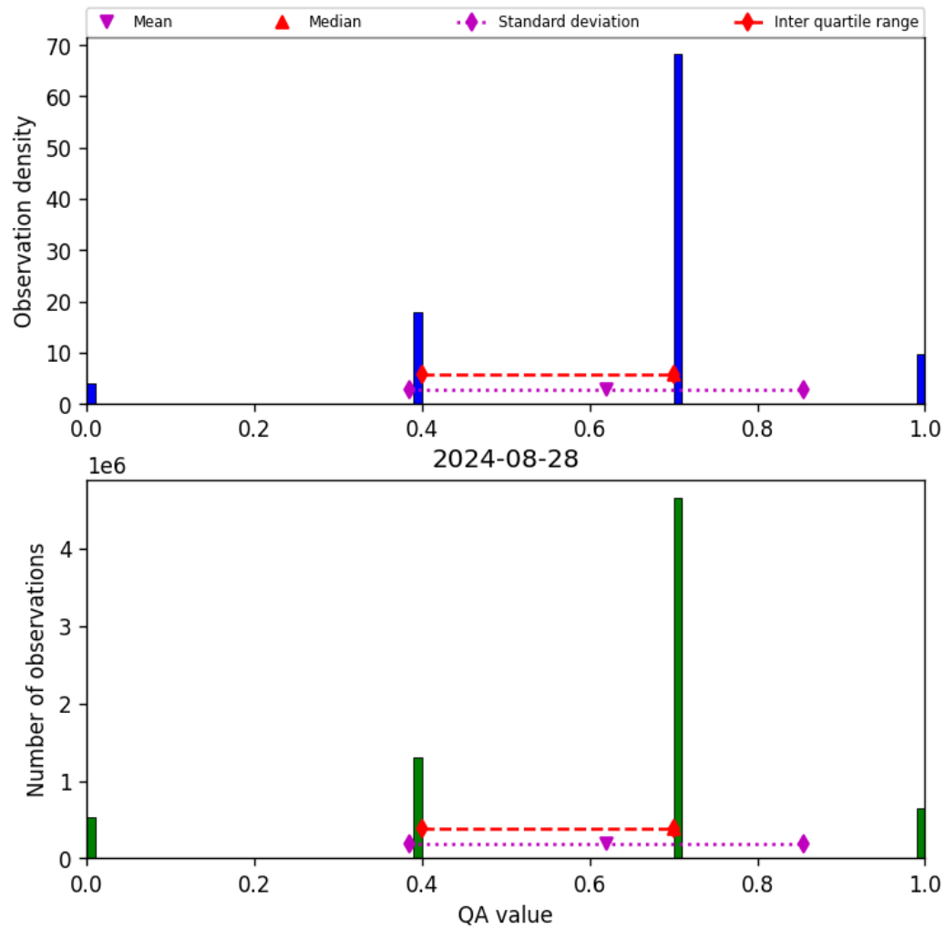
Figure 17: Histogram of “QA value” for 2024-08-27 to 2024-08-29
