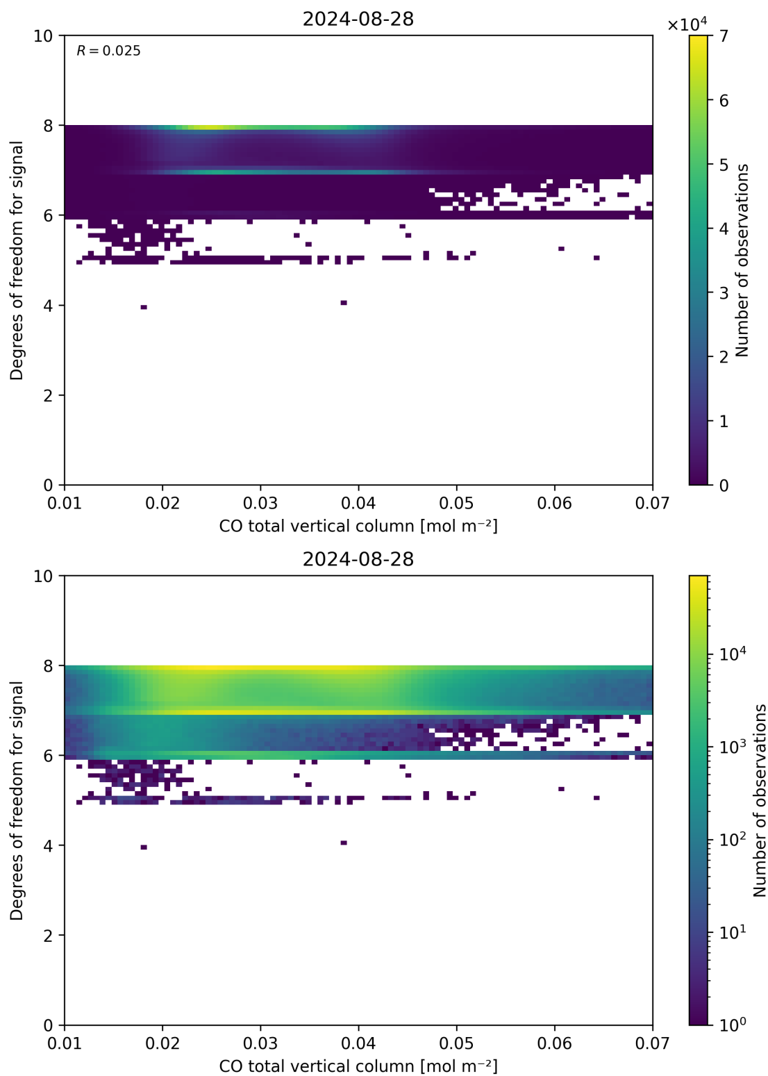
Figure 41: Scatter density plot of “CO total vertical column” against “Degrees of freedom for signal” for 2024-08-27 to 2024-08-29.
