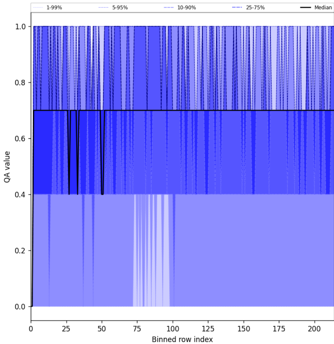
Figure 25: Along track statistics of “QA value” for 2024-08-27 to 2024-08-29
