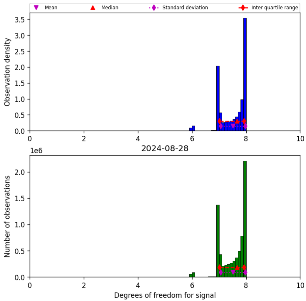
Figure 23: Histogram of “Degrees of freedom for signal” for 2024-08-27 to 2024-08-29
