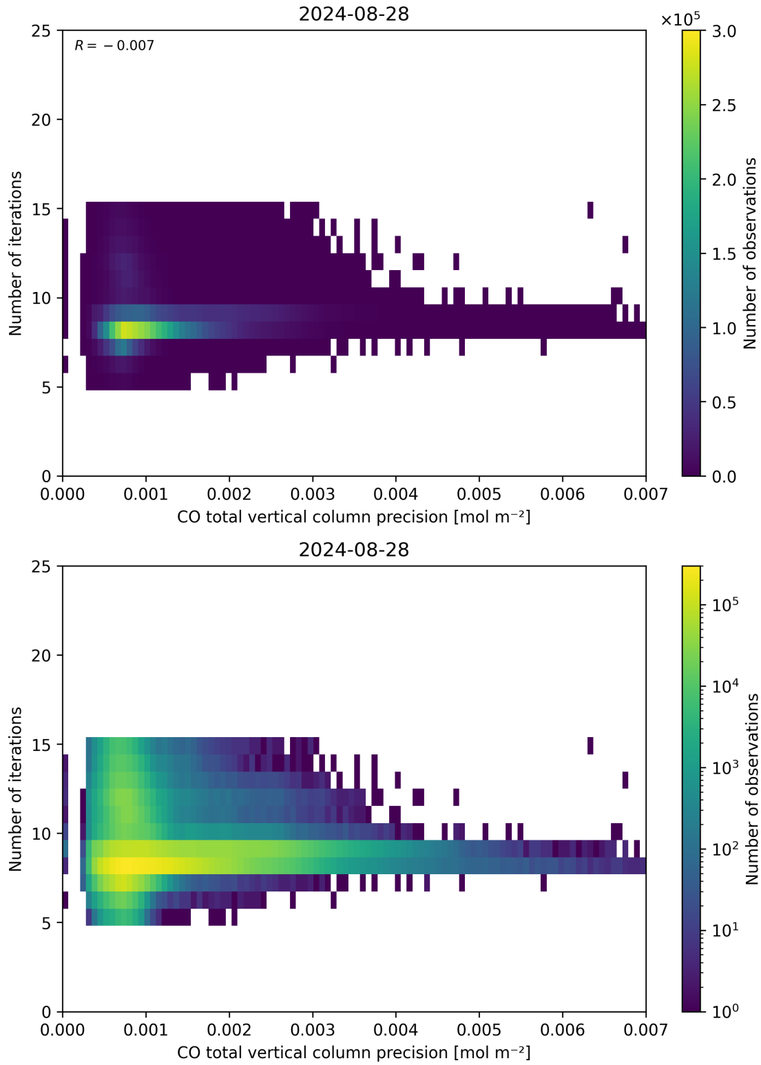
Figure 46: Scatter density plot of “CO total vertical column precision” against “Number of iterations” for 2024-08-27 to 2024-08-29.
