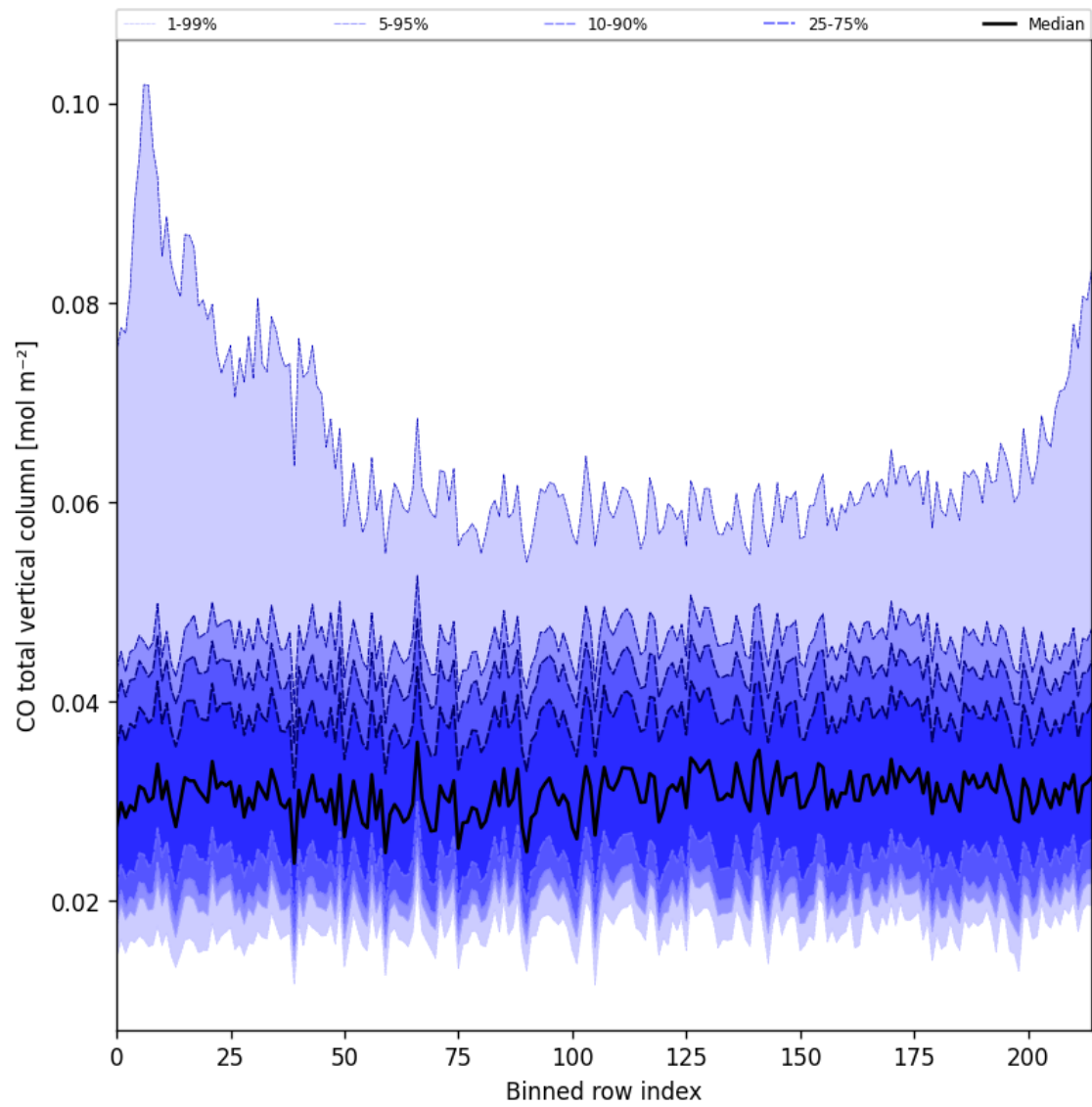
Figure 26: Along track statistics of “CO total vertical column” for 2024-08-27 to 2024-08-29
