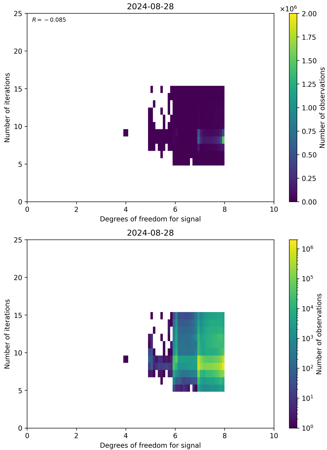
Figure 50: Scatter density plot of “Degrees of freedom for signal” against “Number of iterations” for 2024-08-27 to 2024-08-29.
