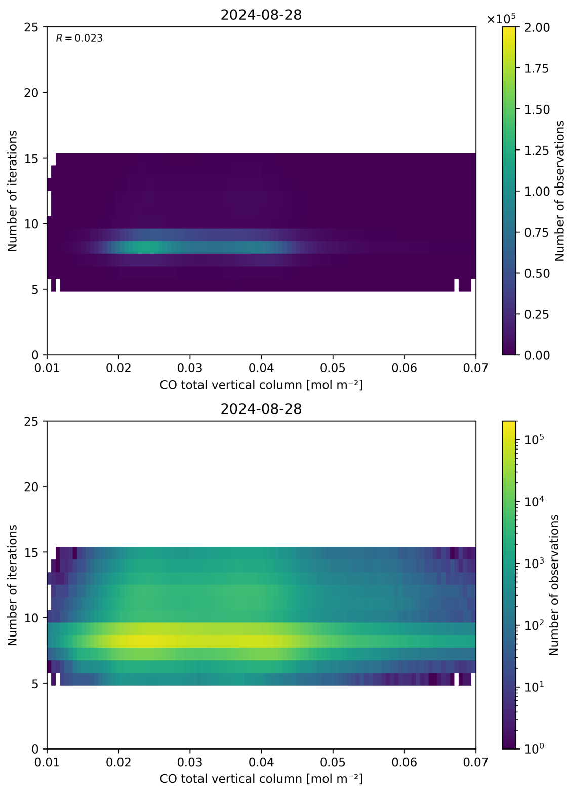
Figure 42: Scatter density plot of “CO total vertical column” against “Number of iterations” for 2024-08-27 to 2024-08-29.
