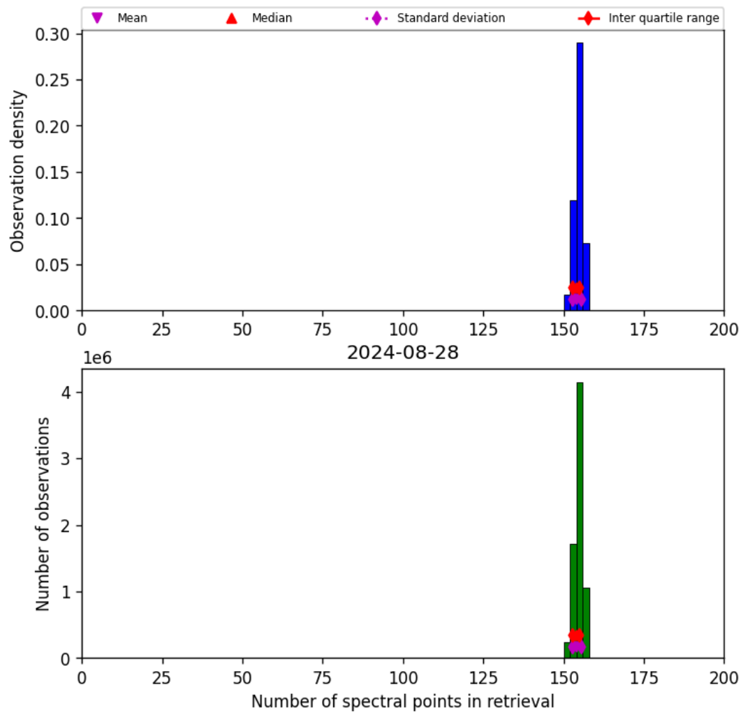
Figure 21: Histogram of “Number of spectral points in retrieval” for 2024-08-27 to 2024-08-29
