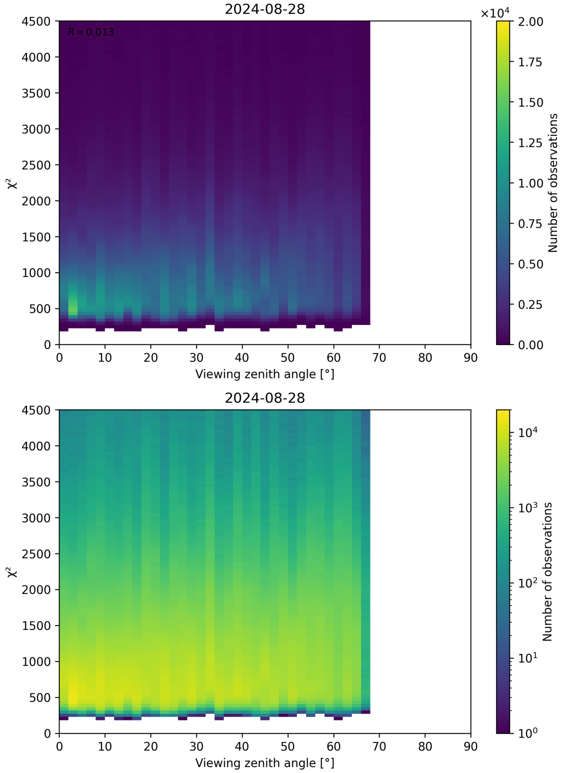
Figure 72: Scatter density plot of “Viewing zenith angle” against “ \chi^2 ” for 2024-08-27 to 2024-08-29.
