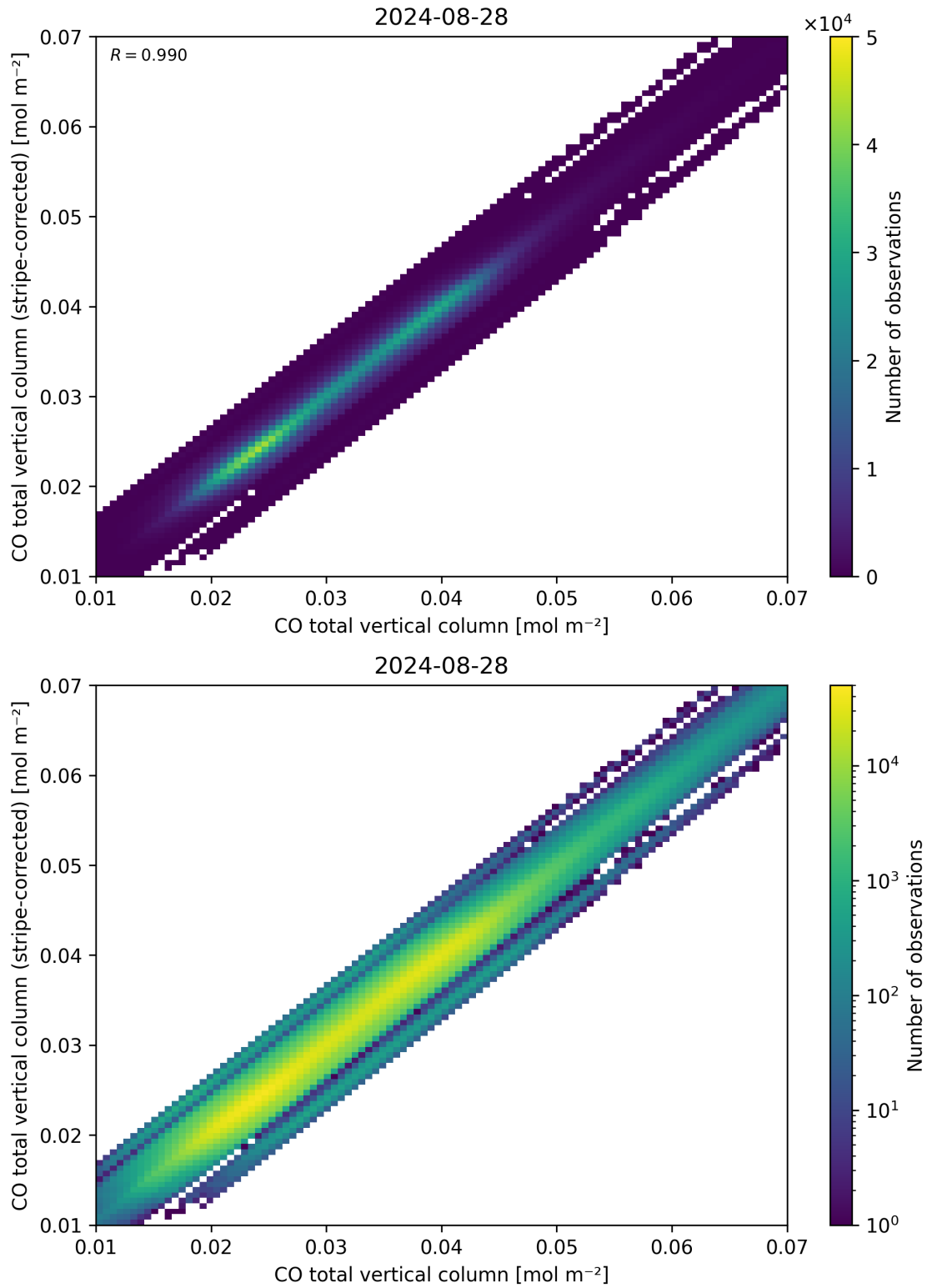
Figure 33: Scatter density plot of “CO total vertical column” against “CO total vertical column (stripe-corrected)” for 2024-08-27 to 2024-08-29.
