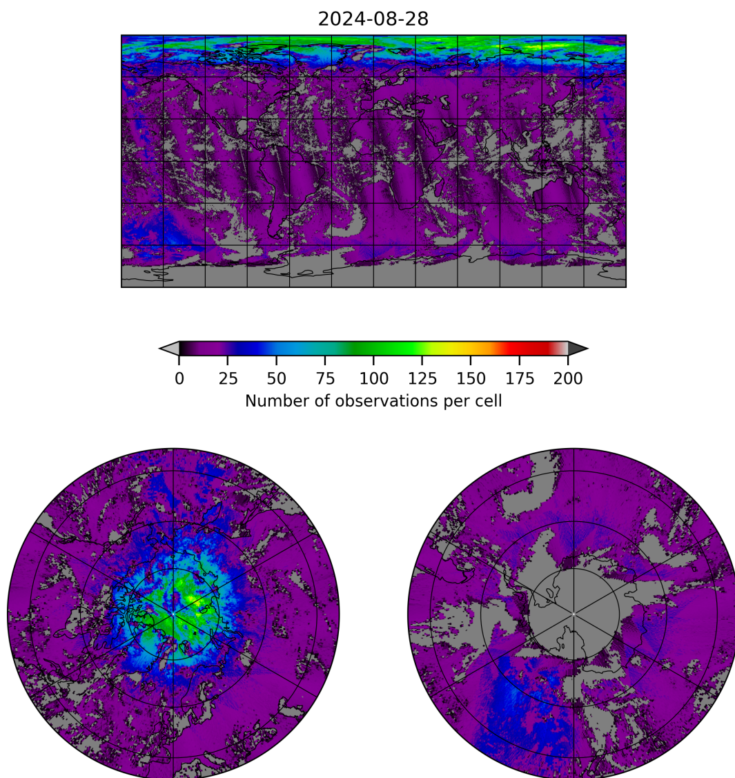
Figure 8: Map of the number of observations for 2024-08-27 to 2024-08-29
