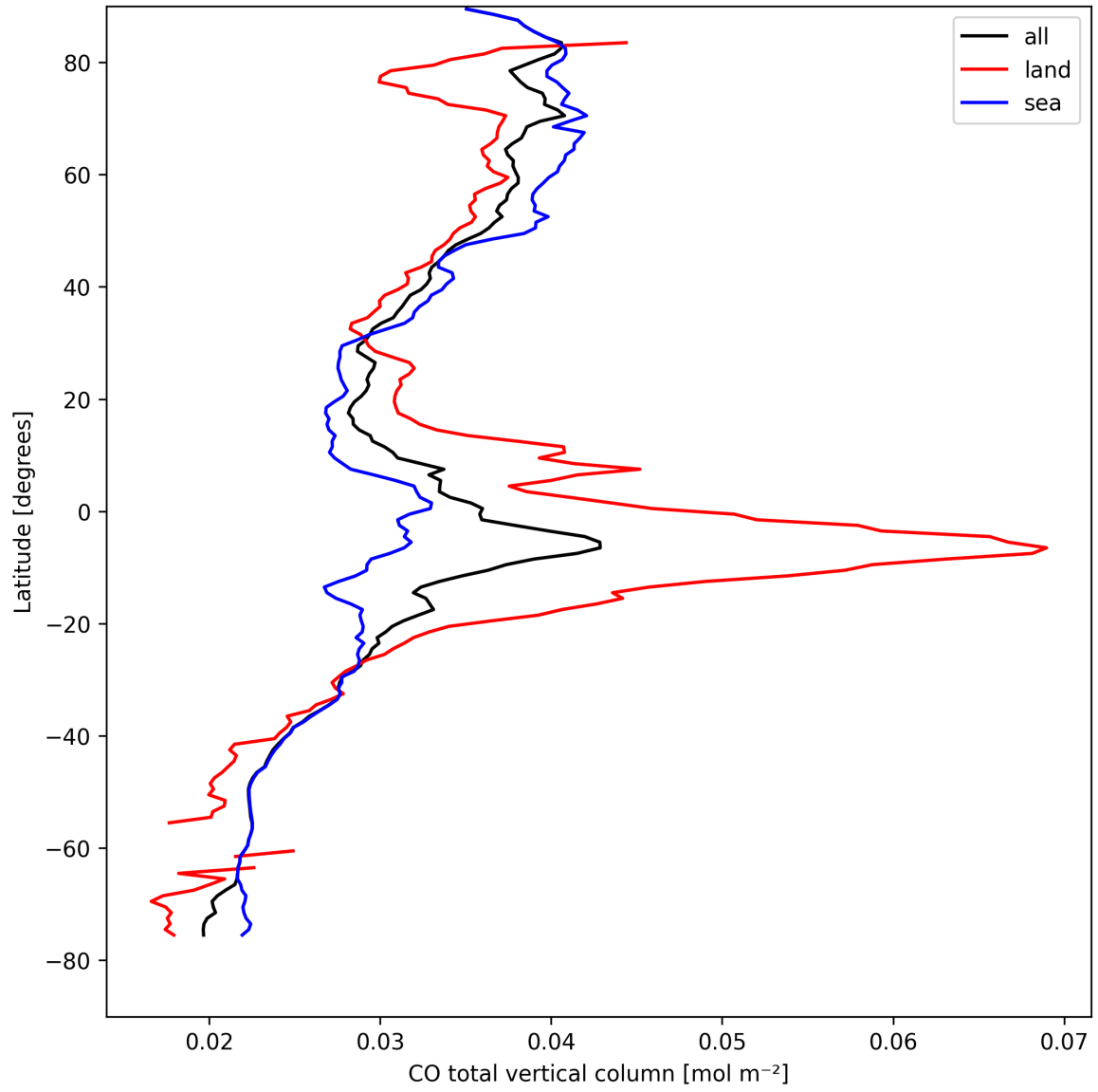
Figure 10: Zonal average of “CO total vertical column” for 2024-08-27 to 2024-08-29.
