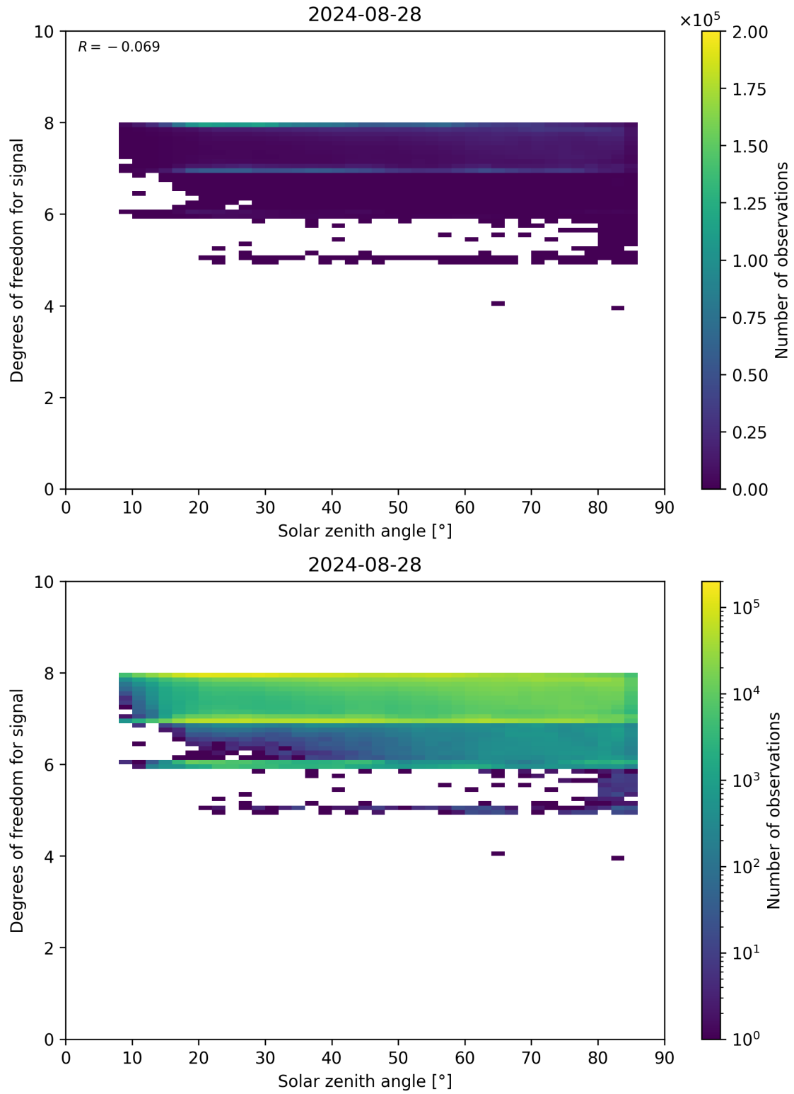
Figure 65: Scatter density plot of “Solar zenith angle” against “Degrees of freedom for signal” for 2024-08-27 to 2024-08-29.
