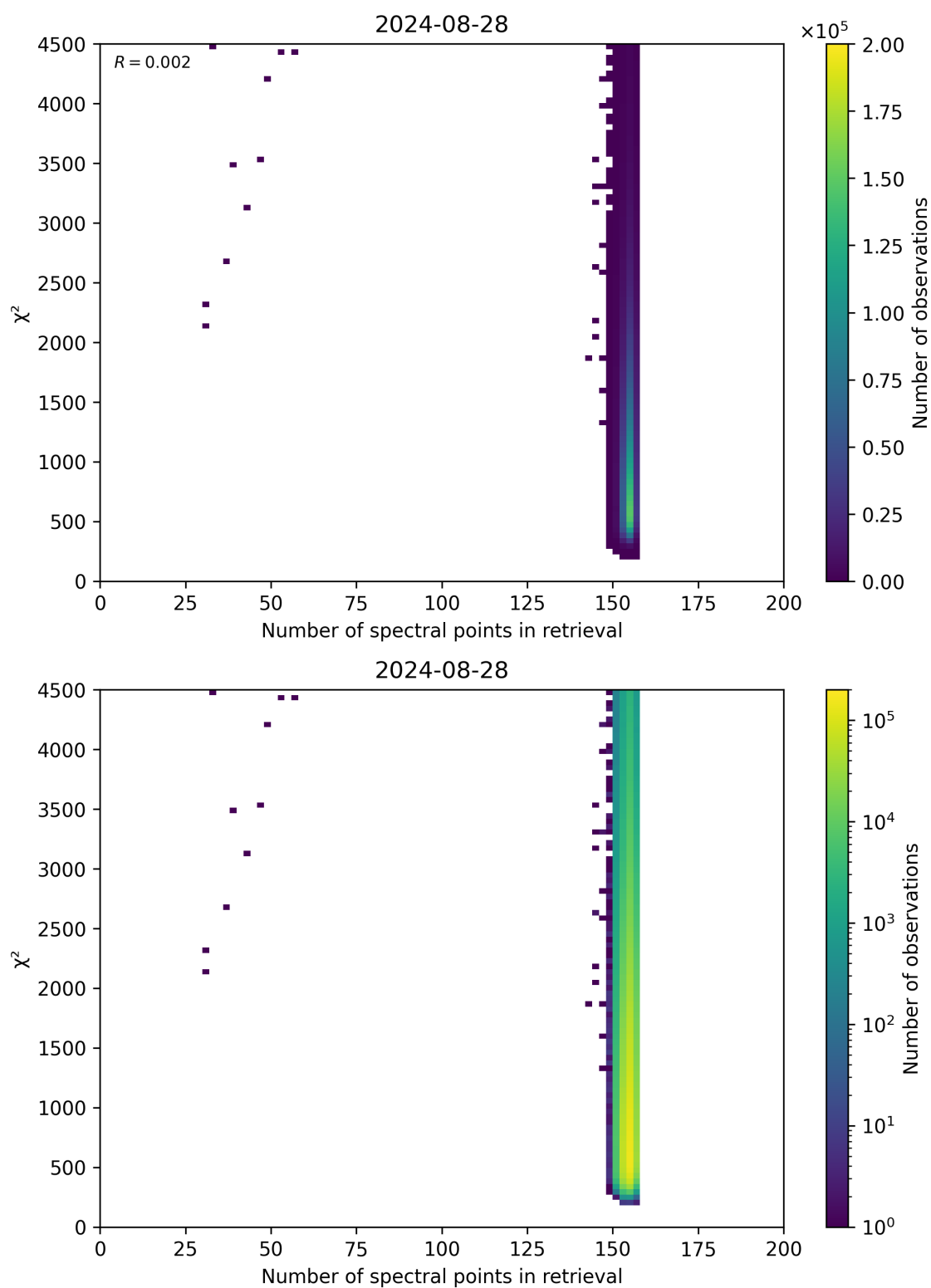
Figure 58: Scatter density plot of “Number of spectral points in retrieval” against “ \chi^2 ” for 2024-08-27 to 2024-08-29.
