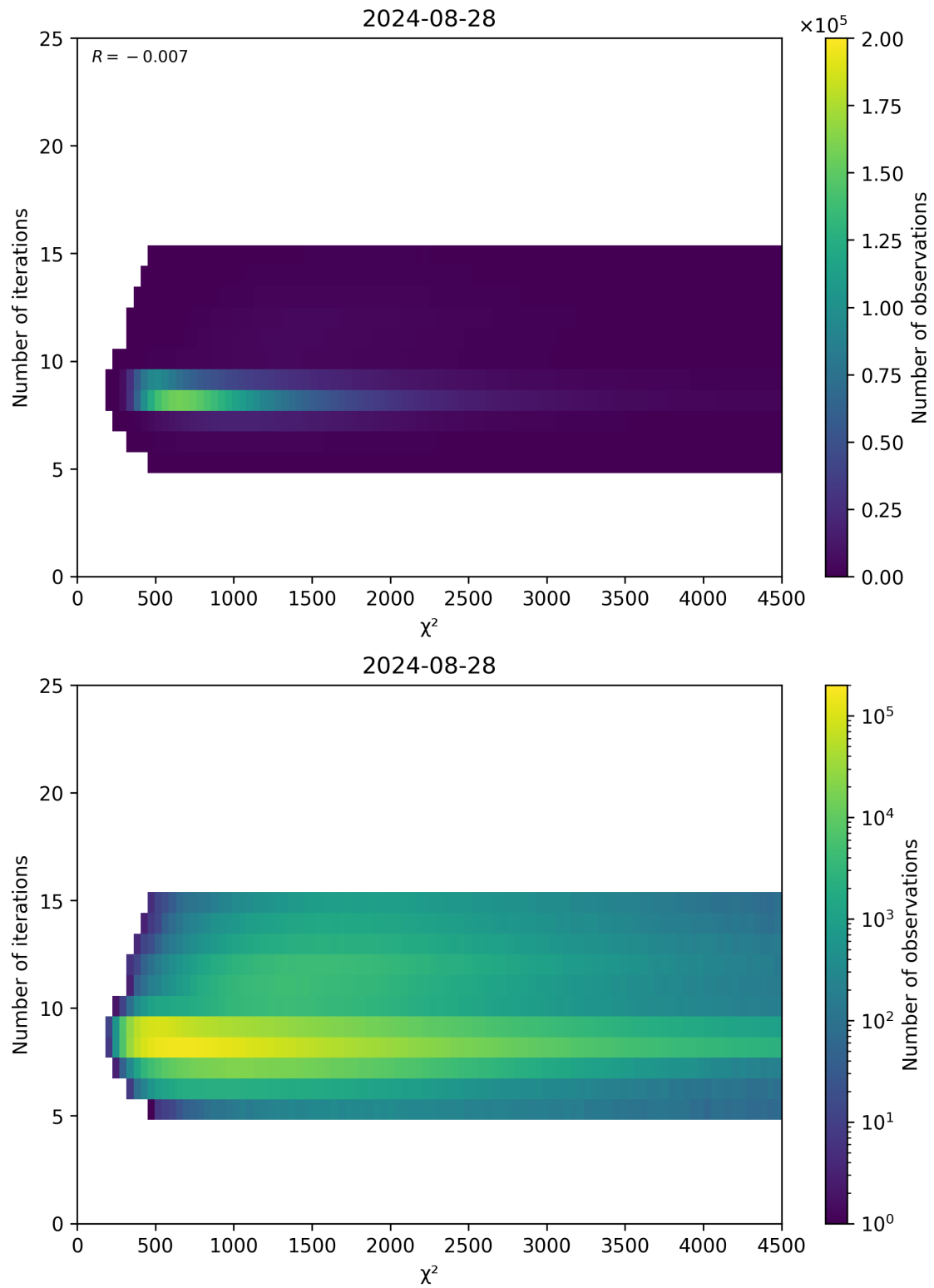
Figure 49: Scatter density plot of “ \chi^2 ” against “Number of iterations” for 2024-08-27 to 2024-08-29.
