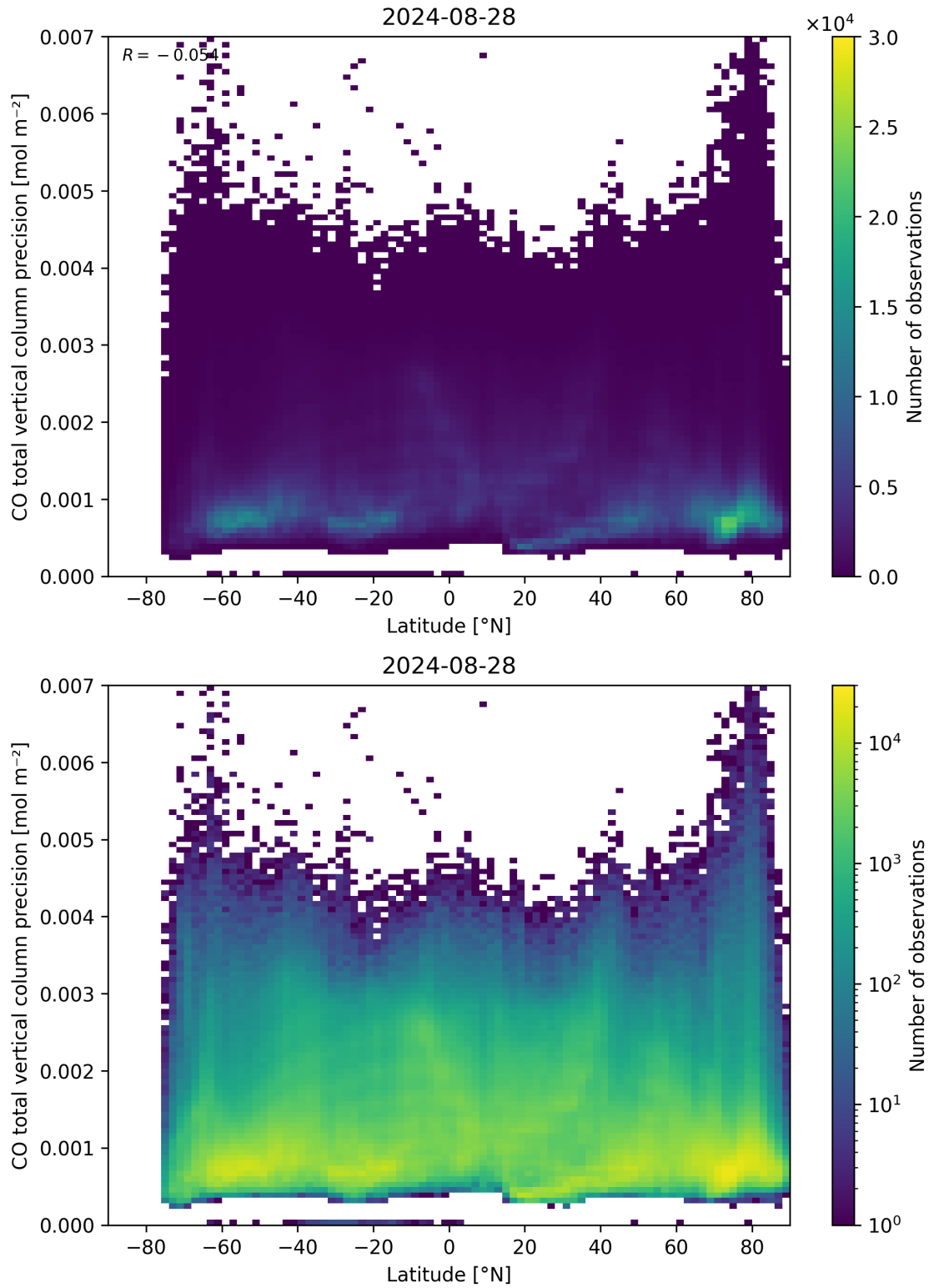
Figure 53: Scatter density plot of “Latitude” against “CO total vertical column precision” for 2024-08-27 to 2024-08-29.
