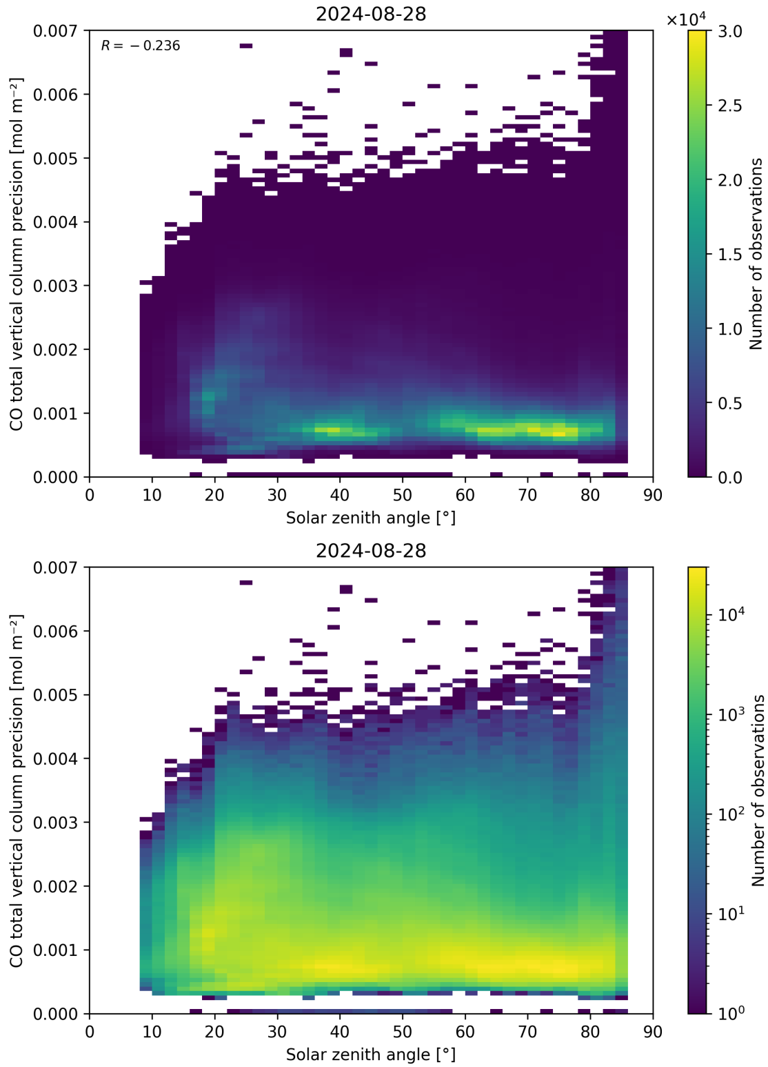
Figure 63: Scatter density plot of “Solar zenith angle” against “CO total vertical column precision” for 2024-08-27 to 2024-08-29.
