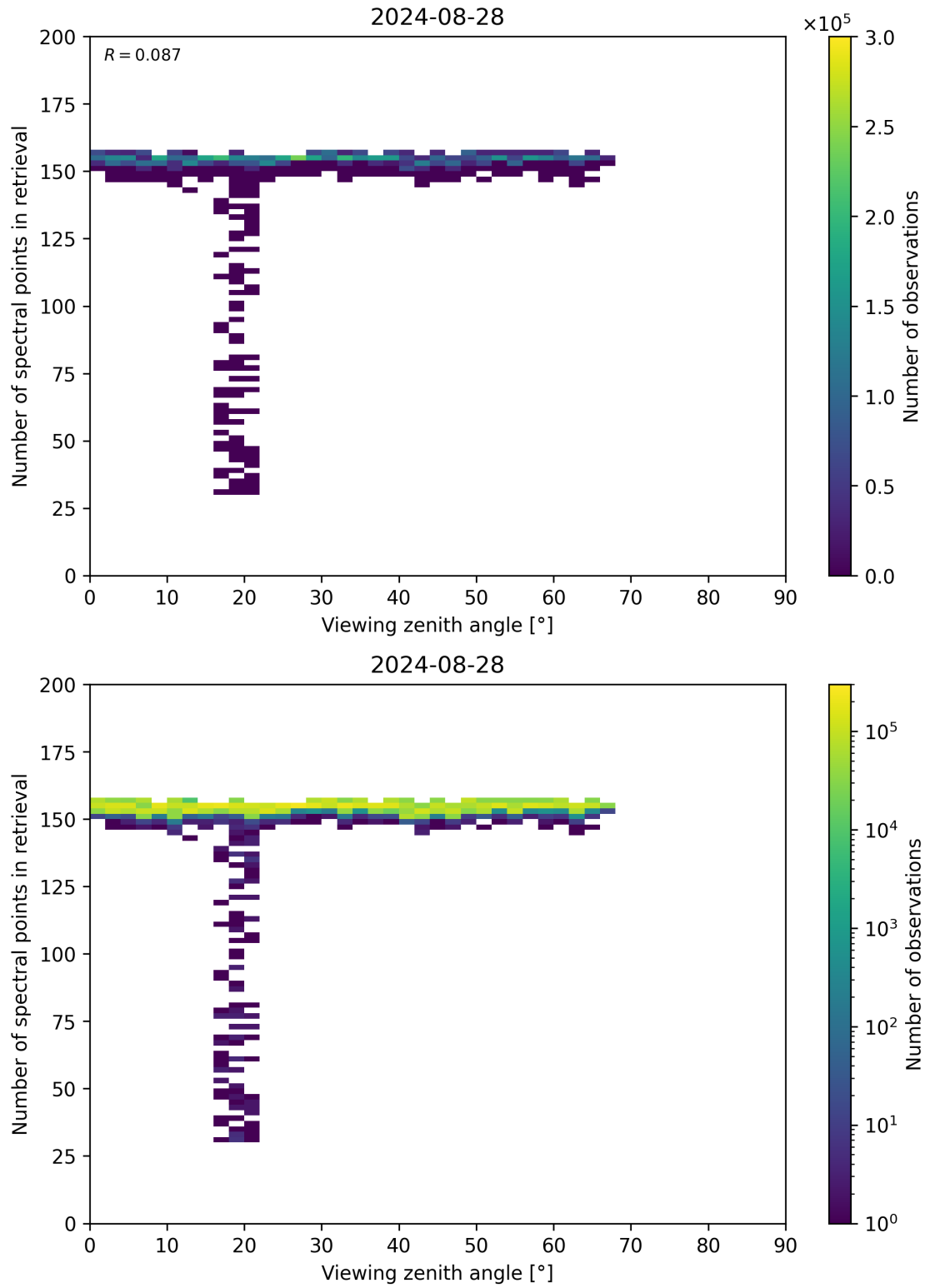
Figure 76: Scatter density plot of “Viewing zenith angle” against “Number of spectral points in retrieval” for 2024-08-27 to 2024-08-29.
