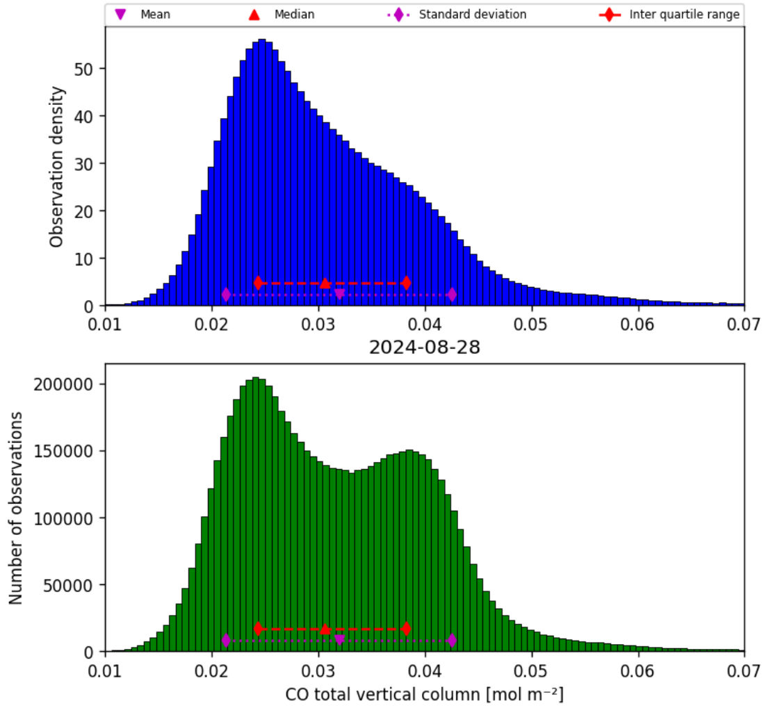
Figure 18: Histogram of “CO total vertical column” for 2024-08-27 to 2024-08-29
