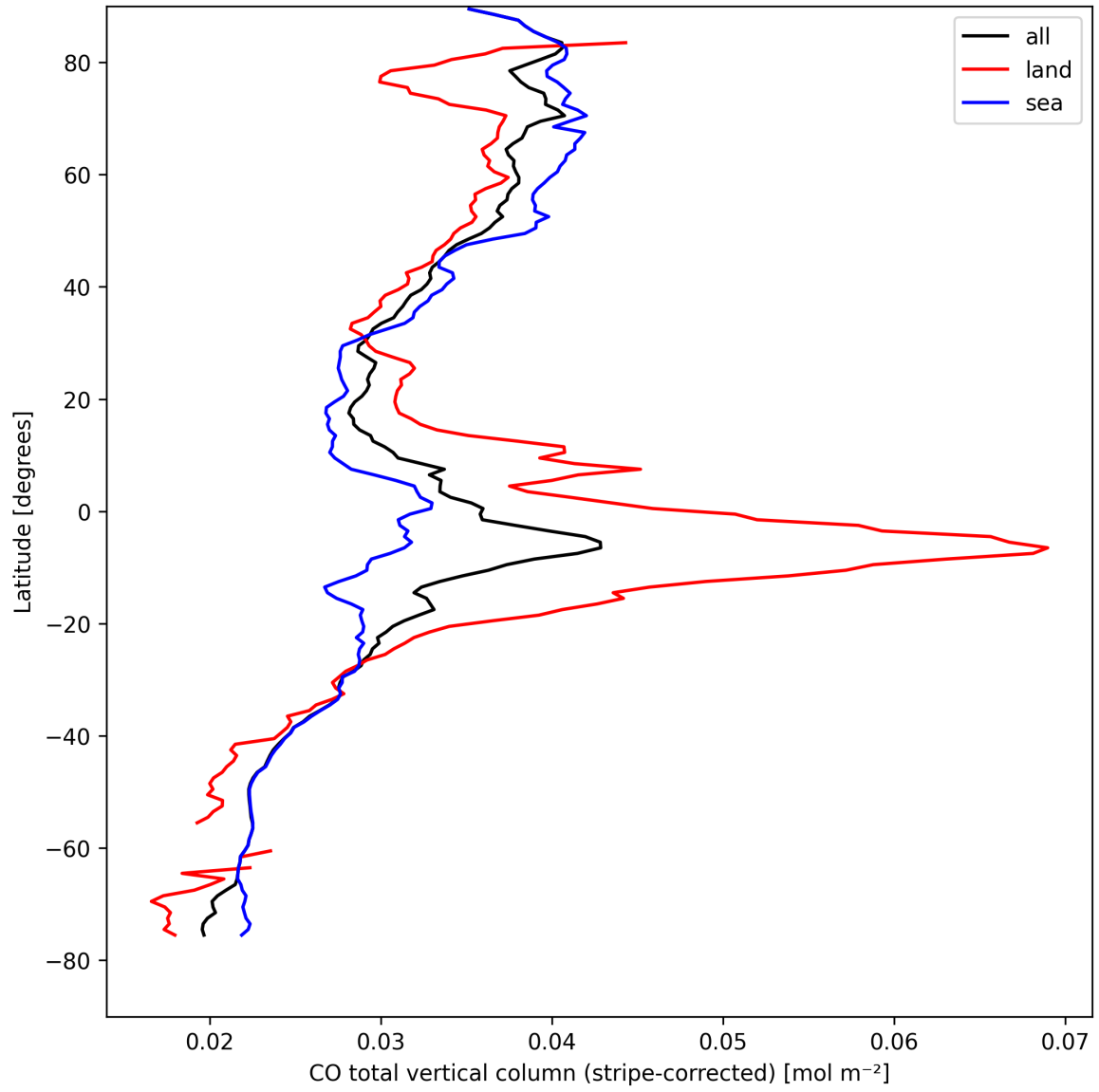
Figure 11: Zonal average of “CO total vertical column (stripe-corrected)” for 2024-08-27 to 2024-08-29.
