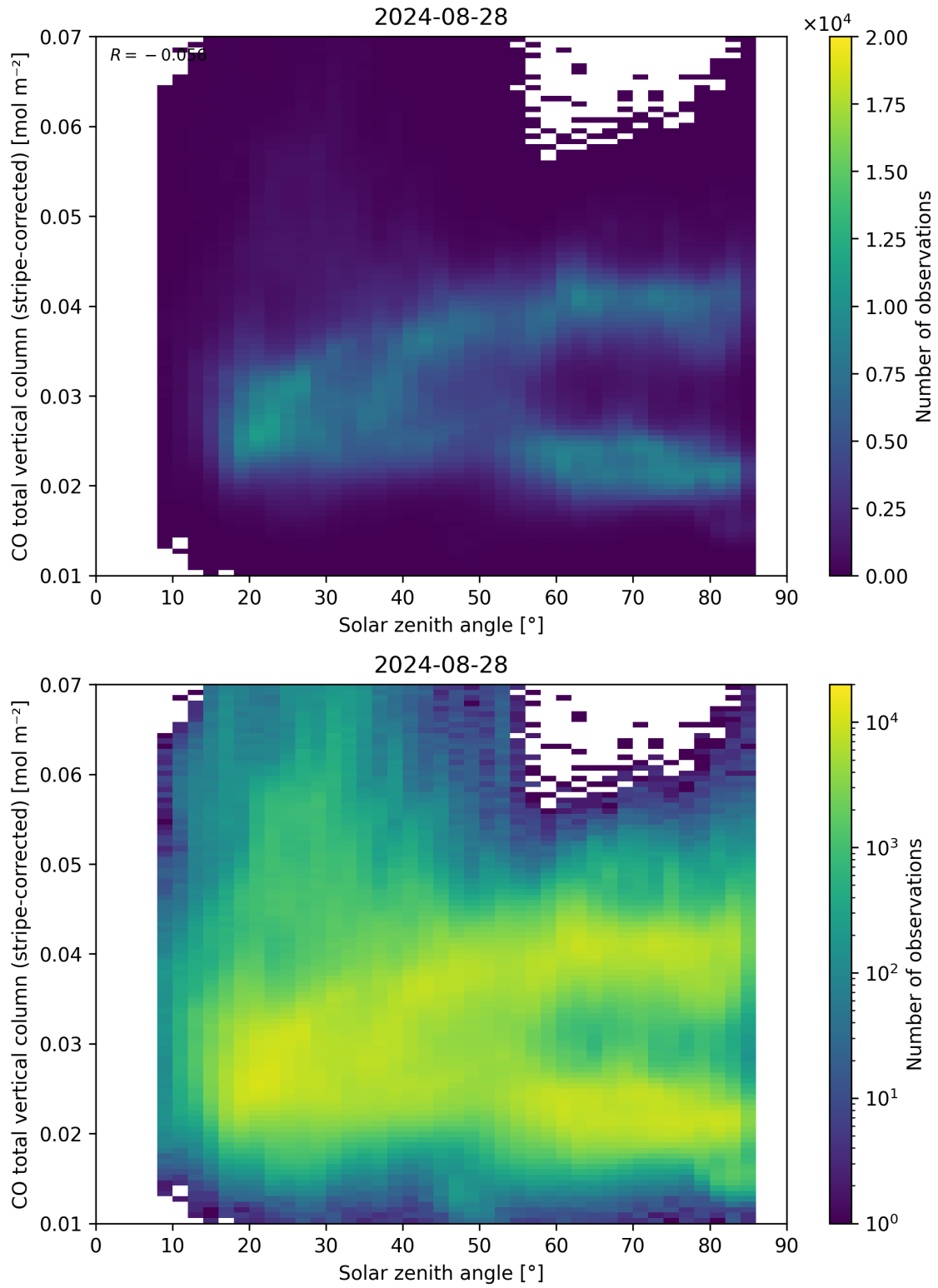
Figure 62: Scatter density plot of “Solar zenith angle” against “CO total vertical column (stripe-corrected)” for 2024-08-27 to 2024-08-29.
