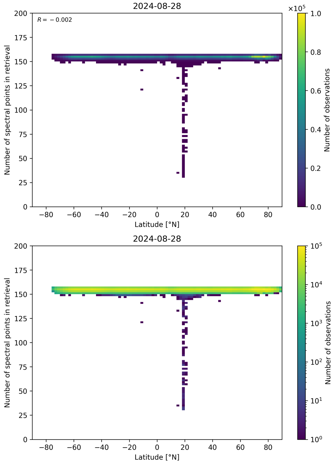
Figure 57: Scatter density plot of “Latitude” against “Number of spectral points in retrieval” for 2024-08-27 to 2024-08-29.
