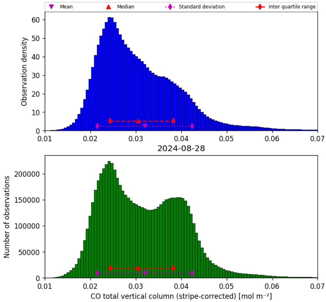
Figure 19: Histogram of “CO total vertical column (stripe-corrected)” for 2024-08-27 to 2024-08-29
