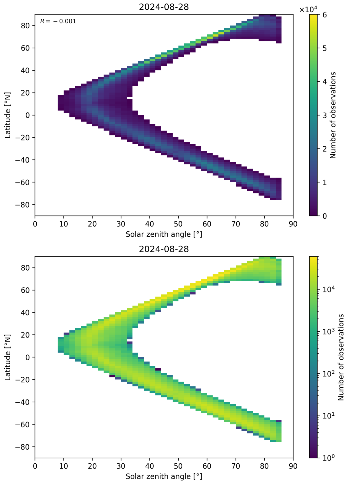
Figure 66: Scatter density plot of “Solar zenith angle” against “Latitude” for 2024-08-27 to 2024-08-29.
