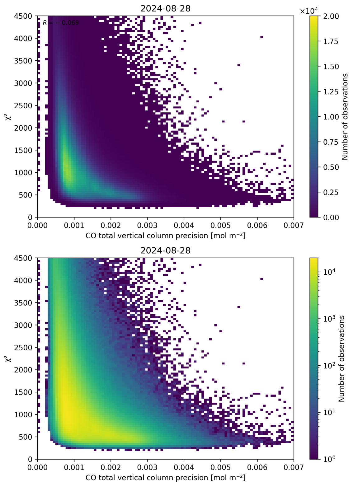
Figure 44: Scatter density plot of “CO total vertical column precision” against “ \chi^2 ” for 2024-08-27 to 2024-08-29.
