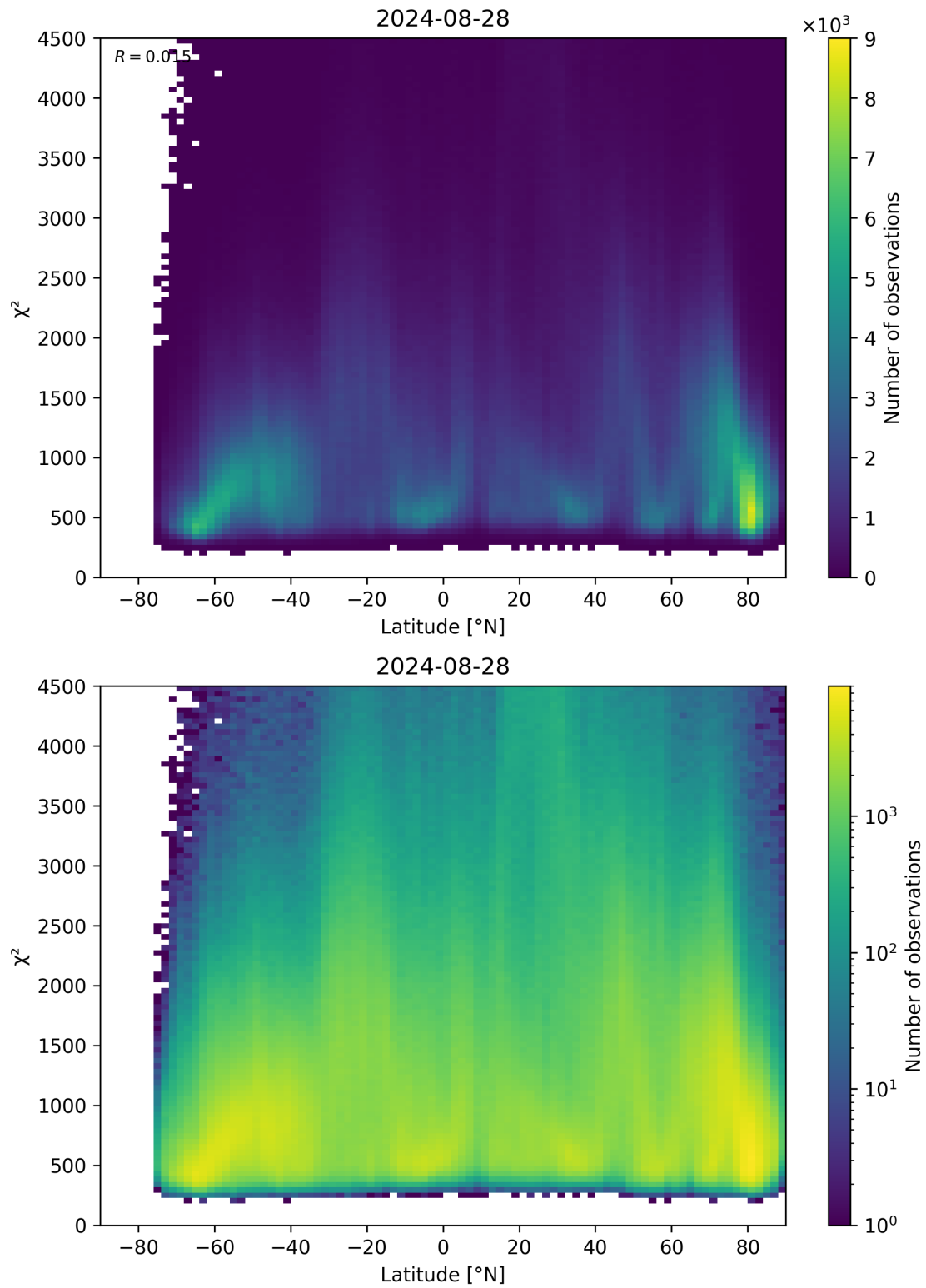
Figure 54: Scatter density plot of “Latitude” against “ \chi^2 ” for 2024-08-27 to 2024-08-29.
