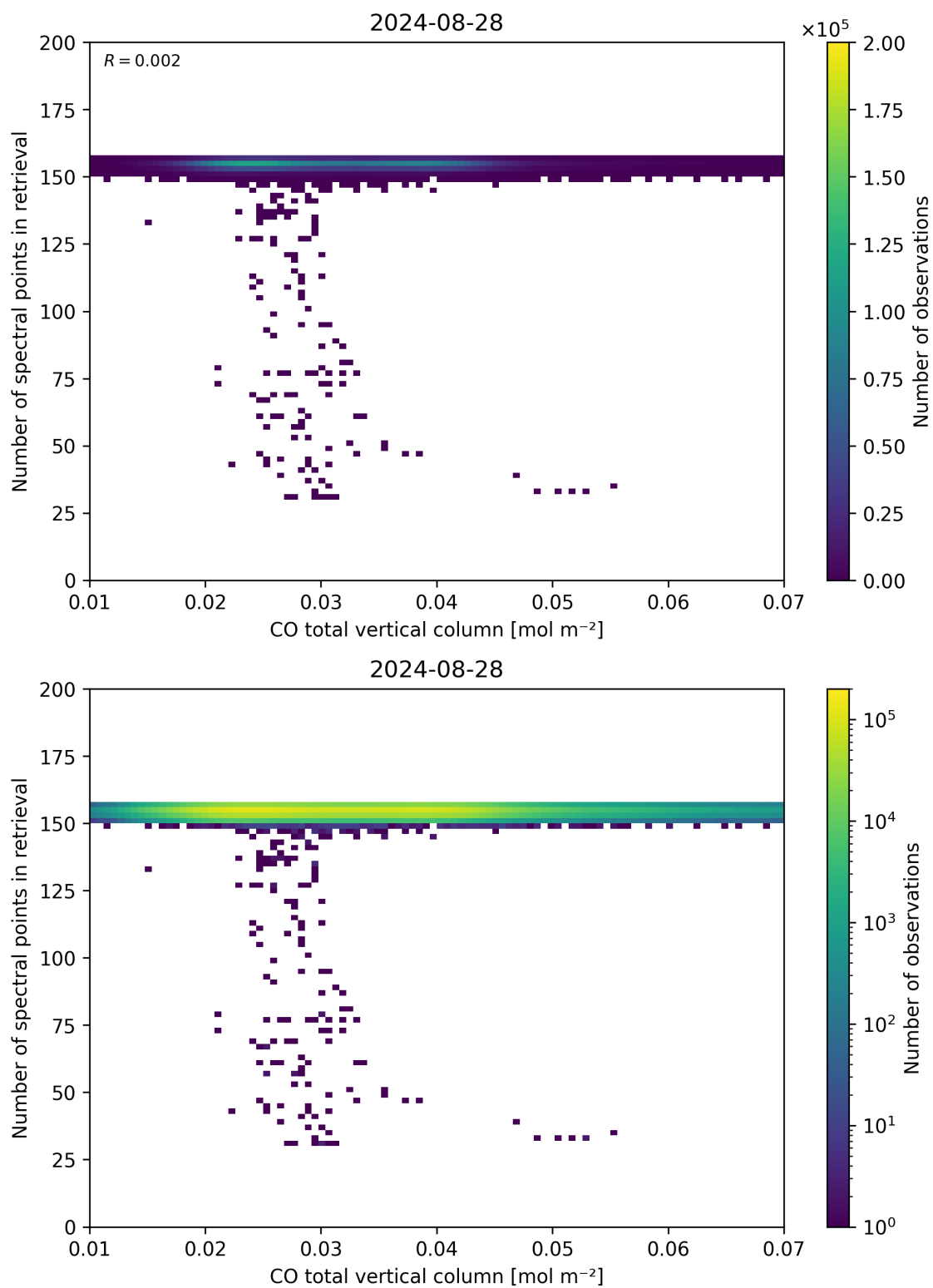
Figure 43: Scatter density plot of “CO total vertical column” against “Number of spectral points in retrieval” for 2024-08-27 to 2024-08-29.
