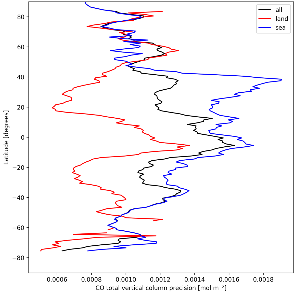
Figure 12: Zonal average of “CO total vertical column precision” for 2024-08-27 to 2024-08-29.
