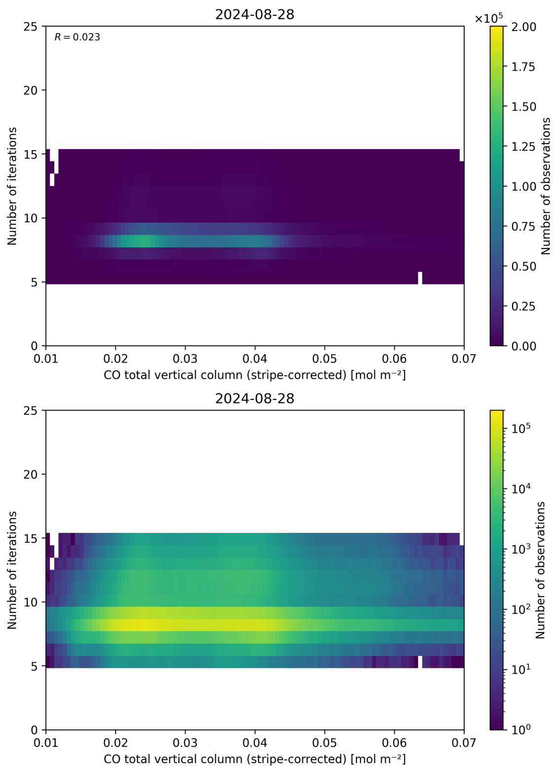
Figure 39: Scatter density plot of “CO total vertical column (stripe-corrected)” against “Number of iterations” for 2024-08-27 to 2024-08-29.
