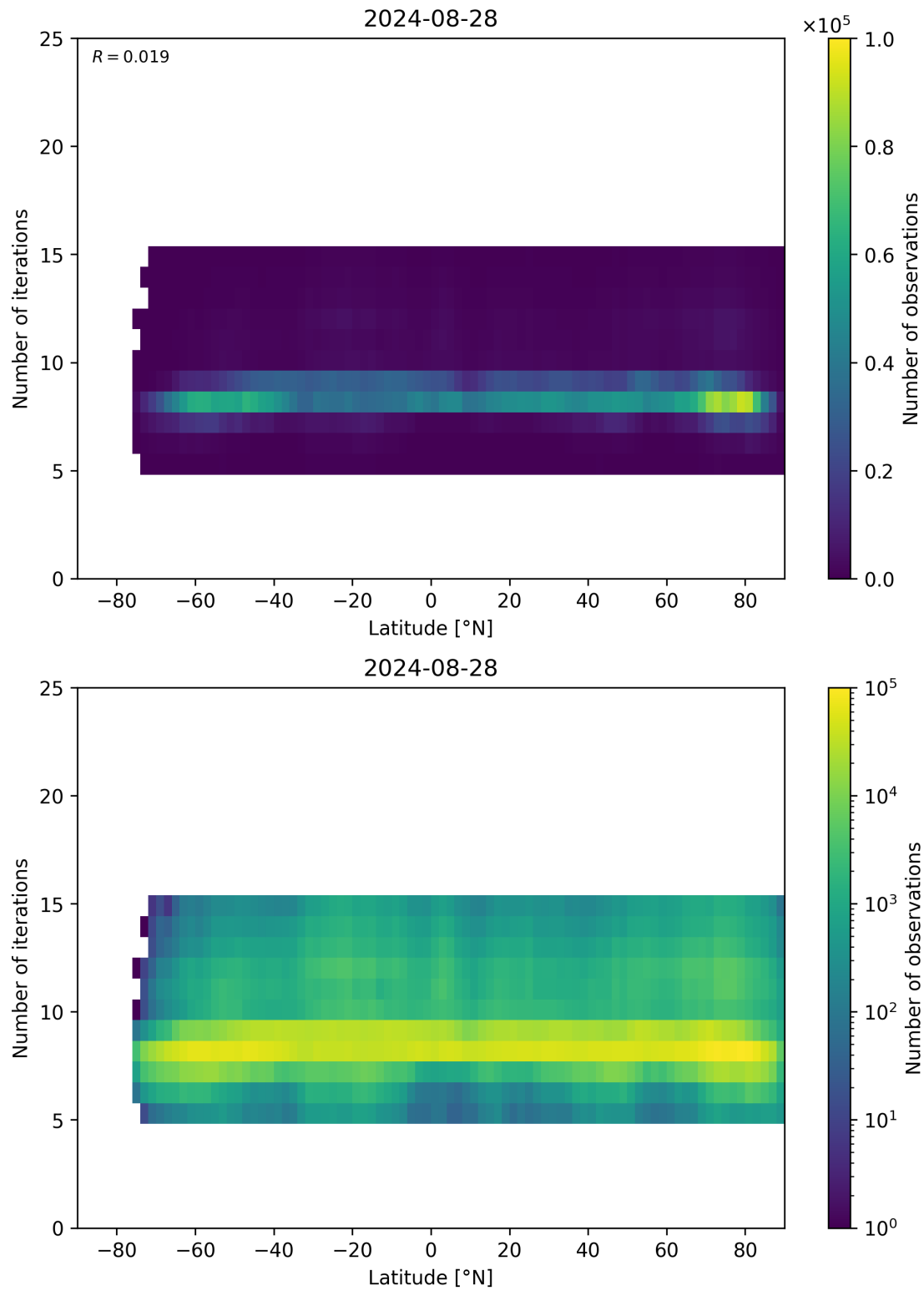
Figure 56: Scatter density plot of “Latitude” against “Number of iterations” for 2024-08-27 to 2024-08-29.
