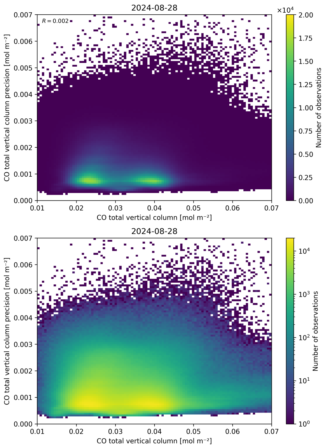
Figure 34: Scatter density plot of “CO total vertical column” against “CO total vertical column precision” for 2024-08-27 to 2024-08-29.
