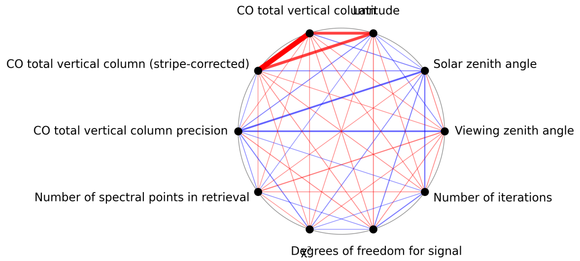
Figure 1: Map of correlation graph for 2024-08-27 to 2024-08-29.
