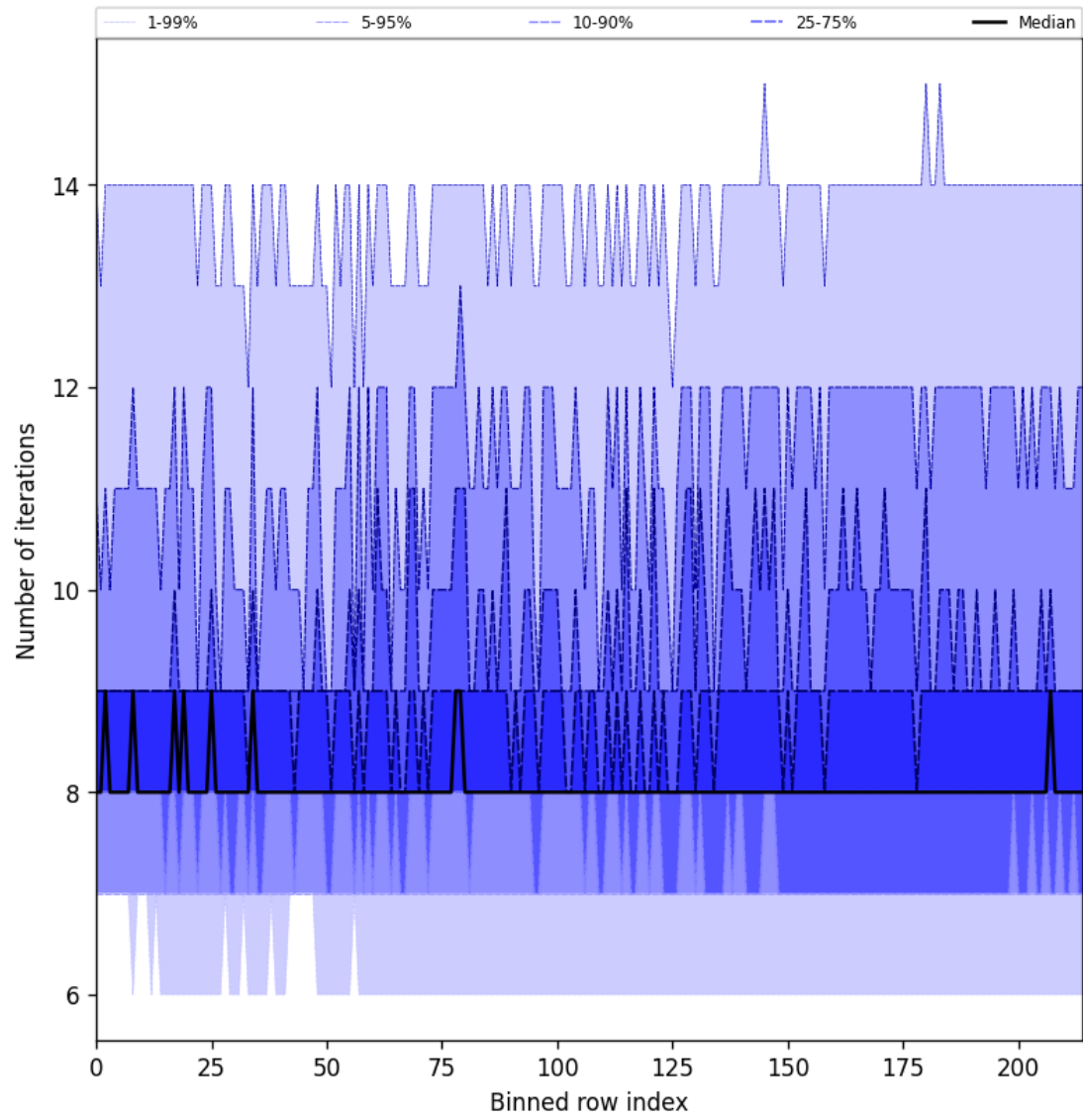
Figure 32: Along track statistics of “Number of iterations” for 2024-08-27 to 2024-08-29
