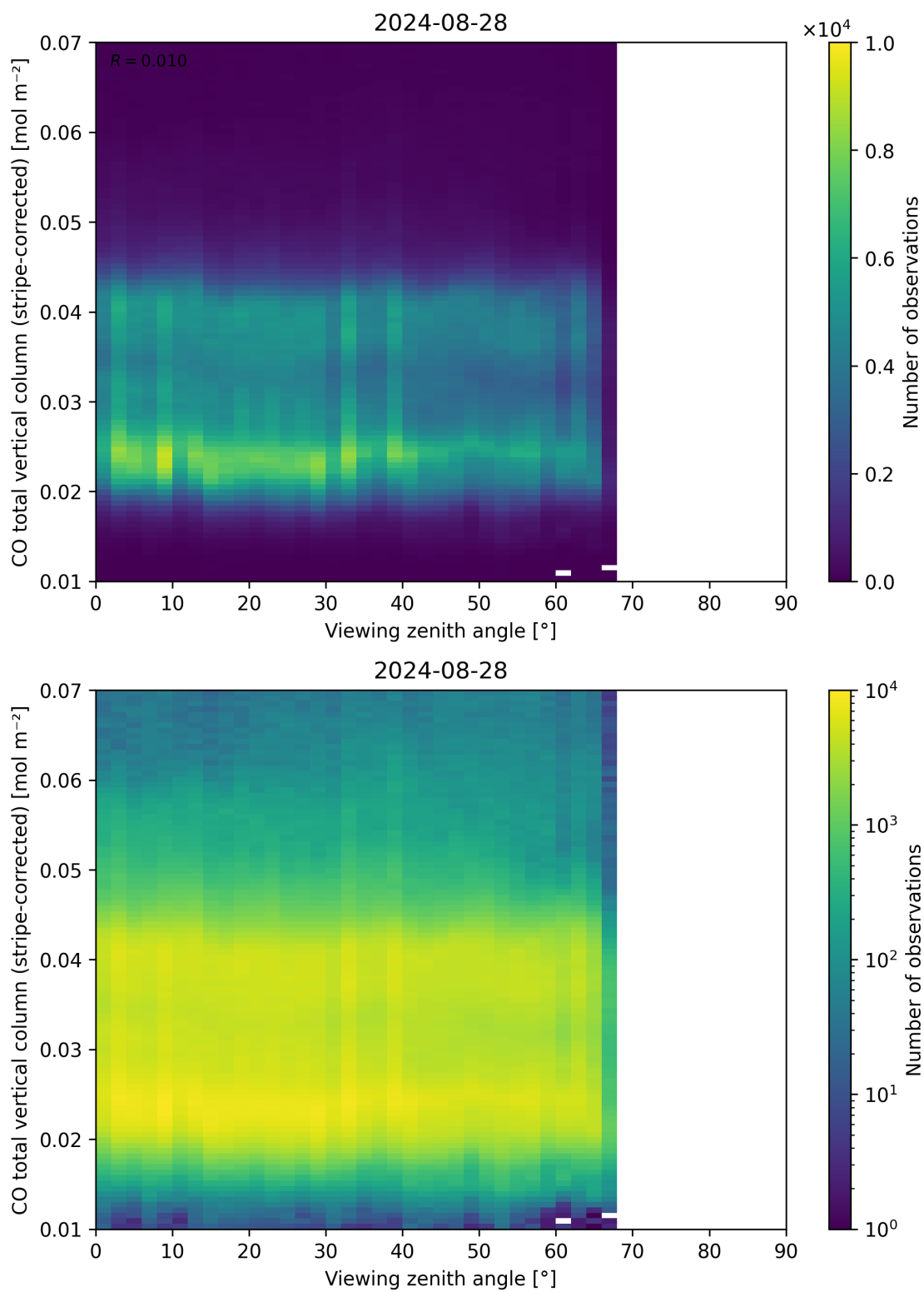
Figure 70: Scatter density plot of “Viewing zenith angle” against “CO total vertical column (stripe-corrected)” for 2024-08-27 to 2024-08-29.
