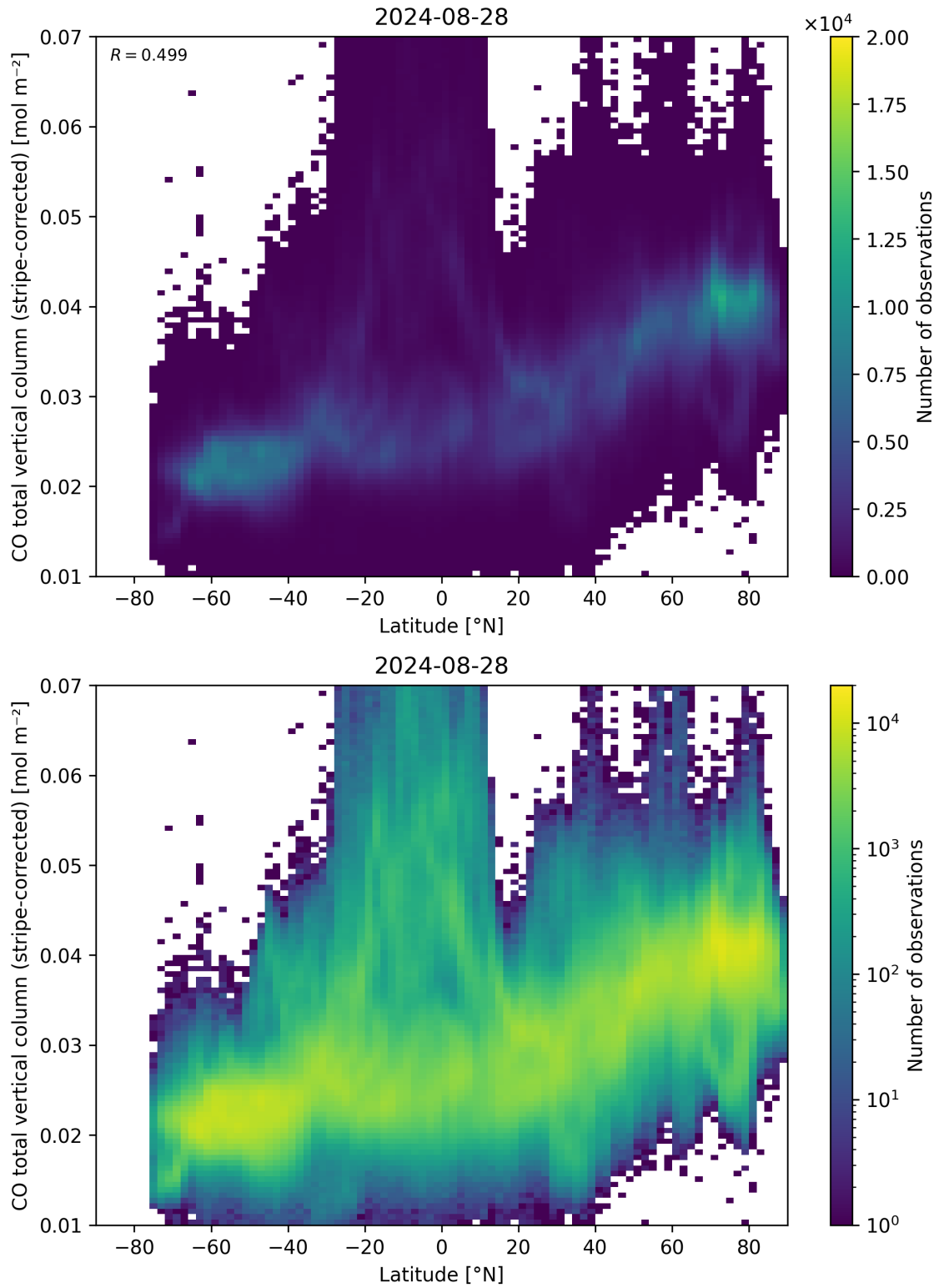
Figure 52: Scatter density plot of “Latitude” against “CO total vertical column (stripe-corrected)” for 2024-08-27 to 2024-08-29.
