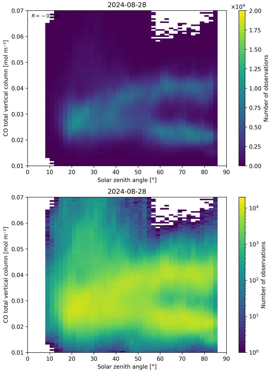
Figure 61: Scatter density plot of “Solar zenith angle” against “CO total vertical column” for 2024-08-27 to 2024-08-29.
