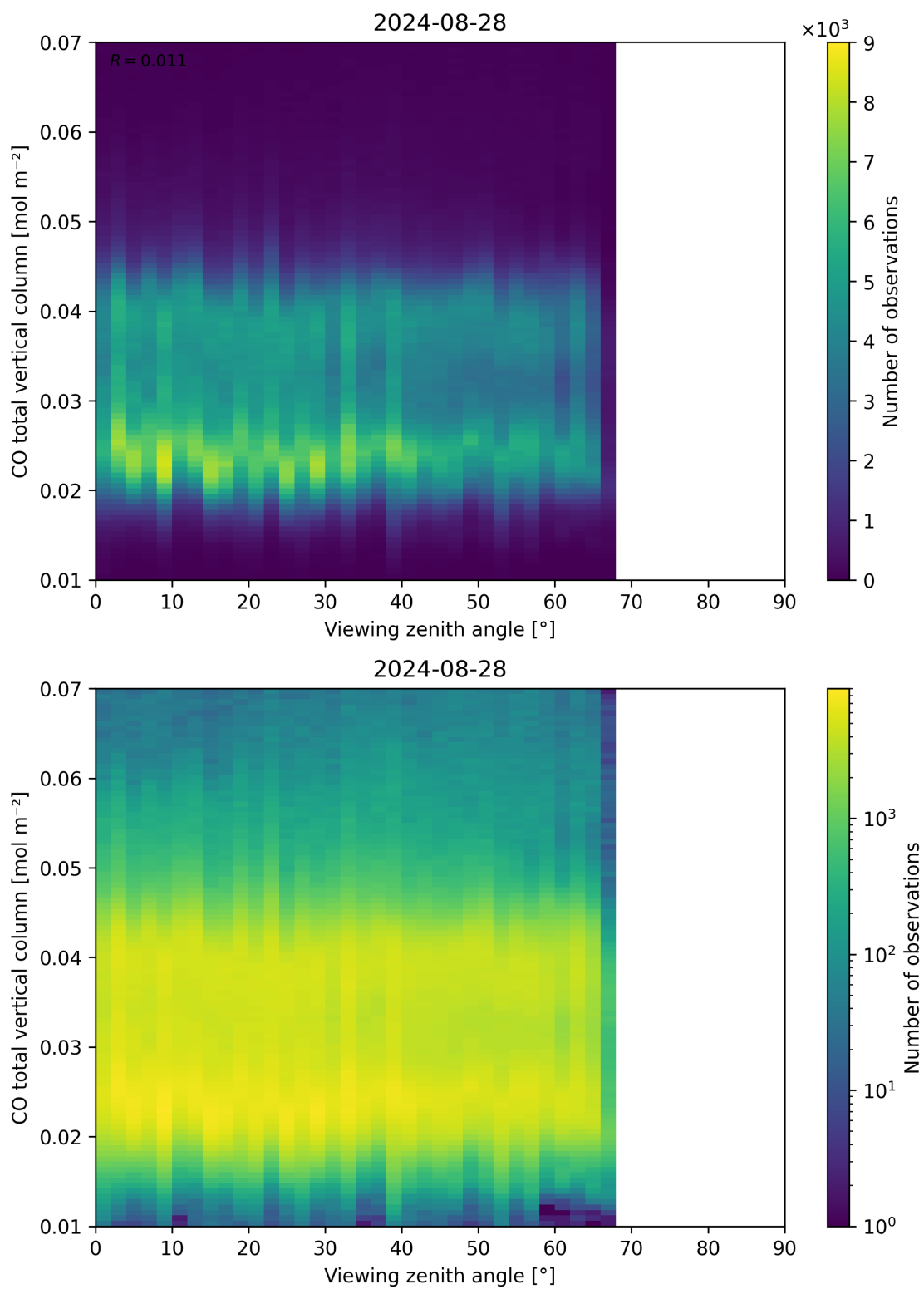
Figure 69: Scatter density plot of “Viewing zenith angle” against “CO total vertical column” for 2024-08-27 to 2024-08-29.
