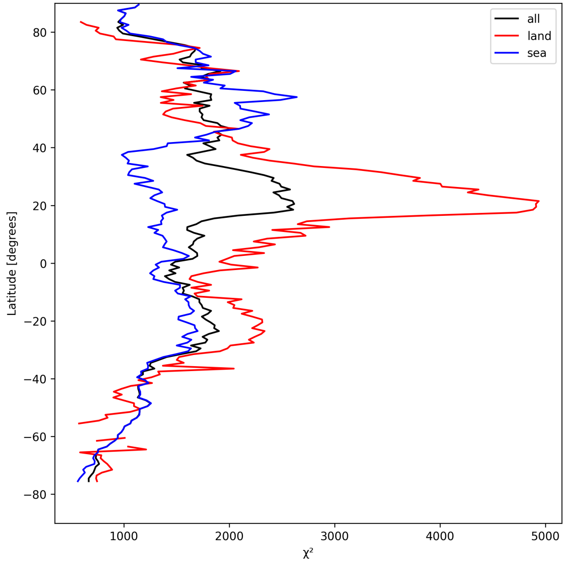
Figure 14: Zonal average of “ \chi^2 ” for 2024-08-27 to 2024-08-29.
