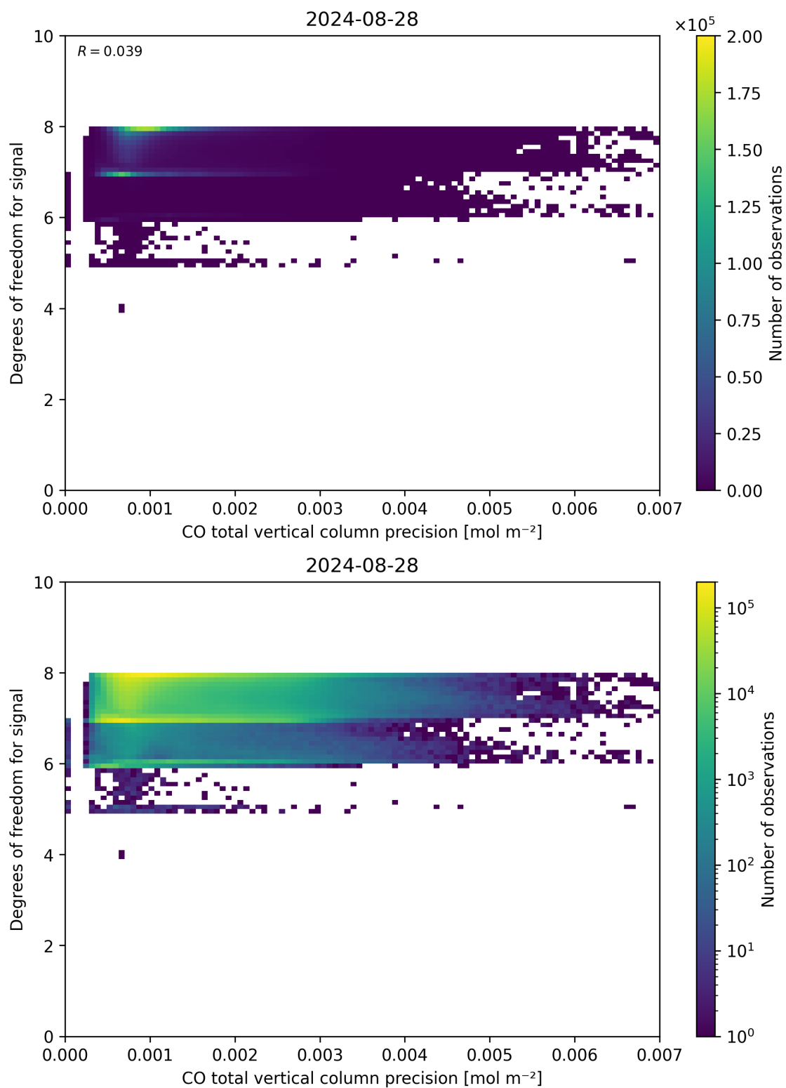
Figure 45: Scatter density plot of “CO total vertical column precision” against “Degrees of freedom for signal” for 2024-08-27 to 2024-08-29.
