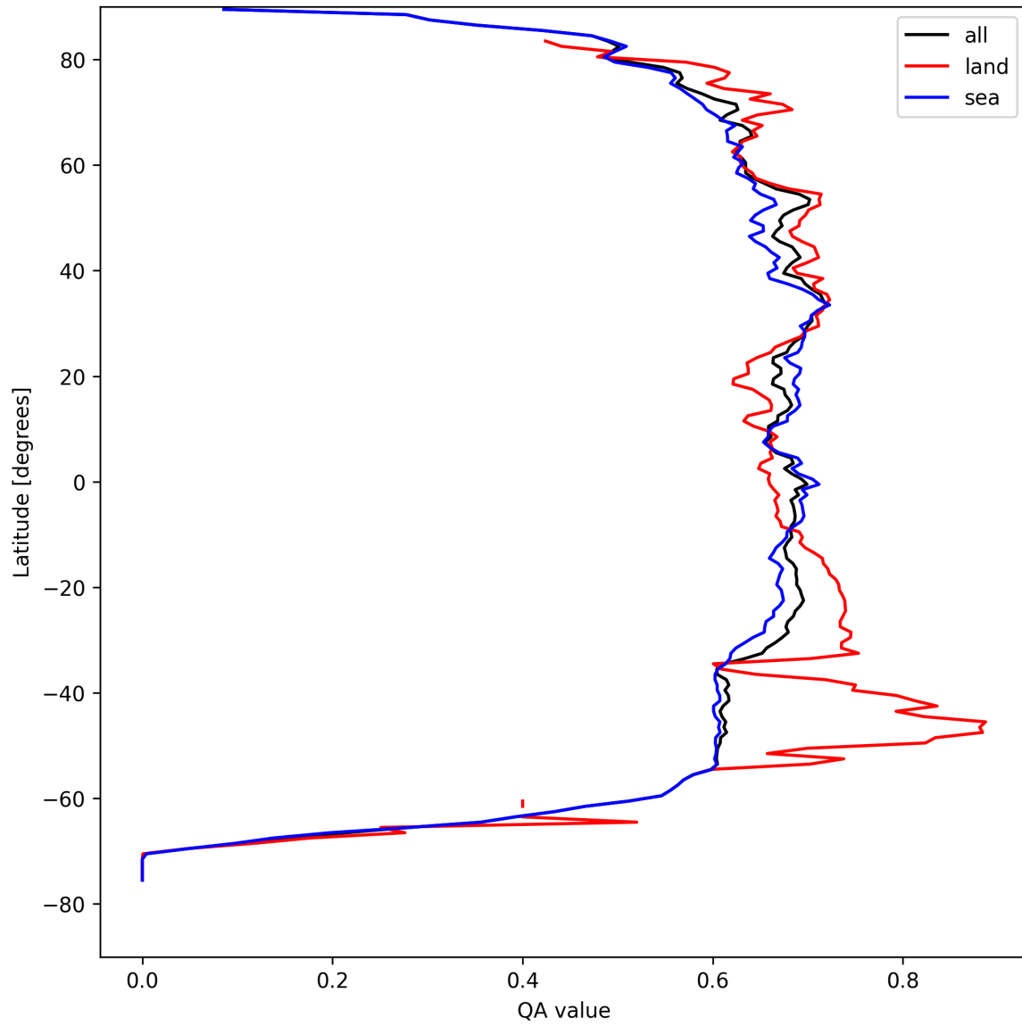
Figure 9: Zonal average of “QA value” for 2024-08-27 to 2024-08-29.
