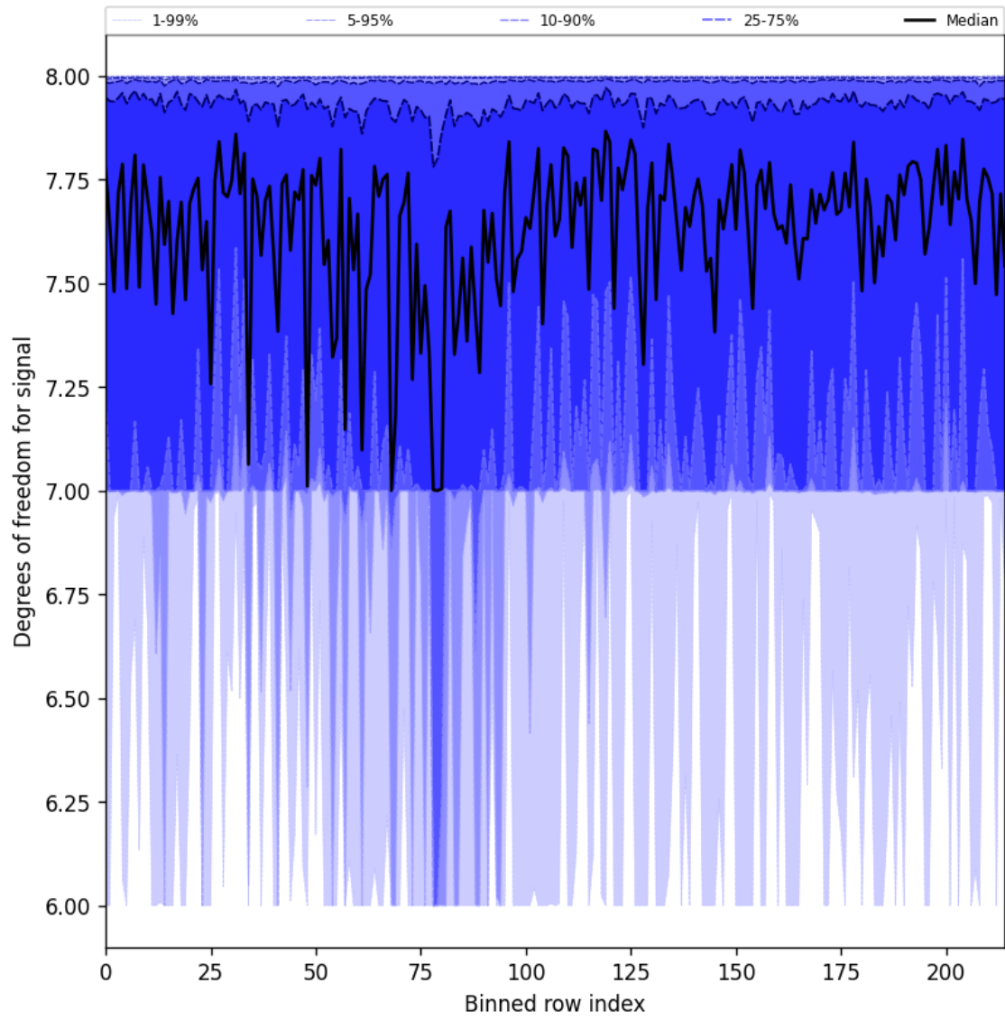
Figure 31: Along track statistics of “Degrees of freedom for signal” for 2024-08-27 to 2024-08-29
