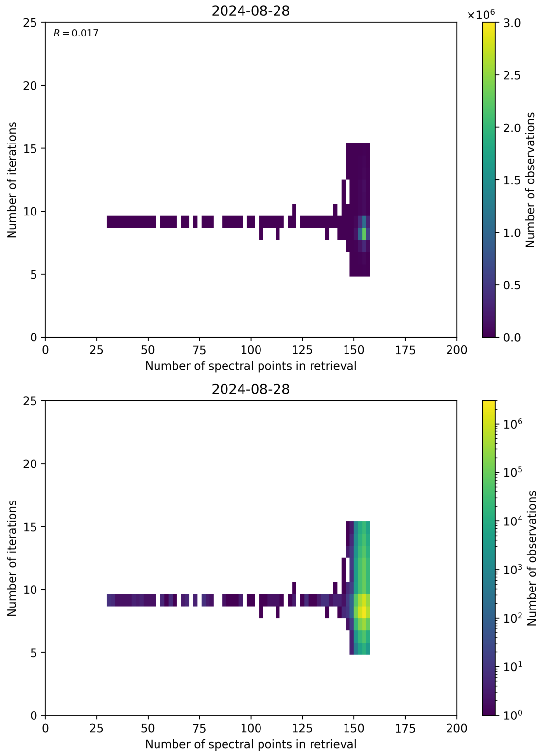
Figure 60: Scatter density plot of “Number of spectral points in retrieval” against “Number of iterations” for 2024-08-27 to 2024-08-29.
