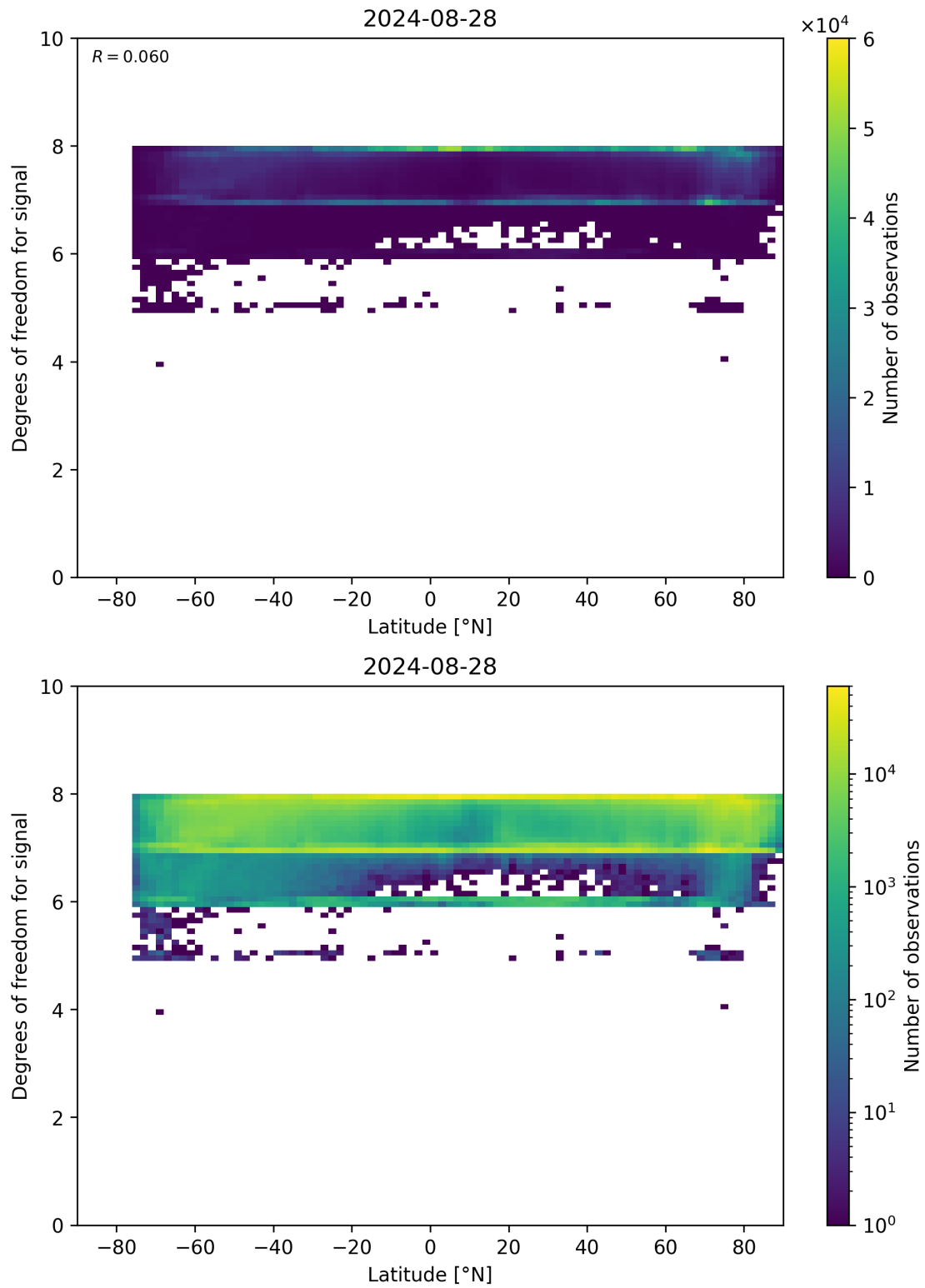
Figure 55: Scatter density plot of “Latitude” against “Degrees of freedom for signal” for 2024-08-27 to 2024-08-29.
