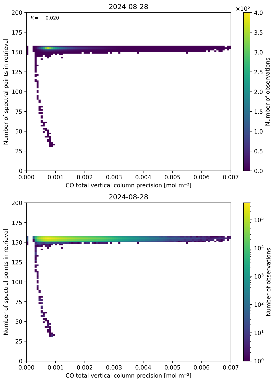
Figure 47: Scatter density plot of “CO total vertical column precision” against “Number of spectral points in retrieval” for 2024-08-27 to 2024-08-29.
