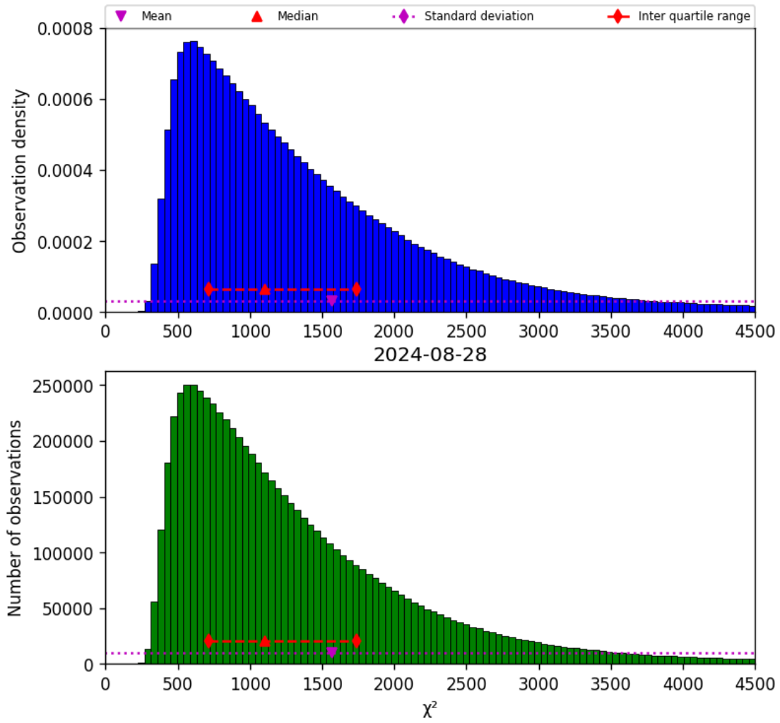
Figure 22: Histogram of “ \chi^2 ” for 2024-08-27 to 2024-08-29
