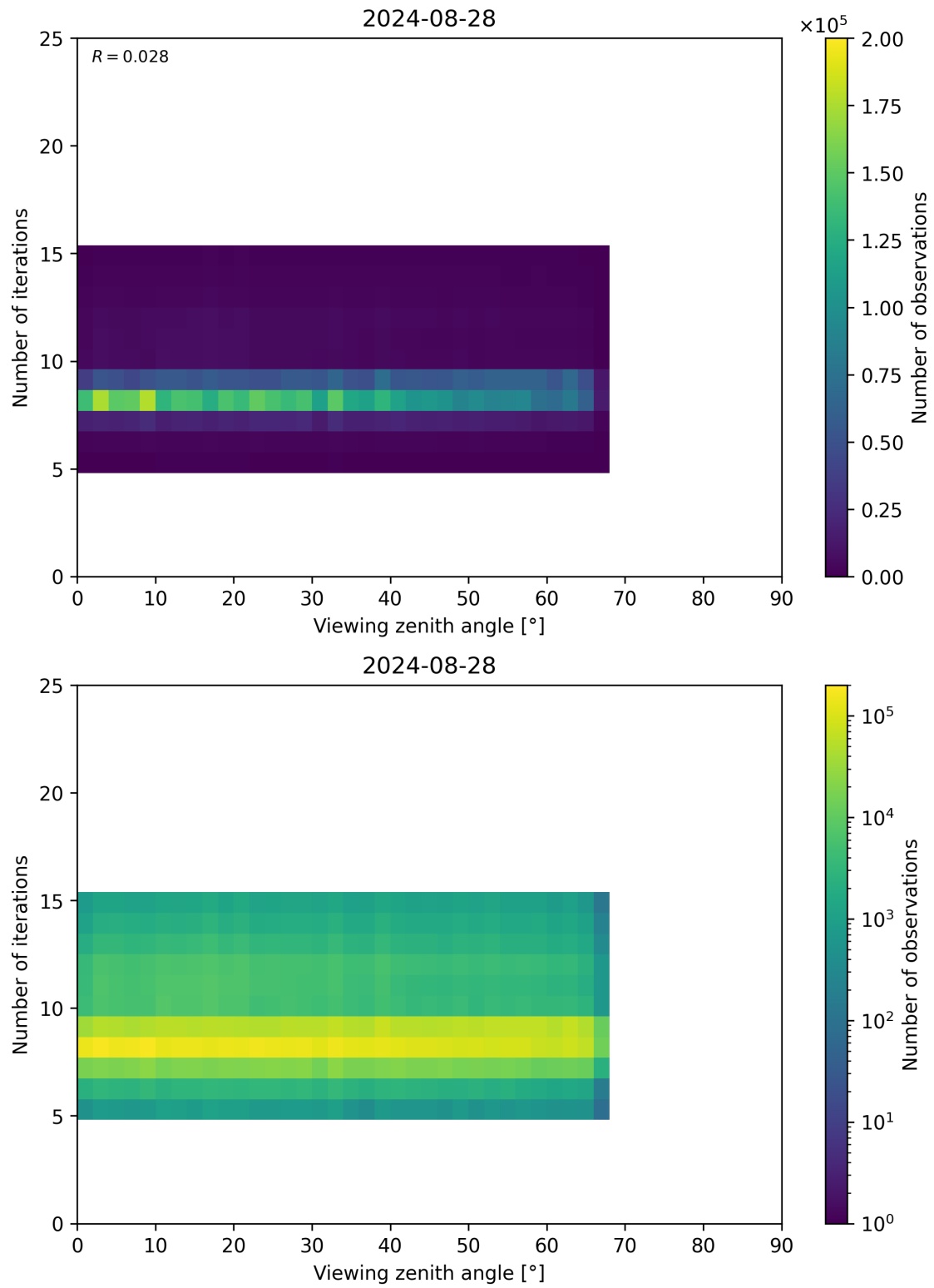
Figure 75: Scatter density plot of “Viewing zenith angle” against “Number of iterations” for 2024-08-27 to 2024-08-29.
