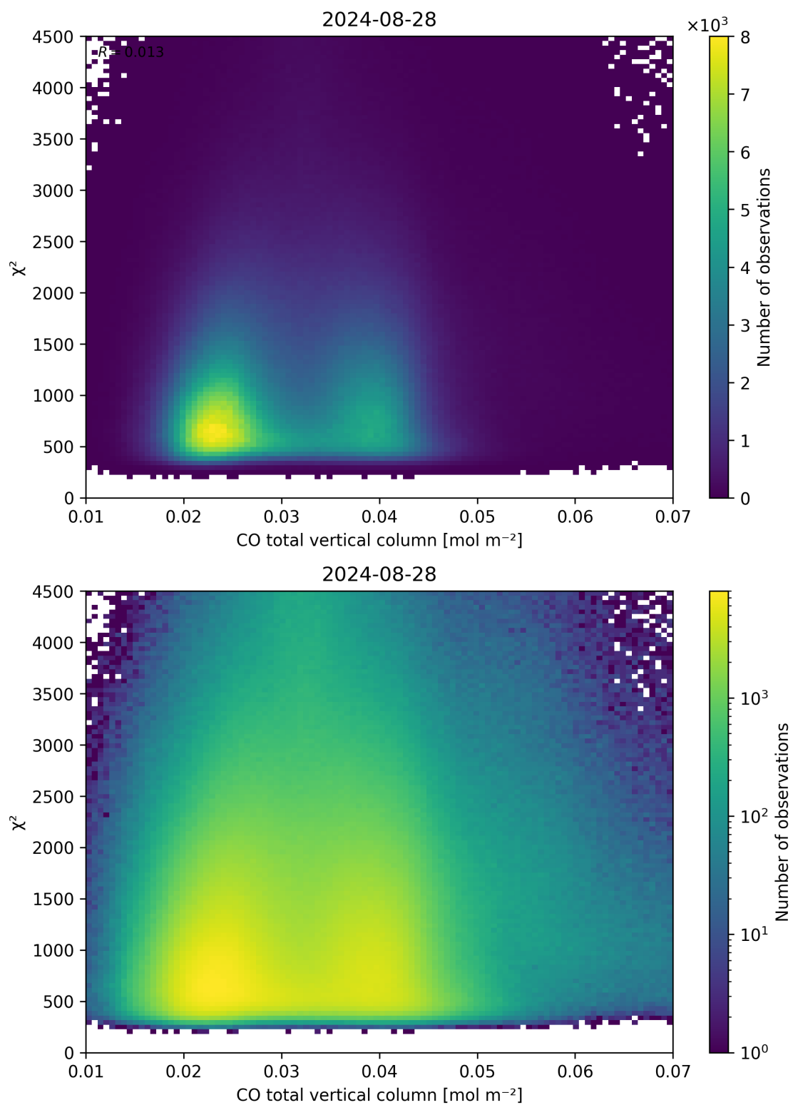
Figure 35: Scatter density plot of “CO total vertical column” against “ \chi^2 ” for 2024-08-27 to 2024-08-29.
