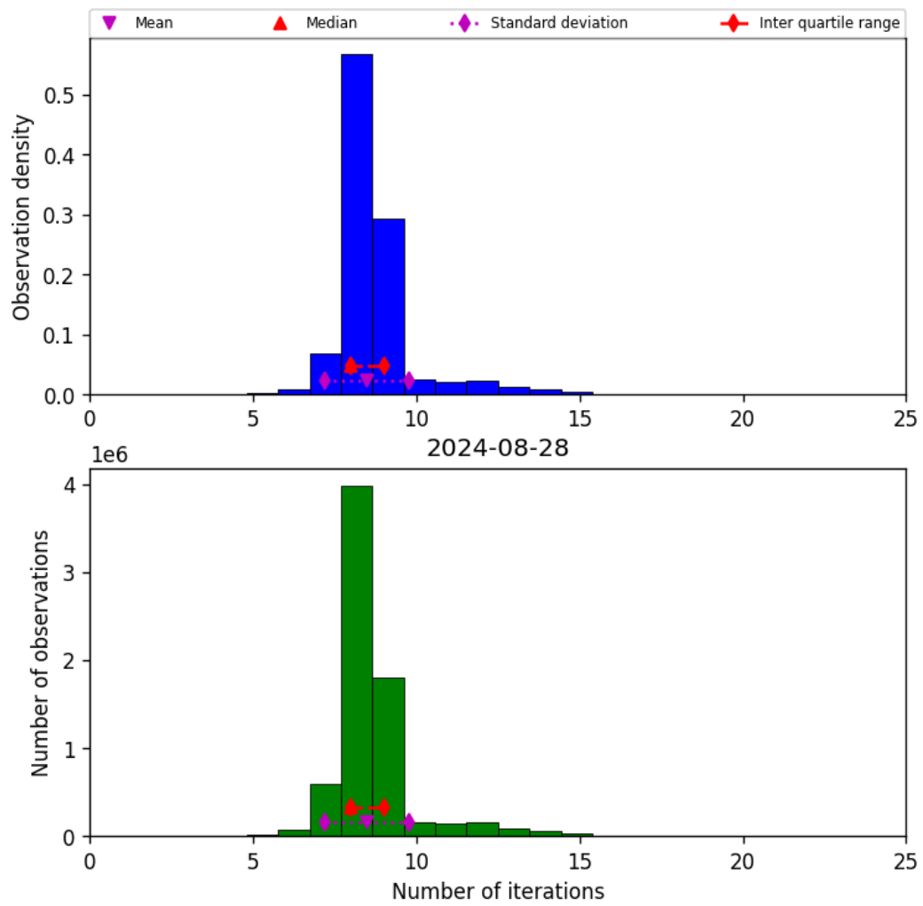
Figure 24: Histogram of “Number of iterations” for 2024-08-27 to 2024-08-29
