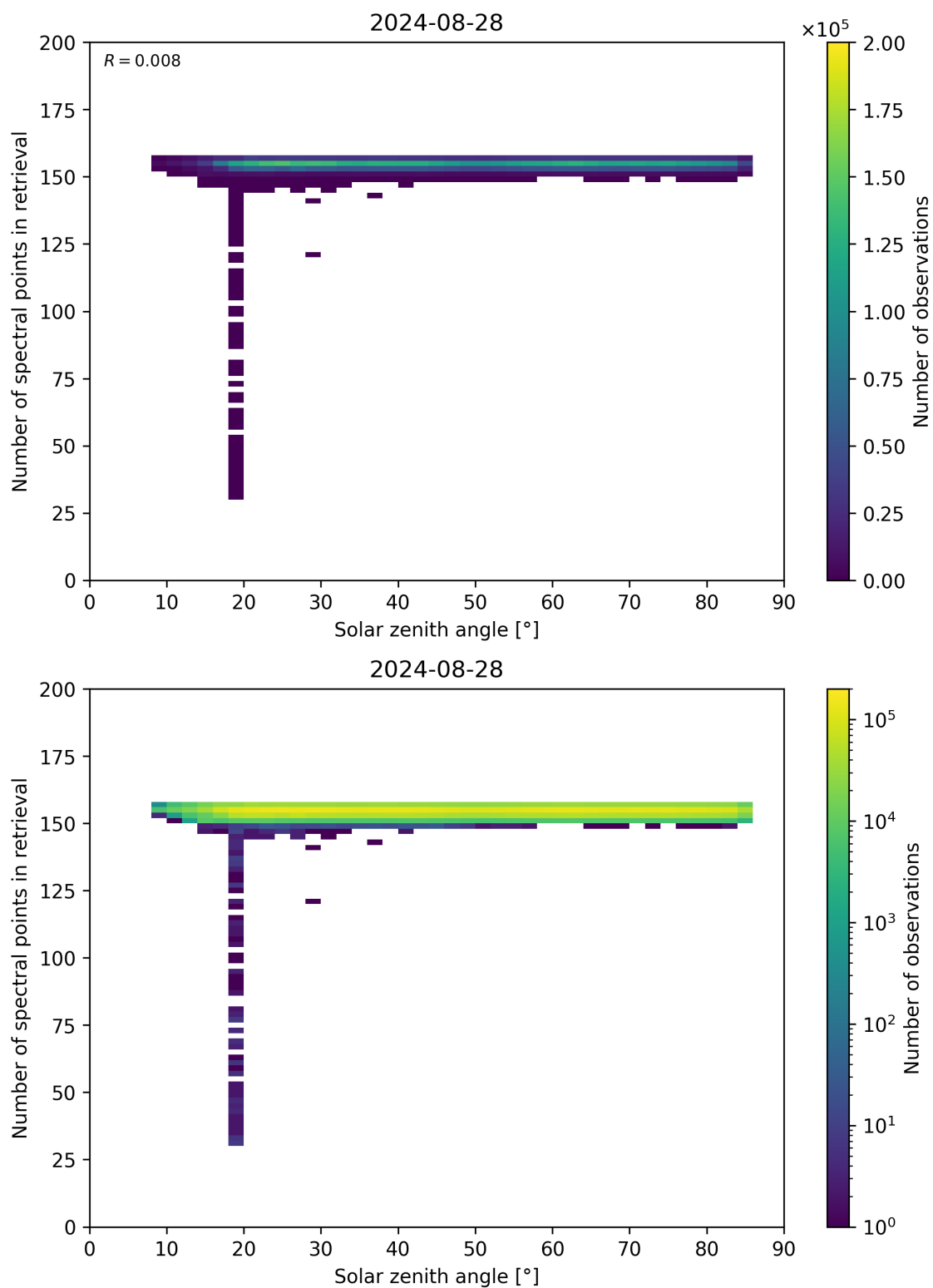
Figure 68: Scatter density plot of “Solar zenith angle” against “Number of spectral points in retrieval” for 2024-08-27 to 2024-08-29.
