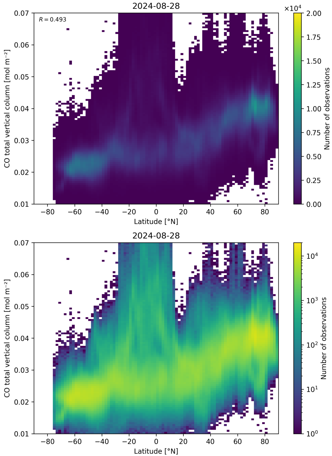
Figure 51: Scatter density plot of “Latitude” against “CO total vertical column” for 2024-08-27 to 2024-08-29.
