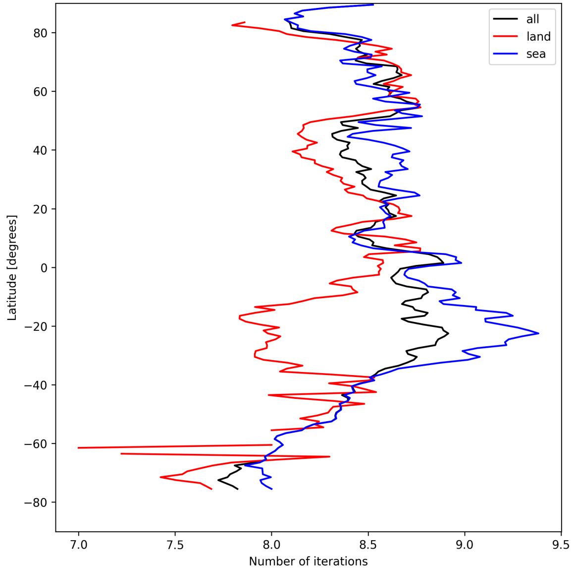
Figure 16: Zonal average of “Number of iterations” for 2024-08-27 to 2024-08-29.
