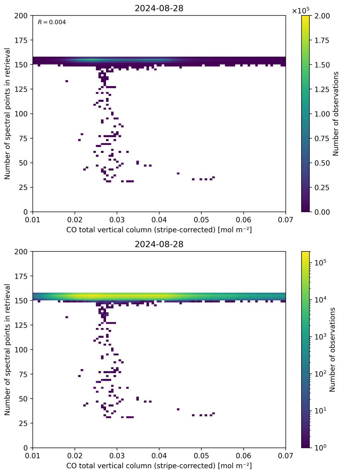
Figure 40: Scatter density plot of “CO total vertical column (stripe-corrected)” against “Number of spectral points in retrieval” for 2024-08-27 to 2024-08-29.
