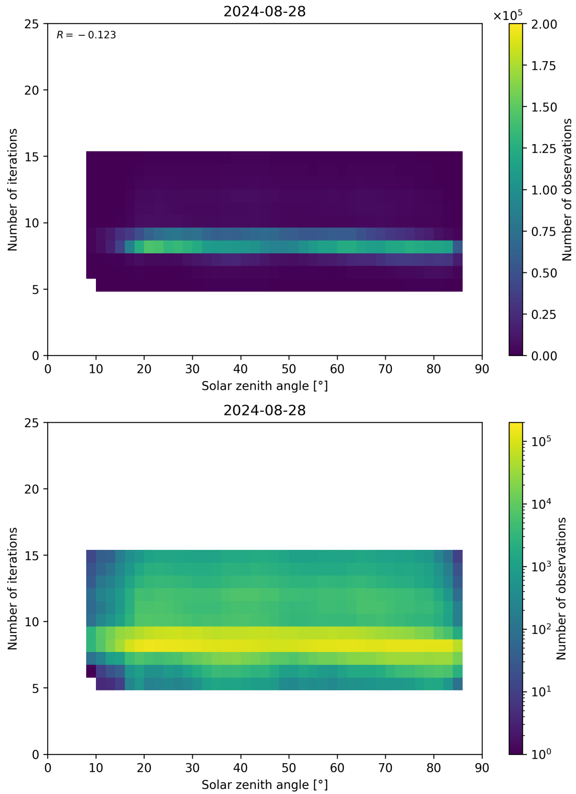
Figure 67: Scatter density plot of “Solar zenith angle” against “Number of iterations” for 2024-08-27 to 2024-08-29.
