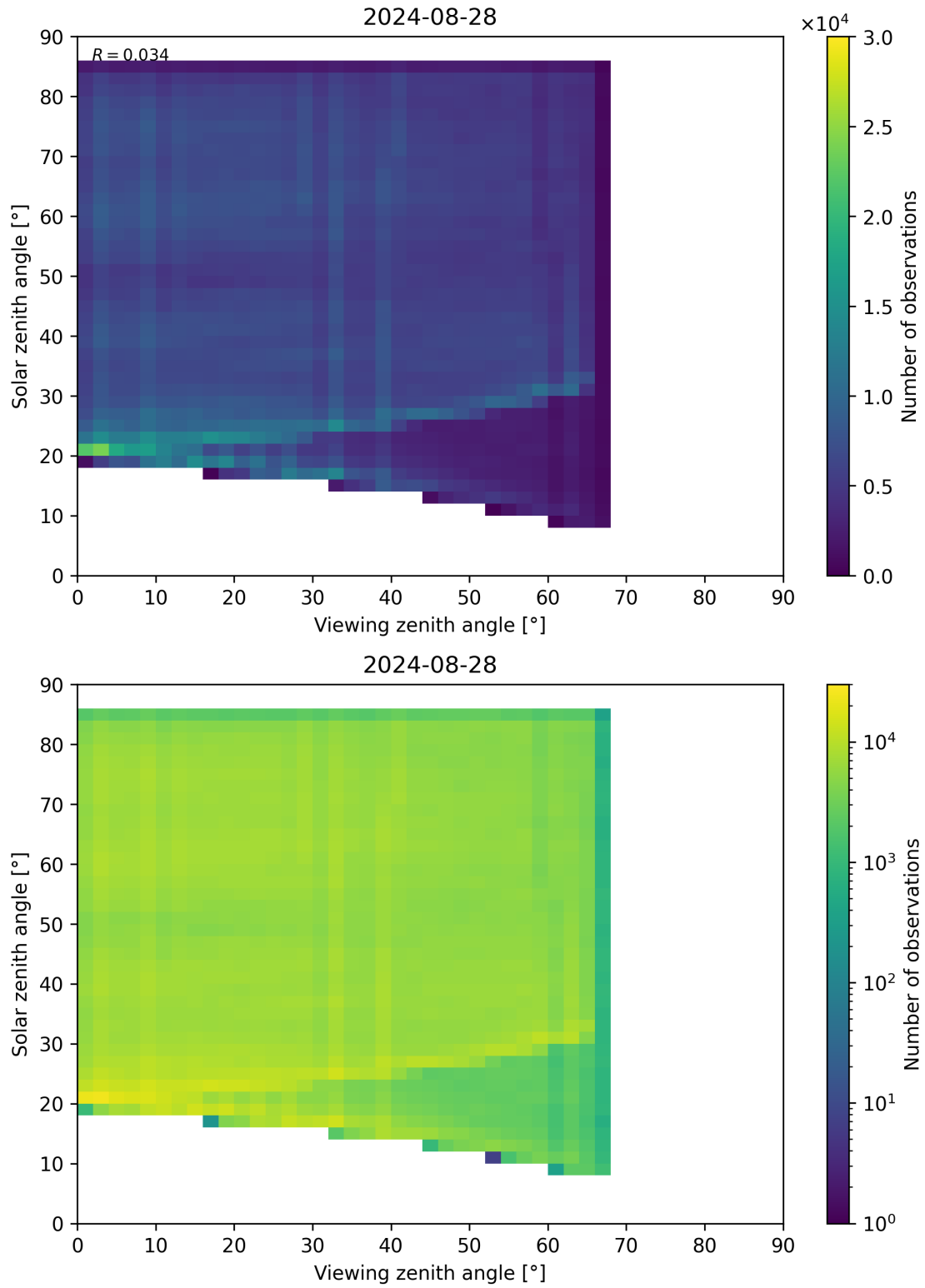
Figure 77: Scatter density plot of “Viewing zenith angle” against “Solar zenith angle” for 2024-08-27 to 2024-08-29.
