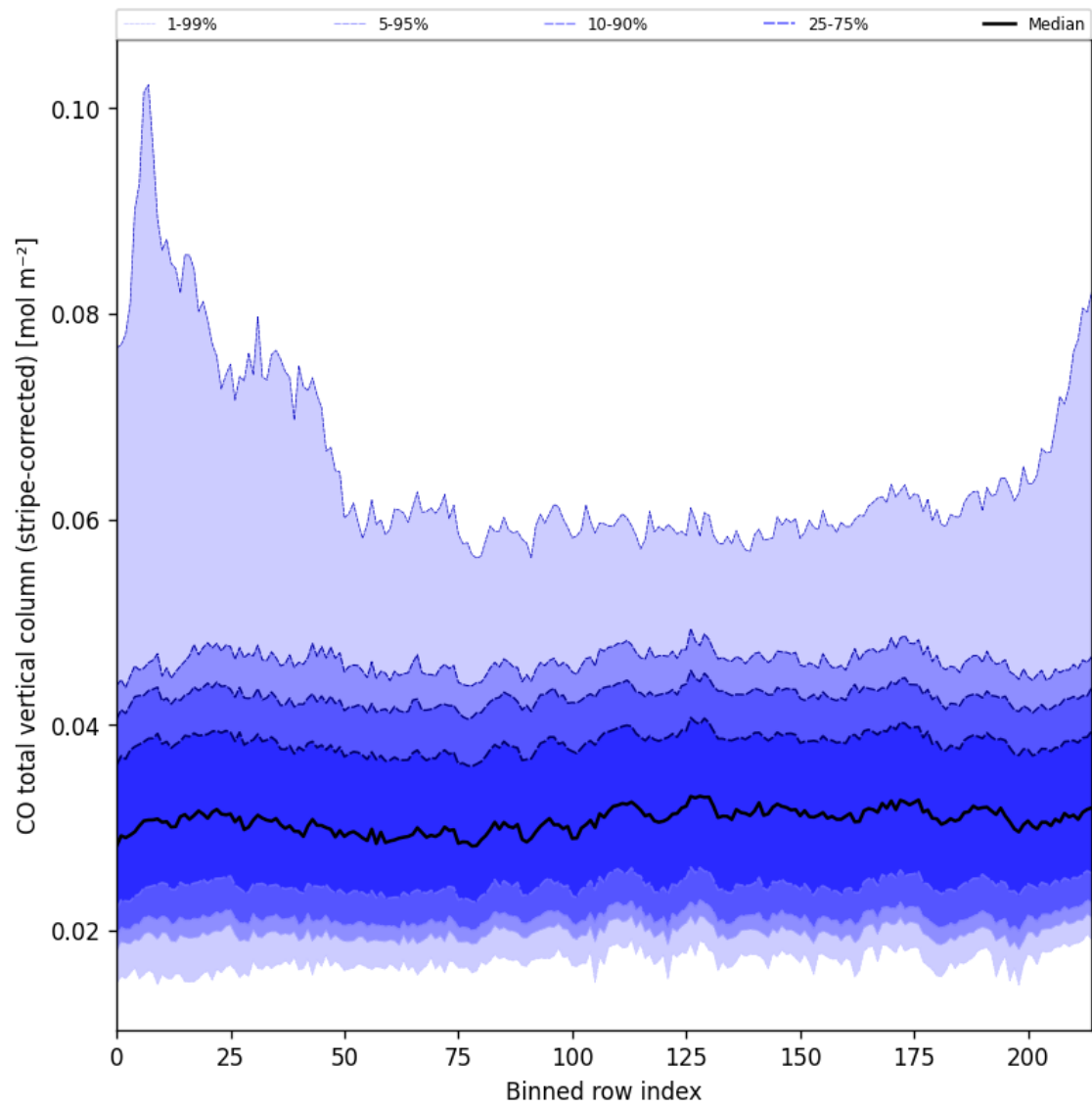
Figure 27: Along track statistics of “CO total vertical column (stripe-corrected)” for 2024-08-27 to 2024-08-29
