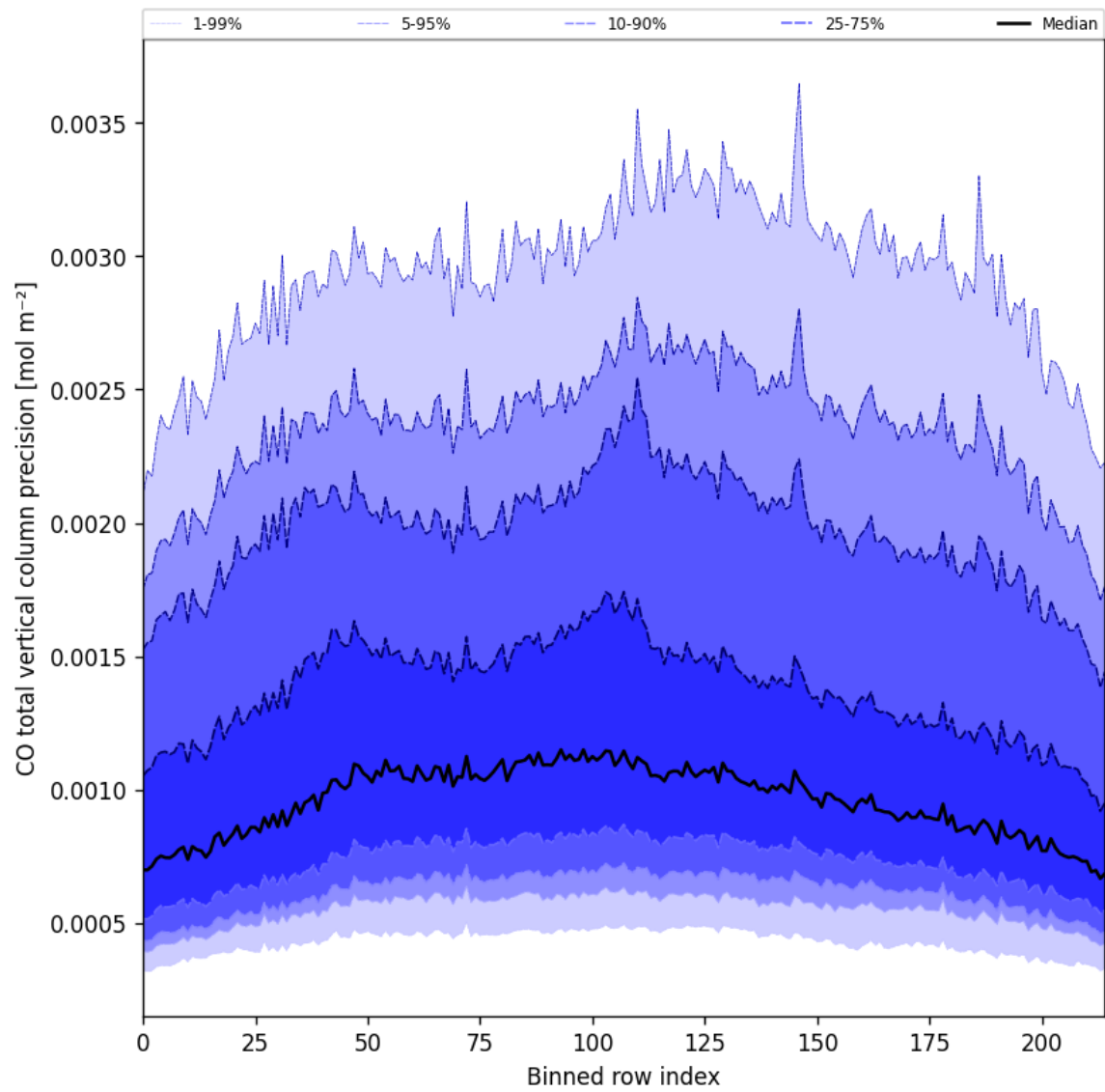
Figure 28: Along track statistics of "CO total vertical column precision" for 2024-08-27 to 2024-08-29
