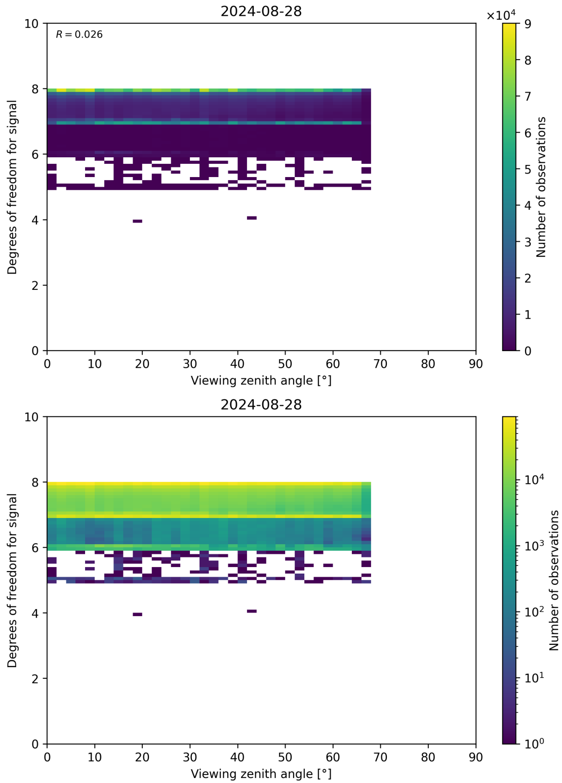
Figure 73: Scatter density plot of “Viewing zenith angle” against “Degrees of freedom for signal” for 2024-08-27 to 2024-08-29.
