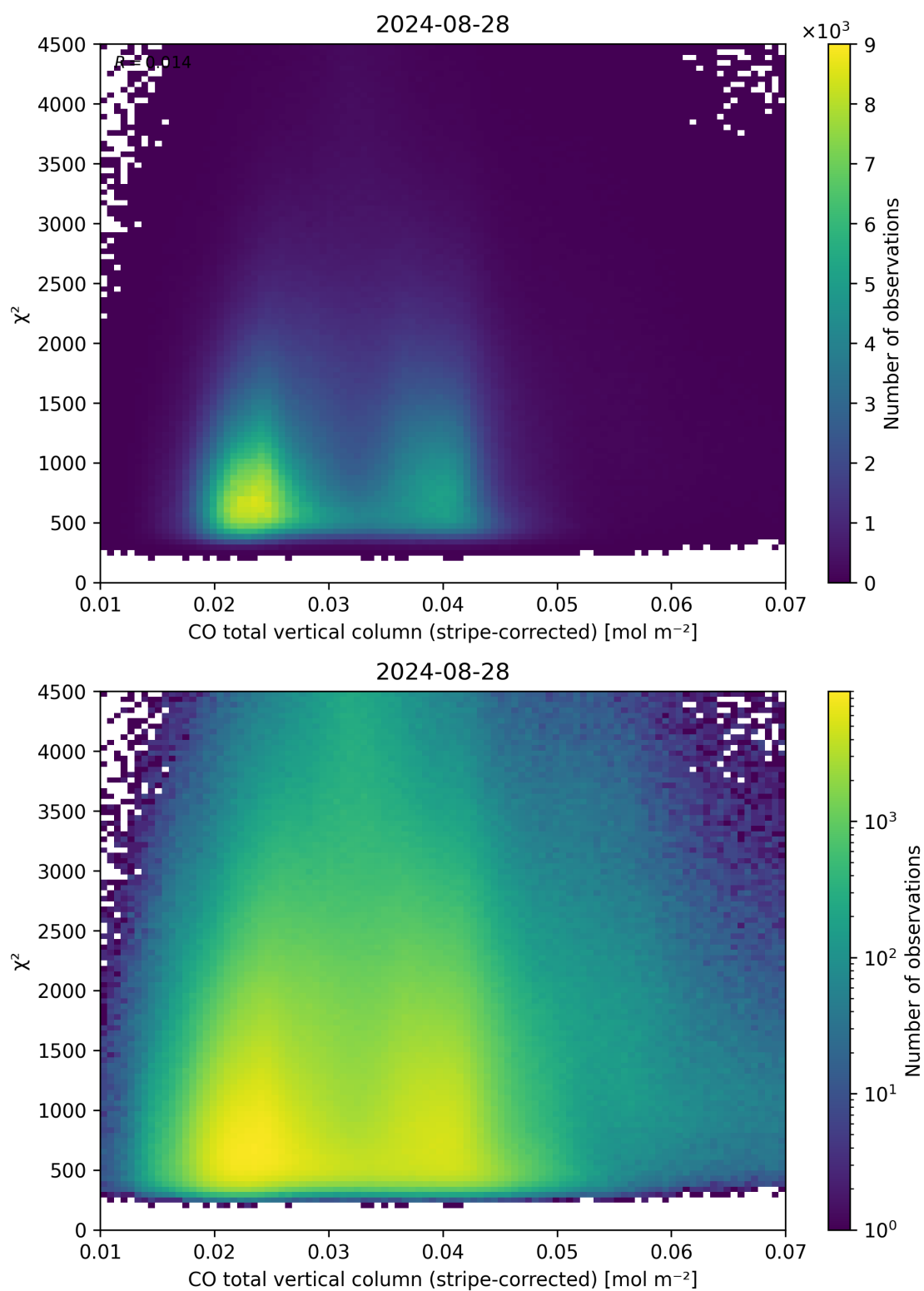
Figure 37: Scatter density plot of “CO total vertical column (stripe-corrected)” against “ \chi^2 ” for 2024-08-27 to 2024-08-29.
