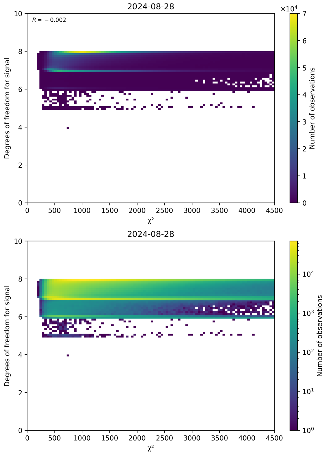
Figure 48: Scatter density plot of “ \chi^2 ” against “Degrees of freedom for signal” for 2024-08-27 to 2024-08-29.
