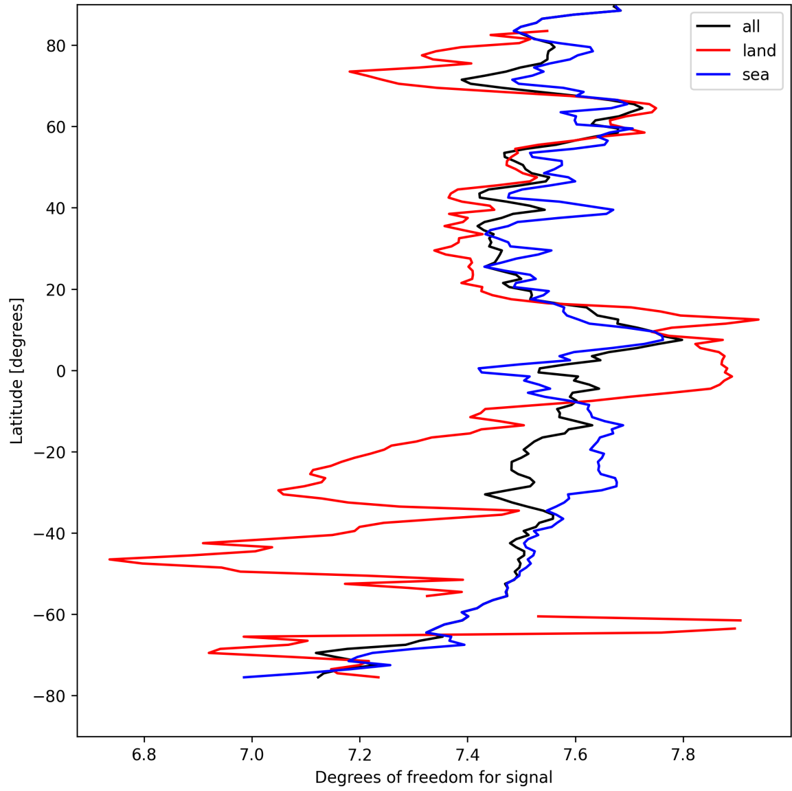
Figure 15: Zonal average of “Degrees of freedom for signal” for 2024-08-27 to 2024-08-29.
