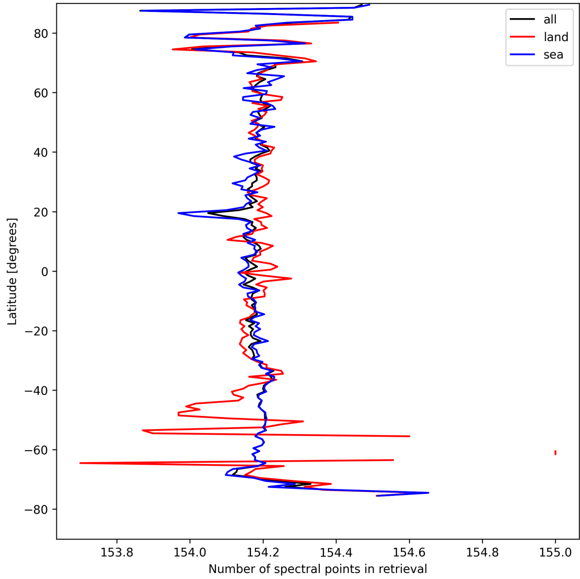
Figure 13: Zonal average of “Number of spectral points in retrieval” for 2024-08-27 to 2024-08-29.
