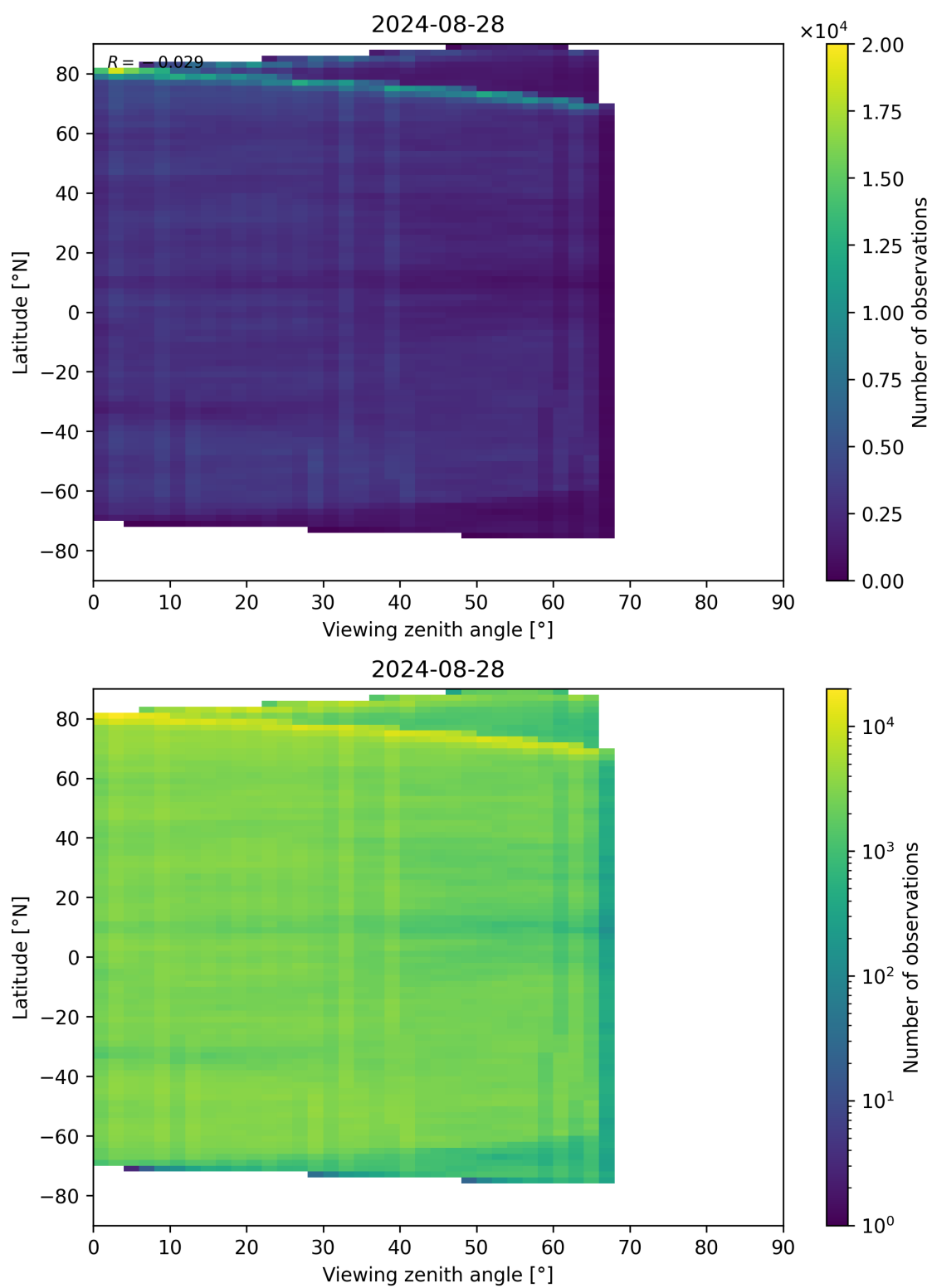
Figure 74: Scatter density plot of “Viewing zenith angle” against “Latitude” for 2024-08-27 to 2024-08-29.
