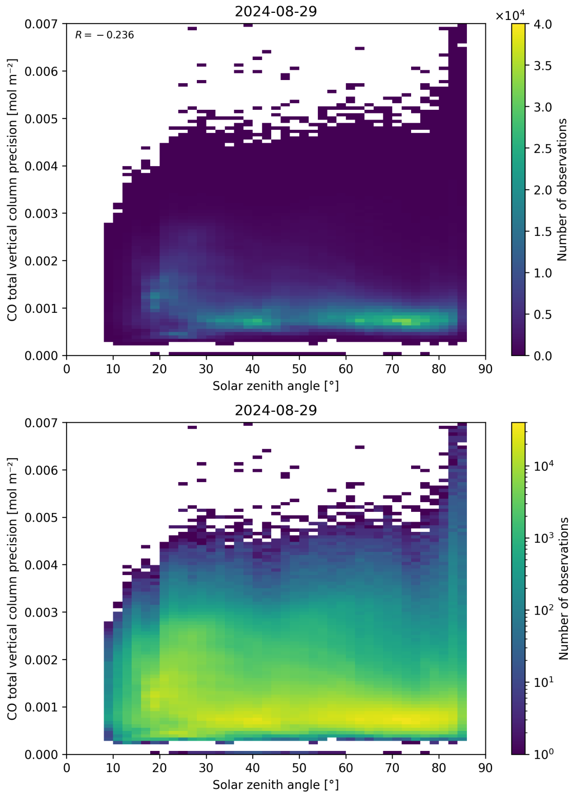
Figure 63: Scatter density plot of “Solar zenith angle” against “CO total vertical column precision” for 2024-08-28 to 2024-08-30.
