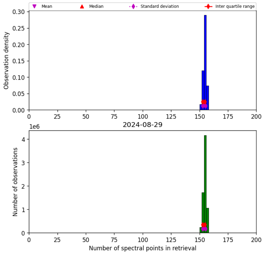
Figure 21: Histogram of “Number of spectral points in retrieval” for 2024-08-28 to 2024-08-30
