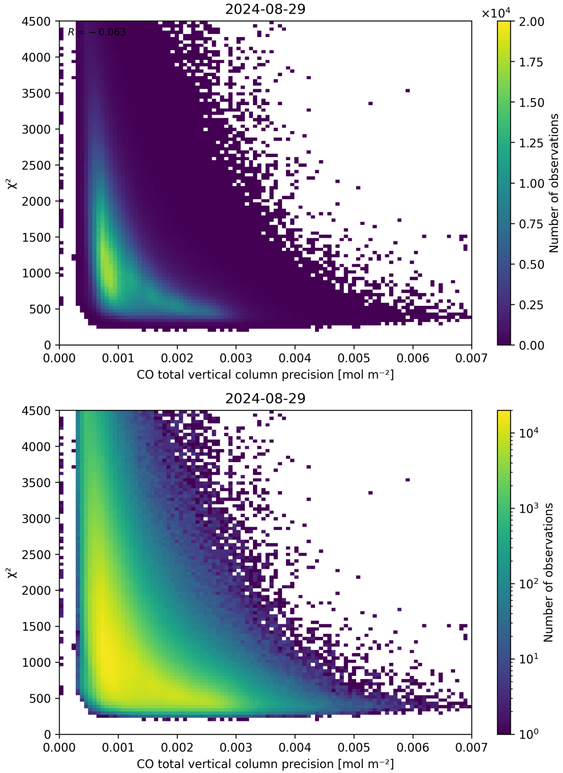
Figure 44: Scatter density plot of “CO total vertical column precision” against “ \chi^2 ” for 2024-08-28 to 2024-08-30.
