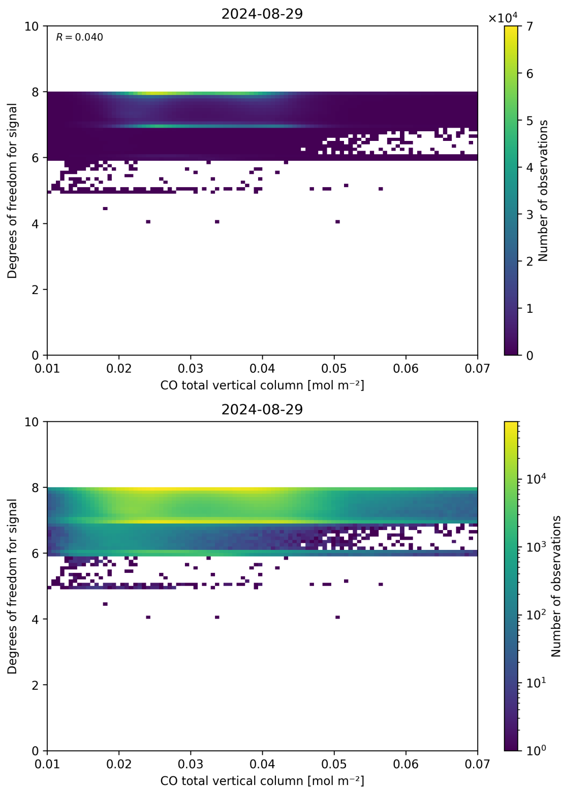
Figure 41: Scatter density plot of “CO total vertical column” against “Degrees of freedom for signal” for 2024-08-28 to 2024-08-30.
