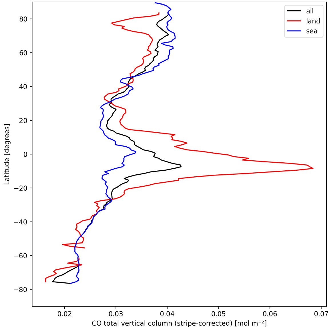
Figure 11: Zonal average of “CO total vertical column (stripe-corrected)” for 2024-08-28 to 2024-08-30.
