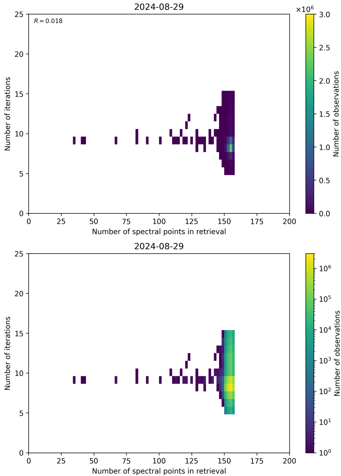
Figure 60: Scatter density plot of “Number of spectral points in retrieval” against “Number of iterations” for 2024-08-28 to 2024-08-30.
