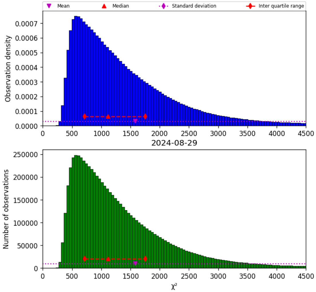
Figure 22: Histogram of “ \chi^2 ” for 2024-08-28 to 2024-08-30
