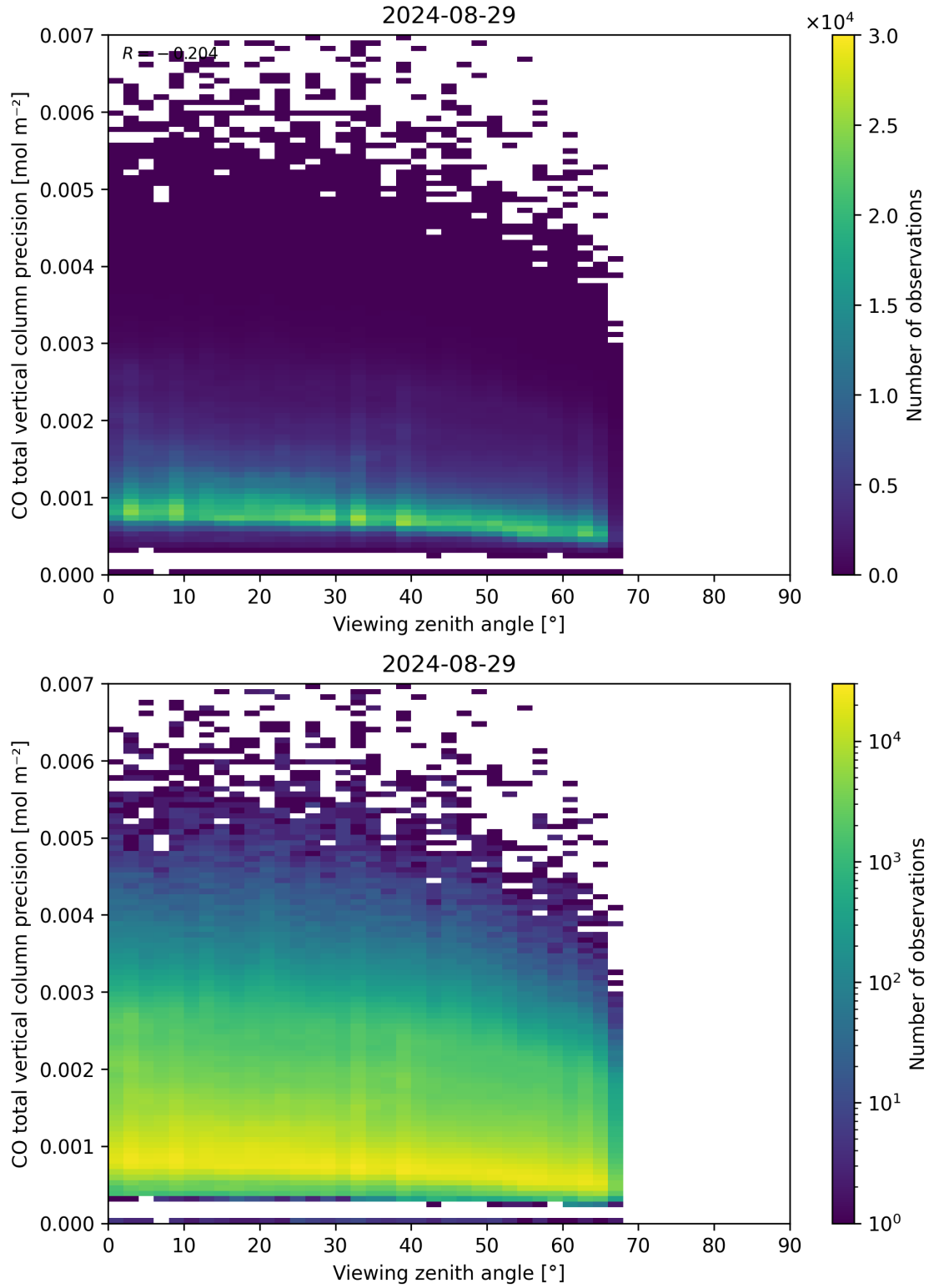
Figure 71: Scatter density plot of “Viewing zenith angle” against “CO total vertical column precision” for 2024-08-28 to 2024-08-30.
