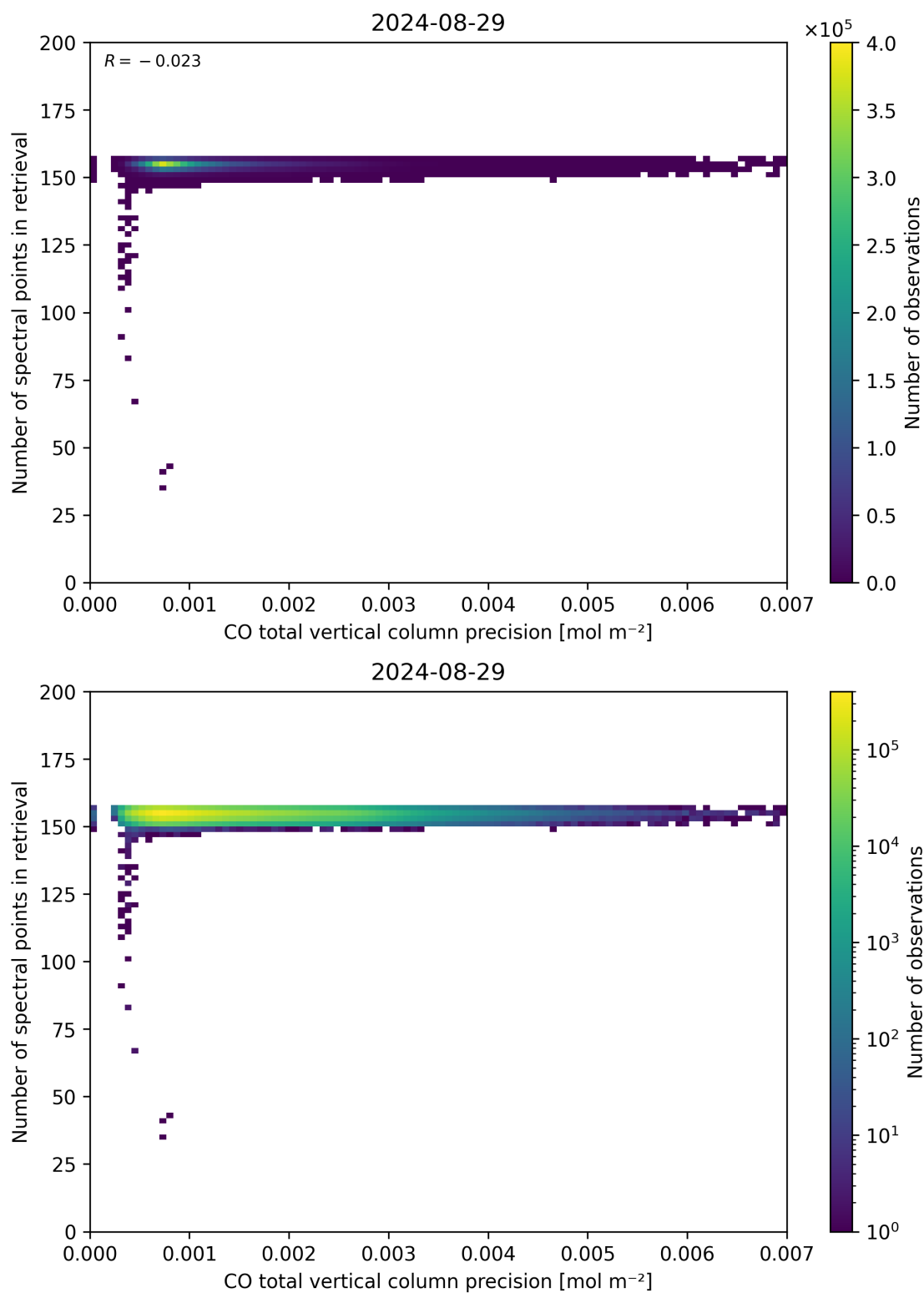
Figure 47: Scatter density plot of “CO total vertical column precision” against “Number of spectral points in retrieval” for 2024-08-28 to 2024-08-30.
