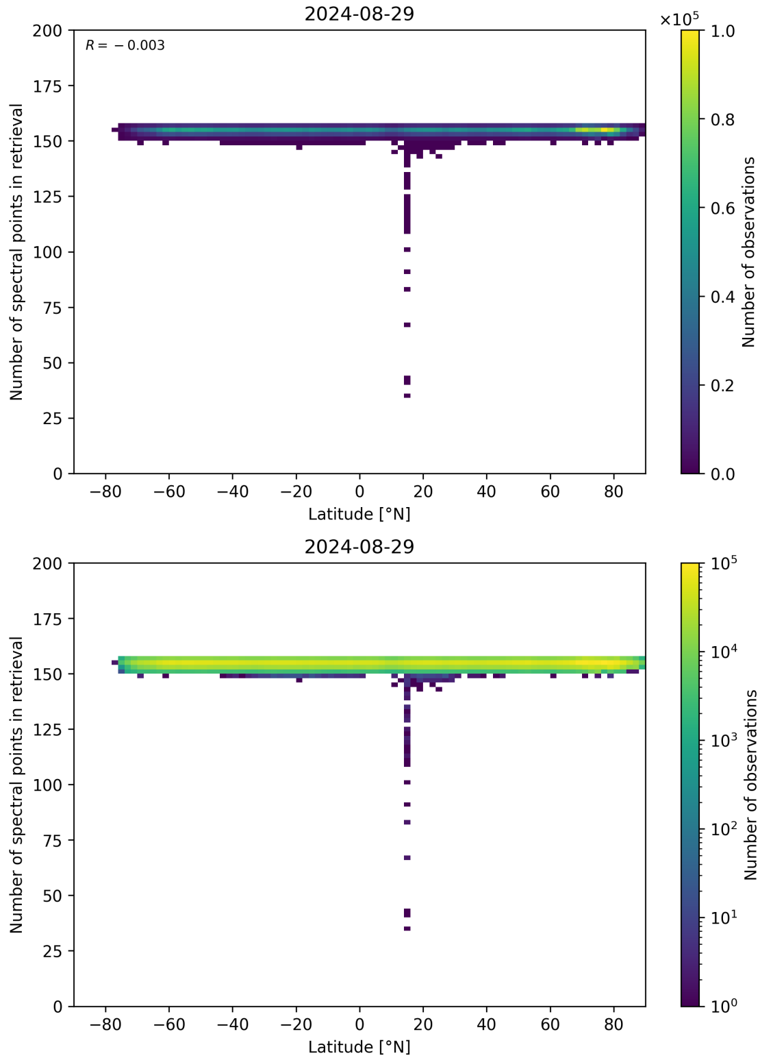
Figure 57: Scatter density plot of “Latitude” against “Number of spectral points in retrieval” for 2024-08-28 to 2024-08-30.
