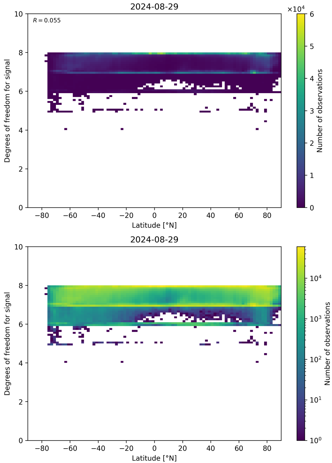
Figure 55: Scatter density plot of “Latitude” against “Degrees of freedom for signal” for 2024-08-28 to 2024-08-30.
