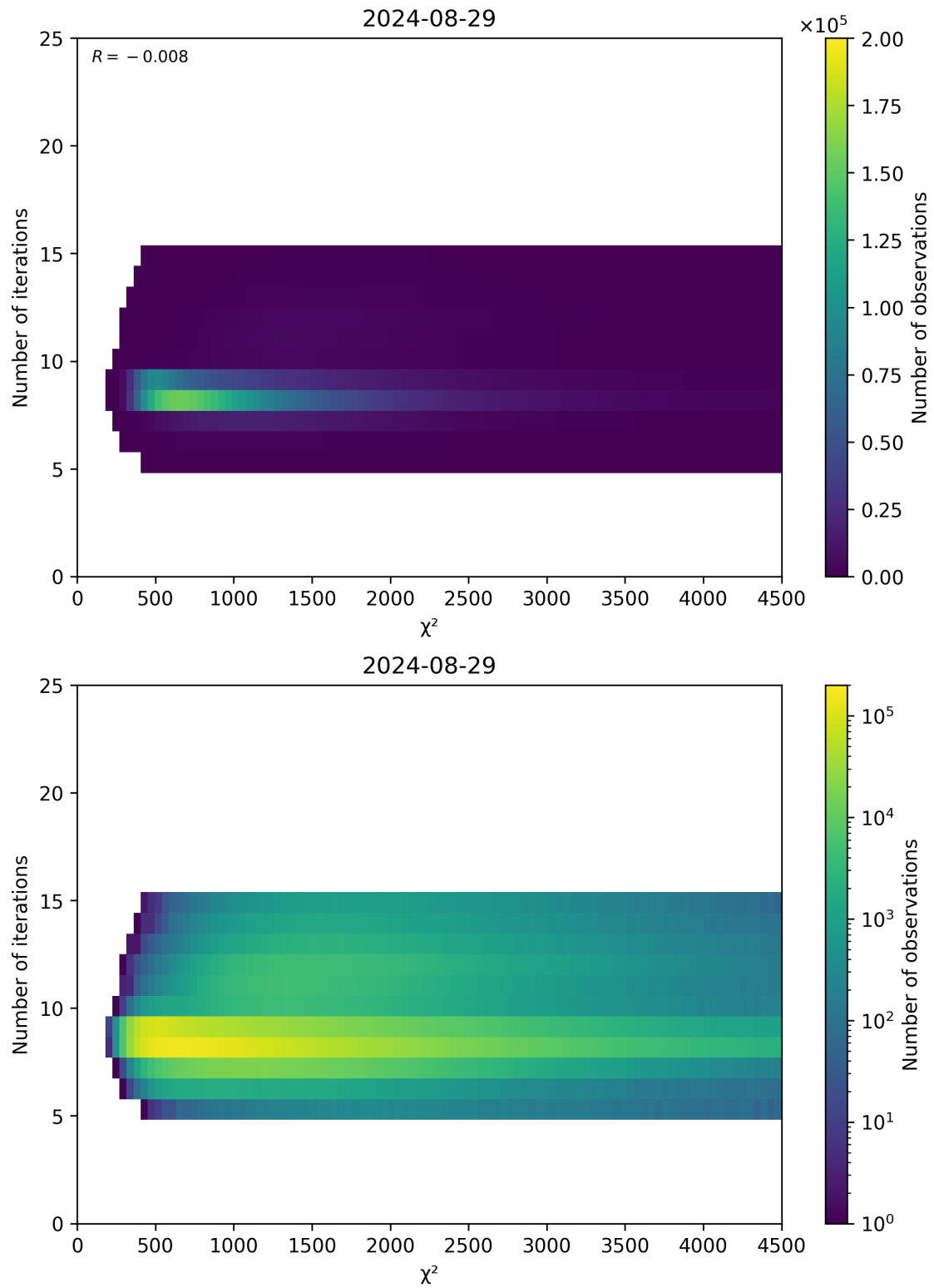
Figure 49: Scatter density plot of “ \chi^2 ” against “Number of iterations” for 2024-08-28 to 2024-08-30.
