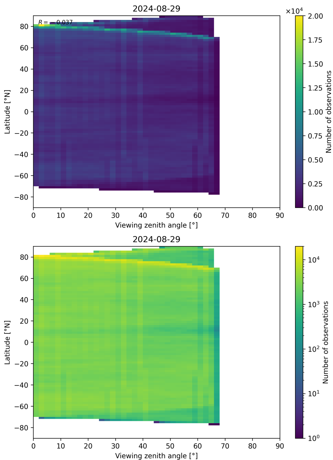
Figure 74: Scatter density plot of “Viewing zenith angle” against “Latitude” for 2024-08-28 to 2024-08-30.
