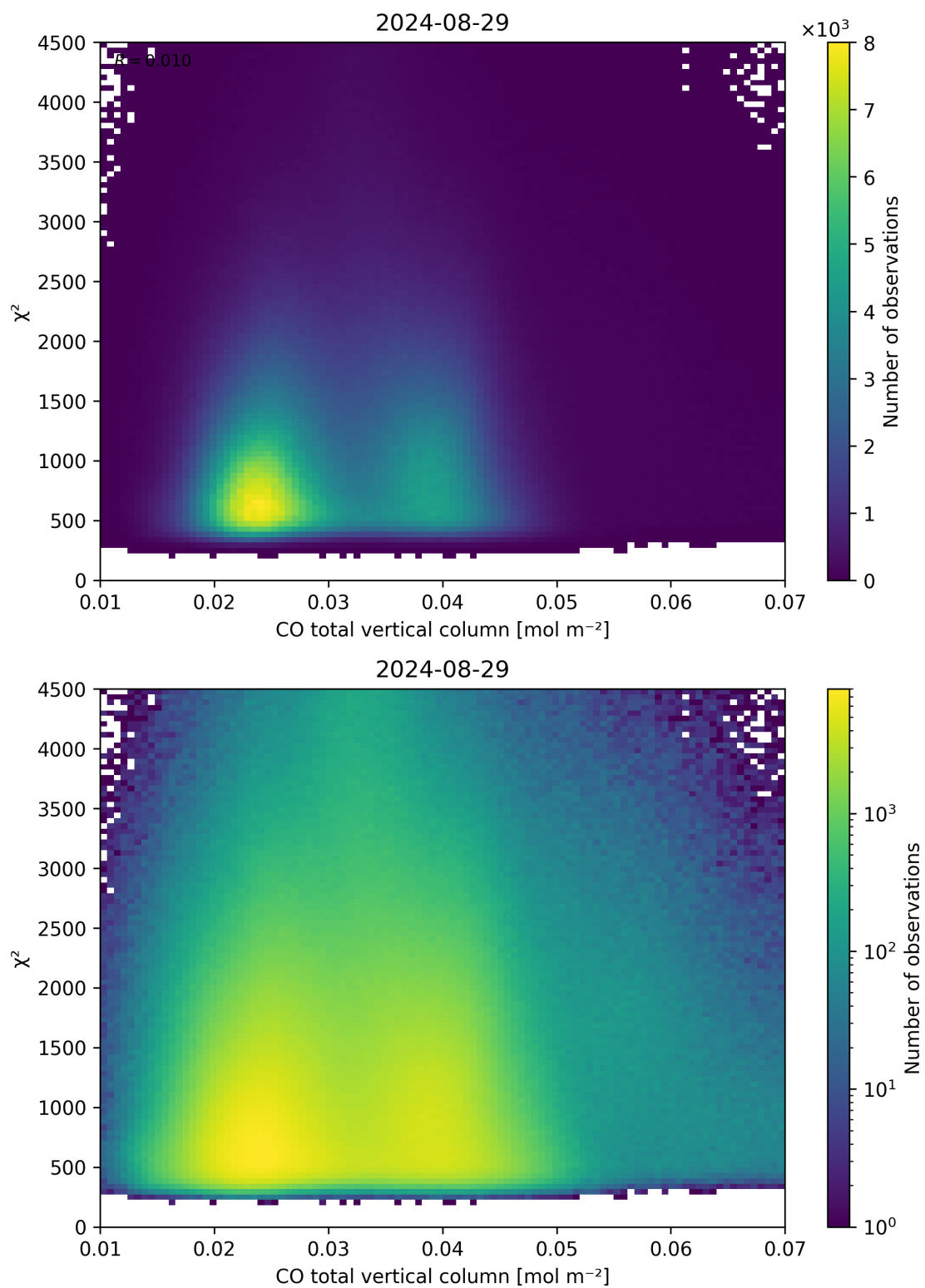
Figure 35: Scatter density plot of “CO total vertical column” against “ \chi^2 ” for 2024-08-28 to 2024-08-30.
