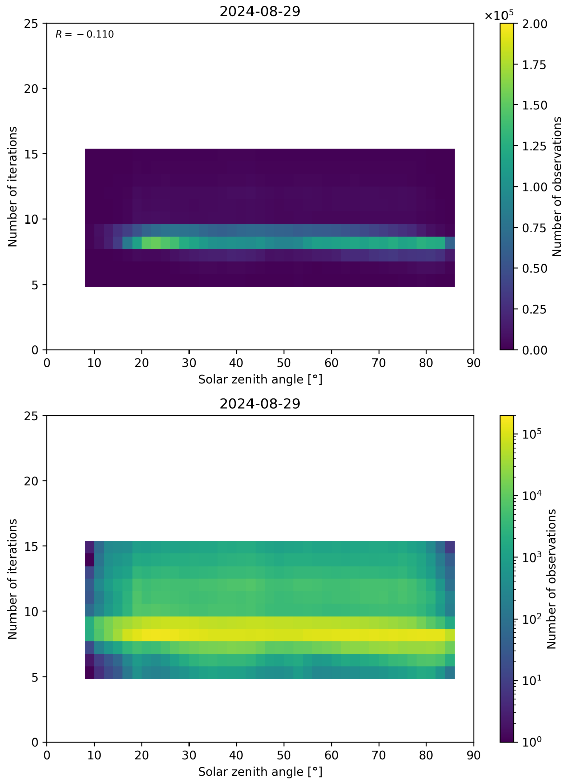
Figure 67: Scatter density plot of “Solar zenith angle” against “Number of iterations” for 2024-08-28 to 2024-08-30.
