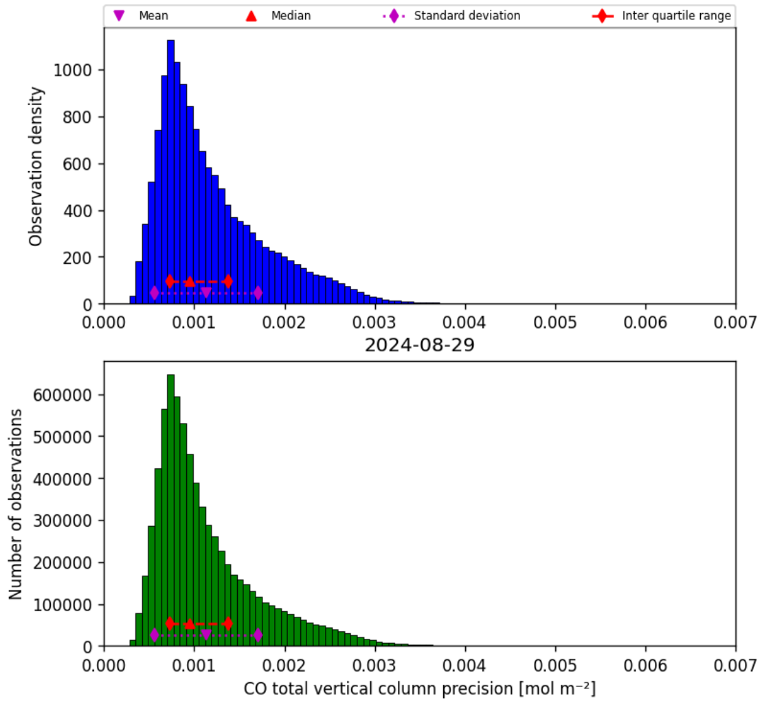
Figure 20: Histogram of “CO total vertical column precision” for 2024-08-28 to 2024-08-30
