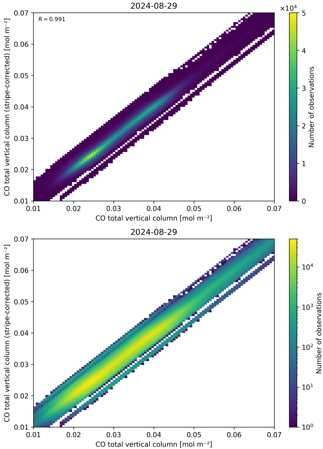
Figure 33: Scatter density plot of “CO total vertical column” against “CO total vertical column (stripe-corrected)” for 2024-08-28 to 2024-08-30.
