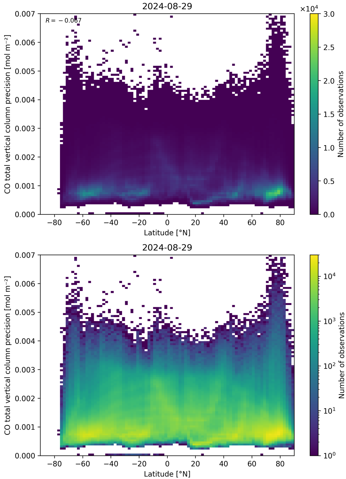
Figure 53: Scatter density plot of “Latitude” against “CO total vertical column precision” for 2024-08-28 to 2024-08-30.
