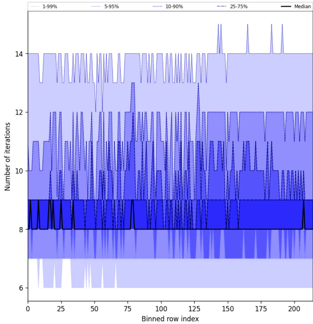
Figure 32: Along track statistics of “Number of iterations” for 2024-08-28 to 2024-08-30
