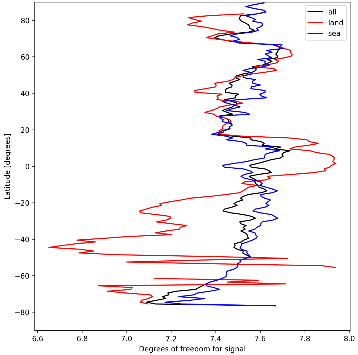
Figure 15: Zonal average of “Degrees of freedom for signal” for 2024-08-28 to 2024-08-30.
