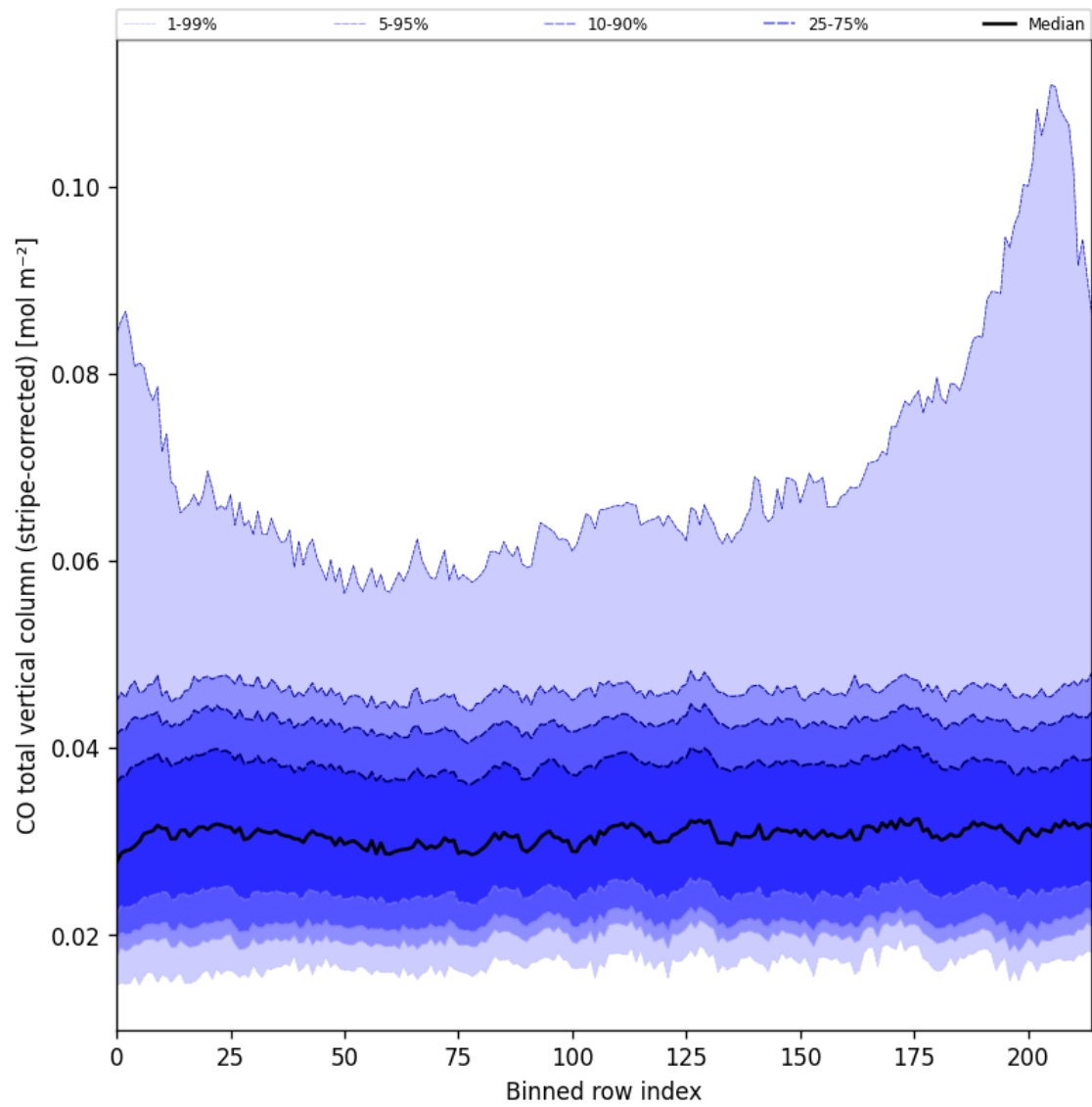
Figure 27: Along track statistics of “CO total vertical column (stripe-corrected)” for 2024-08-28 to 2024-08-30
