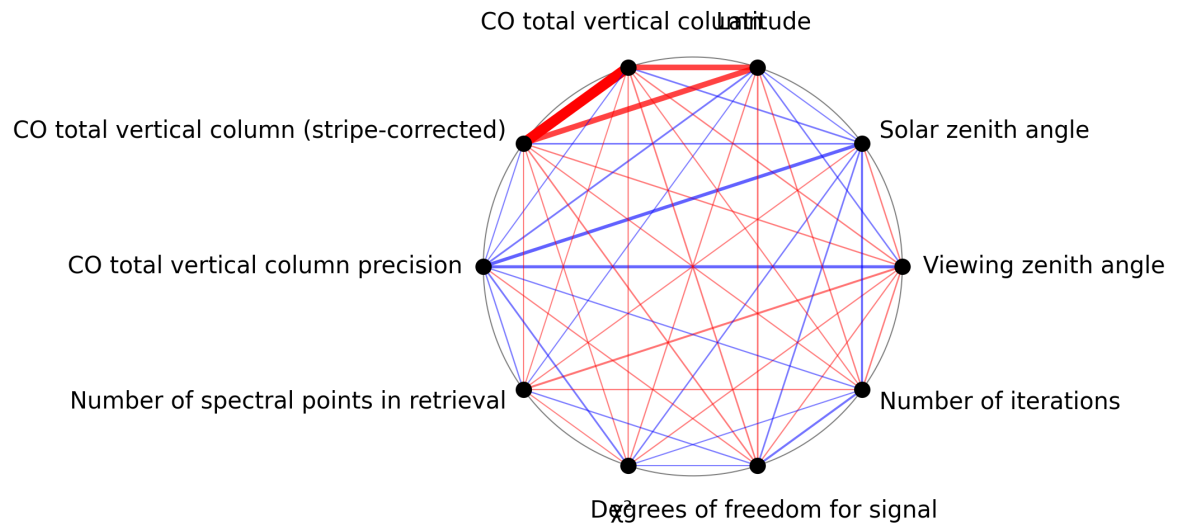
Figure 1: Map of correlation graph for 2024-08-28 to 2024-08-30.
