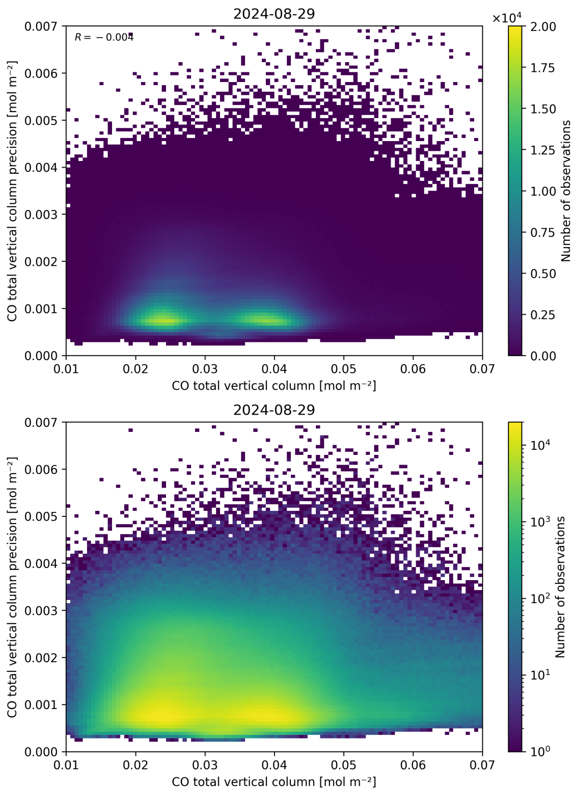
Figure 34: Scatter density plot of “CO total vertical column” against “CO total vertical column precision” for 2024-08-28 to 2024-08-30.
