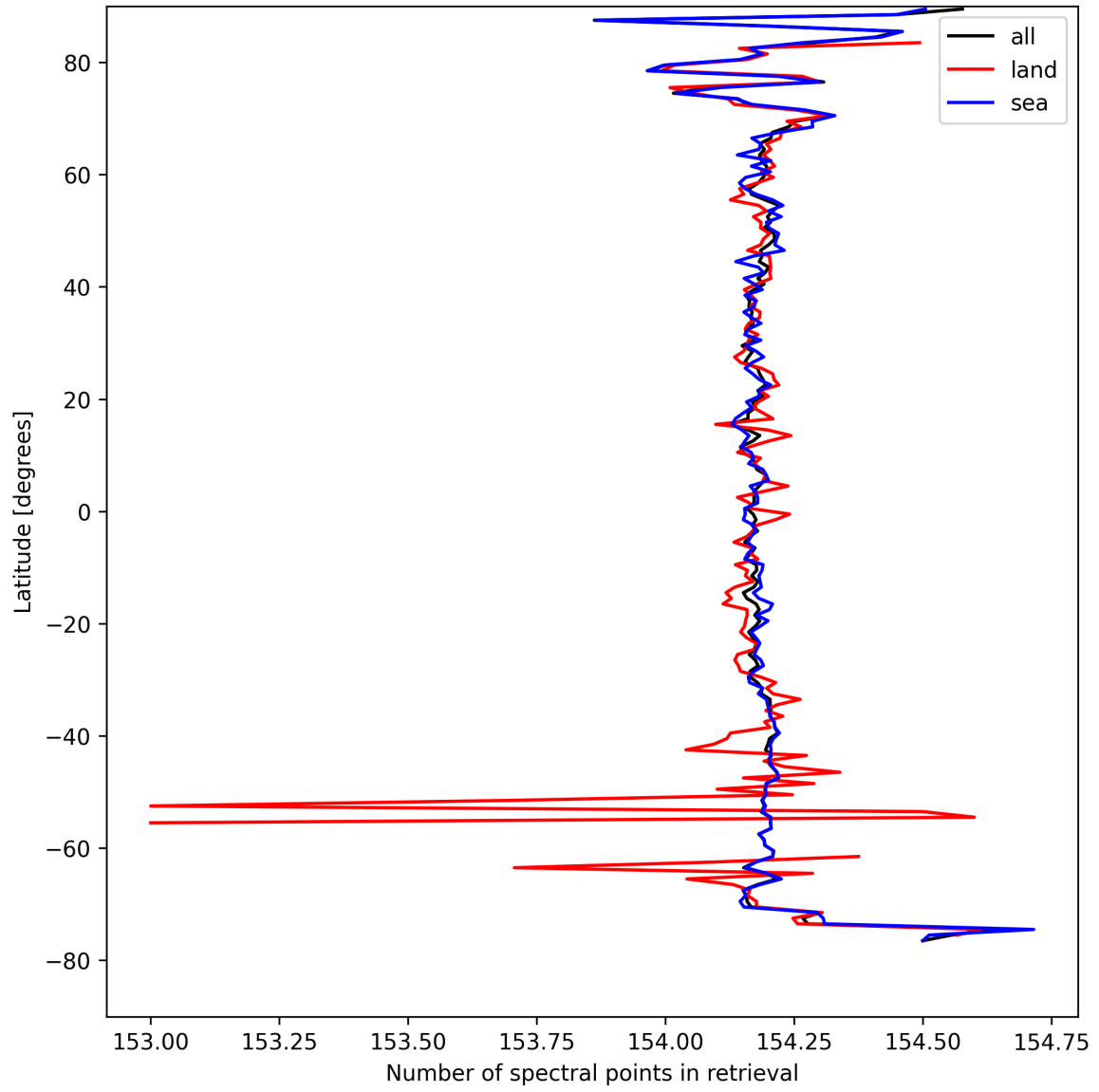
Figure 13: Zonal average of “Number of spectral points in retrieval” for 2024-08-28 to 2024-08-30.
