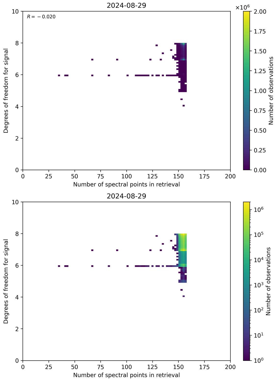
Figure 59: Scatter density plot of “Number of spectral points in retrieval” against “Degrees of freedom for signal” for 2024-08-28 to 2024-08-30.
