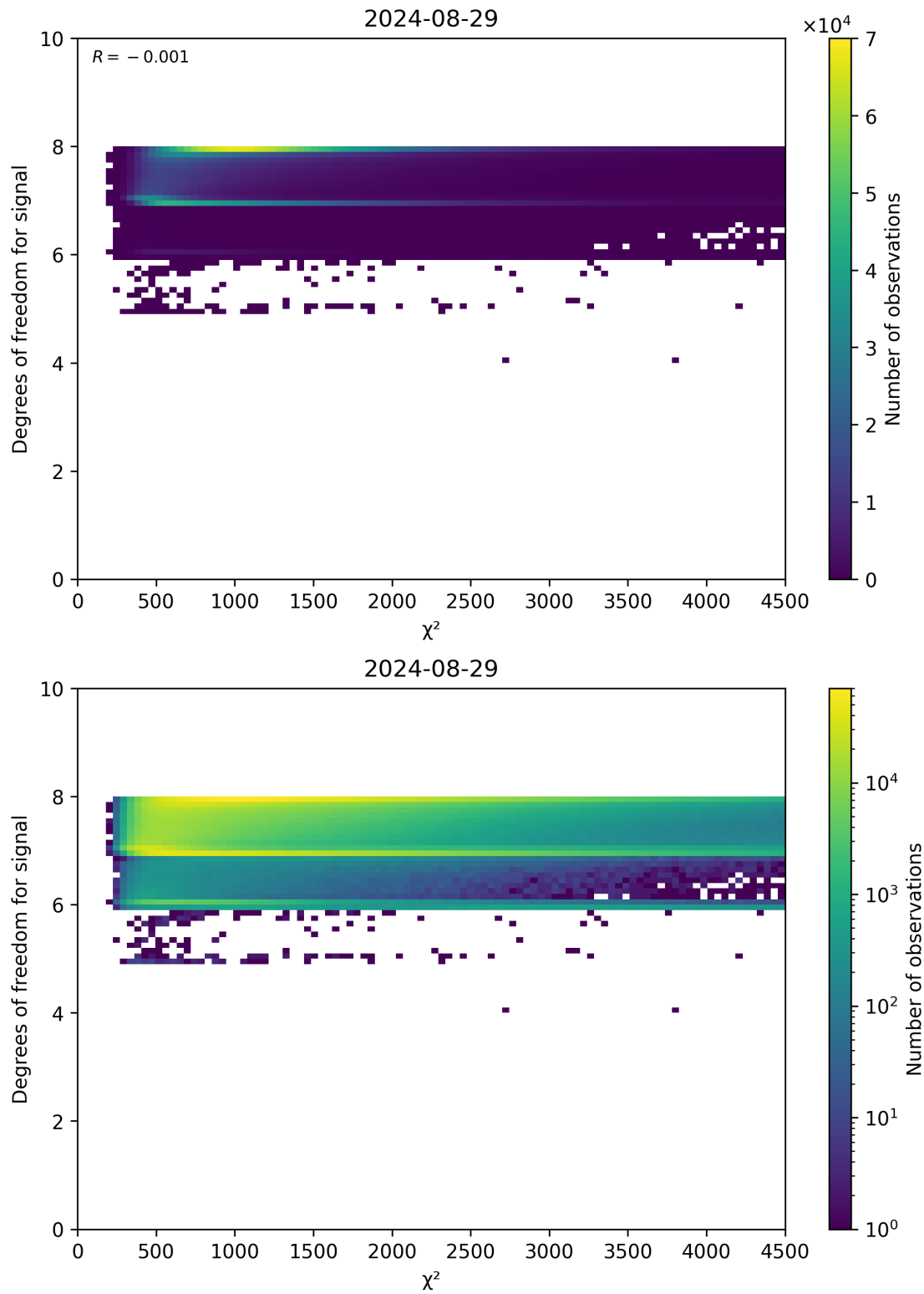
Figure 48: Scatter density plot of “ \chi^2 ” against “Degrees of freedom for signal” for 2024-08-28 to 2024-08-30.
