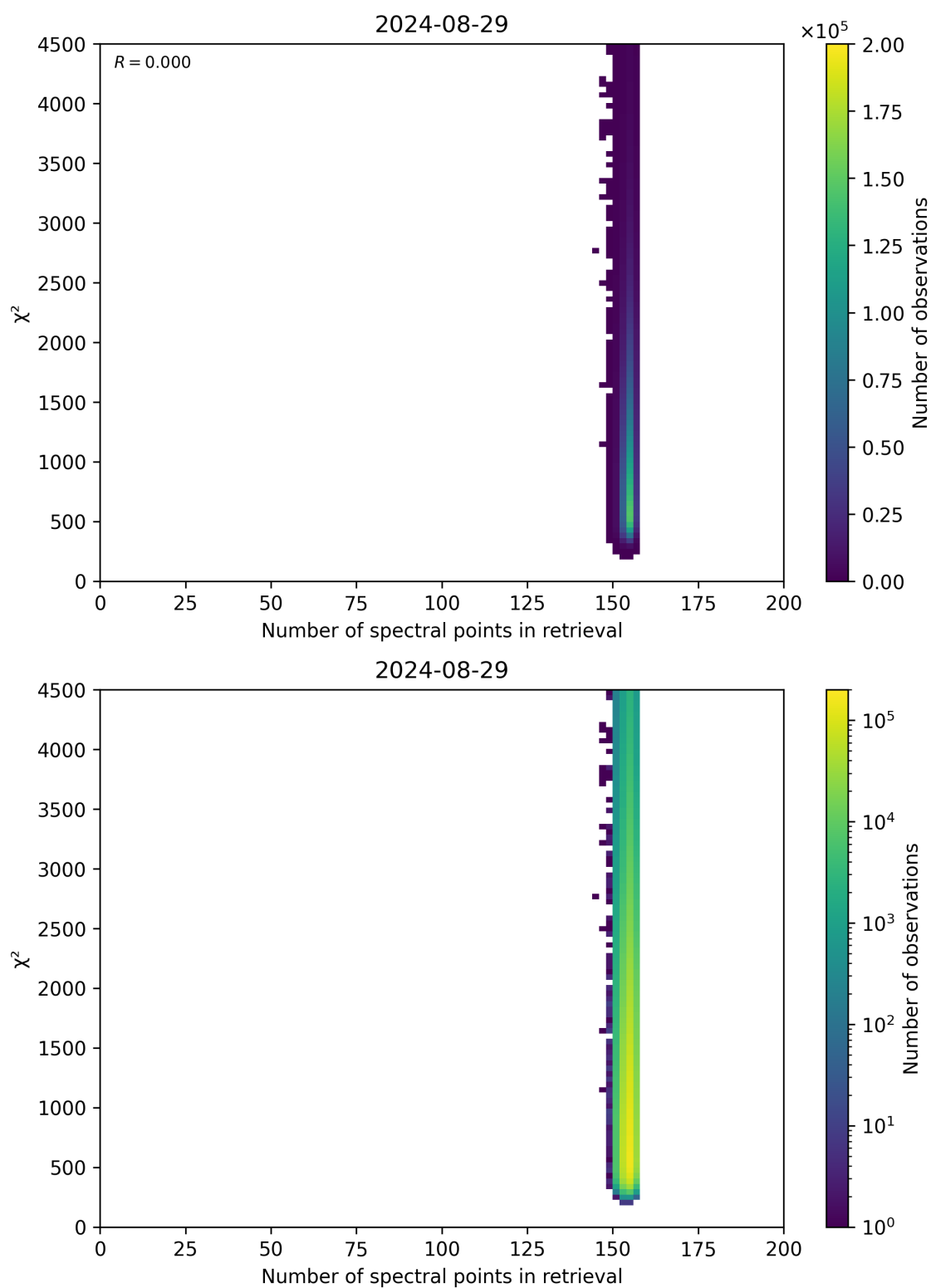
Figure 58: Scatter density plot of “Number of spectral points in retrieval” against “ \chi^2 ” for 2024-08-28 to 2024-08-30.
