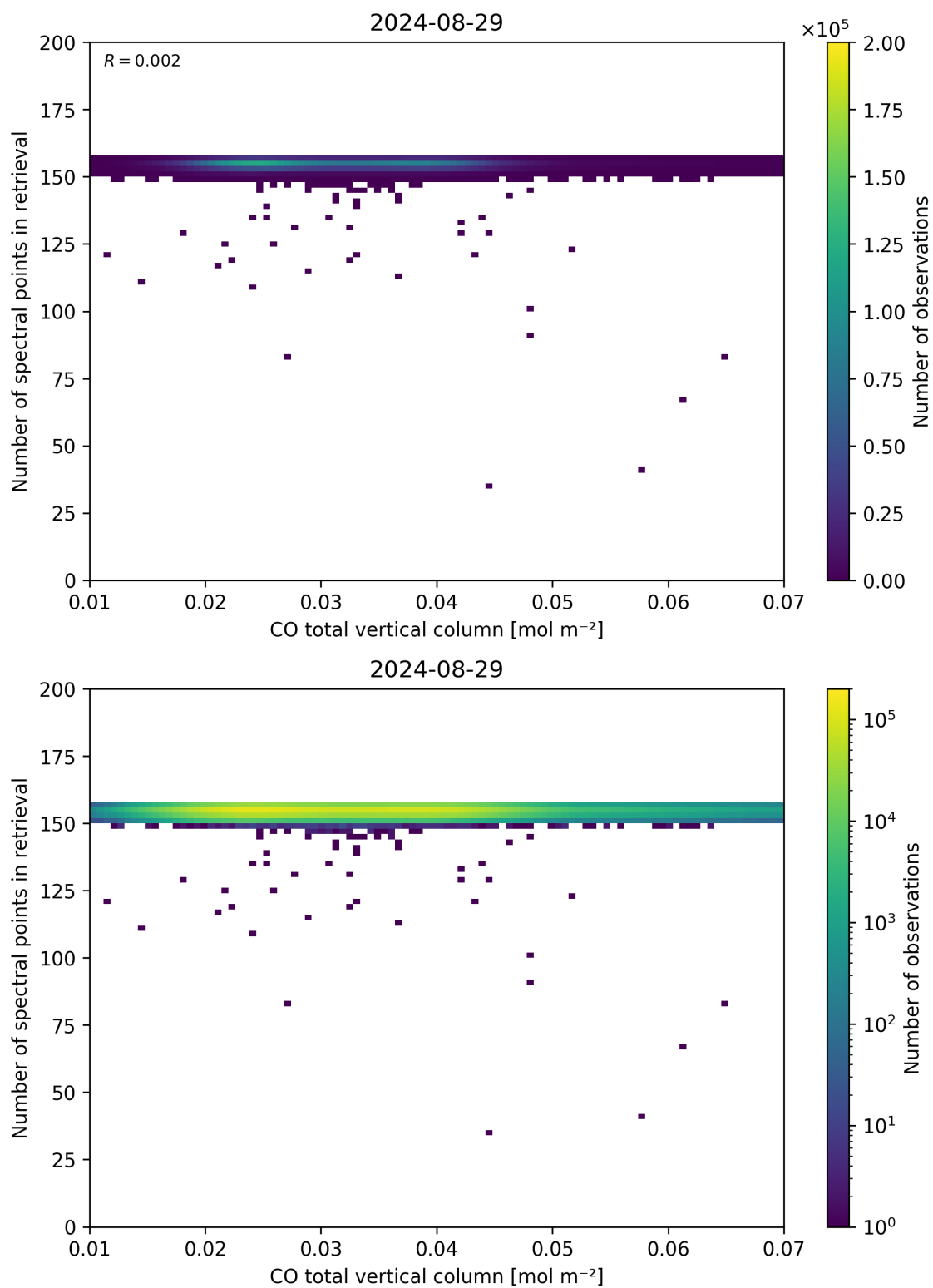
Figure 43: Scatter density plot of “CO total vertical column” against “Number of spectral points in retrieval” for 2024-08-28 to 2024-08-30.
