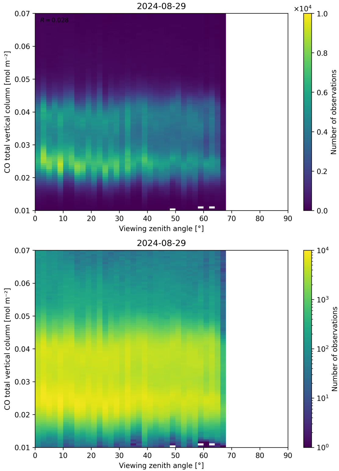
Figure 69: Scatter density plot of “Viewing zenith angle” against “CO total vertical column” for 2024-08-28 to 2024-08-30.
