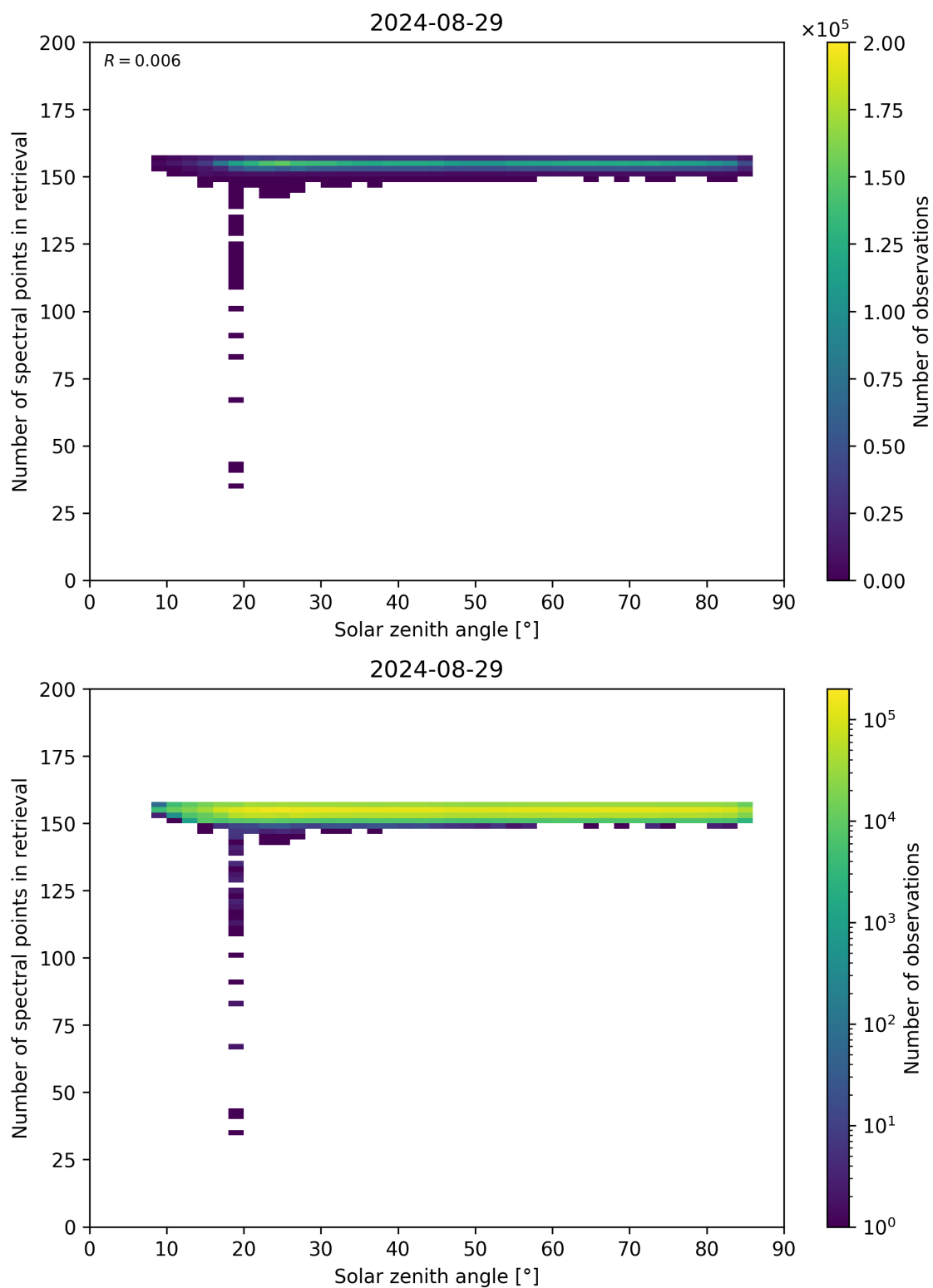
Figure 68: Scatter density plot of “Solar zenith angle” against “Number of spectral points in retrieval” for 2024-08-28 to 2024-08-30.
