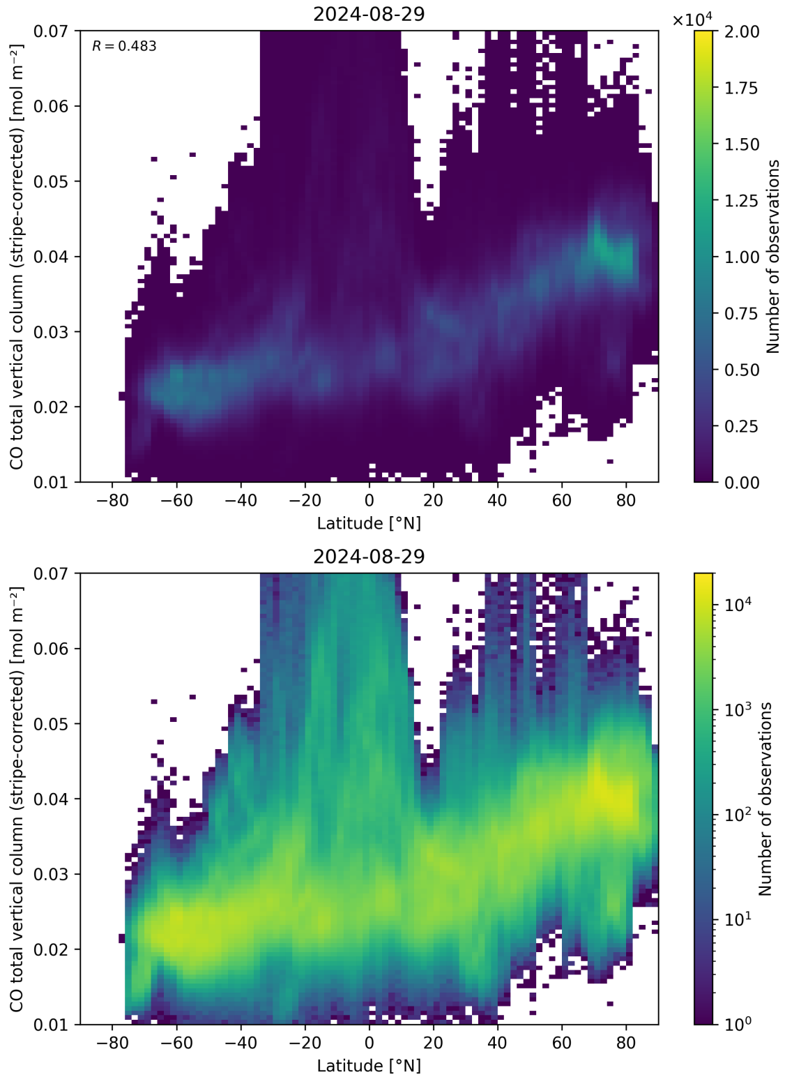
Figure 52: Scatter density plot of “Latitude” against “CO total vertical column (stripe-corrected)” for 2024-08-28 to 2024-08-30.
