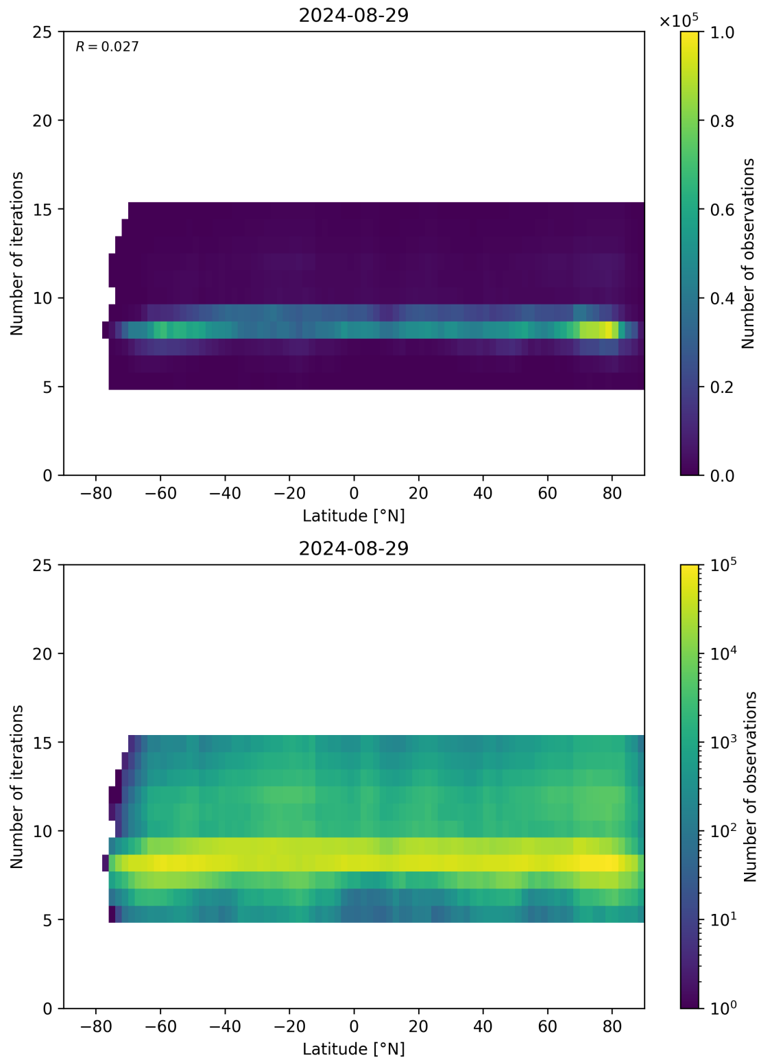
Figure 56: Scatter density plot of “Latitude” against “Number of iterations” for 2024-08-28 to 2024-08-30.
