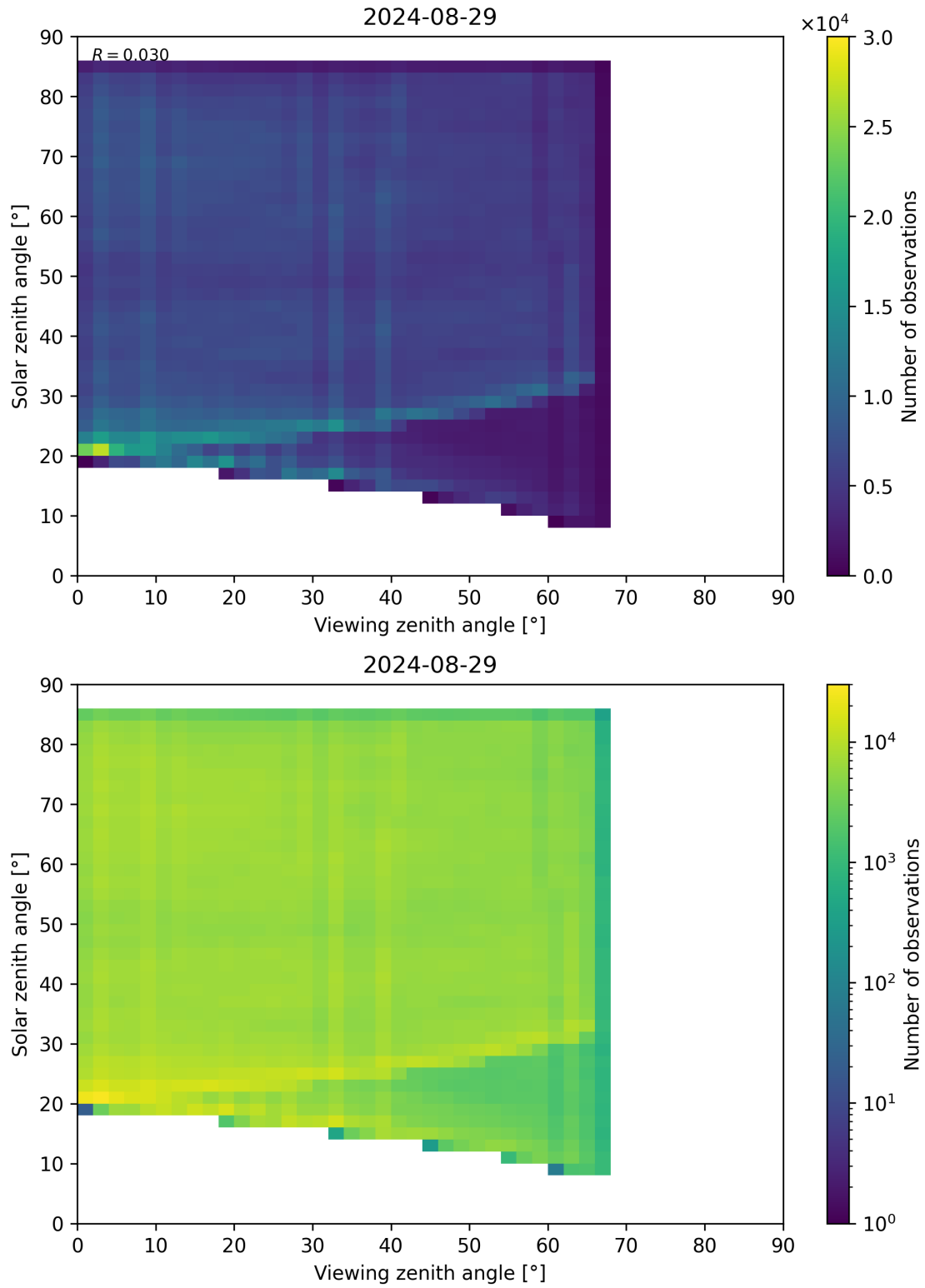
Figure 77: Scatter density plot of “Viewing zenith angle” against “Solar zenith angle” for 2024-08-28 to 2024-08-30.
