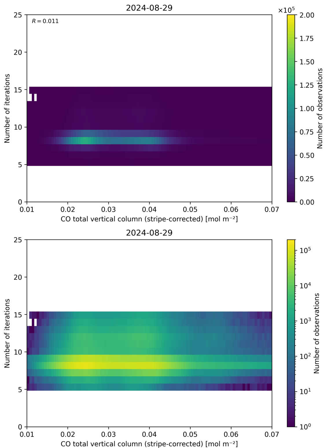
Figure 39: Scatter density plot of “CO total vertical column (stripe-corrected)” against “Number of iterations” for 2024-08-28 to 2024-08-30.
