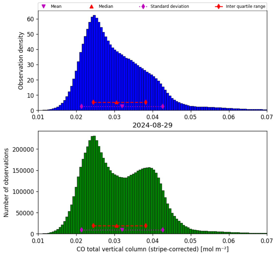
Figure 19: Histogram of “CO total vertical column (stripe-corrected)” for 2024-08-28 to 2024-08-30
