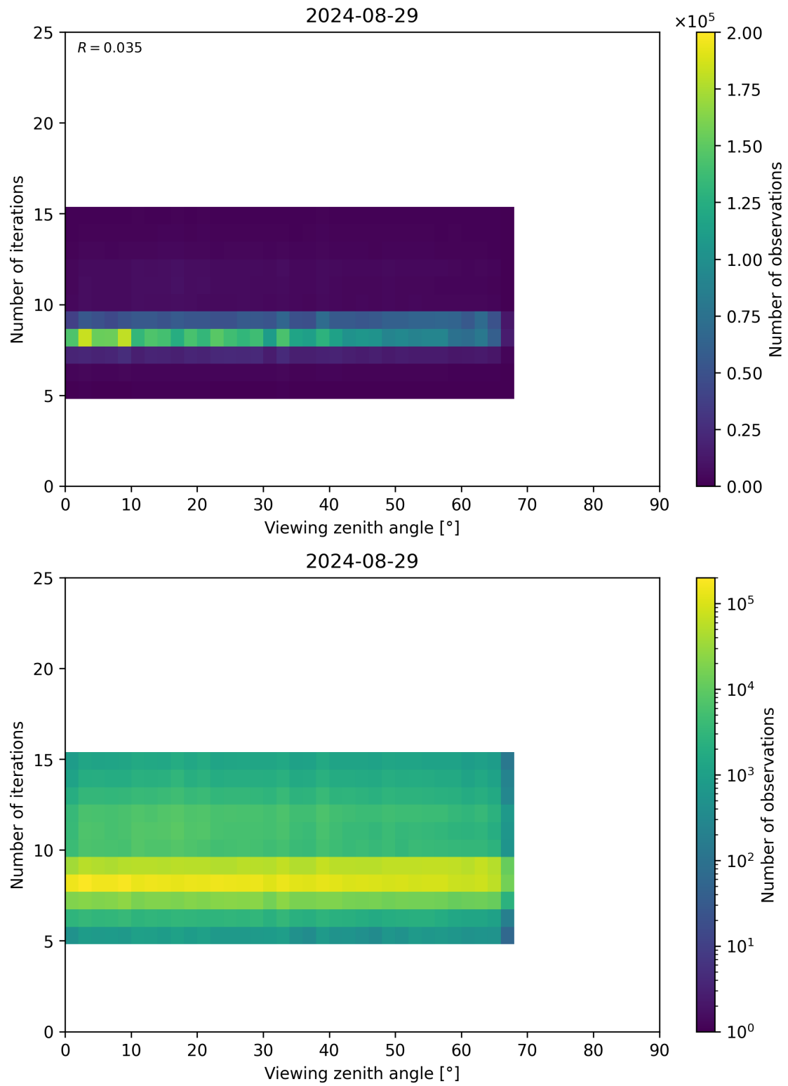
Figure 75: Scatter density plot of “Viewing zenith angle” against “Number of iterations” for 2024-08-28 to 2024-08-30.
