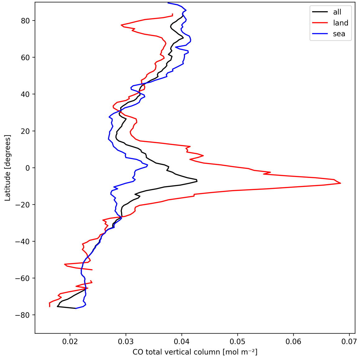
Figure 10: Zonal average of “CO total vertical column” for 2024-08-28 to 2024-08-30.
