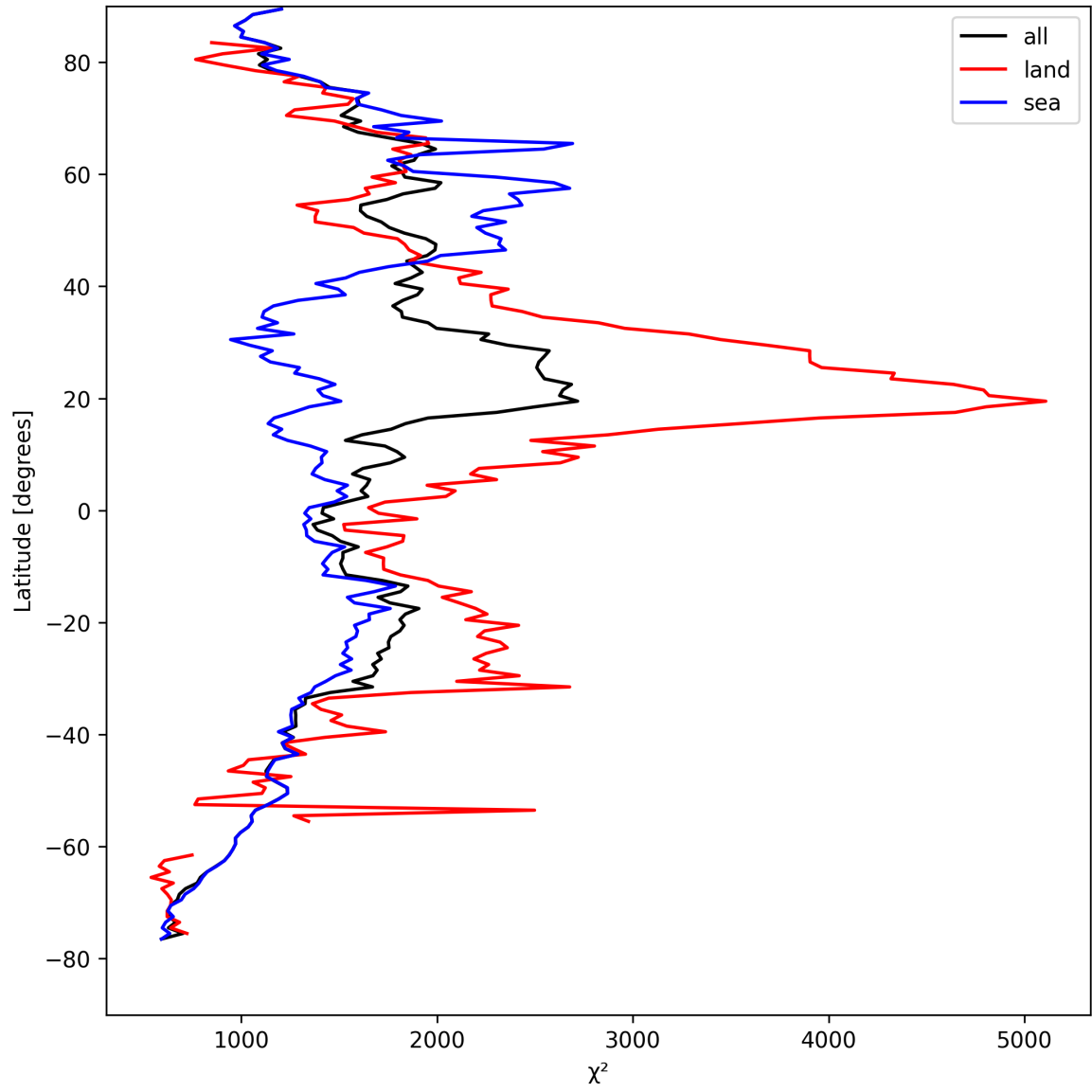
Figure 14: Zonal average of “ \chi^2 ” for 2024-08-28 to 2024-08-30.
