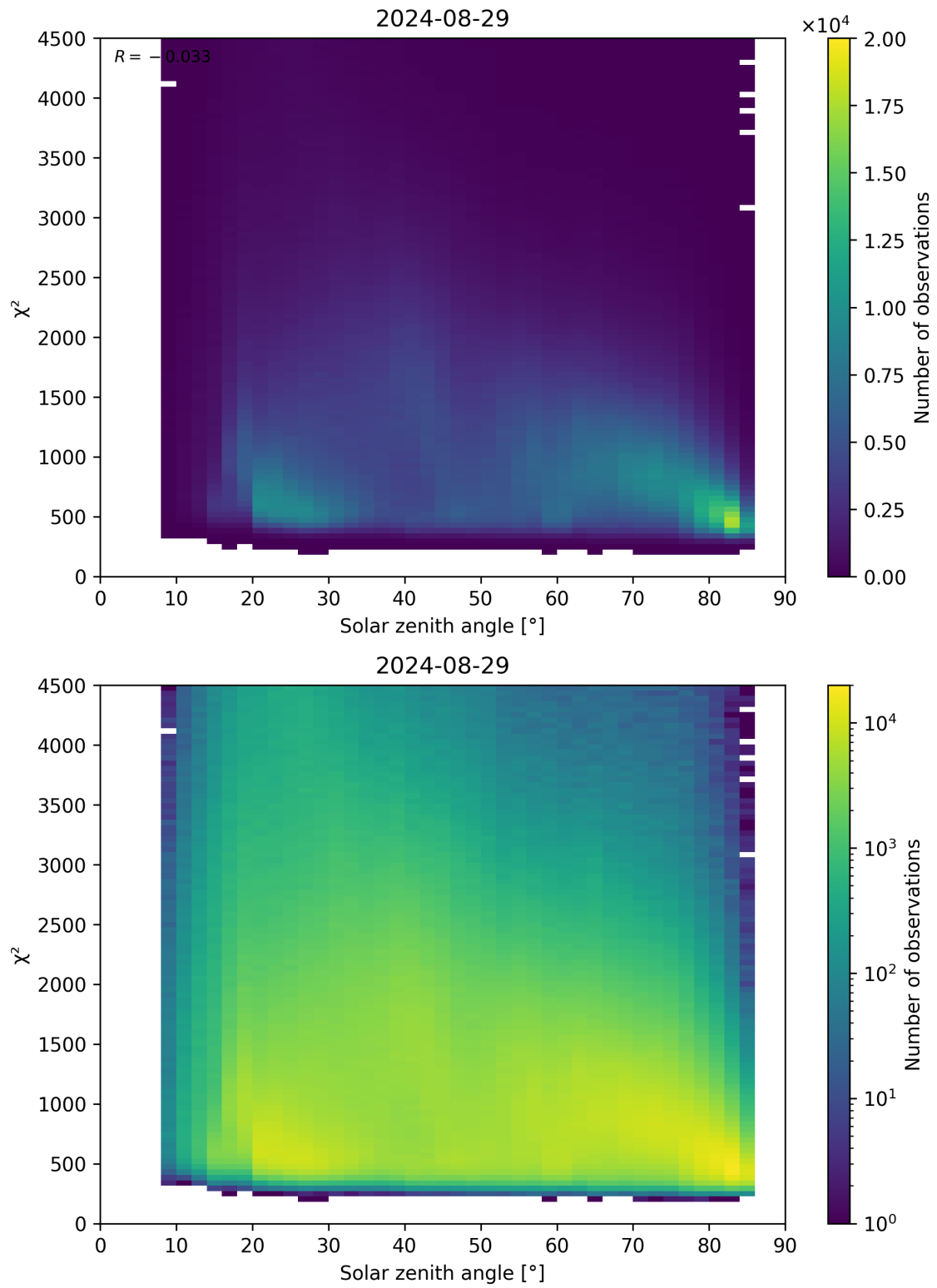
Figure 64: Scatter density plot of “Solar zenith angle” against “ \chi^2 ” for 2024-08-28 to 2024-08-30.
