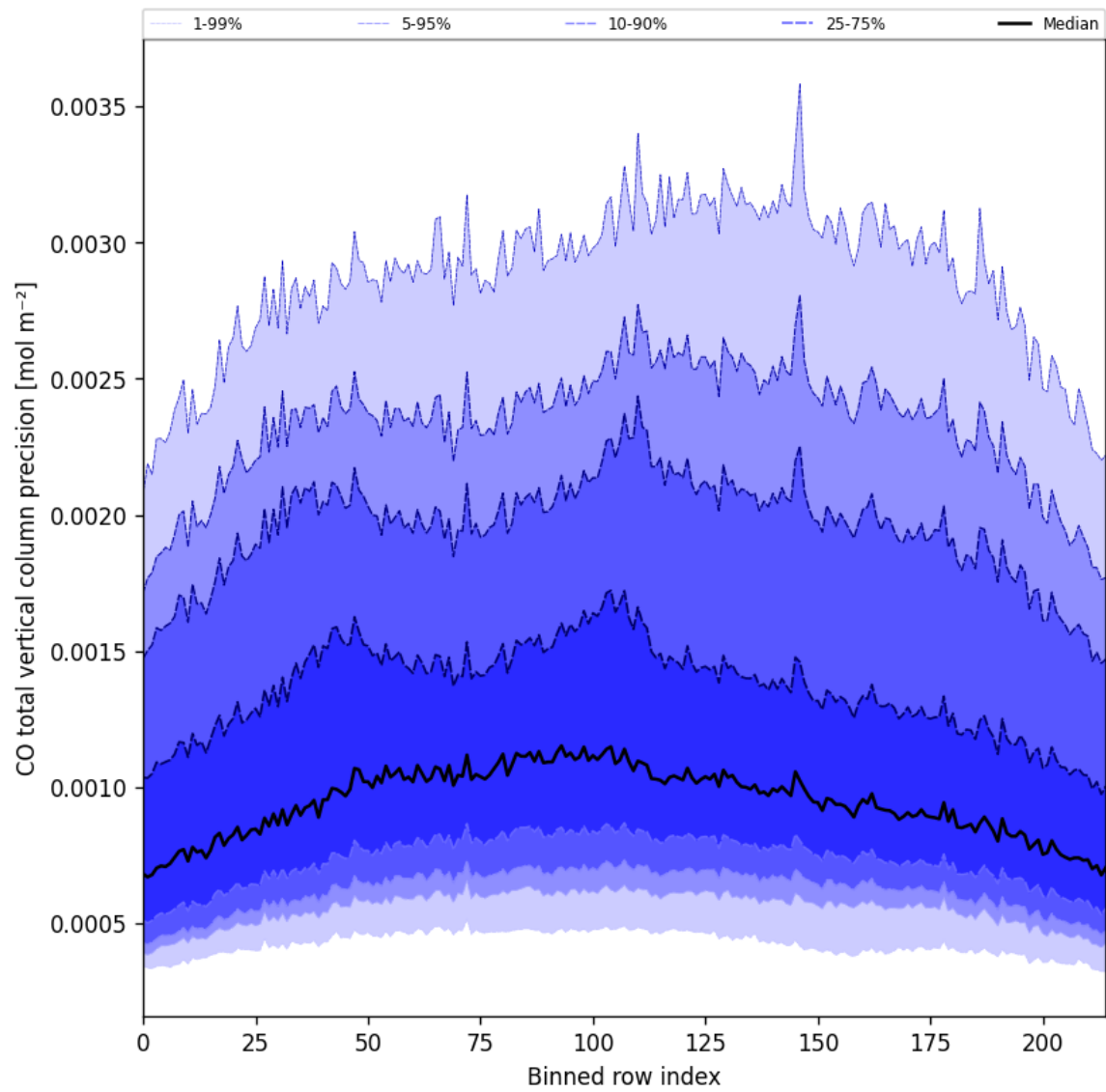
Figure 28: Along track statistics of “CO total vertical column precision” for 2024-08-28 to 2024-08-30
