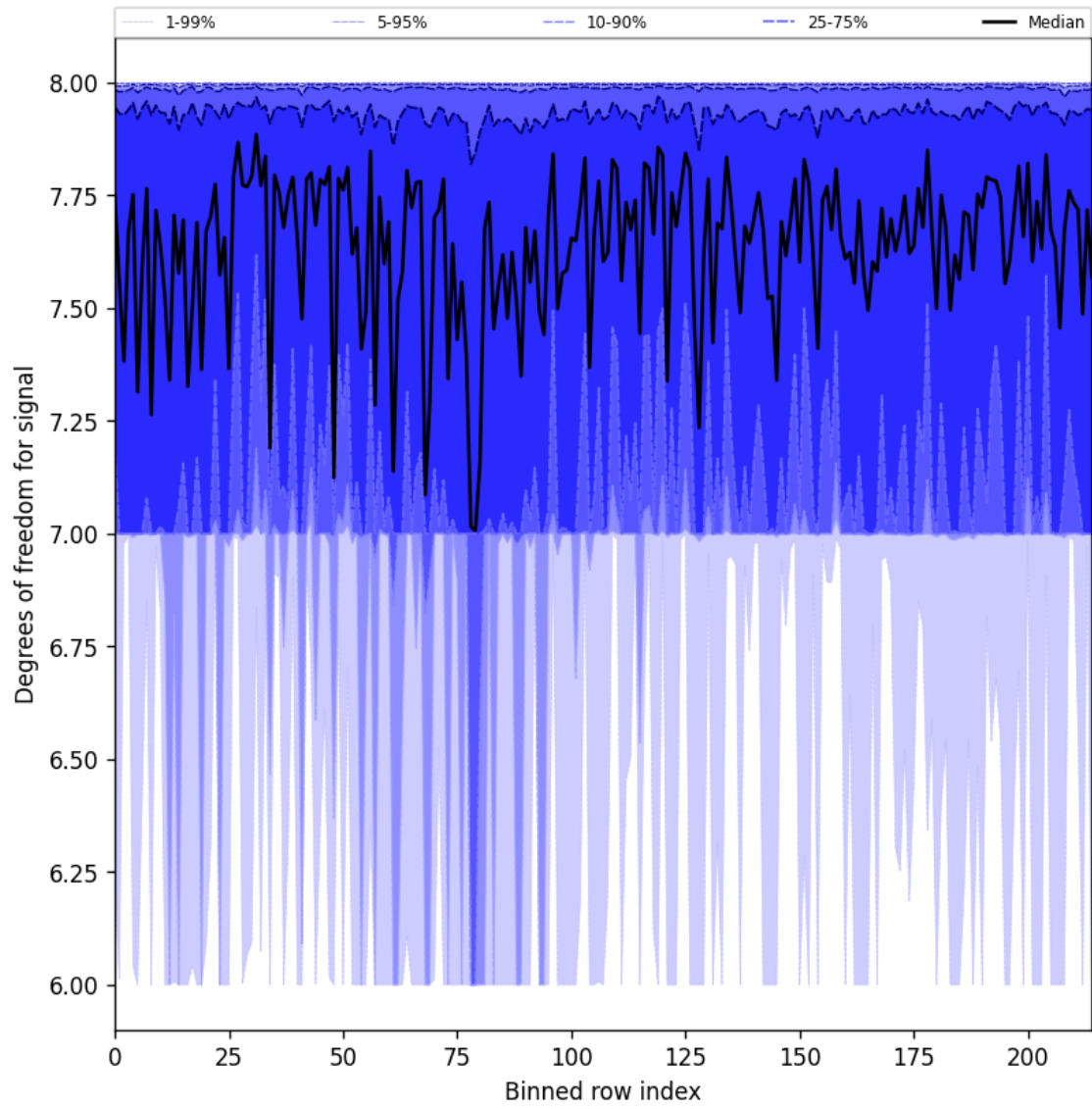
Figure 31: Along track statistics of “Degrees of freedom for signal” for 2024-08-28 to 2024-08-30
