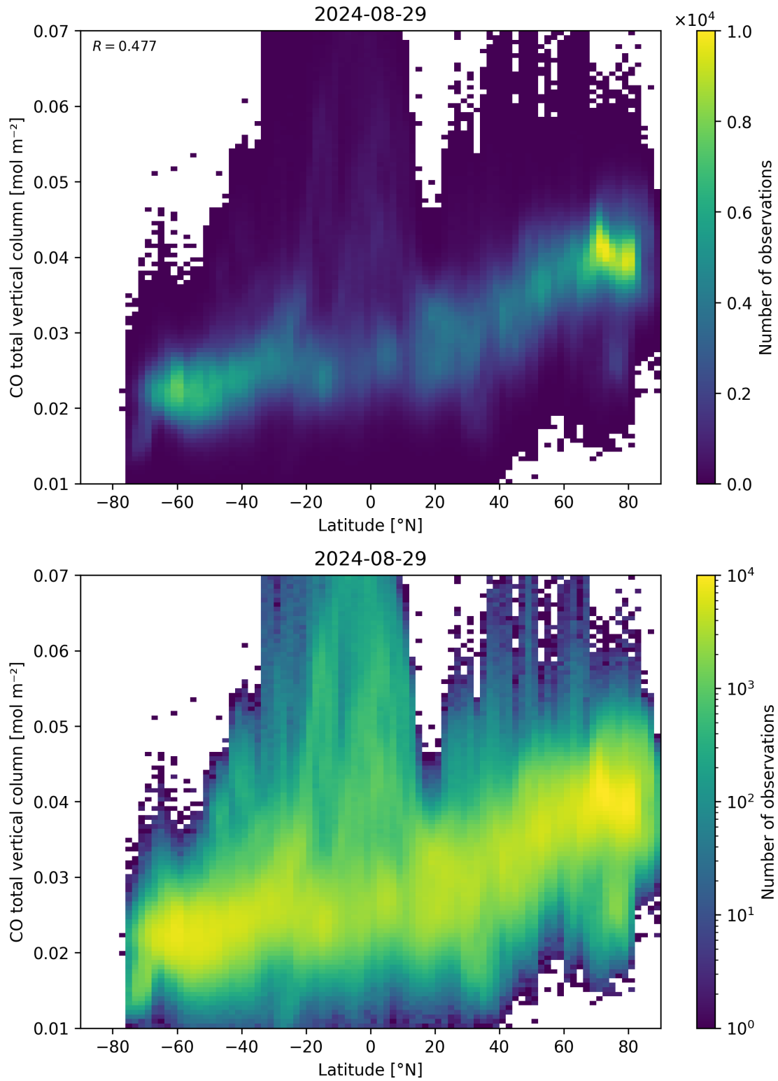
Figure 51: Scatter density plot of “Latitude” against “CO total vertical column” for 2024-08-28 to 2024-08-30.
