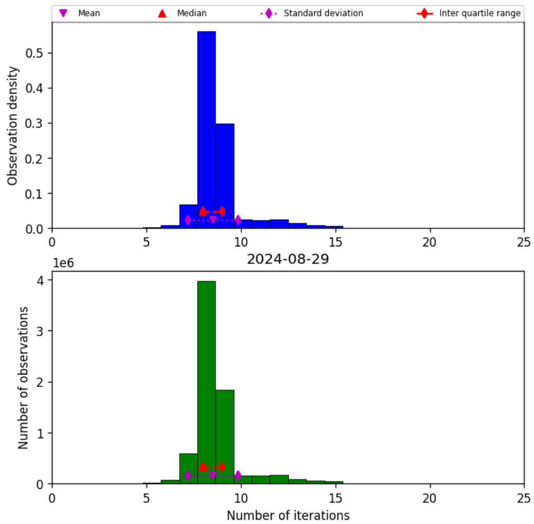
Figure 24: Histogram of “Number of iterations” for 2024-08-28 to 2024-08-30
