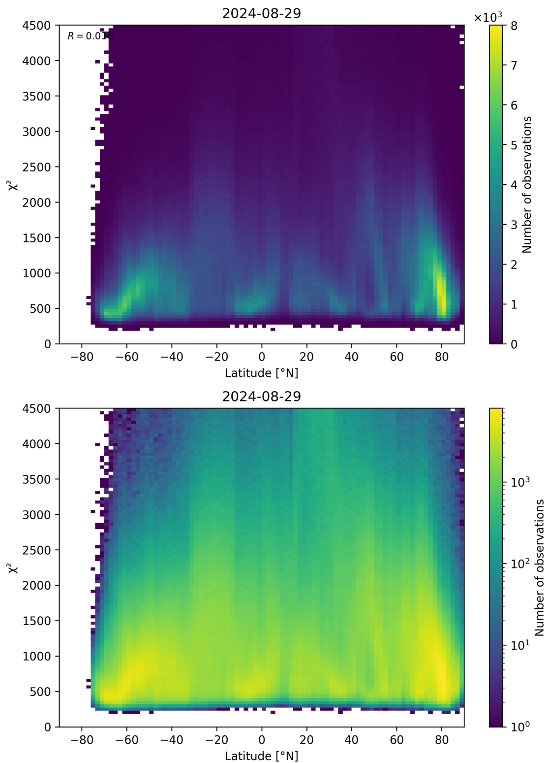
Figure 54: Scatter density plot of “Latitude” against “ \chi^2 ” for 2024-08-28 to 2024-08-30.
