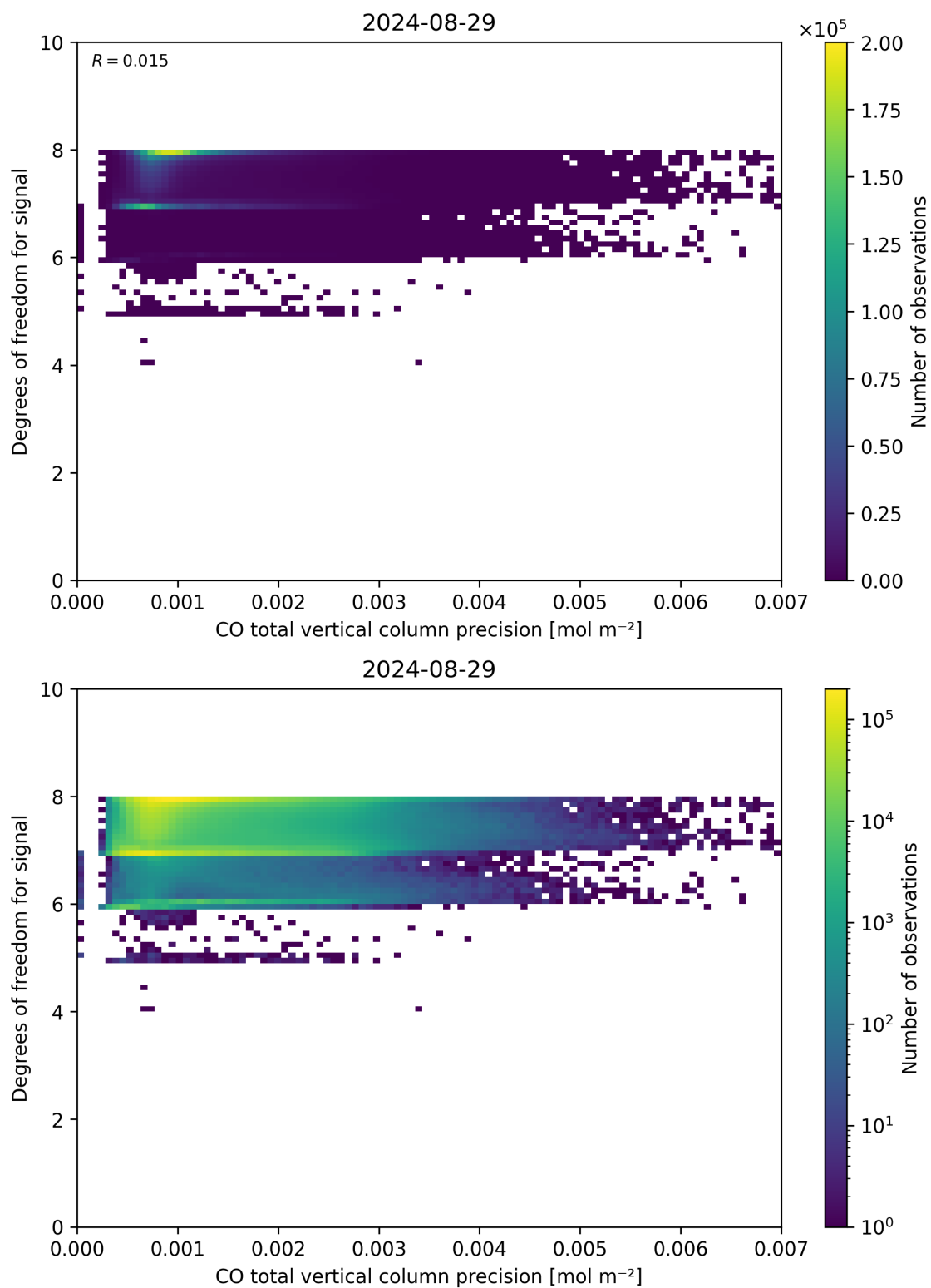
Figure 45: Scatter density plot of “CO total vertical column precision” against “Degrees of freedom for signal” for 2024-08-28 to 2024-08-30.
