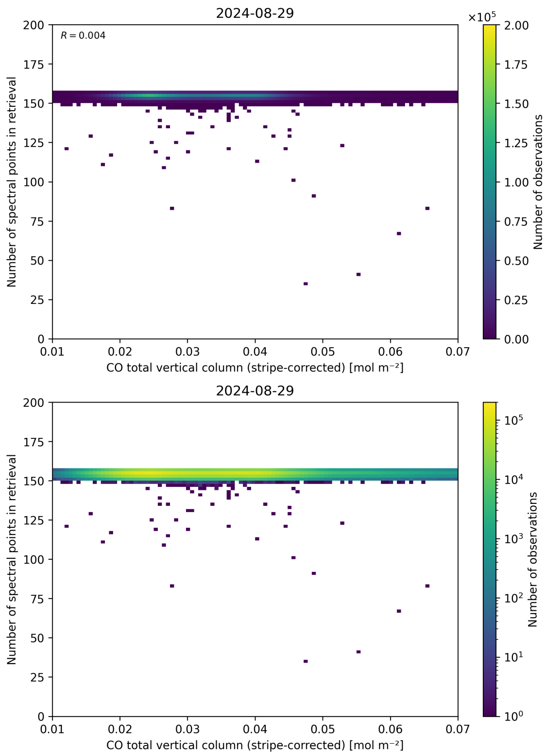
Figure 40: Scatter density plot of “CO total vertical column (stripe-corrected)” against “Number of spectral points in retrieval” for 2024-08-28 to 2024-08-30.
