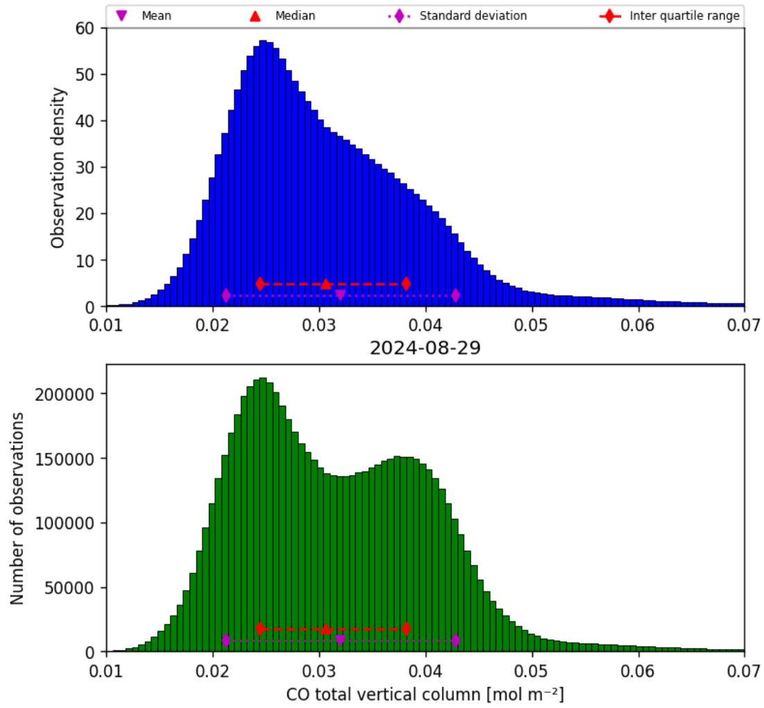
Figure 18: Histogram of “CO total vertical column” for 2024-08-28 to 2024-08-30
