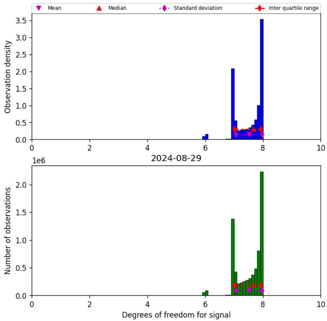
Figure 23: Histogram of “Degrees of freedom for signal” for 2024-08-28 to 2024-08-30
