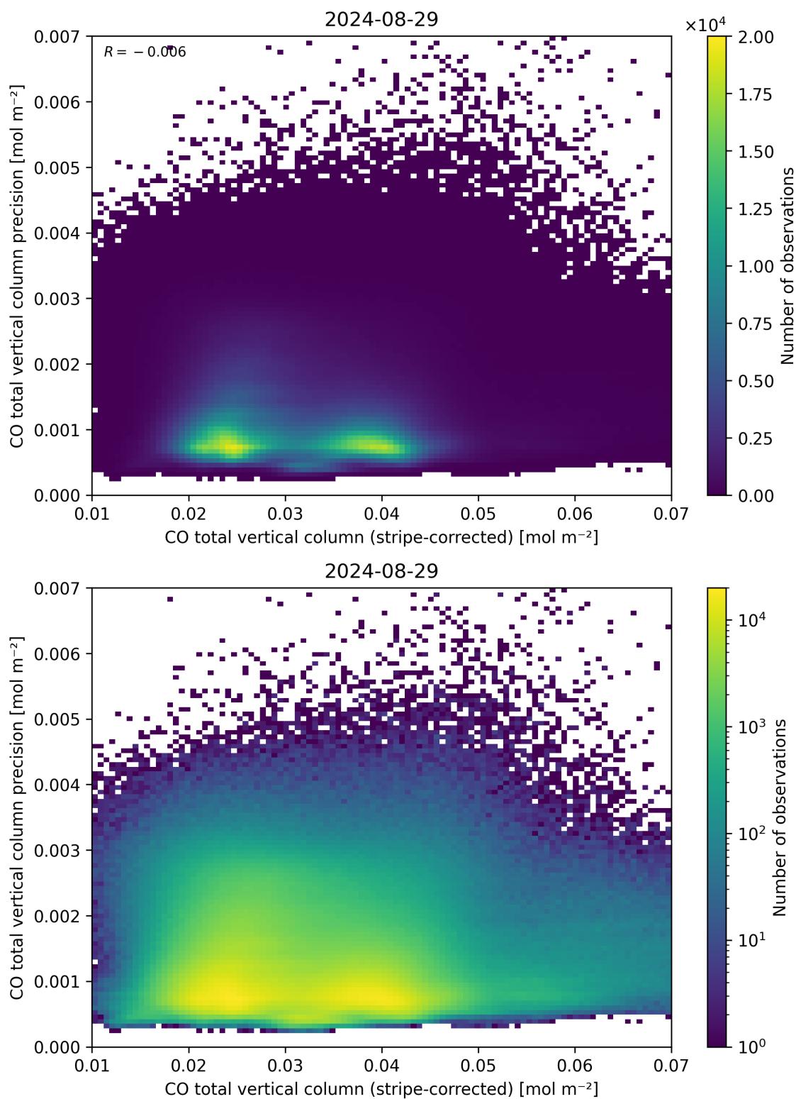
Figure 36: Scatter density plot of “CO total vertical column (stripe-corrected)” against “CO total vertical column precision” for 2024-08-28 to 2024-08-30.
