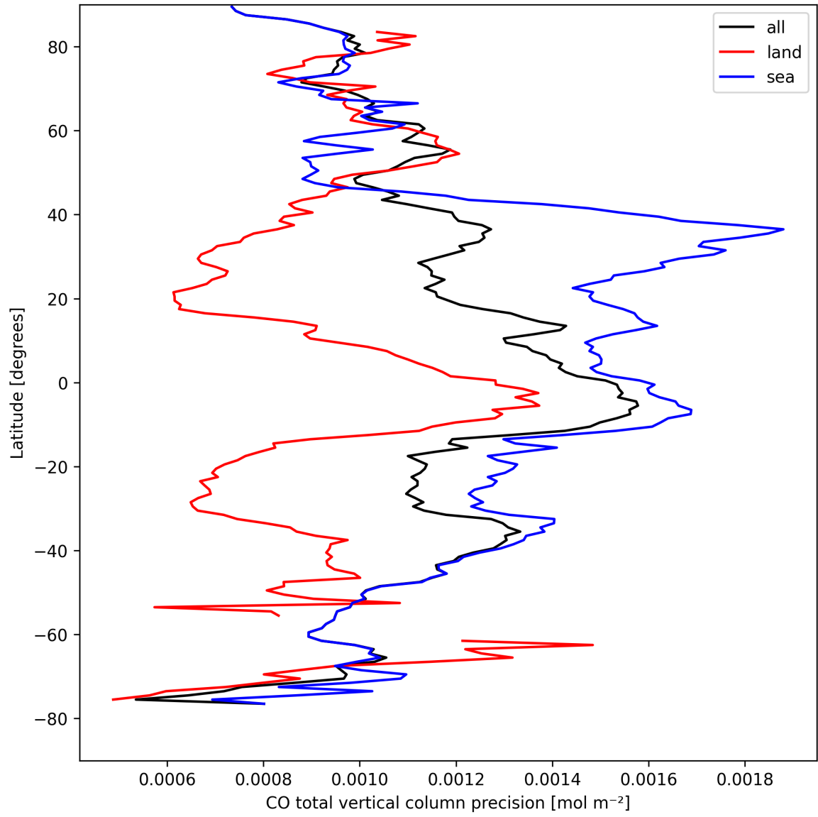
Figure 12: Zonal average of “CO total vertical column precision” for 2024-08-28 to 2024-08-30.
