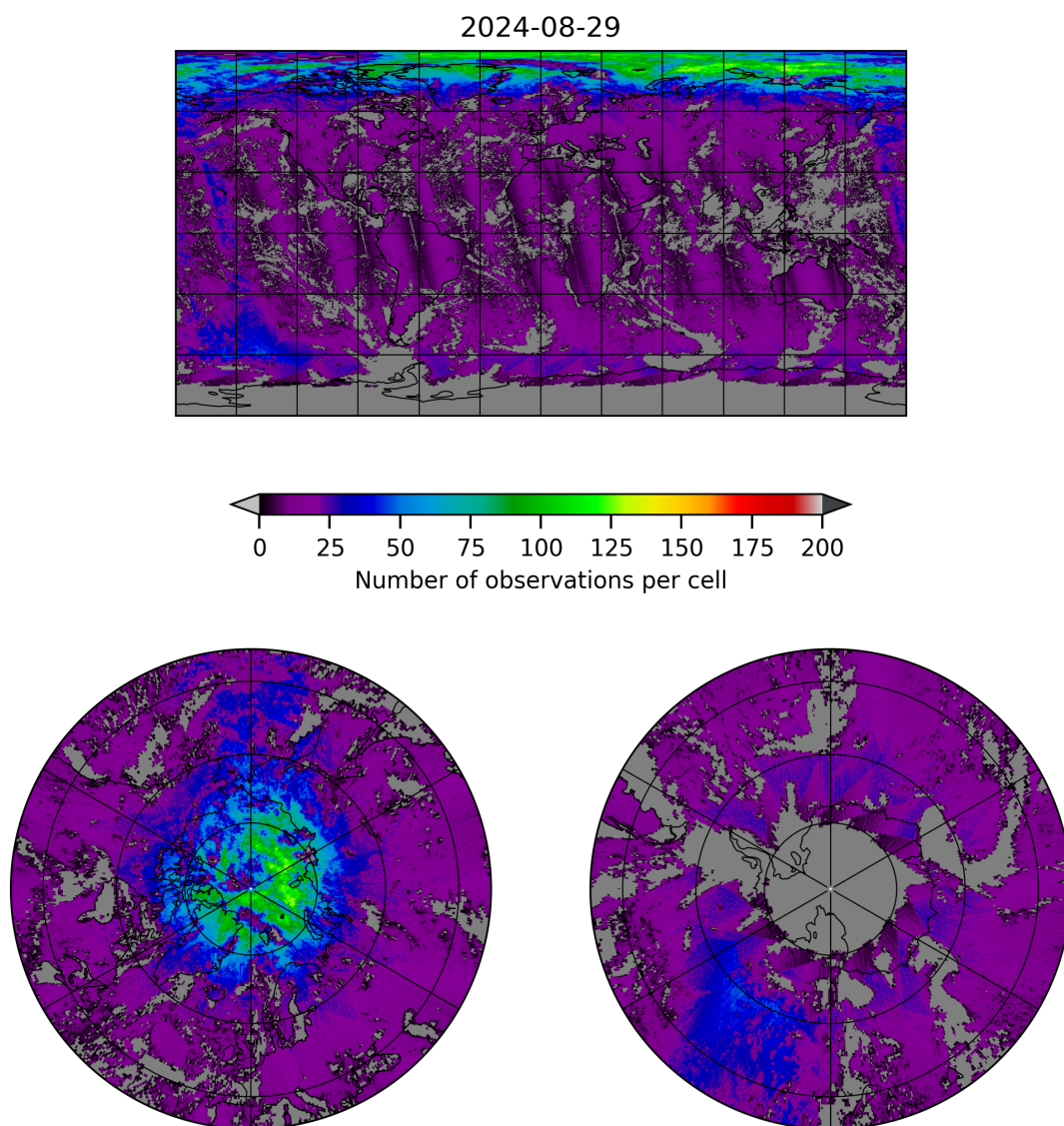
Figure 8: Map of the number of observations for 2024-08-28 to 2024-08-30
