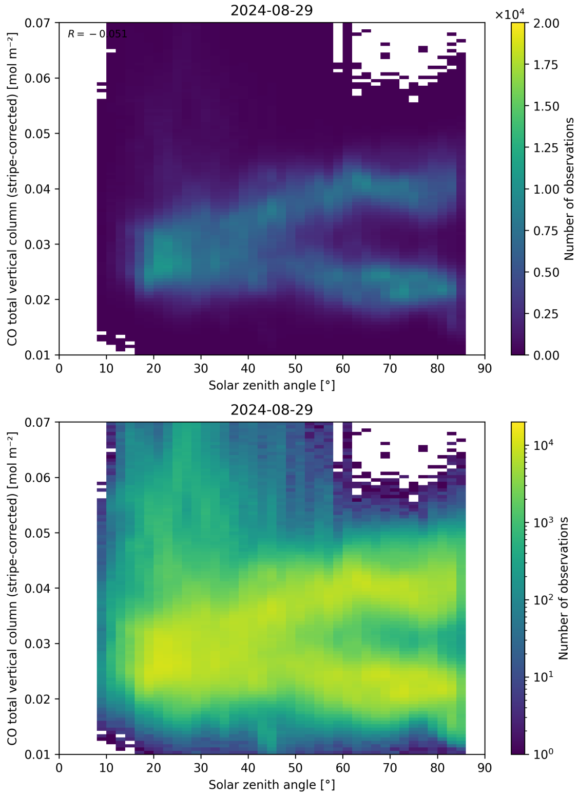
Figure 62: Scatter density plot of “Solar zenith angle” against “CO total vertical column (stripe-corrected)” for 2024-08-28 to 2024-08-30.
