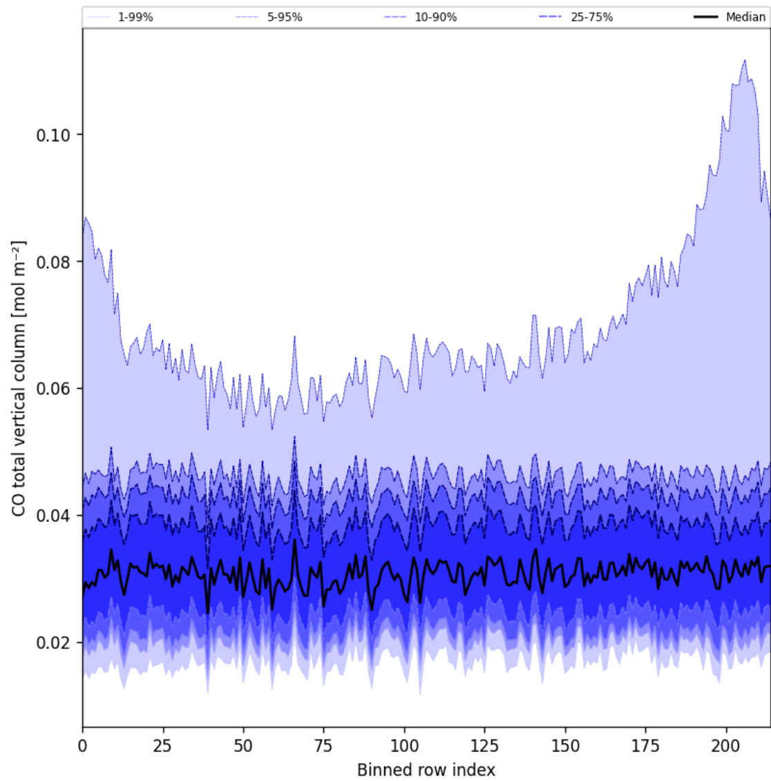
Figure 26: Along track statistics of “CO total vertical column” for 2024-08-28 to 2024-08-30
