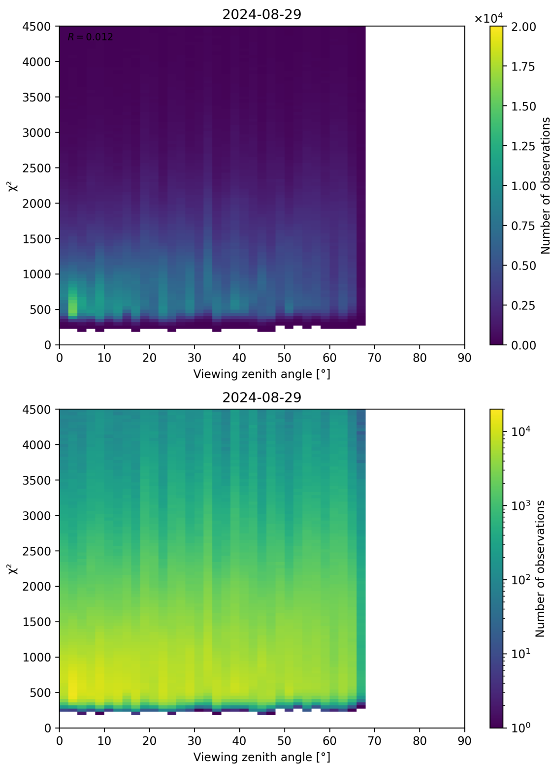
Figure 72: Scatter density plot of “Viewing zenith angle” against “ \chi^2 ” for 2024-08-28 to 2024-08-30.
