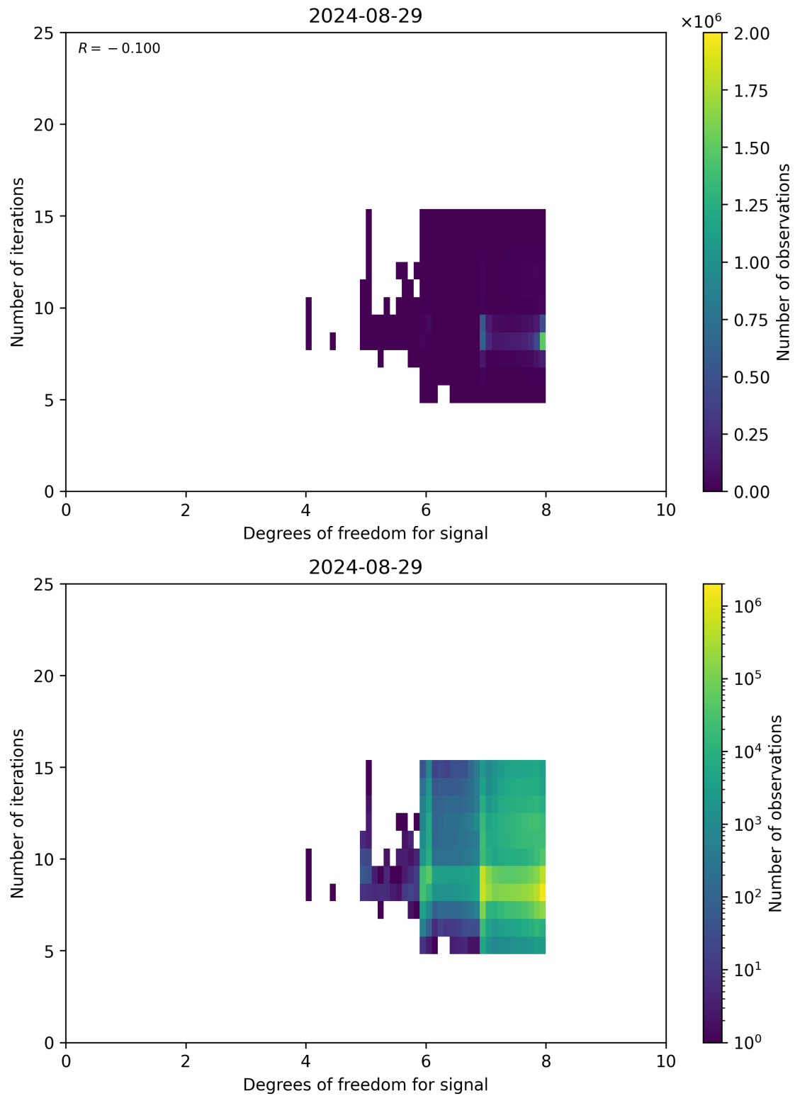
Figure 50: Scatter density plot of “Degrees of freedom for signal” against “Number of iterations” for 2024-08-28 to 2024-08-30.
