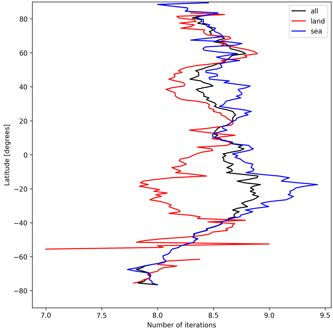
Figure 16: Zonal average of “Number of iterations” for 2024-08-28 to 2024-08-30.
