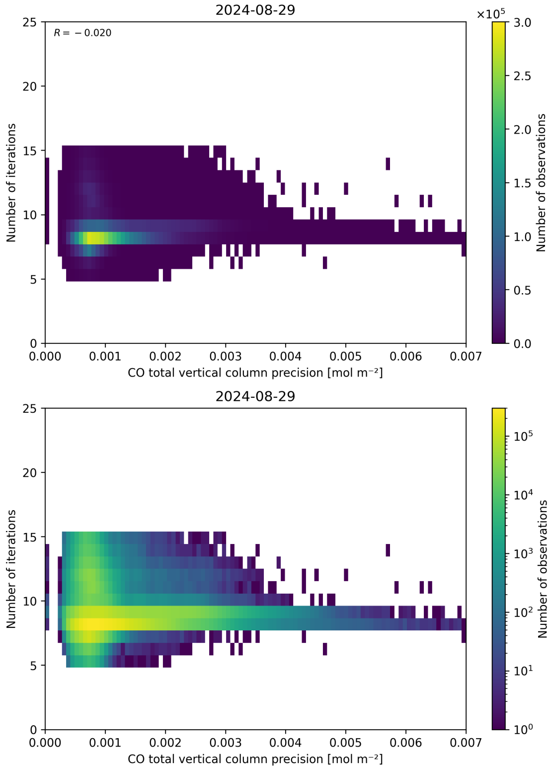
Figure 46: Scatter density plot of “CO total vertical column precision” against “Number of iterations” for 2024-08-28 to 2024-08-30.
