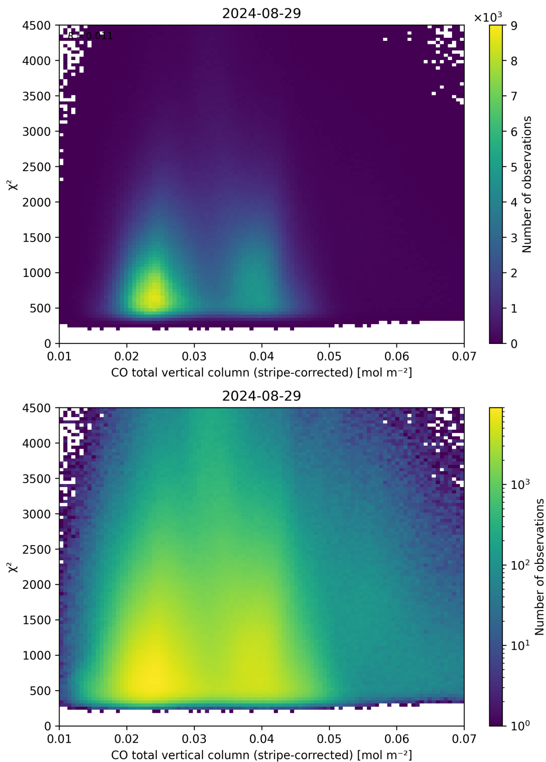
Figure 37: Scatter density plot of “CO total vertical column (stripe-corrected)” against “ \chi^2 ” for 2024-08-28 to 2024-08-30.
