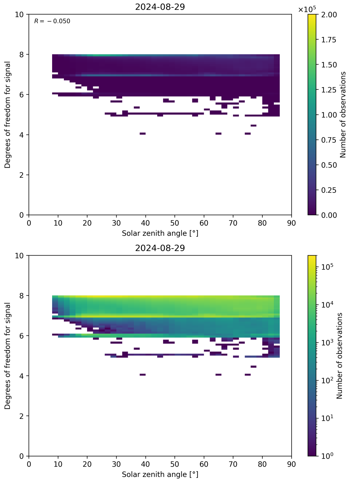
Figure 65: Scatter density plot of “Solar zenith angle” against “Degrees of freedom for signal” for 2024-08-28 to 2024-08-30.
