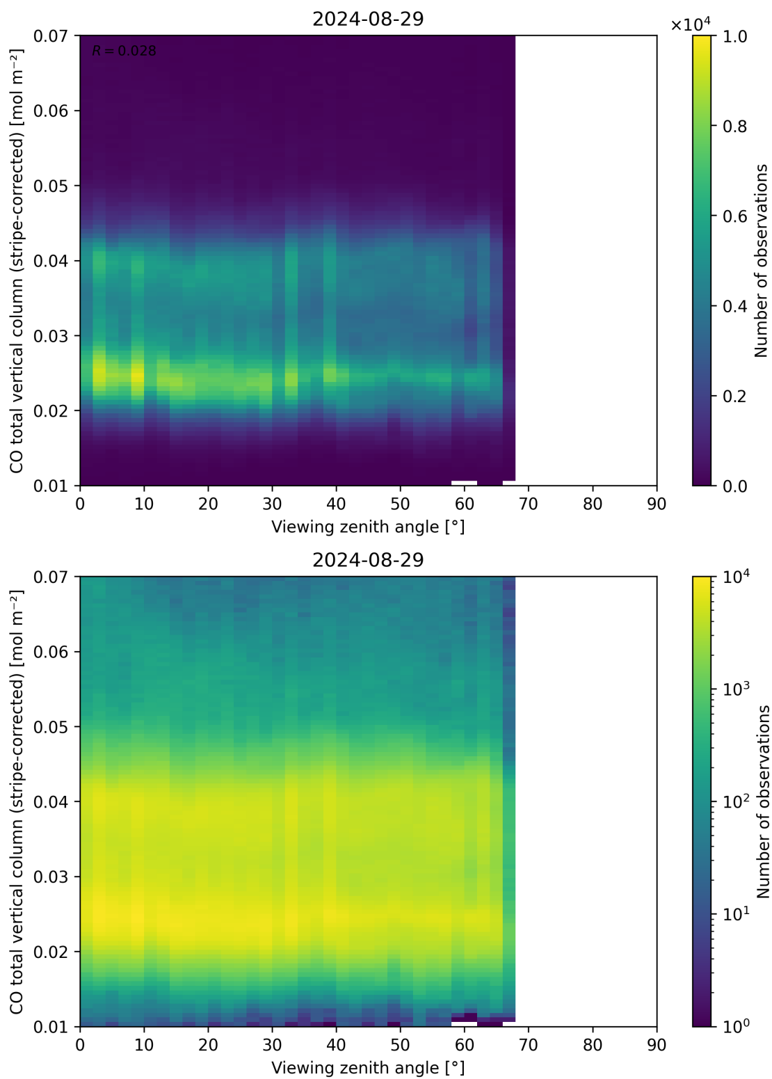
Figure 70: Scatter density plot of “Viewing zenith angle” against “CO total vertical column (stripe-corrected)” for 2024-08-28 to 2024-08-30.
