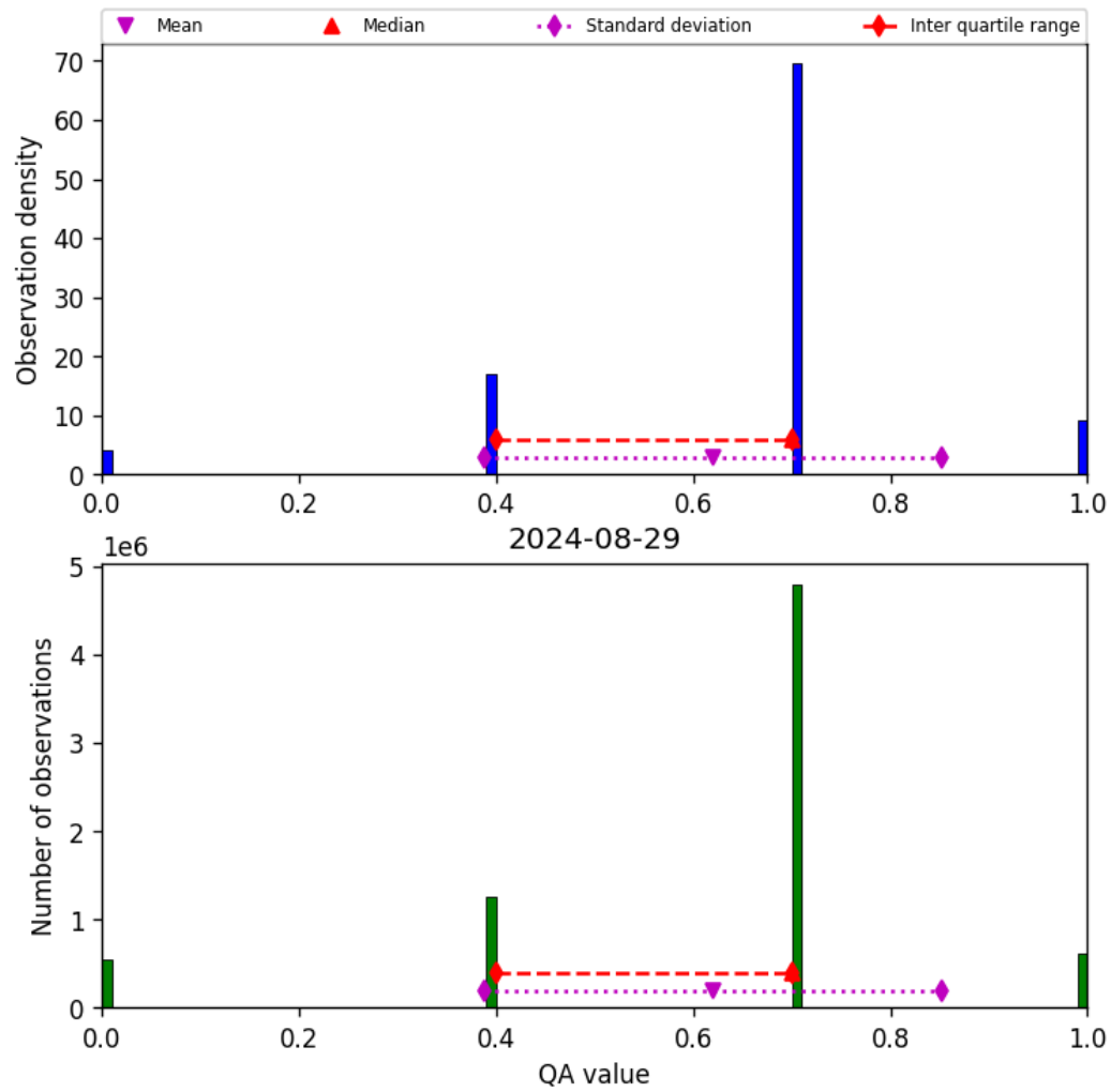
Figure 17: Histogram of “QA value” for 2024-08-28 to 2024-08-30
