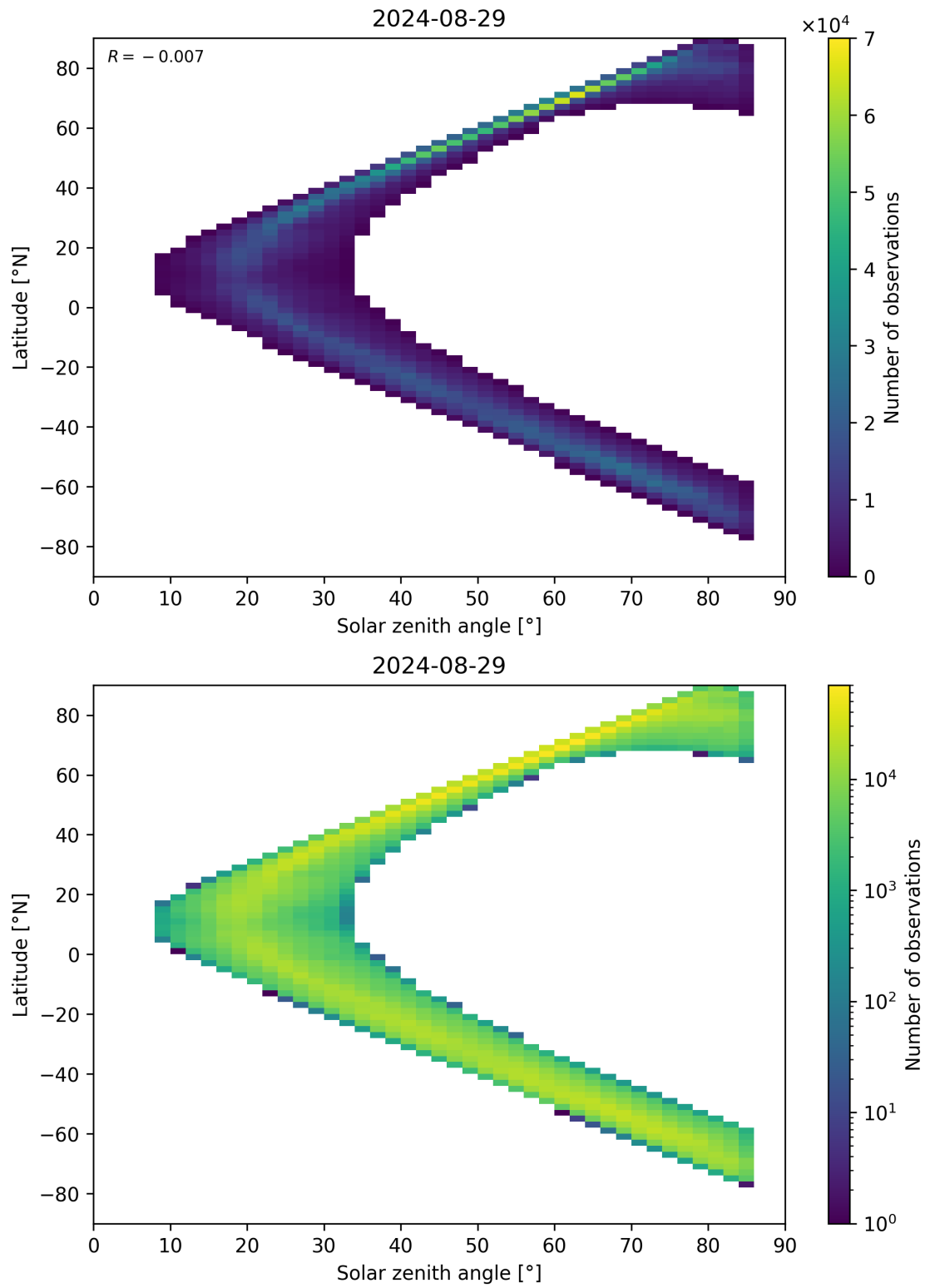
Figure 66: Scatter density plot of “Solar zenith angle” against “Latitude” for 2024-08-28 to 2024-08-30.
