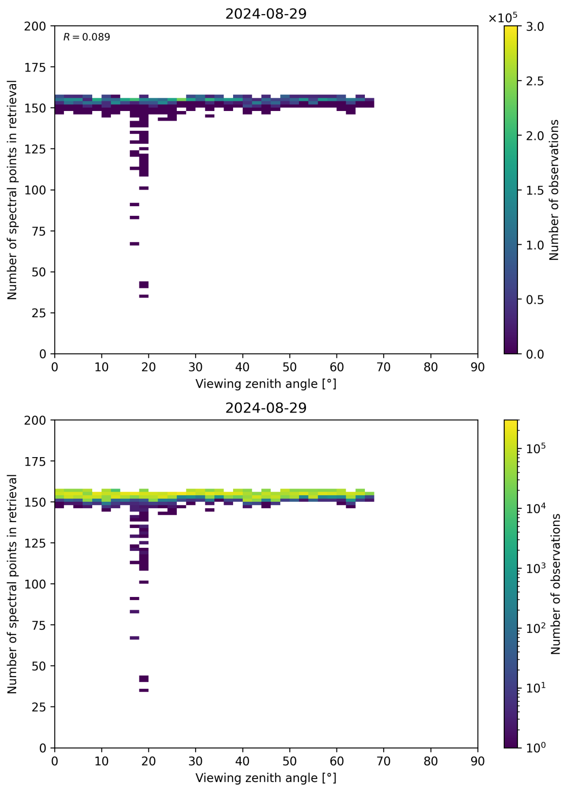
Figure 76: Scatter density plot of “Viewing zenith angle” against “Number of spectral points in retrieval” for 2024-08-28 to 2024-08-30.
