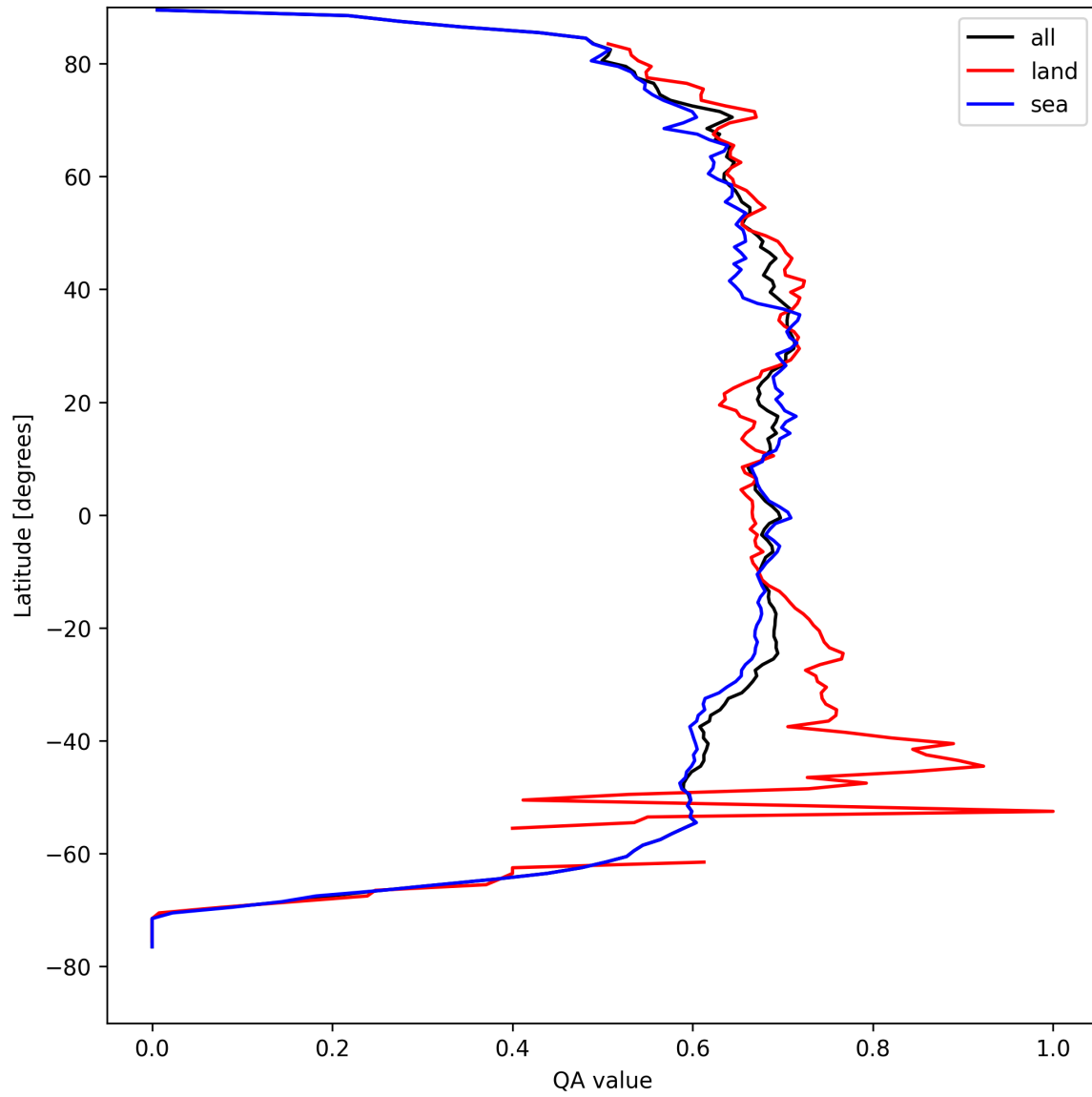
Figure 9: Zonal average of “QA value” for 2024-08-28 to 2024-08-30.
