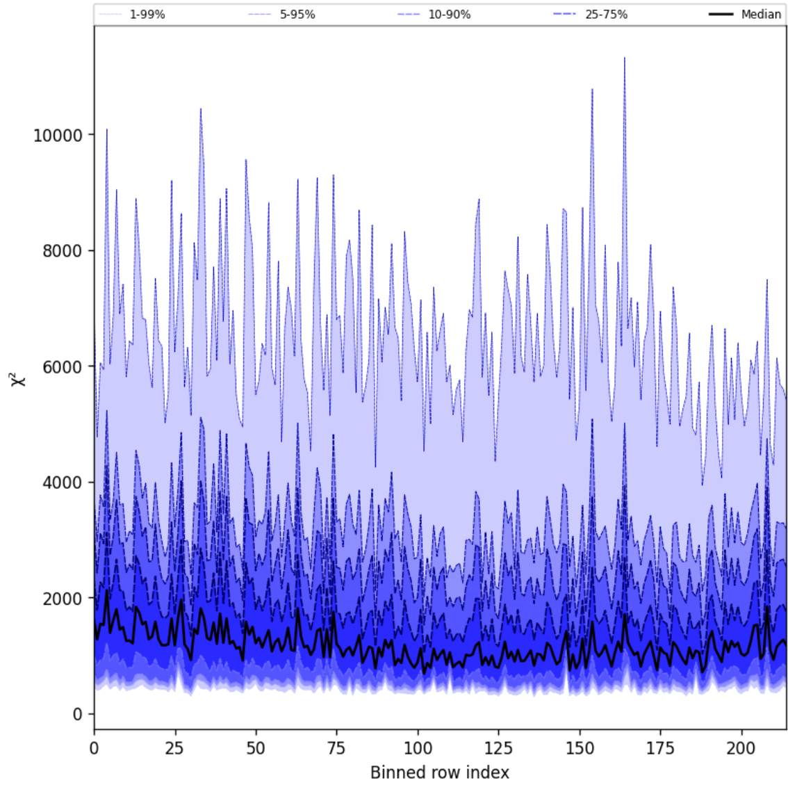
Figure 30: Along track statistics of “ \chi^2 ” for 2024-08-28 to 2024-08-30
