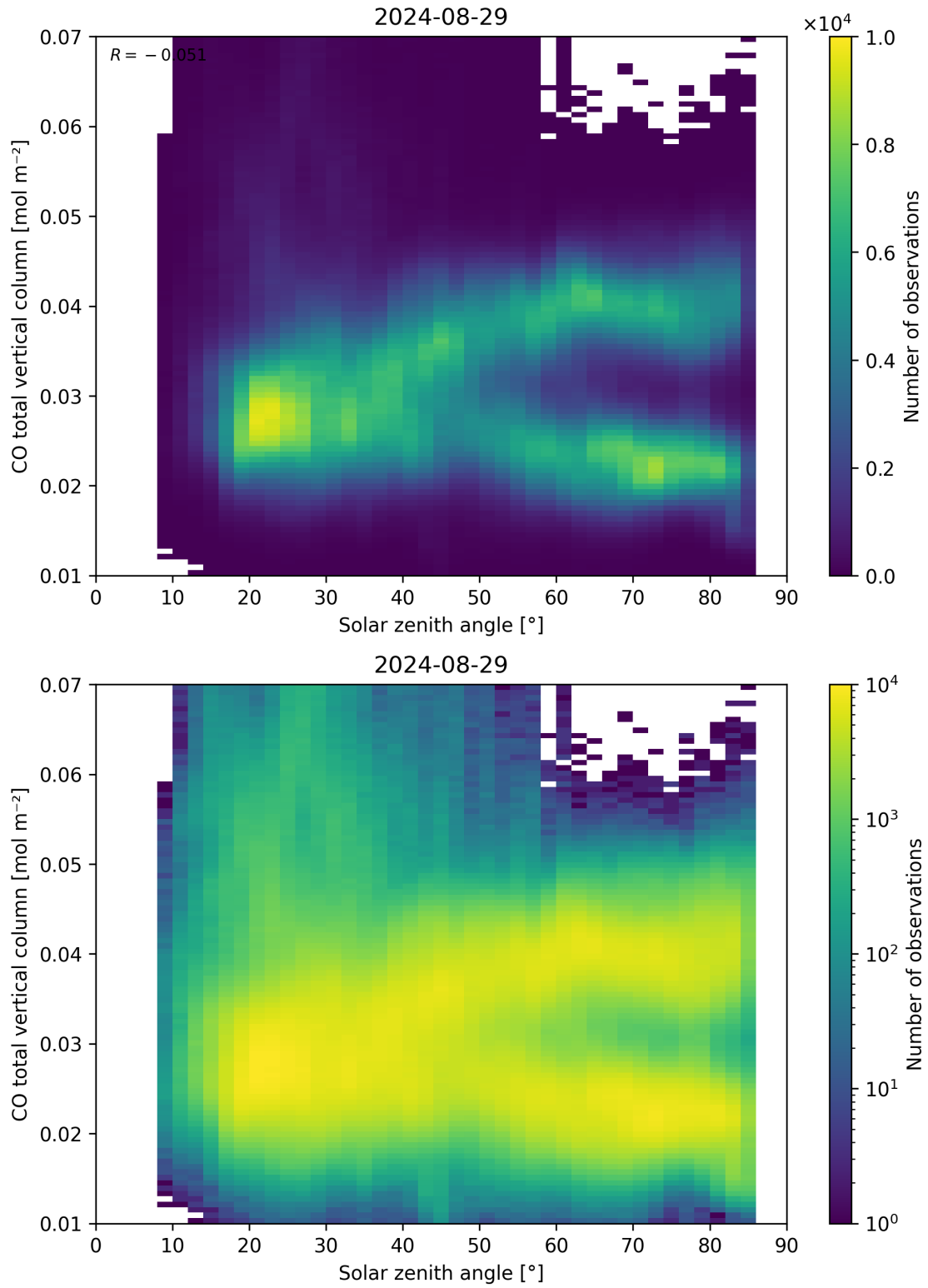
Figure 61: Scatter density plot of “Solar zenith angle” against “CO total vertical column” for 2024-08-28 to 2024-08-30.
