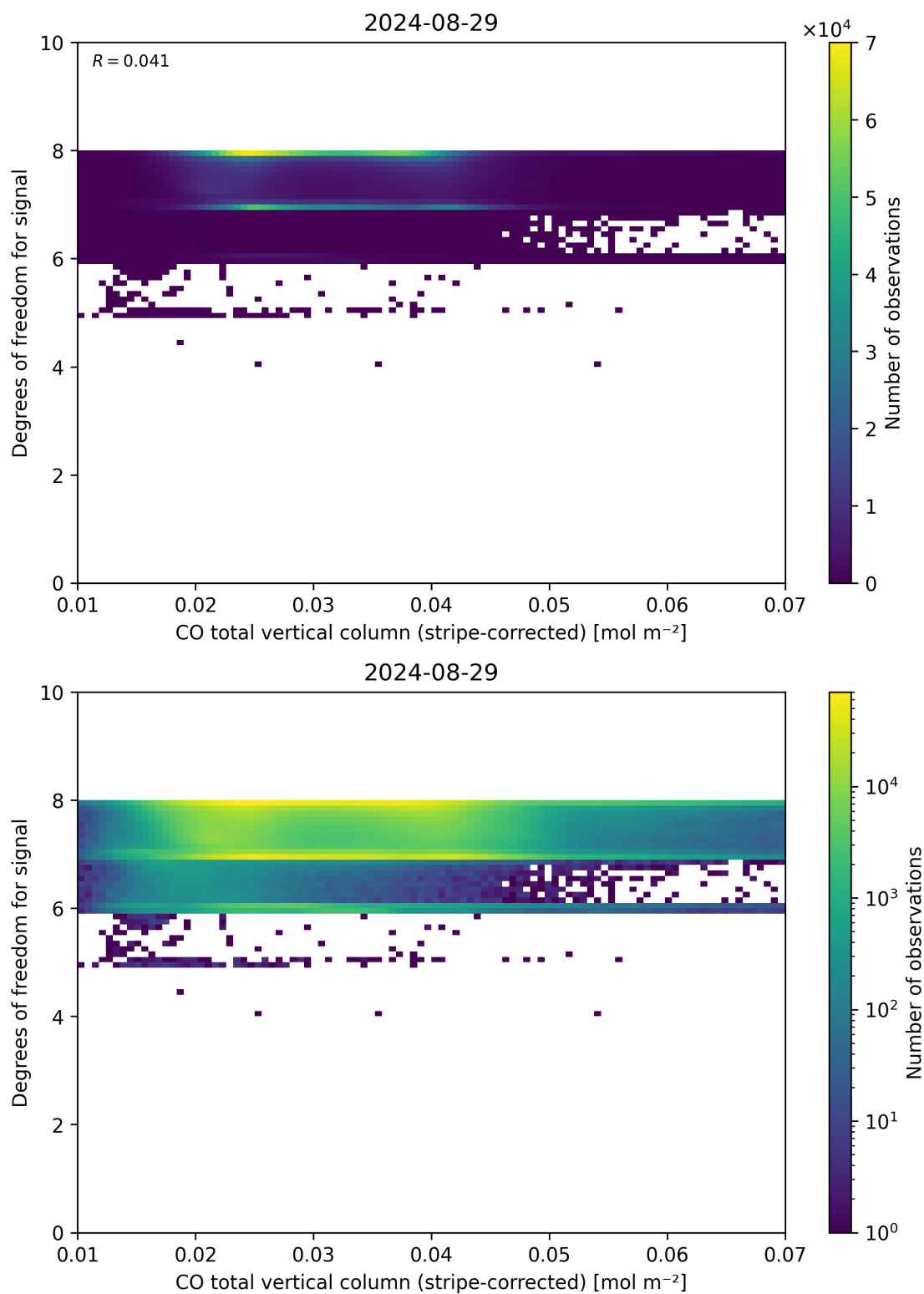
Figure 38: Scatter density plot of “CO total vertical column (stripe-corrected)” against “Degrees of freedom for signal” for 2024-08-28 to 2024-08-30.
