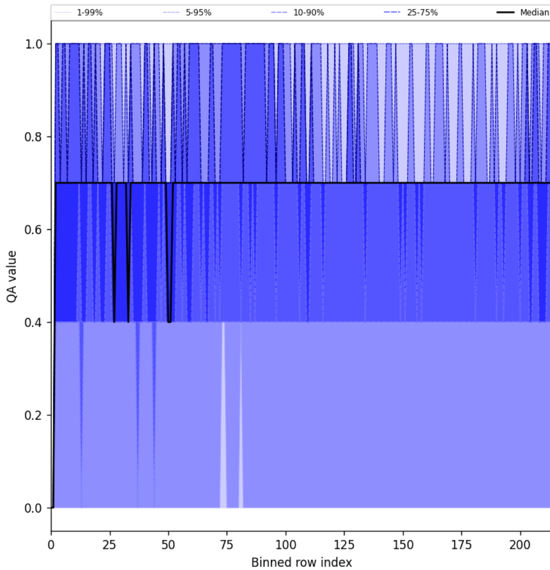
Figure 25: Along track statistics of “QA value” for 2024-08-28 to 2024-08-30
