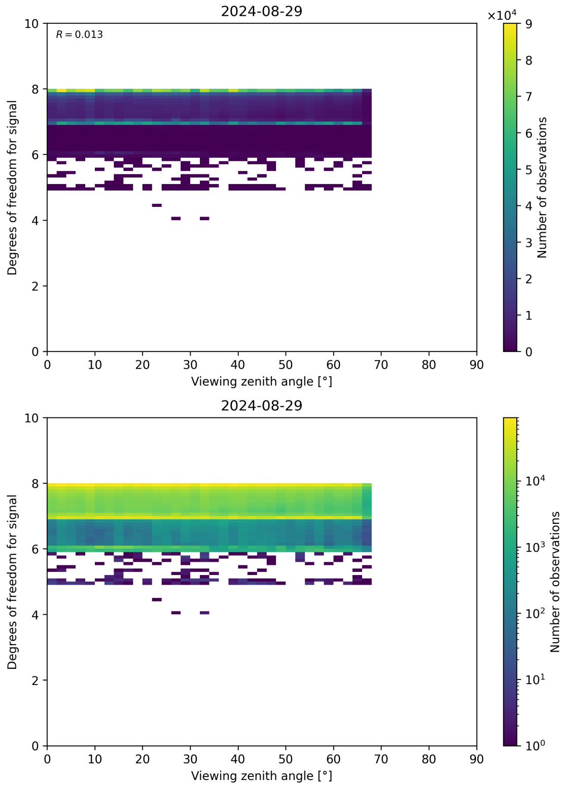
Figure 73: Scatter density plot of “Viewing zenith angle” against “Degrees of freedom for signal” for 2024-08-28 to 2024-08-30.
