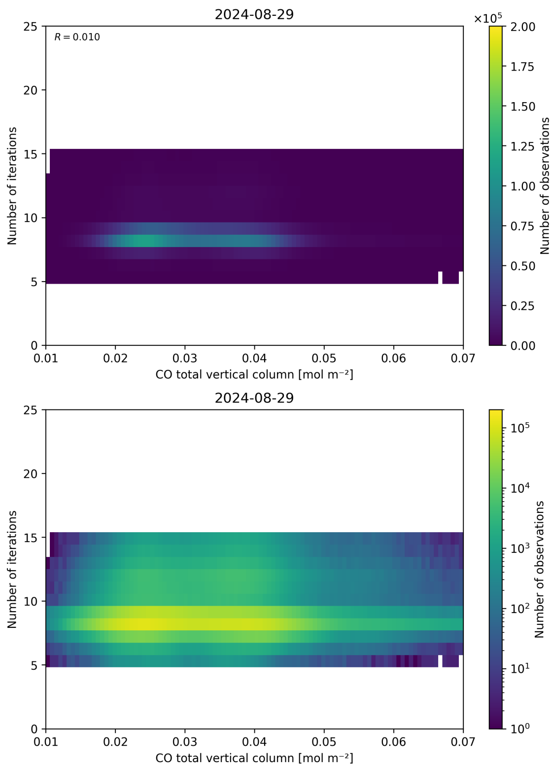
Figure 42: Scatter density plot of “CO total vertical column” against “Number of iterations” for 2024-08-28 to 2024-08-30.
