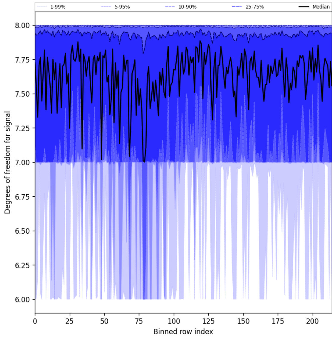
Figure 31: Along track statistics of “Degrees of freedom for signal” for 2024-08-29 to 2024-08-31
