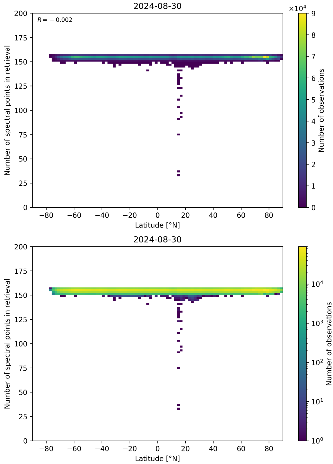
Figure 57: Scatter density plot of “Latitude” against “Number of spectral points in retrieval” for 2024-08-29 to 2024-08-31.
