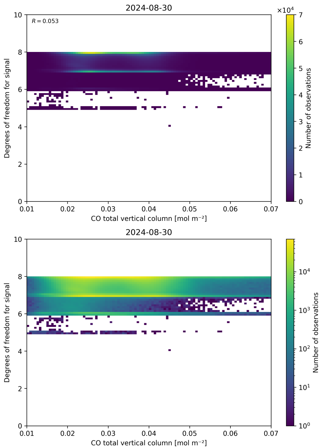
Figure 41: Scatter density plot of “CO total vertical column” against “Degrees of freedom for signal” for 2024-08-29 to 2024-08-31.
