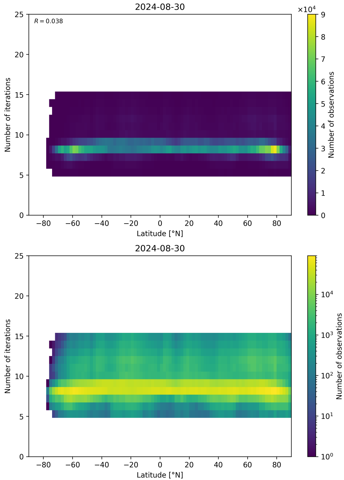
Figure 56: Scatter density plot of “Latitude” against “Number of iterations” for 2024-08-29 to 2024-08-31.
