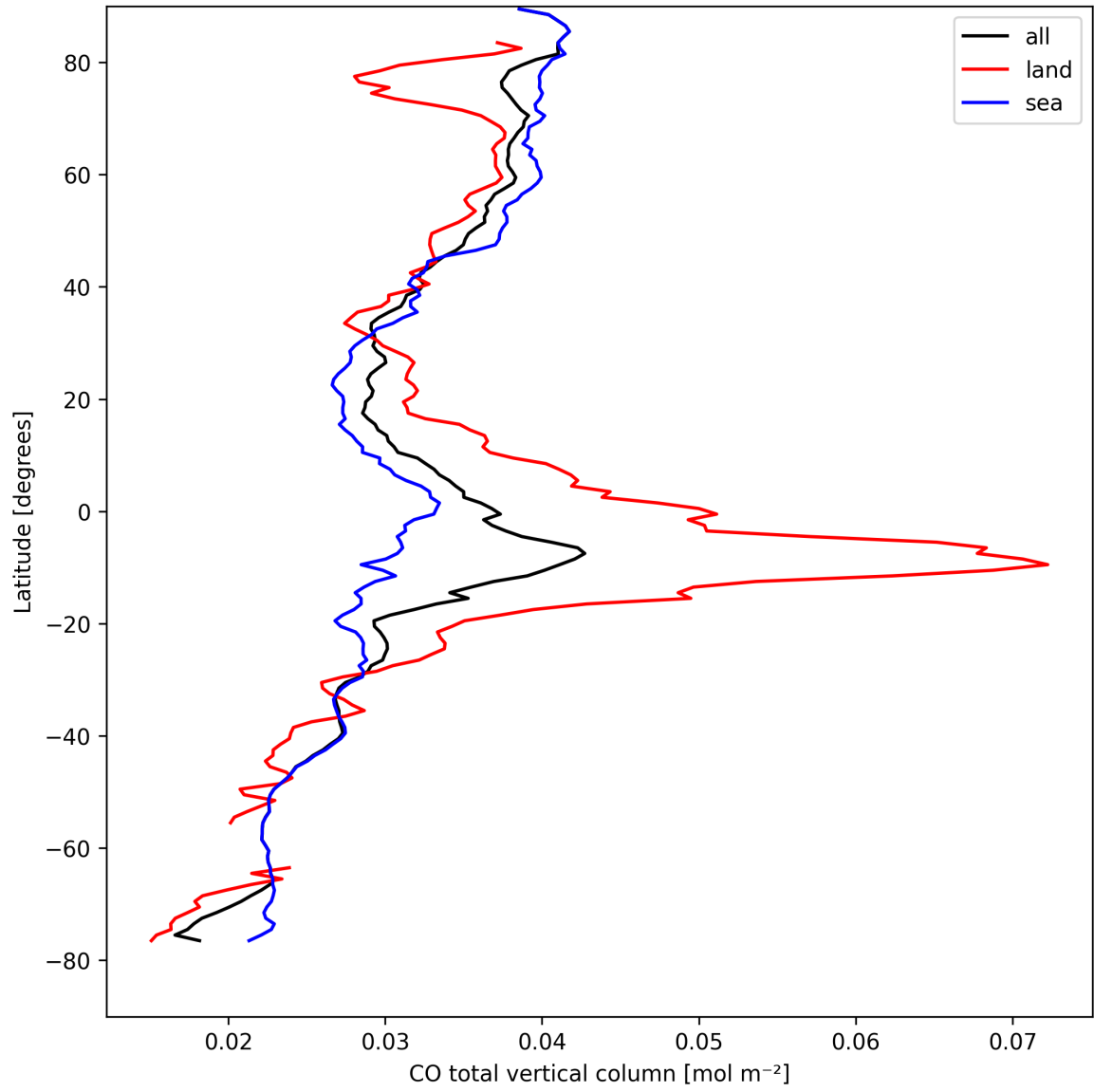
Figure 10: Zonal average of “CO total vertical column” for 2024-08-29 to 2024-08-31.
