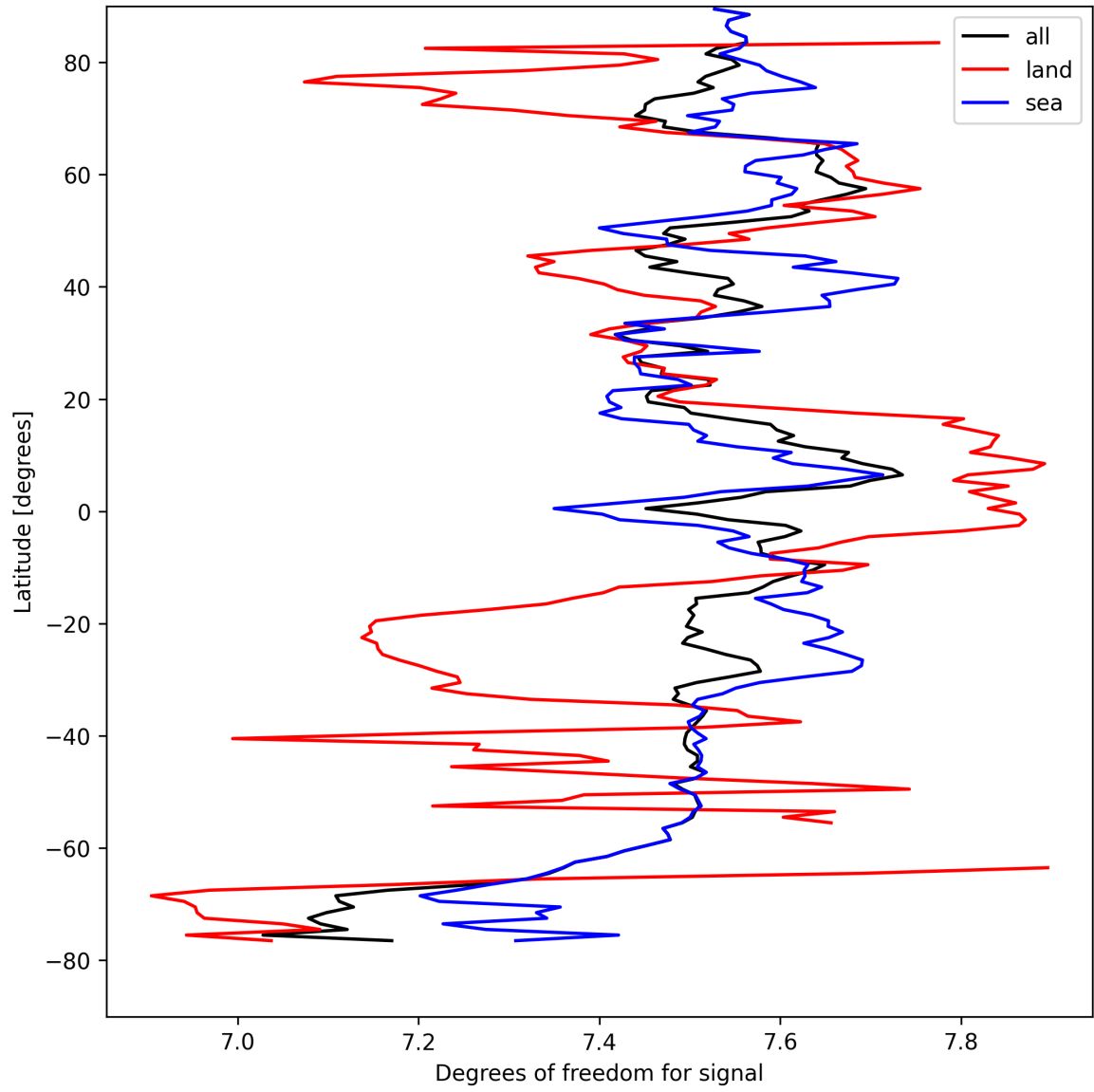
Figure 15: Zonal average of “Degrees of freedom for signal” for 2024-08-29 to 2024-08-31.
