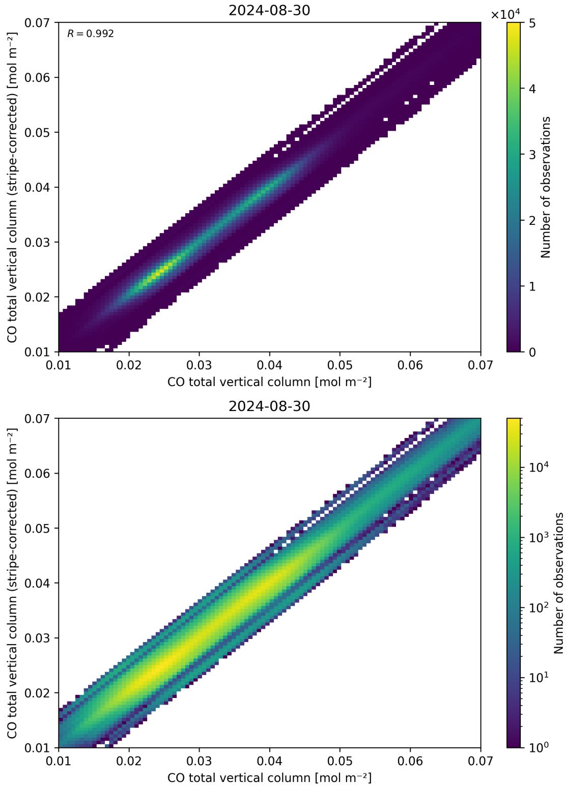
Figure 33: Scatter density plot of “CO total vertical column” against “CO total vertical column (stripe-corrected)” for 2024-08-29 to 2024-08-31.
