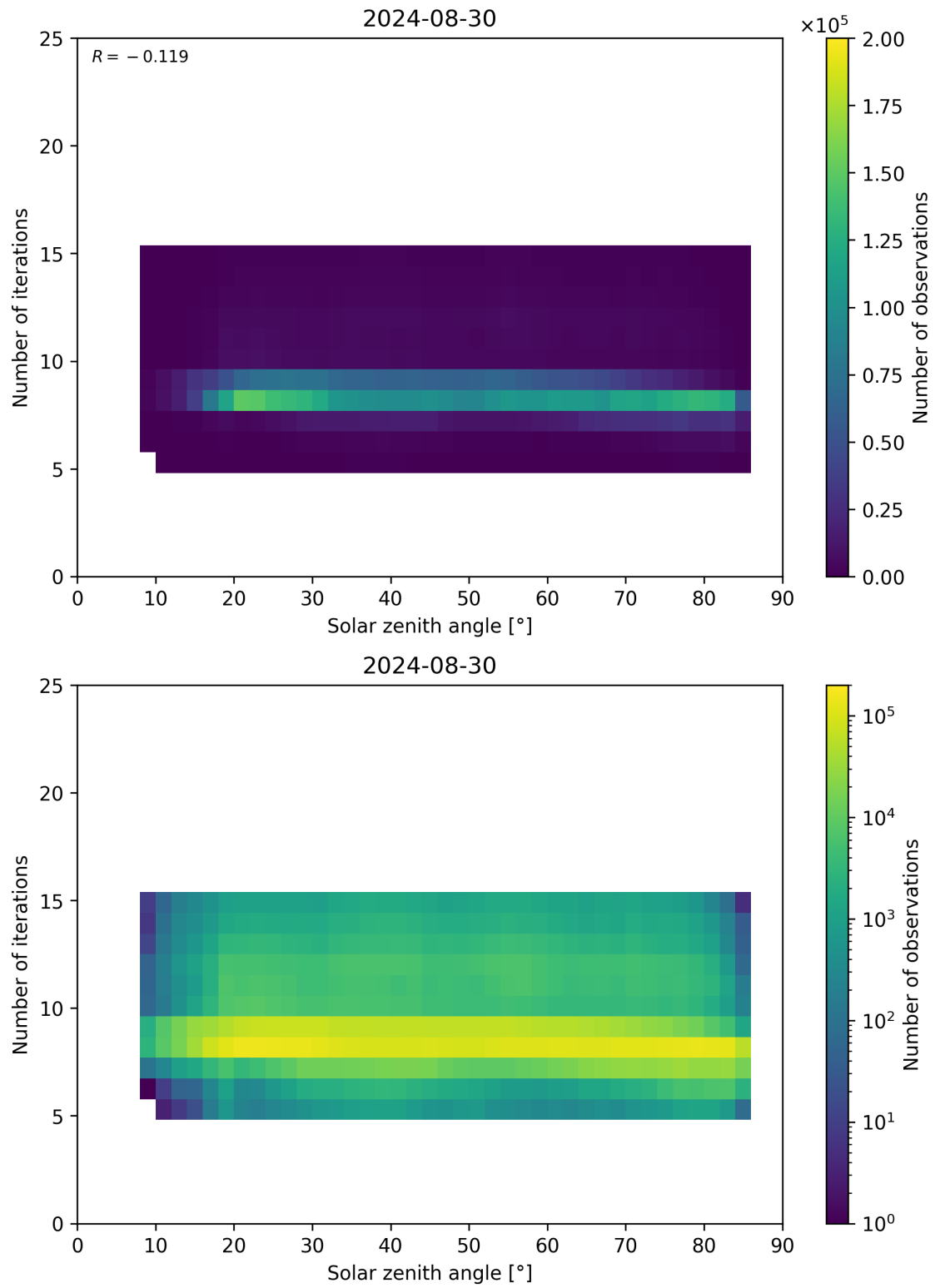
Figure 67: Scatter density plot of “Solar zenith angle” against “Number of iterations” for 2024-08-29 to 2024-08-31.
