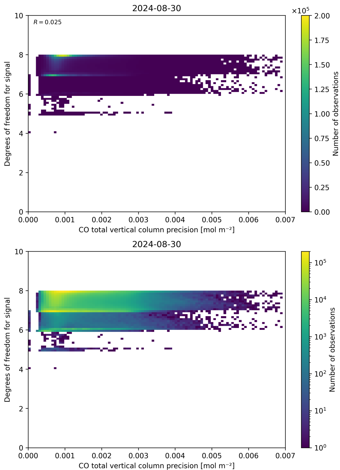
Figure 45: Scatter density plot of “CO total vertical column precision” against “Degrees of freedom for signal” for 2024-08-29 to 2024-08-31.
