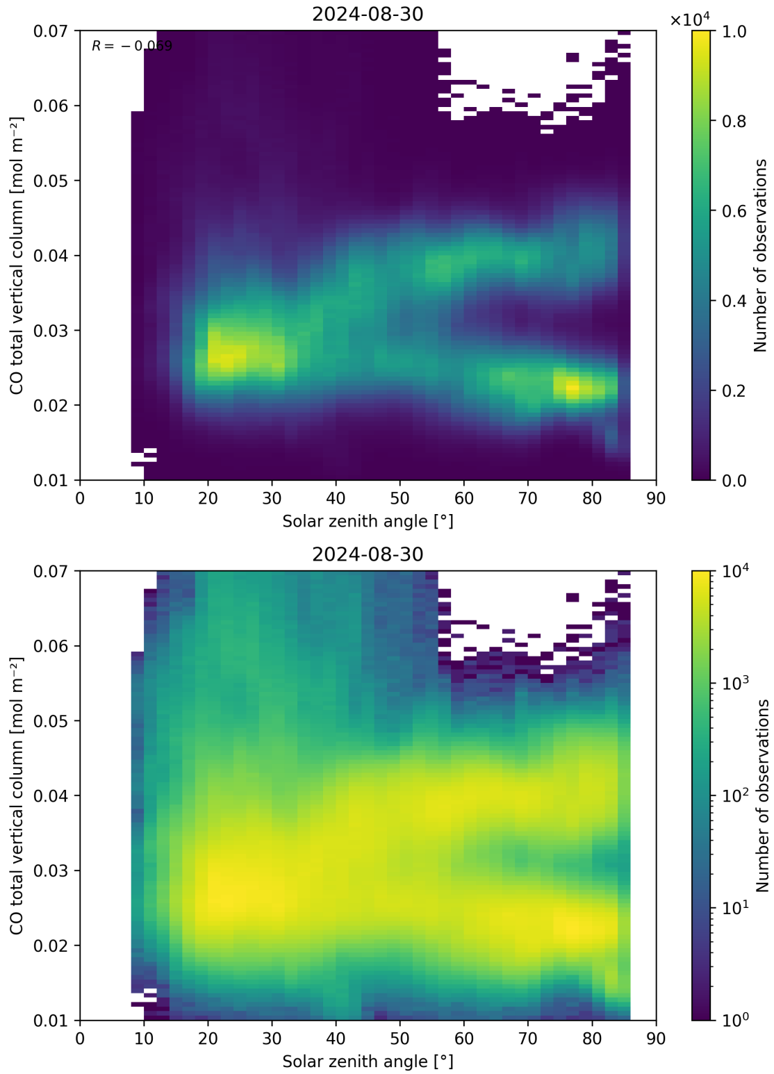
Figure 61: Scatter density plot of “Solar zenith angle” against “CO total vertical column” for 2024-08-29 to 2024-08-31.
