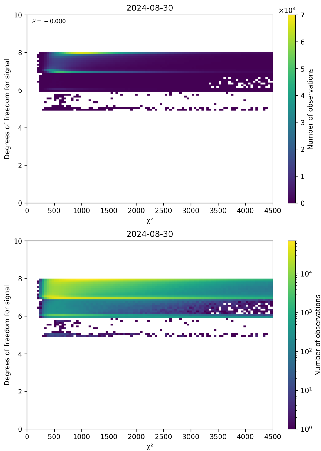
Figure 48: Scatter density plot of “ \chi^2 ” against “Degrees of freedom for signal” for 2024-08-29 to 2024-08-31.
