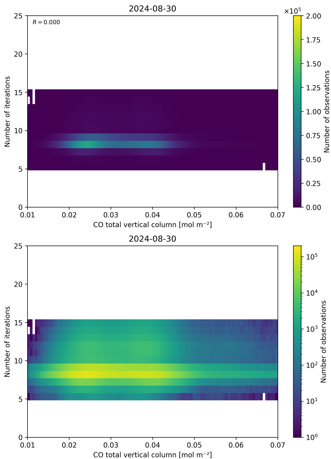
Figure 42: Scatter density plot of “CO total vertical column” against “Number of iterations” for 2024-08-29 to 2024-08-31.
