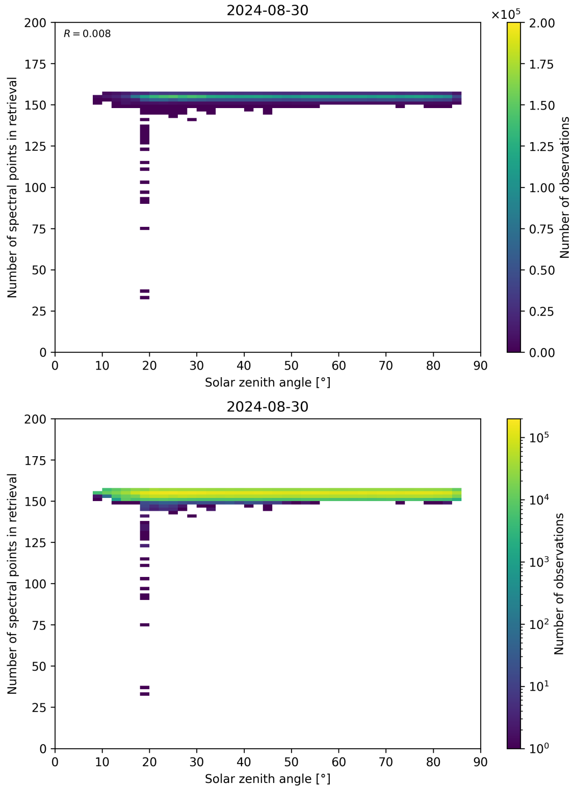
Figure 68: Scatter density plot of “Solar zenith angle” against “Number of spectral points in retrieval” for 2024-08-29 to 2024-08-31.
