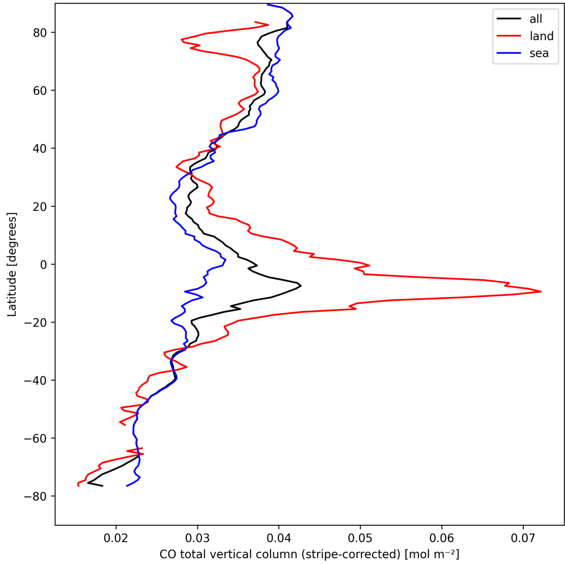
Figure 11: Zonal average of “CO total vertical column (stripe-corrected)” for 2024-08-29 to 2024-08-31.
