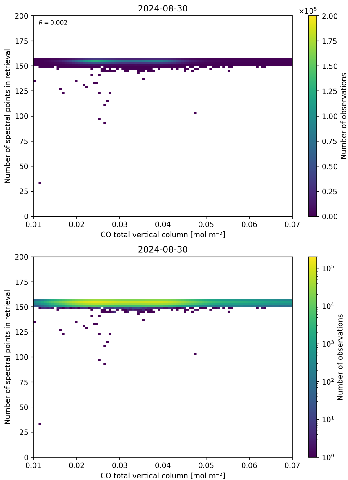
Figure 43: Scatter density plot of “CO total vertical column” against “Number of spectral points in retrieval” for 2024-08-29 to 2024-08-31.
