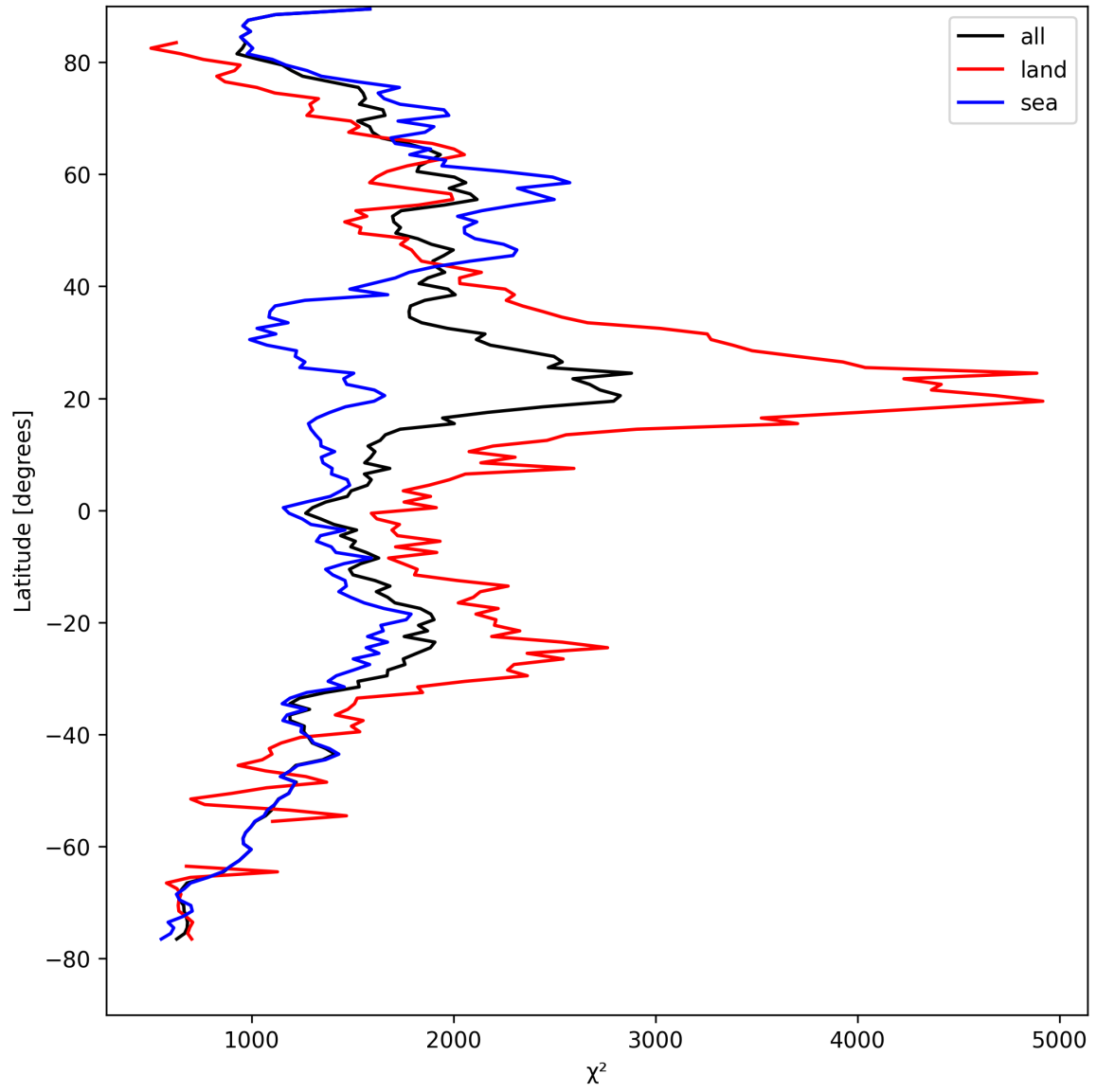
Figure 14: Zonal average of “ \chi^2 ” for 2024-08-29 to 2024-08-31.
