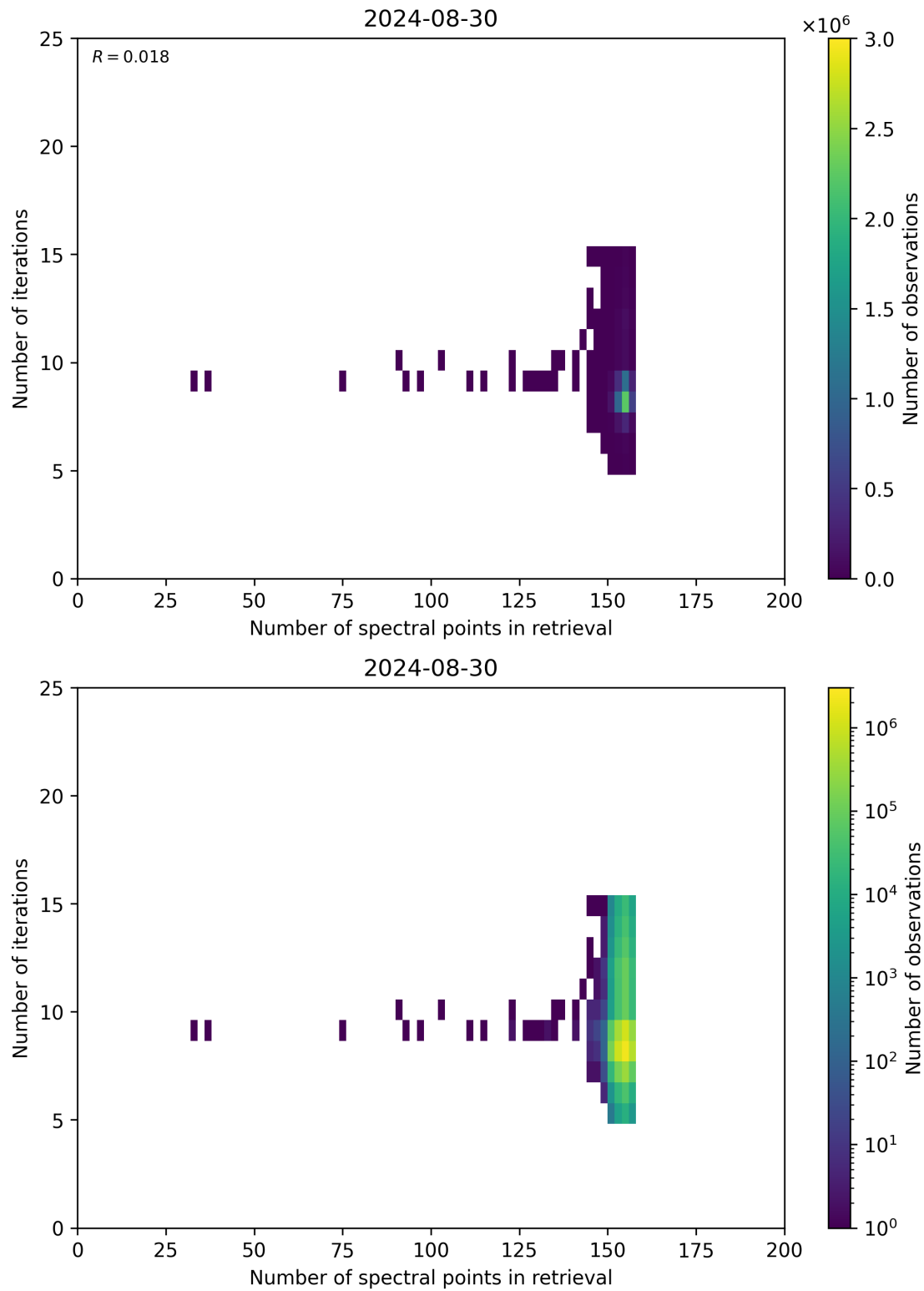
Figure 60: Scatter density plot of “Number of spectral points in retrieval” against “Number of iterations” for 2024-08-29 to 2024-08-31.
