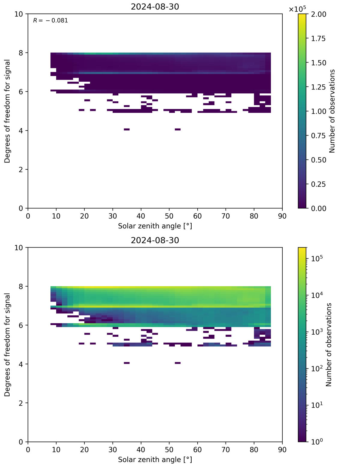
Figure 65: Scatter density plot of “Solar zenith angle” against “Degrees of freedom for signal” for 2024-08-29 to 2024-08-31.
