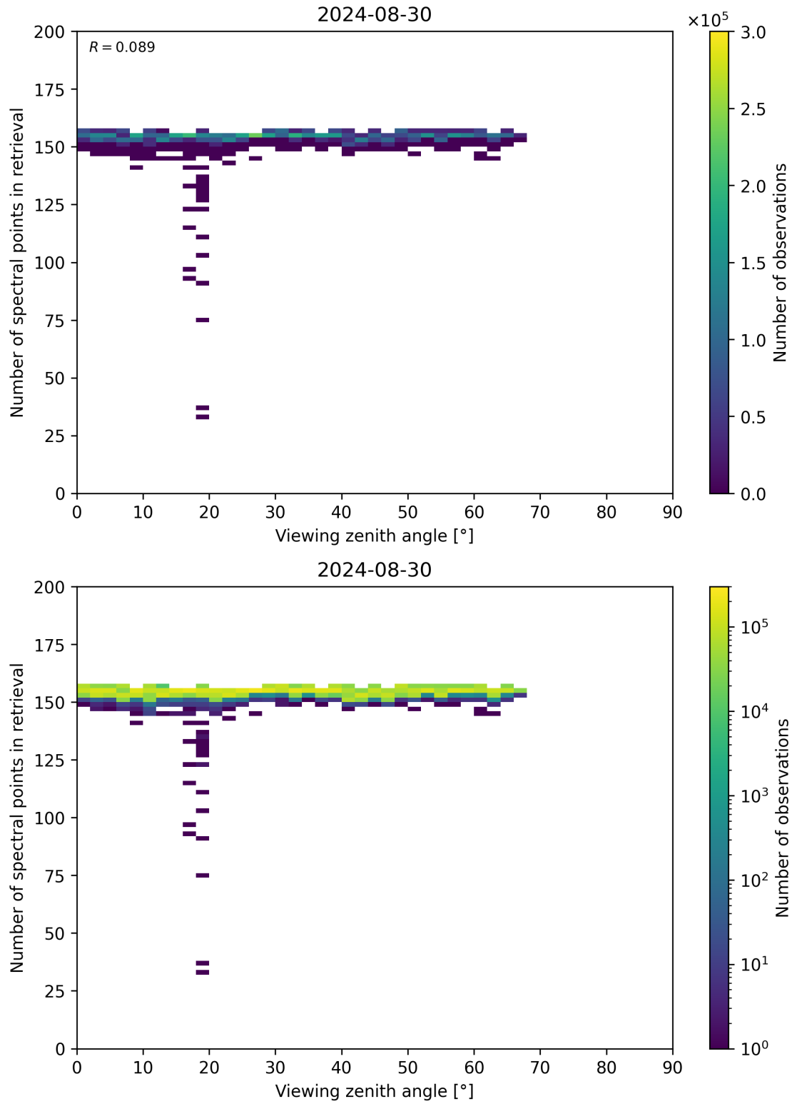
Figure 76: Scatter density plot of “Viewing zenith angle” against “Number of spectral points in retrieval” for 2024-08-29 to 2024-08-31.
