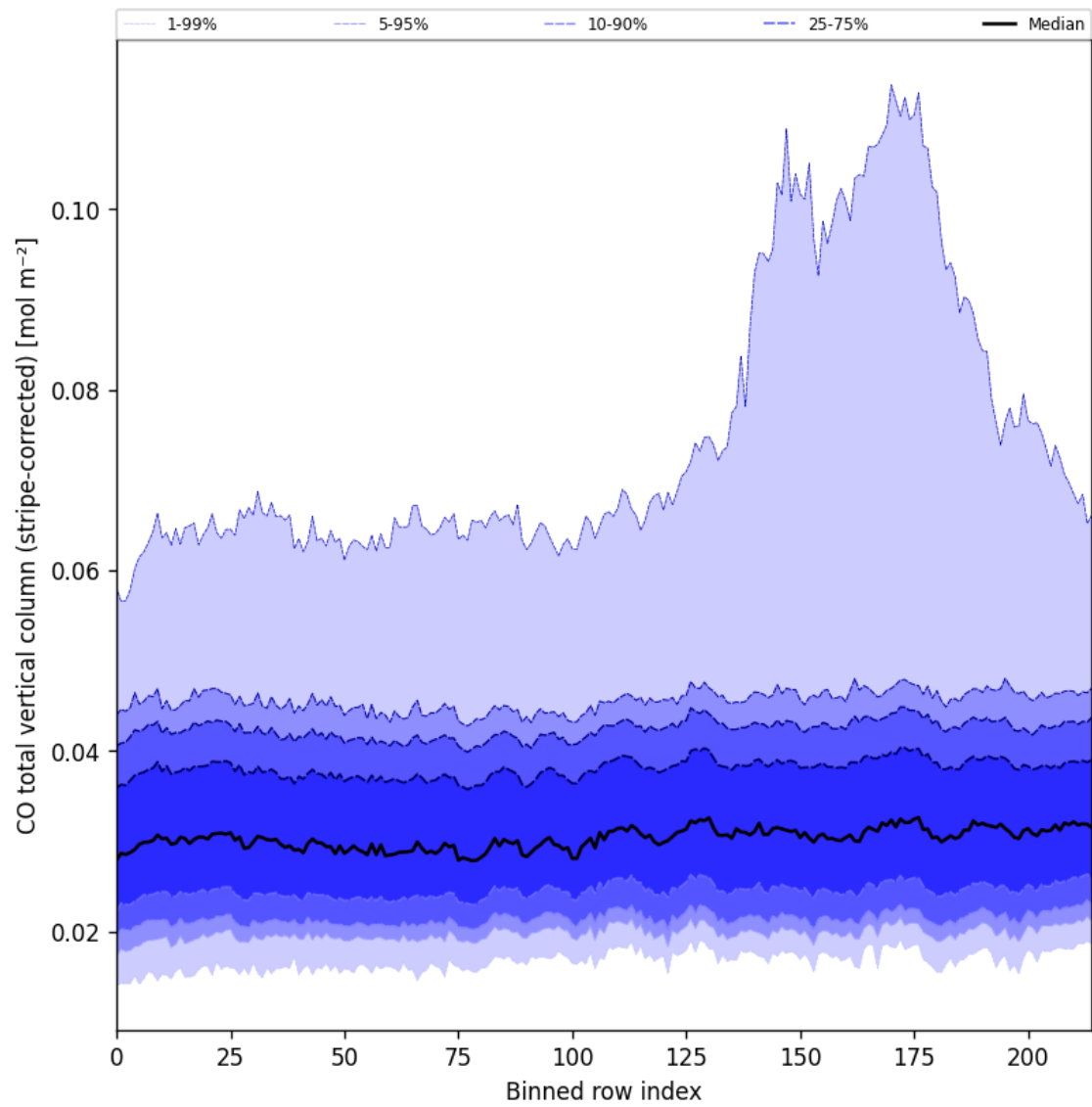
Figure 27: Along track statistics of “CO total vertical column (stripe-corrected)” for 2024-08-29 to 2024-08-31
