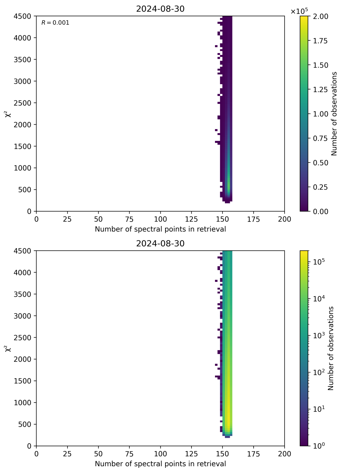
Figure 58: Scatter density plot of “Number of spectral points in retrieval” against “ \chi^2 ” for 2024-08-29 to 2024-08-31.
