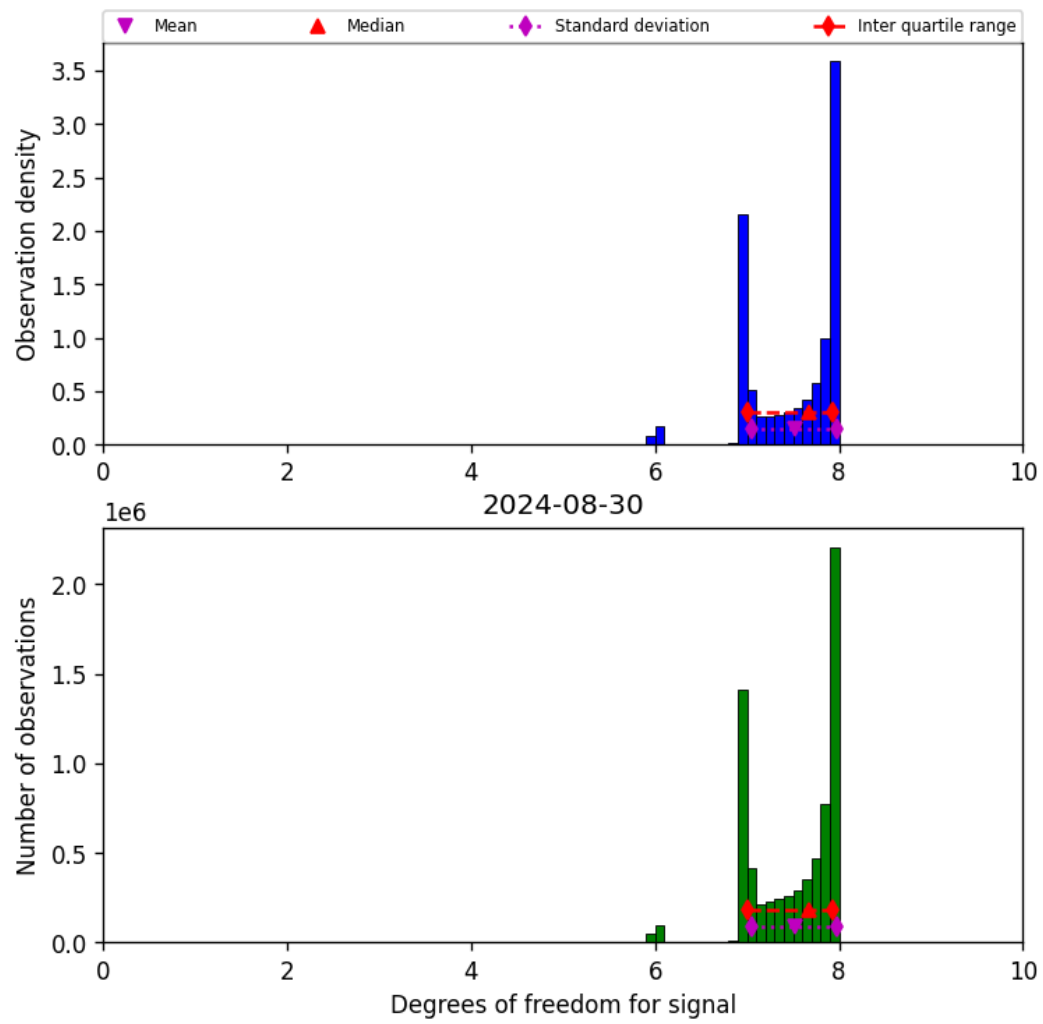
Figure 23: Histogram of “Degrees of freedom for signal” for 2024-08-29 to 2024-08-31
