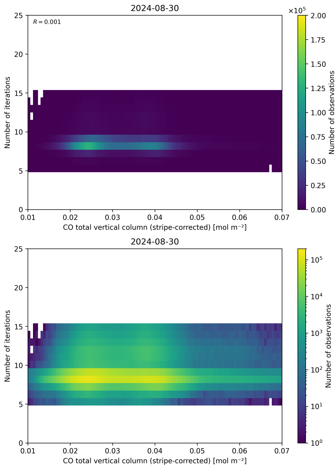
Figure 39: Scatter density plot of “CO total vertical column (stripe-corrected)” against “Number of iterations” for 2024-08-29 to 2024-08-31.
