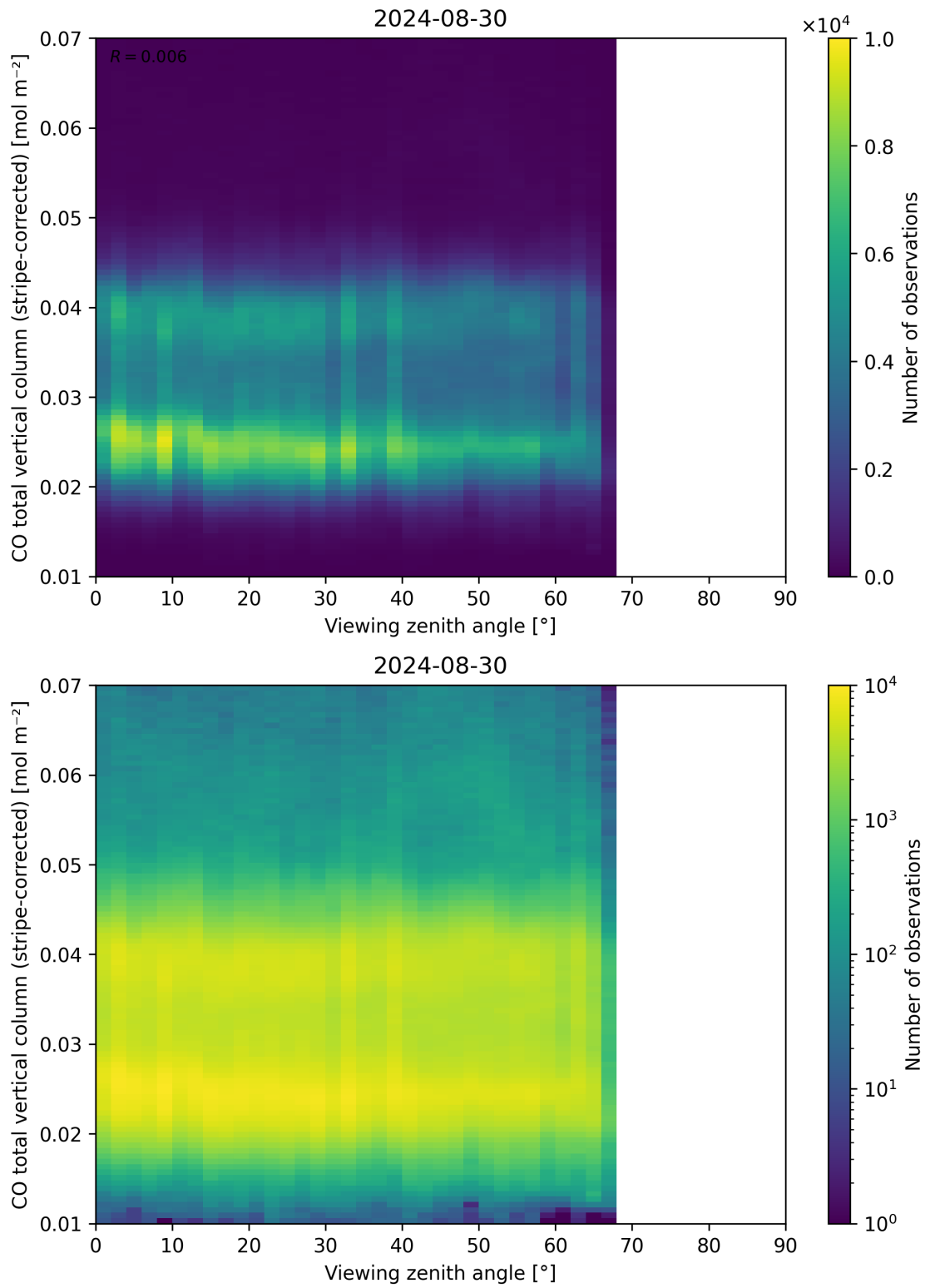
Figure 70: Scatter density plot of “Viewing zenith angle” against “CO total vertical column (stripe-corrected)” for 2024-08-29 to 2024-08-31.
