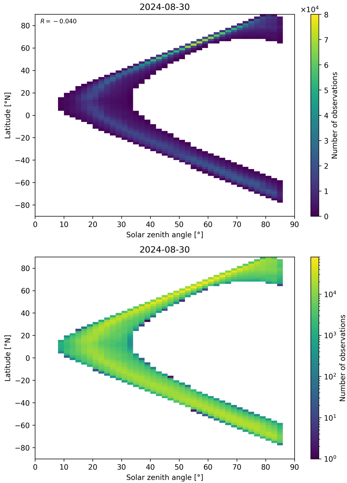
Figure 66: Scatter density plot of “Solar zenith angle” against “Latitude” for 2024-08-29 to 2024-08-31.
