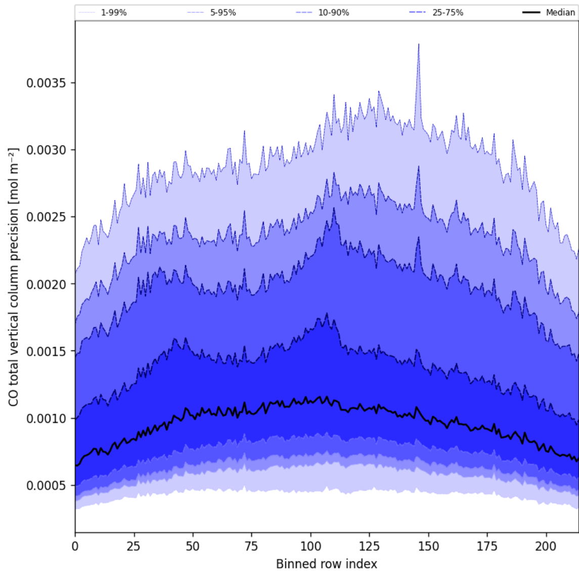
Figure 28: Along track statistics of “CO total vertical column precision” for 2024-08-29 to 2024-08-31
