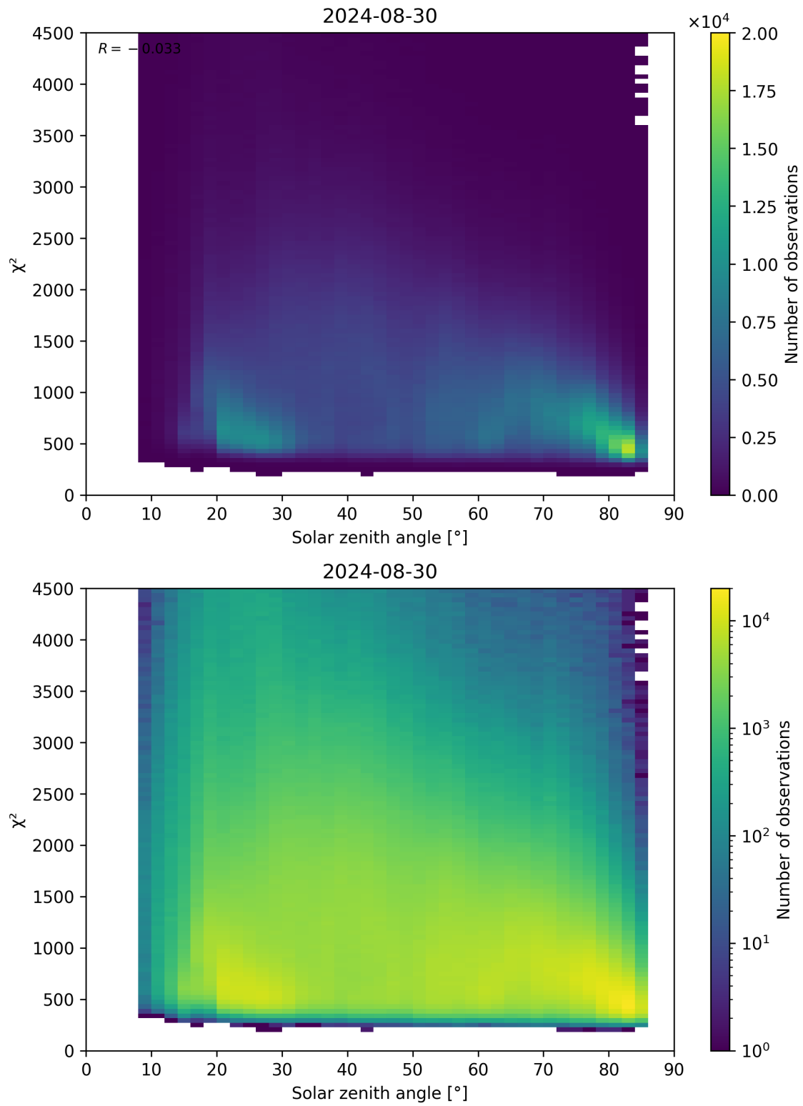
Figure 64: Scatter density plot of “Solar zenith angle” against “ \chi^2 ” for 2024-08-29 to 2024-08-31.
