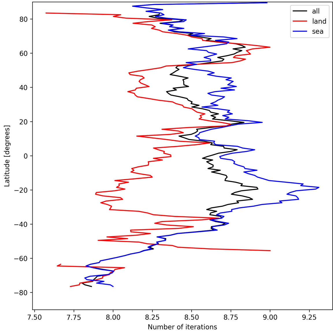
Figure 16: Zonal average of “Number of iterations” for 2024-08-29 to 2024-08-31.
