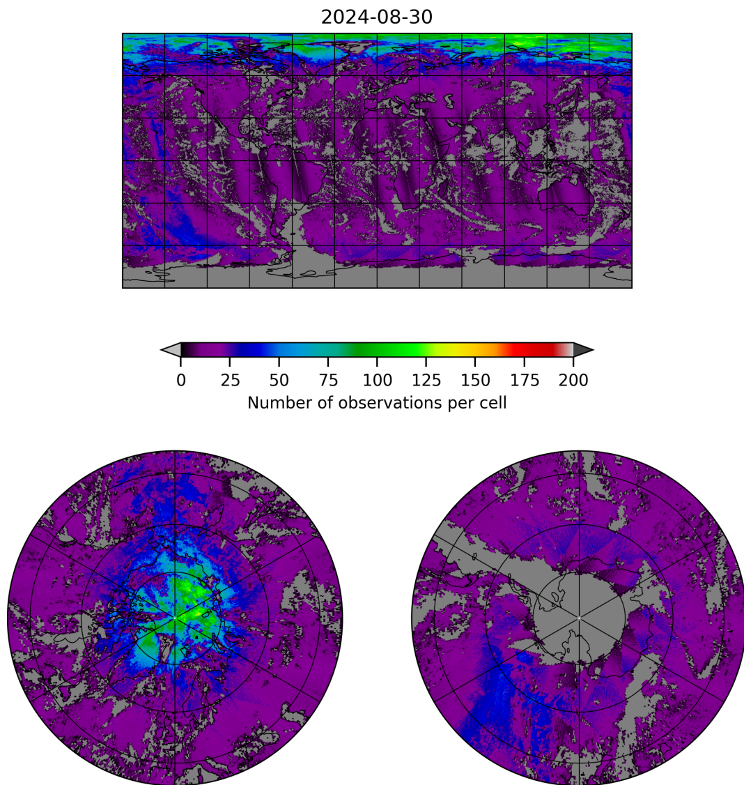
Figure 8: Map of the number of observations for 2024-08-29 to 2024-08-31
