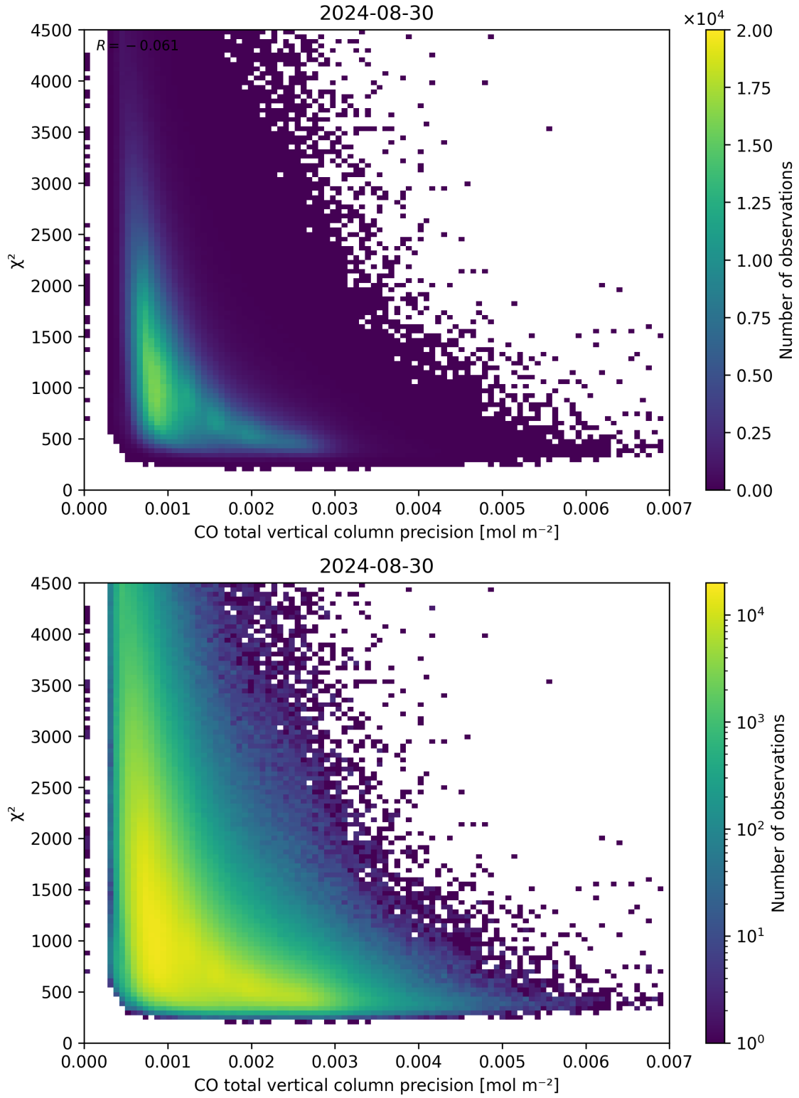
Figure 44: Scatter density plot of “CO total vertical column precision” against “ \chi^2 ” for 2024-08-29 to 2024-08-31.
