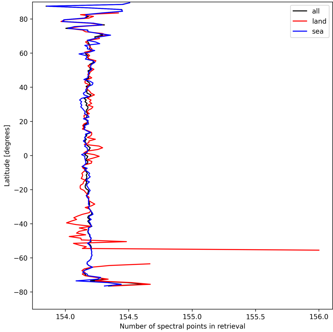
Figure 13: Zonal average of “Number of spectral points in retrieval” for 2024-08-29 to 2024-08-31.
