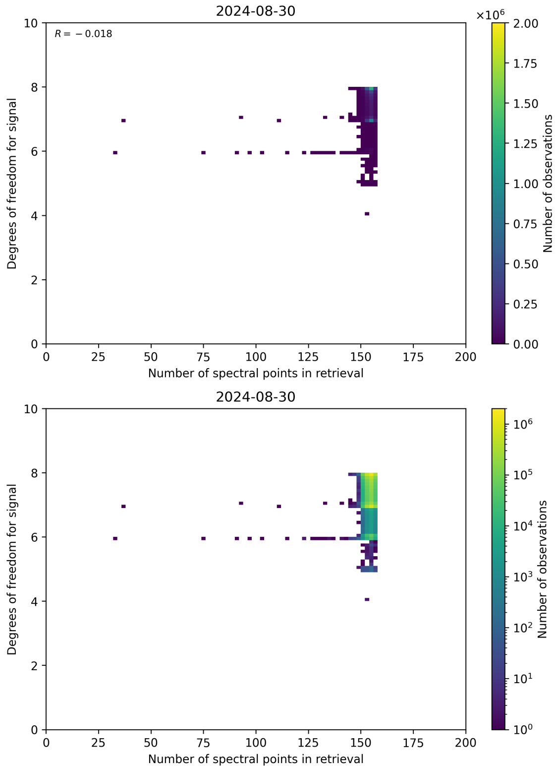
Figure 59: Scatter density plot of “Number of spectral points in retrieval” against “Degrees of freedom for signal” for 2024-08-29 to 2024-08-31.
