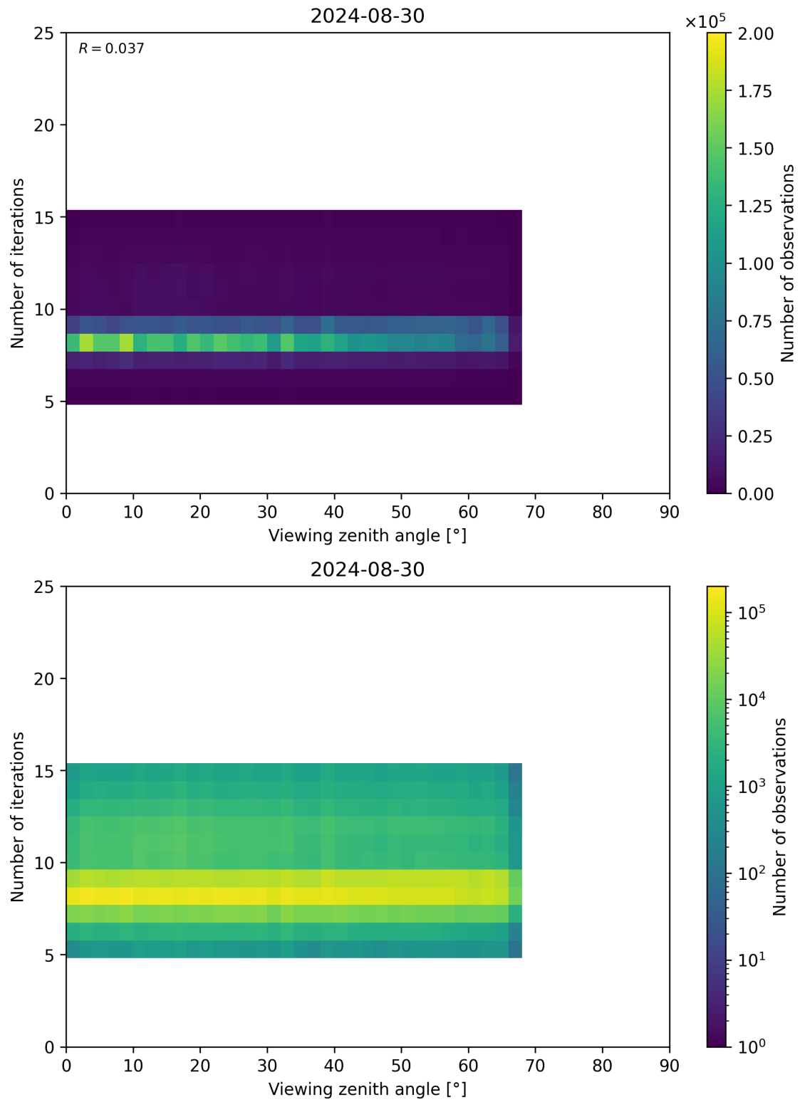
Figure 75: Scatter density plot of “Viewing zenith angle” against “Number of iterations” for 2024-08-29 to 2024-08-31.
