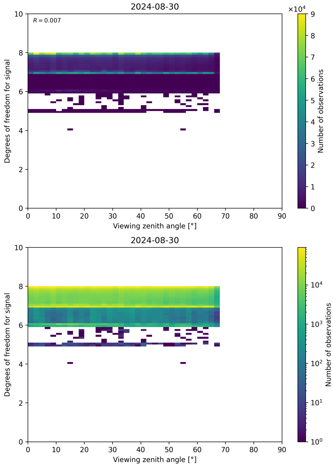
Figure 73: Scatter density plot of “Viewing zenith angle” against “Degrees of freedom for signal” for 2024-08-29 to 2024-08-31.
