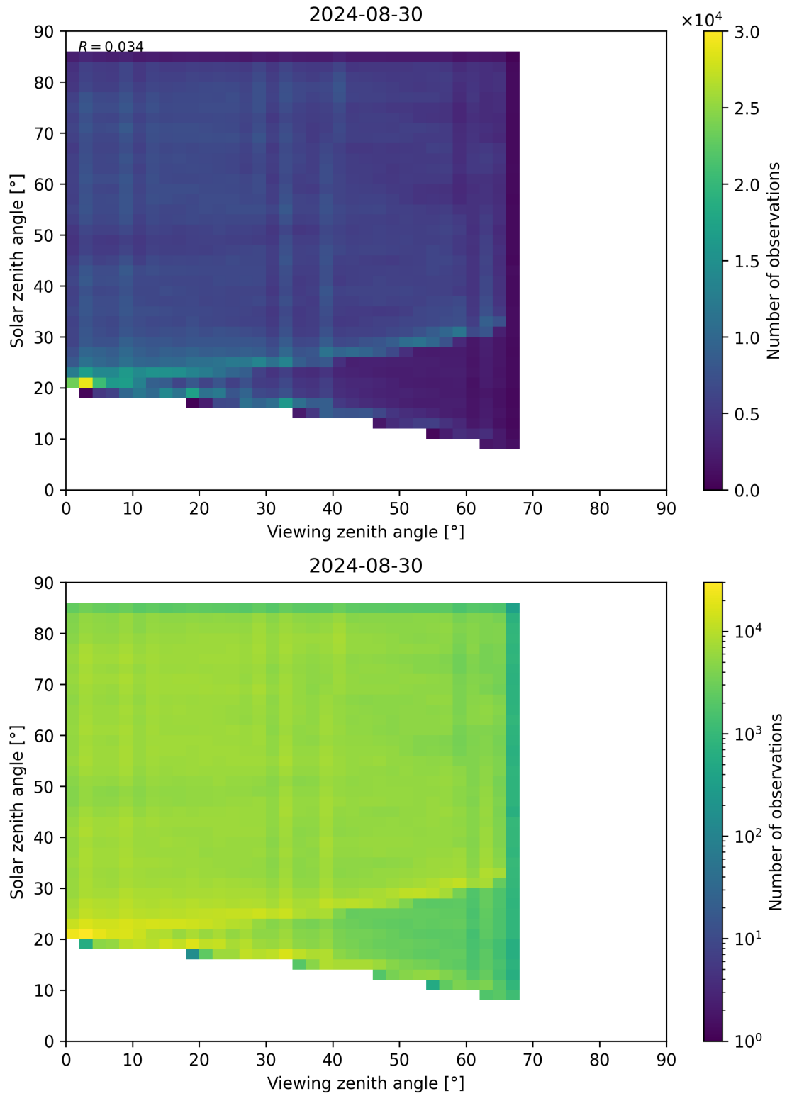
Figure 77: Scatter density plot of “Viewing zenith angle” against “Solar zenith angle” for 2024-08-29 to 2024-08-31.
