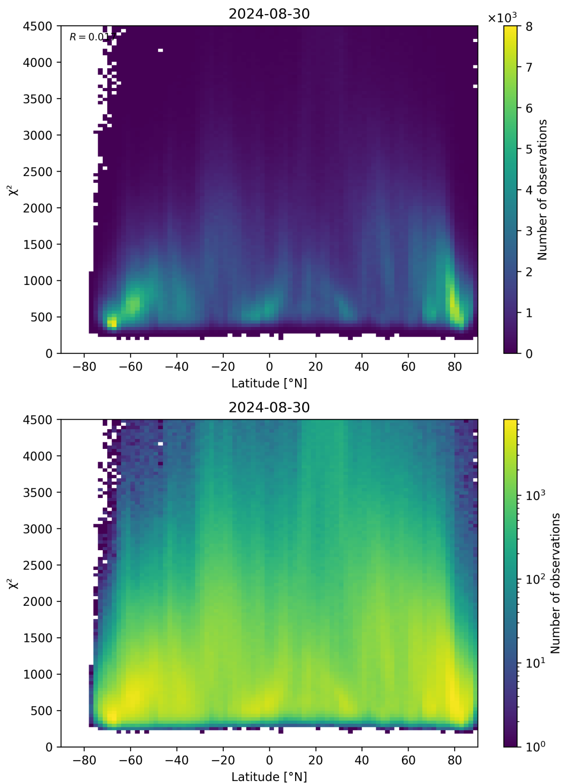
Figure 54: Scatter density plot of “Latitude” against “ \chi^2 ” for 2024-08-29 to 2024-08-31.
