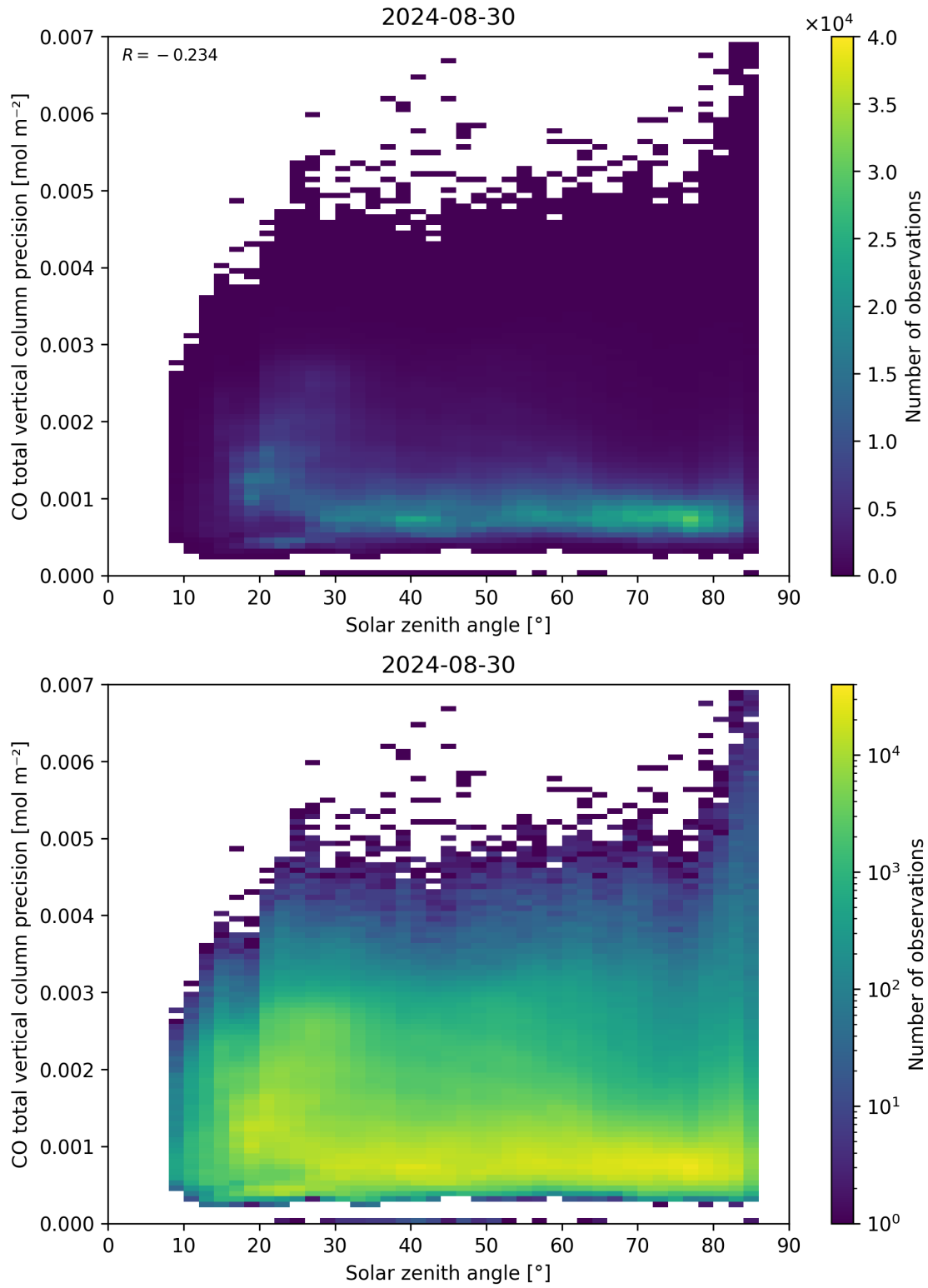
Figure 63: Scatter density plot of “Solar zenith angle” against “CO total vertical column precision” for 2024-08-29 to 2024-08-31.
