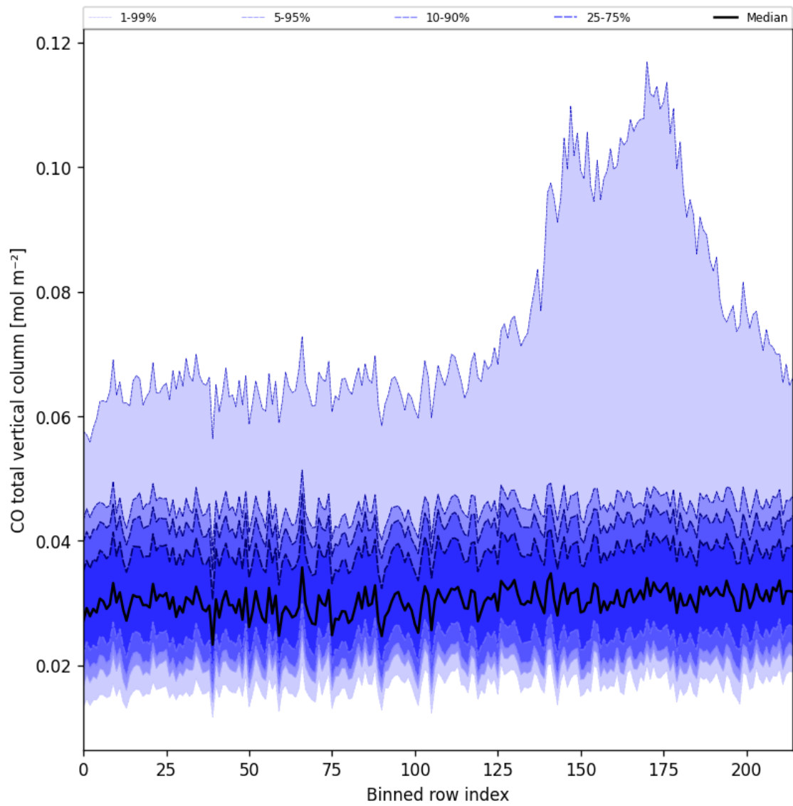
Figure 26: Along track statistics of “CO total vertical column” for 2024-08-29 to 2024-08-31
