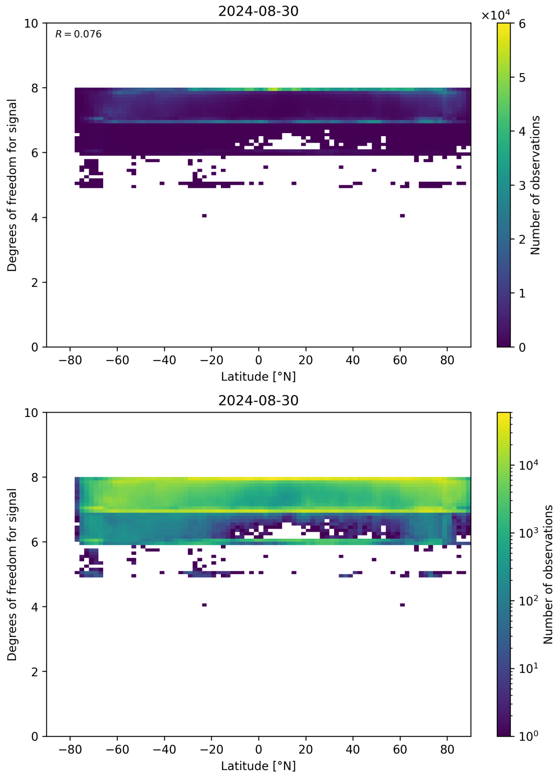
Figure 55: Scatter density plot of “Latitude” against “Degrees of freedom for signal” for 2024-08-29 to 2024-08-31.
