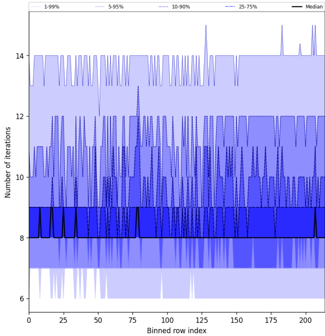
Figure 32: Along track statistics of “Number of iterations” for 2024-08-29 to 2024-08-31
