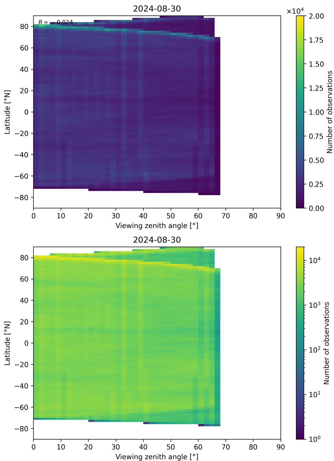
Figure 74: Scatter density plot of “Viewing zenith angle” against “Latitude” for 2024-08-29 to 2024-08-31.
