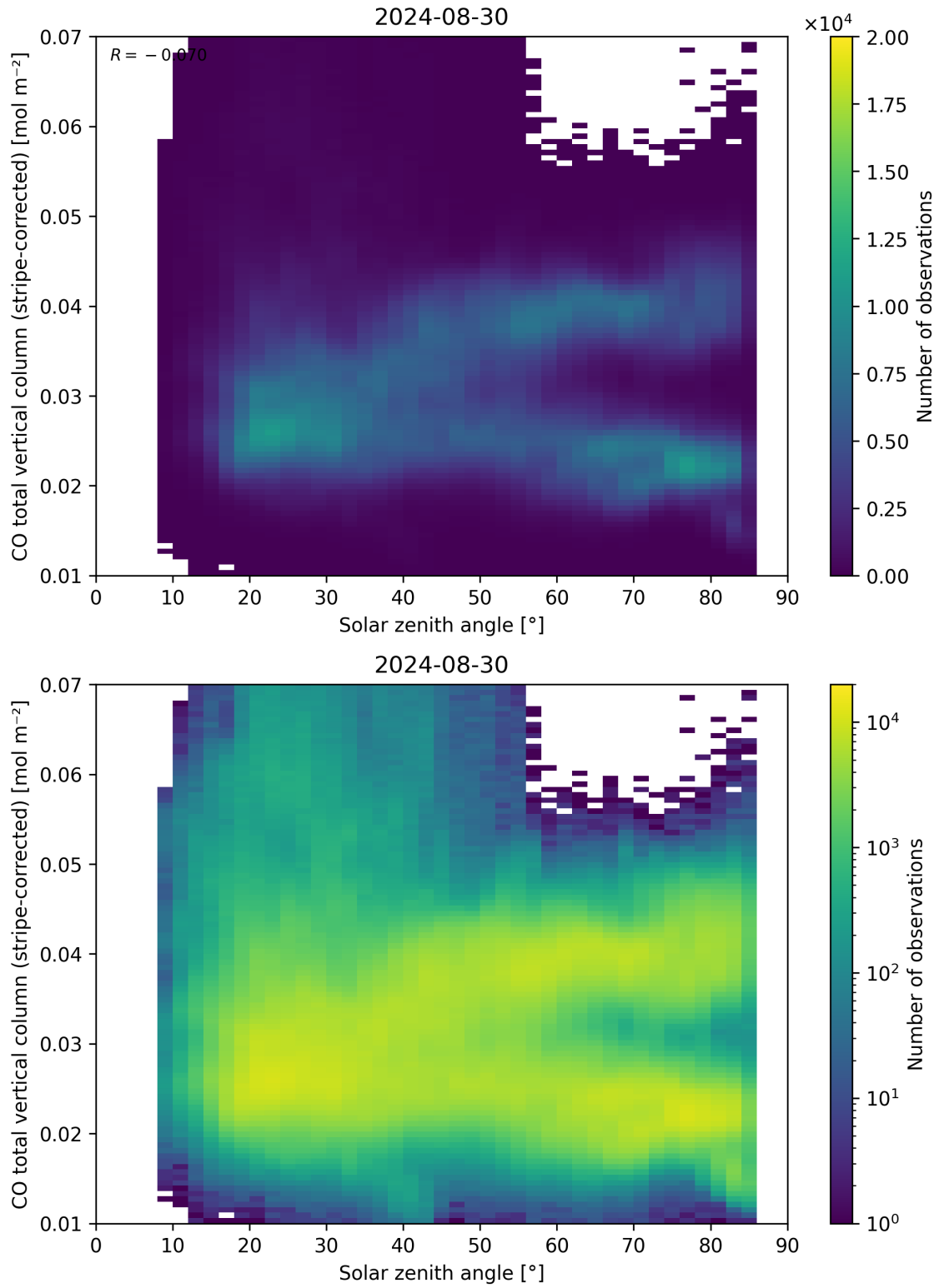
Figure 62: Scatter density plot of “Solar zenith angle” against “CO total vertical column (stripe-corrected)” for 2024-08-29 to 2024-08-31.
