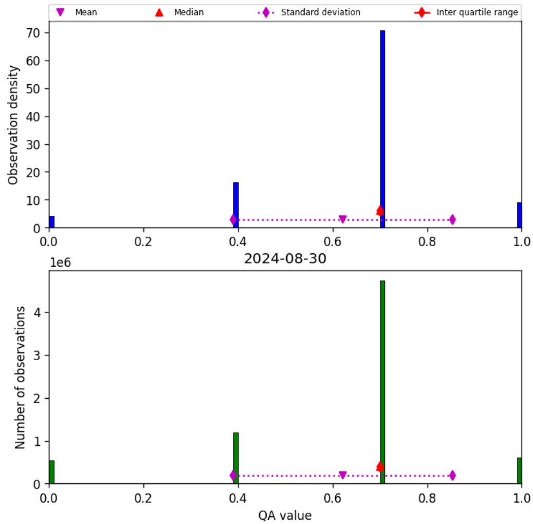
Figure 17: Histogram of “QA value” for 2024-08-29 to 2024-08-31
