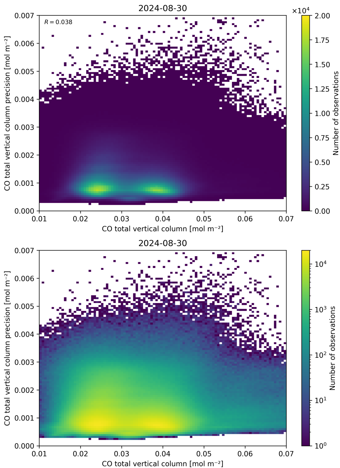
Figure 34: Scatter density plot of “CO total vertical column” against “CO total vertical column precision” for 2024-08-29 to 2024-08-31.
