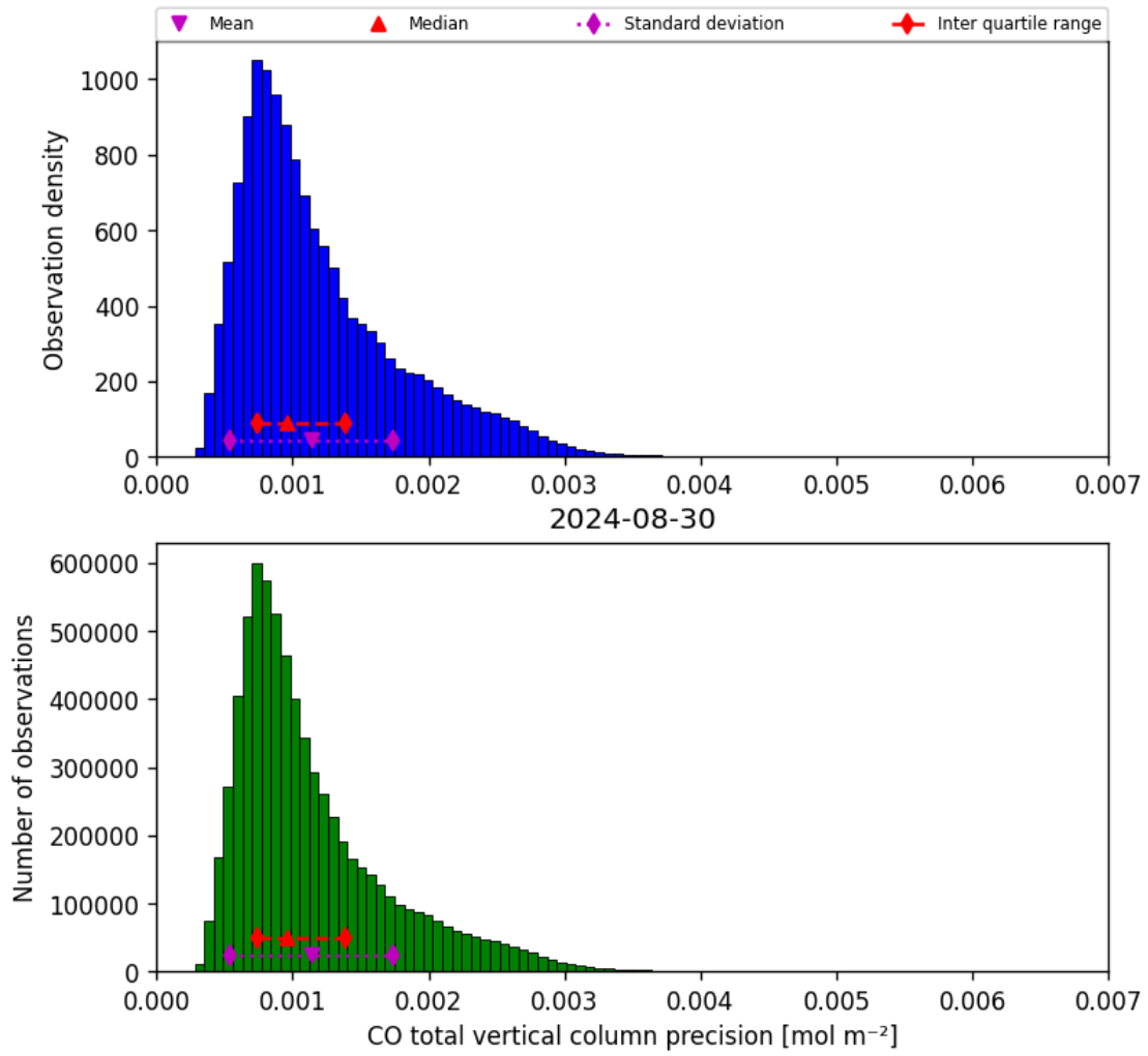
Figure 20: Histogram of “CO total vertical column precision” for 2024-08-29 to 2024-08-31
