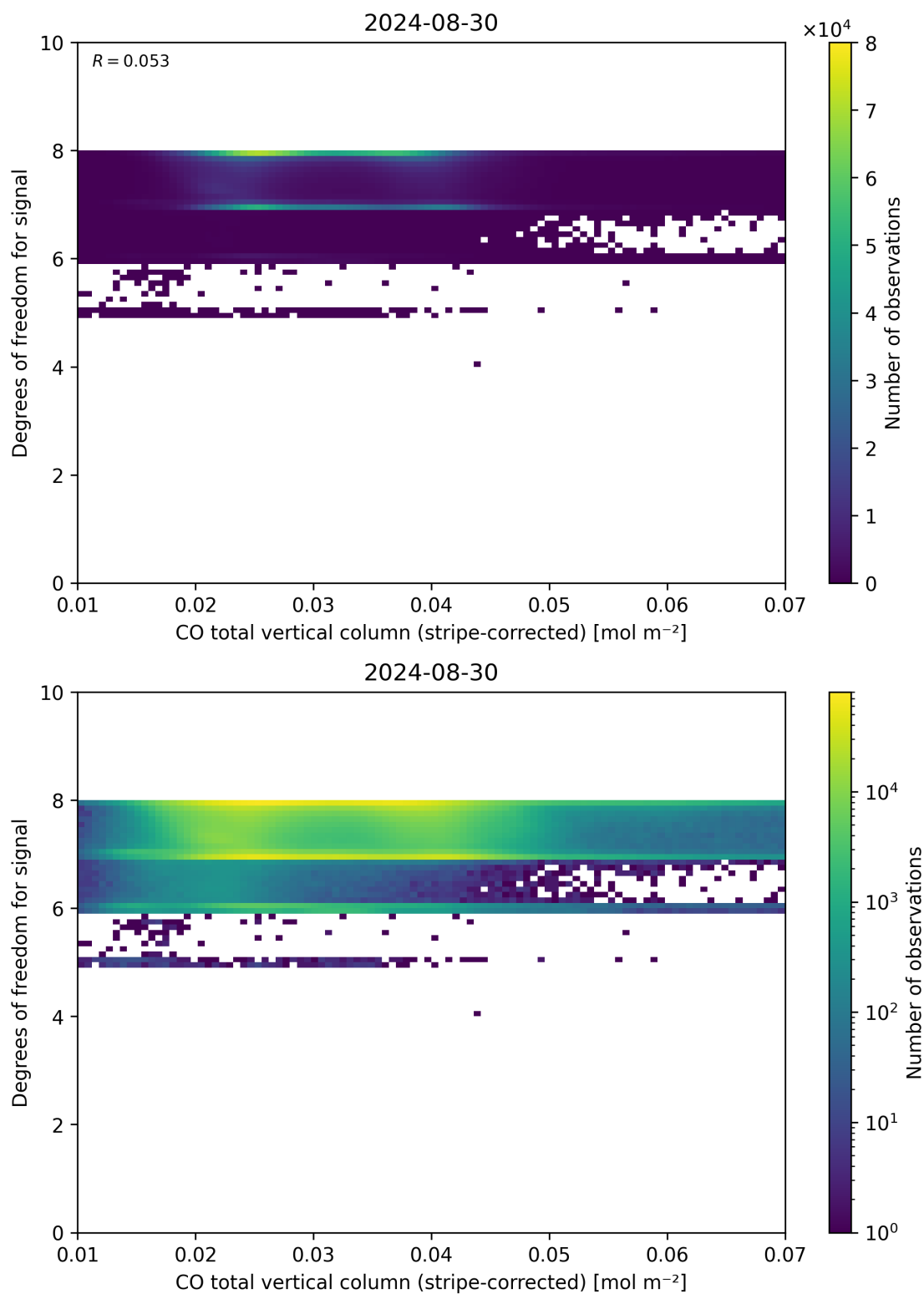
Figure 38: Scatter density plot of “CO total vertical column (stripe-corrected)” against “Degrees of freedom for signal” for 2024-08-29 to 2024-08-31.
