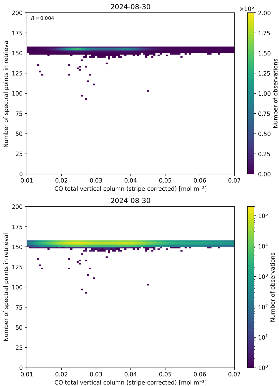
Figure 40: Scatter density plot of “CO total vertical column (stripe-corrected)” against “Number of spectral points in retrieval” for 2024-08-29 to 2024-08-31.
