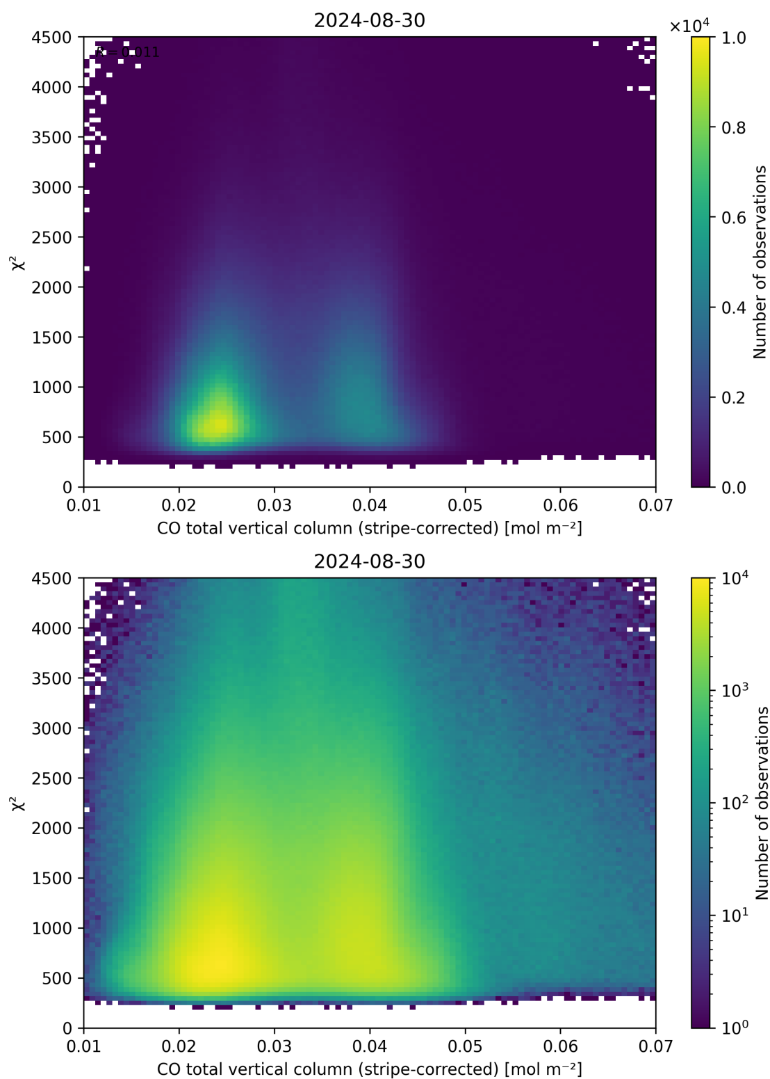
Figure 37: Scatter density plot of “CO total vertical column (stripe-corrected)” against “ \chi^2 ” for 2024-08-29 to 2024-08-31.
