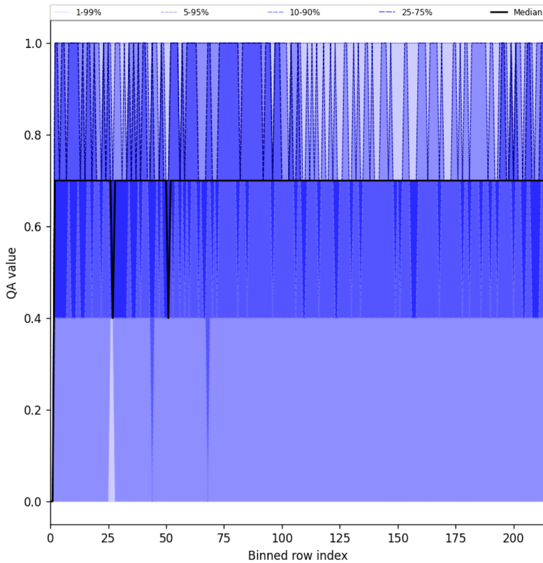
Figure 25: Along track statistics of “QA value” for 2024-08-29 to 2024-08-31
