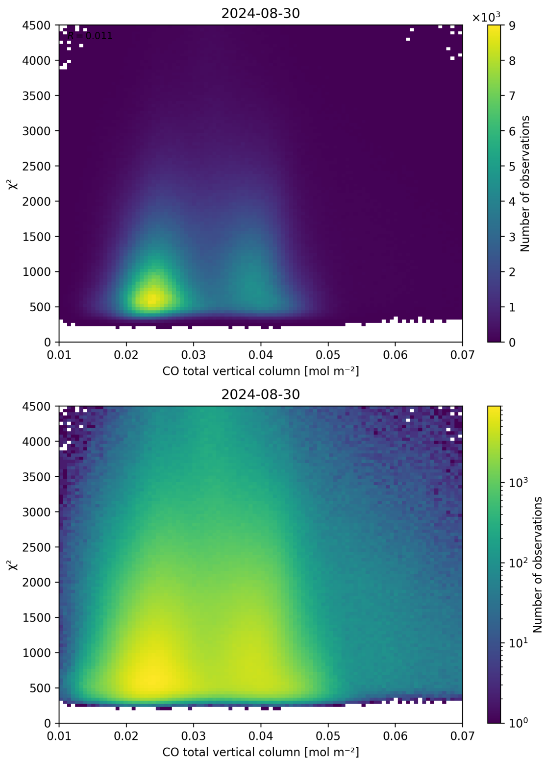
Figure 35: Scatter density plot of “CO total vertical column” against “ \chi^2 ” for 2024-08-29 to 2024-08-31.
