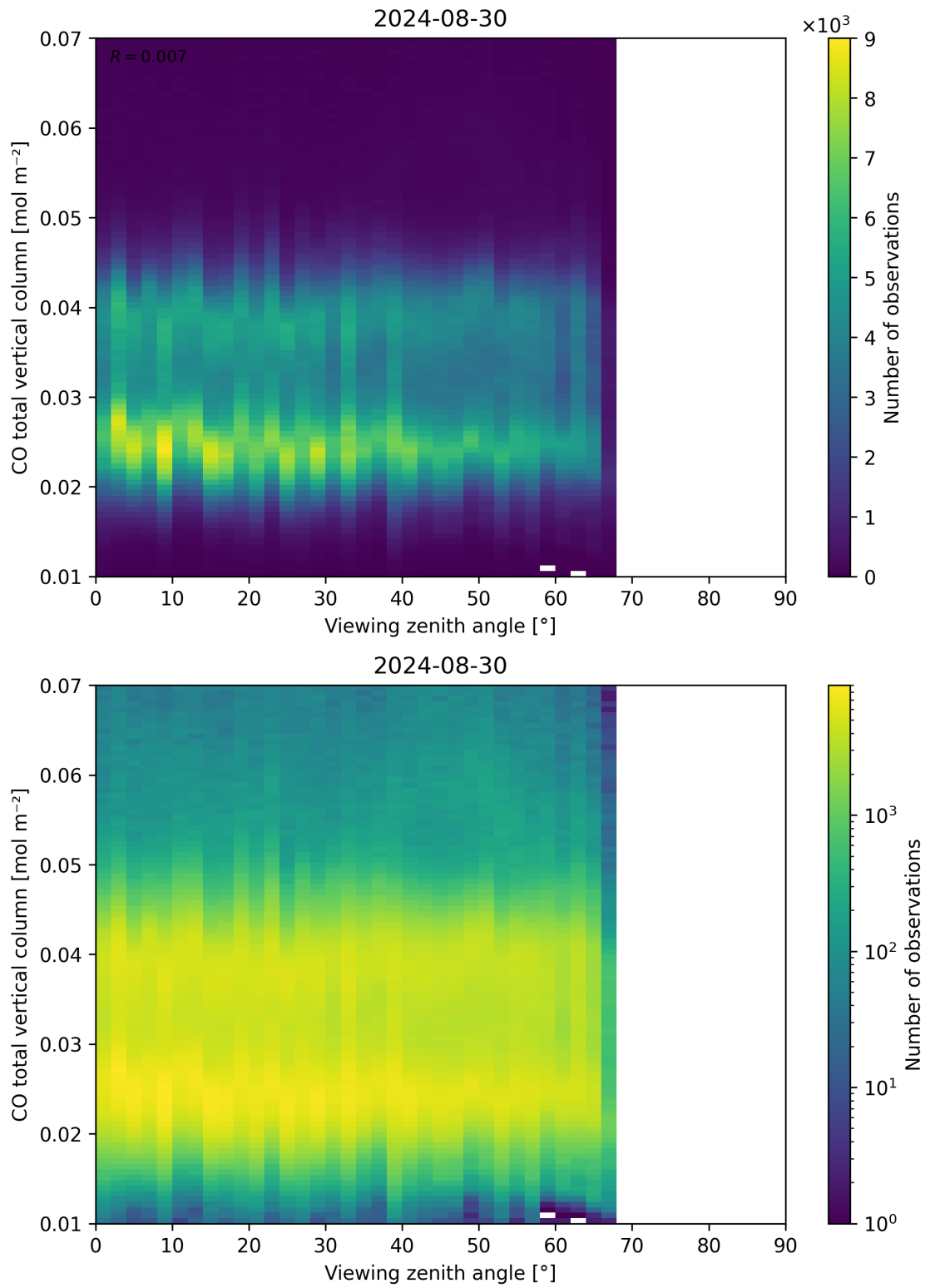
Figure 69: Scatter density plot of “Viewing zenith angle” against “CO total vertical column” for 2024-08-29 to 2024-08-31.
