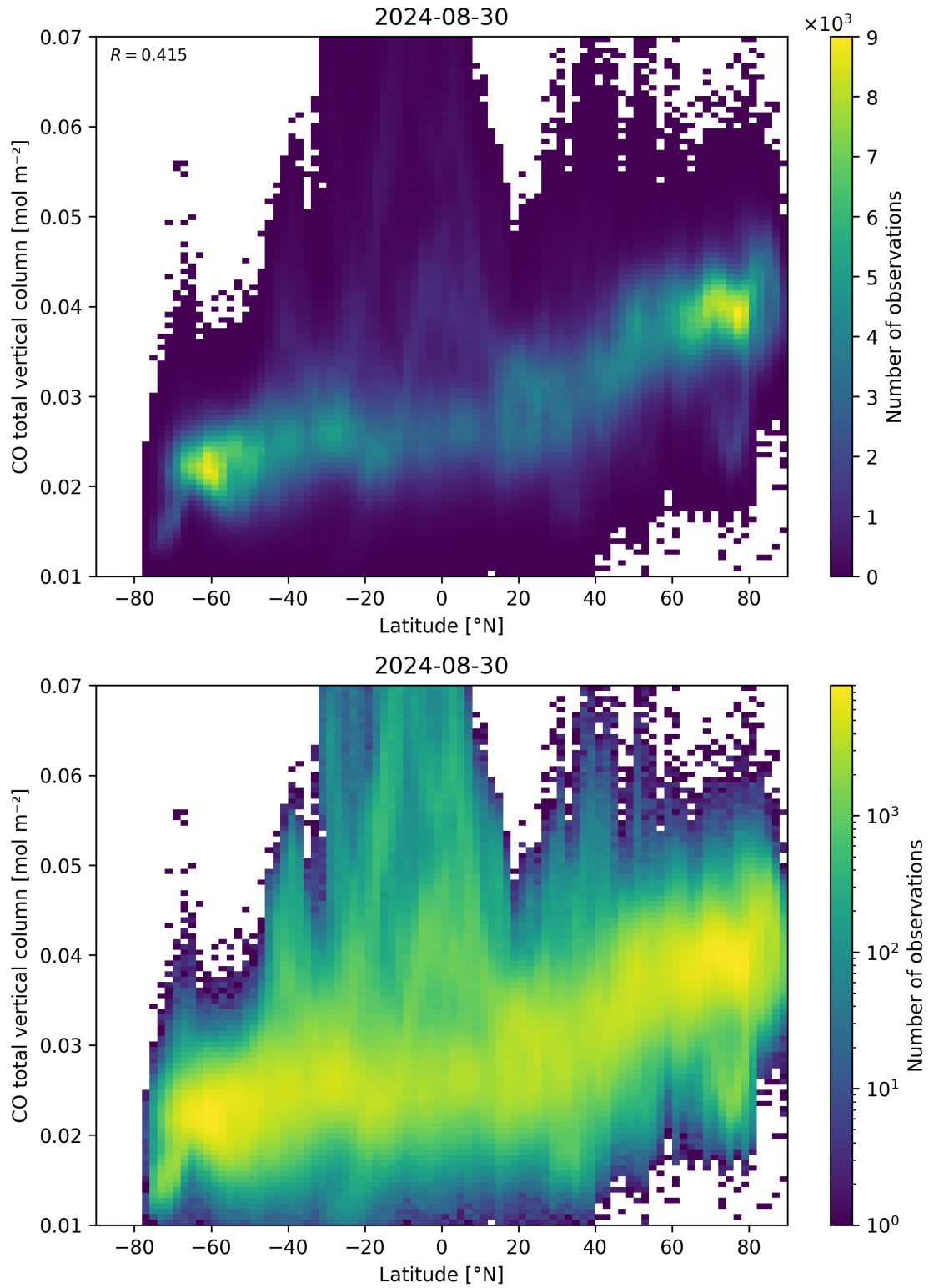
Figure 51: Scatter density plot of “Latitude” against “CO total vertical column” for 2024-08-29 to 2024-08-31.
