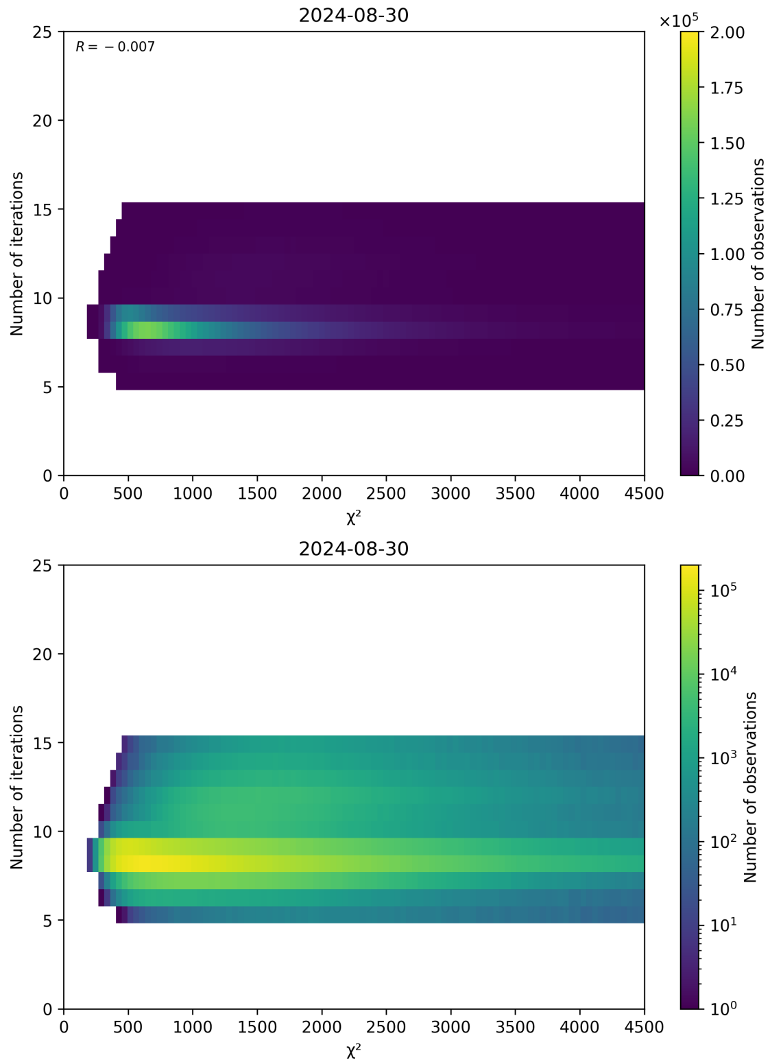
Figure 49: Scatter density plot of “ \chi^2 ” against “Number of iterations” for 2024-08-29 to 2024-08-31.
