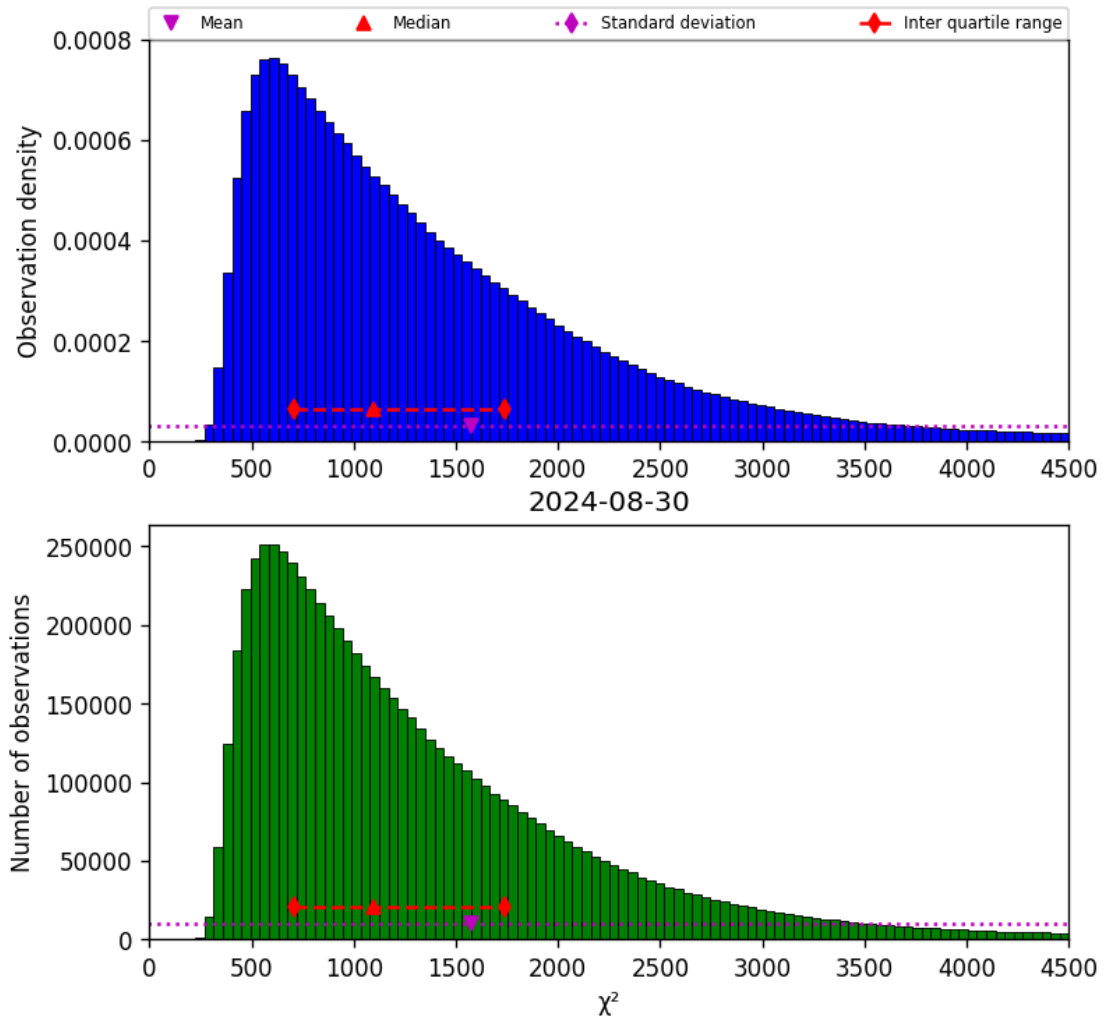
Figure 22: Histogram of " \chi^2 " for 2024-08-29 to 2024-08-31
