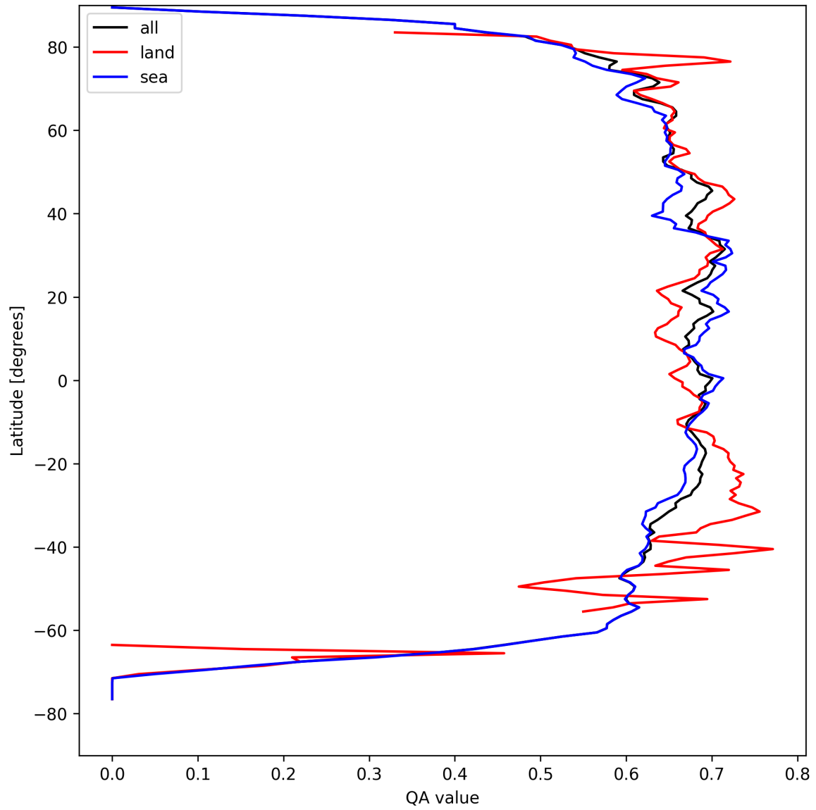
Figure 9: Zonal average of “QA value” for 2024-08-29 to 2024-08-31.
