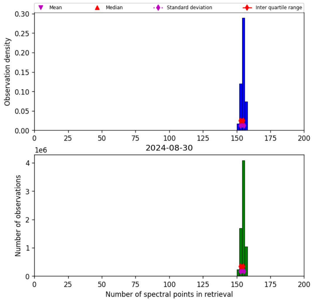
Figure 21: Histogram of “Number of spectral points in retrieval” for 2024-08-29 to 2024-08-31
