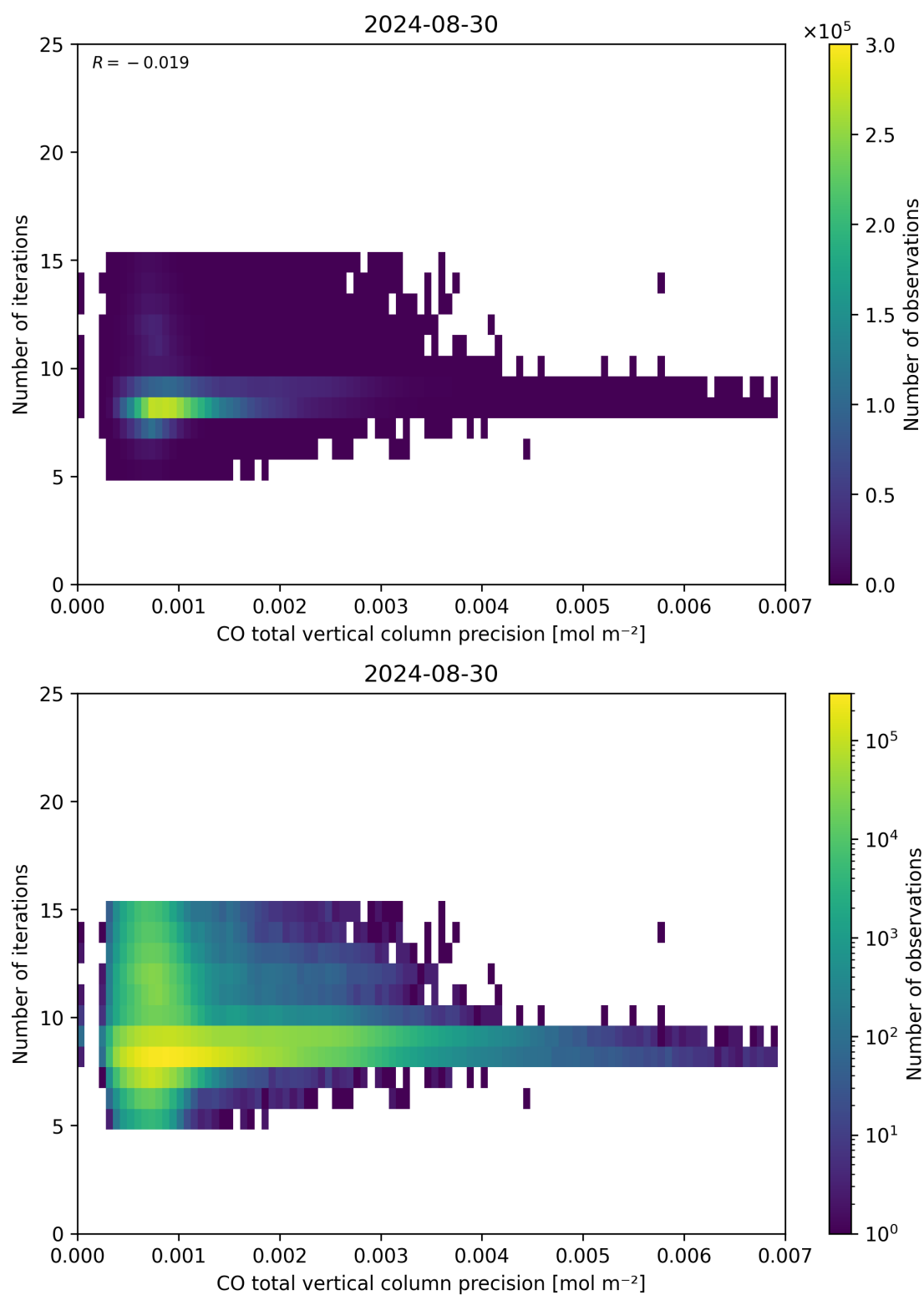
Figure 46: Scatter density plot of “CO total vertical column precision” against “Number of iterations” for 2024-08-29 to 2024-08-31.
