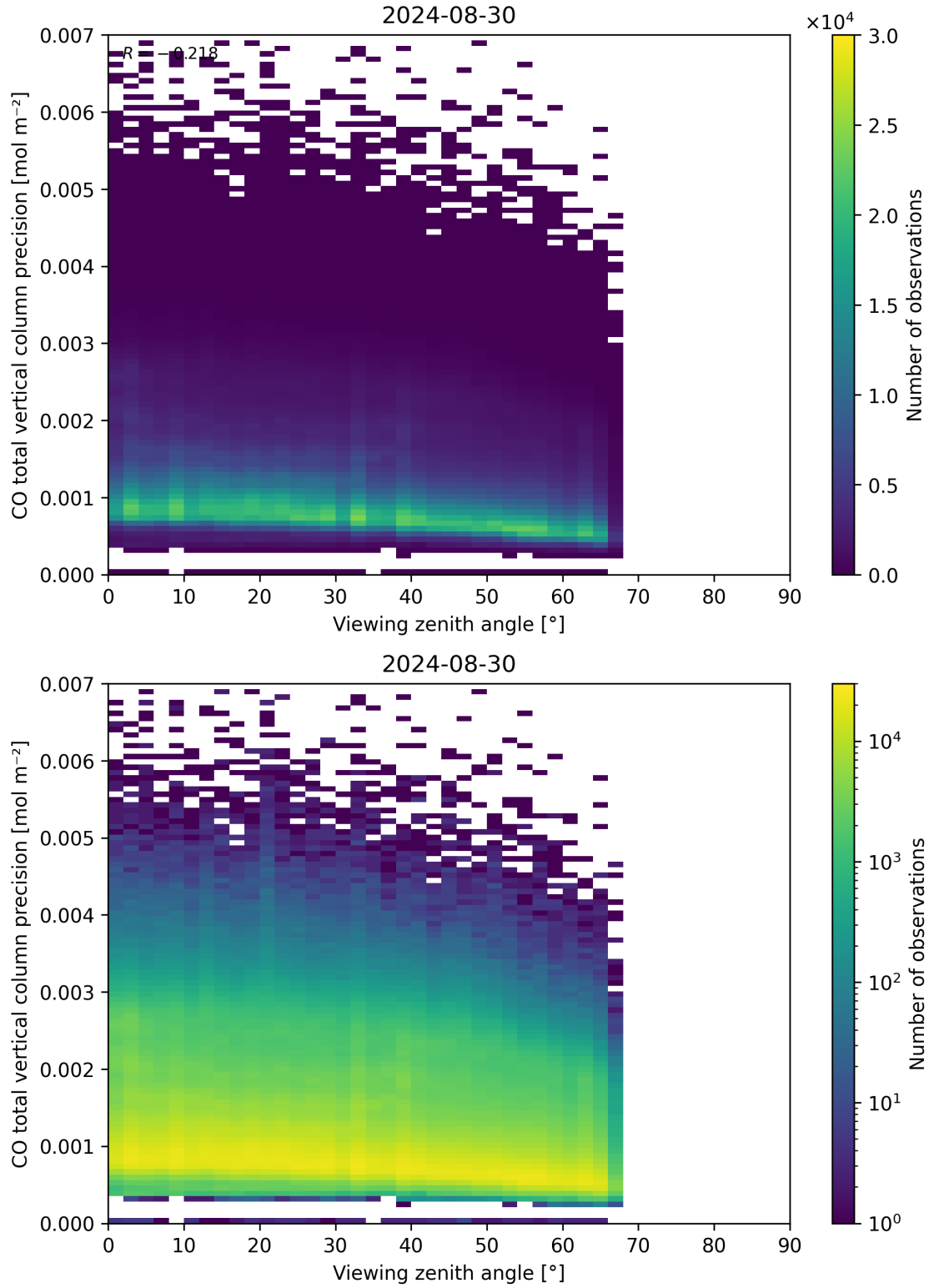
Figure 71: Scatter density plot of “Viewing zenith angle” against “CO total vertical column precision” for 2024-08-29 to 2024-08-31.
