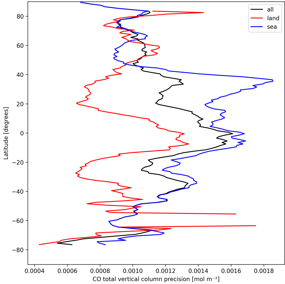
Figure 12: Zonal average of “CO total vertical column precision” for 2024-08-29 to 2024-08-31.
