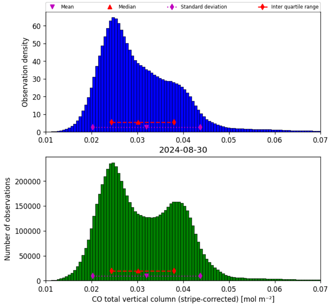
Figure 19: Histogram of “CO total vertical column (stripe-corrected)” for 2024-08-29 to 2024-08-31
