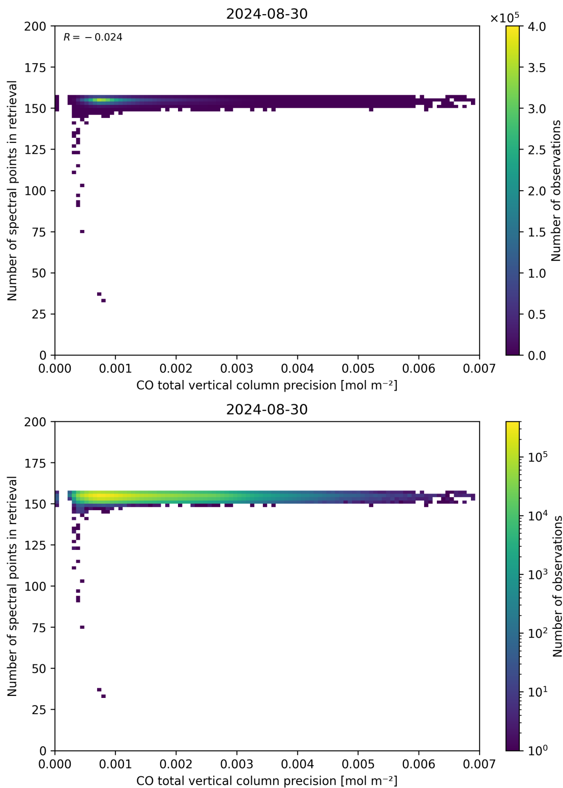
Figure 47: Scatter density plot of “CO total vertical column precision” against “Number of spectral points in retrieval” for 2024-08-29 to 2024-08-31.
