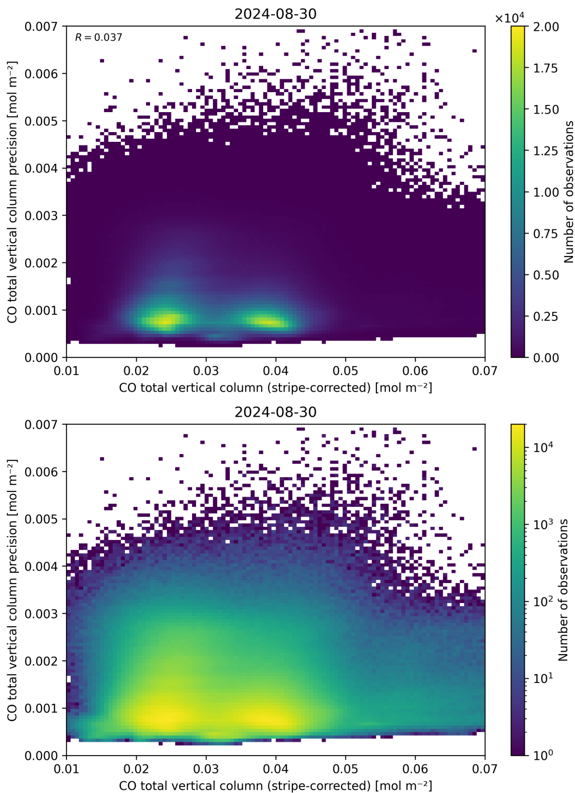
Figure 36: Scatter density plot of “CO total vertical column (stripe-corrected)” against “CO total vertical column precision” for 2024-08-29 to 2024-08-31.
