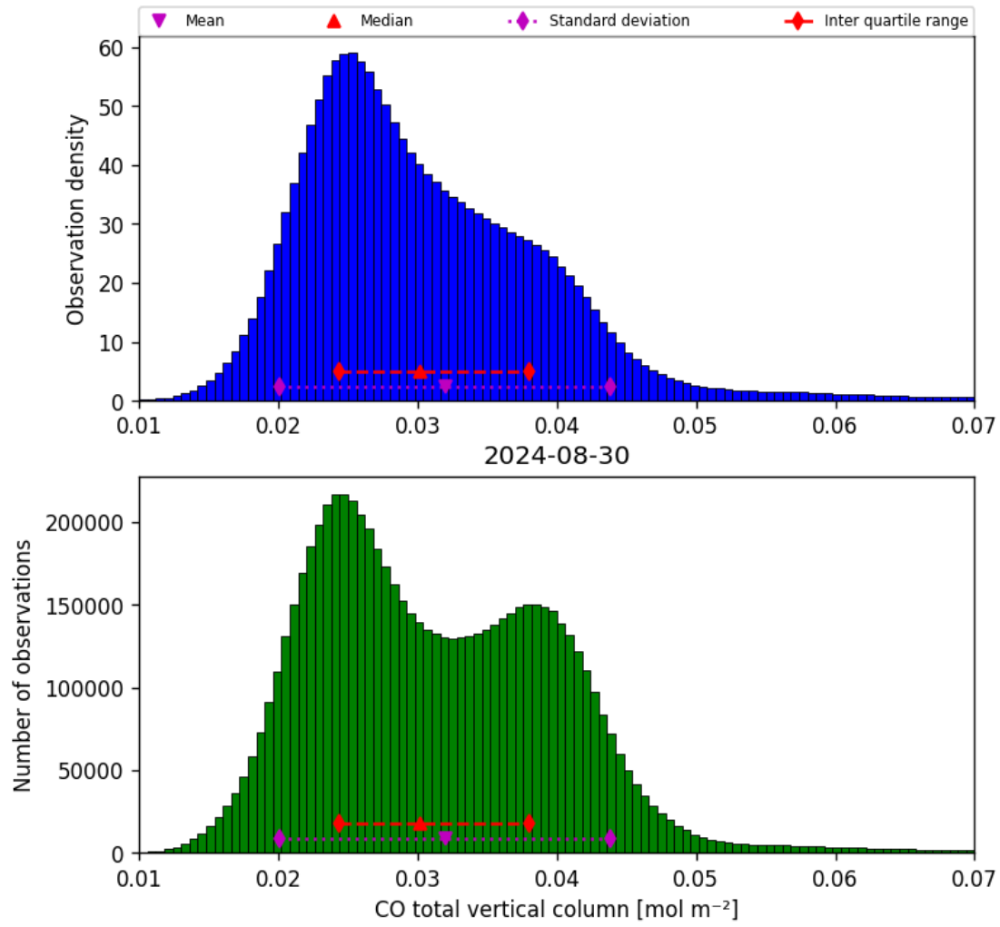
Figure 18: Histogram of “CO total vertical column” for 2024-08-29 to 2024-08-31
