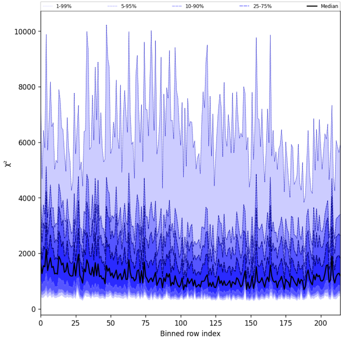
Figure 30: Along track statistics of “ \chi^2 ” for 2024-08-29 to 2024-08-31
