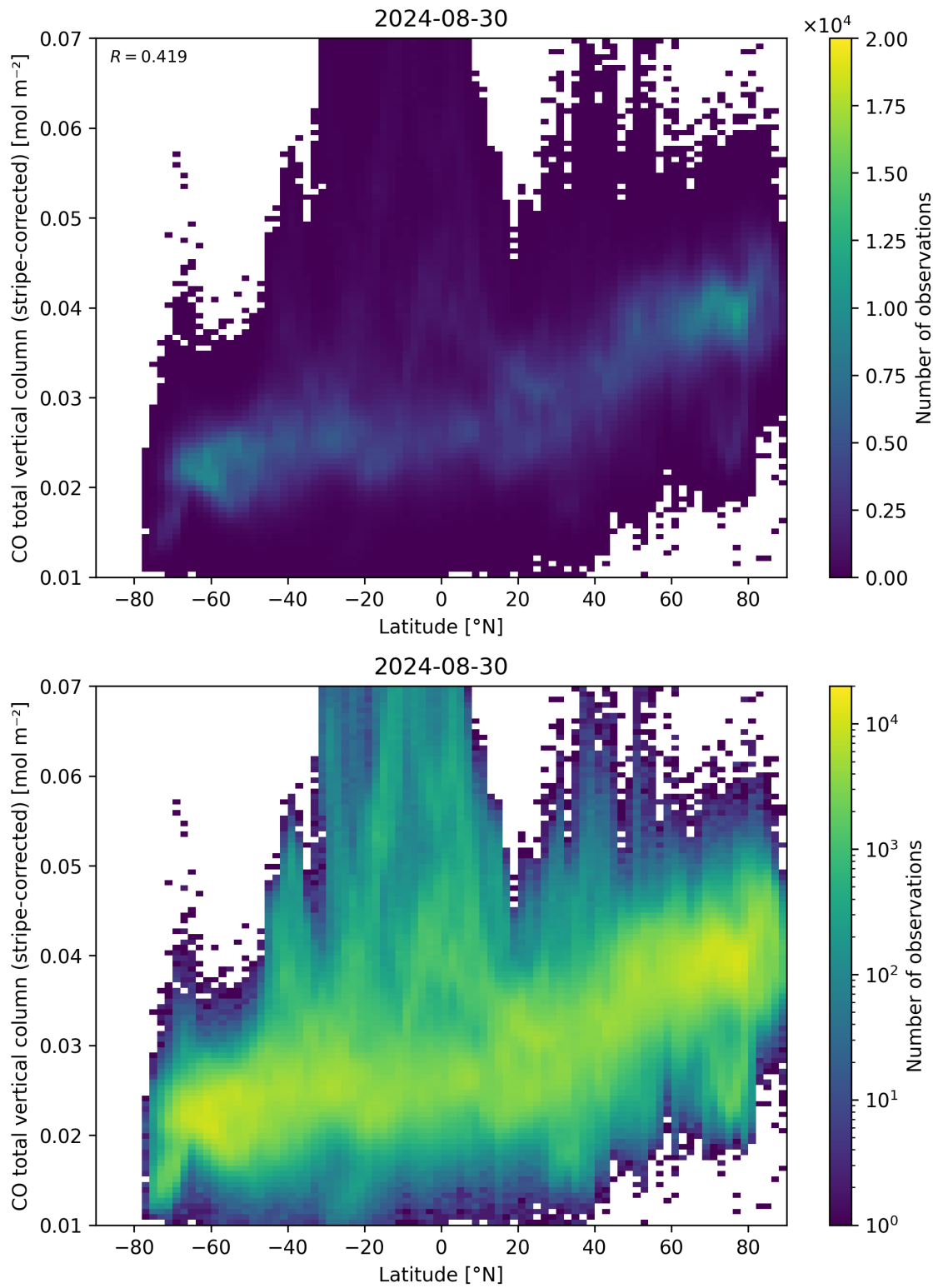
Figure 52: Scatter density plot of “Latitude” against “CO total vertical column (stripe-corrected)” for 2024-08-29 to 2024-08-31.
