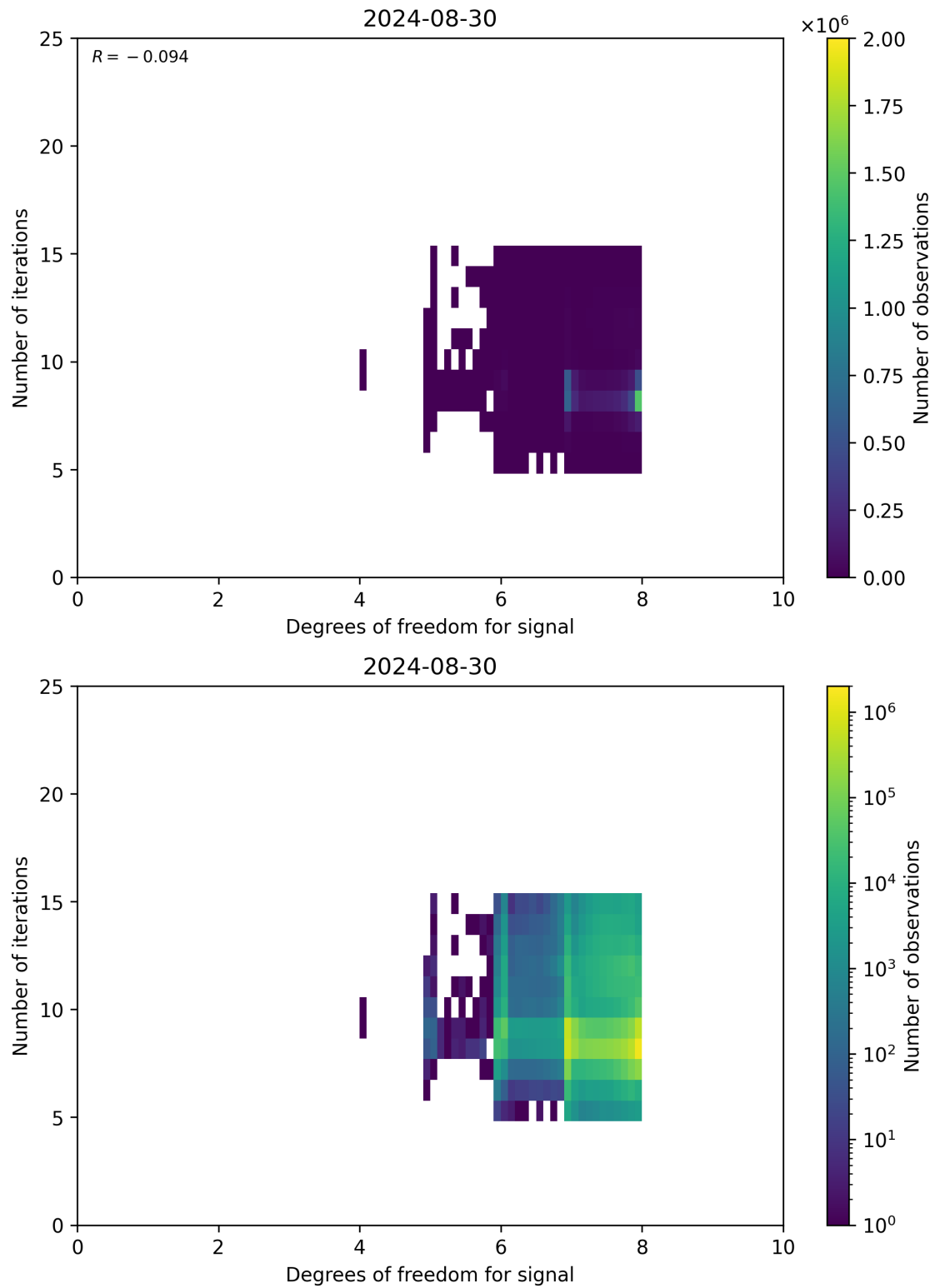
Figure 50: Scatter density plot of “Degrees of freedom for signal” against “Number of iterations” for 2024-08-29 to 2024-08-31.
