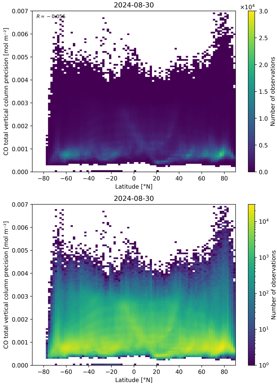
Figure 53: Scatter density plot of “Latitude” against “CO total vertical column precision” for 2024-08-29 to 2024-08-31.
