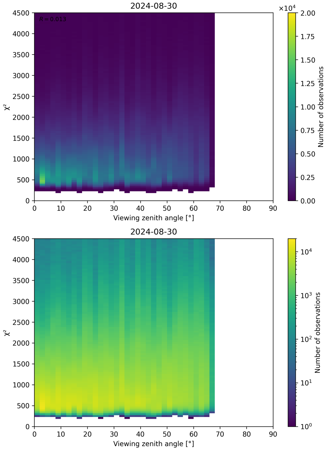
Figure 72: Scatter density plot of “Viewing zenith angle” against “ \chi^2 ” for 2024-08-29 to 2024-08-31.
