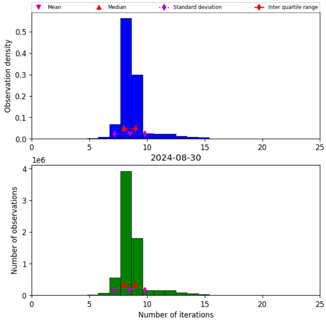
Figure 24: Histogram of “Number of iterations” for 2024-08-29 to 2024-08-31
