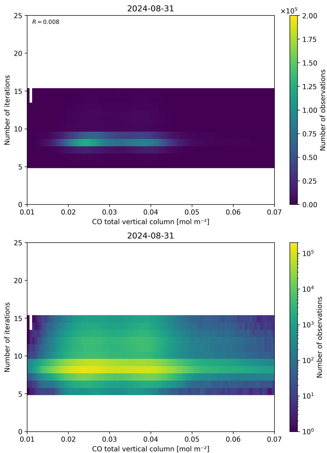
Figure 42: Scatter density plot of “CO total vertical column” against “Number of iterations” for 2024-08-30 to 2024-09-01.
