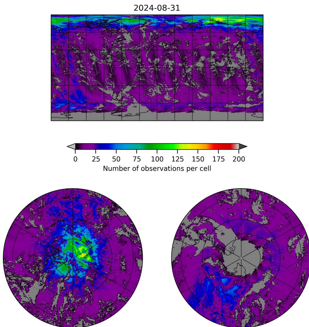
Figure 8: Map of the number of observations for 2024-08-30 to 2024-09-01
