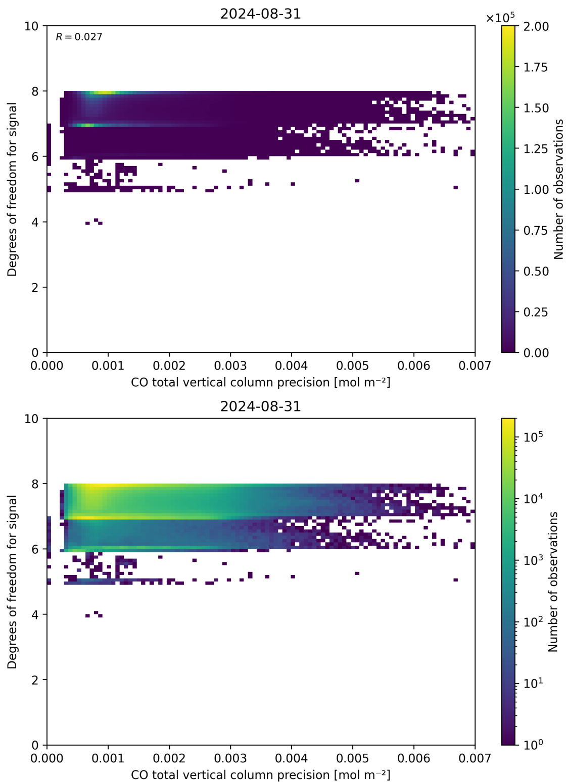
Figure 45: Scatter density plot of “CO total vertical column precision” against “Degrees of freedom for signal” for 2024-08-30 to 2024-09-01.
