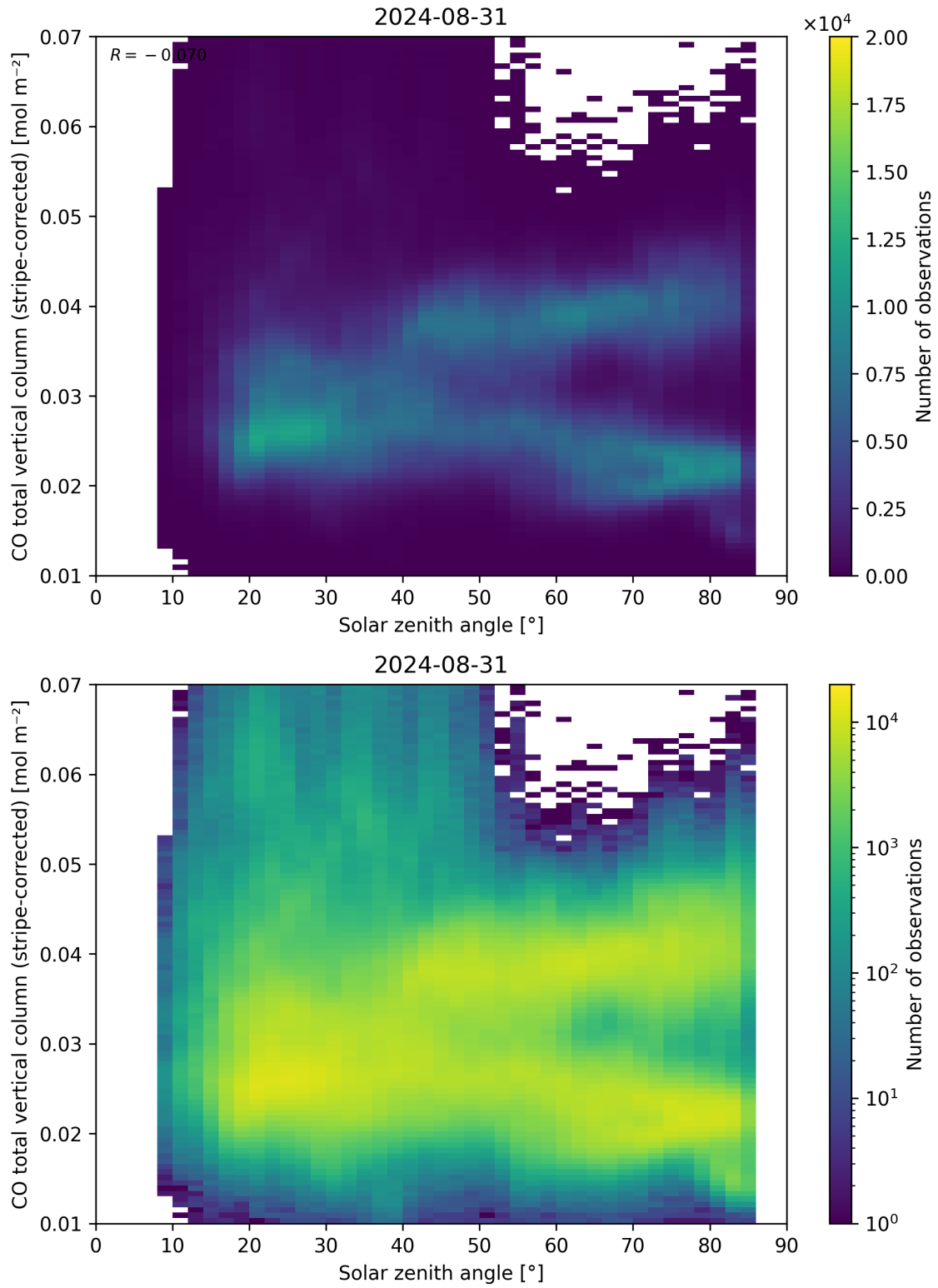
Figure 62: Scatter density plot of “Solar zenith angle” against “CO total vertical column (stripe-corrected)” for 2024-08-30 to 2024-09-01.
