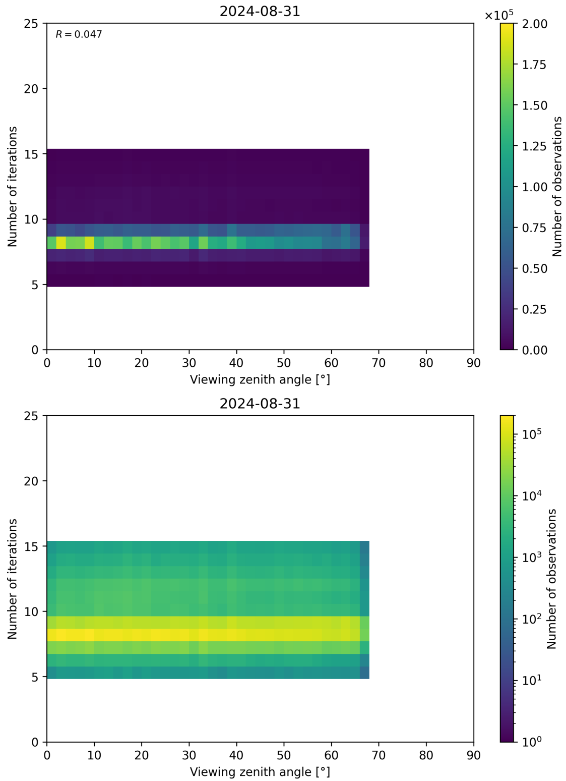
Figure 75: Scatter density plot of “Viewing zenith angle” against “Number of iterations” for 2024-08-30 to 2024-09-01.
