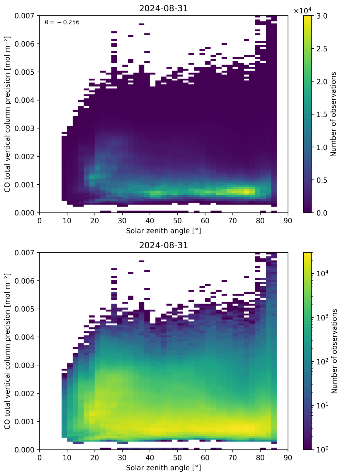
Figure 63: Scatter density plot of “Solar zenith angle” against “CO total vertical column precision” for 2024-08-30 to 2024-09-01.
