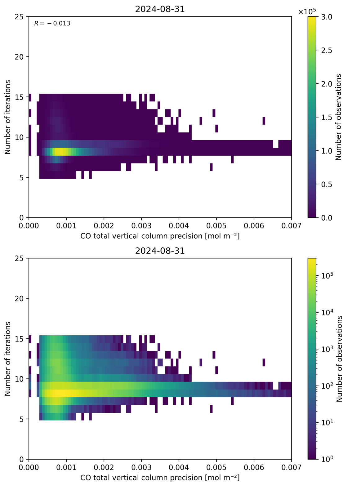
Figure 46: Scatter density plot of “CO total vertical column precision” against “Number of iterations” for 2024-08-30 to 2024-09-01.
