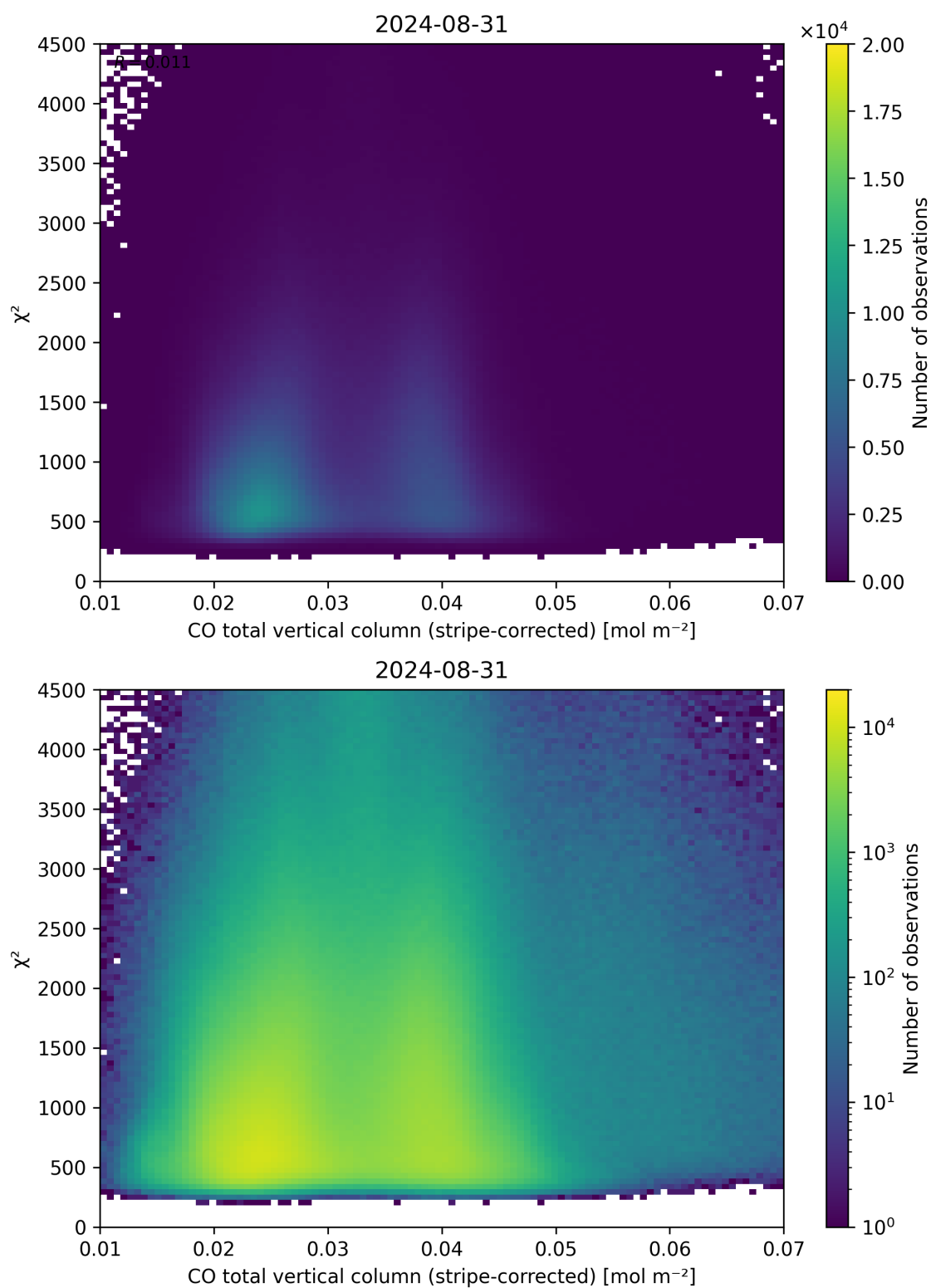
Figure 37: Scatter density plot of “CO total vertical column (stripe-corrected)” against “ \chi^2 ” for 2024-08-30 to 2024-09-01.
