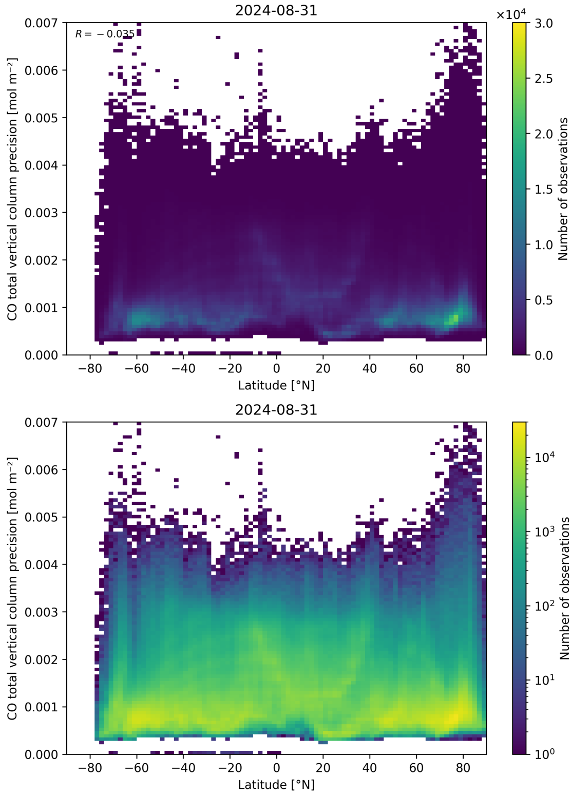
Figure 53: Scatter density plot of “Latitude” against “CO total vertical column precision” for 2024-08-30 to 2024-09-01.
