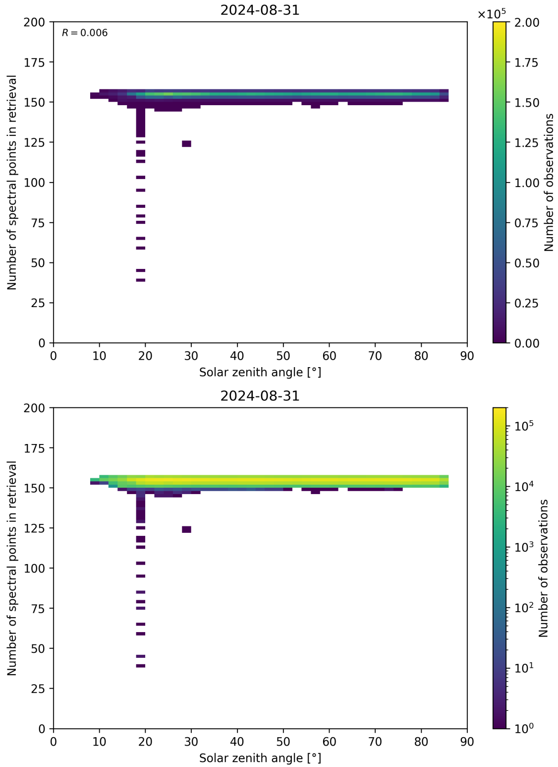
Figure 68: Scatter density plot of “Solar zenith angle” against “Number of spectral points in retrieval” for 2024-08-30 to 2024-09-01.
