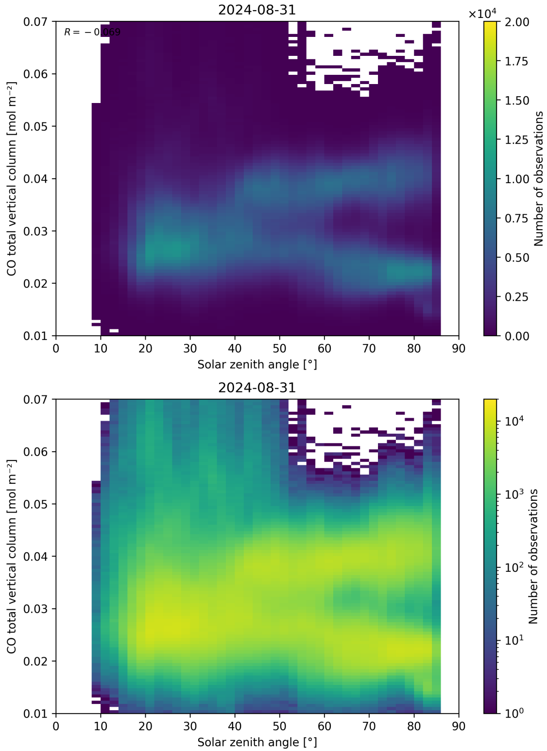
Figure 61: Scatter density plot of “Solar zenith angle” against “CO total vertical column” for 2024-08-30 to 2024-09-01.
