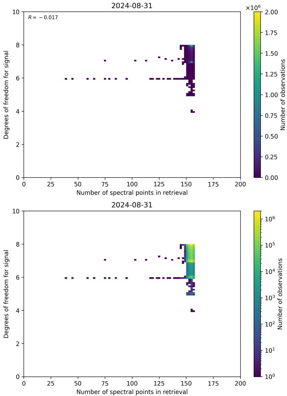
Figure 59: Scatter density plot of “Number of spectral points in retrieval” against “Degrees of freedom for signal” for 2024-08-30 to 2024-09-01.
