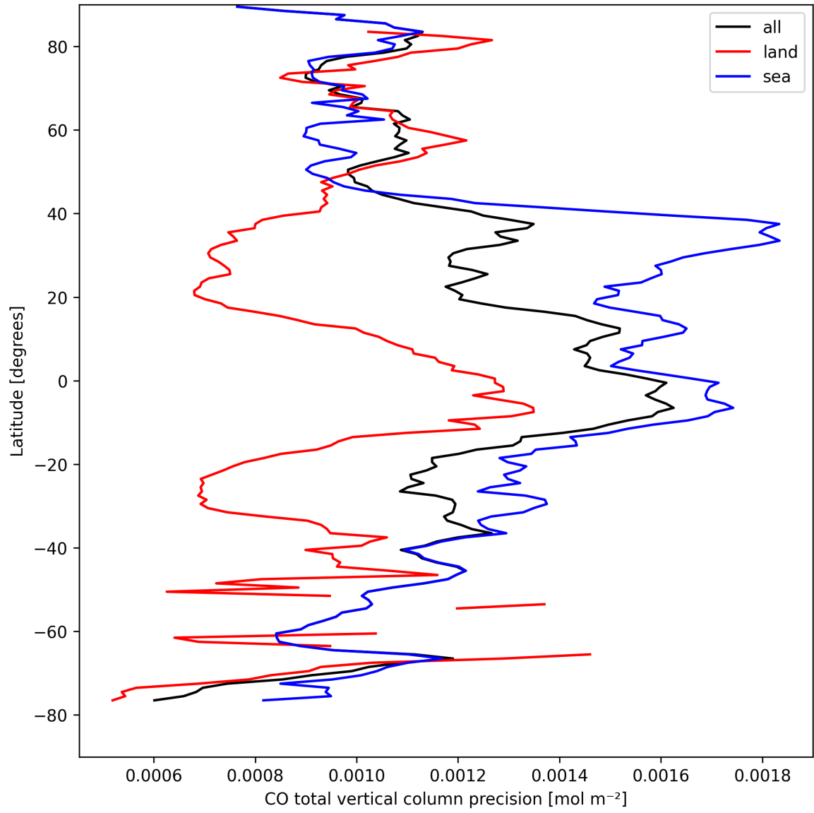
Figure 12: Zonal average of "CO total vertical column precision" for 2024-08-30 to 2024-09-01.
