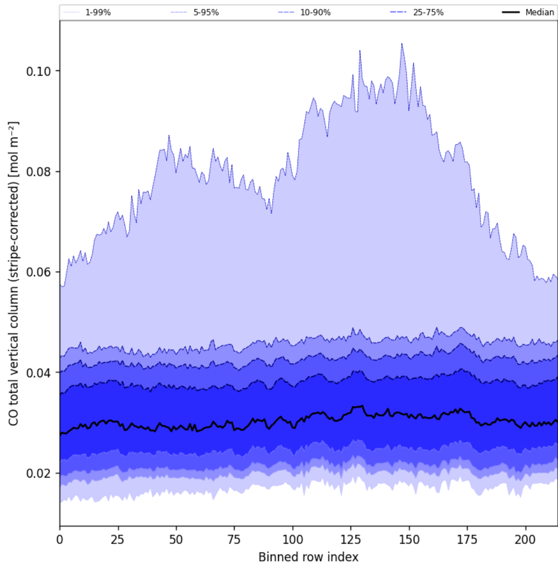
Figure 27: Along track statistics of “CO total vertical column (stripe-corrected)” for 2024-08-30 to 2024-09-01
