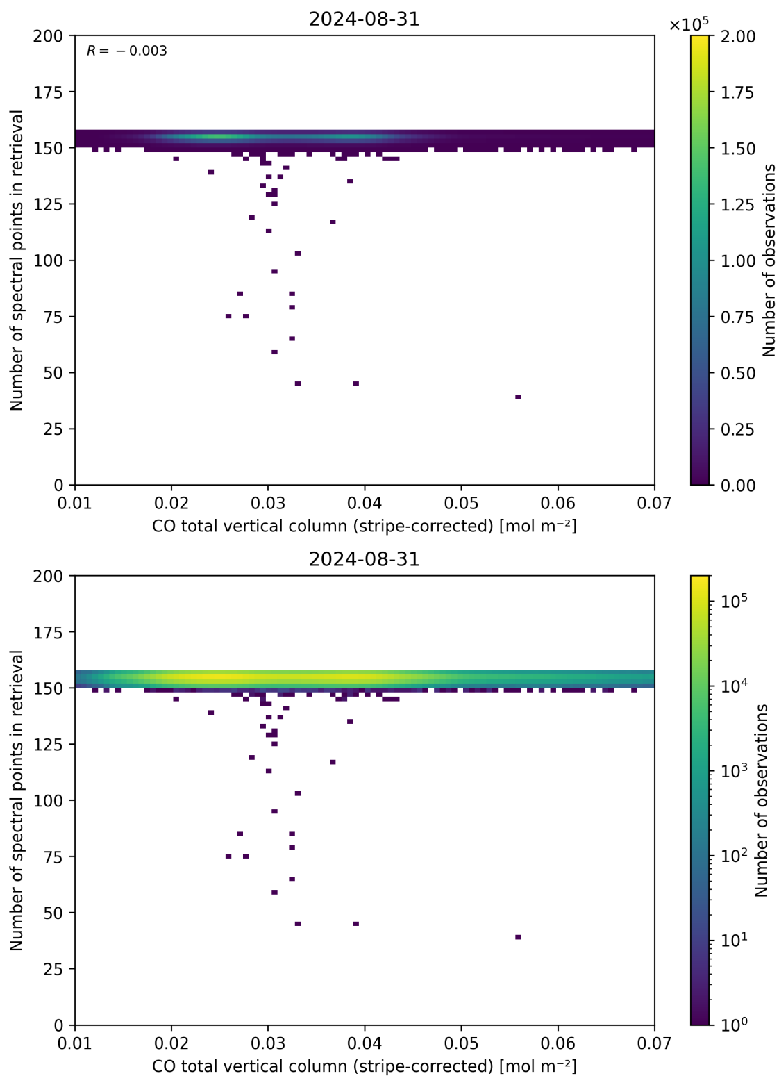
Figure 40: Scatter density plot of “CO total vertical column (stripe-corrected)” against “Number of spectral points in retrieval” for 2024-08-30 to 2024-09-01.
