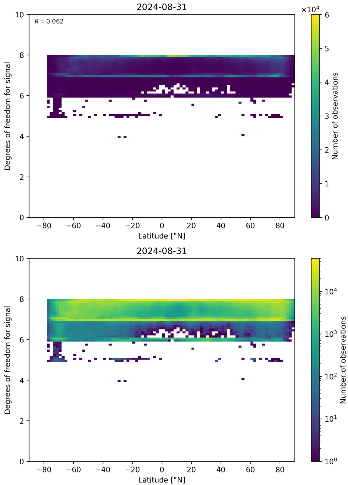
Figure 55: Scatter density plot of “Latitude” against “Degrees of freedom for signal” for 2024-08-30 to 2024-09-01.
