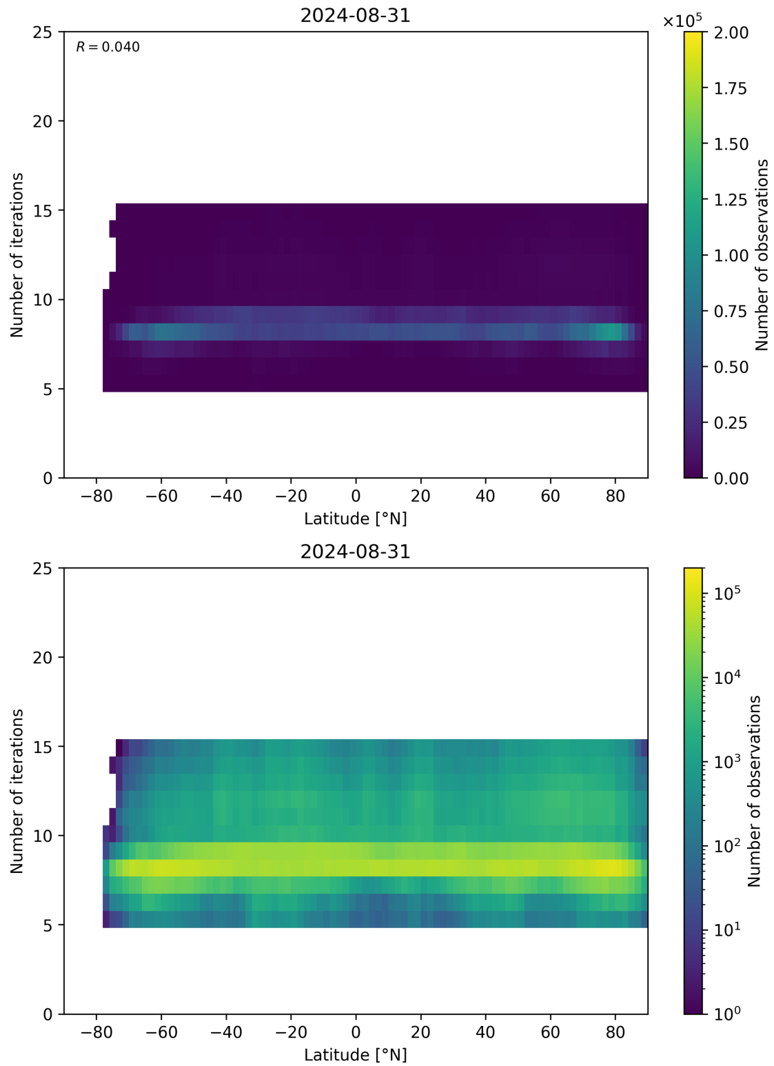
Figure 56: Scatter density plot of “Latitude” against “Number of iterations” for 2024-08-30 to 2024-09-01.
