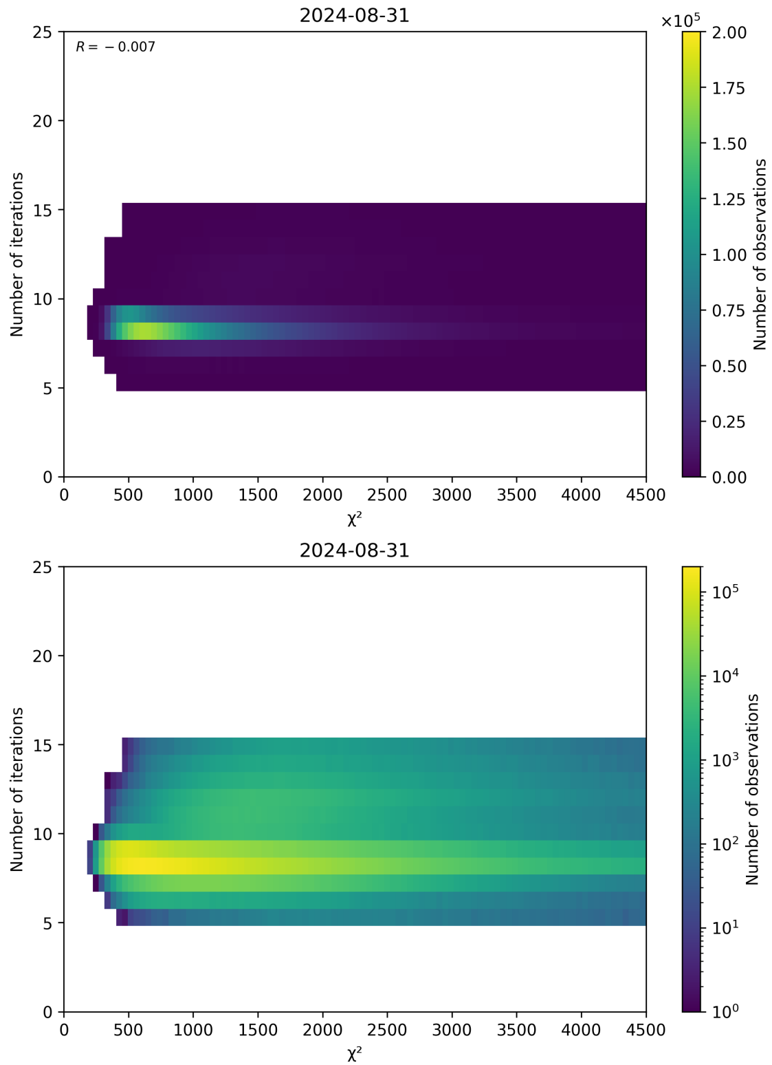
Figure 49: Scatter density plot of “ \chi^2 ” against “Number of iterations” for 2024-08-30 to 2024-09-01.
