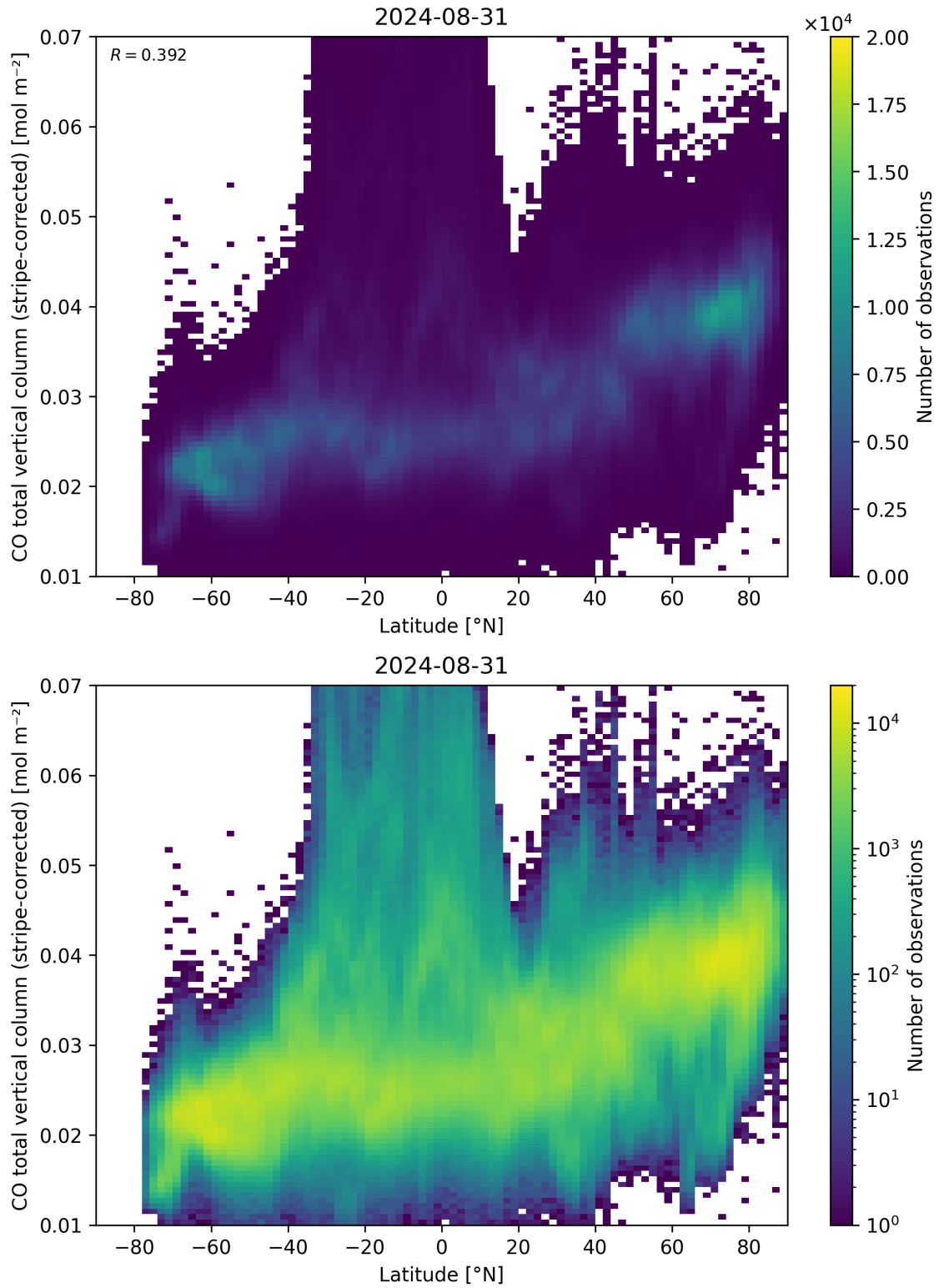
Figure 52: Scatter density plot of “Latitude” against “CO total vertical column (stripe-corrected)” for 2024-08-30 to 2024-09-01.
