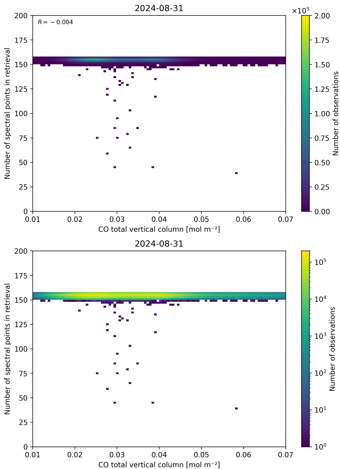
Figure 43: Scatter density plot of “CO total vertical column” against “Number of spectral points in retrieval” for 2024-08-30 to 2024-09-01.
