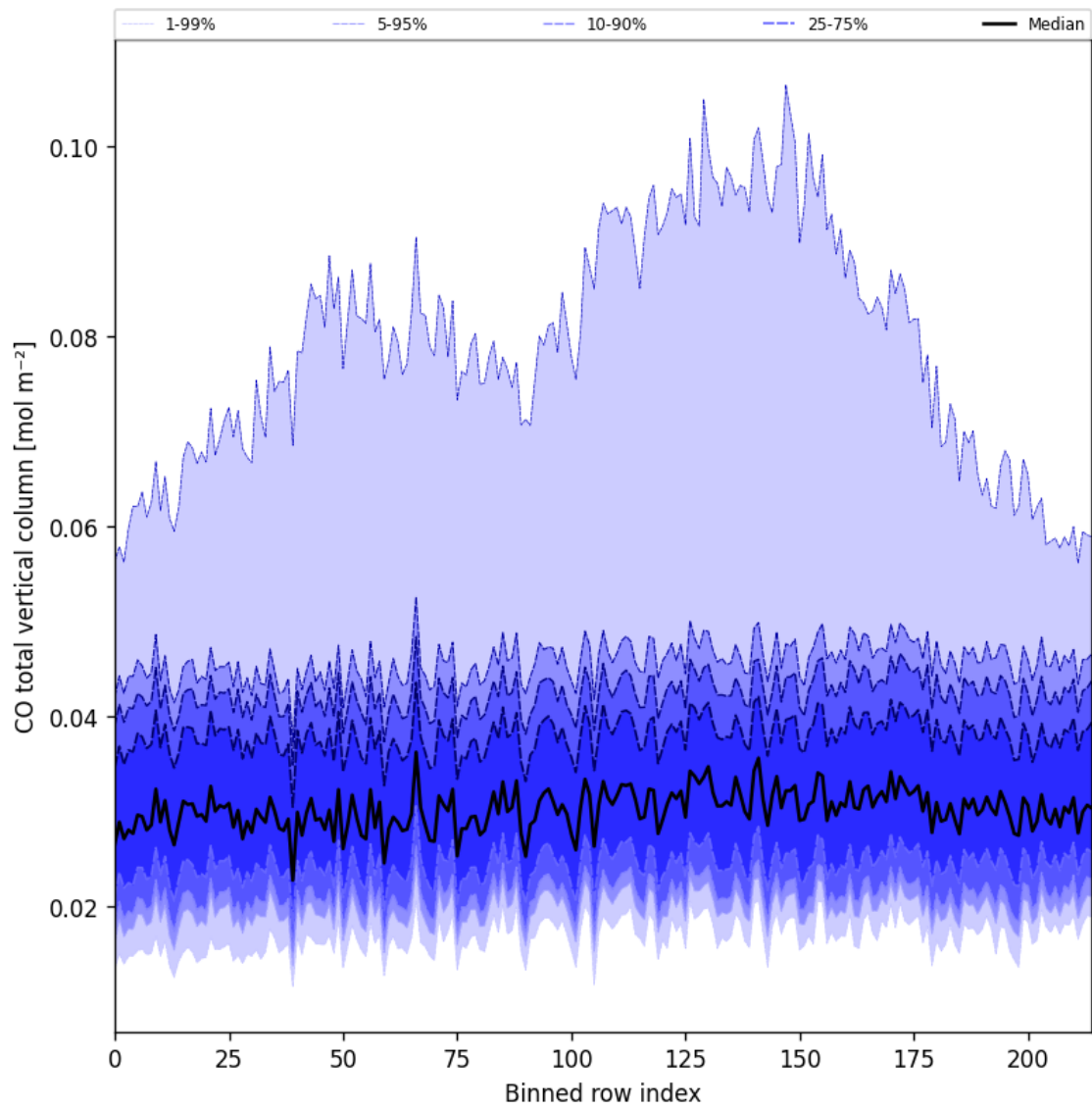
Figure 26: Along track statistics of “CO total vertical column” for 2024-08-30 to 2024-09-01
