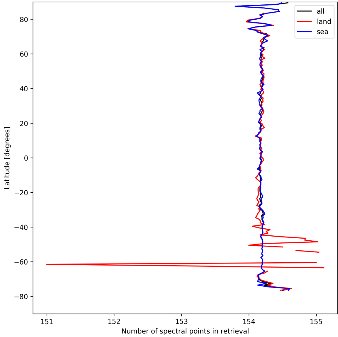
Figure 13: Zonal average of “Number of spectral points in retrieval” for 2024-08-30 to 2024-09-01.
