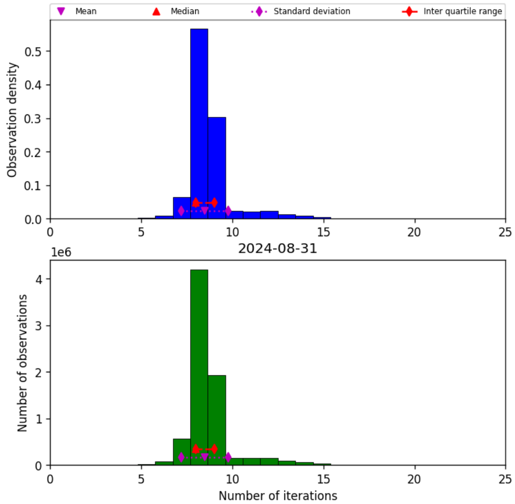
Figure 24: Histogram of “Number of iterations” for 2024-08-30 to 2024-09-01
