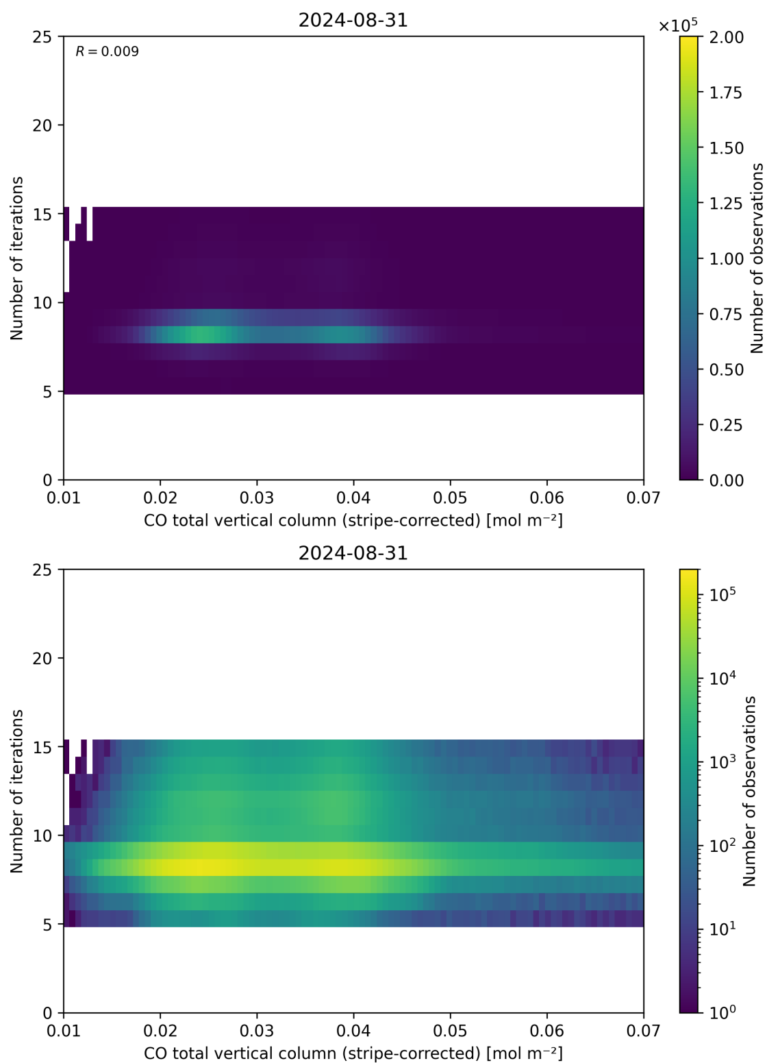
Figure 39: Scatter density plot of “CO total vertical column (stripe-corrected)” against “Number of iterations” for 2024-08-30 to 2024-09-01.
