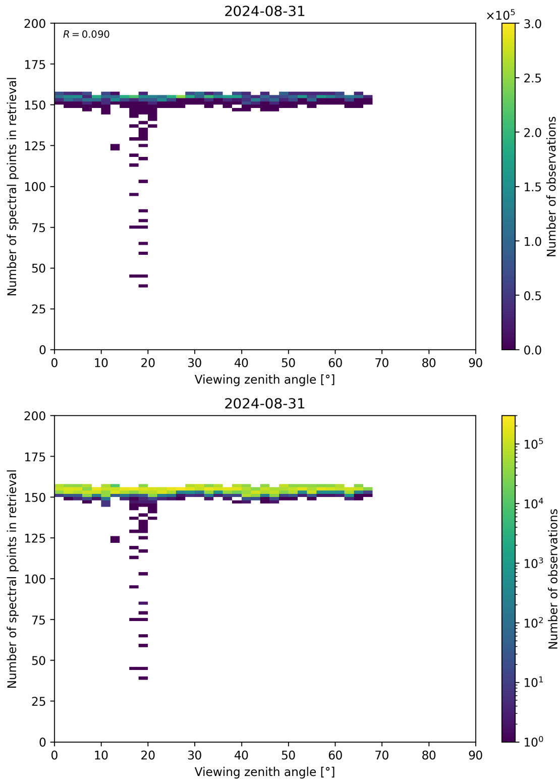
Figure 76: Scatter density plot of “Viewing zenith angle” against “Number of spectral points in retrieval” for 2024-08-30 to 2024-09-01.
