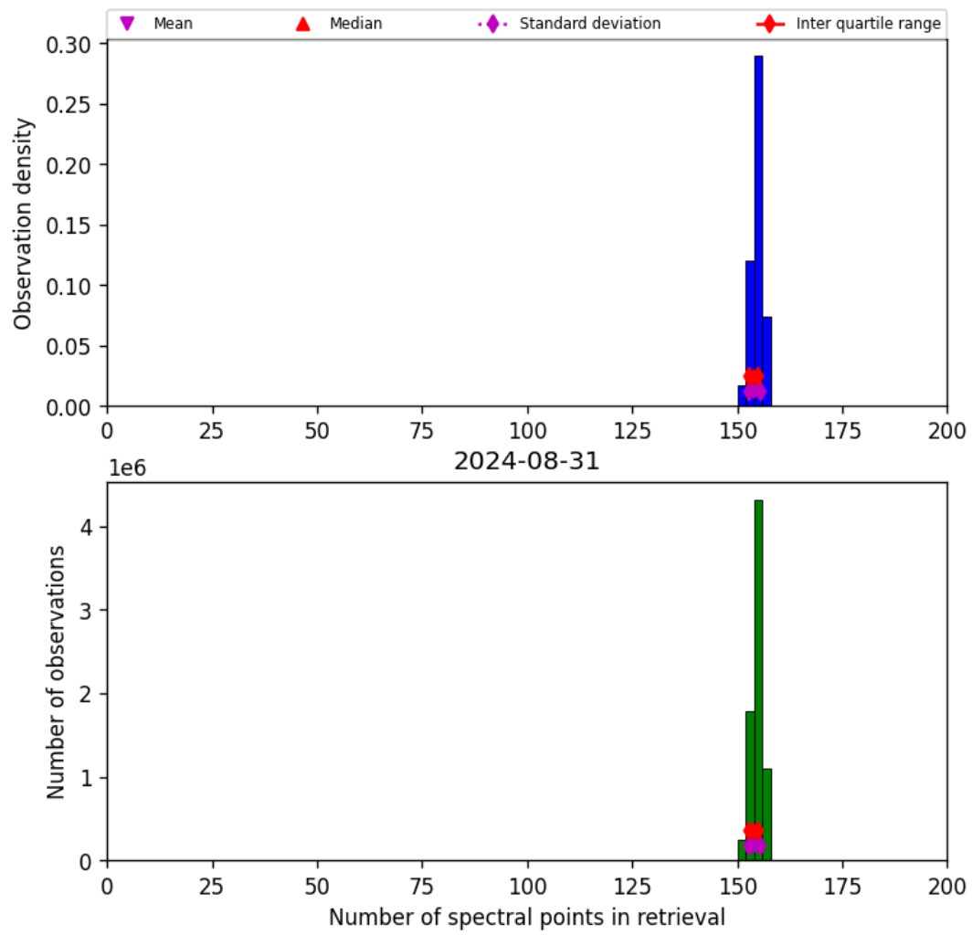
Figure 21: Histogram of “Number of spectral points in retrieval” for 2024-08-30 to 2024-09-01
