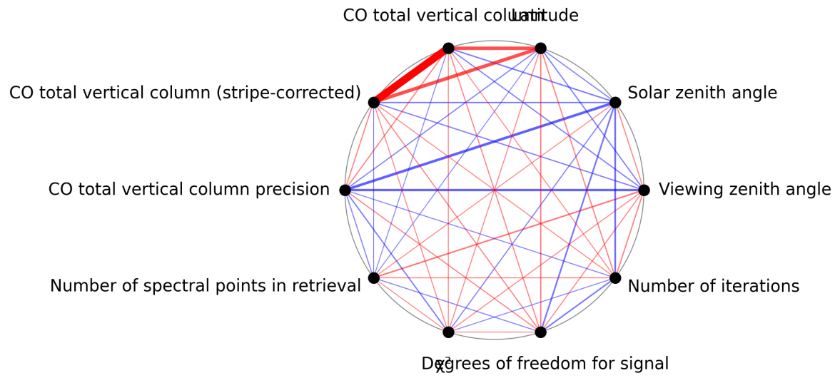
Figure 1: Map of correlation graph for 2024-08-30 to 2024-09-01.
