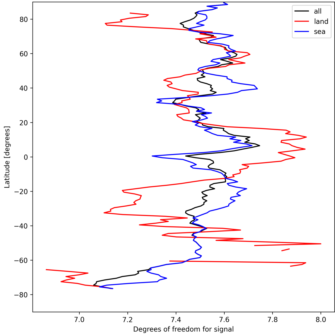
Figure 15: Zonal average of “Degrees of freedom for signal” for 2024-08-30 to 2024-09-01.
