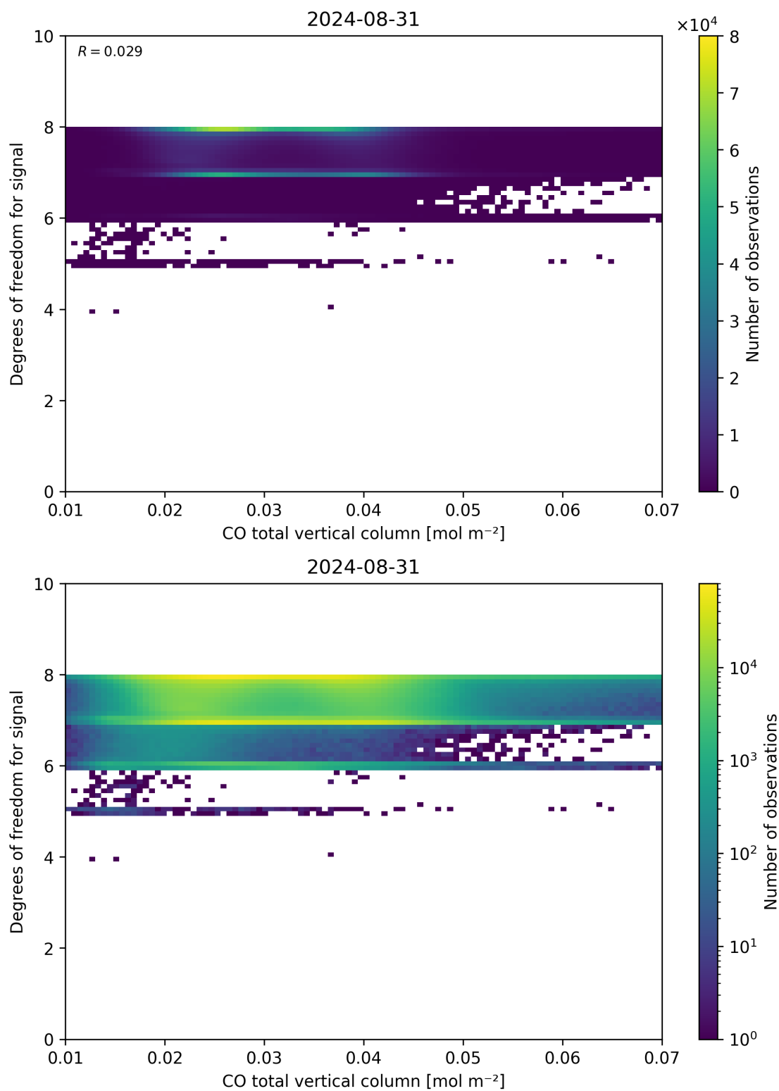
Figure 41: Scatter density plot of “CO total vertical column” against “Degrees of freedom for signal” for 2024-08-30 to 2024-09-01.
