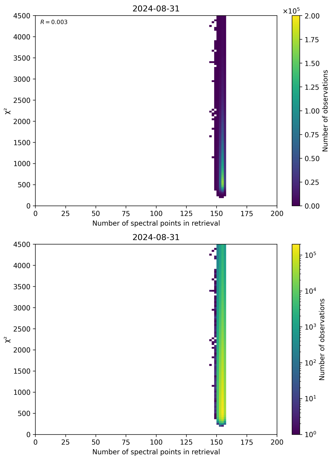
Figure 58: Scatter density plot of “Number of spectral points in retrieval” against “ \chi^2 ” for 2024-08-30 to 2024-09-01.
