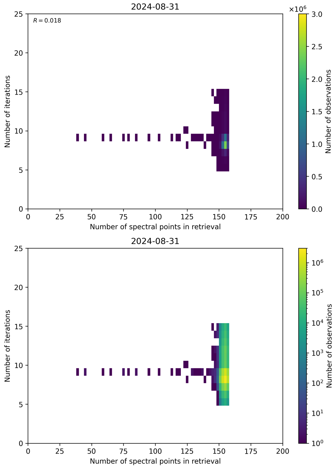
Figure 60: Scatter density plot of “Number of spectral points in retrieval” against “Number of iterations” for 2024-08-30 to 2024-09-01.
