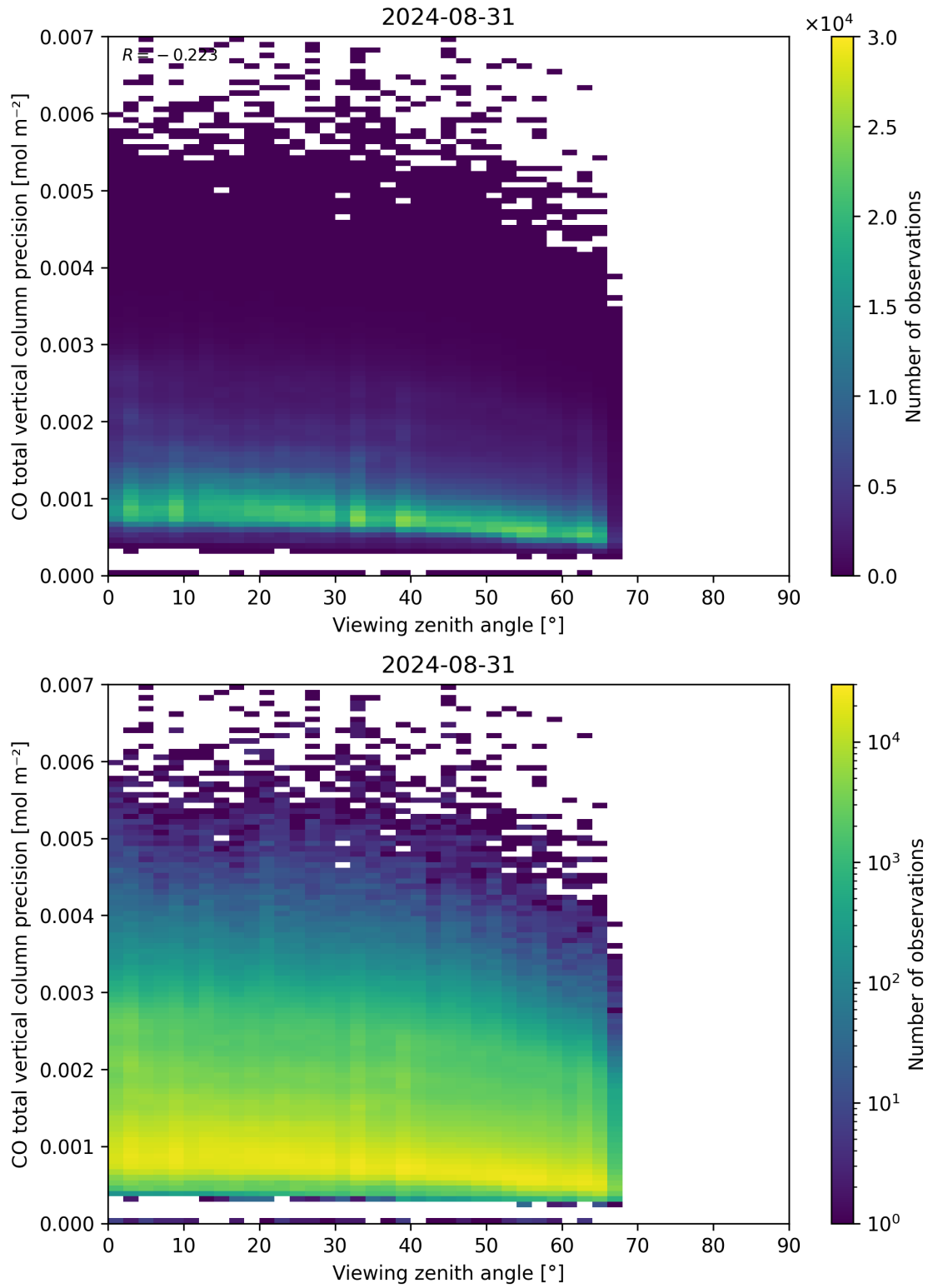
Figure 71: Scatter density plot of “Viewing zenith angle” against “CO total vertical column precision” for 2024-08-30 to 2024-09-01.
