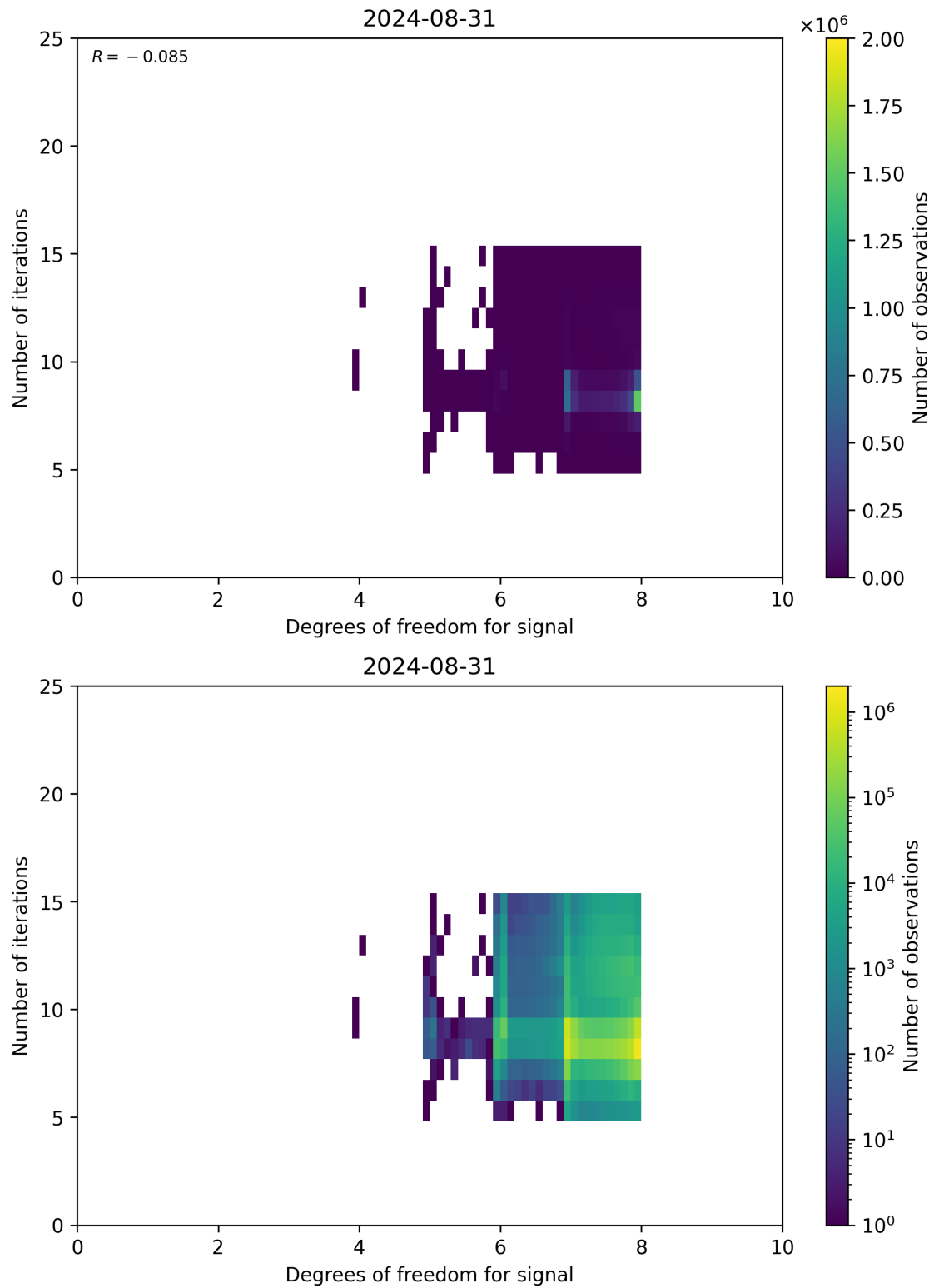
Figure 50: Scatter density plot of “Degrees of freedom for signal” against “Number of iterations” for 2024-08-30 to 2024-09-01.
