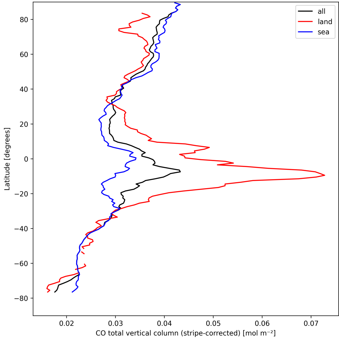
Figure 11: Zonal average of “CO total vertical column (stripe-corrected)” for 2024-08-30 to 2024-09-01.
