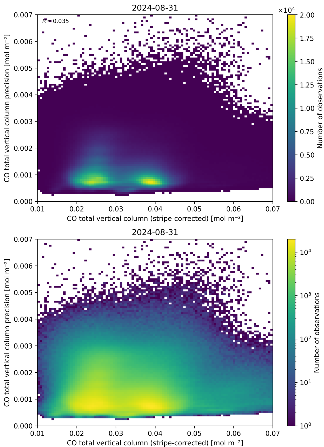
Figure 36: Scatter density plot of “CO total vertical column (stripe-corrected)” against “CO total vertical column precision” for 2024-08-30 to 2024-09-01.
