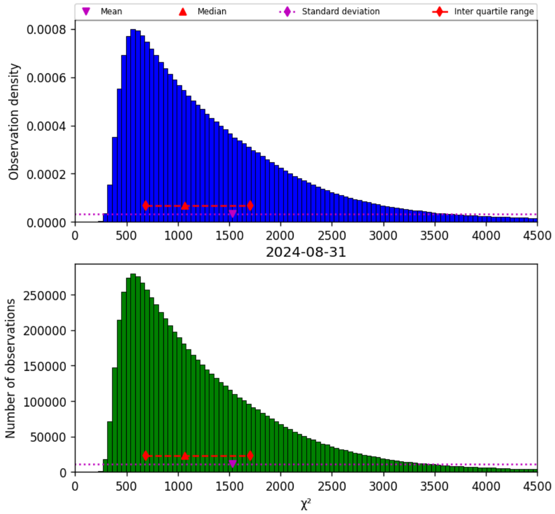
Figure 22: Histogram of “ \chi^2 ” for 2024-08-30 to 2024-09-01
