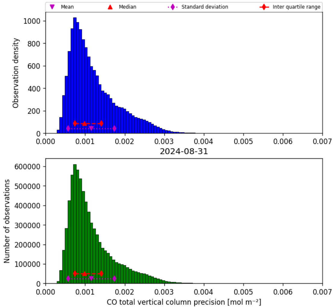
Figure 20: Histogram of “CO total vertical column precision” for 2024-08-30 to 2024-09-01
