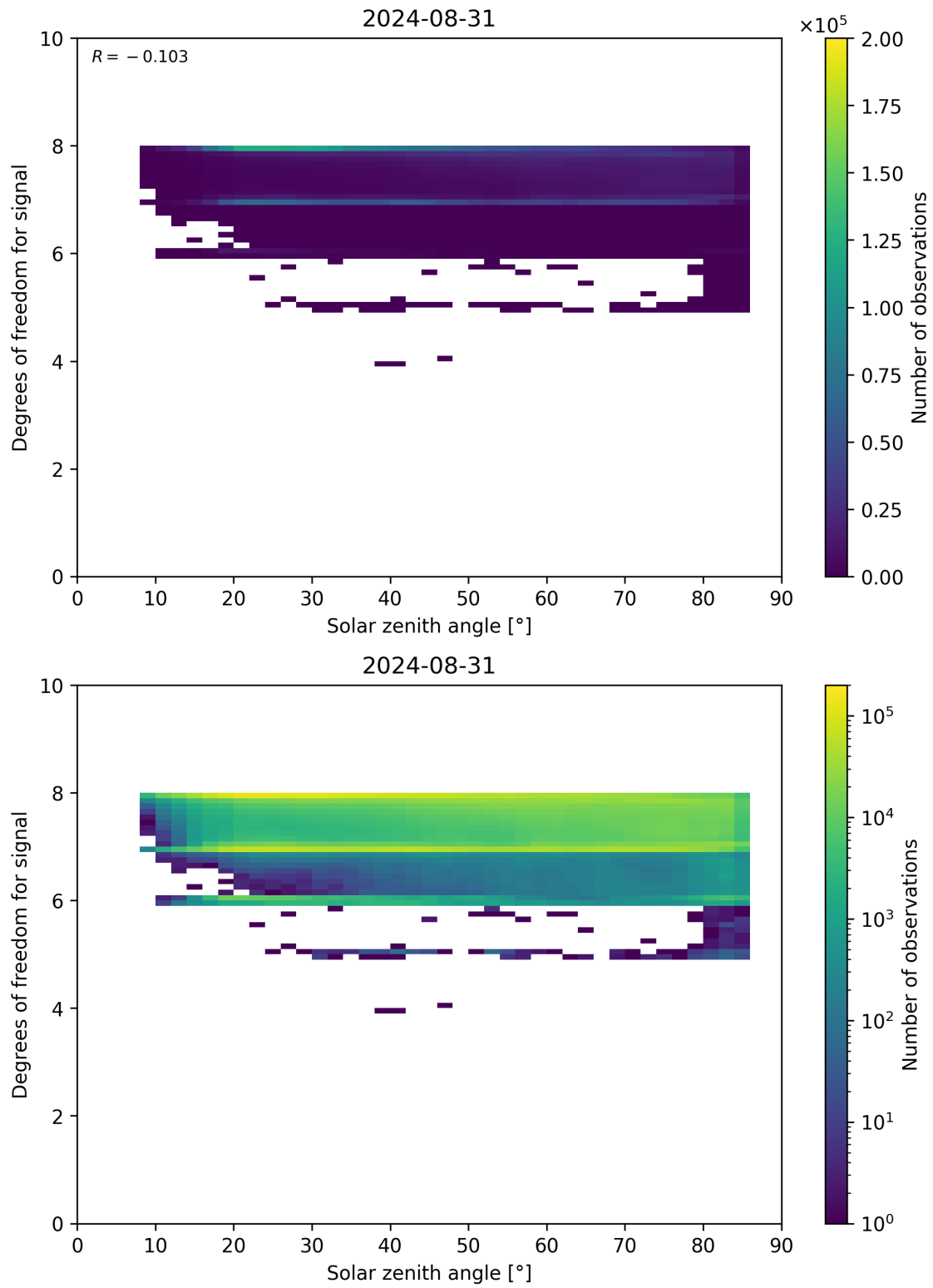
Figure 65: Scatter density plot of “Solar zenith angle” against “Degrees of freedom for signal” for 2024-08-30 to 2024-09-01.
