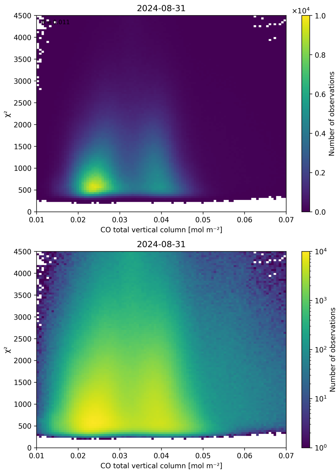
Figure 35: Scatter density plot of “CO total vertical column” against “ \chi^2 ” for 2024-08-30 to 2024-09-01.
