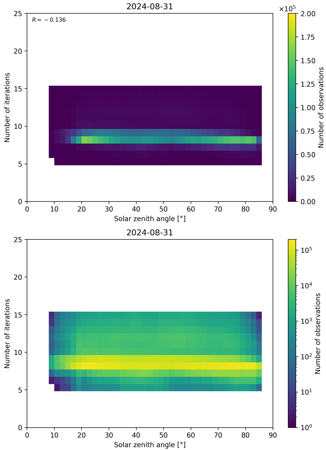
Figure 67: Scatter density plot of “Solar zenith angle” against “Number of iterations” for 2024-08-30 to 2024-09-01.
