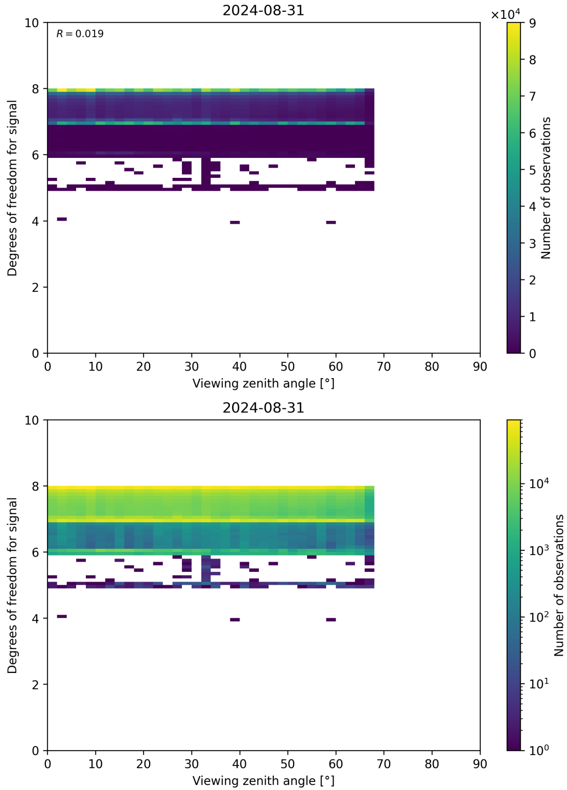
Figure 73: Scatter density plot of “Viewing zenith angle” against “Degrees of freedom for signal” for 2024-08-30 to 2024-09-01.
