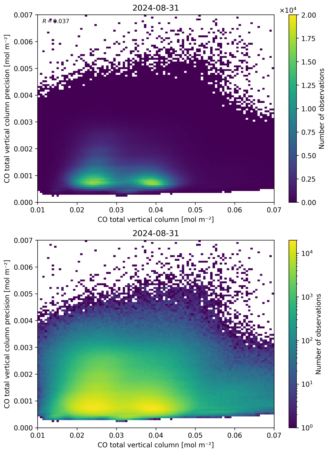
Figure 34: Scatter density plot of “CO total vertical column” against “CO total vertical column precision” for 2024-08-30 to 2024-09-01.
