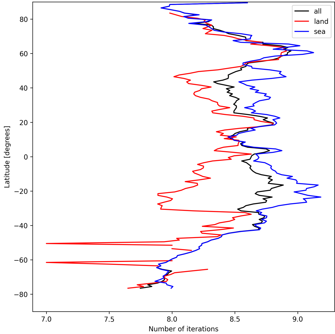
Figure 16: Zonal average of “Number of iterations” for 2024-08-30 to 2024-09-01.
