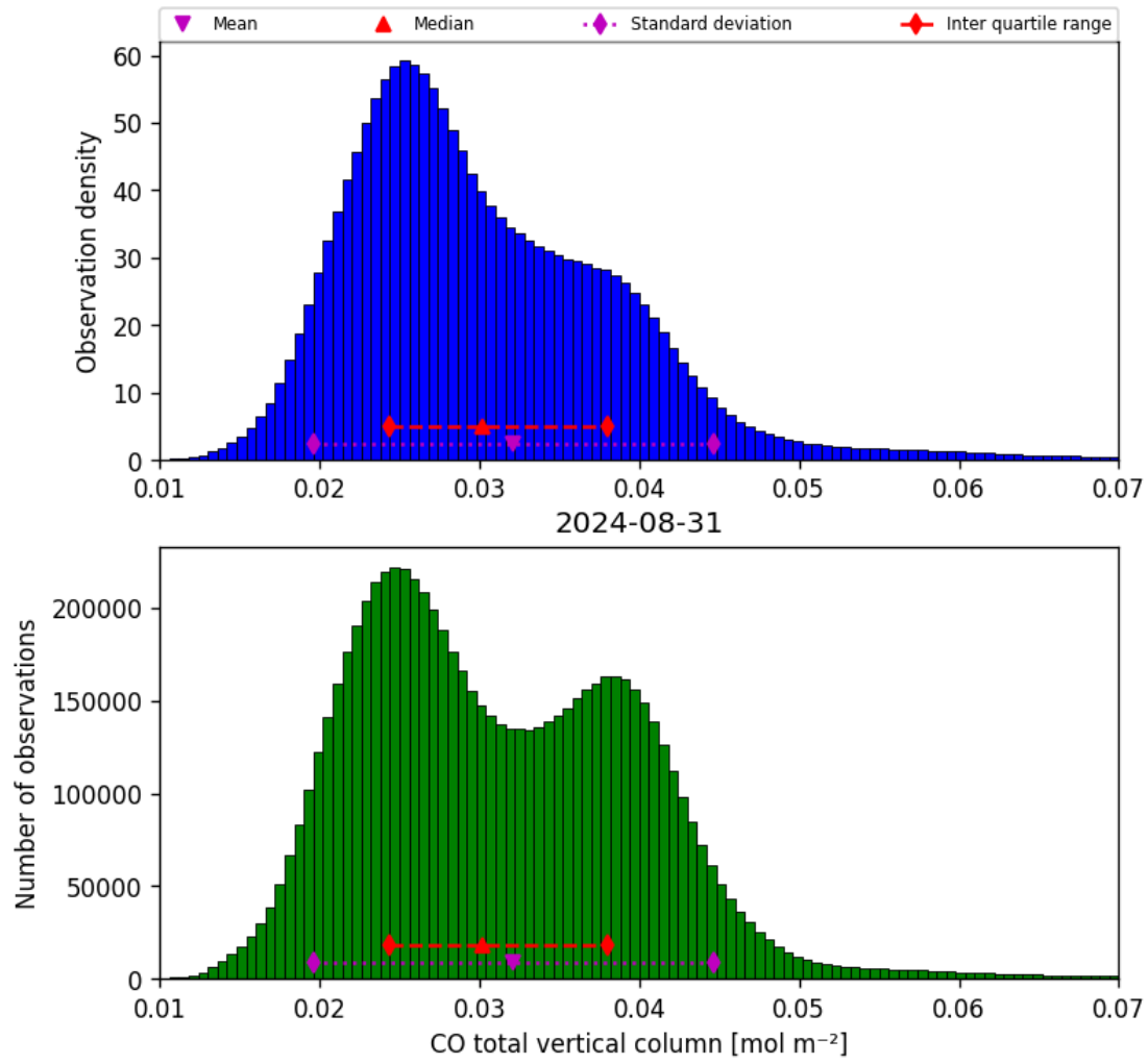
Figure 18: Histogram of “CO total vertical column” for 2024-08-30 to 2024-09-01
