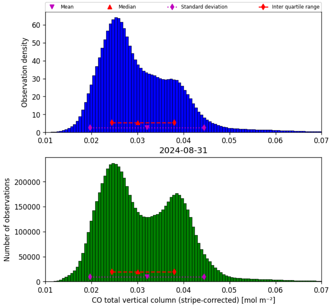
Figure 19: Histogram of “CO total vertical column (stripe-corrected)” for 2024-08-30 to 2024-09-01
