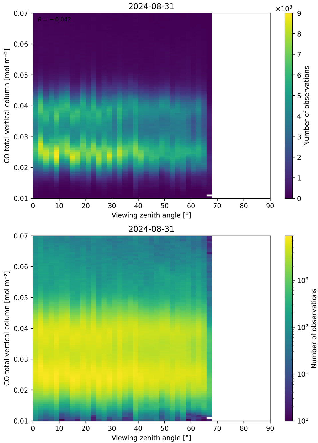
Figure 69: Scatter density plot of “Viewing zenith angle” against “CO total vertical column” for 2024-08-30 to 2024-09-01.
