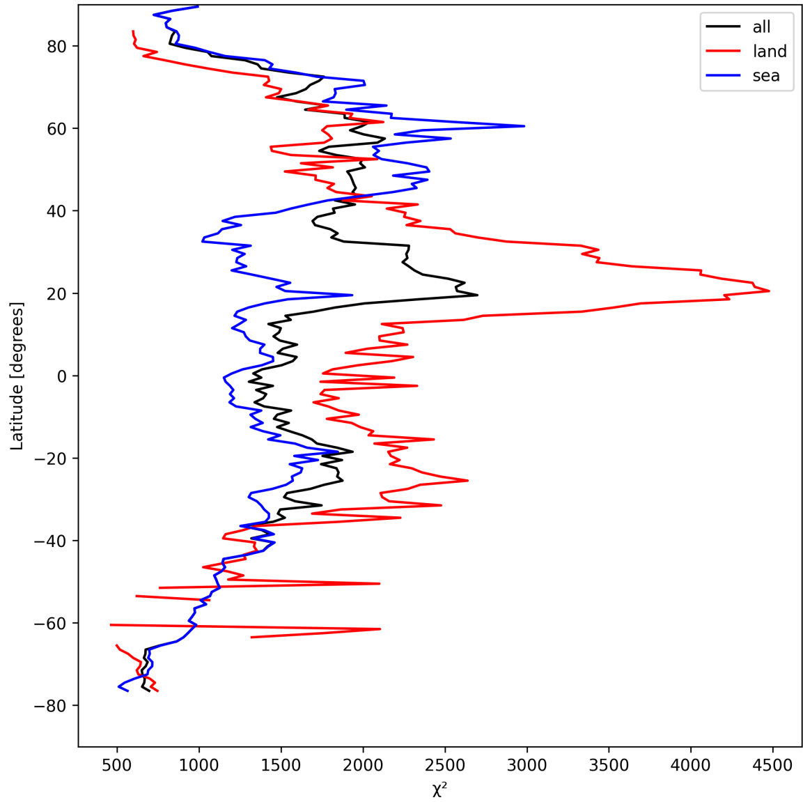
Figure 14: Zonal average of “ \chi^2 ” for 2024-08-30 to 2024-09-01.
