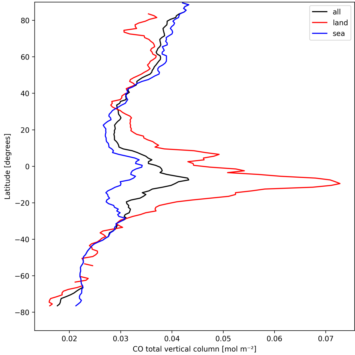
Figure 10: Zonal average of “CO total vertical column” for 2024-08-30 to 2024-09-01.
