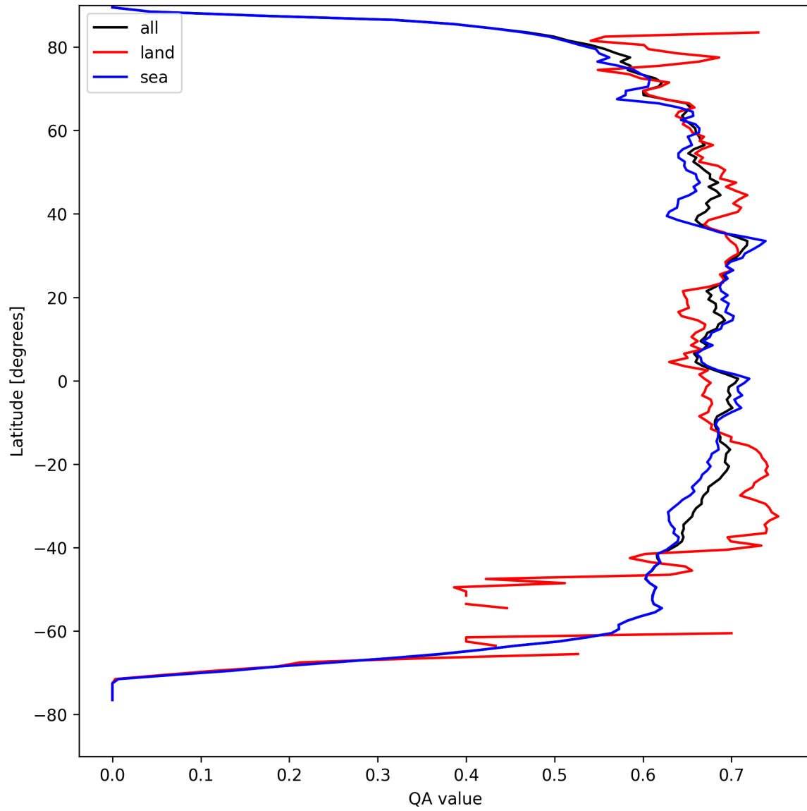
Figure 9: Zonal average of “QA value” for 2024-08-30 to 2024-09-01.
