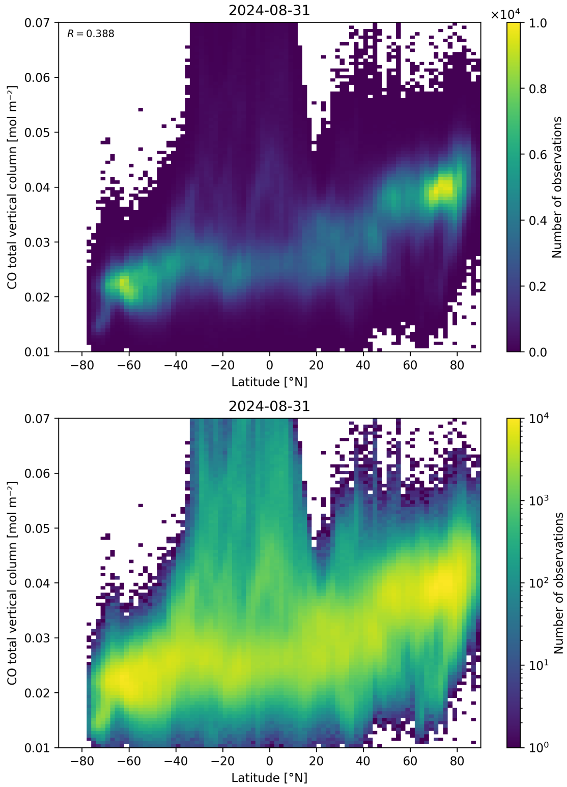
Figure 51: Scatter density plot of “Latitude” against “CO total vertical column” for 2024-08-30 to 2024-09-01.
