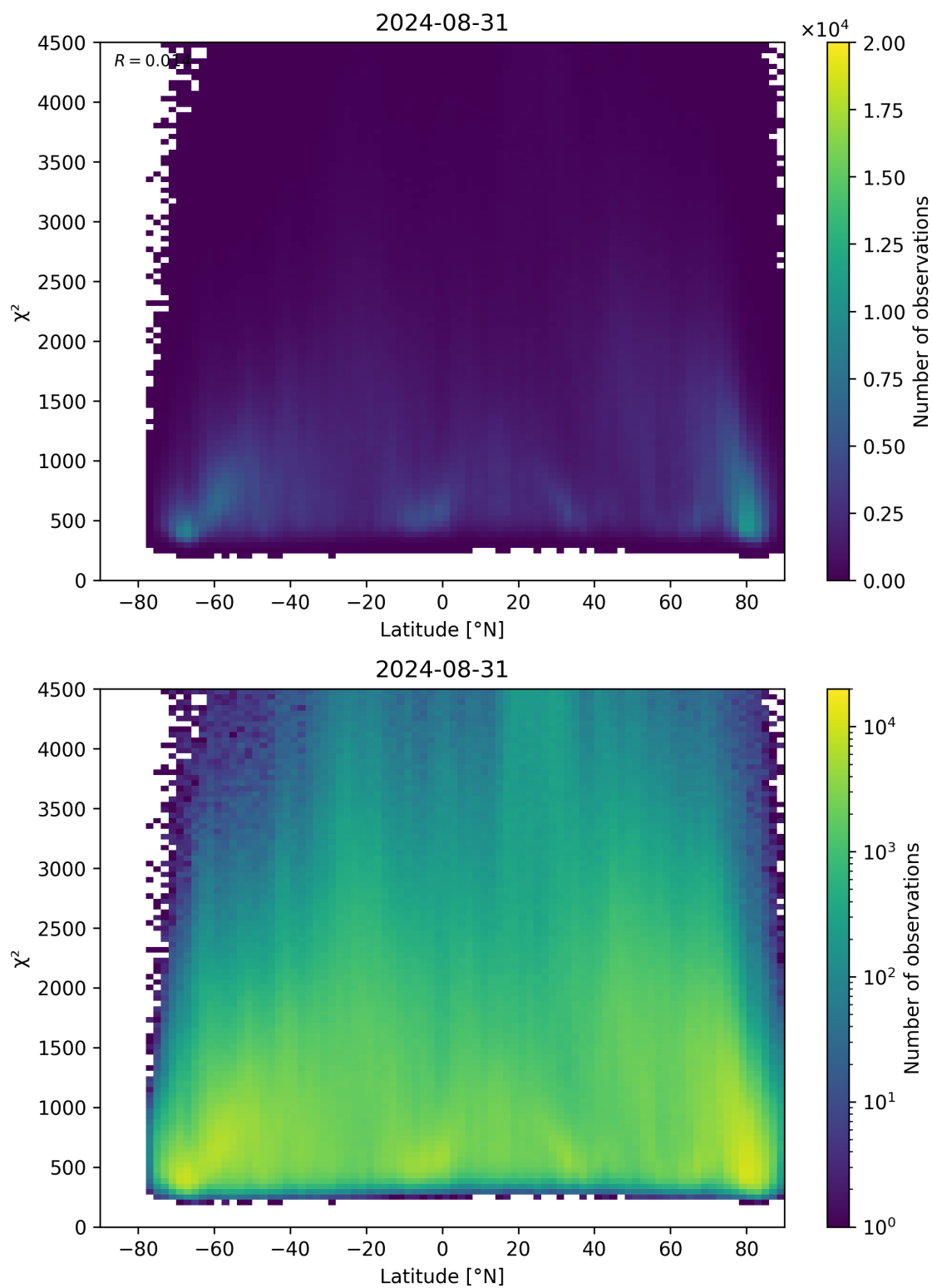
Figure 54: Scatter density plot of “Latitude” against “ \chi^2 ” for 2024-08-30 to 2024-09-01.
