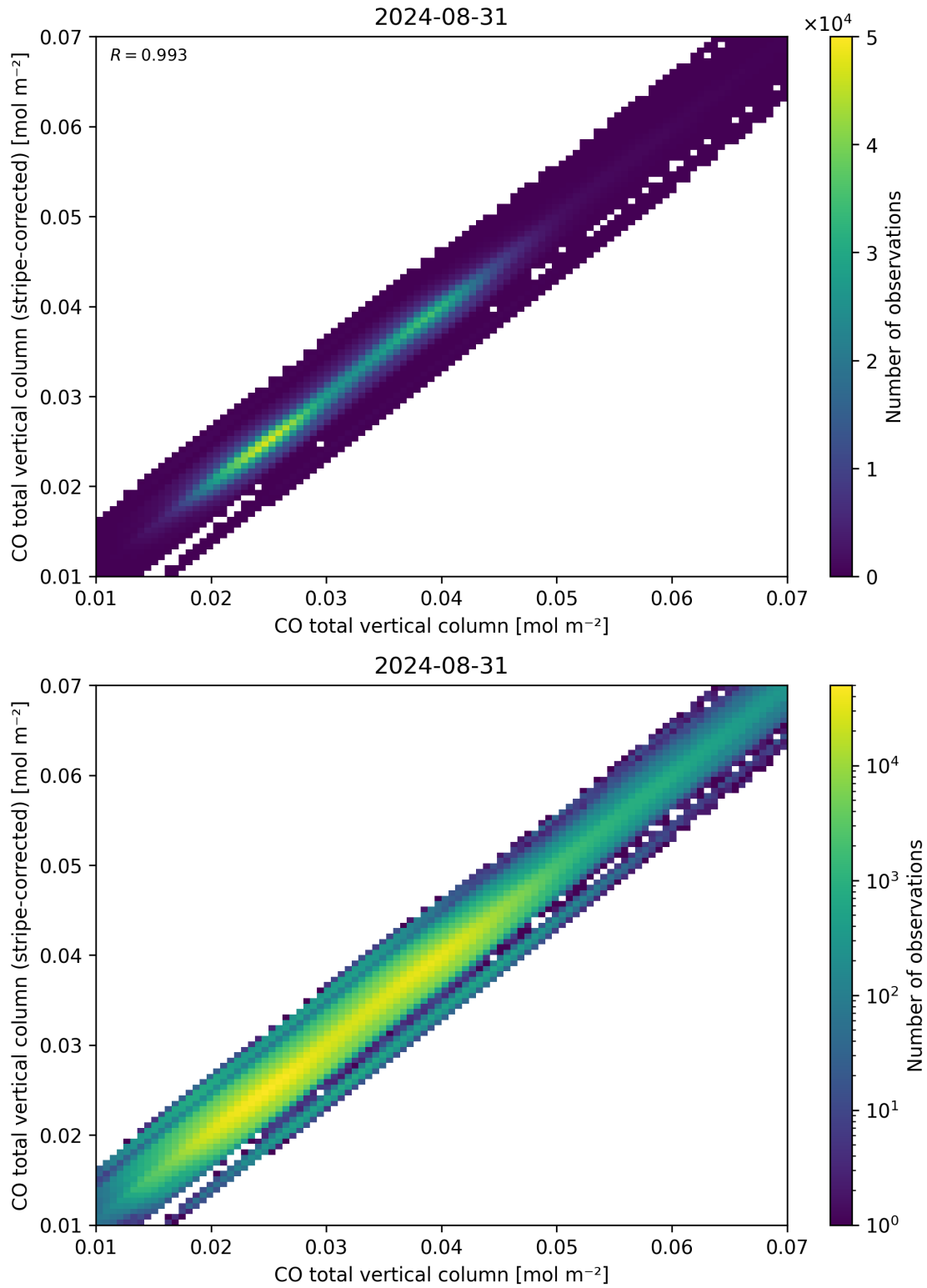
Figure 33: Scatter density plot of “CO total vertical column” against “CO total vertical column (stripe-corrected)” for 2024-08-30 to 2024-09-01.
