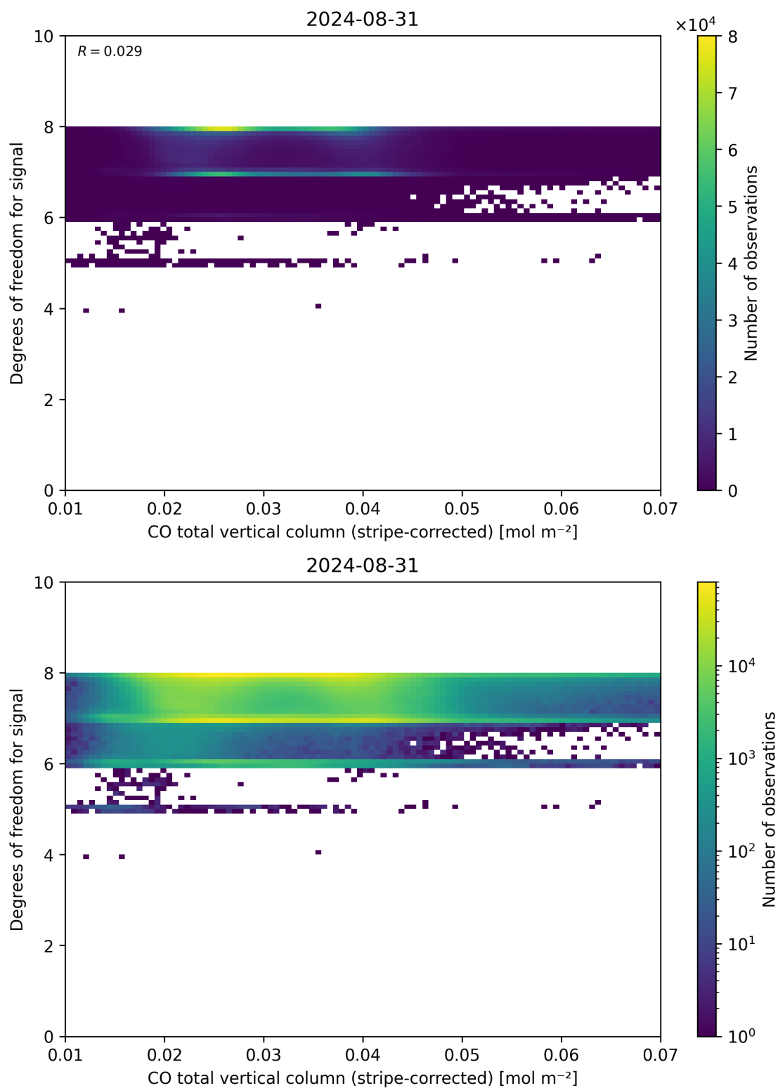
Figure 38: Scatter density plot of “CO total vertical column (stripe-corrected)” against “Degrees of freedom for signal” for 2024-08-30 to 2024-09-01.
