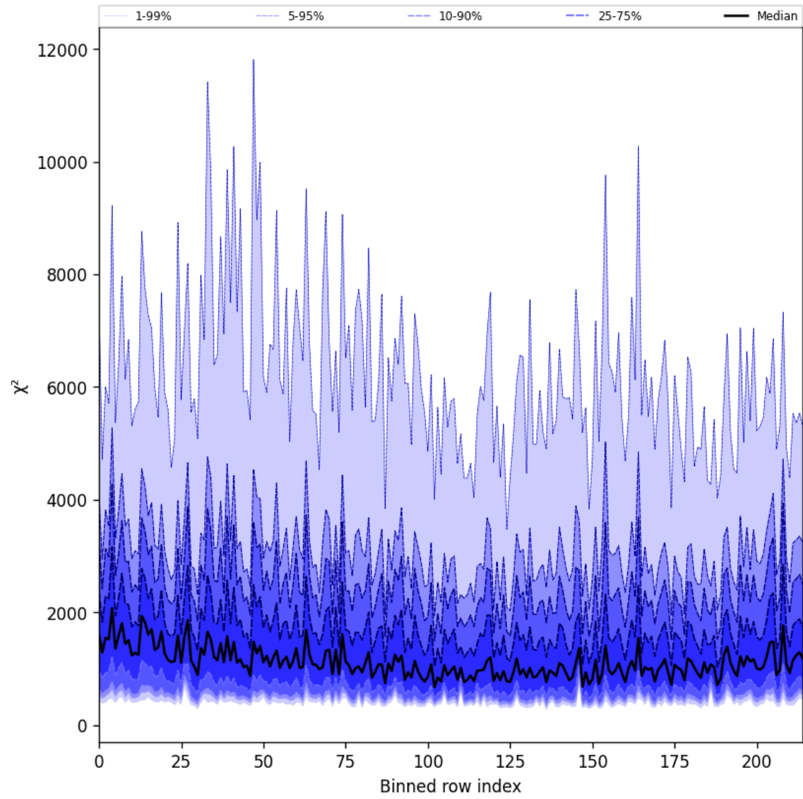
Figure 30: Along track statistics of “ \chi^2 ” for 2024-08-30 to 2024-09-01
