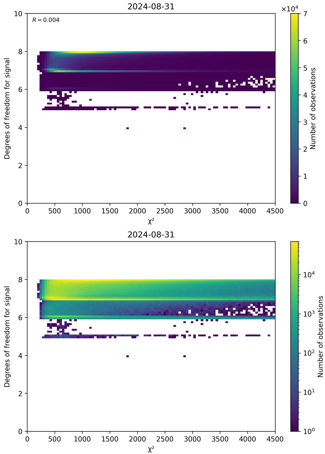
Figure 48: Scatter density plot of “ \chi^2 ” against “Degrees of freedom for signal” for 2024-08-30 to 2024-09-01.
