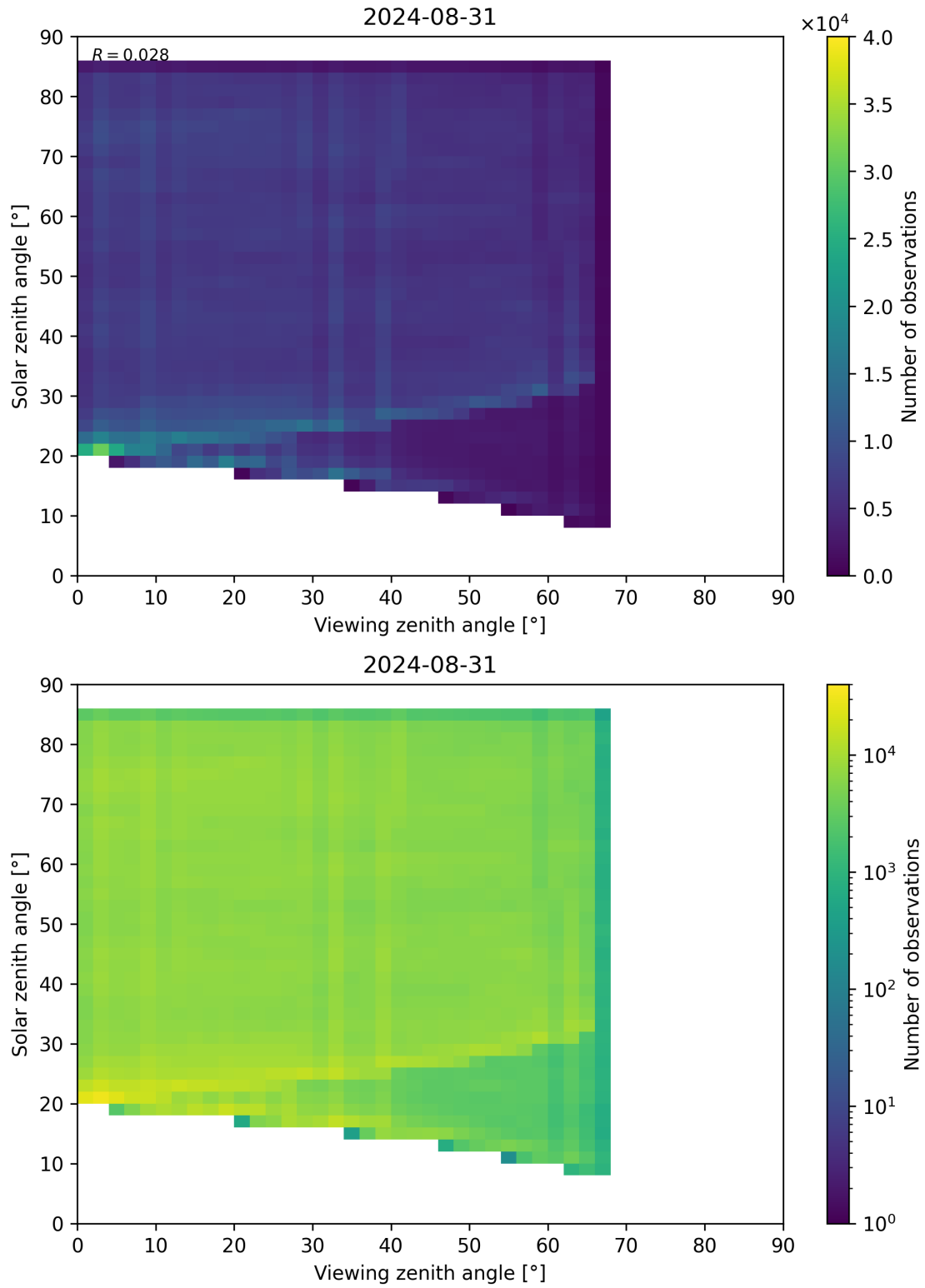
Figure 77: Scatter density plot of “Viewing zenith angle” against “Solar zenith angle” for 2024-08-30 to 2024-09-01.
