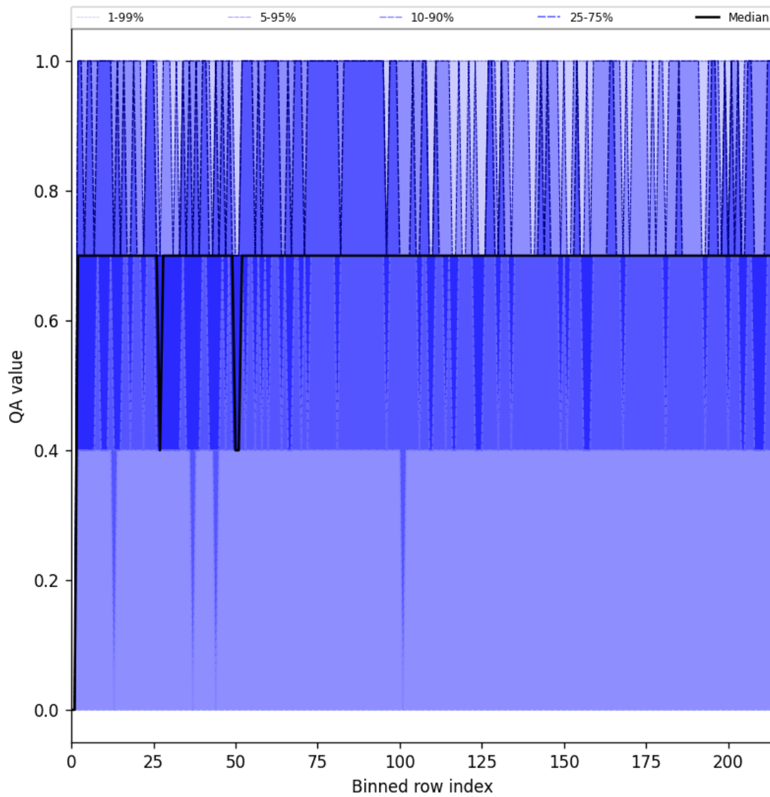
Figure 25: Along track statistics of “QA value” for 2024-08-30 to 2024-09-01
