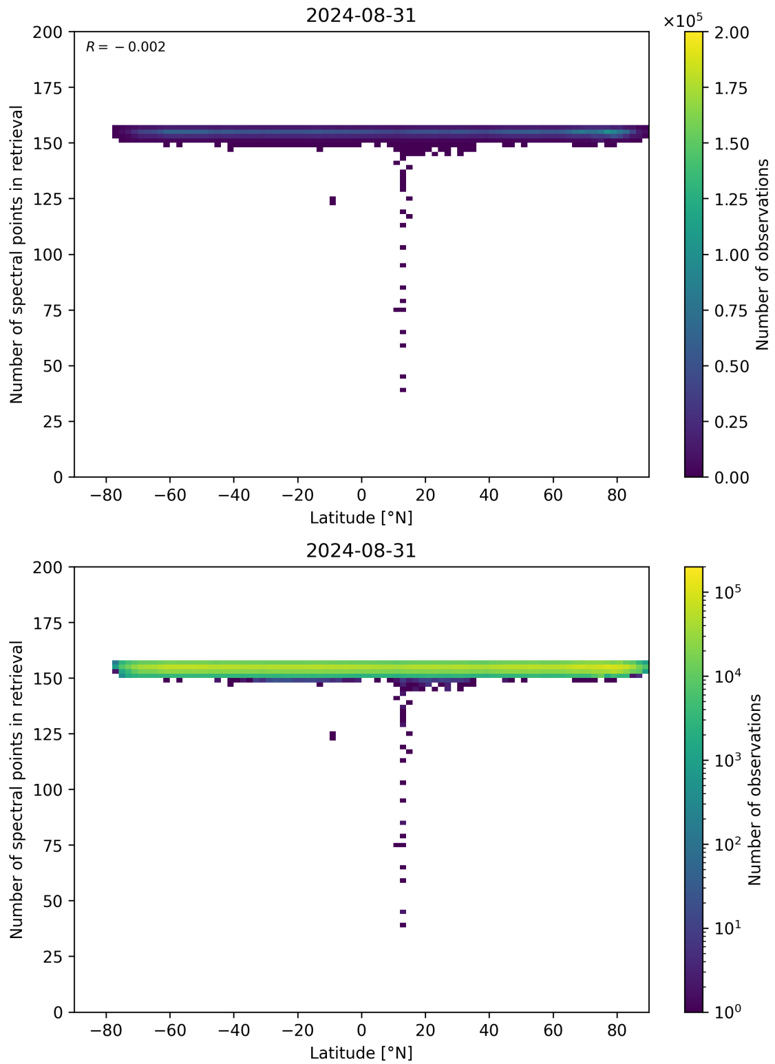
Figure 57: Scatter density plot of “Latitude” against “Number of spectral points in retrieval” for 2024-08-30 to 2024-09-01.
