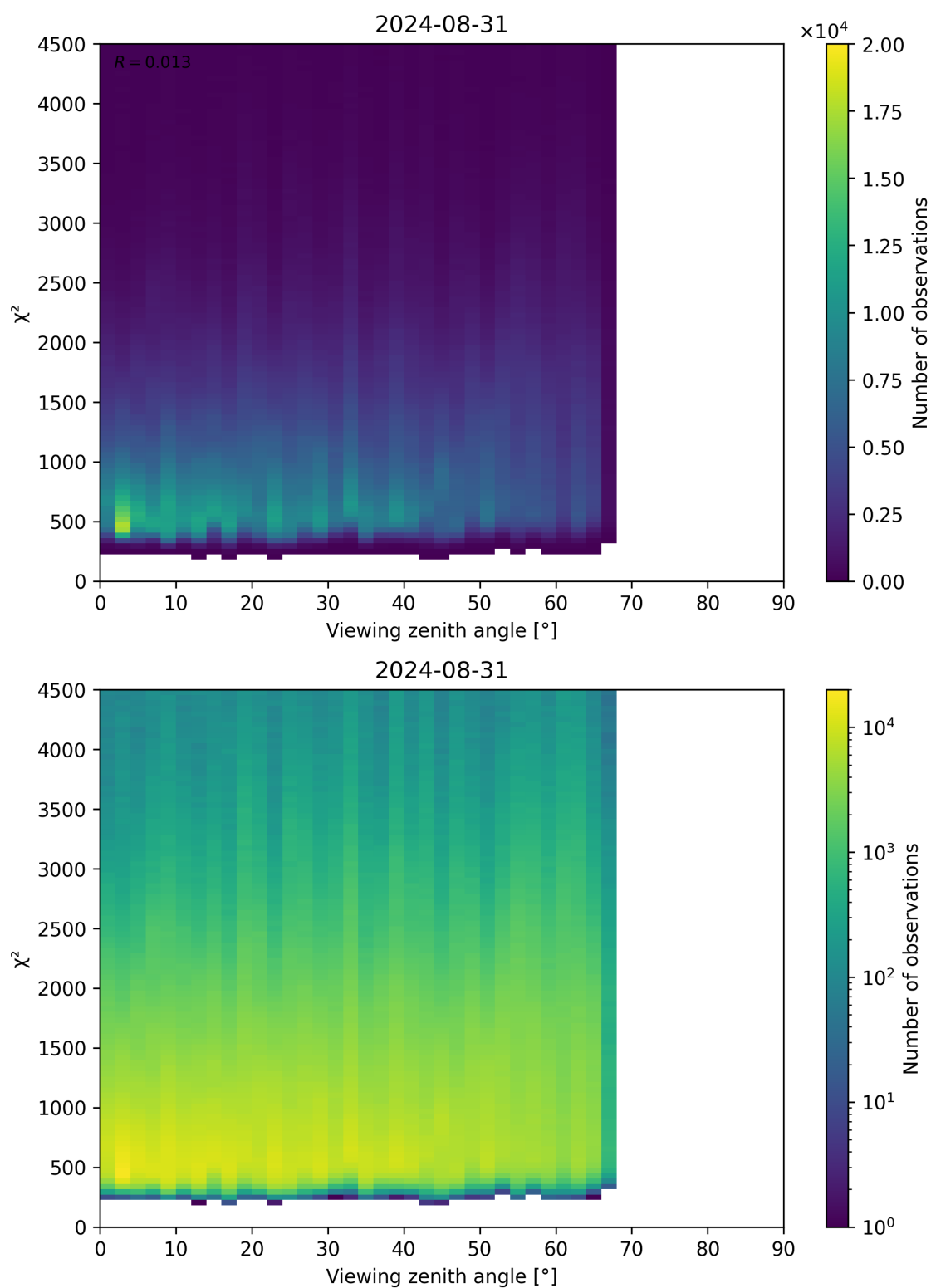
Figure 72: Scatter density plot of “Viewing zenith angle” against “ \chi^2 ” for 2024-08-30 to 2024-09-01.
