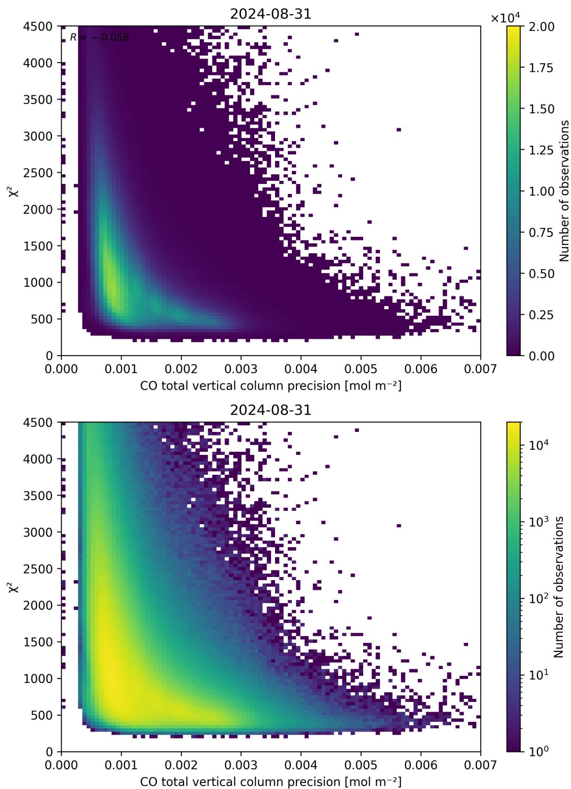
Figure 44: Scatter density plot of “CO total vertical column precision” against “ \chi^2 ” for 2024-08-30 to 2024-09-01.
