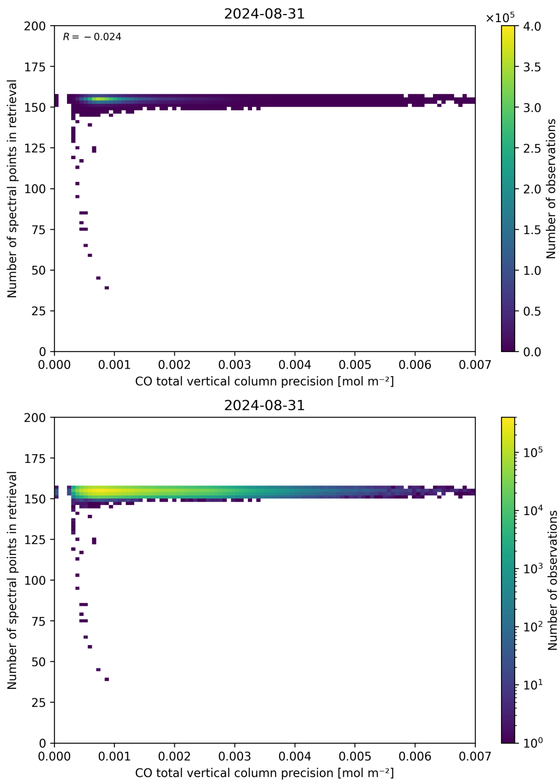
Figure 47: Scatter density plot of “CO total vertical column precision” against “Number of spectral points in retrieval” for 2024-08-30 to 2024-09-01.
