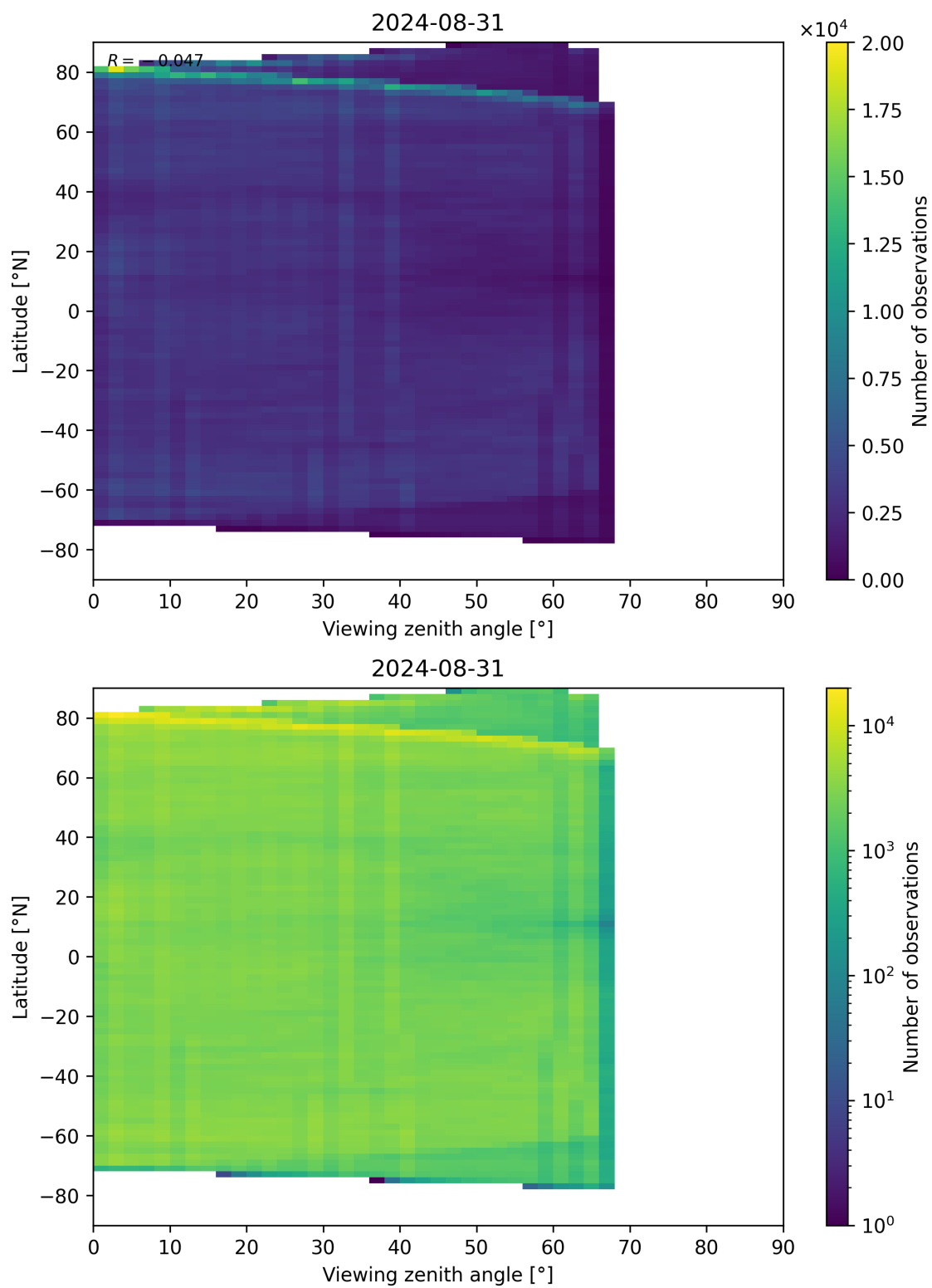
Figure 74: Scatter density plot of “Viewing zenith angle” against “Latitude” for 2024-08-30 to 2024-09-01.
