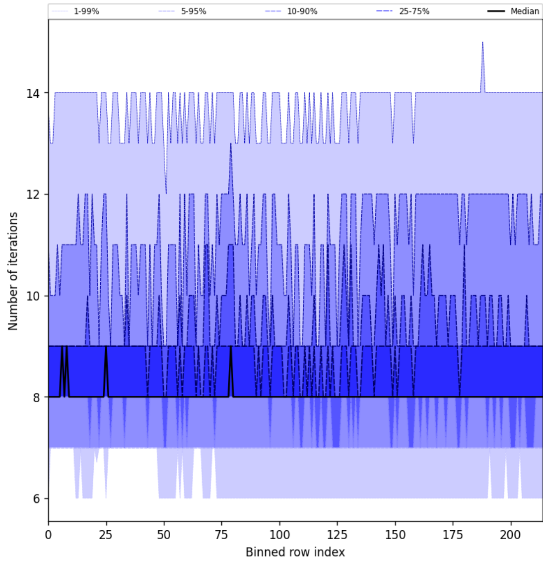
Figure 32: Along track statistics of “Number of iterations” for 2024-08-30 to 2024-09-01
