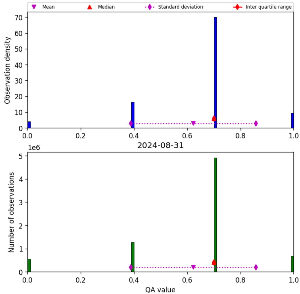
Figure 17: Histogram of “QA value” for 2024-08-30 to 2024-09-01
