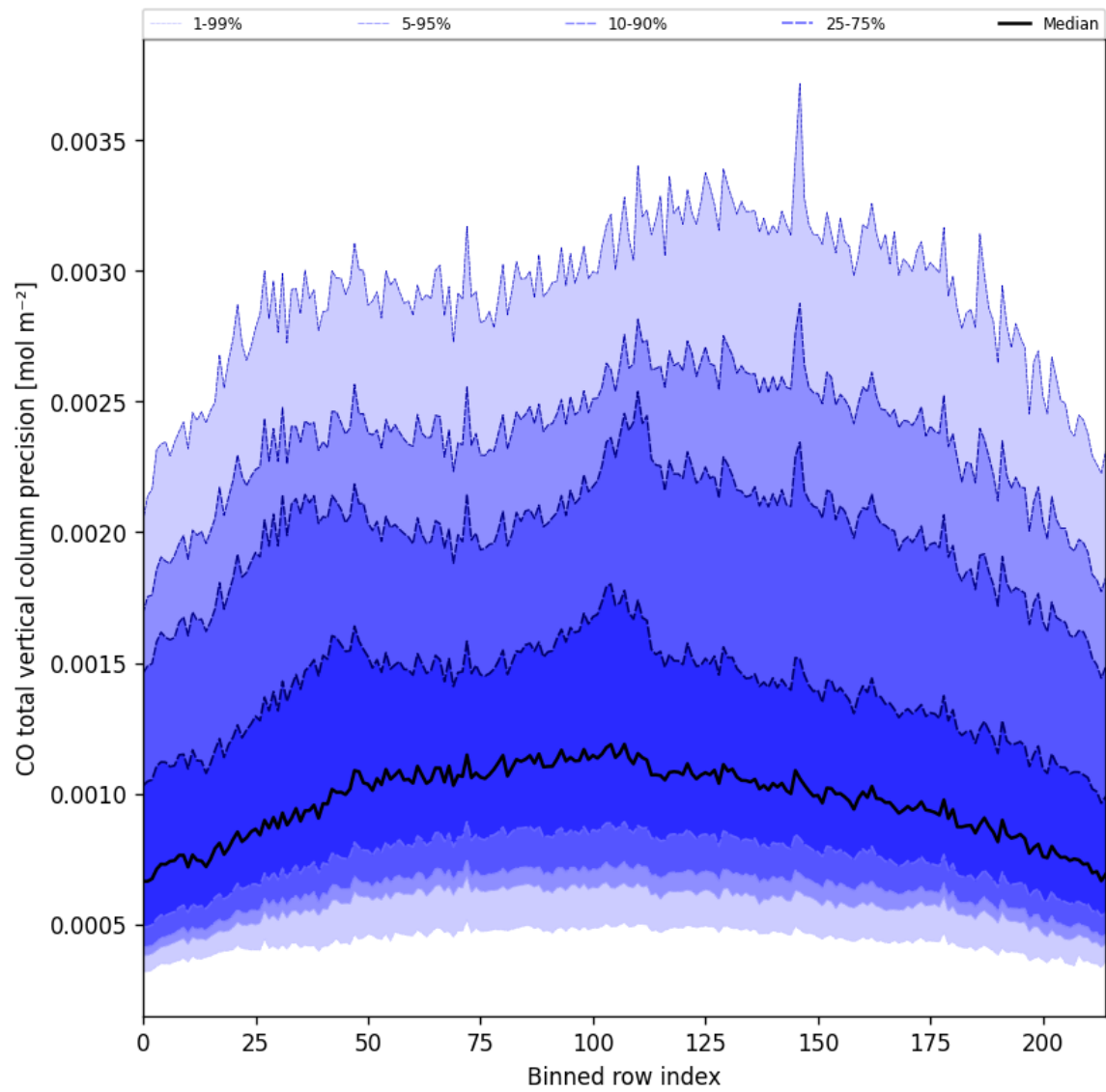
Figure 28: Along track statistics of “CO total vertical column precision” for 2024-08-30 to 2024-09-01
