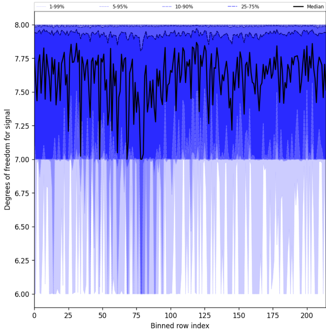
Figure 31: Along track statistics of “Degrees of freedom for signal” for 2024-08-30 to 2024-09-01
