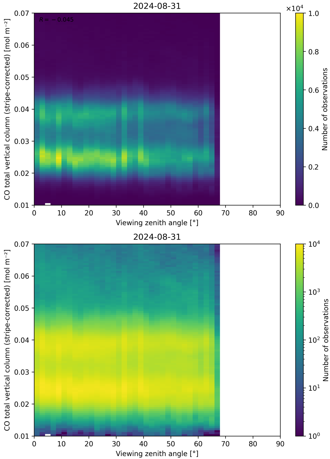
Figure 70: Scatter density plot of “Viewing zenith angle” against “CO total vertical column (stripe-corrected)” for 2024-08-30 to 2024-09-01.
