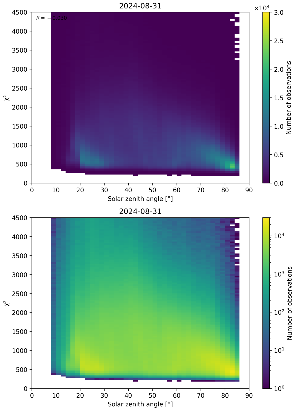
Figure 64: Scatter density plot of “Solar zenith angle” against “ \chi^2 ” for 2024-08-30 to 2024-09-01.
