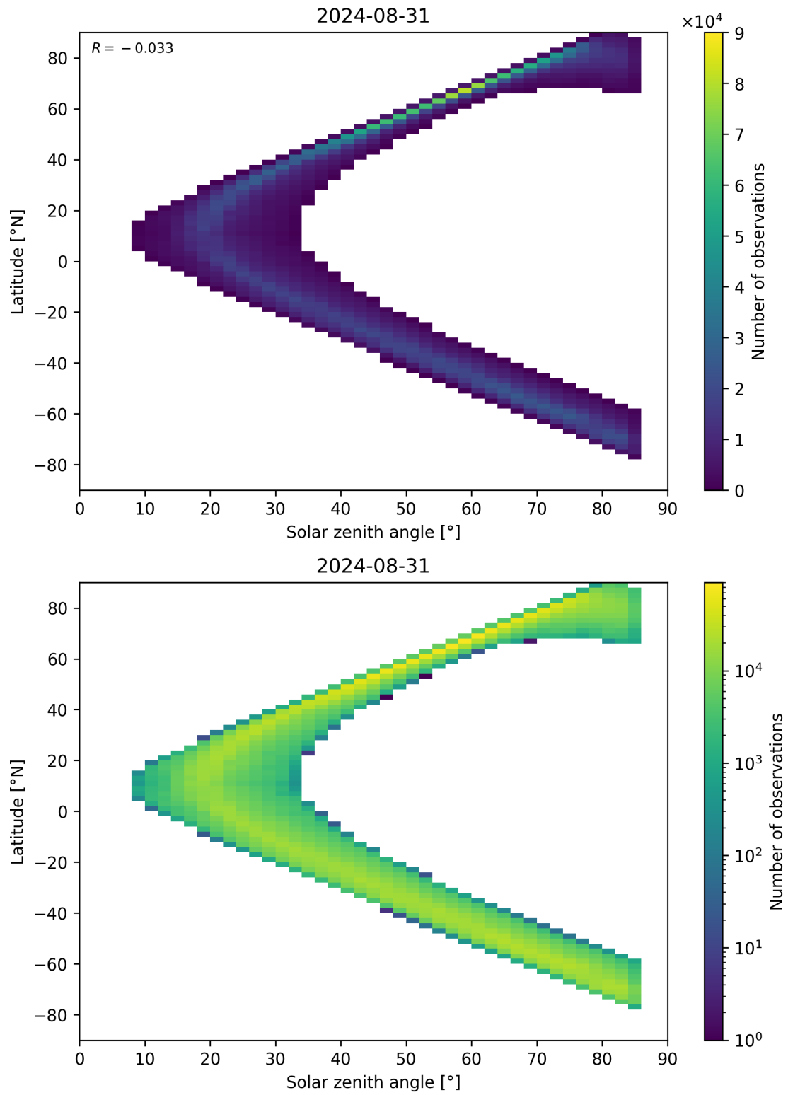
Figure 66: Scatter density plot of “Solar zenith angle” against “Latitude” for 2024-08-30 to 2024-09-01.
