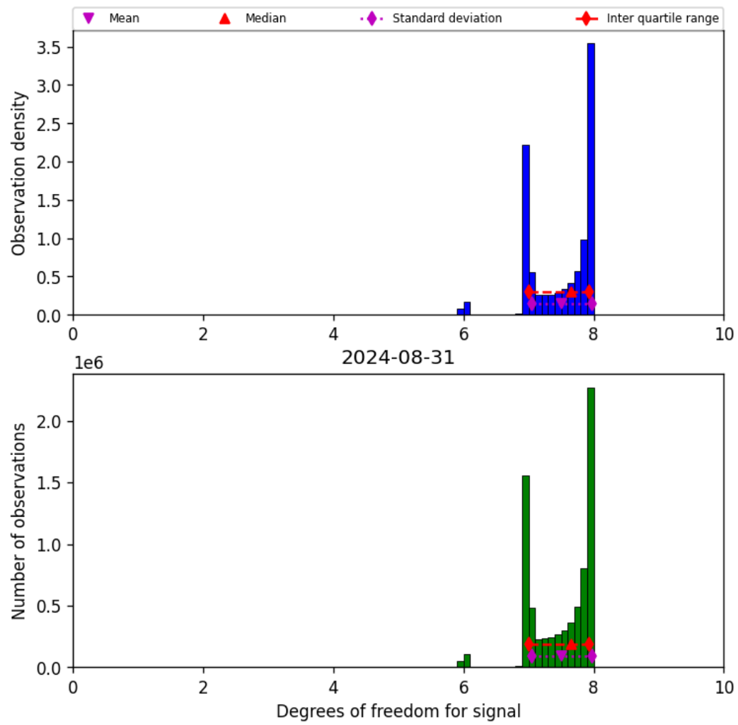
Figure 23: Histogram of “Degrees of freedom for signal” for 2024-08-30 to 2024-09-01
