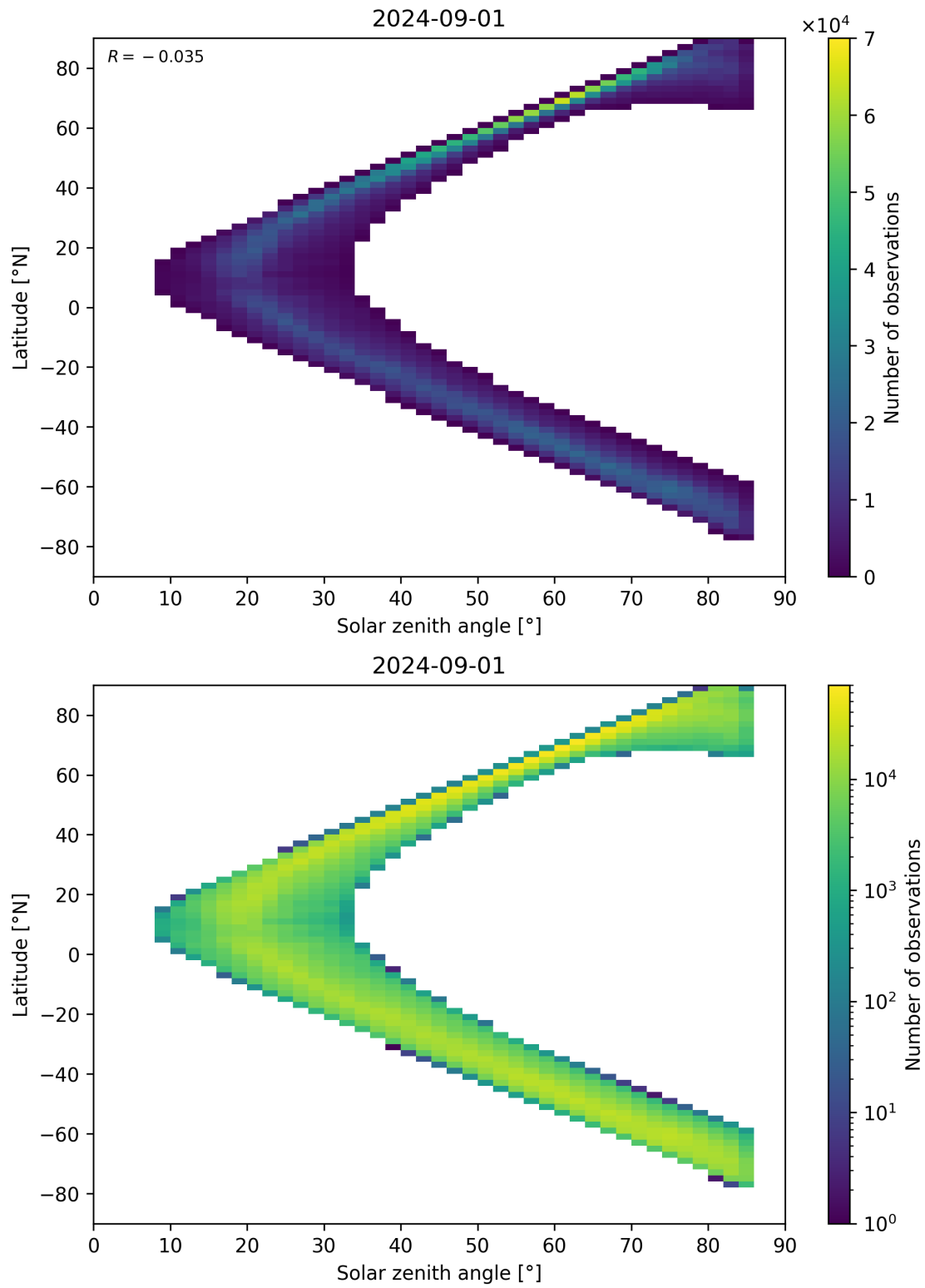
Figure 66: Scatter density plot of “Solar zenith angle” against “Latitude” for 2024-09-01 to 2024-09-02.
