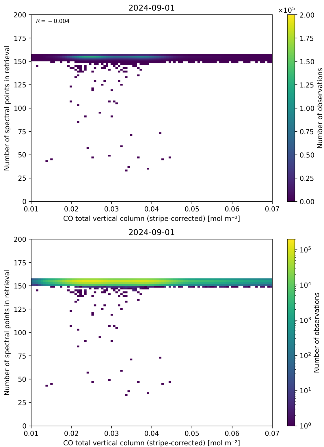
Figure 40: Scatter density plot of “CO total vertical column (stripe-corrected)” against “Number of spectral points in retrieval” for 2024-09-01 to 2024-09-02.
