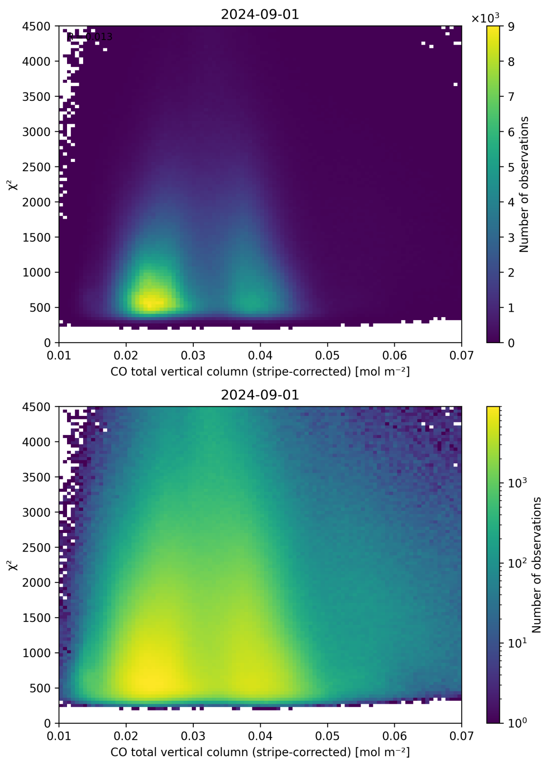
Figure 37: Scatter density plot of “CO total vertical column (stripe-corrected)” against “ \chi^2 ” for 2024-09-01 to 2024-09-02.
