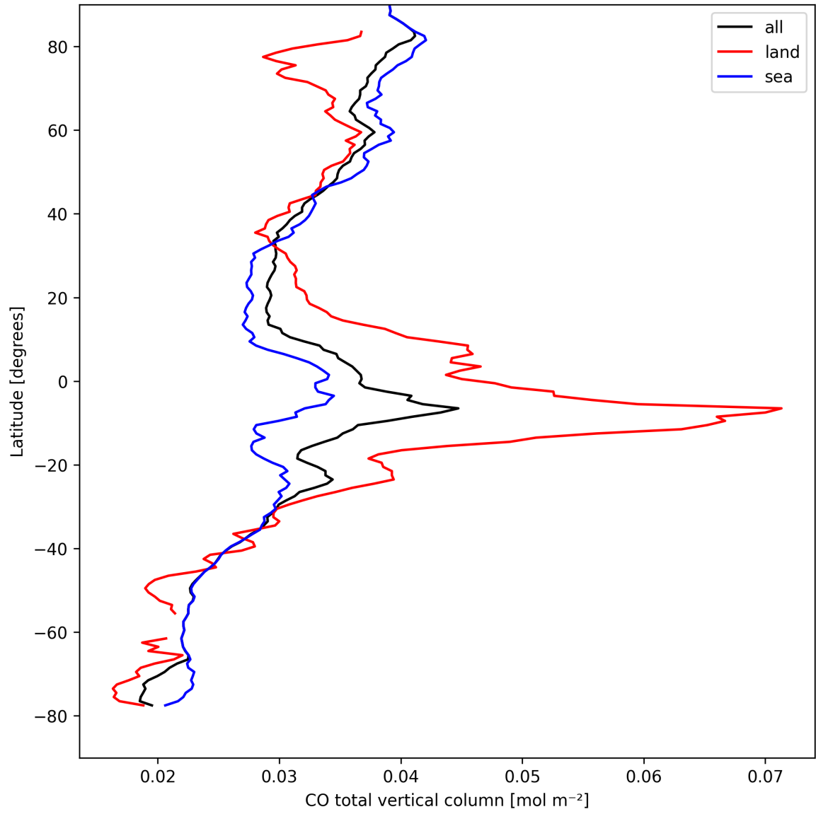
Figure 10: Zonal average of “CO total vertical column” for 2024-09-01 to 2024-09-02.
