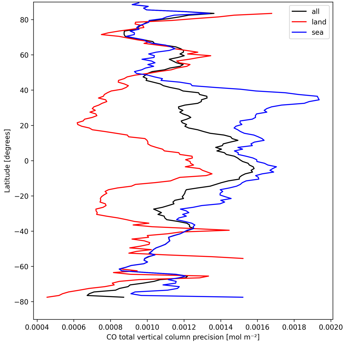
Figure 12: Zonal average of "CO total vertical column precision" for 2024-09-01 to 2024-09-02.
