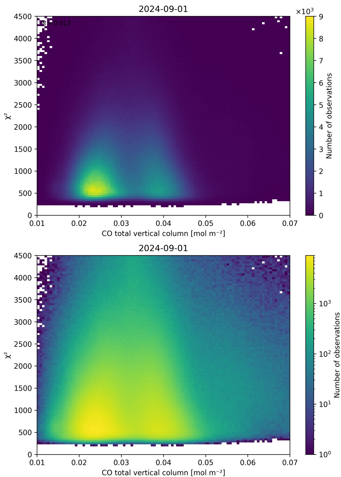
Figure 35: Scatter density plot of “CO total vertical column” against “ \chi^2 ” for 2024-09-01 to 2024-09-02.
