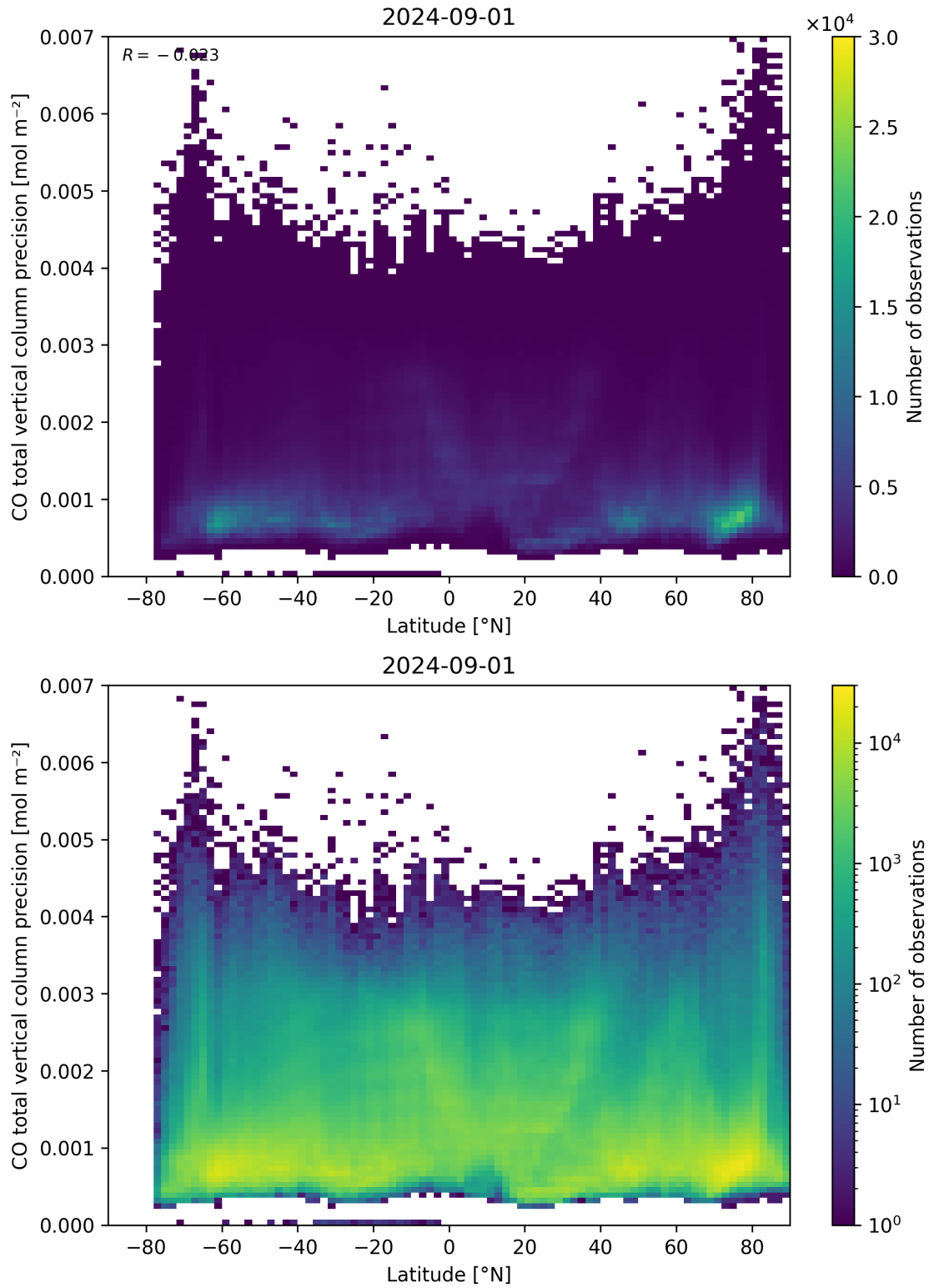
Figure 53: Scatter density plot of “Latitude” against “CO total vertical column precision” for 2024-09-01 to 2024-09-02.
