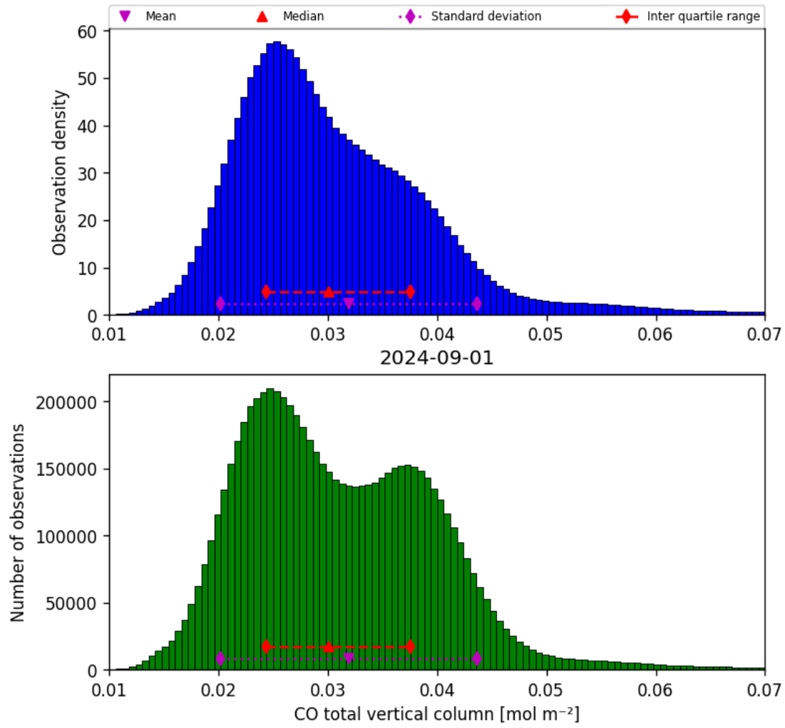
Figure 18: Histogram of “CO total vertical column” for 2024-09-01 to 2024-09-02
