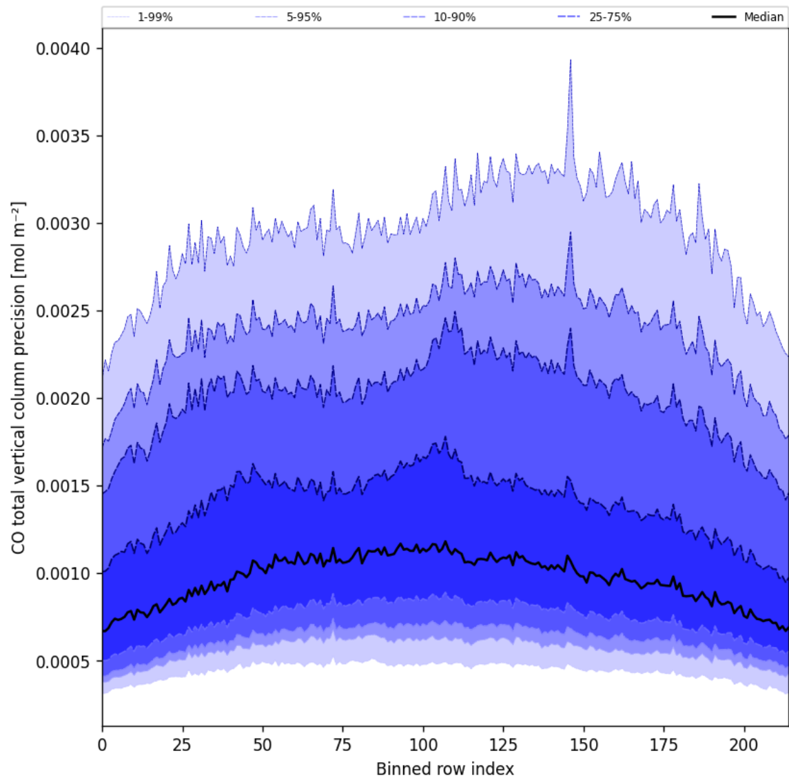
Figure 28: Along track statistics of “CO total vertical column precision” for 2024-09-01 to 2024-09-02
