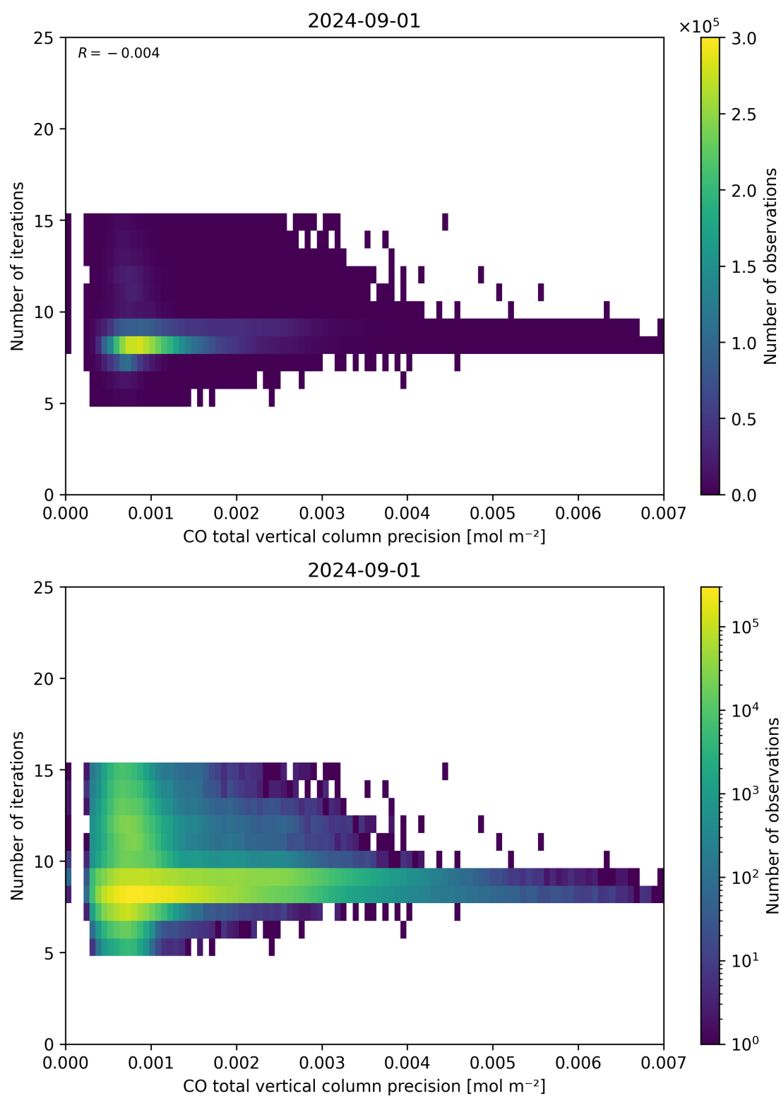
Figure 46: Scatter density plot of “CO total vertical column precision” against “Number of iterations” for 2024-09-01 to 2024-09-02.
