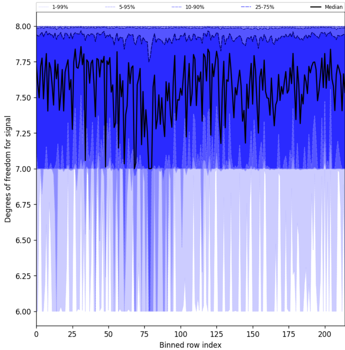
Figure 31: Along track statistics of “Degrees of freedom for signal” for 2024-09-01 to 2024-09-02
