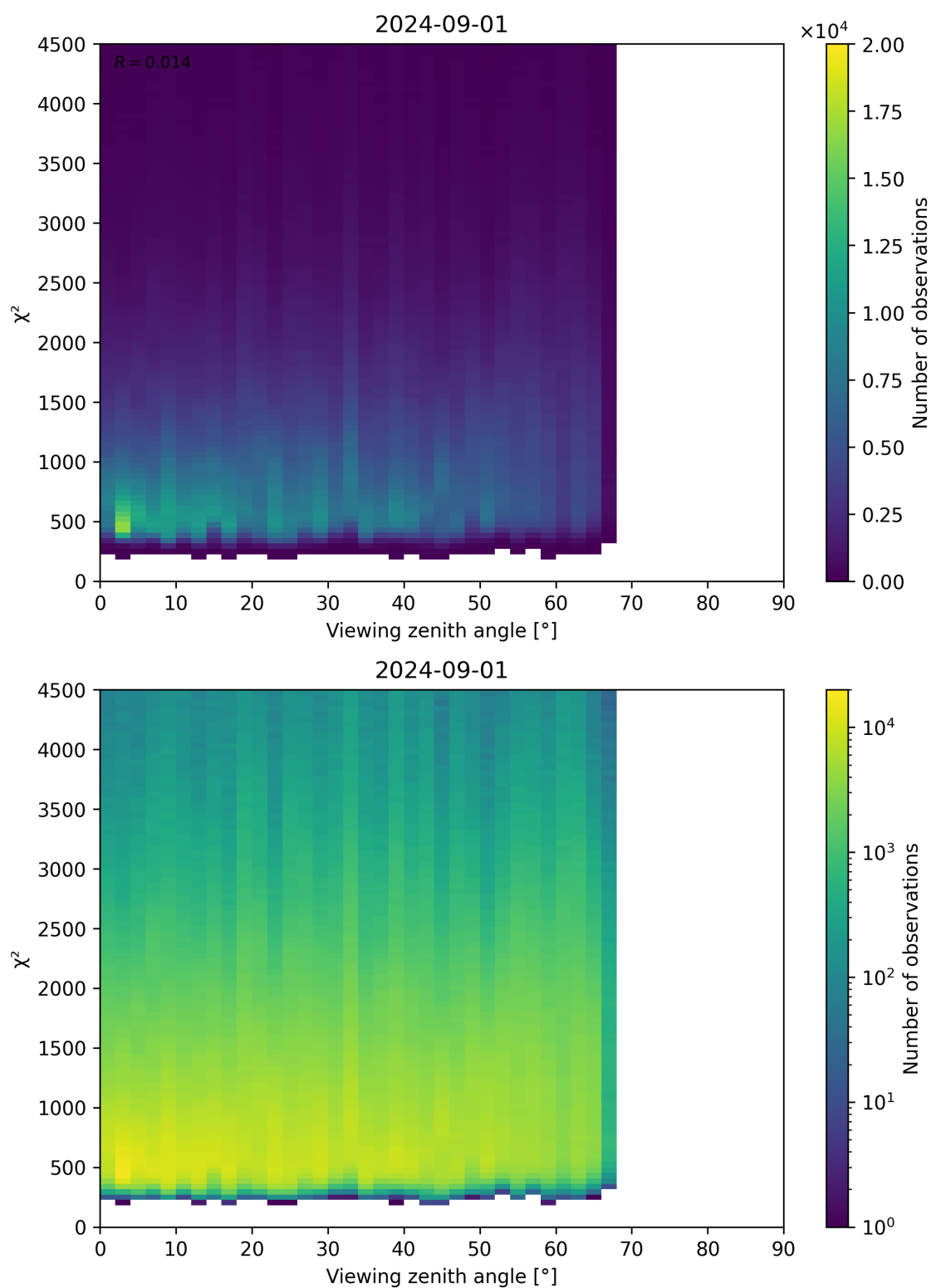
Figure 72: Scatter density plot of “Viewing zenith angle” against “ \chi^2 ” for 2024-09-01 to 2024-09-02.
