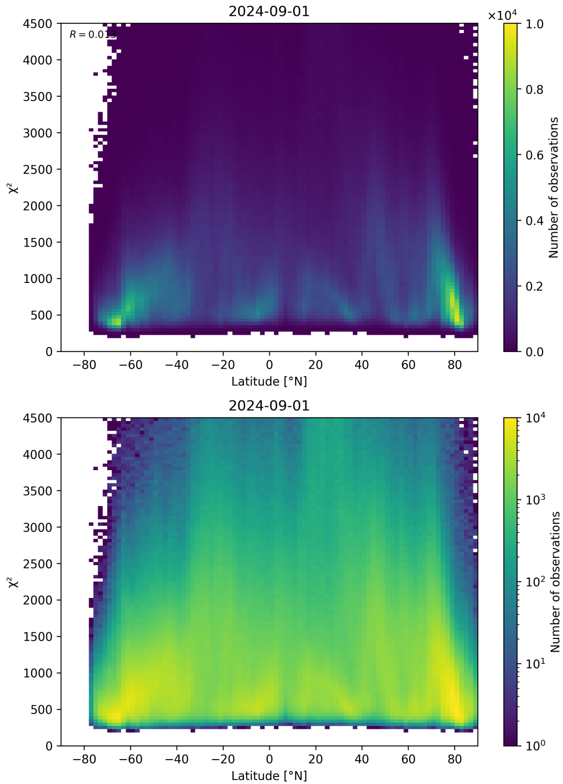
Figure 54: Scatter density plot of “Latitude” against “ \chi^2 ” for 2024-09-01 to 2024-09-02.
