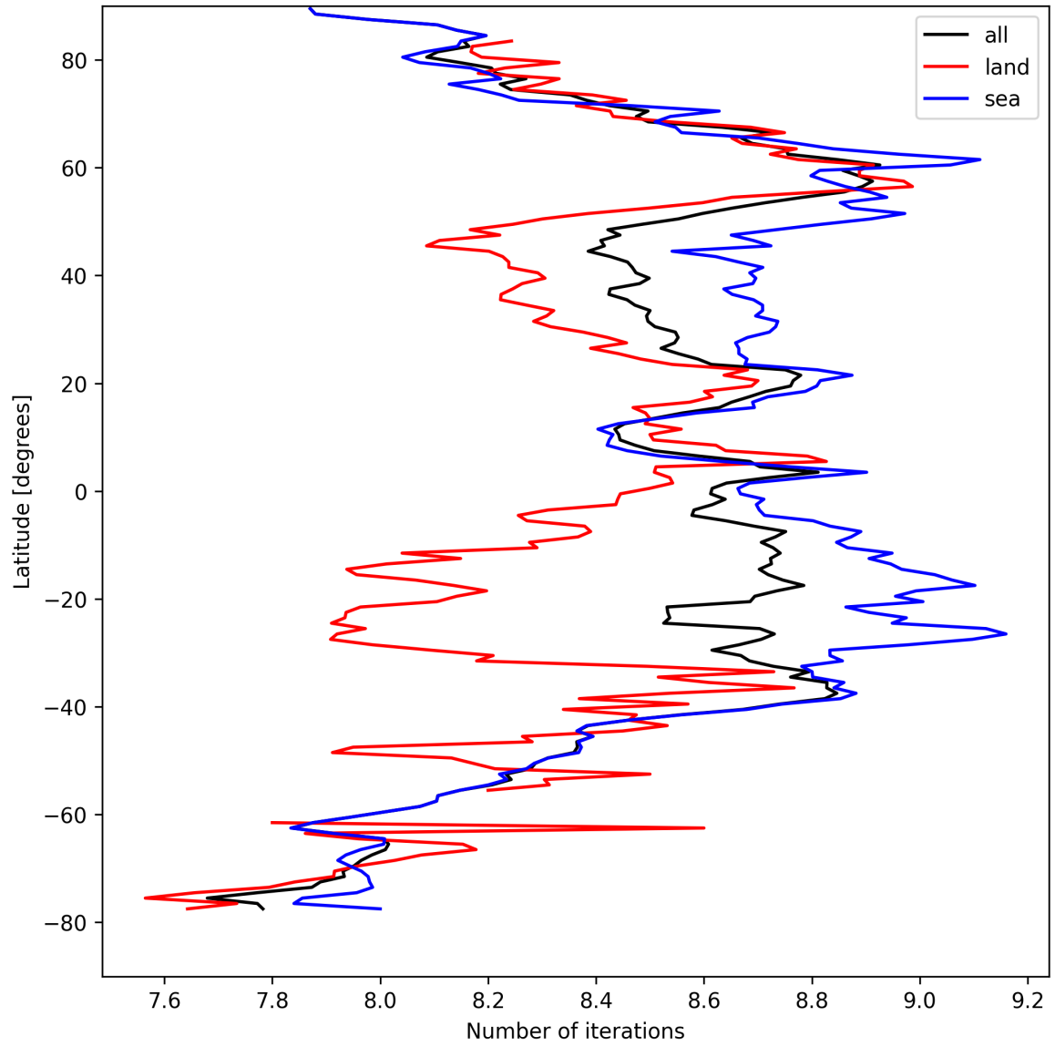
Figure 16: Zonal average of “Number of iterations” for 2024-09-01 to 2024-09-02.
