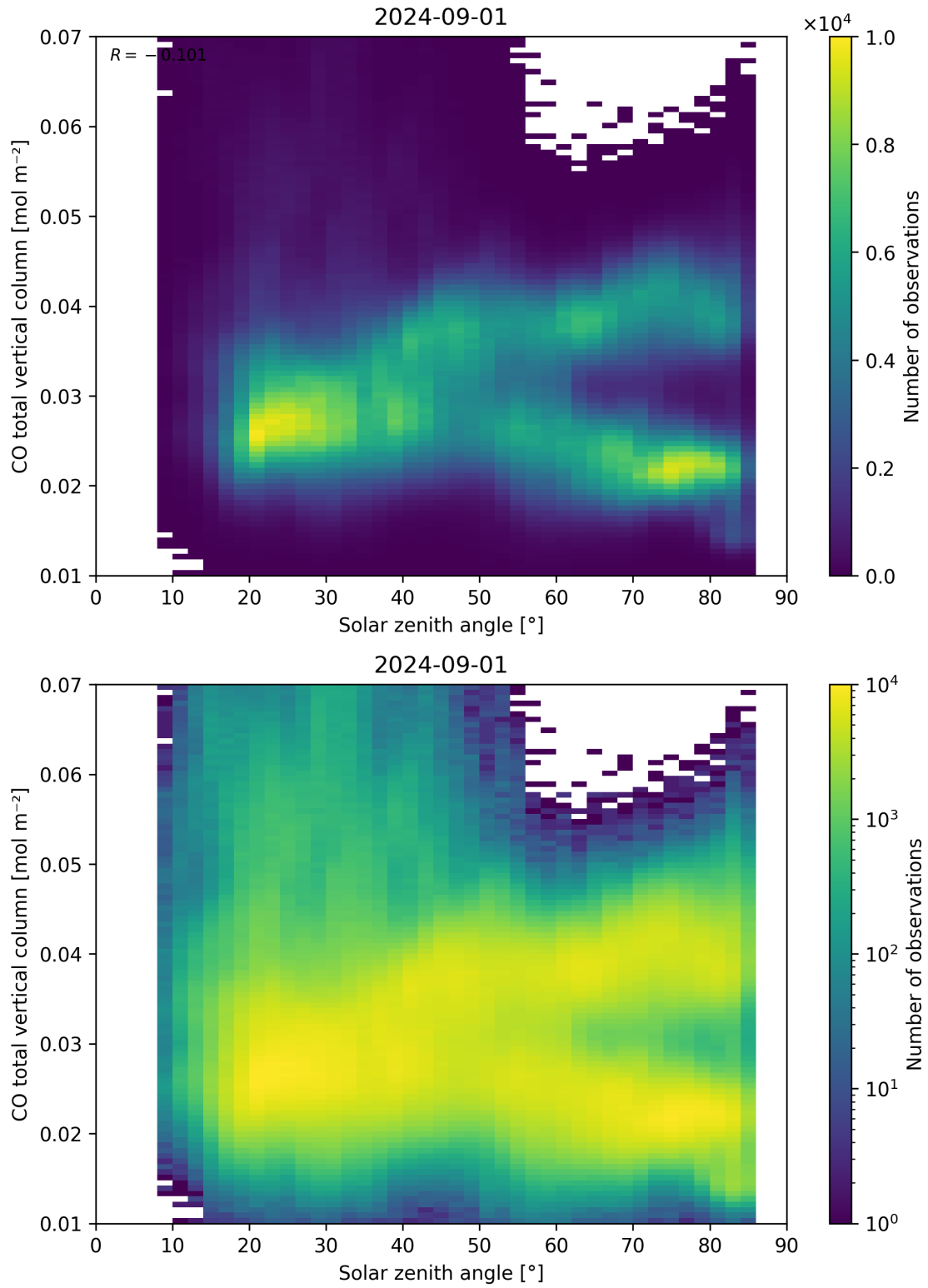
Figure 61: Scatter density plot of “Solar zenith angle” against “CO total vertical column” for 2024-09-01 to 2024-09-02.
