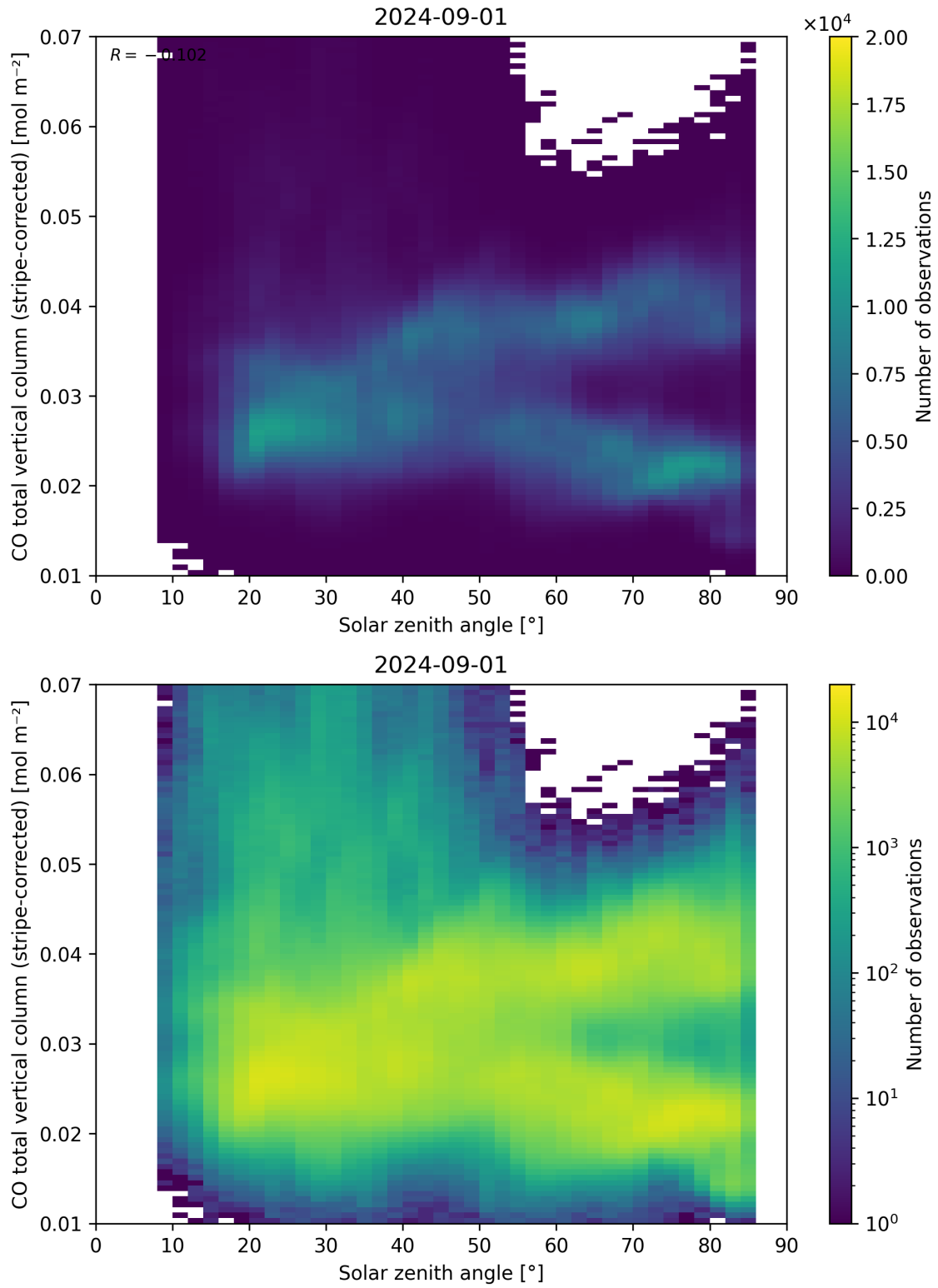
Figure 62: Scatter density plot of “Solar zenith angle” against “CO total vertical column (stripe-corrected)” for 2024-09-01 to 2024-09-02.
