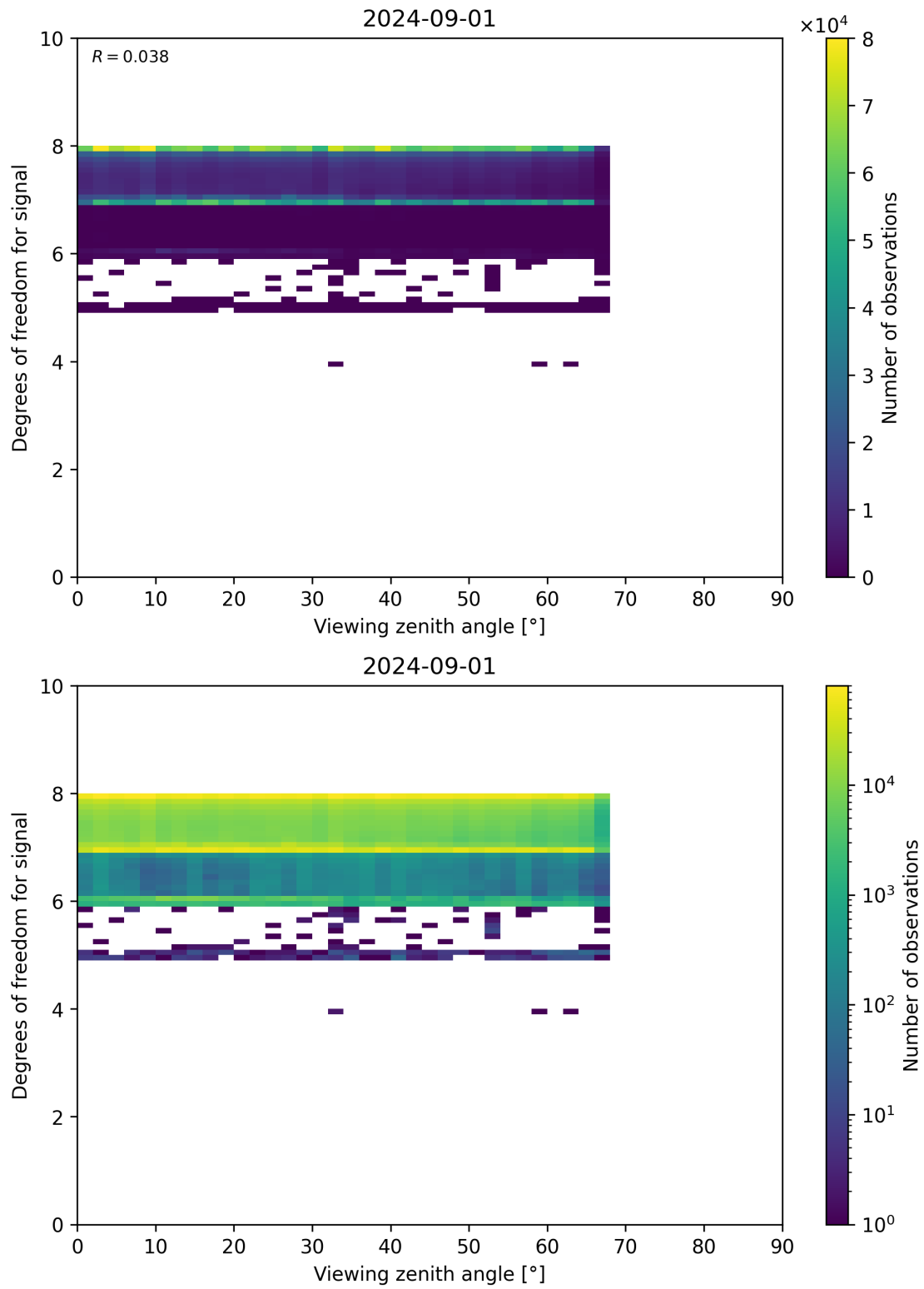
Figure 73: Scatter density plot of “Viewing zenith angle” against “Degrees of freedom for signal” for 2024-09-01 to 2024-09-02.
