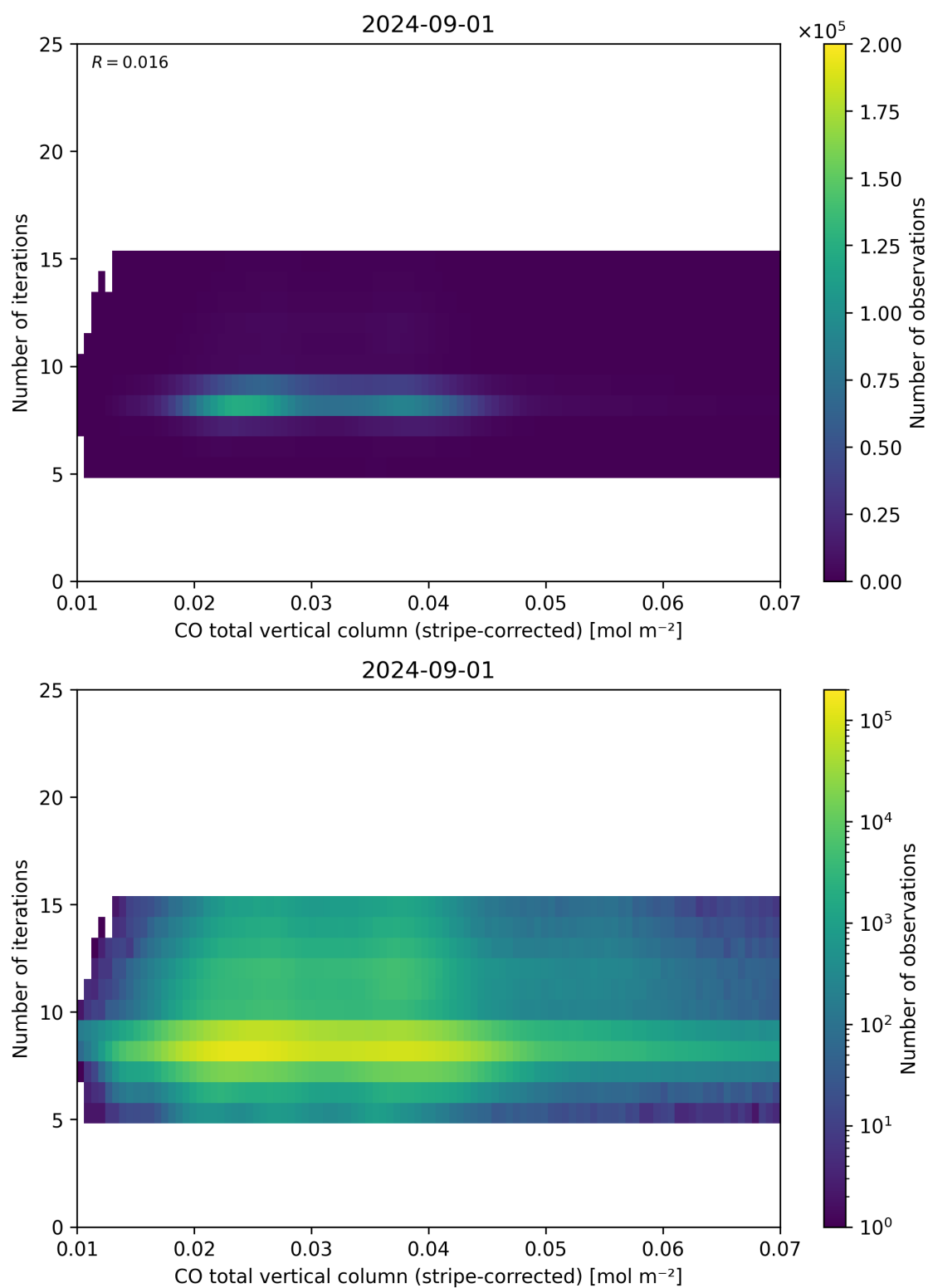
Figure 39: Scatter density plot of “CO total vertical column (stripe-corrected)” against “Number of iterations” for 2024-09-01 to 2024-09-02.
