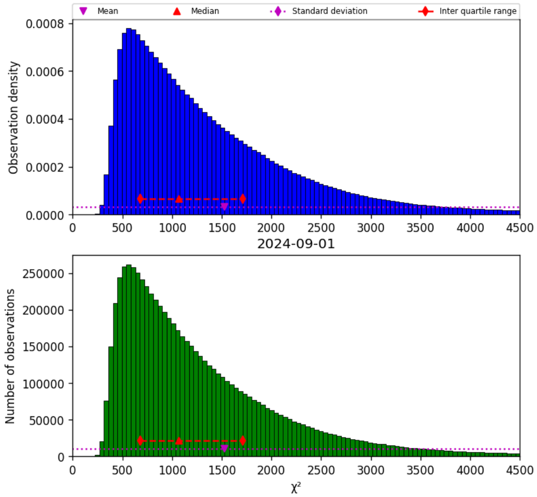
Figure 22: Histogram of “ \chi^2 ” for 2024-09-01 to 2024-09-02
