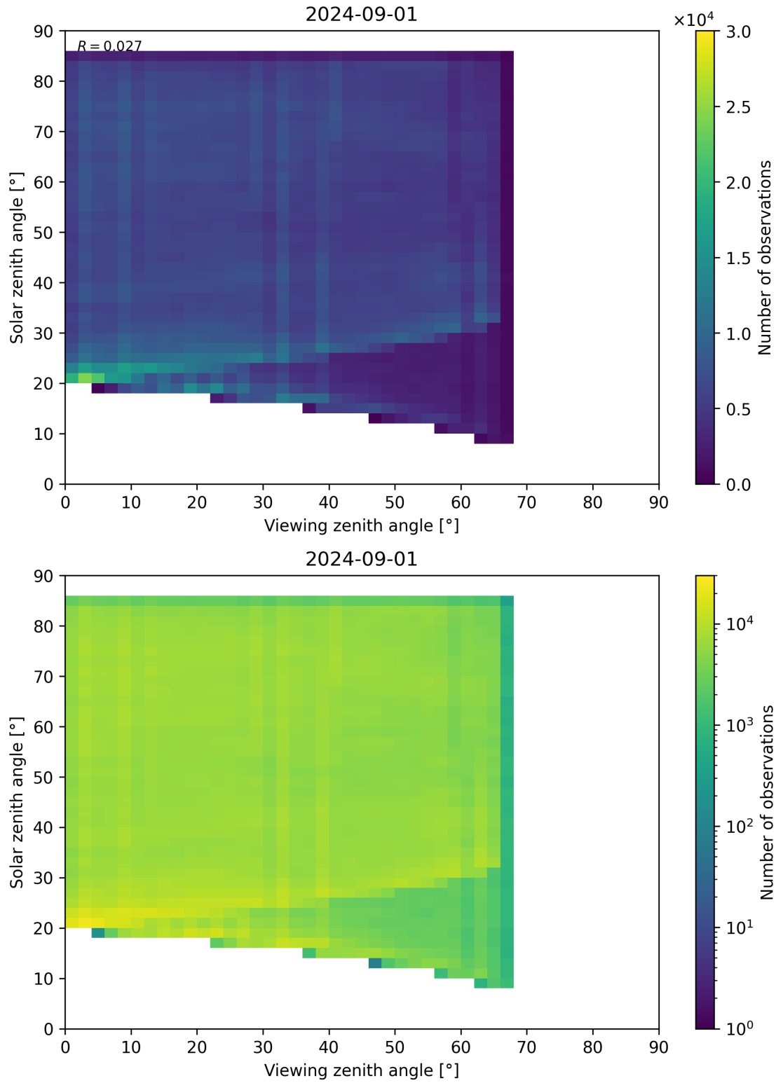
Figure 77: Scatter density plot of “Viewing zenith angle” against “Solar zenith angle” for 2024-09-01 to 2024-09-02.
