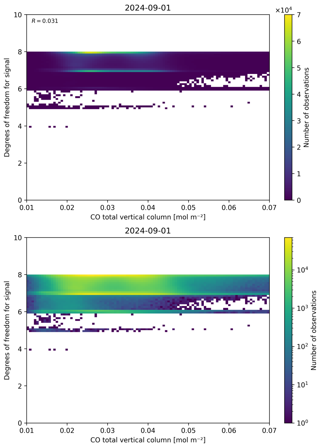
Figure 41: Scatter density plot of “CO total vertical column” against “Degrees of freedom for signal” for 2024-09-01 to 2024-09-02.
