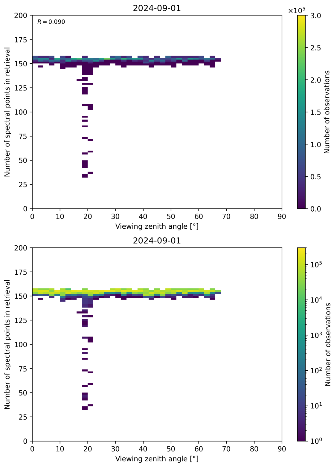
Figure 76: Scatter density plot of “Viewing zenith angle” against “Number of spectral points in retrieval” for 2024-09-01 to 2024-09-02.
