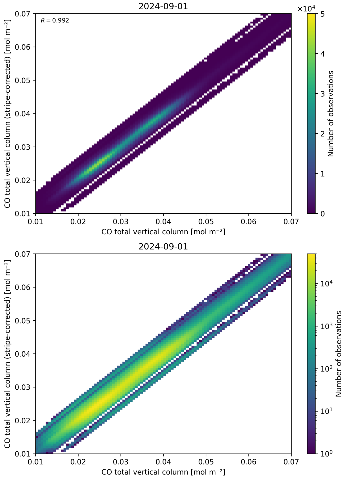
Figure 33: Scatter density plot of “CO total vertical column” against “CO total vertical column (stripe-corrected)” for 2024-09-01 to 2024-09-02.
