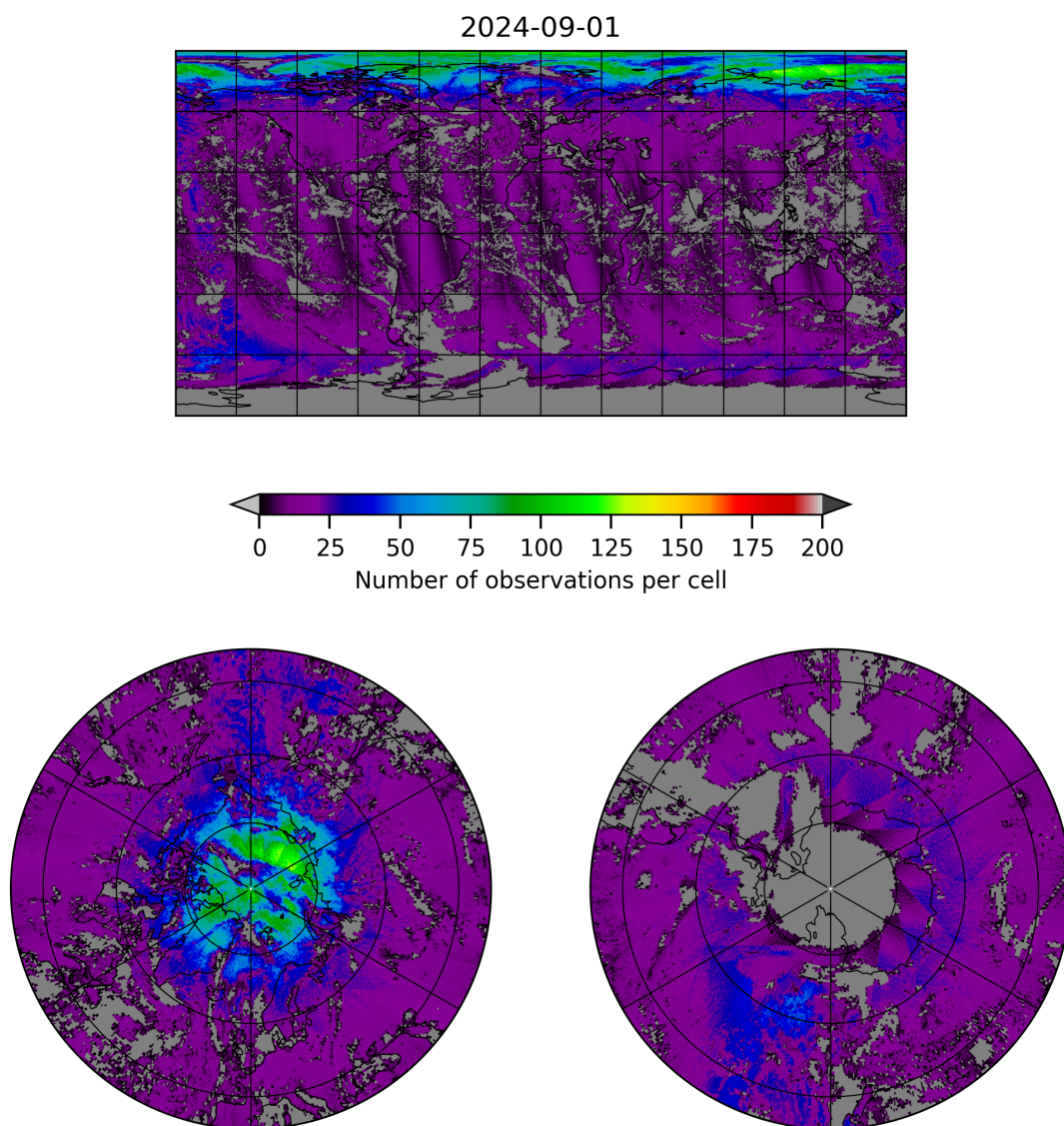
Figure 8: Map of the number of observations for 2024-09-01 to 2024-09-02
