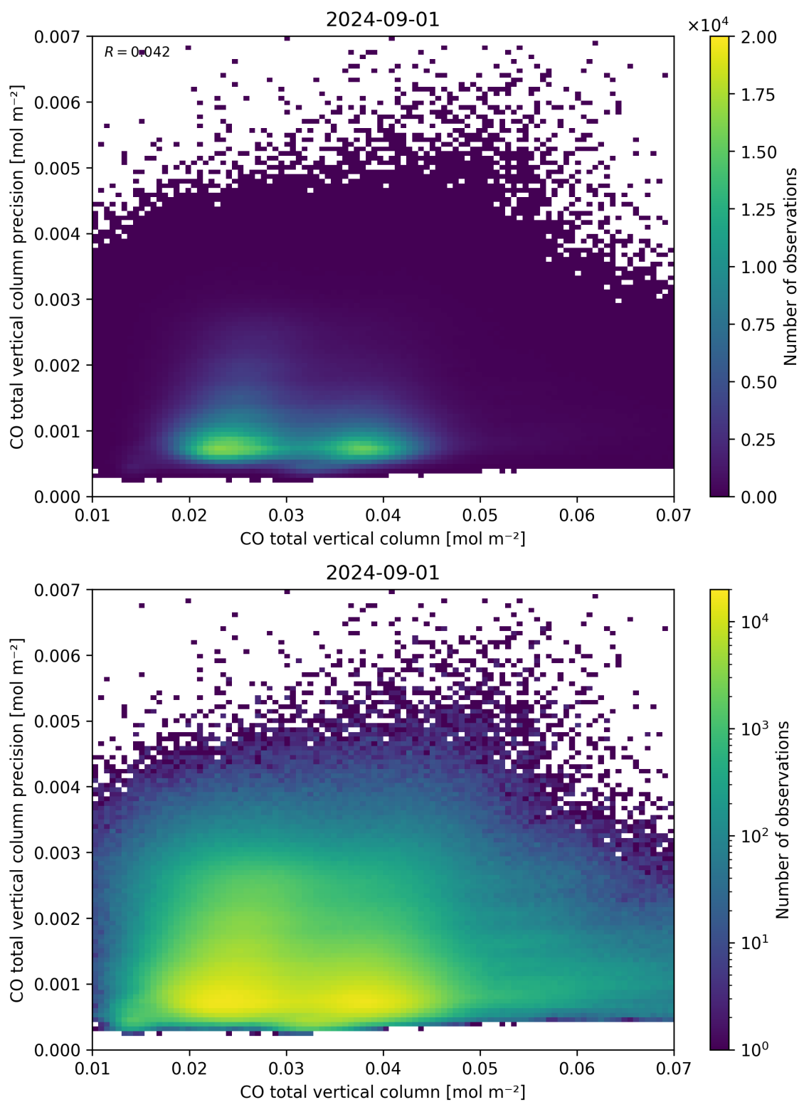
Figure 34: Scatter density plot of “CO total vertical column” against “CO total vertical column precision” for 2024-09-01 to 2024-09-02.
