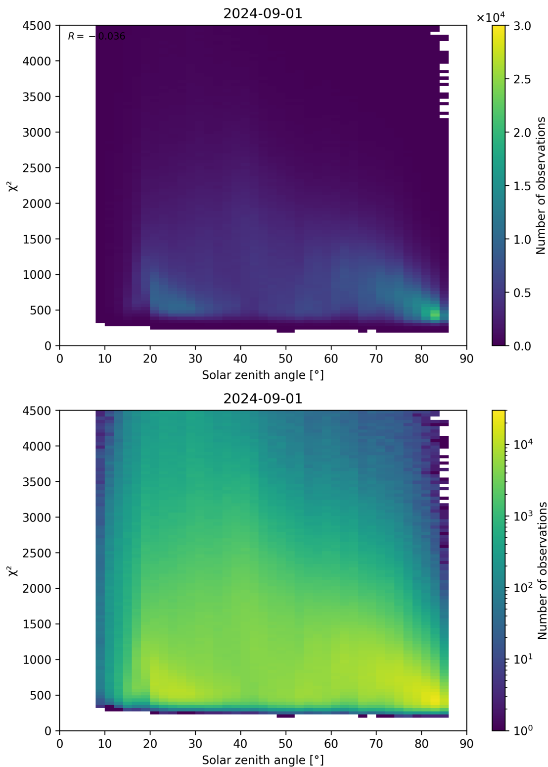
Figure 64: Scatter density plot of “Solar zenith angle” against “ \chi^2 ” for 2024-09-01 to 2024-09-02.
