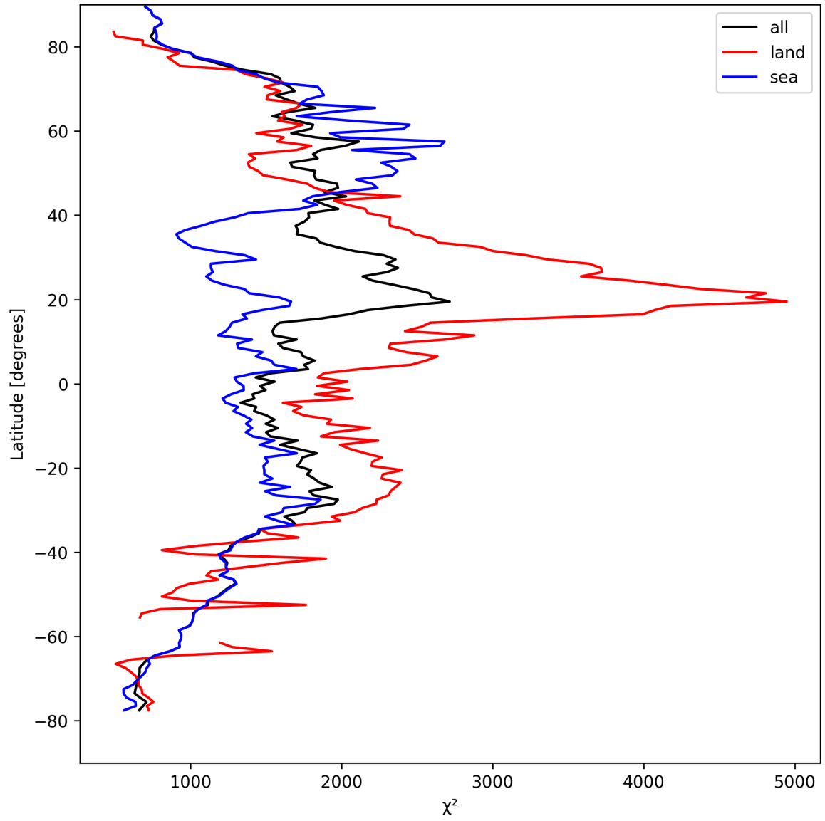
Figure 14: Zonal average of “ \chi^2 ” for 2024-09-01 to 2024-09-02.
