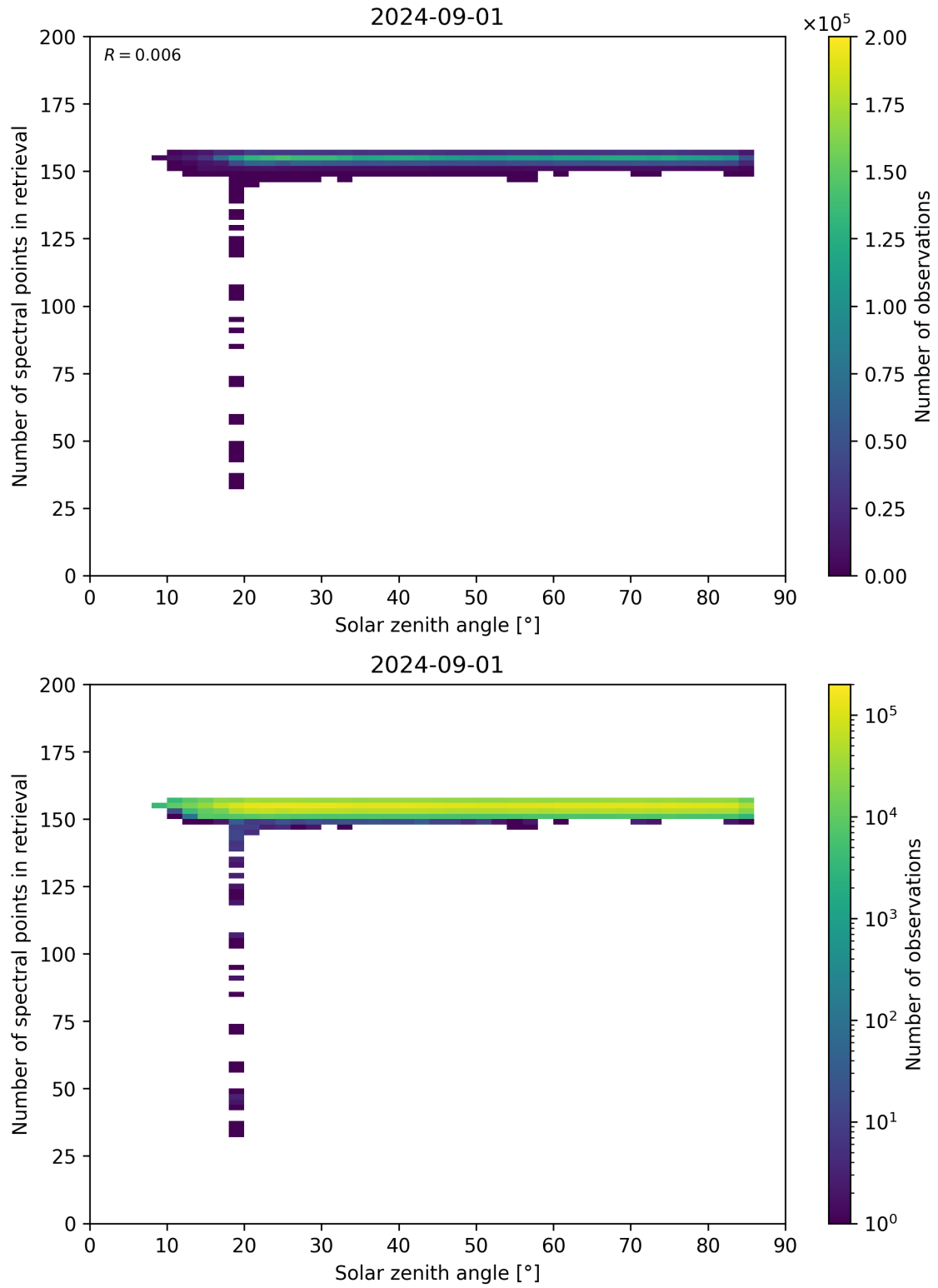
Figure 68: Scatter density plot of “Solar zenith angle” against “Number of spectral points in retrieval” for 2024-09-01 to 2024-09-02.
