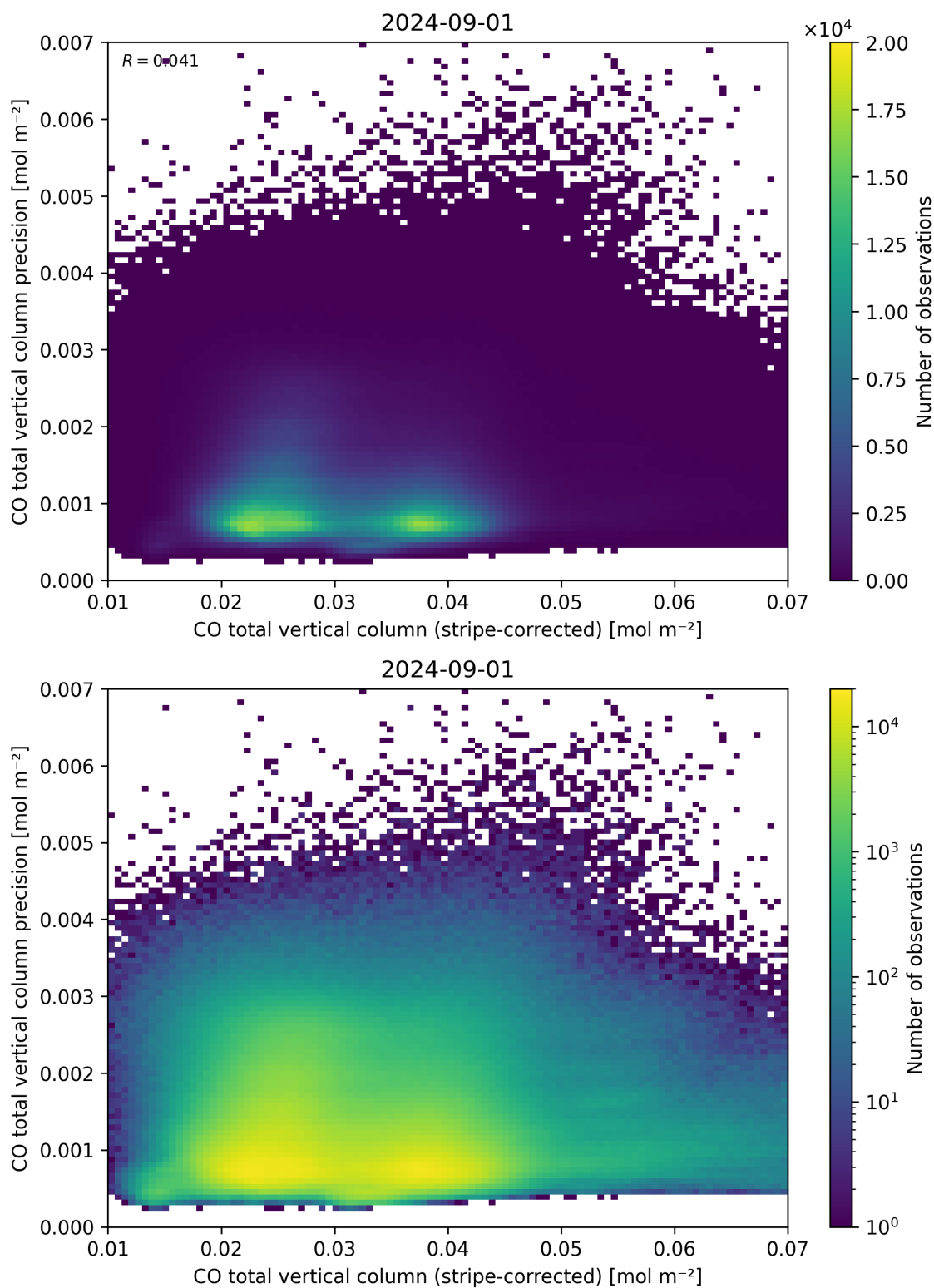
Figure 36: Scatter density plot of “CO total vertical column (stripe-corrected)” against “CO total vertical column precision” for 2024-09-01 to 2024-09-02.
