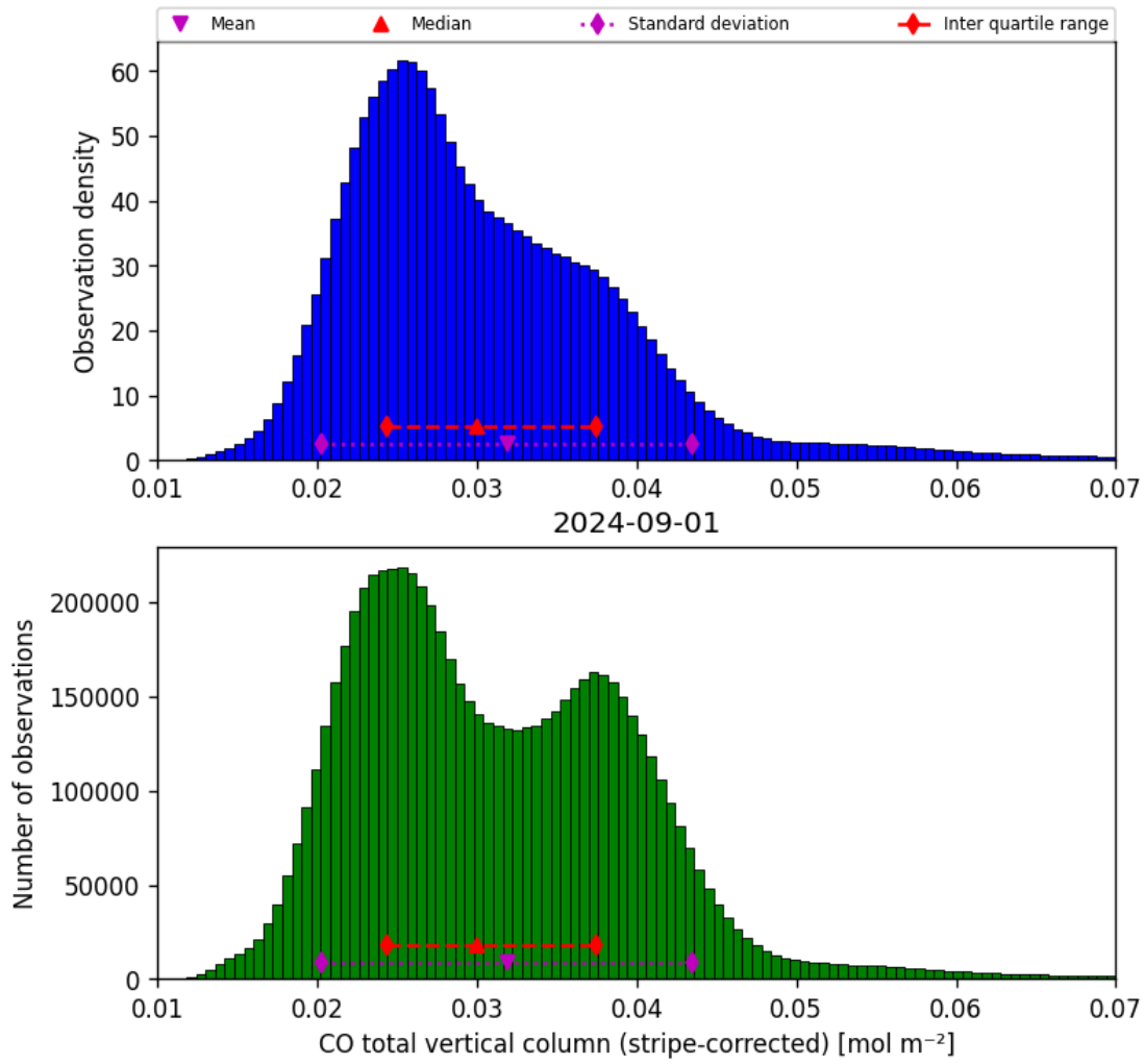
Figure 19: Histogram of “CO total vertical column (stripe-corrected)” for 2024-09-01 to 2024-09-02
