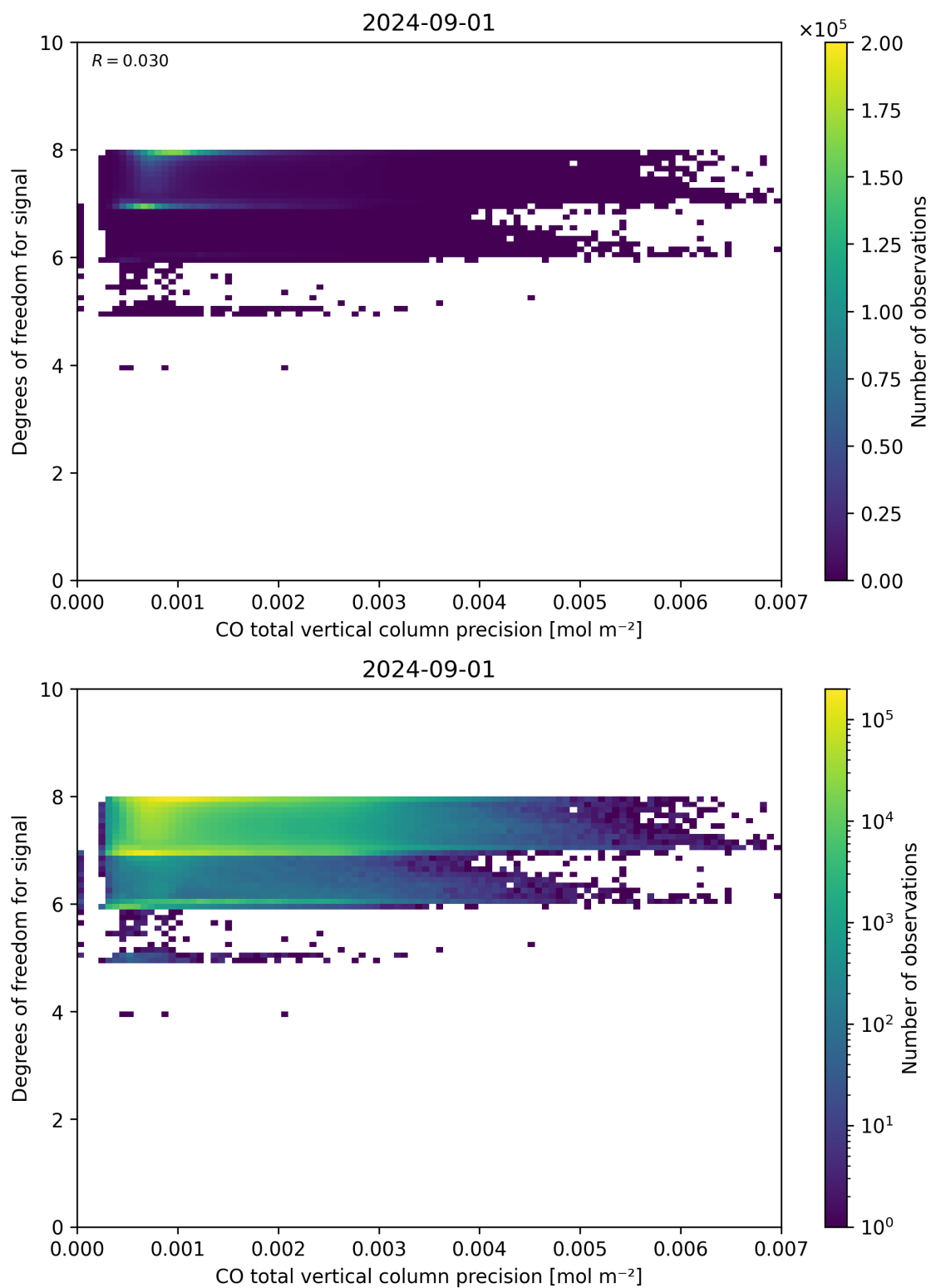
Figure 45: Scatter density plot of “CO total vertical column precision” against “Degrees of freedom for signal” for 2024-09-01 to 2024-09-02.
