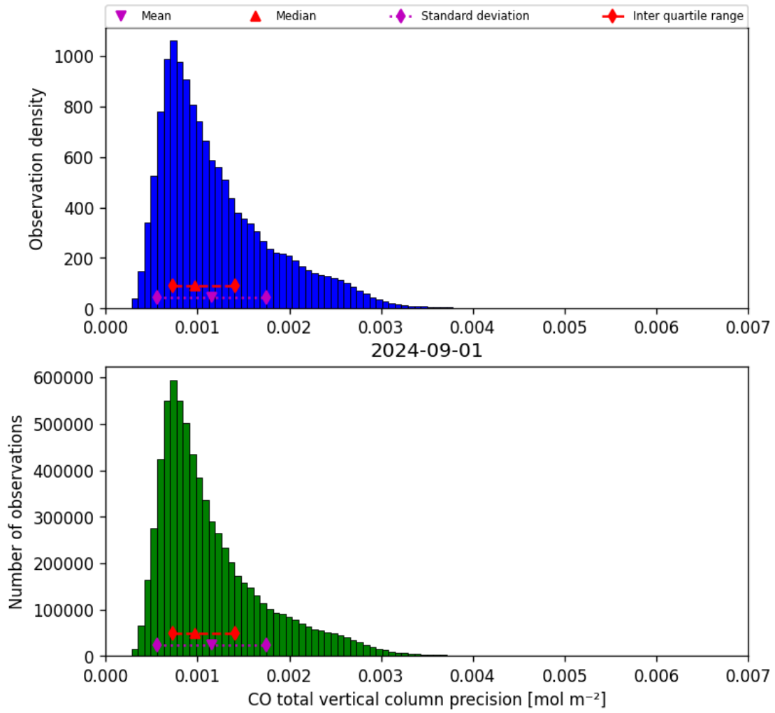
Figure 20: Histogram of “CO total vertical column precision” for 2024-09-01 to 2024-09-02
