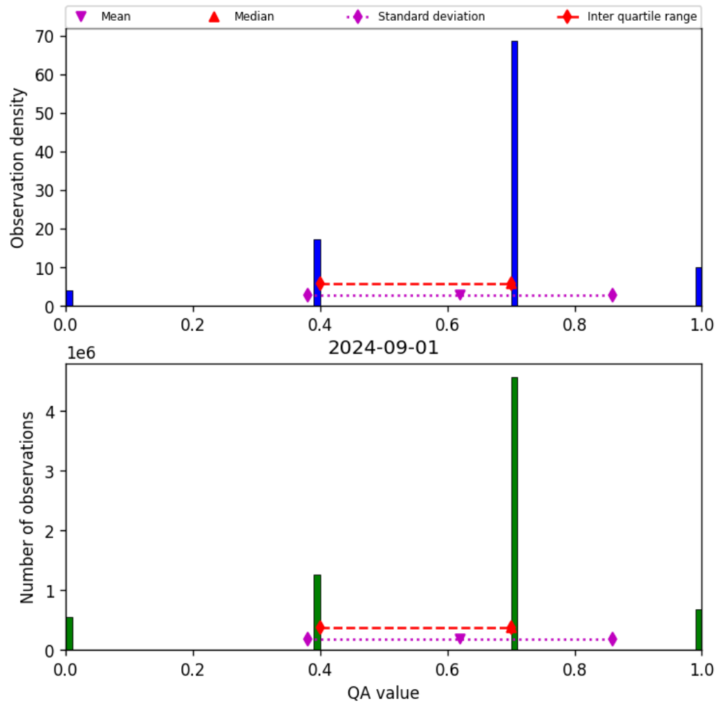
Figure 17: Histogram of “QA value” for 2024-09-01 to 2024-09-02
