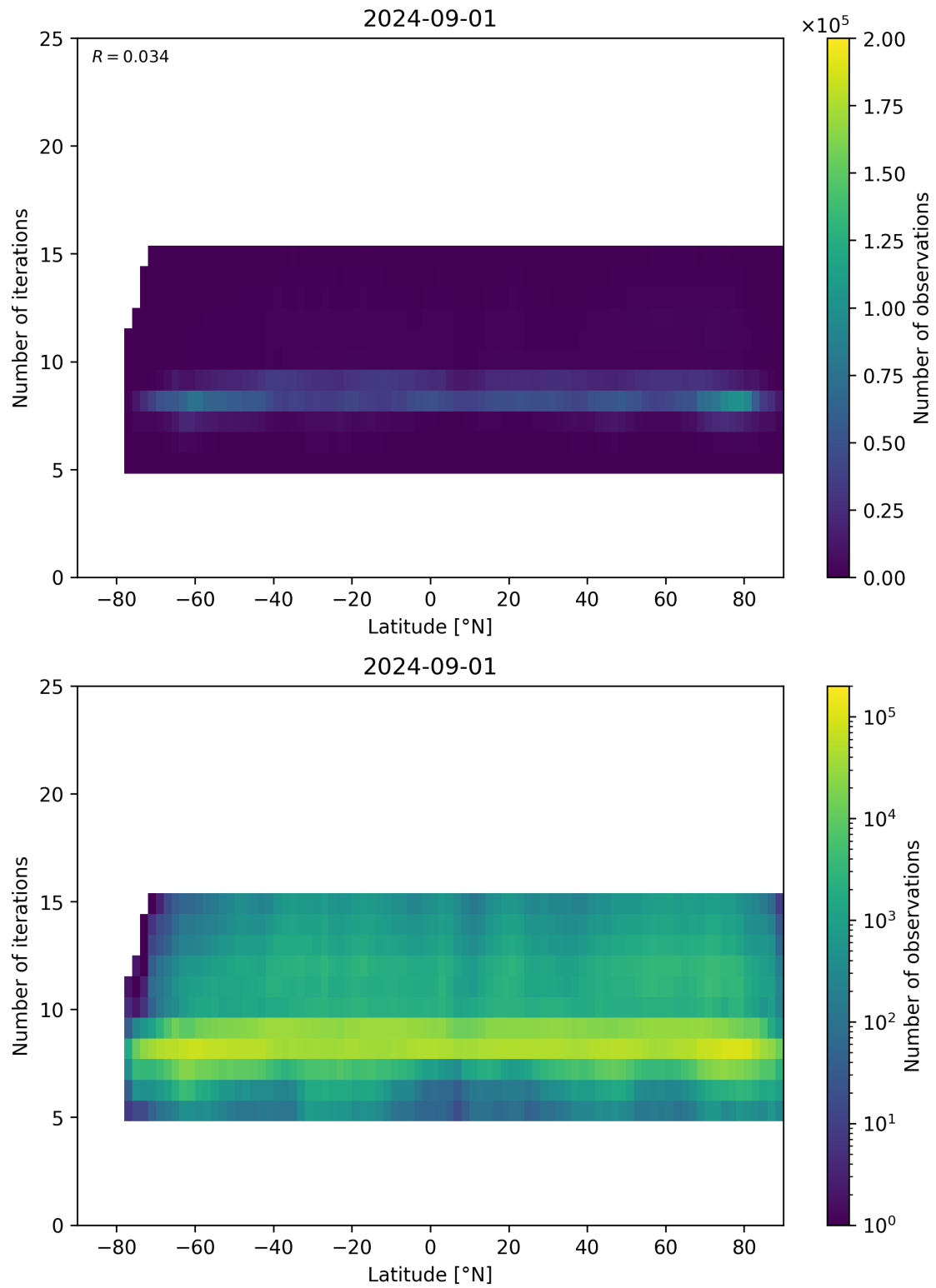
Figure 56: Scatter density plot of “Latitude” against “Number of iterations” for 2024-09-01 to 2024-09-02.
