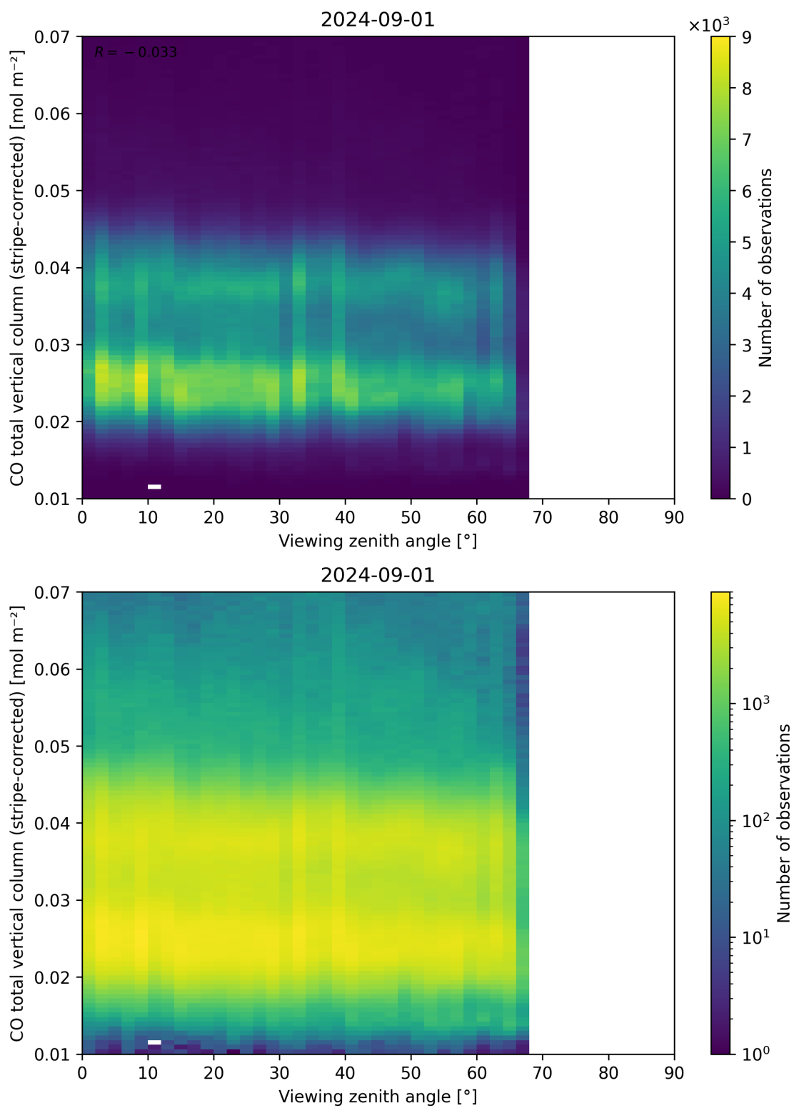
Figure 70: Scatter density plot of “Viewing zenith angle” against “CO total vertical column (stripe-corrected)” for 2024-09-01 to 2024-09-02.
