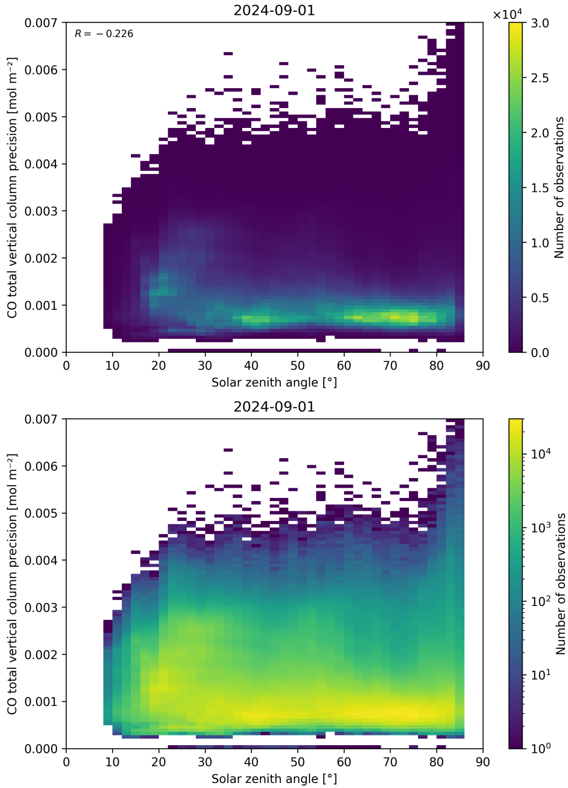
Figure 63: Scatter density plot of “Solar zenith angle” against “CO total vertical column precision” for 2024-09-01 to 2024-09-02.
