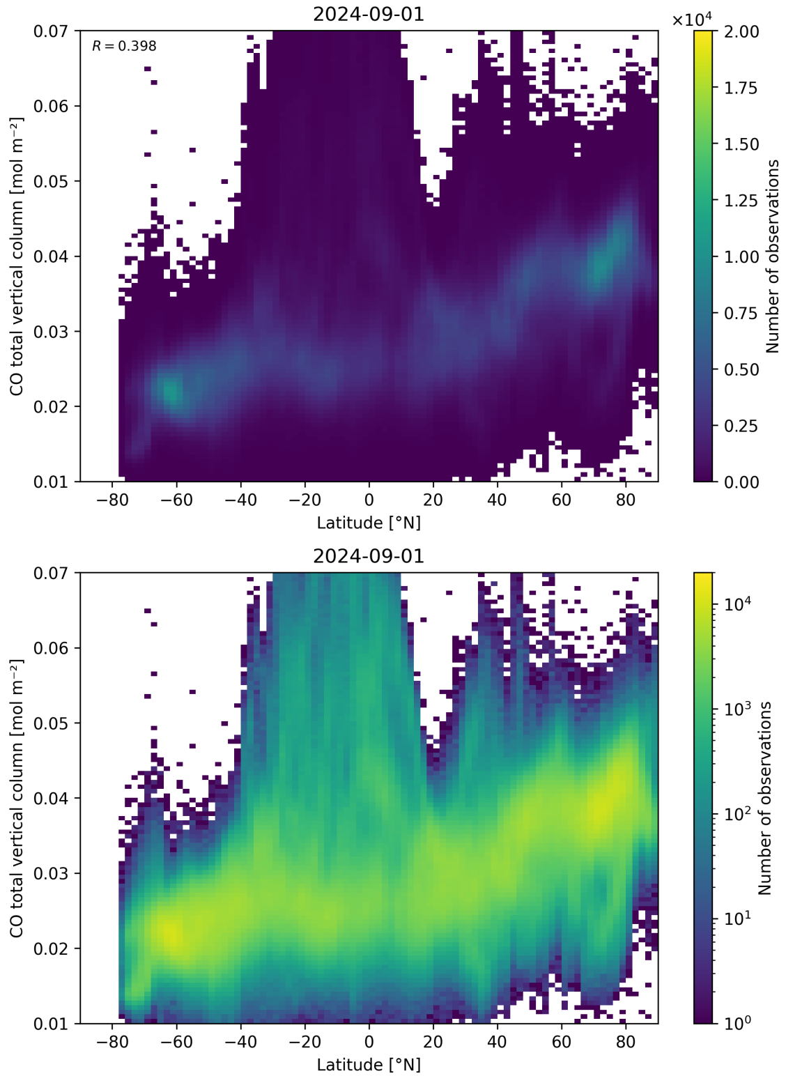
Figure 51: Scatter density plot of “Latitude” against “CO total vertical column” for 2024-09-01 to 2024-09-02.
