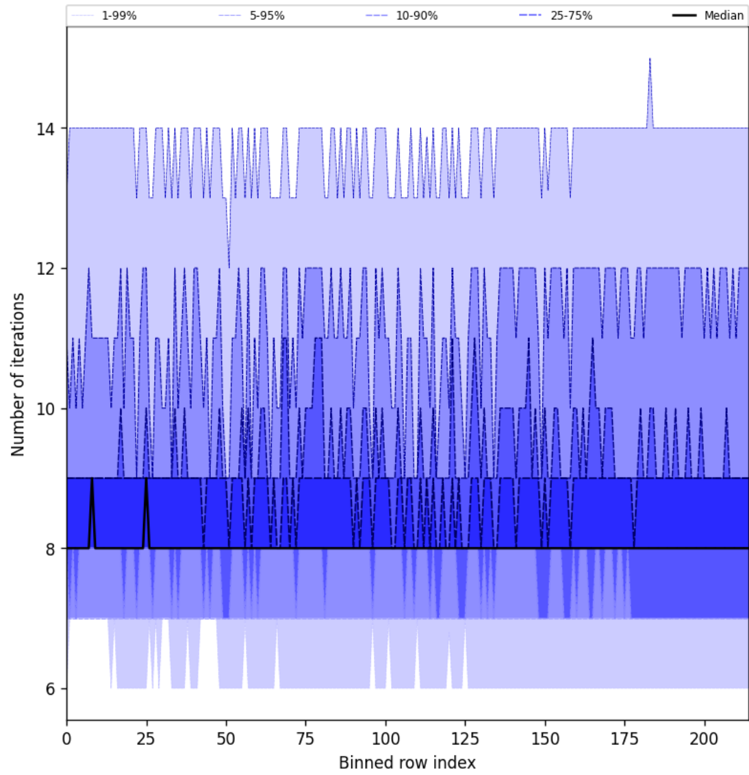
Figure 32: Along track statistics of “Number of iterations” for 2024-09-01 to 2024-09-02
