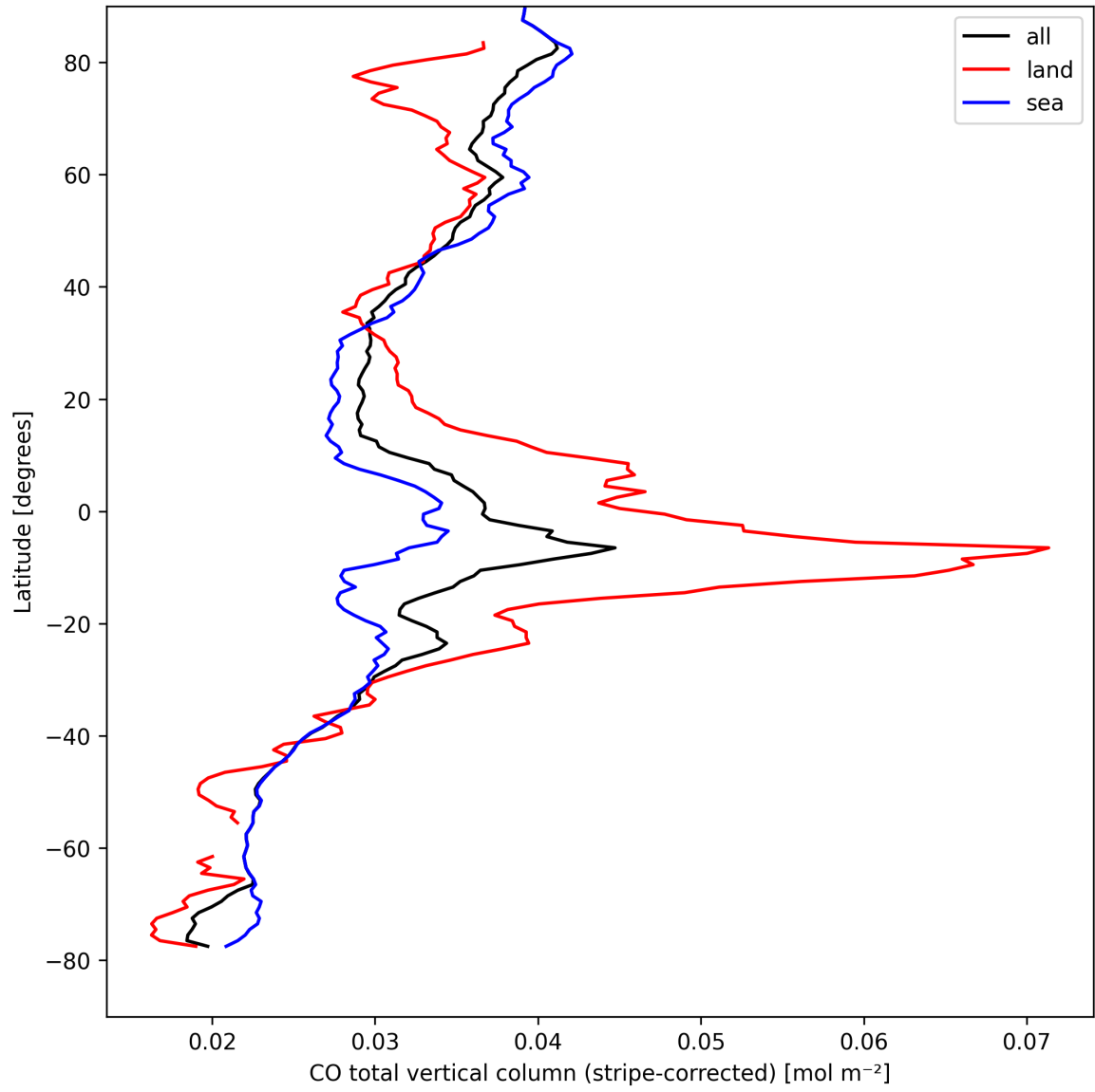
Figure 11: Zonal average of “CO total vertical column (stripe-corrected)” for 2024-09-01 to 2024-09-02.
