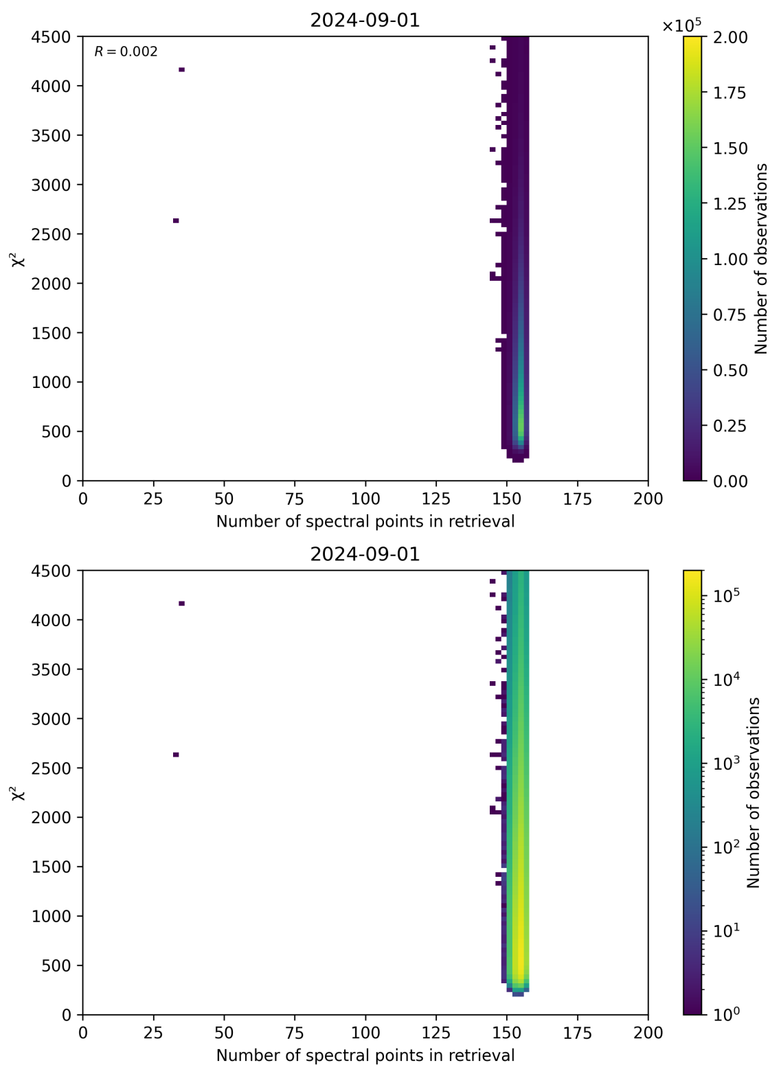
Figure 58: Scatter density plot of “Number of spectral points in retrieval” against “ \chi^2 ” for 2024-09-01 to 2024-09-02.
