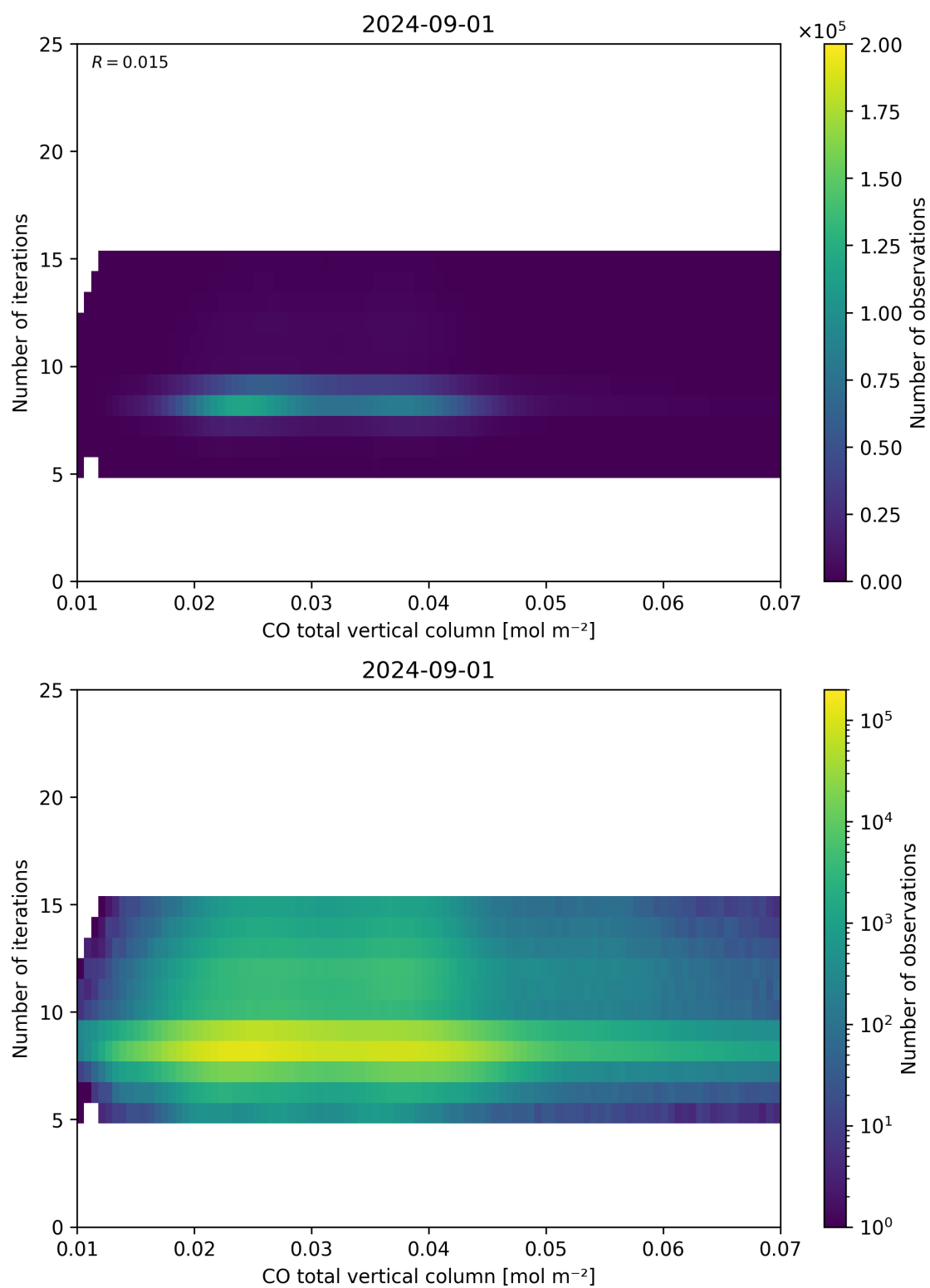
Figure 42: Scatter density plot of “CO total vertical column” against “Number of iterations” for 2024-09-01 to 2024-09-02.
