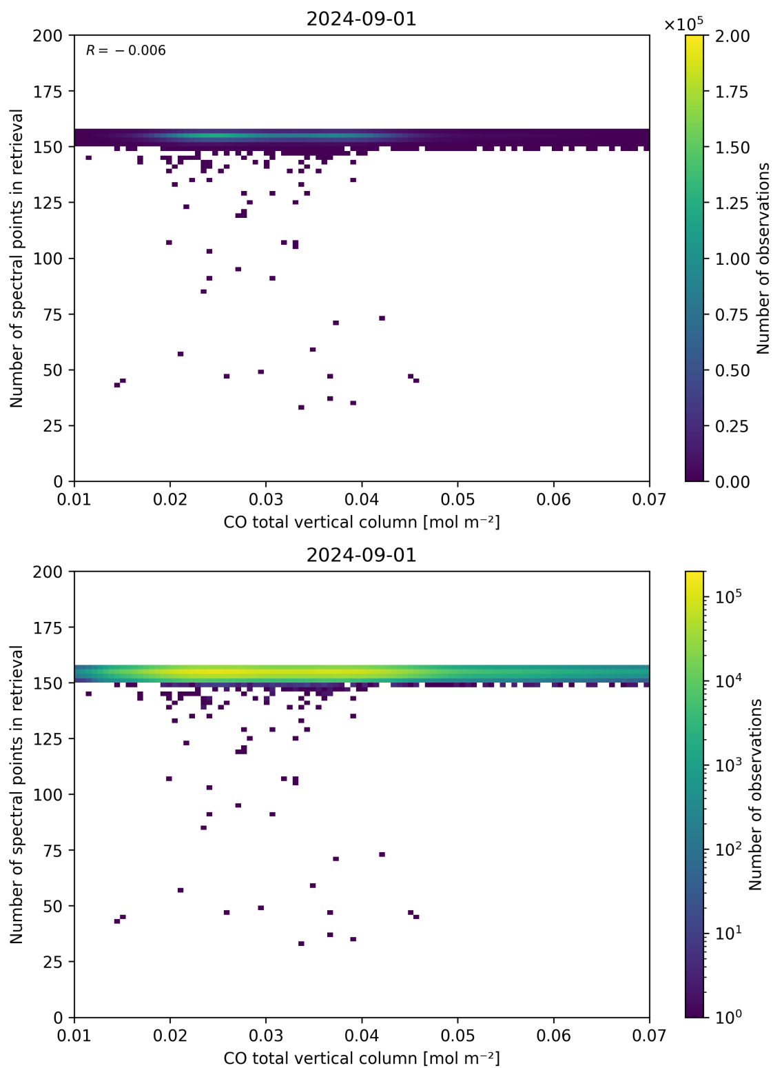
Figure 43: Scatter density plot of “CO total vertical column” against “Number of spectral points in retrieval” for 2024-09-01 to 2024-09-02.
