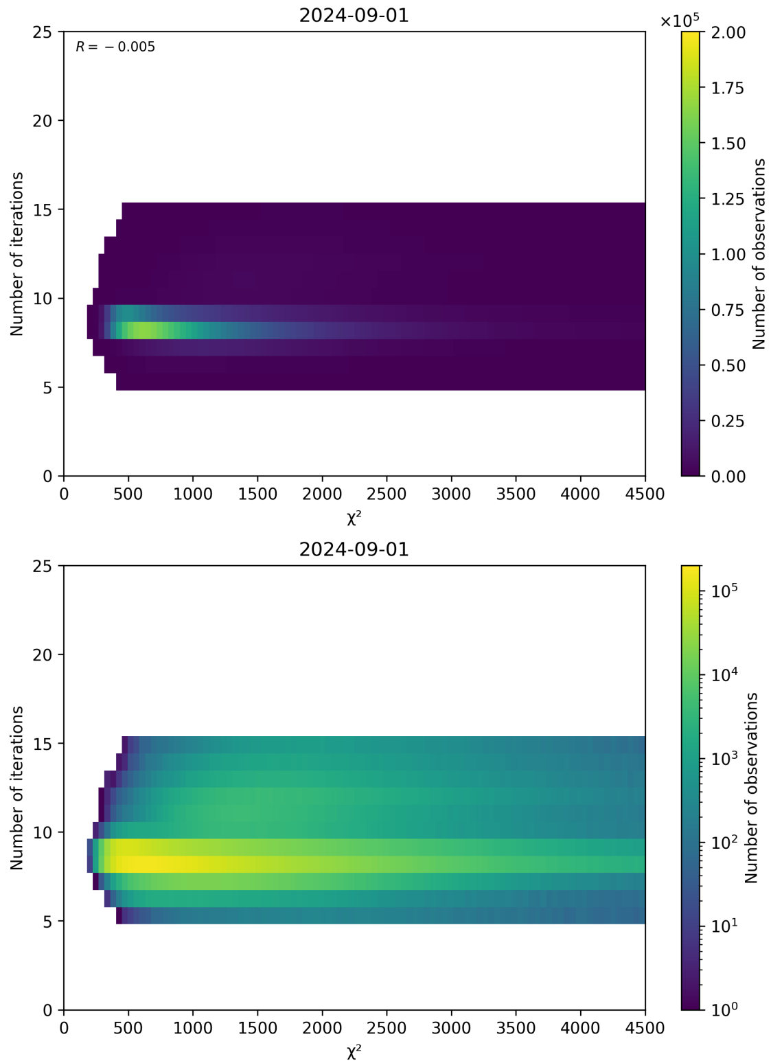
Figure 49: Scatter density plot of “ \chi^2 ” against “Number of iterations” for 2024-09-01 to 2024-09-02.
