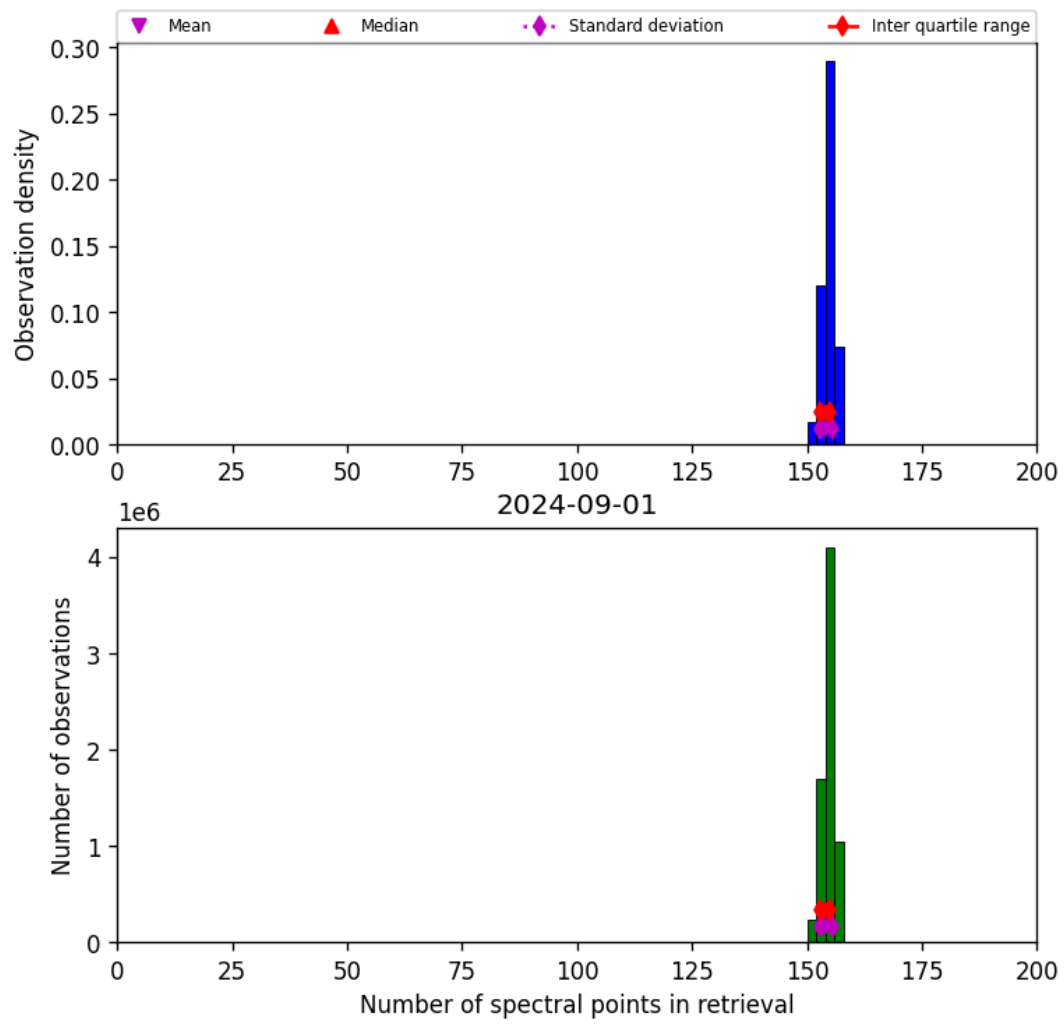
Figure 21: Histogram of “Number of spectral points in retrieval” for 2024-09-01 to 2024-09-02
