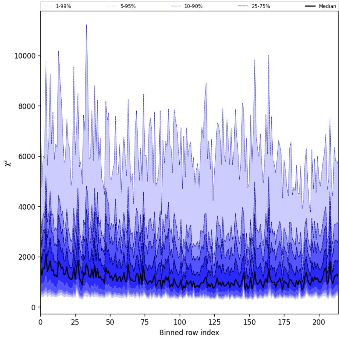
Figure 30: Along track statistics of “ \chi^2 ” for 2024-09-01 to 2024-09-02
