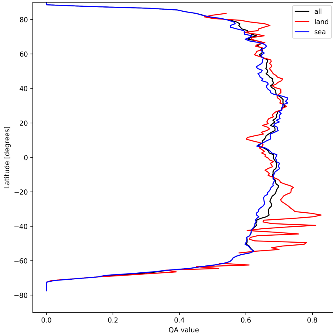
Figure 9: Zonal average of “QA value” for 2024-09-01 to 2024-09-02.
