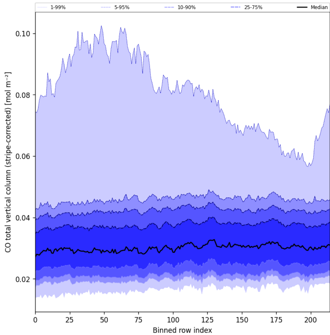
Figure 27: Along track statistics of “CO total vertical column (stripe-corrected)” for 2024-09-01 to 2024-09-02
