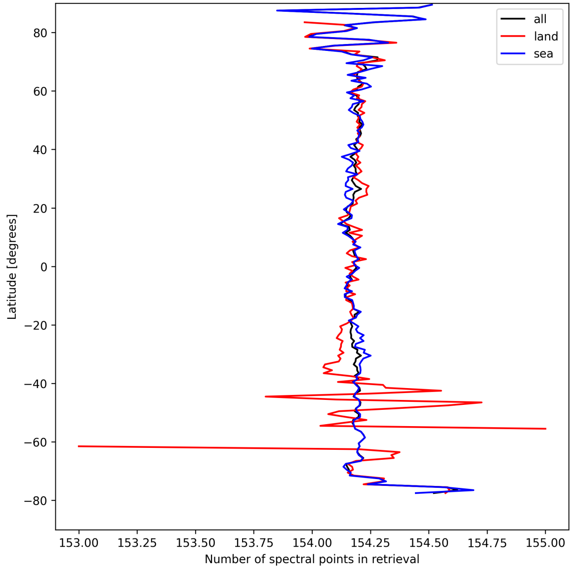
Figure 13: Zonal average of “Number of spectral points in retrieval” for 2024-09-01 to 2024-09-02.
