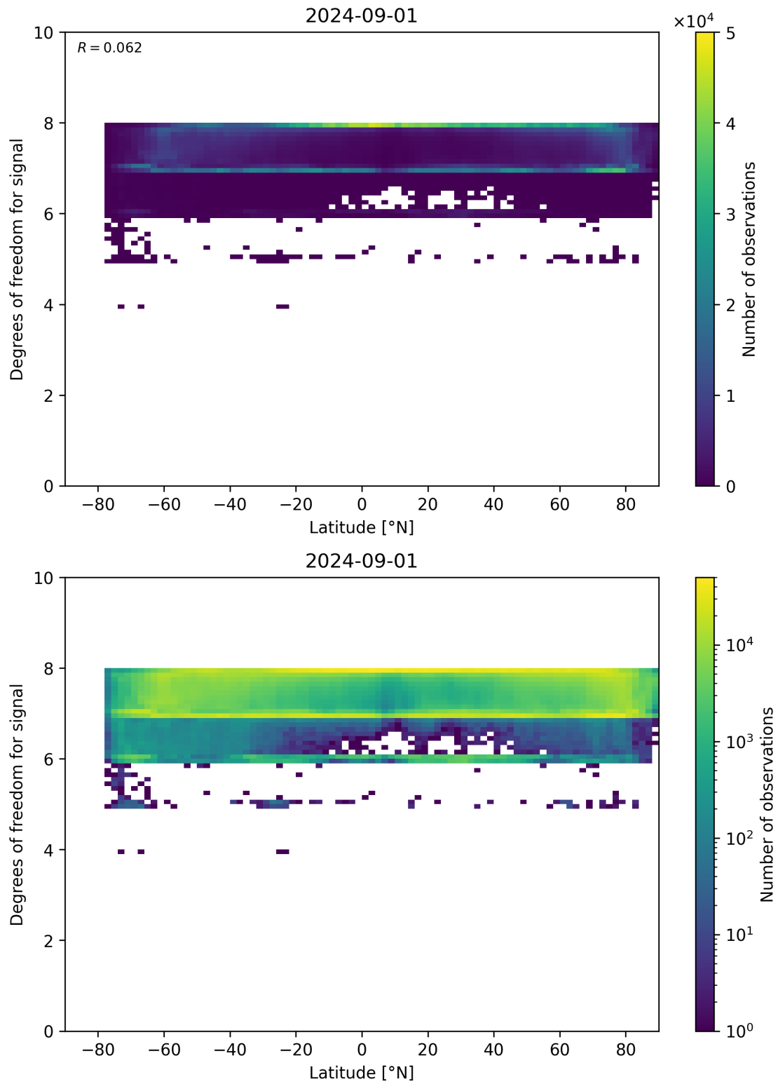
Figure 55: Scatter density plot of “Latitude” against “Degrees of freedom for signal” for 2024-09-01 to 2024-09-02.
