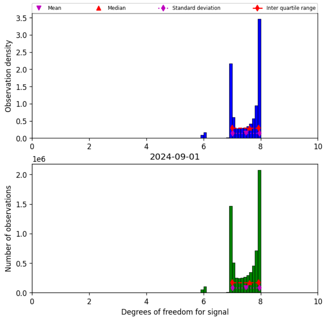
Figure 23: Histogram of “Degrees of freedom for signal” for 2024-09-01 to 2024-09-02
