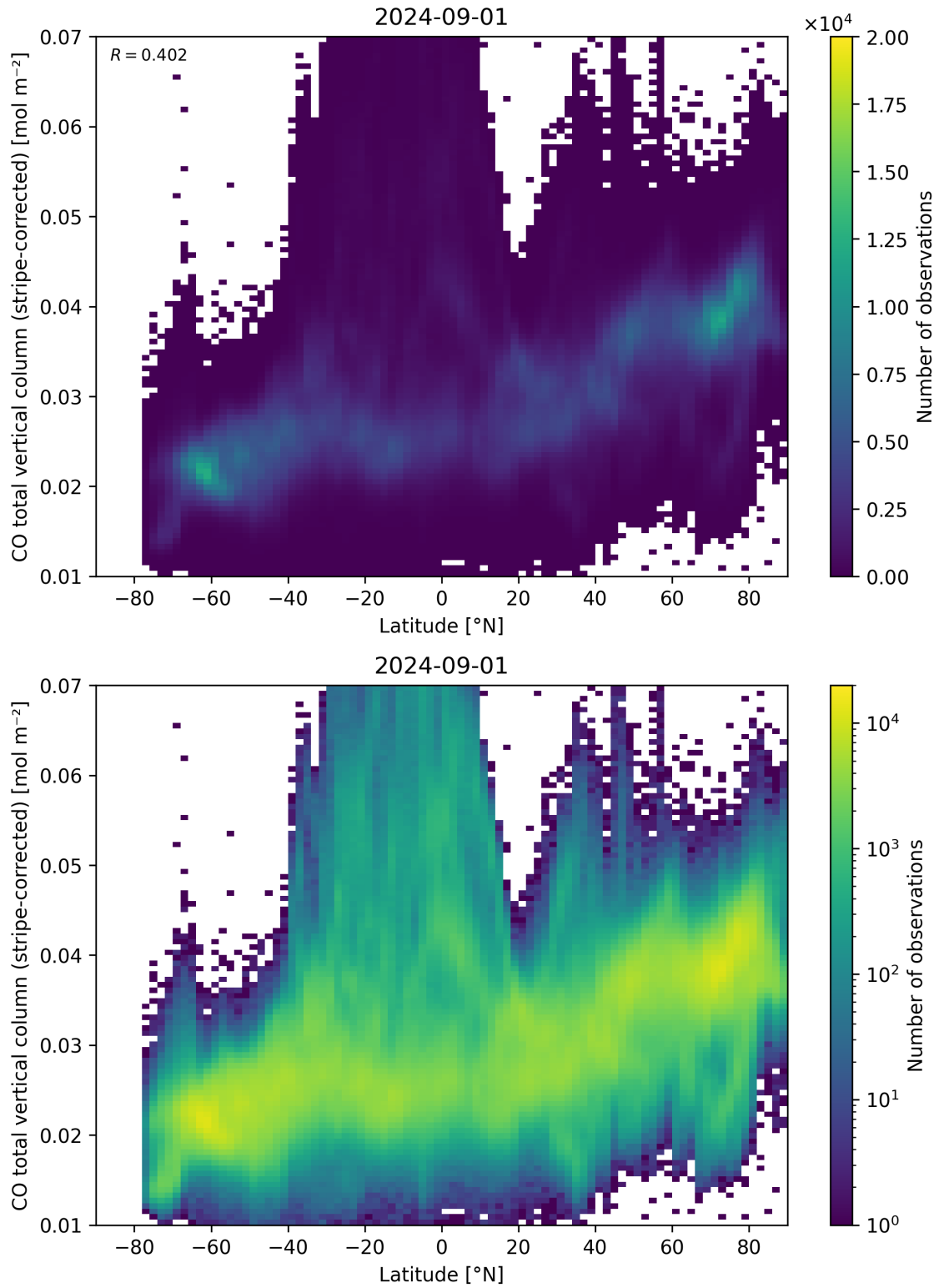
Figure 52: Scatter density plot of “Latitude” against “CO total vertical column (stripe-corrected)” for 2024-09-01 to 2024-09-02.
