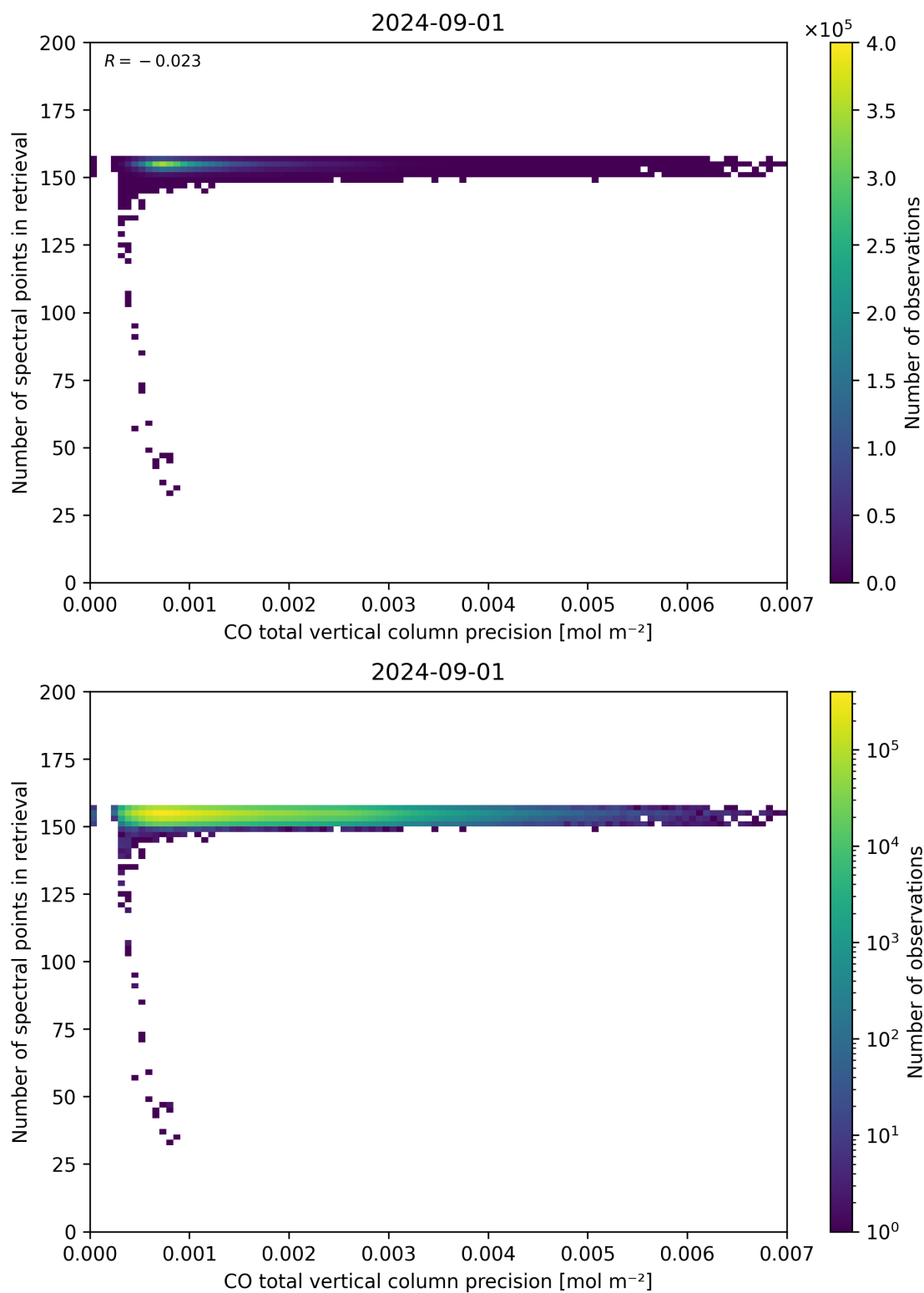
Figure 47: Scatter density plot of “CO total vertical column precision” against “Number of spectral points in retrieval” for 2024-09-01 to 2024-09-02.
