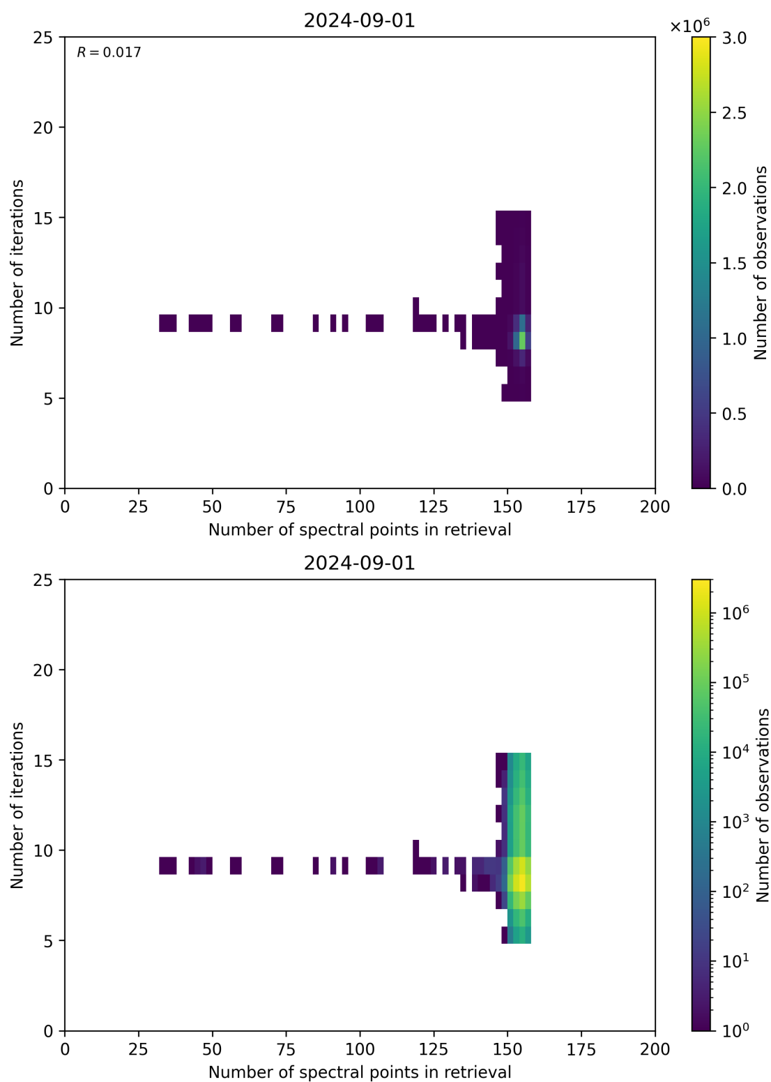
Figure 60: Scatter density plot of “Number of spectral points in retrieval” against “Number of iterations” for 2024-09-01 to 2024-09-02.
