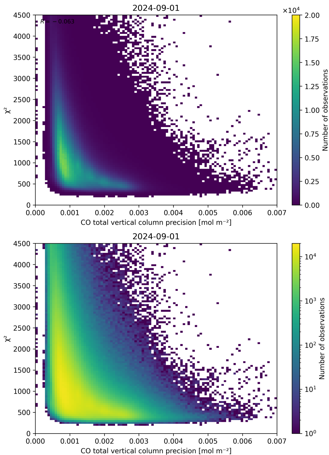
Figure 44: Scatter density plot of “CO total vertical column precision” against “ \chi^2 ” for 2024-09-01 to 2024-09-02.
