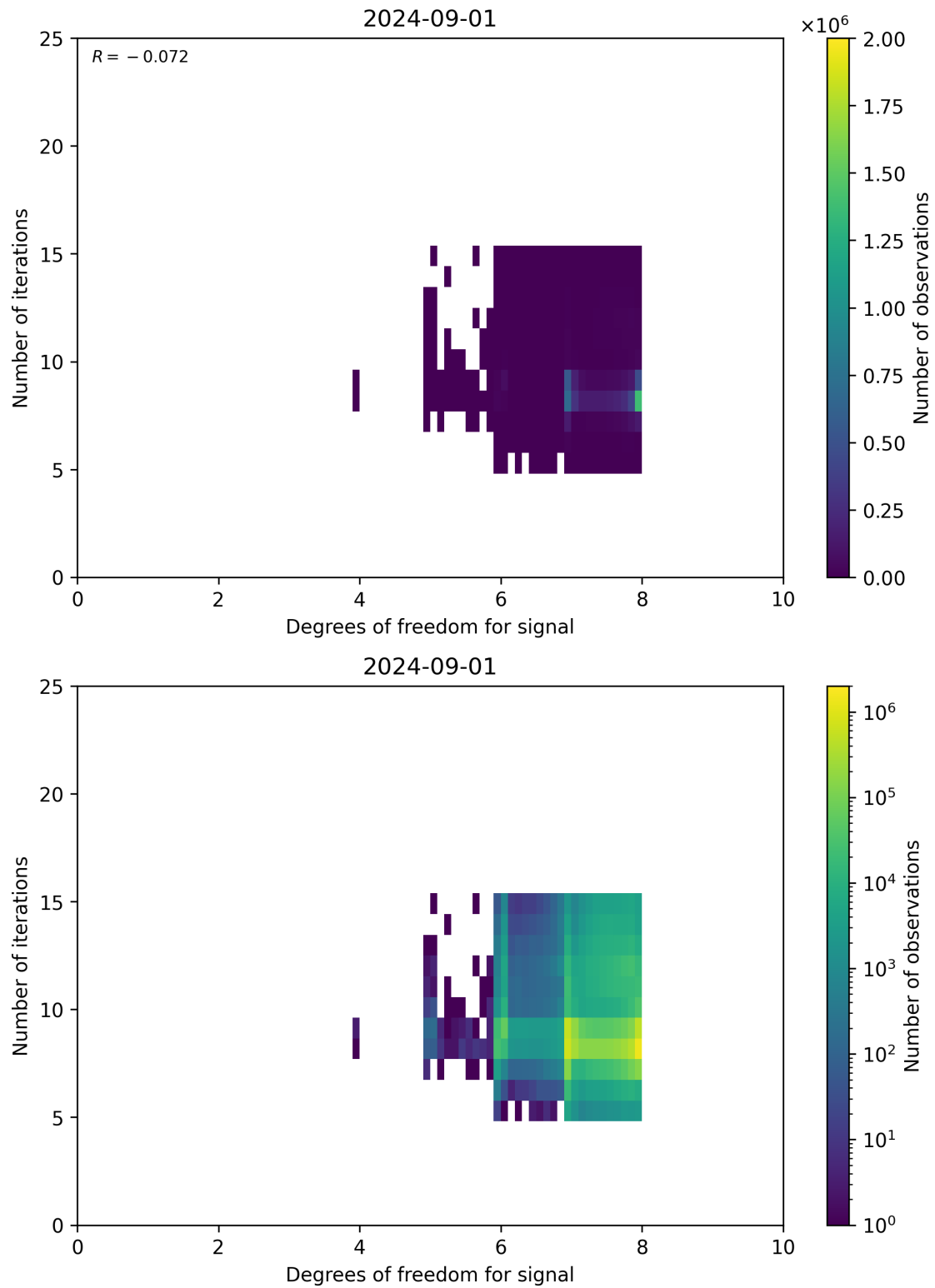
Figure 50: Scatter density plot of “Degrees of freedom for signal” against “Number of iterations” for 2024-09-01 to 2024-09-02.
