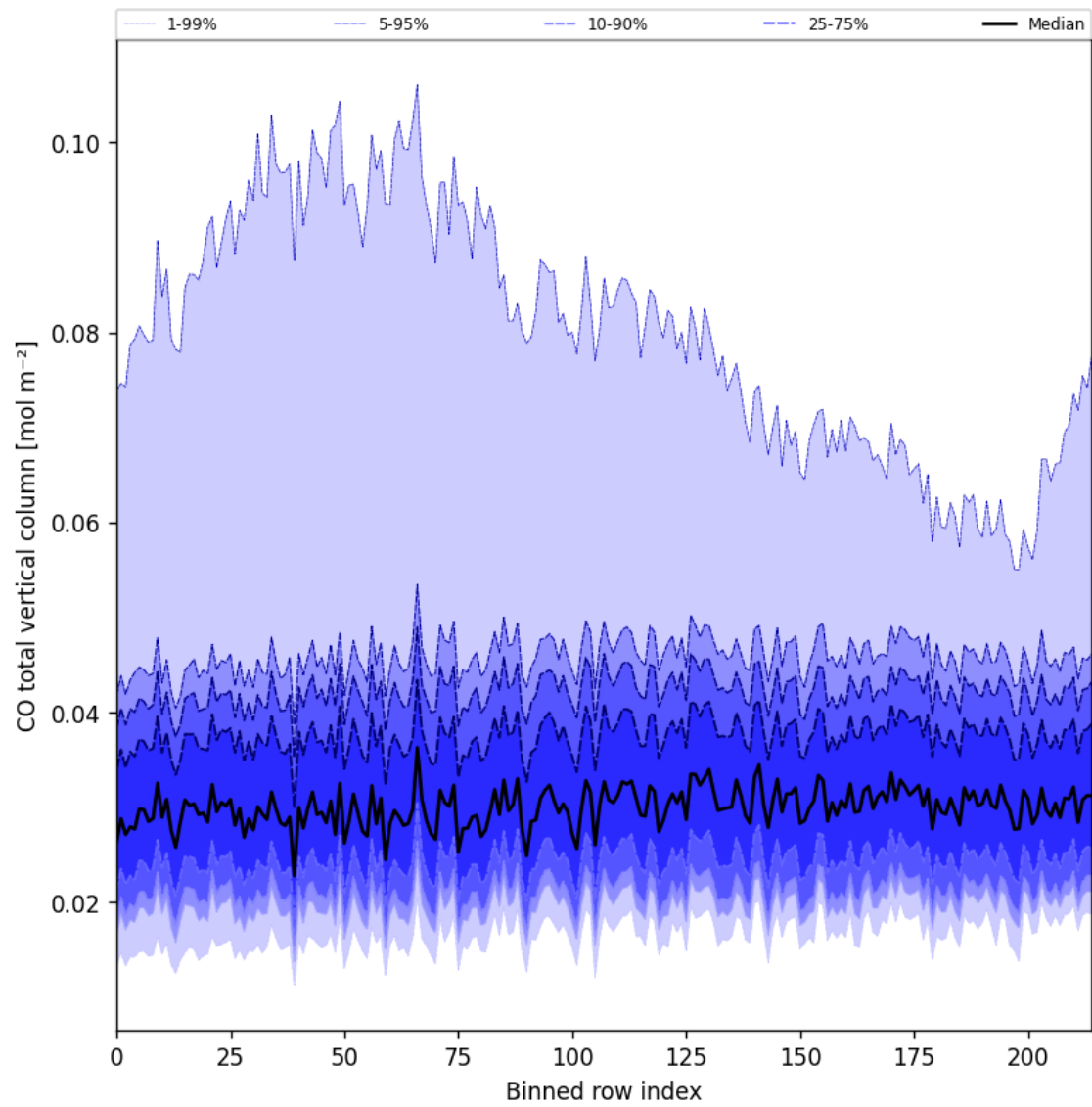
Figure 26: Along track statistics of “CO total vertical column” for 2024-09-01 to 2024-09-02
