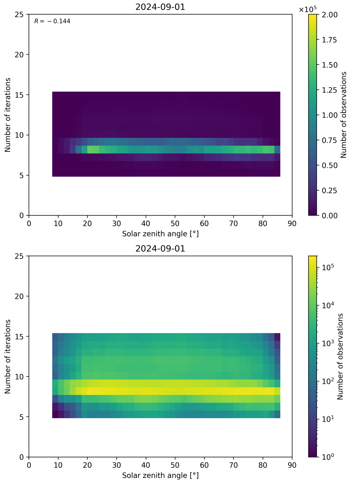
Figure 67: Scatter density plot of “Solar zenith angle” against “Number of iterations” for 2024-09-01 to 2024-09-02.
