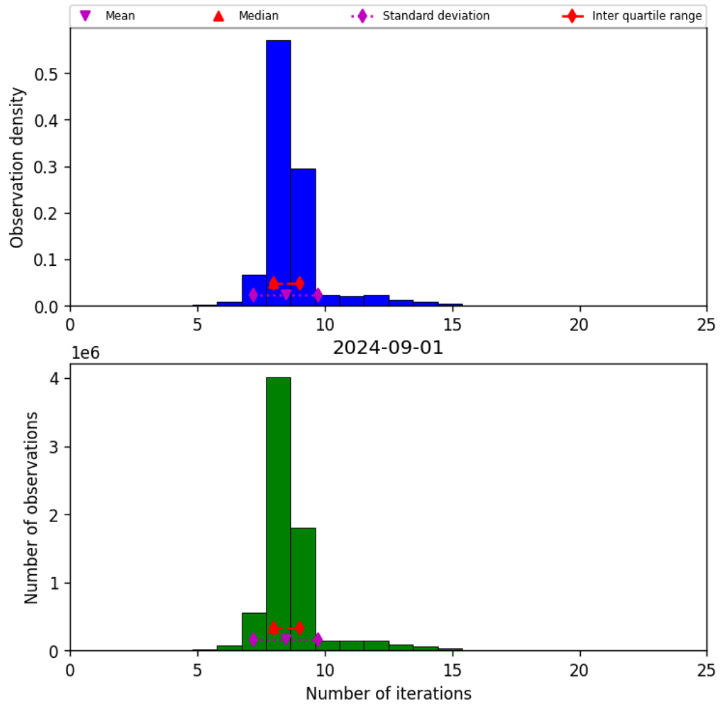
Figure 24: Histogram of “Number of iterations” for 2024-09-01 to 2024-09-02
