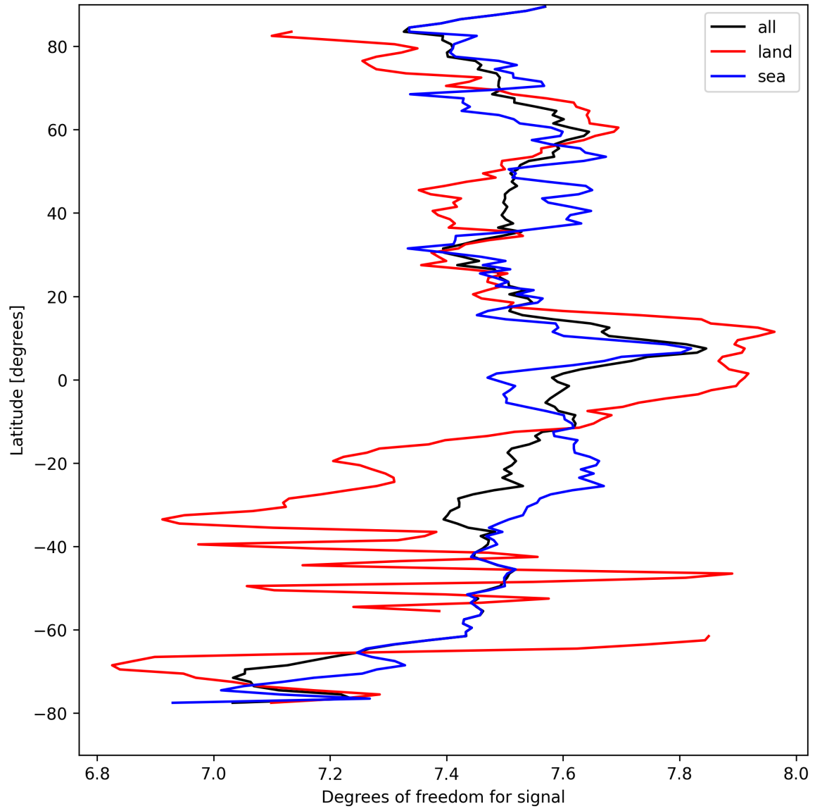
Figure 15: Zonal average of “Degrees of freedom for signal” for 2024-09-01 to 2024-09-02.
