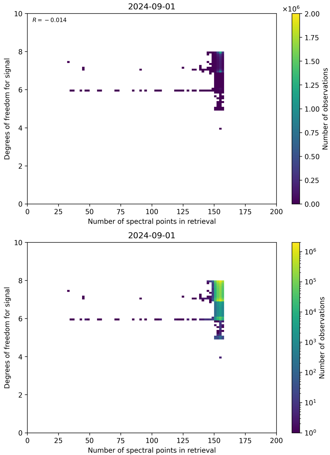
Figure 59: Scatter density plot of “Number of spectral points in retrieval” against “Degrees of freedom for signal” for 2024-09-01 to 2024-09-02.
