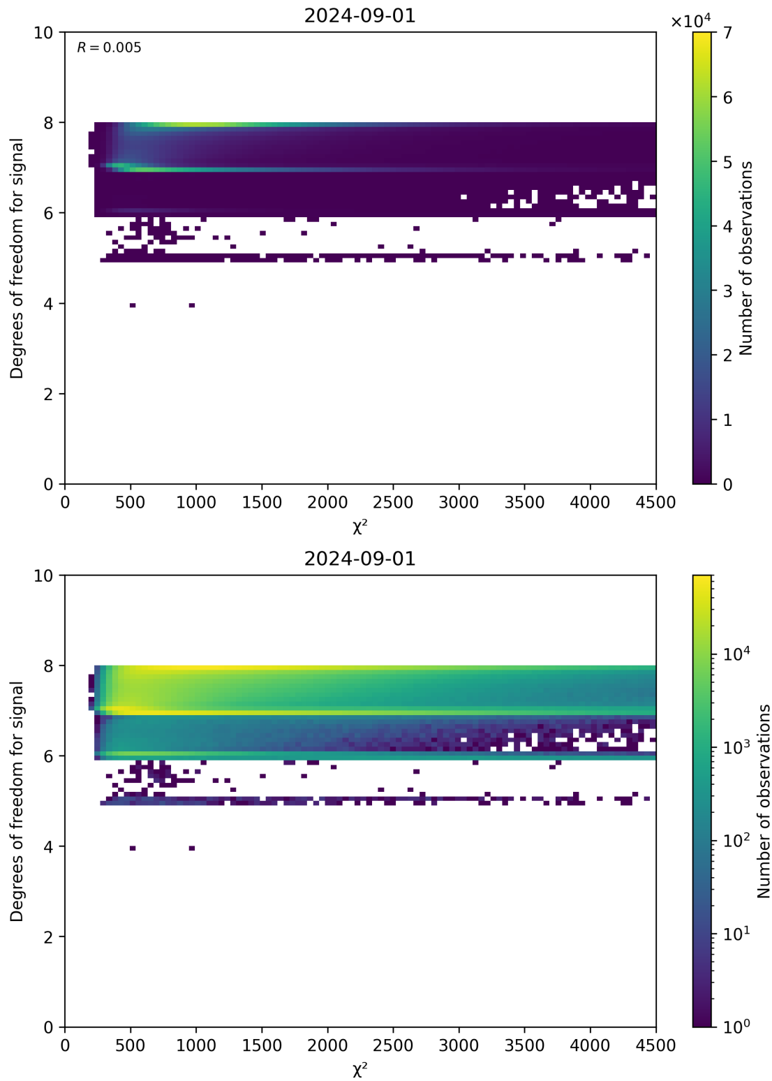
Figure 48: Scatter density plot of " \chi^2 " against "Degrees of freedom for signal" for 2024-09-01 to 2024-09-02.
