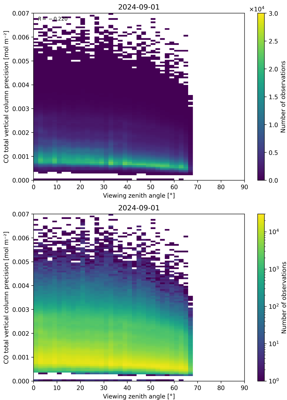
Figure 71: Scatter density plot of “Viewing zenith angle” against “CO total vertical column precision” for 2024-09-01 to 2024-09-02.
