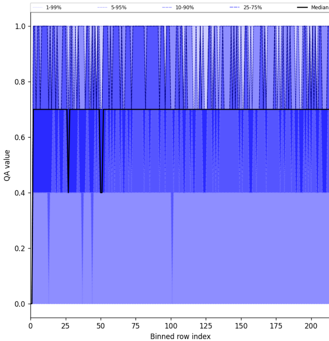
Figure 25: Along track statistics of “QA value” for 2024-09-01 to 2024-09-02
