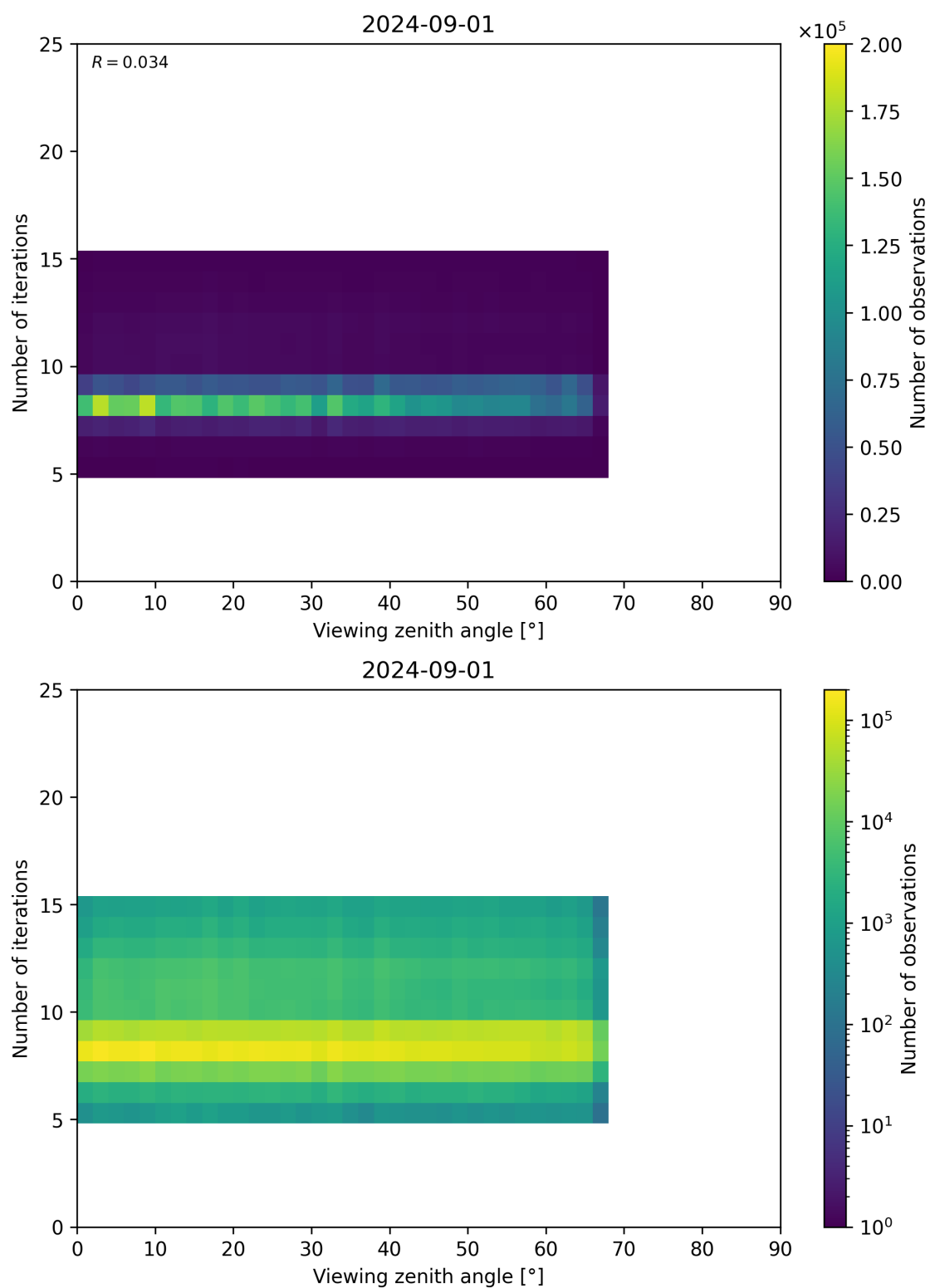
Figure 75: Scatter density plot of “Viewing zenith angle” against “Number of iterations” for 2024-09-01 to 2024-09-02.
