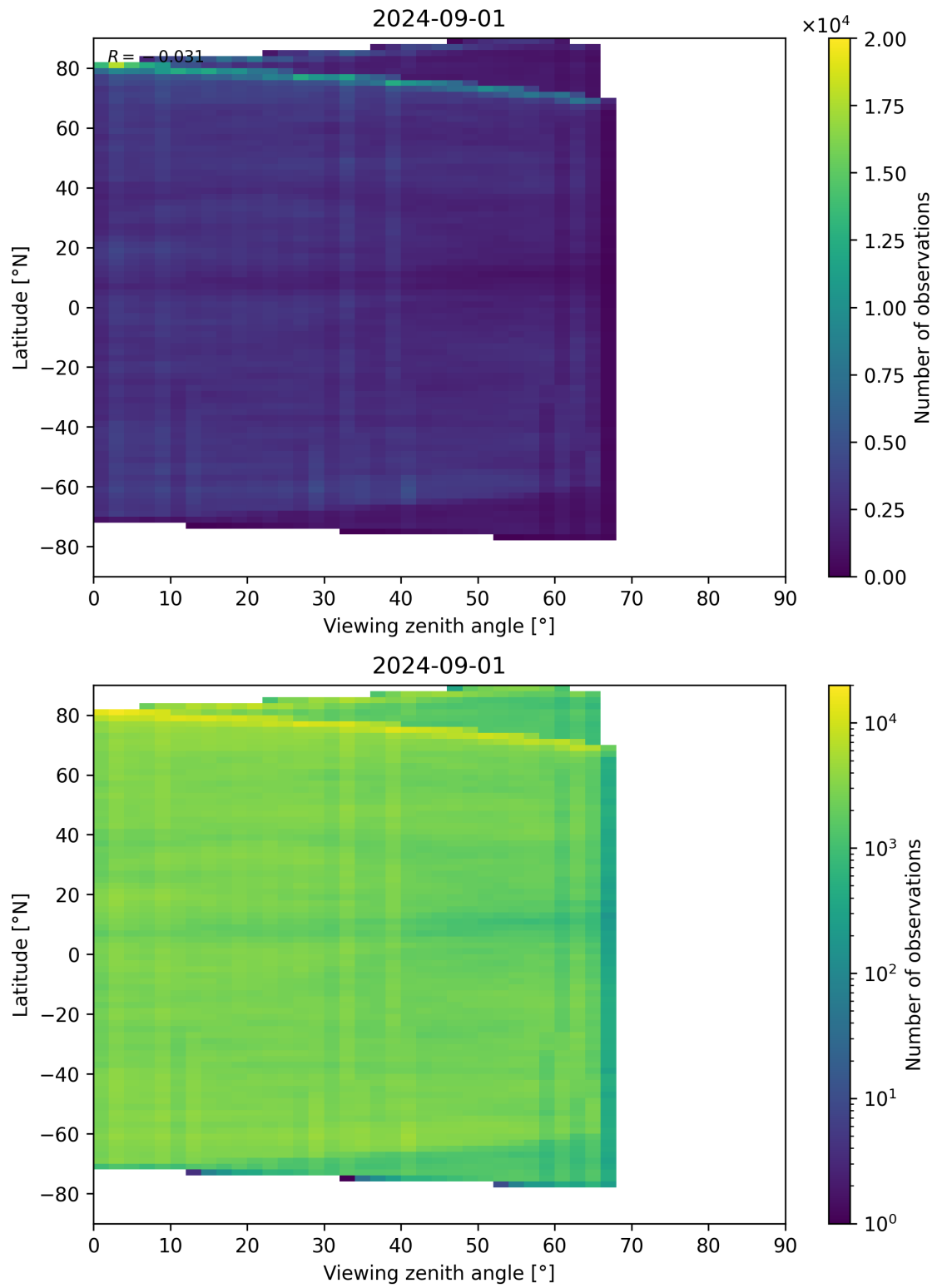
Figure 74: Scatter density plot of “Viewing zenith angle” against “Latitude” for 2024-09-01 to 2024-09-02.
