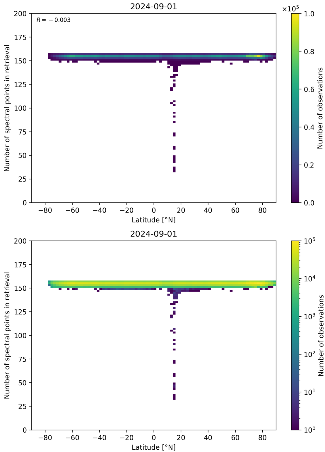
Figure 57: Scatter density plot of “Latitude” against “Number of spectral points in retrieval” for 2024-09-01 to 2024-09-02.
