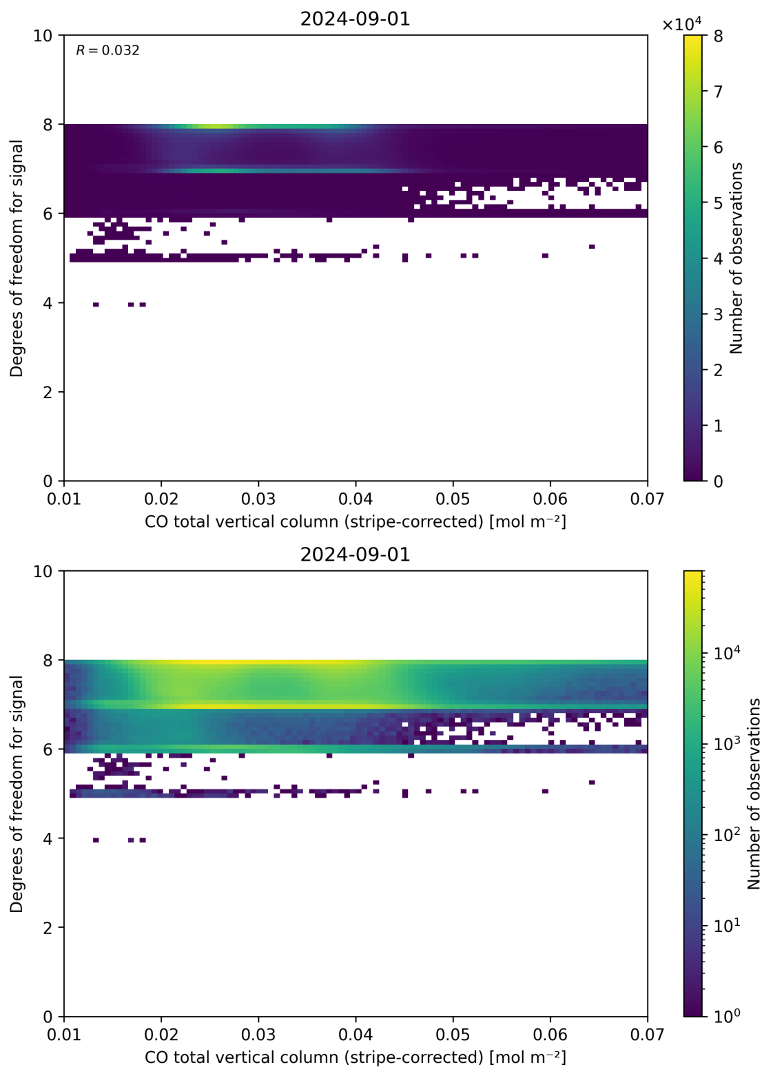
Figure 38: Scatter density plot of “CO total vertical column (stripe-corrected)” against “Degrees of freedom for signal” for 2024-09-01 to 2024-09-02.
