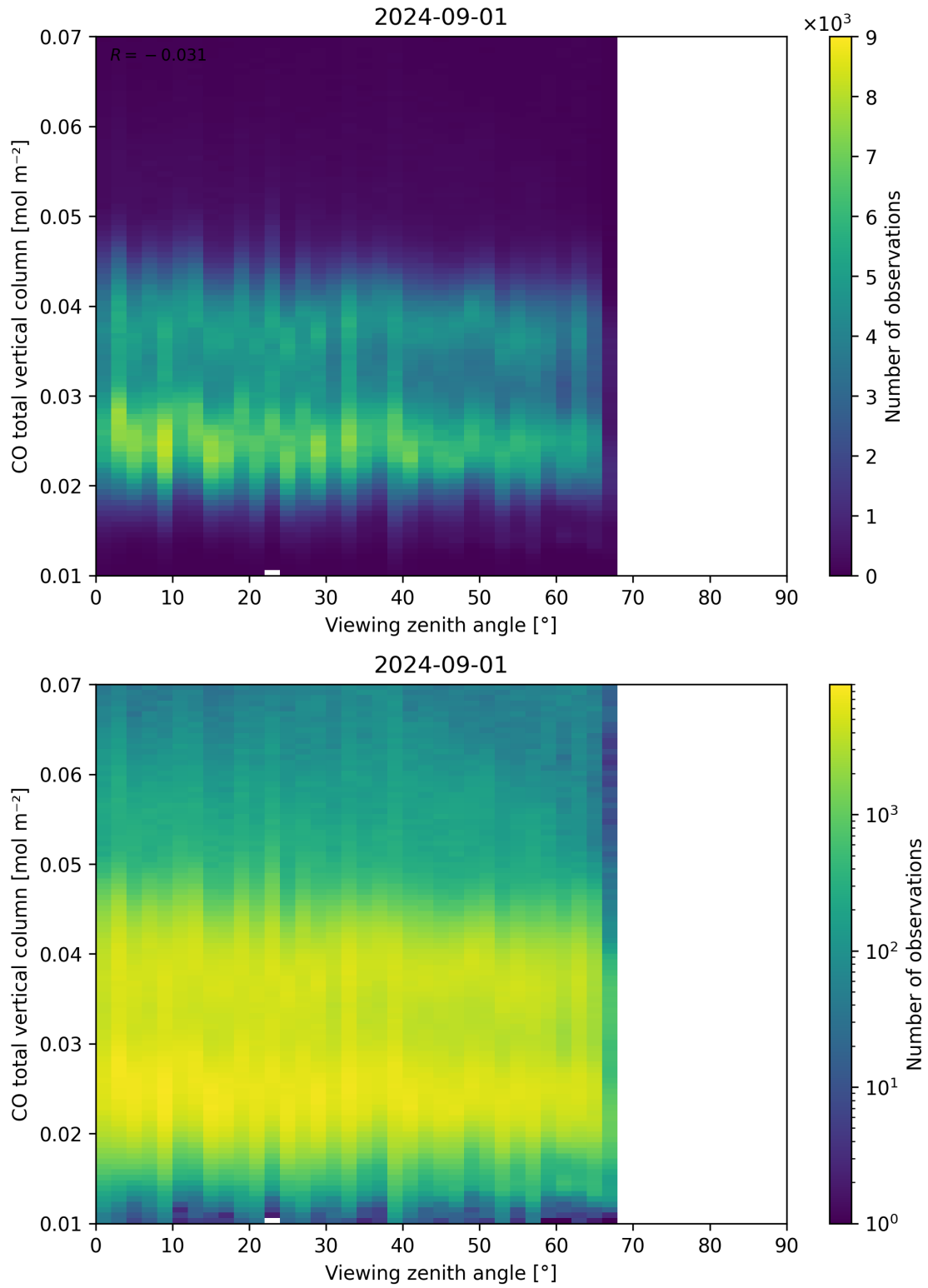
Figure 69: Scatter density plot of “Viewing zenith angle” against “CO total vertical column” for 2024-09-01 to 2024-09-02.
