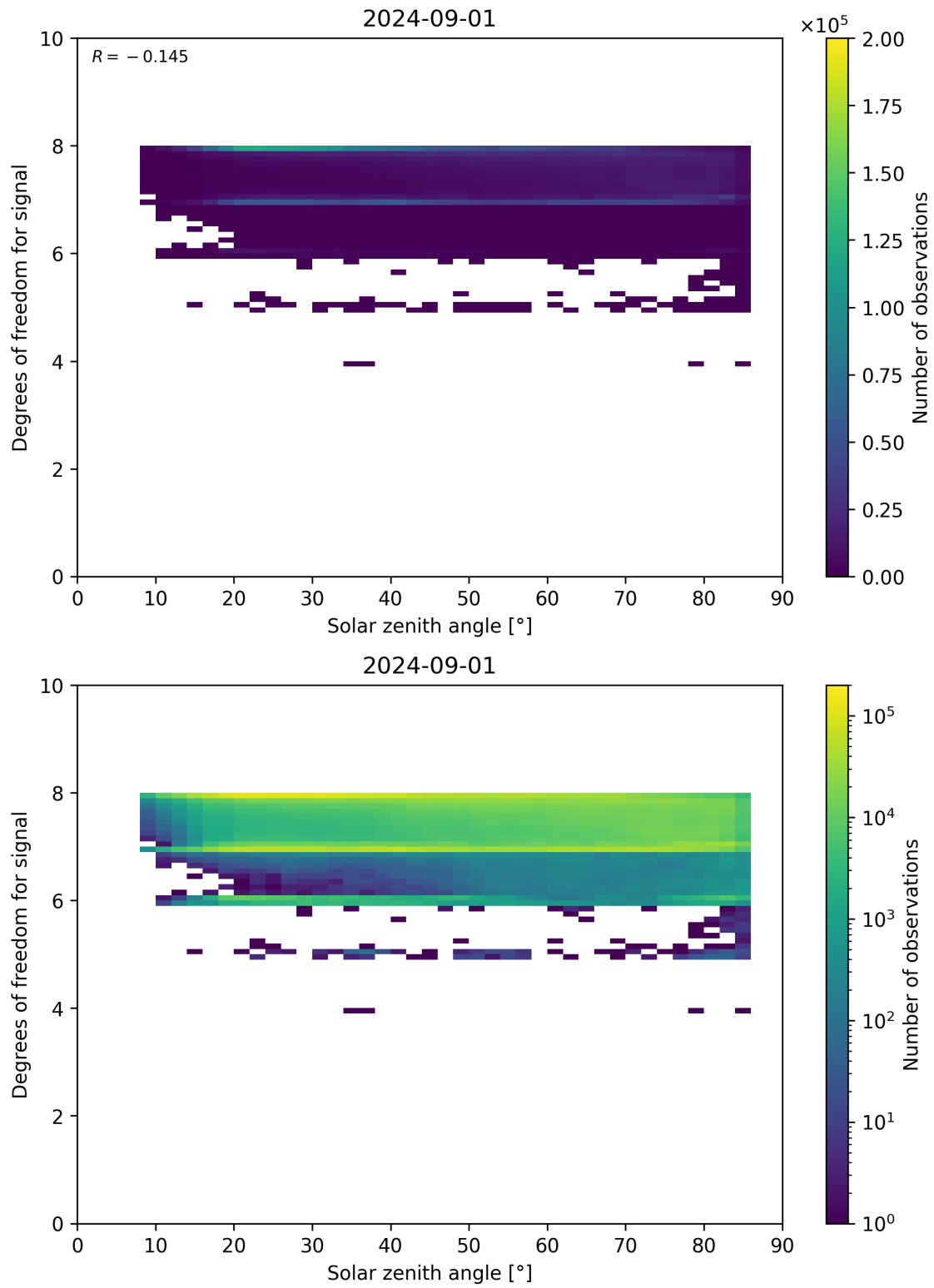
Figure 65: Scatter density plot of “Solar zenith angle” against “Degrees of freedom for signal” for 2024-09-01 to 2024-09-02.
