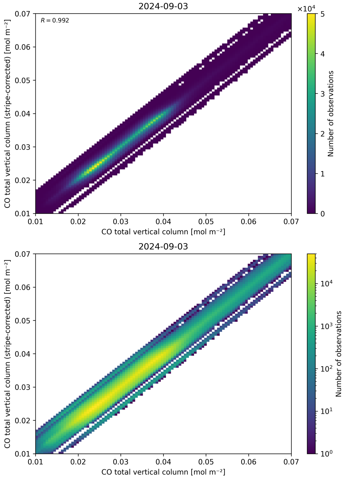
Figure 33: Scatter density plot of “CO total vertical column” against “CO total vertical column (stripe-corrected)” for 2024-09-02 to 2024-09-04.
