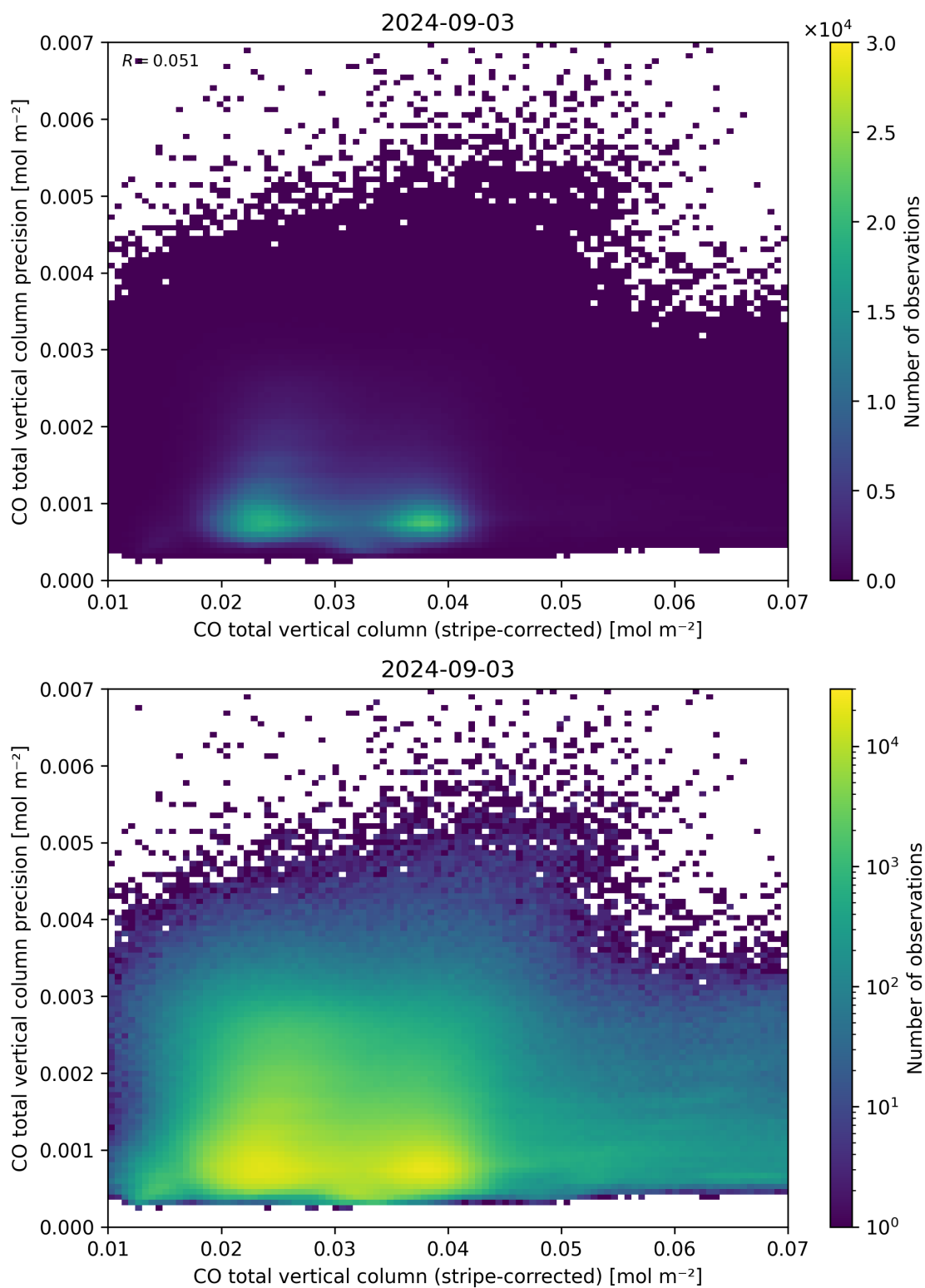
Figure 36: Scatter density plot of “CO total vertical column (stripe-corrected)” against “CO total vertical column precision” for 2024-09-02 to 2024-09-04.
