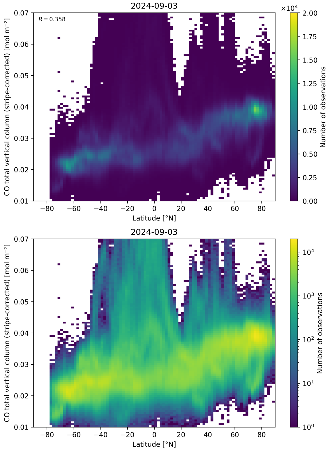
Figure 52: Scatter density plot of “Latitude” against “CO total vertical column (stripe-corrected)” for 2024-09-02 to 2024-09-04.
