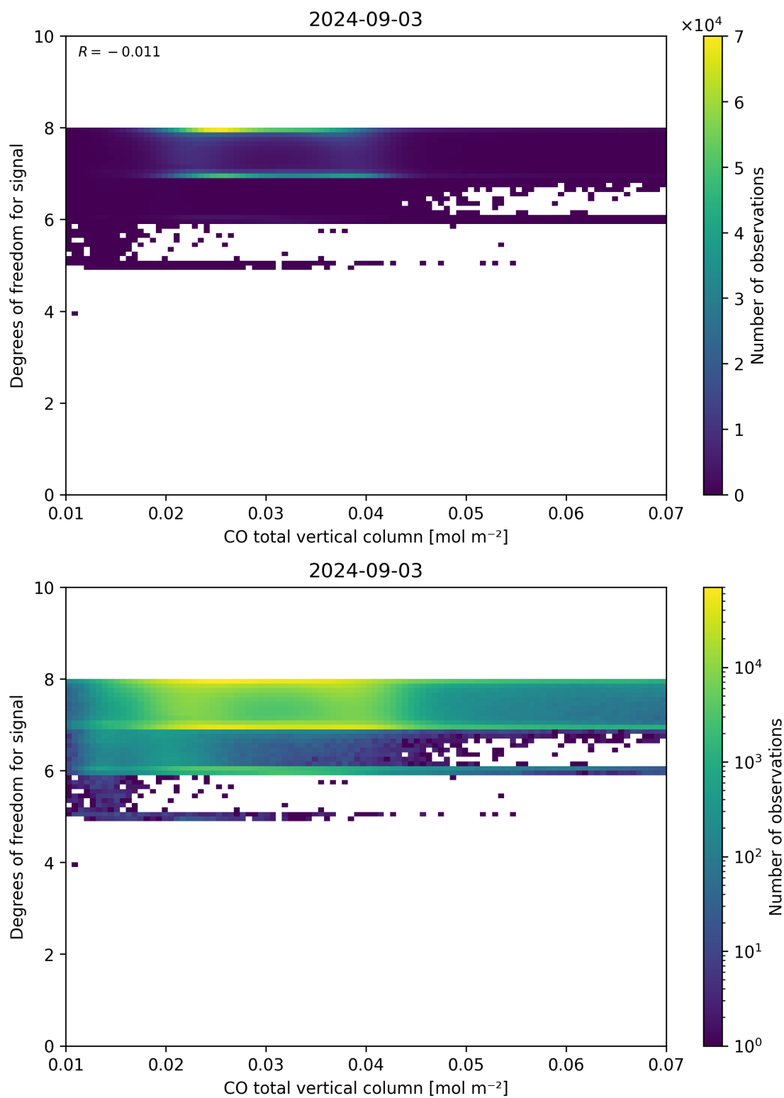
Figure 41: Scatter density plot of “CO total vertical column” against “Degrees of freedom for signal” for 2024-09-02 to 2024-09-04.
