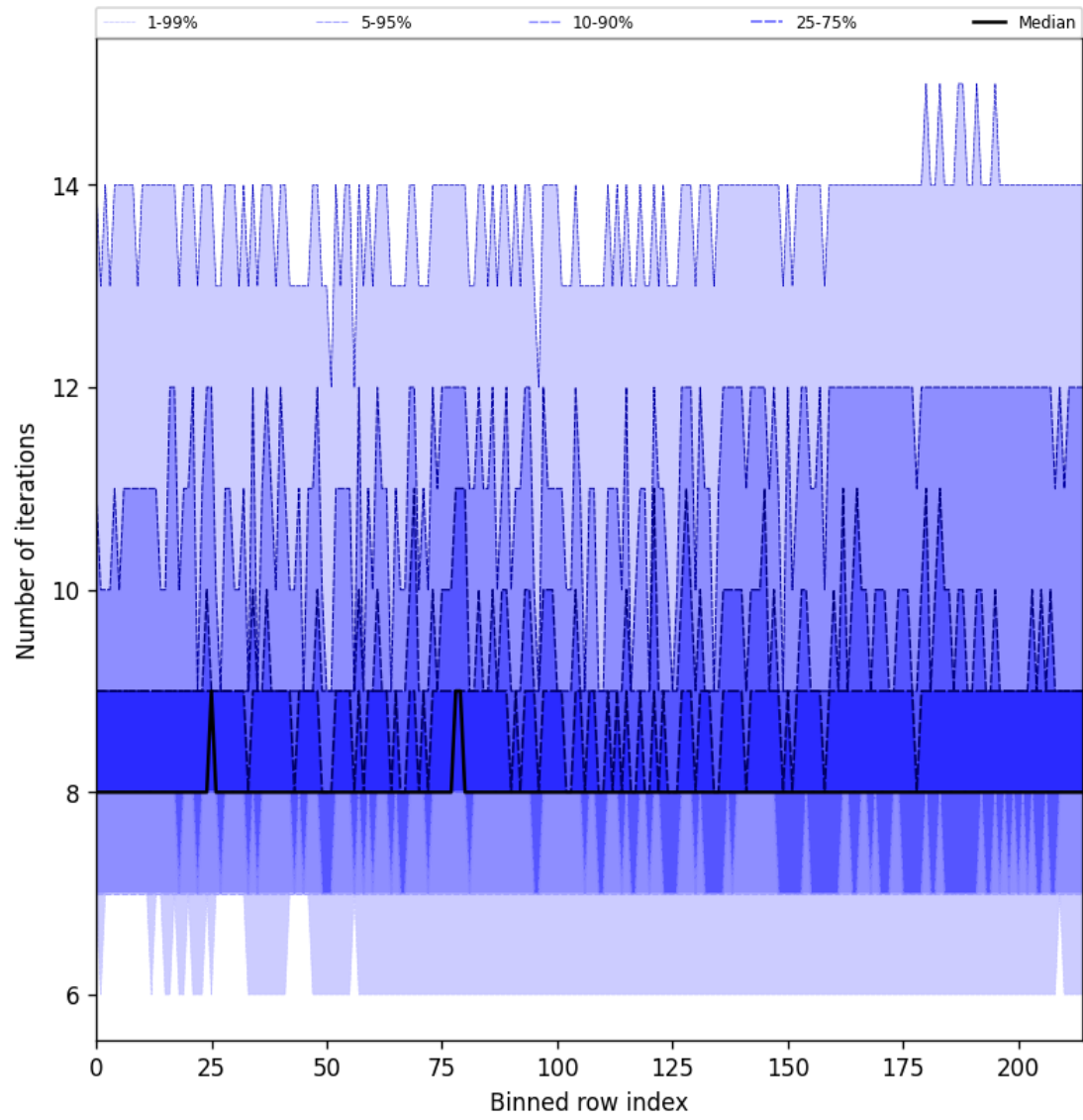
Figure 32: Along track statistics of “Number of iterations” for 2024-09-02 to 2024-09-04
