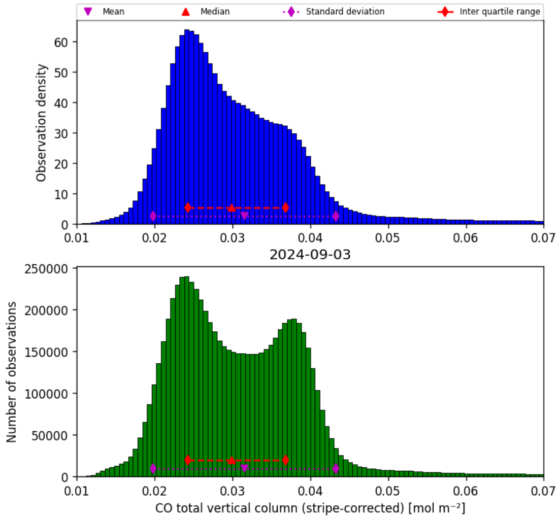
Figure 19: Histogram of “CO total vertical column (stripe-corrected)” for 2024-09-02 to 2024-09-04
