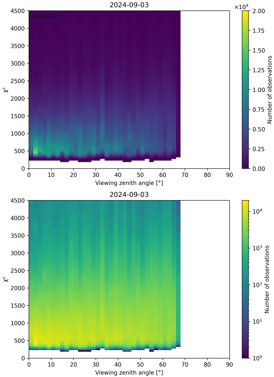
Figure 72: Scatter density plot of “Viewing zenith angle” against “ \chi^2 ” for 2024-09-02 to 2024-09-04.
