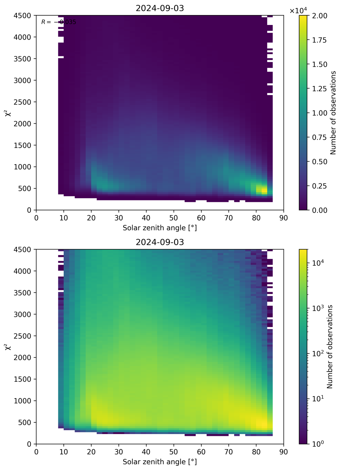
Figure 64: Scatter density plot of “Solar zenith angle” against “ \chi^2 ” for 2024-09-02 to 2024-09-04.
