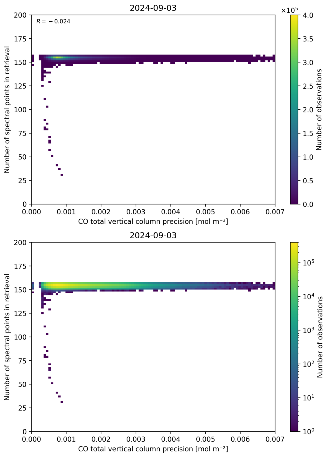
Figure 47: Scatter density plot of “CO total vertical column precision” against “Number of spectral points in retrieval” for 2024-09-02 to 2024-09-04.
