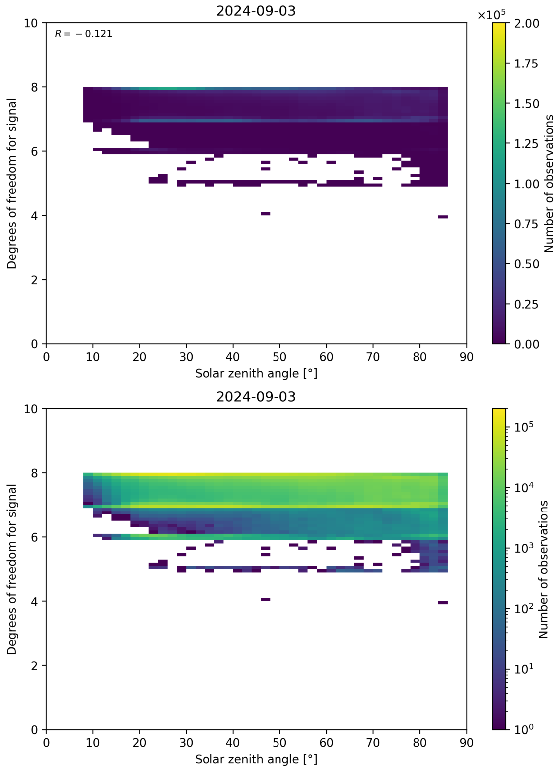
Figure 65: Scatter density plot of “Solar zenith angle” against “Degrees of freedom for signal” for 2024-09-02 to 2024-09-04.
