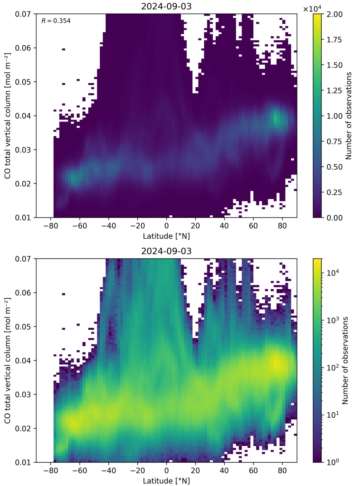
Figure 51: Scatter density plot of “Latitude” against “CO total vertical column” for 2024-09-02 to 2024-09-04.
