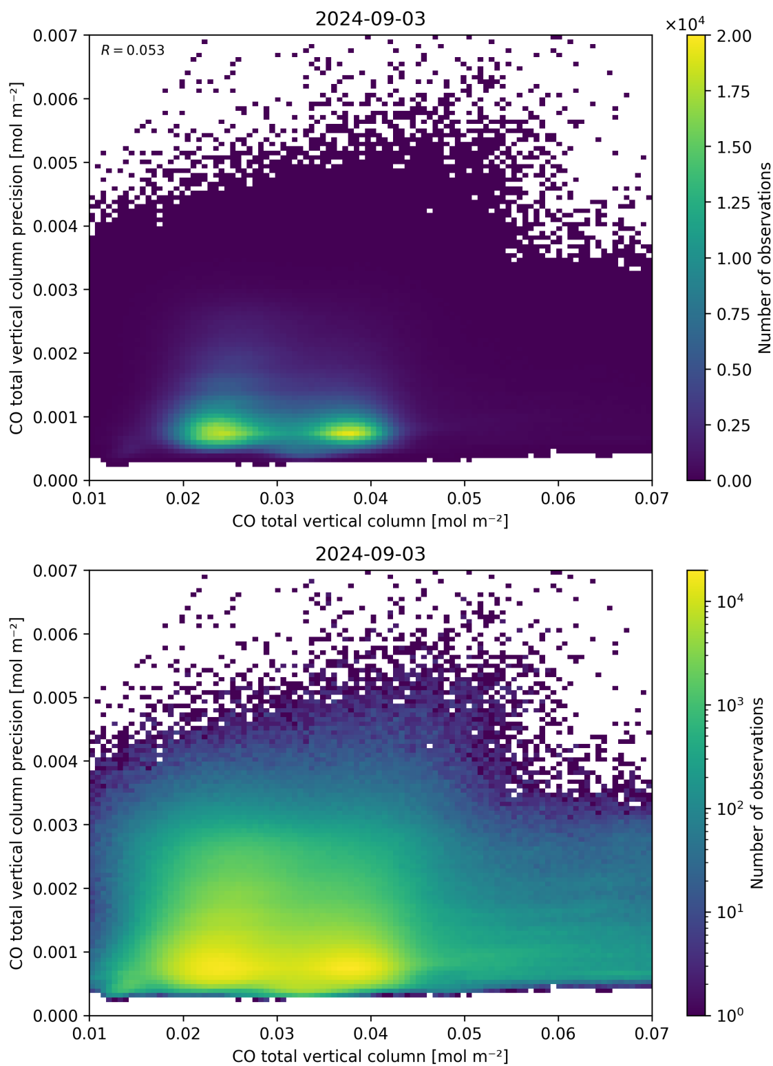
Figure 34: Scatter density plot of “CO total vertical column” against “CO total vertical column precision” for 2024-09-02 to 2024-09-04.
