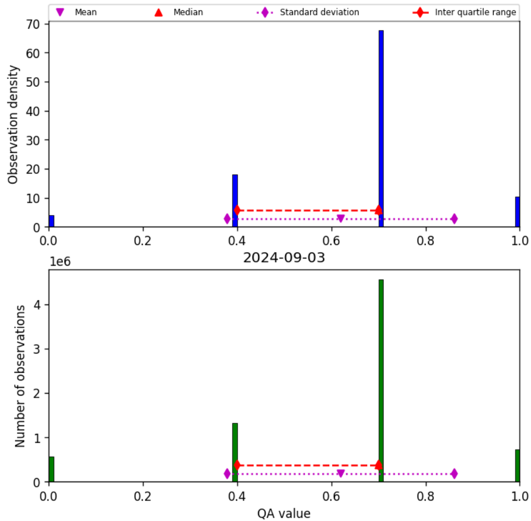
Figure 17: Histogram of “QA value” for 2024-09-02 to 2024-09-04
