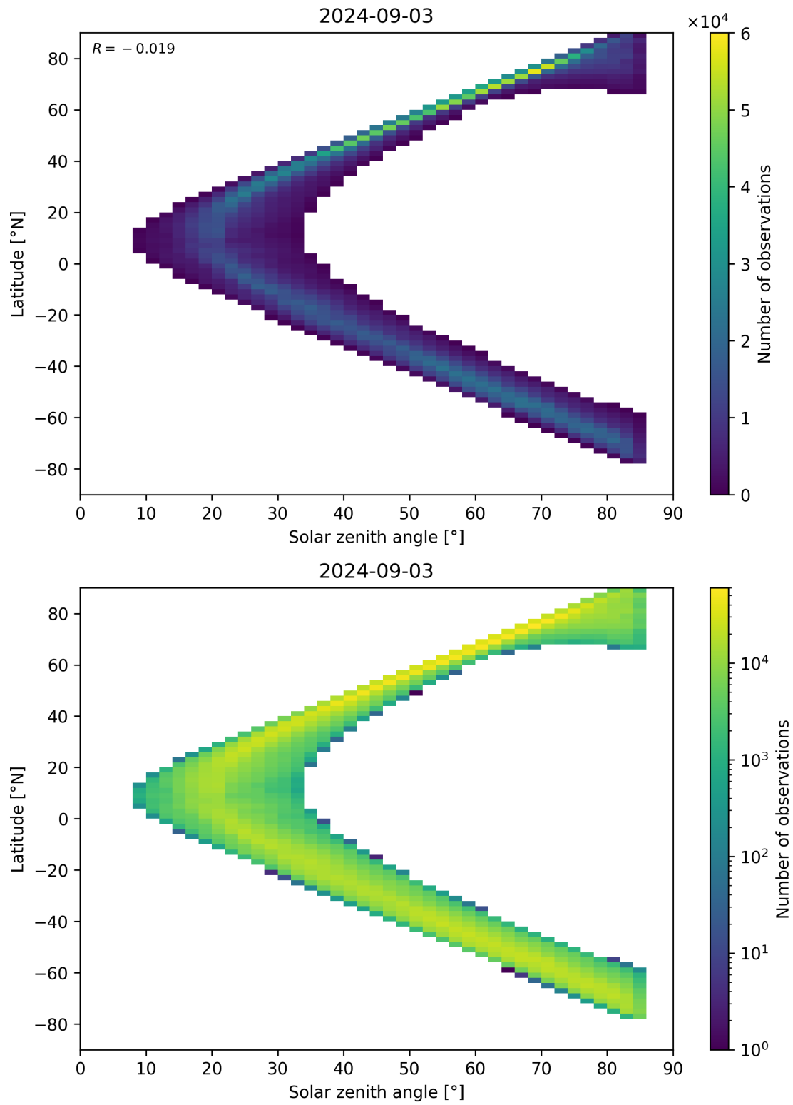
Figure 66: Scatter density plot of “Solar zenith angle” against “Latitude” for 2024-09-02 to 2024-09-04.
