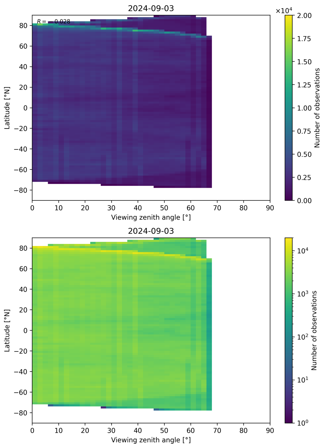
Figure 74: Scatter density plot of “Viewing zenith angle” against “Latitude” for 2024-09-02 to 2024-09-04.
