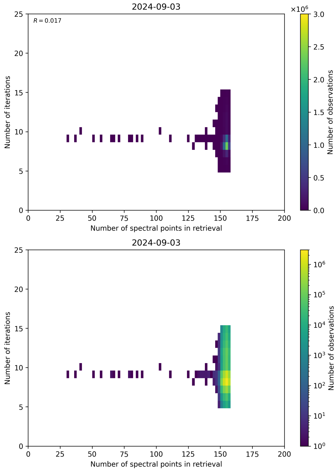
Figure 60: Scatter density plot of “Number of spectral points in retrieval” against “Number of iterations” for 2024-09-02 to 2024-09-04.
