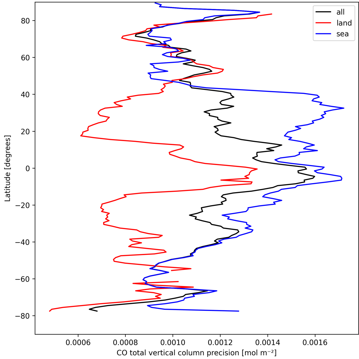
Figure 12: Zonal average of “CO total vertical column precision” for 2024-09-02 to 2024-09-04.
