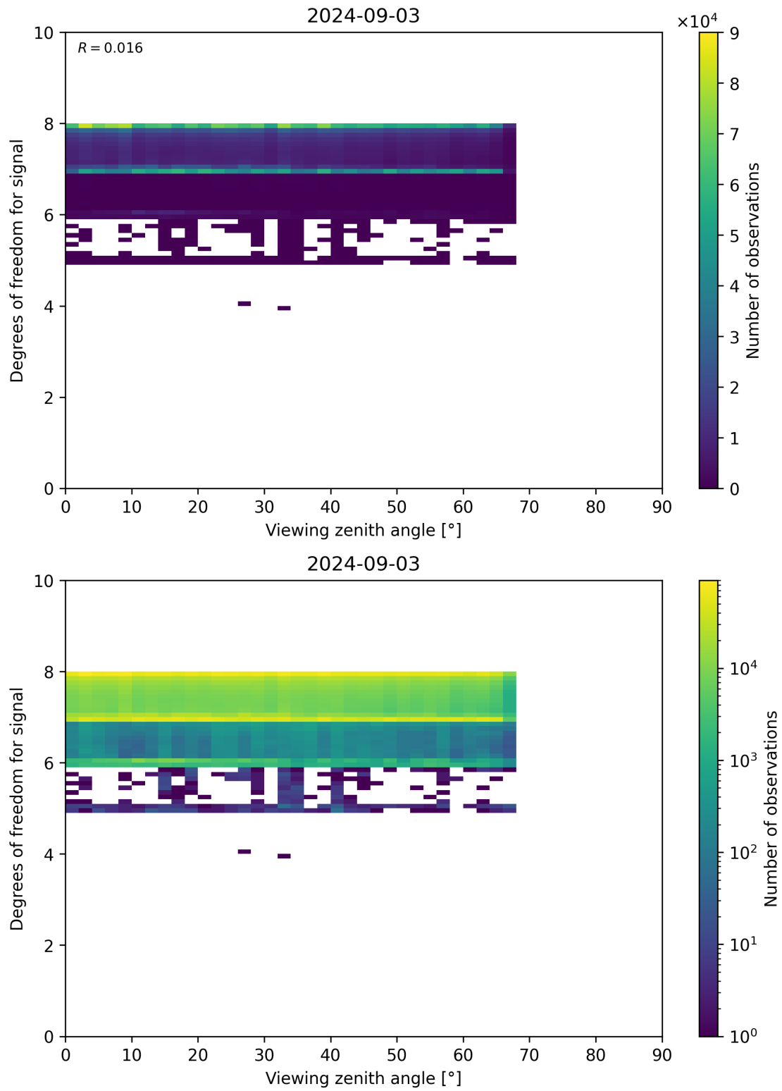
Figure 73: Scatter density plot of “Viewing zenith angle” against “Degrees of freedom for signal” for 2024-09-02 to 2024-09-04.
