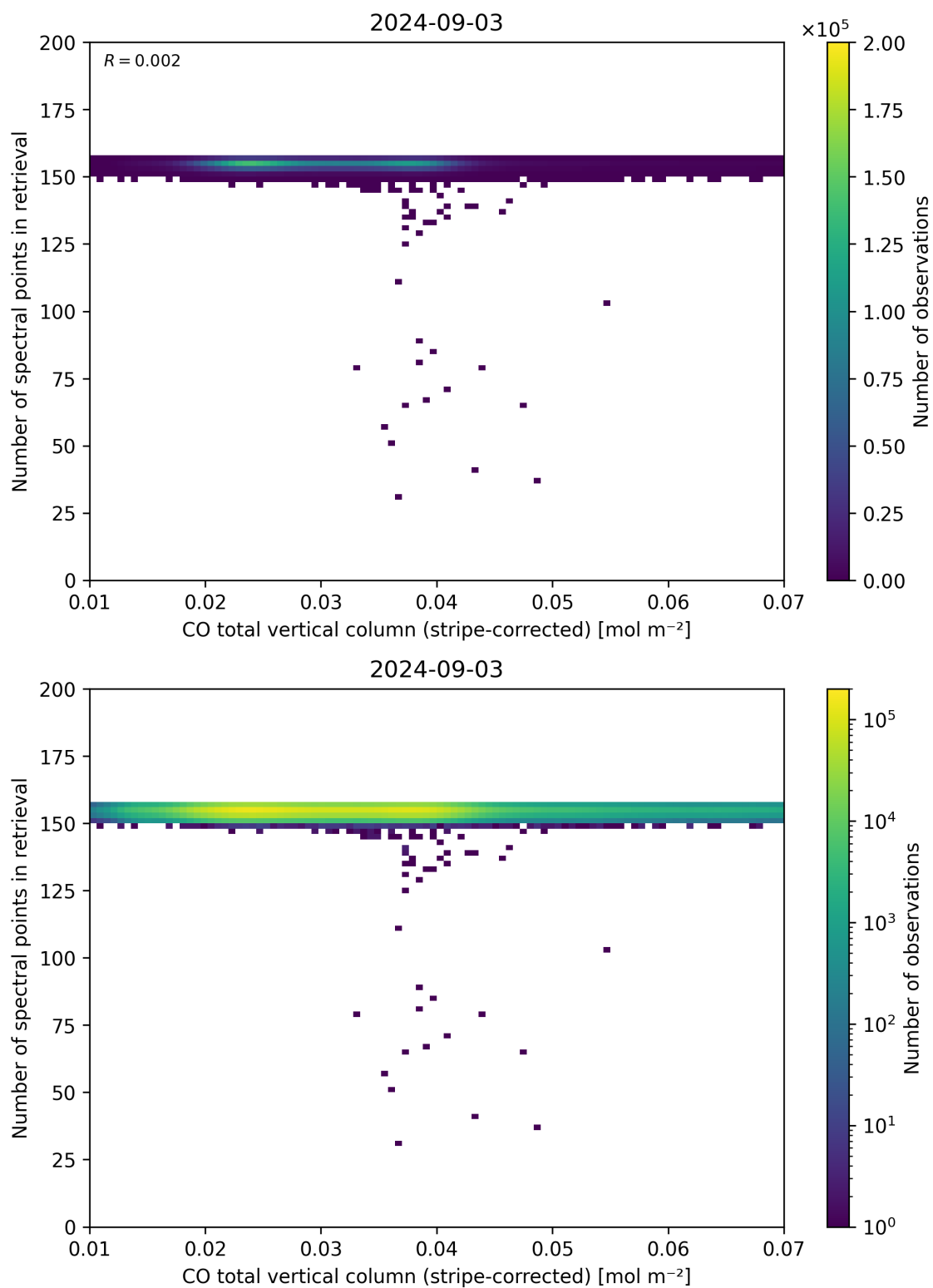
Figure 40: Scatter density plot of “CO total vertical column (stripe-corrected)” against “Number of spectral points in retrieval” for 2024-09-02 to 2024-09-04.
