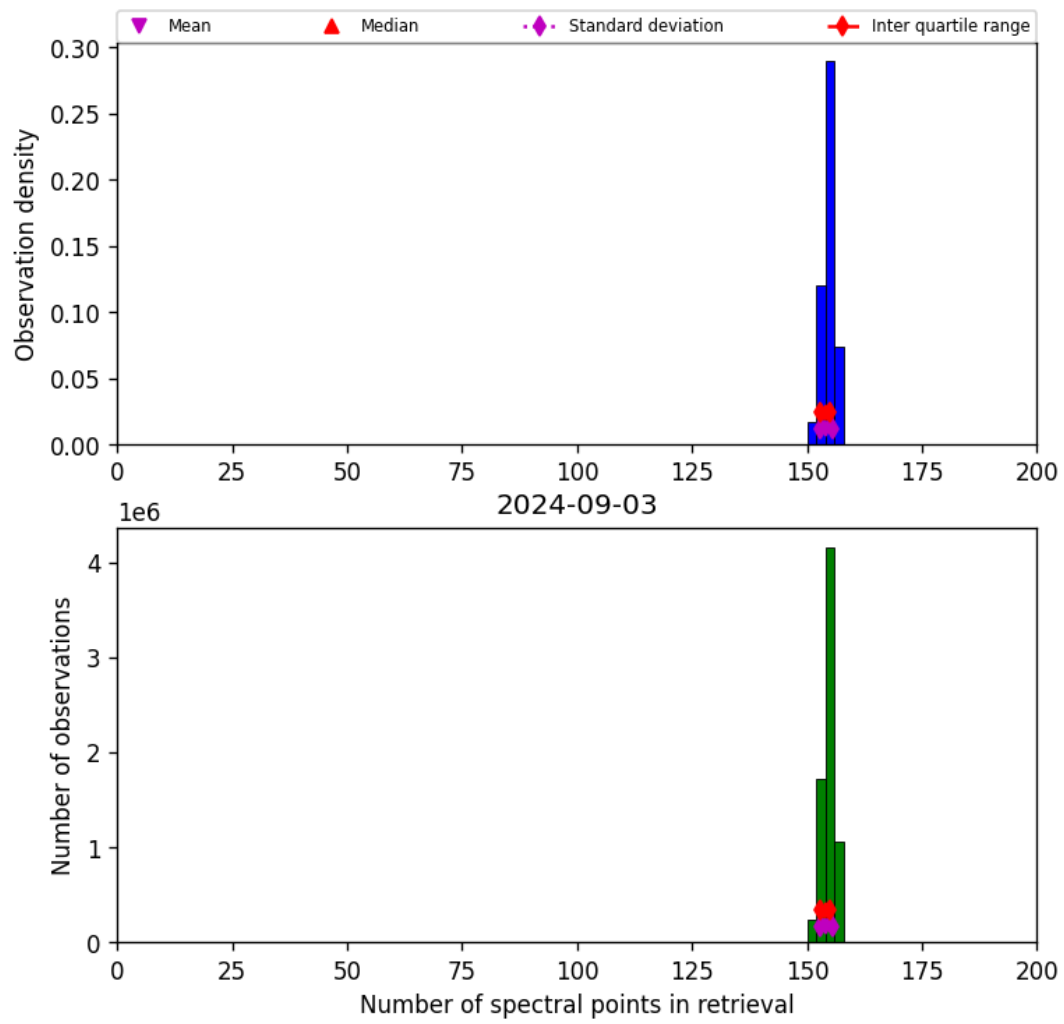
Figure 21: Histogram of “Number of spectral points in retrieval” for 2024-09-02 to 2024-09-04
