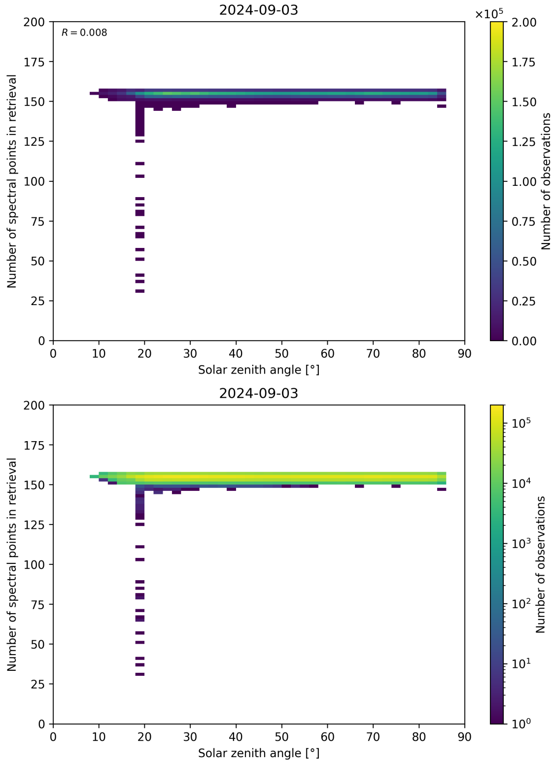
Figure 68: Scatter density plot of “Solar zenith angle” against “Number of spectral points in retrieval” for 2024-09-02 to 2024-09-04.
