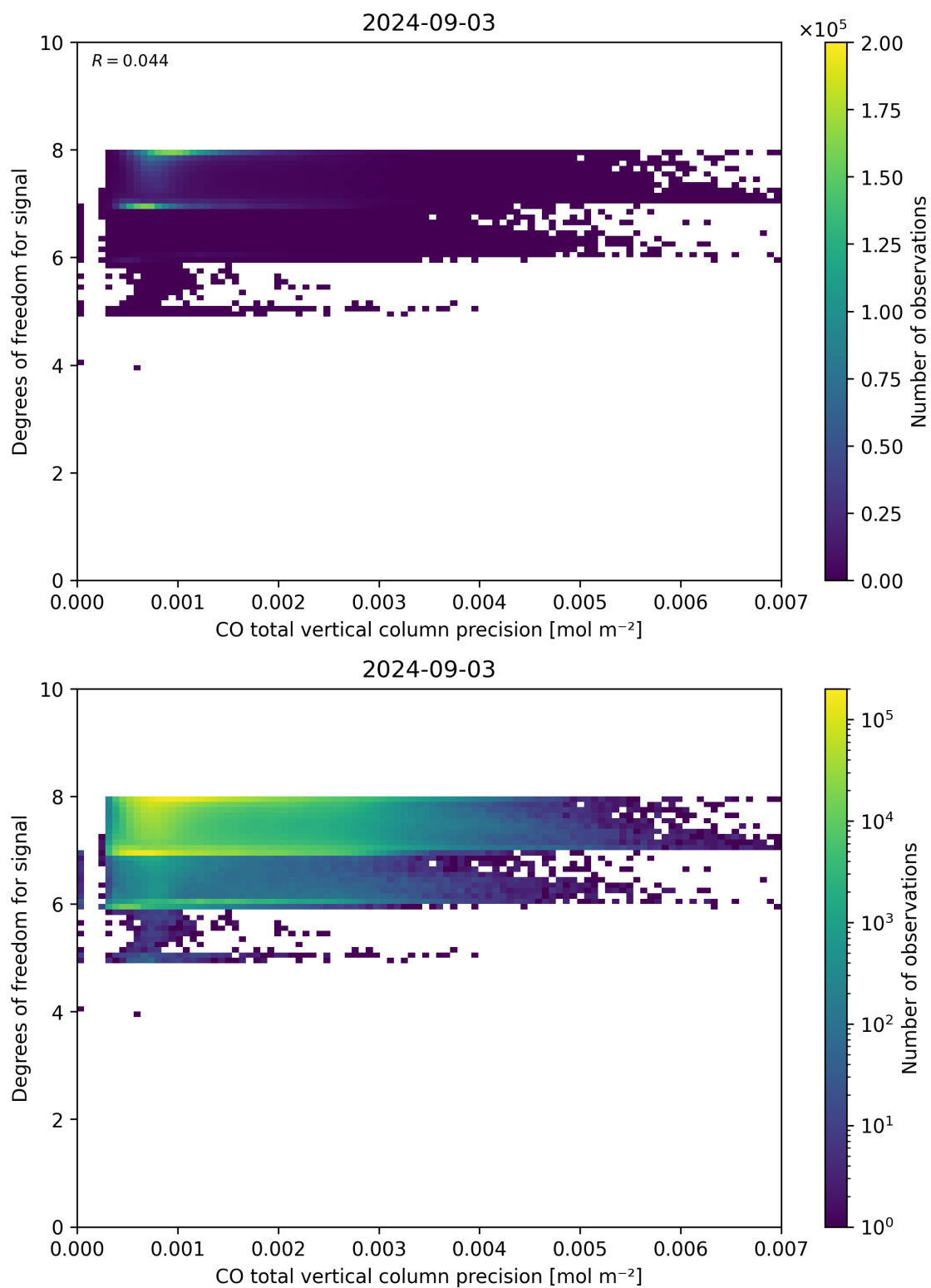
Figure 45: Scatter density plot of “CO total vertical column precision” against “Degrees of freedom for signal” for 2024-09-02 to 2024-09-04.
