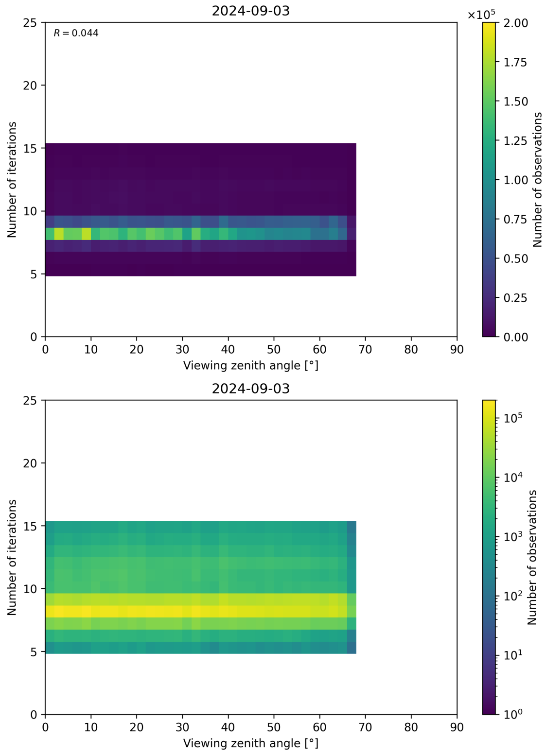
Figure 75: Scatter density plot of “Viewing zenith angle” against “Number of iterations” for 2024-09-02 to 2024-09-04.
