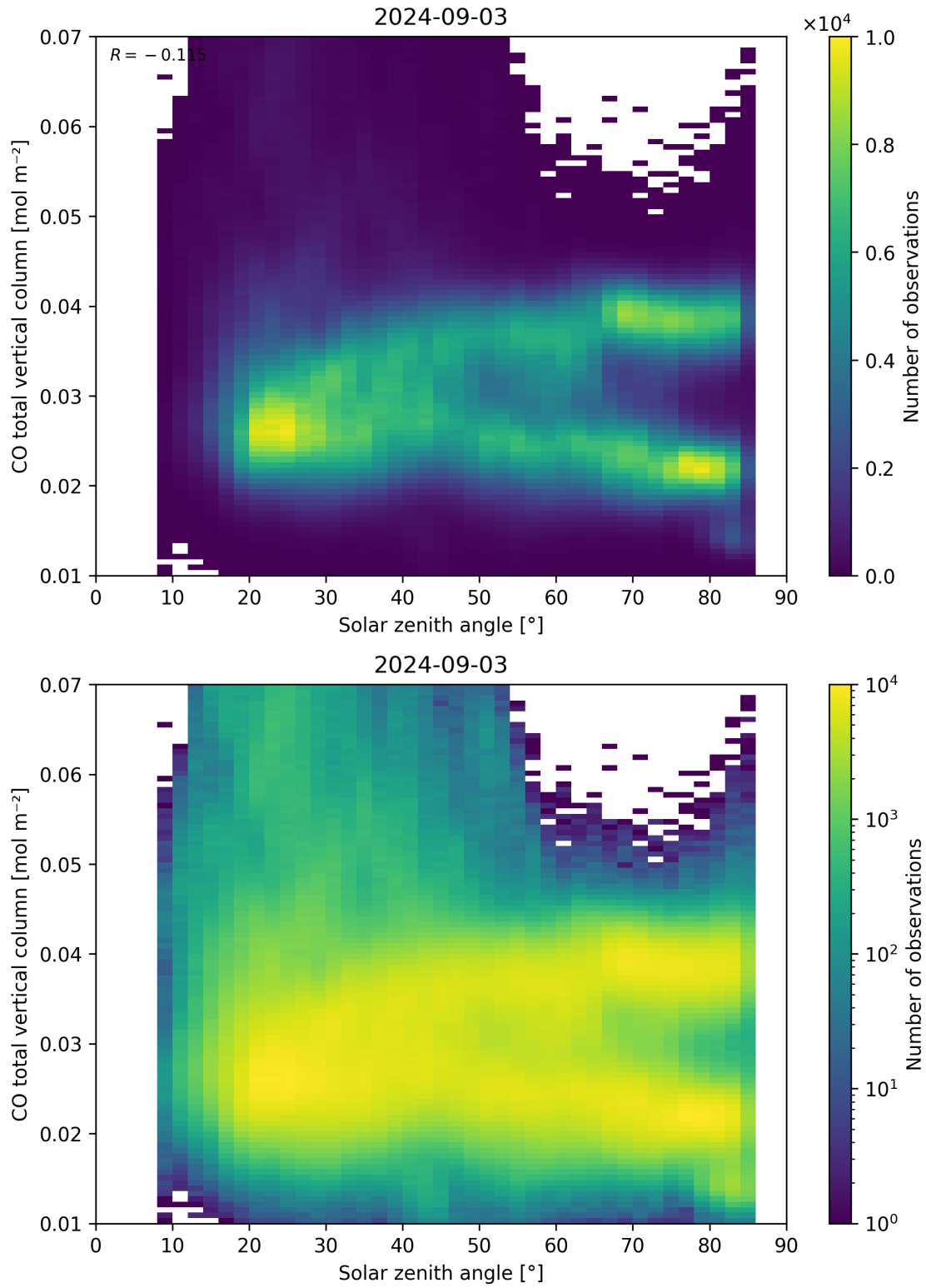
Figure 61: Scatter density plot of “Solar zenith angle” against “CO total vertical column” for 2024-09-02 to 2024-09-04.
