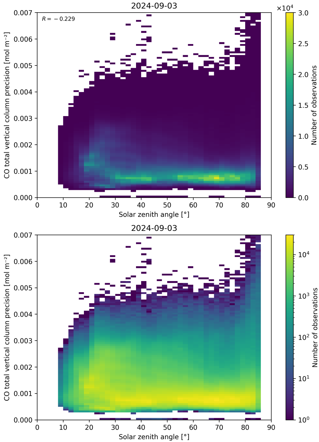
Figure 63: Scatter density plot of “Solar zenith angle” against “CO total vertical column precision” for 2024-09-02 to 2024-09-04.
