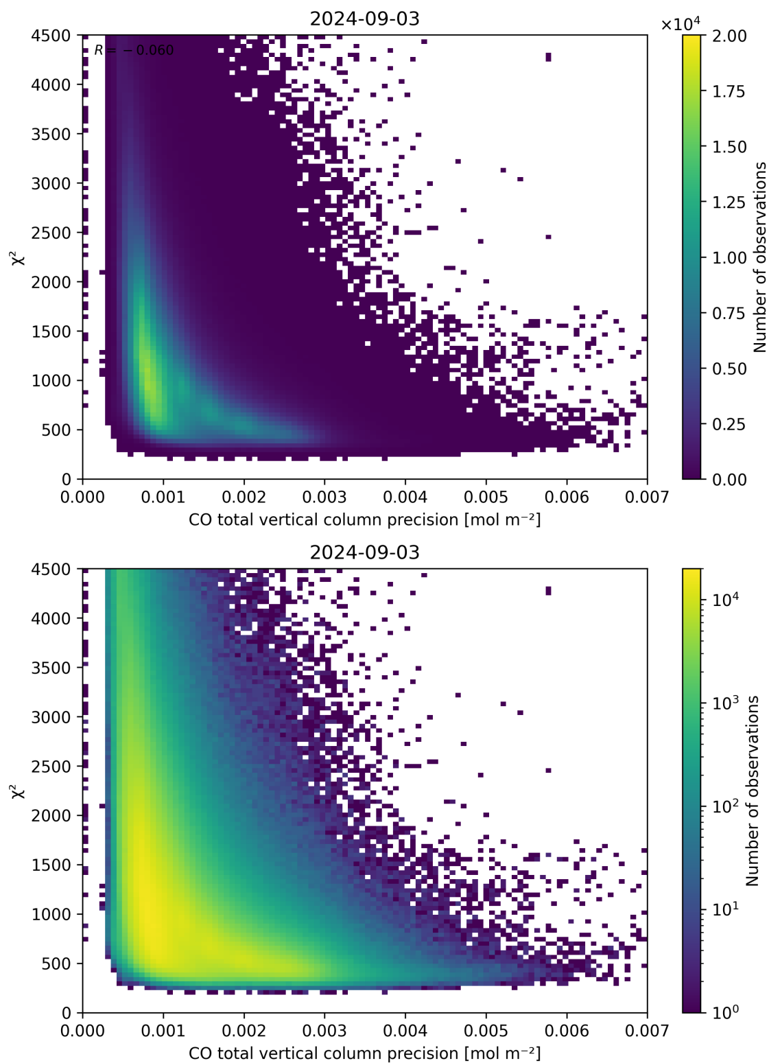
Figure 44: Scatter density plot of “CO total vertical column precision” against “ \chi^2 ” for 2024-09-02 to 2024-09-04.
