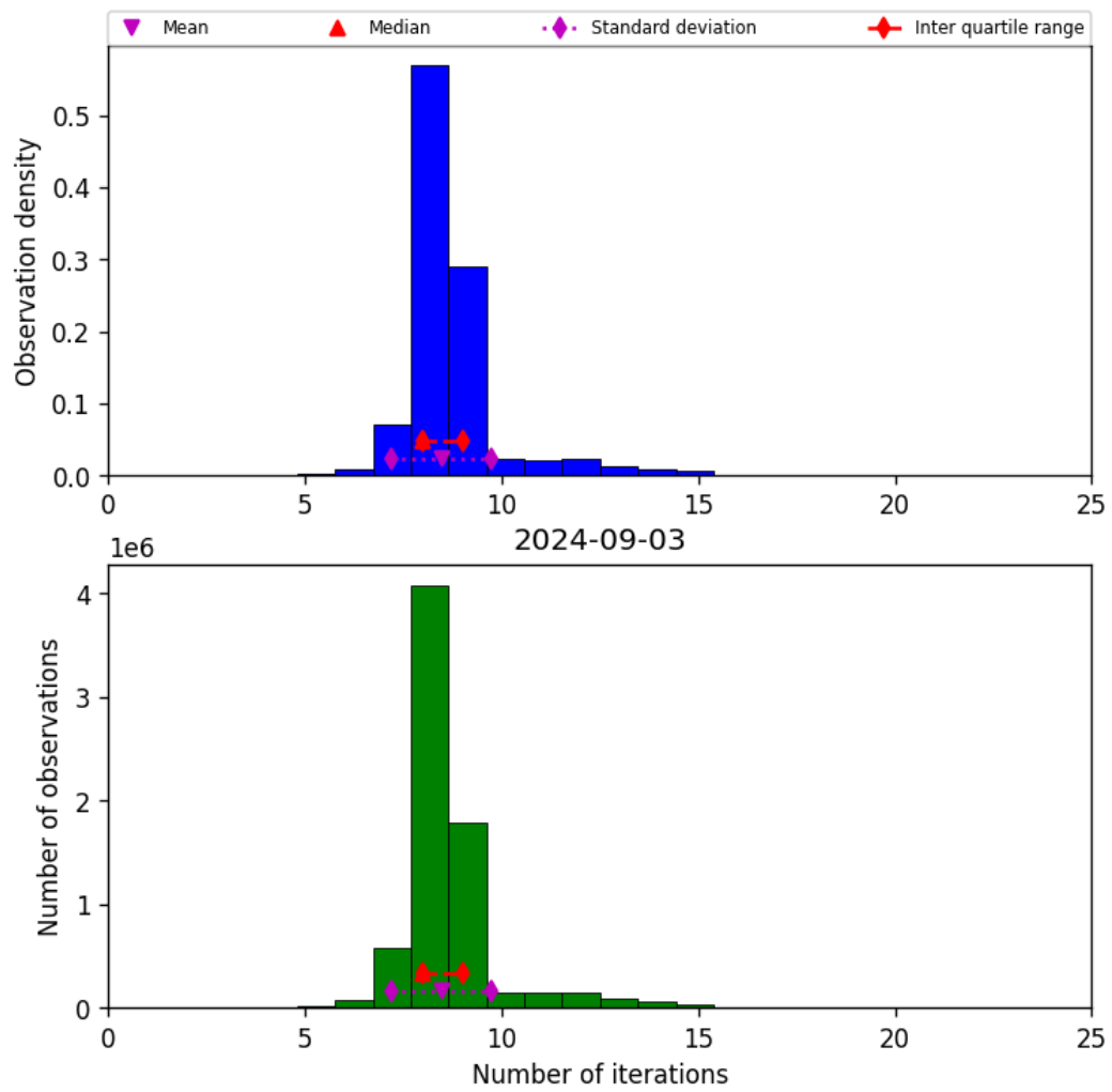
Figure 24: Histogram of “Number of iterations” for 2024-09-02 to 2024-09-04
