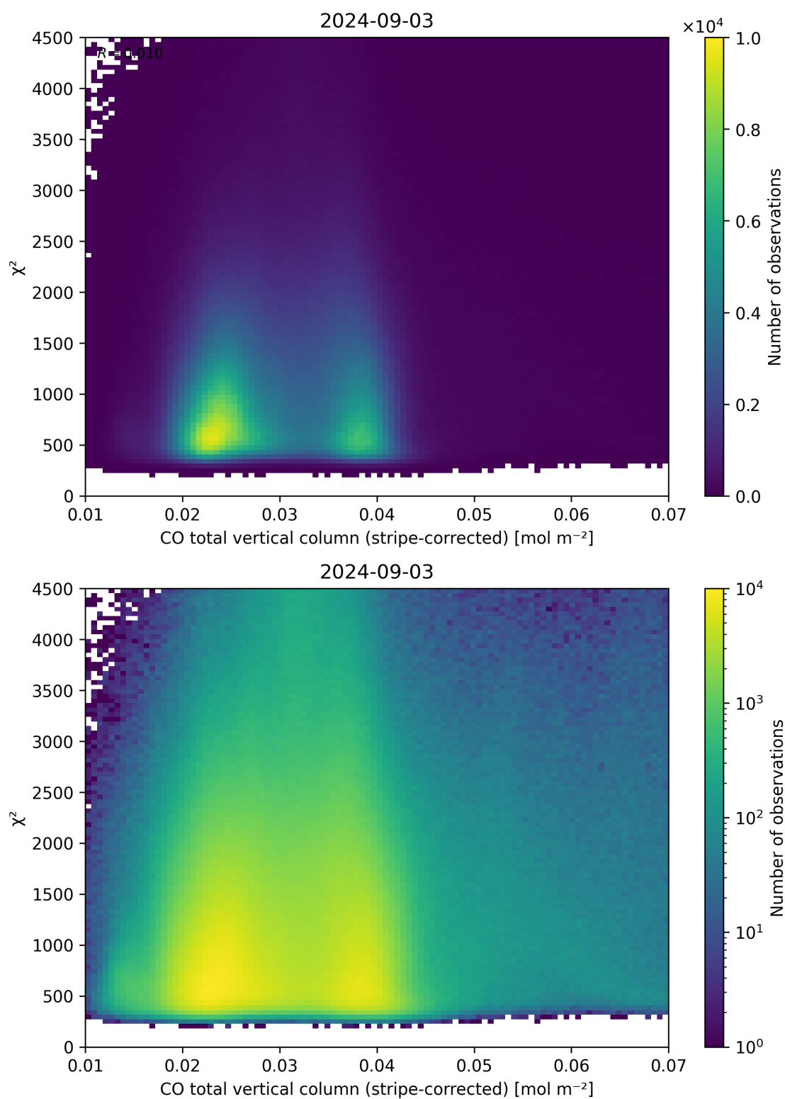
Figure 37: Scatter density plot of “CO total vertical column (stripe-corrected)” against “ \chi^2 ” for 2024-09-02 to 2024-09-04.
