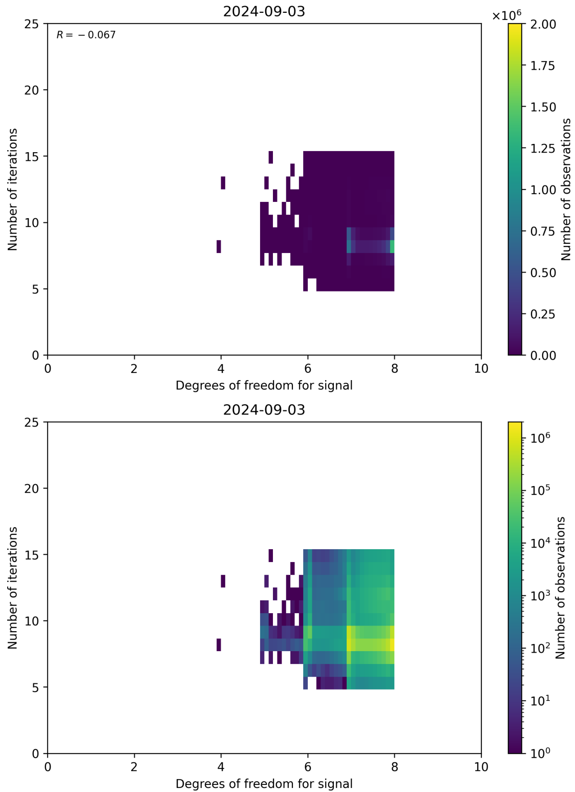
Figure 50: Scatter density plot of “Degrees of freedom for signal” against “Number of iterations” for 2024-09-02 to 2024-09-04.
