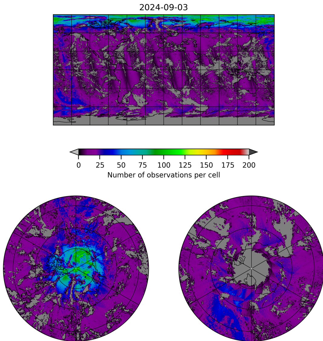
Figure 8: Map of the number of observations for 2024-09-02 to 2024-09-04
