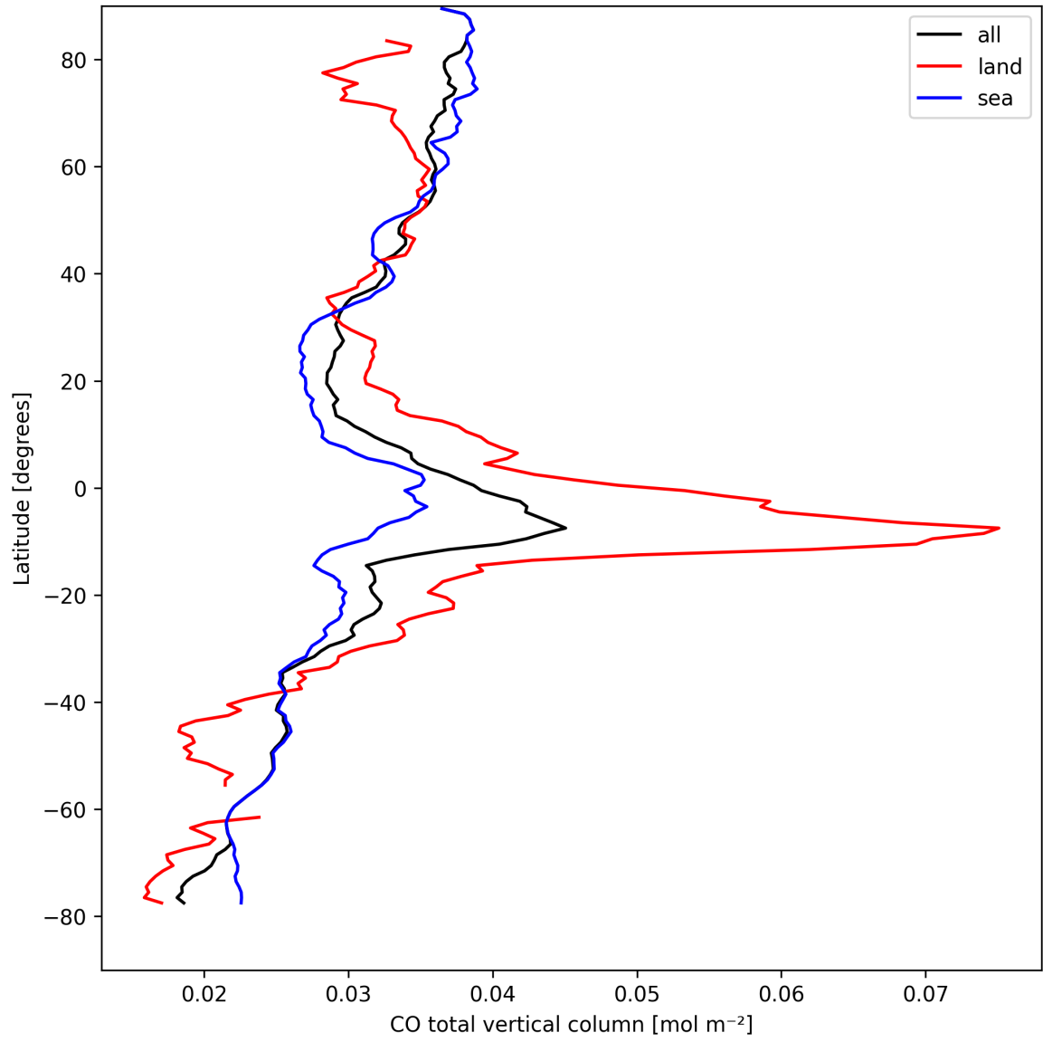
Figure 10: Zonal average of “CO total vertical column” for 2024-09-02 to 2024-09-04.
