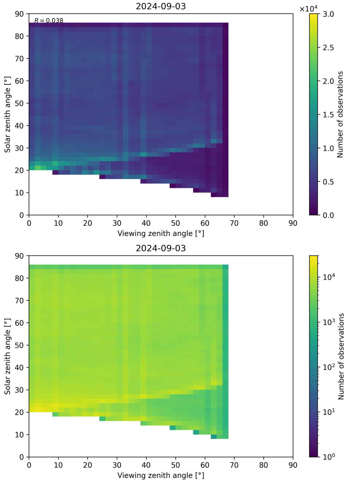
Figure 77: Scatter density plot of “Viewing zenith angle” against “Solar zenith angle” for 2024-09-02 to 2024-09-04.
