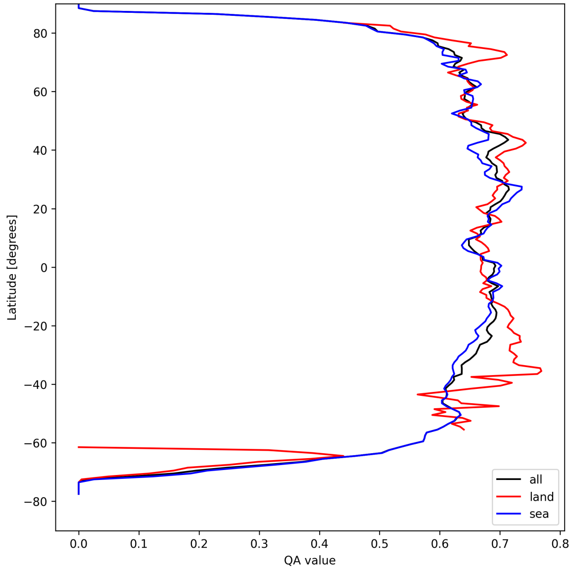
Figure 9: Zonal average of “QA value” for 2024-09-02 to 2024-09-04.
