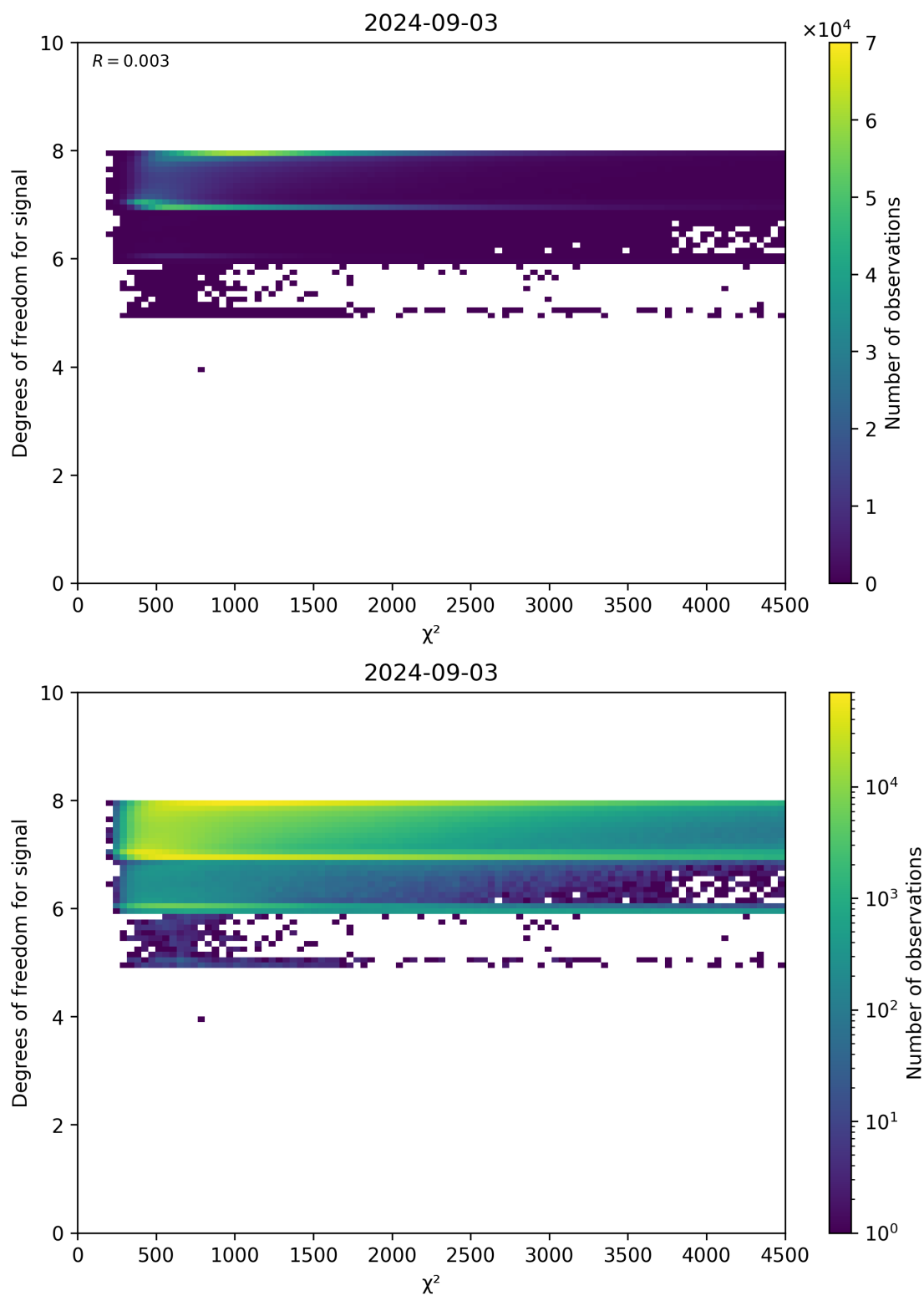
Figure 48: Scatter density plot of “ \chi^2 ” against “Degrees of freedom for signal” for 2024-09-02 to 2024-09-04.
