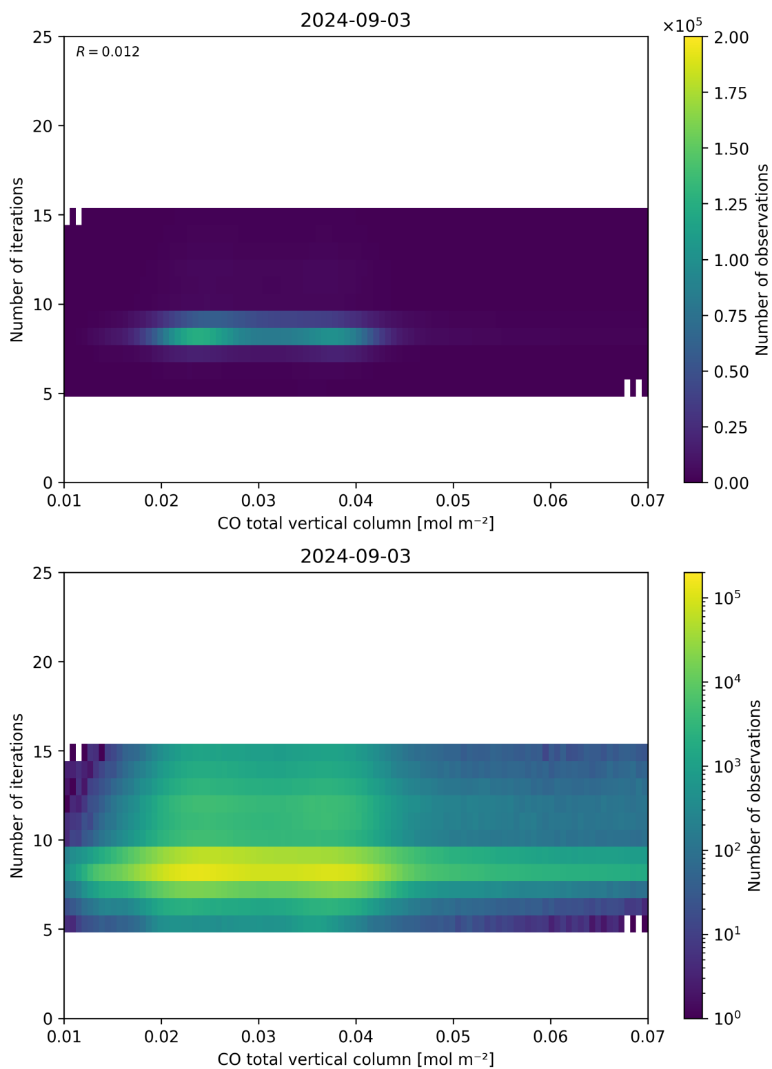
Figure 42: Scatter density plot of “CO total vertical column” against “Number of iterations” for 2024-09-02 to 2024-09-04.
