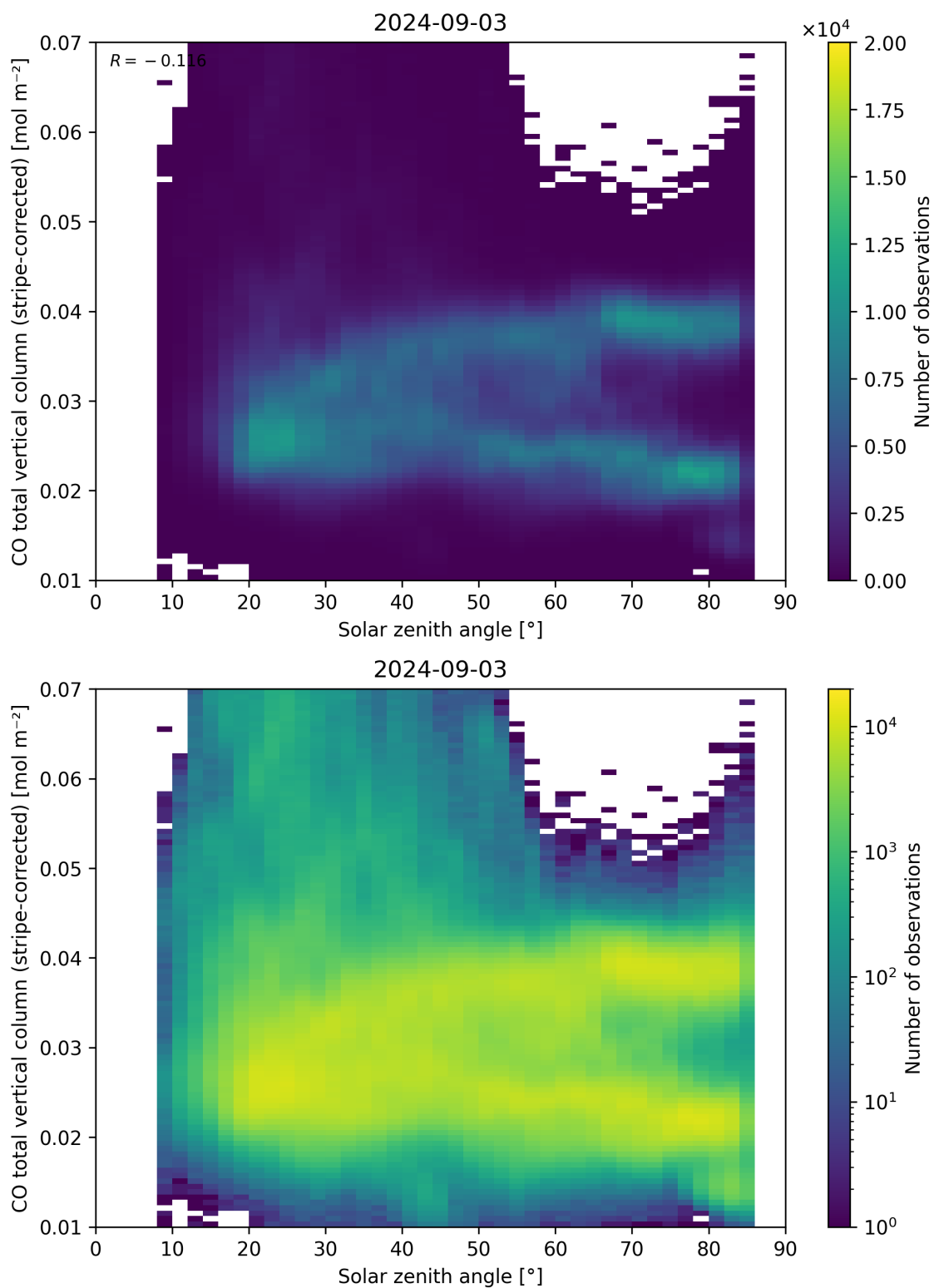
Figure 62: Scatter density plot of “Solar zenith angle” against “CO total vertical column (stripe-corrected)” for 2024-09-02 to 2024-09-04.
