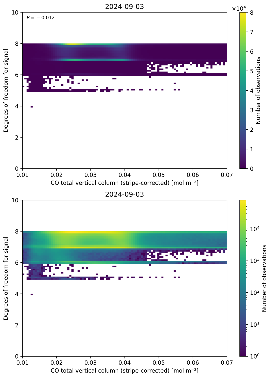
Figure 38: Scatter density plot of “CO total vertical column (stripe-corrected)” against “Degrees of freedom for signal” for 2024-09-02 to 2024-09-04.
