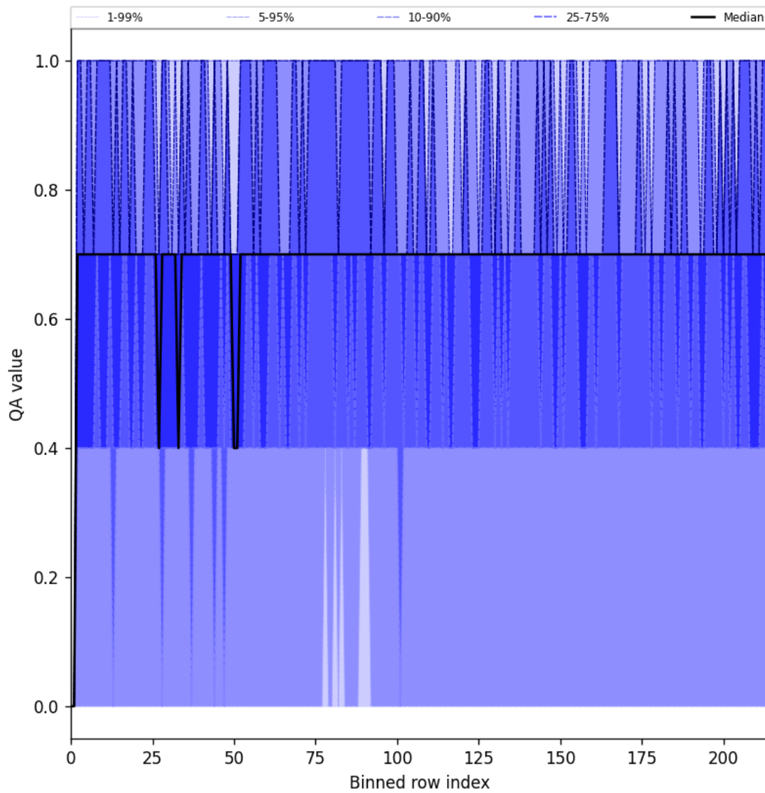
Figure 25: Along track statistics of “QA value” for 2024-09-02 to 2024-09-04
