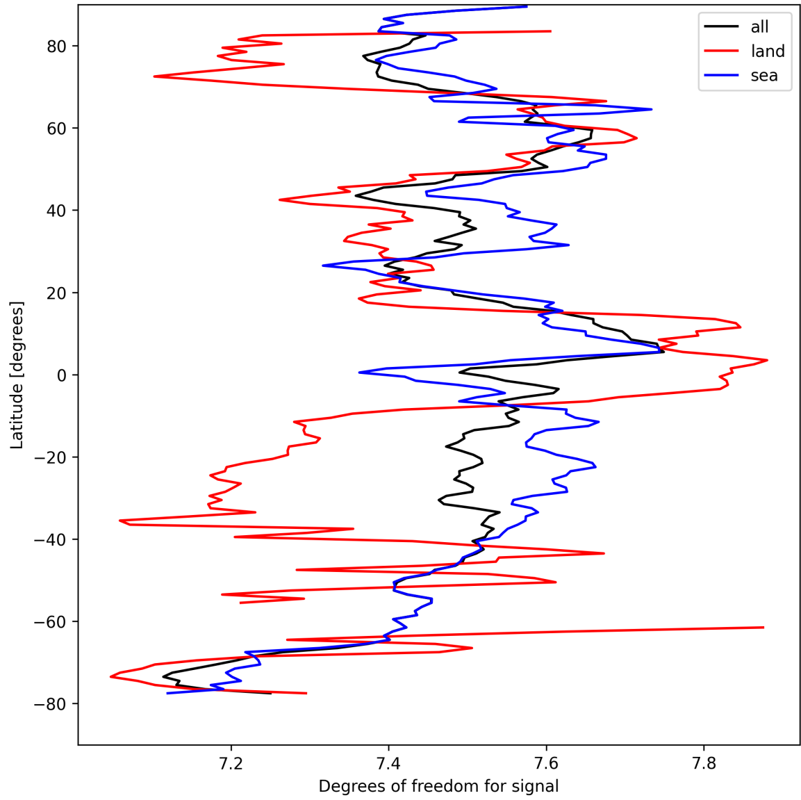
Figure 15: Zonal average of “Degrees of freedom for signal” for 2024-09-02 to 2024-09-04.
