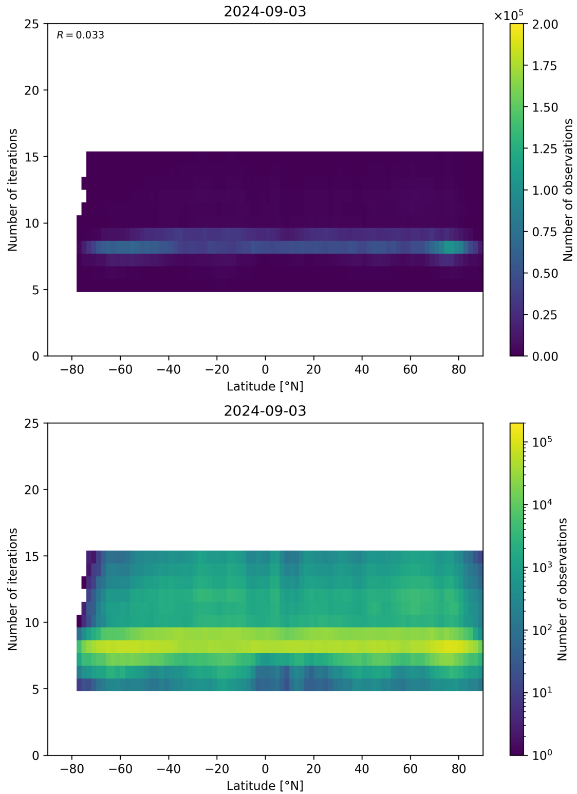
Figure 56: Scatter density plot of “Latitude” against “Number of iterations” for 2024-09-02 to 2024-09-04.
