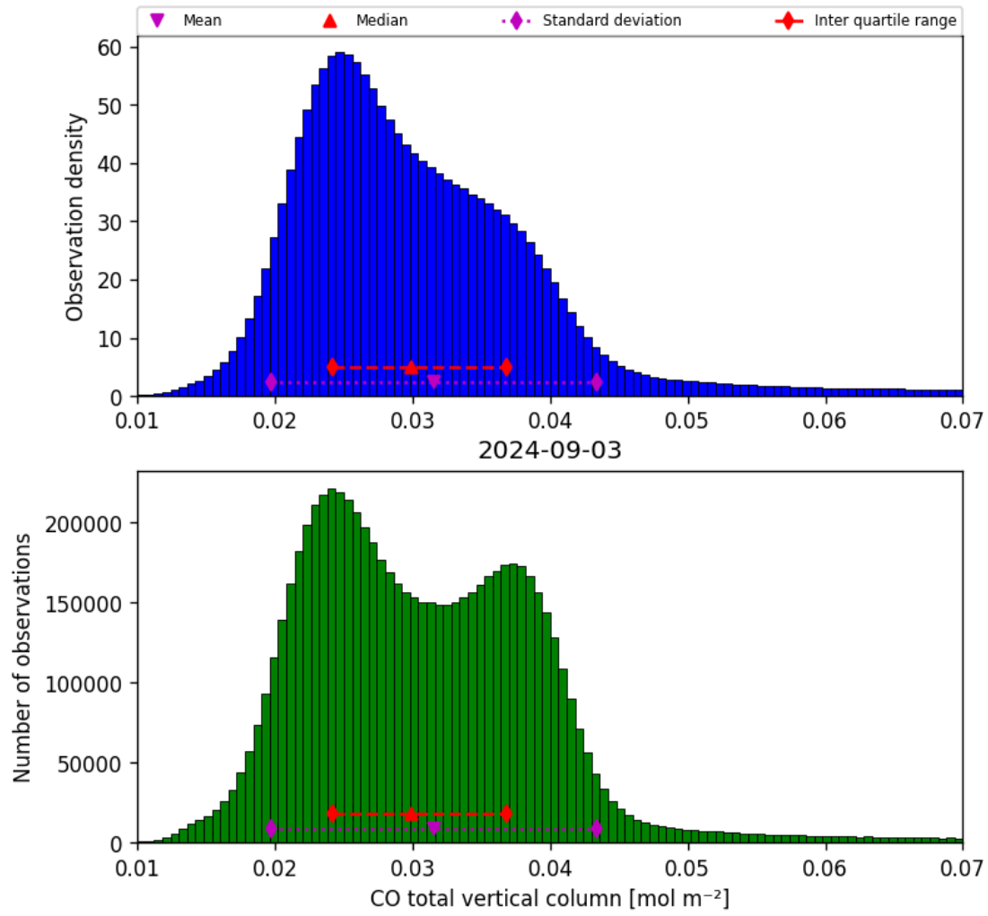
Figure 18: Histogram of “CO total vertical column” for 2024-09-02 to 2024-09-04
