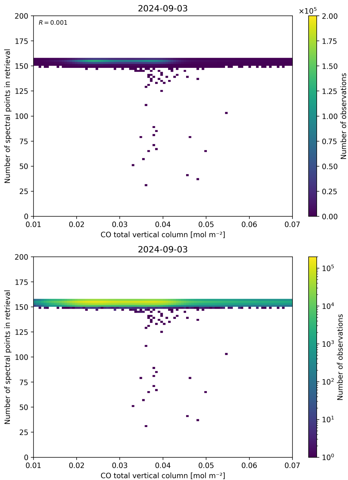
Figure 43: Scatter density plot of “CO total vertical column” against “Number of spectral points in retrieval” for 2024-09-02 to 2024-09-04.
