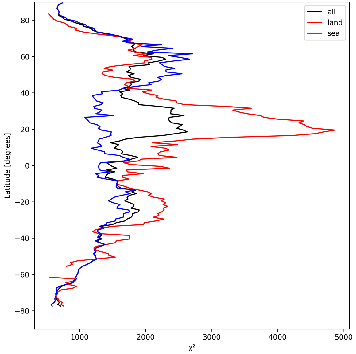
Figure 14: Zonal average of “ \chi^2 ” for 2024-09-02 to 2024-09-04.
