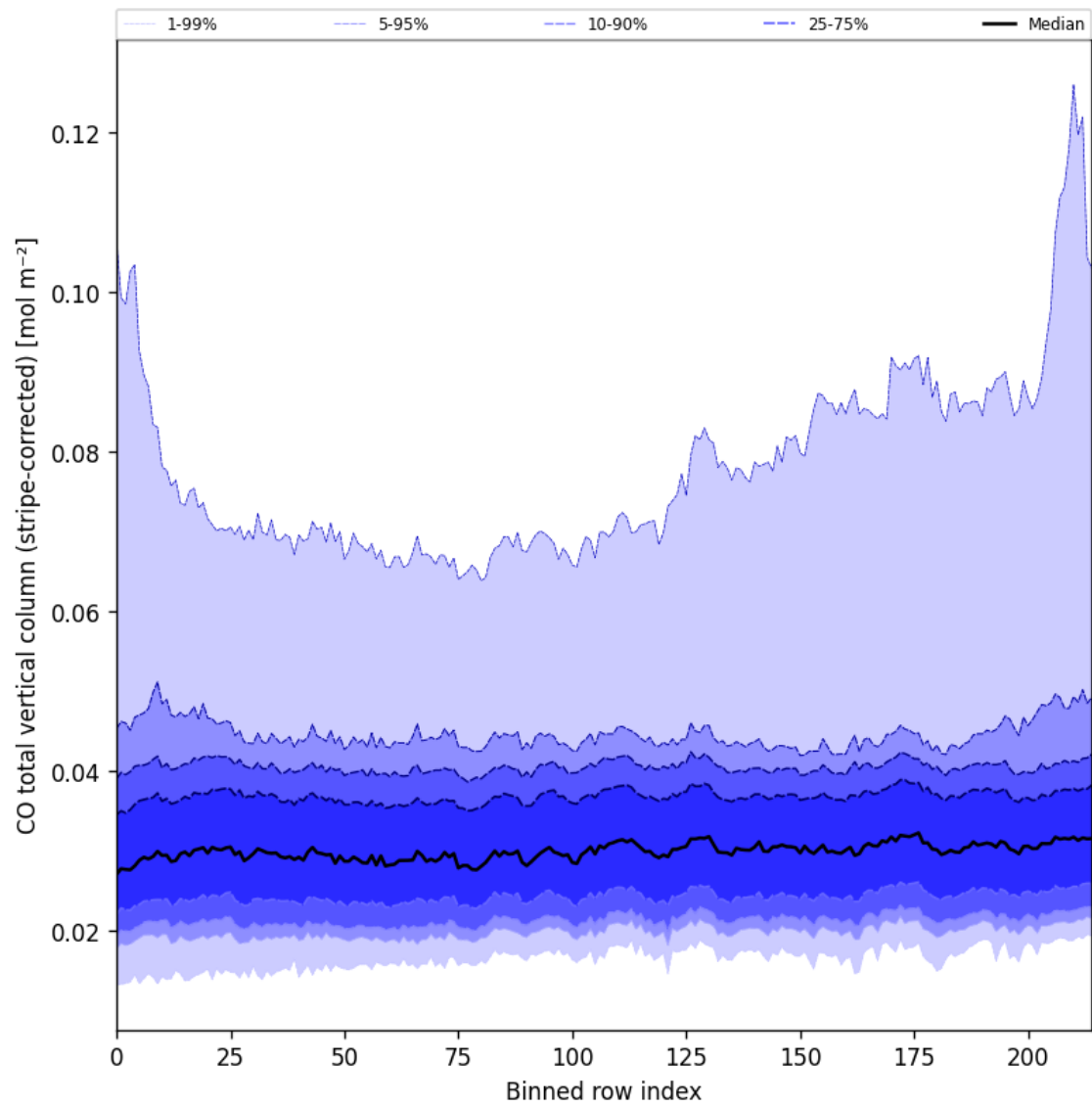
Figure 27: Along track statistics of “CO total vertical column (stripe-corrected)” for 2024-09-02 to 2024-09-04
