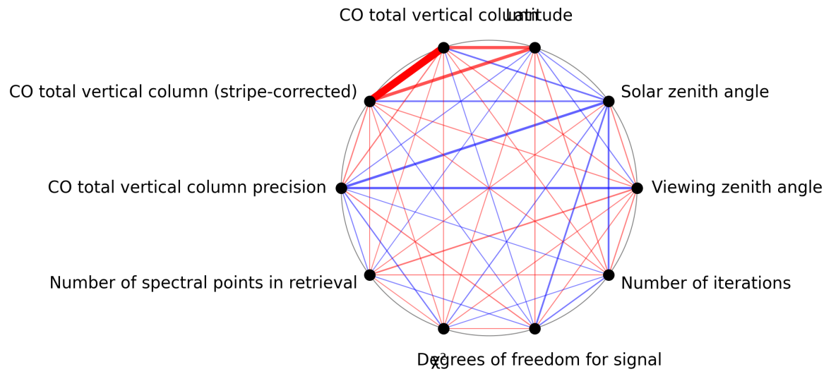
Figure 1: Map of correlation graph for 2024-09-02 to 2024-09-04.
