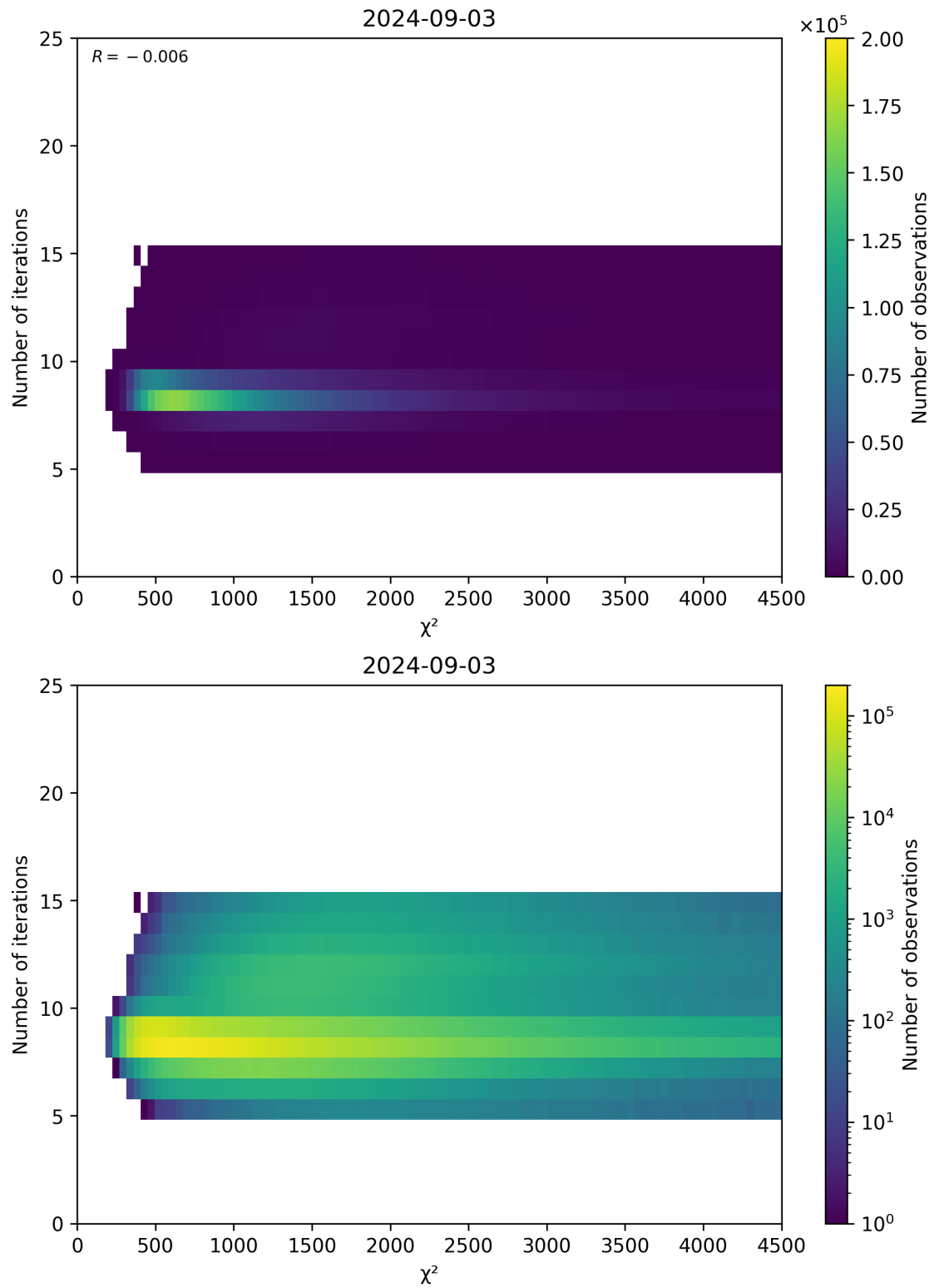
Figure 49: Scatter density plot of “ \chi^2 ” against “Number of iterations” for 2024-09-02 to 2024-09-04.
