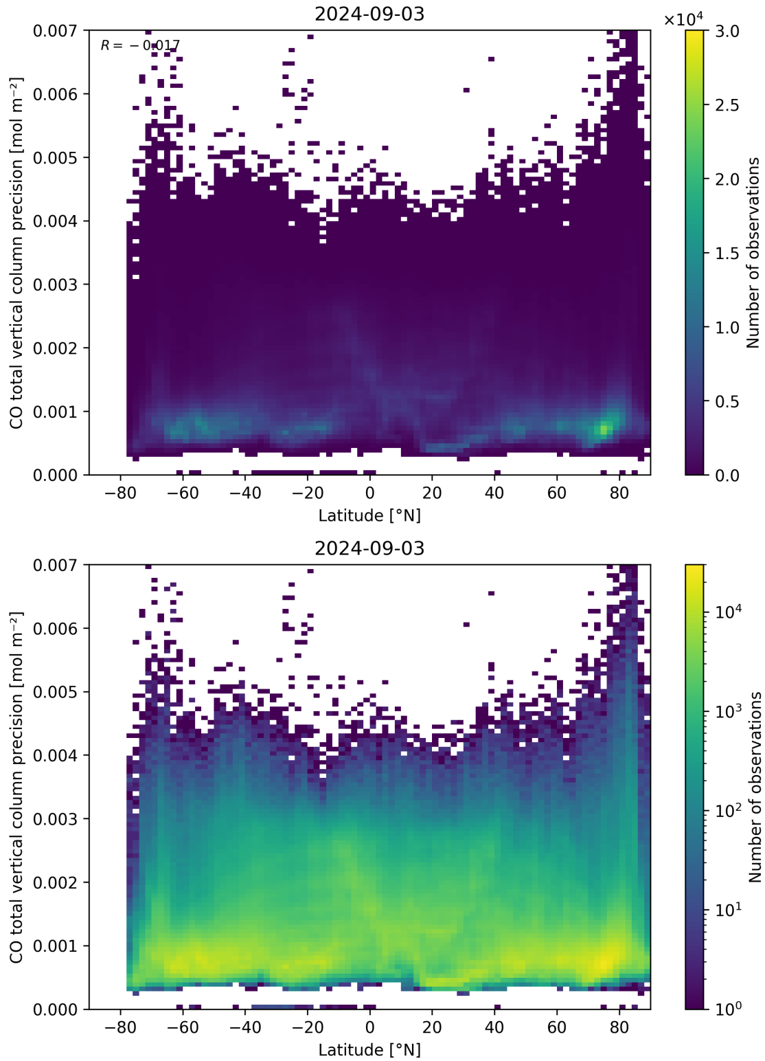
Figure 53: Scatter density plot of “Latitude” against “CO total vertical column precision” for 2024-09-02 to 2024-09-04.
