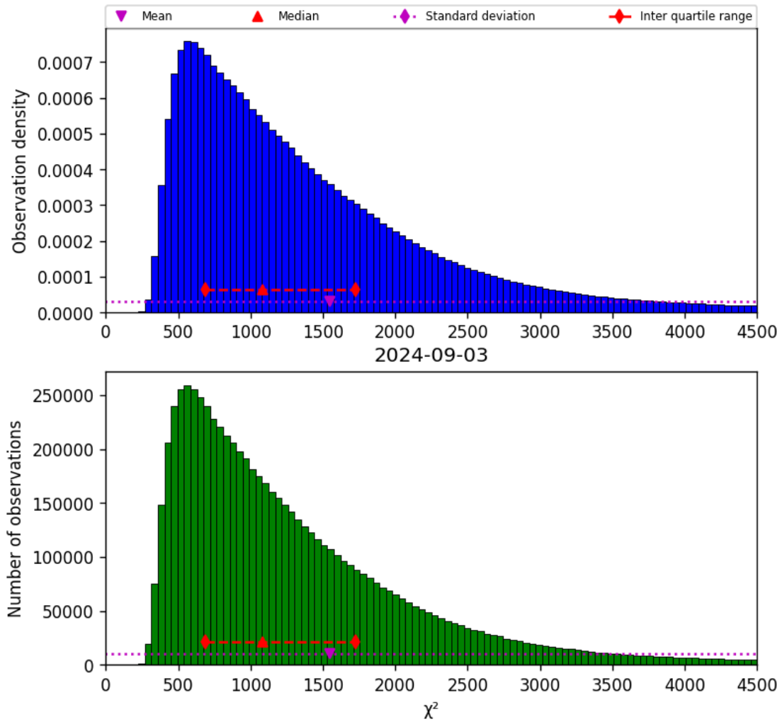
Figure 22: Histogram of “ \chi^2 ” for 2024-09-02 to 2024-09-04
