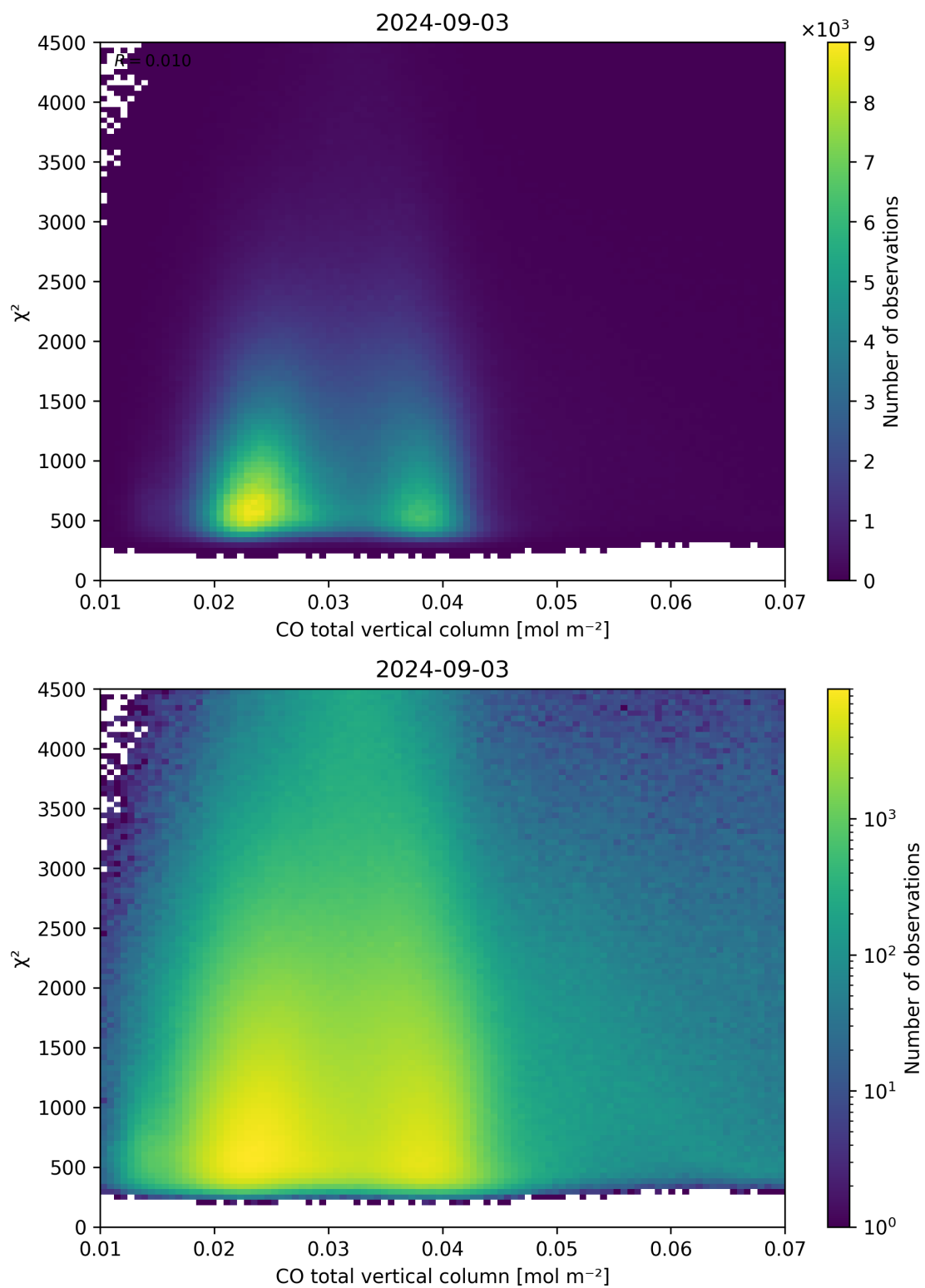
Figure 35: Scatter density plot of “CO total vertical column” against “ \chi^2 ” for 2024-09-02 to 2024-09-04.
