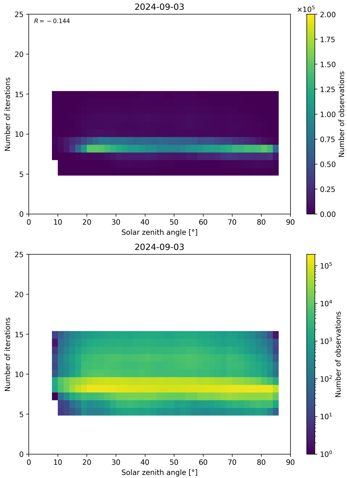
Figure 67: Scatter density plot of “Solar zenith angle” against “Number of iterations” for 2024-09-02 to 2024-09-04.
