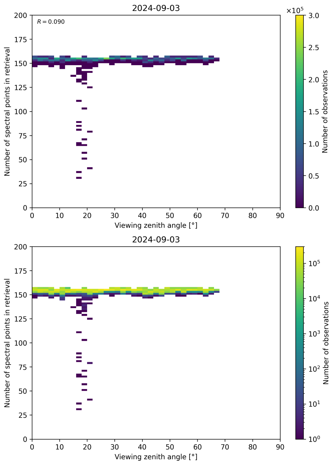
Figure 76: Scatter density plot of “Viewing zenith angle” against “Number of spectral points in retrieval” for 2024-09-02 to 2024-09-04.
