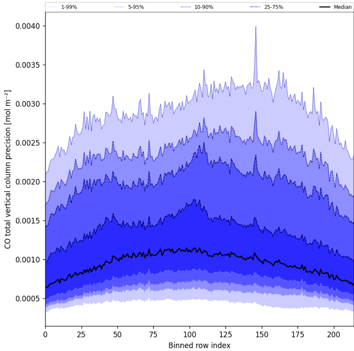
Figure 28: Along track statistics of “CO total vertical column precision” for 2024-09-02 to 2024-09-04
