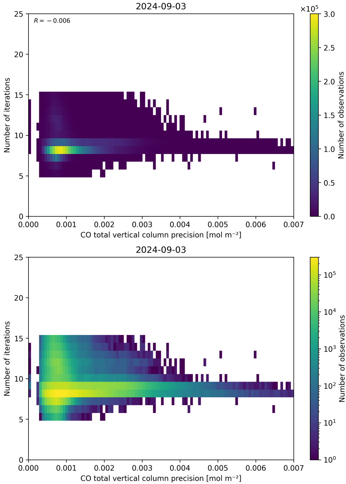
Figure 46: Scatter density plot of “CO total vertical column precision” against “Number of iterations” for 2024-09-02 to 2024-09-04.
