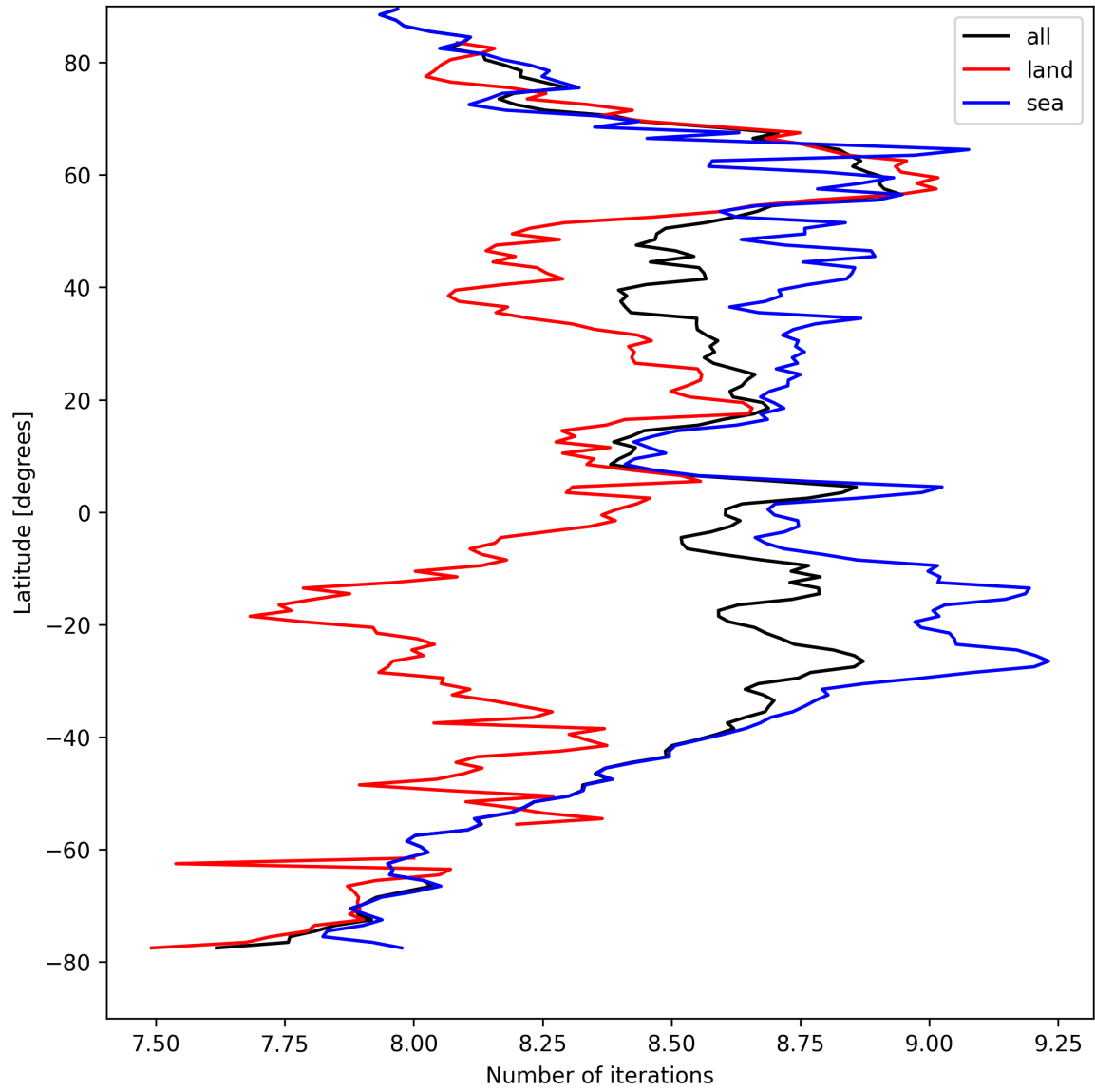
Figure 16: Zonal average of “Number of iterations” for 2024-09-02 to 2024-09-04.
