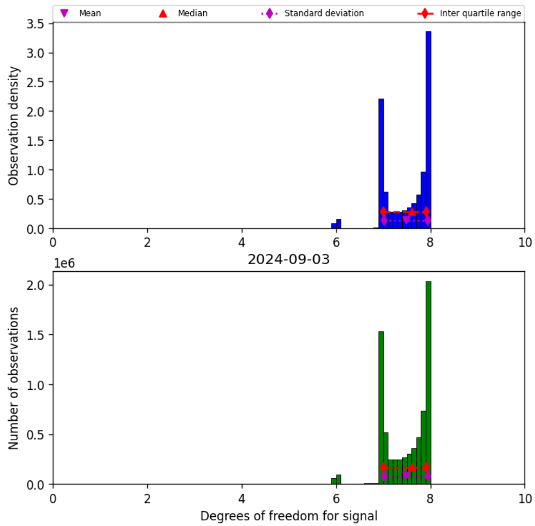
Figure 23: Histogram of “Degrees of freedom for signal” for 2024-09-02 to 2024-09-04
