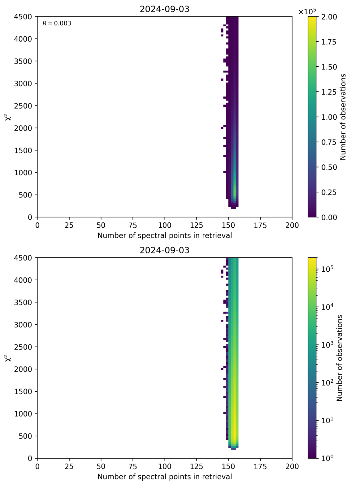
Figure 58: Scatter density plot of “Number of spectral points in retrieval” against “ \chi^2 ” for 2024-09-02 to 2024-09-04.
