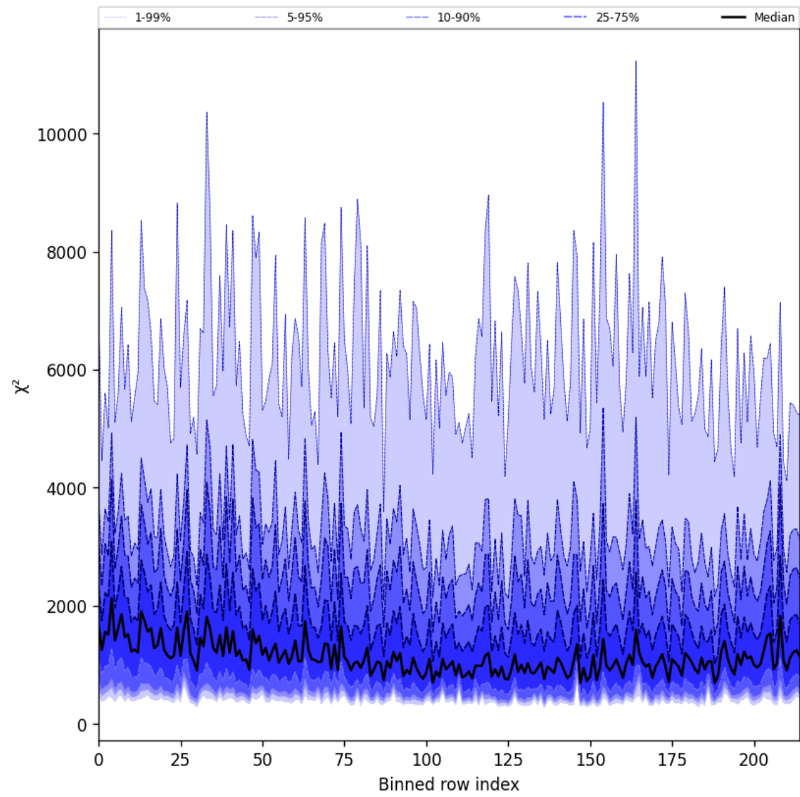
Figure 30: Along track statistics of “ \chi^2 ” for 2024-09-02 to 2024-09-04
