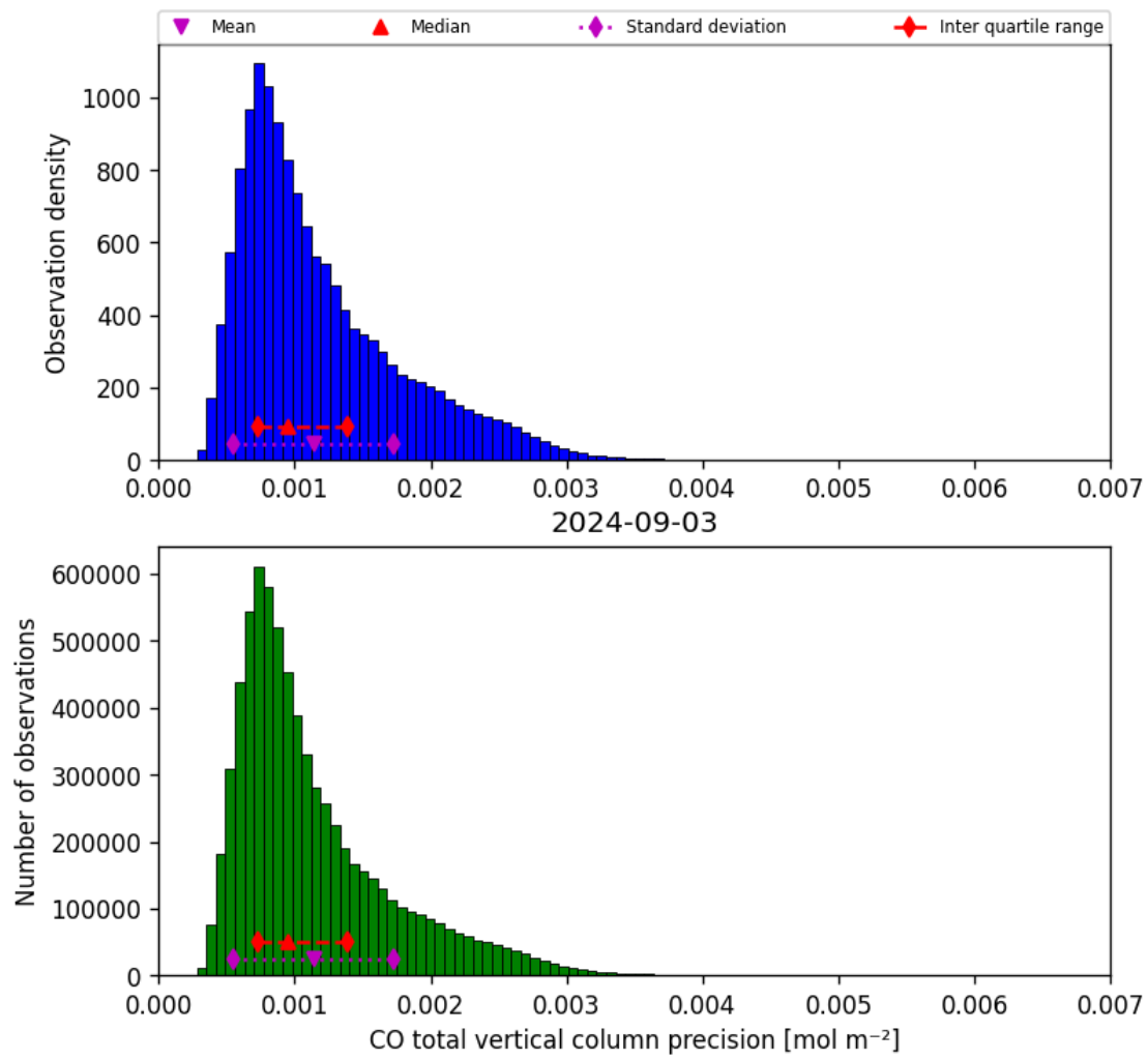
Figure 20: Histogram of “CO total vertical column precision” for 2024-09-02 to 2024-09-04
