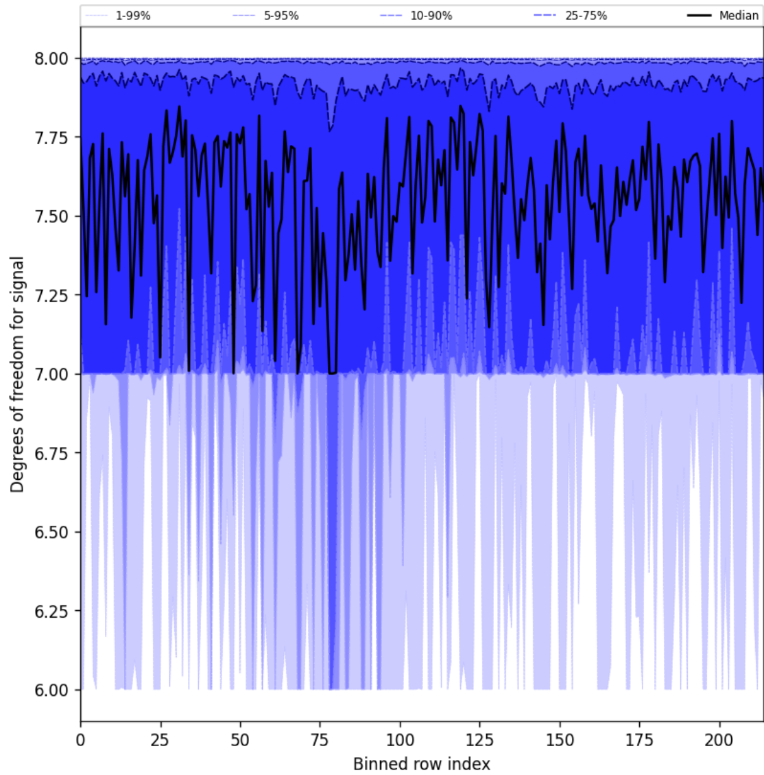
Figure 31: Along track statistics of “Degrees of freedom for signal” for 2024-09-02 to 2024-09-04
