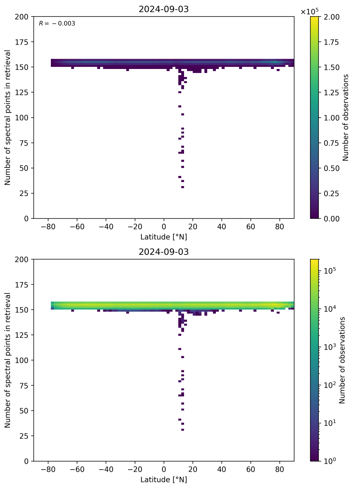
Figure 57: Scatter density plot of “Latitude” against “Number of spectral points in retrieval” for 2024-09-02 to 2024-09-04.
