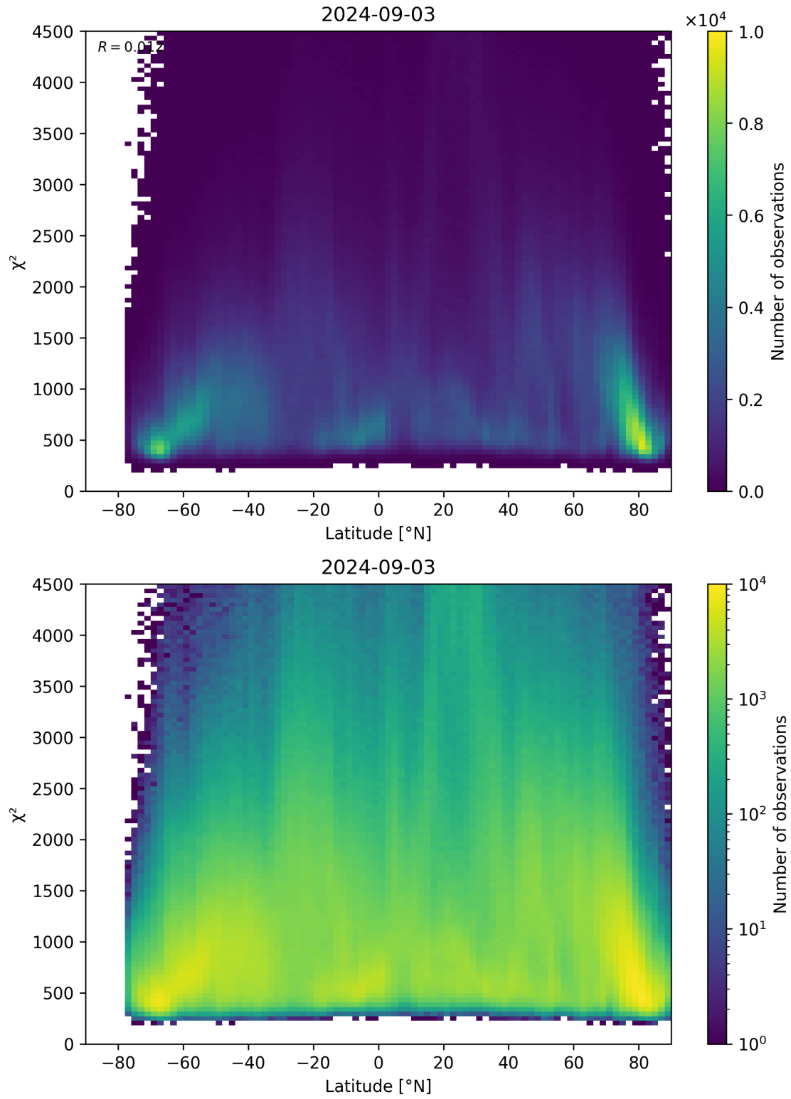
Figure 54: Scatter density plot of “Latitude” against “ \chi^2 ” for 2024-09-02 to 2024-09-04.
