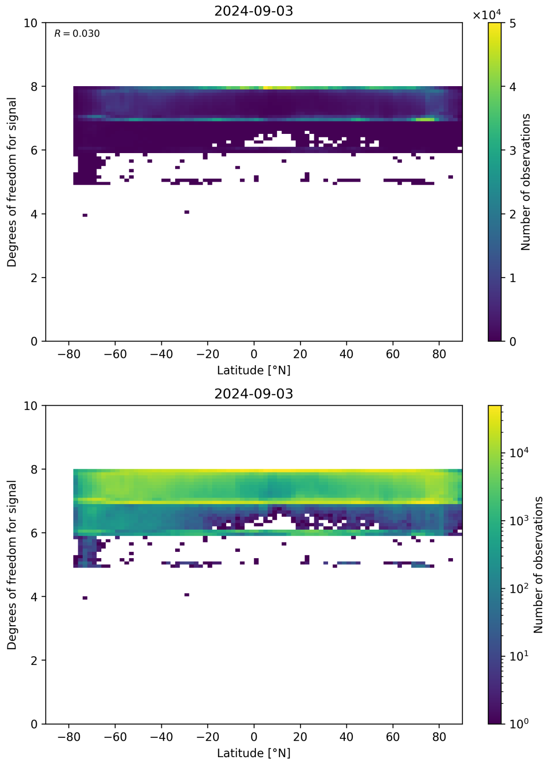
Figure 55: Scatter density plot of “Latitude” against “Degrees of freedom for signal” for 2024-09-02 to 2024-09-04.
