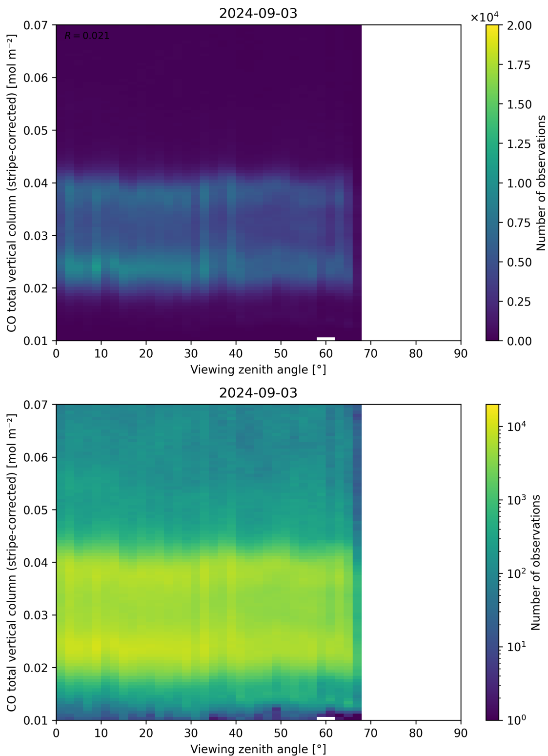
Figure 70: Scatter density plot of “Viewing zenith angle” against “CO total vertical column (stripe-corrected)” for 2024-09-02 to 2024-09-04.
