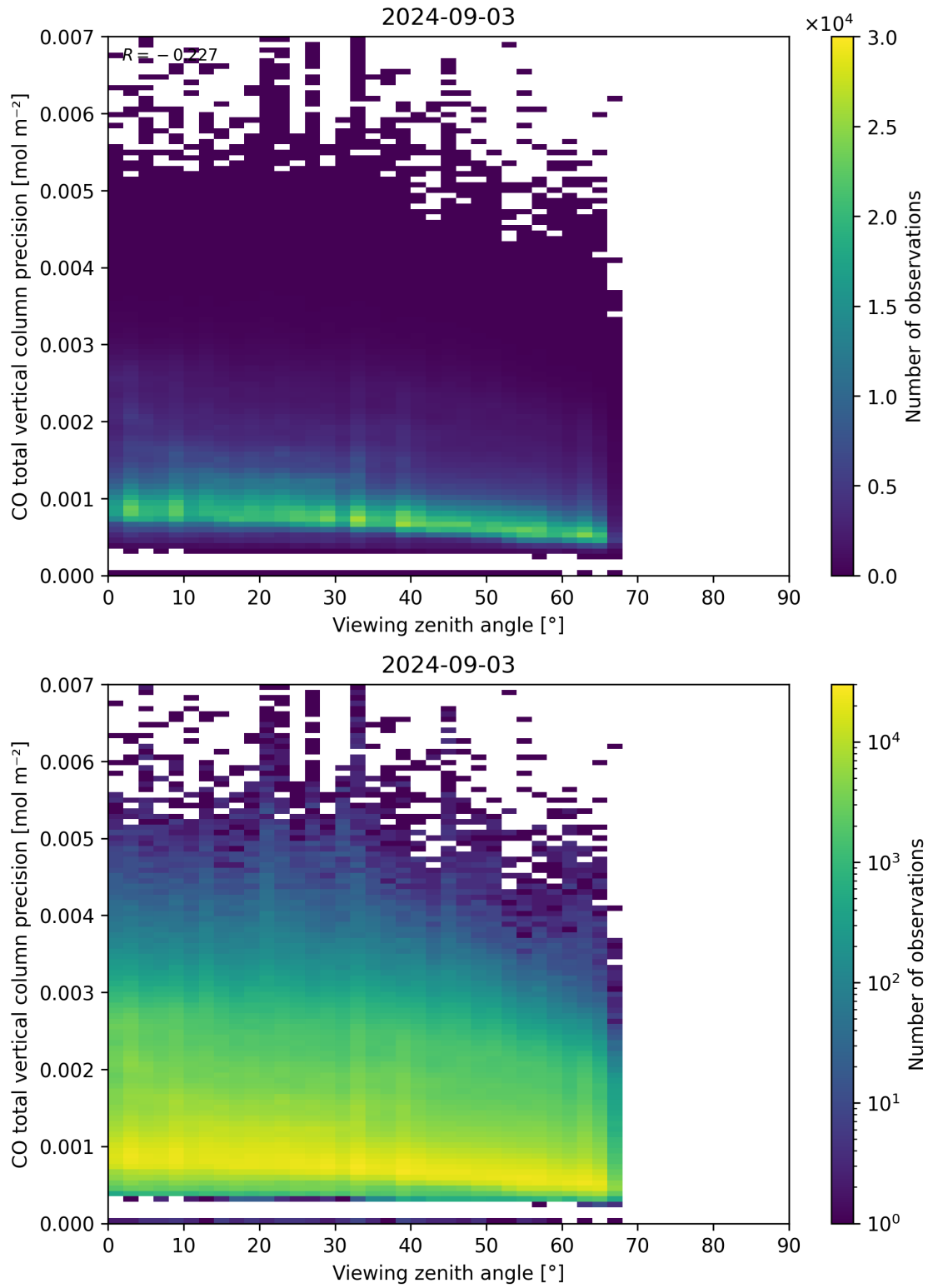
Figure 71: Scatter density plot of “Viewing zenith angle” against “CO total vertical column precision” for 2024-09-02 to 2024-09-04.
