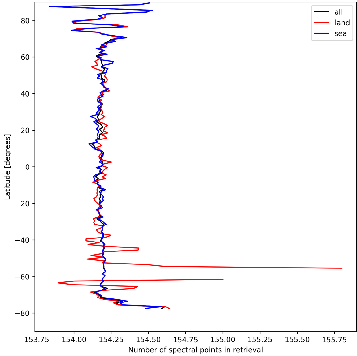
Figure 13: Zonal average of “Number of spectral points in retrieval” for 2024-09-02 to 2024-09-04.
