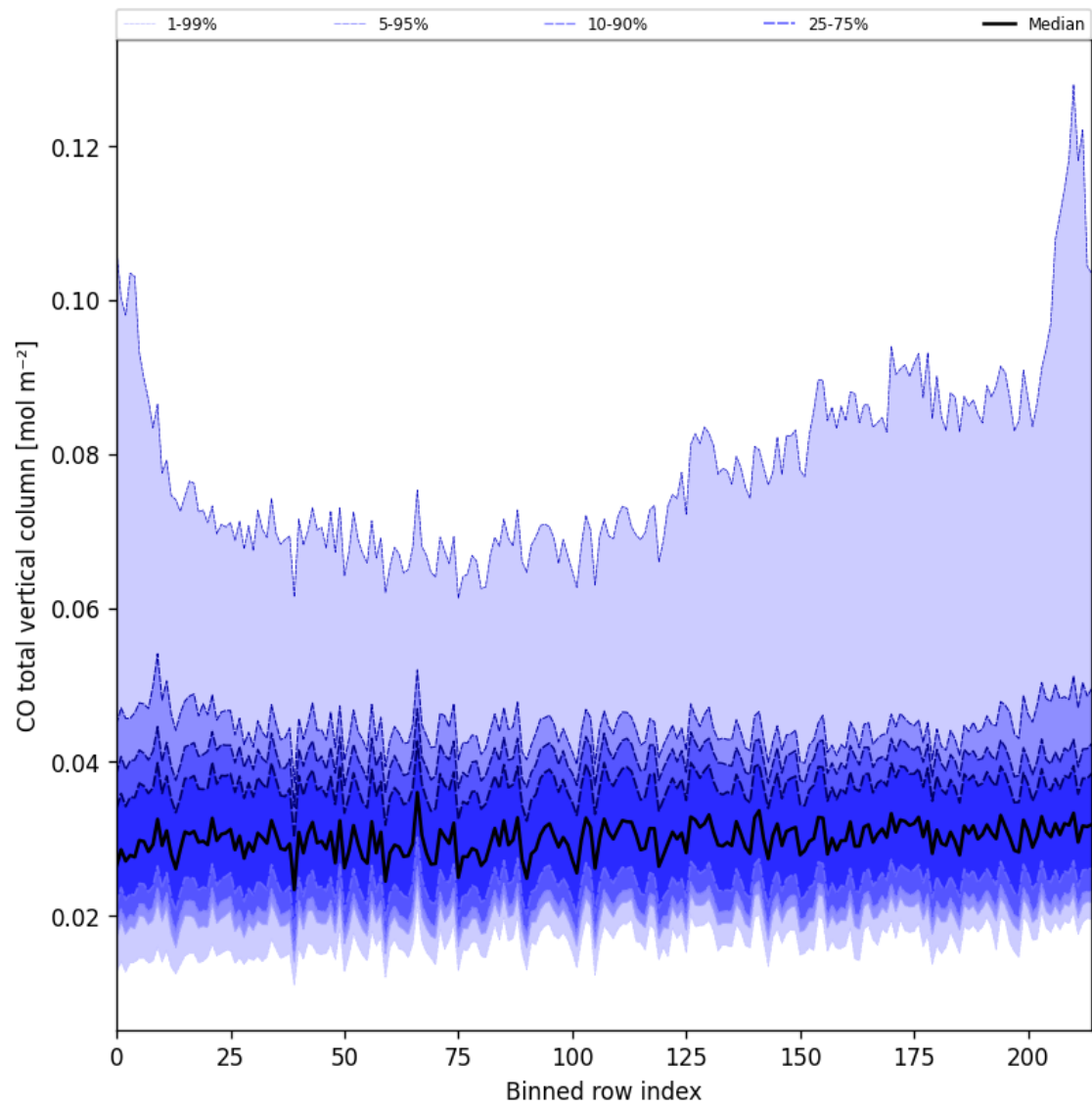
Figure 26: Along track statistics of “CO total vertical column” for 2024-09-02 to 2024-09-04
