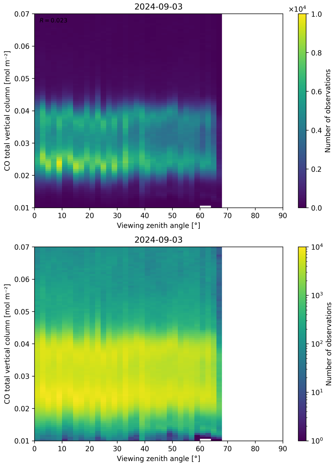
Figure 69: Scatter density plot of “Viewing zenith angle” against “CO total vertical column” for 2024-09-02 to 2024-09-04.
