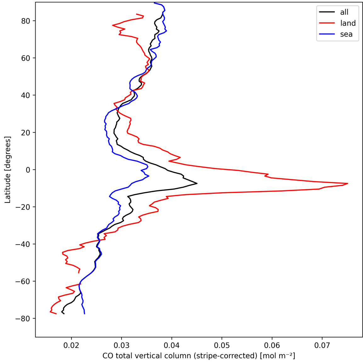
Figure 11: Zonal average of “CO total vertical column (stripe-corrected)” for 2024-09-02 to 2024-09-04.
