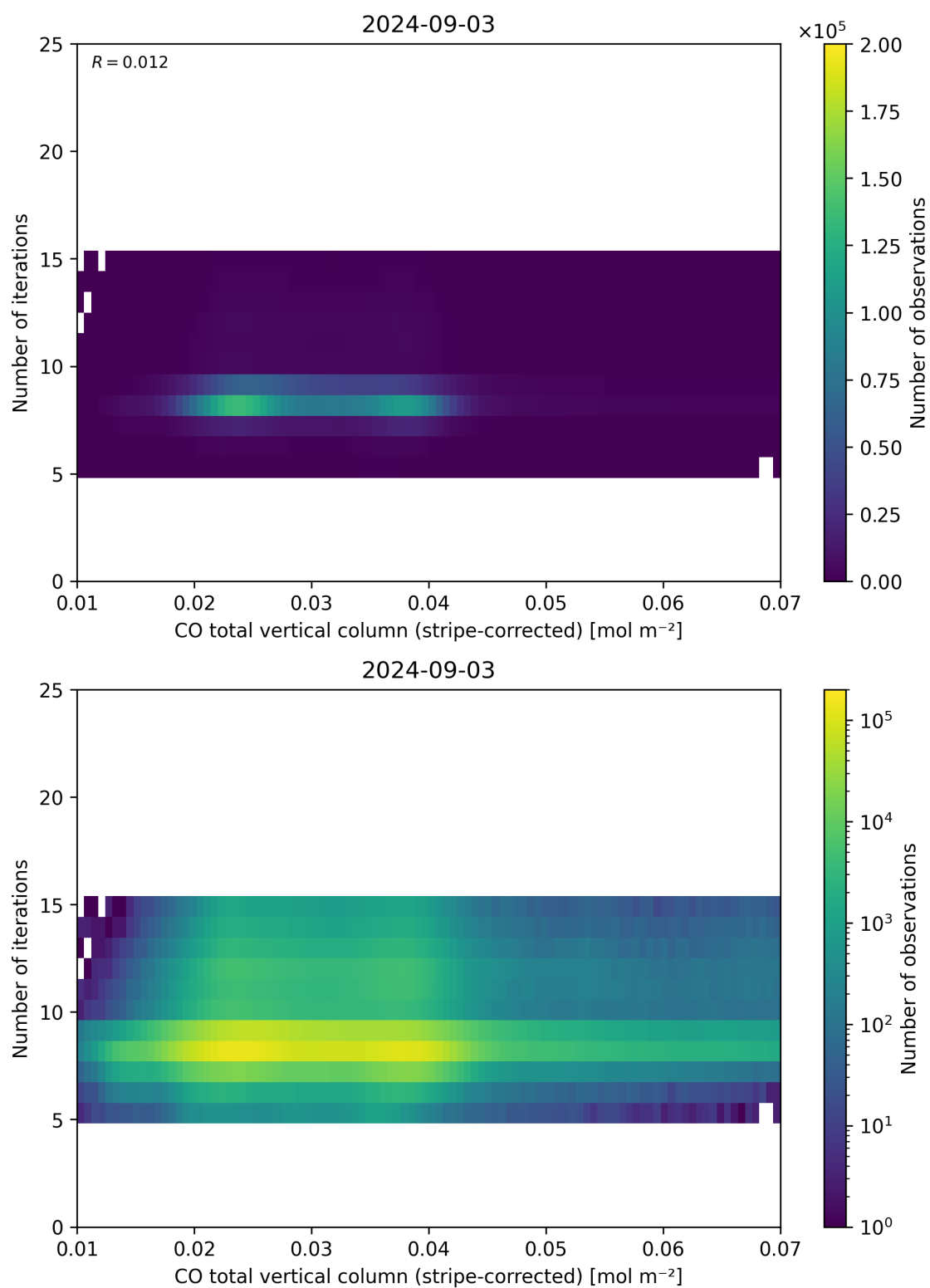
Figure 39: Scatter density plot of “CO total vertical column (stripe-corrected)” against “Number of iterations” for 2024-09-02 to 2024-09-04.
