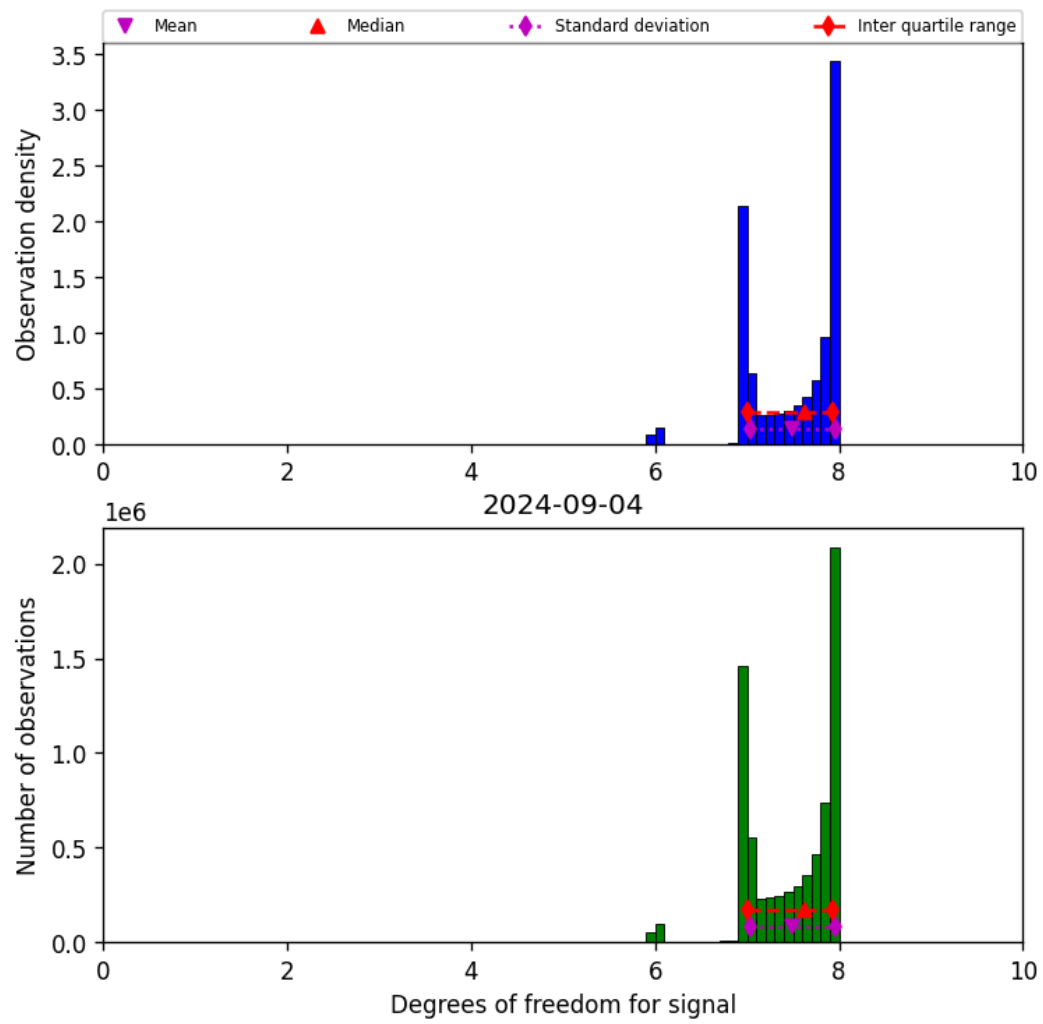
Figure 23: Histogram of “Degrees of freedom for signal” for 2024-09-03 to 2024-09-05
