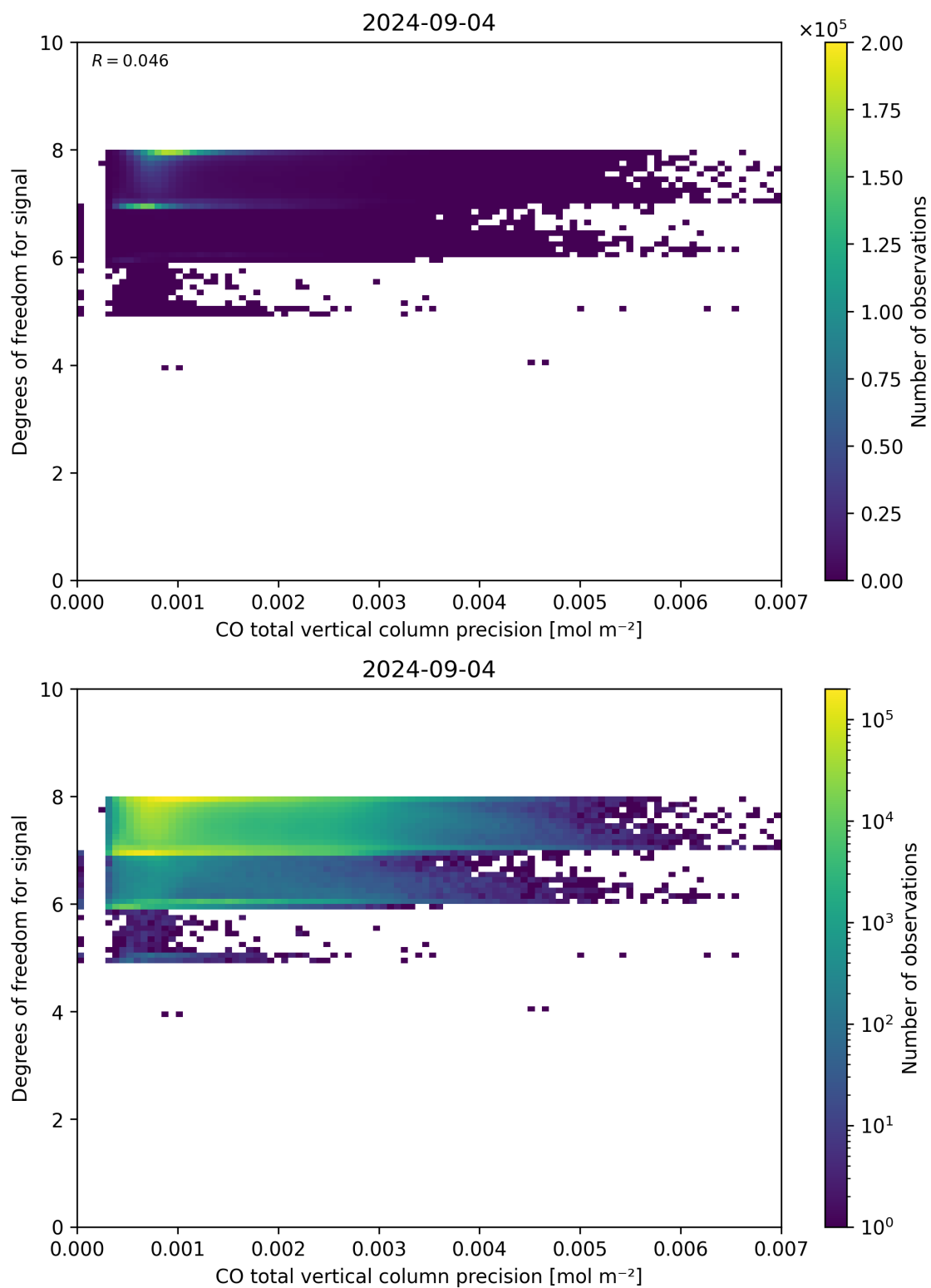
Figure 45: Scatter density plot of “CO total vertical column precision” against “Degrees of freedom for signal” for 2024-09-03 to 2024-09-05.
