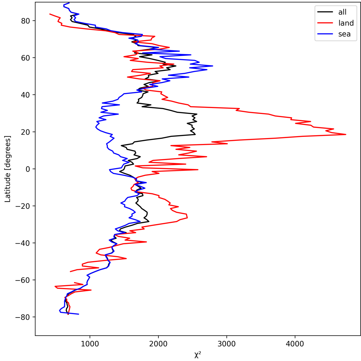
Figure 14: Zonal average of “ \chi^2 ” for 2024-09-03 to 2024-09-05.
