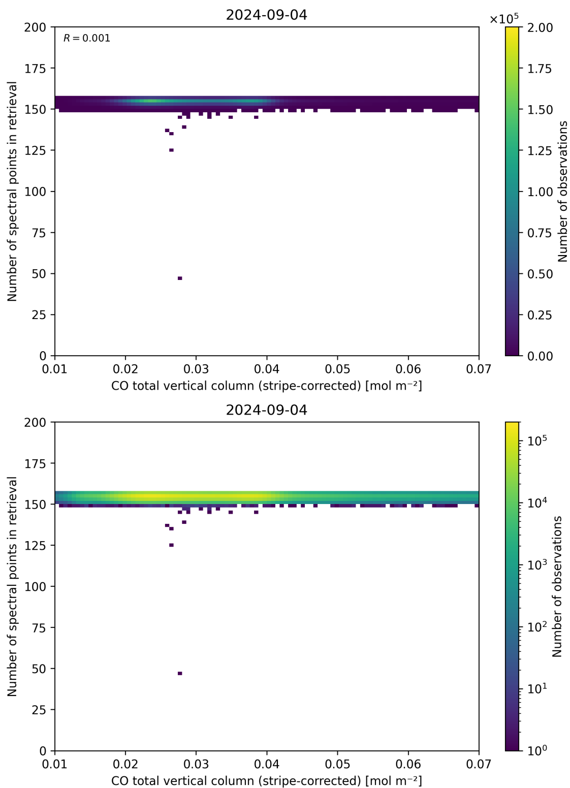
Figure 40: Scatter density plot of “CO total vertical column (stripe-corrected)” against “Number of spectral points in retrieval” for 2024-09-03 to 2024-09-05.
