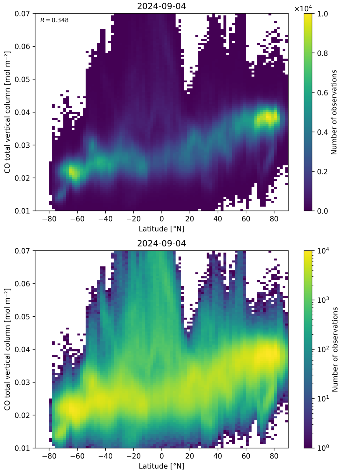
Figure 51: Scatter density plot of “Latitude” against “CO total vertical column” for 2024-09-03 to 2024-09-05.
