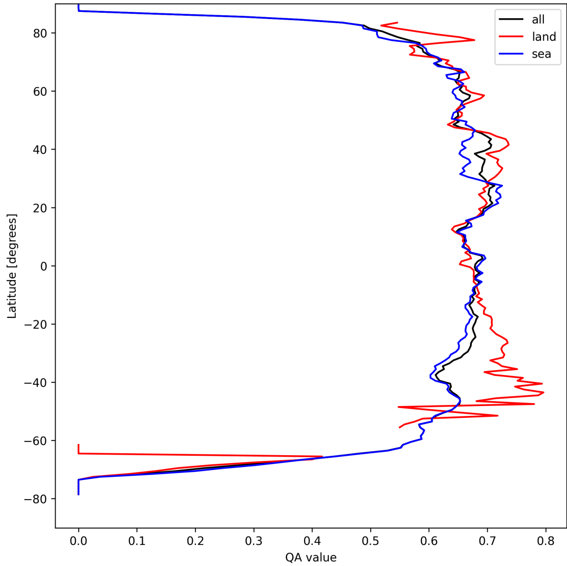
Figure 9: Zonal average of “QA value” for 2024-09-03 to 2024-09-05.
