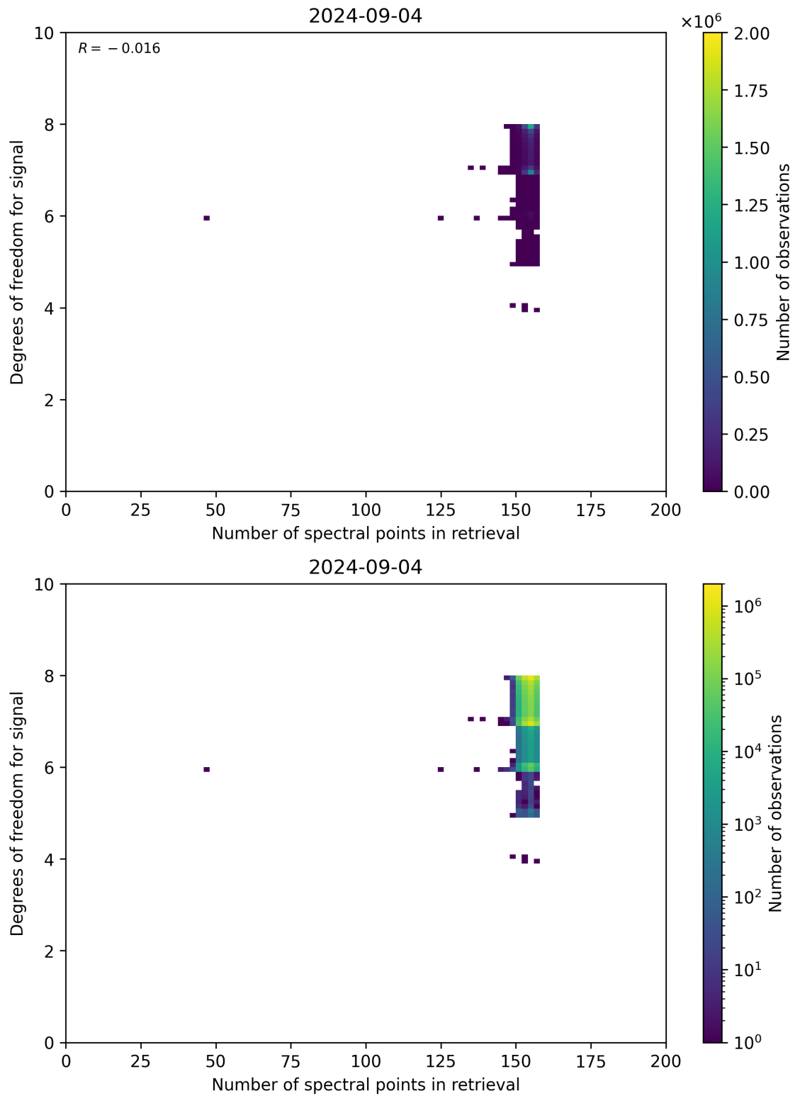
Figure 59: Scatter density plot of “Number of spectral points in retrieval” against “Degrees of freedom for signal” for 2024-09-03 to 2024-09-05.
