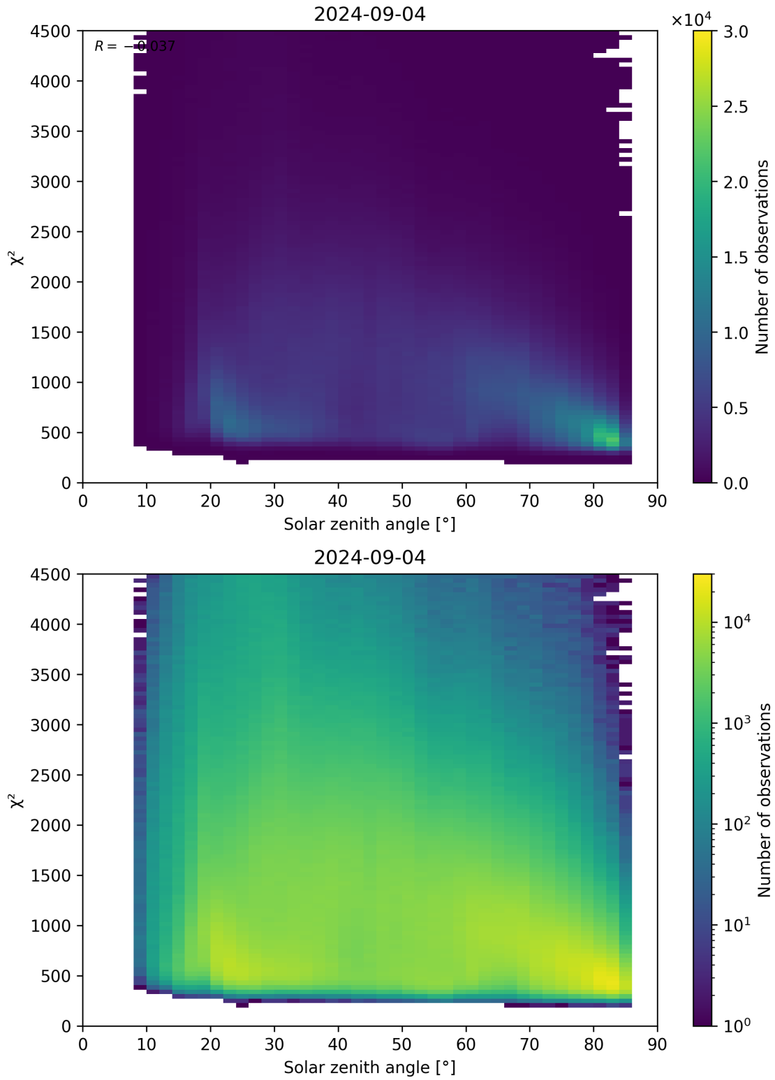
Figure 64: Scatter density plot of “Solar zenith angle” against “ \chi^2 ” for 2024-09-03 to 2024-09-05.
