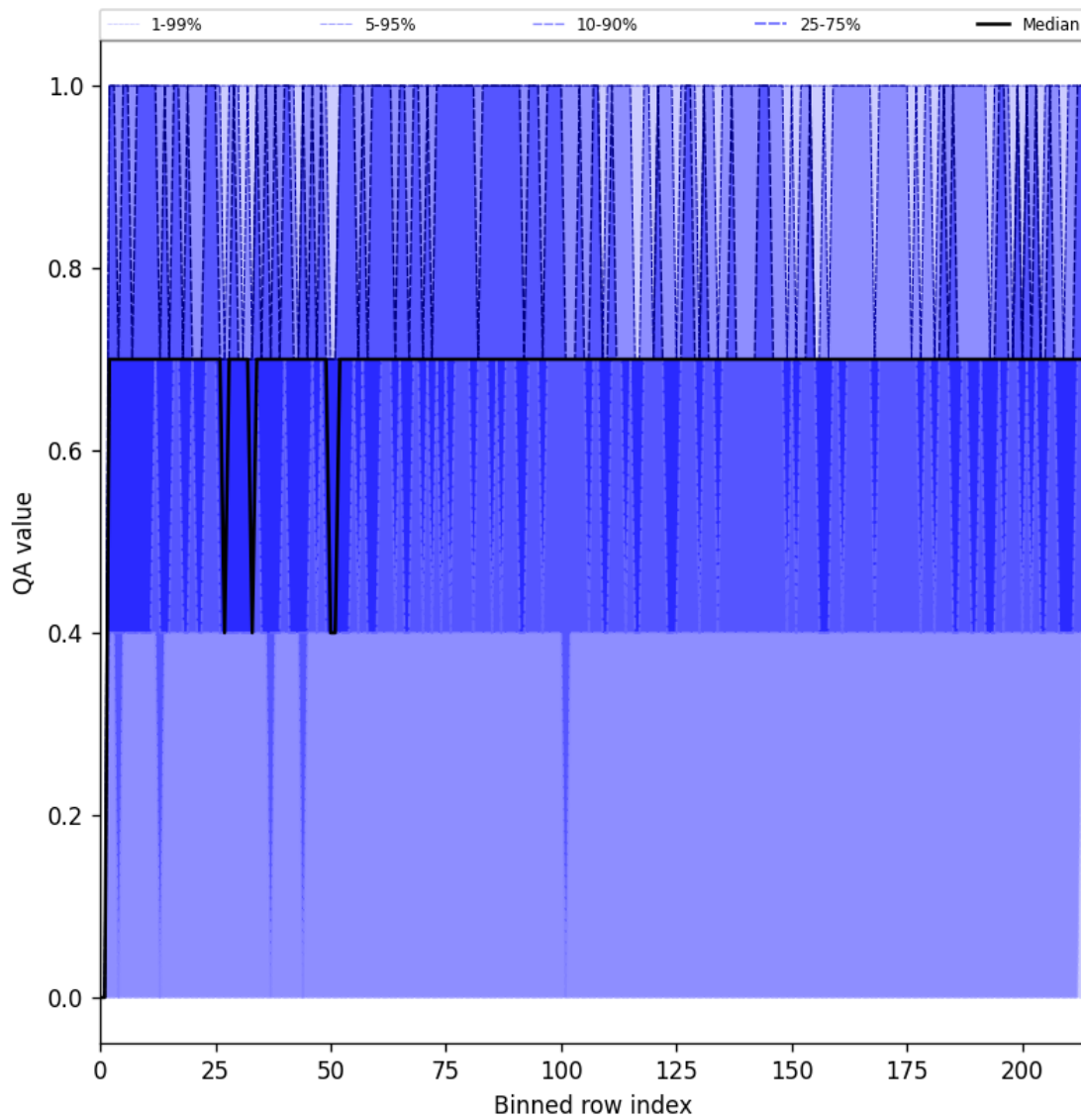
Figure 25: Along track statistics of “QA value” for 2024-09-03 to 2024-09-05
