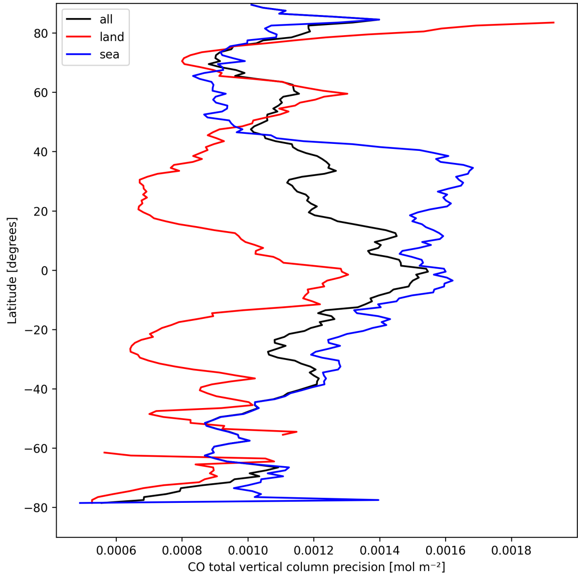
Figure 12: Zonal average of “CO total vertical column precision” for 2024-09-03 to 2024-09-05.
