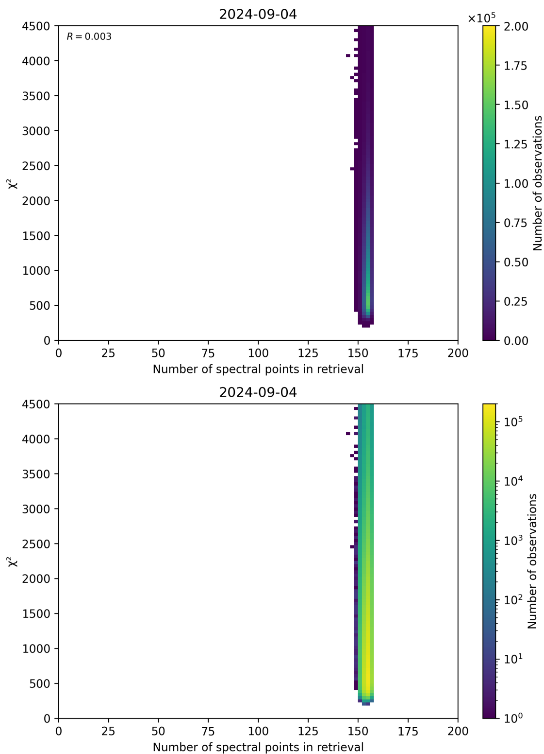
Figure 58: Scatter density plot of “Number of spectral points in retrieval” against “ \chi^2 ” for 2024-09-03 to 2024-09-05.
