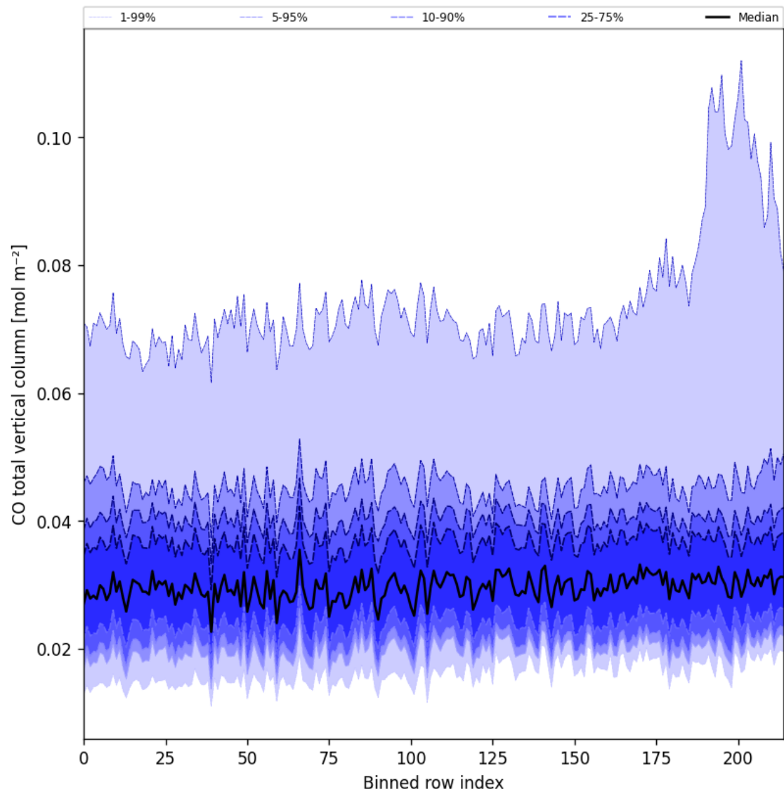
Figure 26: Along track statistics of “CO total vertical column” for 2024-09-03 to 2024-09-05
