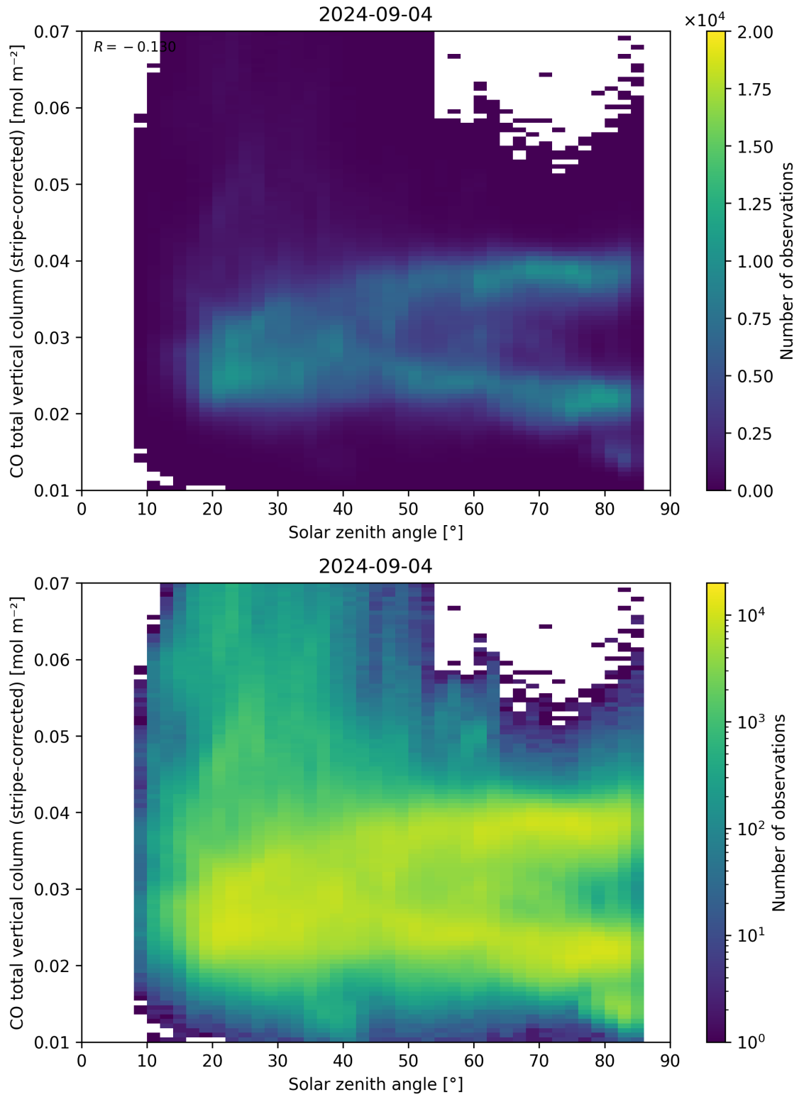
Figure 62: Scatter density plot of “Solar zenith angle” against “CO total vertical column (stripe-corrected)” for 2024-09-03 to 2024-09-05.
