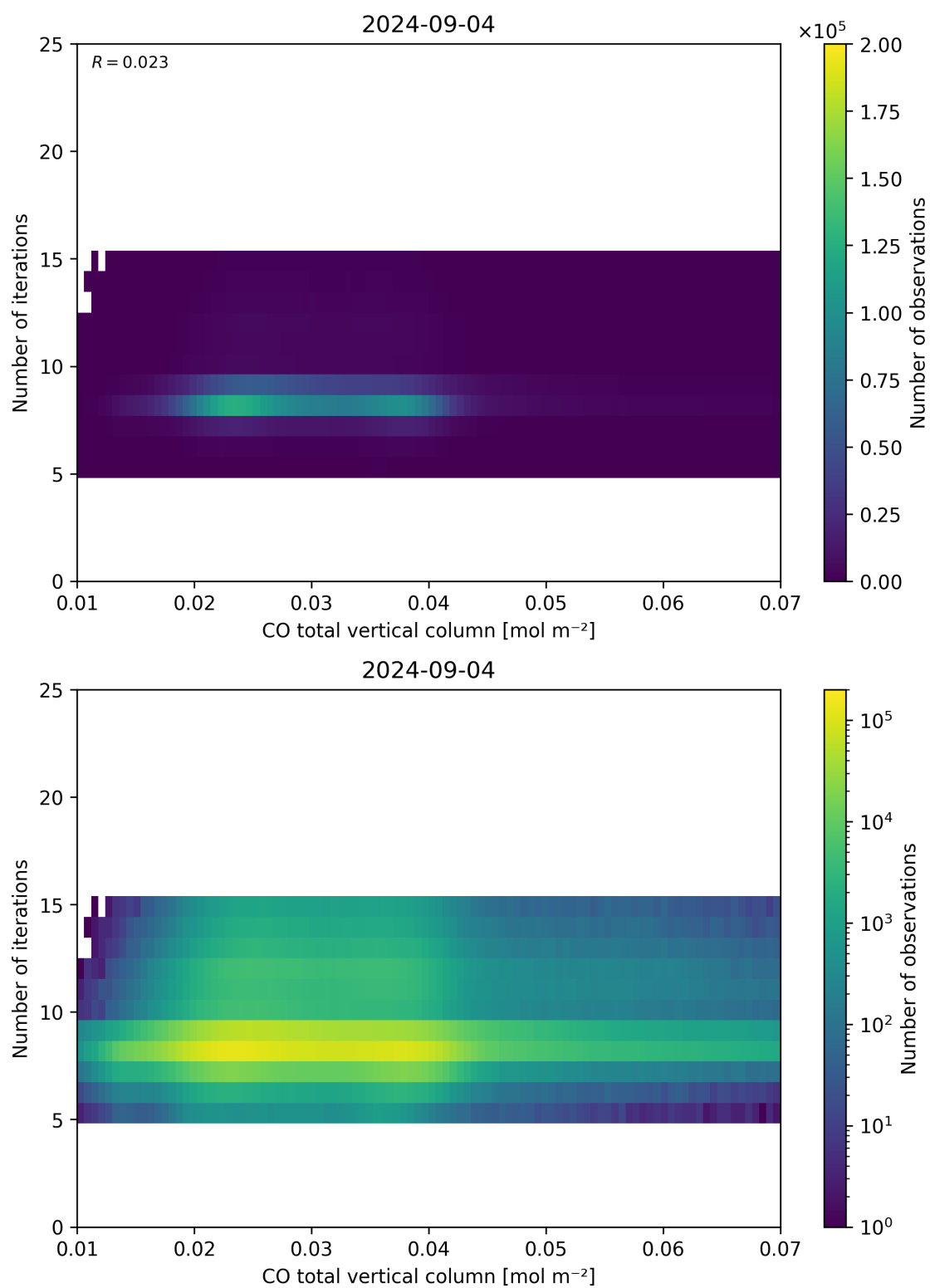
Figure 42: Scatter density plot of “CO total vertical column” against “Number of iterations” for 2024-09-03 to 2024-09-05.
