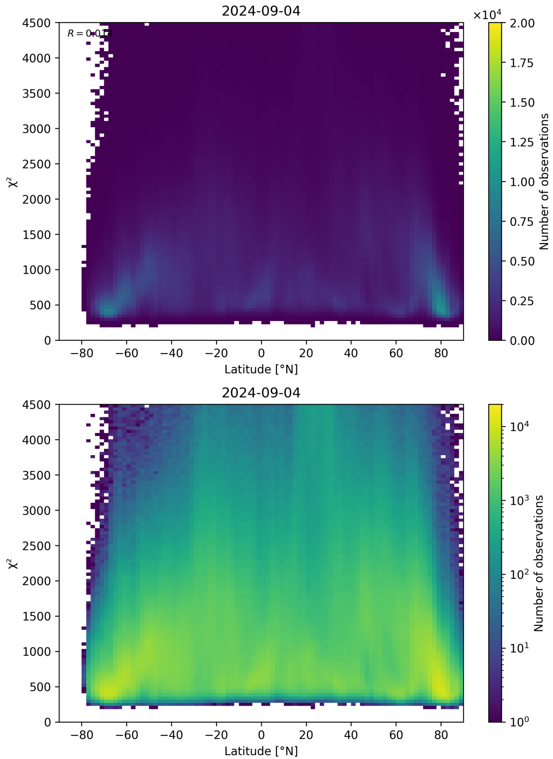
Figure 54: Scatter density plot of “Latitude” against “ \chi^2 ” for 2024-09-03 to 2024-09-05.
