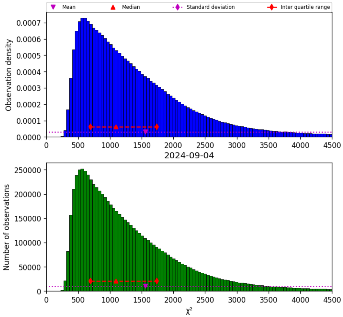
Figure 22: Histogram of " \chi^2 " for 2024-09-03 to 2024-09-05
