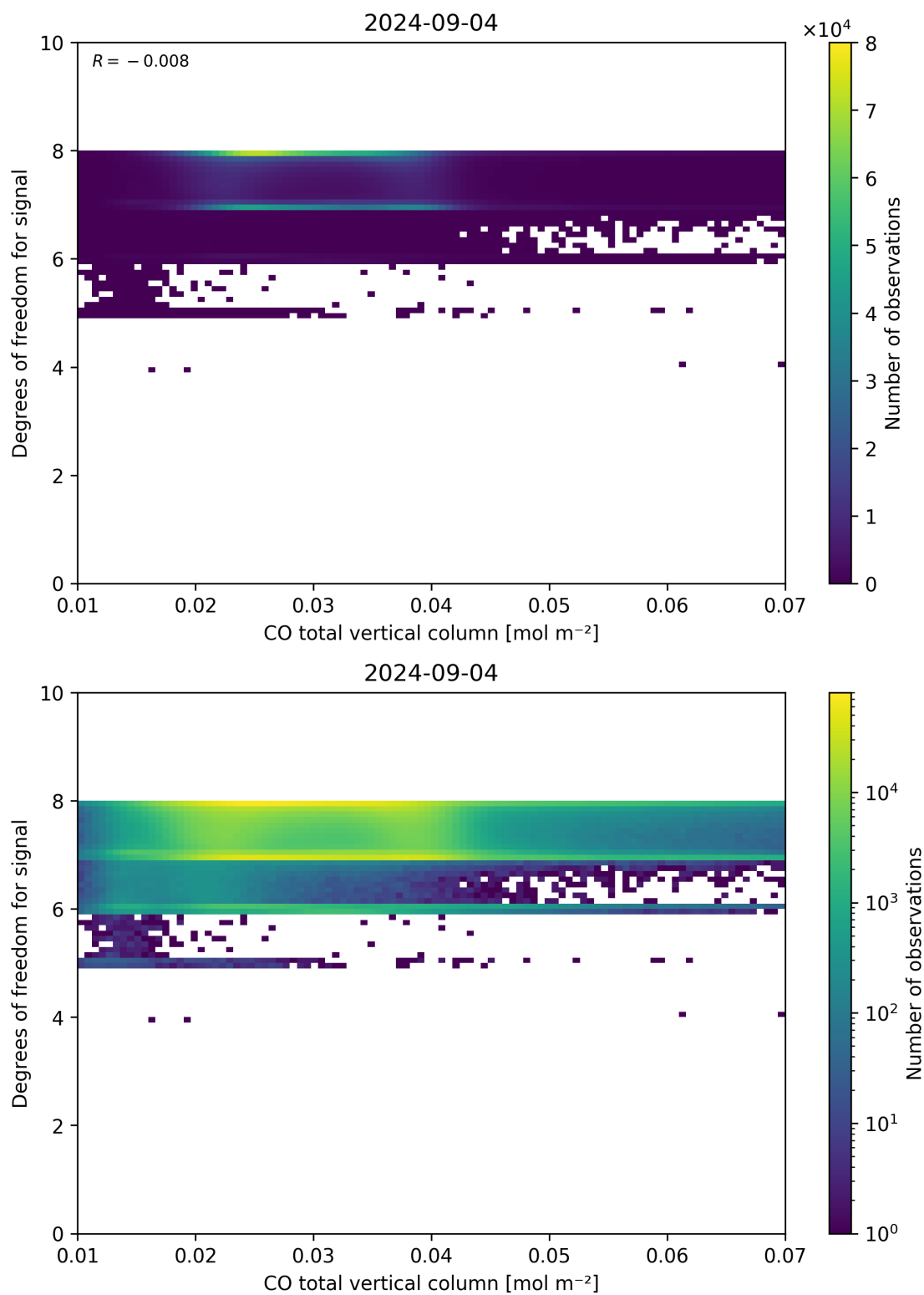
Figure 41: Scatter density plot of “CO total vertical column” against “Degrees of freedom for signal” for 2024-09-03 to 2024-09-05.
