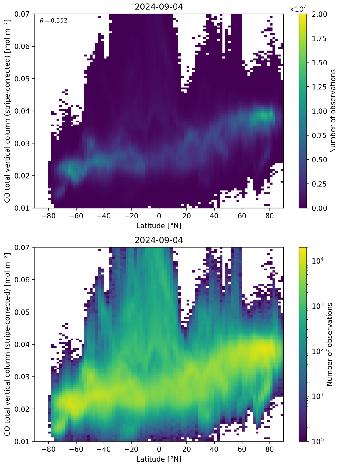
Figure 52: Scatter density plot of “Latitude” against “CO total vertical column (stripe-corrected)” for 2024-09-03 to 2024-09-05.
