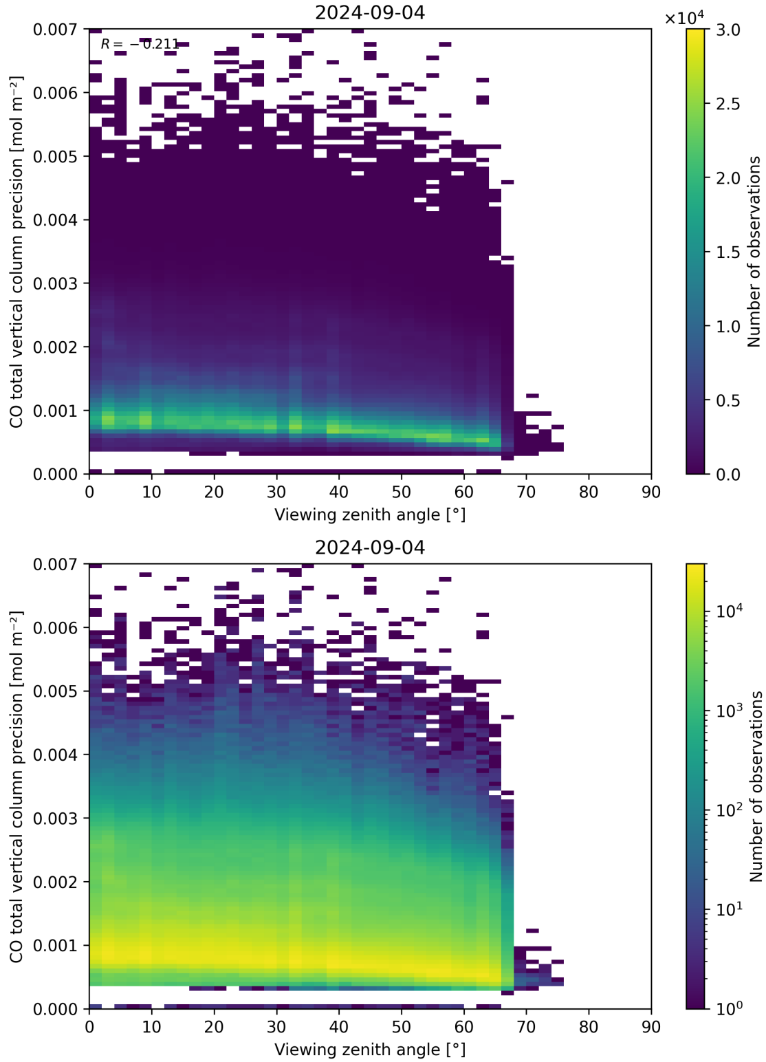
Figure 71: Scatter density plot of “Viewing zenith angle” against “CO total vertical column precision” for 2024-09-03 to 2024-09-05.
