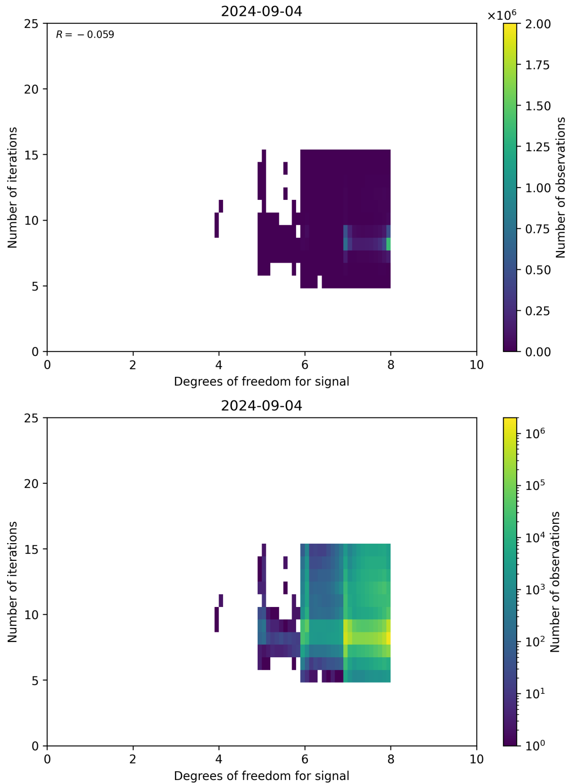
Figure 50: Scatter density plot of “Degrees of freedom for signal” against “Number of iterations” for 2024-09-03 to 2024-09-05.
