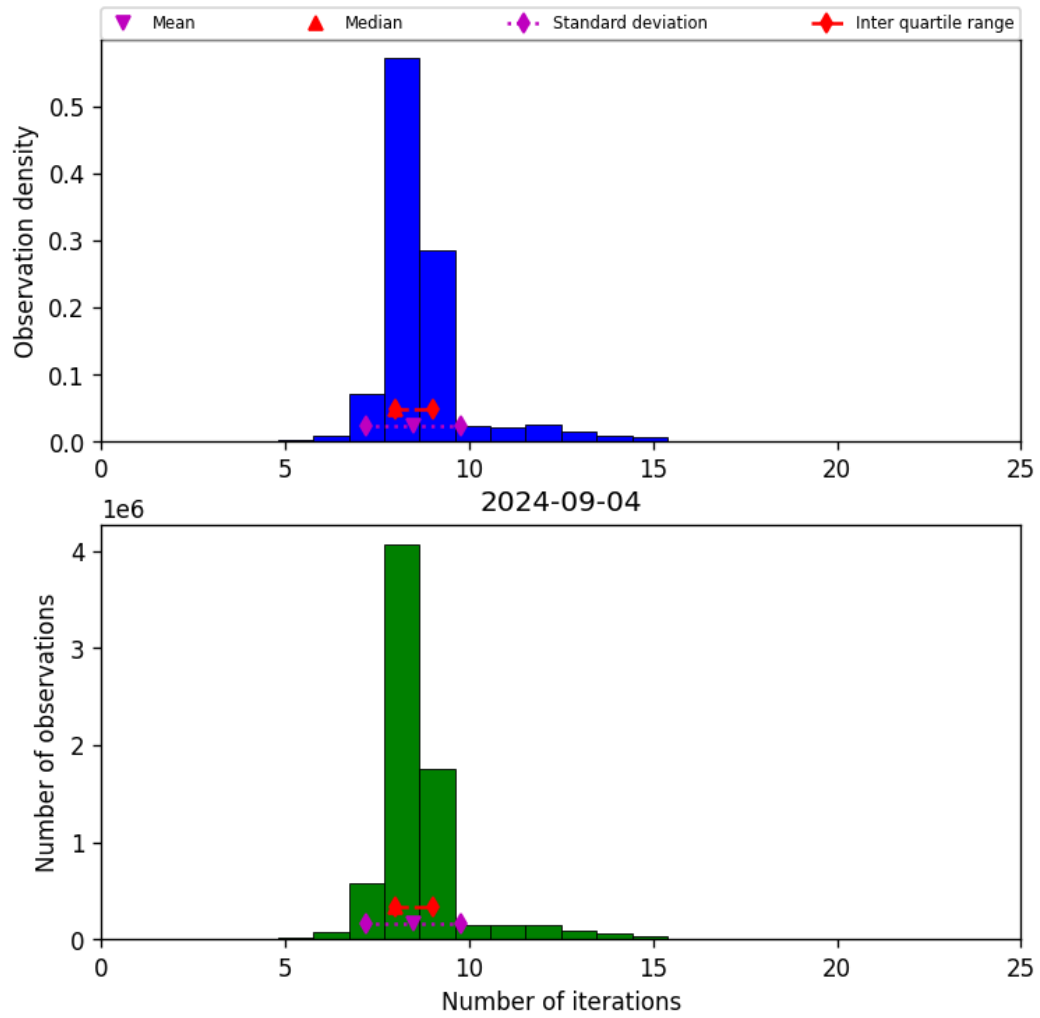
Figure 24: Histogram of “Number of iterations” for 2024-09-03 to 2024-09-05
