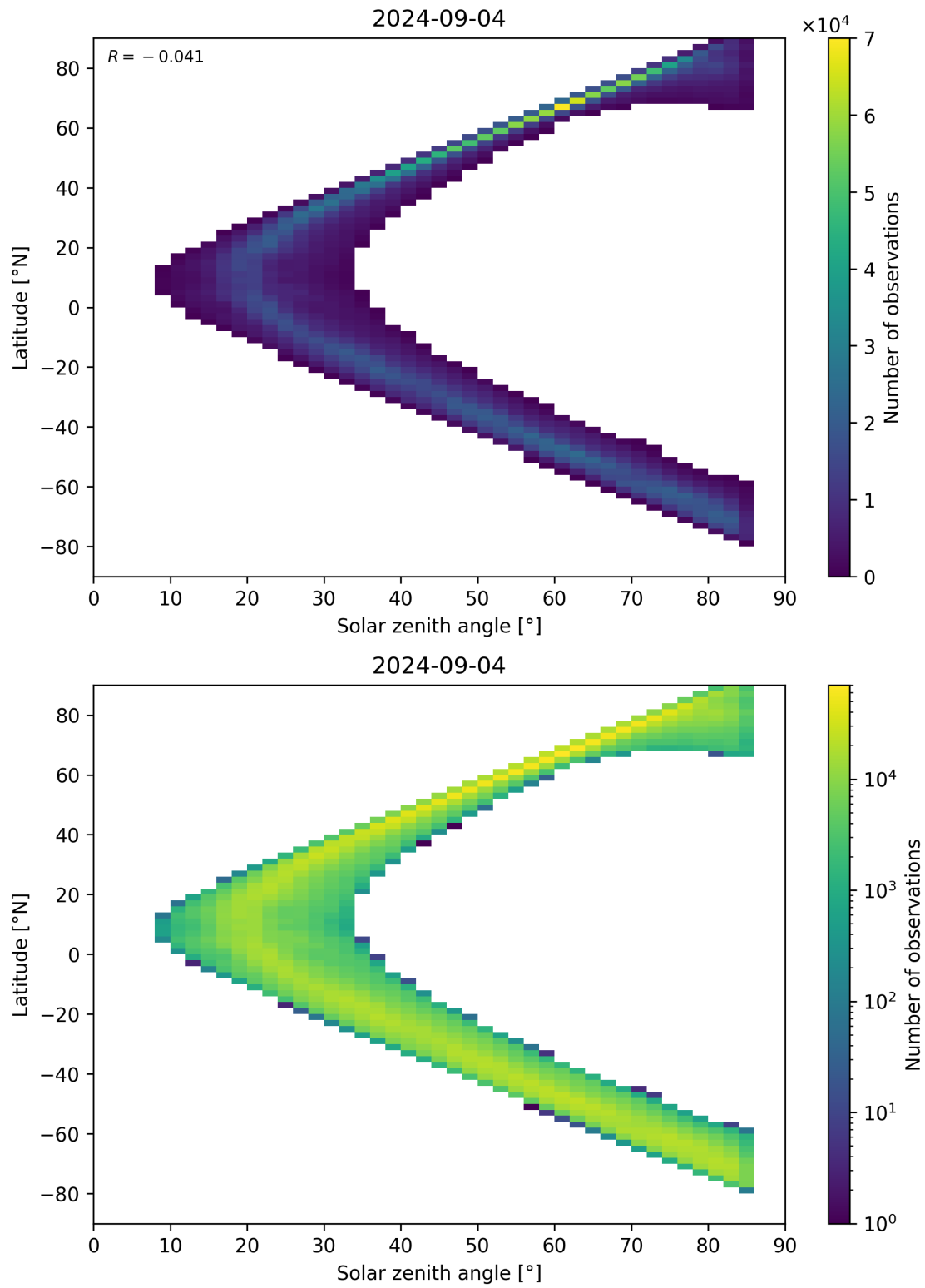
Figure 66: Scatter density plot of “Solar zenith angle” against “Latitude” for 2024-09-03 to 2024-09-05.
