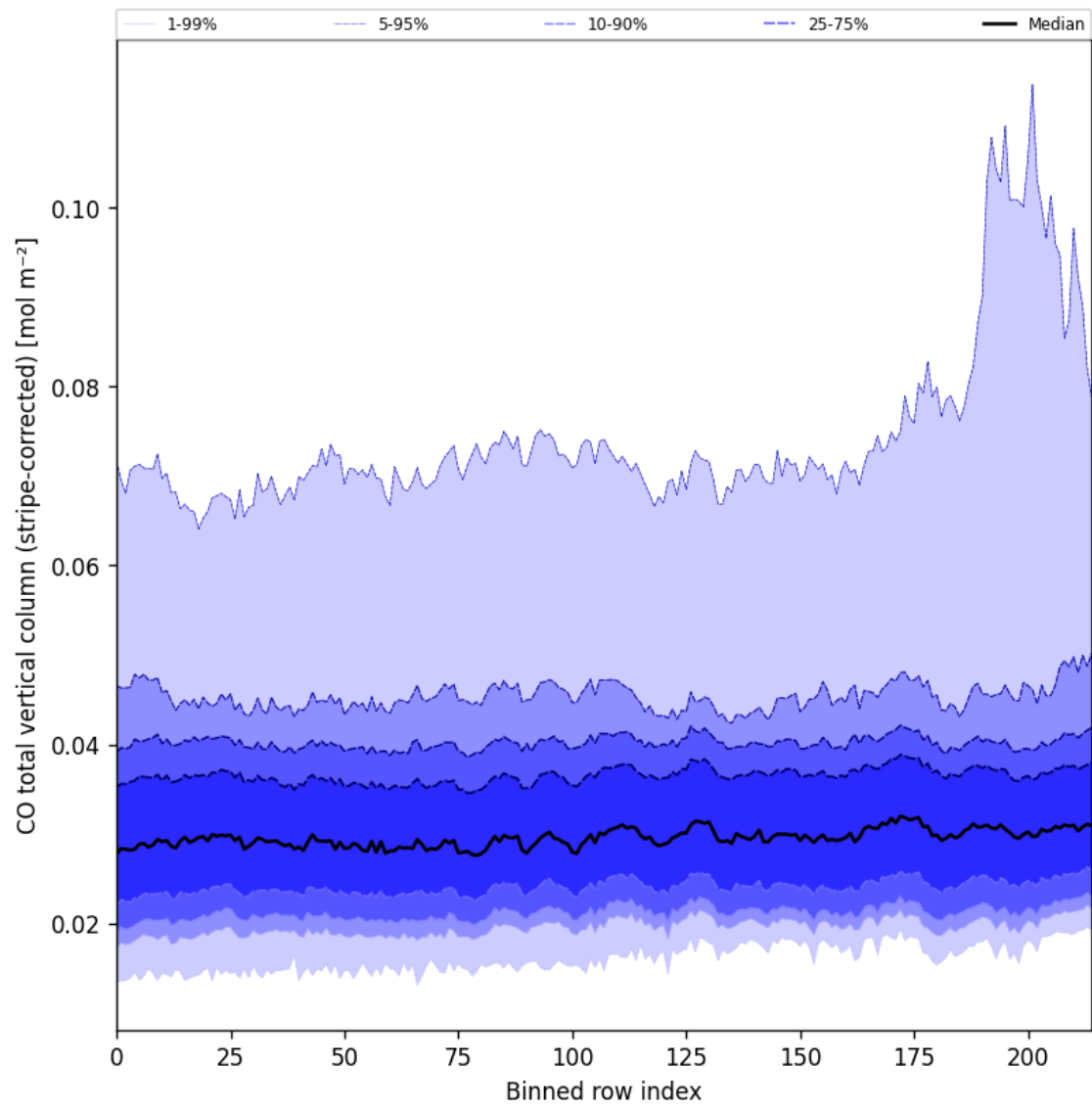
Figure 27: Along track statistics of “CO total vertical column (stripe-corrected)” for 2024-09-03 to 2024-09-05
