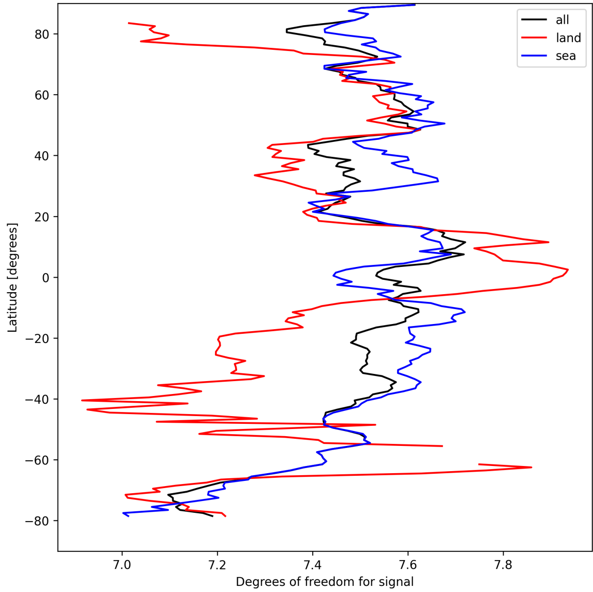
Figure 15: Zonal average of “Degrees of freedom for signal” for 2024-09-03 to 2024-09-05.
