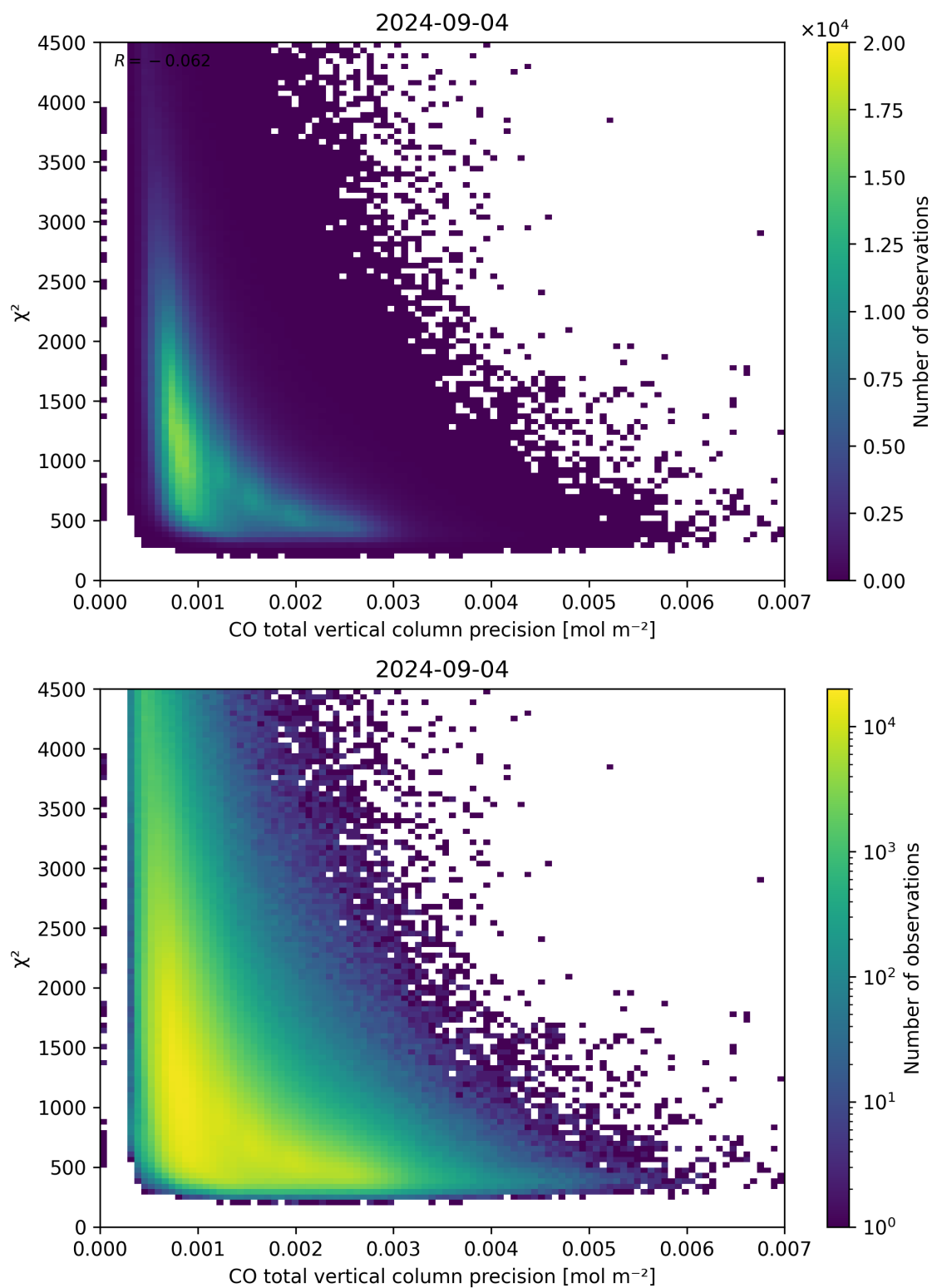
Figure 44: Scatter density plot of “CO total vertical column precision” against “ \chi^2 ” for 2024-09-03 to 2024-09-05.
