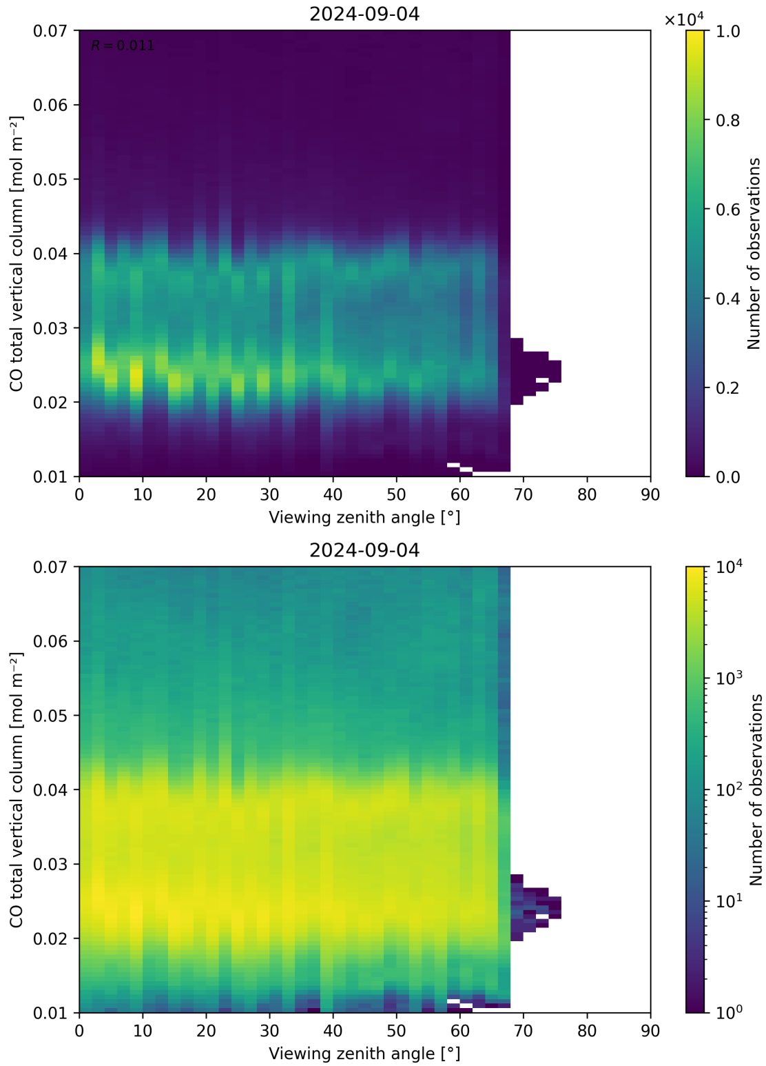
Figure 69: Scatter density plot of “Viewing zenith angle” against “CO total vertical column” for 2024-09-03 to 2024-09-05.
