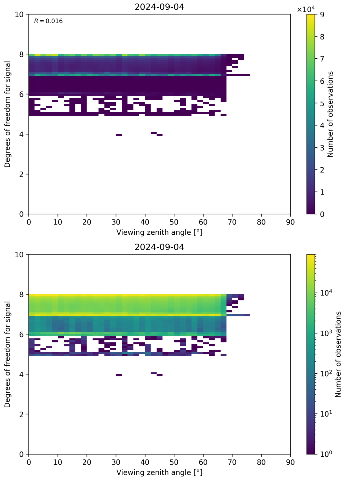
Figure 73: Scatter density plot of “Viewing zenith angle” against “Degrees of freedom for signal” for 2024-09-03 to 2024-09-05.
