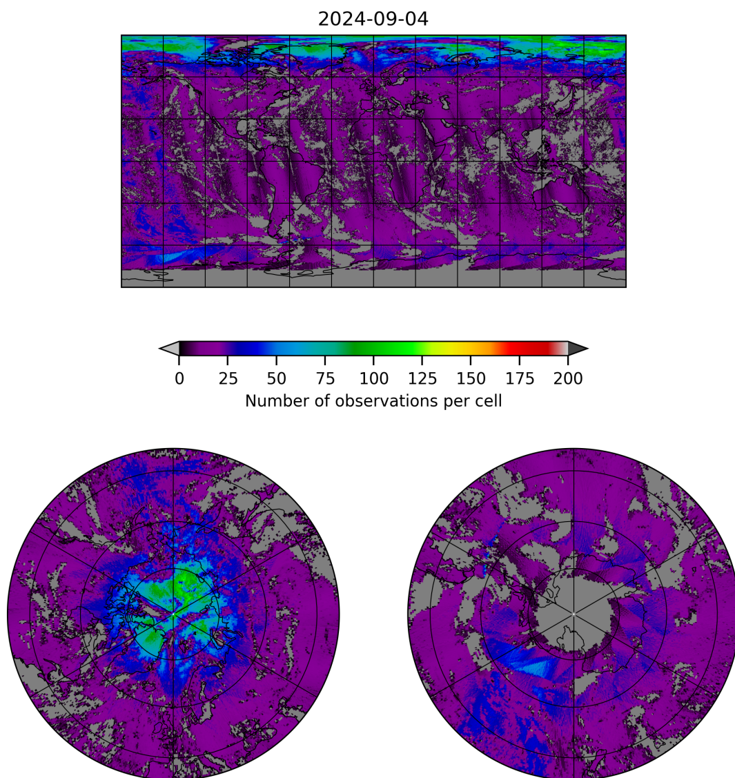
Figure 8: Map of the number of observations for 2024-09-03 to 2024-09-05
