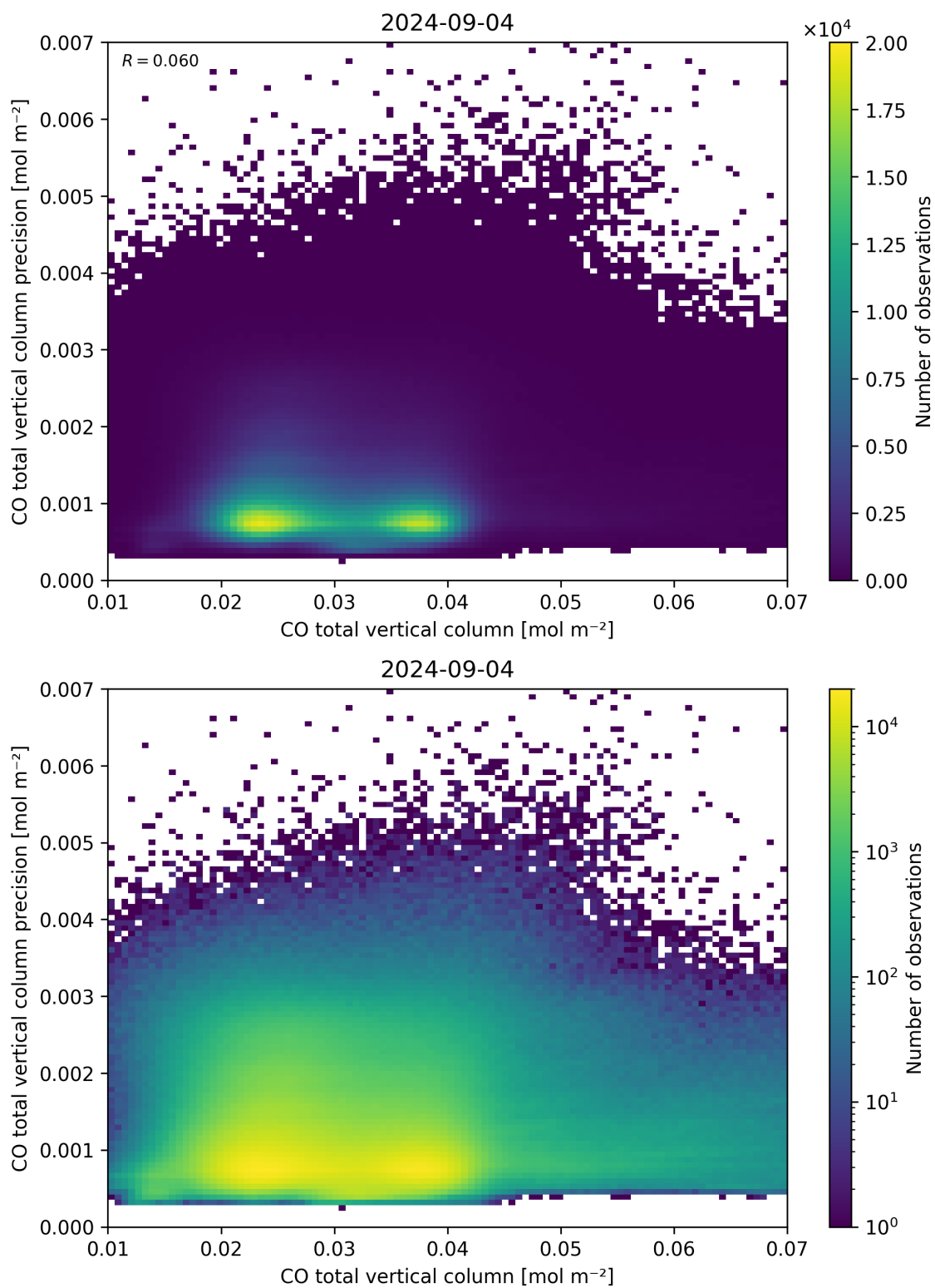
Figure 34: Scatter density plot of “CO total vertical column” against “CO total vertical column precision” for 2024-09-03 to 2024-09-05.
