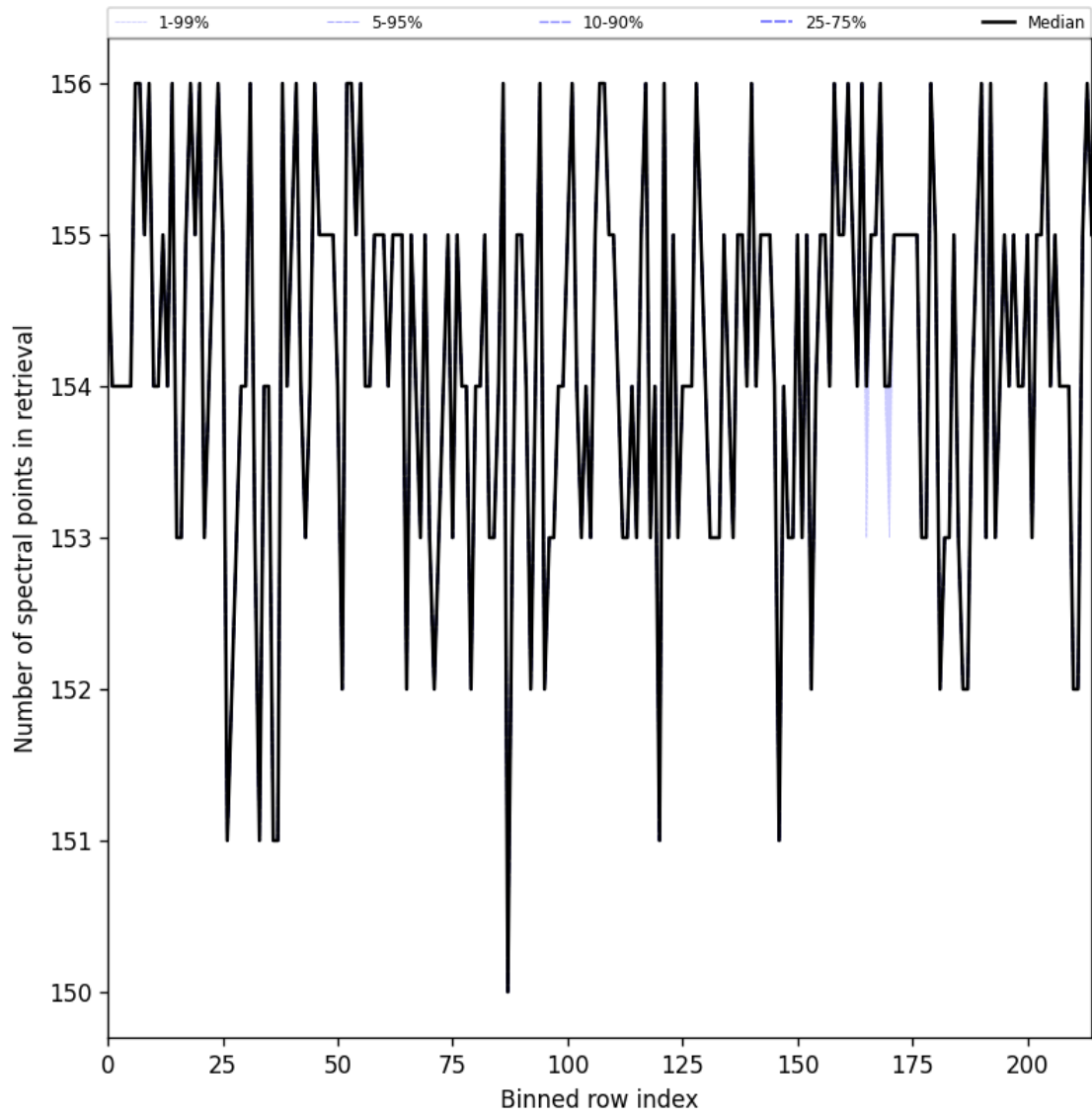
Figure 29: Along track statistics of “Number of spectral points in retrieval” for 2024-09-03 to 2024-09-05
