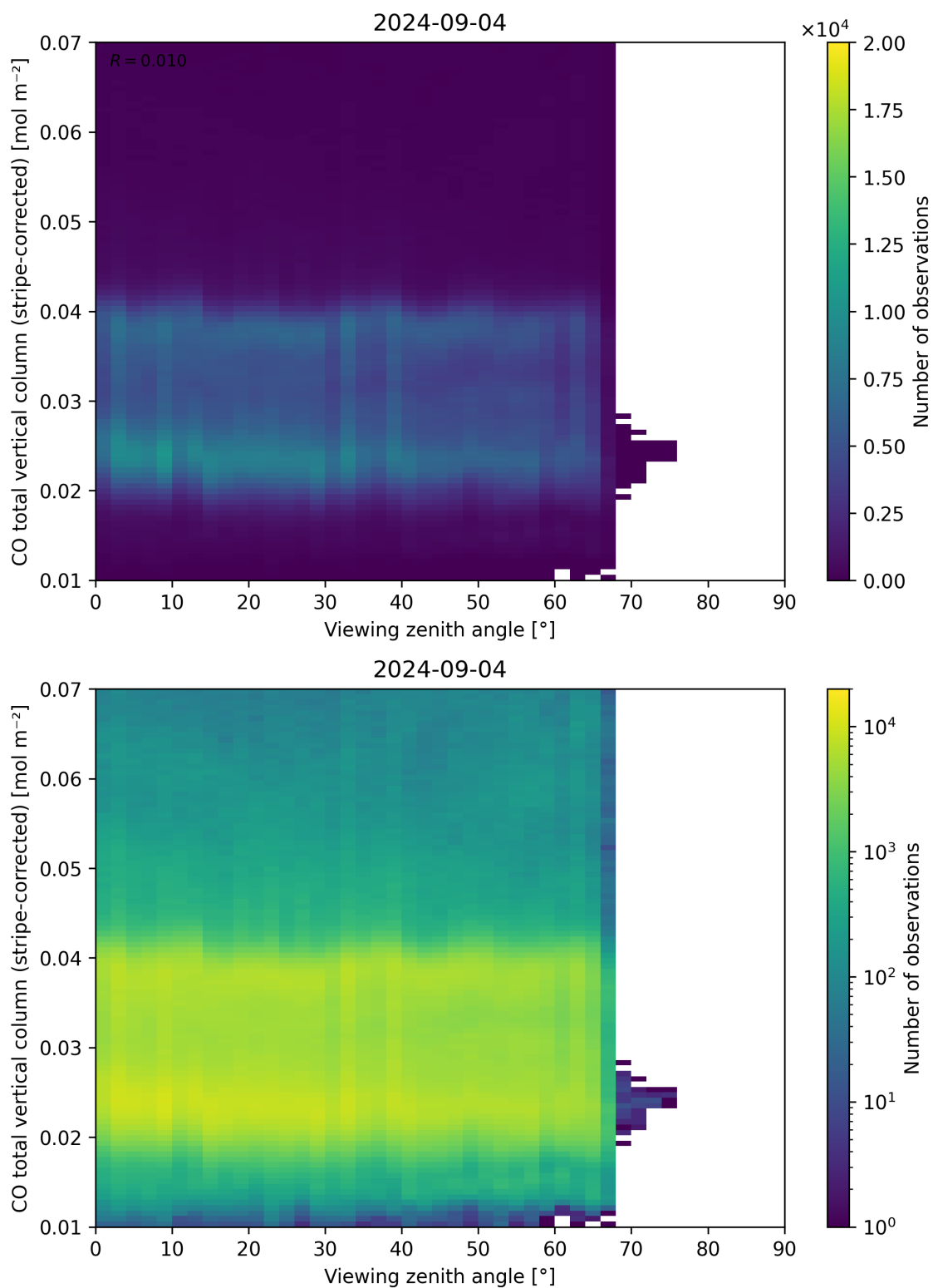
Figure 70: Scatter density plot of “Viewing zenith angle” against “CO total vertical column (stripe-corrected)” for 2024-09-03 to 2024-09-05.
