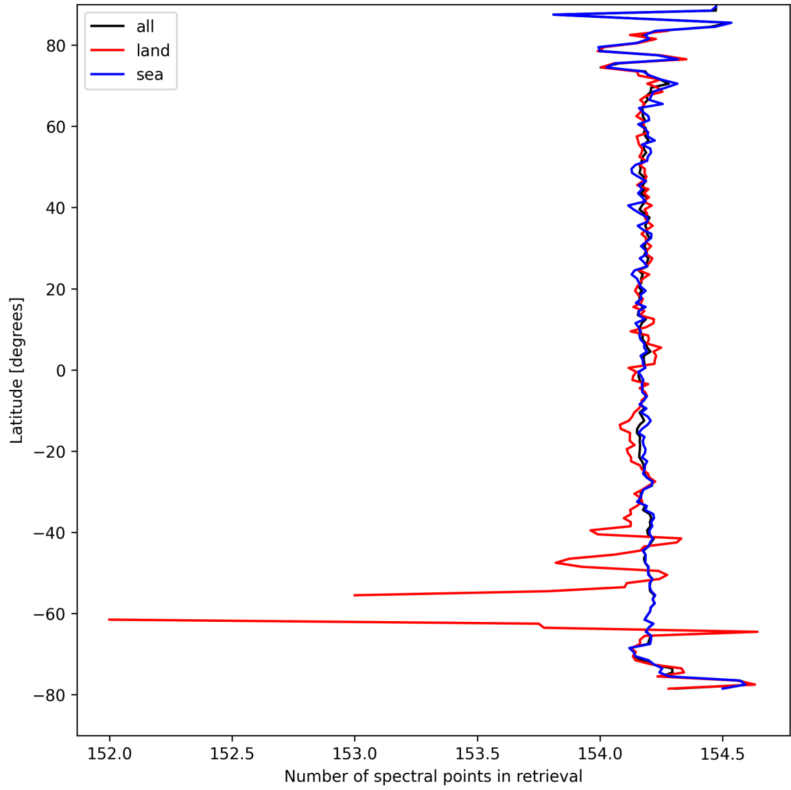
Figure 13: Zonal average of “Number of spectral points in retrieval” for 2024-09-03 to 2024-09-05.
