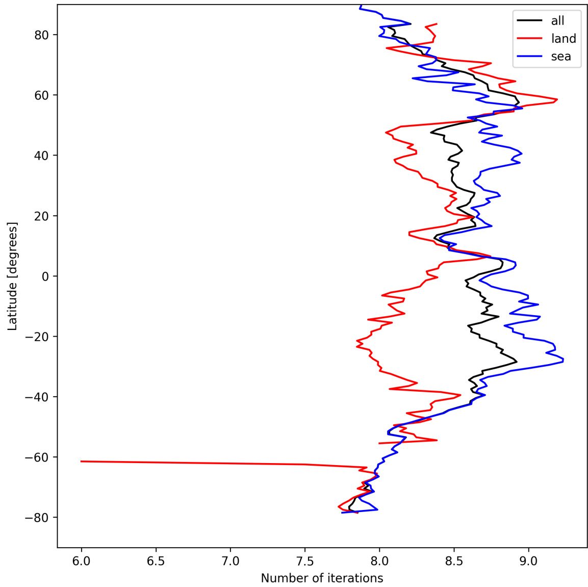
Figure 16: Zonal average of “Number of iterations” for 2024-09-03 to 2024-09-05.
