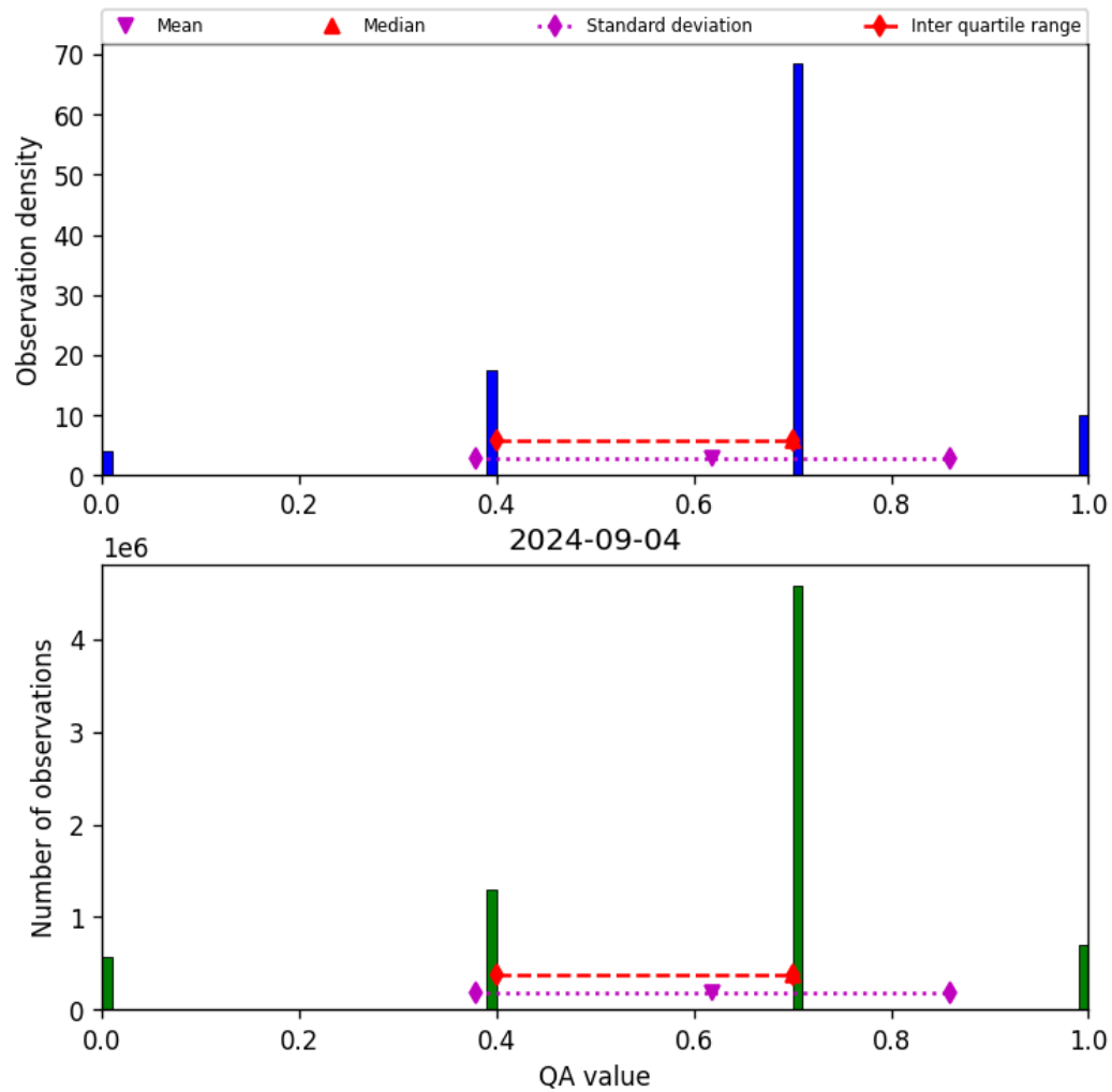
Figure 17: Histogram of “QA value” for 2024-09-03 to 2024-09-05
