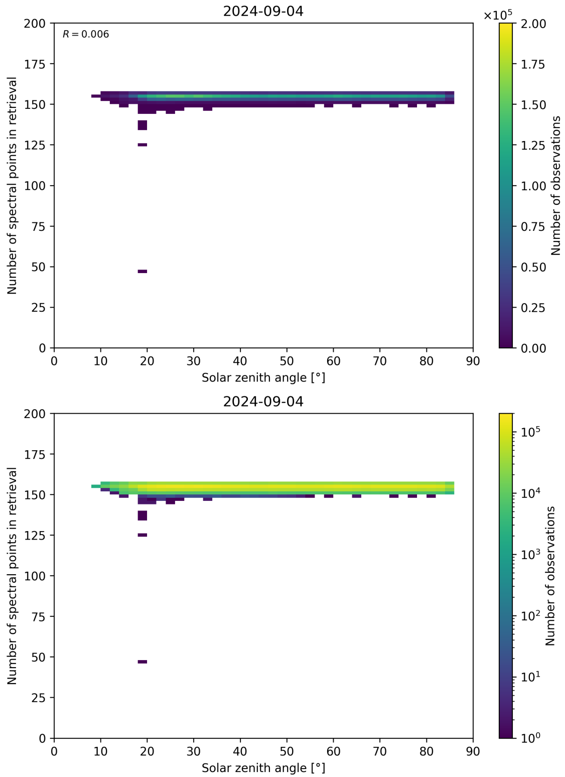
Figure 68: Scatter density plot of “Solar zenith angle” against “Number of spectral points in retrieval” for 2024-09-03 to 2024-09-05.
