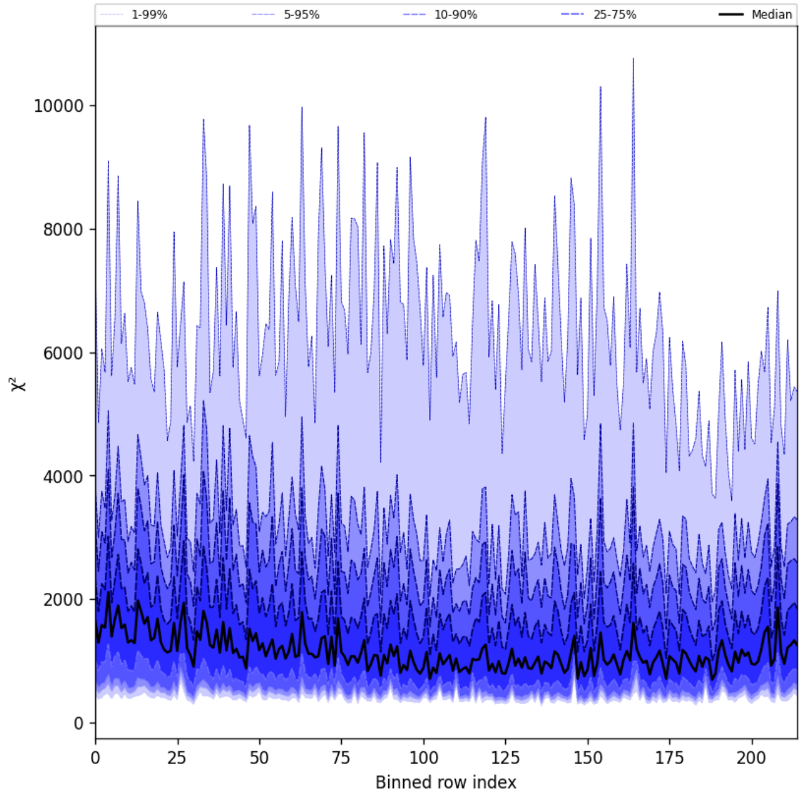
Figure 30: Along track statistics of “ \chi^2 ” for 2024-09-03 to 2024-09-05
