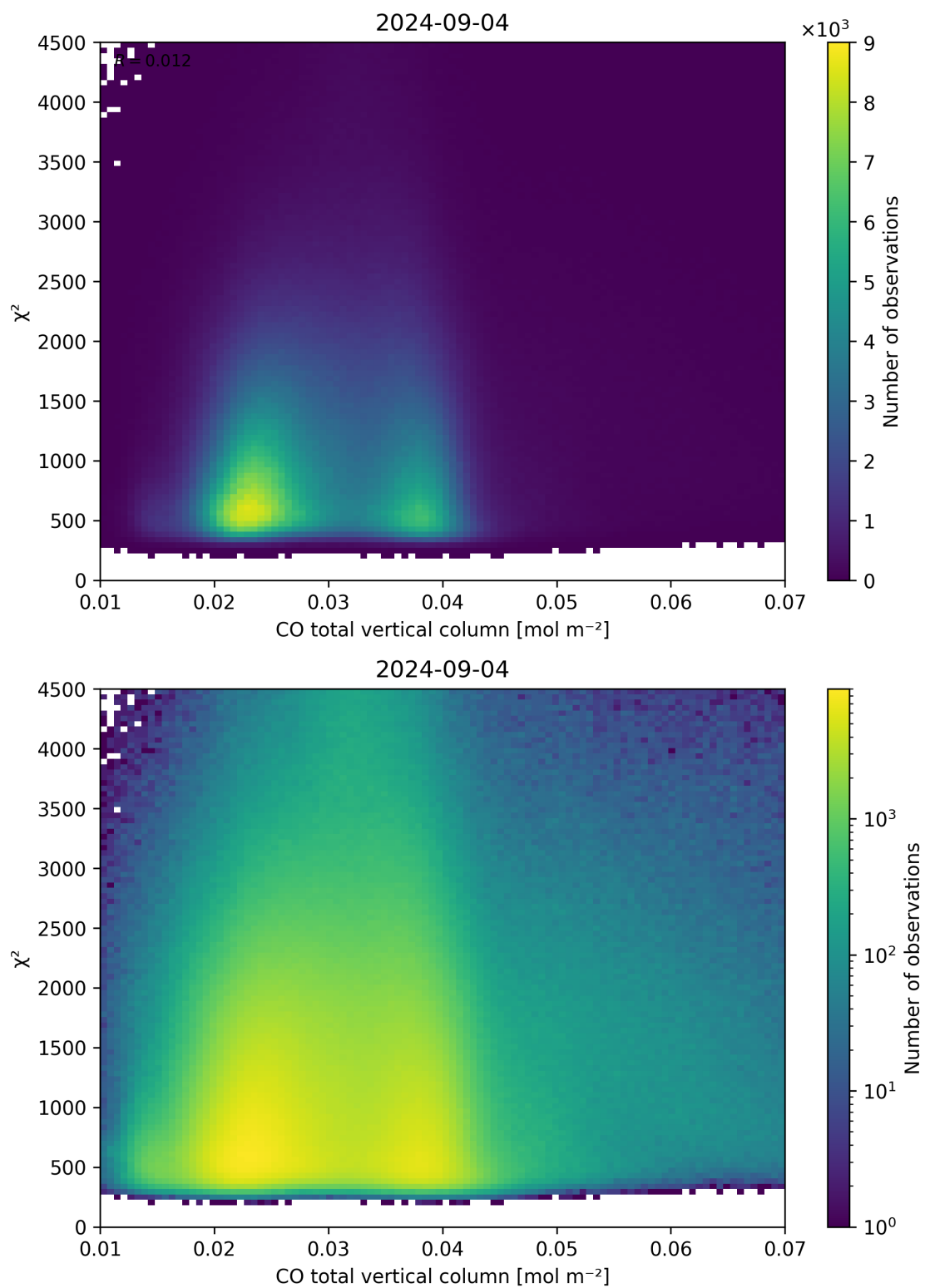
Figure 35: Scatter density plot of “CO total vertical column” against “ \chi^2 ” for 2024-09-03 to 2024-09-05.
