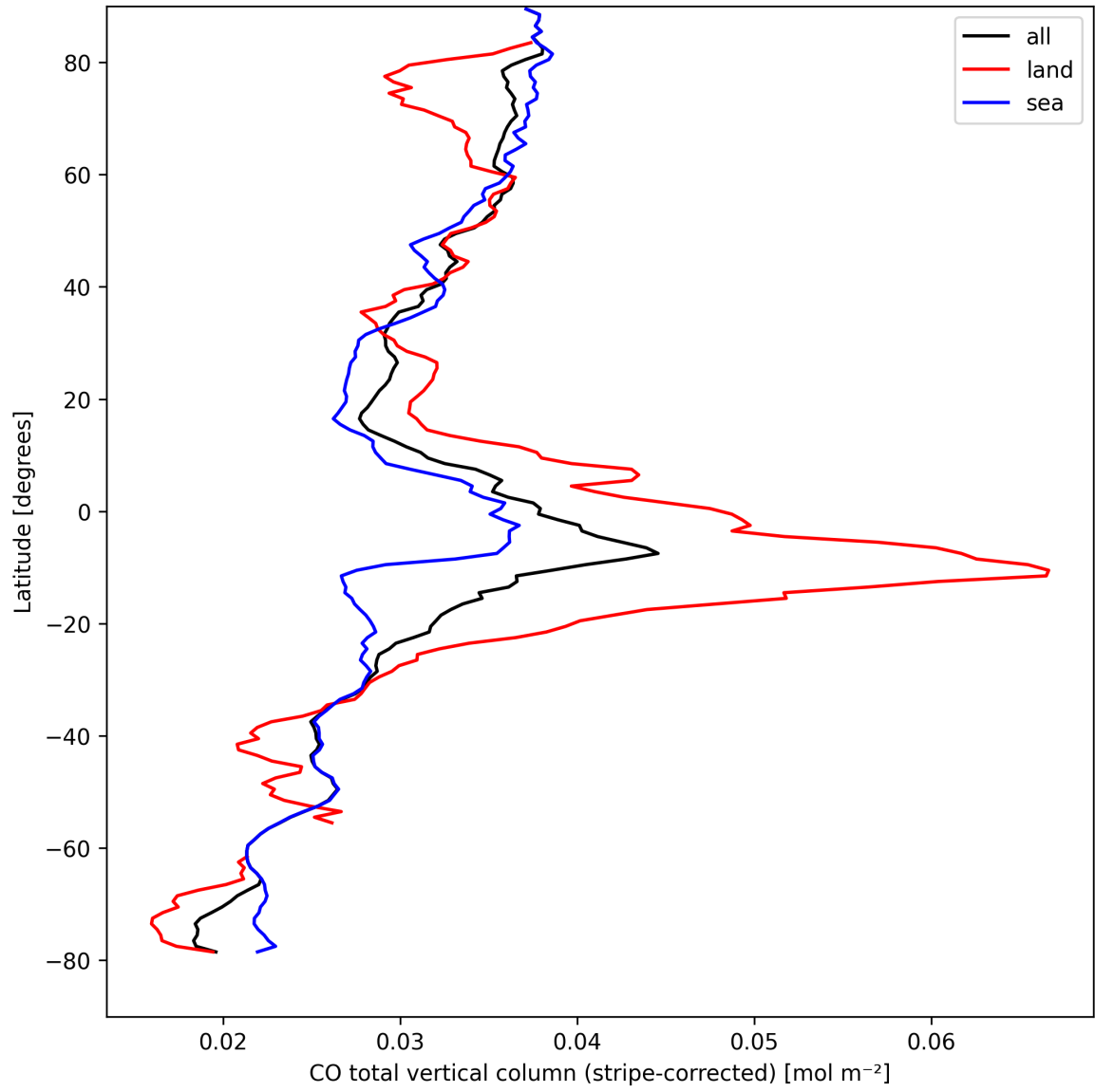
Figure 11: Zonal average of “CO total vertical column (stripe-corrected)” for 2024-09-03 to 2024-09-05.
