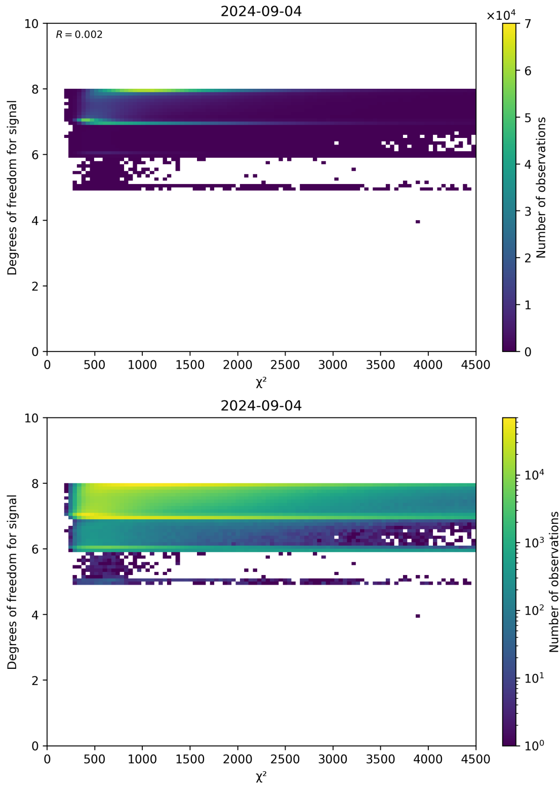
Figure 48: Scatter density plot of “ \chi^2 ” against “Degrees of freedom for signal” for 2024-09-03 to 2024-09-05.
