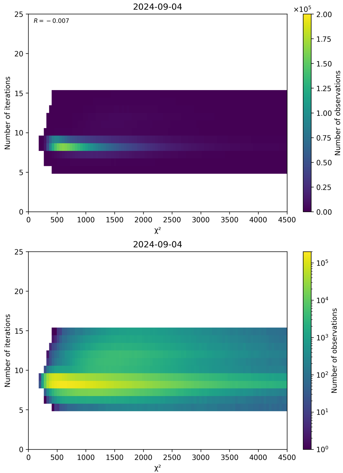
Figure 49: Scatter density plot of “ \chi^2 ” against “Number of iterations” for 2024-09-03 to 2024-09-05.
