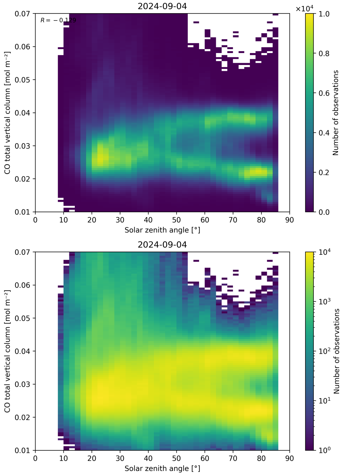
Figure 61: Scatter density plot of “Solar zenith angle” against “CO total vertical column” for 2024-09-03 to 2024-09-05.
