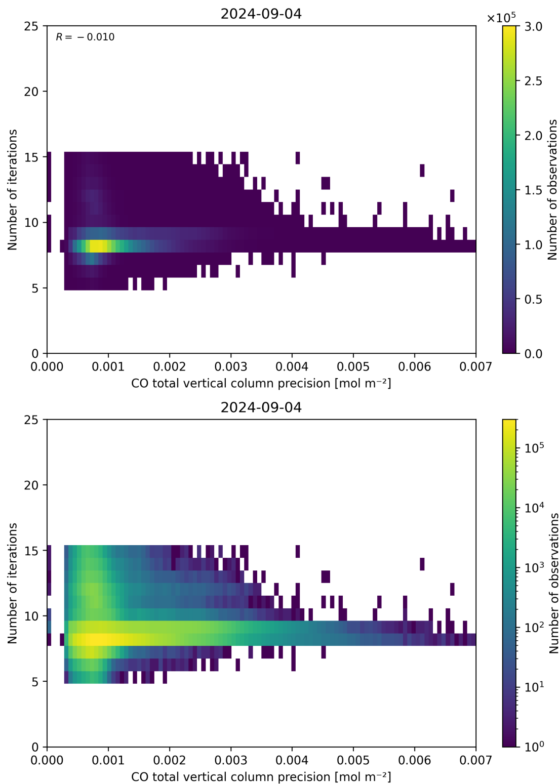
Figure 46: Scatter density plot of “CO total vertical column precision” against “Number of iterations” for 2024-09-03 to 2024-09-05.
