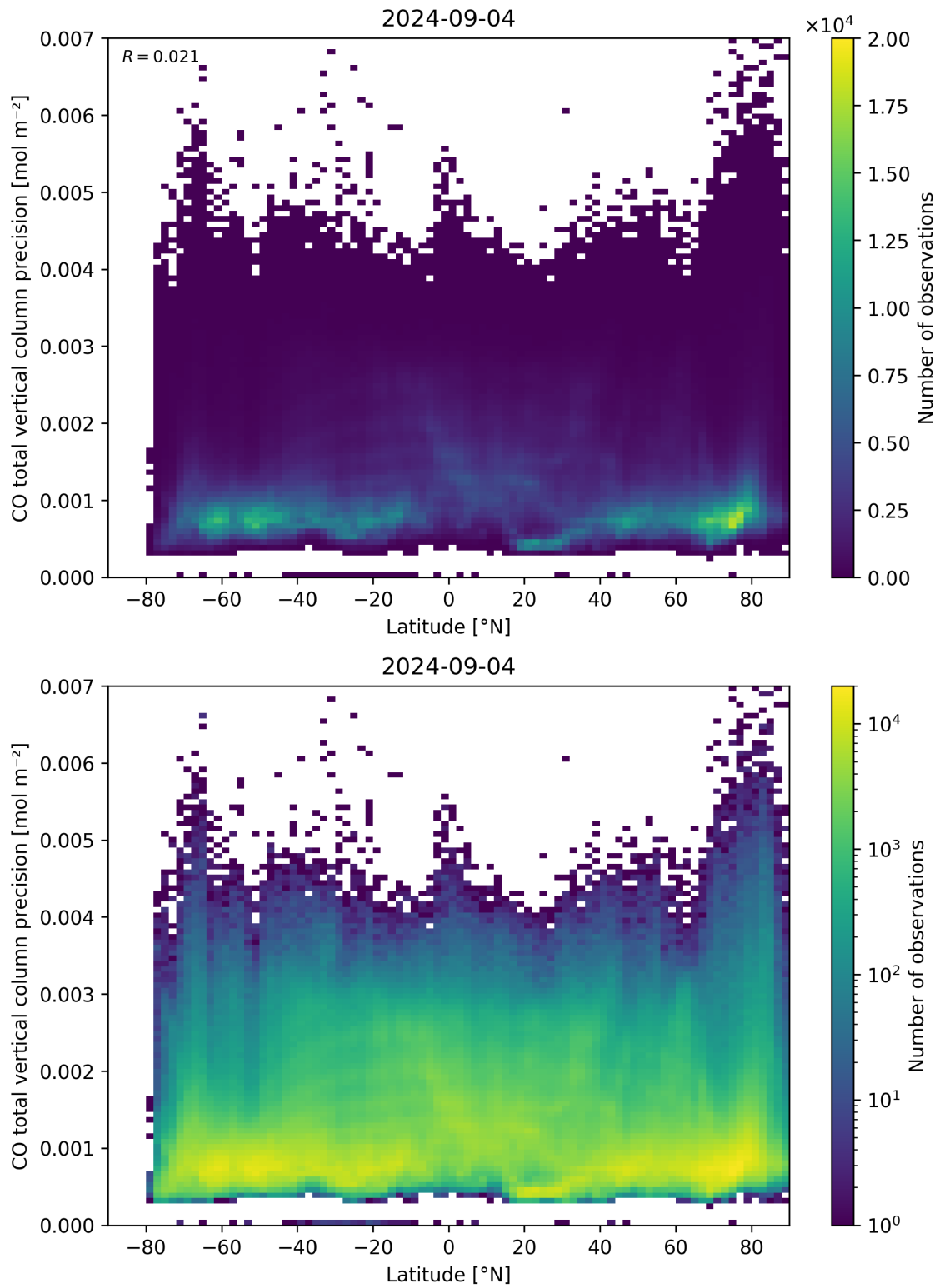
Figure 53: Scatter density plot of “Latitude” against “CO total vertical column precision” for 2024-09-03 to 2024-09-05.
