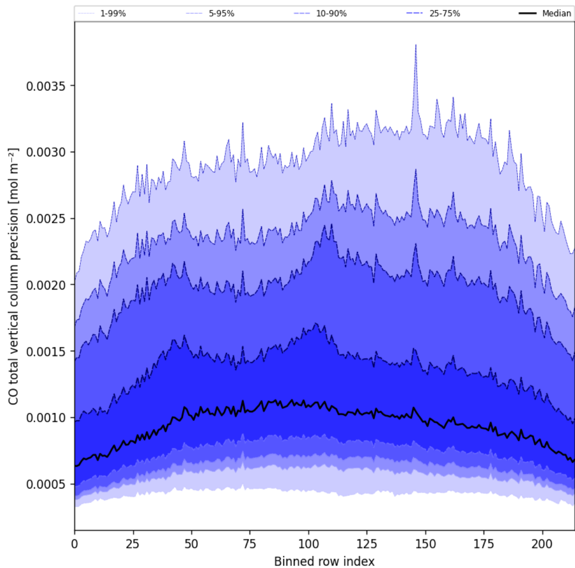
Figure 28: Along track statistics of “CO total vertical column precision” for 2024-09-03 to 2024-09-05
