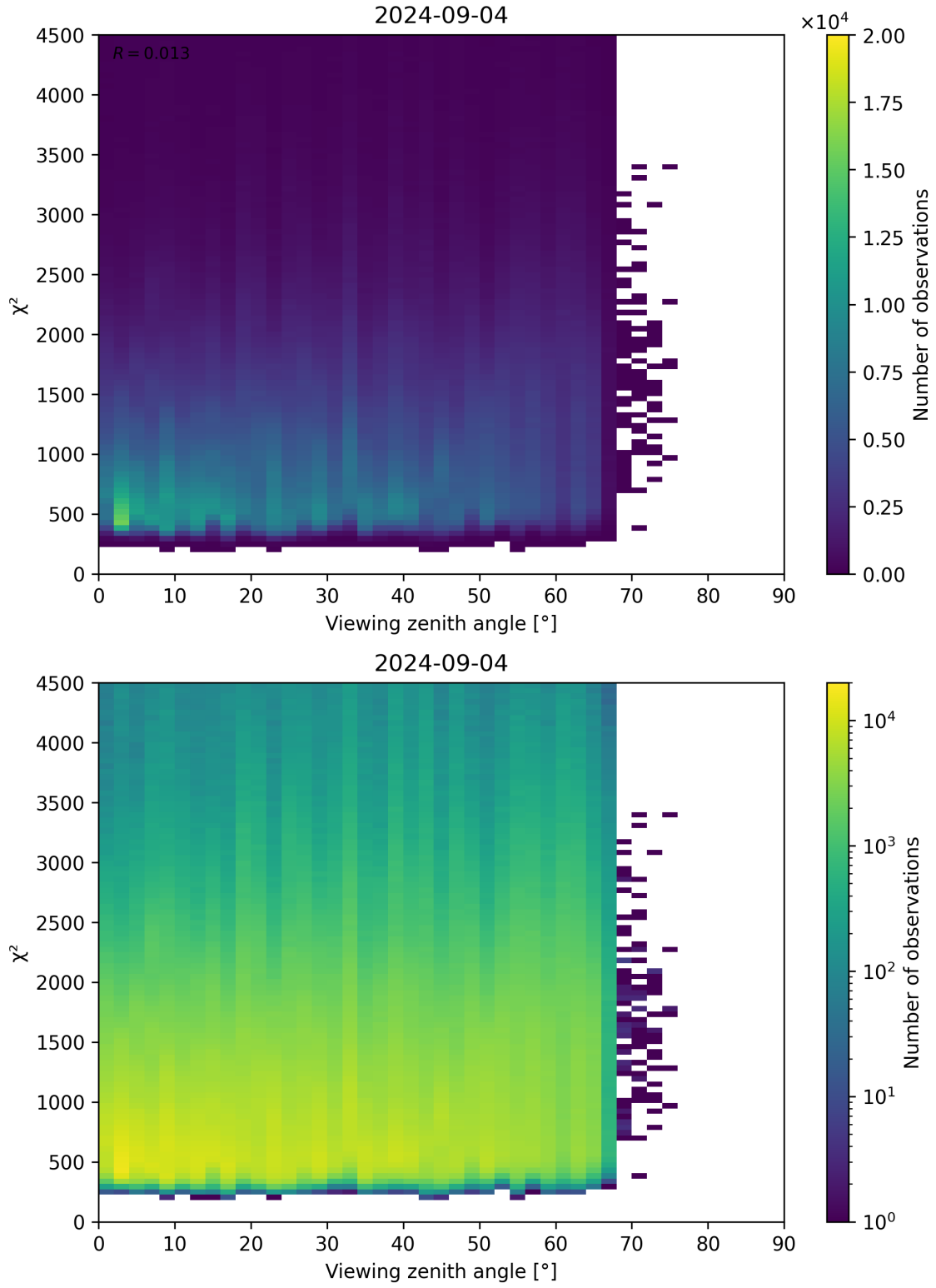
Figure 72: Scatter density plot of “Viewing zenith angle” against “ \chi^2 ” for 2024-09-03 to 2024-09-05.
