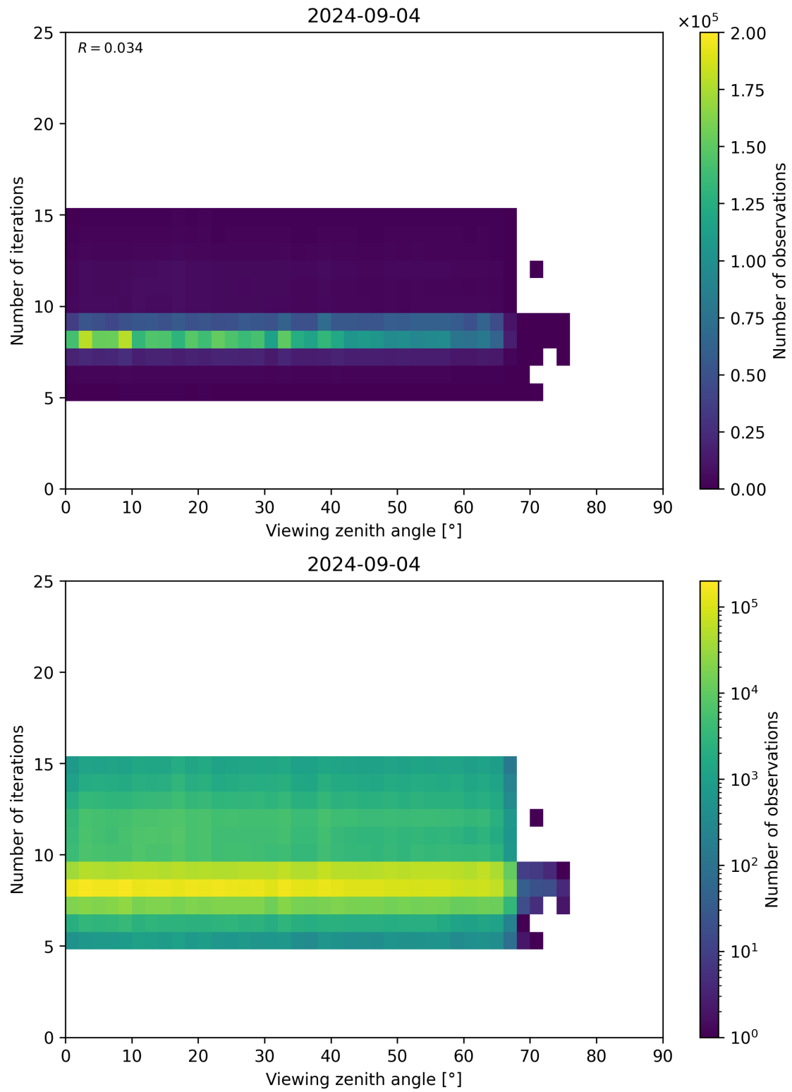
Figure 75: Scatter density plot of “Viewing zenith angle” against “Number of iterations” for 2024-09-03 to 2024-09-05.
