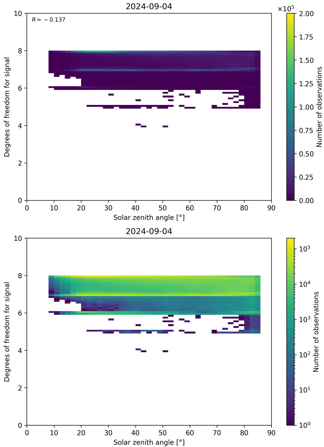
Figure 65: Scatter density plot of “Solar zenith angle” against “Degrees of freedom for signal” for 2024-09-03 to 2024-09-05.
