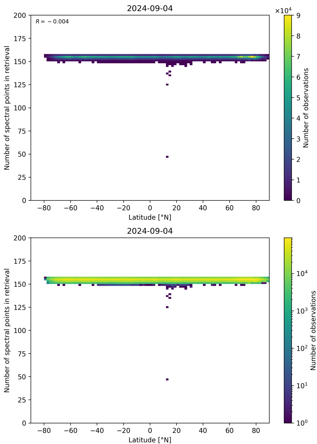
Figure 57: Scatter density plot of “Latitude” against “Number of spectral points in retrieval” for 2024-09-03 to 2024-09-05.
