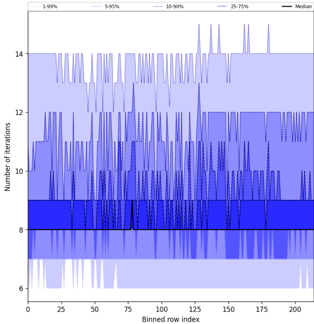
Figure 32: Along track statistics of “Number of iterations” for 2024-09-03 to 2024-09-05
