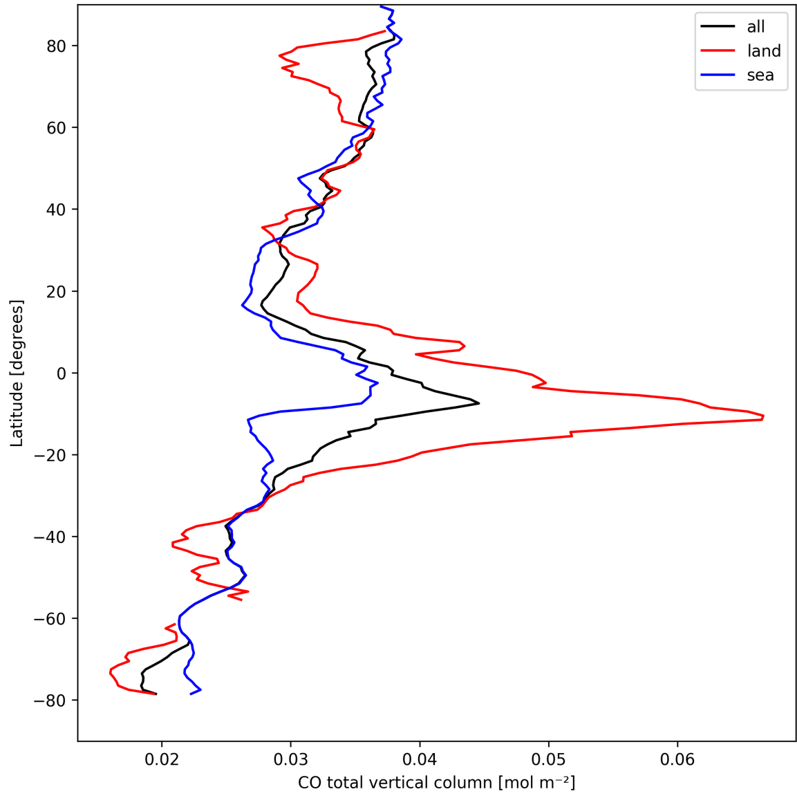
Figure 10: Zonal average of “CO total vertical column” for 2024-09-03 to 2024-09-05.
