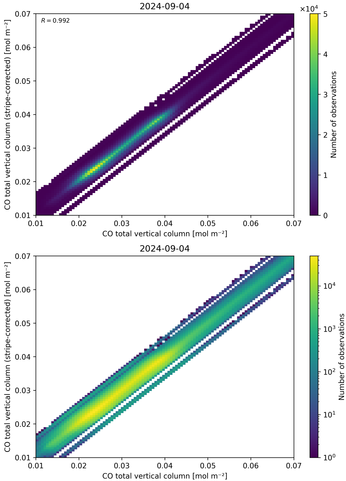
Figure 33: Scatter density plot of “CO total vertical column” against “CO total vertical column (stripe-corrected)” for 2024-09-03 to 2024-09-05.
