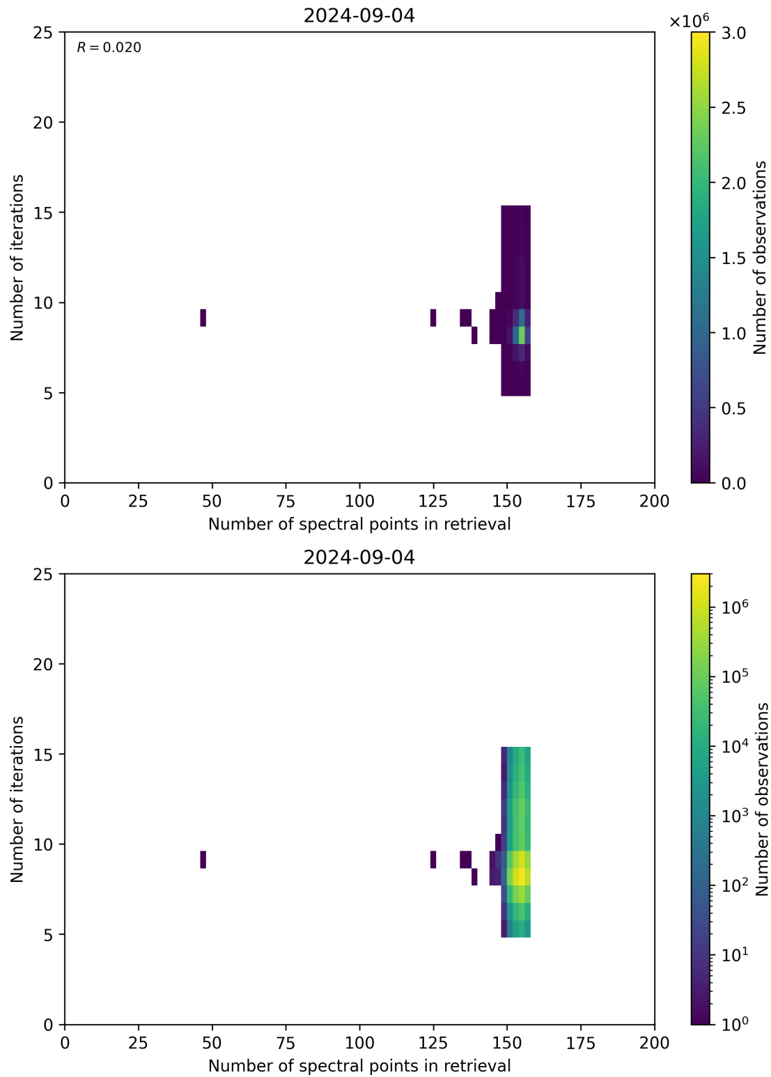
Figure 60: Scatter density plot of “Number of spectral points in retrieval” against “Number of iterations” for 2024-09-03 to 2024-09-05.
