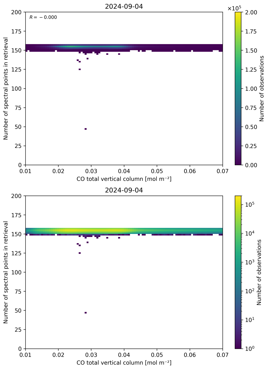
Figure 43: Scatter density plot of “CO total vertical column” against “Number of spectral points in retrieval” for 2024-09-03 to 2024-09-05.
