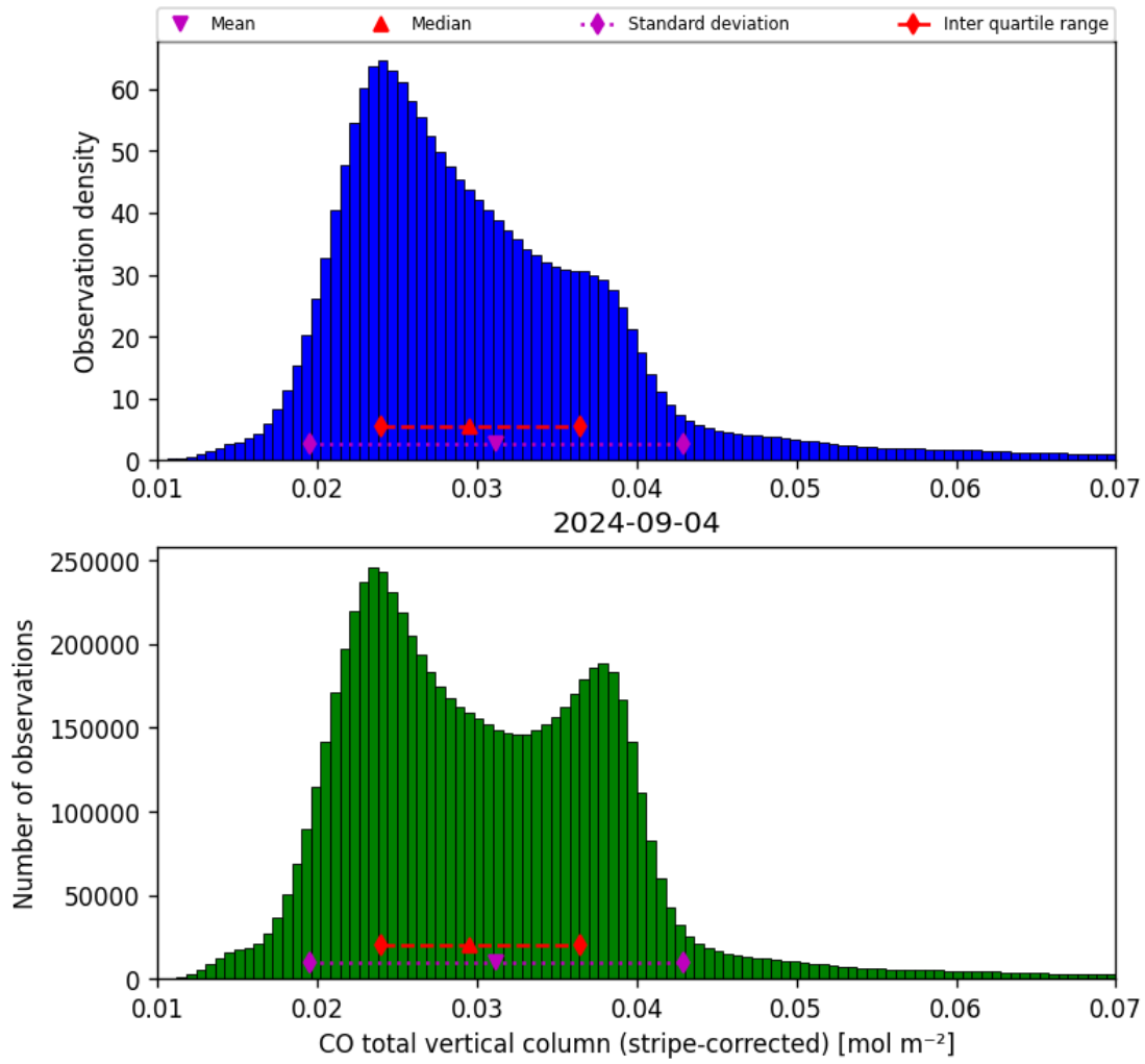
Figure 19: Histogram of “CO total vertical column (stripe-corrected)” for 2024-09-03 to 2024-09-05
