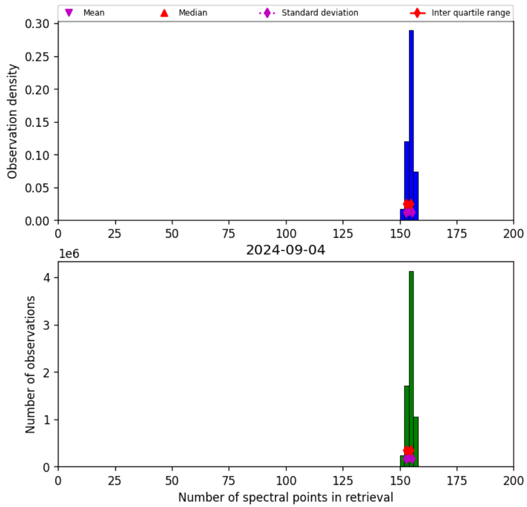
Figure 21: Histogram of “Number of spectral points in retrieval” for 2024-09-03 to 2024-09-05
