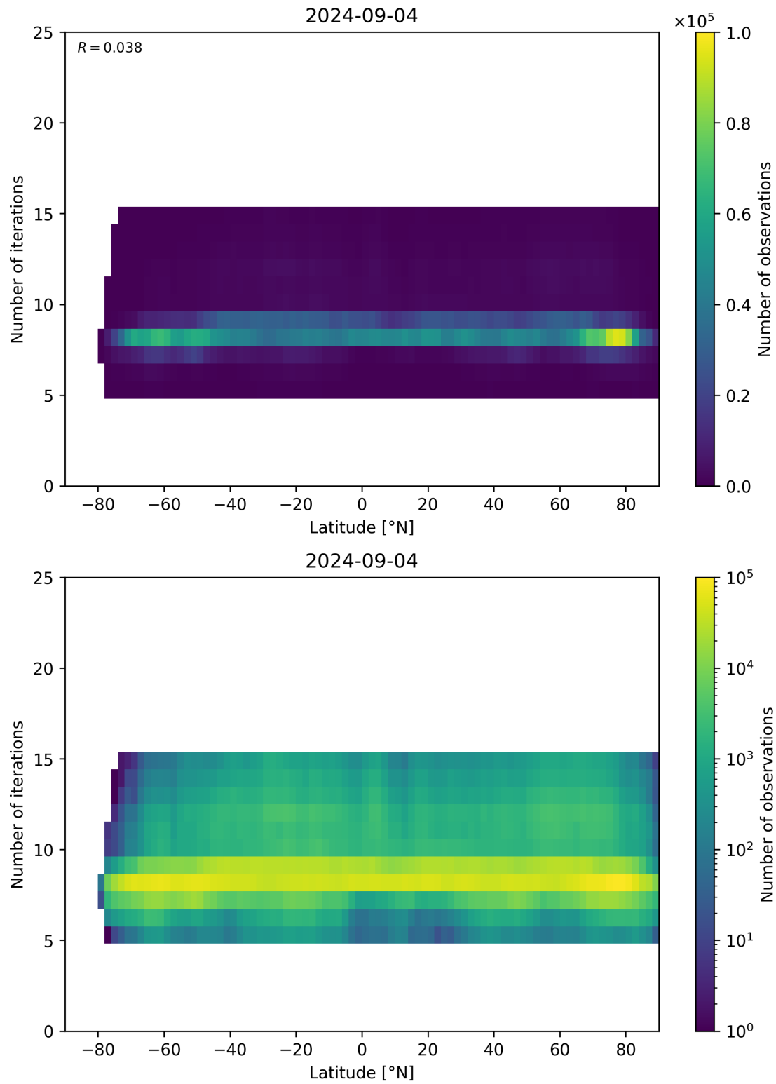
Figure 56: Scatter density plot of “Latitude” against “Number of iterations” for 2024-09-03 to 2024-09-05.
