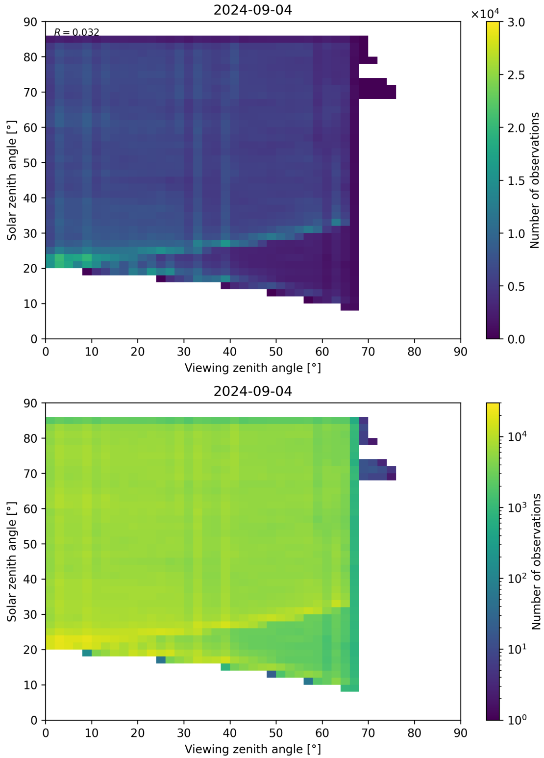
Figure 77: Scatter density plot of “Viewing zenith angle” against “Solar zenith angle” for 2024-09-03 to 2024-09-05.
