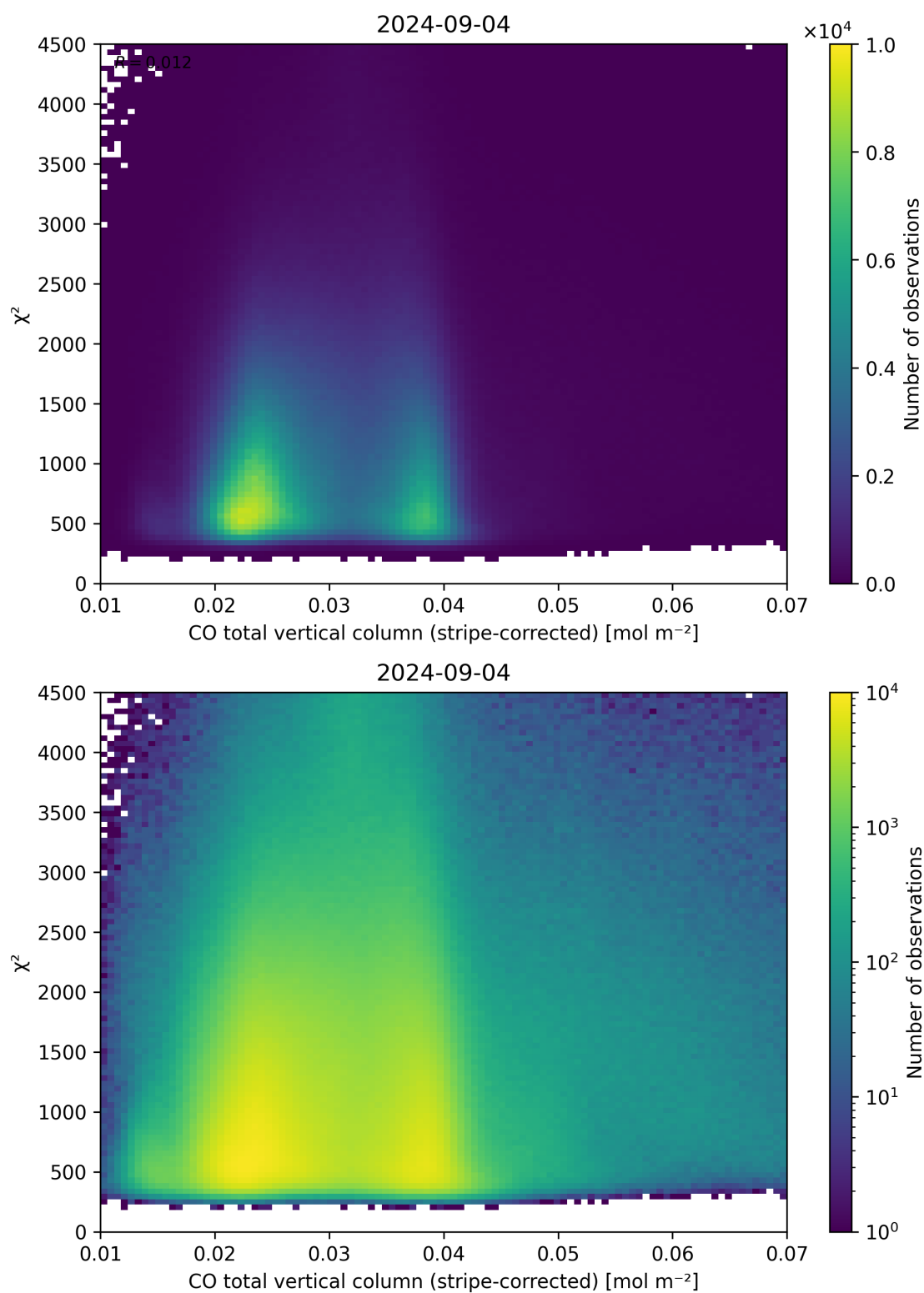
Figure 37: Scatter density plot of “CO total vertical column (stripe-corrected)” against “ \chi^2 ” for 2024-09-03 to 2024-09-05.
