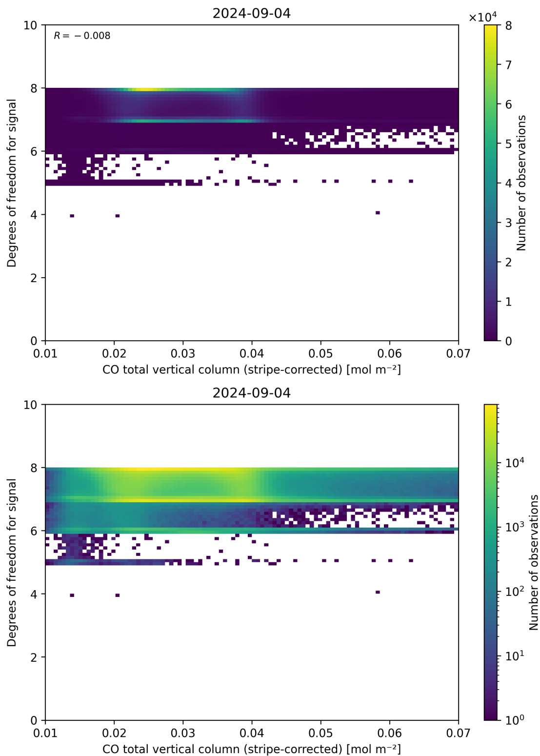
Figure 38: Scatter density plot of “CO total vertical column (stripe-corrected)” against “Degrees of freedom for signal” for 2024-09-03 to 2024-09-05.
