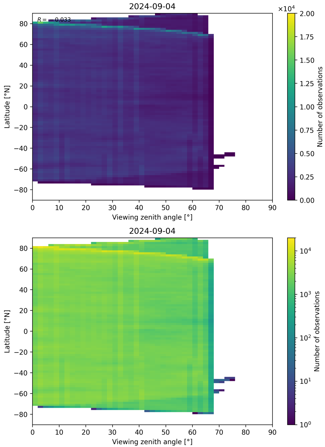
Figure 74: Scatter density plot of “Viewing zenith angle” against “Latitude” for 2024-09-03 to 2024-09-05.
