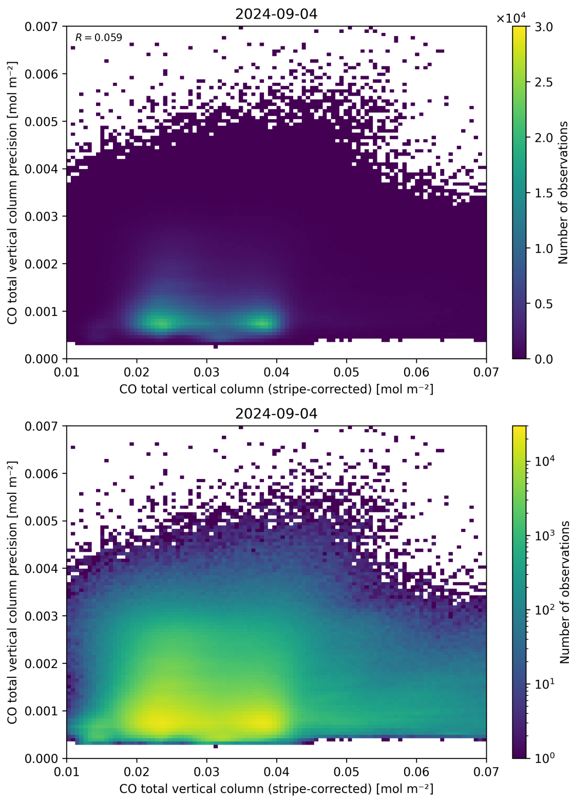
Figure 36: Scatter density plot of “CO total vertical column (stripe-corrected)” against “CO total vertical column precision” for 2024-09-03 to 2024-09-05.
