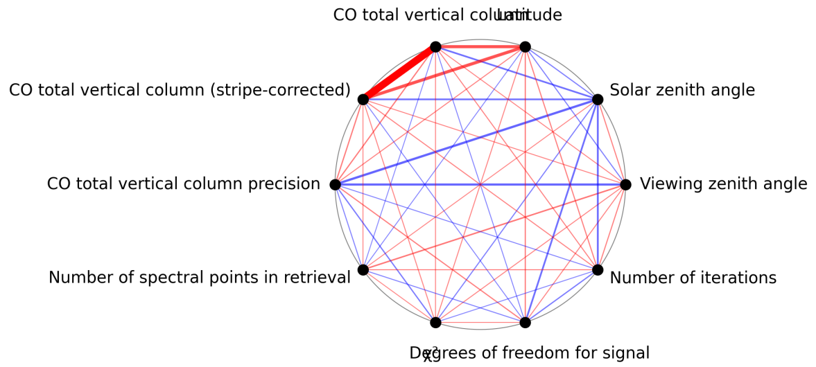
Figure 1: Map of correlation graph for 2024-09-03 to 2024-09-05.
