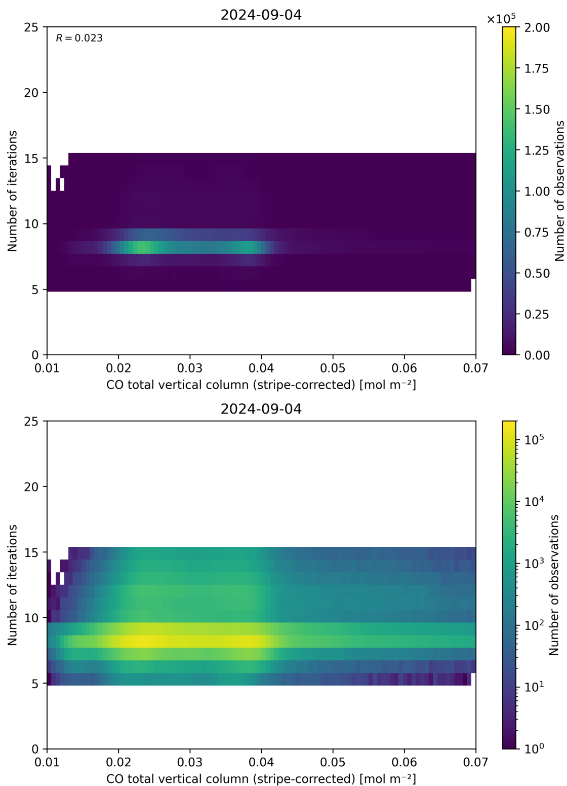
Figure 39: Scatter density plot of “CO total vertical column (stripe-corrected)” against “Number of iterations” for 2024-09-03 to 2024-09-05.
