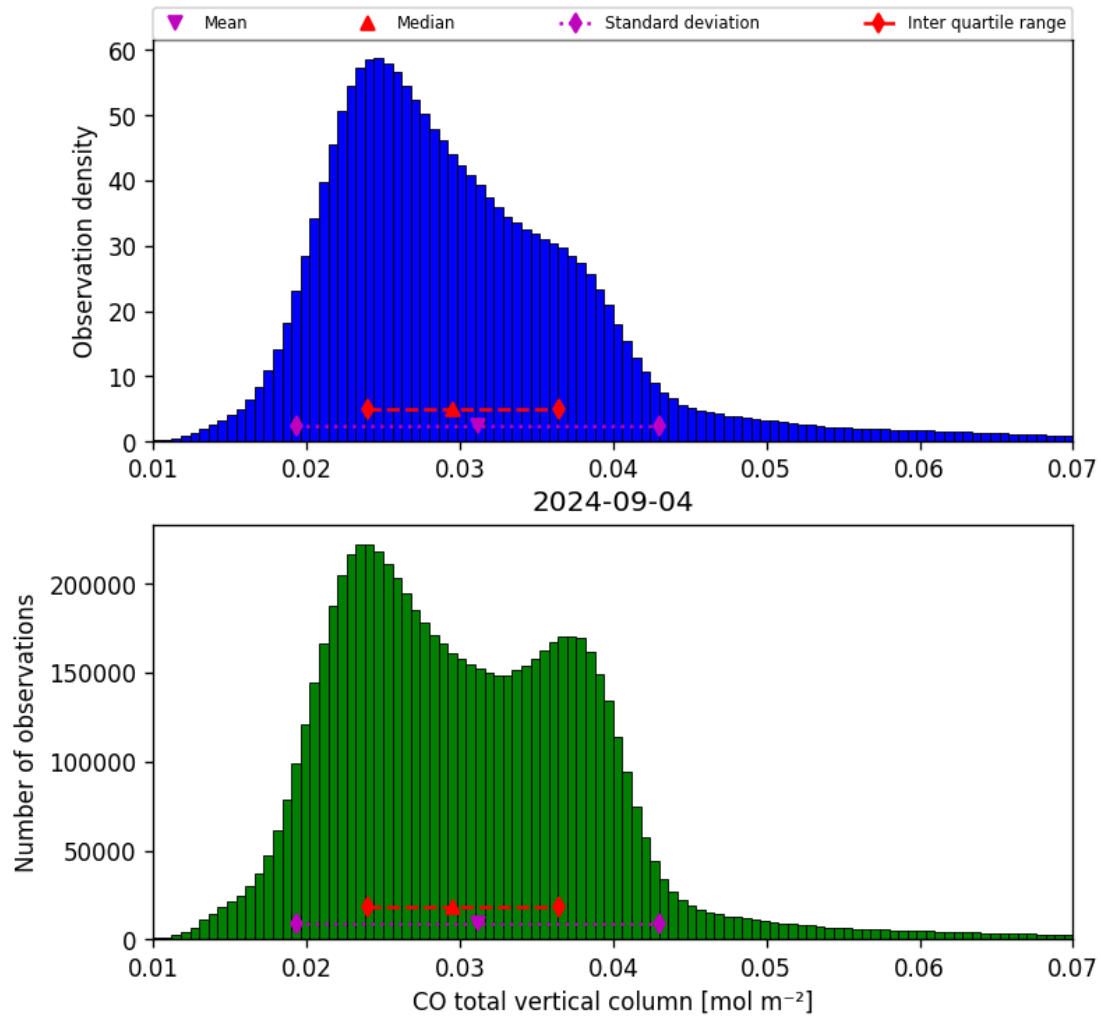
Figure 18: Histogram of “CO total vertical column” for 2024-09-03 to 2024-09-05
