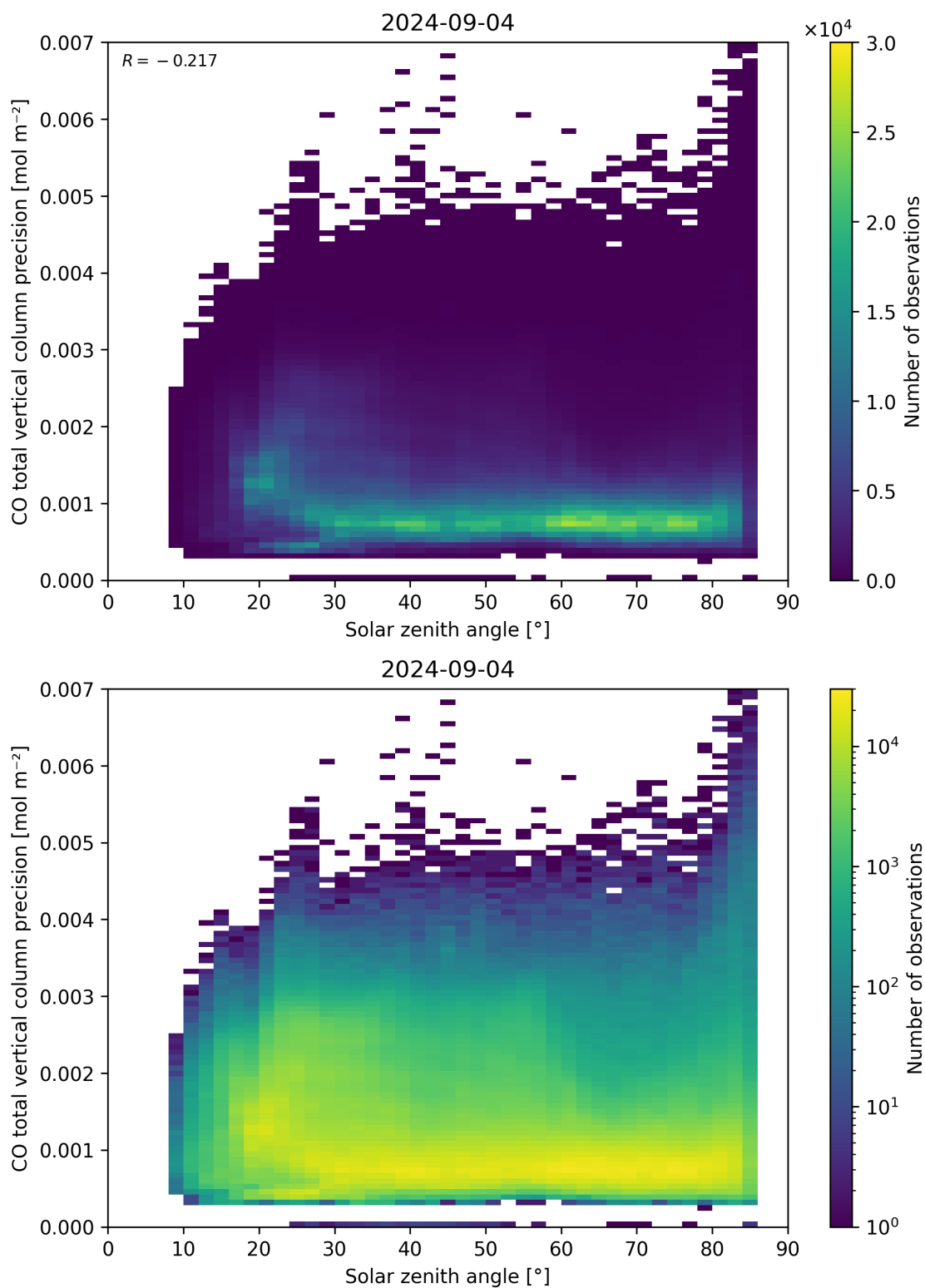
Figure 63: Scatter density plot of “Solar zenith angle” against “CO total vertical column precision” for 2024-09-03 to 2024-09-05.
