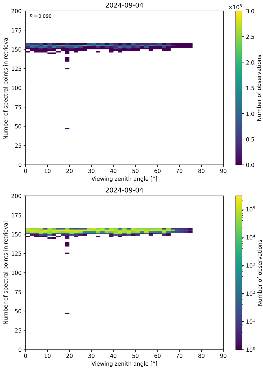
Figure 76: Scatter density plot of “Viewing zenith angle” against “Number of spectral points in retrieval” for 2024-09-03 to 2024-09-05.
