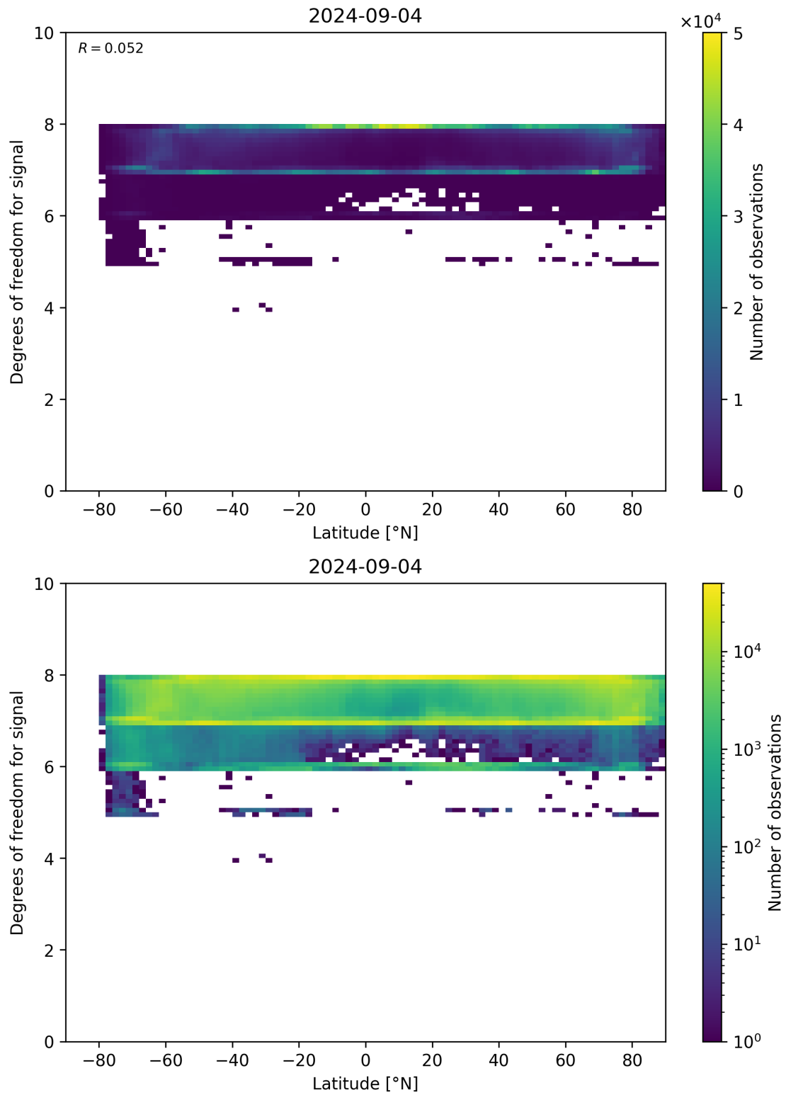
Figure 55: Scatter density plot of “Latitude” against “Degrees of freedom for signal” for 2024-09-03 to 2024-09-05.
