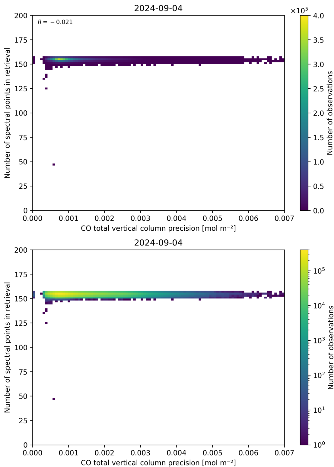
Figure 47: Scatter density plot of “CO total vertical column precision” against “Number of spectral points in retrieval” for 2024-09-03 to 2024-09-05.
