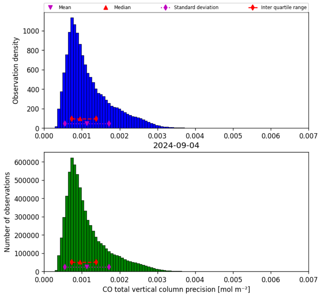
Figure 20: Histogram of “CO total vertical column precision” for 2024-09-03 to 2024-09-05
