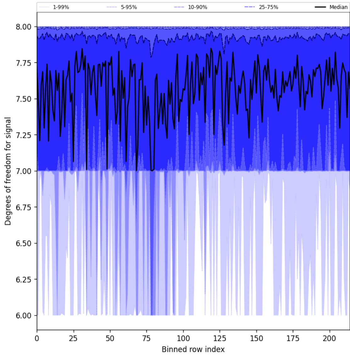
Figure 31: Along track statistics of “Degrees of freedom for signal” for 2024-09-03 to 2024-09-05
