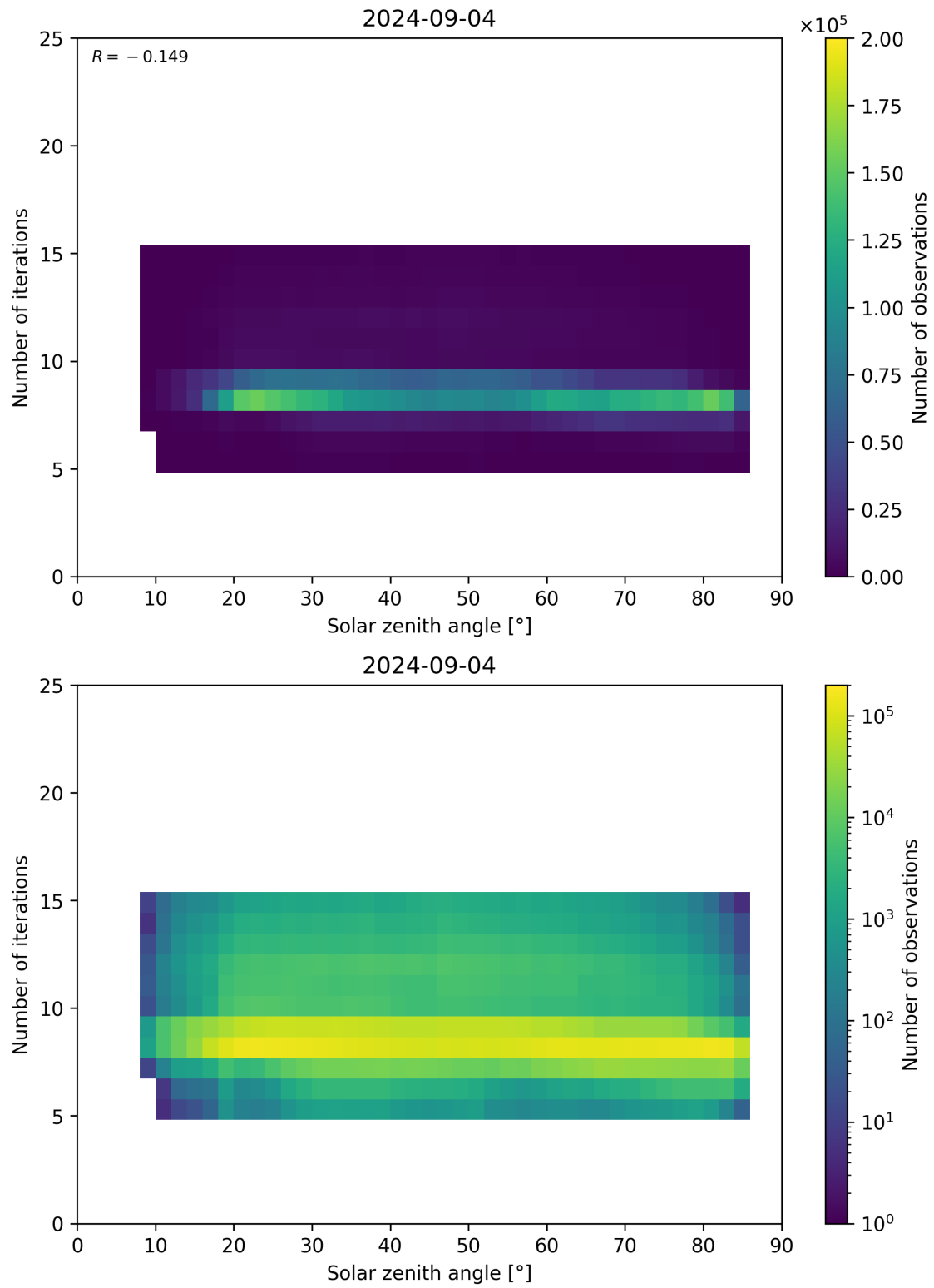
Figure 67: Scatter density plot of “Solar zenith angle” against “Number of iterations” for 2024-09-03 to 2024-09-05.
