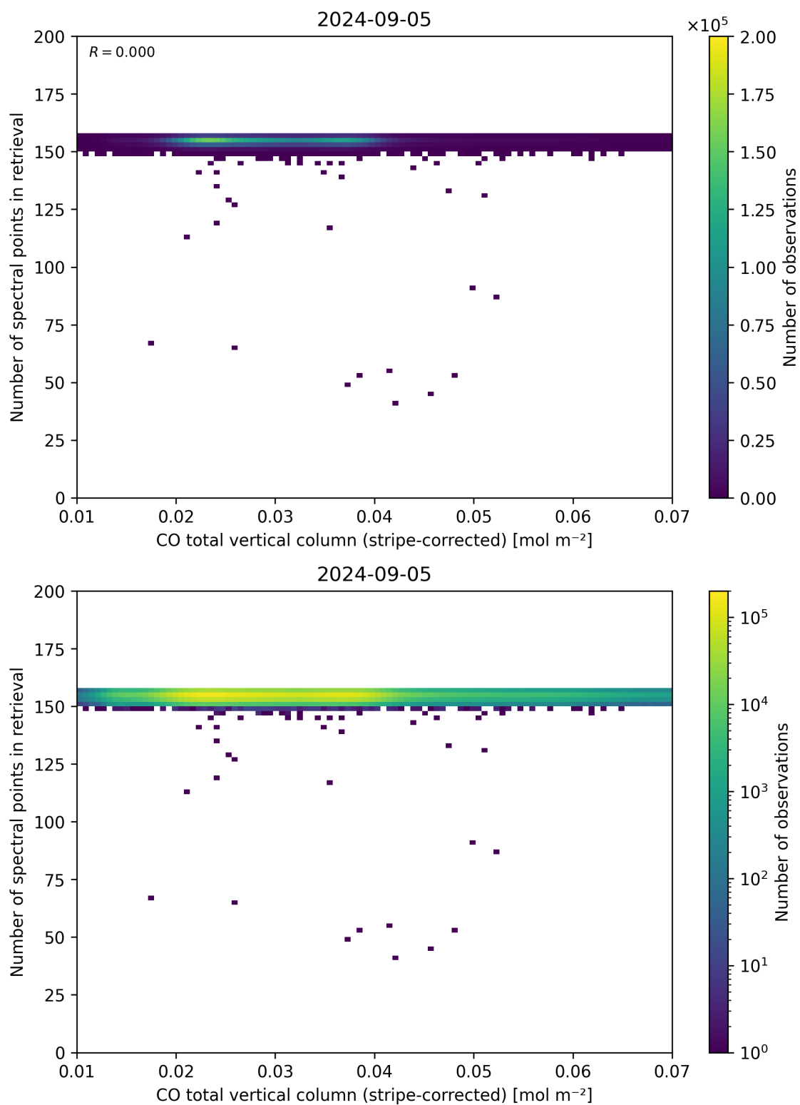
Figure 40: Scatter density plot of “CO total vertical column (stripe-corrected)” against “Number of spectral points in retrieval” for 2024-09-04 to 2024-09-06.
