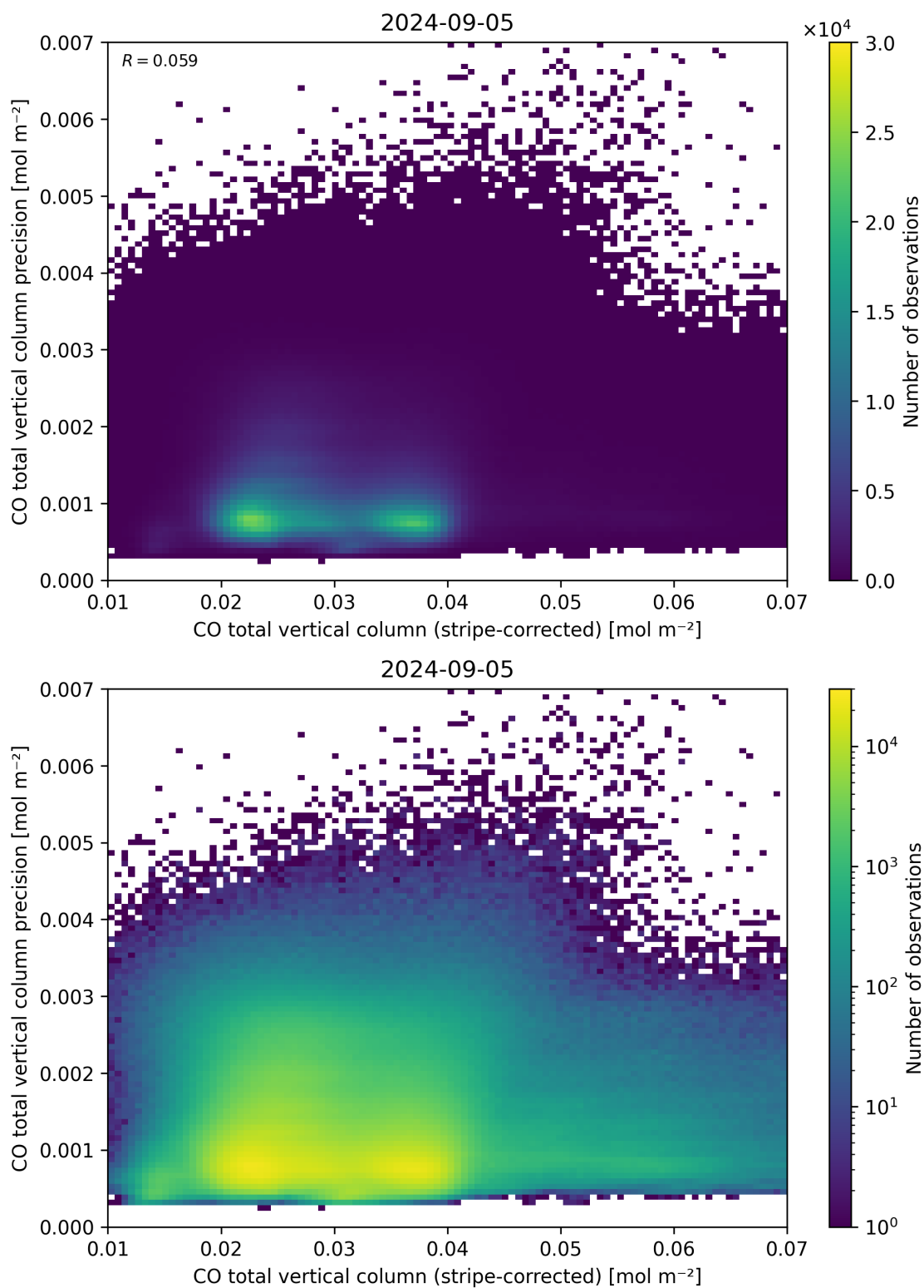
Figure 36: Scatter density plot of “CO total vertical column (stripe-corrected)” against “CO total vertical column precision” for 2024-09-04 to 2024-09-06.
