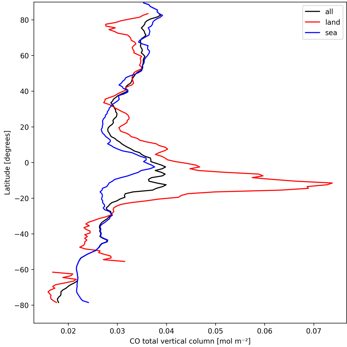
Figure 10: Zonal average of “CO total vertical column” for 2024-09-04 to 2024-09-06.
