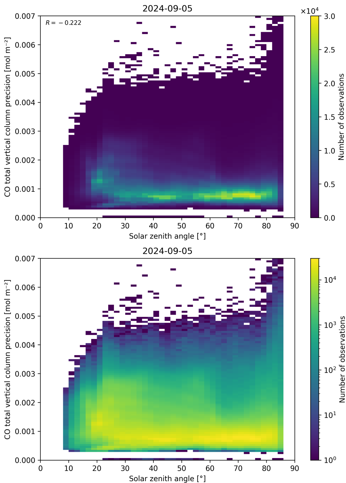
Figure 63: Scatter density plot of “Solar zenith angle” against “CO total vertical column precision” for 2024-09-04 to 2024-09-06.
