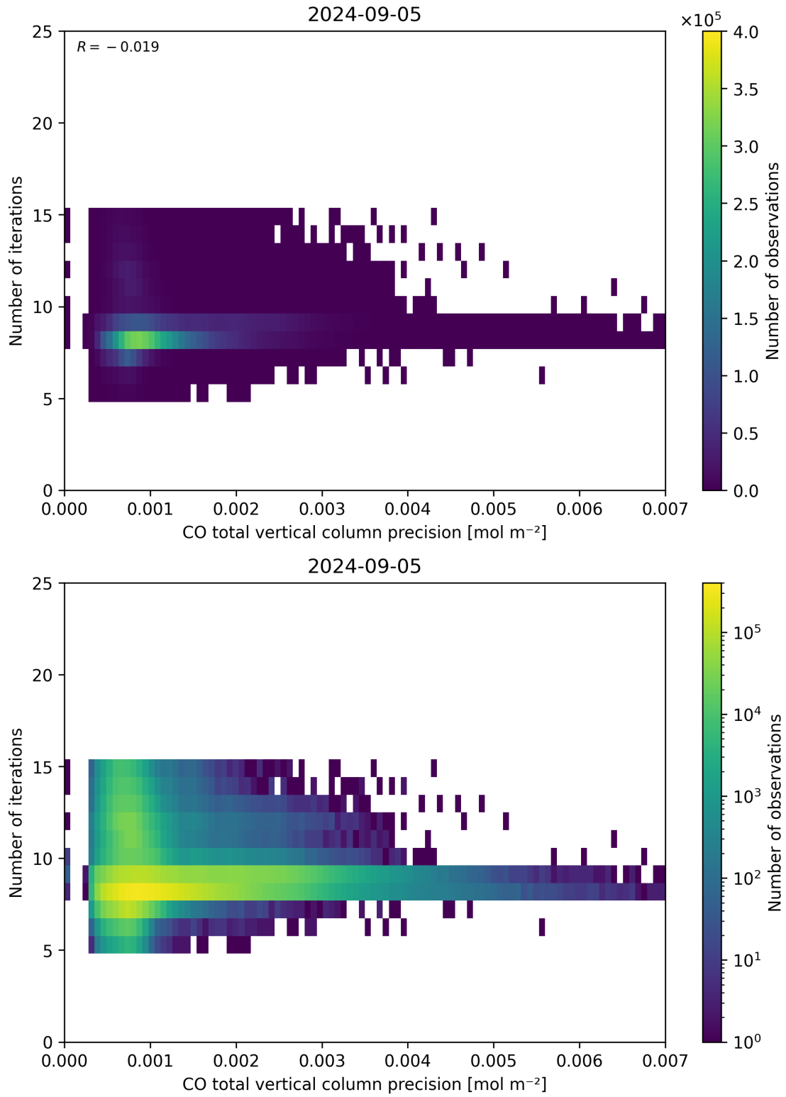
Figure 46: Scatter density plot of “CO total vertical column precision” against “Number of iterations” for 2024-09-04 to 2024-09-06.
