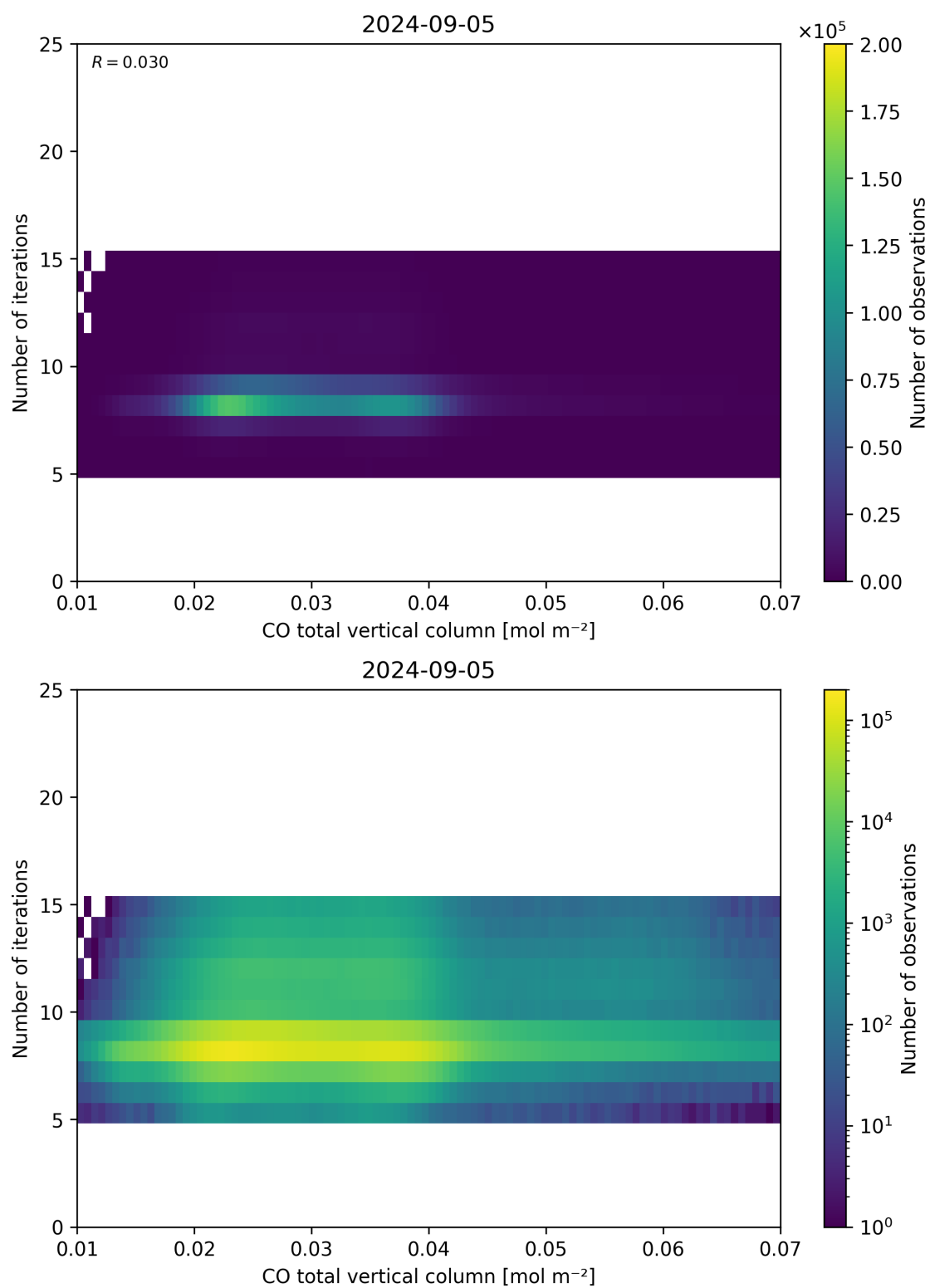
Figure 42: Scatter density plot of “CO total vertical column” against “Number of iterations” for 2024-09-04 to 2024-09-06.
