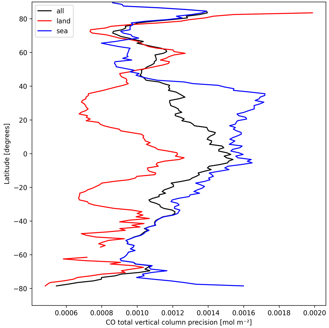
Figure 12: Zonal average of “CO total vertical column precision” for 2024-09-04 to 2024-09-06.
