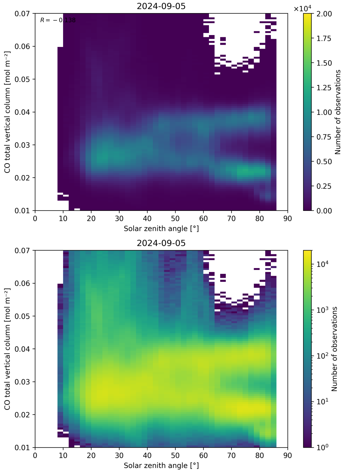
Figure 61: Scatter density plot of “Solar zenith angle” against “CO total vertical column” for 2024-09-04 to 2024-09-06.
