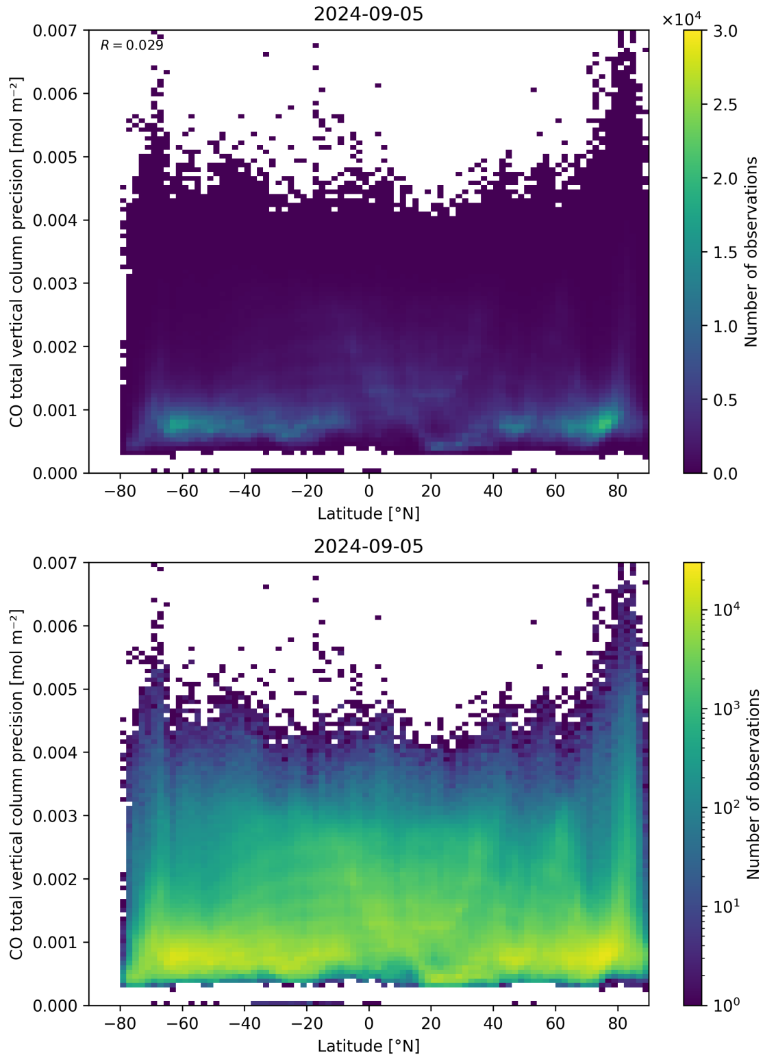
Figure 53: Scatter density plot of “Latitude” against “CO total vertical column precision” for 2024-09-04 to 2024-09-06.
