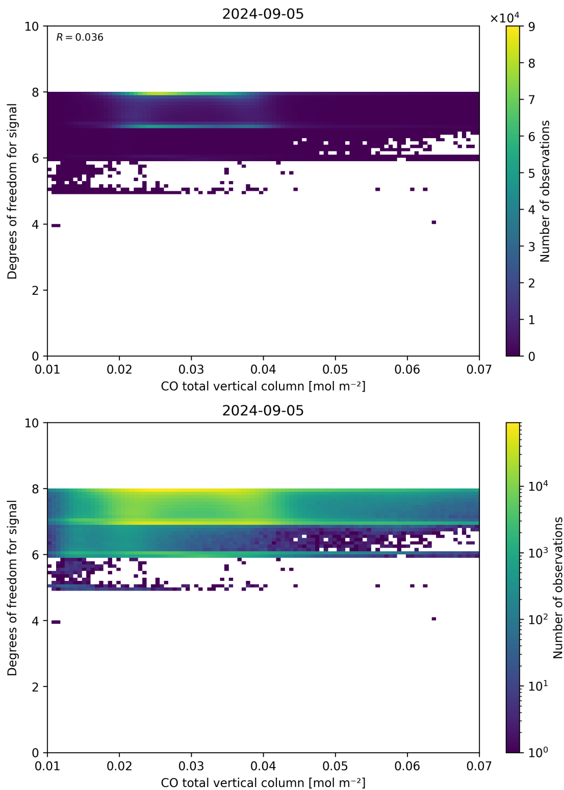
Figure 41: Scatter density plot of “CO total vertical column” against “Degrees of freedom for signal” for 2024-09-04 to 2024-09-06.
