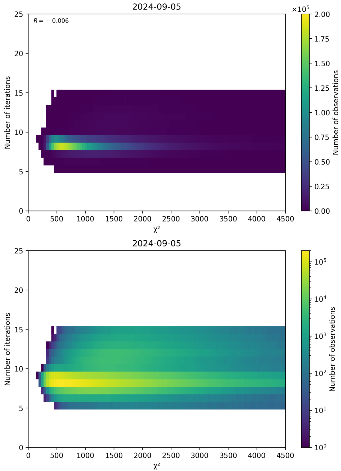
Figure 49: Scatter density plot of “ \chi^2 ” against “Number of iterations” for 2024-09-04 to 2024-09-06.
