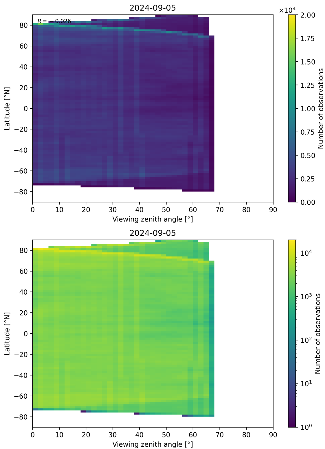
Figure 74: Scatter density plot of “Viewing zenith angle” against “Latitude” for 2024-09-04 to 2024-09-06.
