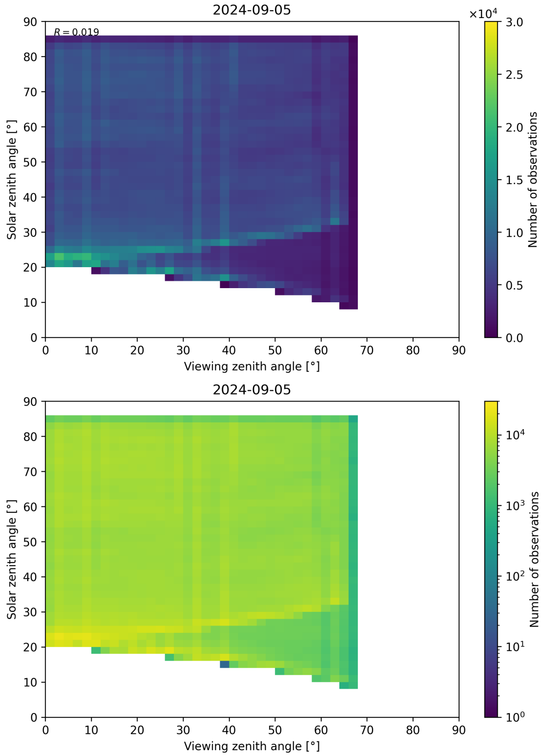
Figure 77: Scatter density plot of “Viewing zenith angle” against “Solar zenith angle” for 2024-09-04 to 2024-09-06.
