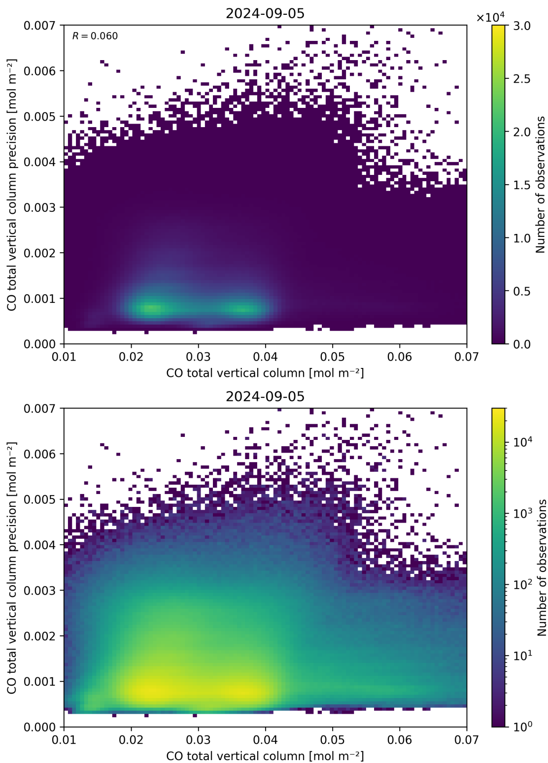
Figure 34: Scatter density plot of “CO total vertical column” against “CO total vertical column precision” for 2024-09-04 to 2024-09-06.
