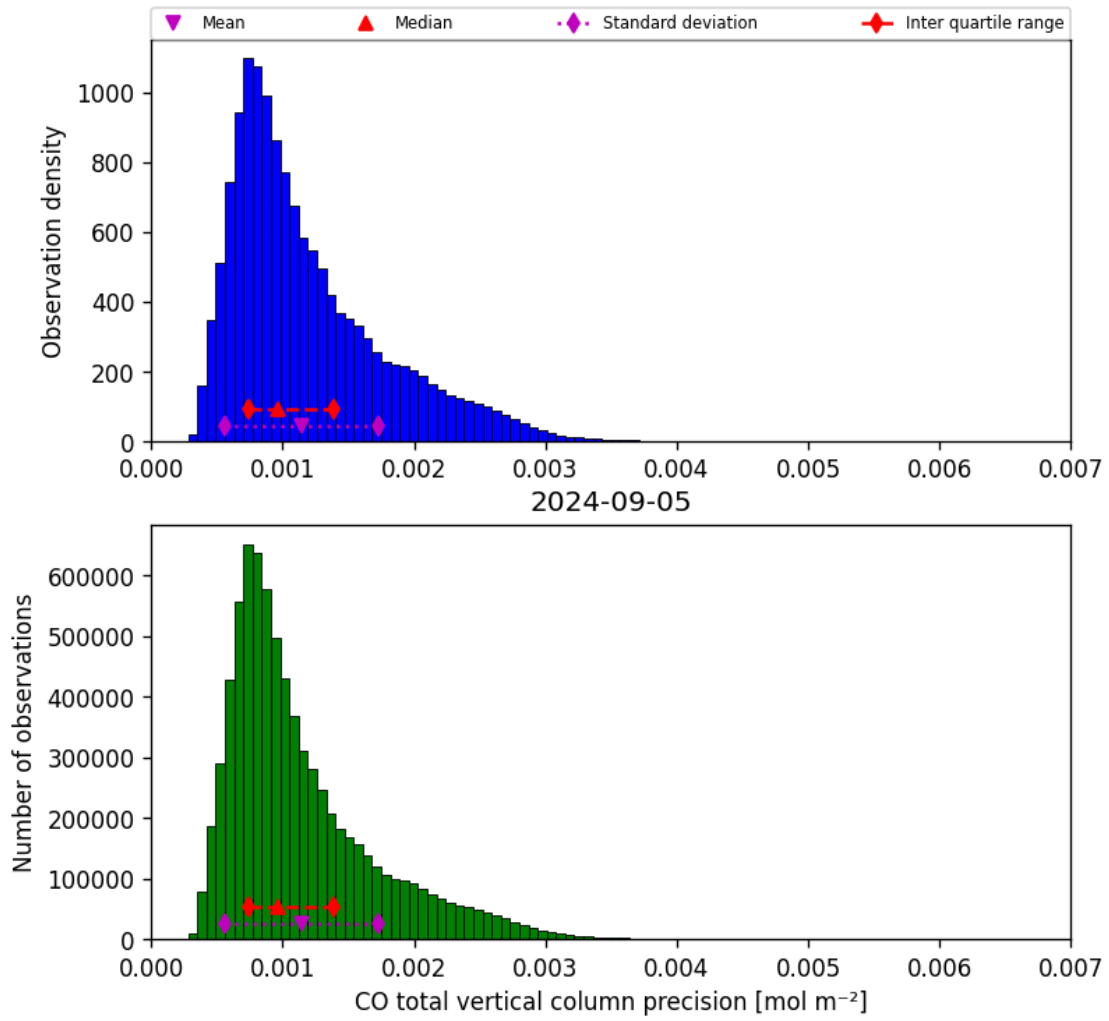
Figure 20: Histogram of “CO total vertical column precision” for 2024-09-04 to 2024-09-06
