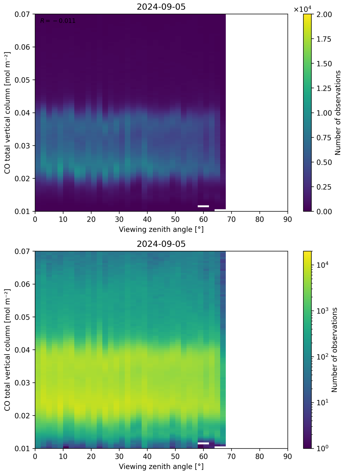
Figure 69: Scatter density plot of “Viewing zenith angle” against “CO total vertical column” for 2024-09-04 to 2024-09-06.
