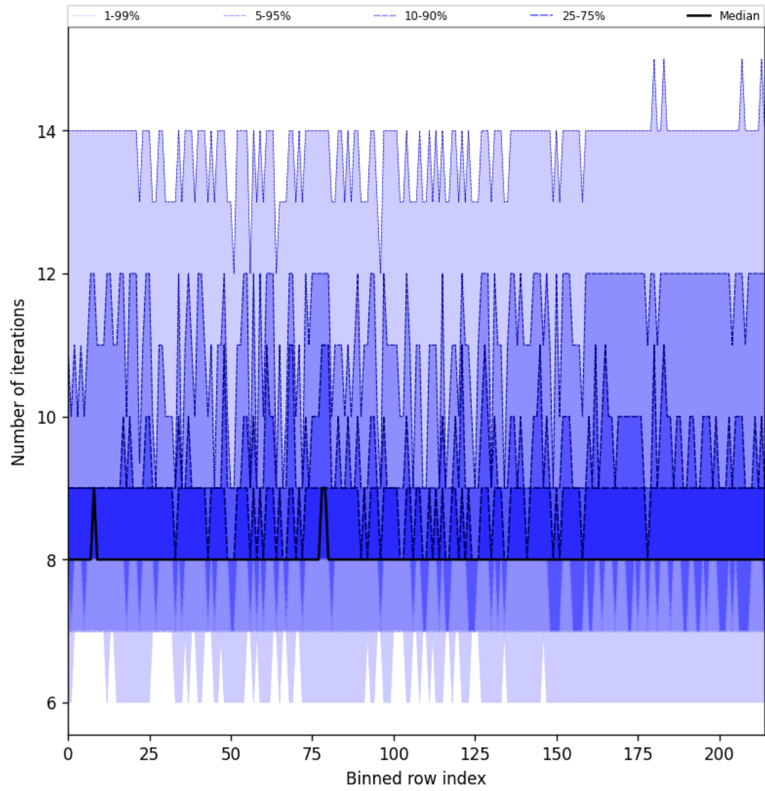
Figure 32: Along track statistics of “Number of iterations” for 2024-09-04 to 2024-09-06
