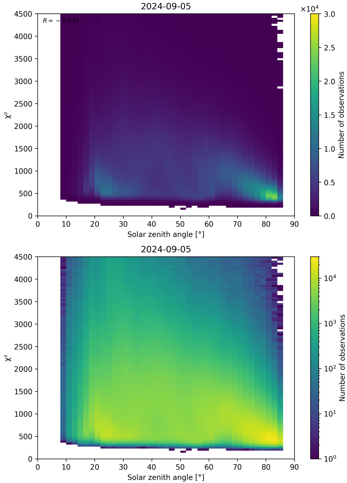
Figure 64: Scatter density plot of “Solar zenith angle” against “ \chi^2 ” for 2024-09-04 to 2024-09-06.
