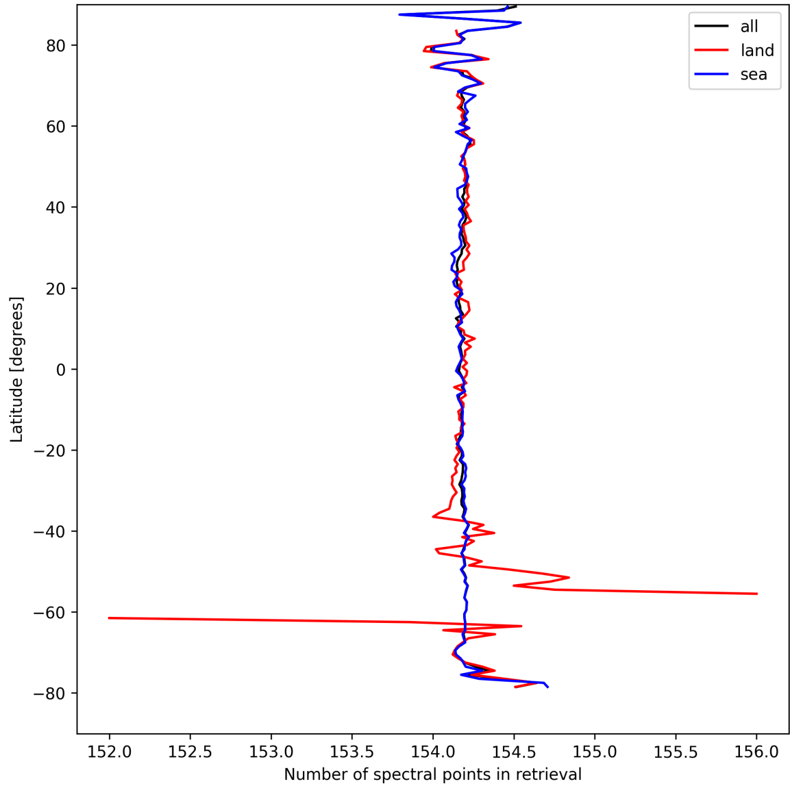
Figure 13: Zonal average of “Number of spectral points in retrieval” for 2024-09-04 to 2024-09-06.
