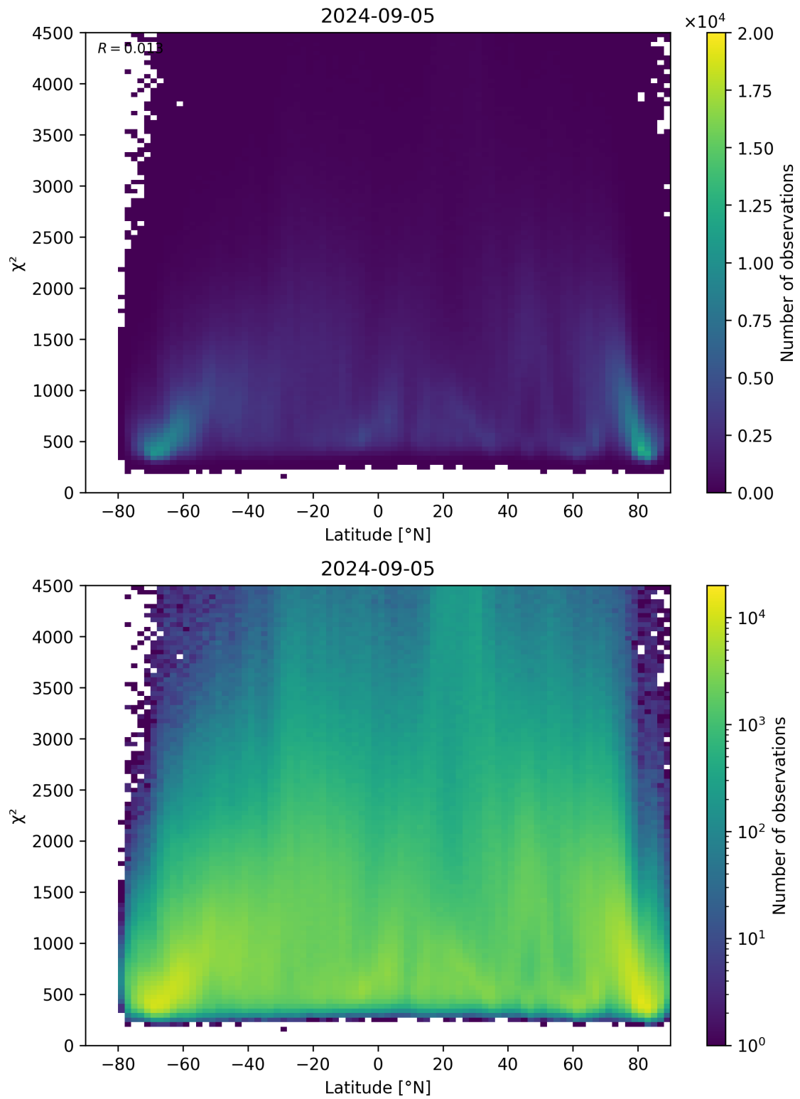
Figure 54: Scatter density plot of “Latitude” against “ \chi^2 ” for 2024-09-04 to 2024-09-06.
