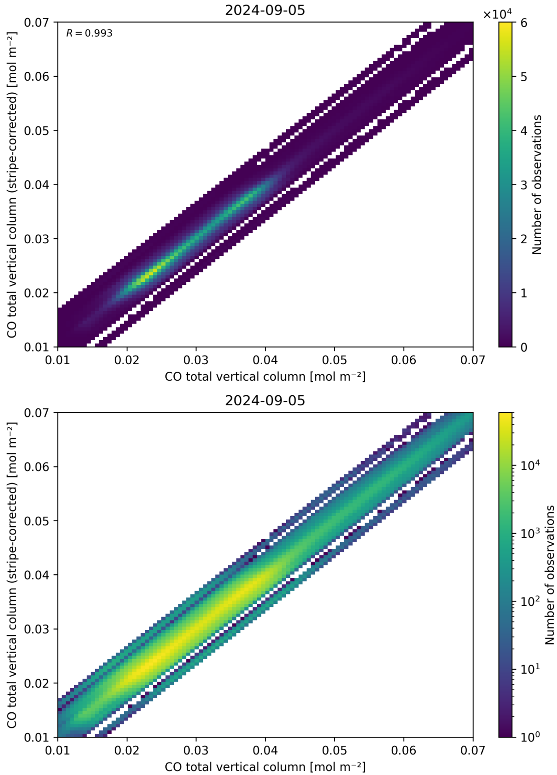
Figure 33: Scatter density plot of “CO total vertical column” against “CO total vertical column (stripe-corrected)” for 2024-09-04 to 2024-09-06.
