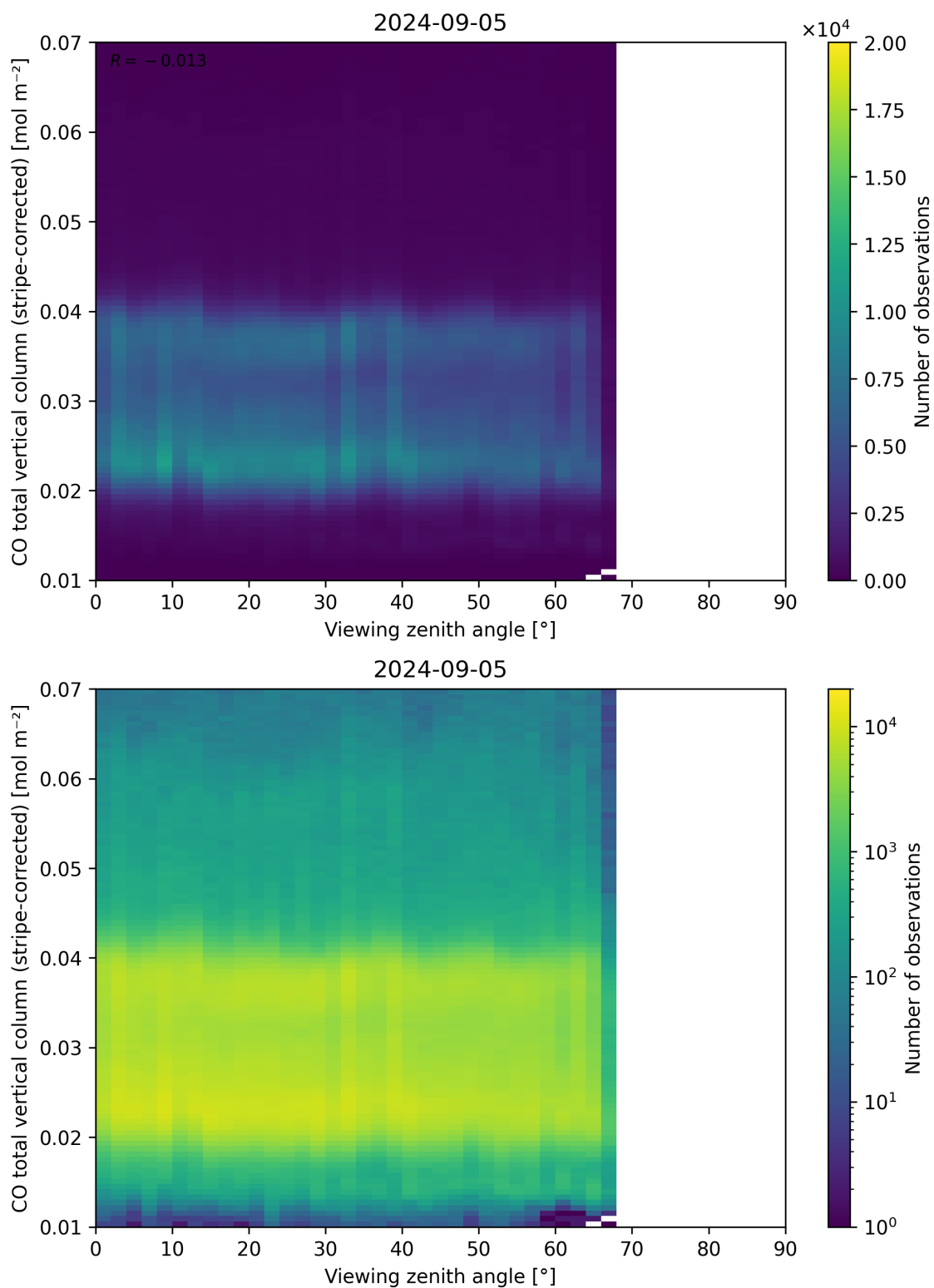
Figure 70: Scatter density plot of “Viewing zenith angle” against “CO total vertical column (stripe-corrected)” for 2024-09-04 to 2024-09-06.
