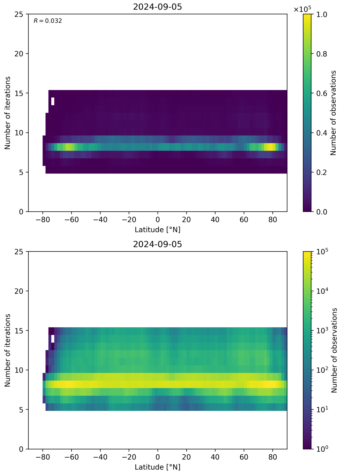
Figure 56: Scatter density plot of “Latitude” against “Number of iterations” for 2024-09-04 to 2024-09-06.
