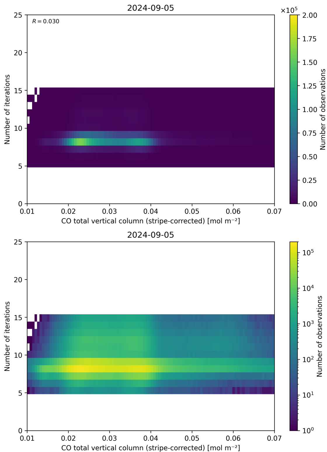
Figure 39: Scatter density plot of “CO total vertical column (stripe-corrected)” against “Number of iterations” for 2024-09-04 to 2024-09-06.
