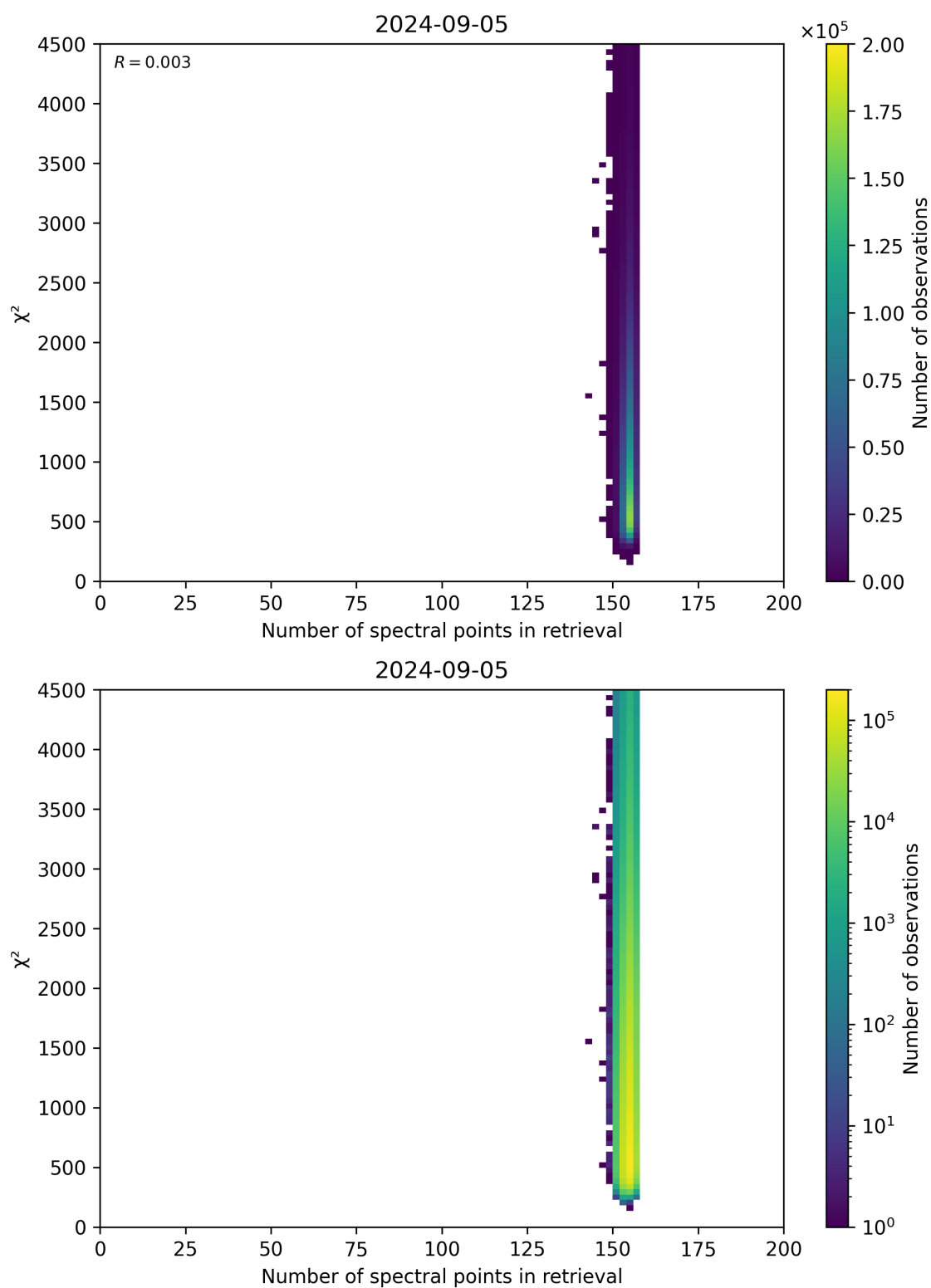
Figure 58: Scatter density plot of “Number of spectral points in retrieval” against “ \chi^2 ” for 2024-09-04 to 2024-09-06.
