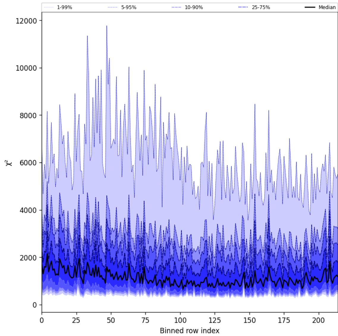
Figure 30: Along track statistics of “ \chi^2 ” for 2024-09-04 to 2024-09-06
