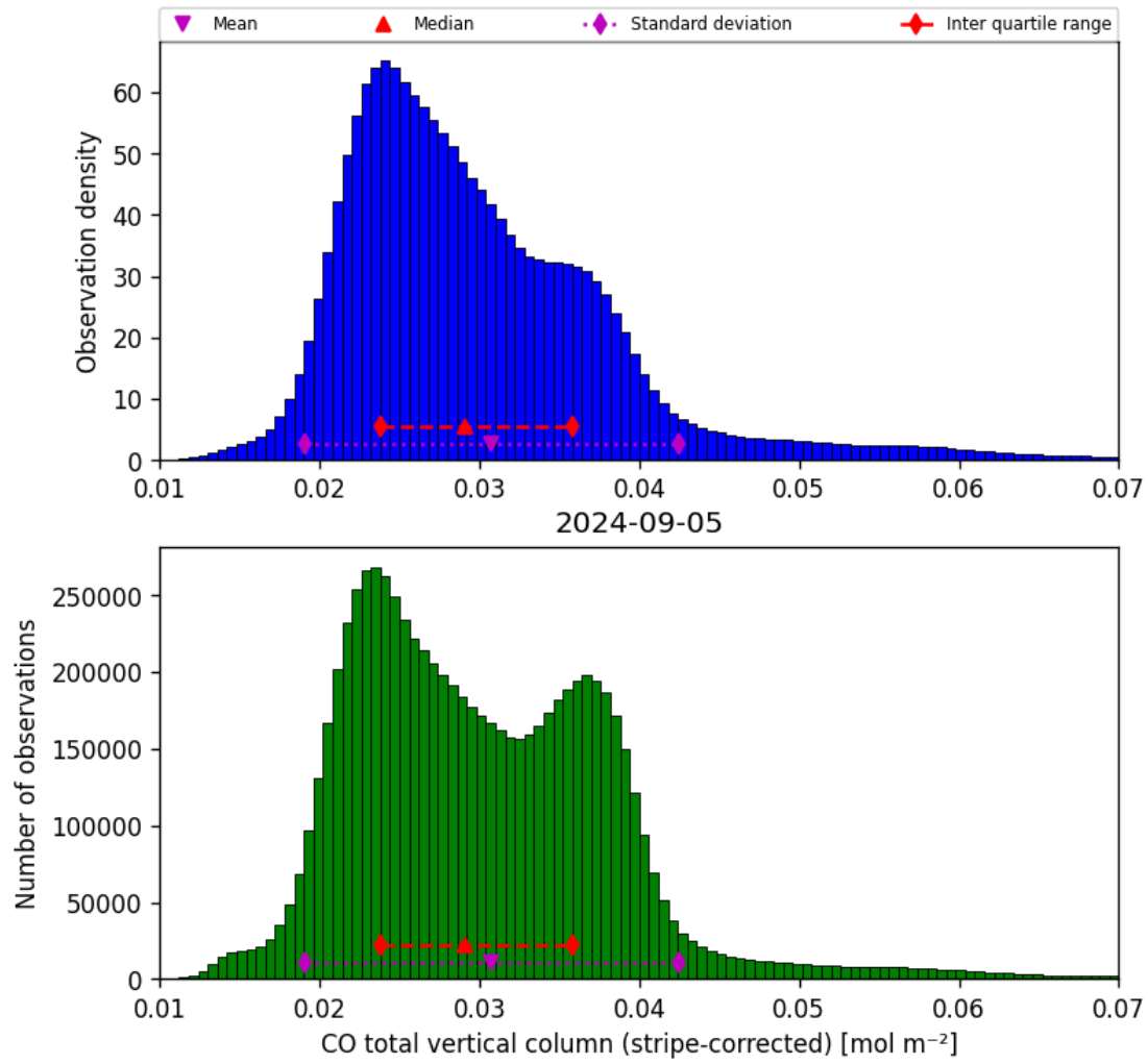
Figure 19: Histogram of “CO total vertical column (stripe-corrected)” for 2024-09-04 to 2024-09-06
