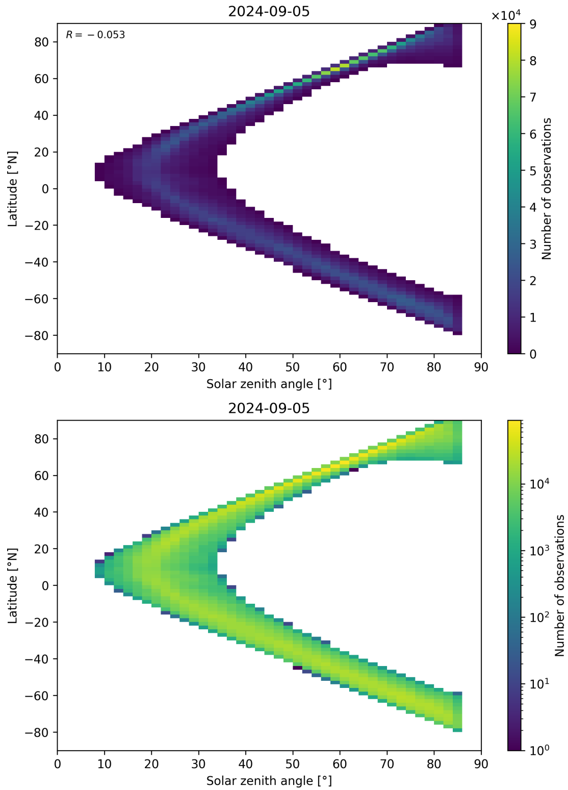
Figure 66: Scatter density plot of “Solar zenith angle” against “Latitude” for 2024-09-04 to 2024-09-06.
