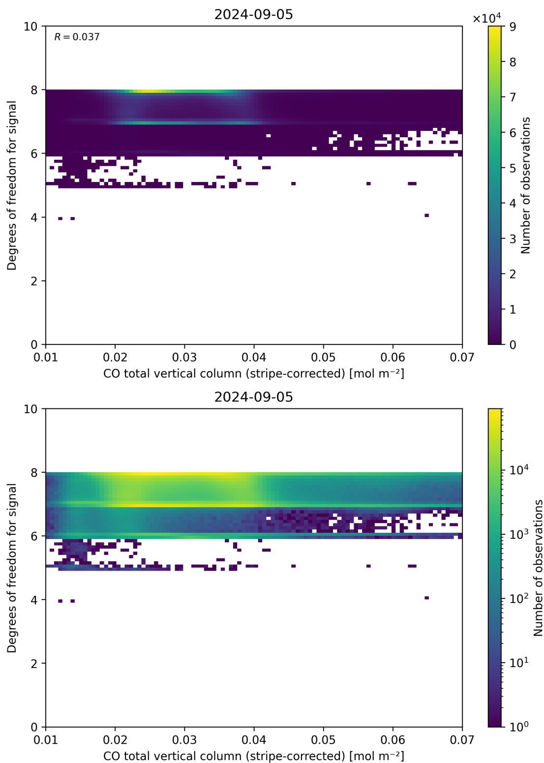
Figure 38: Scatter density plot of “CO total vertical column (stripe-corrected)” against “Degrees of freedom for signal” for 2024-09-04 to 2024-09-06.
