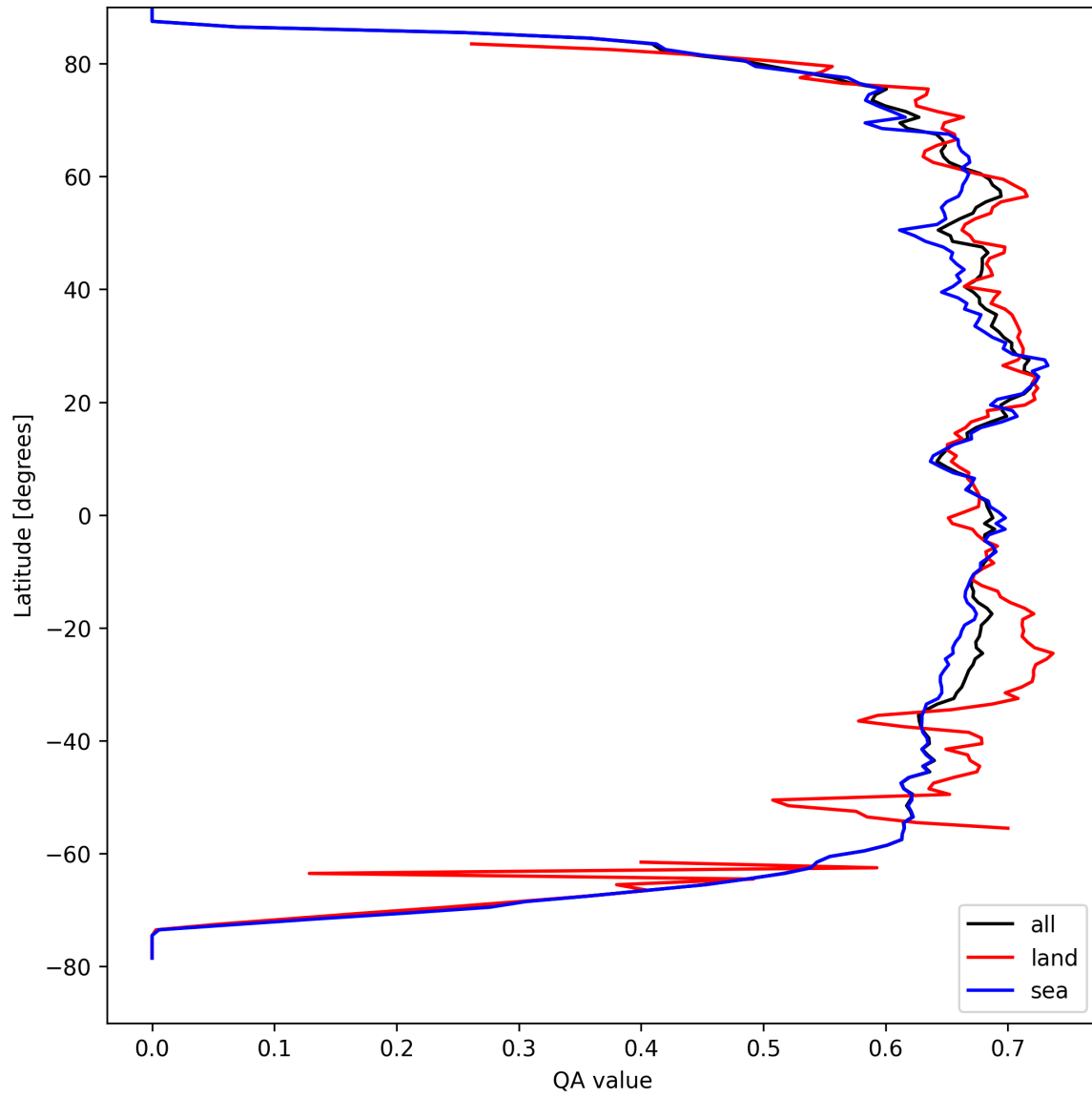
Figure 9: Zonal average of “QA value” for 2024-09-04 to 2024-09-06.
