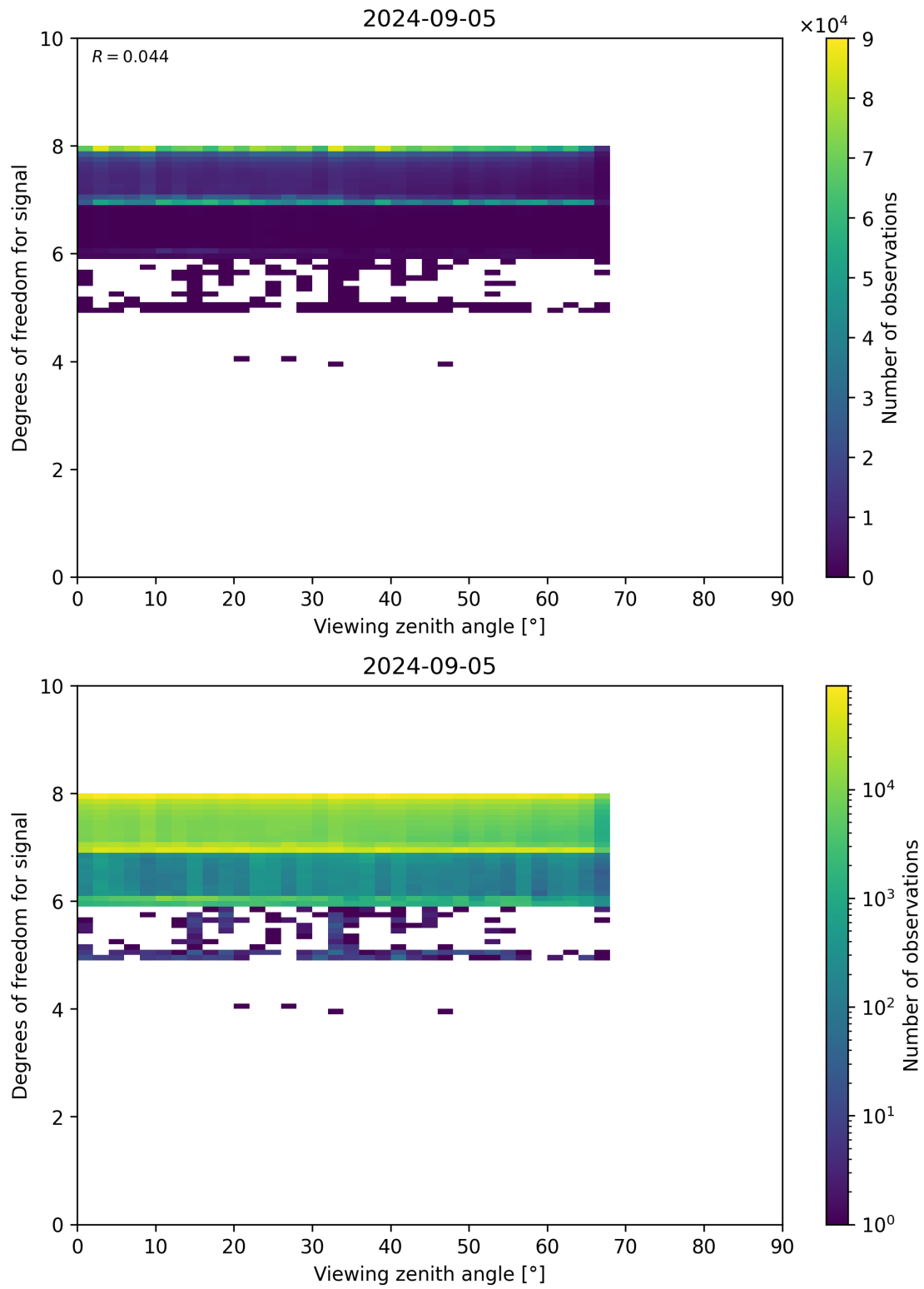
Figure 73: Scatter density plot of “Viewing zenith angle” against “Degrees of freedom for signal” for 2024-09-04 to 2024-09-06.
