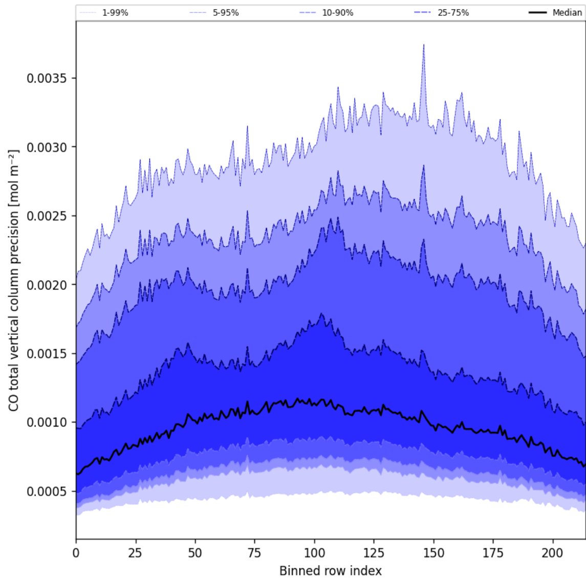
Figure 28: Along track statistics of “CO total vertical column precision” for 2024-09-04 to 2024-09-06
