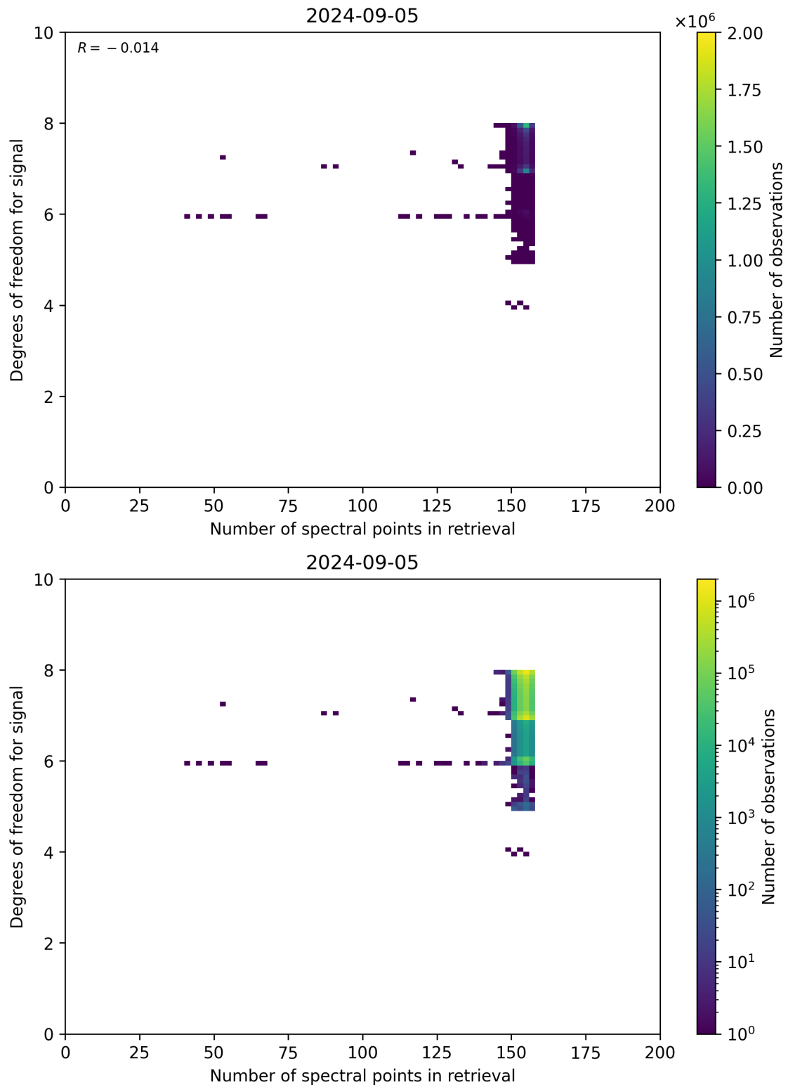
Figure 59: Scatter density plot of “Number of spectral points in retrieval” against “Degrees of freedom for signal” for 2024-09-04 to 2024-09-06.
