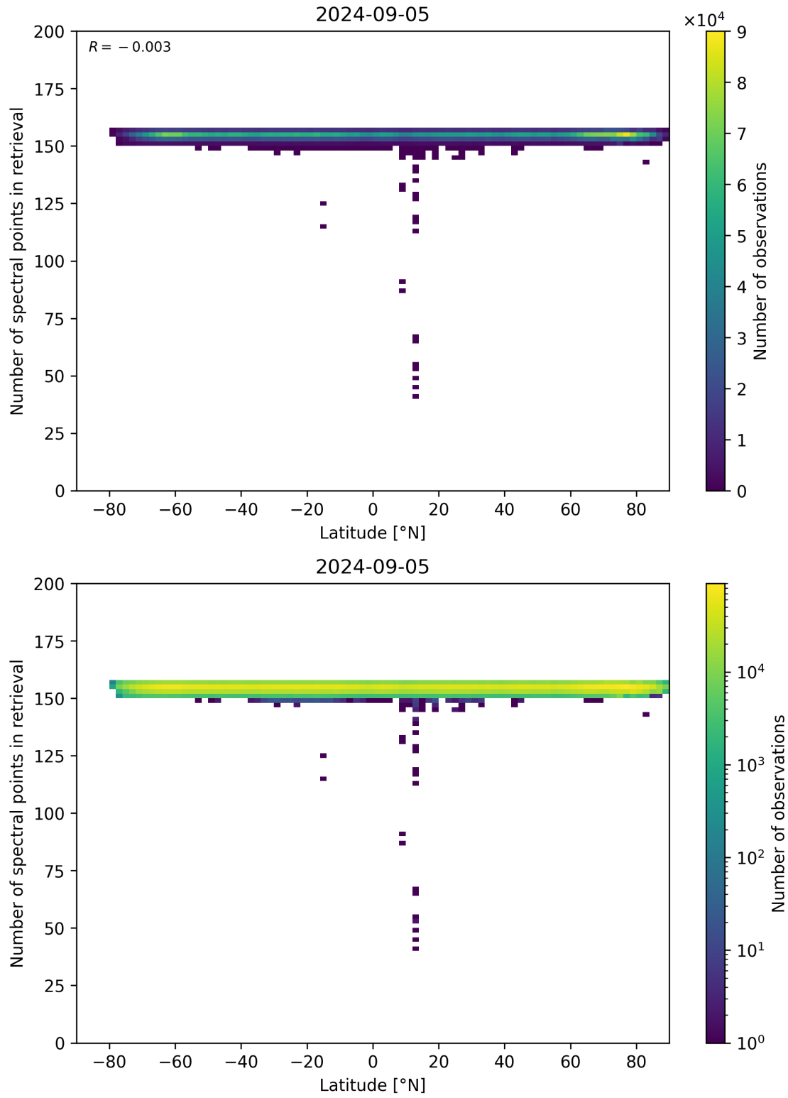
Figure 57: Scatter density plot of “Latitude” against “Number of spectral points in retrieval” for 2024-09-04 to 2024-09-06.
