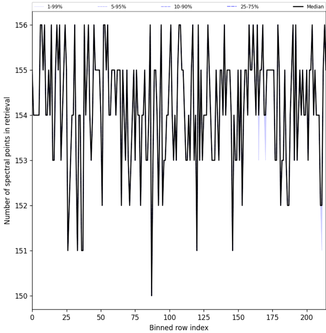
Figure 29: Along track statistics of “Number of spectral points in retrieval” for 2024-09-04 to 2024-09-06
