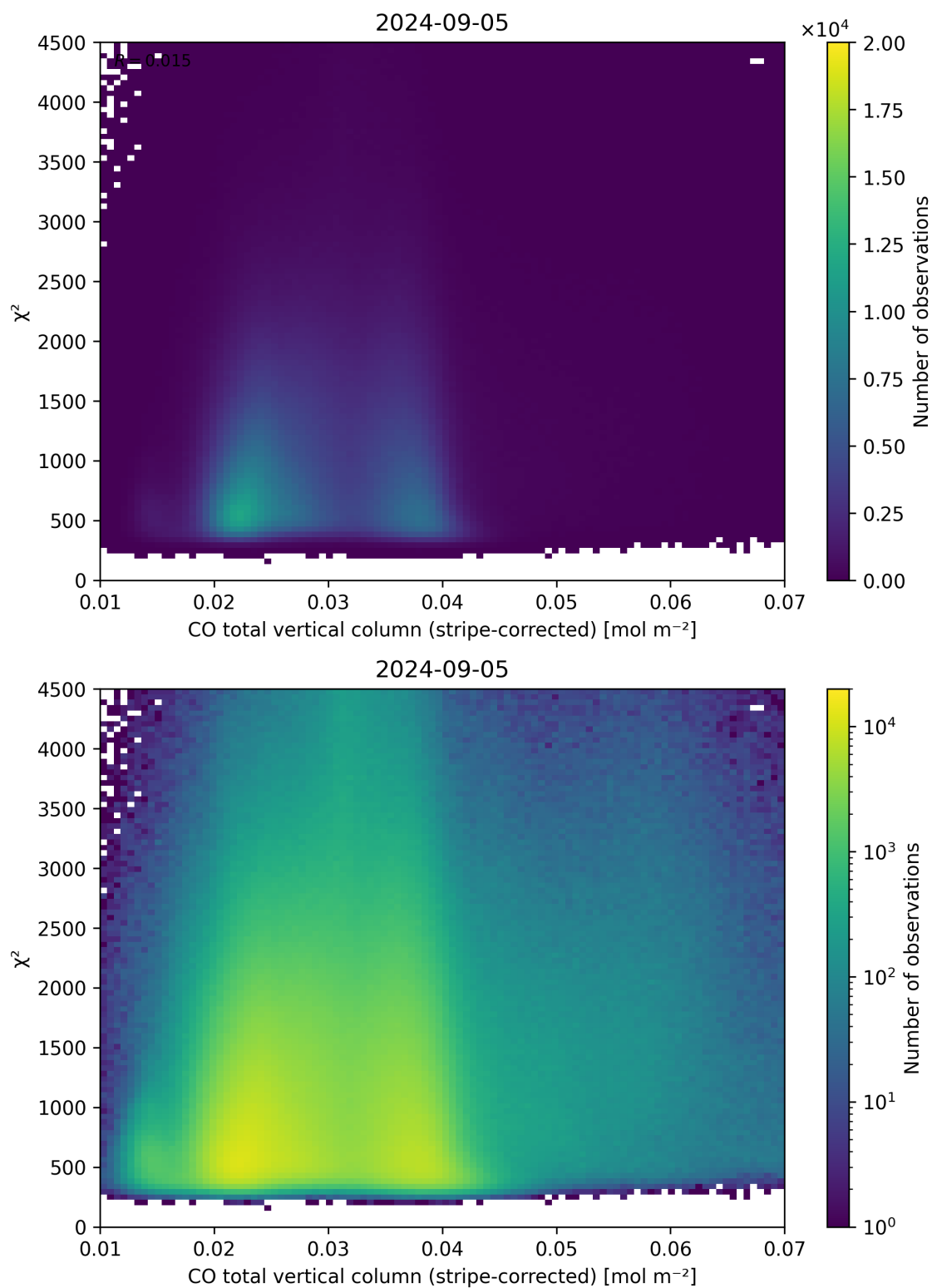
Figure 37: Scatter density plot of “CO total vertical column (stripe-corrected)” against “ \chi^2 ” for 2024-09-04 to 2024-09-06.
