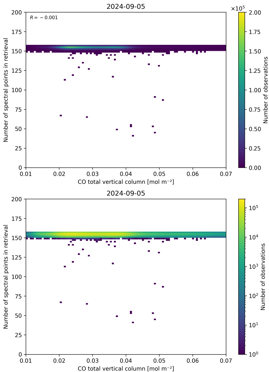
Figure 43: Scatter density plot of “CO total vertical column” against “Number of spectral points in retrieval” for 2024-09-04 to 2024-09-06.
