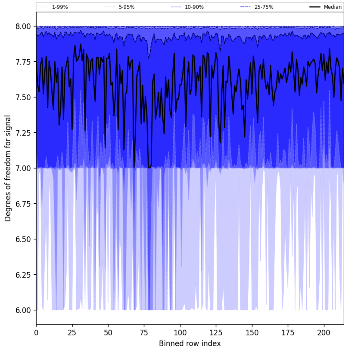
Figure 31: Along track statistics of “Degrees of freedom for signal” for 2024-09-04 to 2024-09-06
