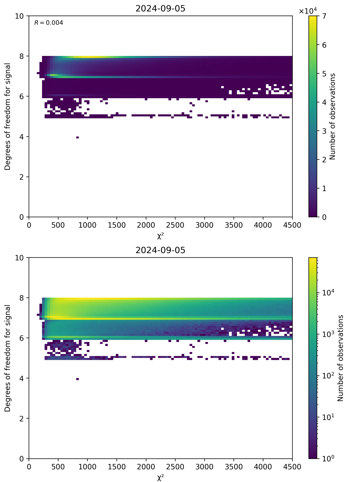
Figure 48: Scatter density plot of “ \chi^2 ” against “Degrees of freedom for signal” for 2024-09-04 to 2024-09-06.
