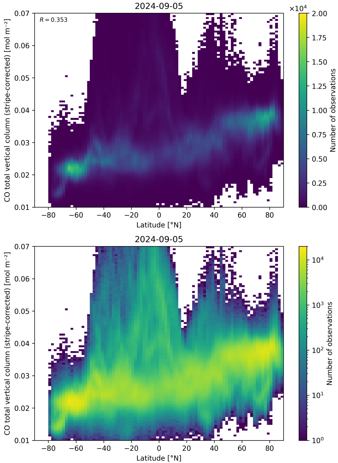
Figure 52: Scatter density plot of “Latitude” against “CO total vertical column (stripe-corrected)” for 2024-09-04 to 2024-09-06.
