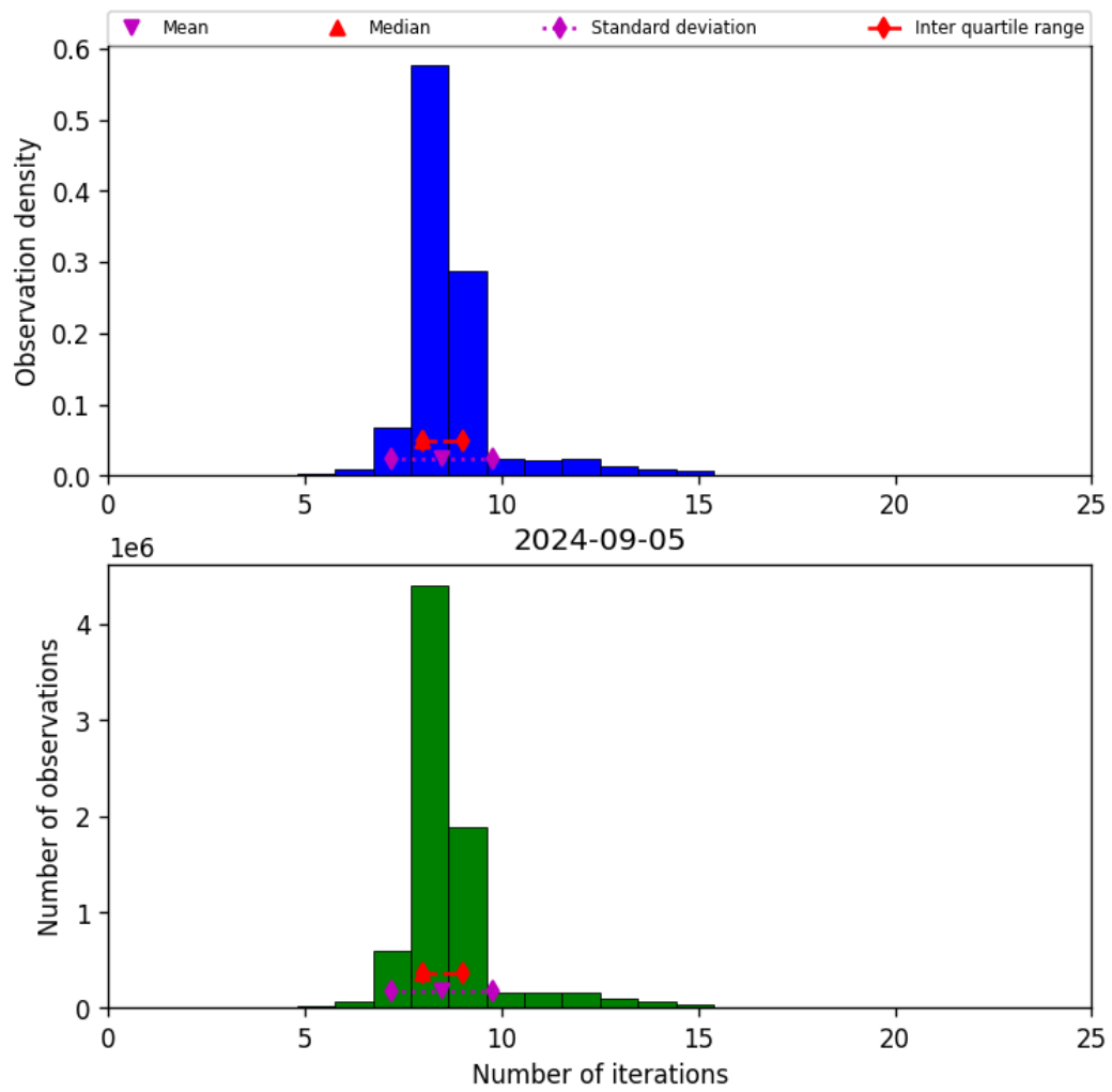
Figure 24: Histogram of “Number of iterations” for 2024-09-04 to 2024-09-06
