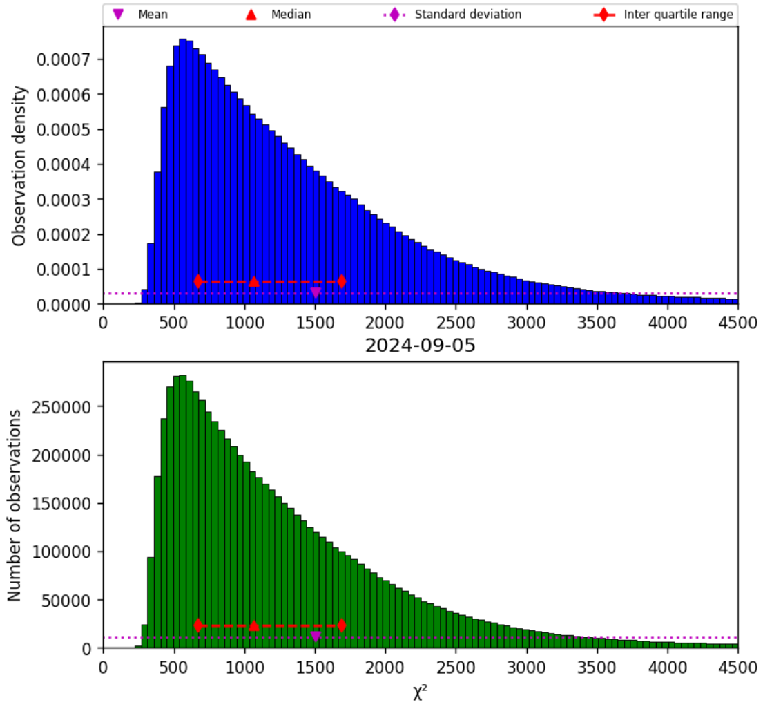
Figure 22: Histogram of " \chi^2 " for 2024-09-04 to 2024-09-06
