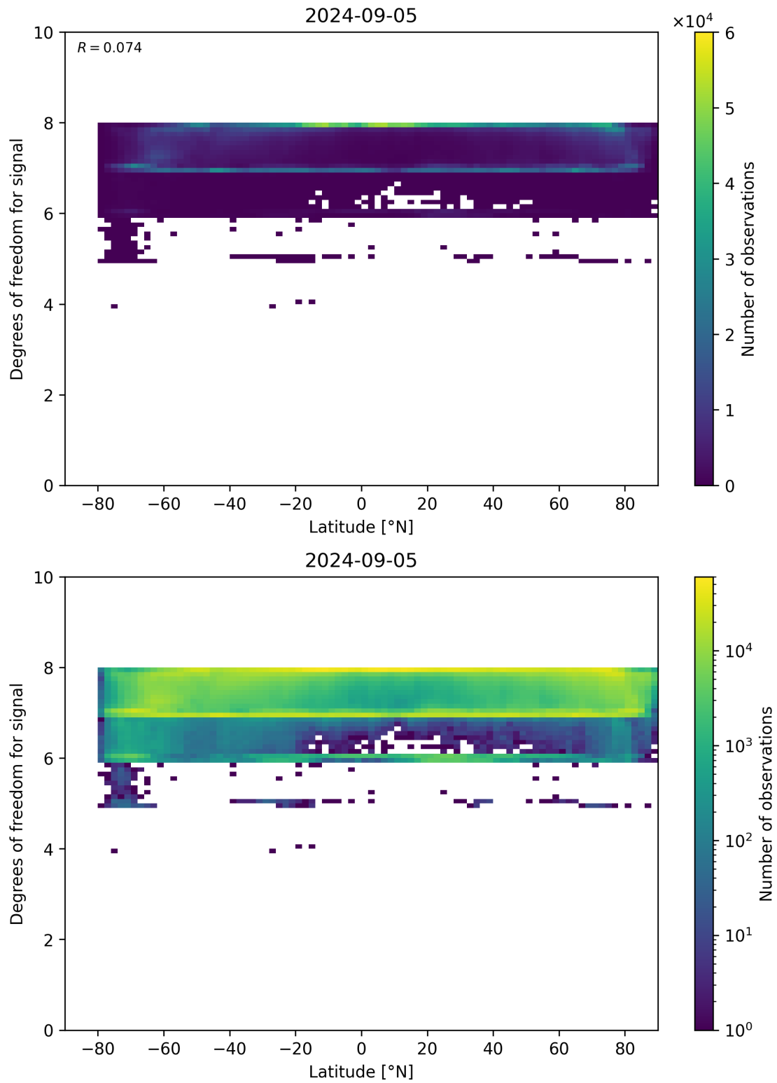
Figure 55: Scatter density plot of “Latitude” against “Degrees of freedom for signal” for 2024-09-04 to 2024-09-06.
