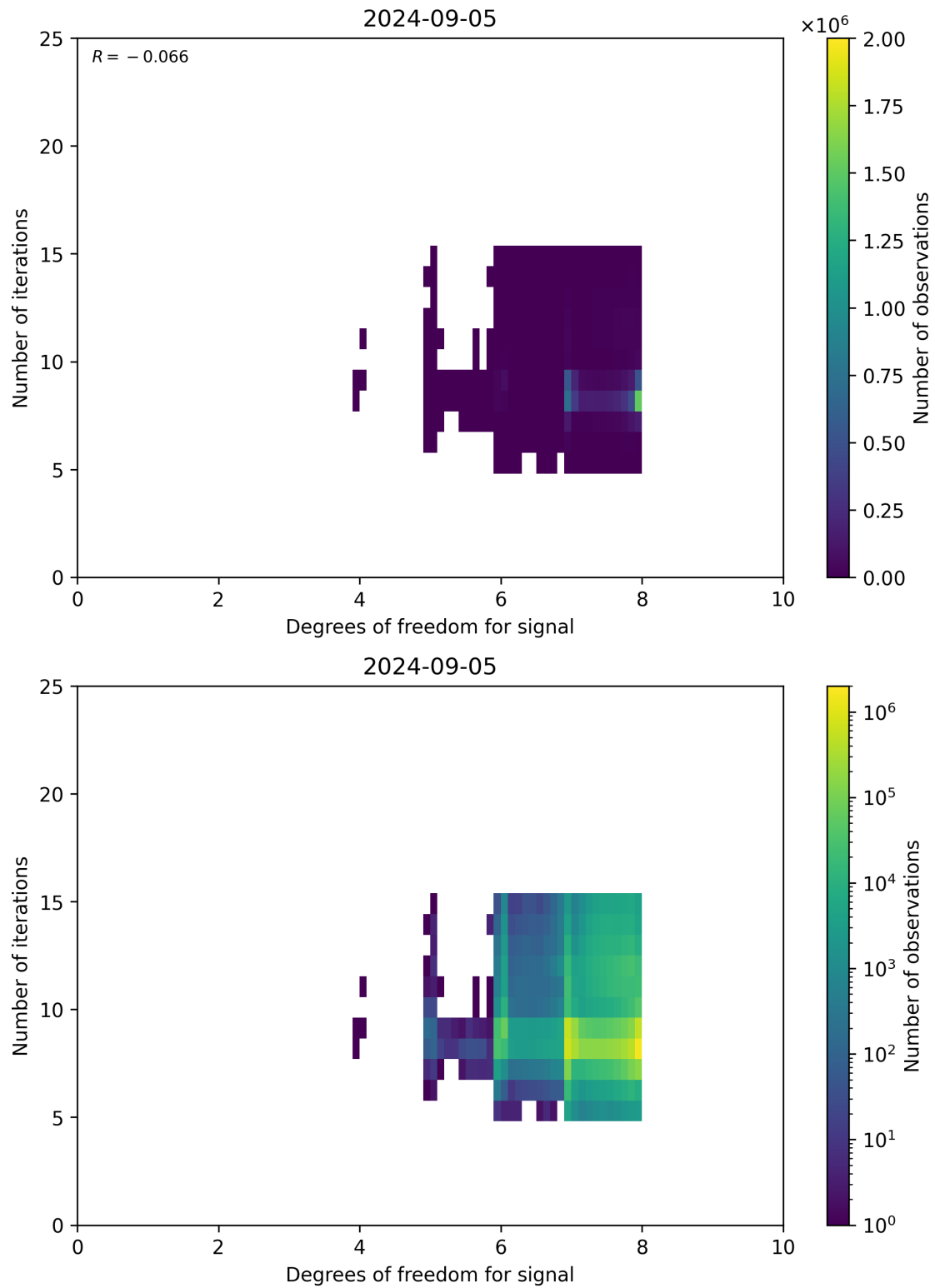
Figure 50: Scatter density plot of “Degrees of freedom for signal” against “Number of iterations” for 2024-09-04 to 2024-09-06.
