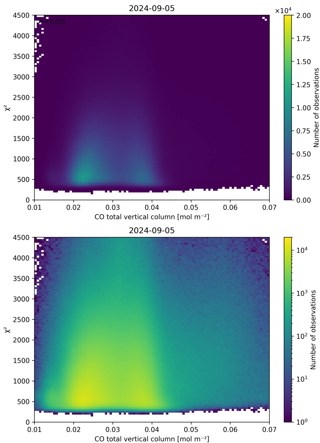
Figure 35: Scatter density plot of “CO total vertical column” against “ \chi^2 ” for 2024-09-04 to 2024-09-06.
