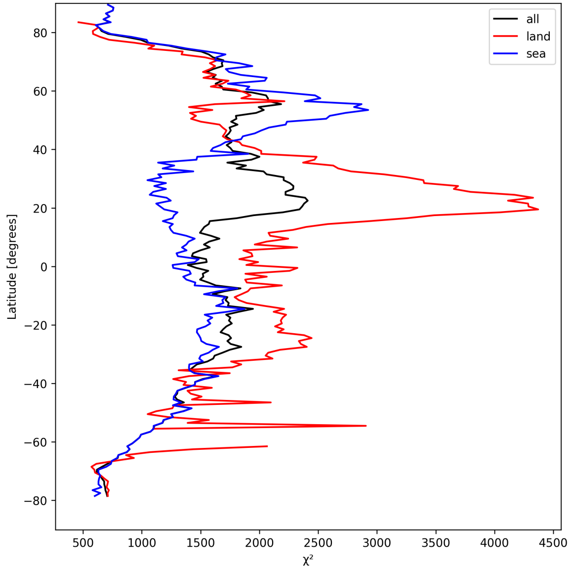
Figure 14: Zonal average of “ \chi^2 ” for 2024-09-04 to 2024-09-06.
