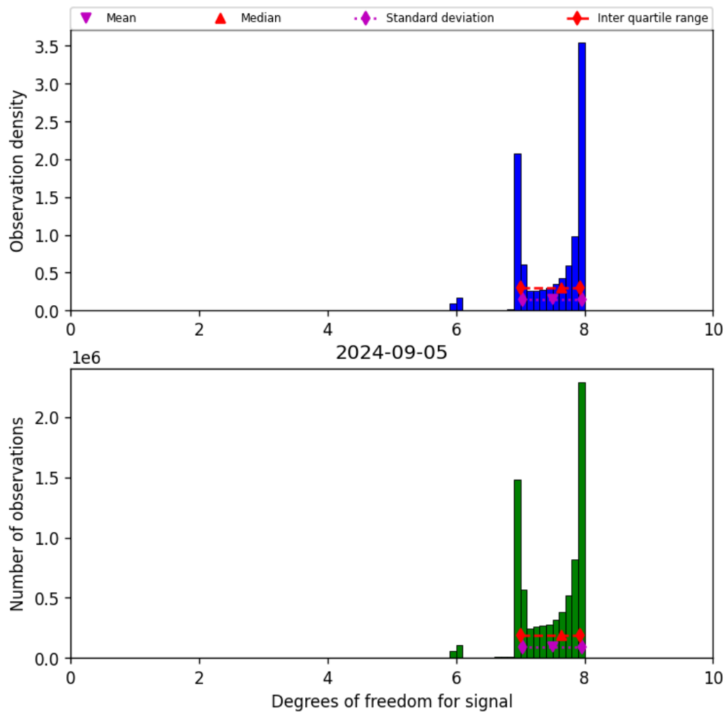
Figure 23: Histogram of “Degrees of freedom for signal” for 2024-09-04 to 2024-09-06
