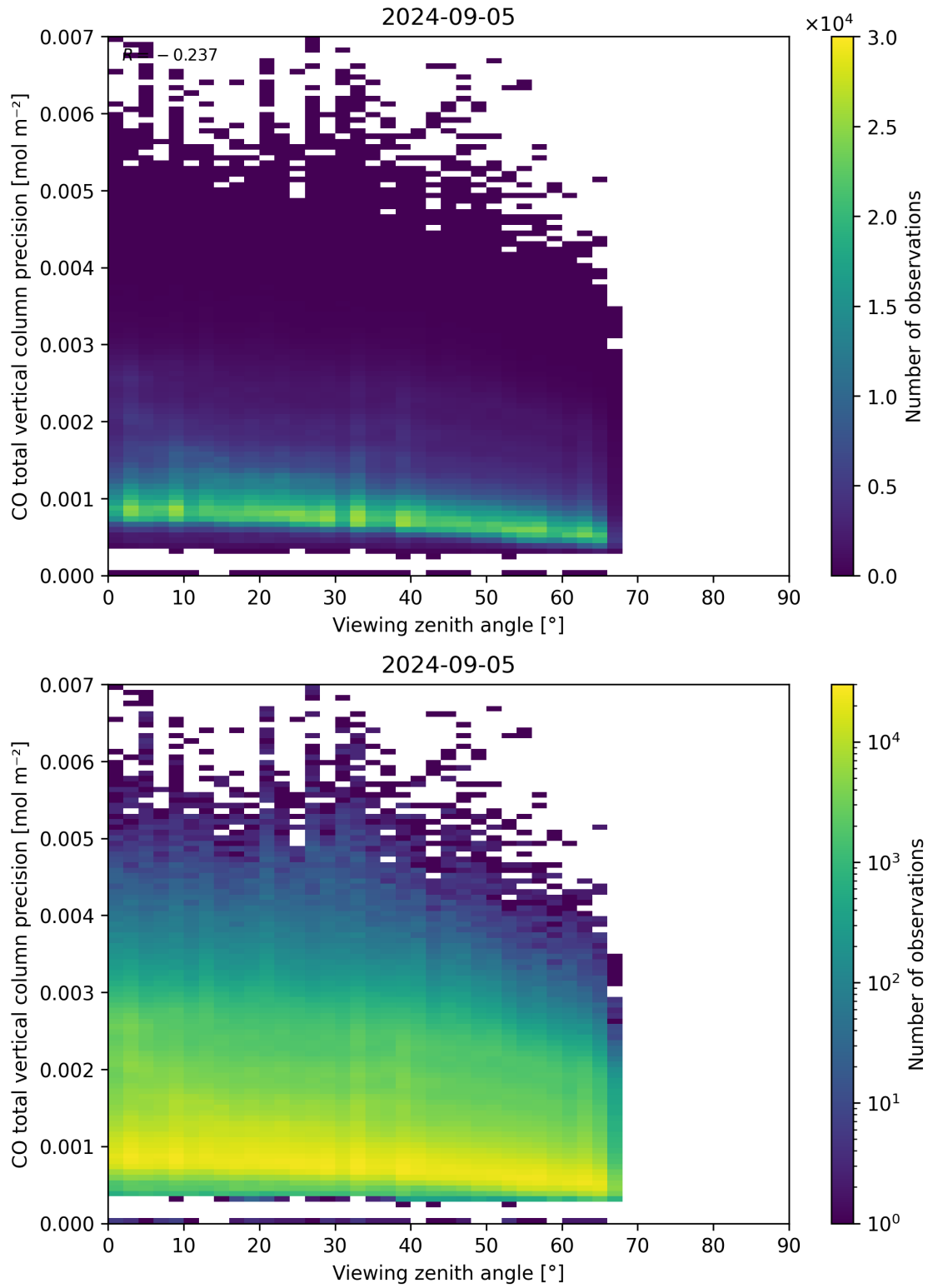
Figure 71: Scatter density plot of “Viewing zenith angle” against “CO total vertical column precision” for 2024-09-04 to 2024-09-06.
