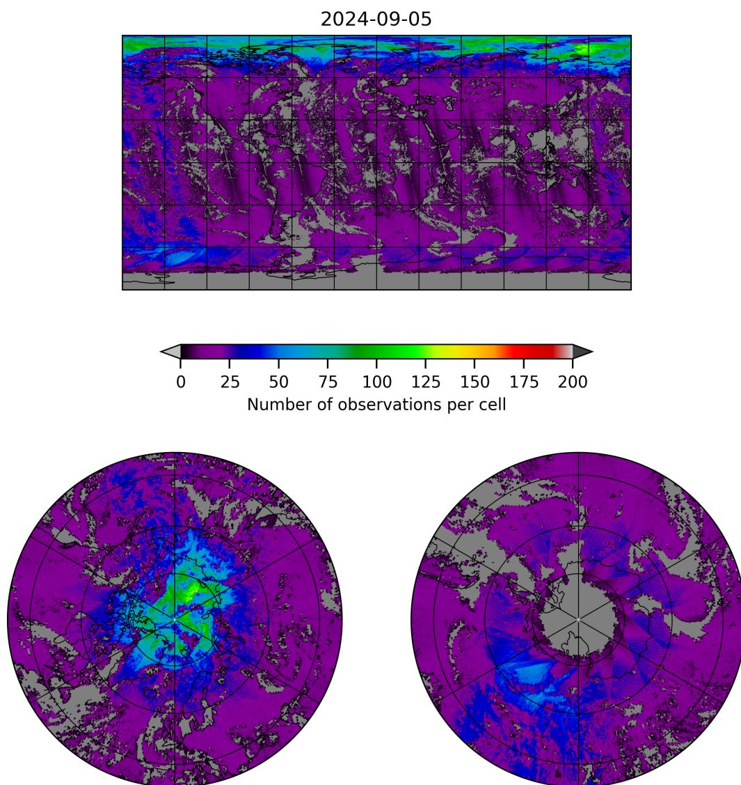
Figure 8: Map of the number of observations for 2024-09-04 to 2024-09-06
