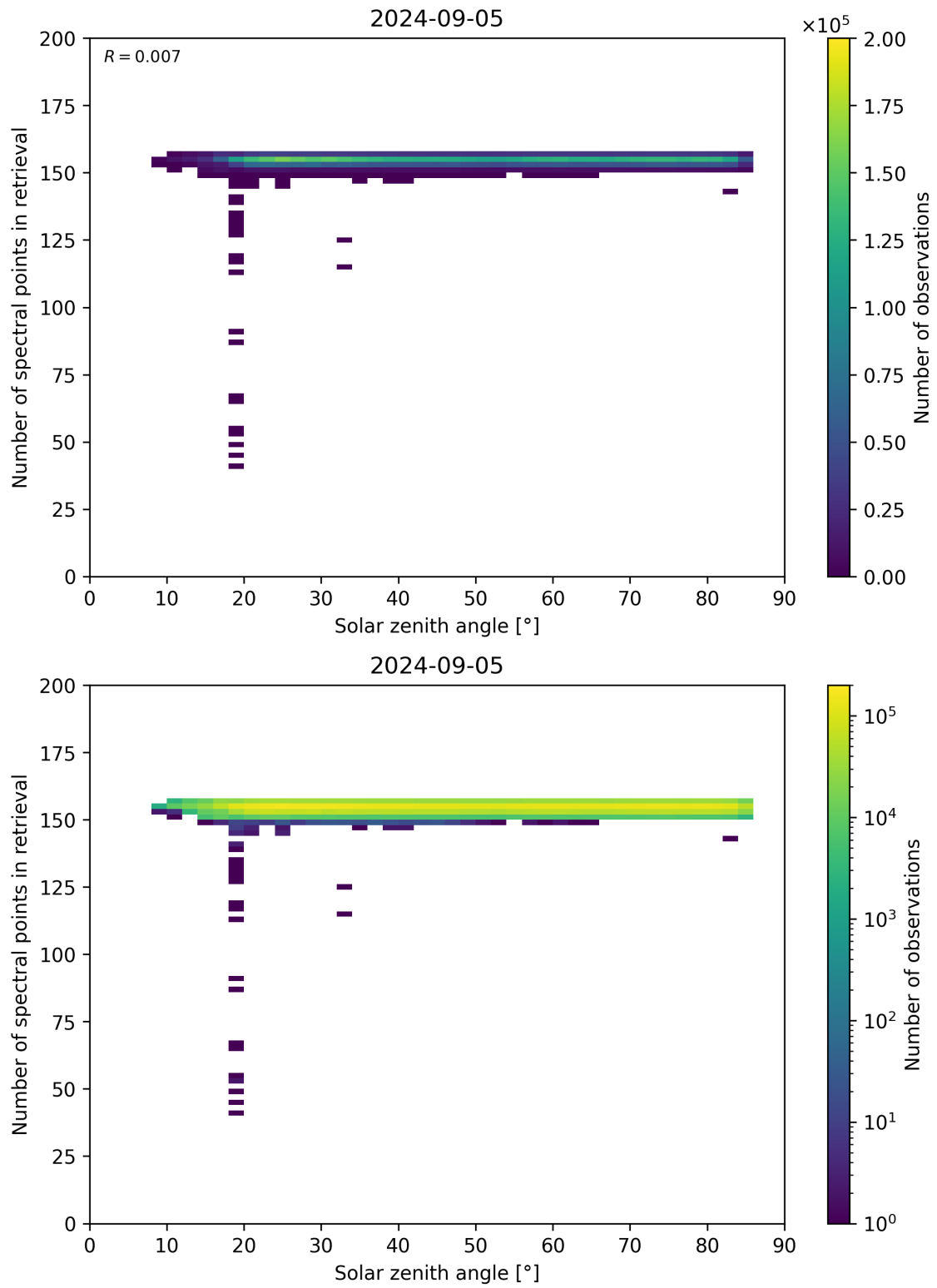
Figure 68: Scatter density plot of “Solar zenith angle” against “Number of spectral points in retrieval” for 2024-09-04 to 2024-09-06.
