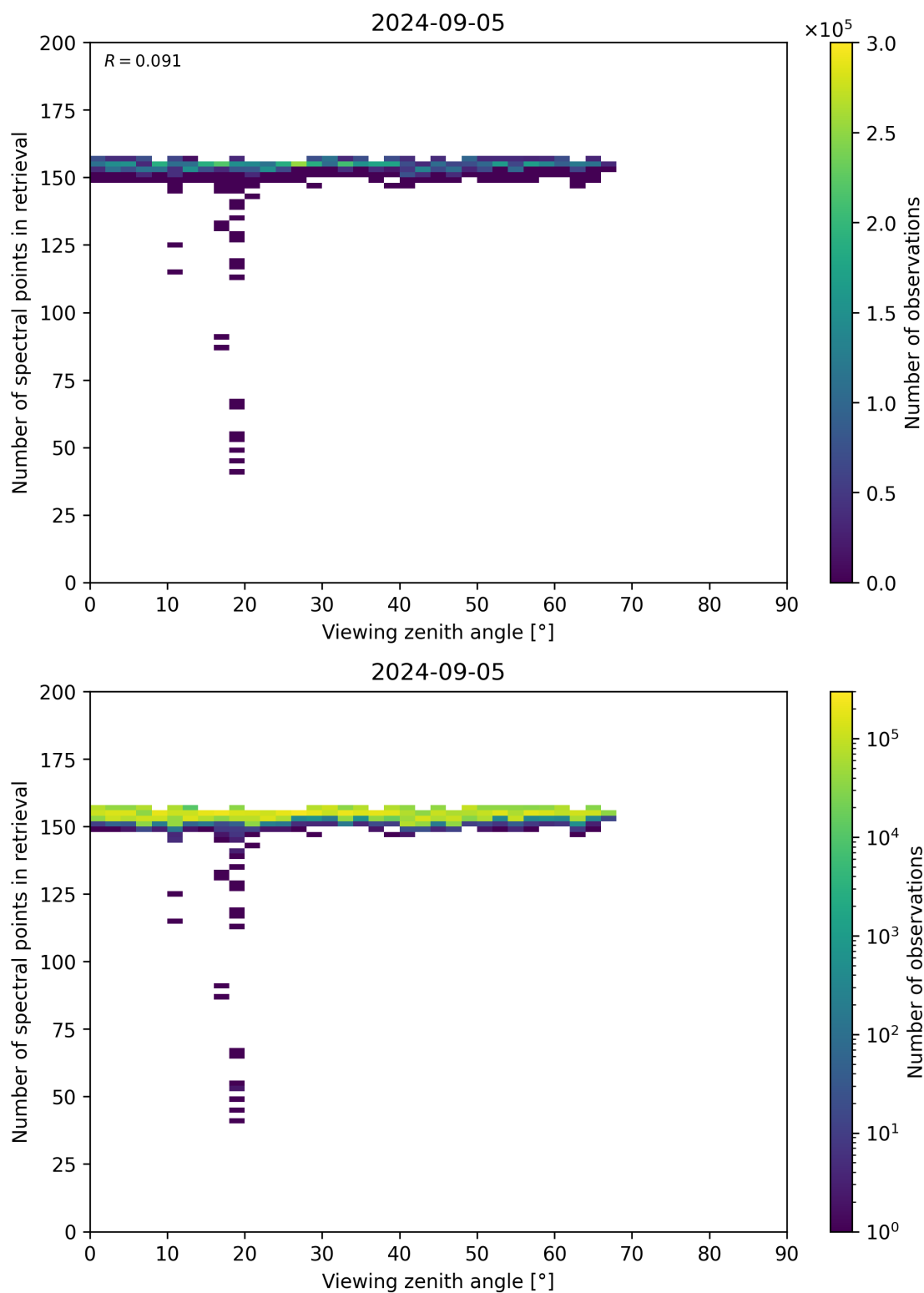
Figure 76: Scatter density plot of “Viewing zenith angle” against “Number of spectral points in retrieval” for 2024-09-04 to 2024-09-06.
