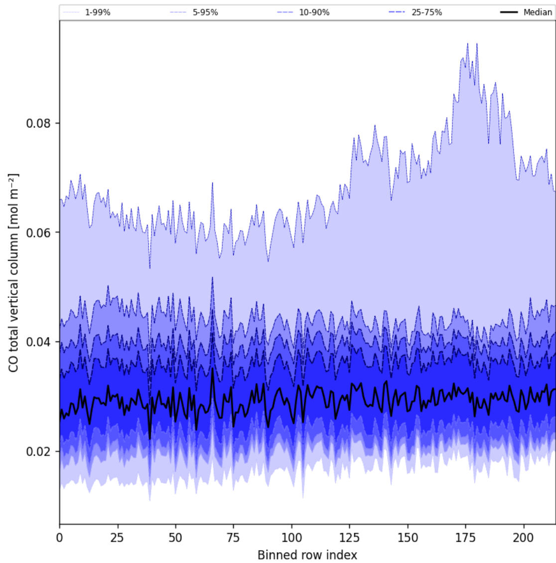
Figure 26: Along track statistics of “CO total vertical column” for 2024-09-04 to 2024-09-06
