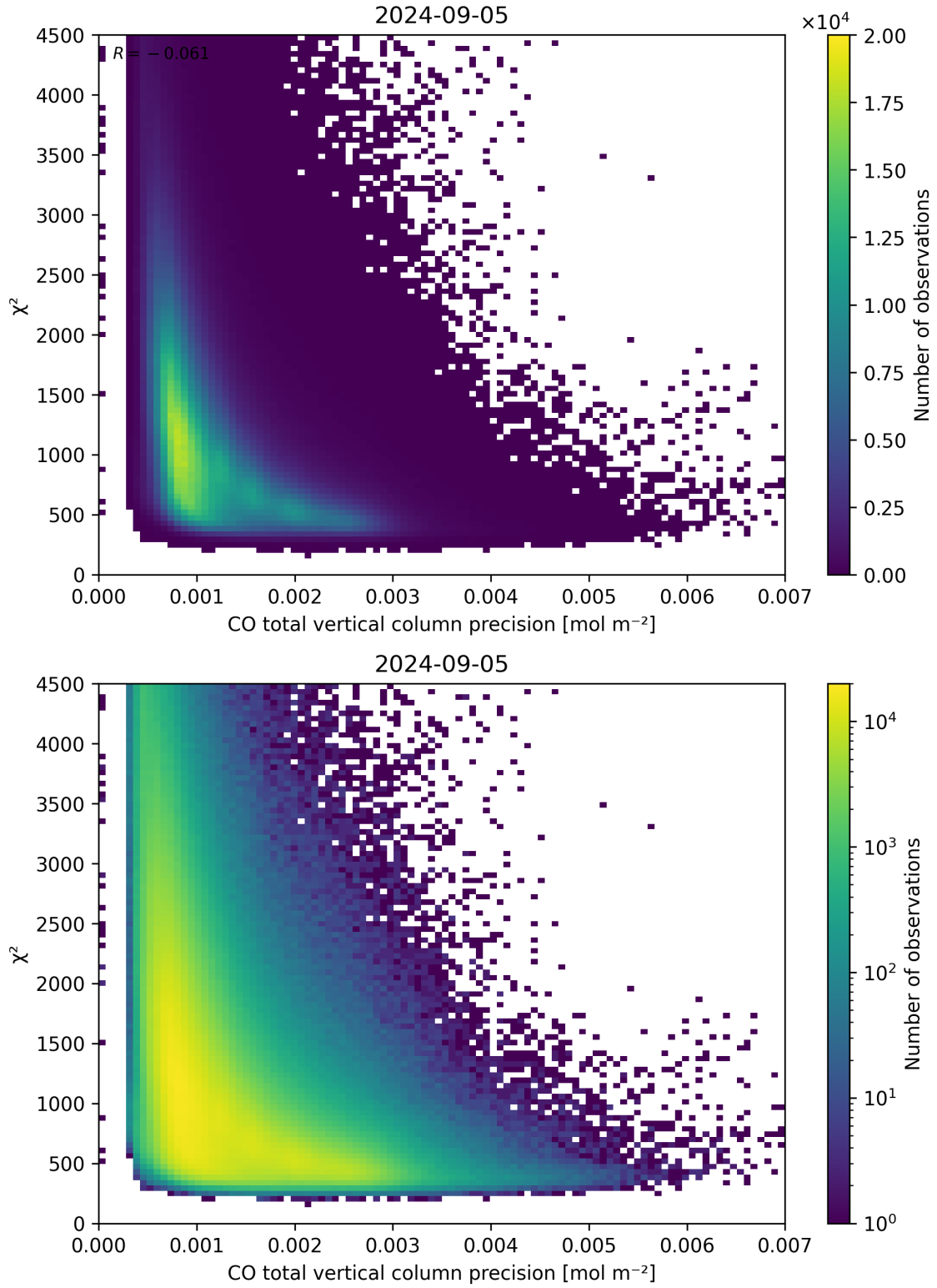
Figure 44: Scatter density plot of “CO total vertical column precision” against “ \chi^2 ” for 2024-09-04 to 2024-09-06.
