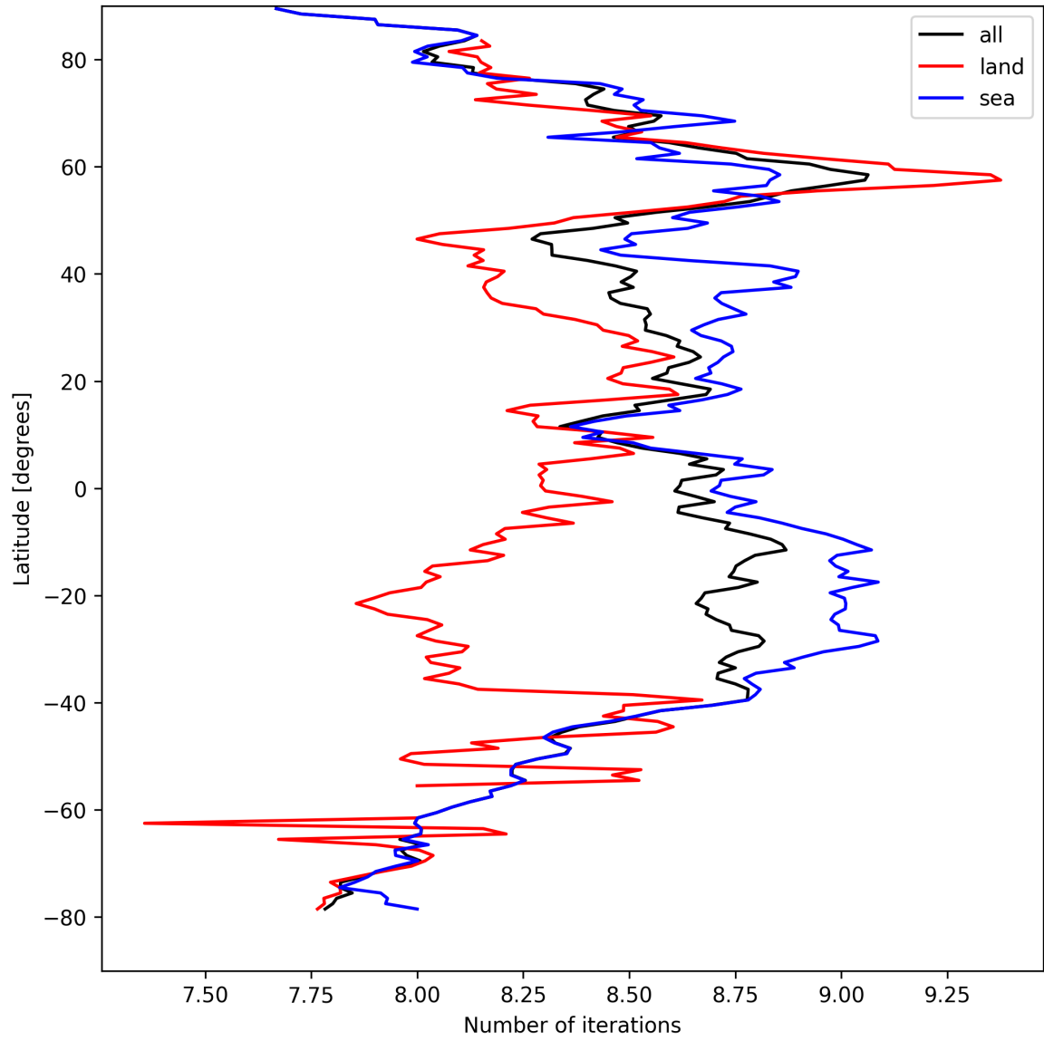
Figure 16: Zonal average of “Number of iterations” for 2024-09-04 to 2024-09-06.
