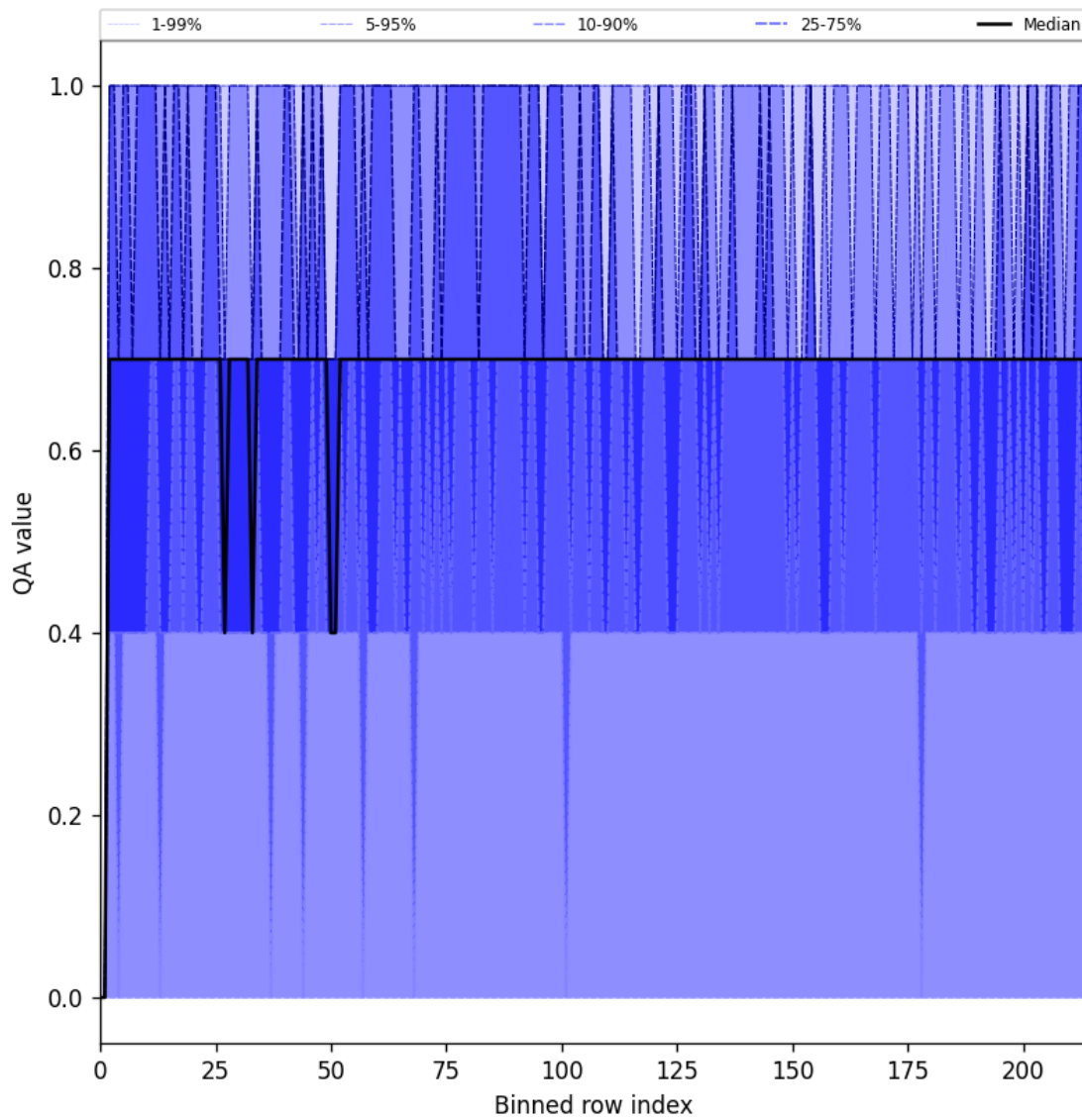
Figure 25: Along track statistics of “QA value” for 2024-09-04 to 2024-09-06
