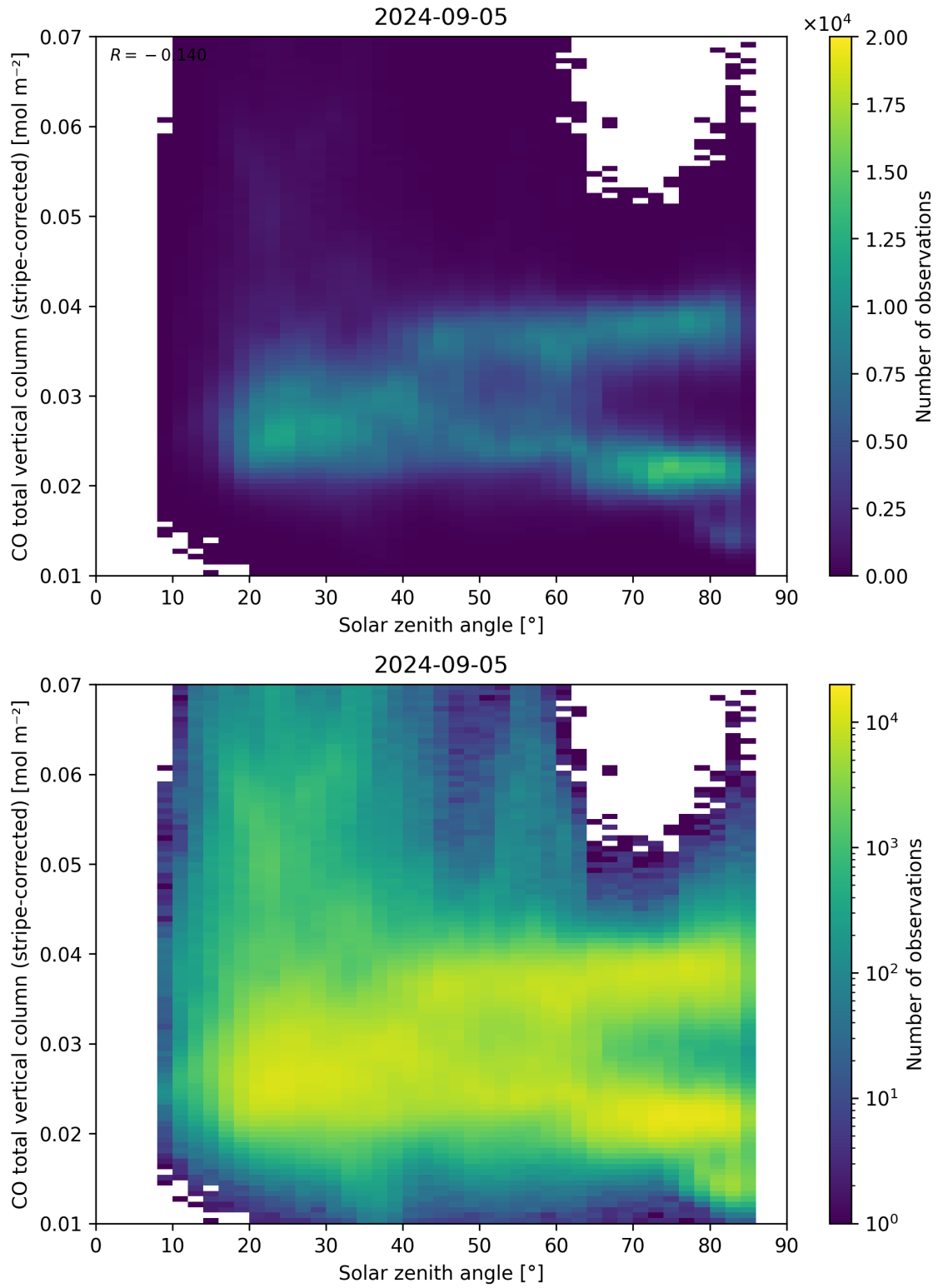
Figure 62: Scatter density plot of “Solar zenith angle” against “CO total vertical column (stripe-corrected)” for 2024-09-04 to 2024-09-06.
