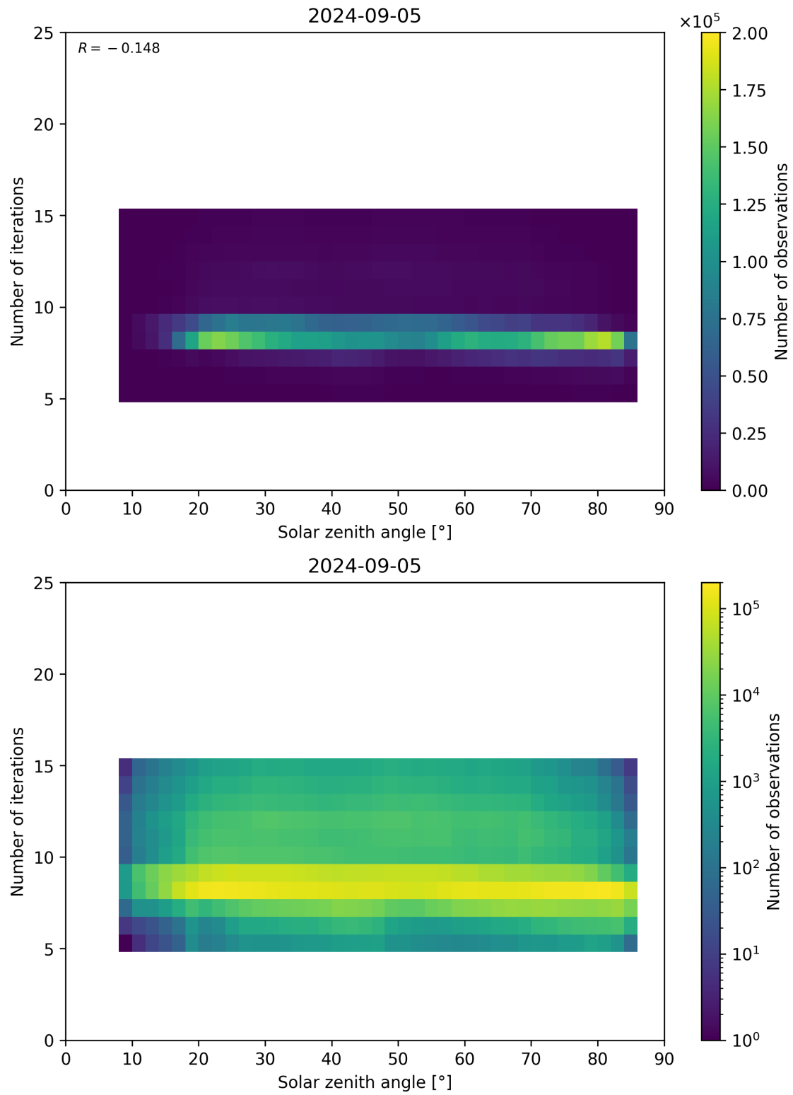
Figure 67: Scatter density plot of “Solar zenith angle” against “Number of iterations” for 2024-09-04 to 2024-09-06.
