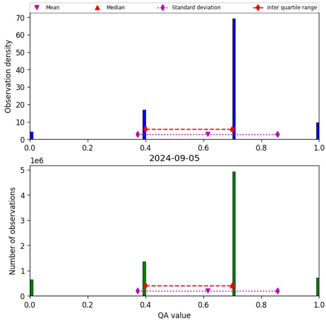
Figure 17: Histogram of “QA value” for 2024-09-04 to 2024-09-06
