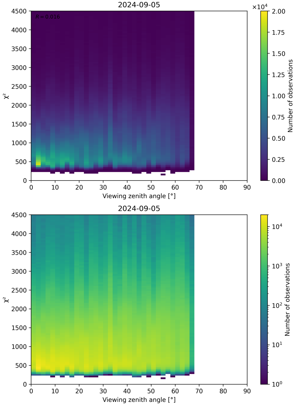
Figure 72: Scatter density plot of “Viewing zenith angle” against “ \chi^2 ” for 2024-09-04 to 2024-09-06.
