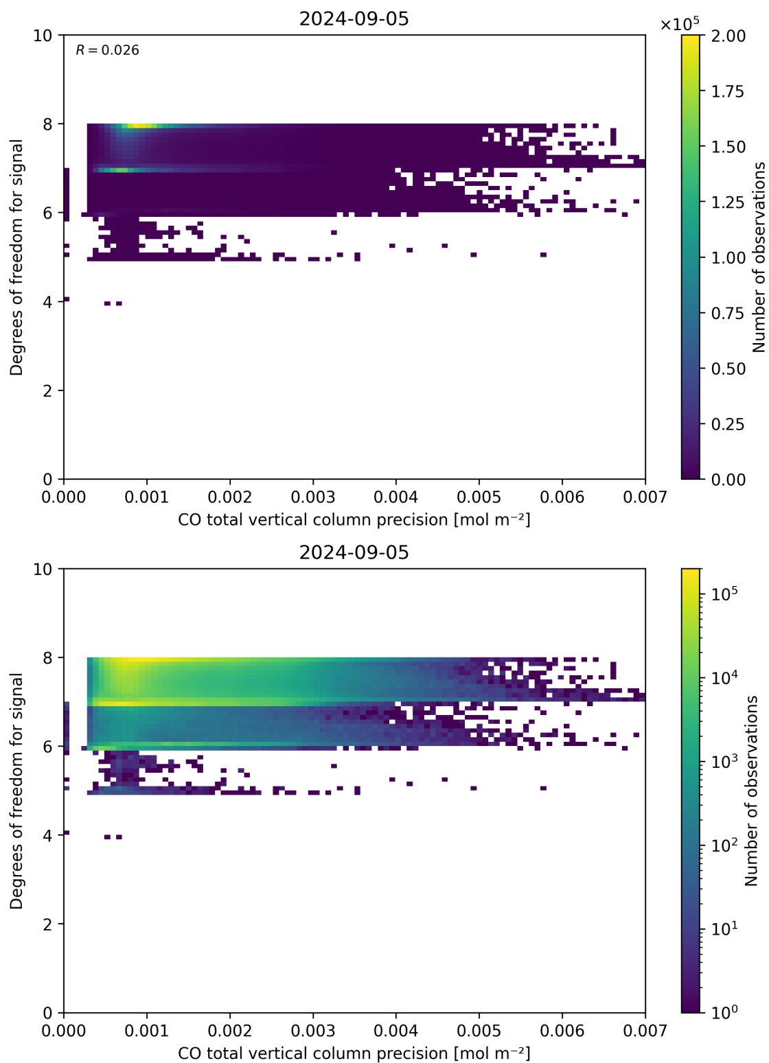
Figure 45: Scatter density plot of “CO total vertical column precision” against “Degrees of freedom for signal” for 2024-09-04 to 2024-09-06.
