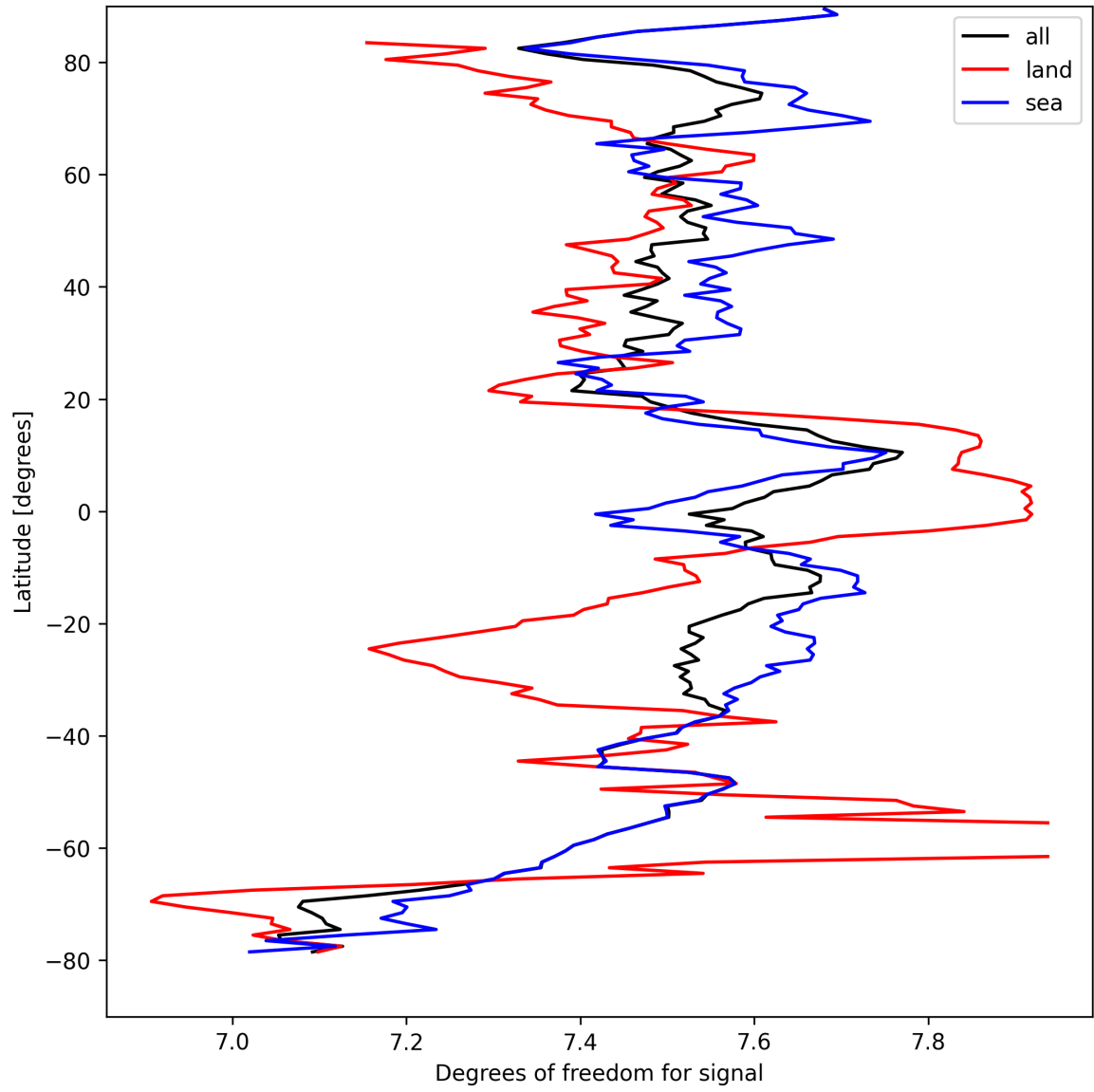
Figure 15: Zonal average of “Degrees of freedom for signal” for 2024-09-04 to 2024-09-06.
