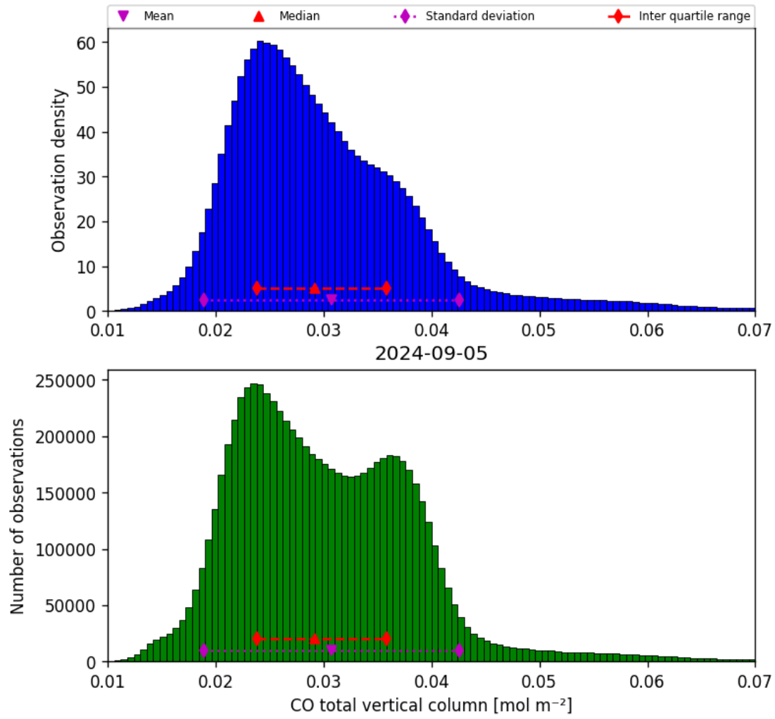
Figure 18: Histogram of “CO total vertical column” for 2024-09-04 to 2024-09-06
