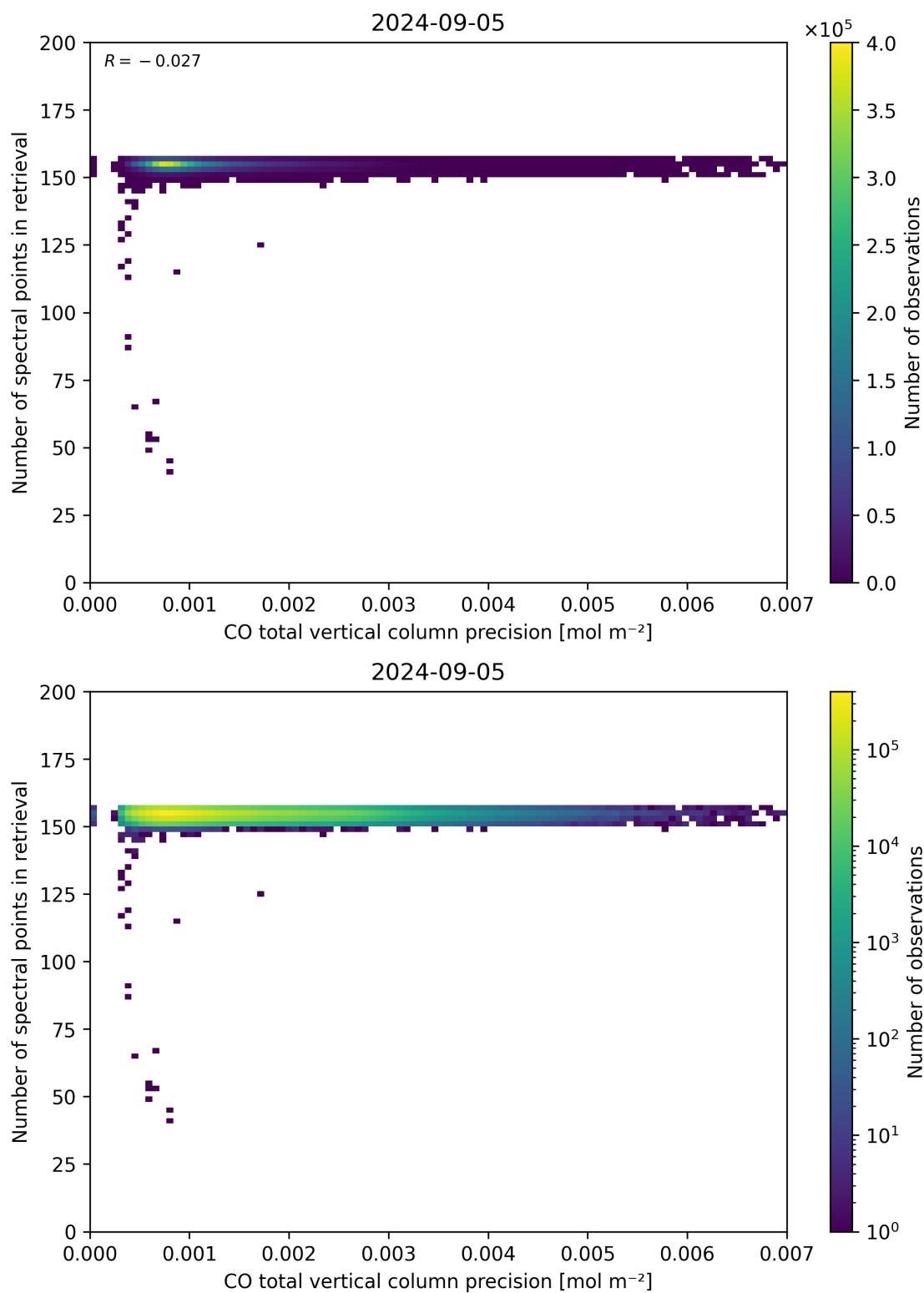
Figure 47: Scatter density plot of “CO total vertical column precision” against “Number of spectral points in retrieval” for 2024-09-04 to 2024-09-06.
