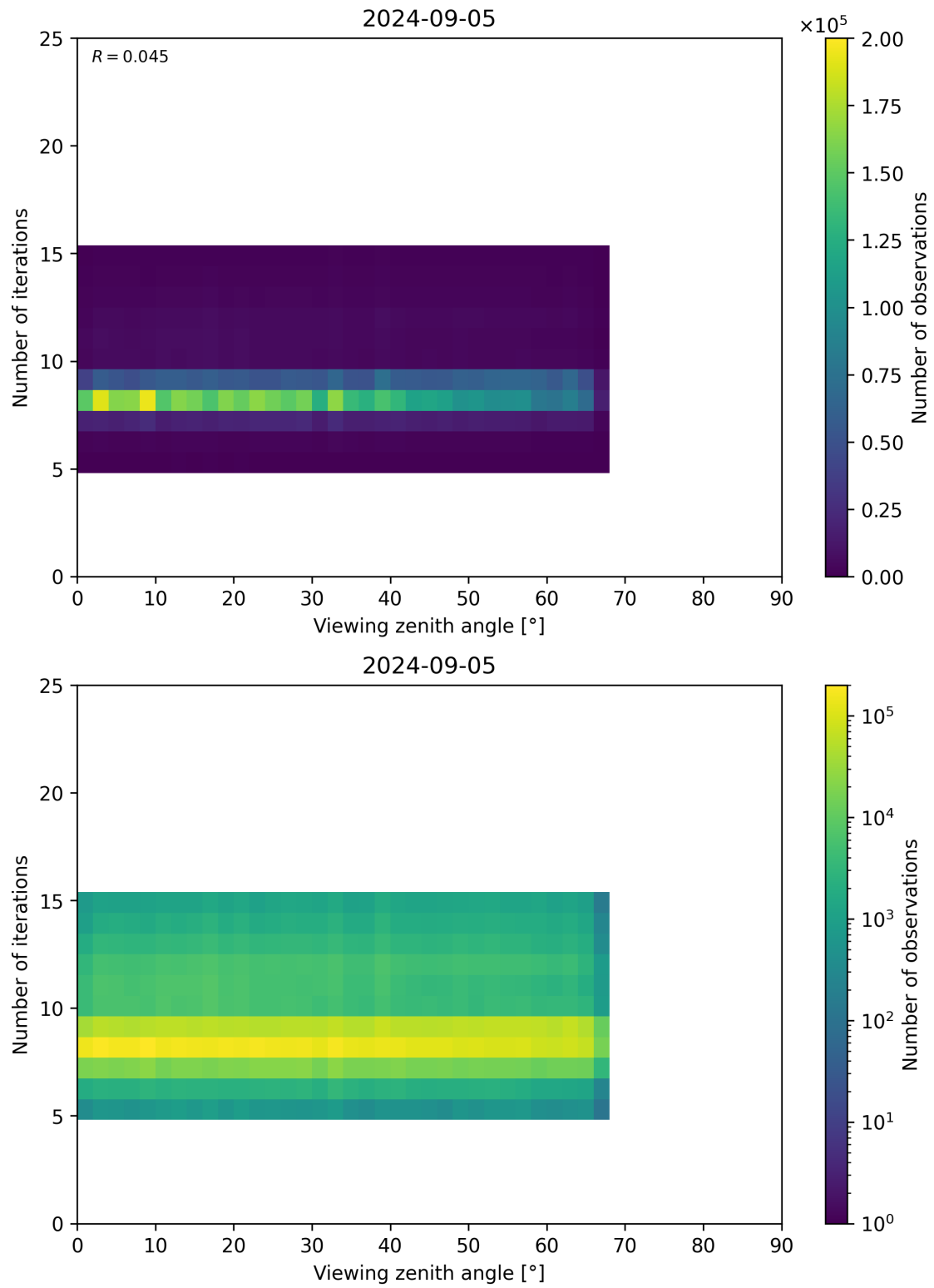
Figure 75: Scatter density plot of “Viewing zenith angle” against “Number of iterations” for 2024-09-04 to 2024-09-06.
