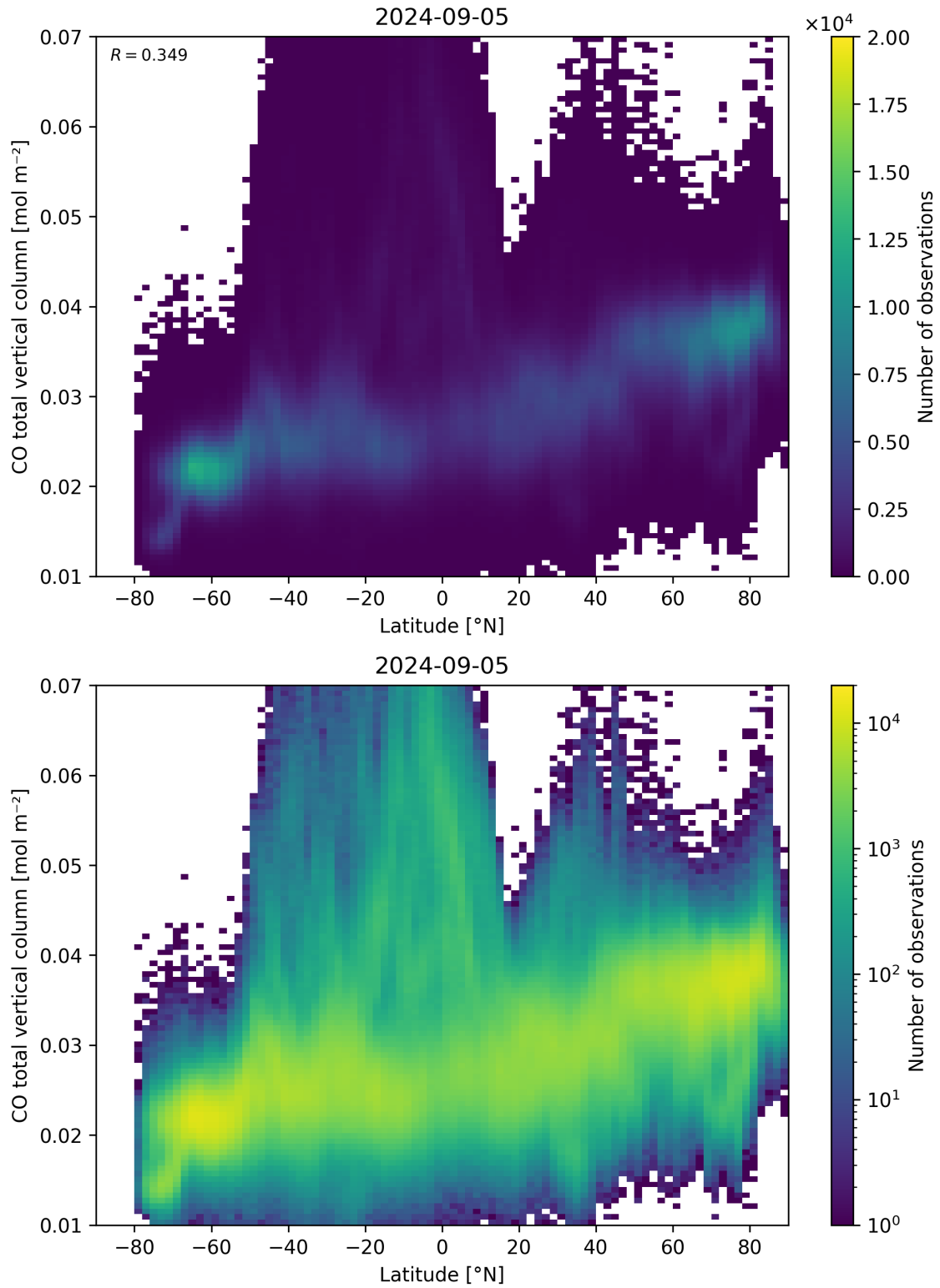
Figure 51: Scatter density plot of “Latitude” against “CO total vertical column” for 2024-09-04 to 2024-09-06.
