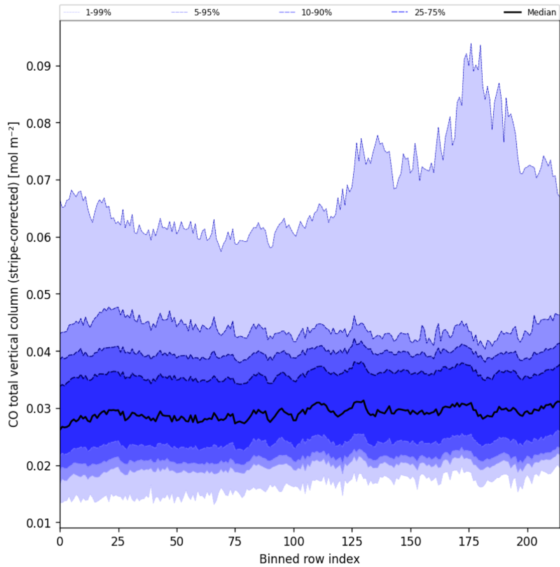
Figure 27: Along track statistics of “CO total vertical column (stripe-corrected)” for 2024-09-04 to 2024-09-06
