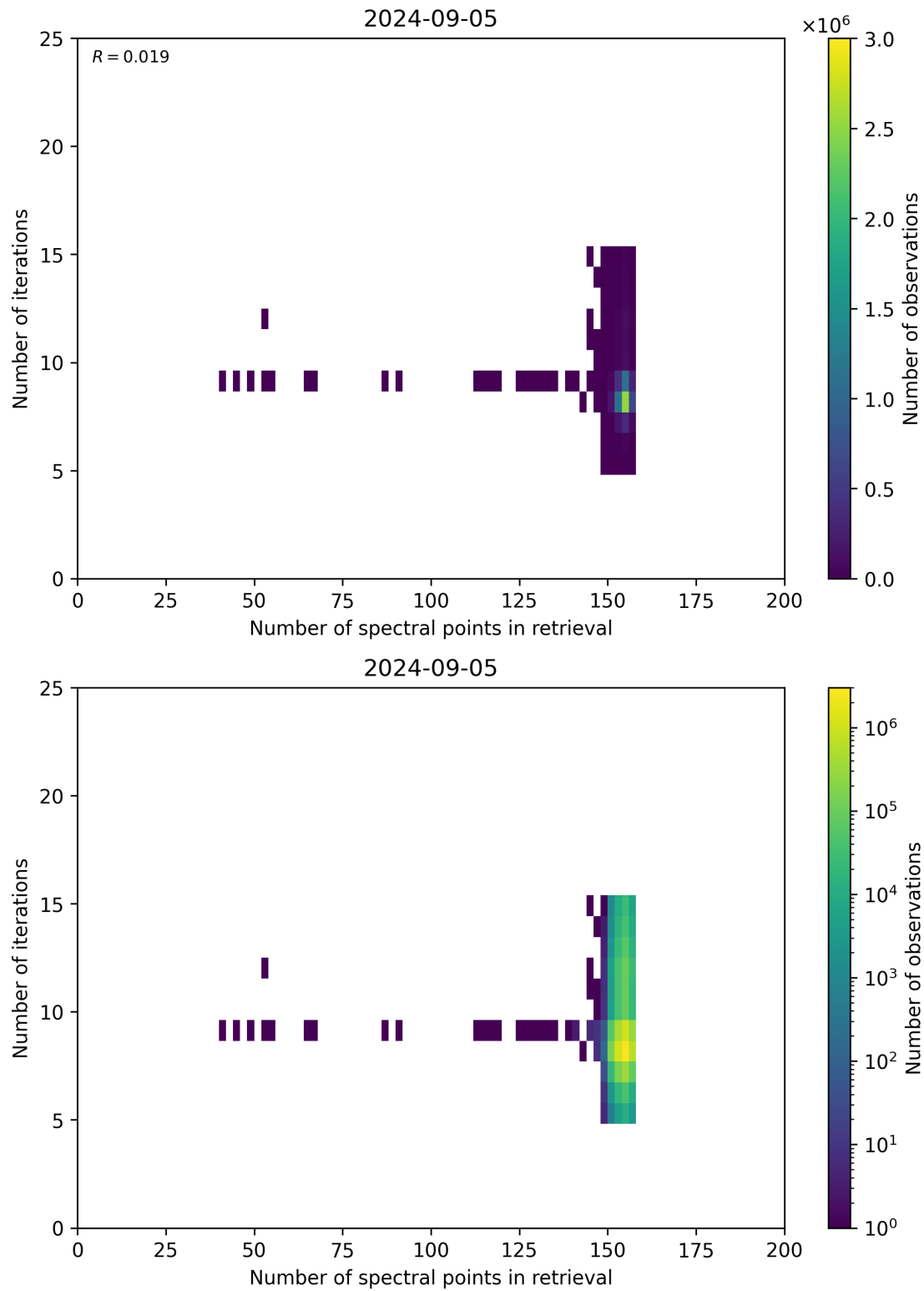
Figure 60: Scatter density plot of “Number of spectral points in retrieval” against “Number of iterations” for 2024-09-04 to 2024-09-06.
