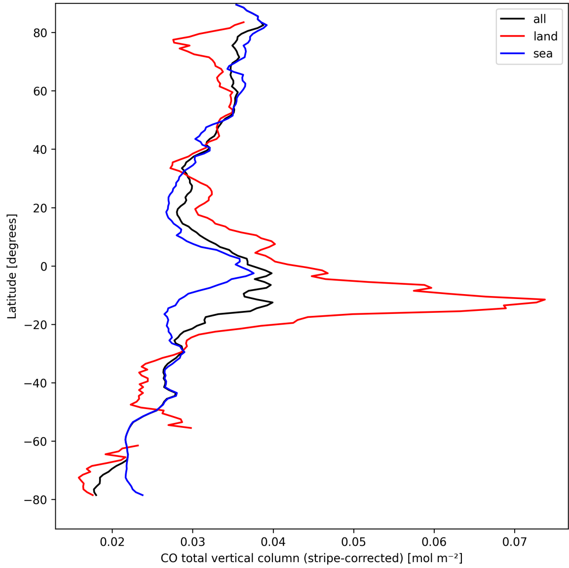
Figure 11: Zonal average of “CO total vertical column (stripe-corrected)” for 2024-09-04 to 2024-09-06.
