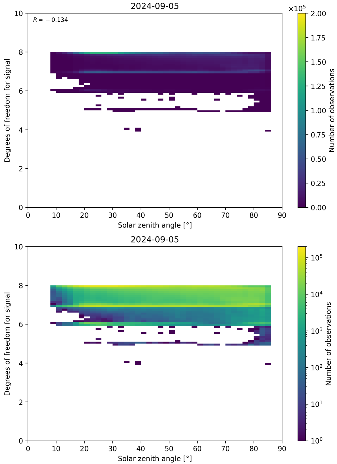
Figure 65: Scatter density plot of “Solar zenith angle” against “Degrees of freedom for signal” for 2024-09-04 to 2024-09-06.
