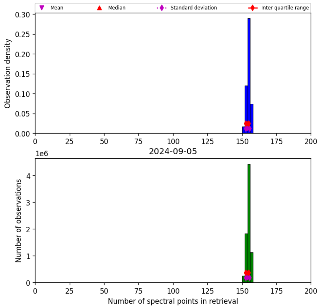
Figure 21: Histogram of “Number of spectral points in retrieval” for 2024-09-04 to 2024-09-06
