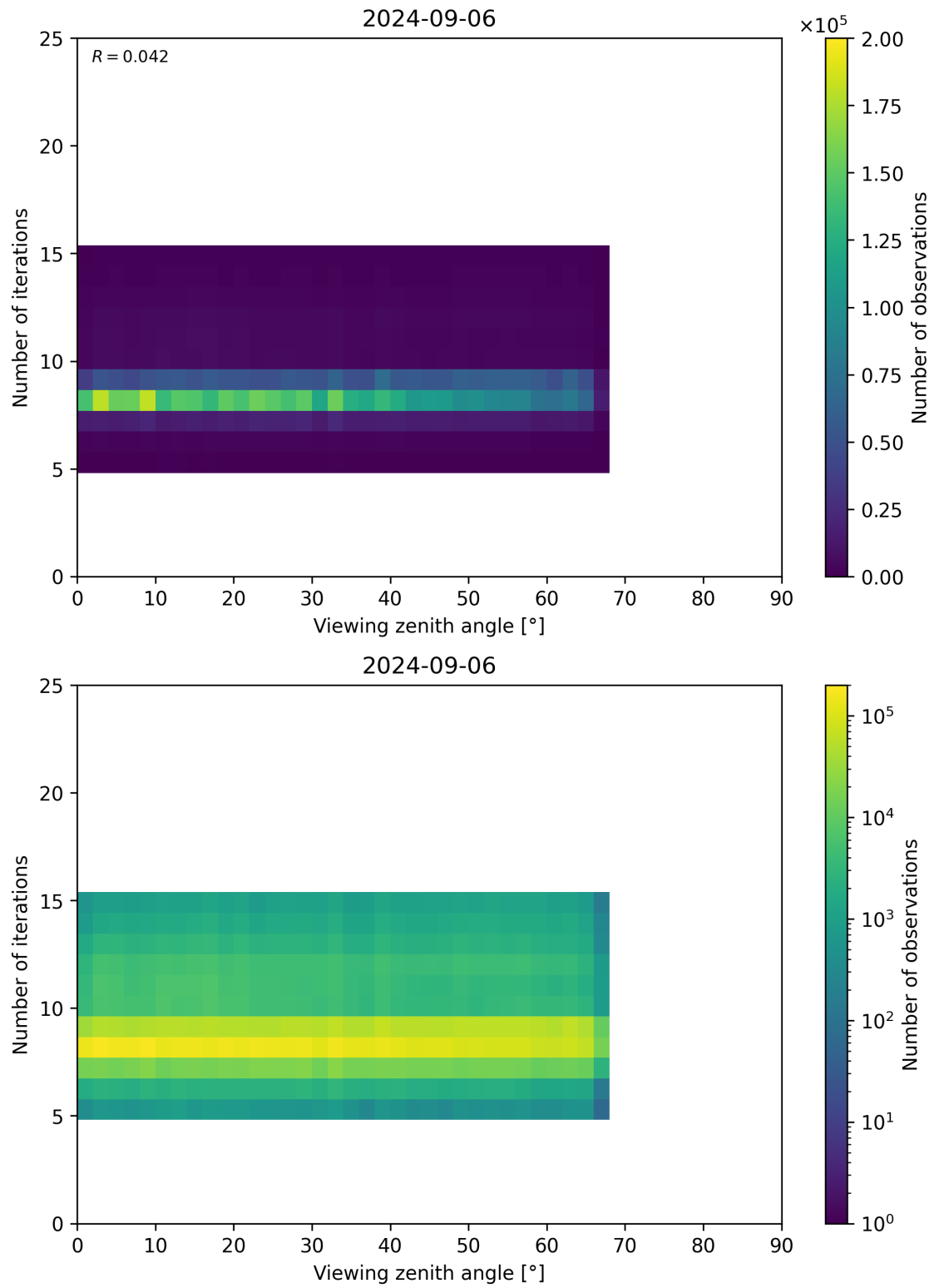
Figure 75: Scatter density plot of “Viewing zenith angle” against “Number of iterations” for 2024-09-06 to 2024-09-07.
