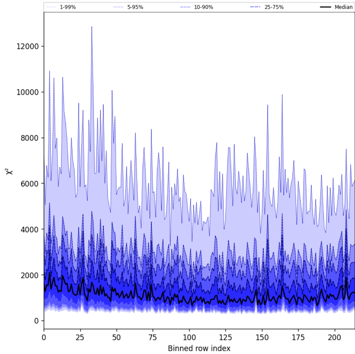
Figure 30: Along track statistics of “ \chi^2 ” for 2024-09-06 to 2024-09-07
