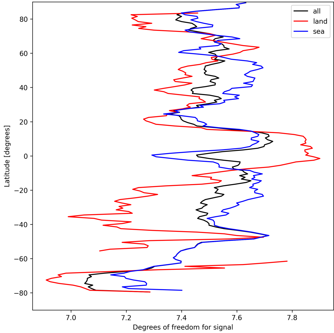
Figure 15: Zonal average of “Degrees of freedom for signal” for 2024-09-06 to 2024-09-07.
