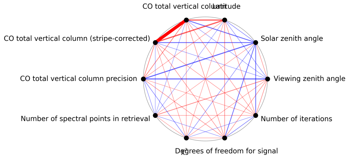
Figure 1: Map of correlation graph for 2024-09-06 to 2024-09-07.
