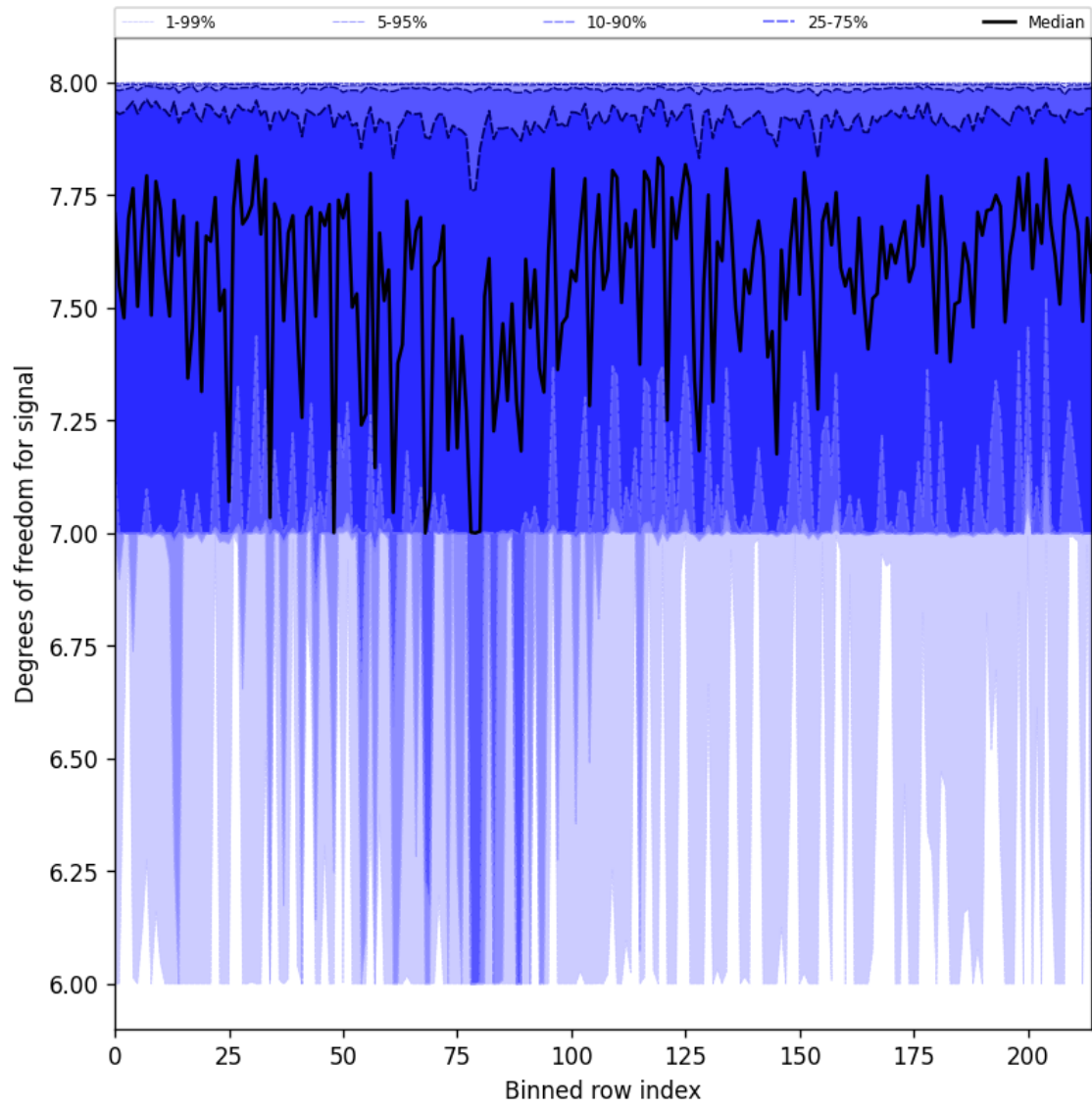
Figure 31: Along track statistics of “Degrees of freedom for signal” for 2024-09-06 to 2024-09-07
