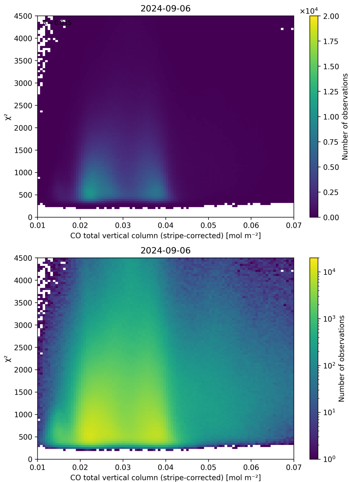
Figure 37: Scatter density plot of “CO total vertical column (stripe-corrected)” against “ \chi^2 ” for 2024-09-06 to 2024-09-07.
