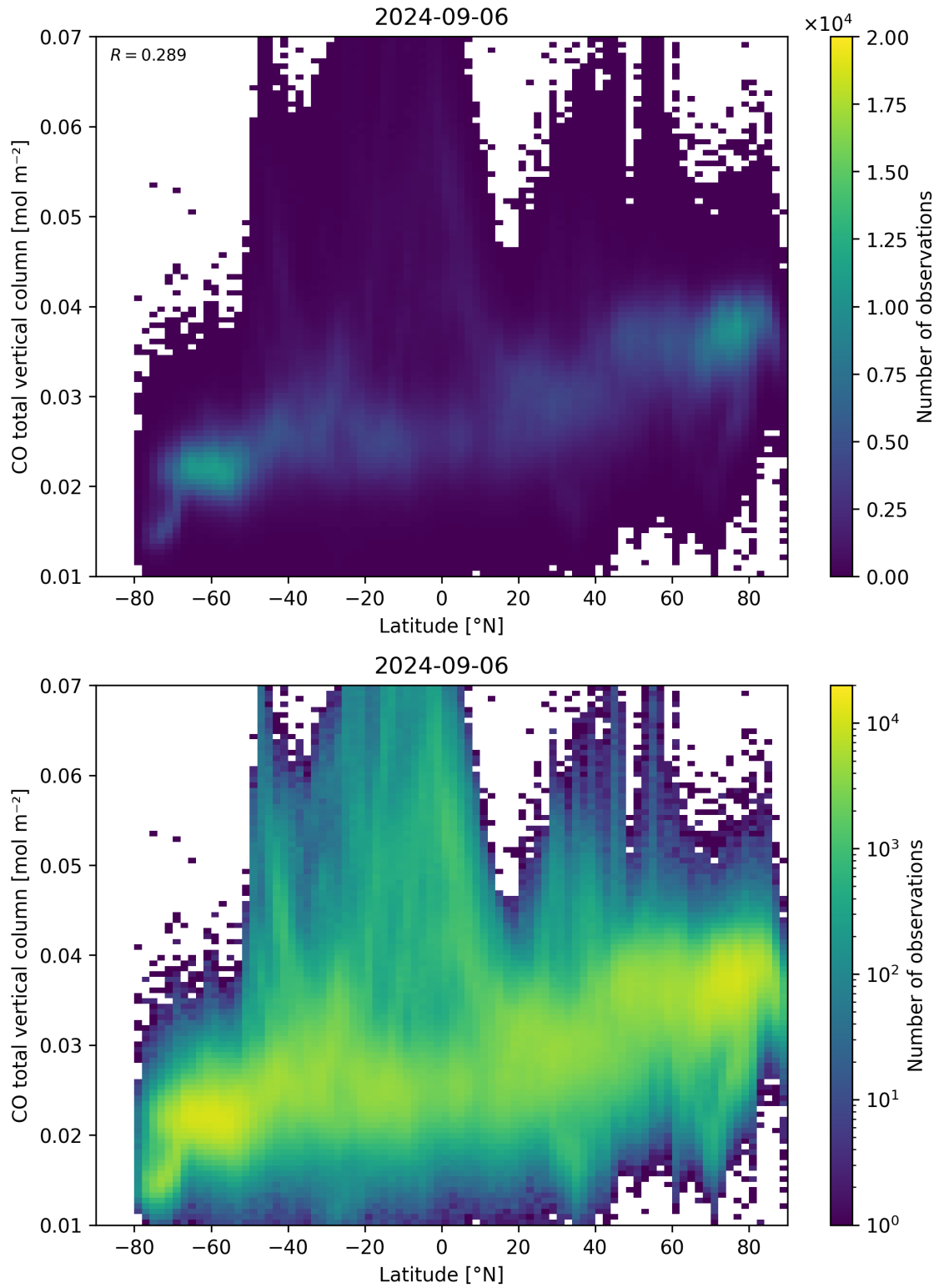
Figure 51: Scatter density plot of “Latitude” against “CO total vertical column” for 2024-09-06 to 2024-09-07.
