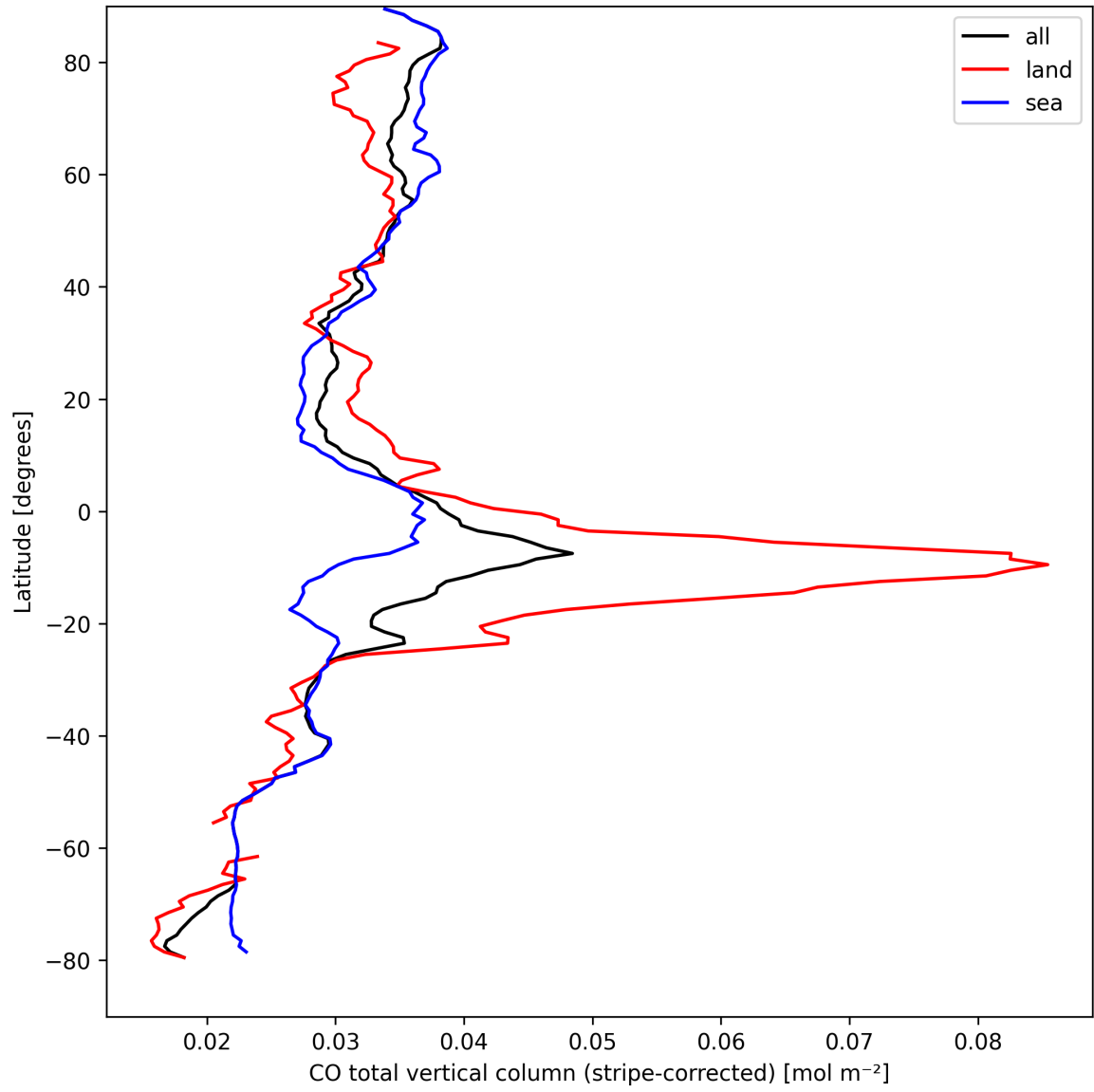
Figure 11: Zonal average of “CO total vertical column (stripe-corrected)” for 2024-09-06 to 2024-09-07.
