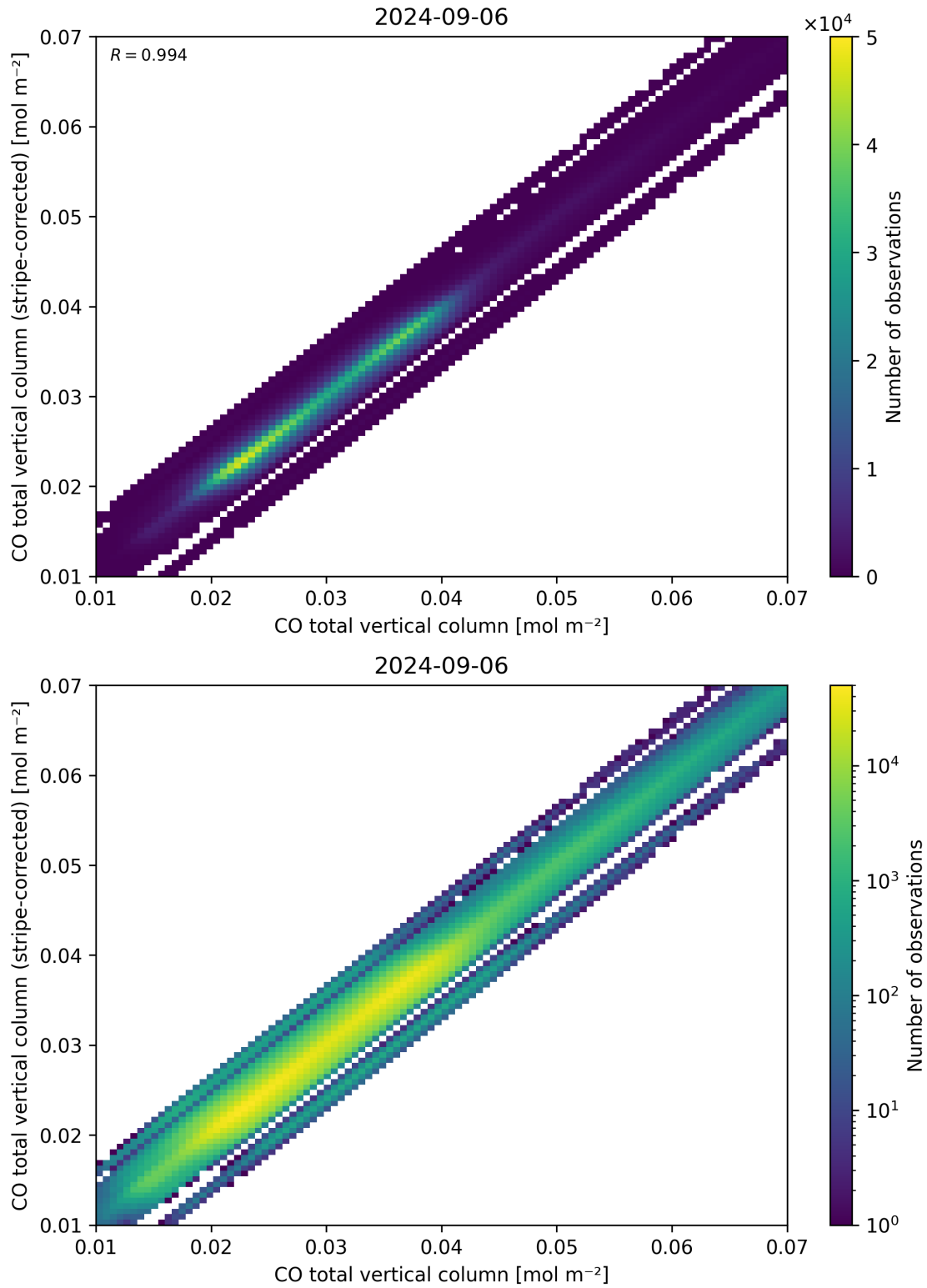
Figure 33: Scatter density plot of “CO total vertical column” against “CO total vertical column (stripe-corrected)” for 2024-09-06 to 2024-09-07.
