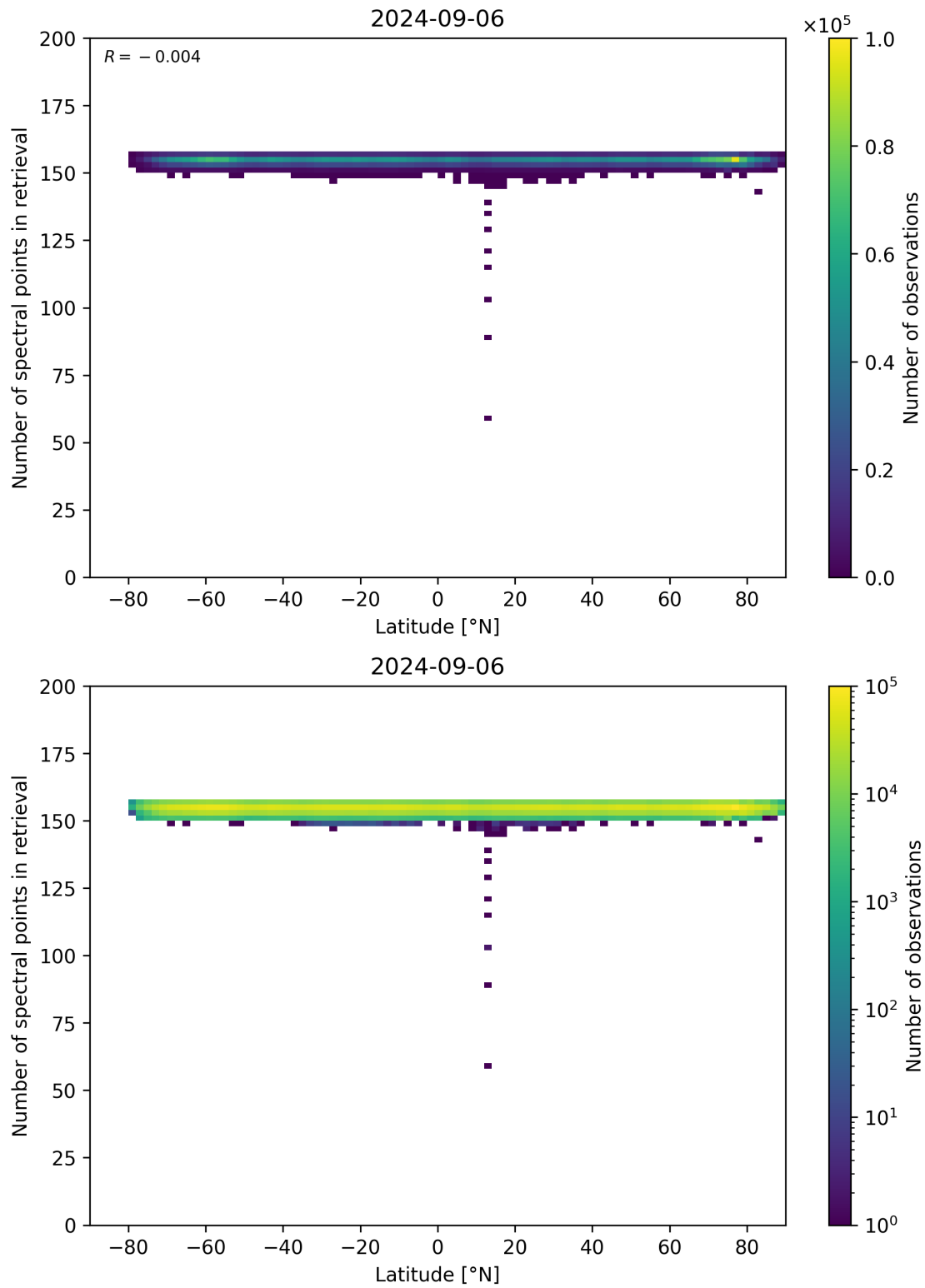
Figure 57: Scatter density plot of “Latitude” against “Number of spectral points in retrieval” for 2024-09-06 to 2024-09-07.
