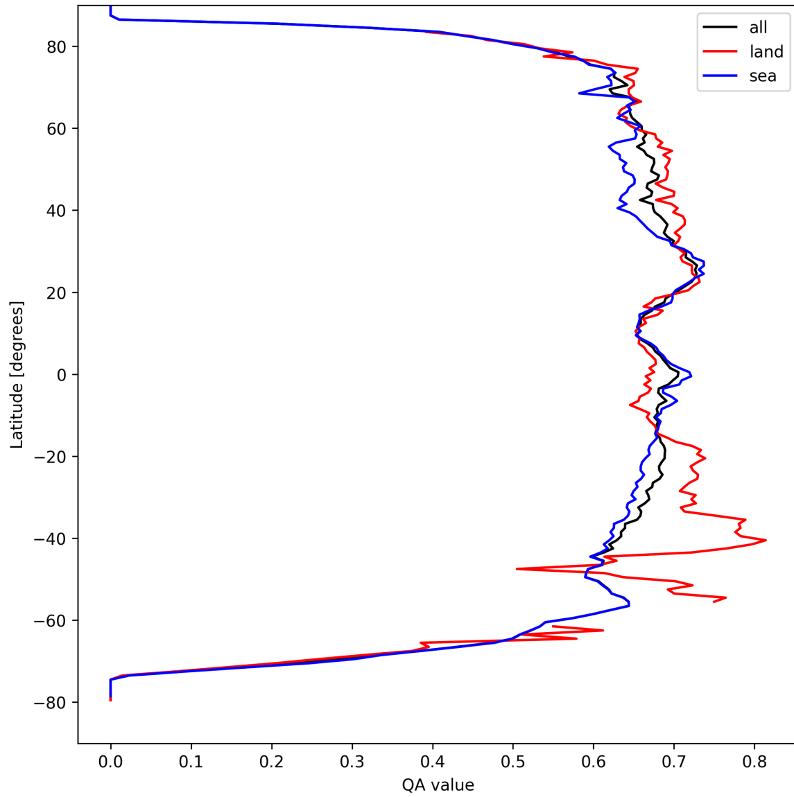
Figure 9: Zonal average of “QA value” for 2024-09-06 to 2024-09-07.
