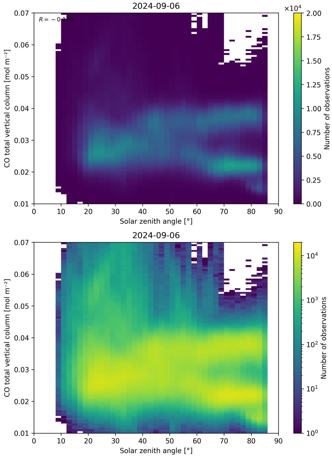
Figure 61: Scatter density plot of “Solar zenith angle” against “CO total vertical column” for 2024-09-06 to 2024-09-07.
