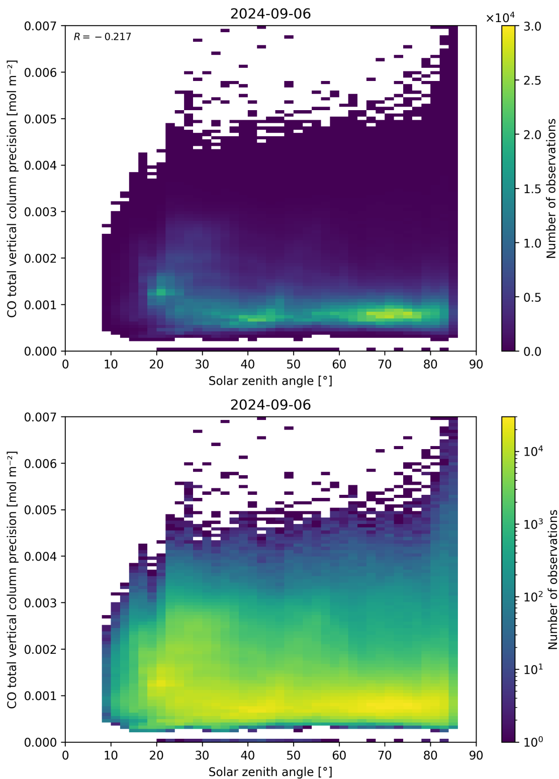
Figure 63: Scatter density plot of “Solar zenith angle” against “CO total vertical column precision” for 2024-09-06 to 2024-09-07.
