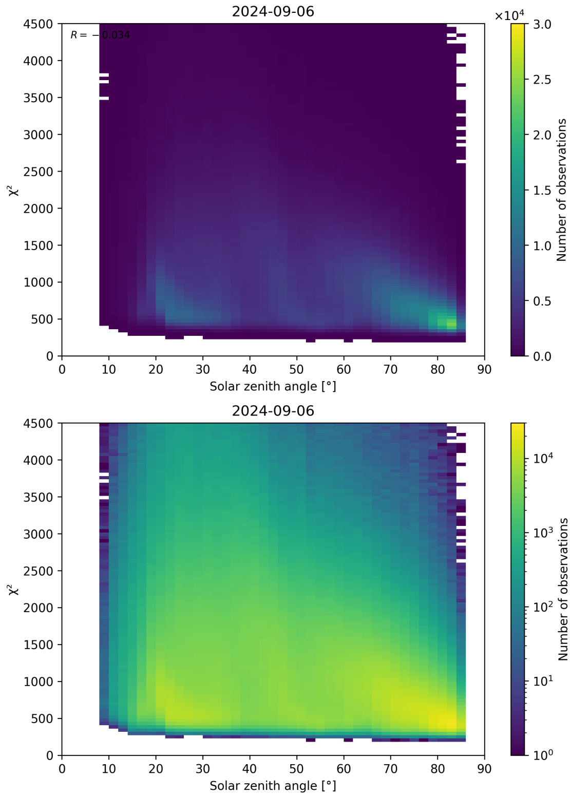
Figure 64: Scatter density plot of “Solar zenith angle” against “ \chi^2 ” for 2024-09-06 to 2024-09-07.
