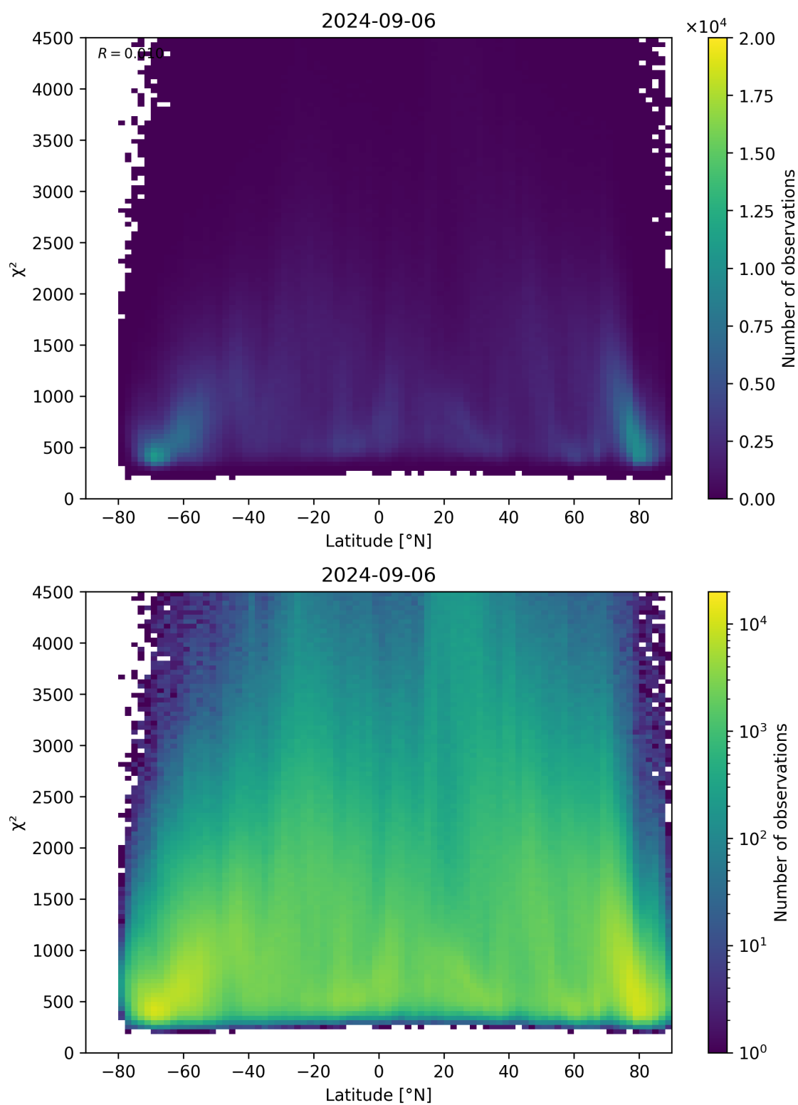
Figure 54: Scatter density plot of “Latitude” against “ \chi^2 ” for 2024-09-06 to 2024-09-07.
