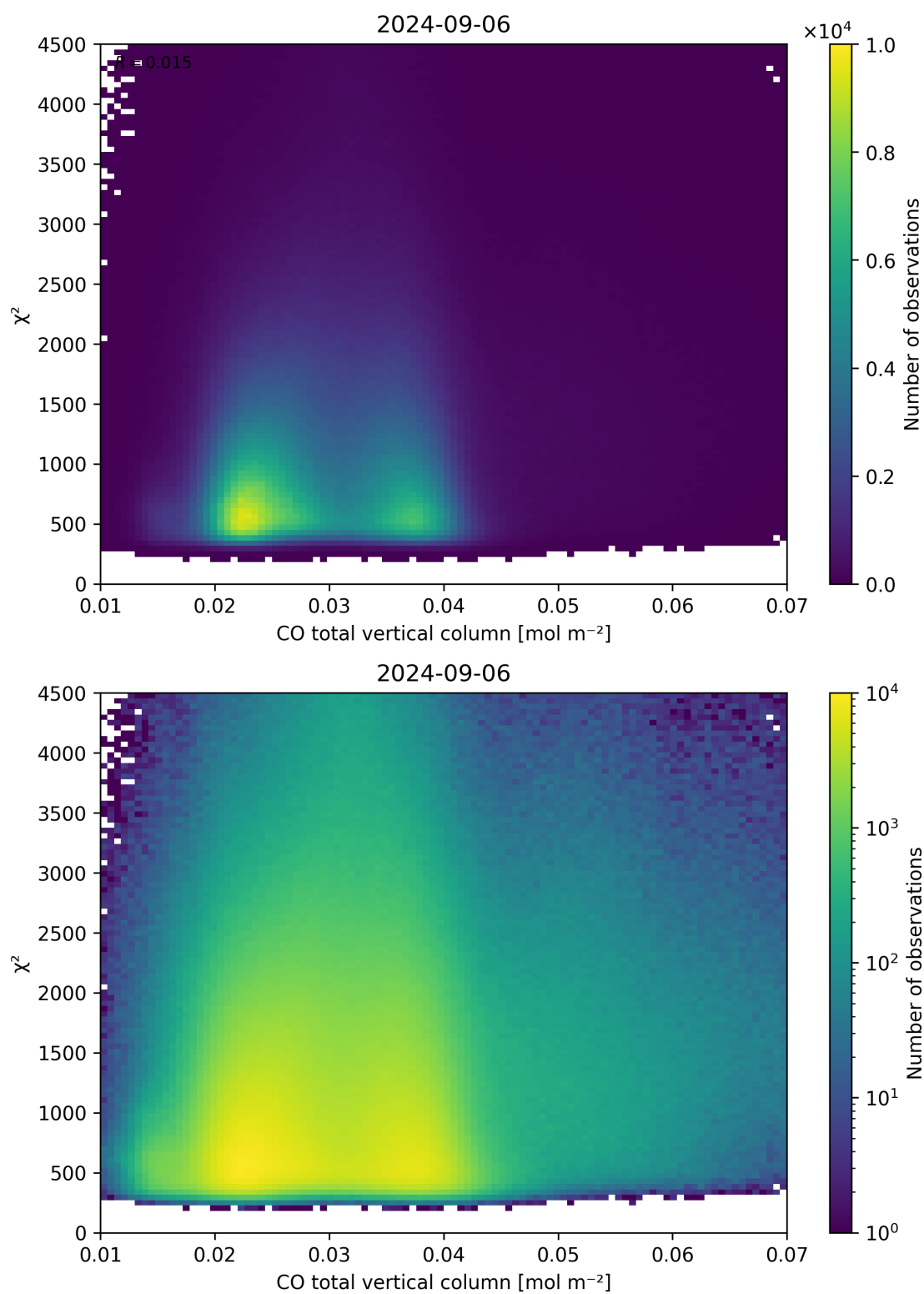
Figure 35: Scatter density plot of “CO total vertical column” against “ \chi^2 ” for 2024-09-06 to 2024-09-07.
