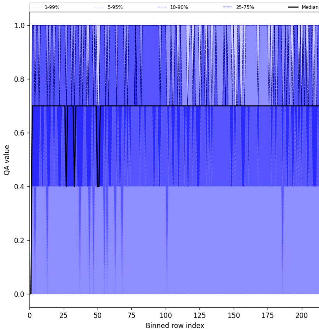
Figure 25: Along track statistics of “QA value” for 2024-09-06 to 2024-09-07
