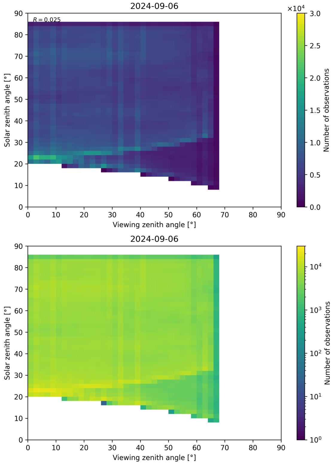
Figure 77: Scatter density plot of “Viewing zenith angle” against “Solar zenith angle” for 2024-09-06 to 2024-09-07.
