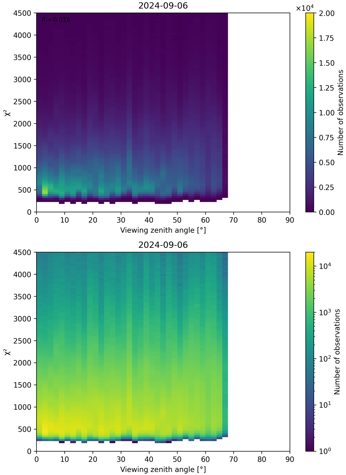
Figure 72: Scatter density plot of “Viewing zenith angle” against “ \chi^2 ” for 2024-09-06 to 2024-09-07.
