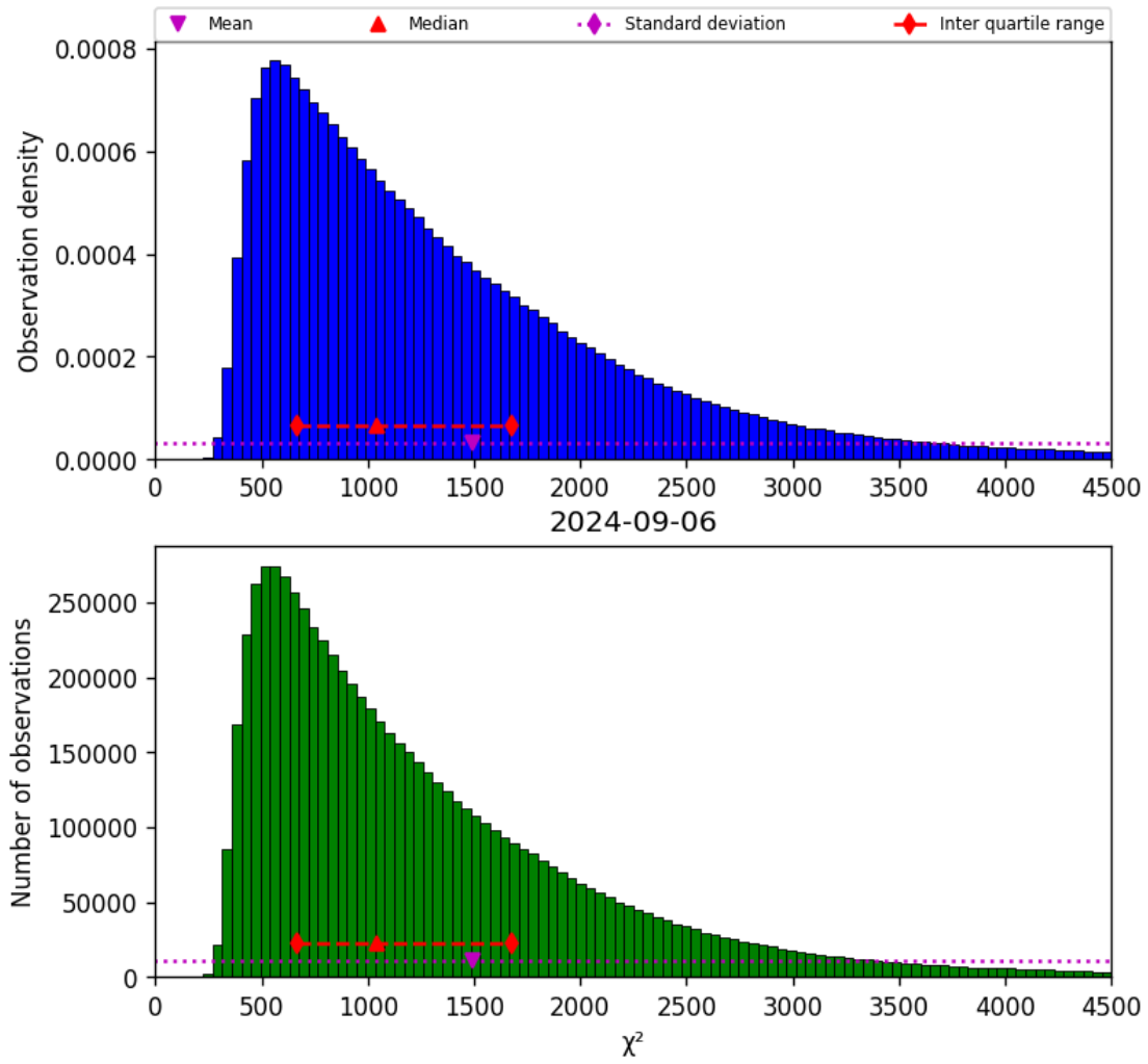
Figure 22: Histogram of " \chi^2 " for 2024-09-06 to 2024-09-07
