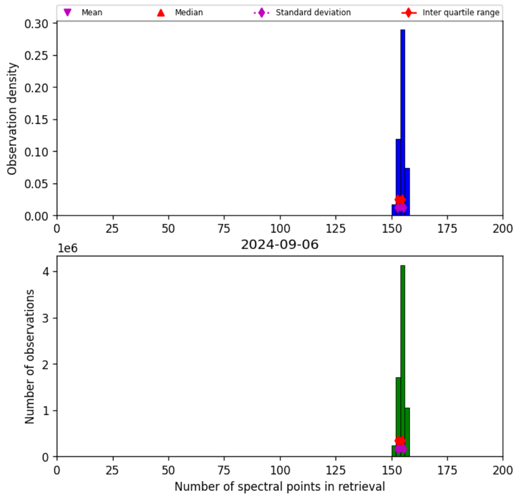
Figure 21: Histogram of “Number of spectral points in retrieval” for 2024-09-06 to 2024-09-07
