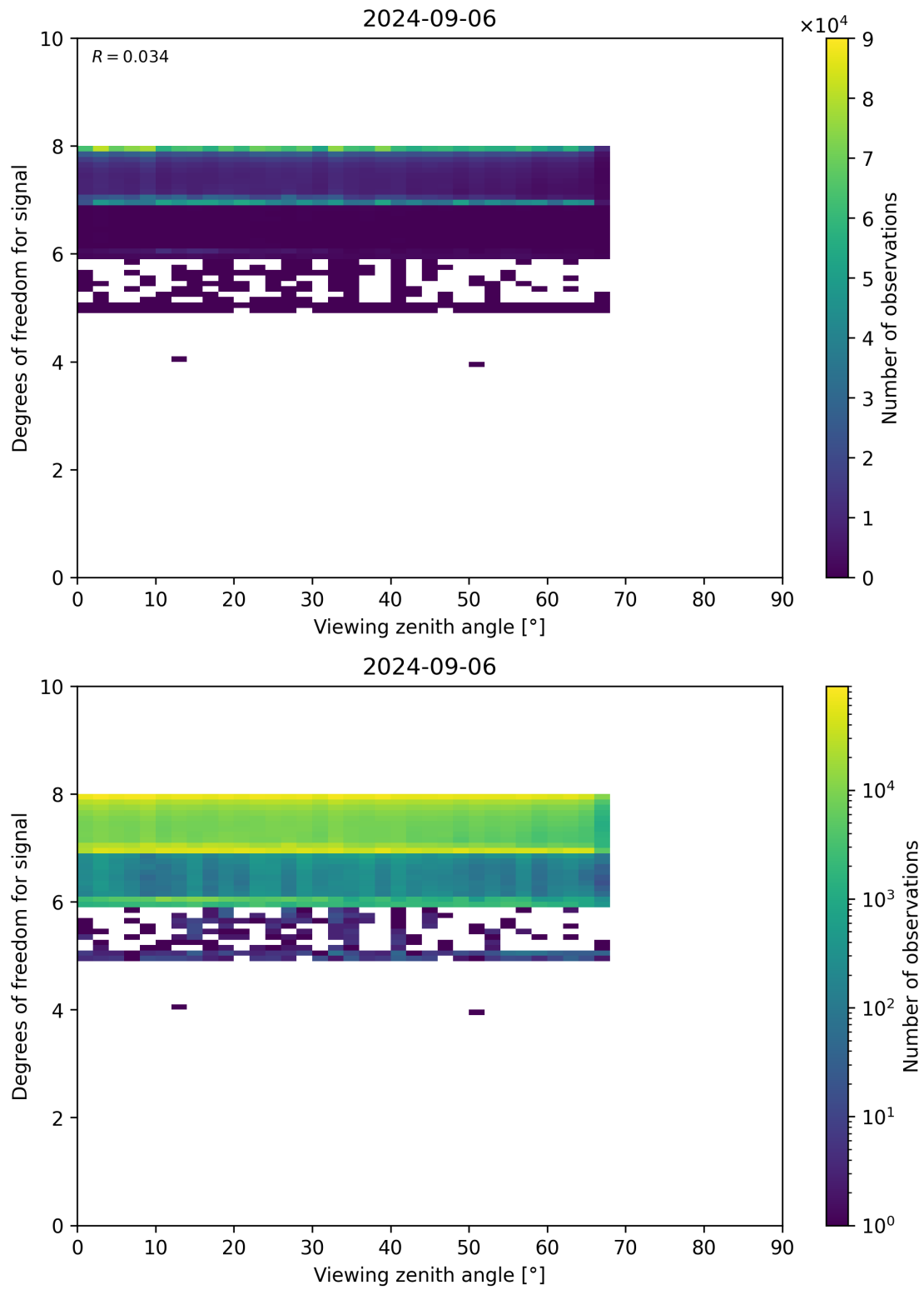
Figure 73: Scatter density plot of “Viewing zenith angle” against “Degrees of freedom for signal” for 2024-09-06 to 2024-09-07.
