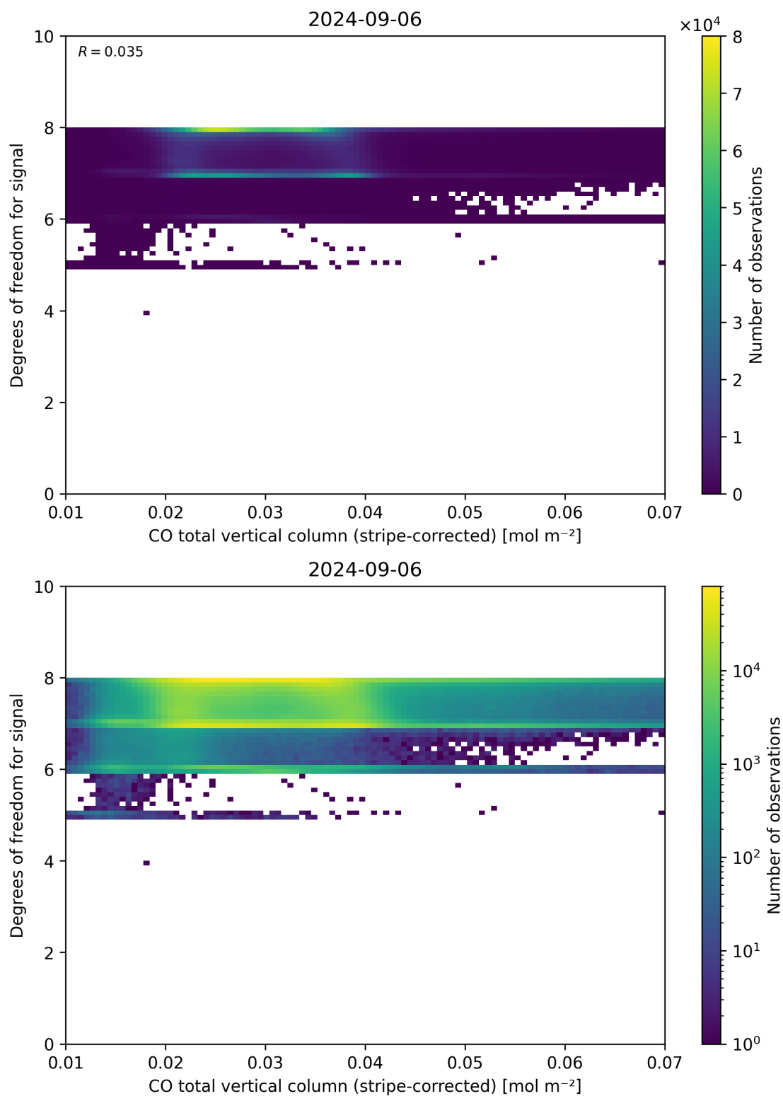
Figure 38: Scatter density plot of “CO total vertical column (stripe-corrected)” against “Degrees of freedom for signal” for 2024-09-06 to 2024-09-07.
