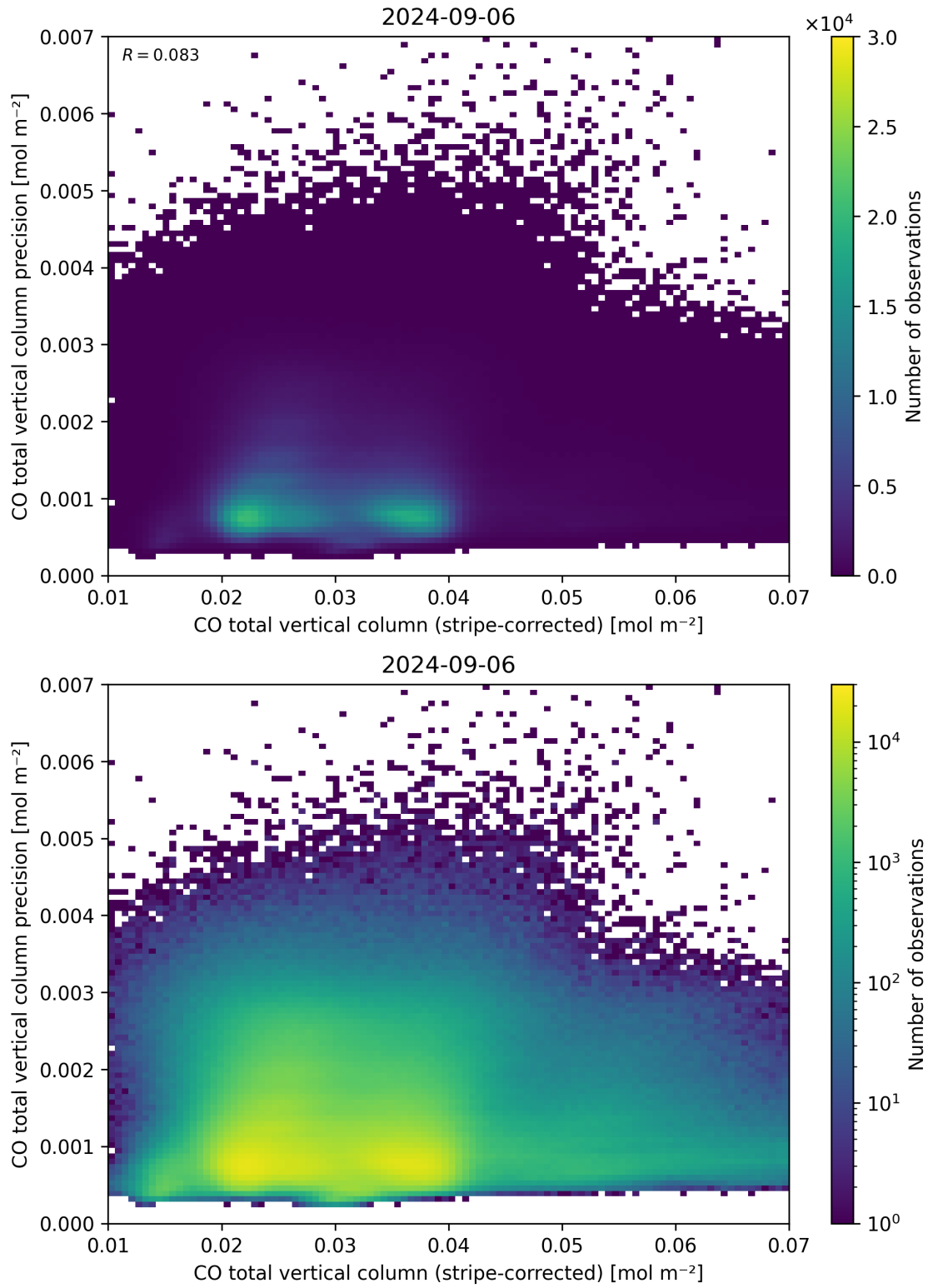
Figure 36: Scatter density plot of “CO total vertical column (stripe-corrected)” against “CO total vertical column precision” for 2024-09-06 to 2024-09-07.
