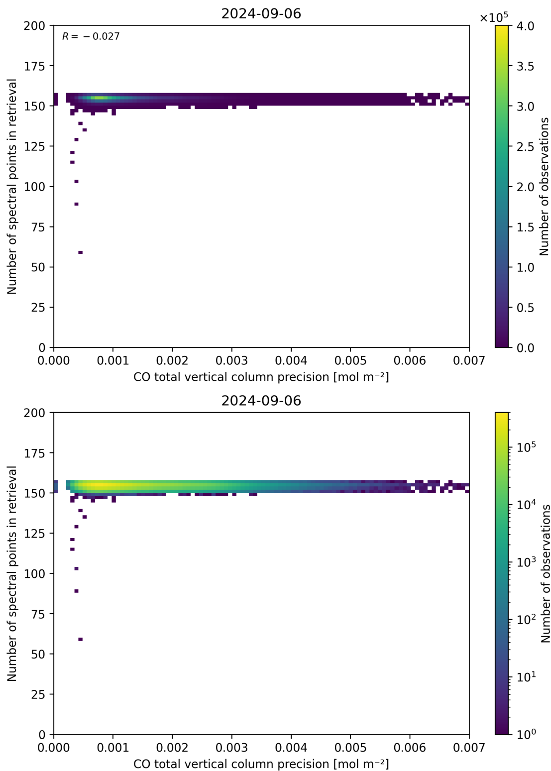
Figure 47: Scatter density plot of “CO total vertical column precision” against “Number of spectral points in retrieval” for 2024-09-06 to 2024-09-07.
