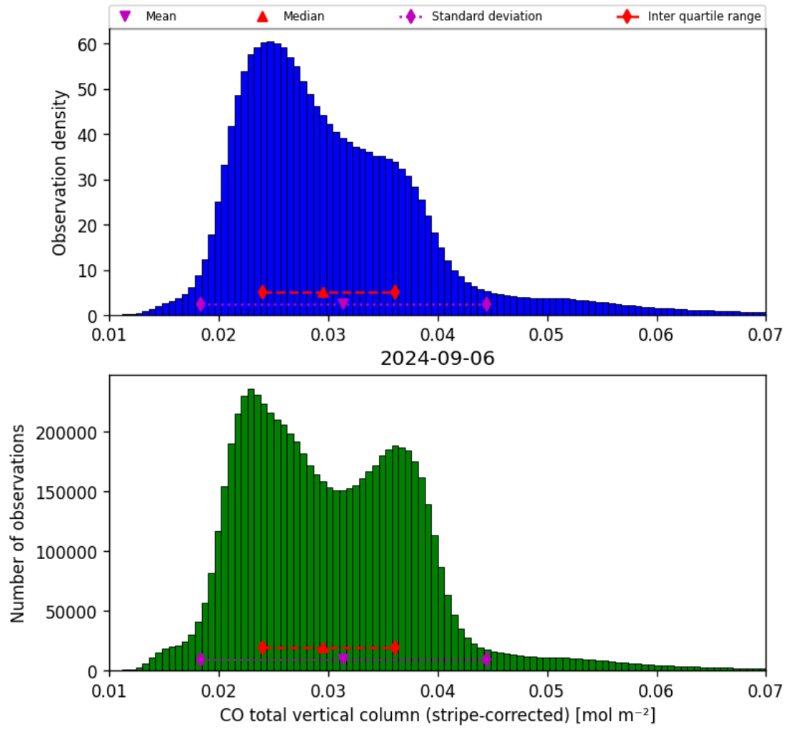
Figure 19: Histogram of “CO total vertical column (stripe-corrected)” for 2024-09-06 to 2024-09-07
