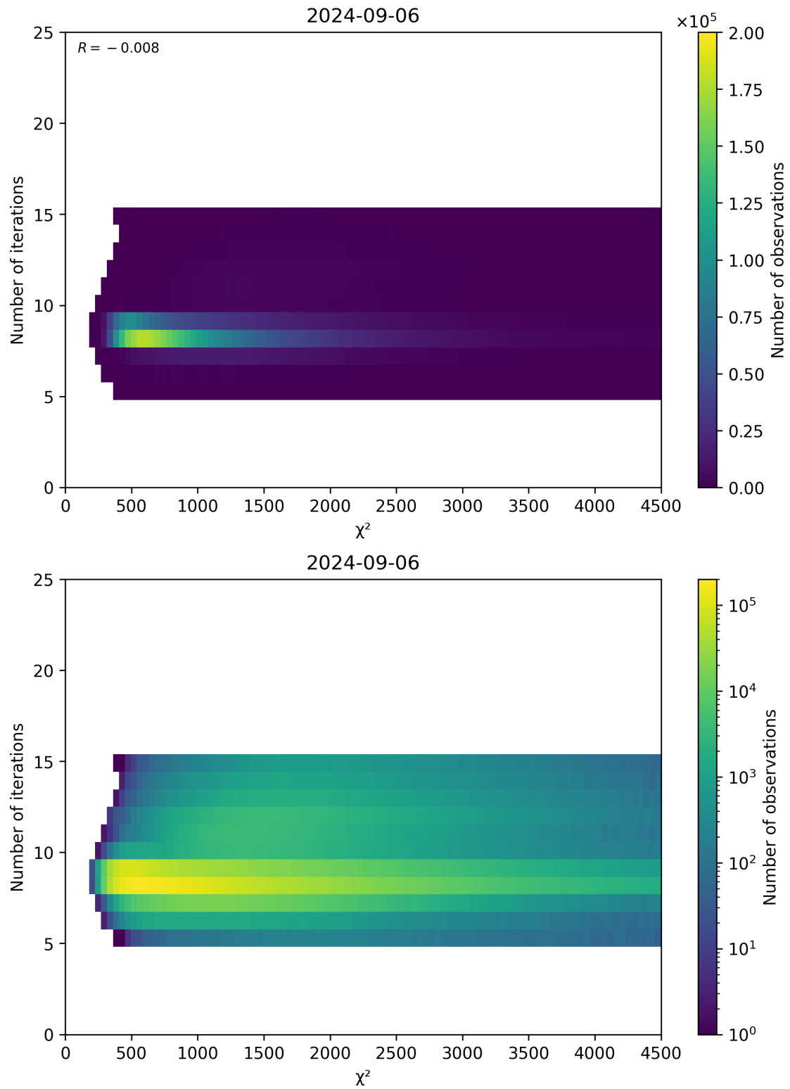
Figure 49: Scatter density plot of “ \chi^2 ” against “Number of iterations” for 2024-09-06 to 2024-09-07.
