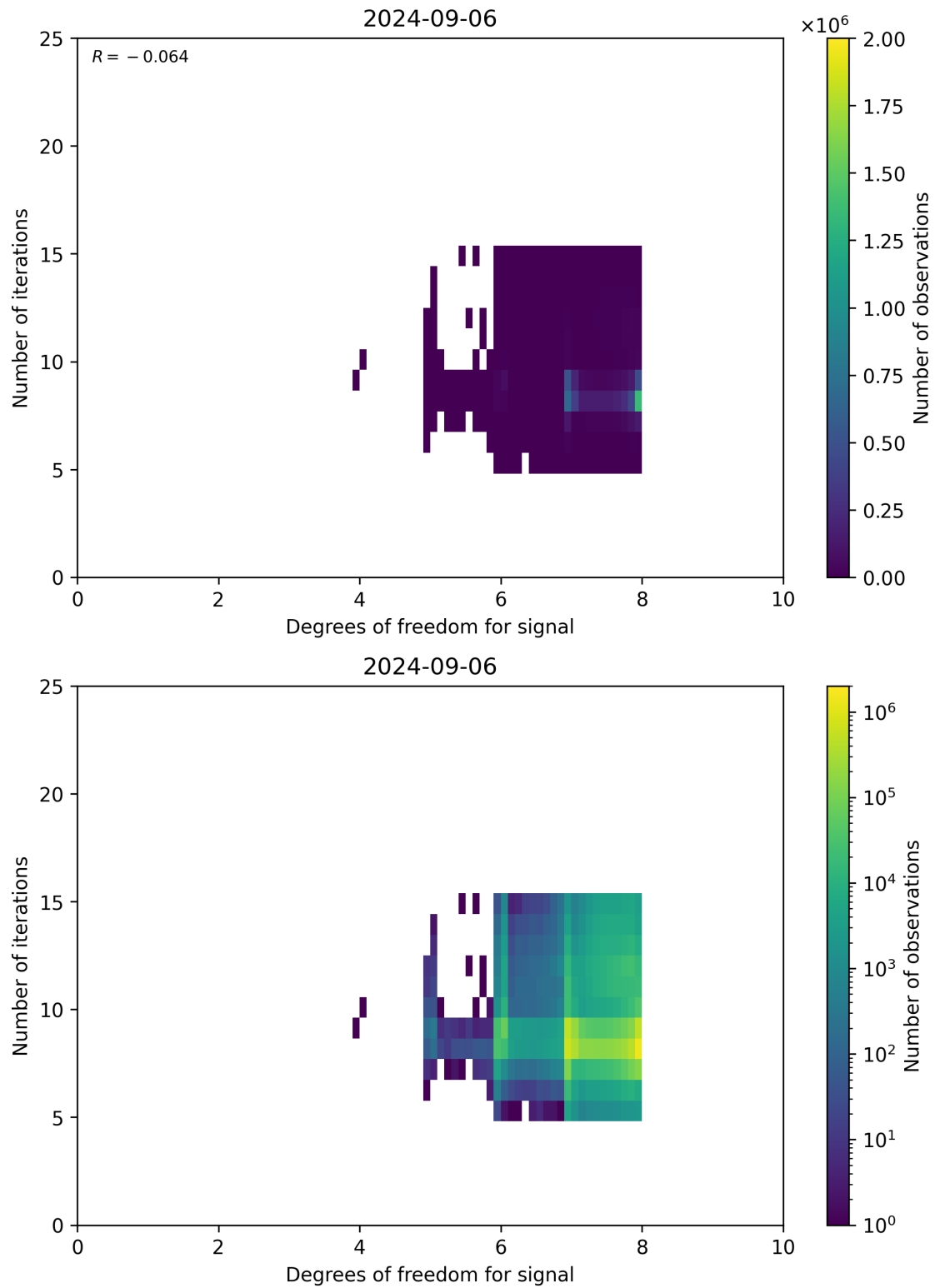
Figure 50: Scatter density plot of “Degrees of freedom for signal” against “Number of iterations” for 2024-09-06 to 2024-09-07.
