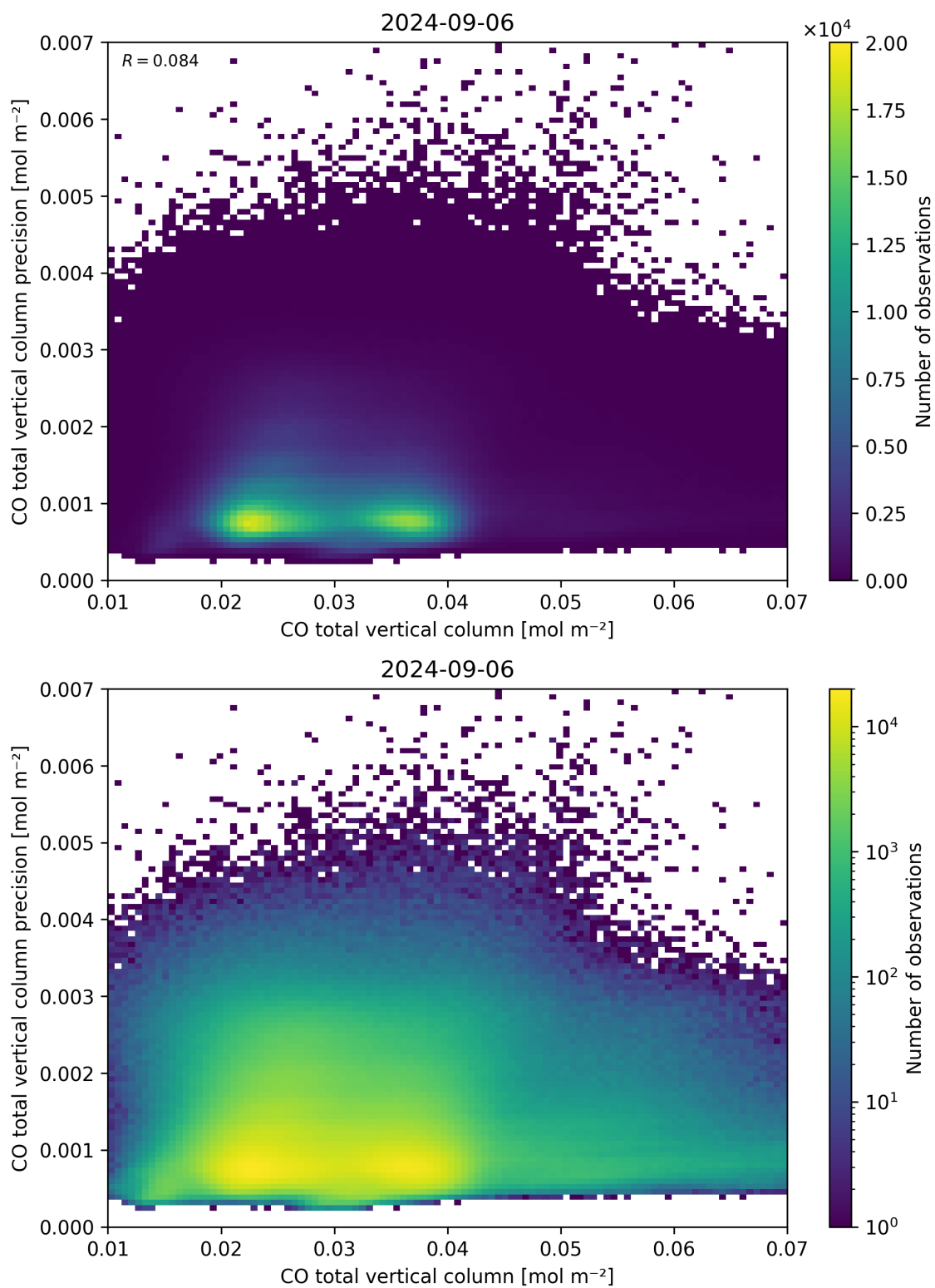
Figure 34: Scatter density plot of “CO total vertical column” against “CO total vertical column precision” for 2024-09-06 to 2024-09-07.
