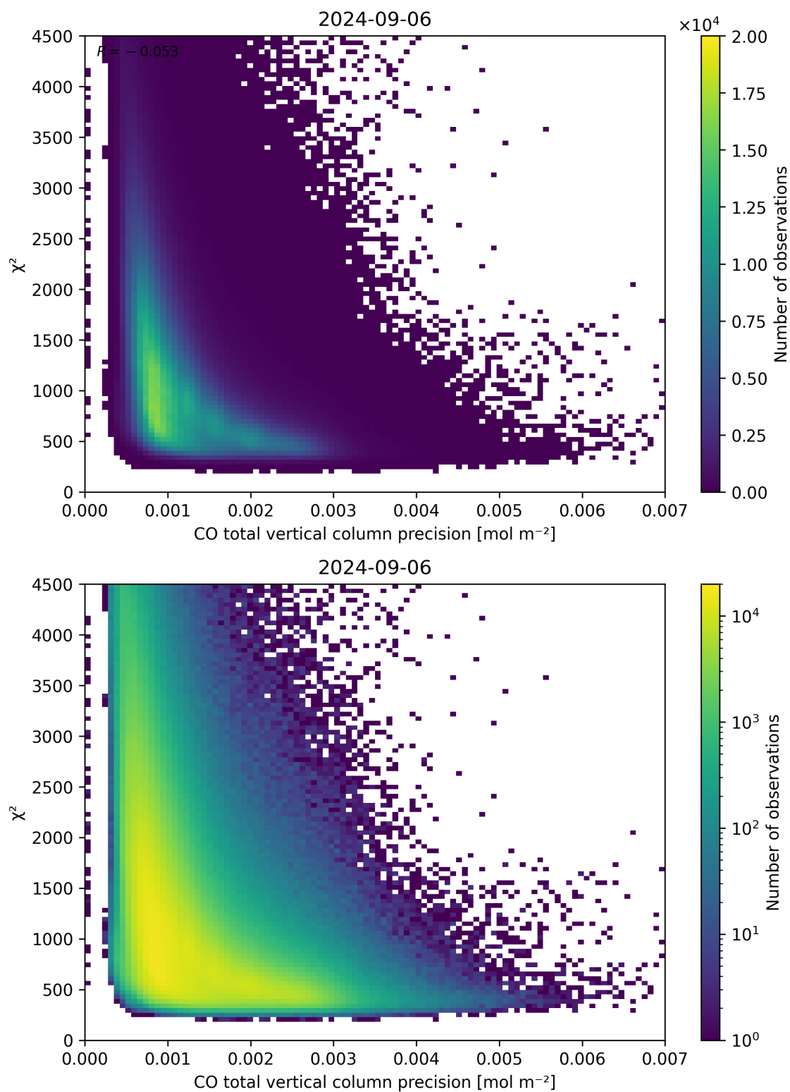
Figure 44: Scatter density plot of “CO total vertical column precision” against “ \chi^2 ” for 2024-09-06 to 2024-09-07.
