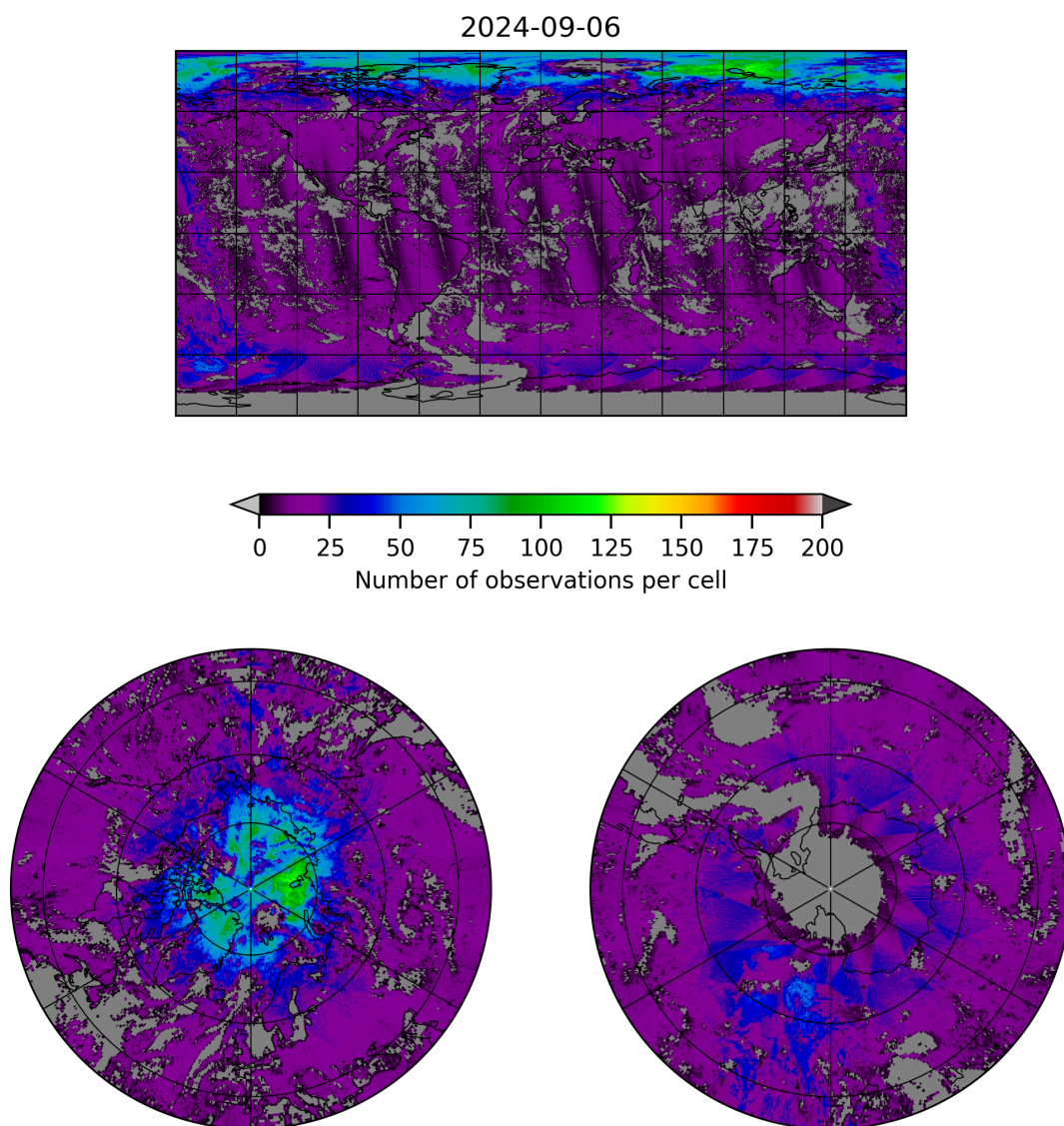
Figure 8: Map of the number of observations for 2024-09-06 to 2024-09-07
