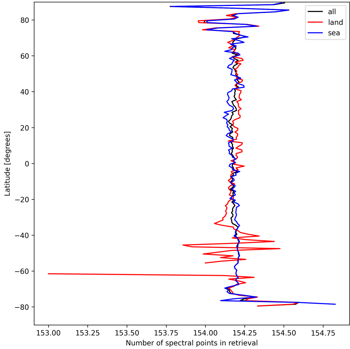
Figure 13: Zonal average of “Number of spectral points in retrieval” for 2024-09-06 to 2024-09-07.
