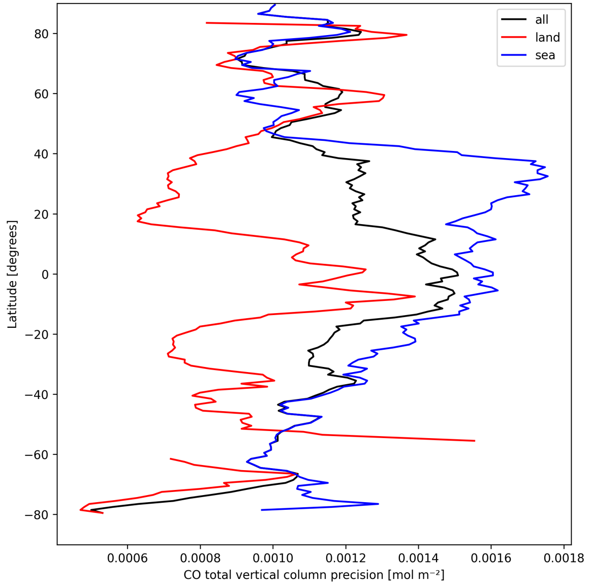
Figure 12: Zonal average of “CO total vertical column precision” for 2024-09-06 to 2024-09-07.
