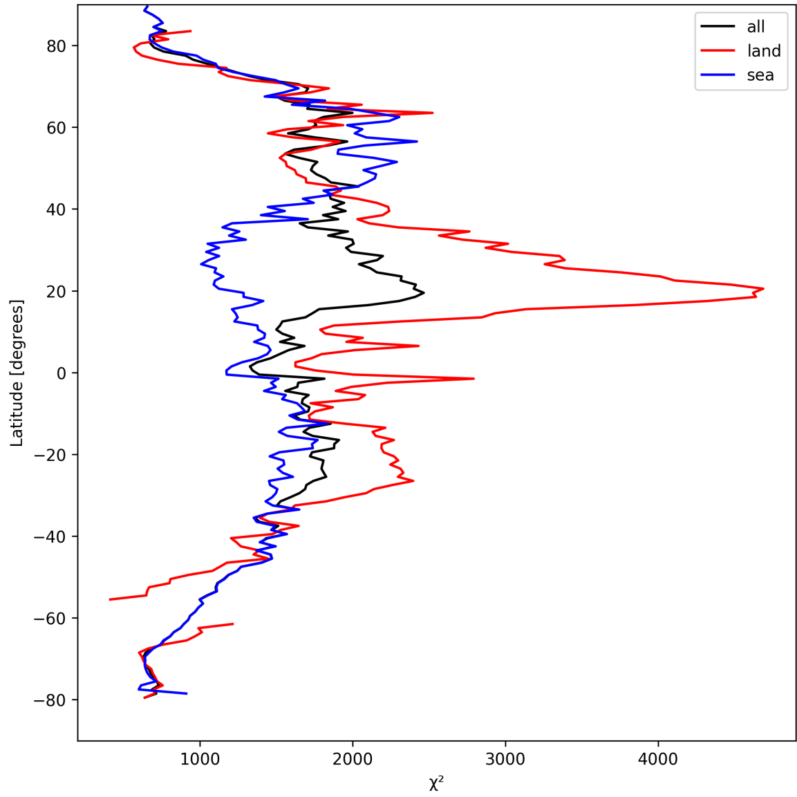
Figure 14: Zonal average of “ \chi^2 ” for 2024-09-06 to 2024-09-07.
