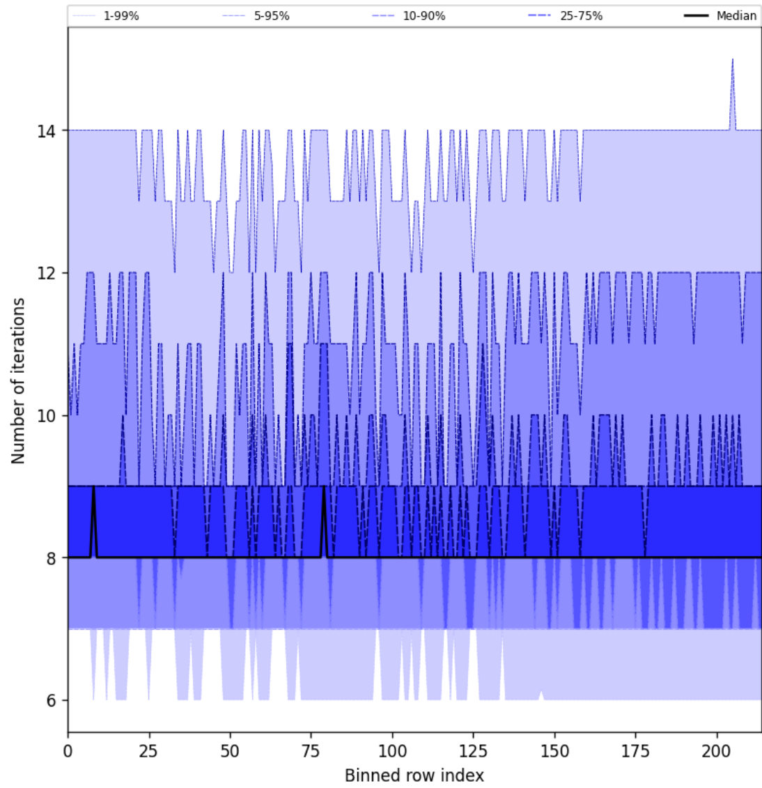
Figure 32: Along track statistics of “Number of iterations” for 2024-09-06 to 2024-09-07
