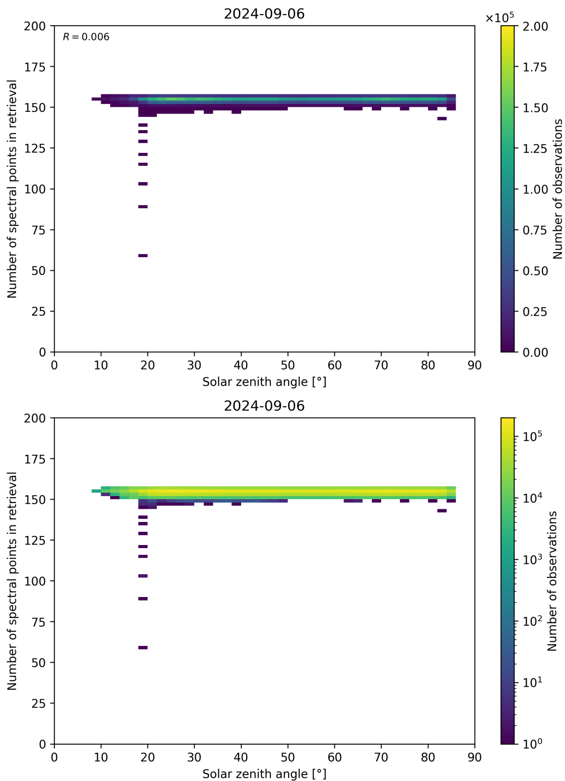
Figure 68: Scatter density plot of “Solar zenith angle” against “Number of spectral points in retrieval” for 2024-09-06 to 2024-09-07.
