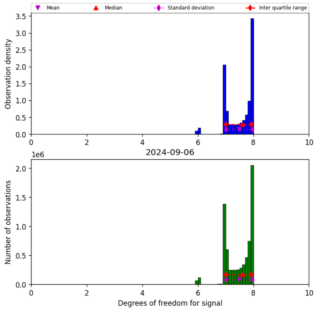
Figure 23: Histogram of “Degrees of freedom for signal” for 2024-09-06 to 2024-09-07
