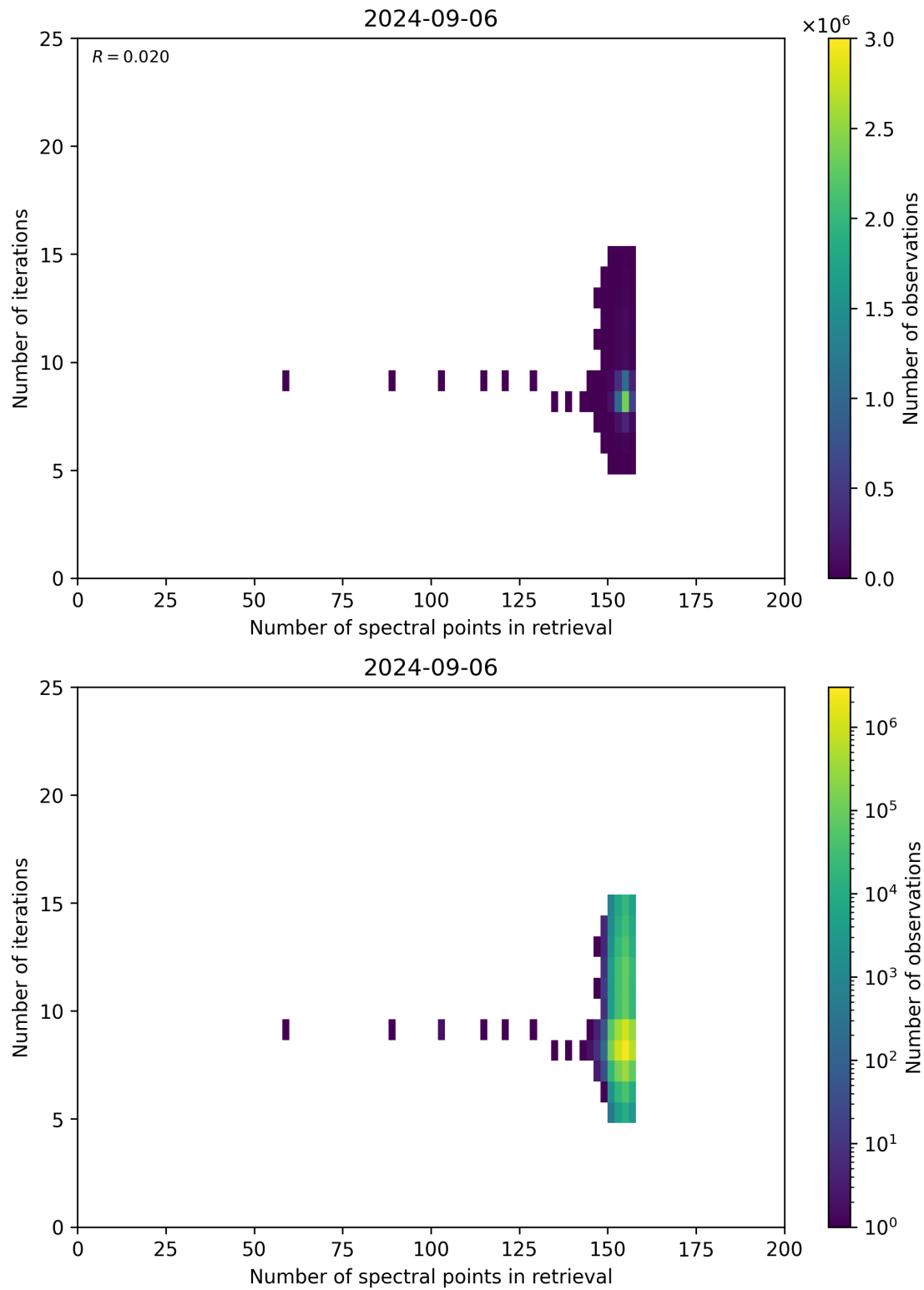
Figure 60: Scatter density plot of “Number of spectral points in retrieval” against “Number of iterations” for 2024-09-06 to 2024-09-07.
