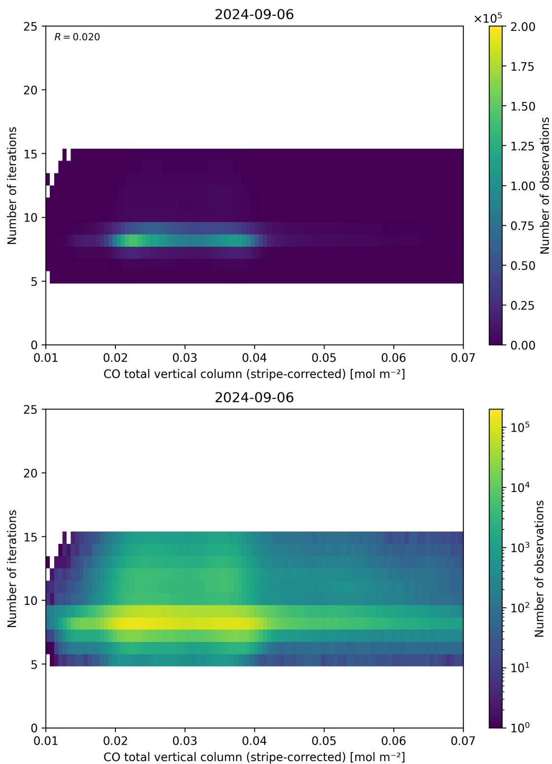
Figure 39: Scatter density plot of “CO total vertical column (stripe-corrected)” against “Number of iterations” for 2024-09-06 to 2024-09-07.
