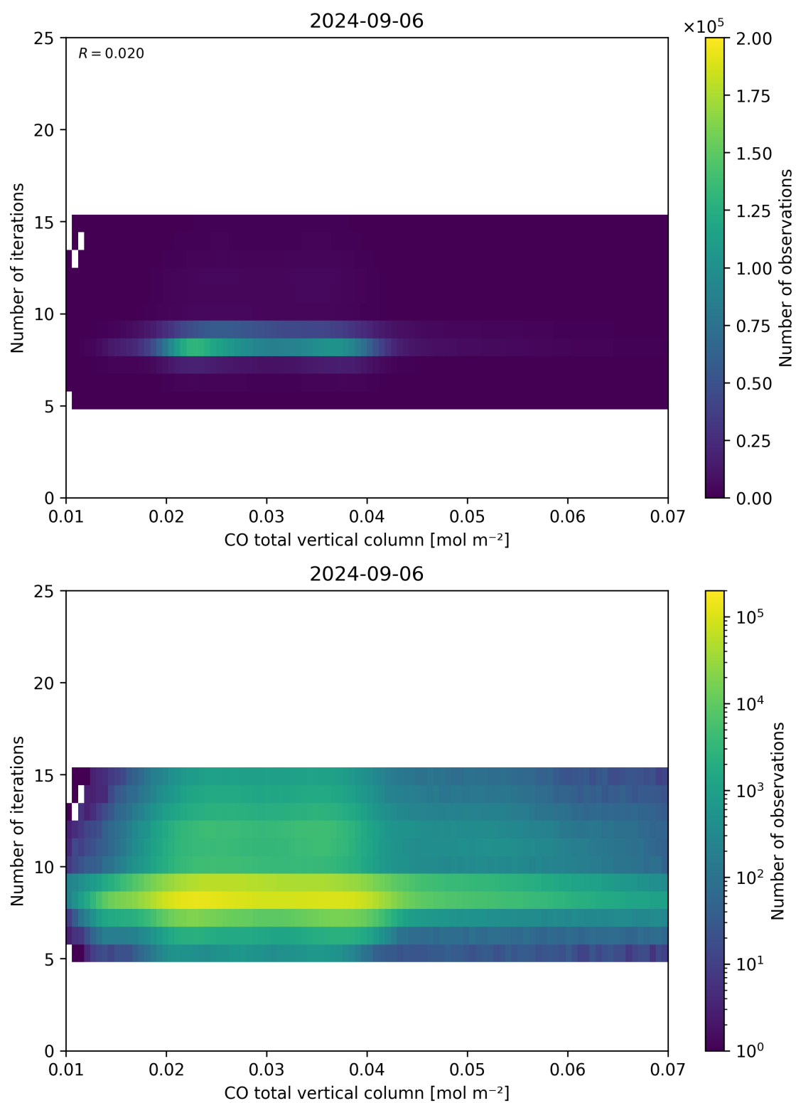
Figure 42: Scatter density plot of “CO total vertical column” against “Number of iterations” for 2024-09-06 to 2024-09-07.
