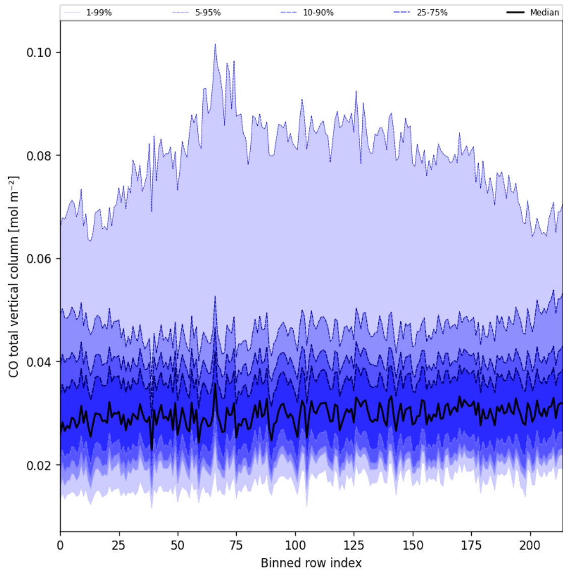
Figure 26: Along track statistics of “CO total vertical column” for 2024-09-06 to 2024-09-07
