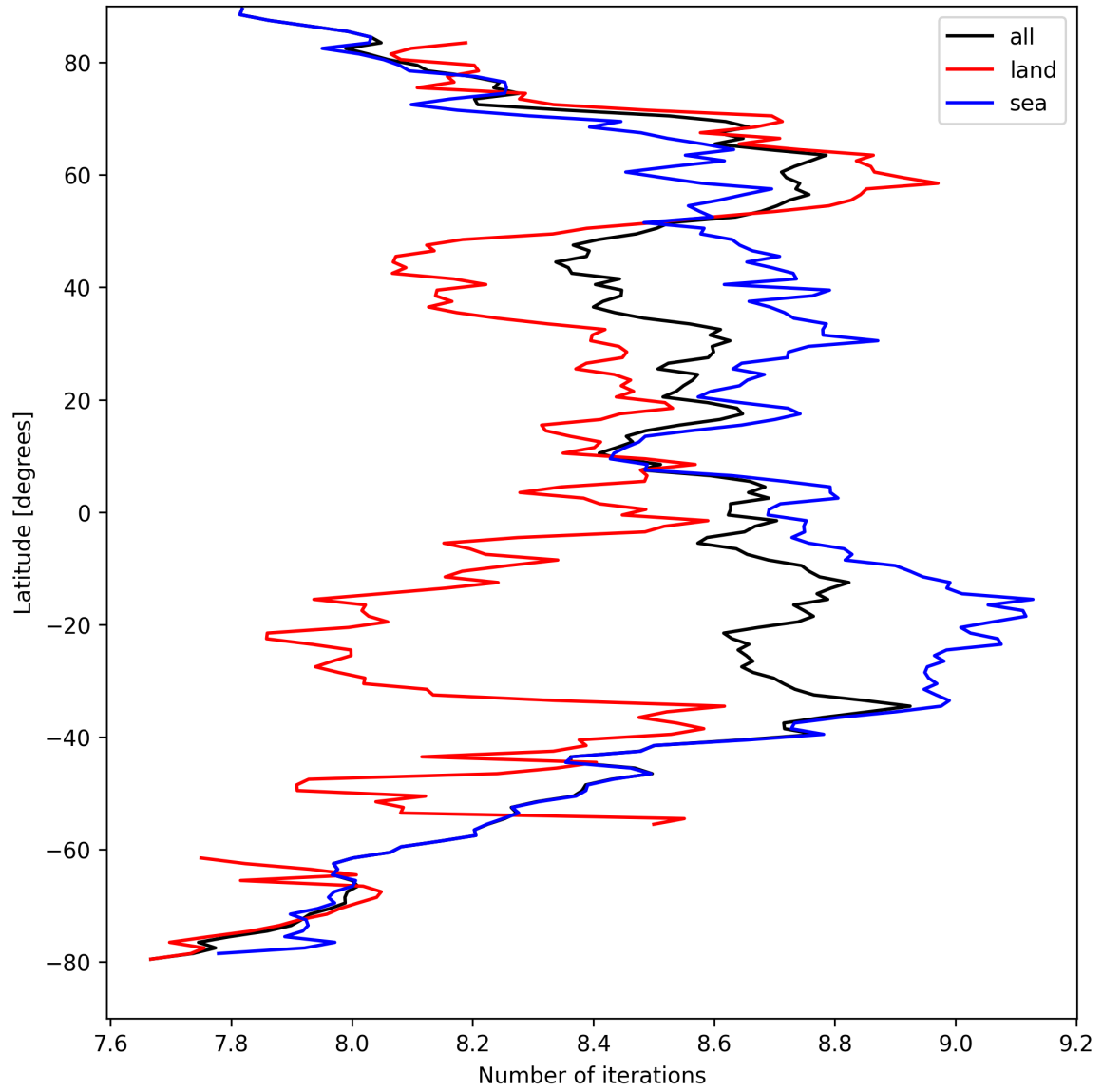
Figure 16: Zonal average of “Number of iterations” for 2024-09-06 to 2024-09-07.
