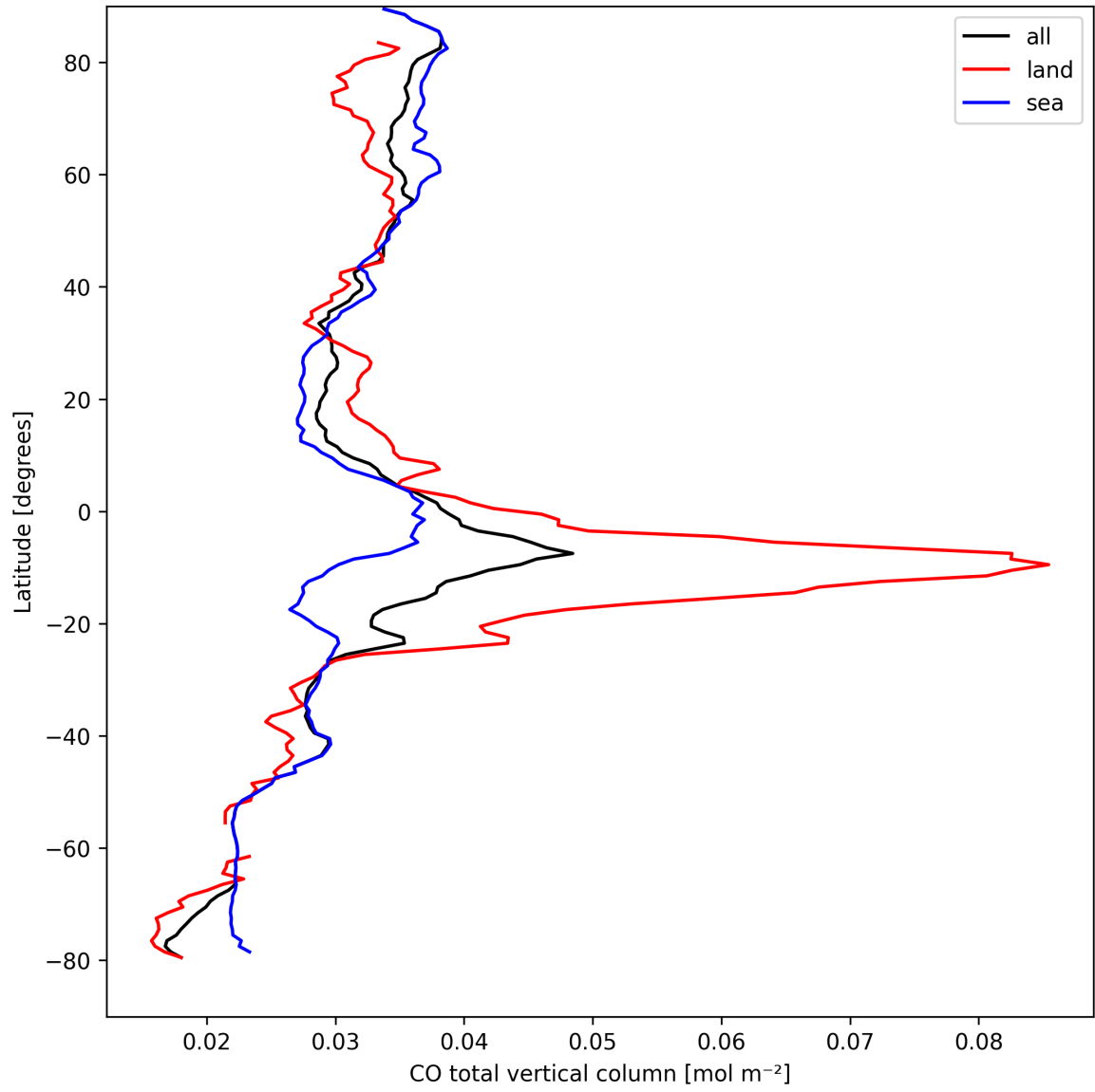
Figure 10: Zonal average of “CO total vertical column” for 2024-09-06 to 2024-09-07.
