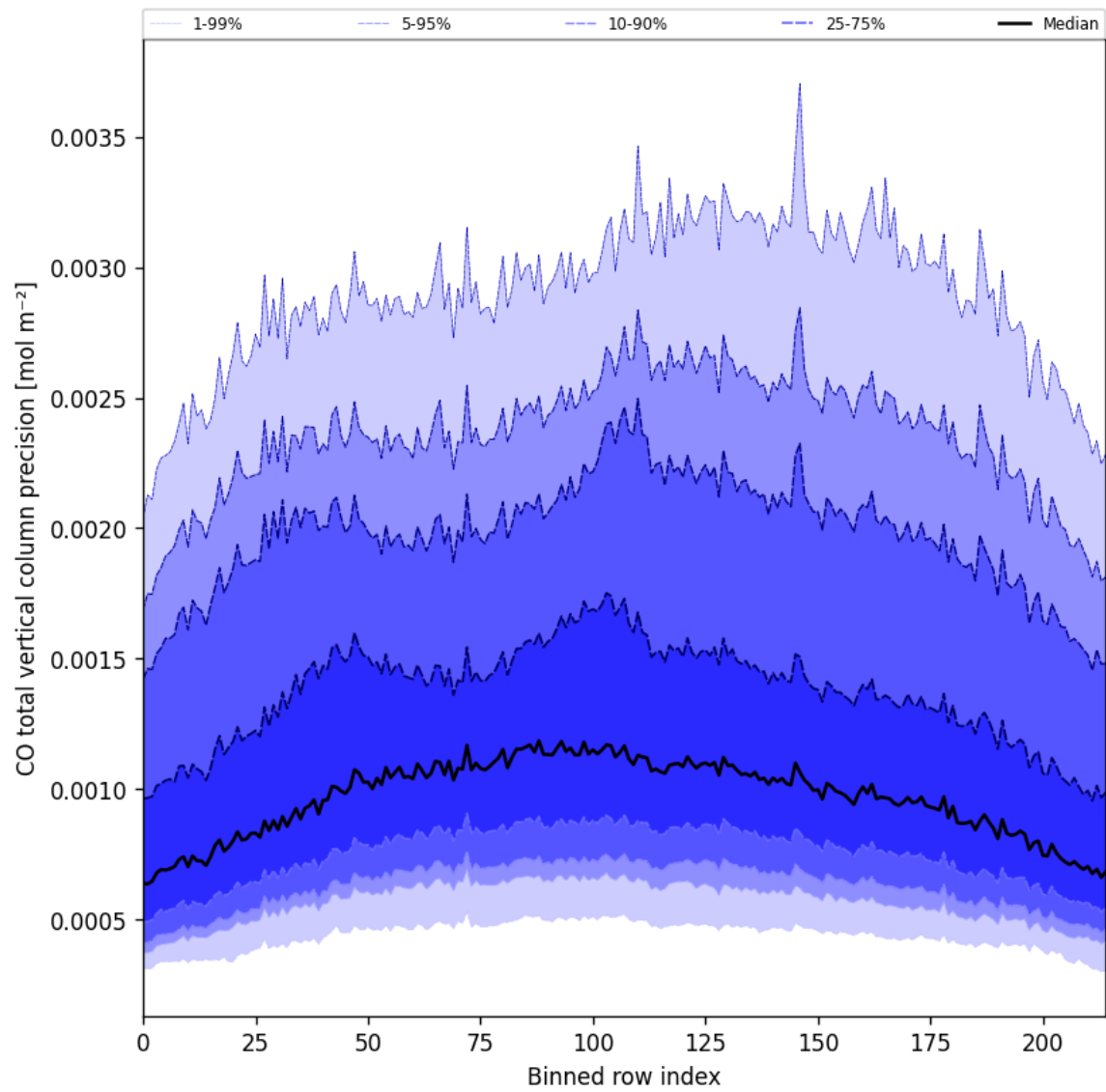
Figure 28: Along track statistics of “CO total vertical column precision” for 2024-09-06 to 2024-09-07
