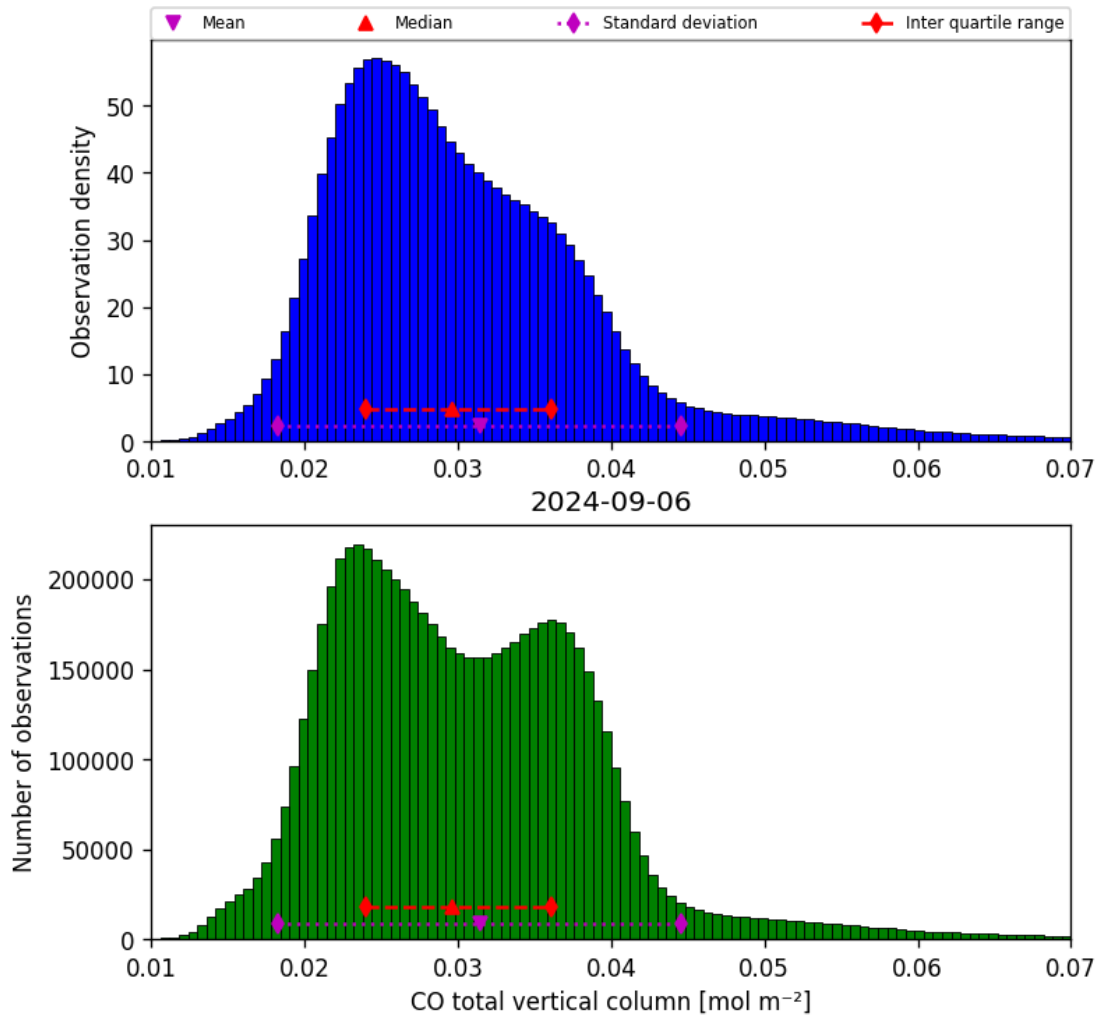
Figure 18: Histogram of “CO total vertical column” for 2024-09-06 to 2024-09-07
