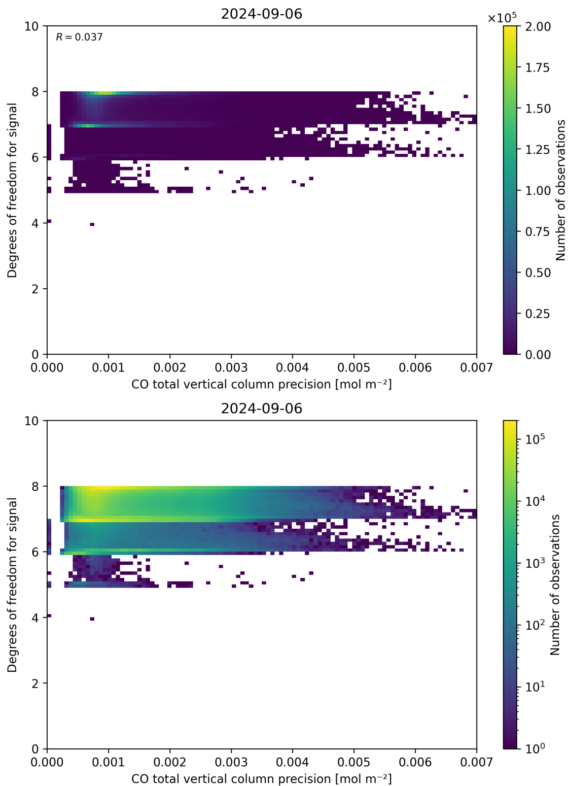
Figure 45: Scatter density plot of “CO total vertical column precision” against “Degrees of freedom for signal” for 2024-09-06 to 2024-09-07.
