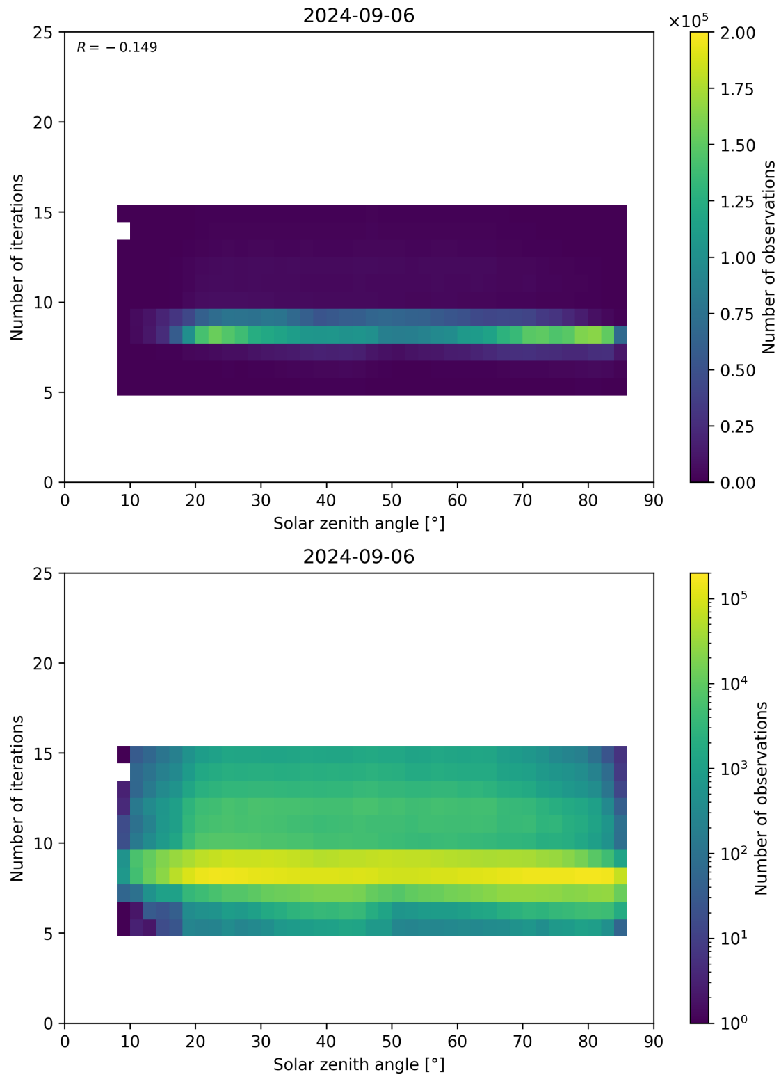
Figure 67: Scatter density plot of “Solar zenith angle” against “Number of iterations” for 2024-09-06 to 2024-09-07.
