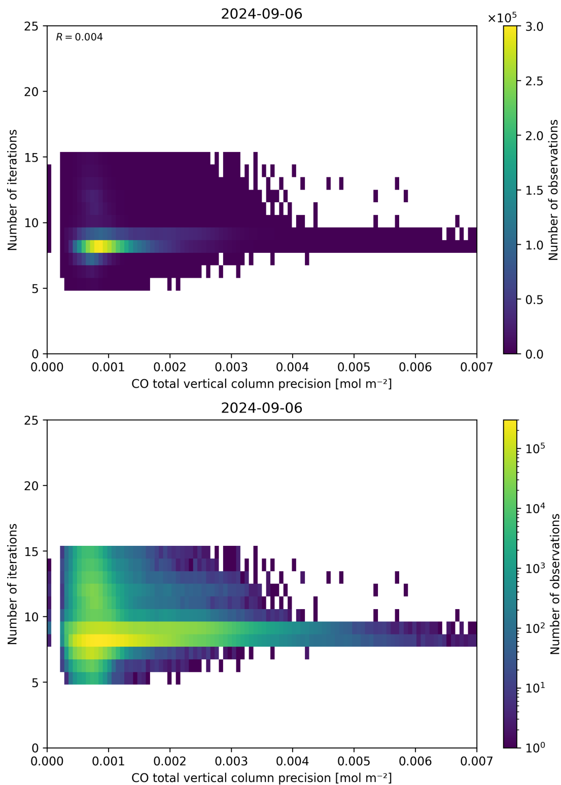
Figure 46: Scatter density plot of “CO total vertical column precision” against “Number of iterations” for 2024-09-06 to 2024-09-07.
