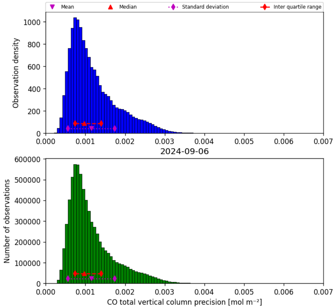
Figure 20: Histogram of “CO total vertical column precision” for 2024-09-06 to 2024-09-07
