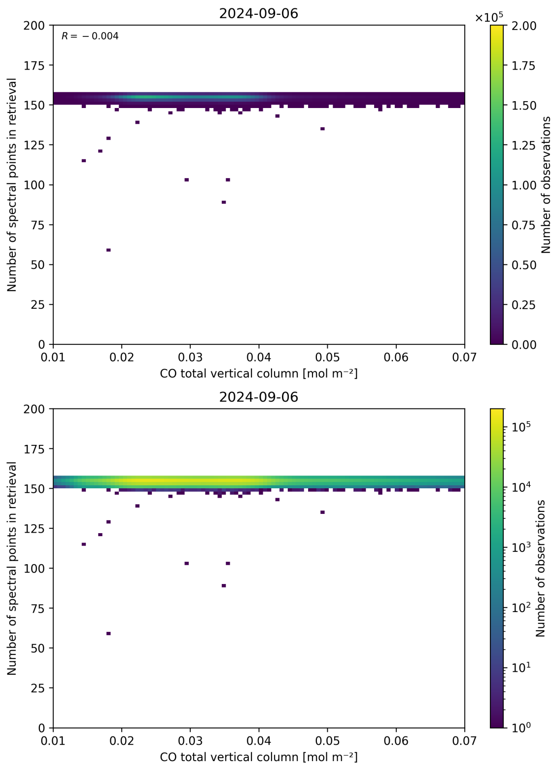
Figure 43: Scatter density plot of “CO total vertical column” against “Number of spectral points in retrieval” for 2024-09-06 to 2024-09-07.
