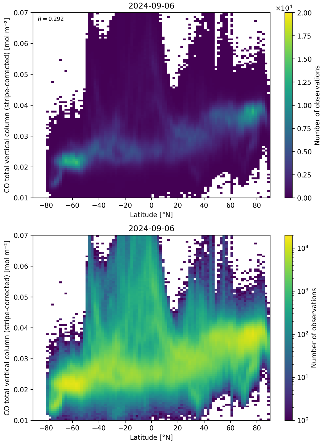
Figure 52: Scatter density plot of “Latitude” against “CO total vertical column (stripe-corrected)” for 2024-09-06 to 2024-09-07.
