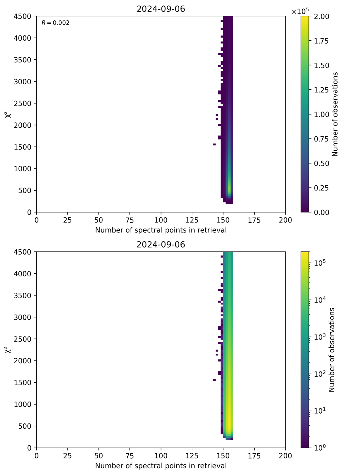
Figure 58: Scatter density plot of “Number of spectral points in retrieval” against “ \chi^2 ” for 2024-09-06 to 2024-09-07.
