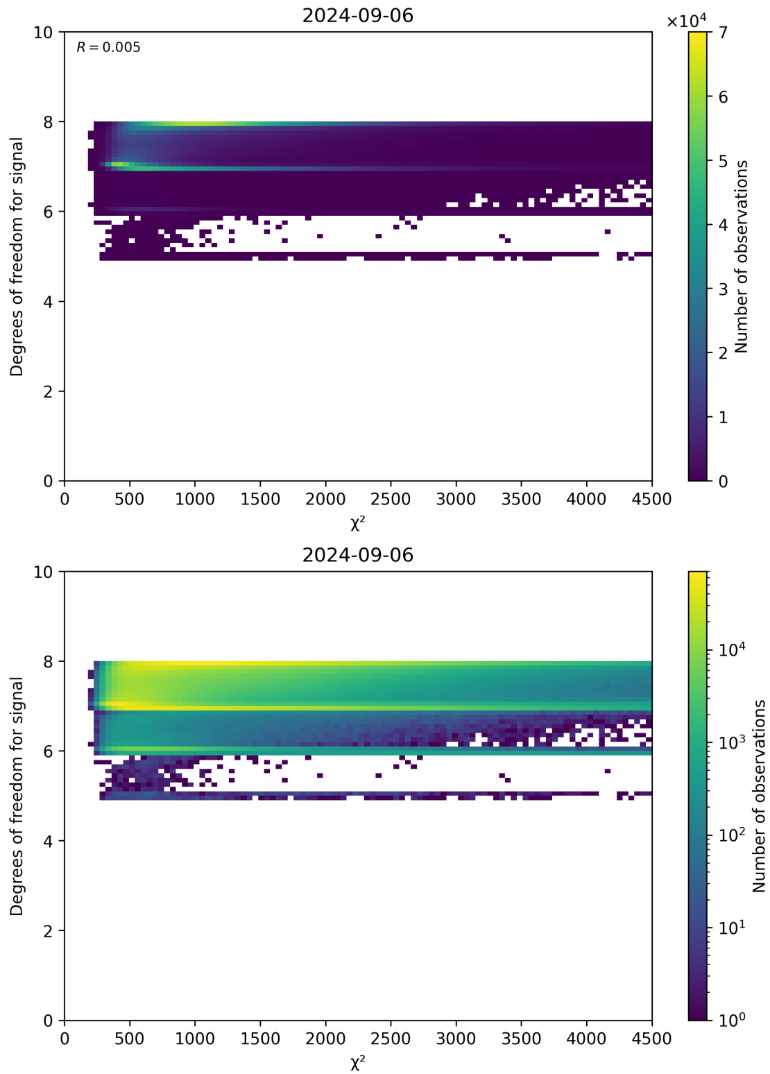
Figure 48: Scatter density plot of “ \chi^2 ” against “Degrees of freedom for signal” for 2024-09-06 to 2024-09-07.
