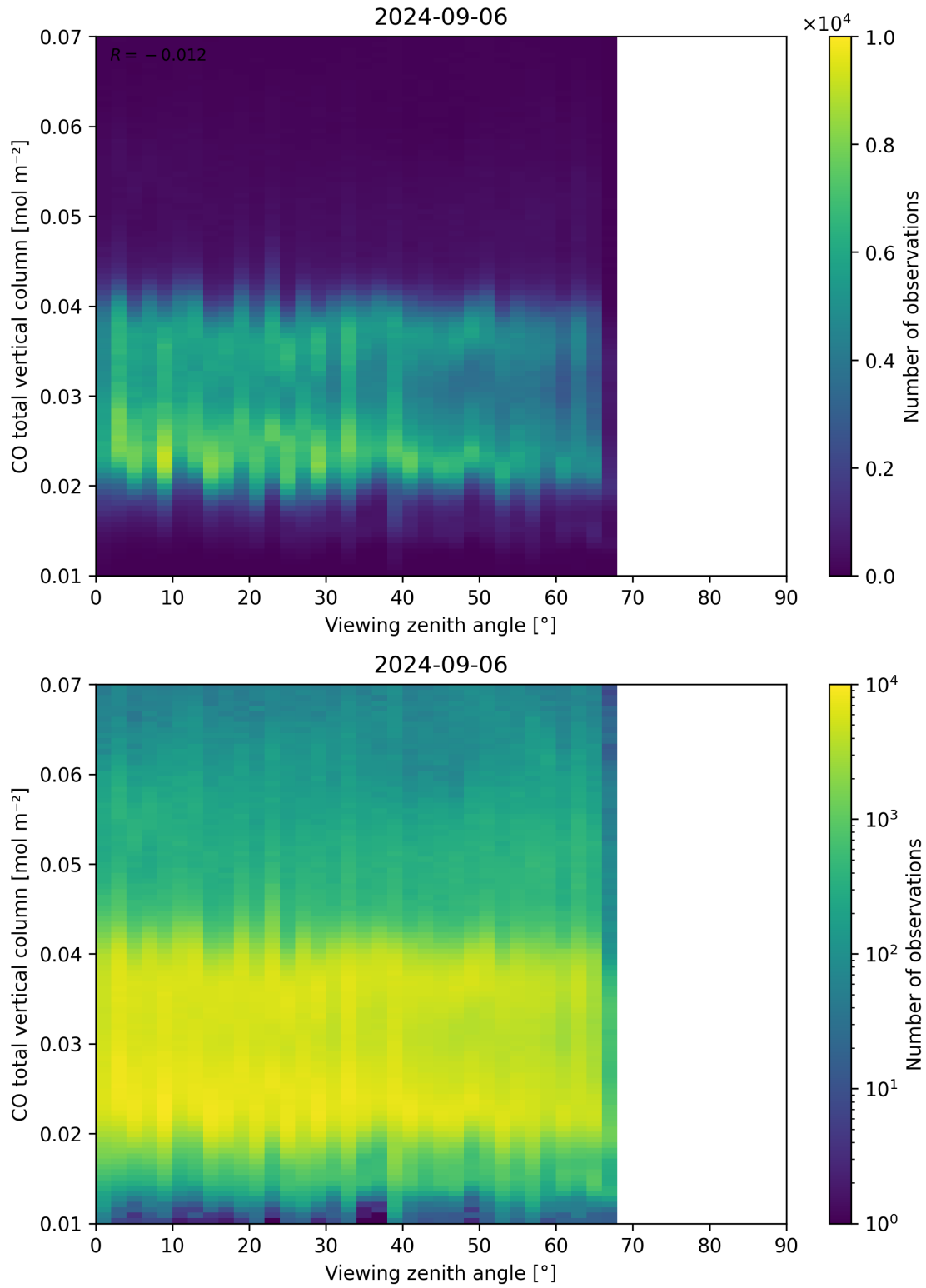
Figure 69: Scatter density plot of “Viewing zenith angle” against “CO total vertical column” for 2024-09-06 to 2024-09-07.
