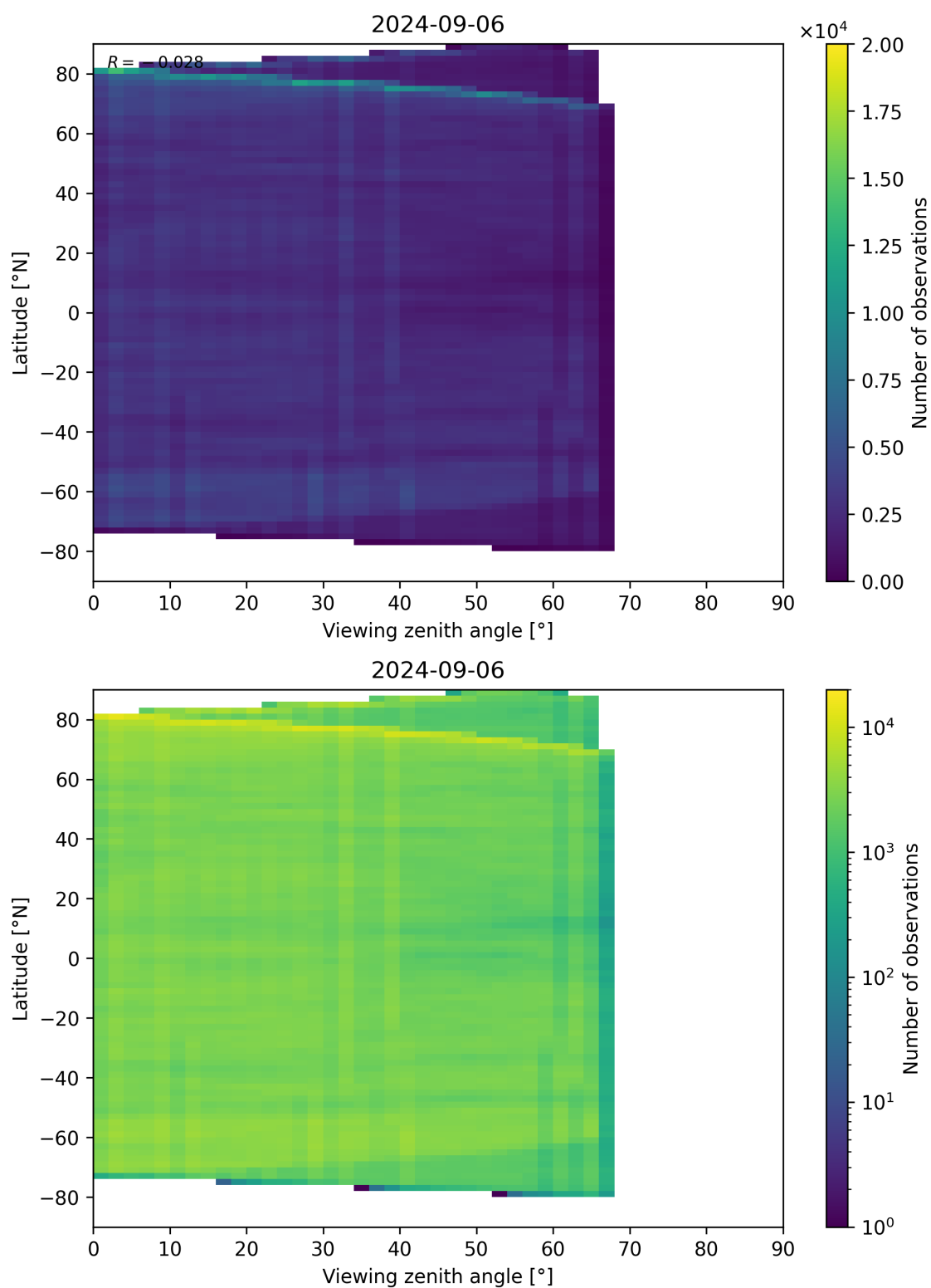
Figure 74: Scatter density plot of “Viewing zenith angle” against “Latitude” for 2024-09-06 to 2024-09-07.
