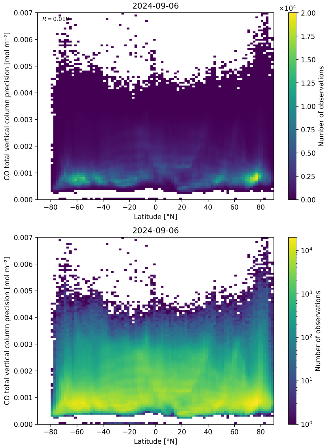
Figure 53: Scatter density plot of “Latitude” against “CO total vertical column precision” for 2024-09-06 to 2024-09-07.
