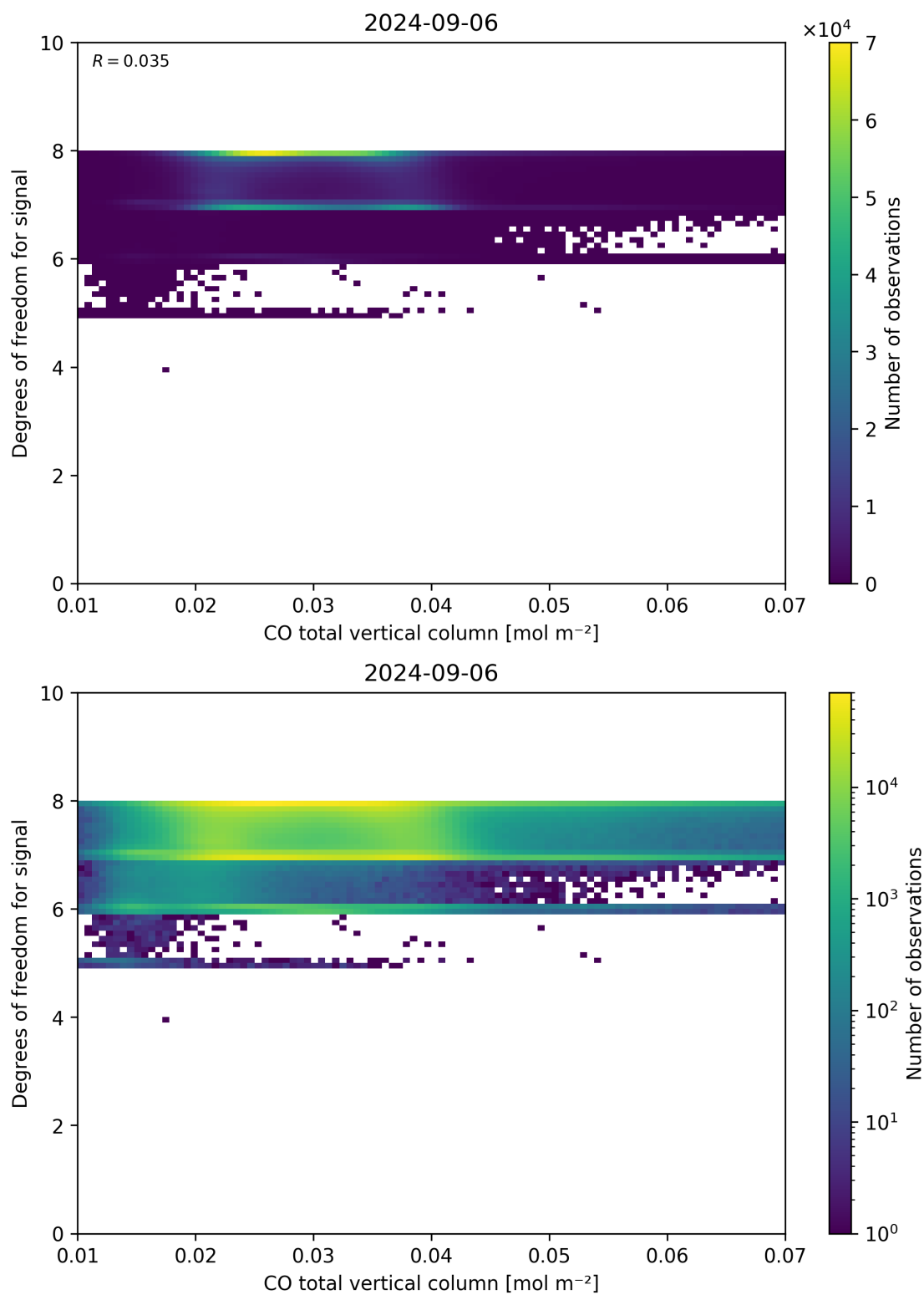
Figure 41: Scatter density plot of “CO total vertical column” against “Degrees of freedom for signal” for 2024-09-06 to 2024-09-07.
