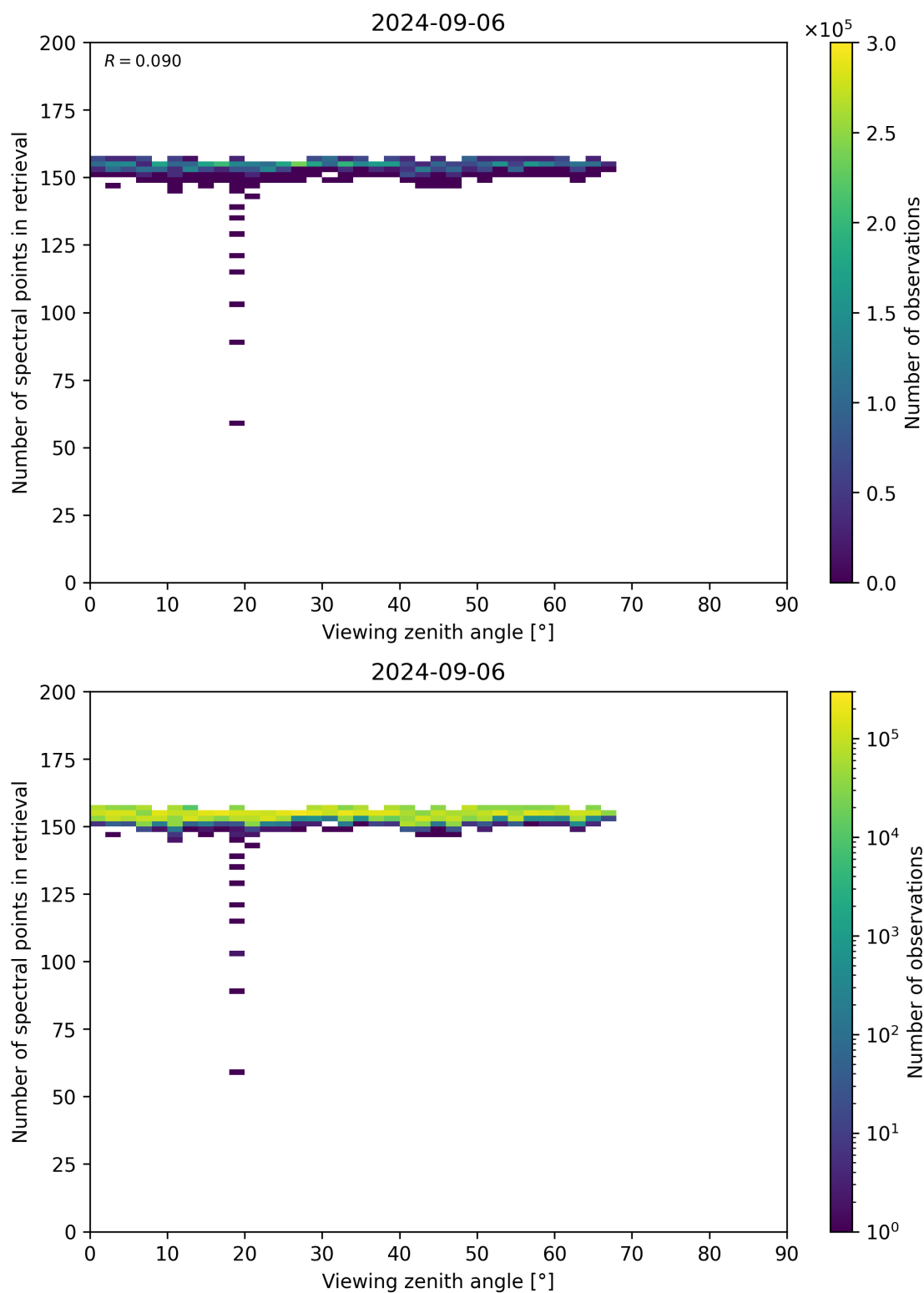
Figure 76: Scatter density plot of “Viewing zenith angle” against “Number of spectral points in retrieval” for 2024-09-06 to 2024-09-07.
