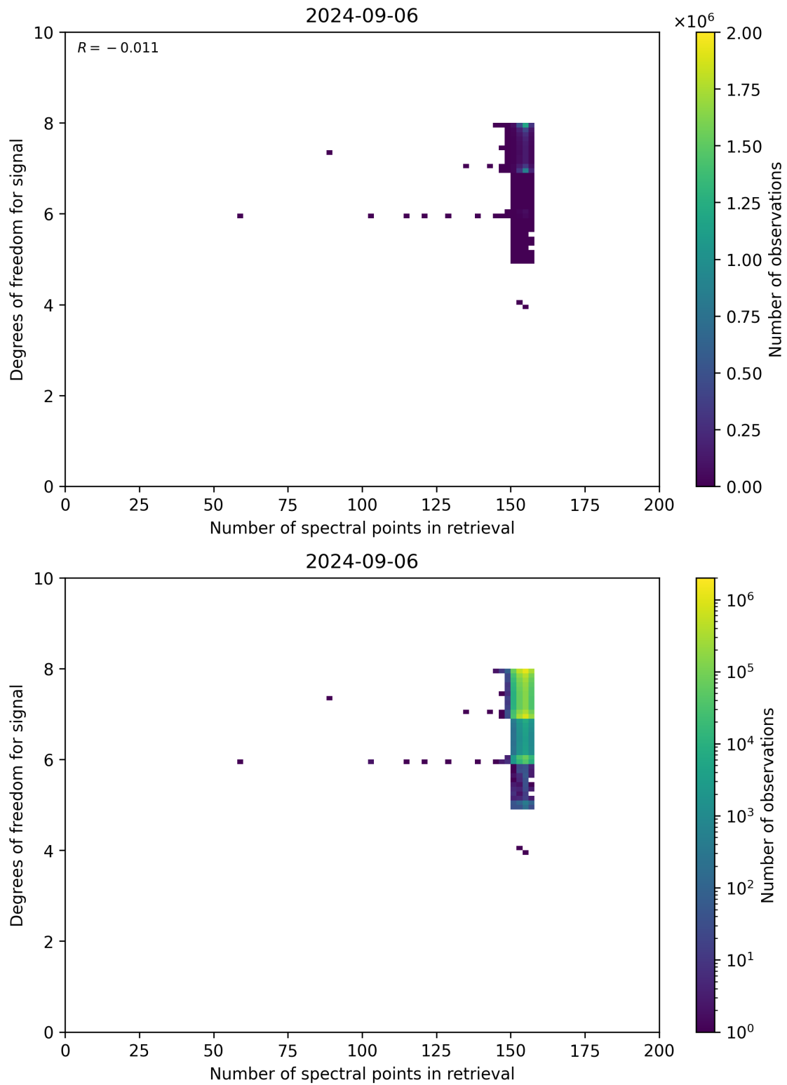
Figure 59: Scatter density plot of “Number of spectral points in retrieval” against “Degrees of freedom for signal” for 2024-09-06 to 2024-09-07.
