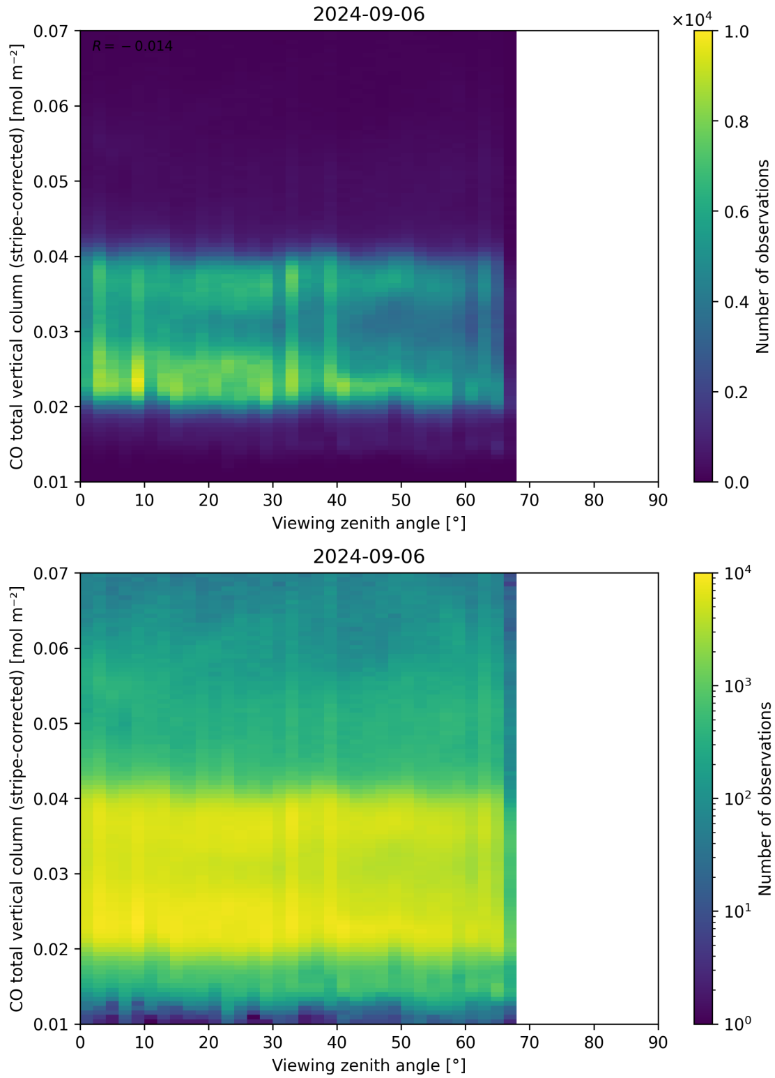
Figure 70: Scatter density plot of “Viewing zenith angle” against “CO total vertical column (stripe-corrected)” for 2024-09-06 to 2024-09-07.
