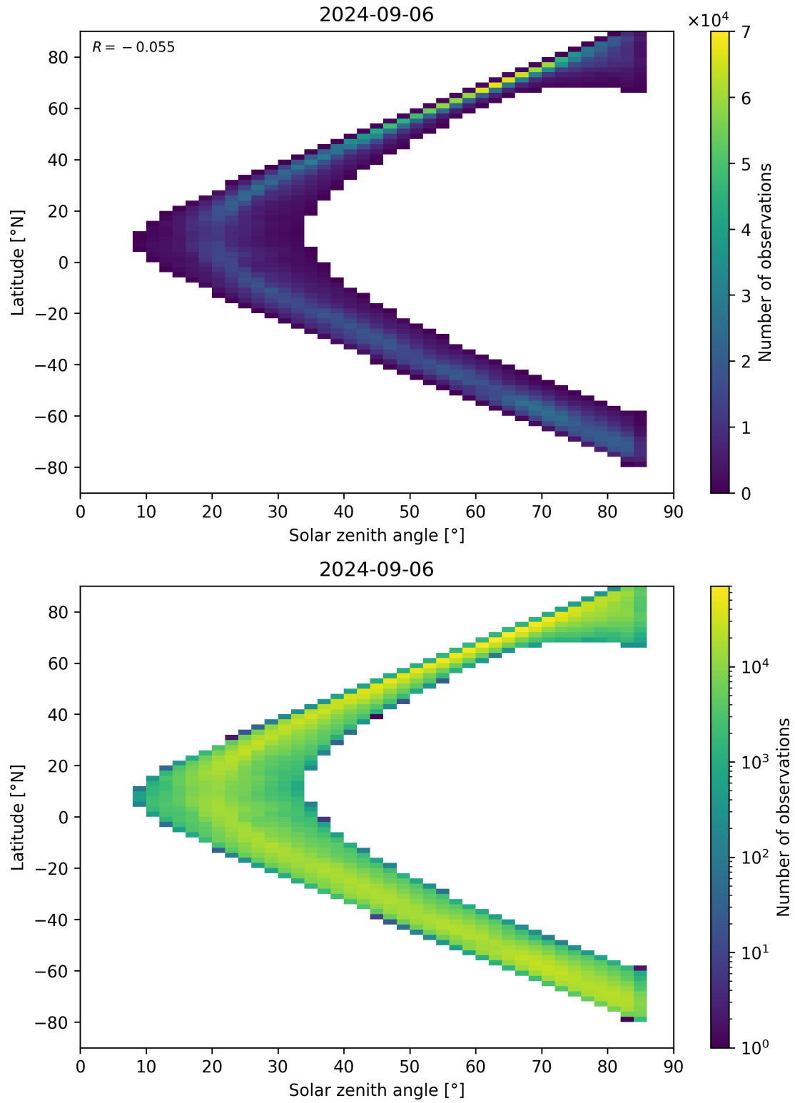
Figure 66: Scatter density plot of “Solar zenith angle” against “Latitude” for 2024-09-06 to 2024-09-07.
