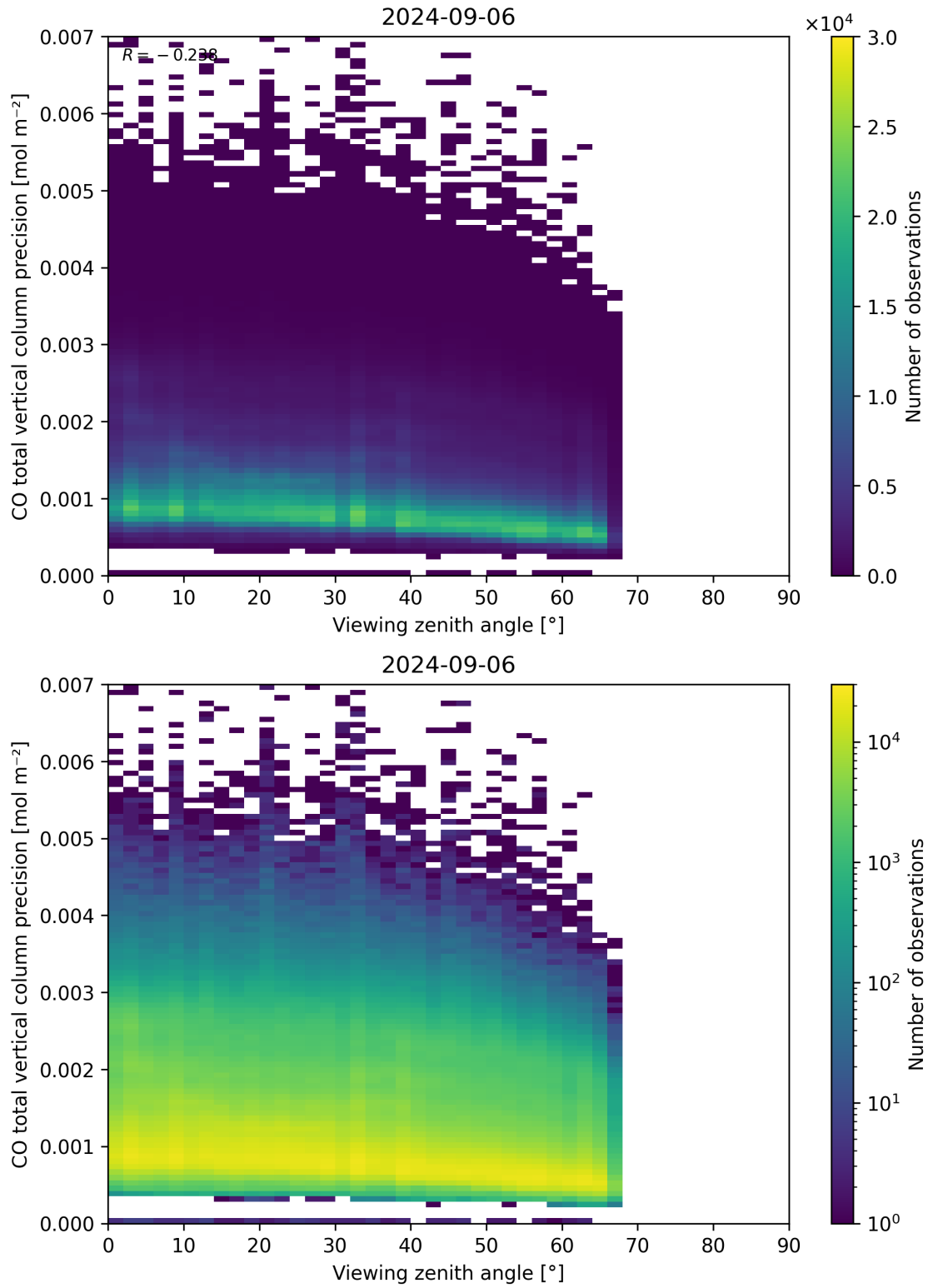
Figure 71: Scatter density plot of “Viewing zenith angle” against “CO total vertical column precision” for 2024-09-06 to 2024-09-07.
