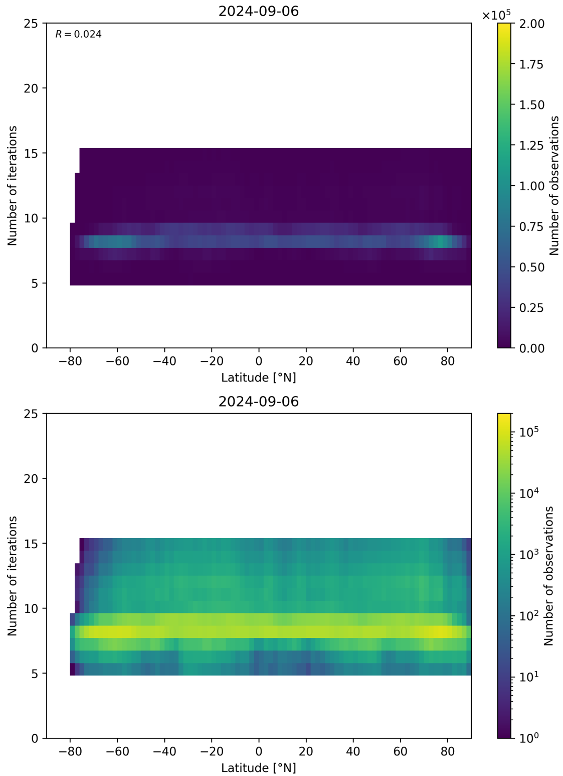
Figure 56: Scatter density plot of “Latitude” against “Number of iterations” for 2024-09-06 to 2024-09-07.
