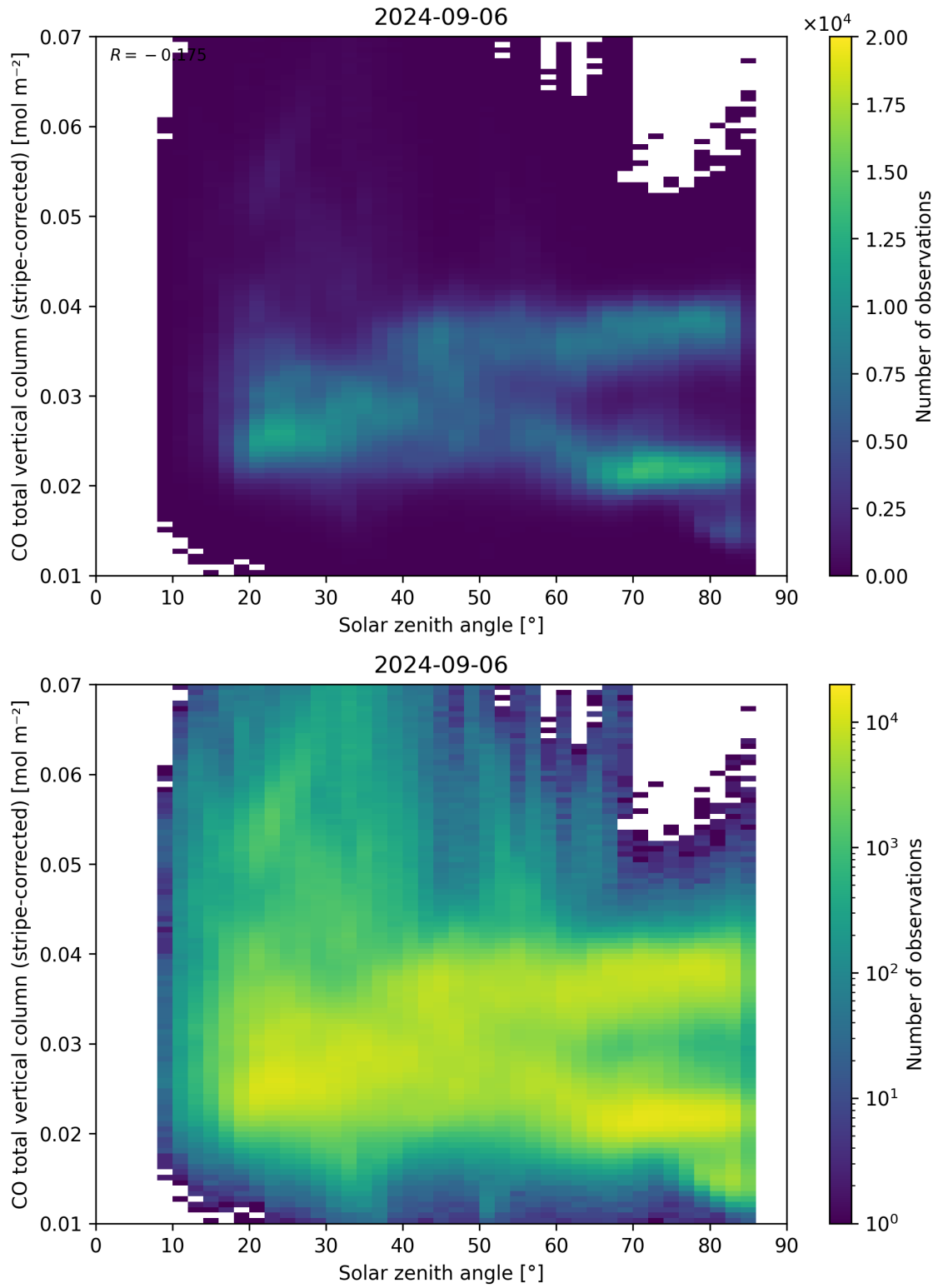
Figure 62: Scatter density plot of “Solar zenith angle” against “CO total vertical column (stripe-corrected)” for 2024-09-06 to 2024-09-07.
