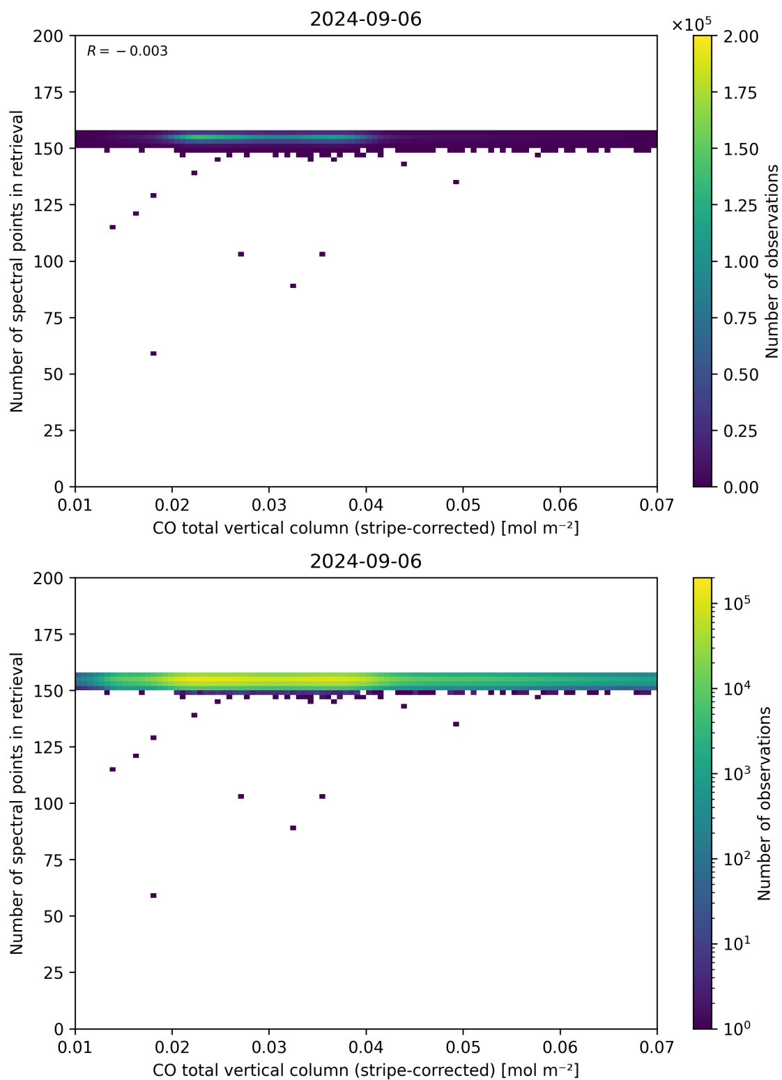
Figure 40: Scatter density plot of “CO total vertical column (stripe-corrected)” against “Number of spectral points in retrieval” for 2024-09-06 to 2024-09-07.
