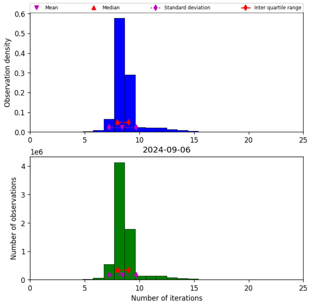
Figure 24: Histogram of “Number of iterations” for 2024-09-06 to 2024-09-07
