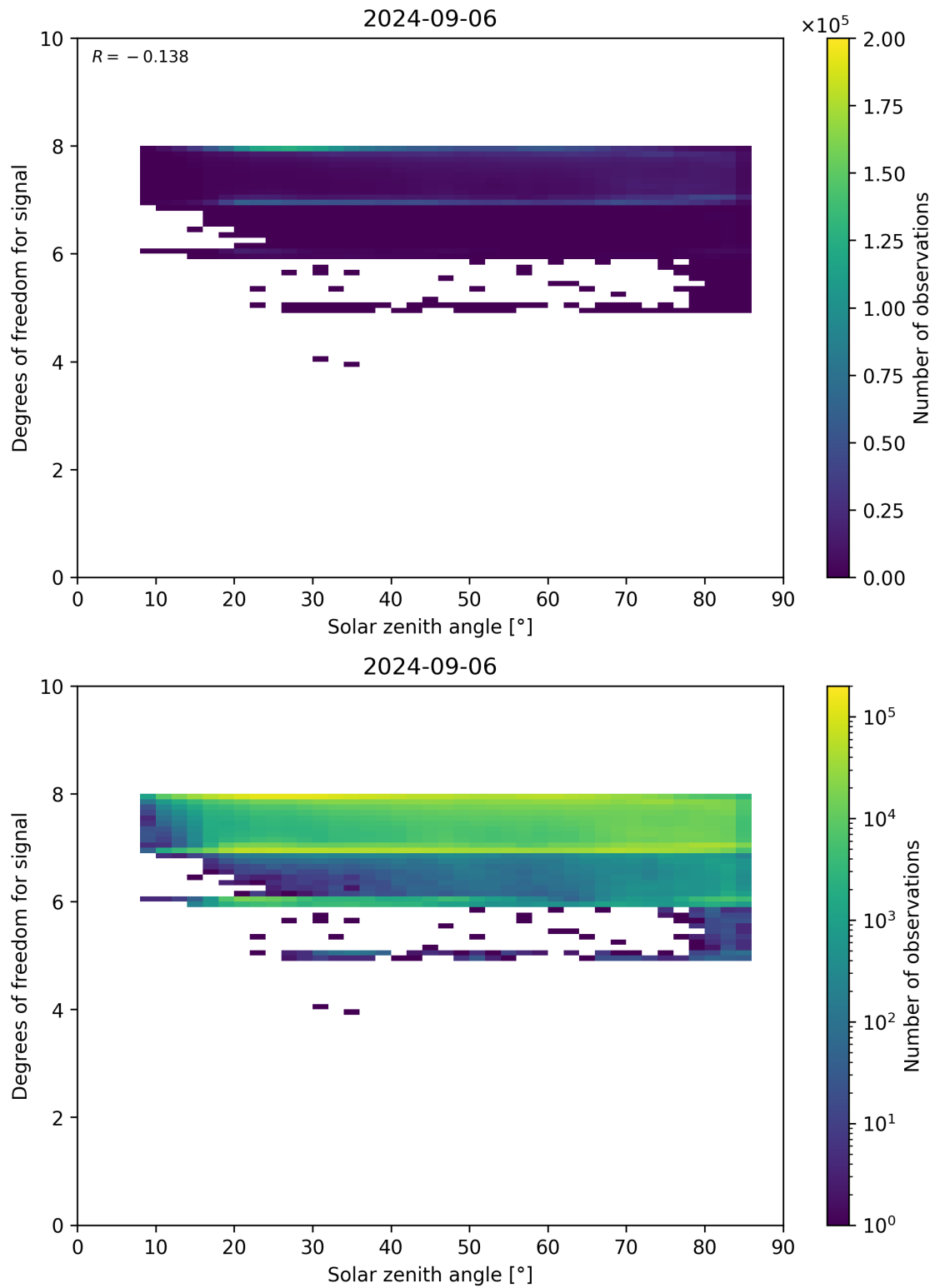
Figure 65: Scatter density plot of “Solar zenith angle” against “Degrees of freedom for signal” for 2024-09-06 to 2024-09-07.
