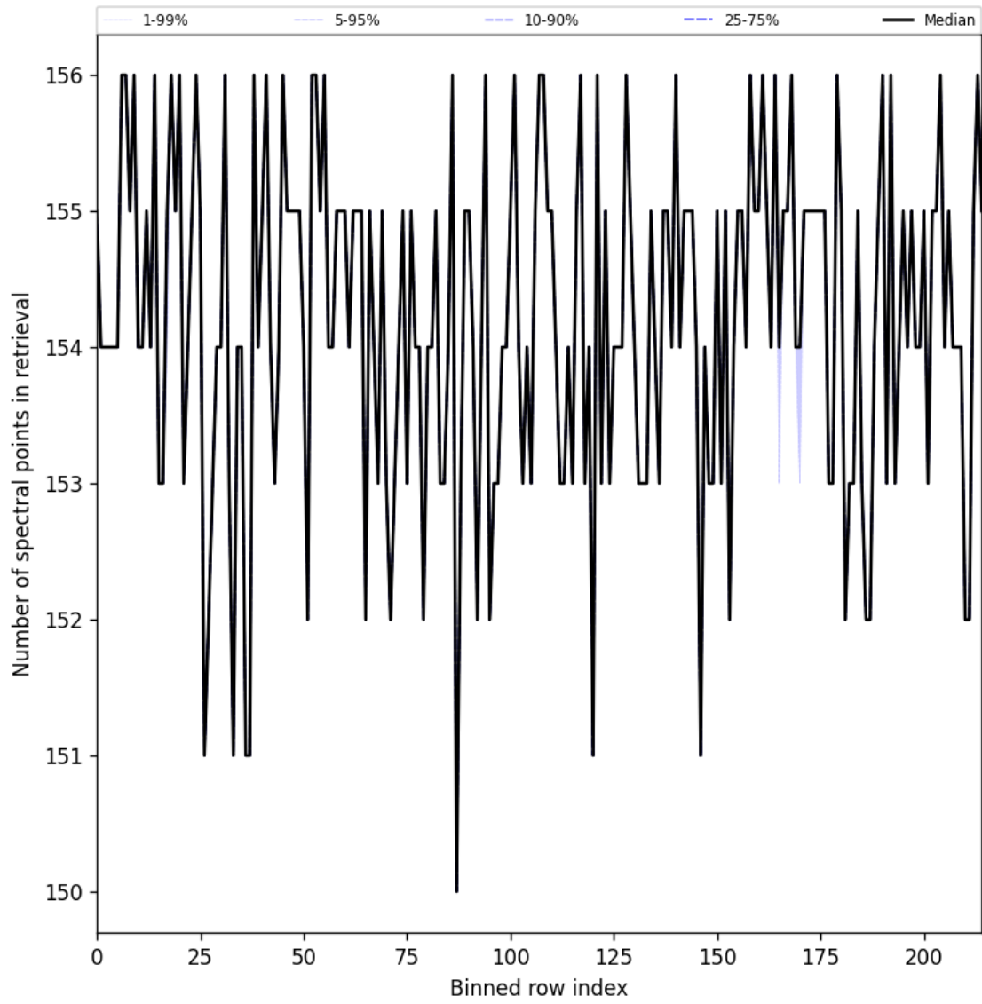
Figure 29: Along track statistics of “Number of spectral points in retrieval” for 2024-09-06 to 2024-09-07
