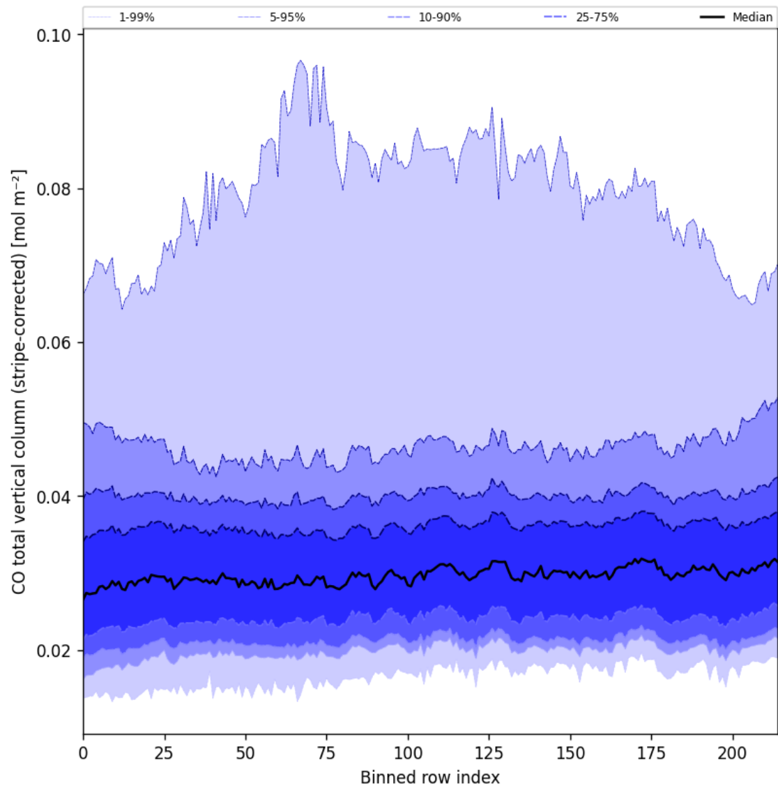
Figure 27: Along track statistics of “CO total vertical column (stripe-corrected)” for 2024-09-06 to 2024-09-07
