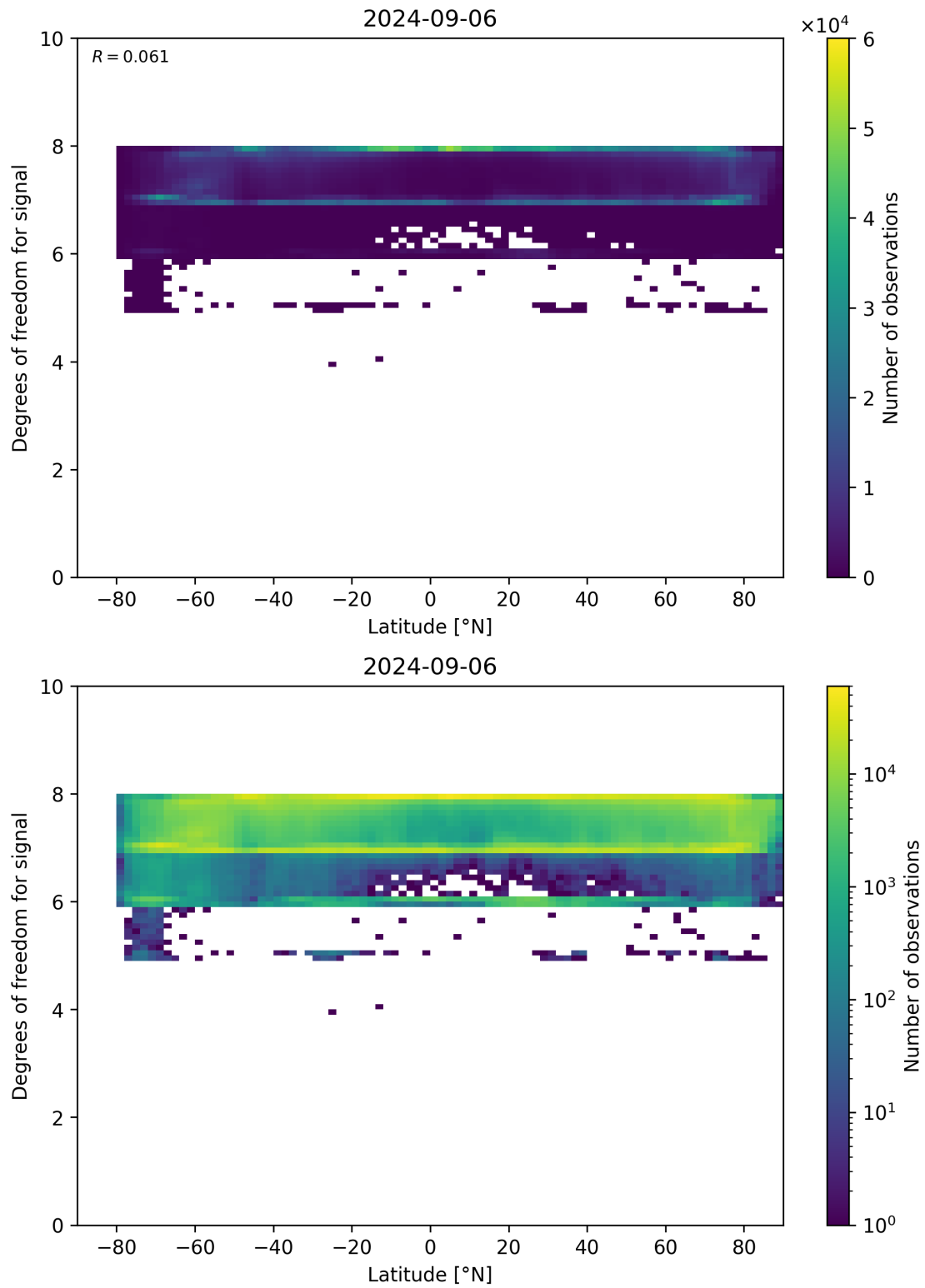
Figure 55: Scatter density plot of “Latitude” against “Degrees of freedom for signal” for 2024-09-06 to 2024-09-07.
