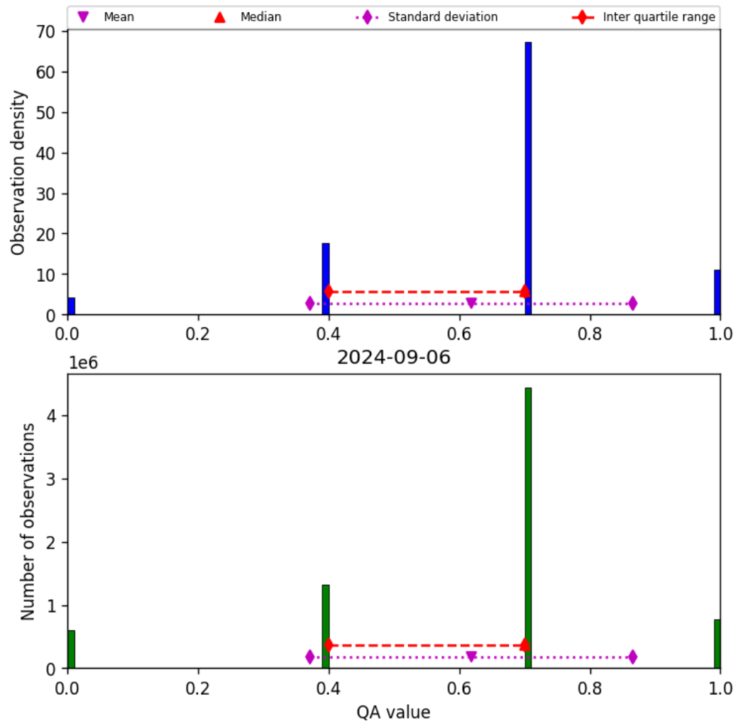
Figure 17: Histogram of “QA value” for 2024-09-06 to 2024-09-07
