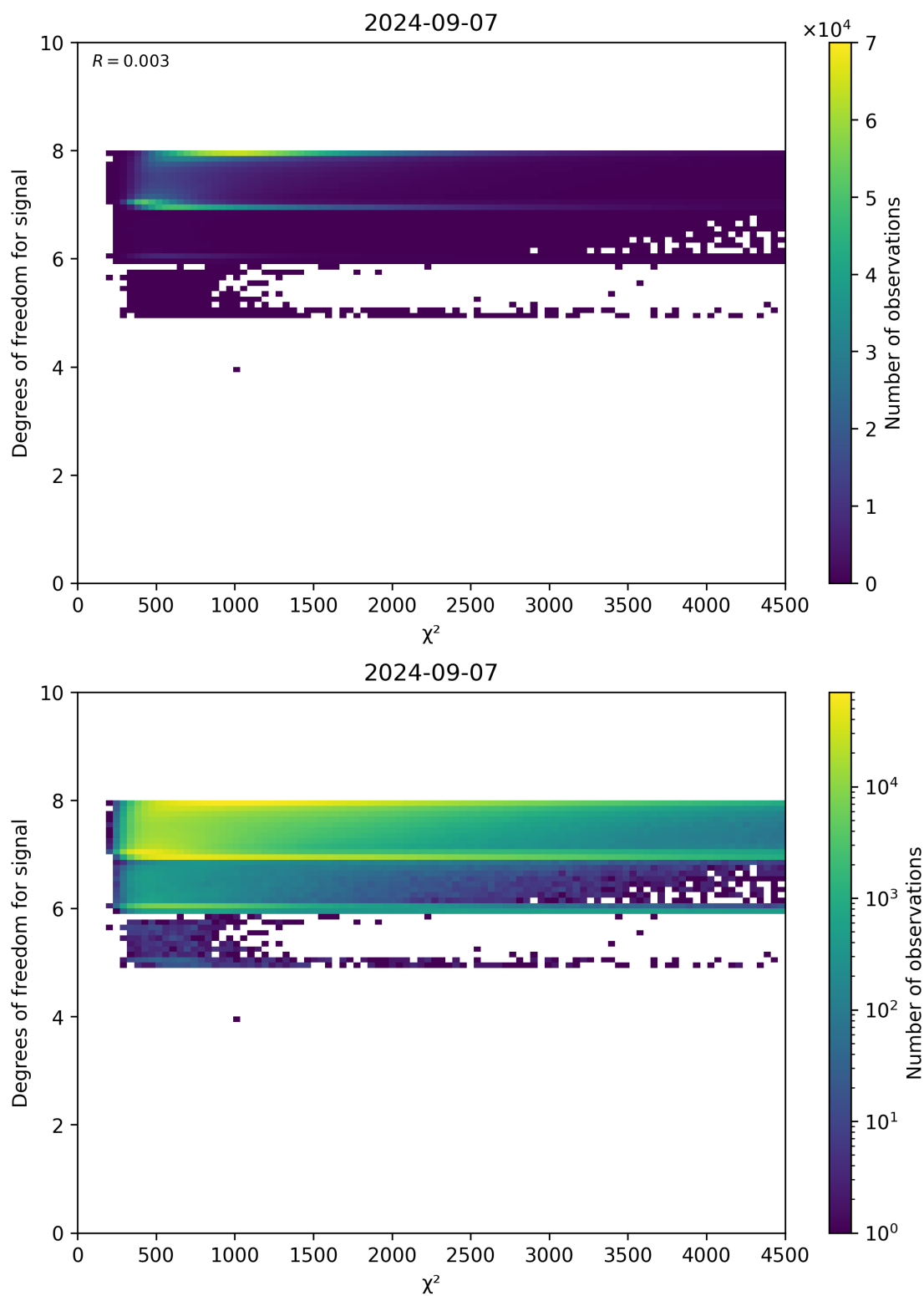
Figure 48: Scatter density plot of “ \chi^2 ” against “Degrees of freedom for signal” for 2024-09-06 to 2024-09-08.
