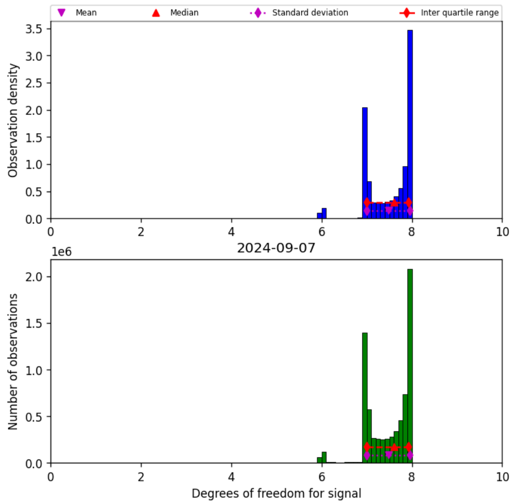
Figure 23: Histogram of “Degrees of freedom for signal” for 2024-09-06 to 2024-09-08
