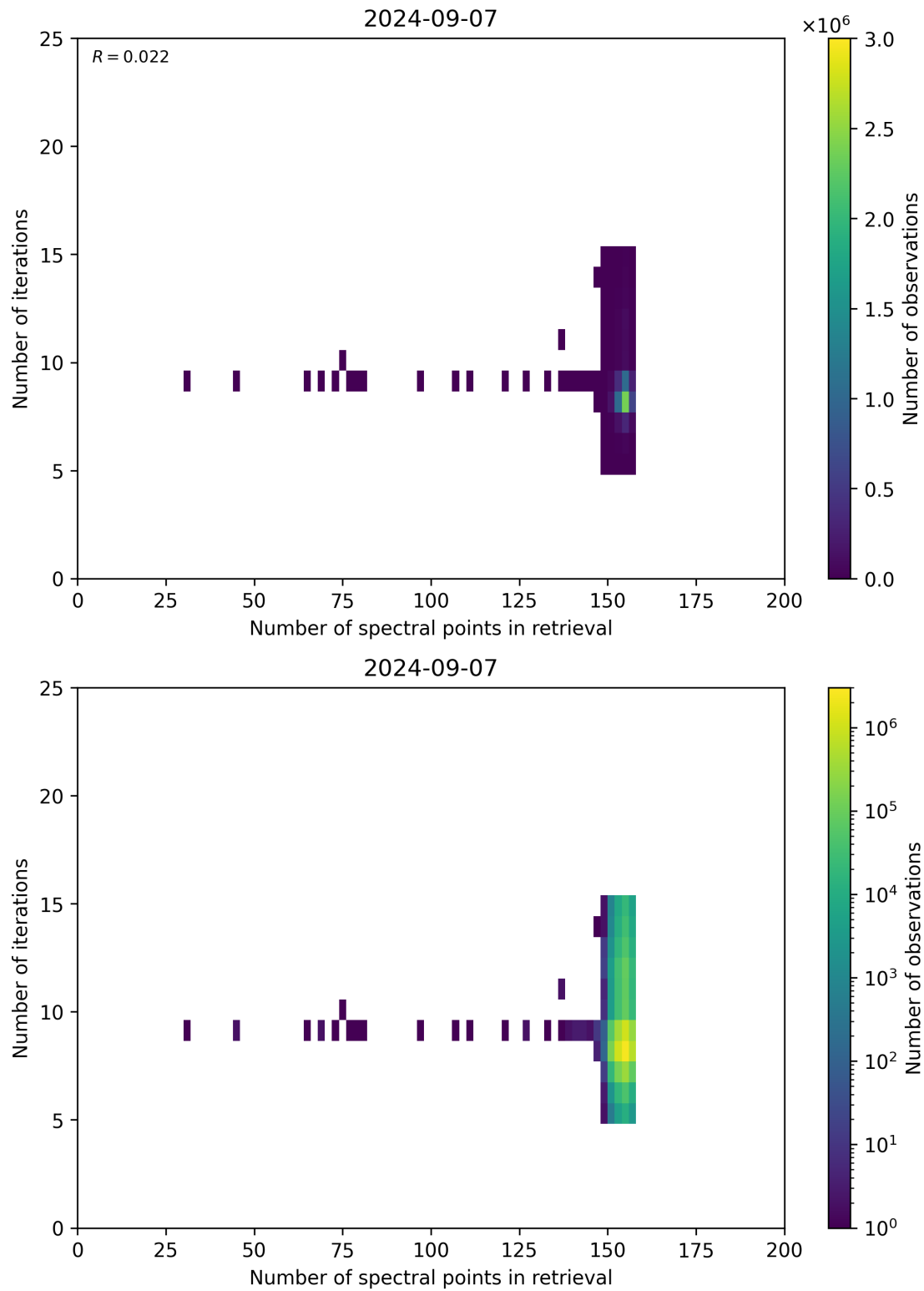
Figure 60: Scatter density plot of “Number of spectral points in retrieval” against “Number of iterations” for 2024-09-06 to 2024-09-08.
