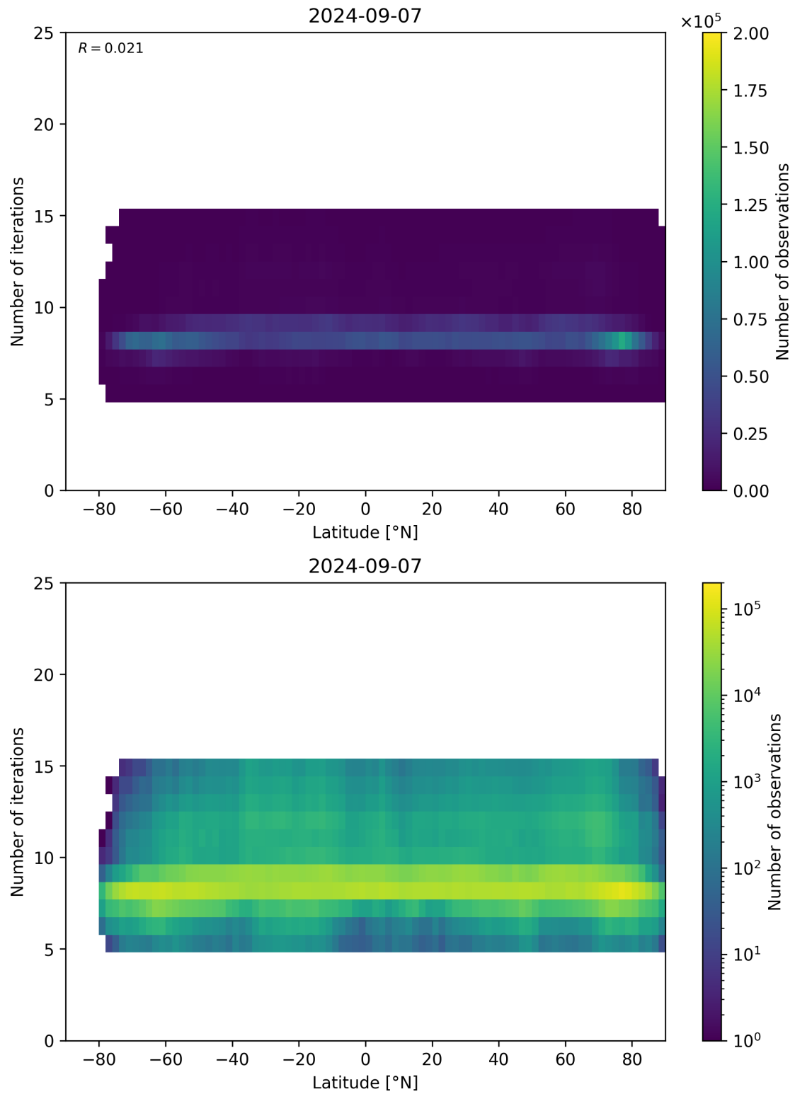
Figure 56: Scatter density plot of “Latitude” against “Number of iterations” for 2024-09-06 to 2024-09-08.
