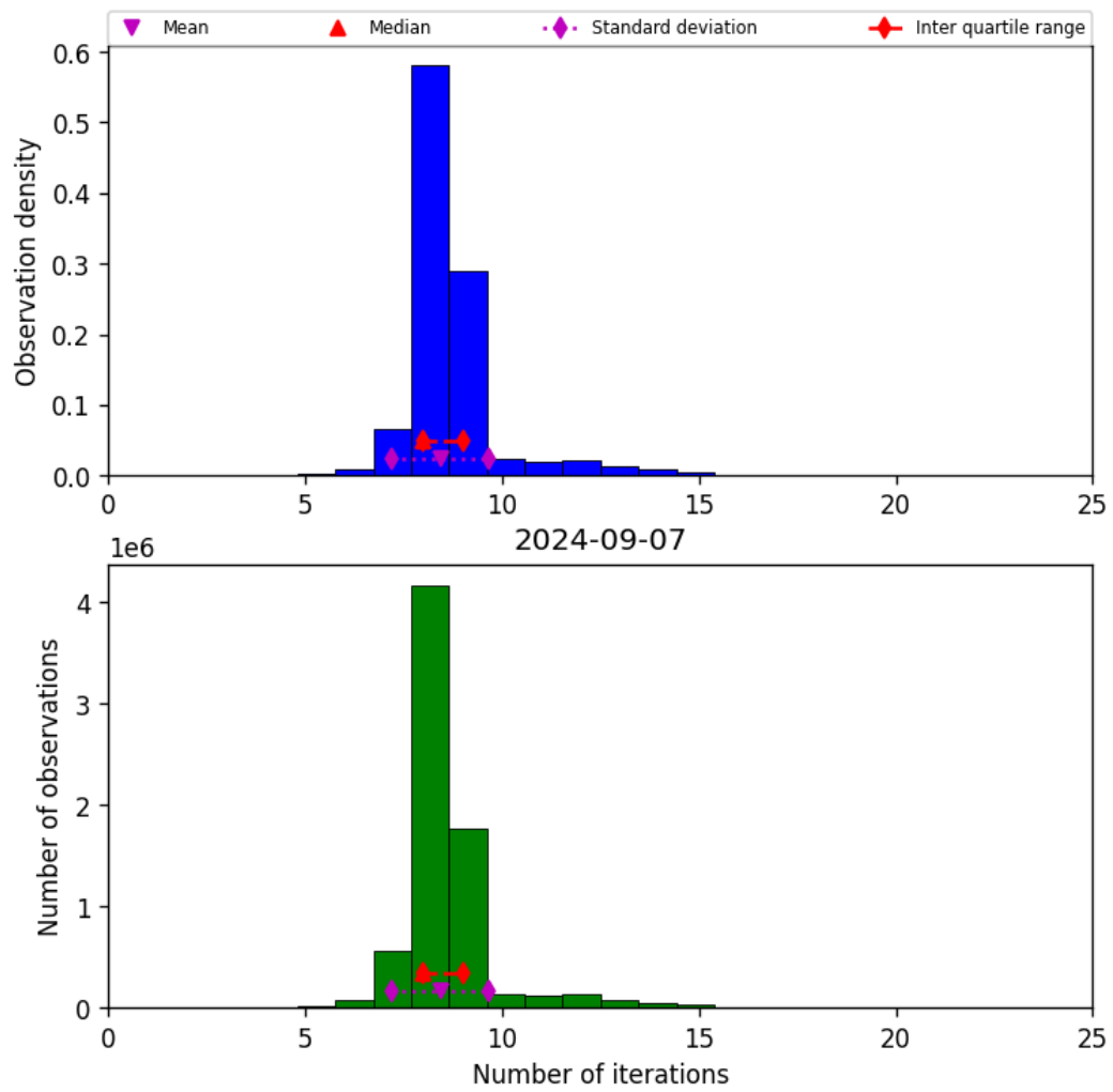
Figure 24: Histogram of “Number of iterations” for 2024-09-06 to 2024-09-08
