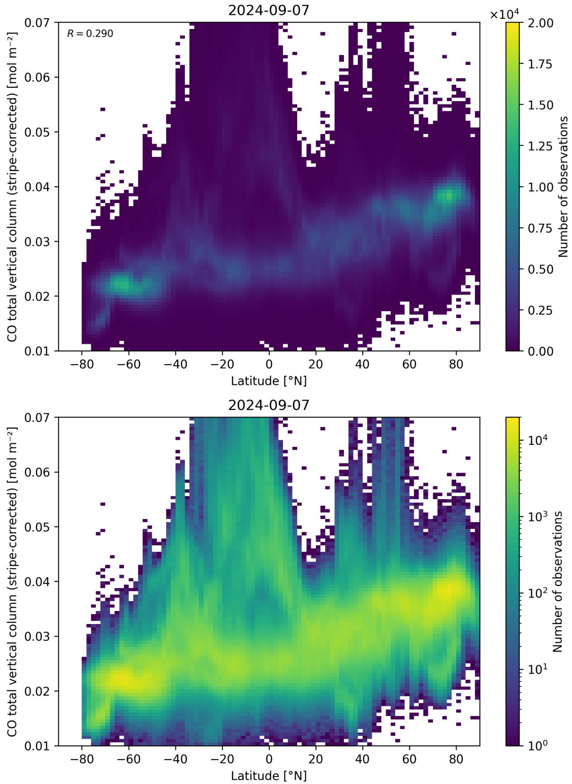
Figure 52: Scatter density plot of “Latitude” against “CO total vertical column (stripe-corrected)” for 2024-09-06 to 2024-09-08.
