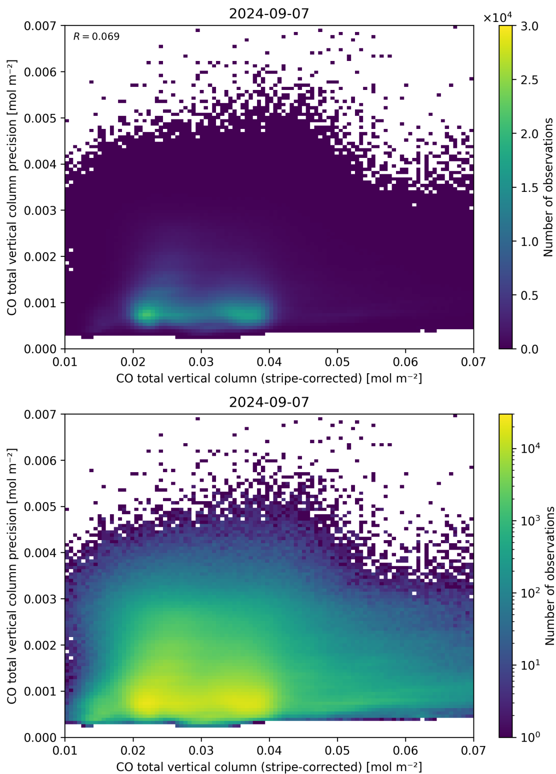
Figure 36: Scatter density plot of “CO total vertical column (stripe-corrected)” against “CO total vertical column precision” for 2024-09-06 to 2024-09-08.
