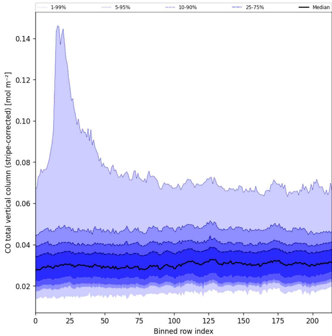
Figure 27: Along track statistics of “CO total vertical column (stripe-corrected)” for 2024-09-06 to 2024-09-08
