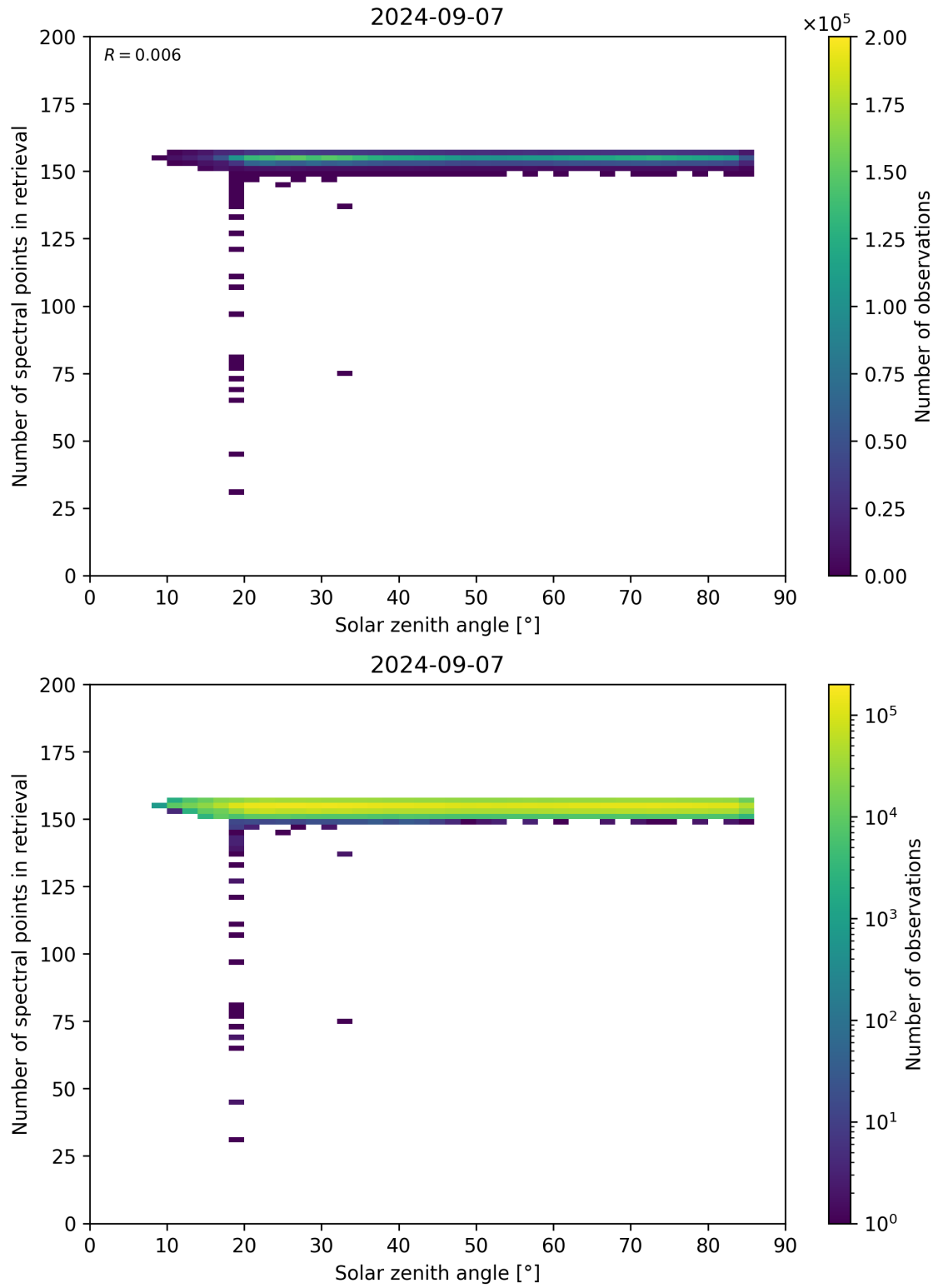
Figure 68: Scatter density plot of “Solar zenith angle” against “Number of spectral points in retrieval” for 2024-09-06 to 2024-09-08.
