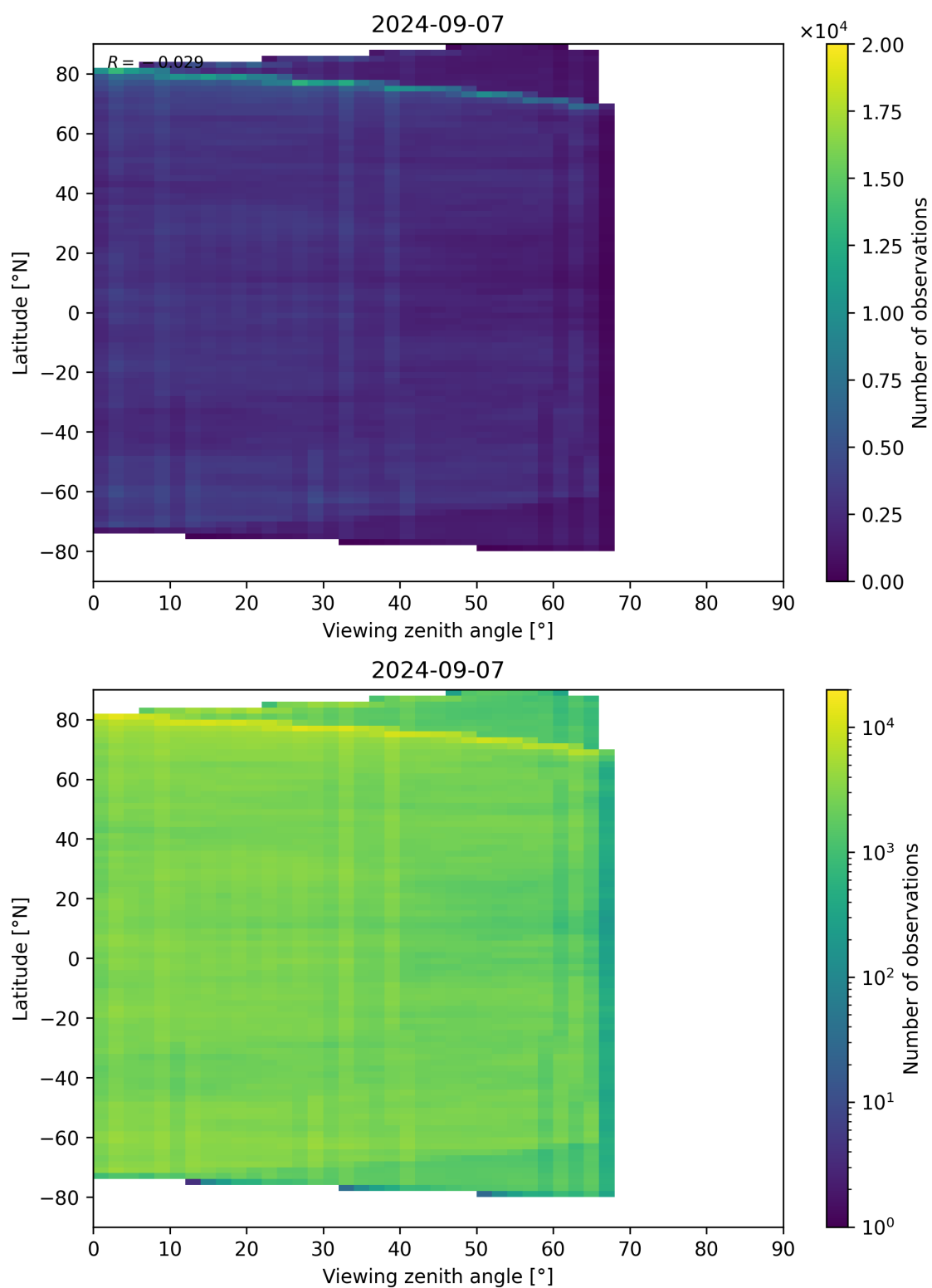
Figure 74: Scatter density plot of “Viewing zenith angle” against “Latitude” for 2024-09-06 to 2024-09-08.
