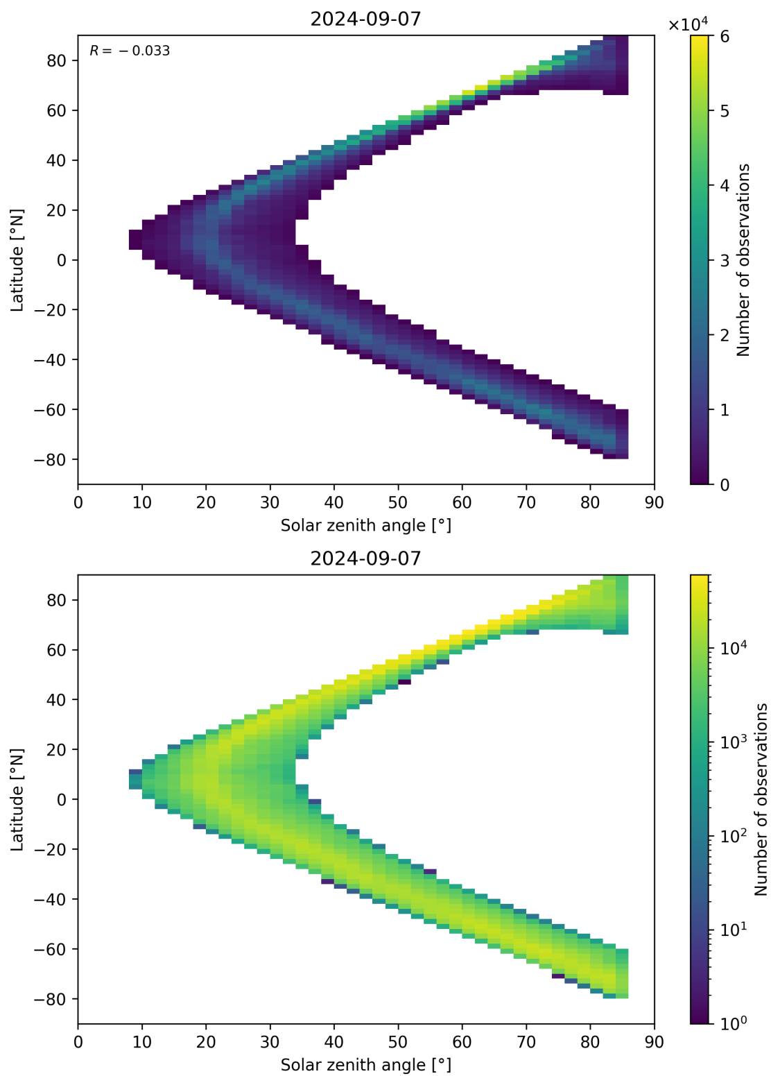
Figure 66: Scatter density plot of “Solar zenith angle” against “Latitude” for 2024-09-06 to 2024-09-08.
