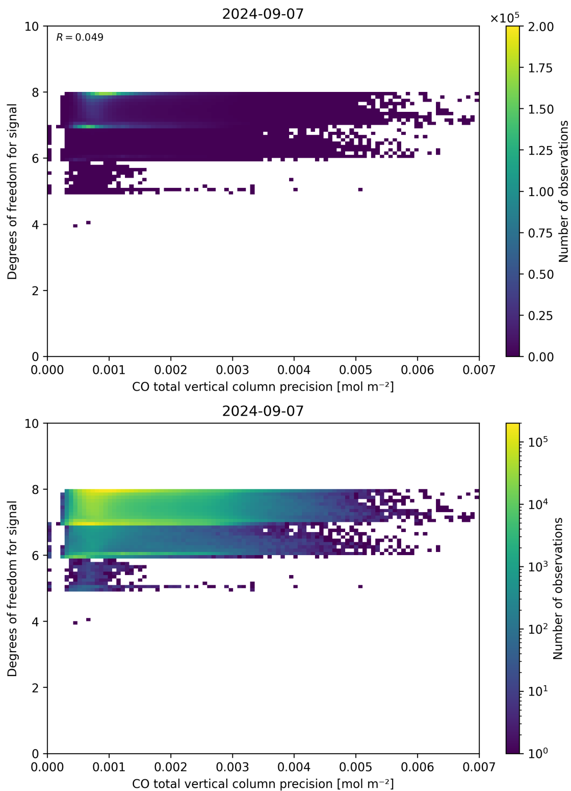
Figure 45: Scatter density plot of “CO total vertical column precision” against “Degrees of freedom for signal” for 2024-09-06 to 2024-09-08.
