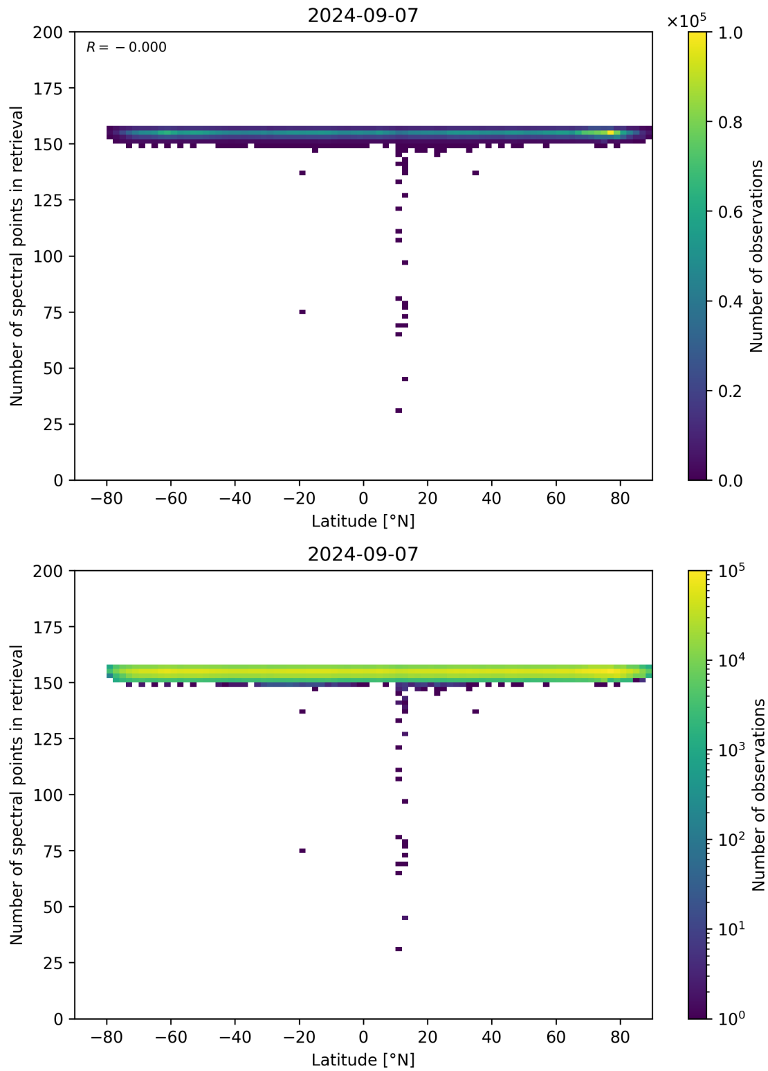
Figure 57: Scatter density plot of “Latitude” against “Number of spectral points in retrieval” for 2024-09-06 to 2024-09-08.
