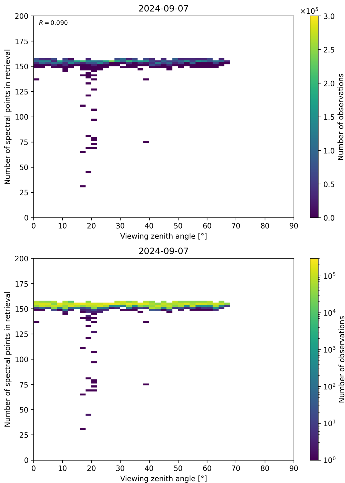
Figure 76: Scatter density plot of “Viewing zenith angle” against “Number of spectral points in retrieval” for 2024-09-06 to 2024-09-08.
