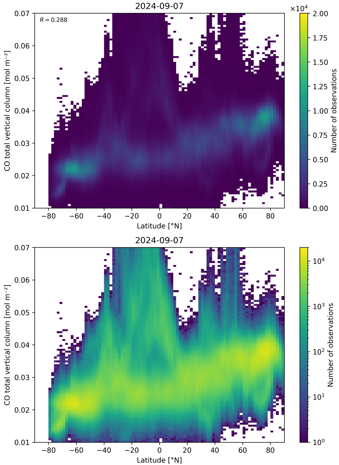
Figure 51: Scatter density plot of “Latitude” against “CO total vertical column” for 2024-09-06 to 2024-09-08.
