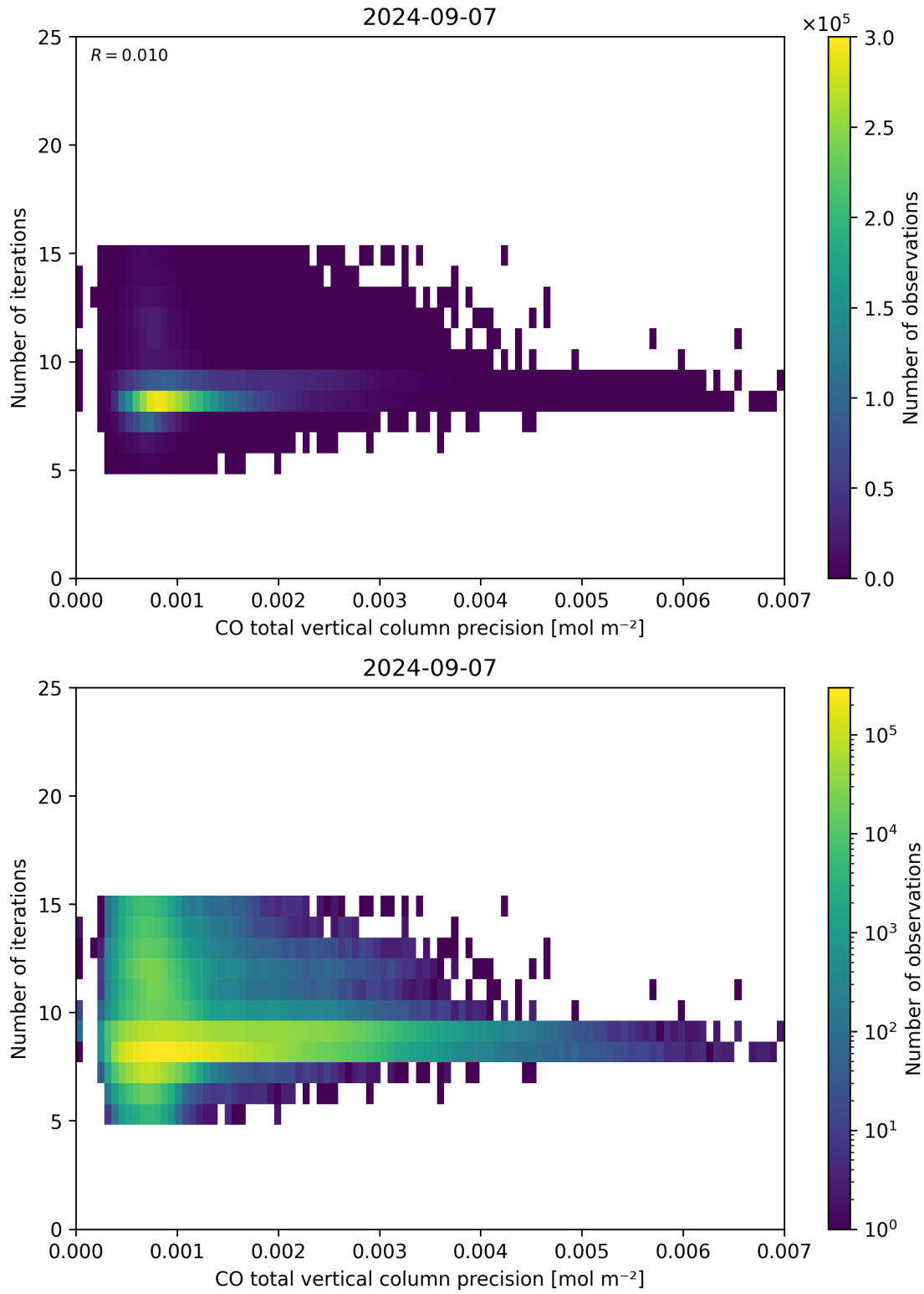
Figure 46: Scatter density plot of “CO total vertical column precision” against “Number of iterations” for 2024-09-06 to 2024-09-08.
