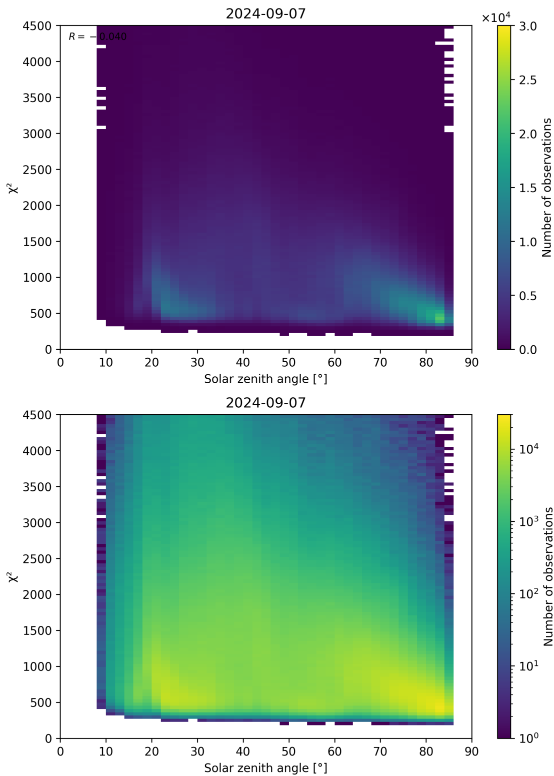
Figure 64: Scatter density plot of “Solar zenith angle” against “ \chi^2 ” for 2024-09-06 to 2024-09-08.
