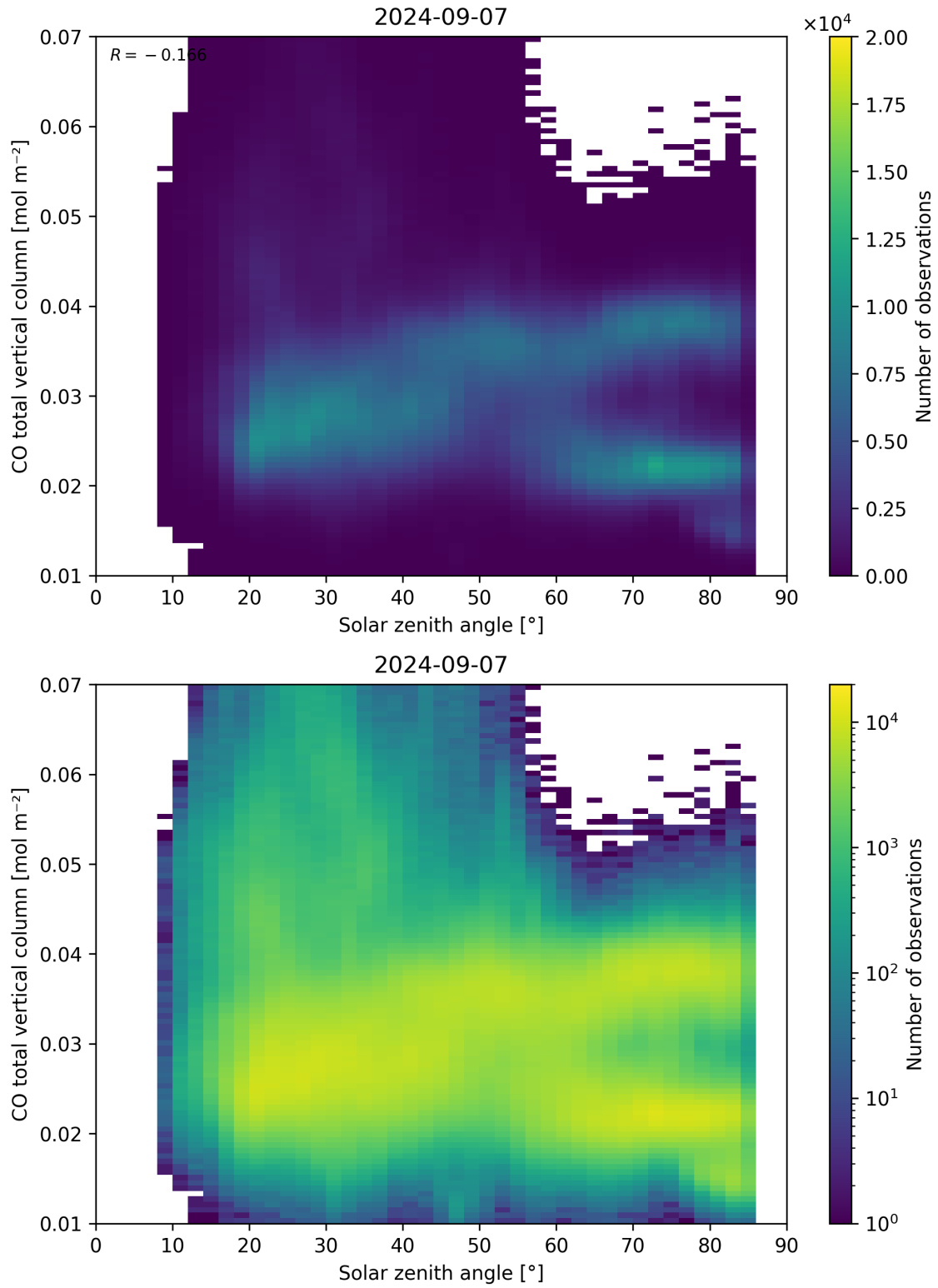
Figure 61: Scatter density plot of “Solar zenith angle” against “CO total vertical column” for 2024-09-06 to 2024-09-08.
