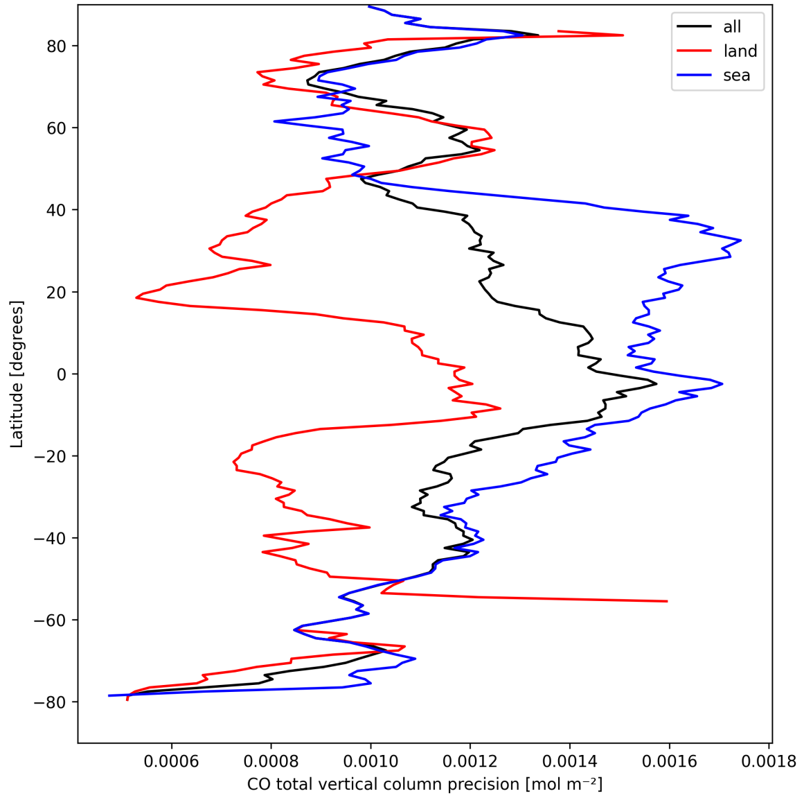
Figure 12: Zonal average of “CO total vertical column precision” for 2024-09-06 to 2024-09-08.
