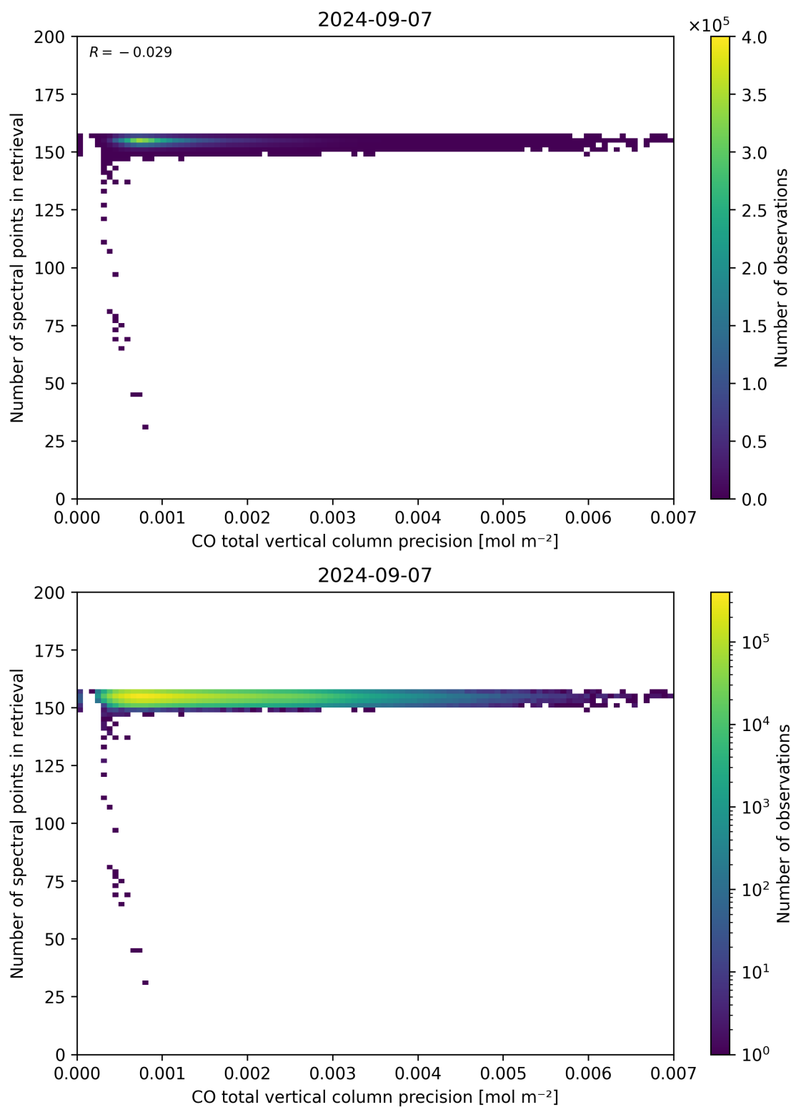
Figure 47: Scatter density plot of “CO total vertical column precision” against “Number of spectral points in retrieval” for 2024-09-06 to 2024-09-08.
