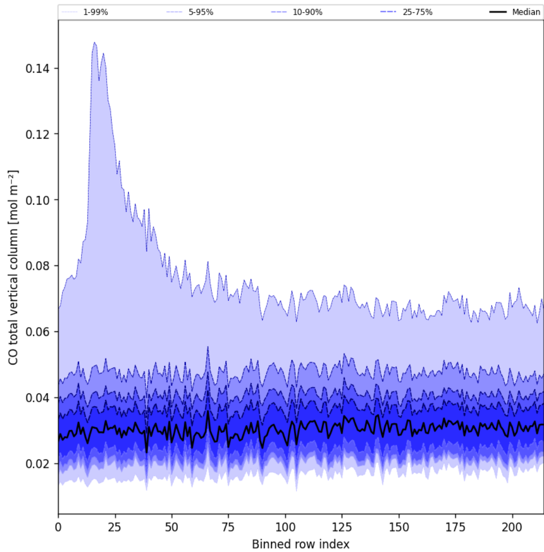
Figure 26: Along track statistics of “CO total vertical column” for 2024-09-06 to 2024-09-08
