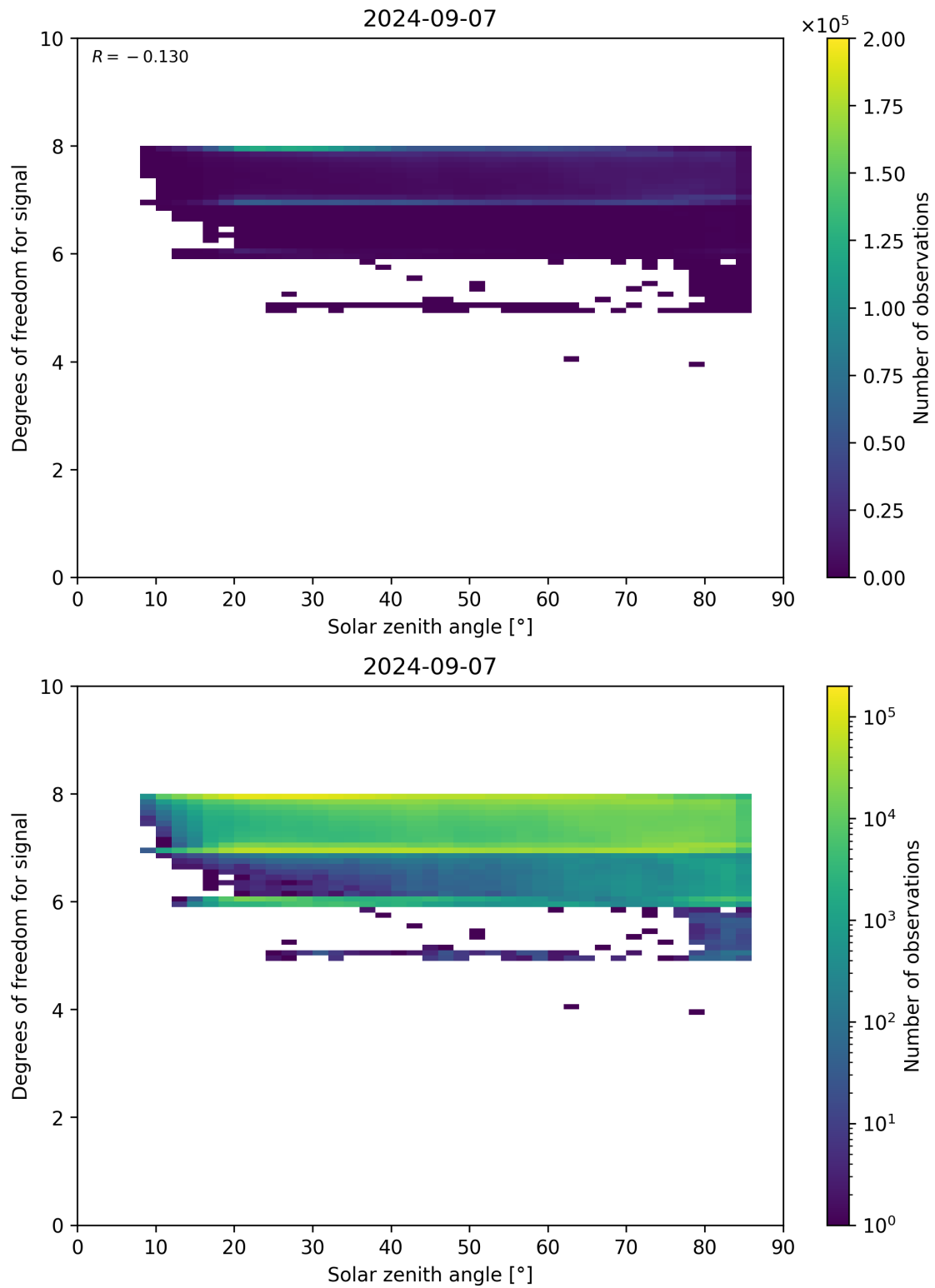
Figure 65: Scatter density plot of “Solar zenith angle” against “Degrees of freedom for signal” for 2024-09-06 to 2024-09-08.
