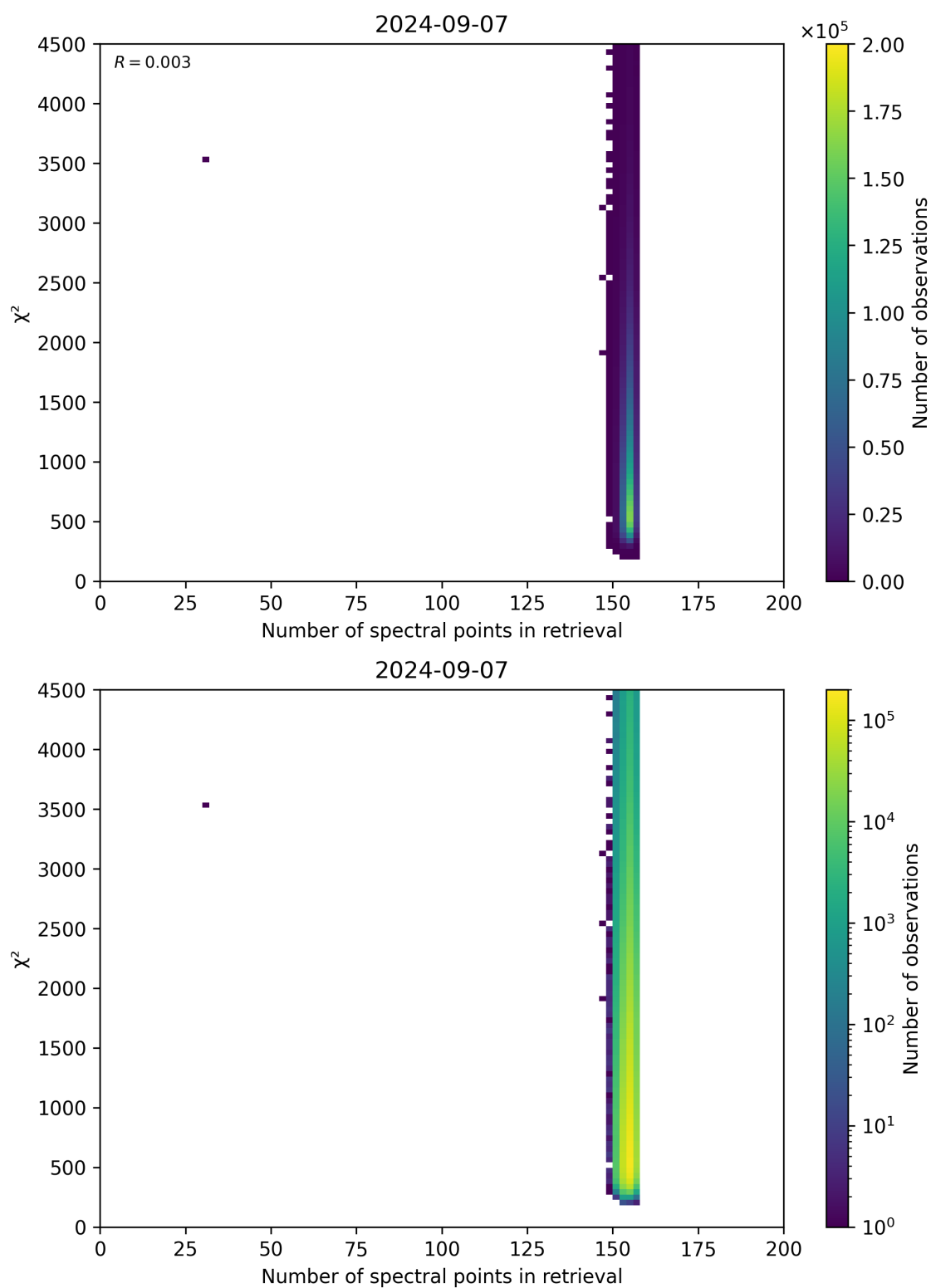
Figure 58: Scatter density plot of “Number of spectral points in retrieval” against “ \chi^2 ” for 2024-09-06 to 2024-09-08.
