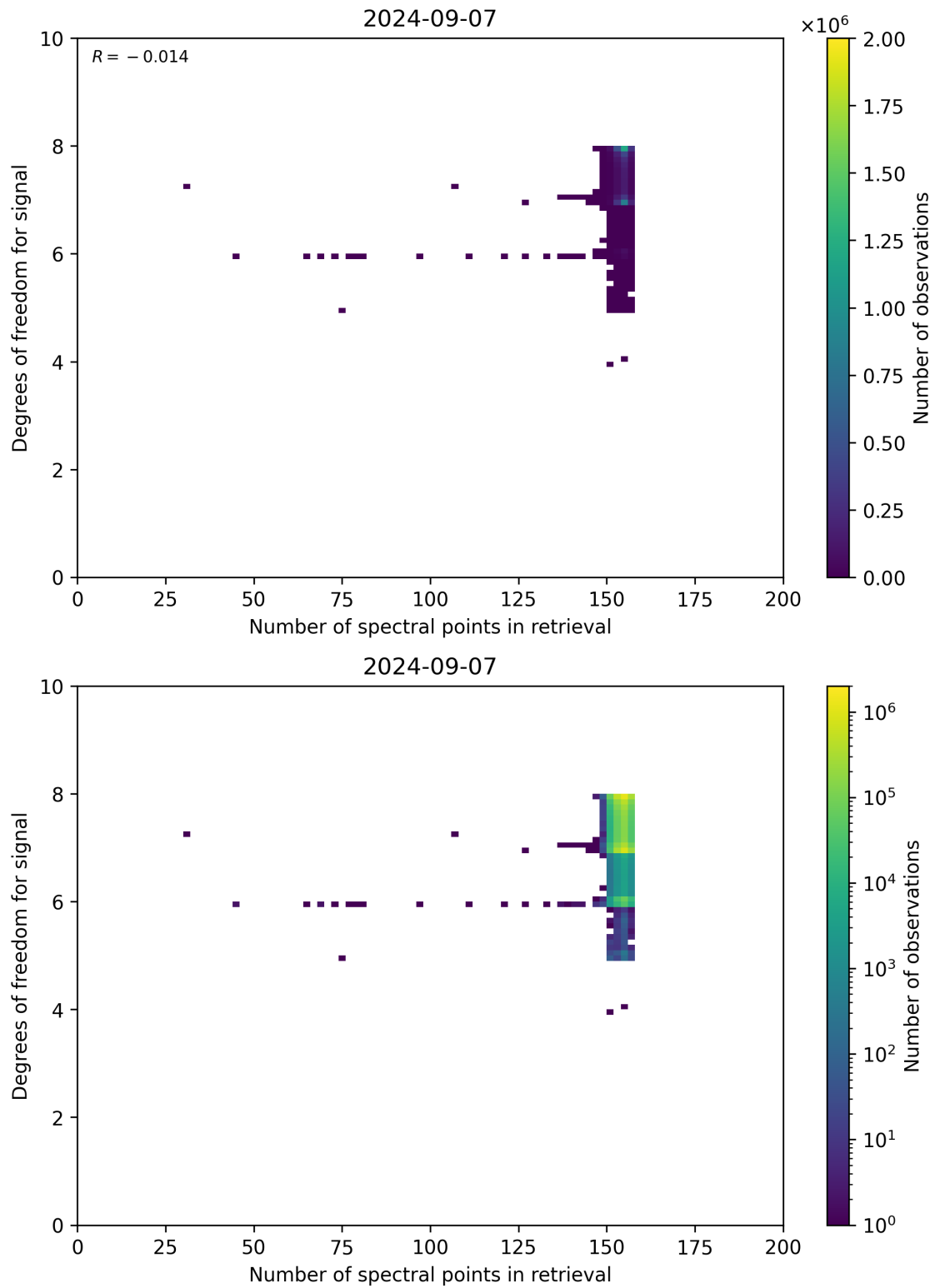
Figure 59: Scatter density plot of “Number of spectral points in retrieval” against “Degrees of freedom for signal” for 2024-09-06 to 2024-09-08.
