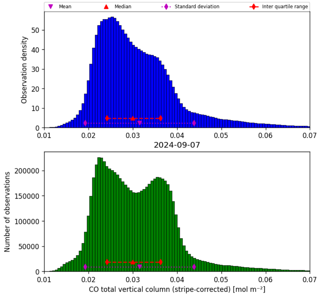
Figure 19: Histogram of “CO total vertical column (stripe-corrected)” for 2024-09-06 to 2024-09-08
