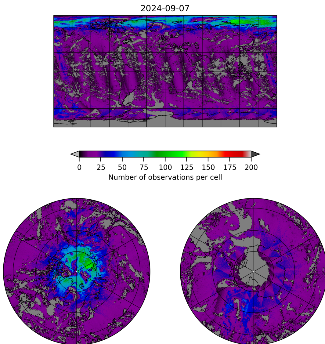
Figure 8: Map of the number of observations for 2024-09-06 to 2024-09-08
