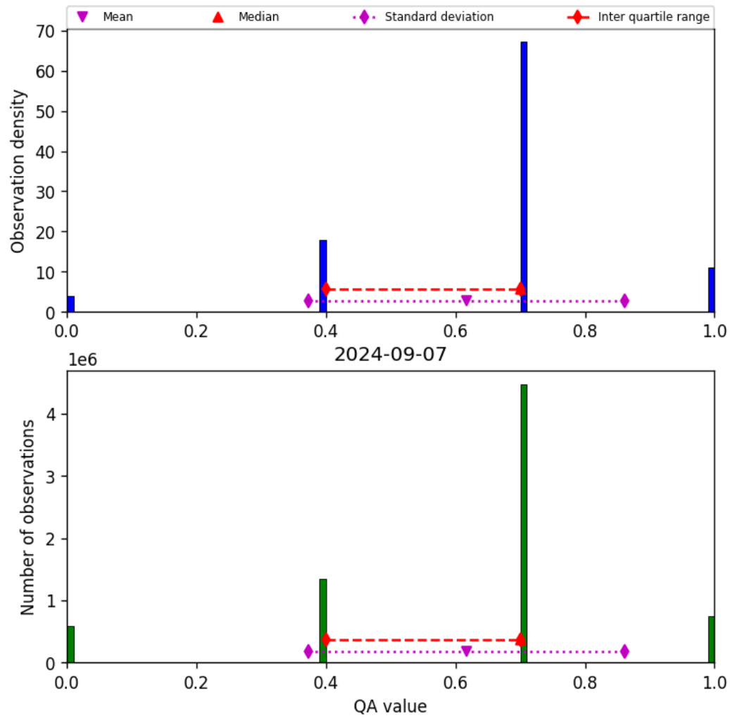
Figure 17: Histogram of “QA value” for 2024-09-06 to 2024-09-08
