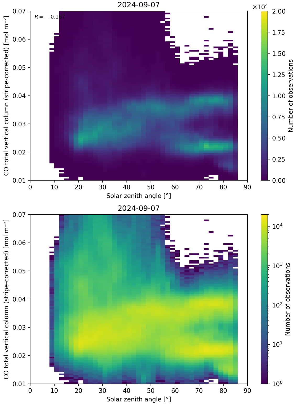
Figure 62: Scatter density plot of “Solar zenith angle” against “CO total vertical column (stripe-corrected)” for 2024-09-06 to 2024-09-08.
