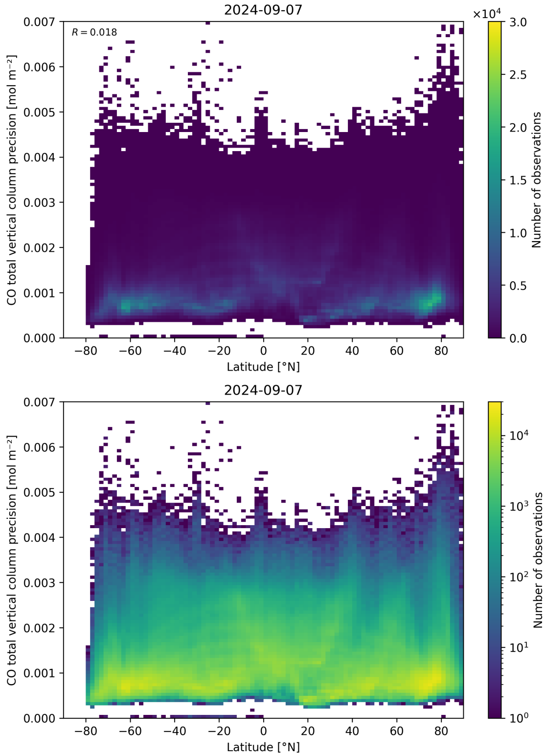
Figure 53: Scatter density plot of “Latitude” against “CO total vertical column precision” for 2024-09-06 to 2024-09-08.
