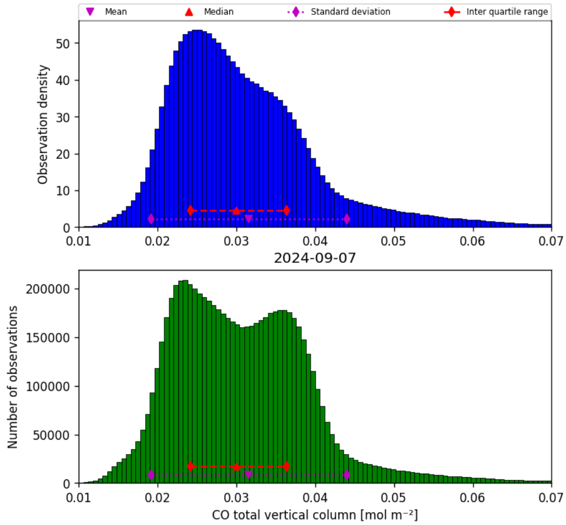
Figure 18: Histogram of “CO total vertical column” for 2024-09-06 to 2024-09-08
