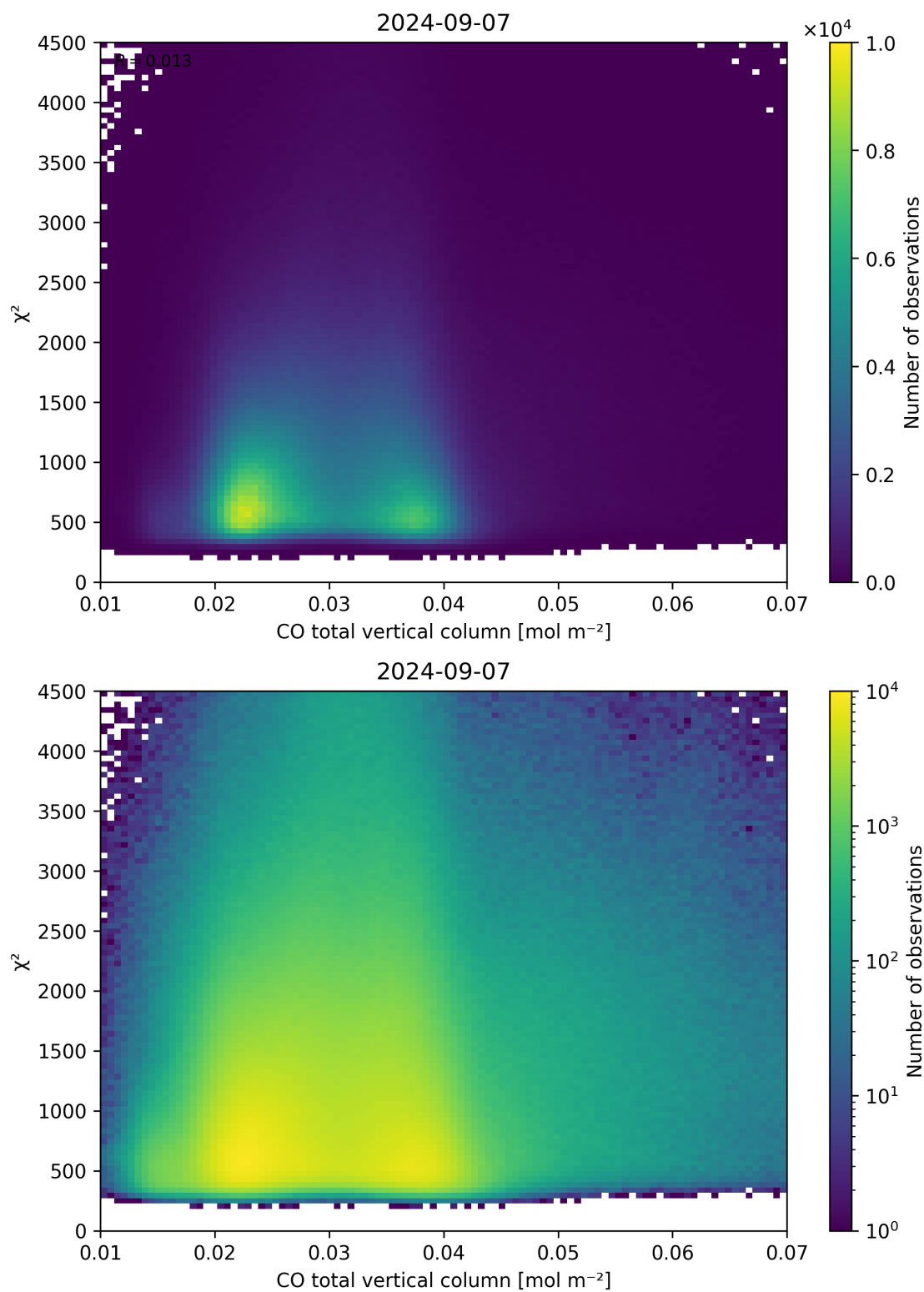
Figure 35: Scatter density plot of “CO total vertical column” against “ \chi^2 ” for 2024-09-06 to 2024-09-08.
