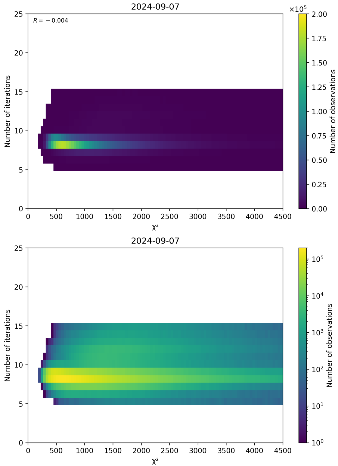
Figure 49: Scatter density plot of “ \chi^2 ” against “Number of iterations” for 2024-09-06 to 2024-09-08.
