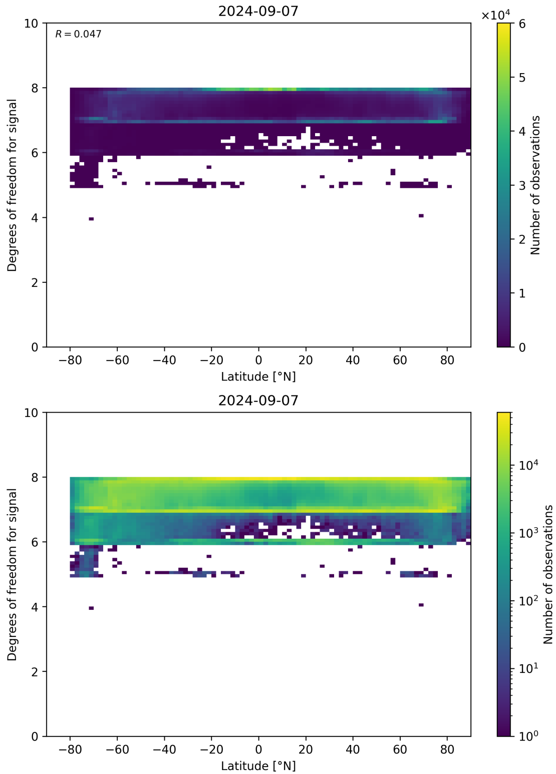
Figure 55: Scatter density plot of “Latitude” against “Degrees of freedom for signal” for 2024-09-06 to 2024-09-08.
