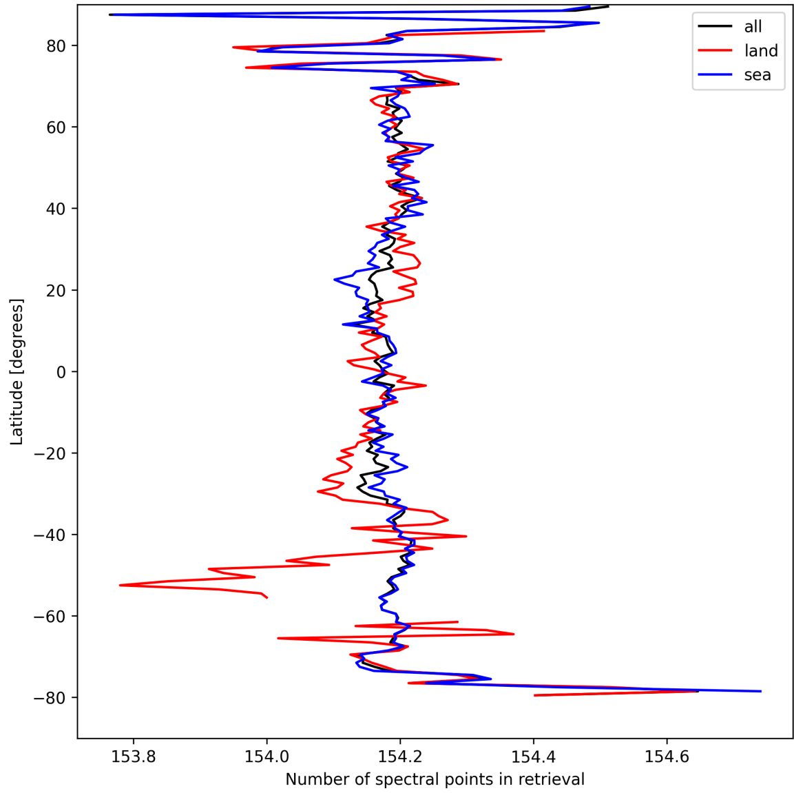
Figure 13: Zonal average of “Number of spectral points in retrieval” for 2024-09-06 to 2024-09-08.
