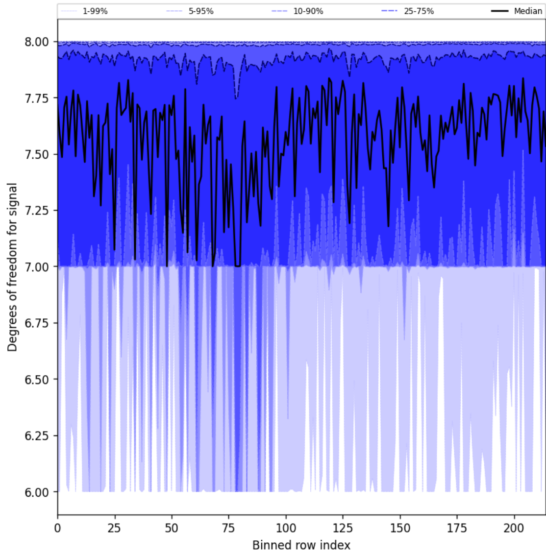
Figure 31: Along track statistics of “Degrees of freedom for signal” for 2024-09-06 to 2024-09-08
