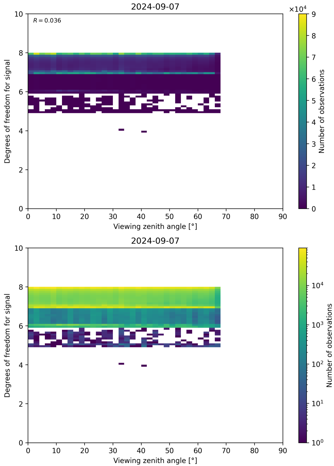
Figure 73: Scatter density plot of “Viewing zenith angle” against “Degrees of freedom for signal” for 2024-09-06 to 2024-09-08.
