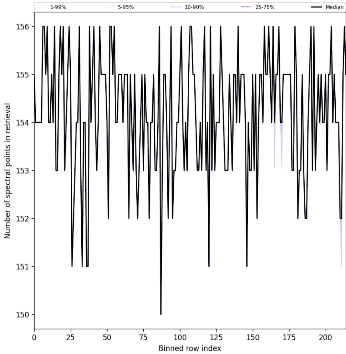
Figure 29: Along track statistics of “Number of spectral points in retrieval” for 2024-09-06 to 2024-09-08
