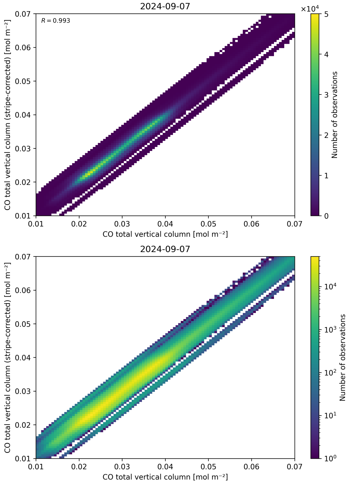
Figure 33: Scatter density plot of “CO total vertical column” against “CO total vertical column (stripe-corrected)” for 2024-09-06 to 2024-09-08.
