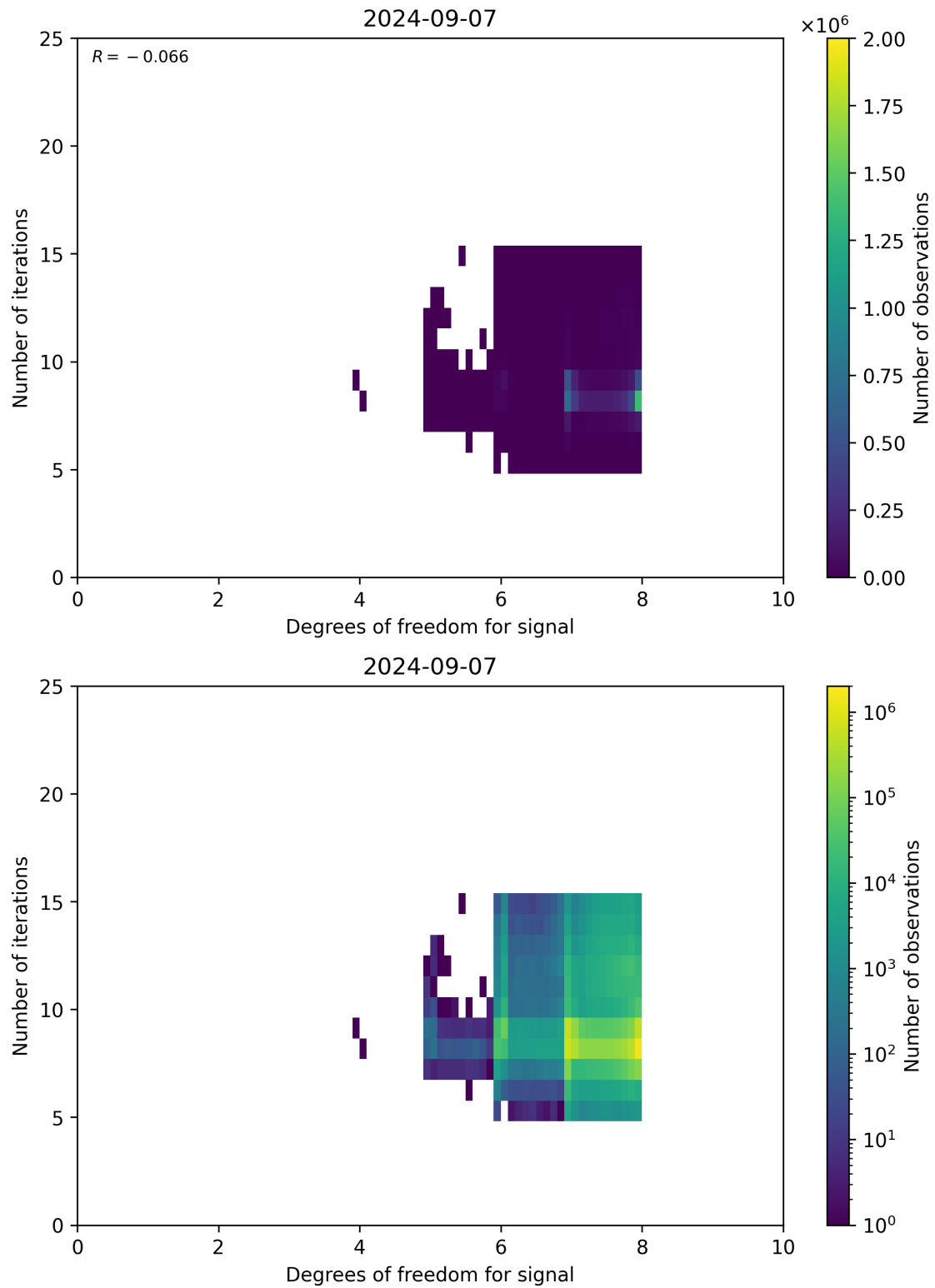
Figure 50: Scatter density plot of “Degrees of freedom for signal” against “Number of iterations” for 2024-09-06 to 2024-09-08.
