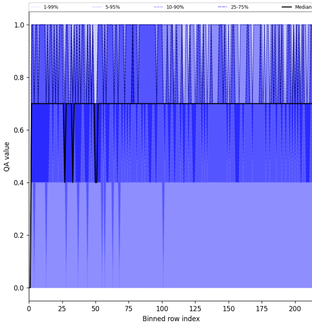
Figure 25: Along track statistics of “QA value” for 2024-09-06 to 2024-09-08
