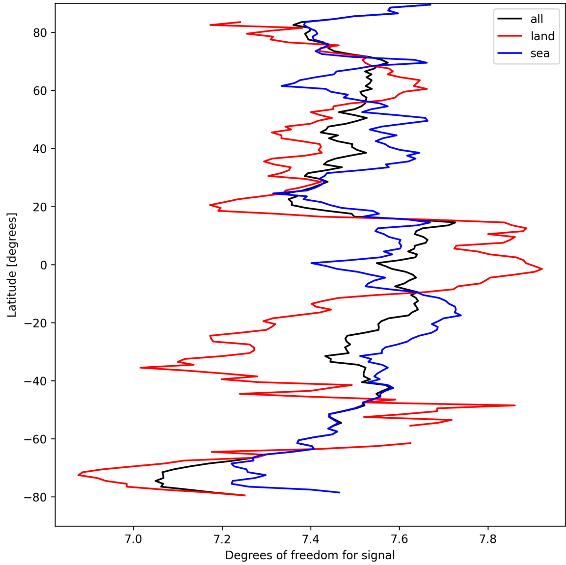
Figure 15: Zonal average of “Degrees of freedom for signal” for 2024-09-06 to 2024-09-08.
