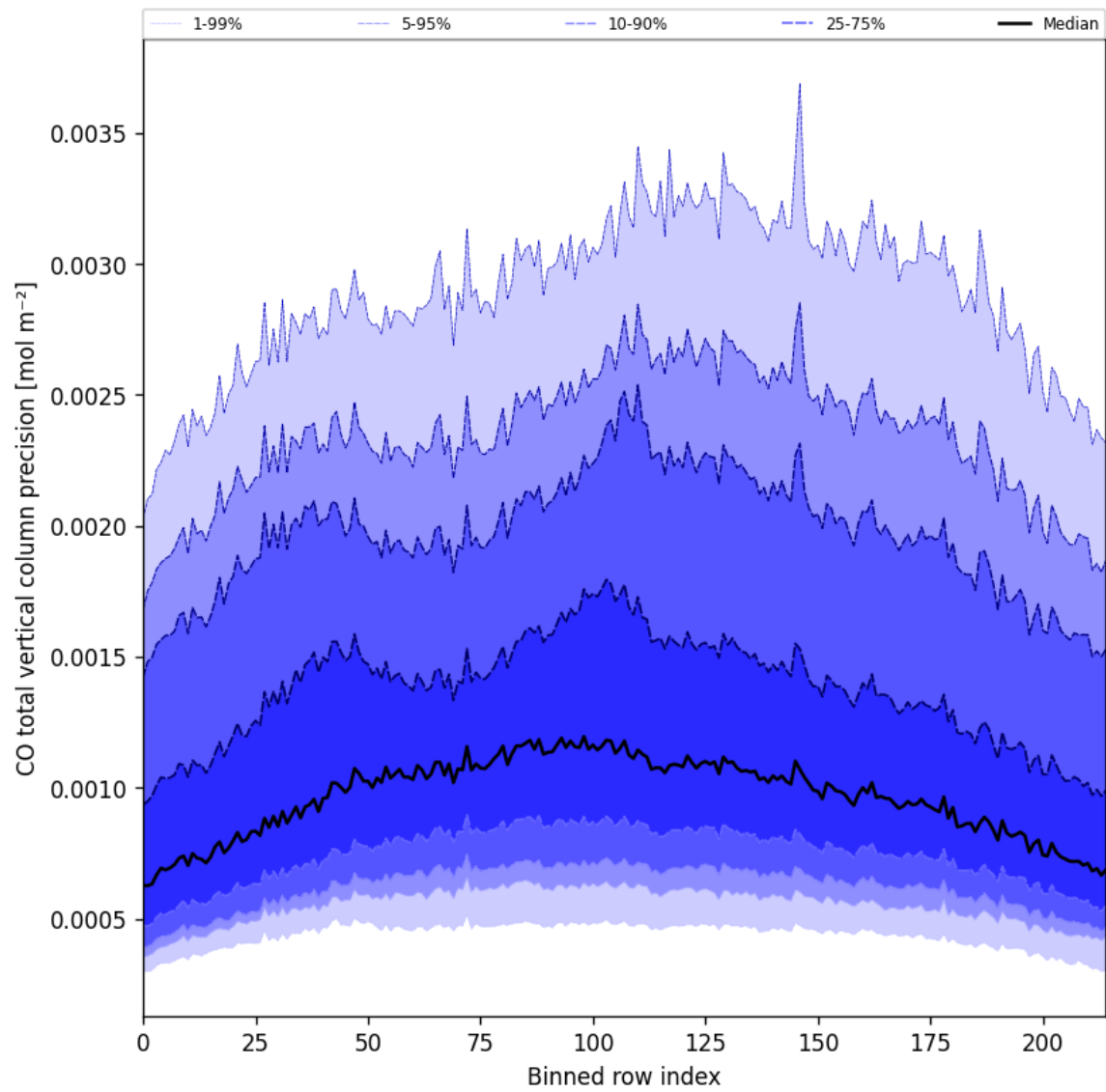
Figure 28: Along track statistics of "CO total vertical column precision" for 2024-09-06 to 2024-09-08
