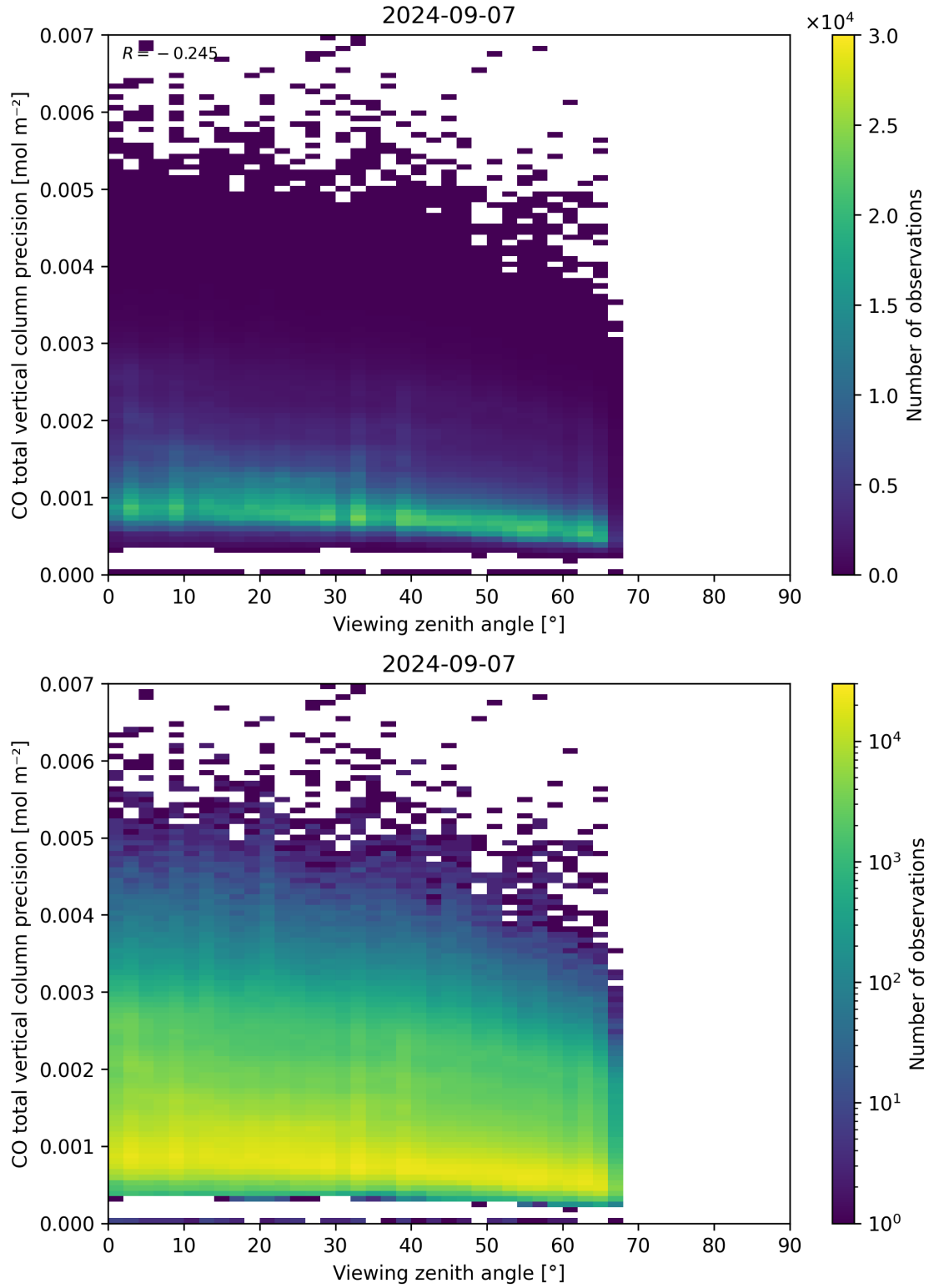
Figure 71: Scatter density plot of “Viewing zenith angle” against “CO total vertical column precision” for 2024-09-06 to 2024-09-08.
