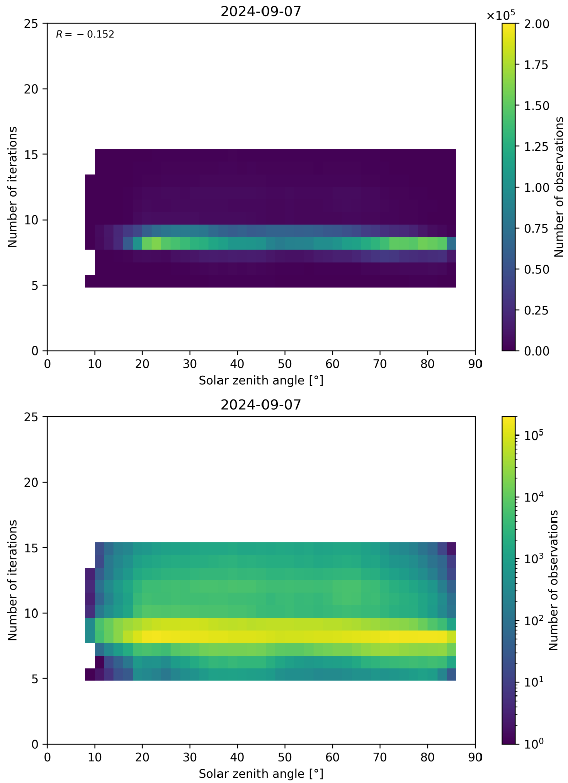
Figure 67: Scatter density plot of “Solar zenith angle” against “Number of iterations” for 2024-09-06 to 2024-09-08.
