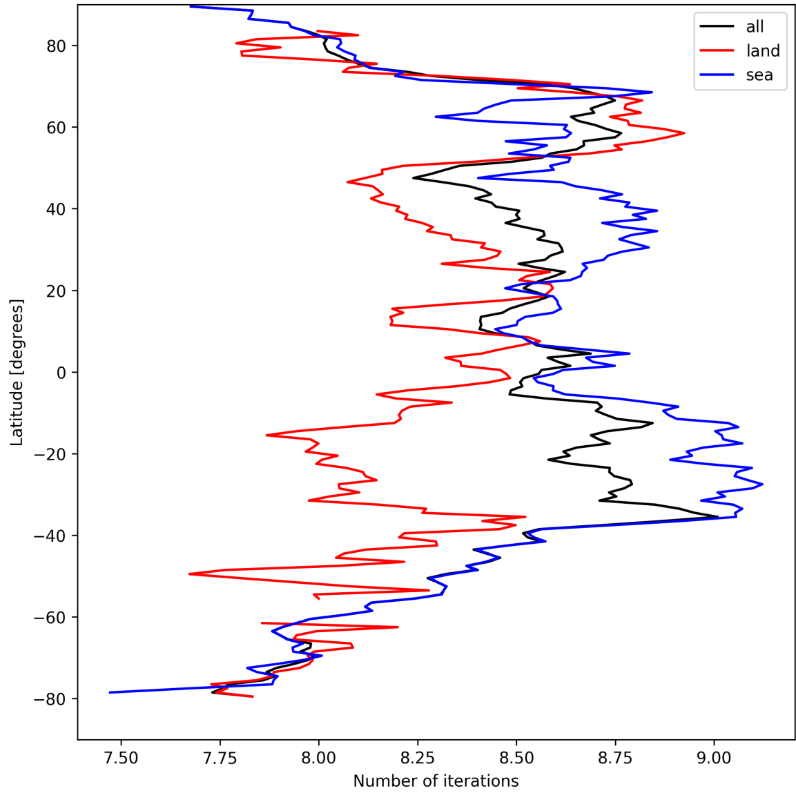
Figure 16: Zonal average of “Number of iterations” for 2024-09-06 to 2024-09-08.
