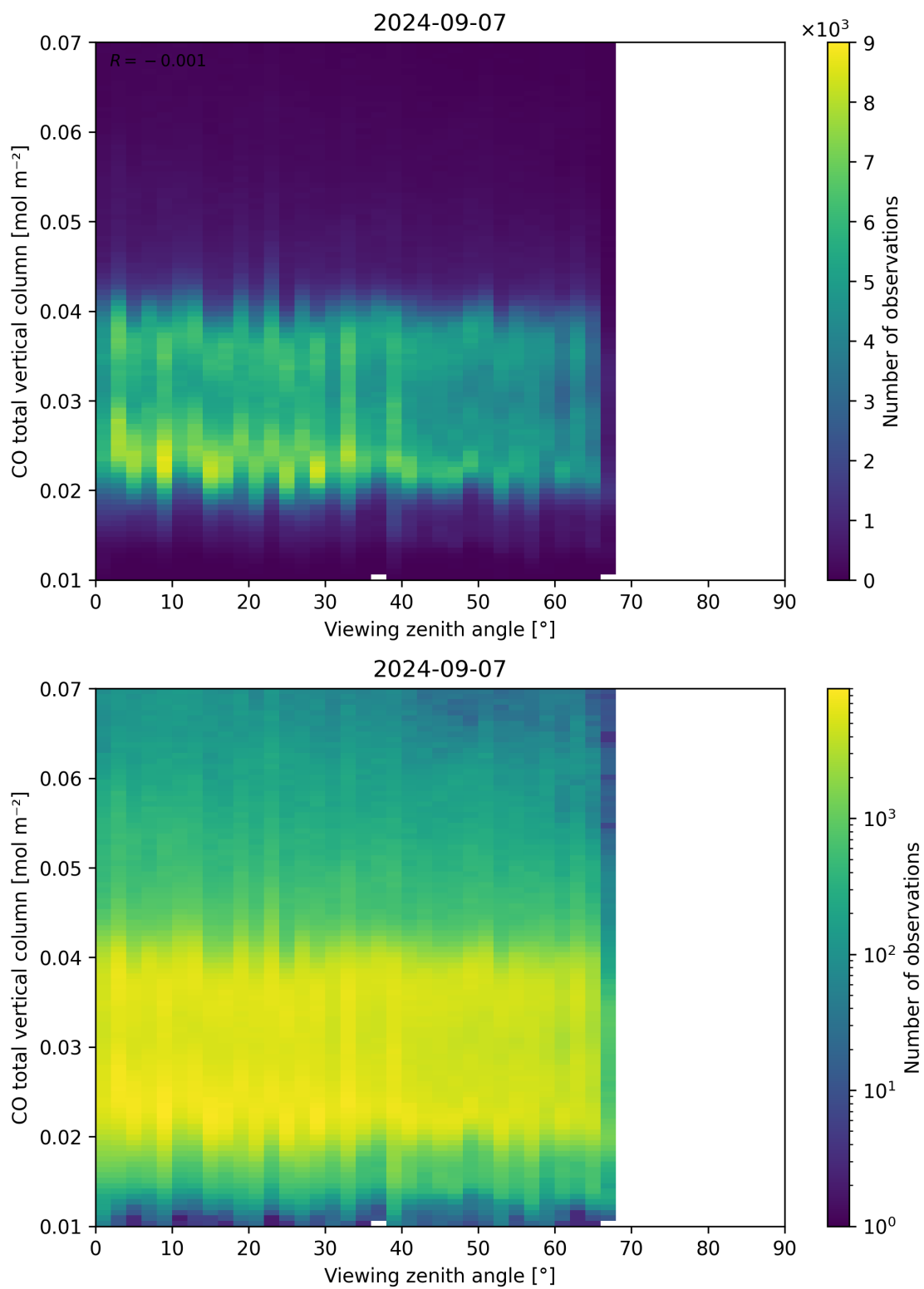
Figure 69: Scatter density plot of “Viewing zenith angle” against “CO total vertical column” for 2024-09-06 to 2024-09-08.
