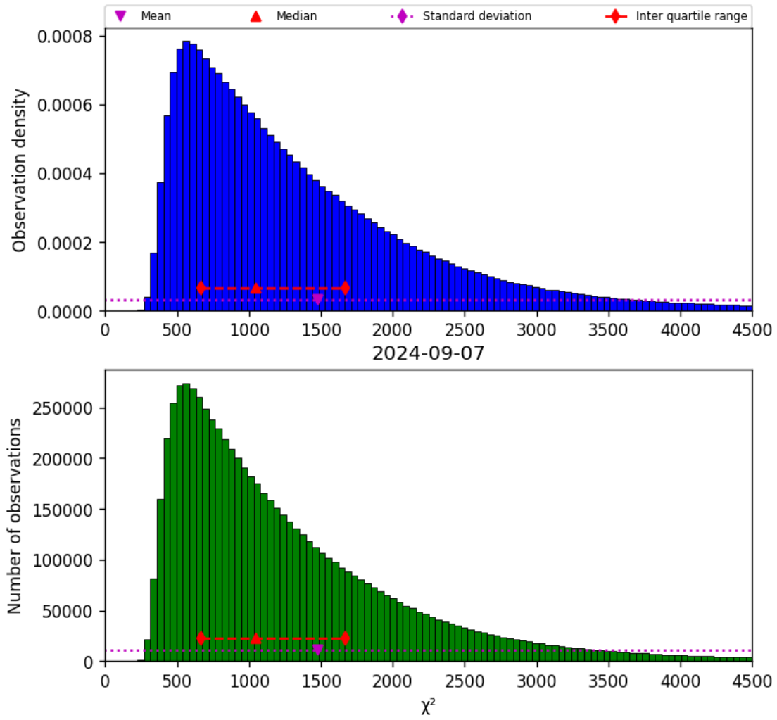
Figure 22: Histogram of " \chi^2 " for 2024-09-06 to 2024-09-08
