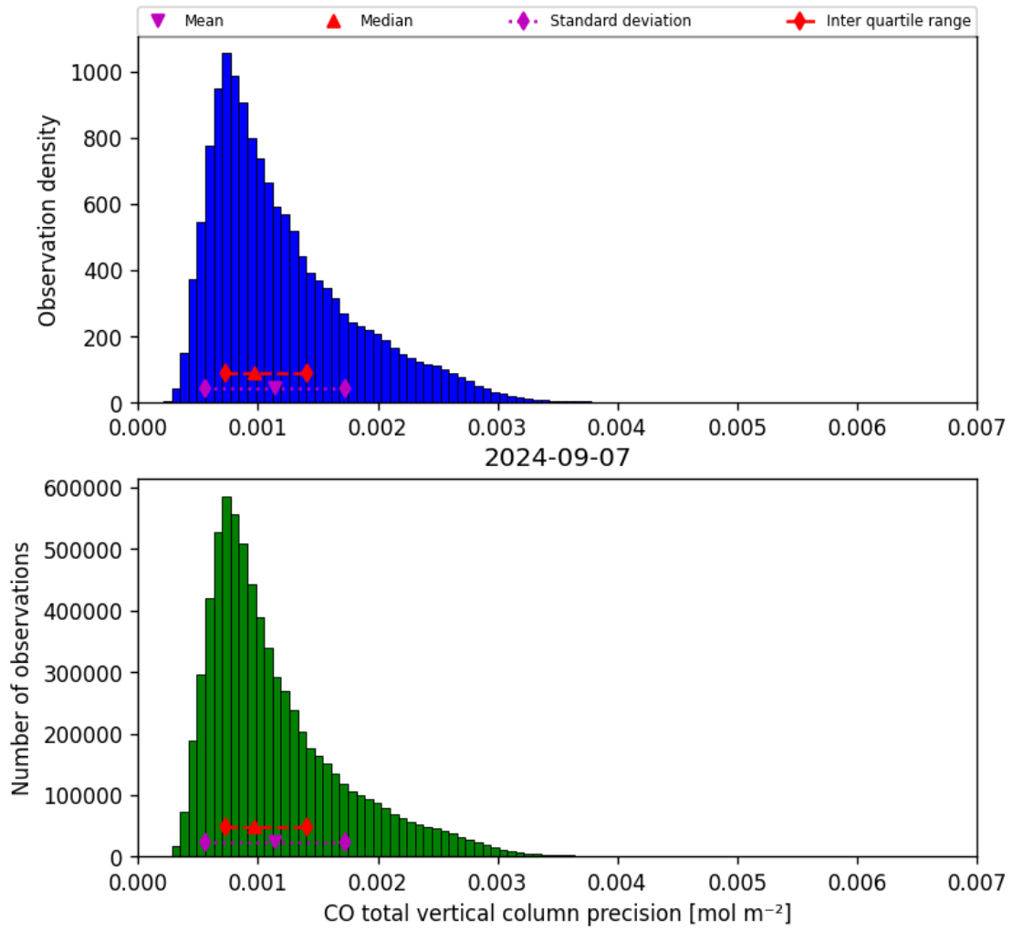
Figure 20: Histogram of “CO total vertical column precision” for 2024-09-06 to 2024-09-08
