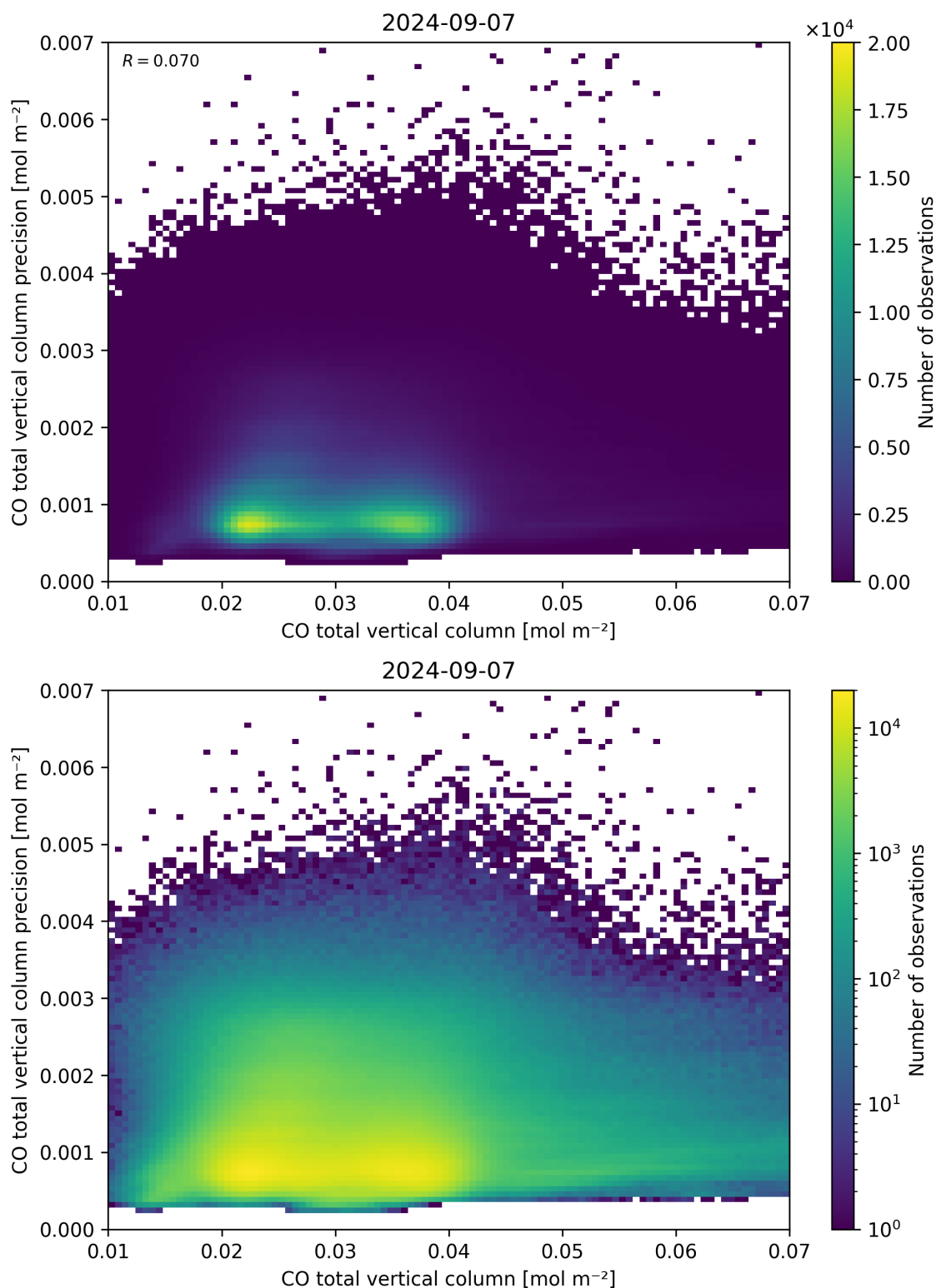
Figure 34: Scatter density plot of “CO total vertical column” against “CO total vertical column precision” for 2024-09-06 to 2024-09-08.
