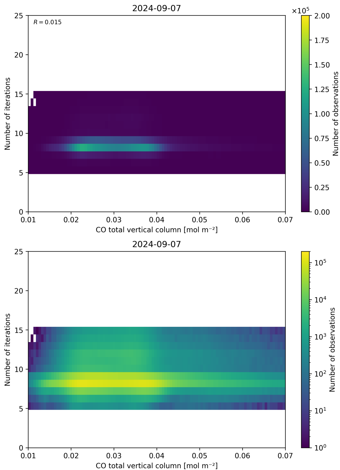
Figure 42: Scatter density plot of “CO total vertical column” against “Number of iterations” for 2024-09-06 to 2024-09-08.
