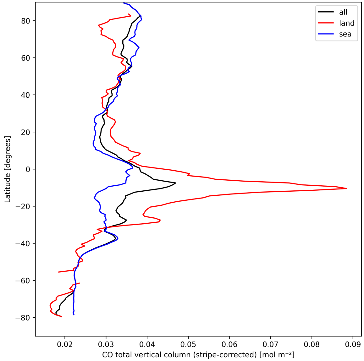
Figure 11: Zonal average of “CO total vertical column (stripe-corrected)” for 2024-09-06 to 2024-09-08.
