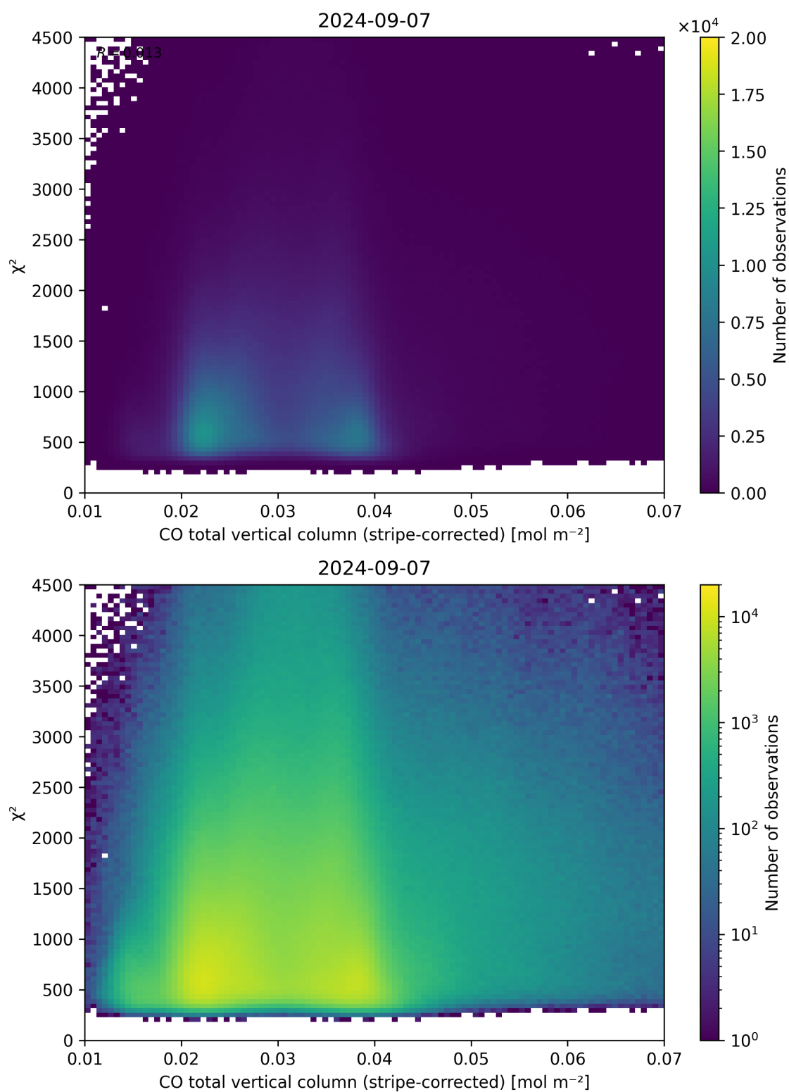
Figure 37: Scatter density plot of “CO total vertical column (stripe-corrected)” against “ \chi^2 ” for 2024-09-06 to 2024-09-08.
