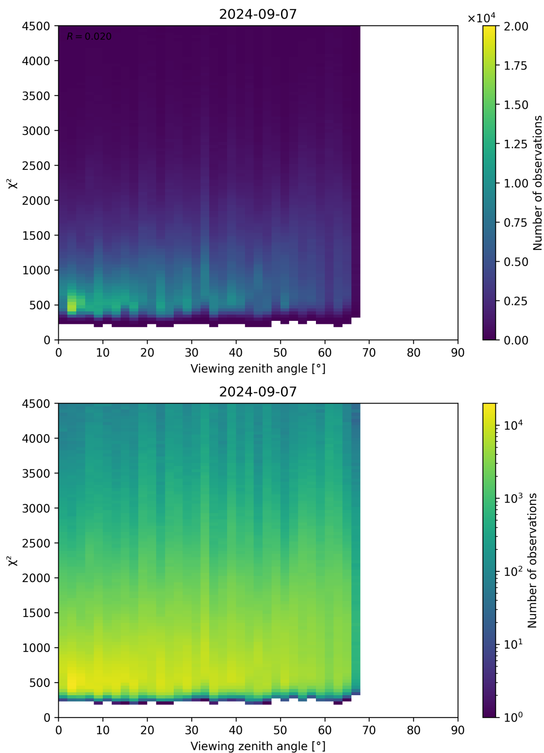
Figure 72: Scatter density plot of “Viewing zenith angle” against “ \chi^2 ” for 2024-09-06 to 2024-09-08.
