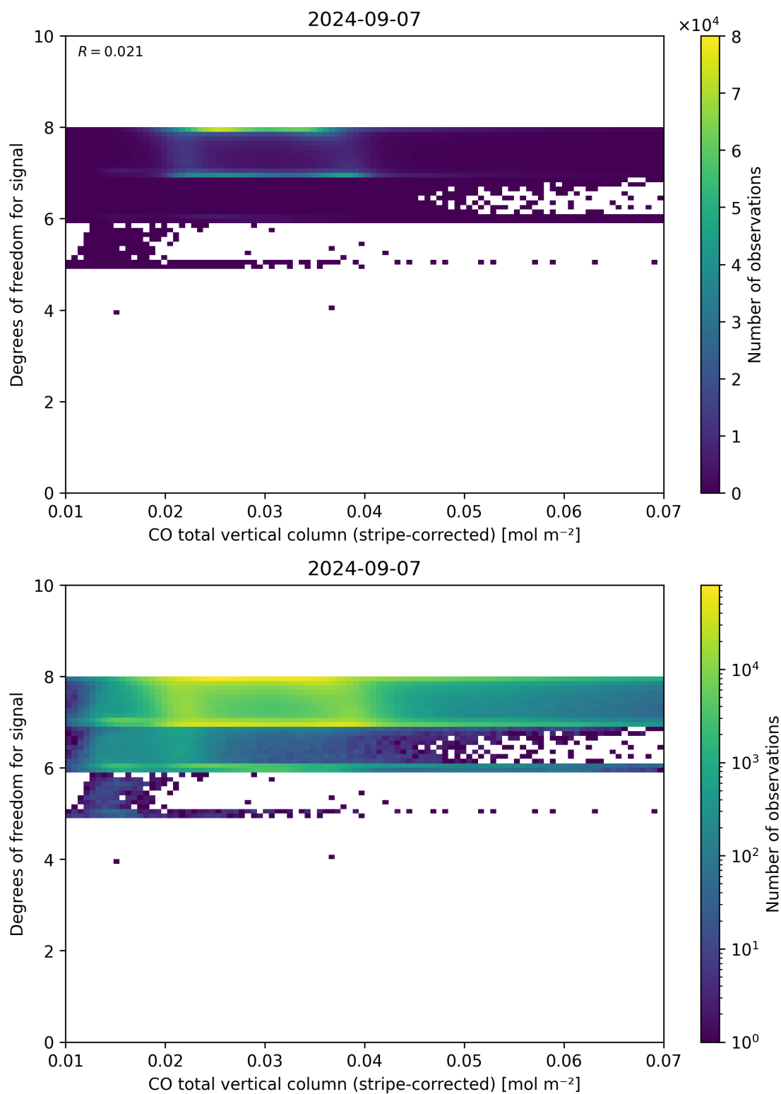
Figure 38: Scatter density plot of “CO total vertical column (stripe-corrected)” against “Degrees of freedom for signal” for 2024-09-06 to 2024-09-08.
