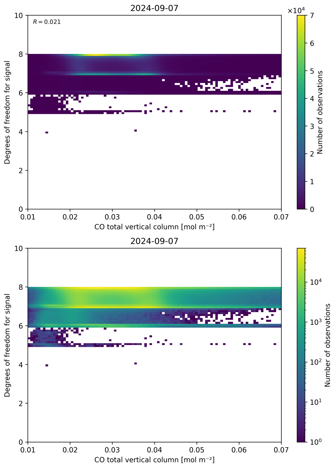
Figure 41: Scatter density plot of “CO total vertical column” against “Degrees of freedom for signal” for 2024-09-06 to 2024-09-08.
