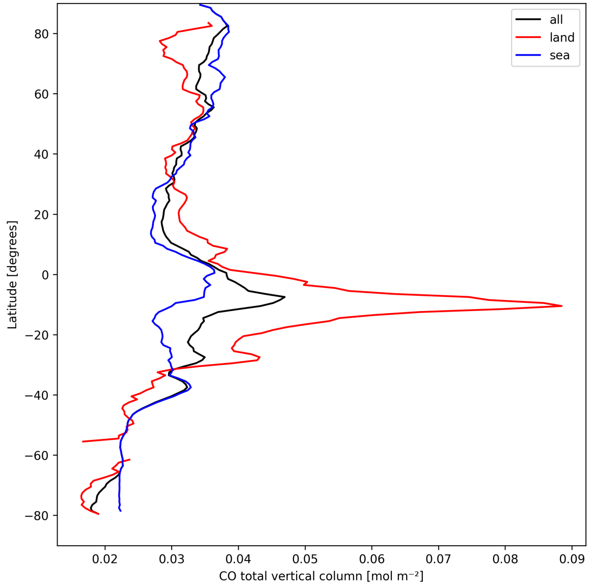
Figure 10: Zonal average of “CO total vertical column” for 2024-09-06 to 2024-09-08.
