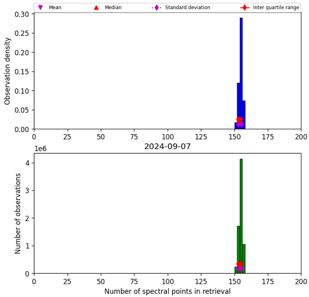
Figure 21: Histogram of “Number of spectral points in retrieval” for 2024-09-06 to 2024-09-08
