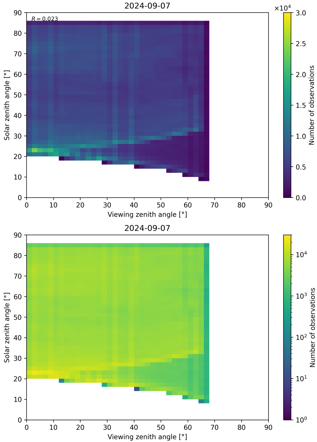
Figure 77: Scatter density plot of “Viewing zenith angle” against “Solar zenith angle” for 2024-09-06 to 2024-09-08.
