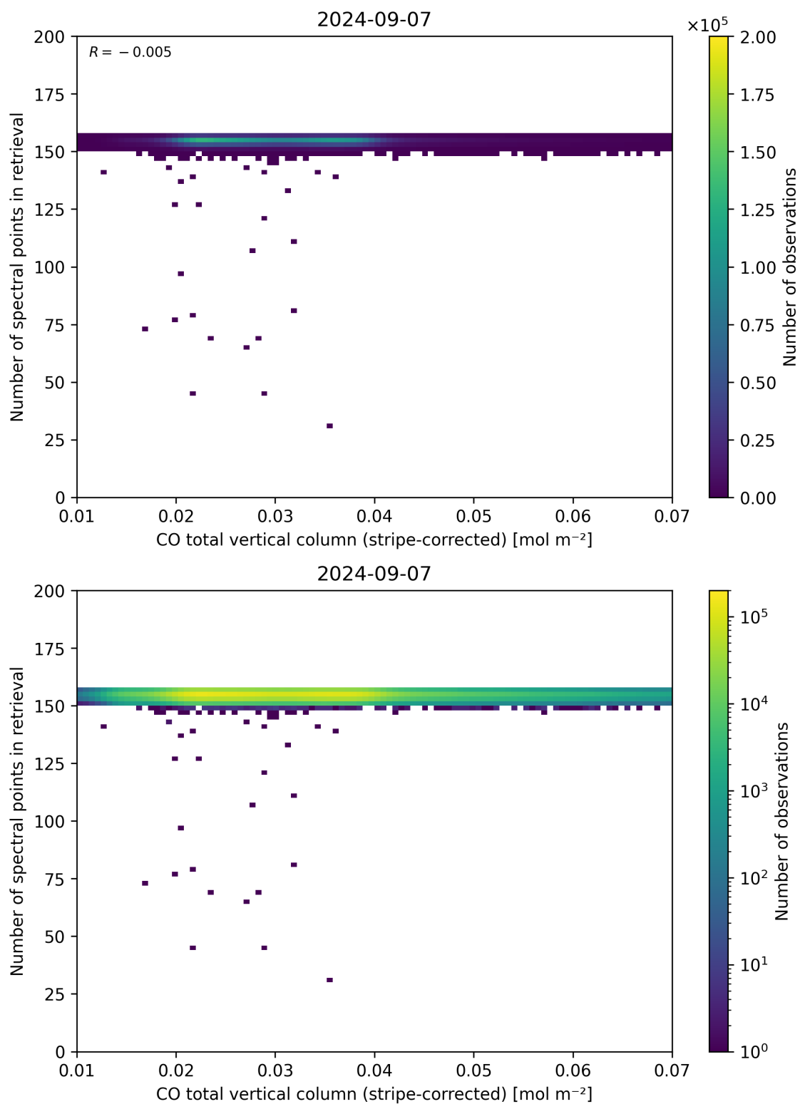
Figure 40: Scatter density plot of “CO total vertical column (stripe-corrected)” against “Number of spectral points in retrieval” for 2024-09-06 to 2024-09-08.
