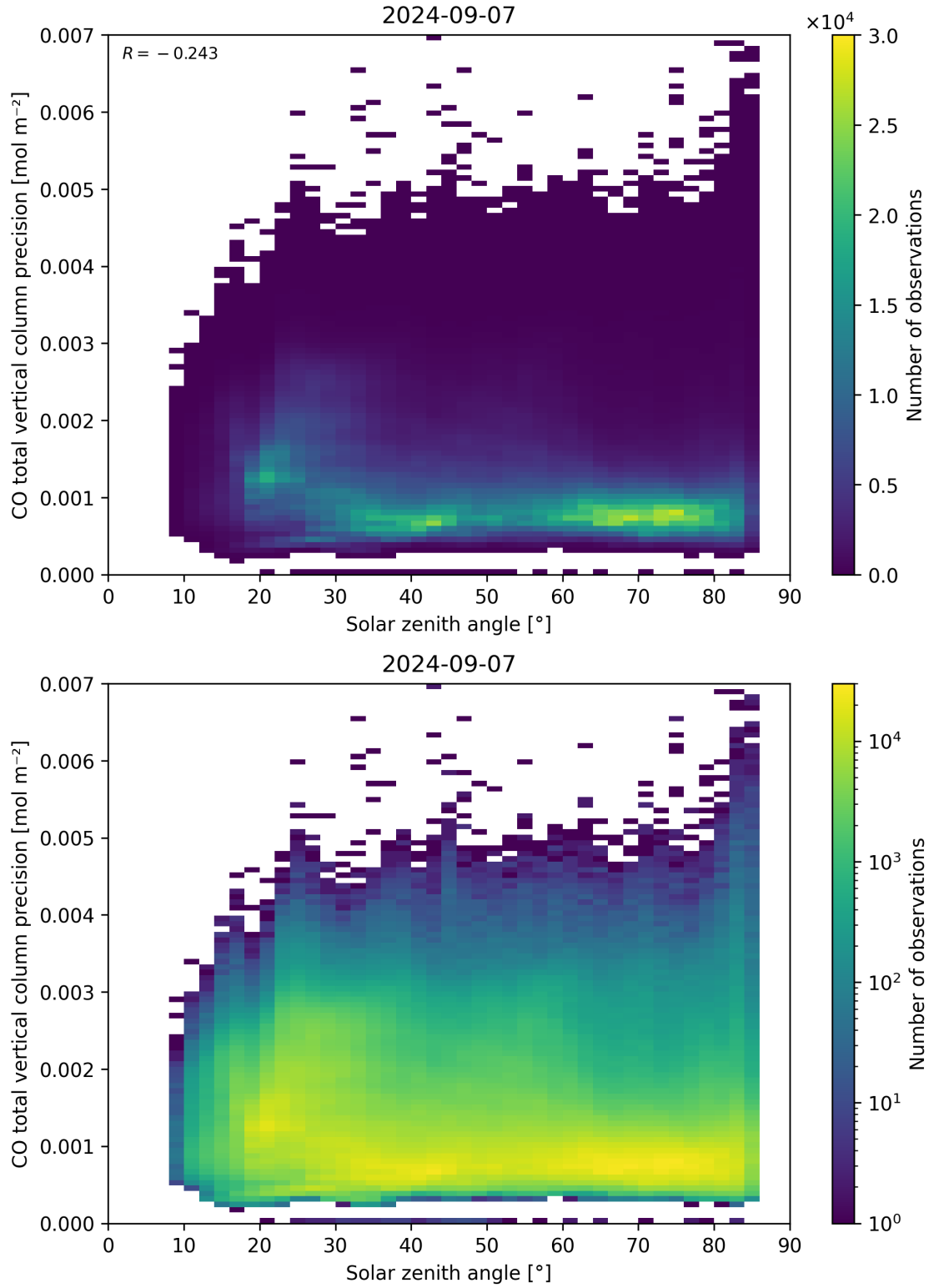
Figure 63: Scatter density plot of “Solar zenith angle” against “CO total vertical column precision” for 2024-09-06 to 2024-09-08.
