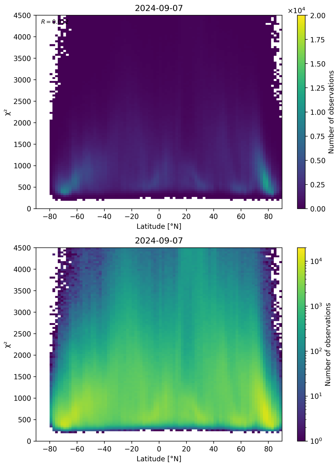
Figure 54: Scatter density plot of “Latitude” against “ \chi^2 ” for 2024-09-06 to 2024-09-08.
