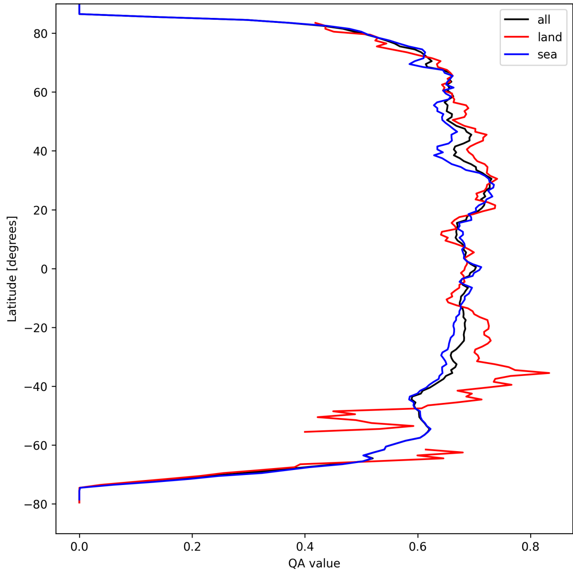
Figure 9: Zonal average of “QA value” for 2024-09-06 to 2024-09-08.
