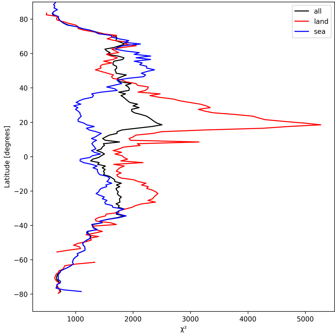
Figure 14: Zonal average of “ \chi^2 ” for 2024-09-06 to 2024-09-08.
