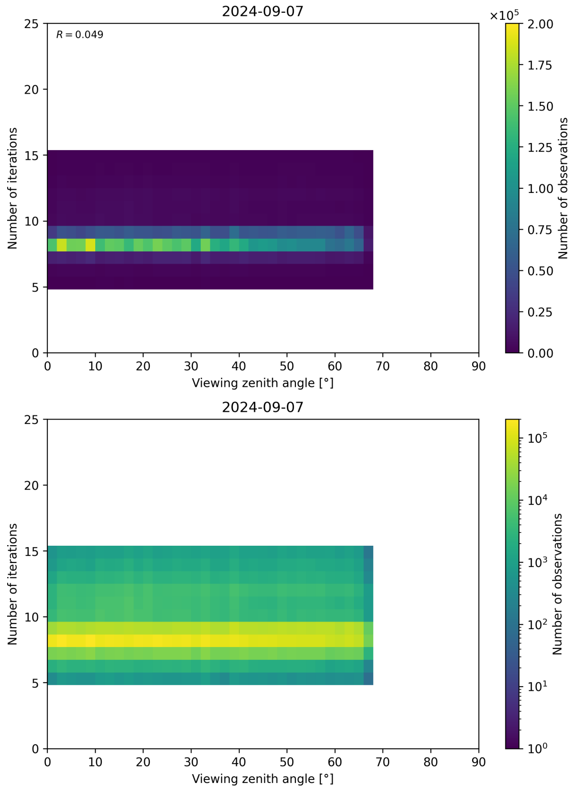
Figure 75: Scatter density plot of “Viewing zenith angle” against “Number of iterations” for 2024-09-06 to 2024-09-08.
