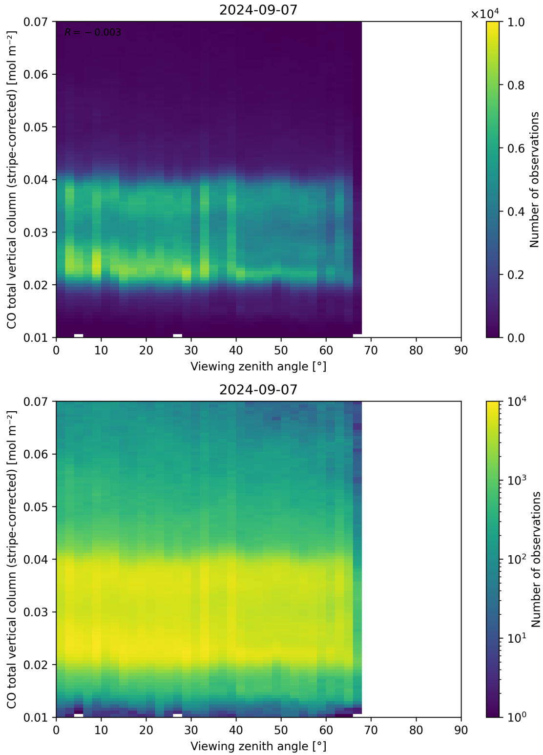
Figure 70: Scatter density plot of “Viewing zenith angle” against “CO total vertical column (stripe-corrected)” for 2024-09-06 to 2024-09-08.
