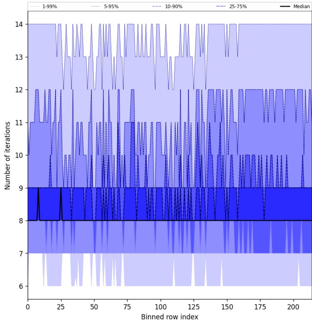
Figure 32: Along track statistics of “Number of iterations” for 2024-09-06 to 2024-09-08
