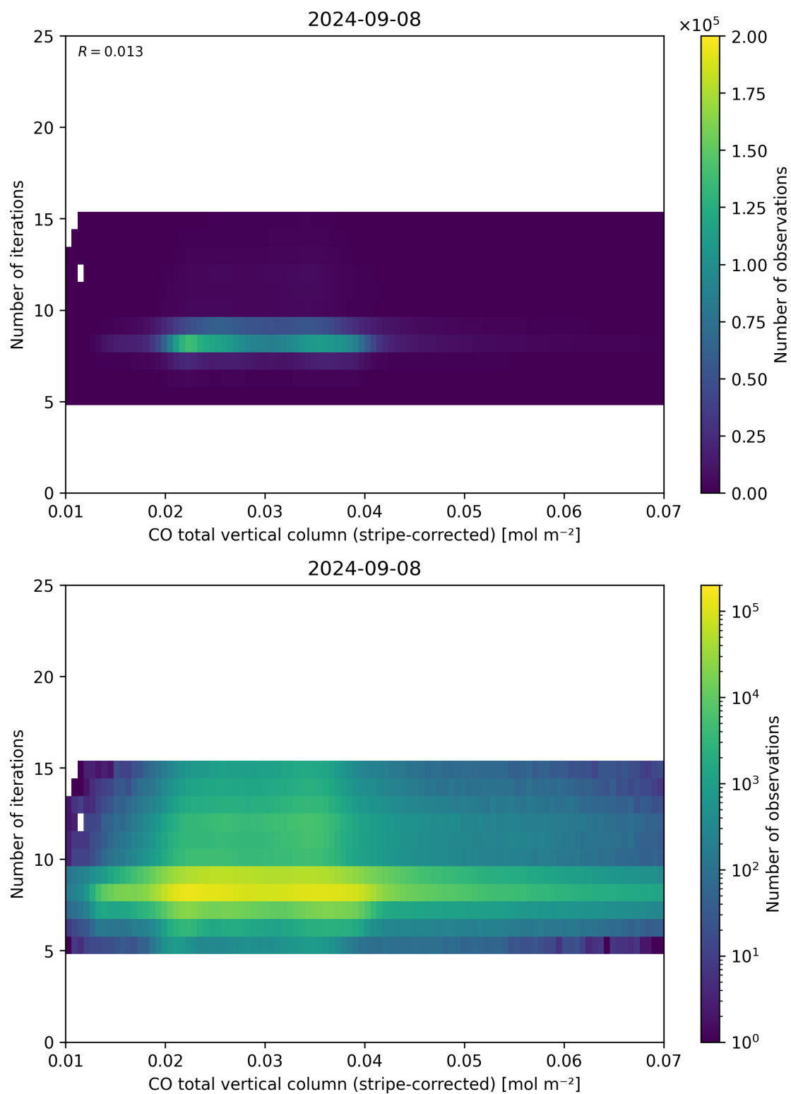
Figure 39: Scatter density plot of “CO total vertical column (stripe-corrected)” against “Number of iterations” for 2024-09-07 to 2024-09-09.
