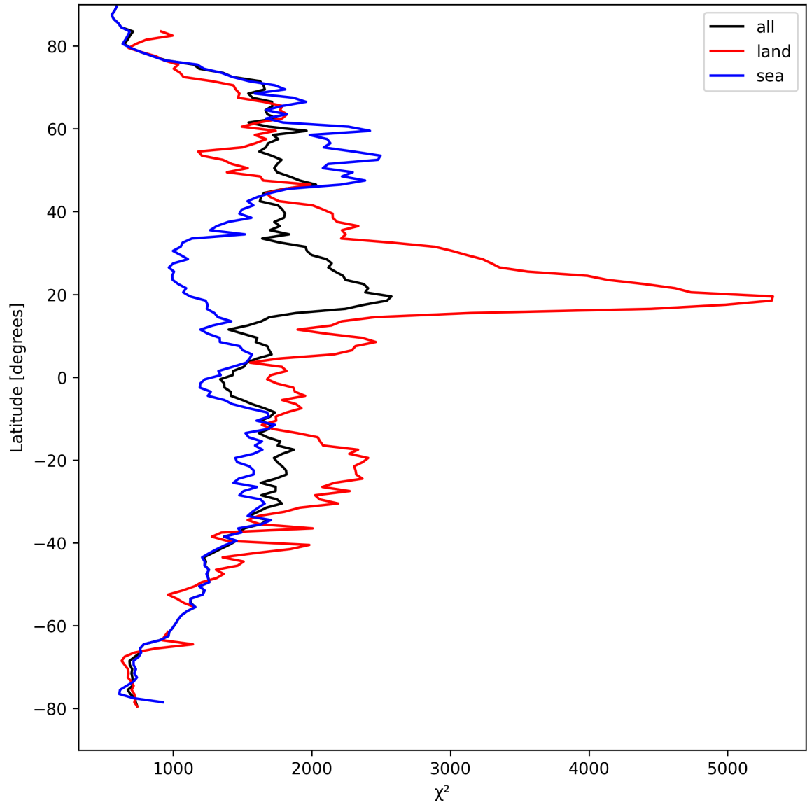
Figure 14: Zonal average of “ \chi^2 ” for 2024-09-07 to 2024-09-09.
