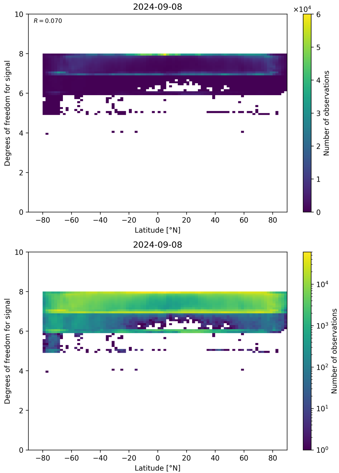
Figure 55: Scatter density plot of “Latitude” against “Degrees of freedom for signal” for 2024-09-07 to 2024-09-09.
