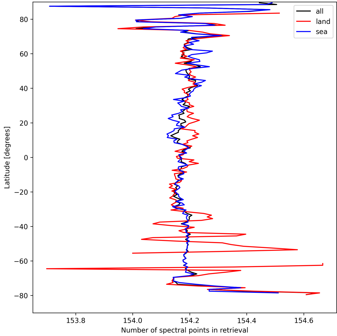
Figure 13: Zonal average of “Number of spectral points in retrieval” for 2024-09-07 to 2024-09-09.
