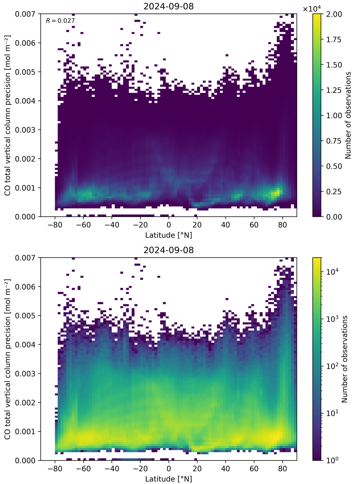
Figure 53: Scatter density plot of “Latitude” against “CO total vertical column precision” for 2024-09-07 to 2024-09-09.
