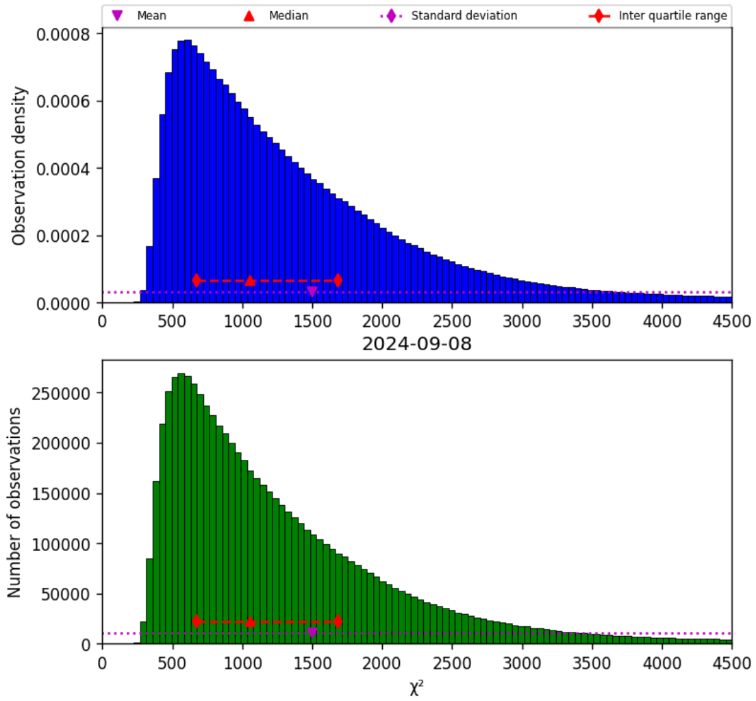
Figure 22: Histogram of “ \chi^2 ” for 2024-09-07 to 2024-09-09
