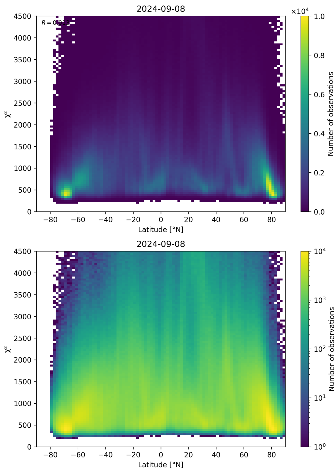
Figure 54: Scatter density plot of “Latitude” against “ \chi^2 ” for 2024-09-07 to 2024-09-09.
