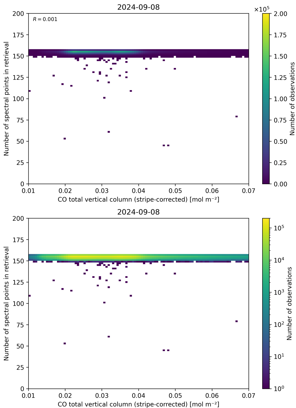
Figure 40: Scatter density plot of “CO total vertical column (stripe-corrected)” against “Number of spectral points in retrieval” for 2024-09-07 to 2024-09-09.
