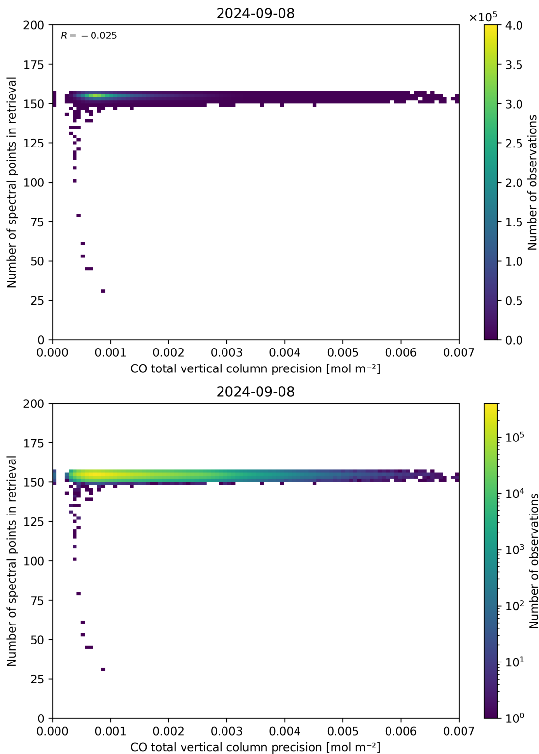
Figure 47: Scatter density plot of “CO total vertical column precision” against “Number of spectral points in retrieval” for 2024-09-07 to 2024-09-09.
