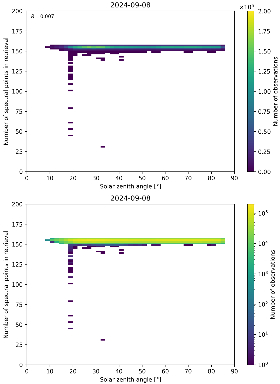
Figure 68: Scatter density plot of “Solar zenith angle” against “Number of spectral points in retrieval” for 2024-09-07 to 2024-09-09.
