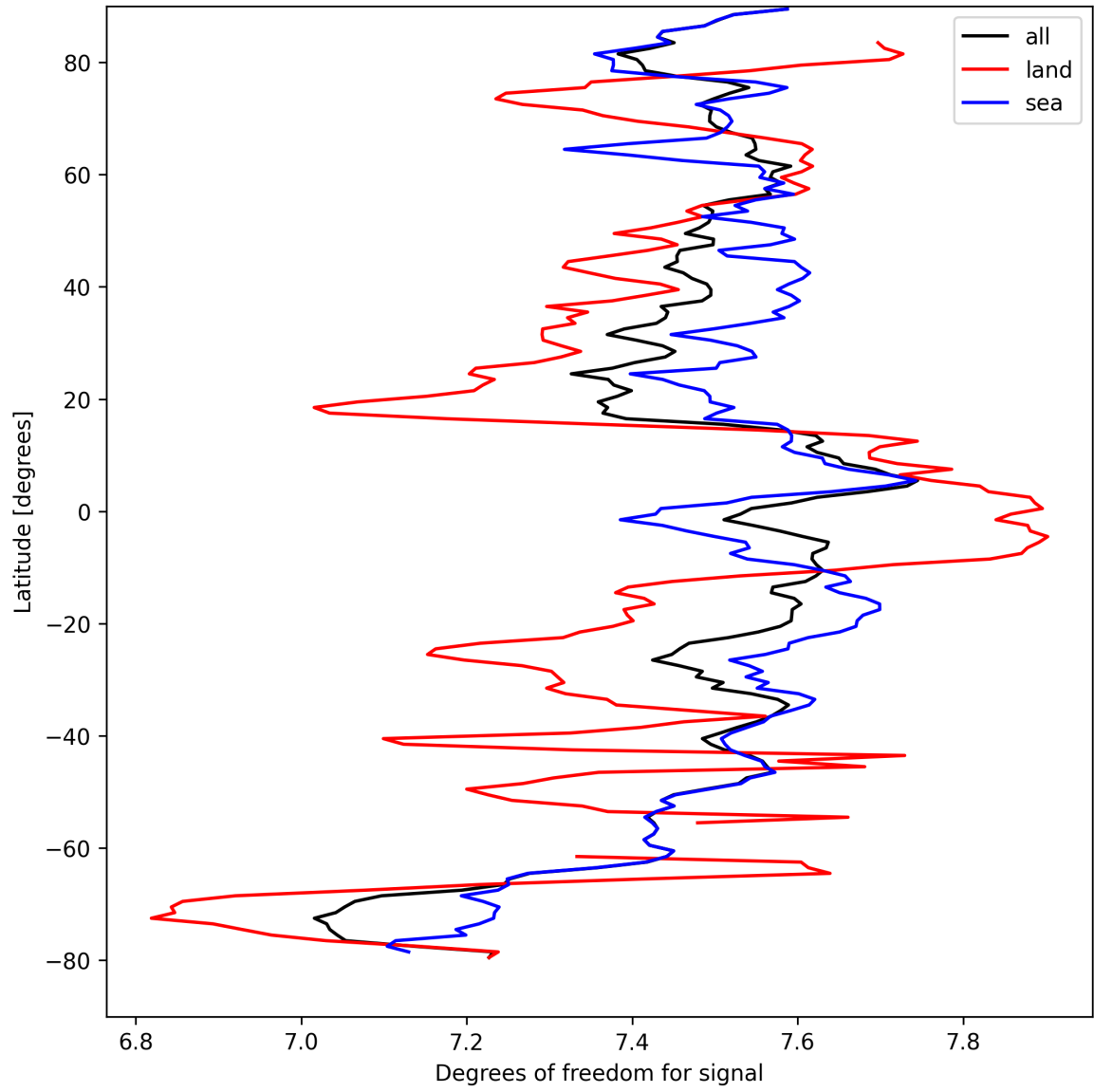
Figure 15: Zonal average of “Degrees of freedom for signal” for 2024-09-07 to 2024-09-09.
