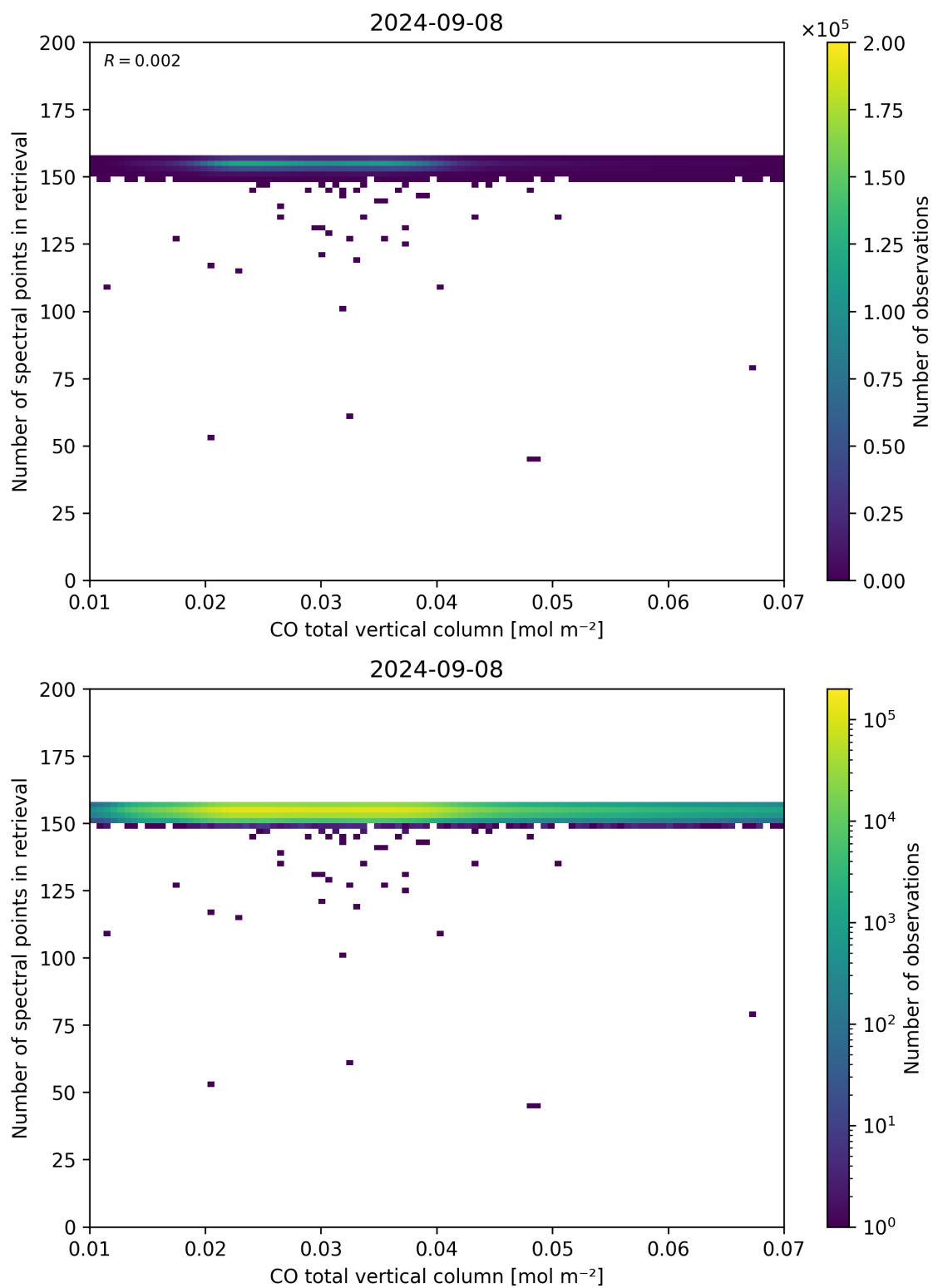
Figure 43: Scatter density plot of “CO total vertical column” against “Number of spectral points in retrieval” for 2024-09-07 to 2024-09-09.
