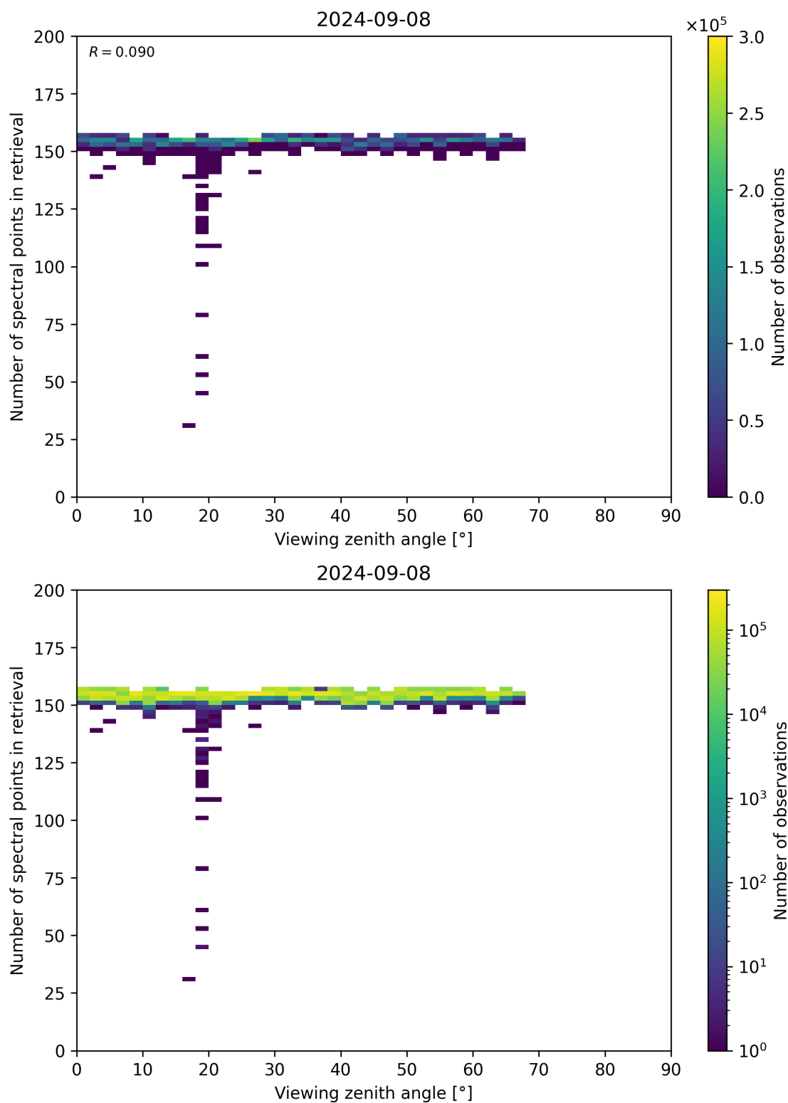
Figure 76: Scatter density plot of “Viewing zenith angle” against “Number of spectral points in retrieval” for 2024-09-07 to 2024-09-09.
