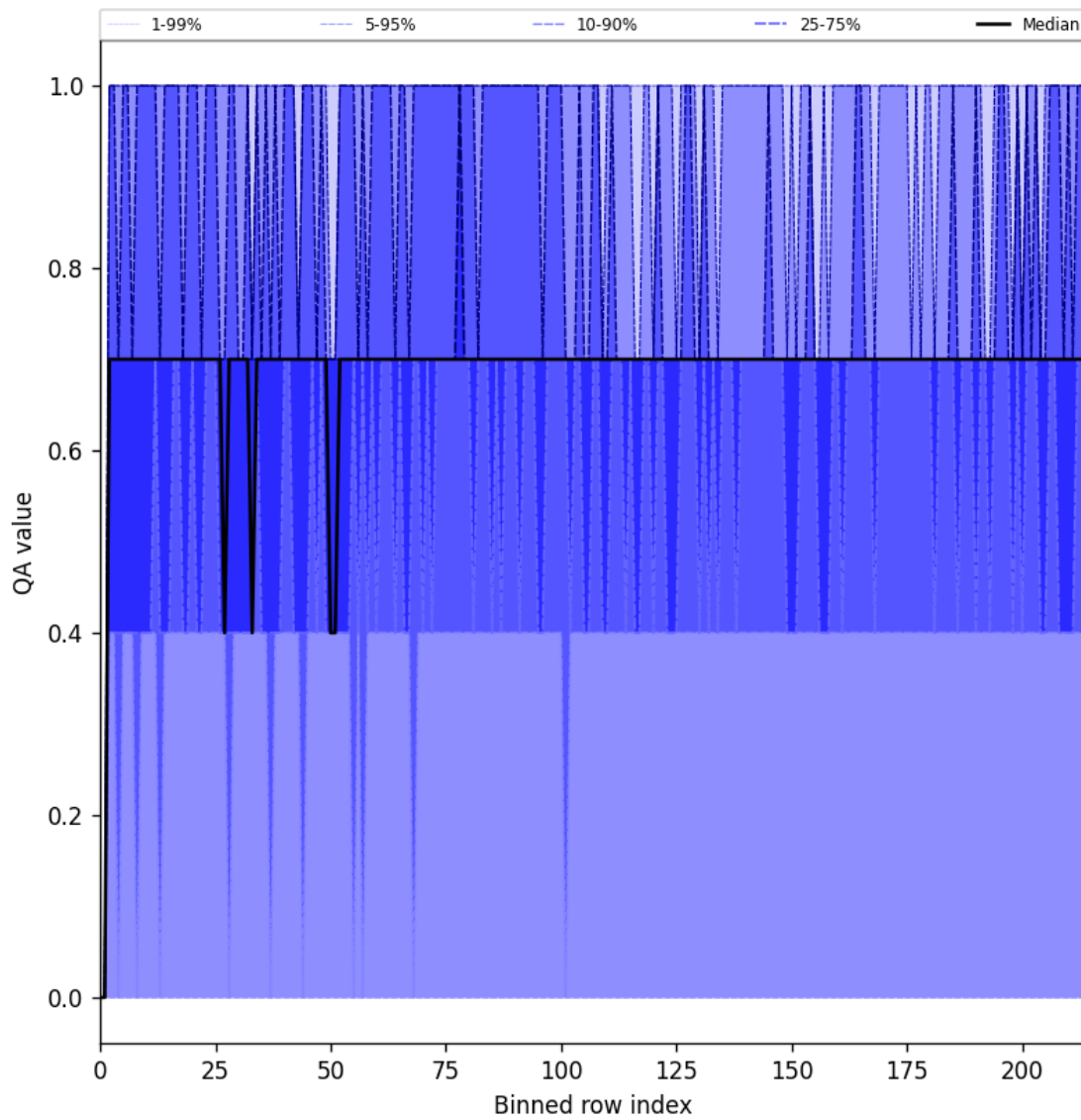
Figure 25: Along track statistics of “QA value” for 2024-09-07 to 2024-09-09
