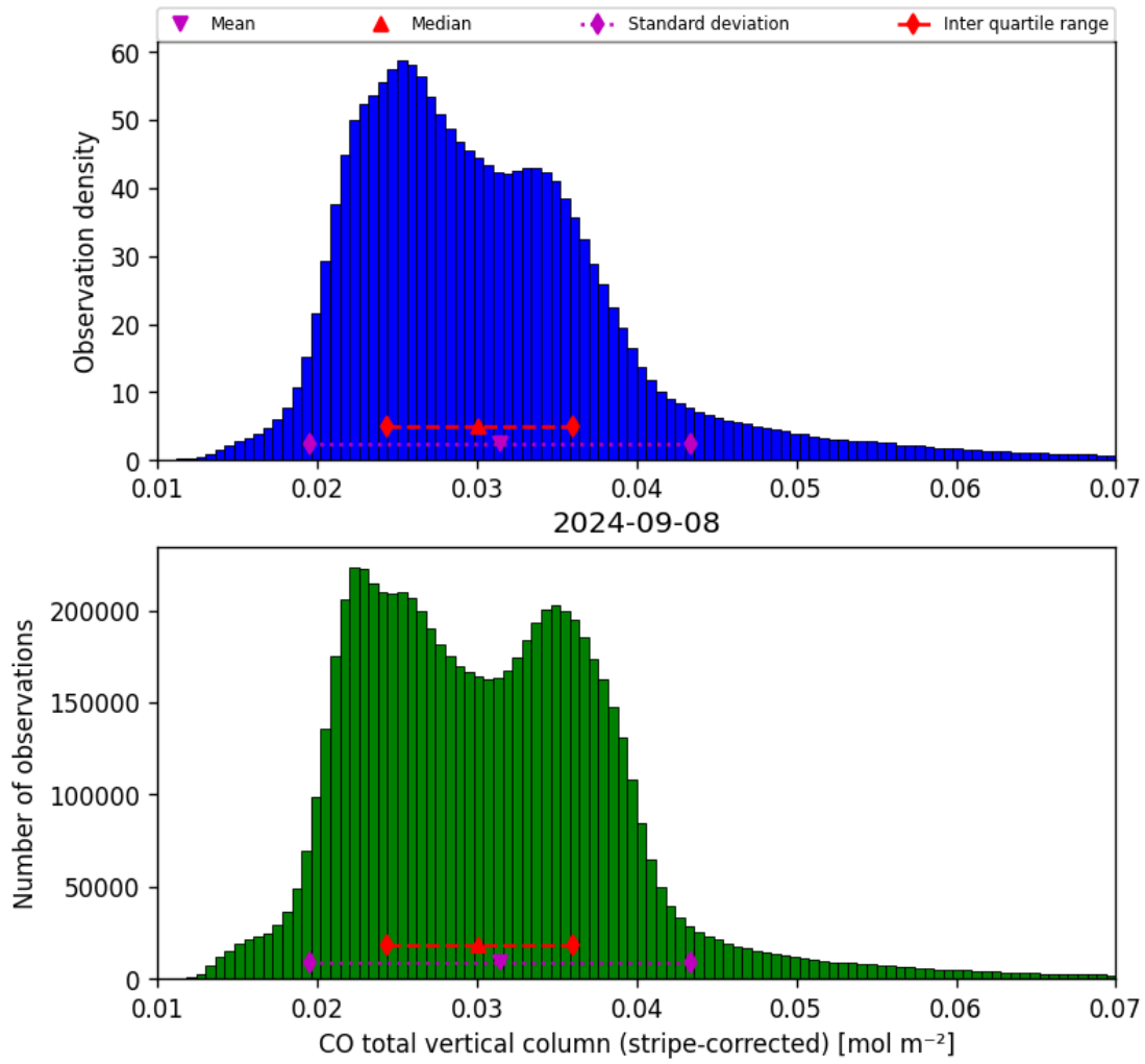
Figure 19: Histogram of “CO total vertical column (stripe-corrected)” for 2024-09-07 to 2024-09-09
