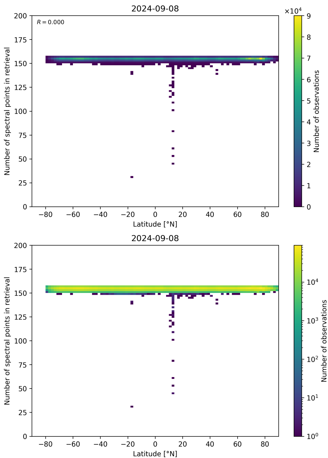
Figure 57: Scatter density plot of “Latitude” against “Number of spectral points in retrieval” for 2024-09-07 to 2024-09-09.
