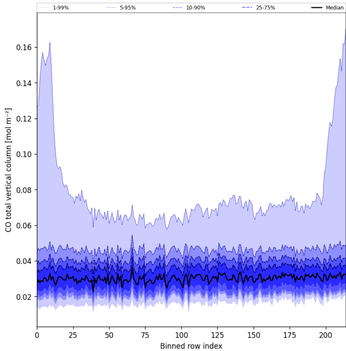
Figure 26: Along track statistics of “CO total vertical column” for 2024-09-07 to 2024-09-09
