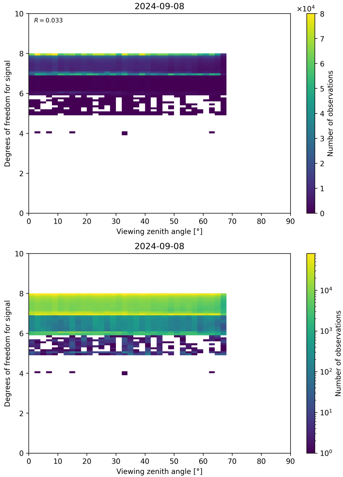
Figure 73: Scatter density plot of “Viewing zenith angle” against “Degrees of freedom for signal” for 2024-09-07 to 2024-09-09.
