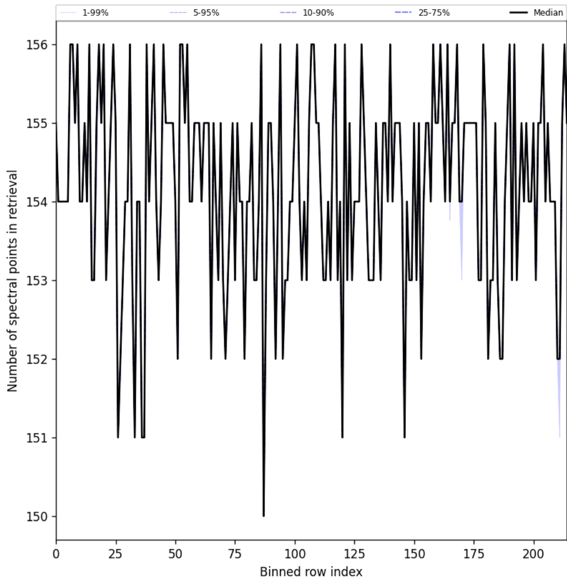
Figure 29: Along track statistics of “Number of spectral points in retrieval” for 2024-09-07 to 2024-09-09
