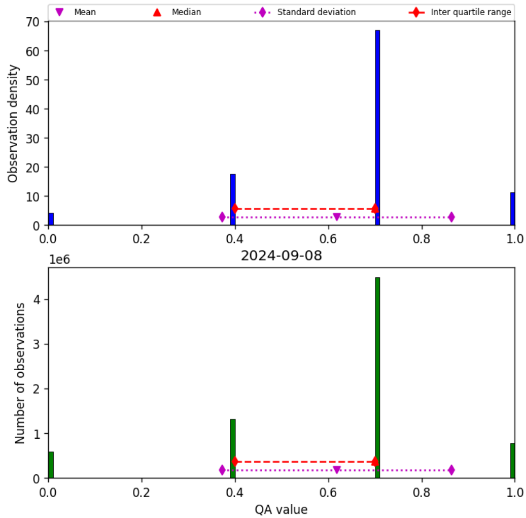
Figure 17: Histogram of “QA value” for 2024-09-07 to 2024-09-09
