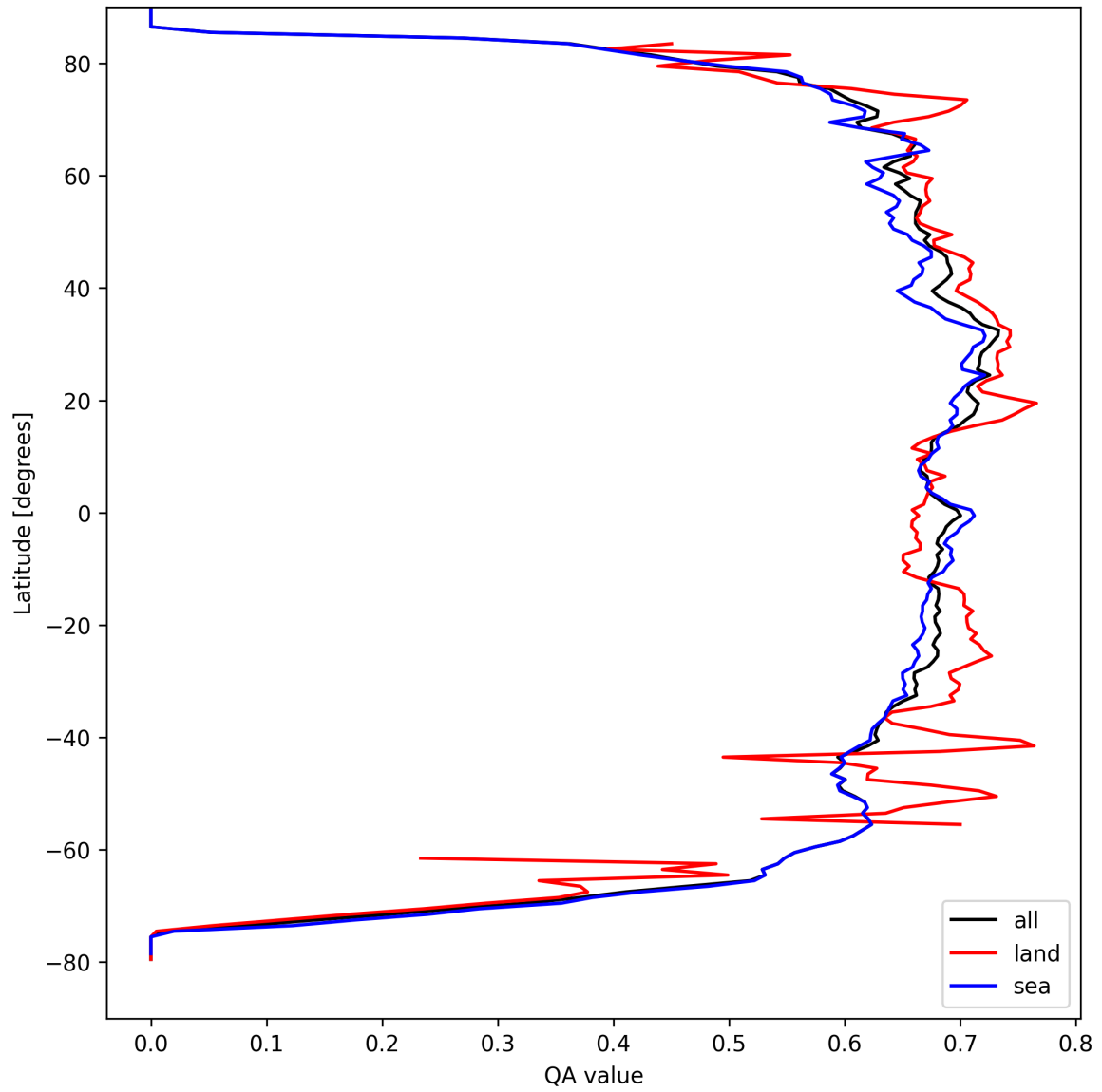
Figure 9: Zonal average of “QA value” for 2024-09-07 to 2024-09-09.
