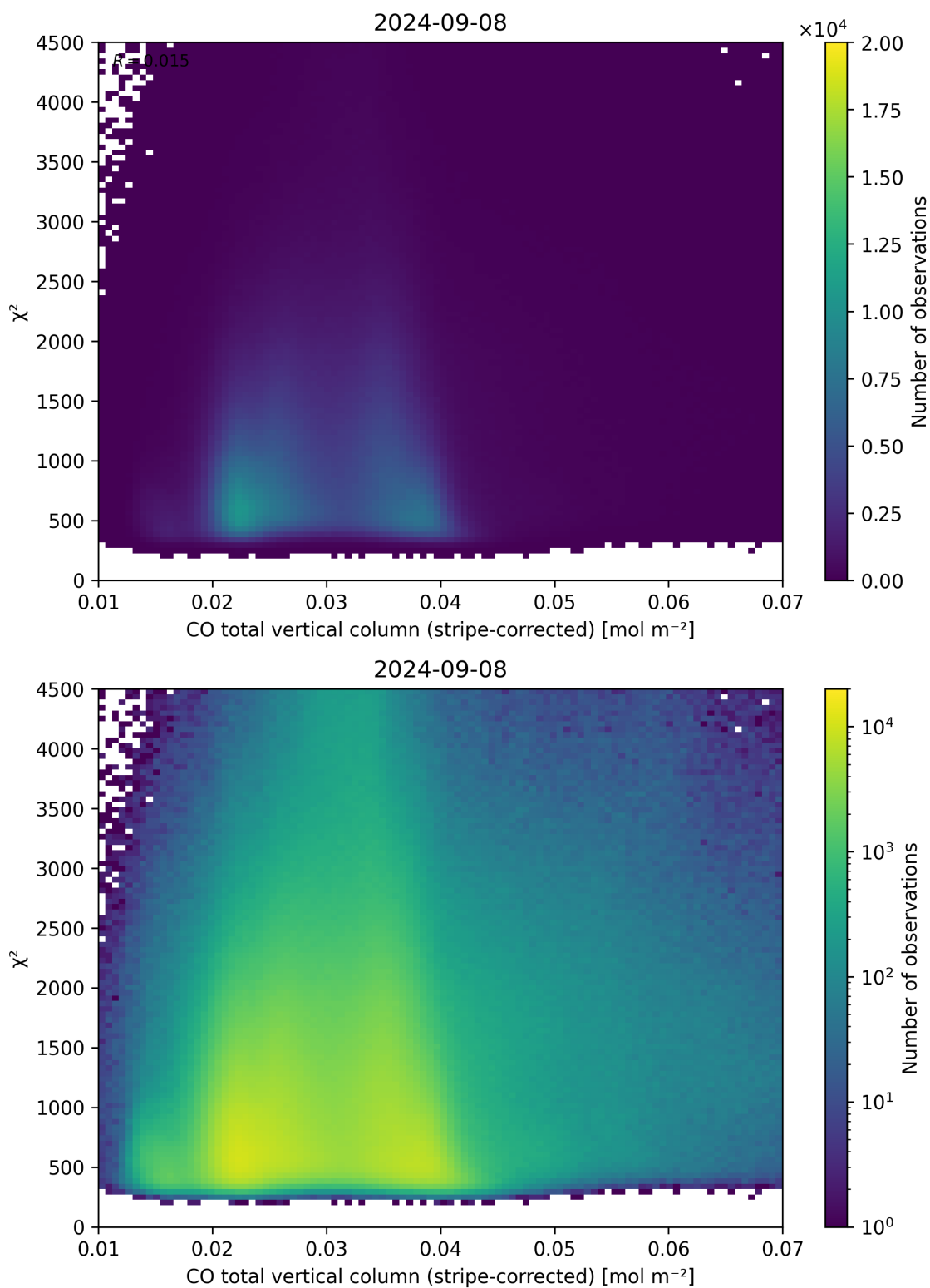
Figure 37: Scatter density plot of “CO total vertical column (stripe-corrected)” against “ \chi^2 ” for 2024-09-07 to 2024-09-09.
