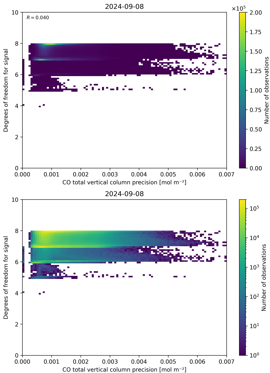
Figure 45: Scatter density plot of “CO total vertical column precision” against “Degrees of freedom for signal” for 2024-09-07 to 2024-09-09.
