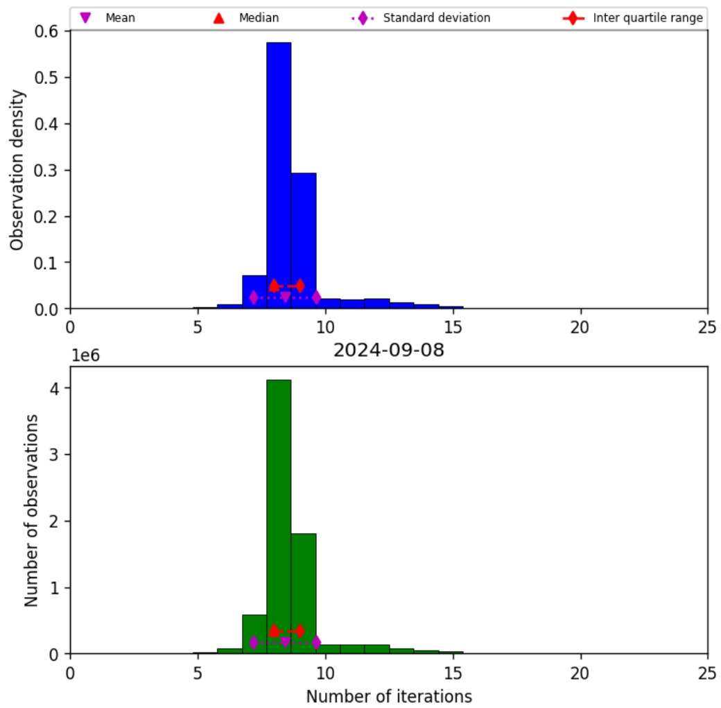
Figure 24: Histogram of “Number of iterations” for 2024-09-07 to 2024-09-09
