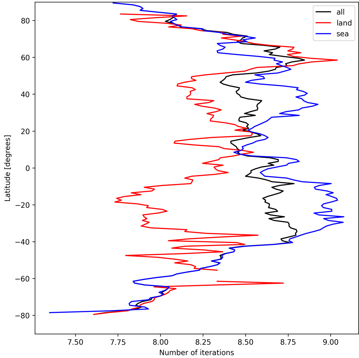
Figure 16: Zonal average of “Number of iterations” for 2024-09-07 to 2024-09-09.
