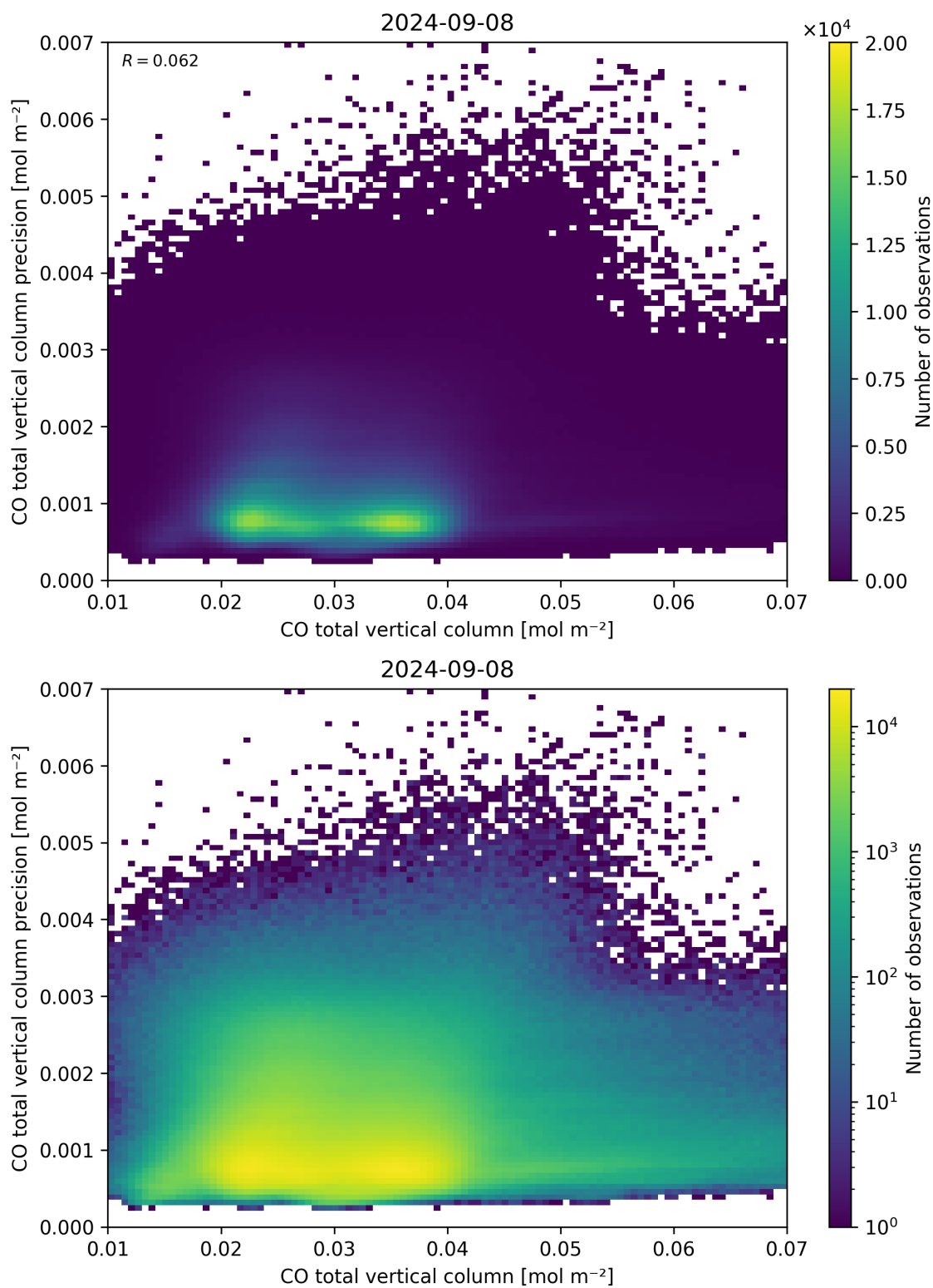
Figure 34: Scatter density plot of “CO total vertical column” against “CO total vertical column precision” for 2024-09-07 to 2024-09-09.
