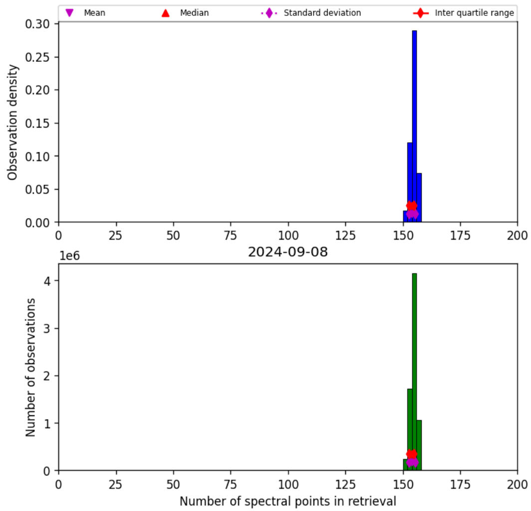
Figure 21: Histogram of “Number of spectral points in retrieval” for 2024-09-07 to 2024-09-09
