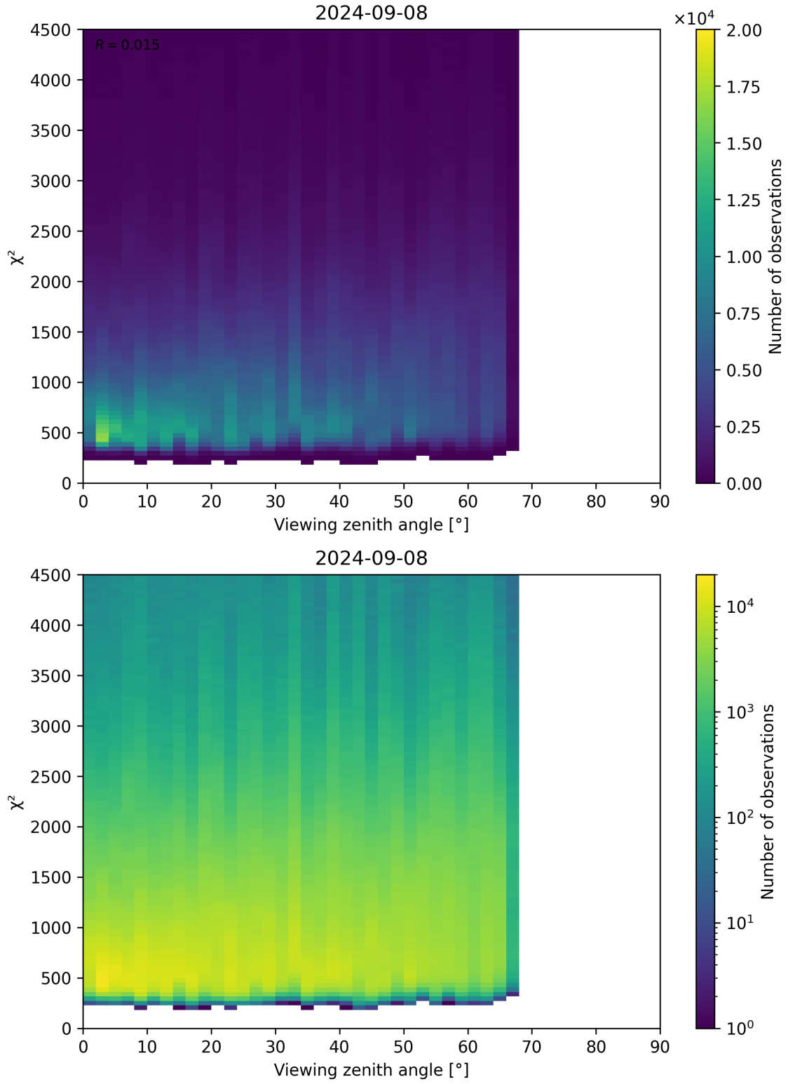
Figure 72: Scatter density plot of “Viewing zenith angle” against “ \chi^2 ” for 2024-09-07 to 2024-09-09.
