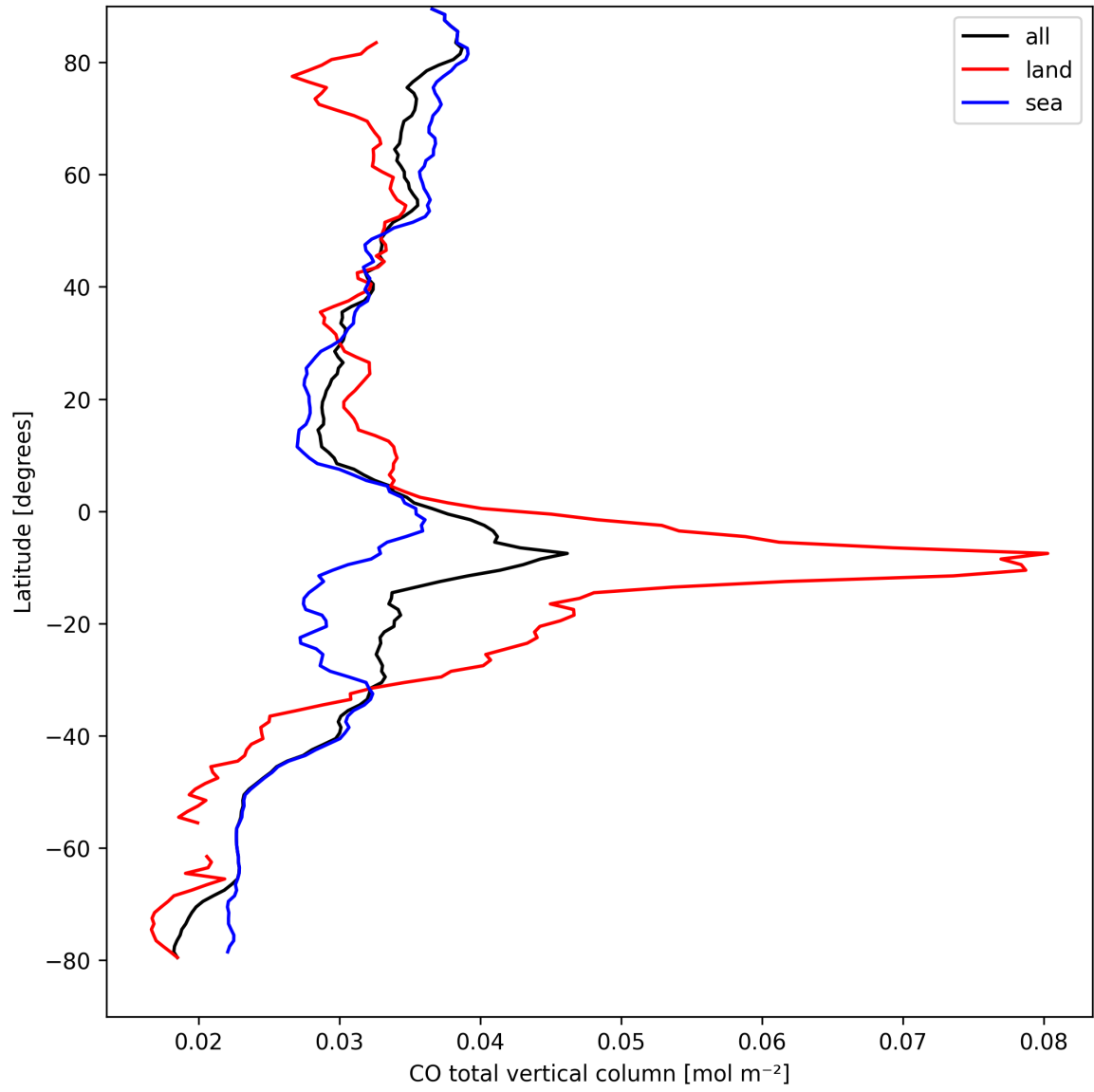
Figure 10: Zonal average of “CO total vertical column” for 2024-09-07 to 2024-09-09.
