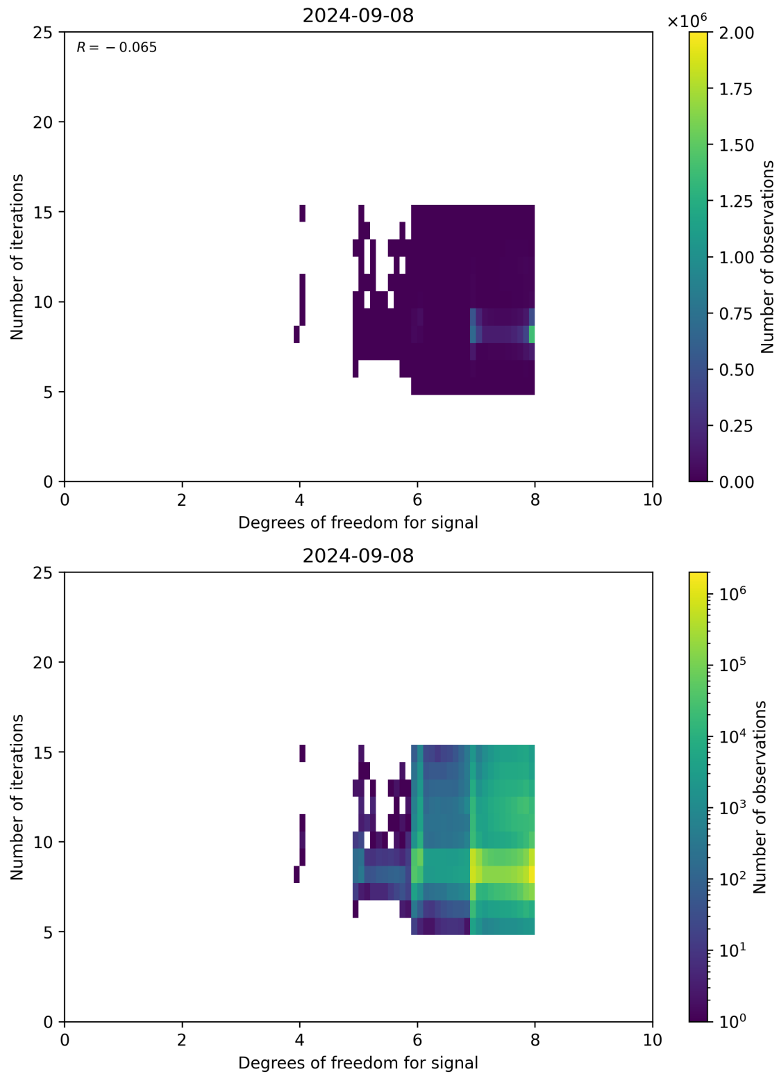
Figure 50: Scatter density plot of “Degrees of freedom for signal” against “Number of iterations” for 2024-09-07 to 2024-09-09.
