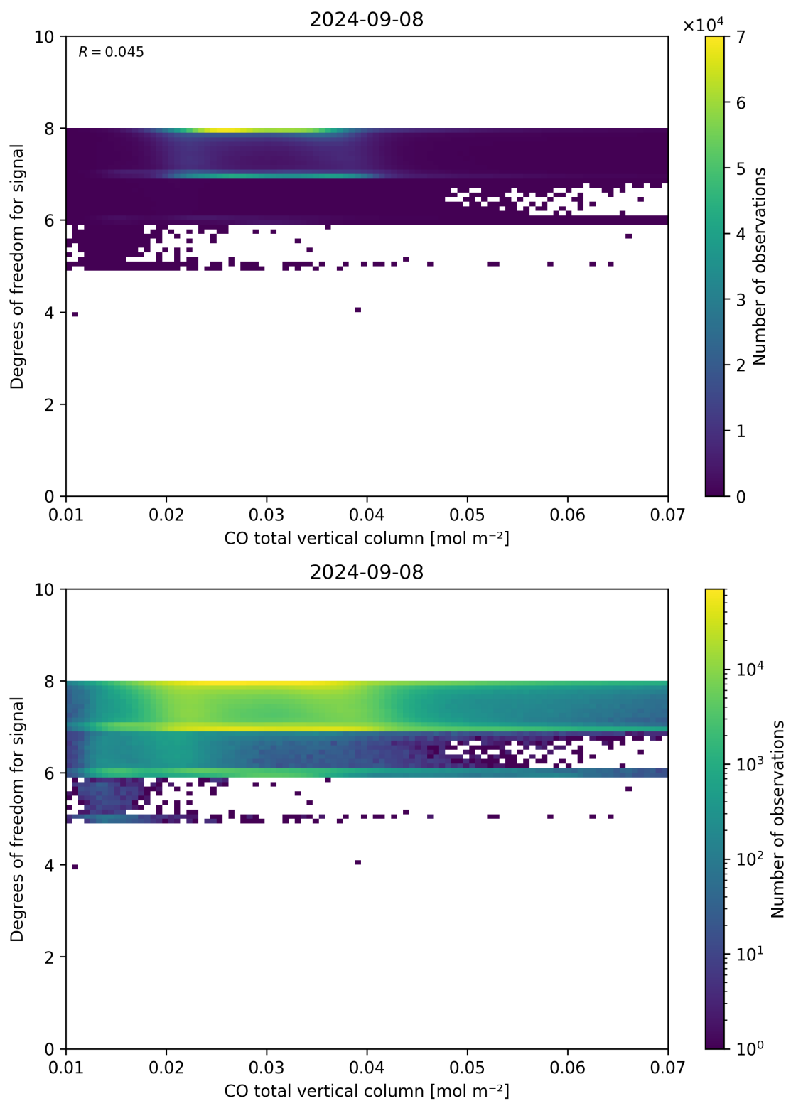
Figure 41: Scatter density plot of “CO total vertical column” against “Degrees of freedom for signal” for 2024-09-07 to 2024-09-09.
