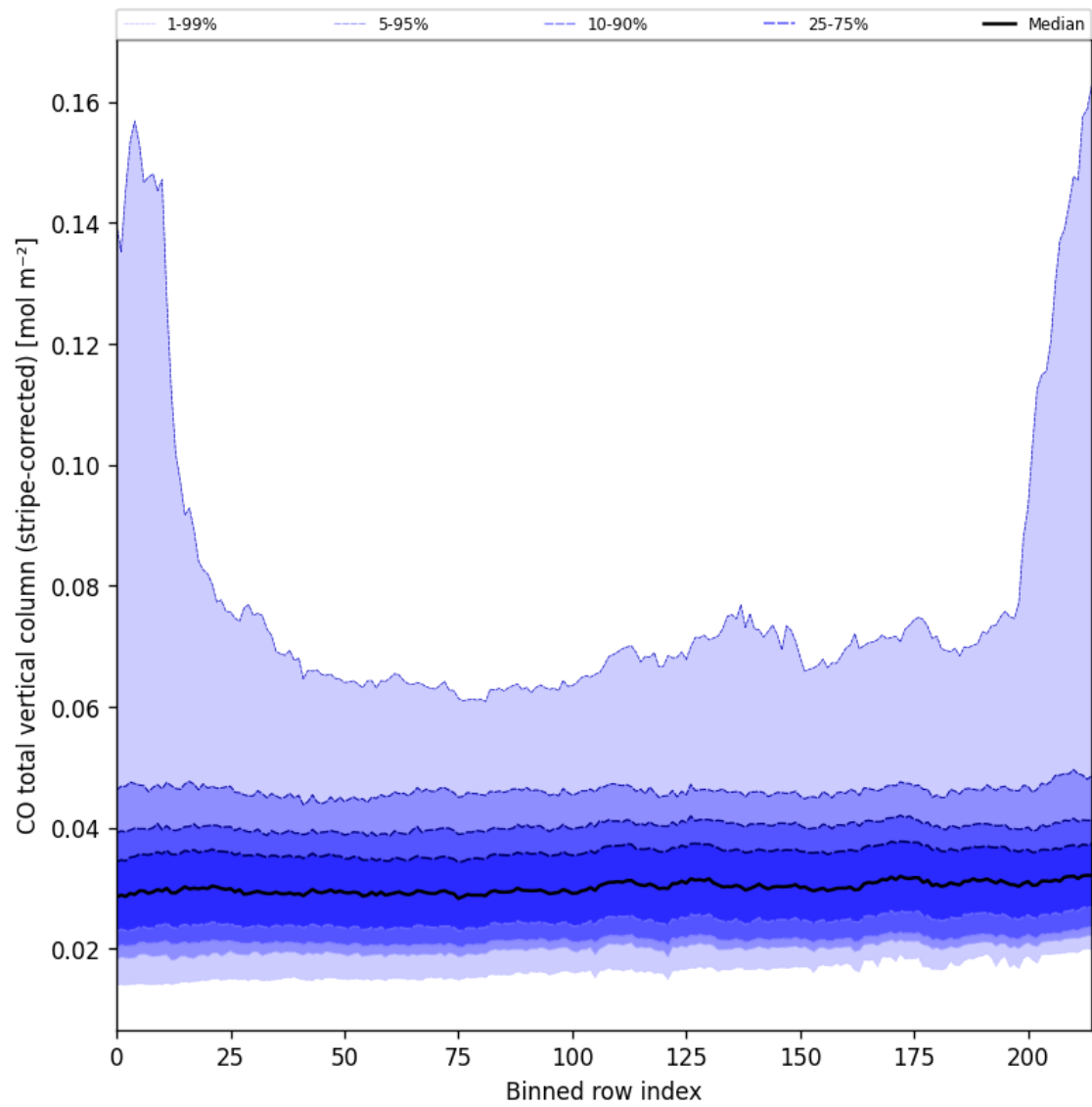
Figure 27: Along track statistics of “CO total vertical column (stripe-corrected)” for 2024-09-07 to 2024-09-09
