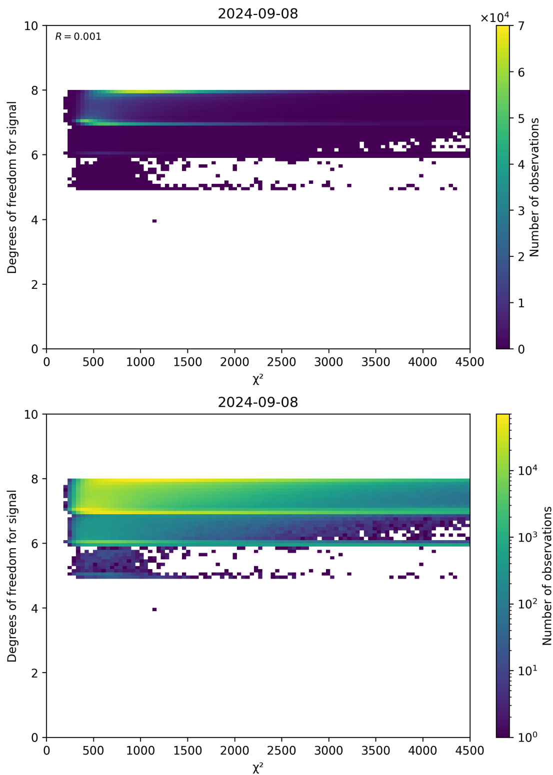
Figure 48: Scatter density plot of “ \chi^2 ” against “Degrees of freedom for signal” for 2024-09-07 to 2024-09-09.
