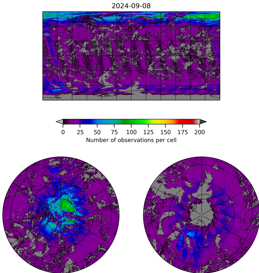
Figure 8: Map of the number of observations for 2024-09-07 to 2024-09-09
