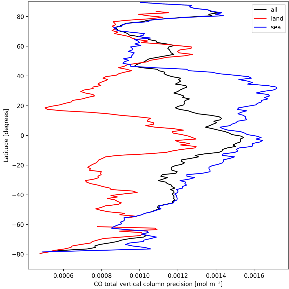
Figure 12: Zonal average of “CO total vertical column precision” for 2024-09-07 to 2024-09-09.
