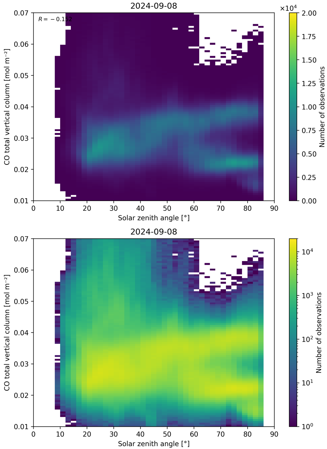
Figure 61: Scatter density plot of “Solar zenith angle” against “CO total vertical column” for 2024-09-07 to 2024-09-09.
