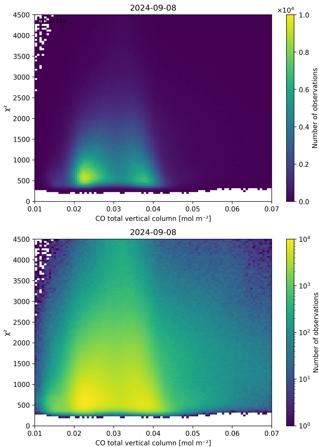
Figure 35: Scatter density plot of “CO total vertical column” against “ \chi^2 ” for 2024-09-07 to 2024-09-09.
