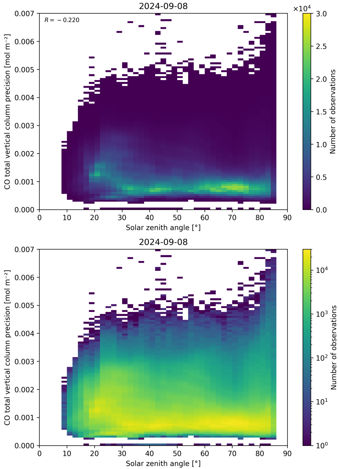
Figure 63: Scatter density plot of “Solar zenith angle” against “CO total vertical column precision” for 2024-09-07 to 2024-09-09.
