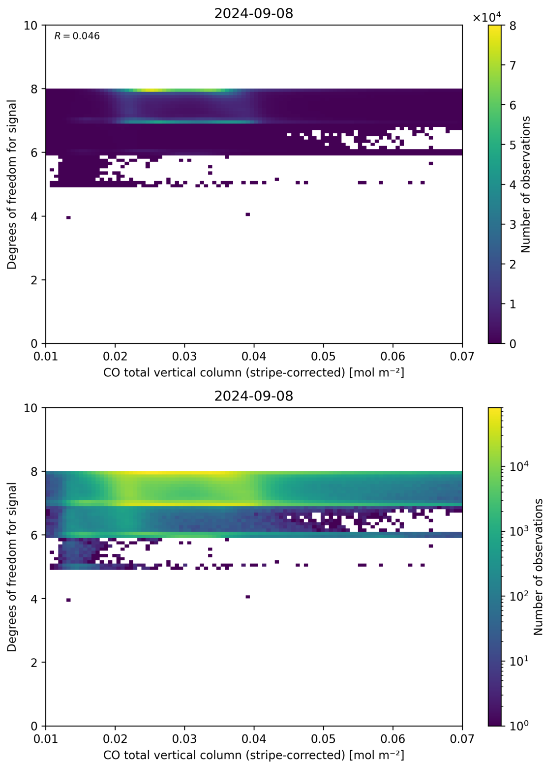
Figure 38: Scatter density plot of “CO total vertical column (stripe-corrected)” against “Degrees of freedom for signal” for 2024-09-07 to 2024-09-09.
