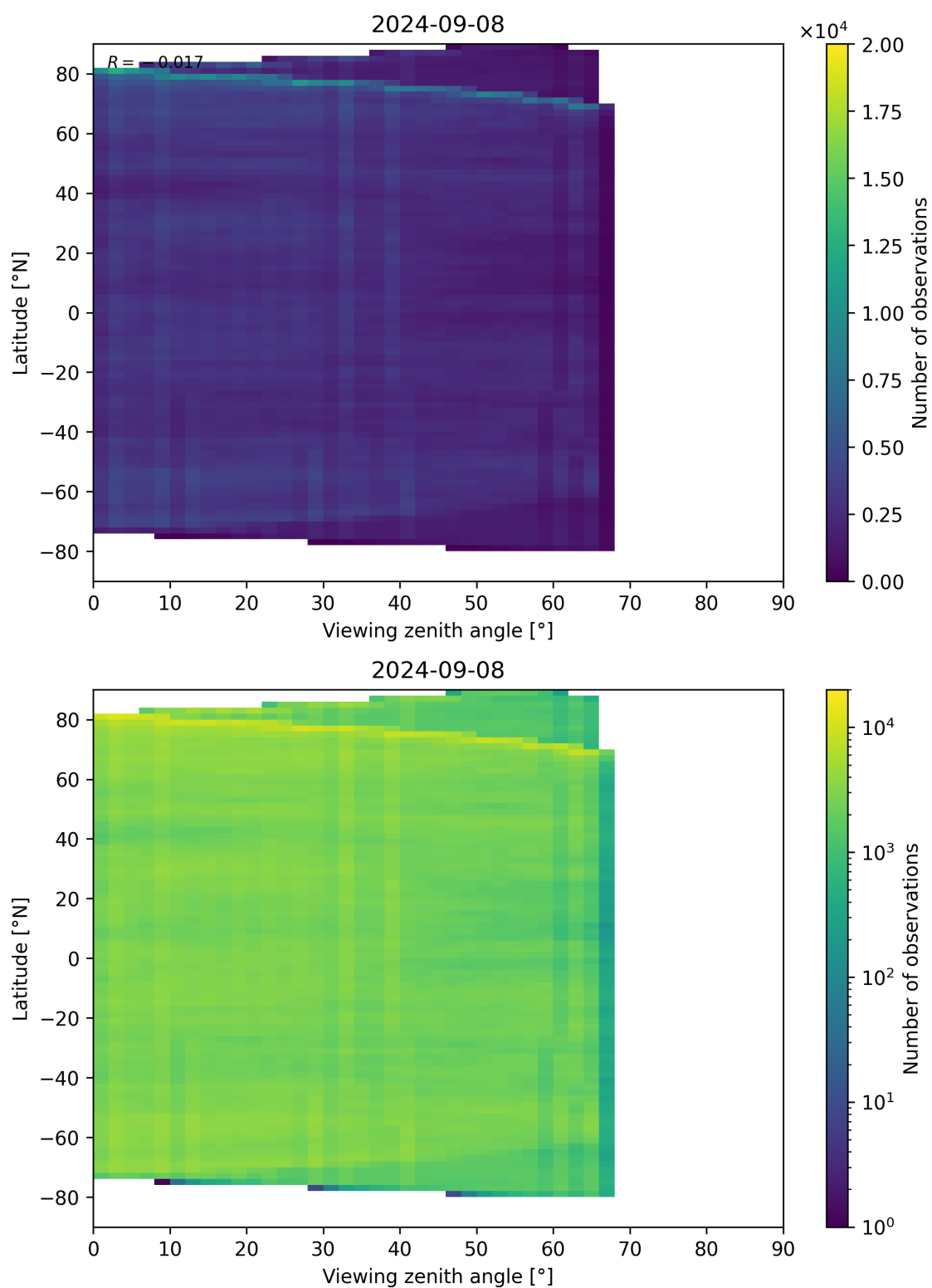
Figure 74: Scatter density plot of “Viewing zenith angle” against “Latitude” for 2024-09-07 to 2024-09-09.
