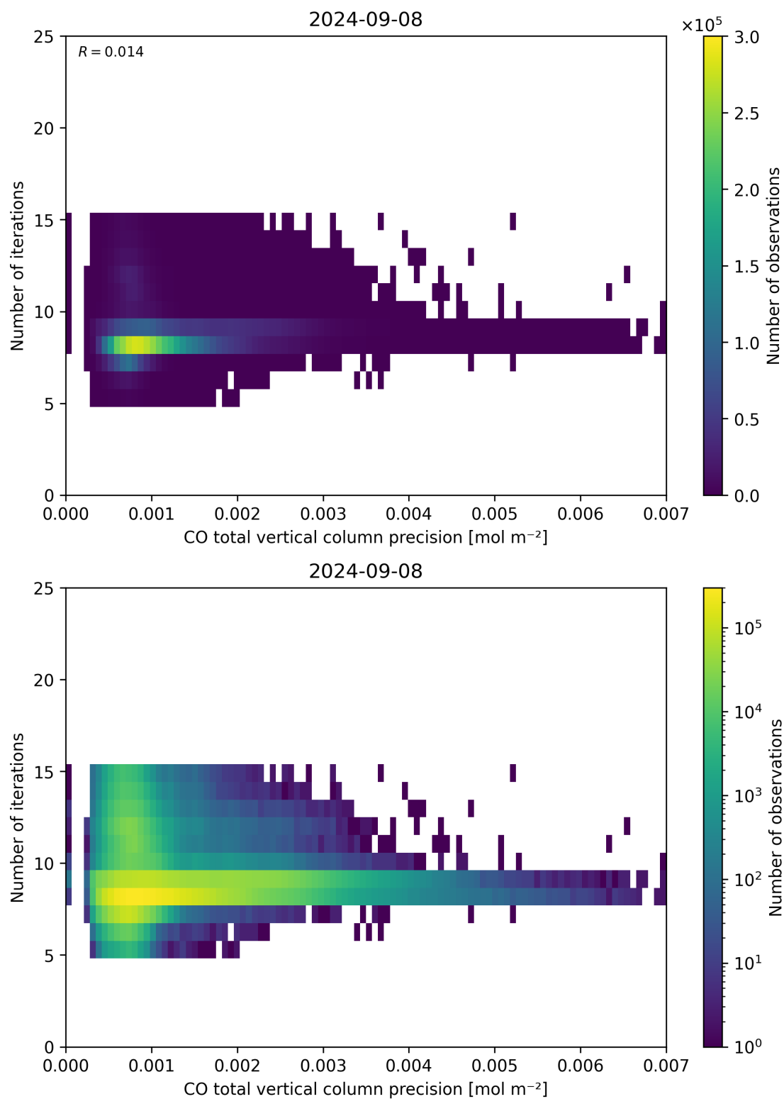
Figure 46: Scatter density plot of “CO total vertical column precision” against “Number of iterations” for 2024-09-07 to 2024-09-09.
