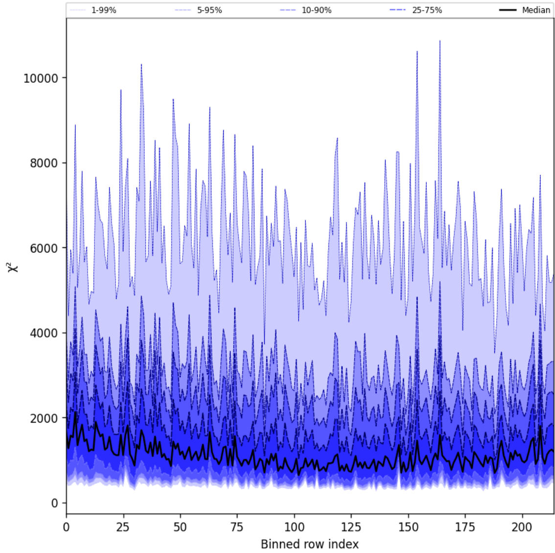
Figure 30: Along track statistics of “ \chi^2 ” for 2024-09-07 to 2024-09-09
