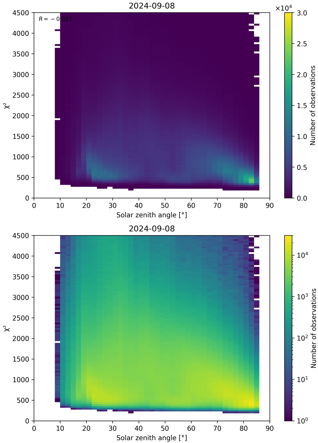
Figure 64: Scatter density plot of “Solar zenith angle” against “ \chi^2 ” for 2024-09-07 to 2024-09-09.
