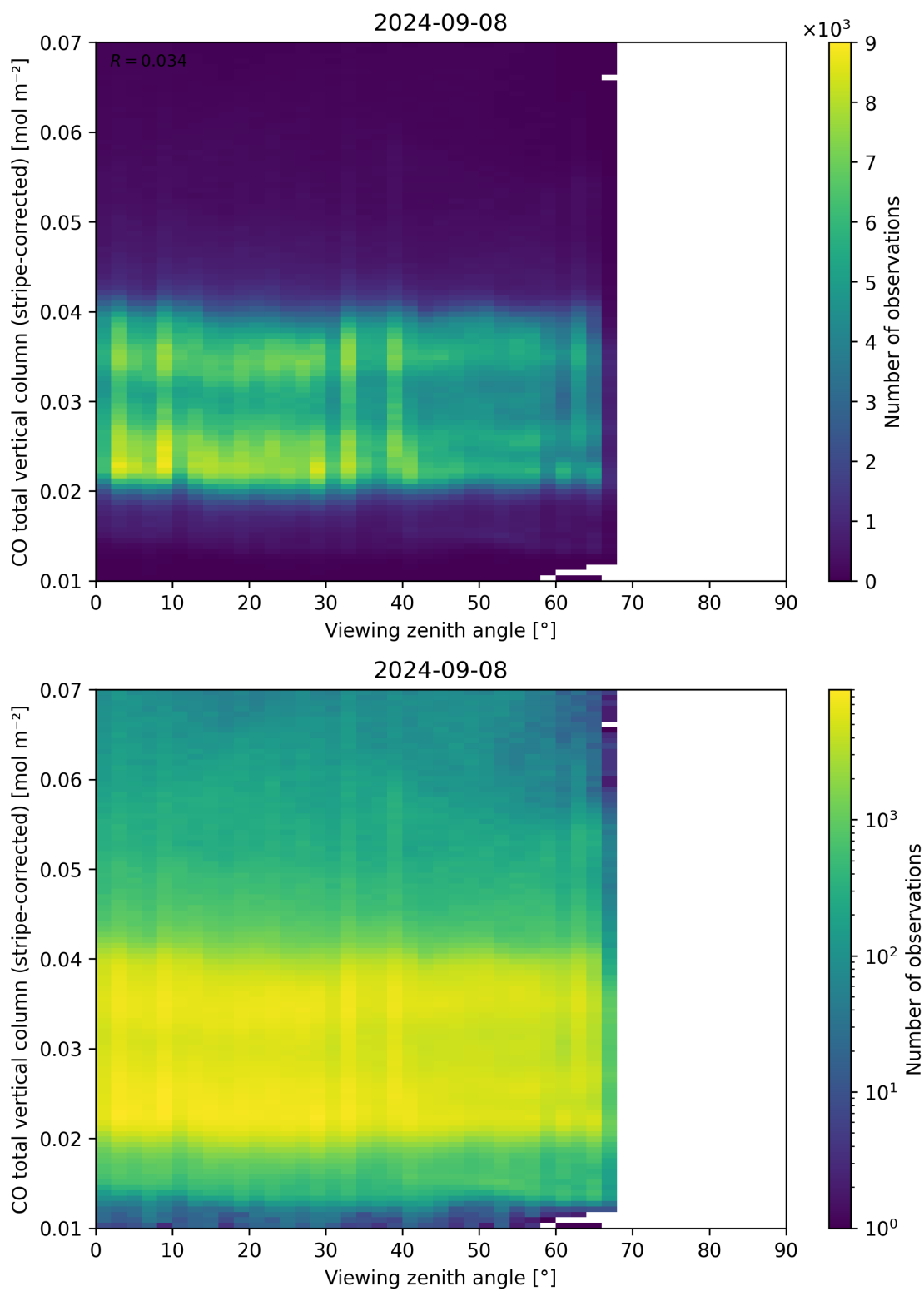
Figure 70: Scatter density plot of “Viewing zenith angle” against “CO total vertical column (stripe-corrected)” for 2024-09-07 to 2024-09-09.
