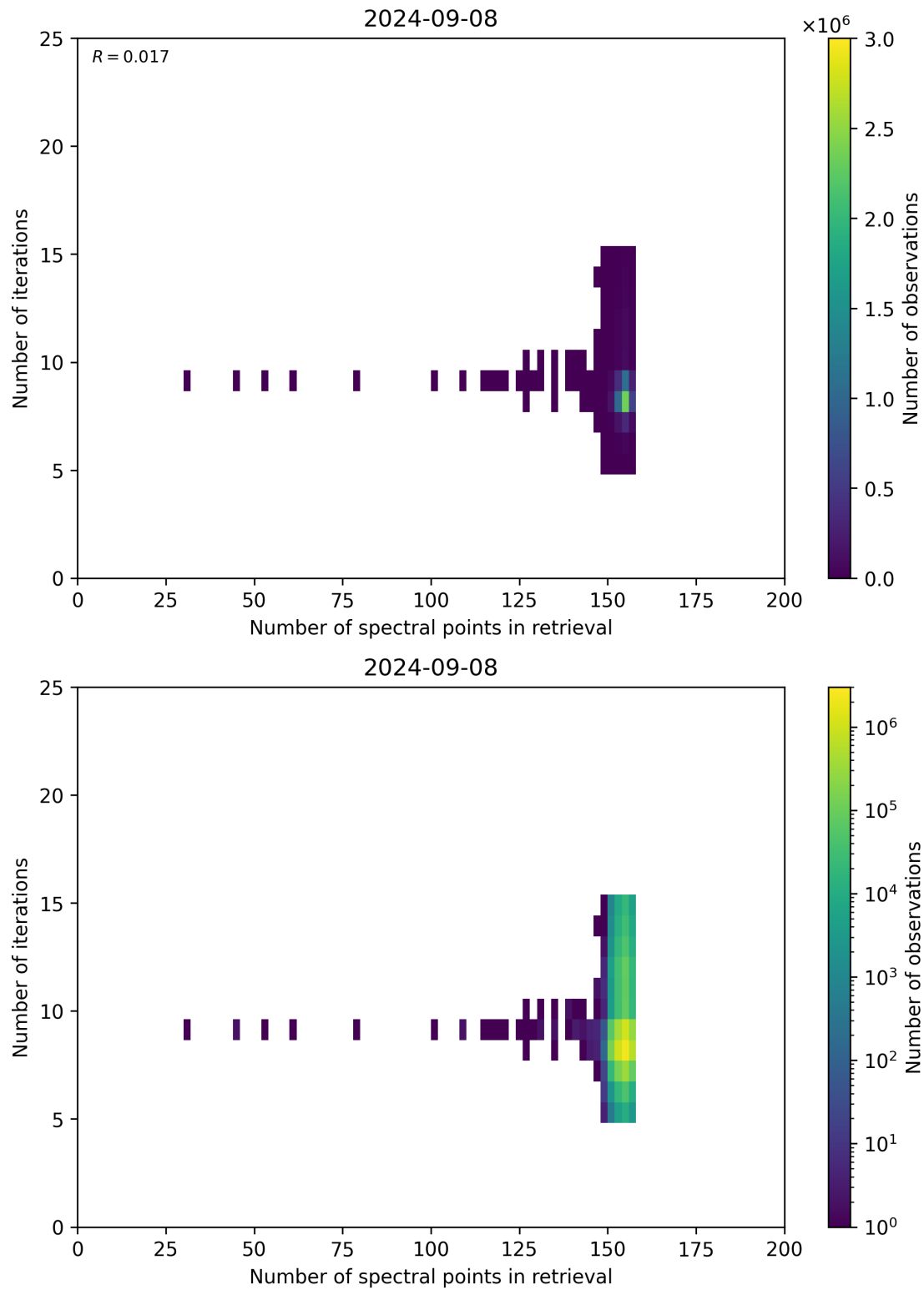
Figure 60: Scatter density plot of “Number of spectral points in retrieval” against “Number of iterations” for 2024-09-07 to 2024-09-09.
