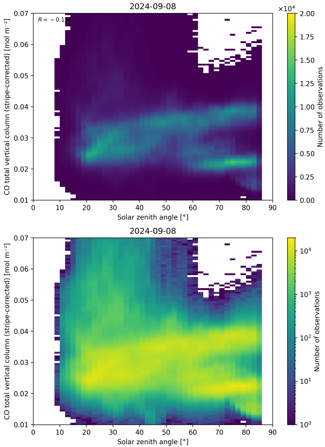
Figure 62: Scatter density plot of “Solar zenith angle” against “CO total vertical column (stripe-corrected)” for 2024-09-07 to 2024-09-09.
