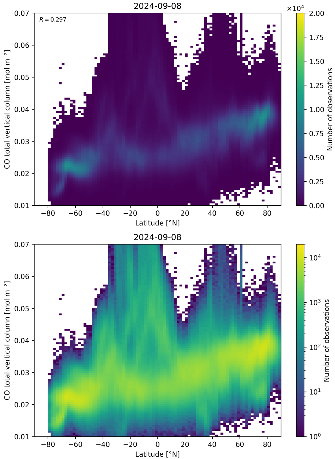
Figure 51: Scatter density plot of “Latitude” against “CO total vertical column” for 2024-09-07 to 2024-09-09.
