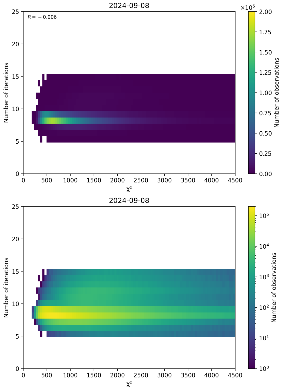
Figure 49: Scatter density plot of “ \chi^2 ” against “Number of iterations” for 2024-09-07 to 2024-09-09.
