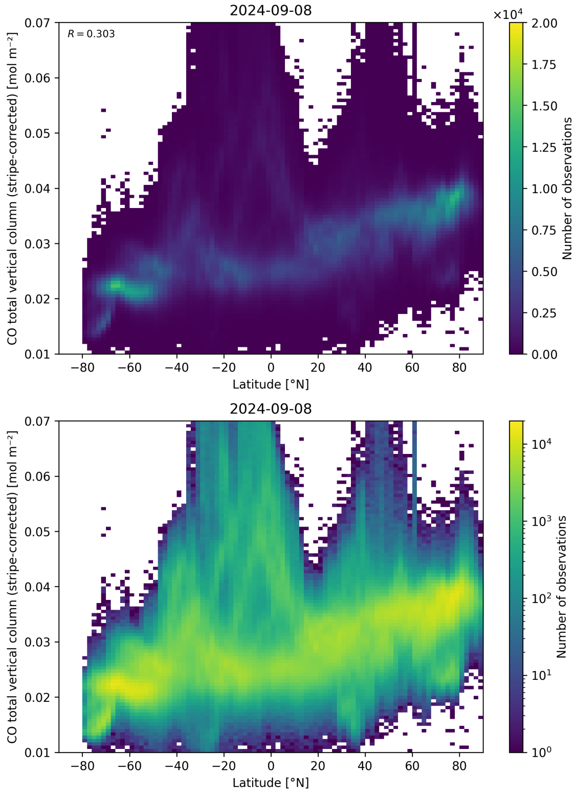
Figure 52: Scatter density plot of “Latitude” against “CO total vertical column (stripe-corrected)” for 2024-09-07 to 2024-09-09.
