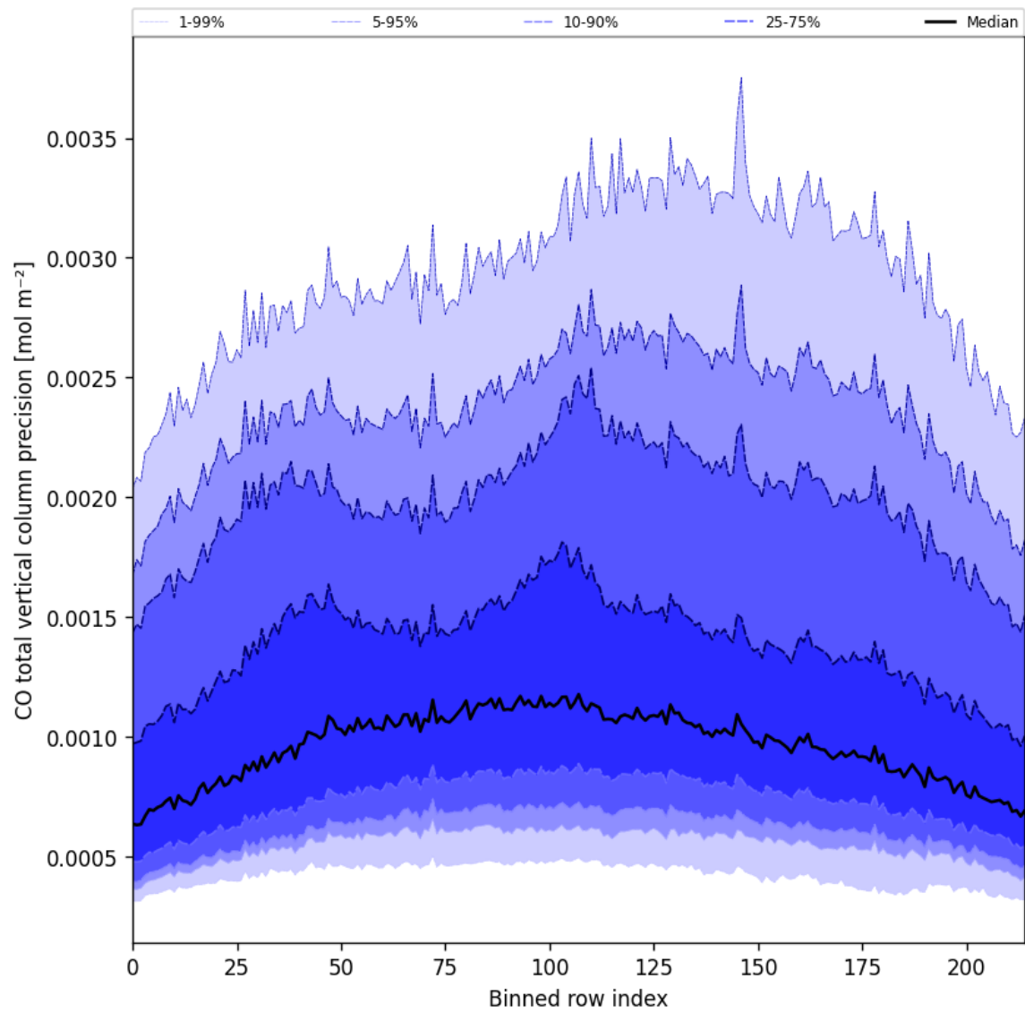
Figure 28: Along track statistics of “CO total vertical column precision” for 2024-09-07 to 2024-09-09
