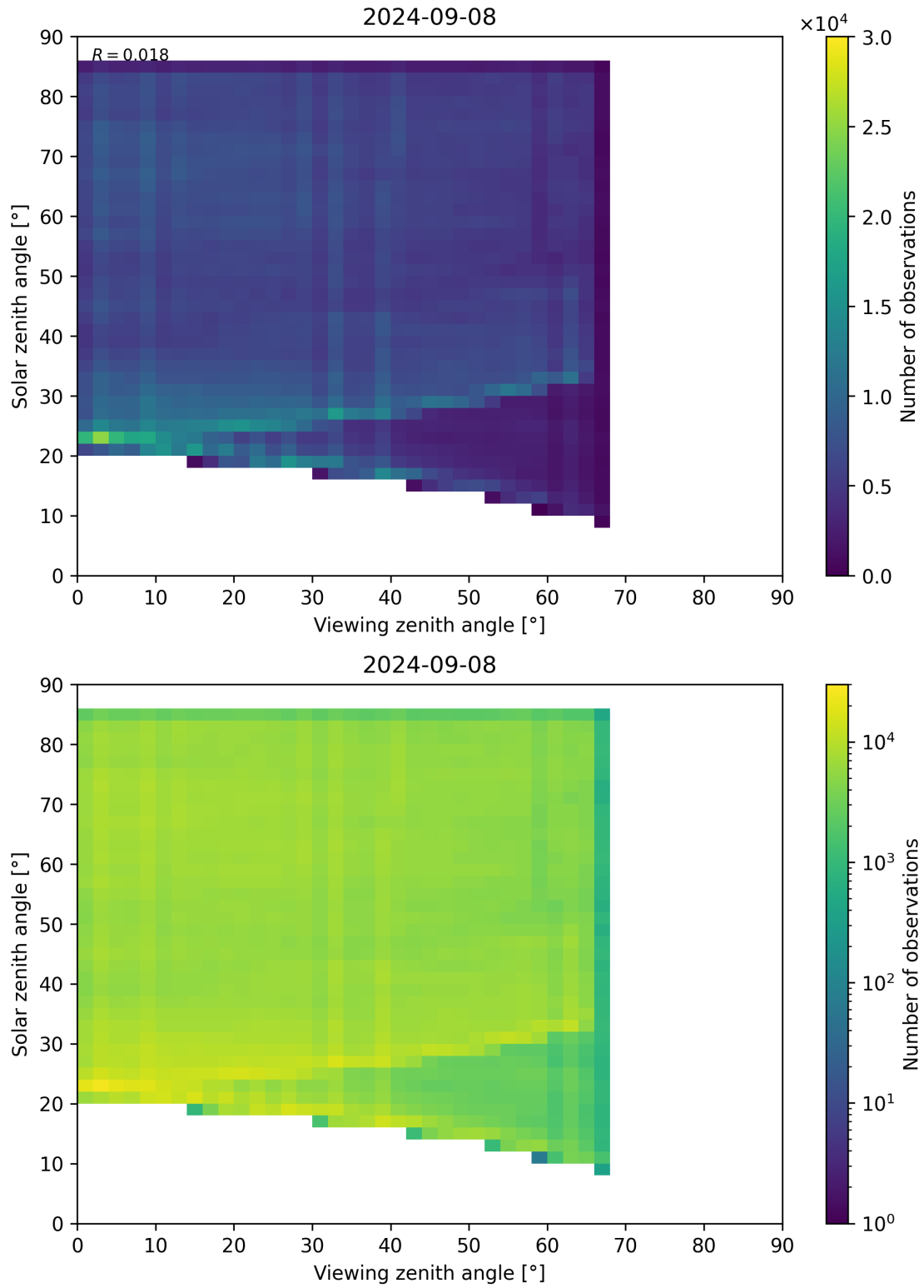
Figure 77: Scatter density plot of “Viewing zenith angle” against “Solar zenith angle” for 2024-09-07 to 2024-09-09.
