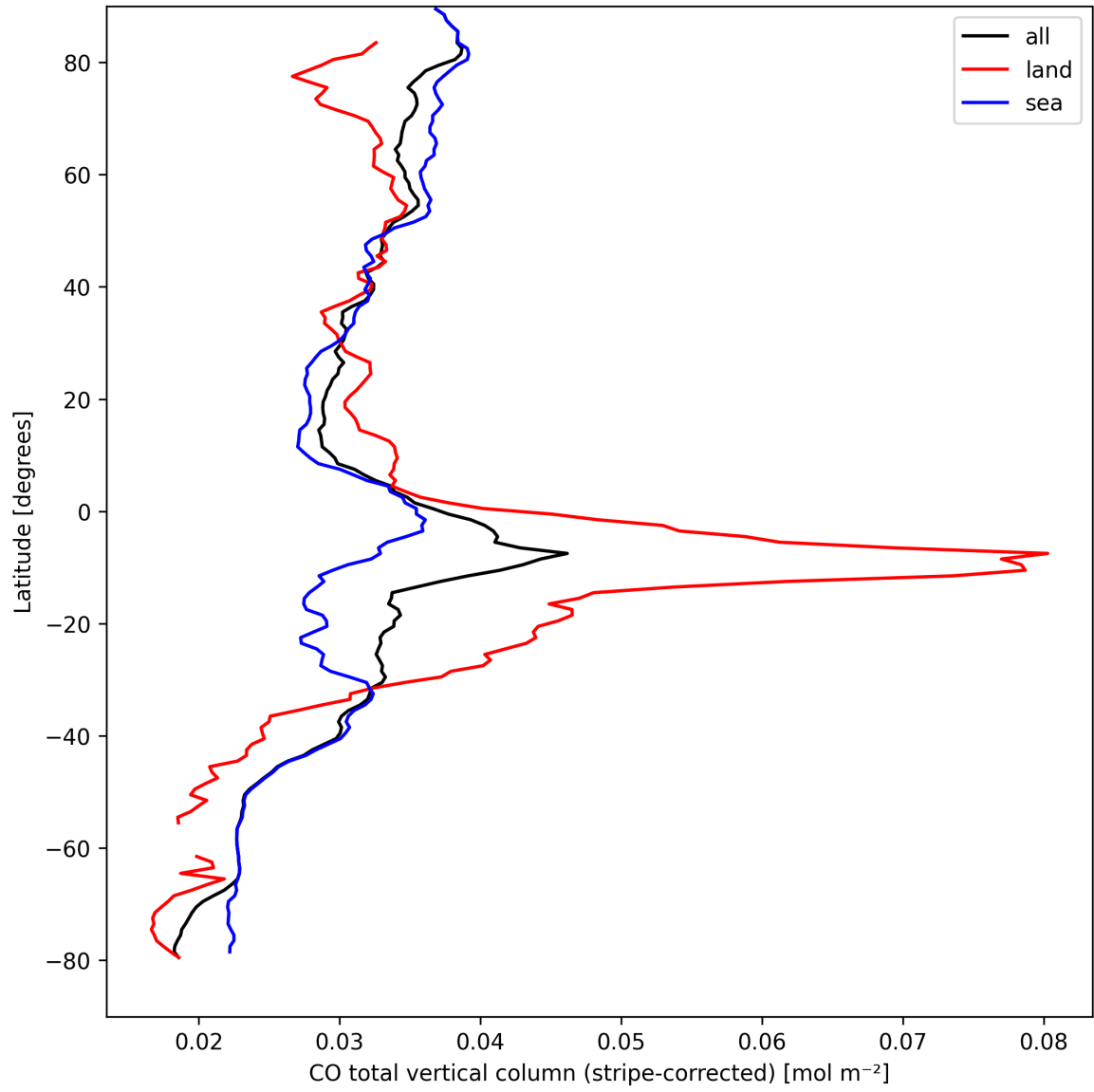
Figure 11: Zonal average of “CO total vertical column (stripe-corrected)” for 2024-09-07 to 2024-09-09.
