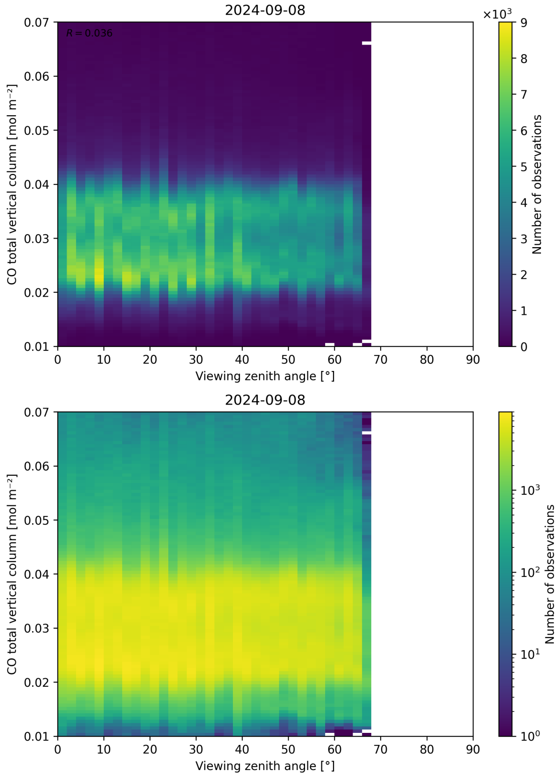
Figure 69: Scatter density plot of “Viewing zenith angle” against “CO total vertical column” for 2024-09-07 to 2024-09-09.
