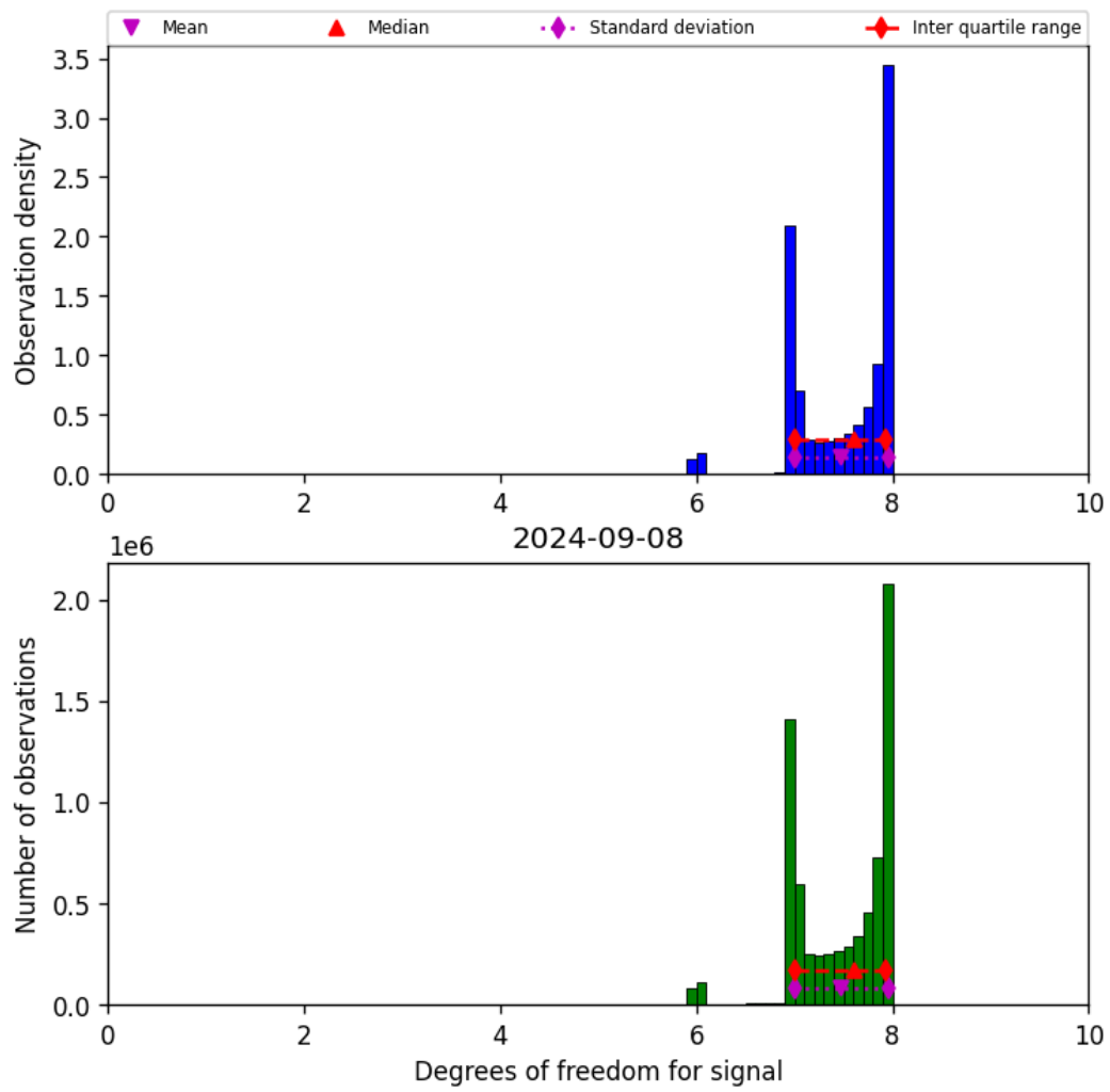
Figure 23: Histogram of “Degrees of freedom for signal” for 2024-09-07 to 2024-09-09
