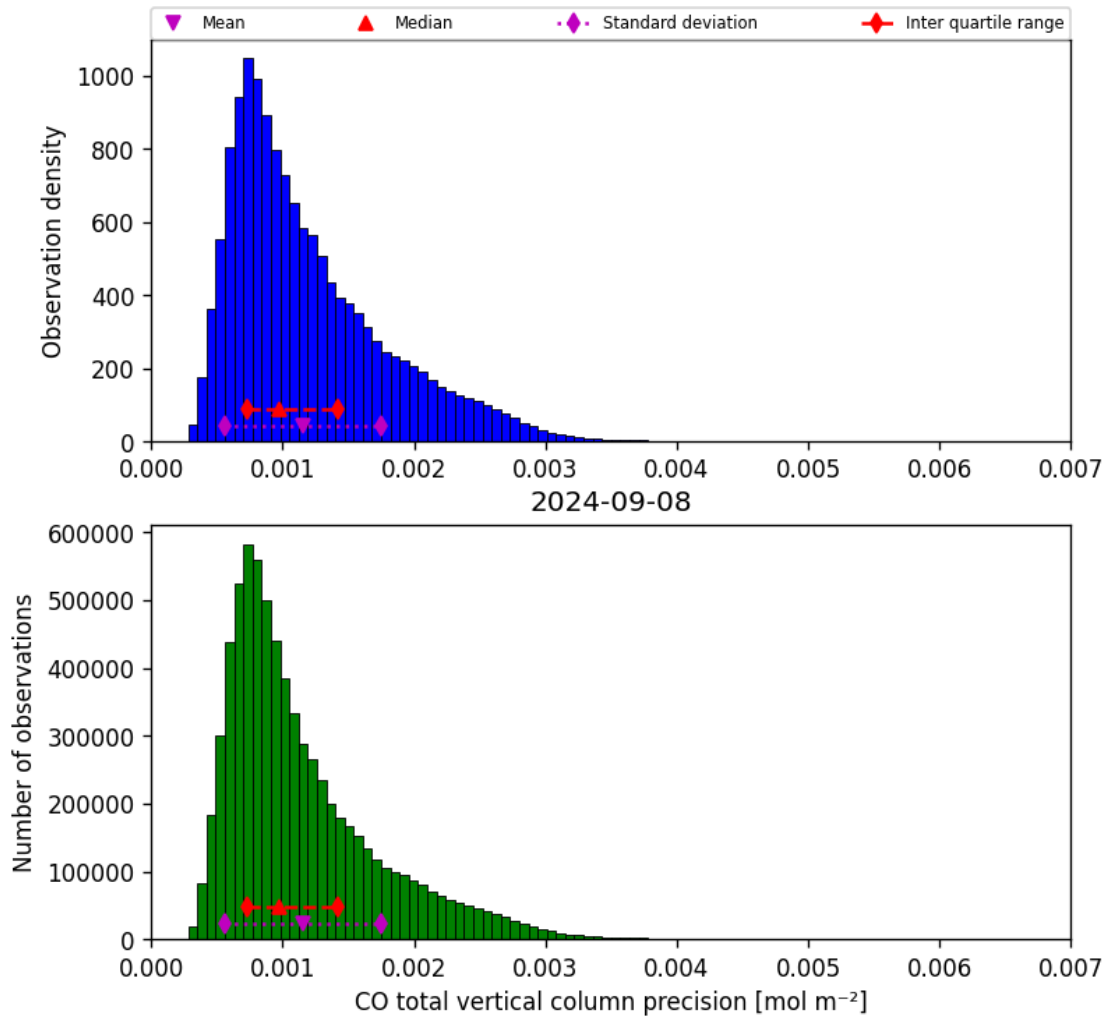
Figure 20: Histogram of “CO total vertical column precision” for 2024-09-07 to 2024-09-09
