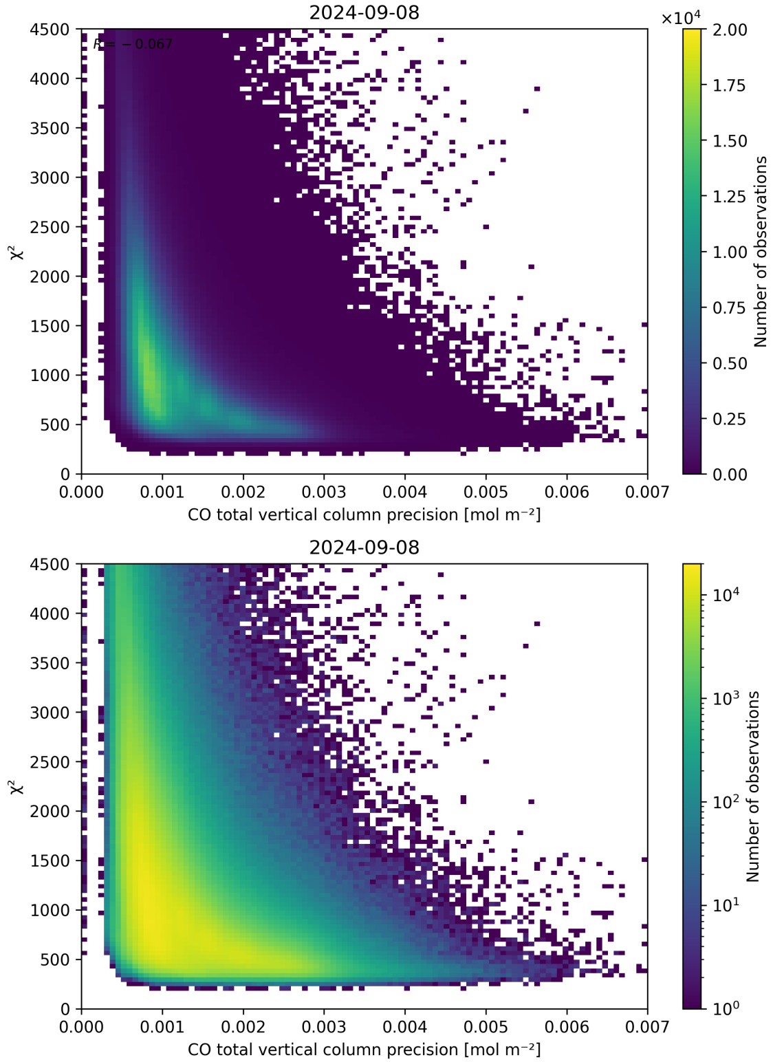
Figure 44: Scatter density plot of “CO total vertical column precision” against “ \chi^2 ” for 2024-09-07 to 2024-09-09.
