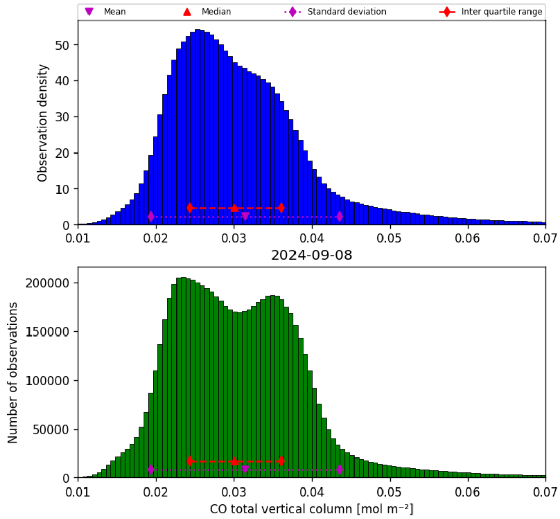
Figure 18: Histogram of “CO total vertical column” for 2024-09-07 to 2024-09-09
