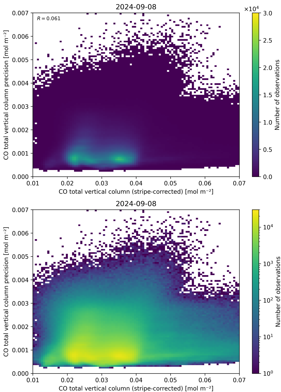
Figure 36: Scatter density plot of “CO total vertical column (stripe-corrected)” against “CO total vertical column precision” for 2024-09-07 to 2024-09-09.
