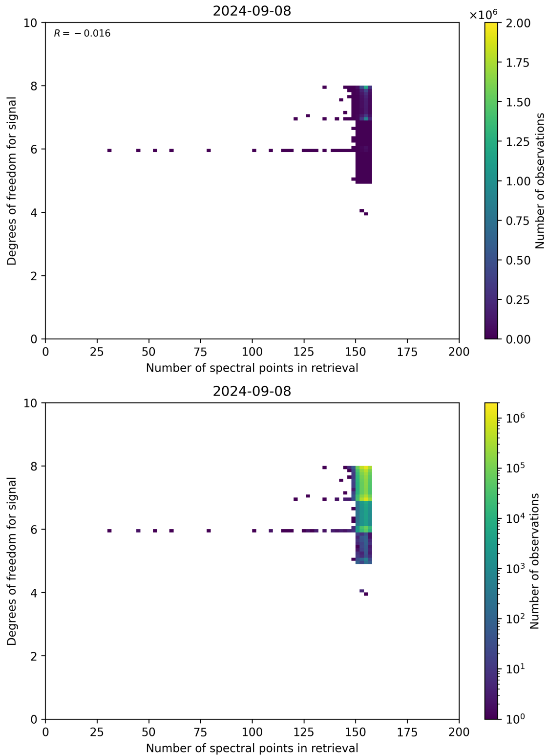
Figure 59: Scatter density plot of “Number of spectral points in retrieval” against “Degrees of freedom for signal” for 2024-09-07 to 2024-09-09.
