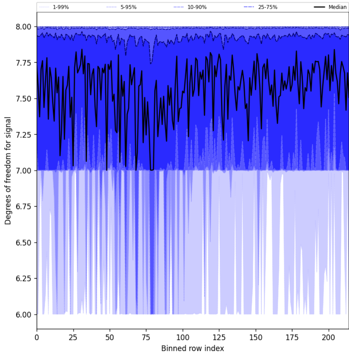
Figure 31: Along track statistics of “Degrees of freedom for signal” for 2024-09-07 to 2024-09-09
