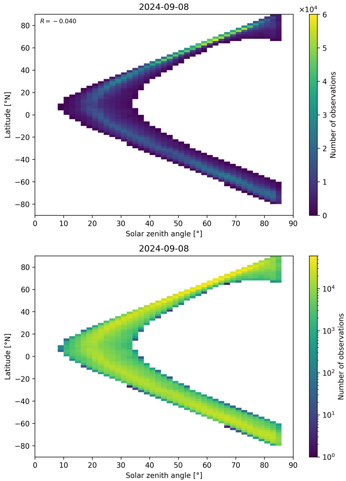
Figure 66: Scatter density plot of “Solar zenith angle” against “Latitude” for 2024-09-07 to 2024-09-09.
