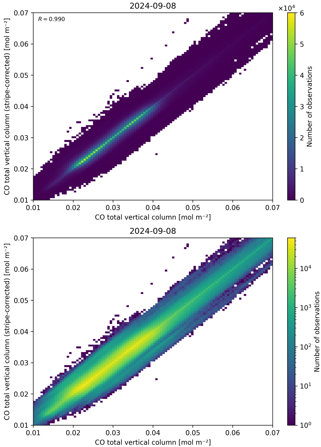
Figure 33: Scatter density plot of “CO total vertical column” against “CO total vertical column (stripe-corrected)” for 2024-09-07 to 2024-09-09.
