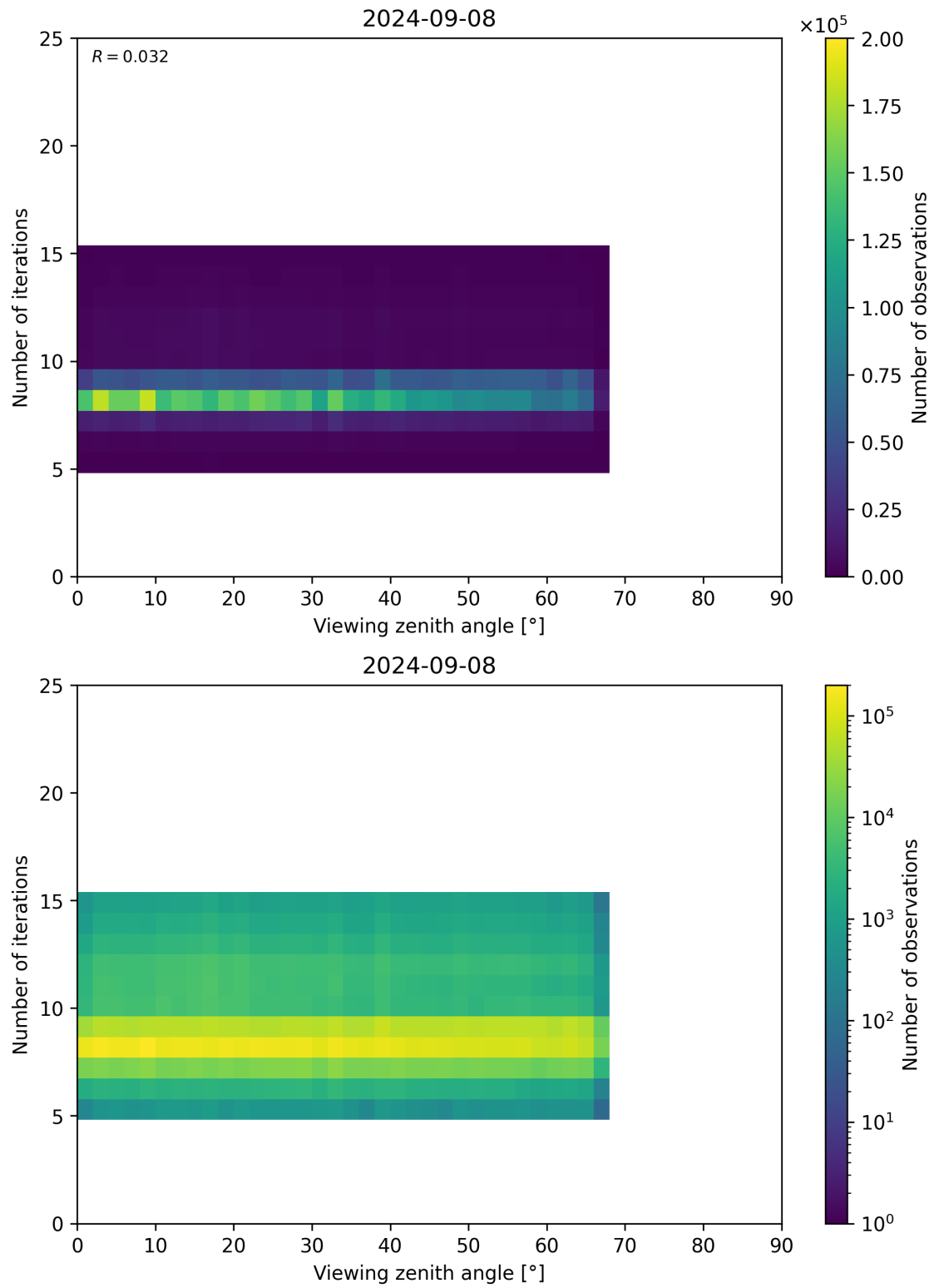
Figure 75: Scatter density plot of “Viewing zenith angle” against “Number of iterations” for 2024-09-07 to 2024-09-09.
