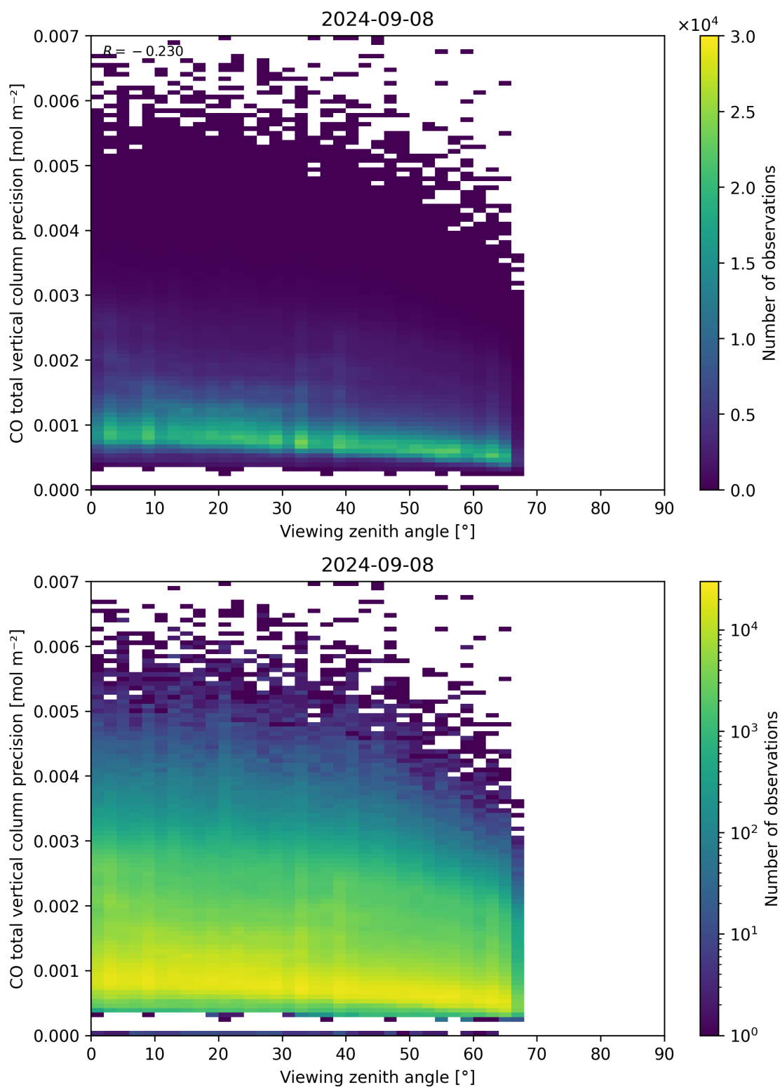
Figure 71: Scatter density plot of “Viewing zenith angle” against “CO total vertical column precision” for 2024-09-07 to 2024-09-09.
