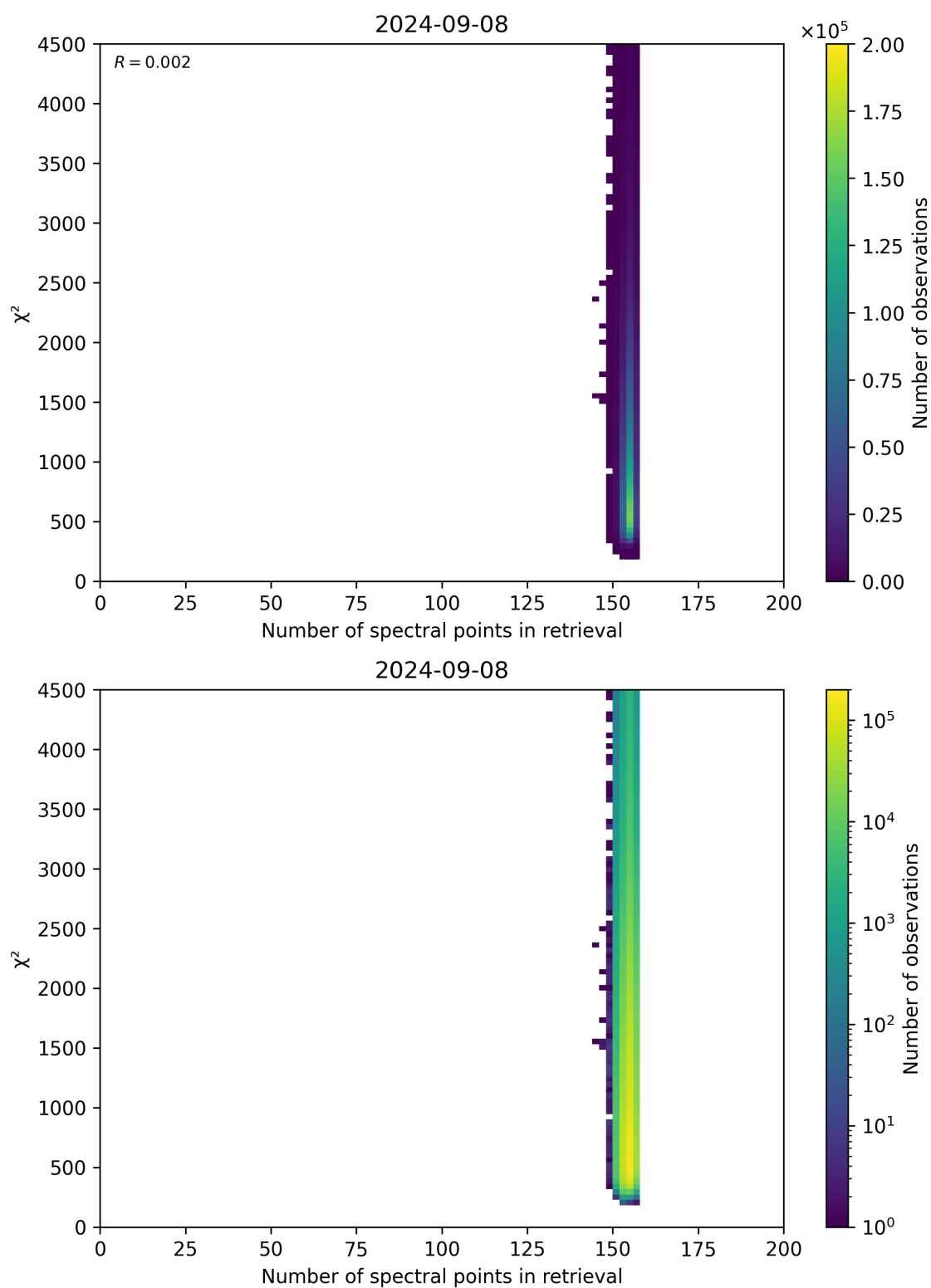
Figure 58: Scatter density plot of “Number of spectral points in retrieval” against “ \chi^2 ” for 2024-09-07 to 2024-09-09.
