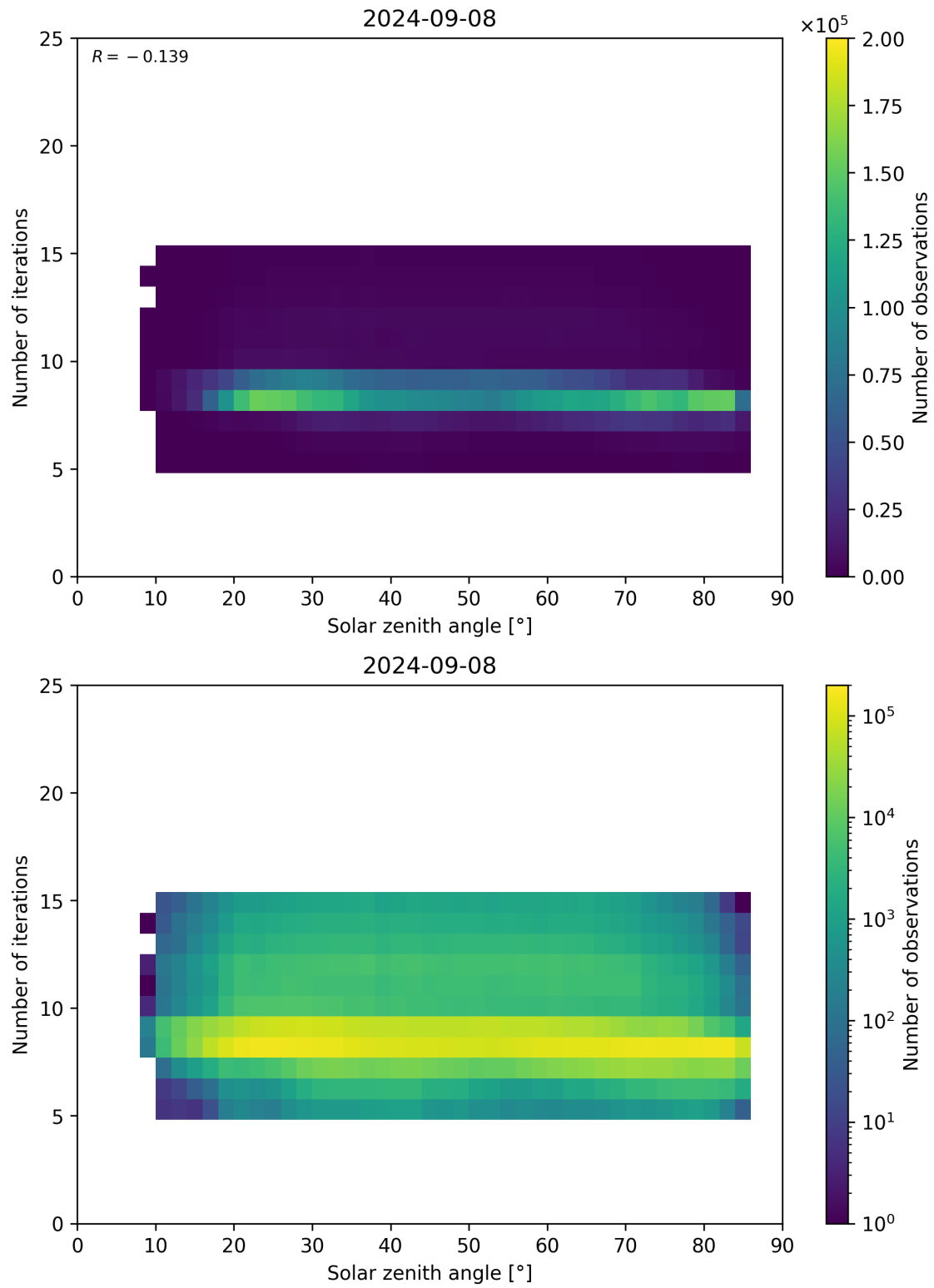
Figure 67: Scatter density plot of “Solar zenith angle” against “Number of iterations” for 2024-09-07 to 2024-09-09.
