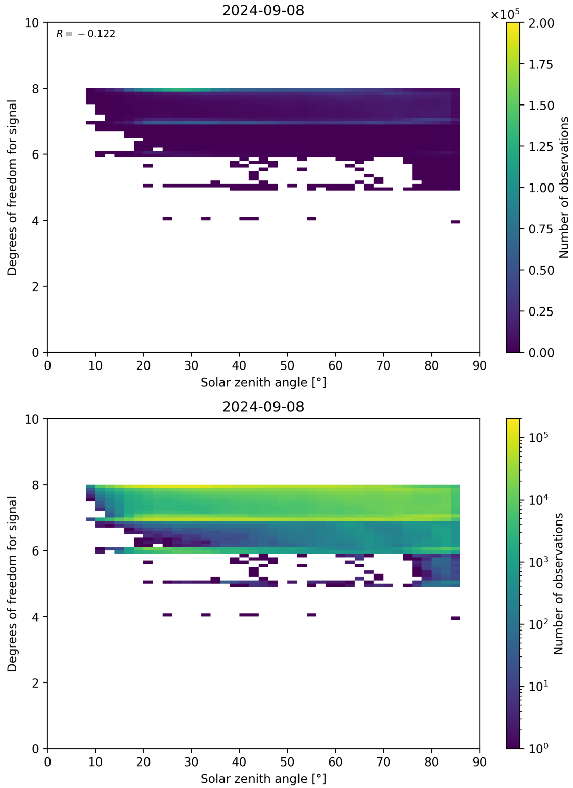
Figure 65: Scatter density plot of “Solar zenith angle” against “Degrees of freedom for signal” for 2024-09-07 to 2024-09-09.
