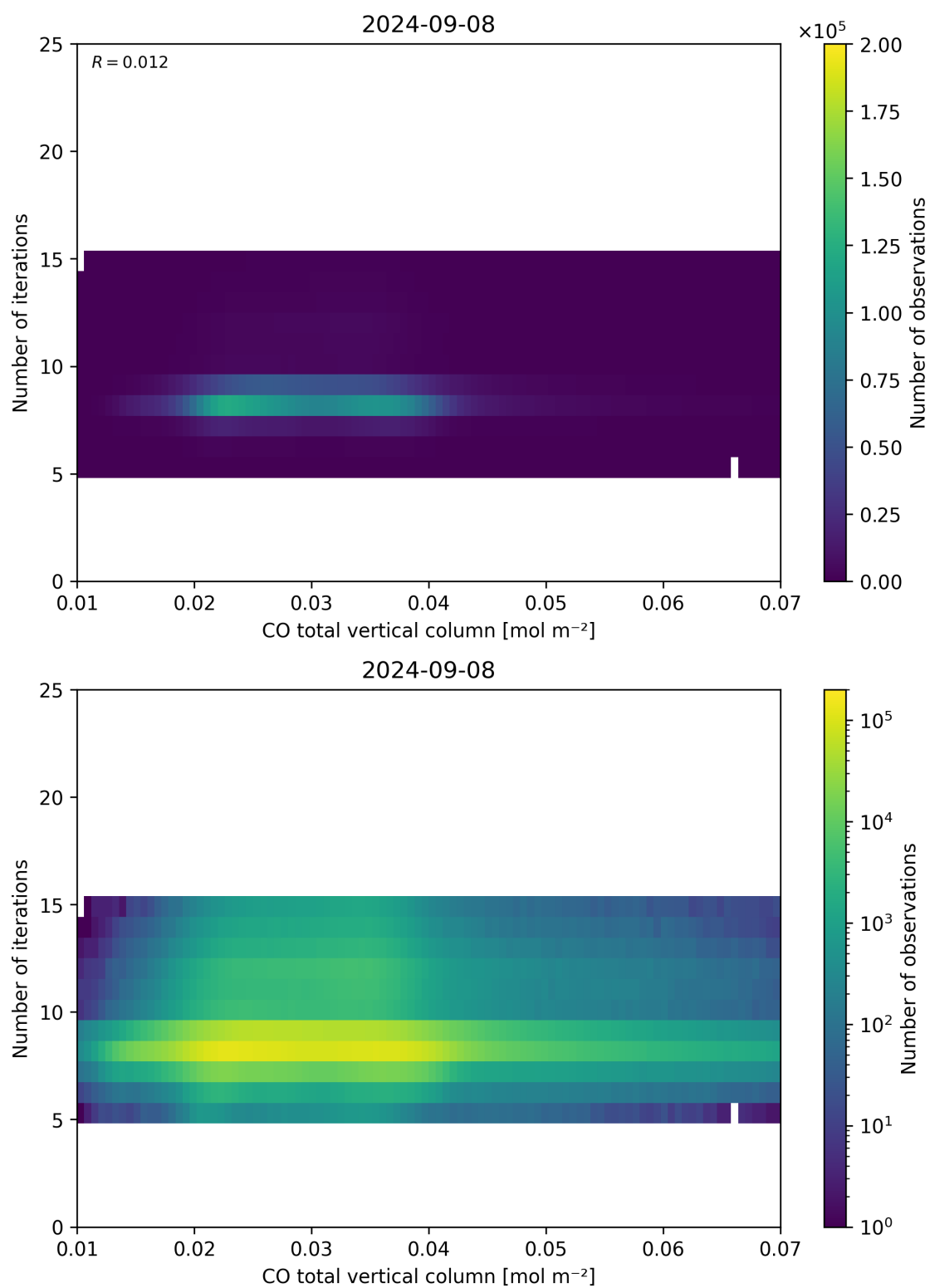
Figure 42: Scatter density plot of “CO total vertical column” against “Number of iterations” for 2024-09-07 to 2024-09-09.
