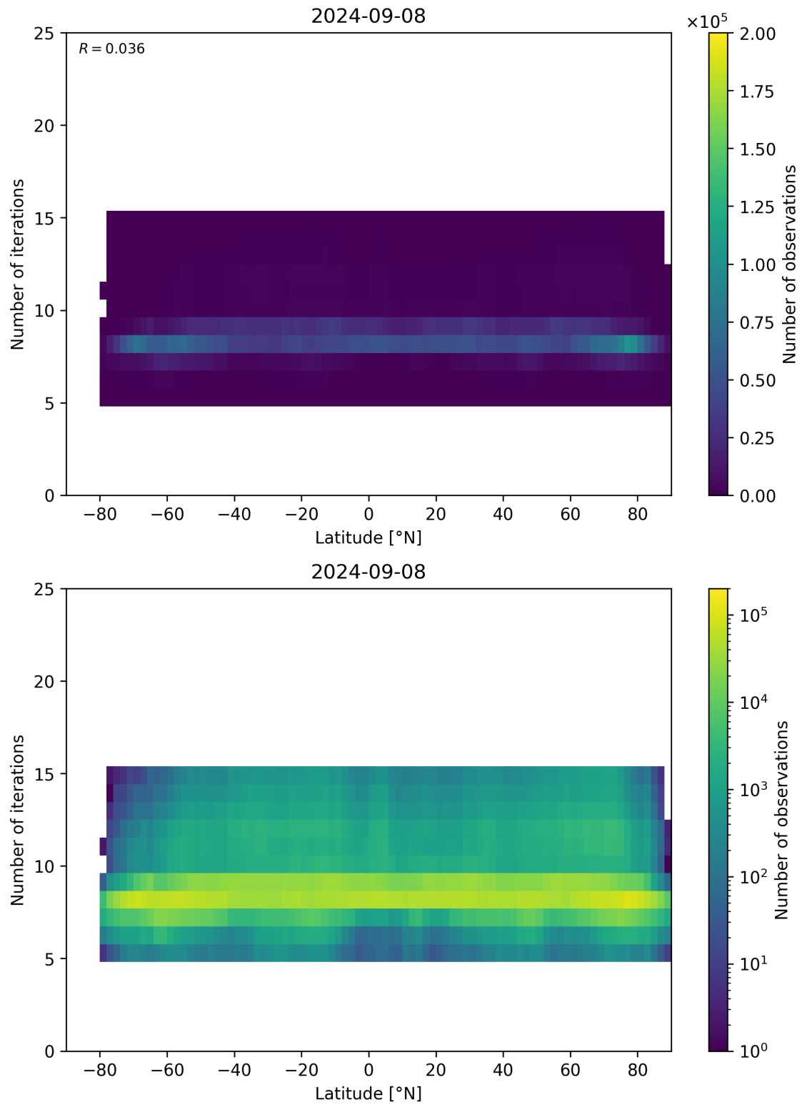
Figure 56: Scatter density plot of “Latitude” against “Number of iterations” for 2024-09-07 to 2024-09-09.
