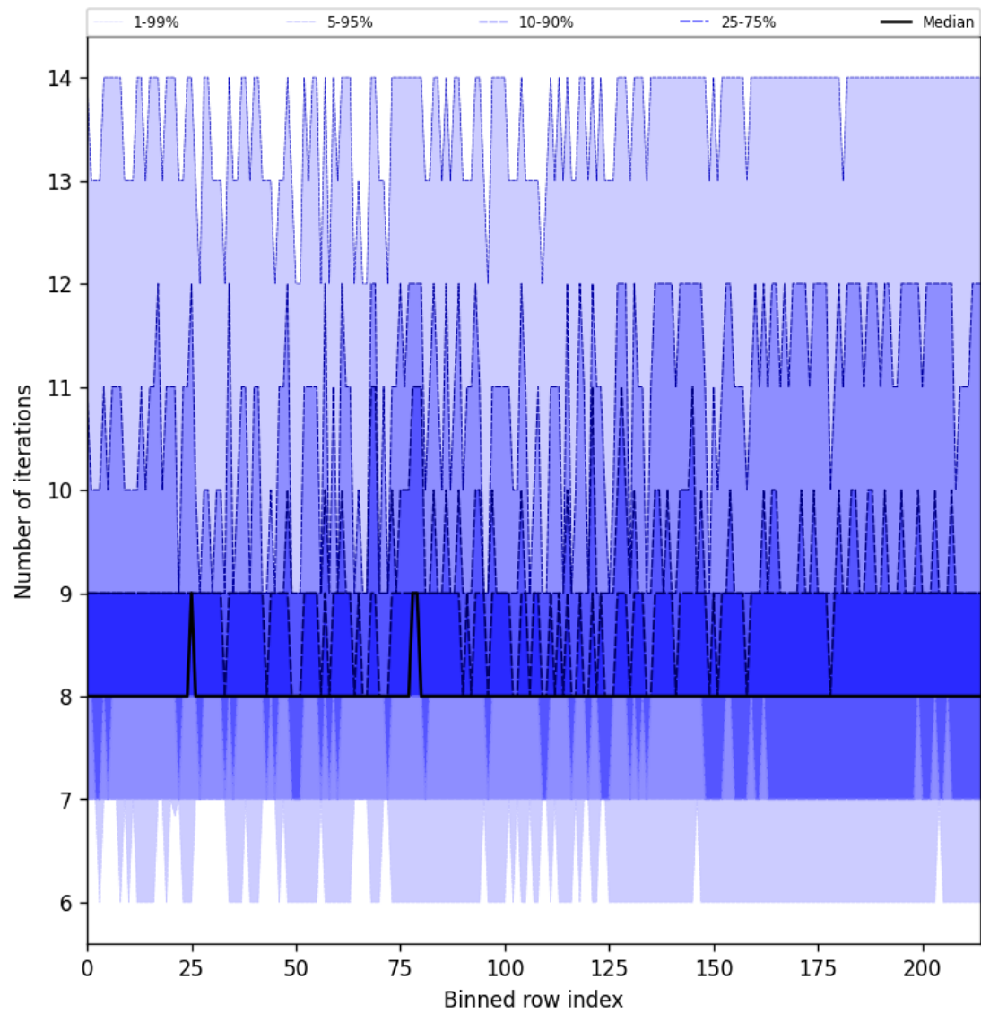
Figure 32: Along track statistics of “Number of iterations” for 2024-09-07 to 2024-09-09
