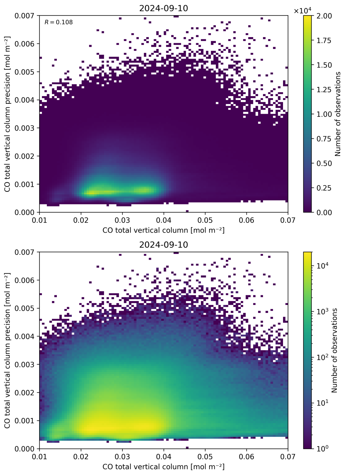
Figure 34: Scatter density plot of “CO total vertical column” against “CO total vertical column precision” for 2024-09-09 to 2024-09-11.
