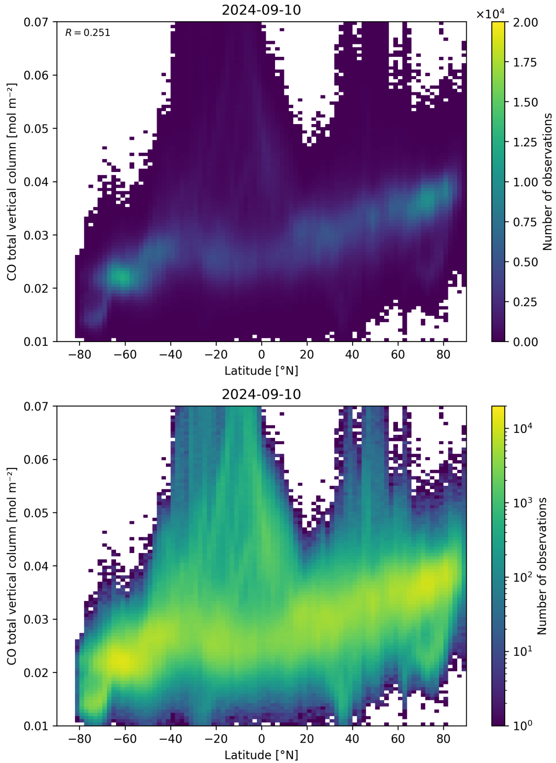
Figure 51: Scatter density plot of “Latitude” against “CO total vertical column” for 2024-09-09 to 2024-09-11.
