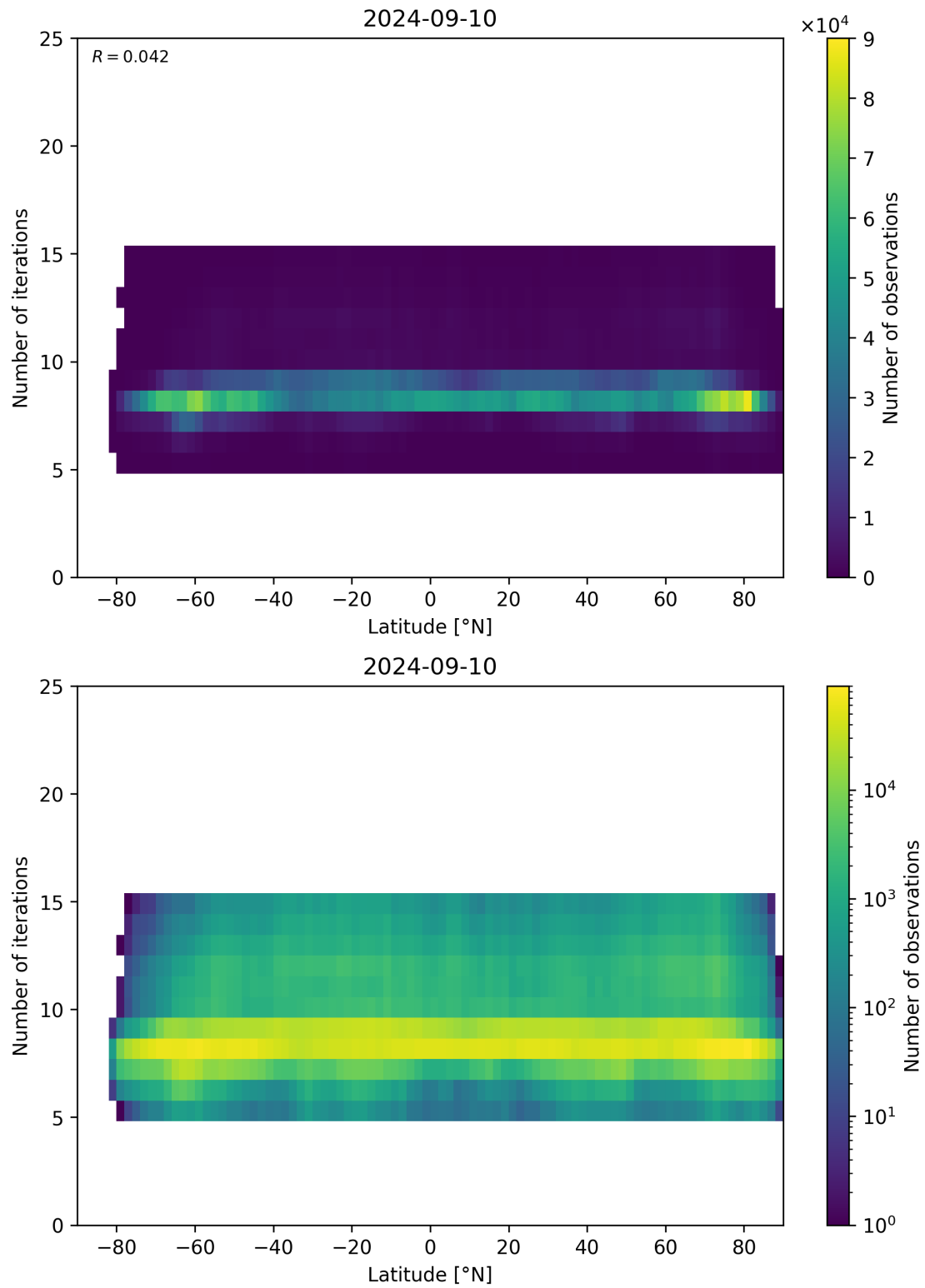
Figure 56: Scatter density plot of “Latitude” against “Number of iterations” for 2024-09-09 to 2024-09-11.
