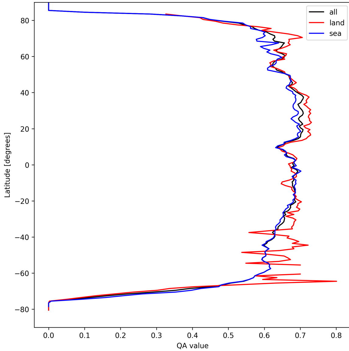
Figure 9: Zonal average of “QA value” for 2024-09-09 to 2024-09-11.
