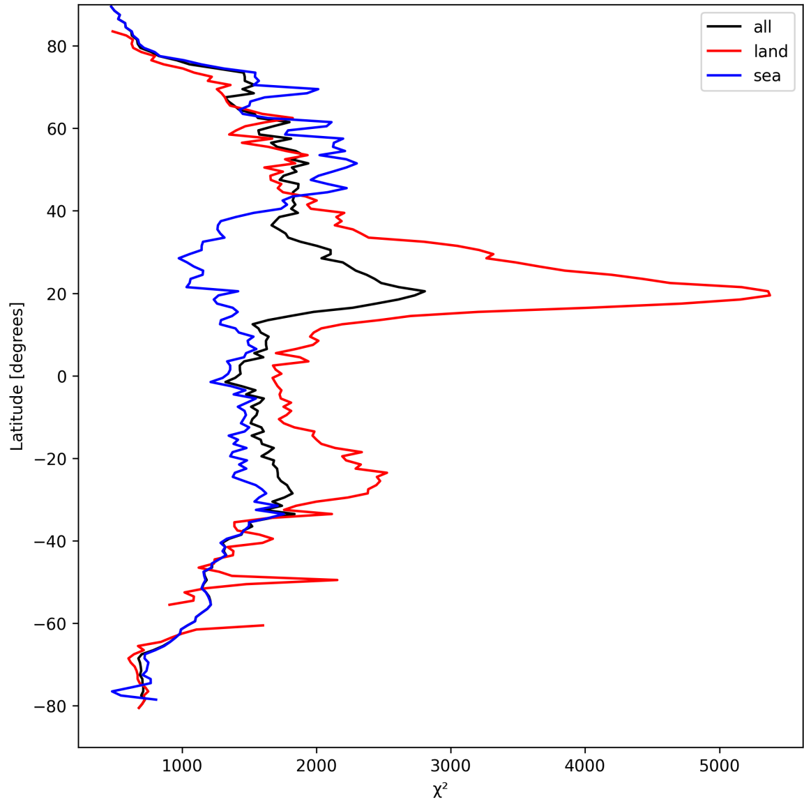
Figure 14: Zonal average of “ \chi^2 ” for 2024-09-09 to 2024-09-11.
