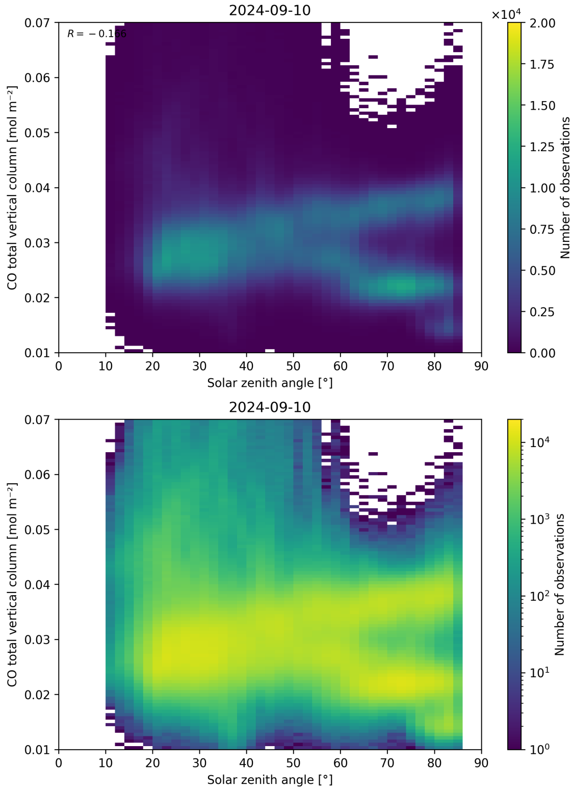
Figure 61: Scatter density plot of “Solar zenith angle” against “CO total vertical column” for 2024-09-09 to 2024-09-11.
