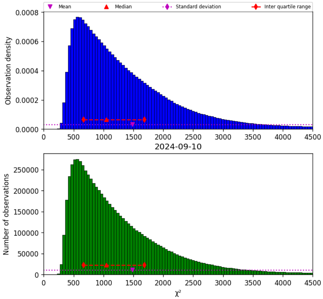
Figure 22: Histogram of “ \chi^2 ” for 2024-09-09 to 2024-09-11
