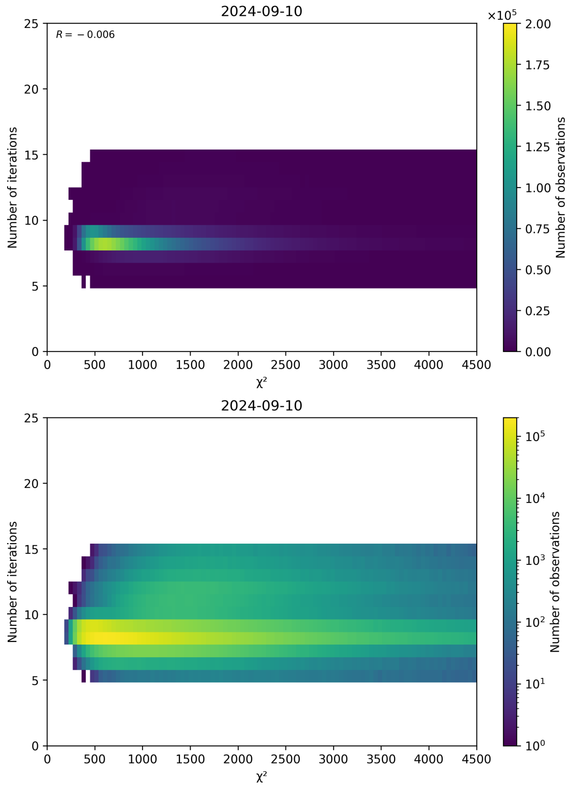
Figure 49: Scatter density plot of “ \chi^2 ” against “Number of iterations” for 2024-09-09 to 2024-09-11.
