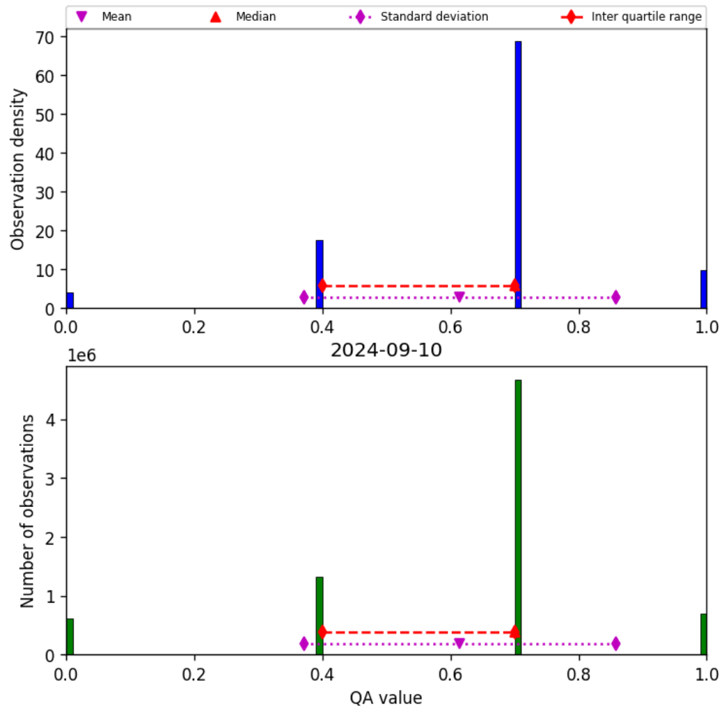
Figure 17: Histogram of “QA value” for 2024-09-09 to 2024-09-11
