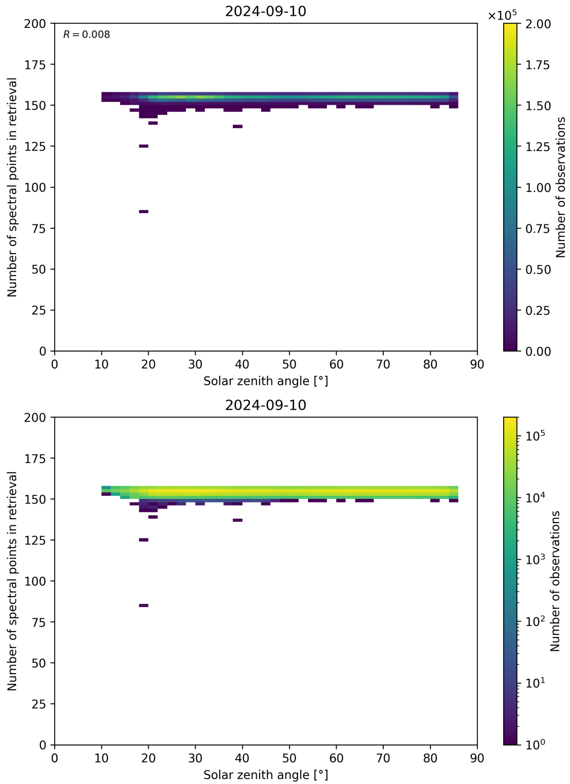
Figure 68: Scatter density plot of “Solar zenith angle” against “Number of spectral points in retrieval” for 2024-09-09 to 2024-09-11.
