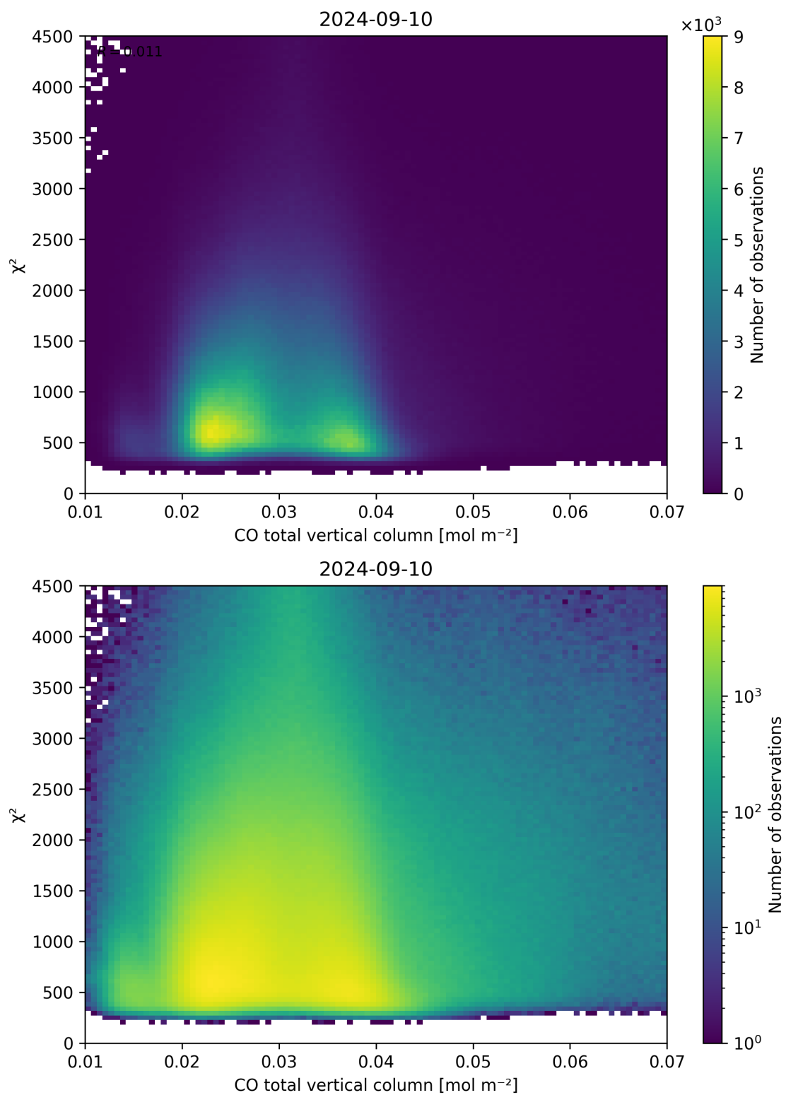
Figure 35: Scatter density plot of “CO total vertical column” against “ \chi^2 ” for 2024-09-09 to 2024-09-11.
