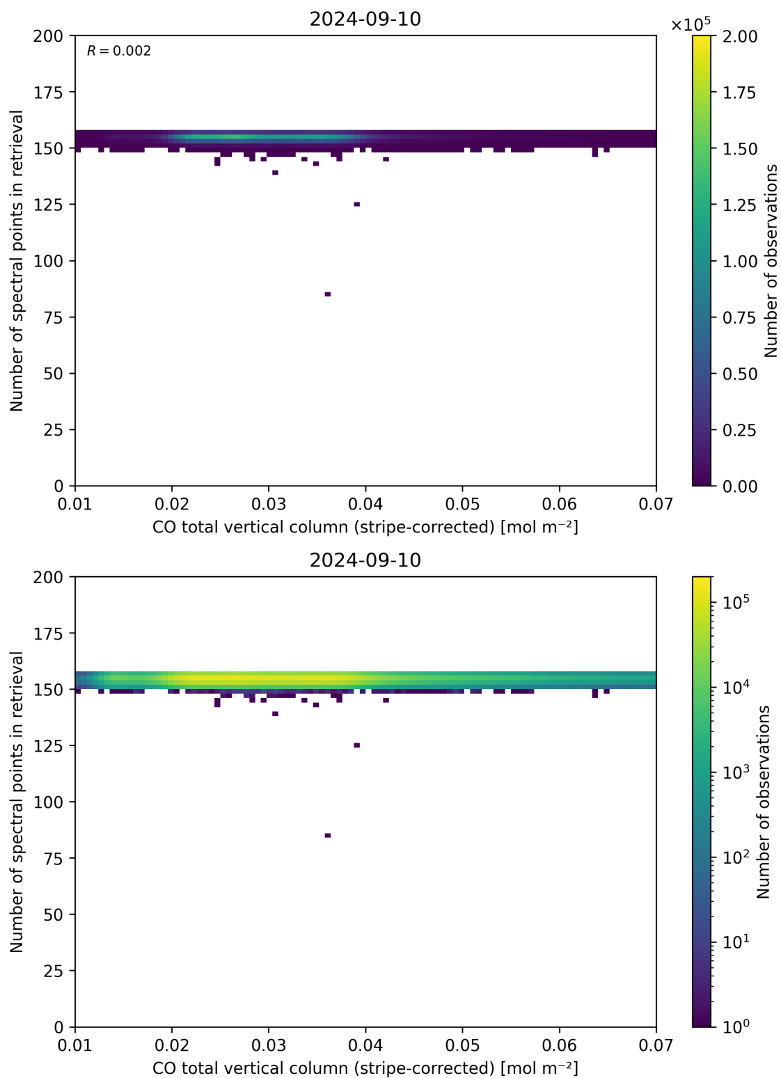
Figure 40: Scatter density plot of “CO total vertical column (stripe-corrected)” against “Number of spectral points in retrieval” for 2024-09-09 to 2024-09-11.
