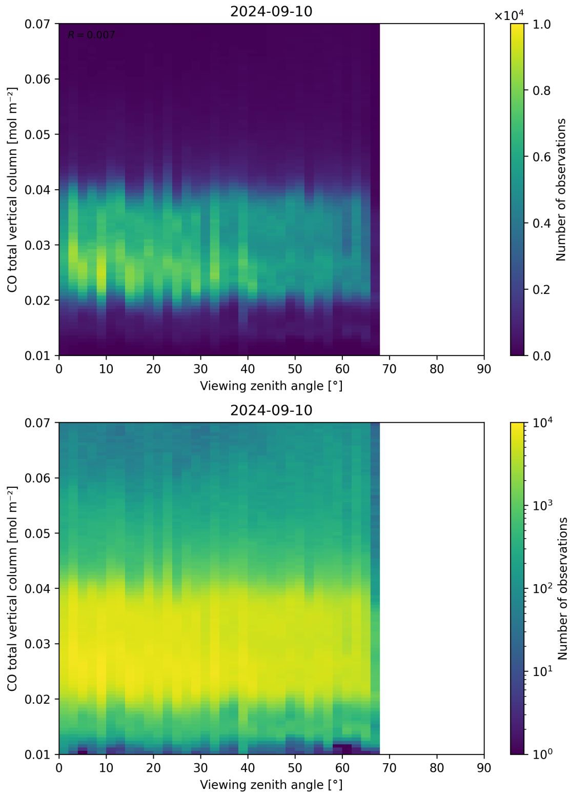
Figure 69: Scatter density plot of “Viewing zenith angle” against “CO total vertical column” for 2024-09-09 to 2024-09-11.
