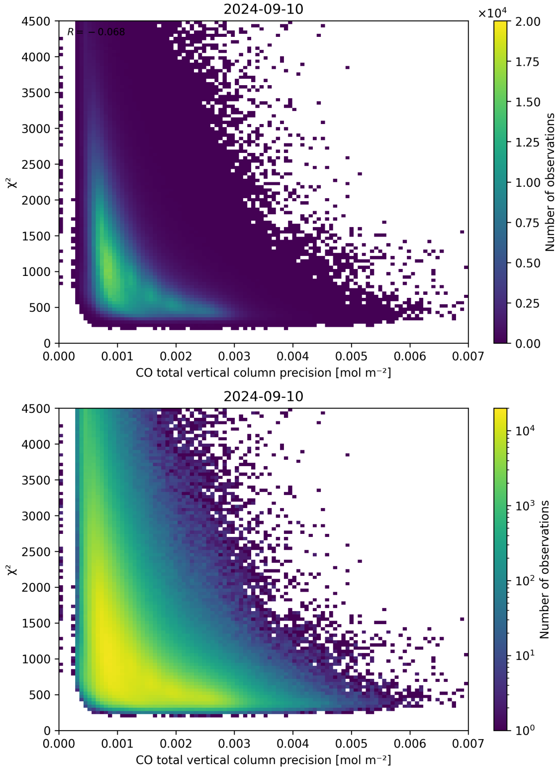
Figure 44: Scatter density plot of “CO total vertical column precision” against “ \chi^2 ” for 2024-09-09 to 2024-09-11.
