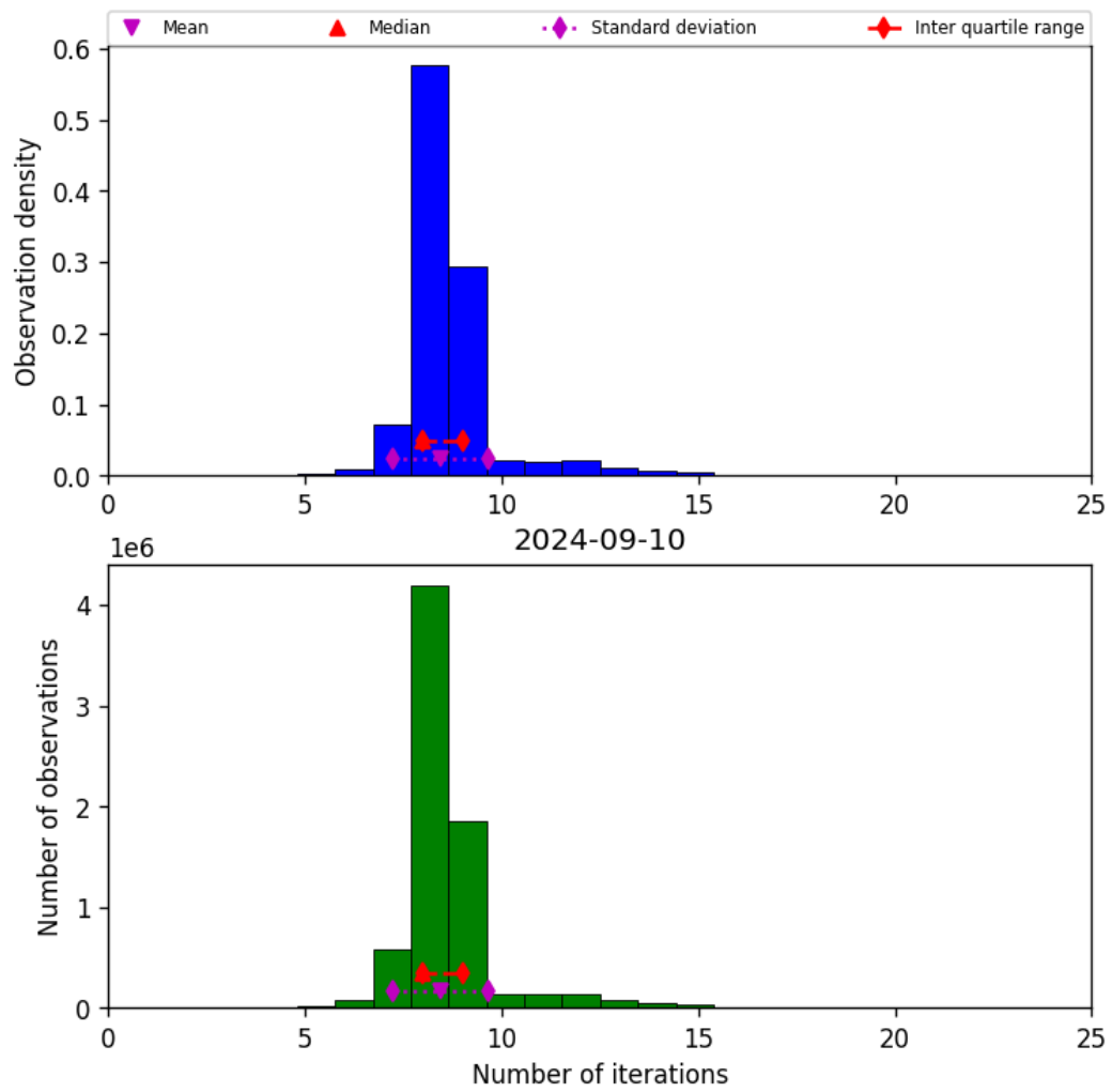
Figure 24: Histogram of “Number of iterations” for 2024-09-09 to 2024-09-11
