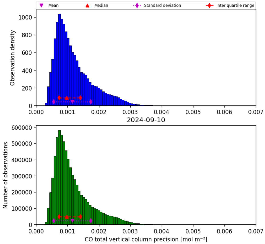
Figure 20: Histogram of “CO total vertical column precision” for 2024-09-09 to 2024-09-11
