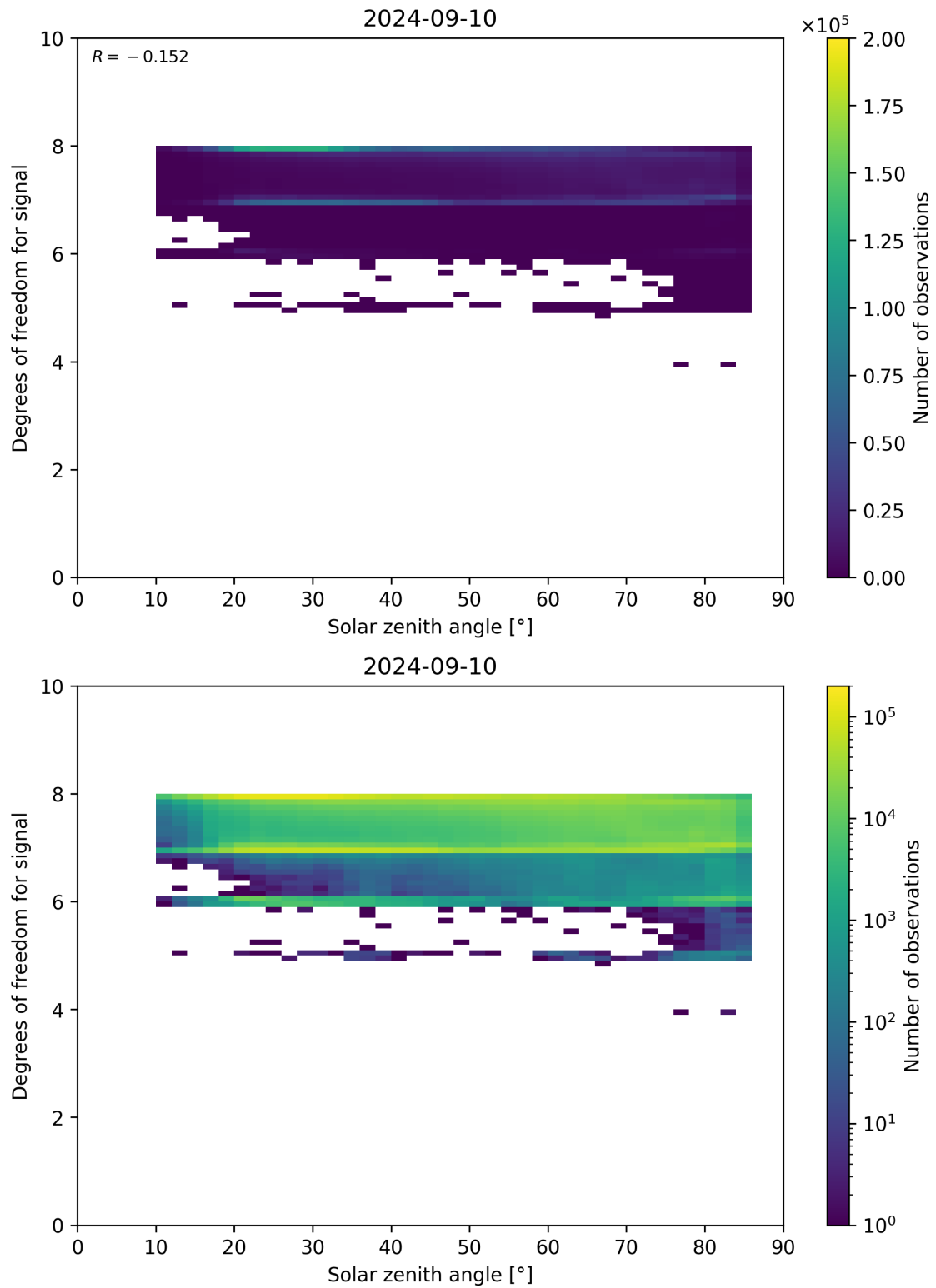
Figure 65: Scatter density plot of “Solar zenith angle” against “Degrees of freedom for signal” for 2024-09-09 to 2024-09-11.
