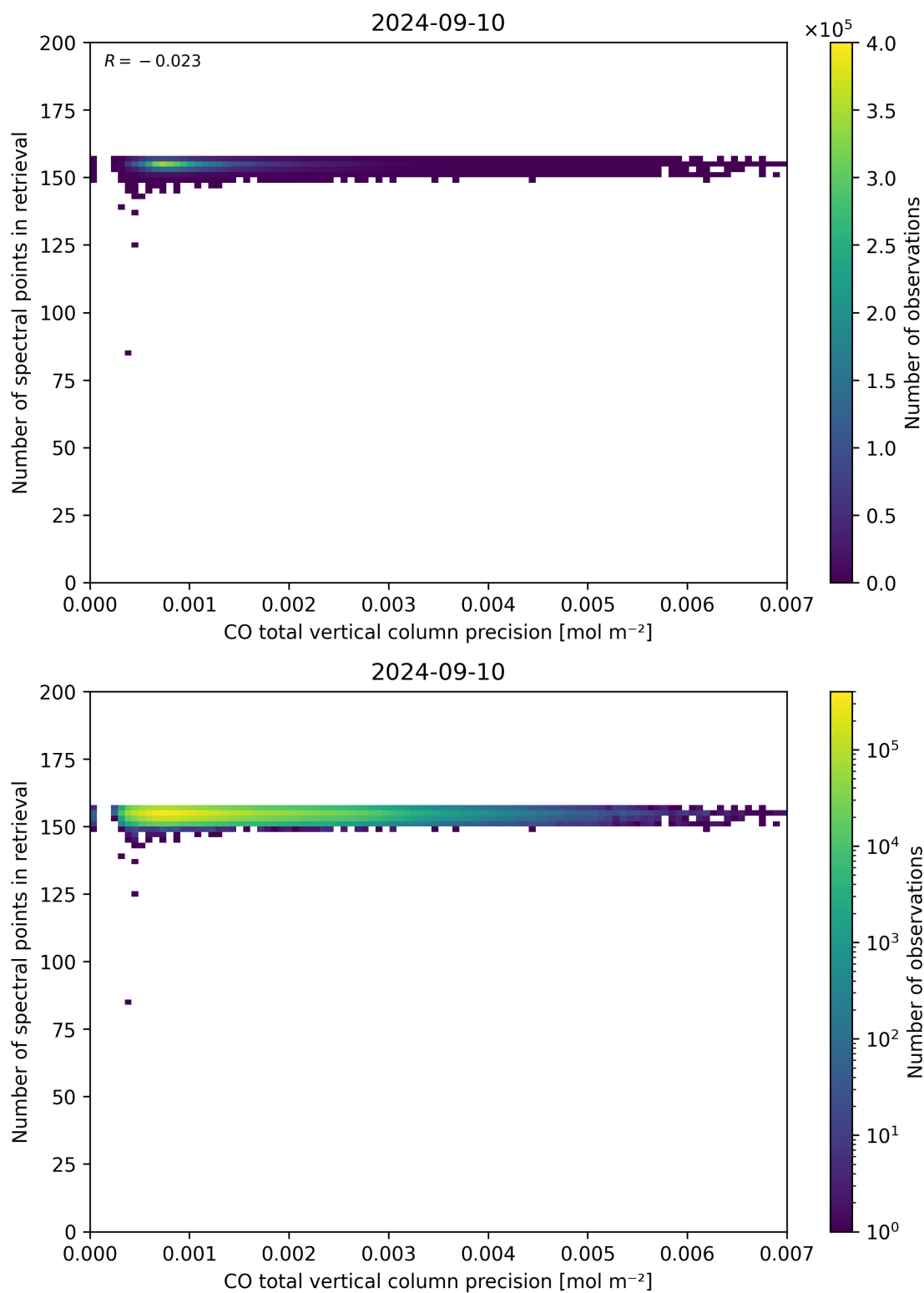
Figure 47: Scatter density plot of “CO total vertical column precision” against “Number of spectral points in retrieval” for 2024-09-09 to 2024-09-11.
