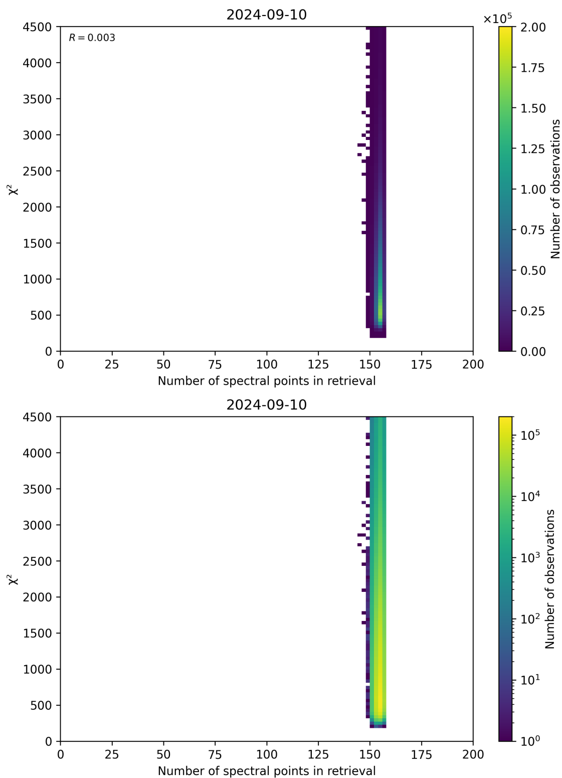
Figure 58: Scatter density plot of “Number of spectral points in retrieval” against “ \chi^2 ” for 2024-09-09 to 2024-09-11.
