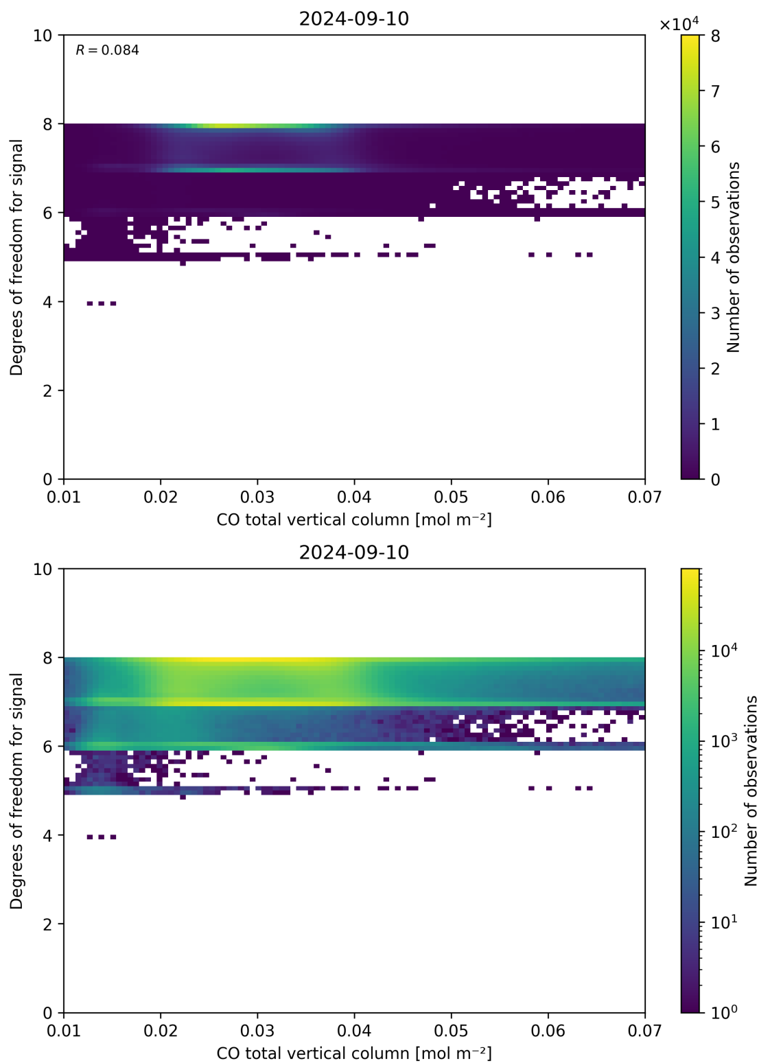
Figure 41: Scatter density plot of “CO total vertical column” against “Degrees of freedom for signal” for 2024-09-09 to 2024-09-11.
