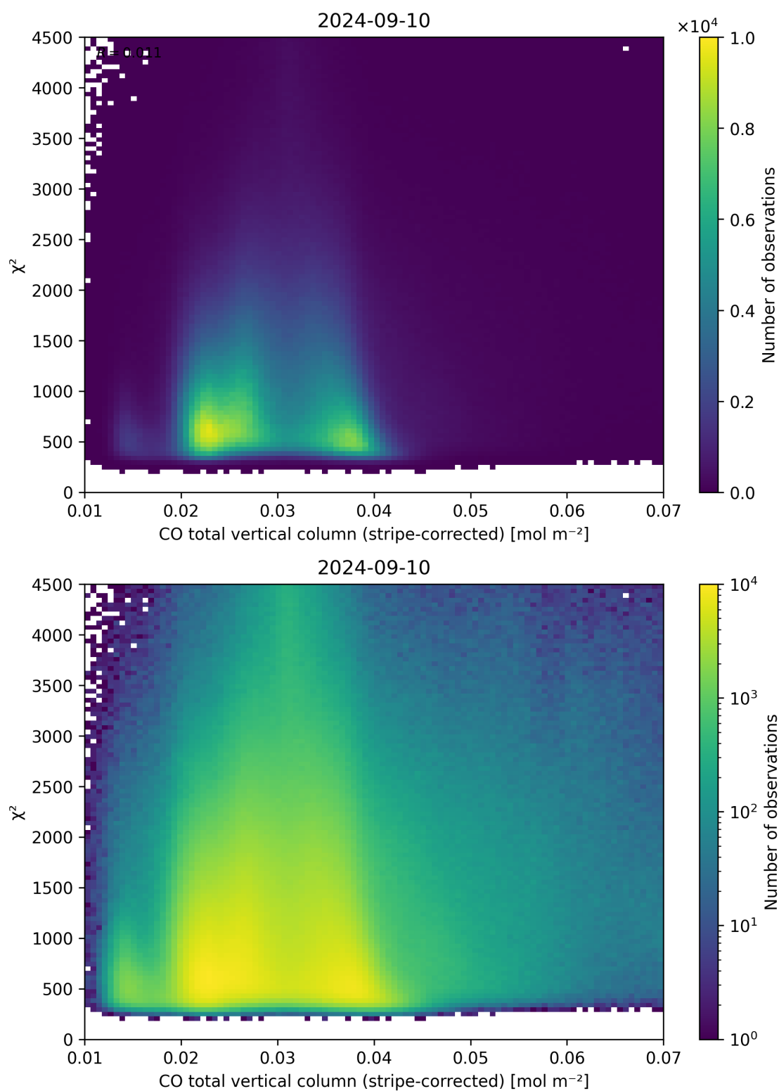
Figure 37: Scatter density plot of “CO total vertical column (stripe-corrected)” against “ \chi^2 ” for 2024-09-09 to 2024-09-11.
