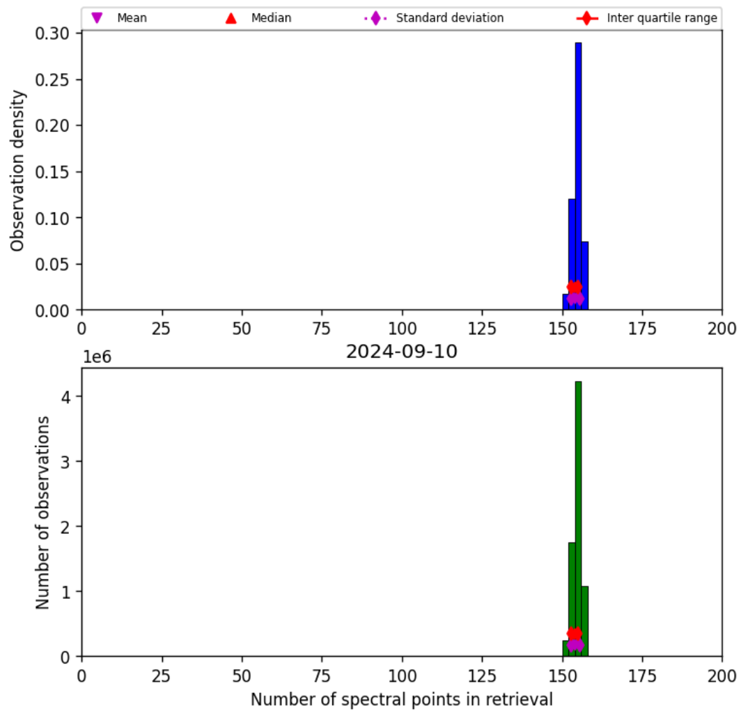
Figure 21: Histogram of “Number of spectral points in retrieval” for 2024-09-09 to 2024-09-11
