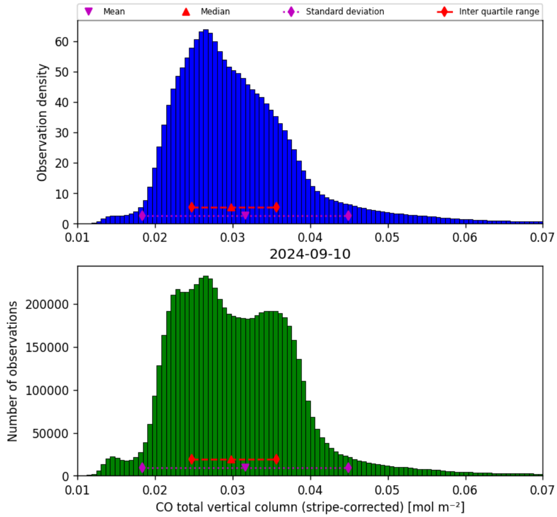
Figure 19: Histogram of “CO total vertical column (stripe-corrected)” for 2024-09-09 to 2024-09-11
