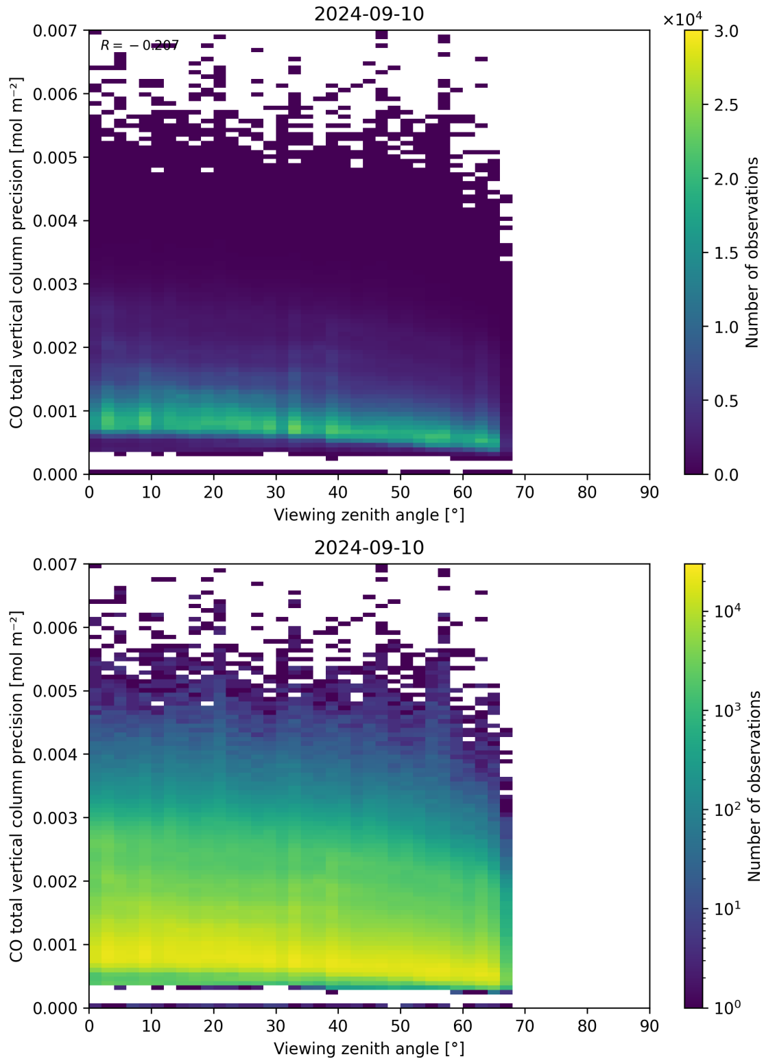
Figure 71: Scatter density plot of “Viewing zenith angle” against “CO total vertical column precision” for 2024-09-09 to 2024-09-11.
