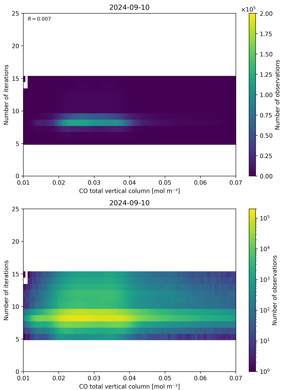
Figure 42: Scatter density plot of “CO total vertical column” against “Number of iterations” for 2024-09-09 to 2024-09-11.
