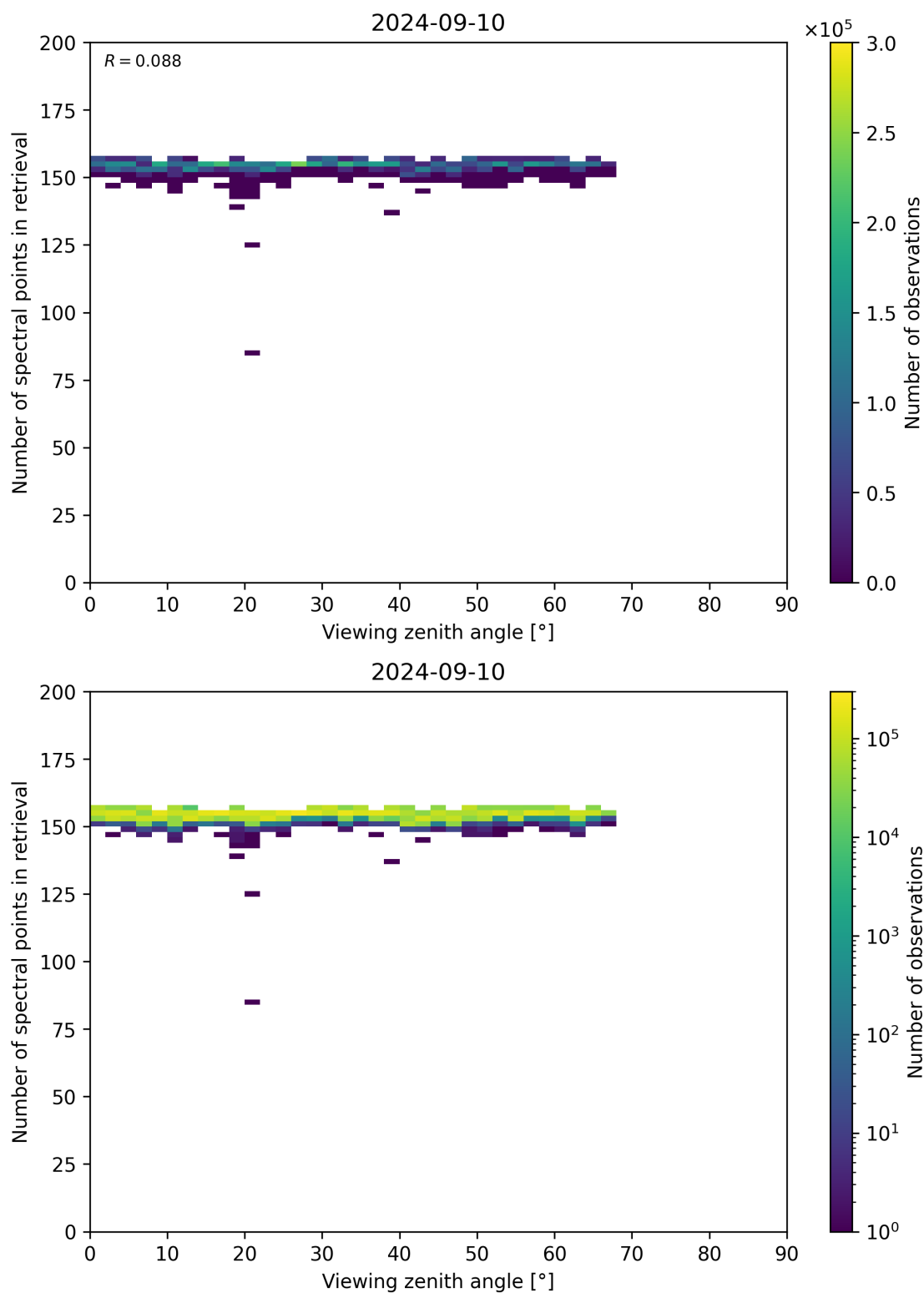
Figure 76: Scatter density plot of “Viewing zenith angle” against “Number of spectral points in retrieval” for 2024-09-09 to 2024-09-11.
