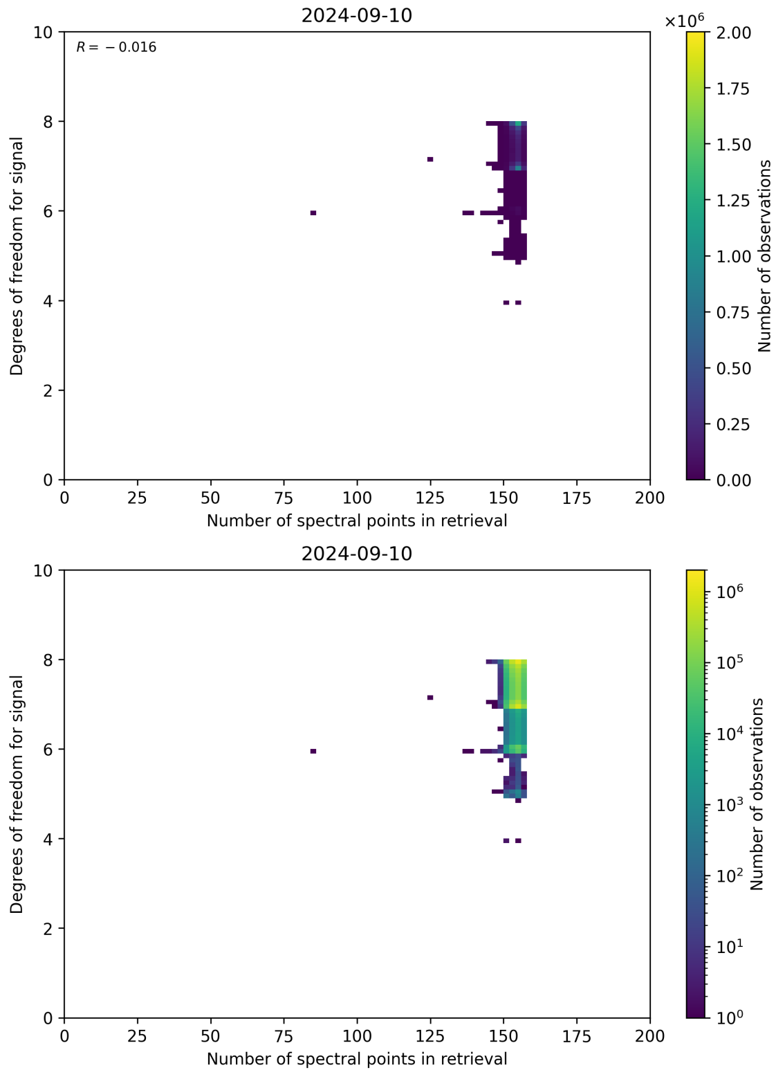
Figure 59: Scatter density plot of “Number of spectral points in retrieval” against “Degrees of freedom for signal” for 2024-09-09 to 2024-09-11.
