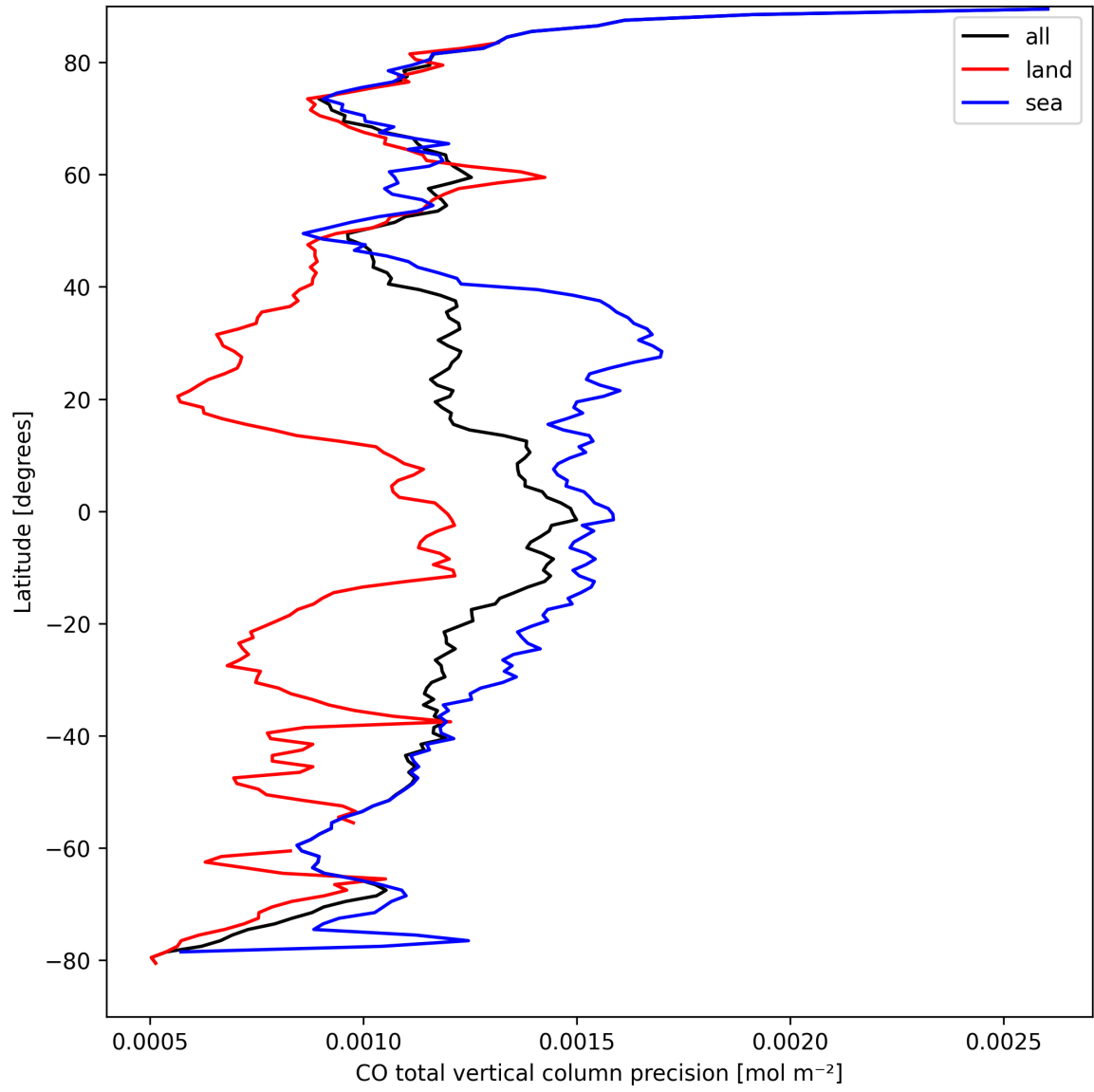
Figure 12: Zonal average of “CO total vertical column precision” for 2024-09-09 to 2024-09-11.
