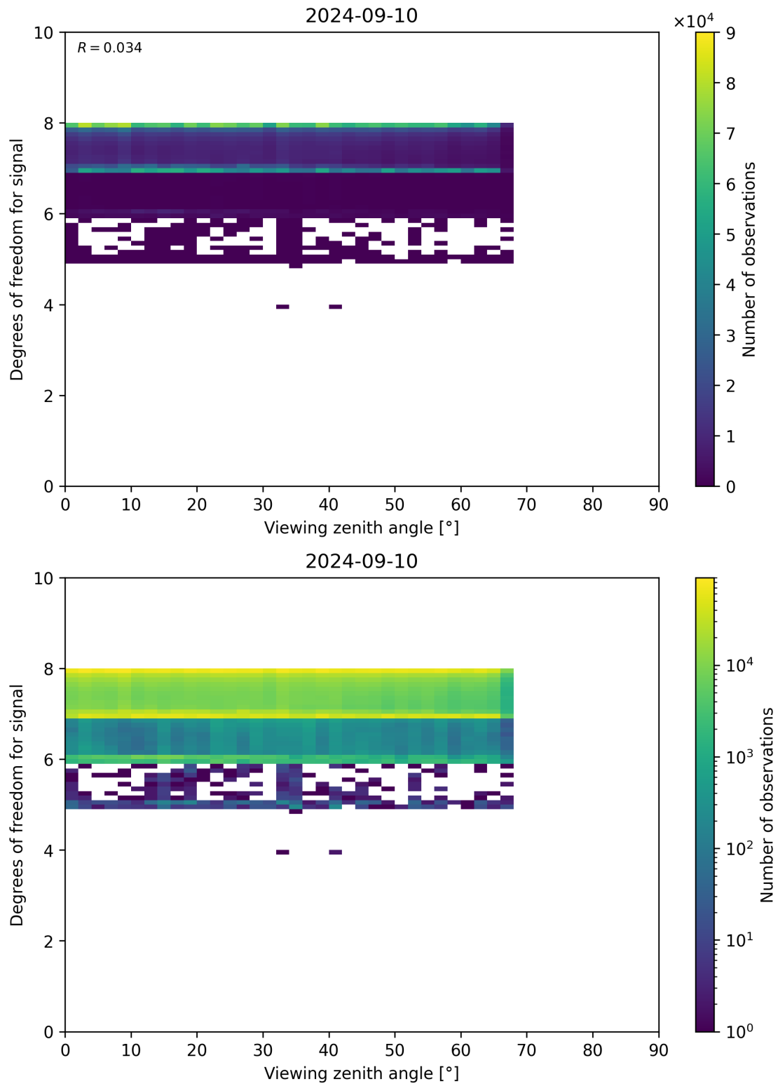
Figure 73: Scatter density plot of “Viewing zenith angle” against “Degrees of freedom for signal” for 2024-09-09 to 2024-09-11.
