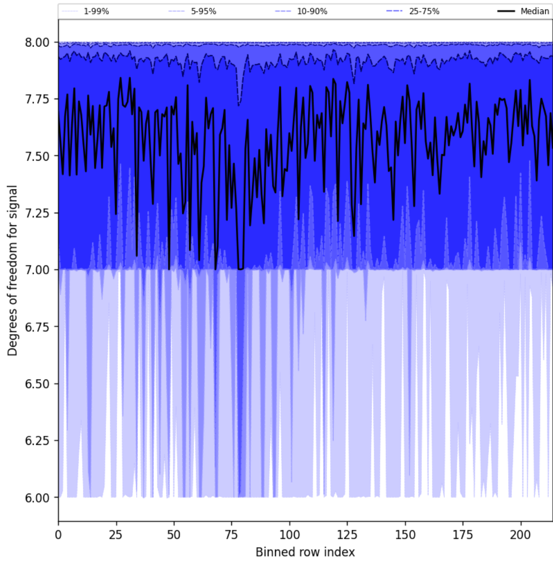
Figure 31: Along track statistics of “Degrees of freedom for signal” for 2024-09-09 to 2024-09-11
