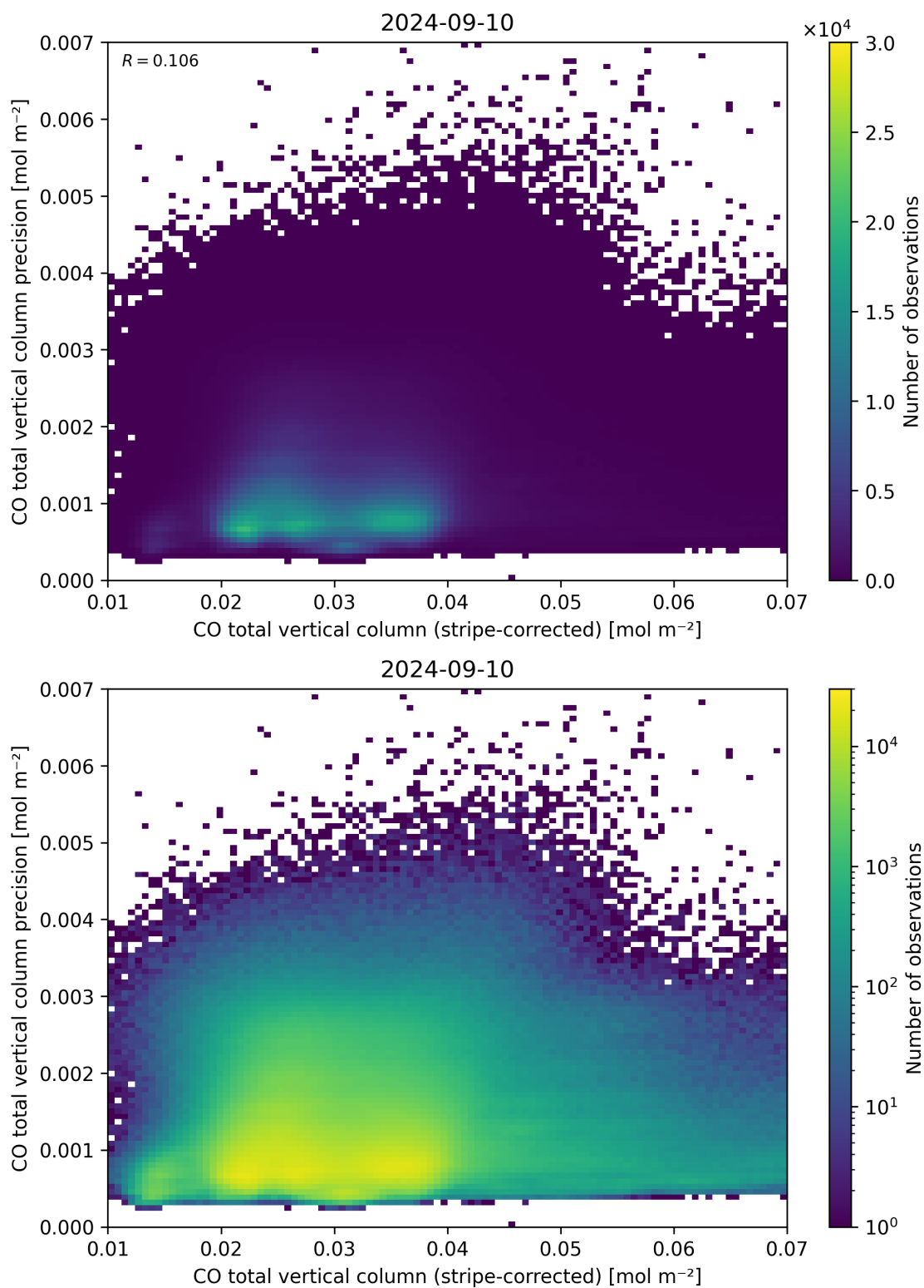
Figure 36: Scatter density plot of “CO total vertical column (stripe-corrected)” against “CO total vertical column precision” for 2024-09-09 to 2024-09-11.
