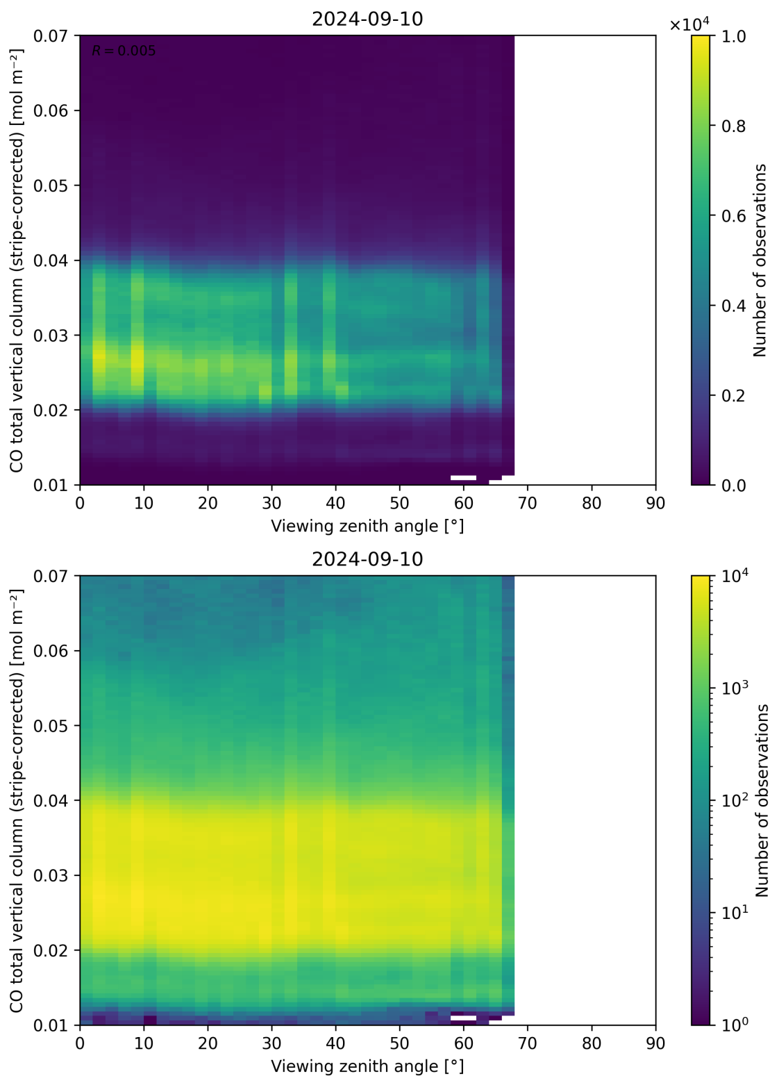
Figure 70: Scatter density plot of “Viewing zenith angle” against “CO total vertical column (stripe-corrected)” for 2024-09-09 to 2024-09-11.
