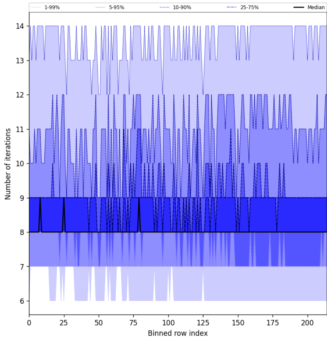
Figure 32: Along track statistics of “Number of iterations” for 2024-09-09 to 2024-09-11
