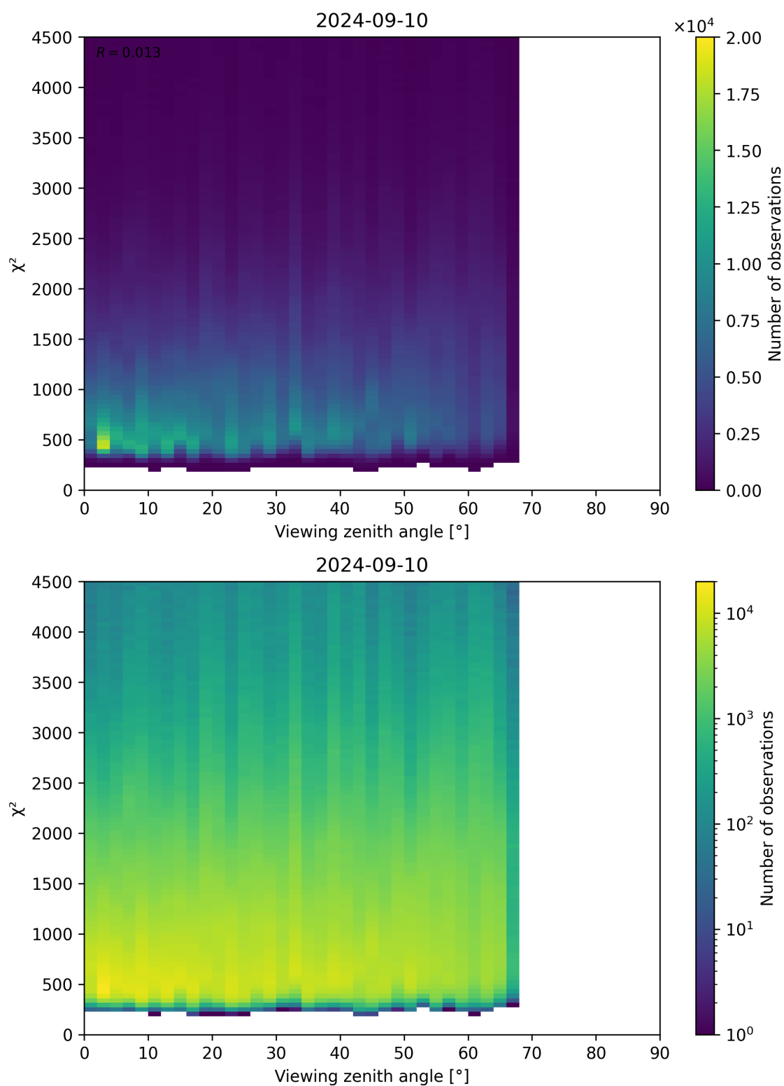
Figure 72: Scatter density plot of “Viewing zenith angle” against “ \chi^2 ” for 2024-09-09 to 2024-09-11.
