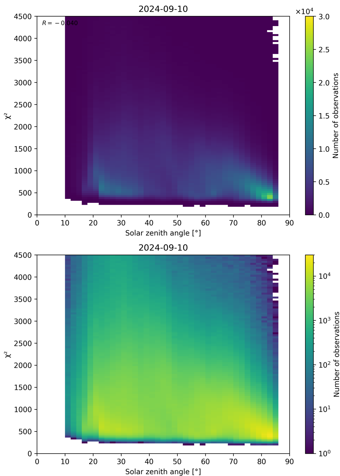
Figure 64: Scatter density plot of “Solar zenith angle” against “ \chi^2 ” for 2024-09-09 to 2024-09-11.
