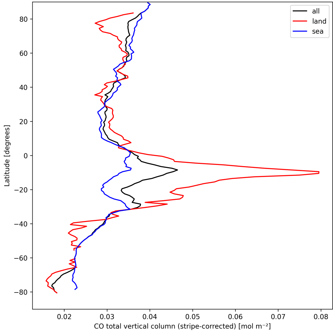
Figure 11: Zonal average of “CO total vertical column (stripe-corrected)” for 2024-09-09 to 2024-09-11.
