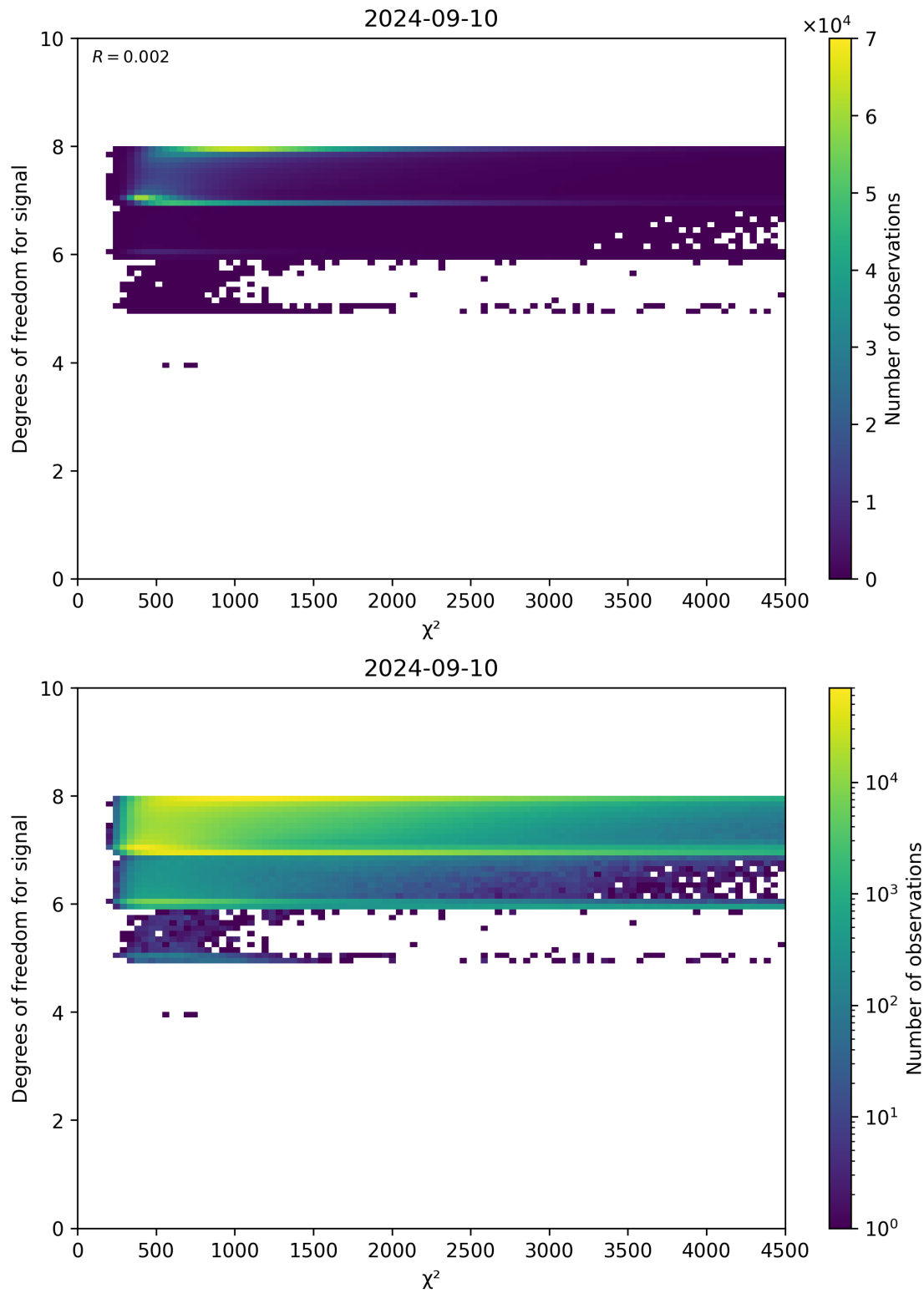
Figure 48: Scatter density plot of “ \chi^2 ” against “Degrees of freedom for signal” for 2024-09-09 to 2024-09-11.
