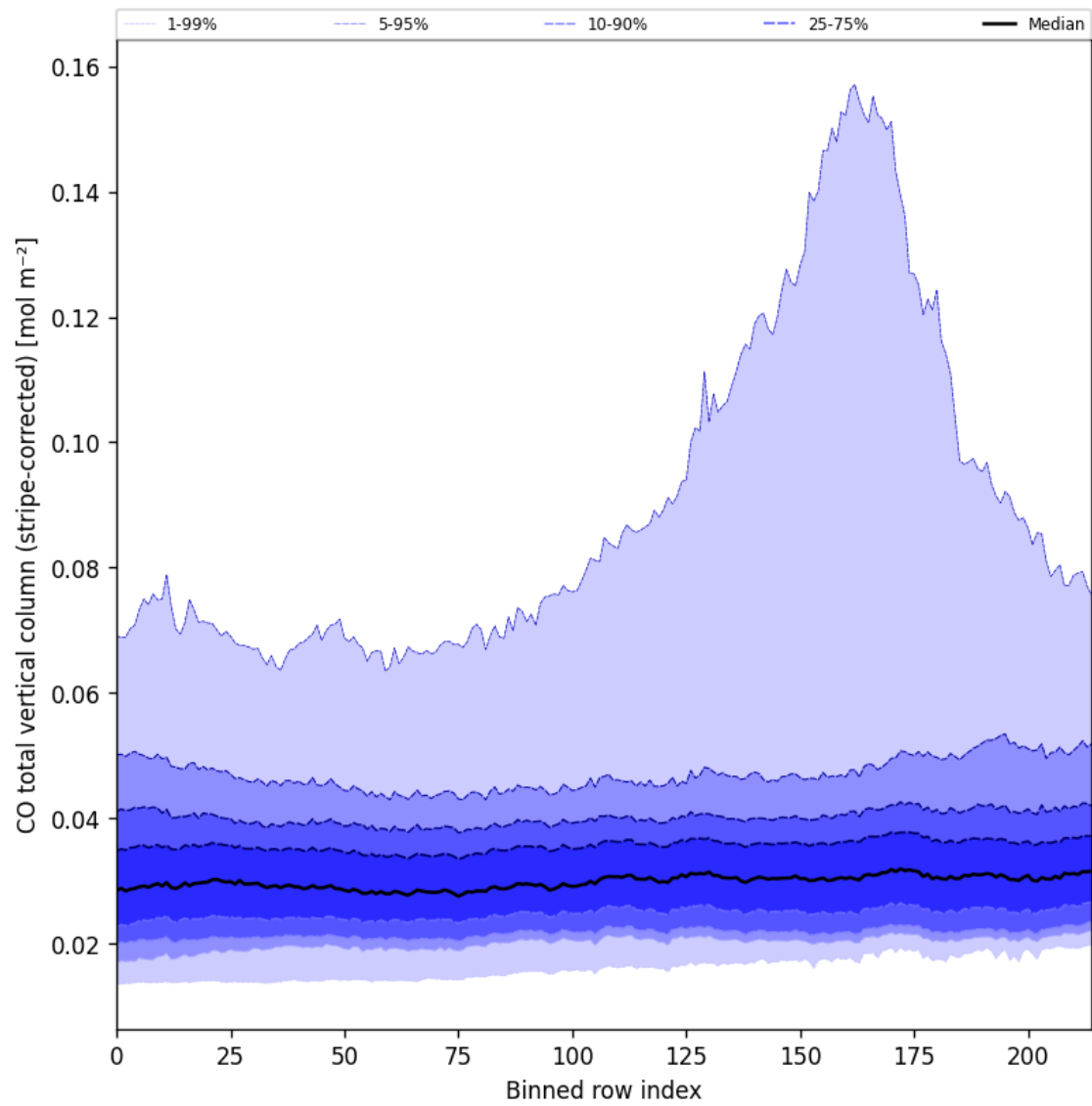
Figure 27: Along track statistics of “CO total vertical column (stripe-corrected)” for 2024-09-09 to 2024-09-11
