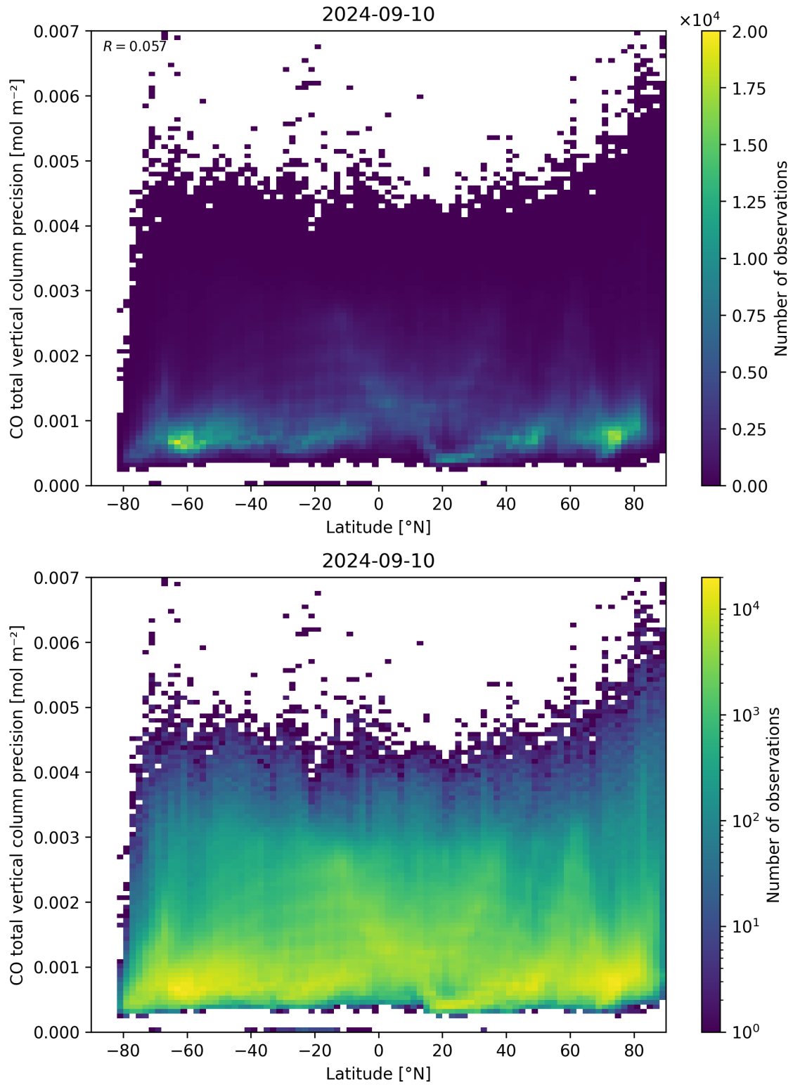
Figure 53: Scatter density plot of “Latitude” against “CO total vertical column precision” for 2024-09-09 to 2024-09-11.
