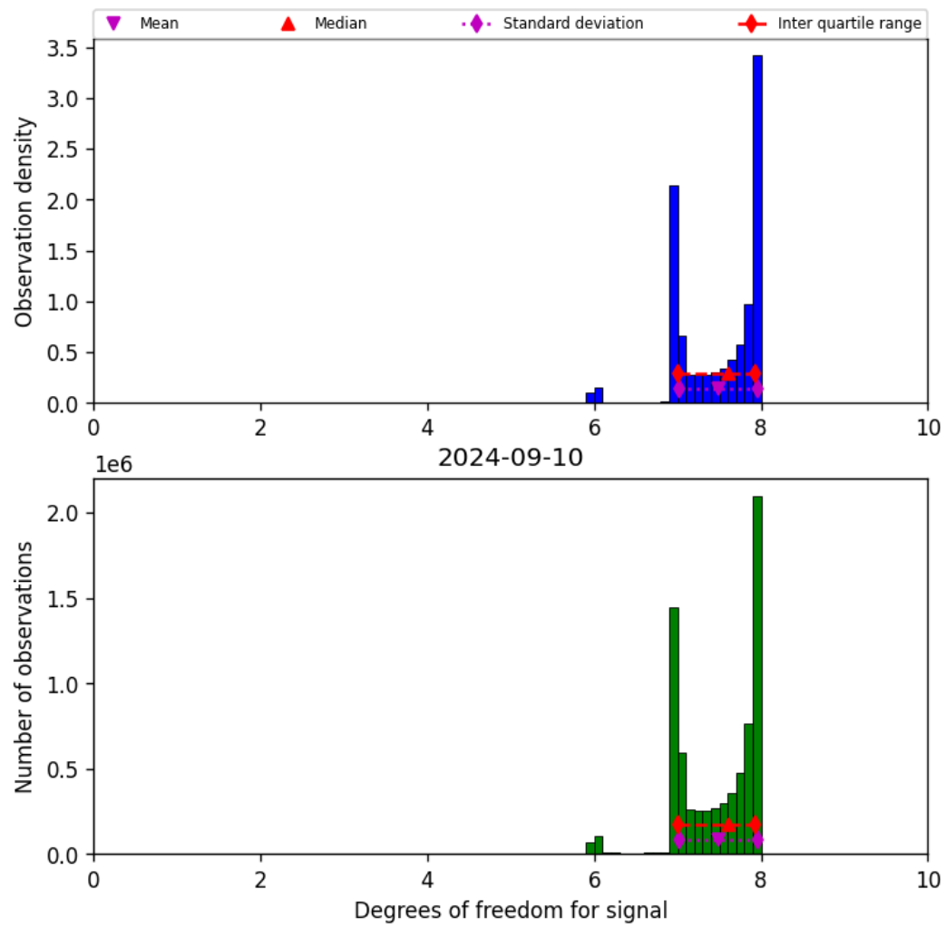
Figure 23: Histogram of “Degrees of freedom for signal” for 2024-09-09 to 2024-09-11
