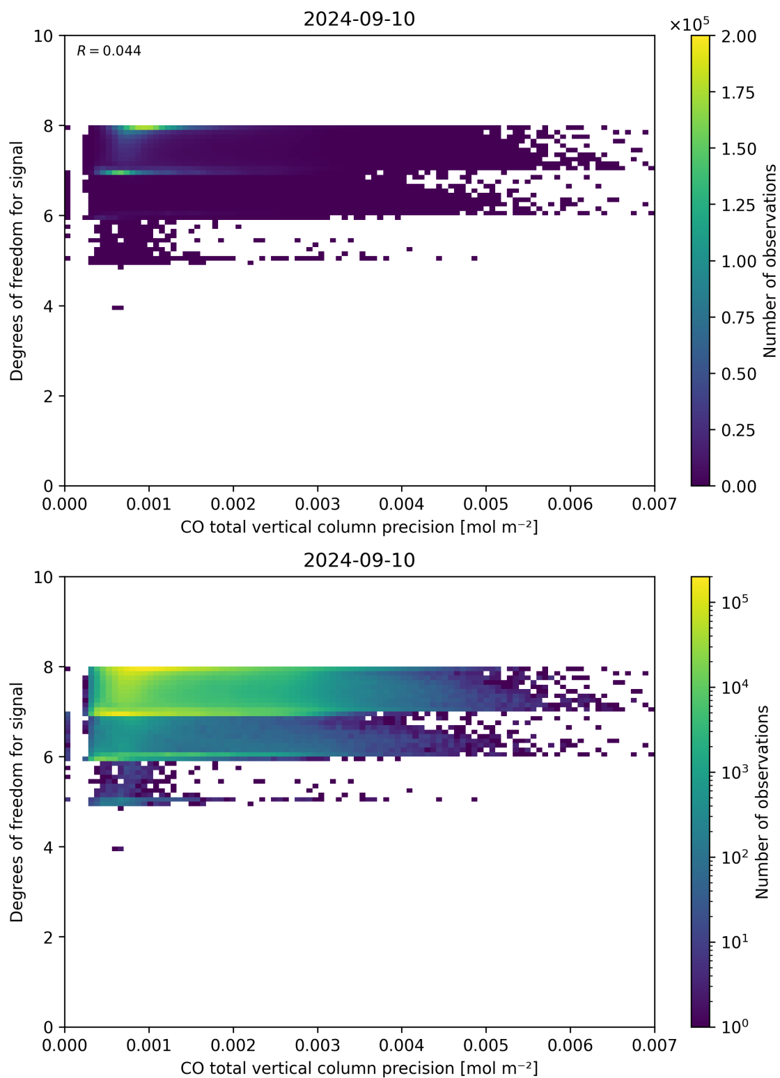
Figure 45: Scatter density plot of “CO total vertical column precision” against “Degrees of freedom for signal” for 2024-09-09 to 2024-09-11.
