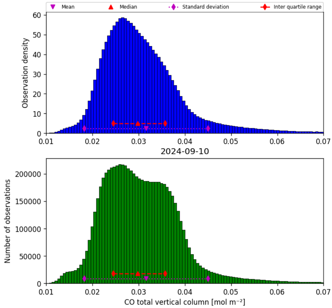
Figure 18: Histogram of “CO total vertical column” for 2024-09-09 to 2024-09-11
