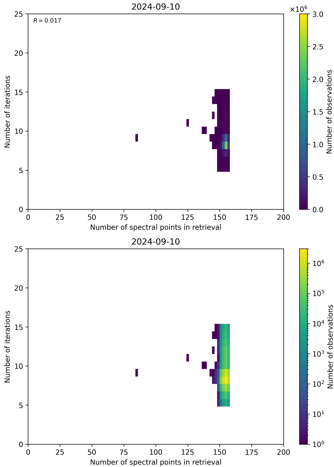
Figure 60: Scatter density plot of “Number of spectral points in retrieval” against “Number of iterations” for 2024-09-09 to 2024-09-11.
