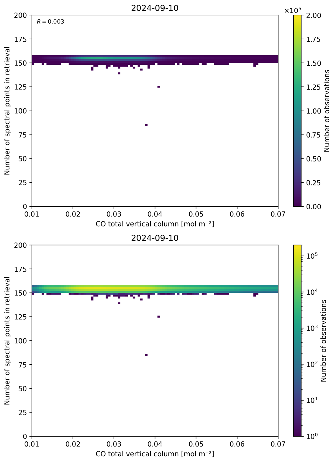
Figure 43: Scatter density plot of “CO total vertical column” against “Number of spectral points in retrieval” for 2024-09-09 to 2024-09-11.
