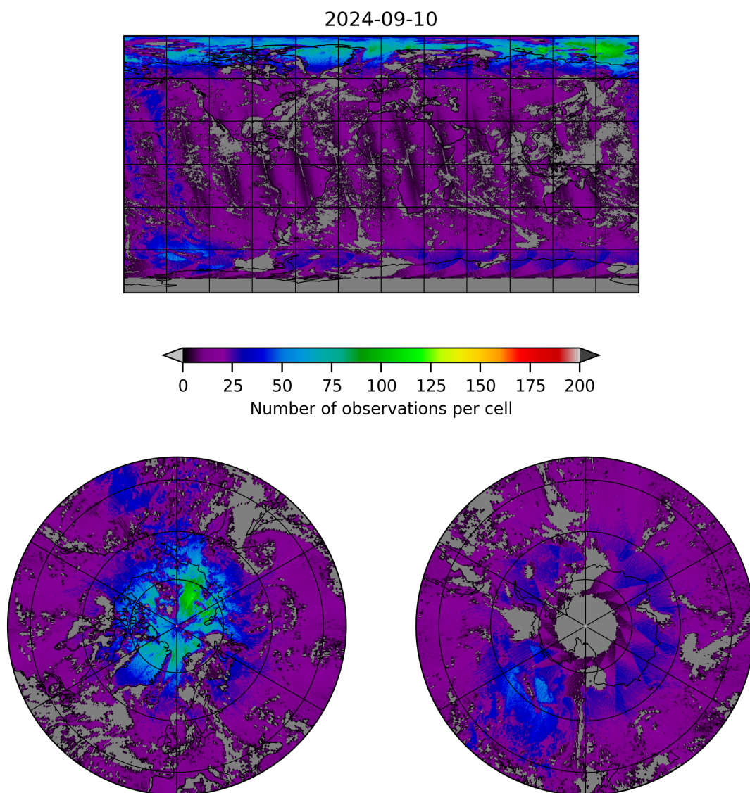
Figure 8: Map of the number of observations for 2024-09-09 to 2024-09-11
