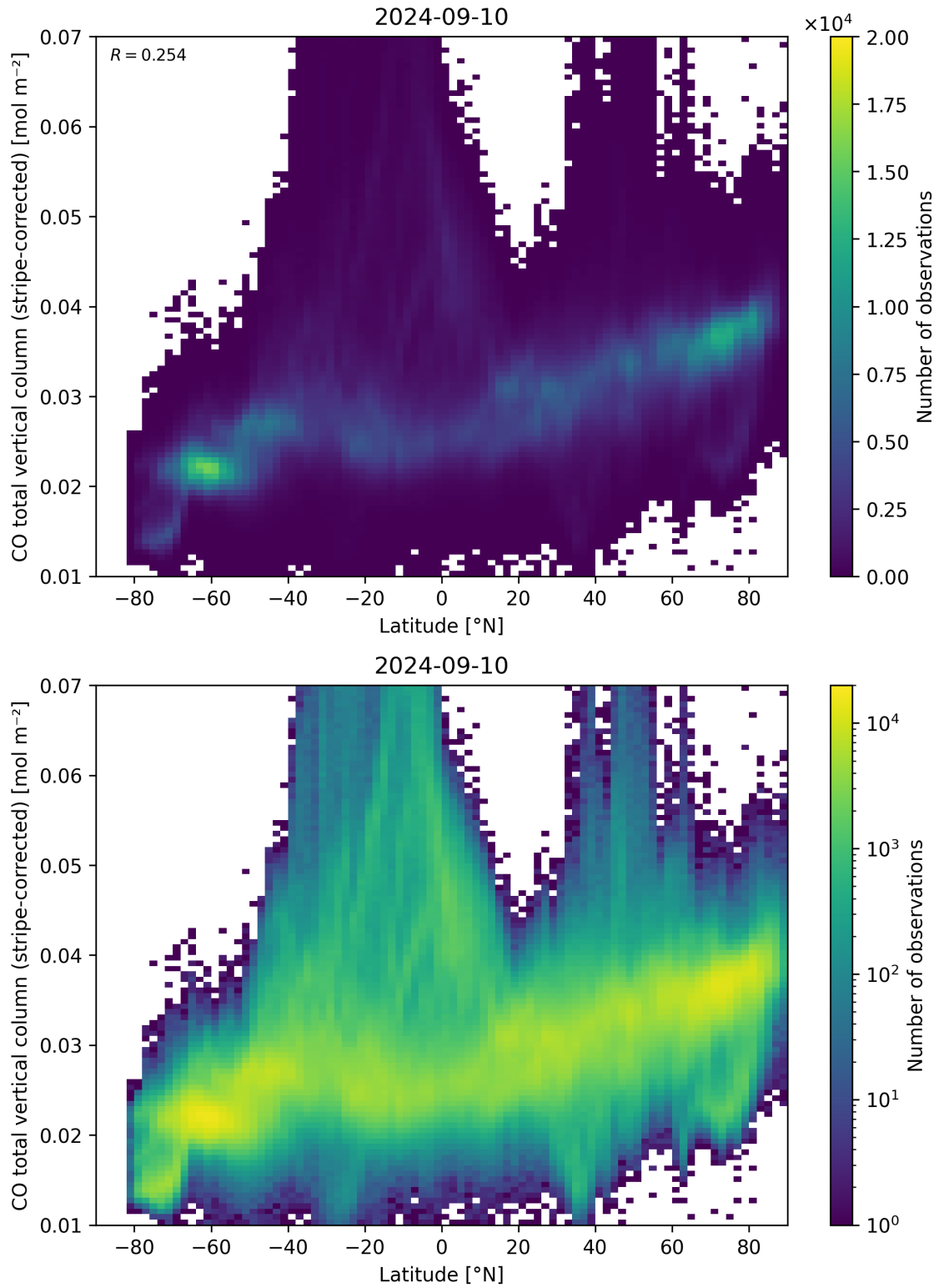
Figure 52: Scatter density plot of “Latitude” against “CO total vertical column (stripe-corrected)” for 2024-09-09 to 2024-09-11.
