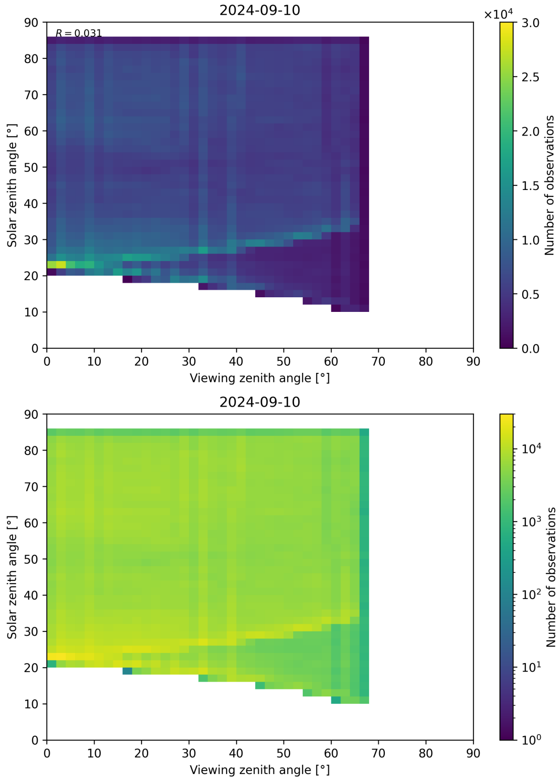
Figure 77: Scatter density plot of “Viewing zenith angle” against “Solar zenith angle” for 2024-09-09 to 2024-09-11.
