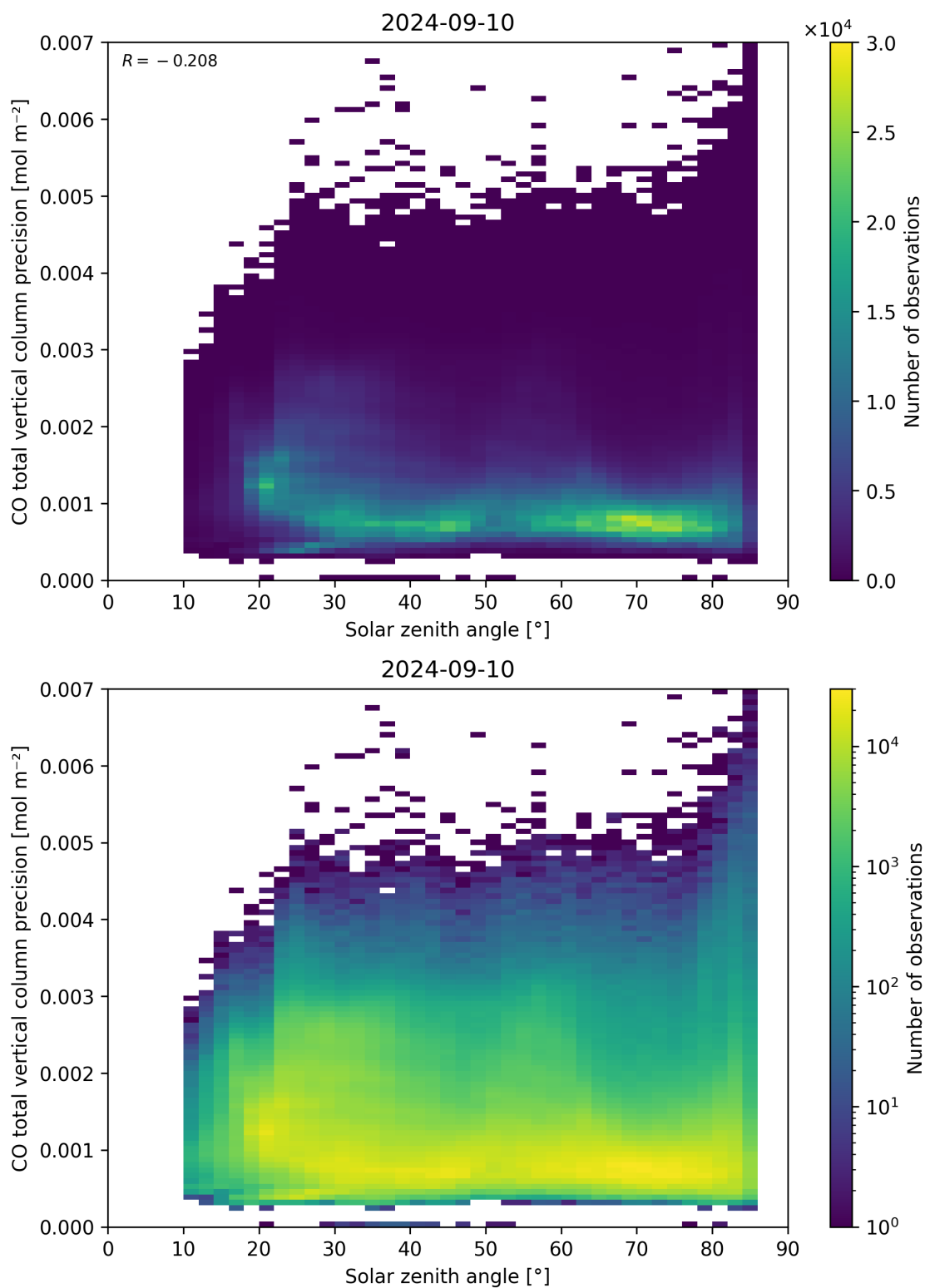
Figure 63: Scatter density plot of “Solar zenith angle” against “CO total vertical column precision” for 2024-09-09 to 2024-09-11.
