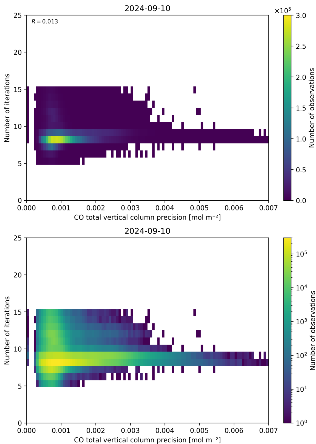
Figure 46: Scatter density plot of “CO total vertical column precision” against “Number of iterations” for 2024-09-09 to 2024-09-11.
