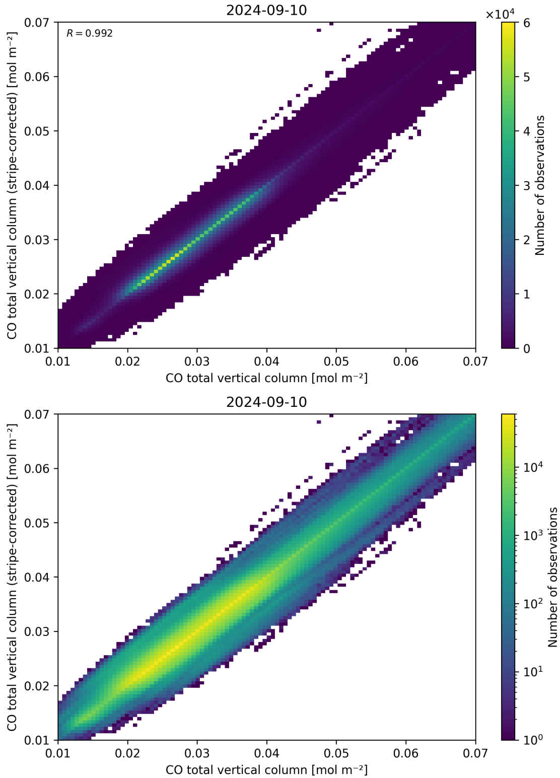
Figure 33: Scatter density plot of “CO total vertical column” against “CO total vertical column (stripe-corrected)” for 2024-09-09 to 2024-09-11.
