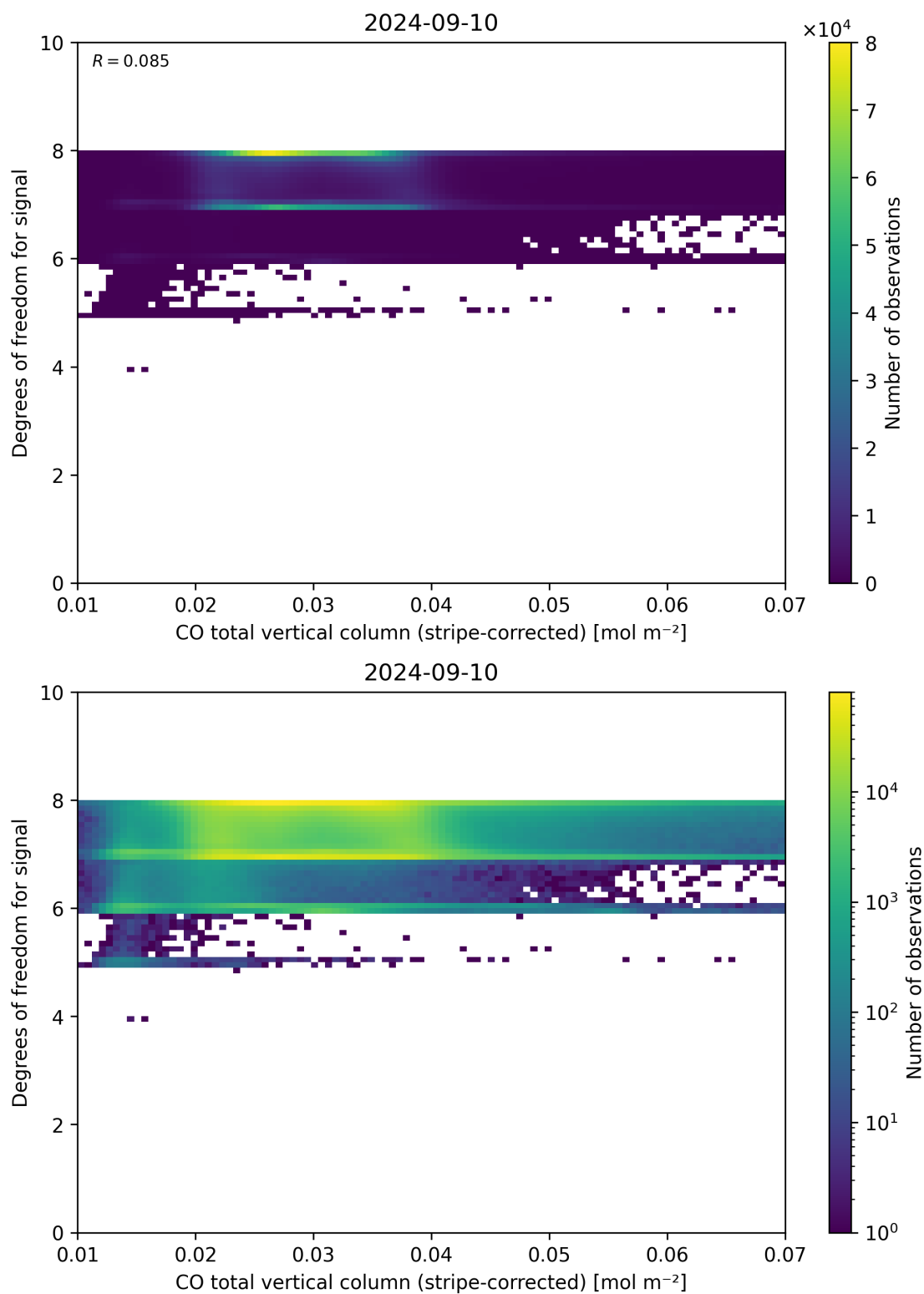
Figure 38: Scatter density plot of “CO total vertical column (stripe-corrected)” against “Degrees of freedom for signal” for 2024-09-09 to 2024-09-11.
