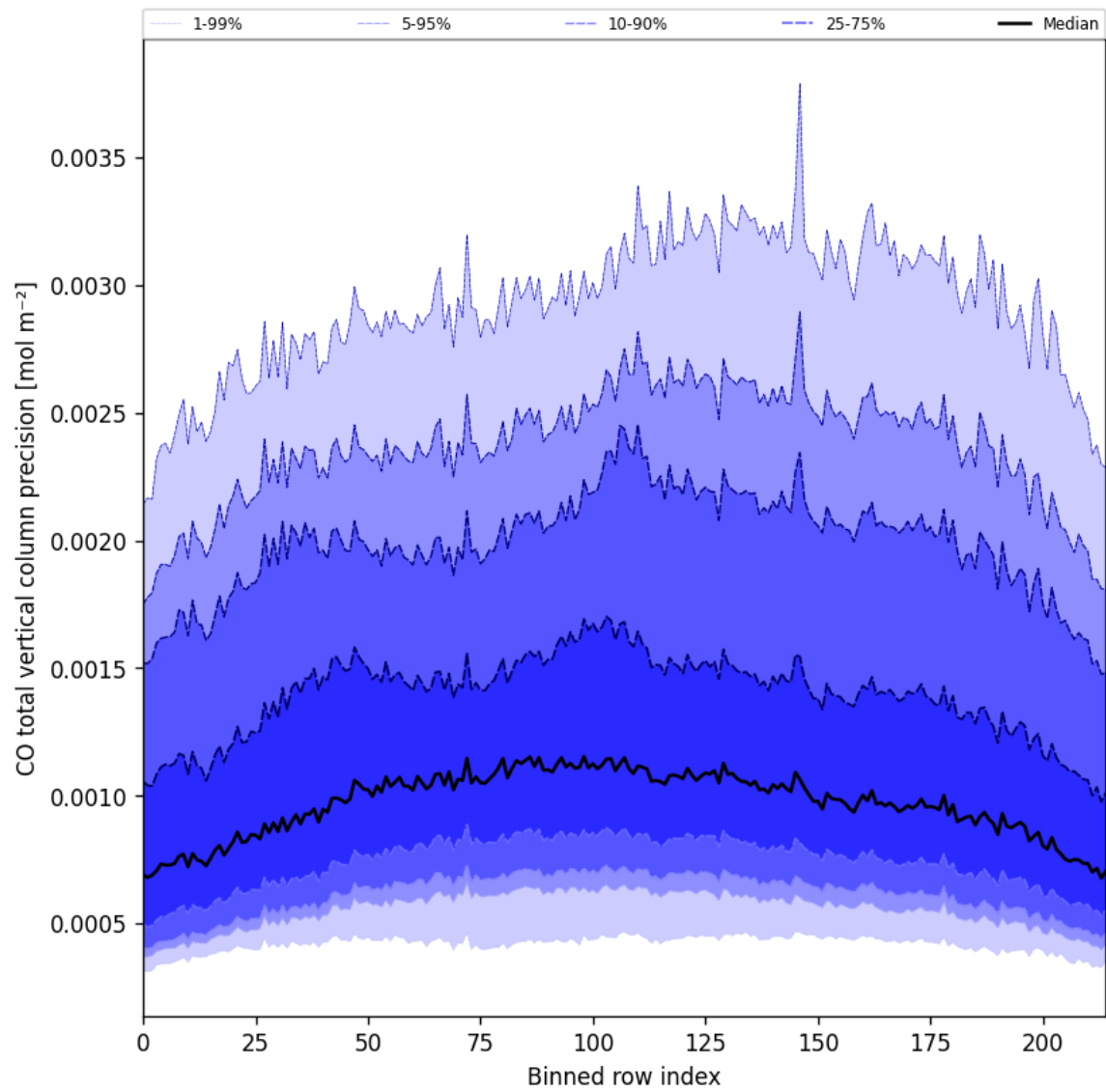
Figure 28: Along track statistics of “CO total vertical column precision” for 2024-09-09 to 2024-09-11
