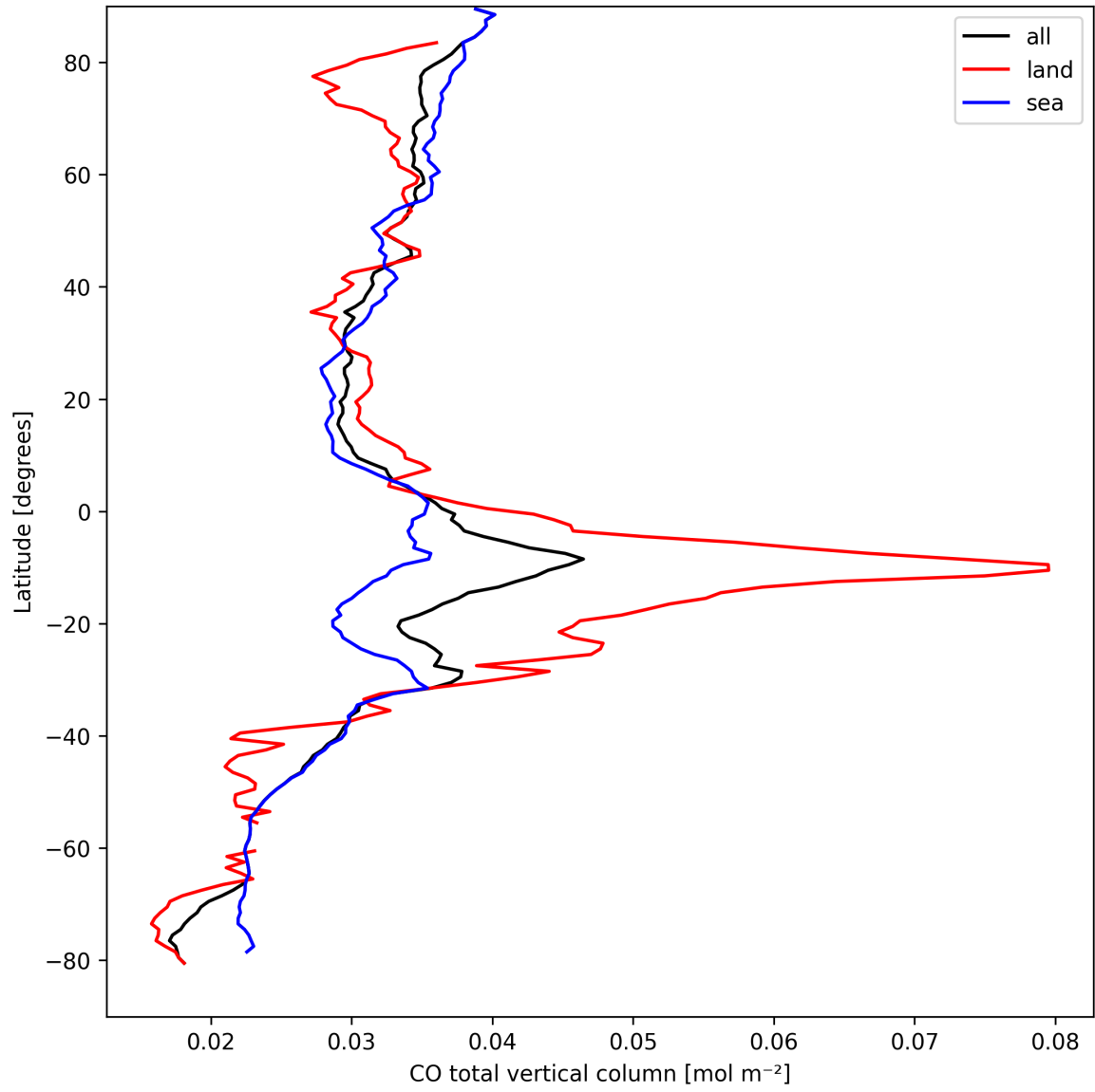
Figure 10: Zonal average of “CO total vertical column” for 2024-09-09 to 2024-09-11.
