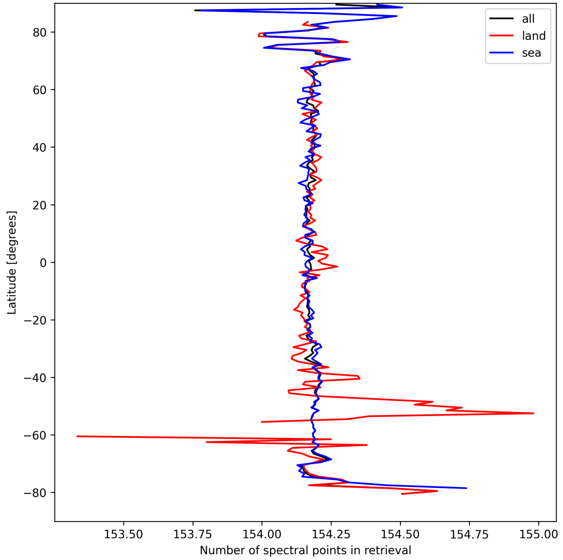
Figure 13: Zonal average of “Number of spectral points in retrieval” for 2024-09-09 to 2024-09-11.
