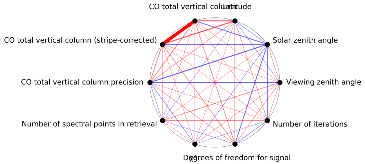
Figure 1: Map of correlation graph for 2024-09-09 to 2024-09-11.
