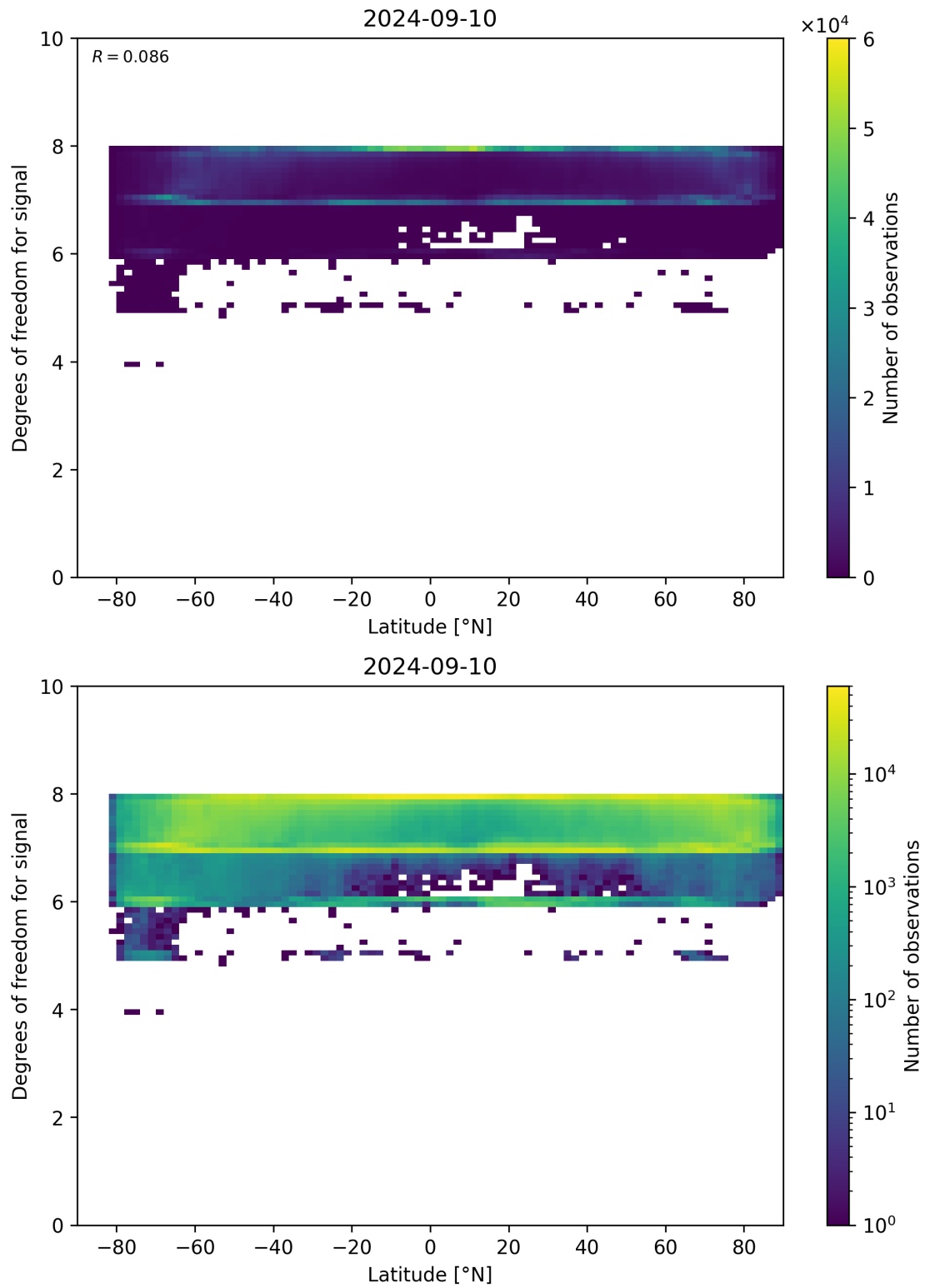
Figure 55: Scatter density plot of “Latitude” against “Degrees of freedom for signal” for 2024-09-09 to 2024-09-11.
