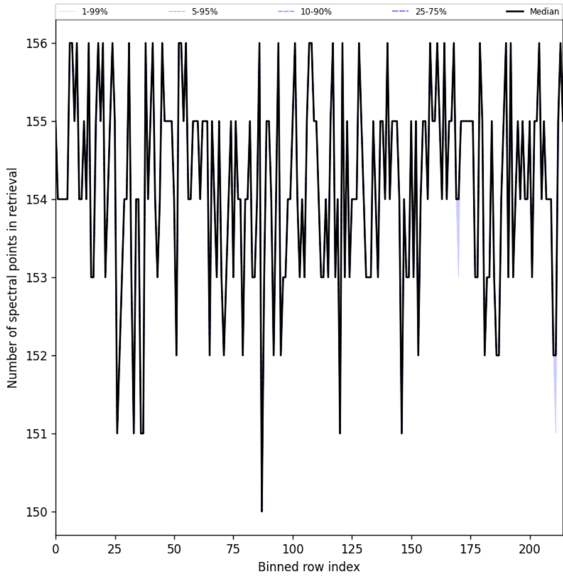
Figure 29: Along track statistics of “Number of spectral points in retrieval” for 2024-09-09 to 2024-09-11
