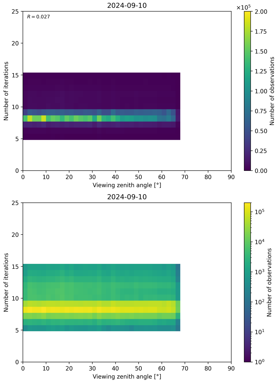
Figure 75: Scatter density plot of “Viewing zenith angle” against “Number of iterations” for 2024-09-09 to 2024-09-11.
