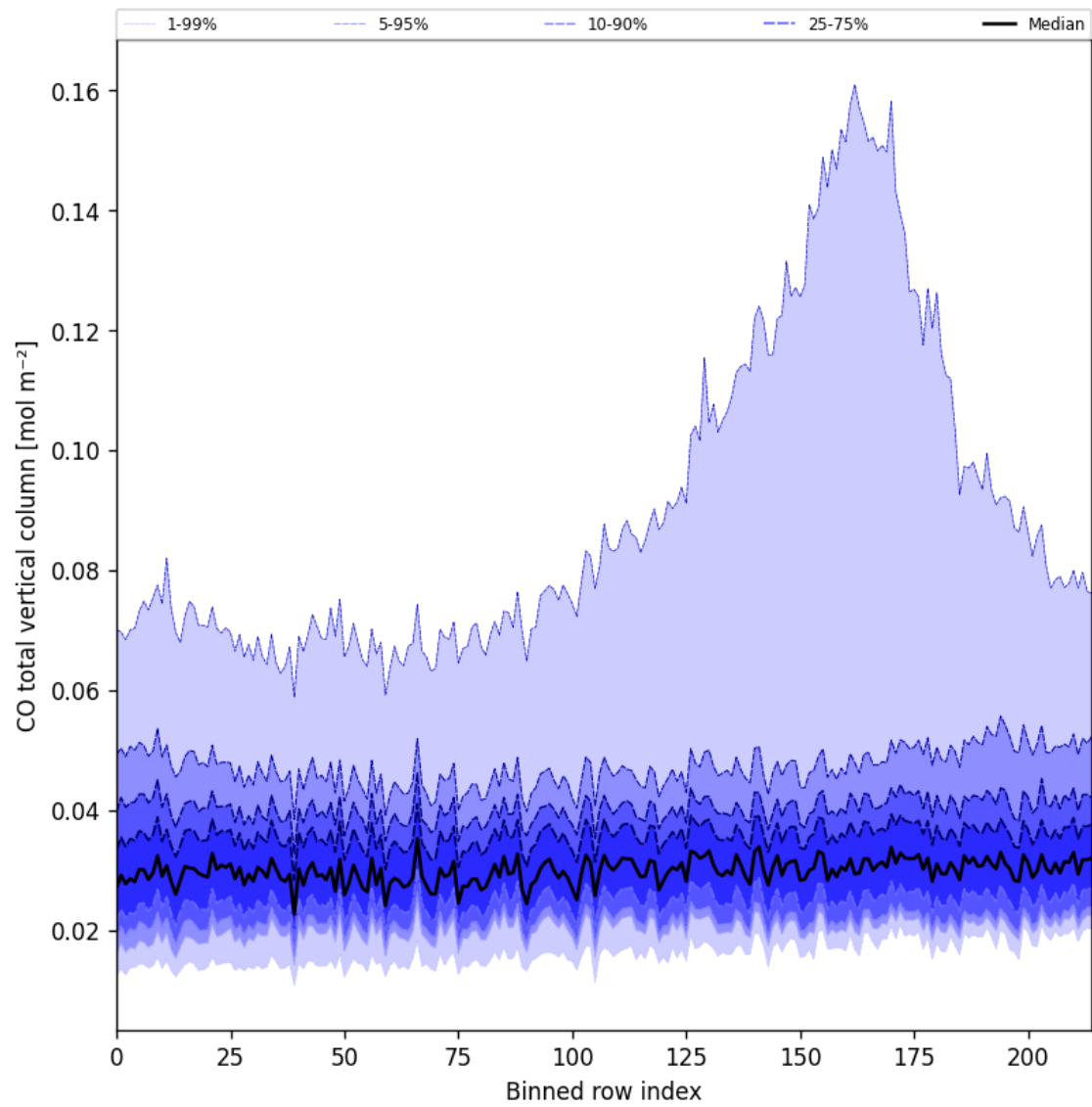
Figure 26: Along track statistics of “CO total vertical column” for 2024-09-09 to 2024-09-11
