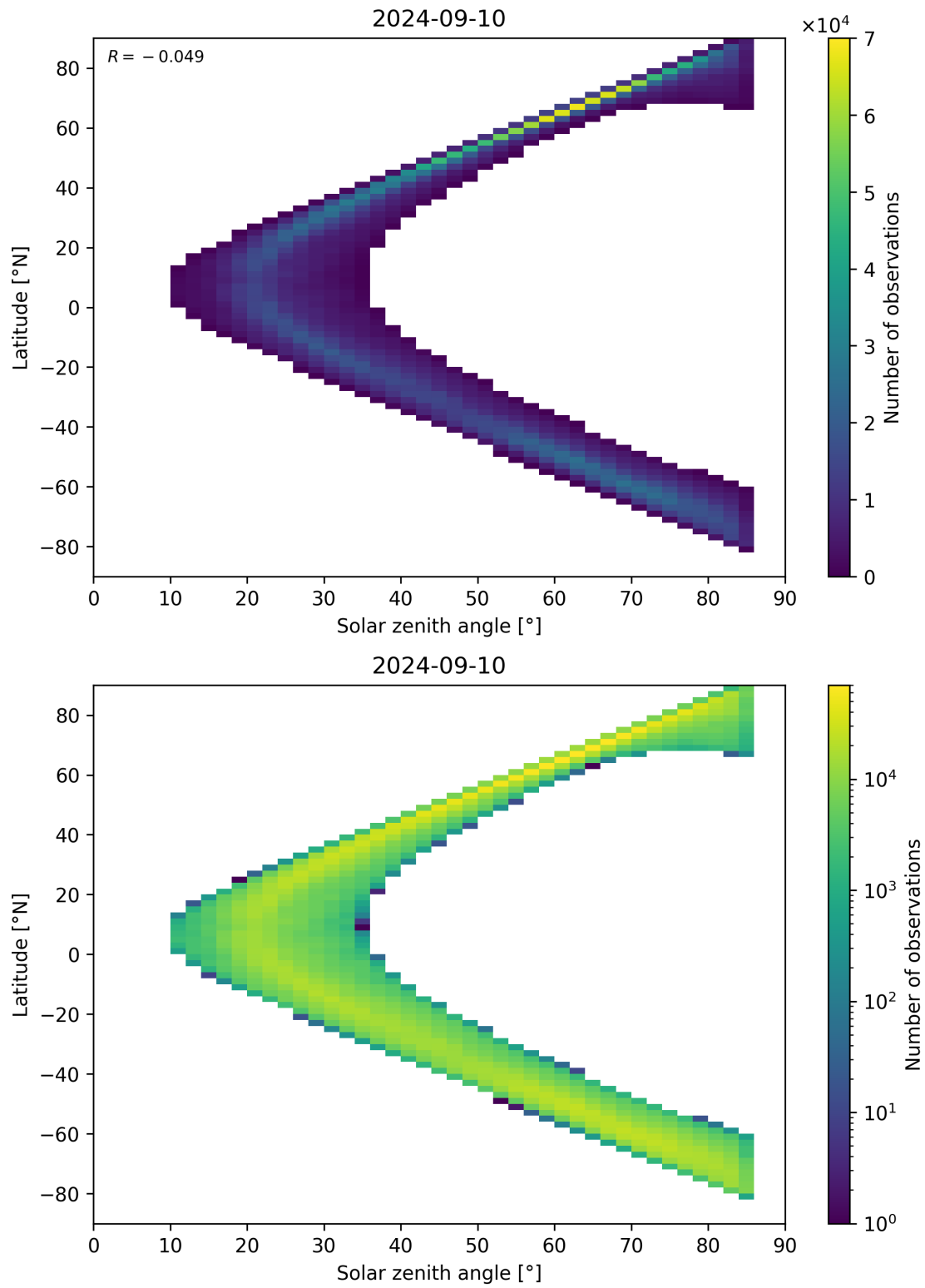
Figure 66: Scatter density plot of “Solar zenith angle” against “Latitude” for 2024-09-09 to 2024-09-11.
