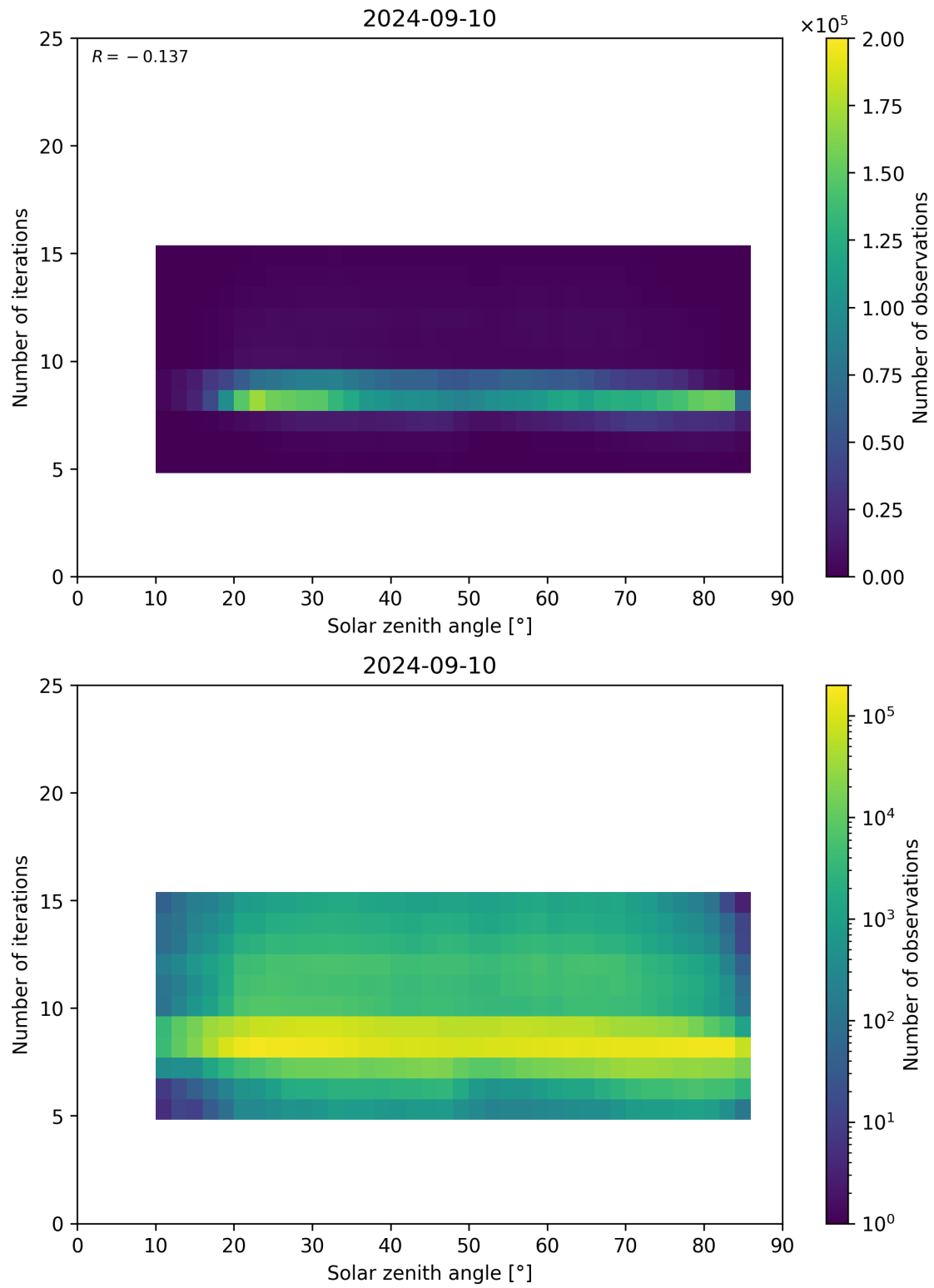
Figure 67: Scatter density plot of “Solar zenith angle” against “Number of iterations” for 2024-09-09 to 2024-09-11.
