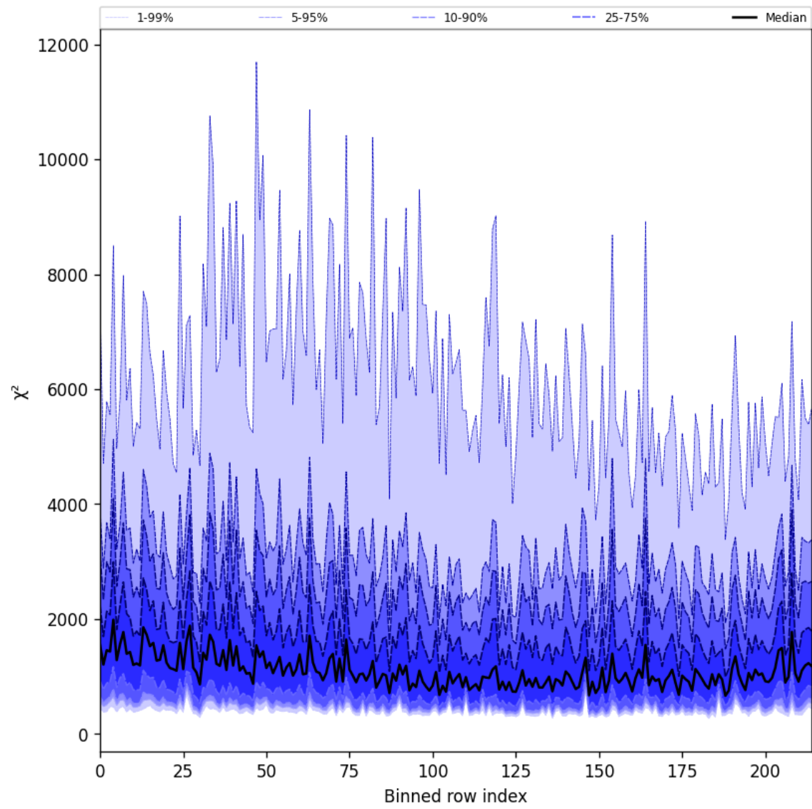
Figure 30: Along track statistics of “ \chi^2 ” for 2024-09-09 to 2024-09-11
