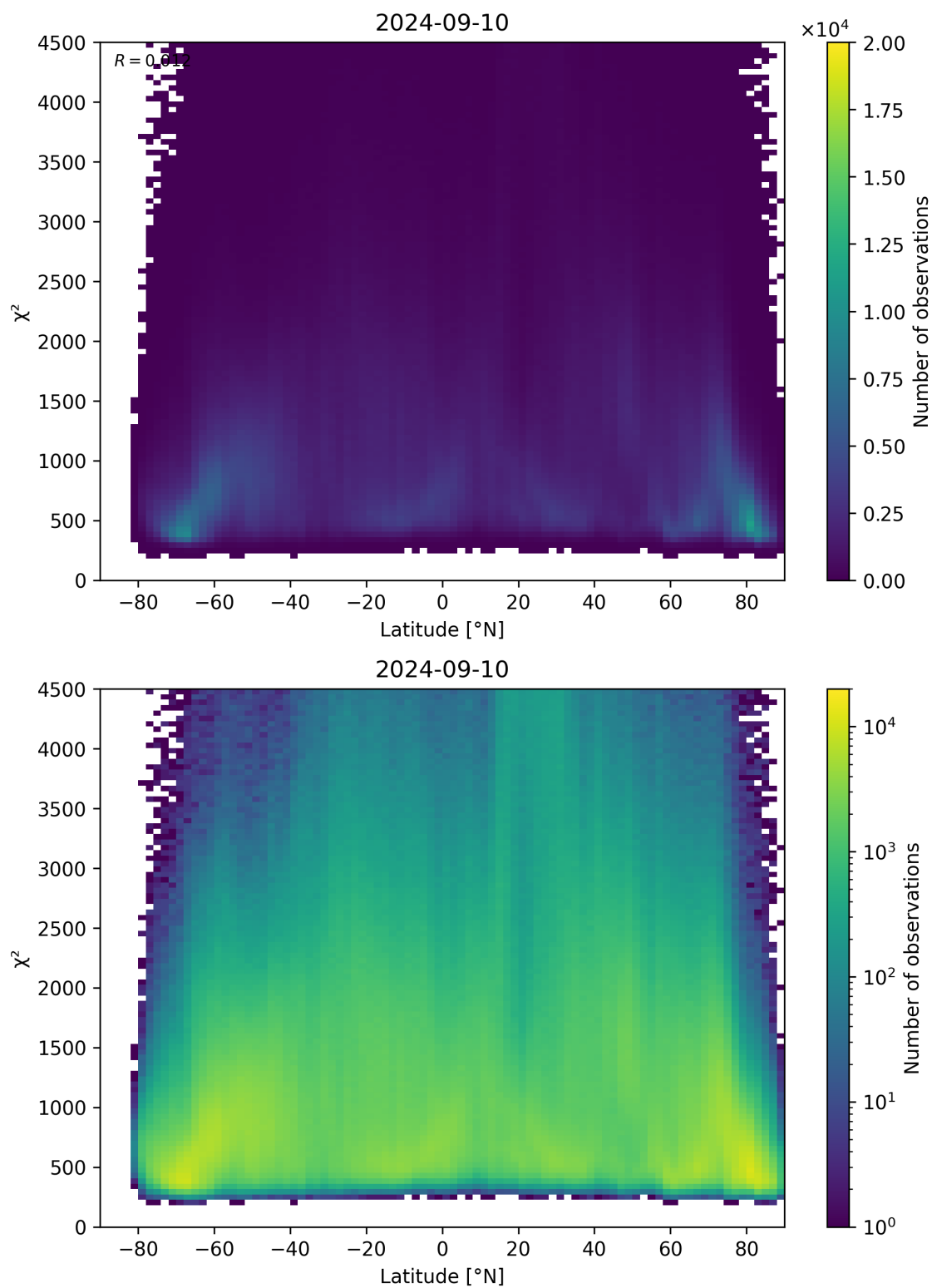
Figure 54: Scatter density plot of “Latitude” against “ \chi^2 ” for 2024-09-09 to 2024-09-11.
