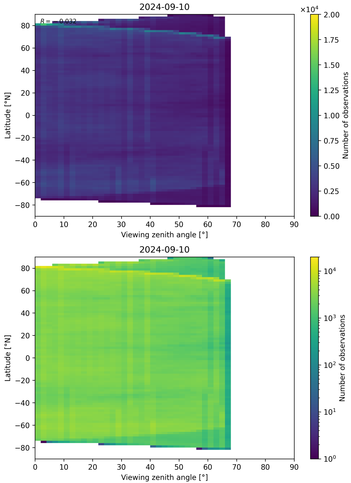
Figure 74: Scatter density plot of “Viewing zenith angle” against “Latitude” for 2024-09-09 to 2024-09-11.
