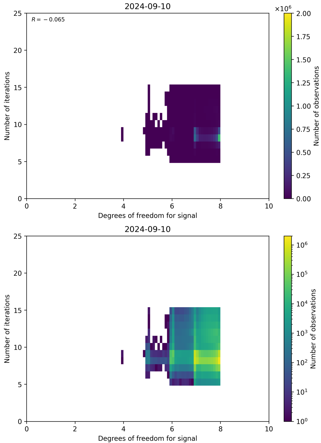
Figure 50: Scatter density plot of “Degrees of freedom for signal” against “Number of iterations” for 2024-09-09 to 2024-09-11.
