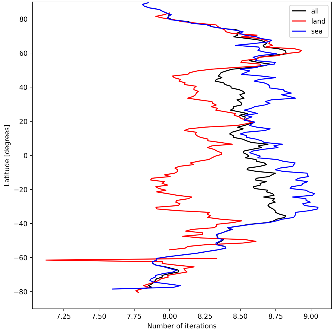
Figure 16: Zonal average of “Number of iterations” for 2024-09-09 to 2024-09-11.
