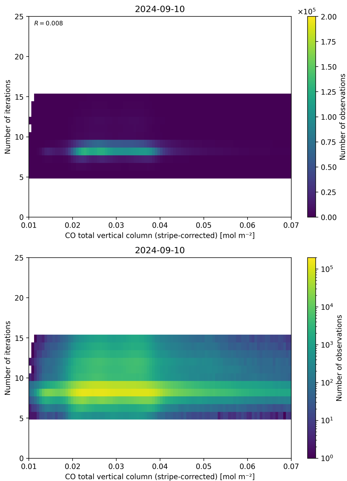
Figure 39: Scatter density plot of “CO total vertical column (stripe-corrected)” against “Number of iterations” for 2024-09-09 to 2024-09-11.
