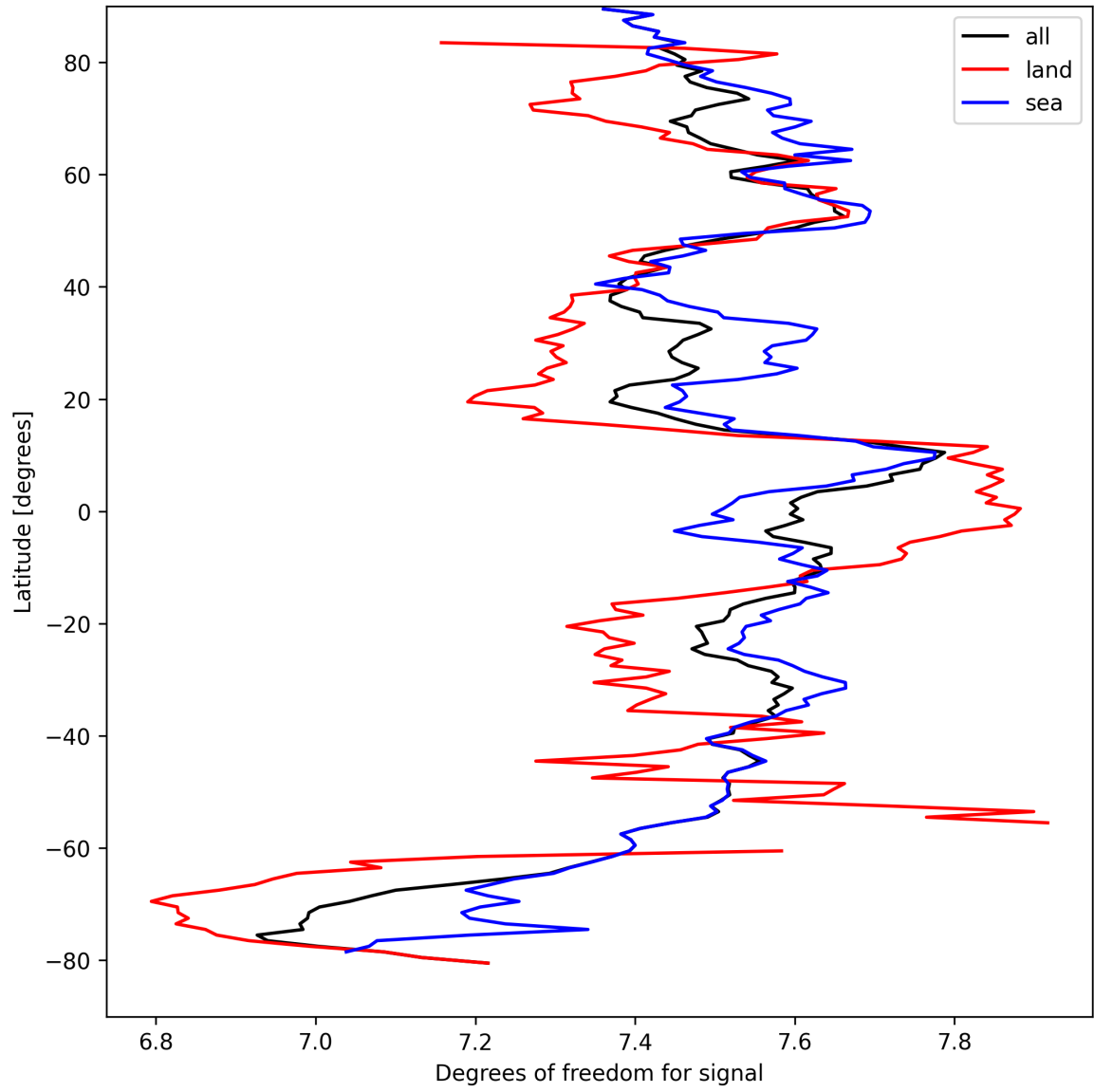
Figure 15: Zonal average of “Degrees of freedom for signal” for 2024-09-09 to 2024-09-11.
