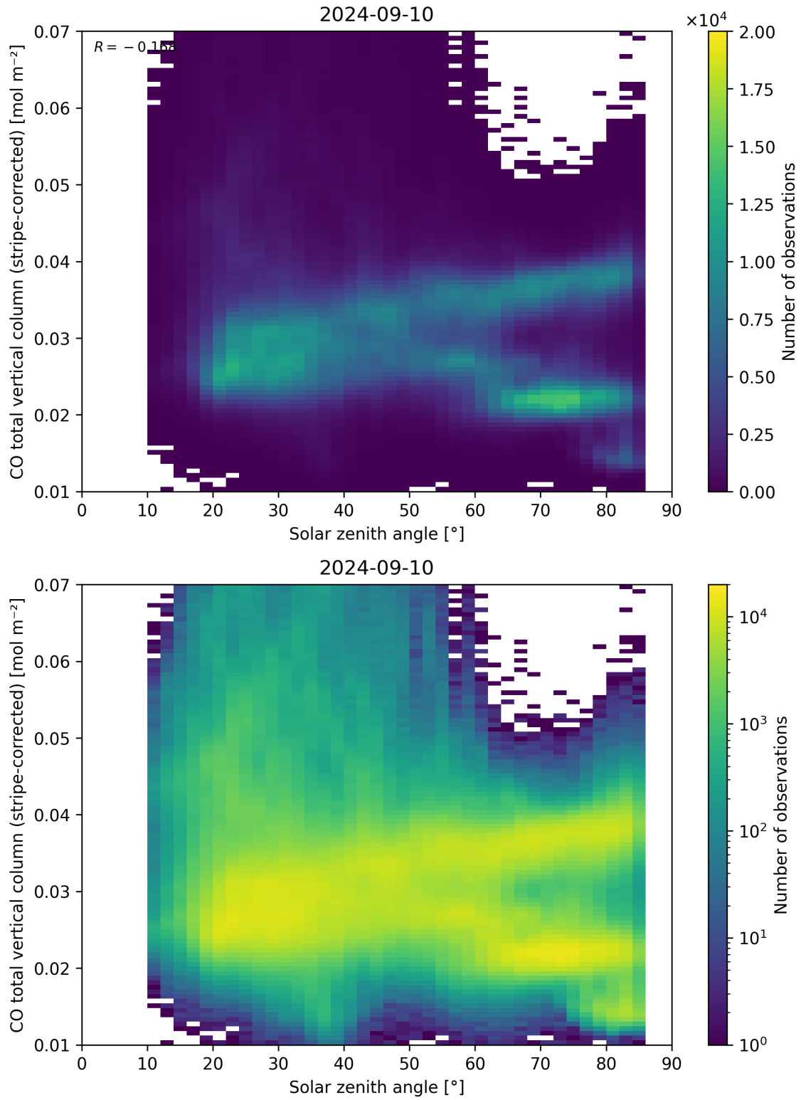
Figure 62: Scatter density plot of “Solar zenith angle” against “CO total vertical column (stripe-corrected)” for 2024-09-09 to 2024-09-11.
