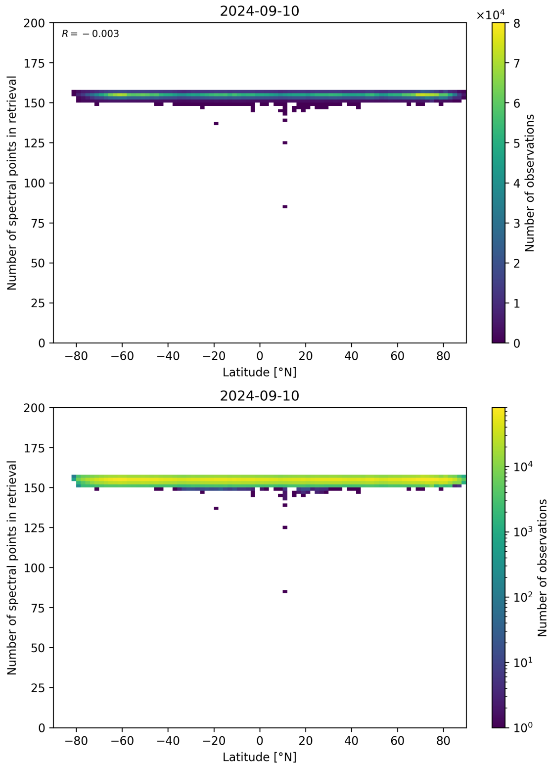
Figure 57: Scatter density plot of “Latitude” against “Number of spectral points in retrieval” for 2024-09-09 to 2024-09-11.
