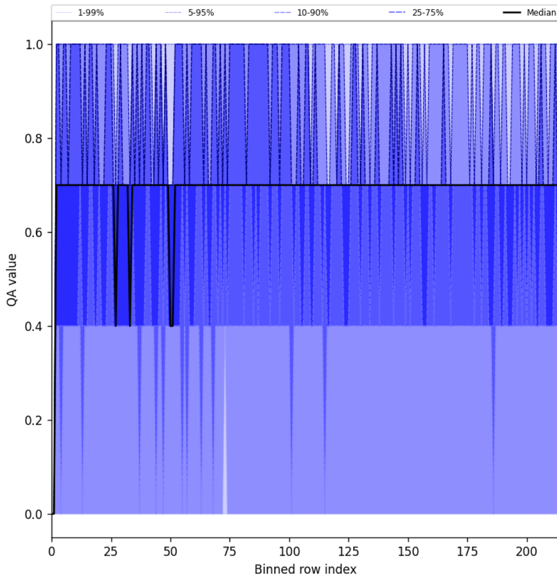
Figure 25: Along track statistics of “QA value” for 2024-09-09 to 2024-09-11
