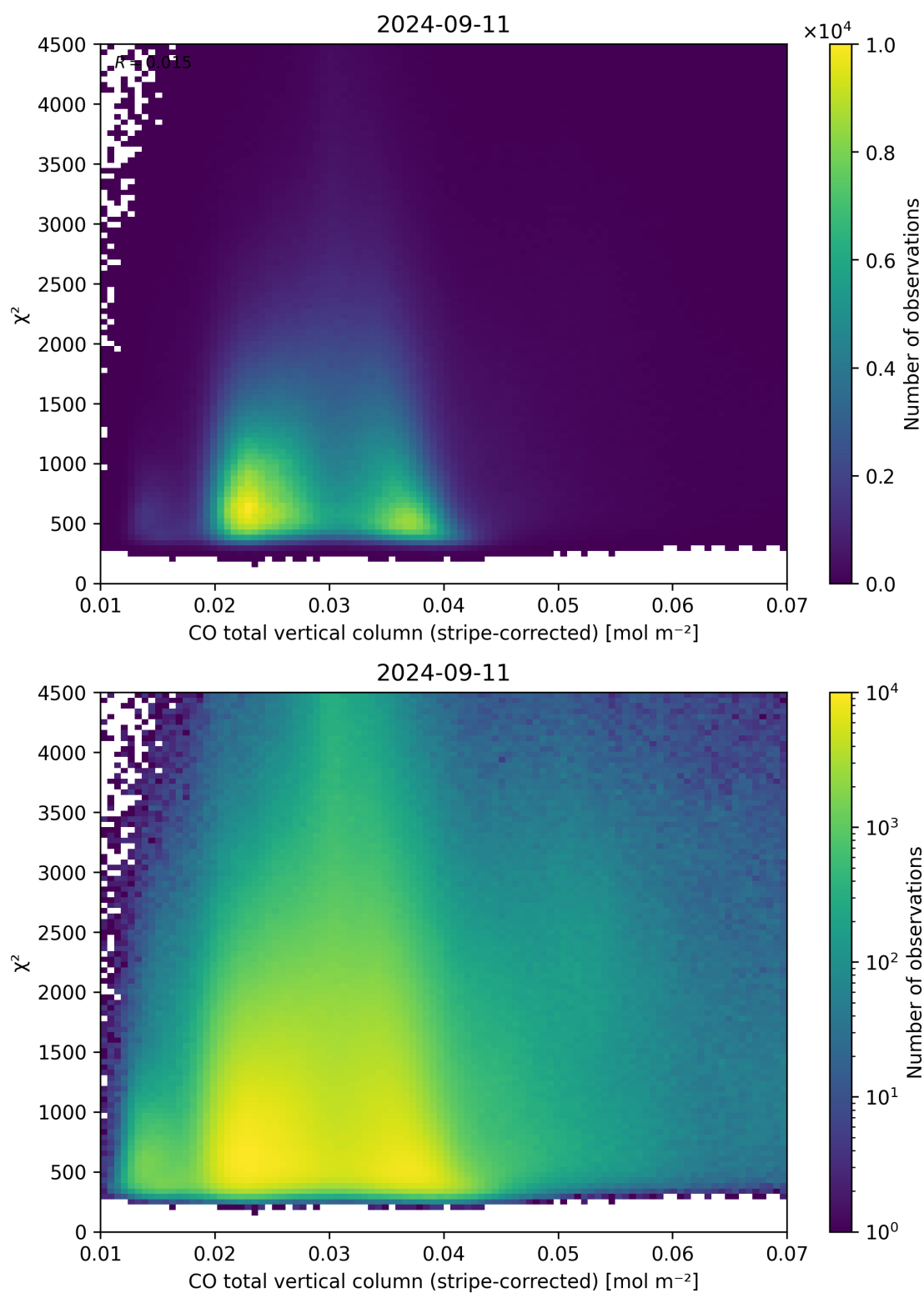
Figure 37: Scatter density plot of “CO total vertical column (stripe-corrected)” against “ \chi^2 ” for 2024-09-10 to 2024-09-12.
