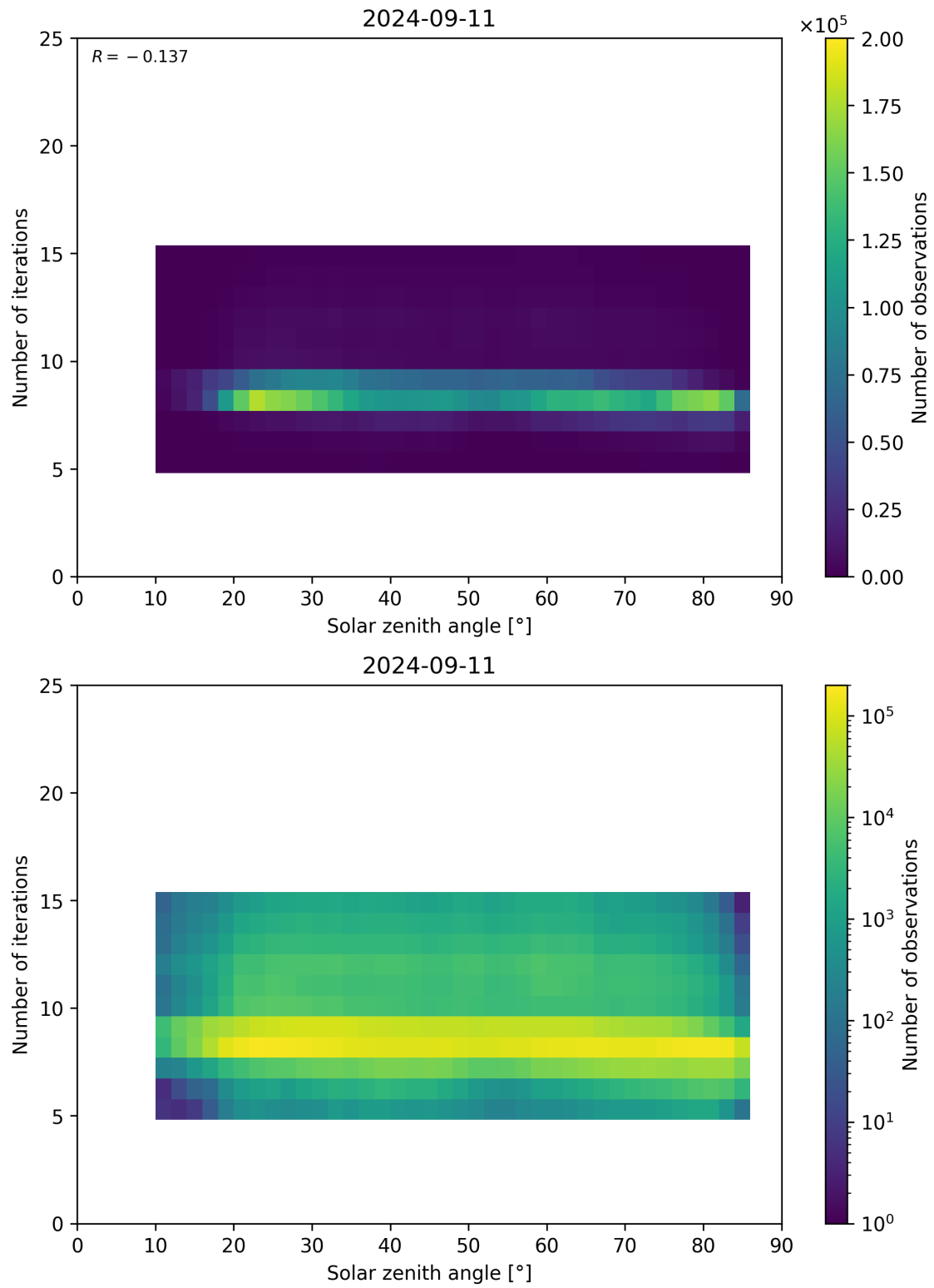
Figure 67: Scatter density plot of “Solar zenith angle” against “Number of iterations” for 2024-09-10 to 2024-09-12.
