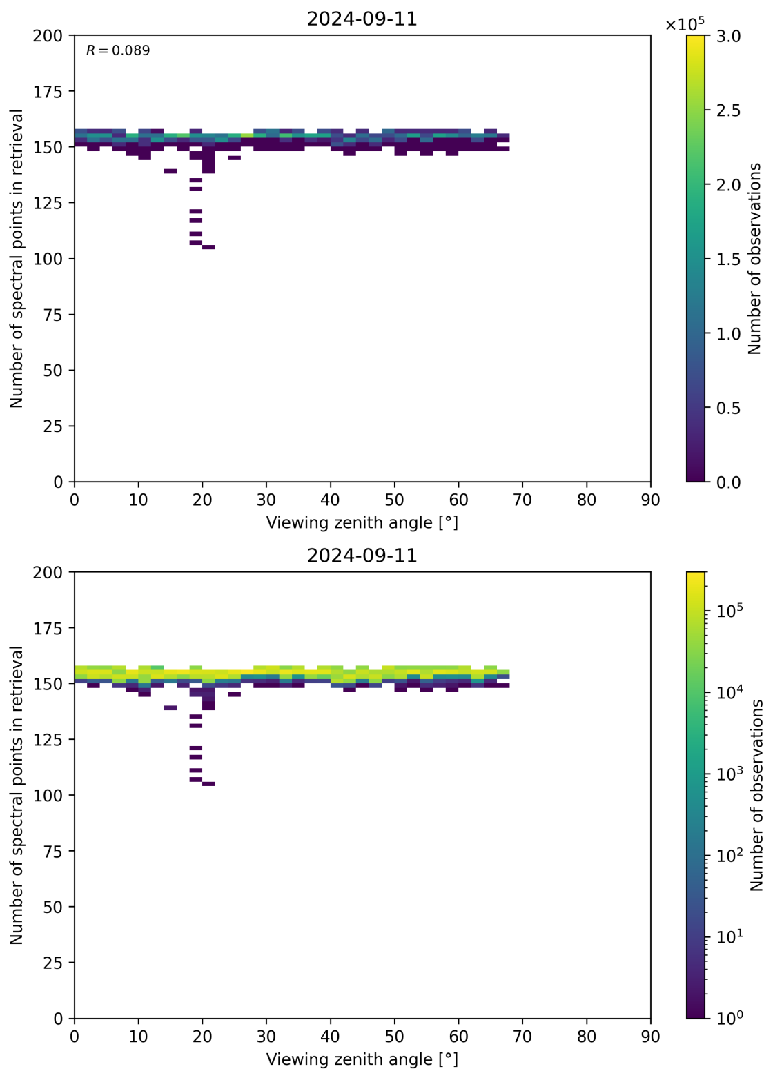
Figure 76: Scatter density plot of “Viewing zenith angle” against “Number of spectral points in retrieval” for 2024-09-10 to 2024-09-12.
