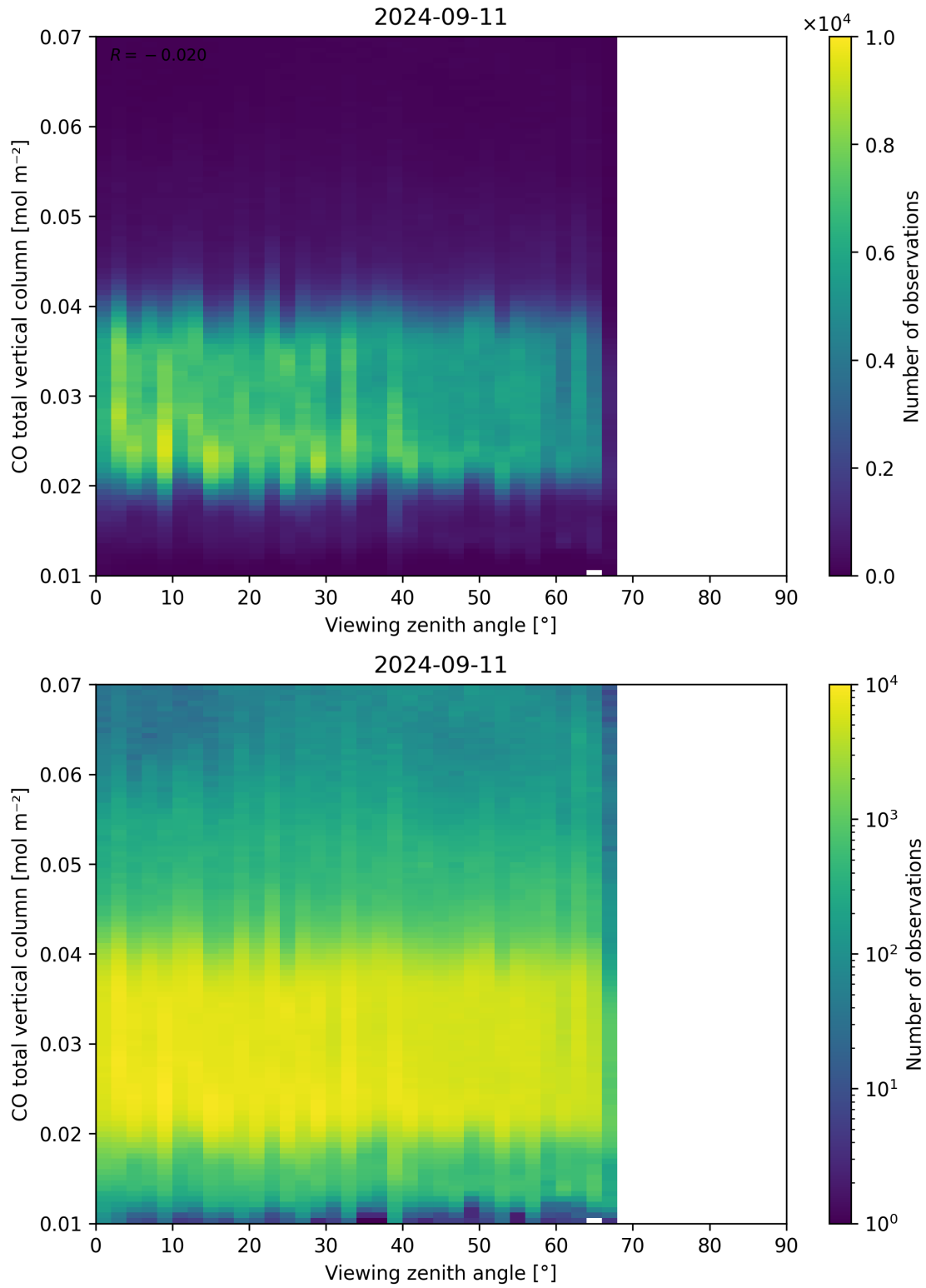
Figure 69: Scatter density plot of “Viewing zenith angle” against “CO total vertical column” for 2024-09-10 to 2024-09-12.
