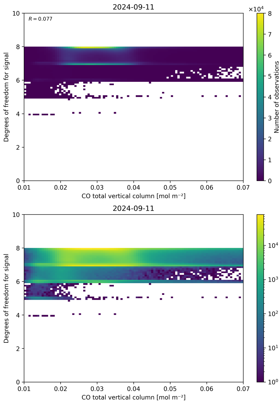
Figure 41: Scatter density plot of “CO total vertical column” against “Degrees of freedom for signal” for 2024-09-10 to 2024-09-12.
