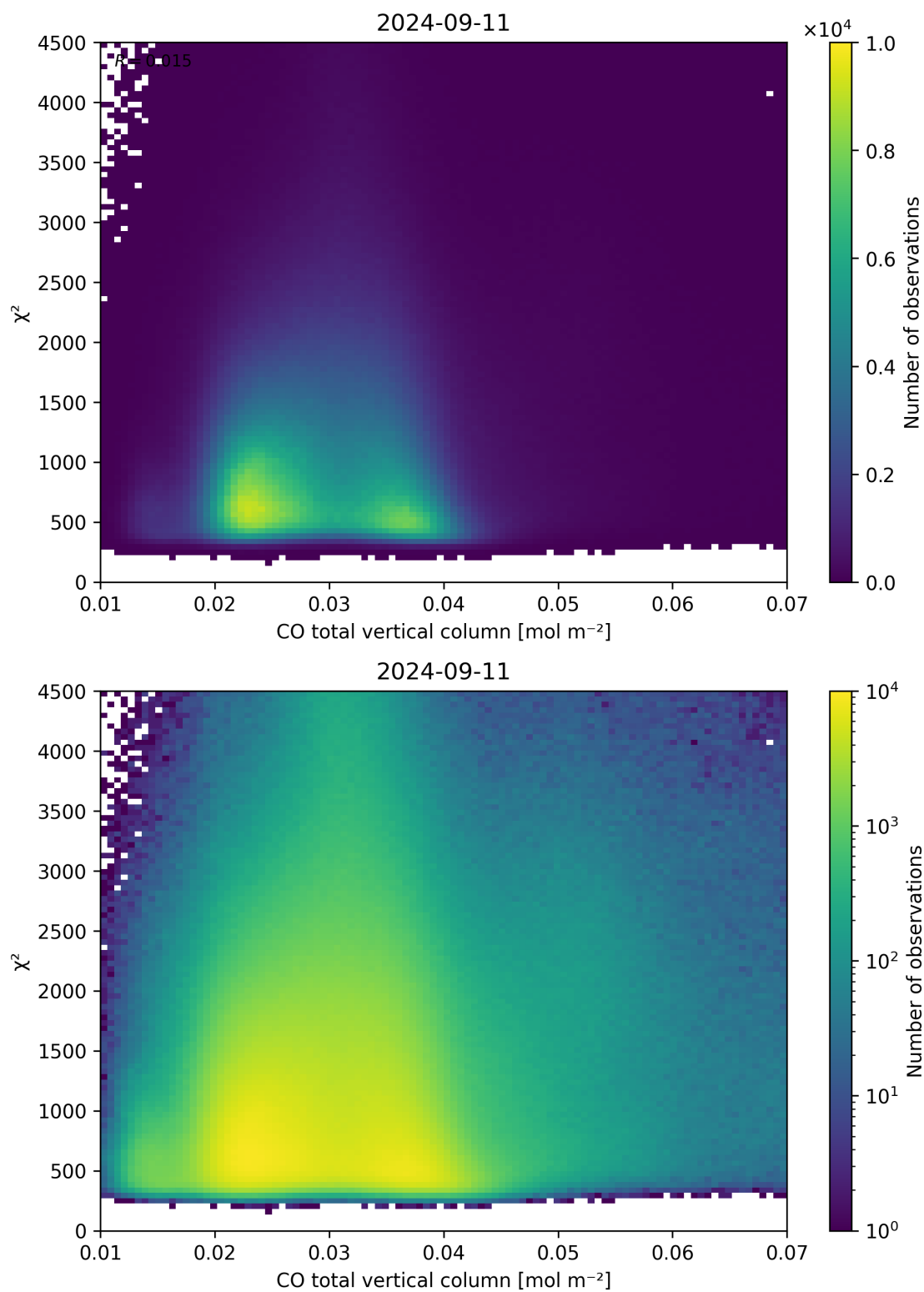
Figure 35: Scatter density plot of “CO total vertical column” against “ \chi^2 ” for 2024-09-10 to 2024-09-12.
