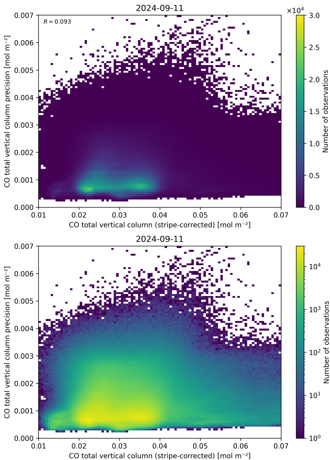
Figure 36: Scatter density plot of “CO total vertical column (stripe-corrected)” against “CO total vertical column precision” for 2024-09-10 to 2024-09-12.
