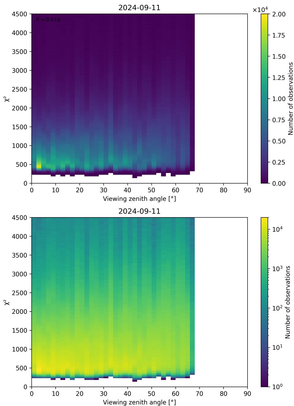
Figure 72: Scatter density plot of “Viewing zenith angle” against “ \chi^2 ” for 2024-09-10 to 2024-09-12.
