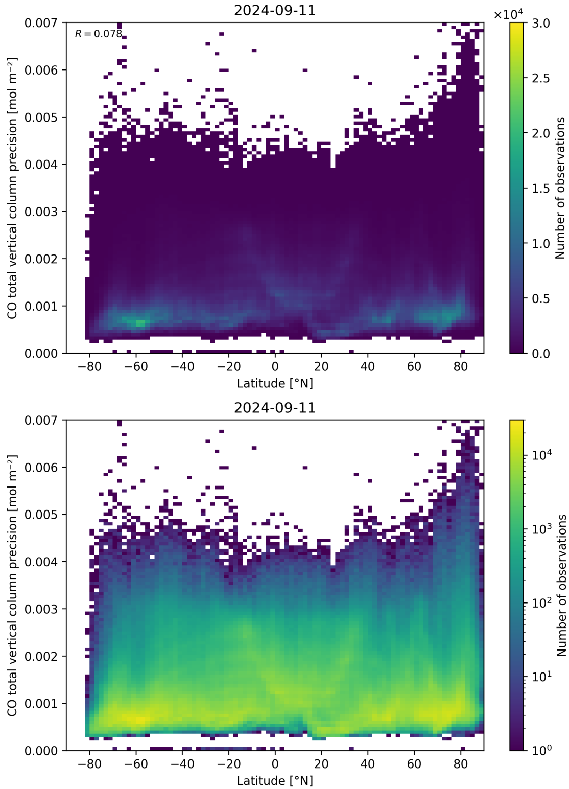
Figure 53: Scatter density plot of “Latitude” against “CO total vertical column precision” for 2024-09-10 to 2024-09-12.
