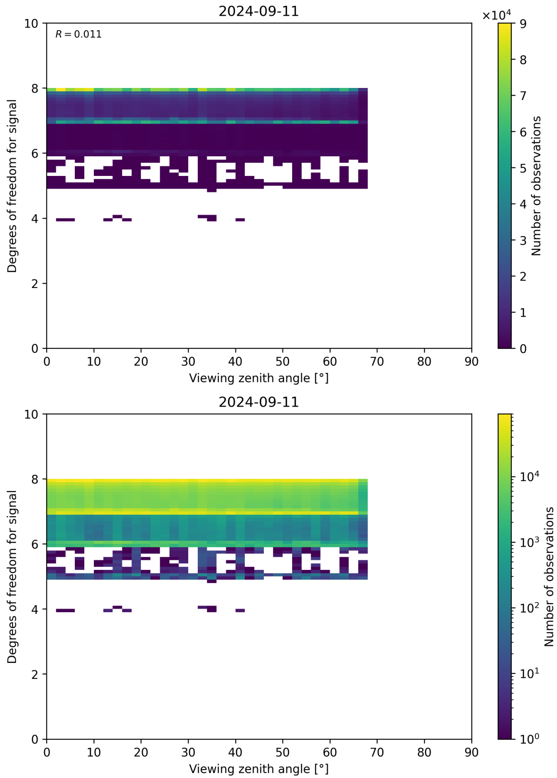
Figure 73: Scatter density plot of “Viewing zenith angle” against “Degrees of freedom for signal” for 2024-09-10 to 2024-09-12.
