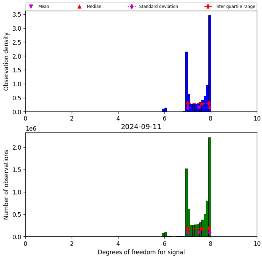
Figure 23: Histogram of “Degrees of freedom for signal” for 2024-09-10 to 2024-09-12
