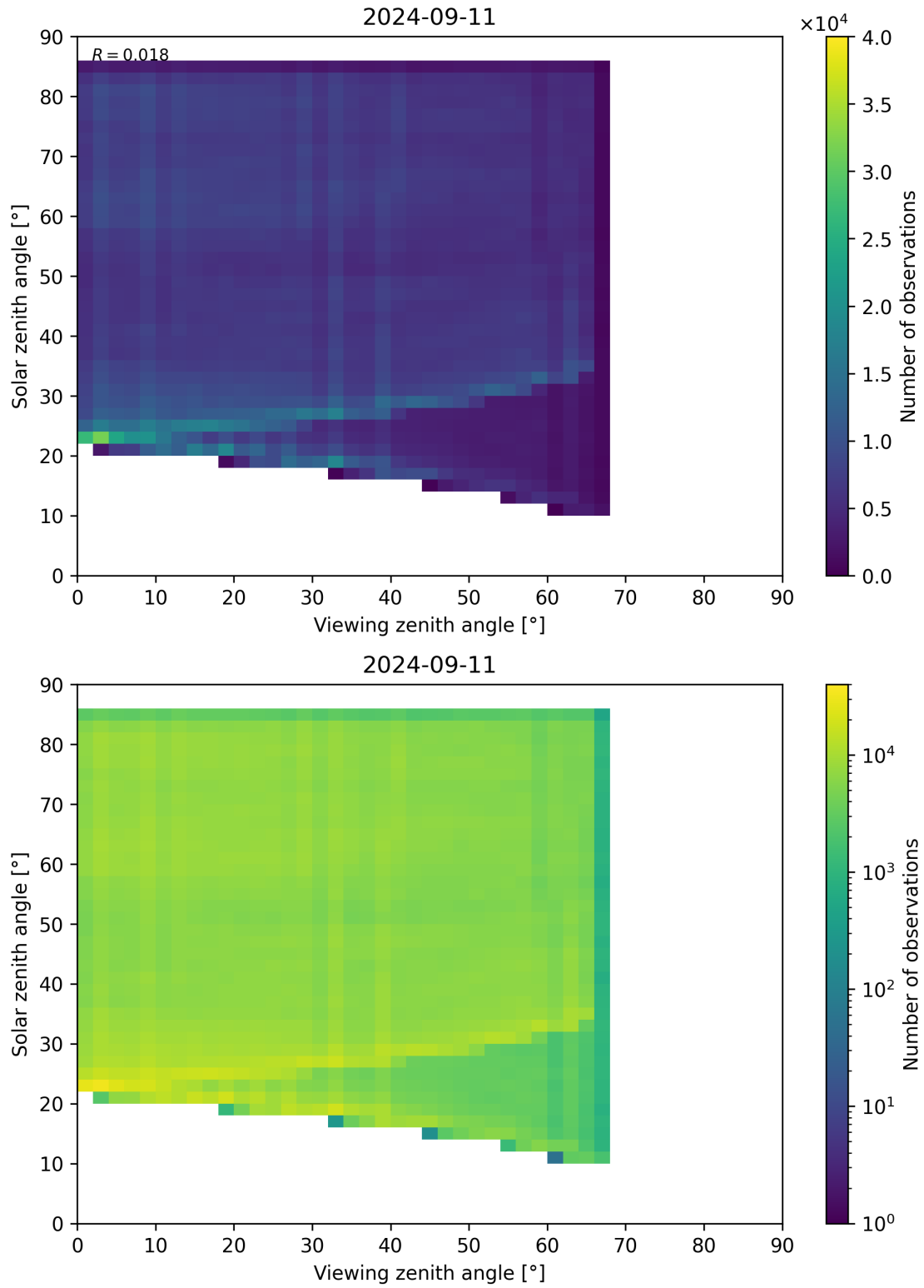
Figure 77: Scatter density plot of “Viewing zenith angle” against “Solar zenith angle” for 2024-09-10 to 2024-09-12.
