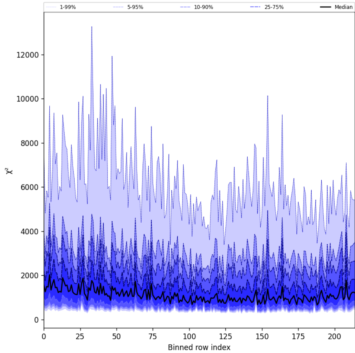
Figure 30: Along track statistics of “ \chi^2 ” for 2024-09-10 to 2024-09-12
