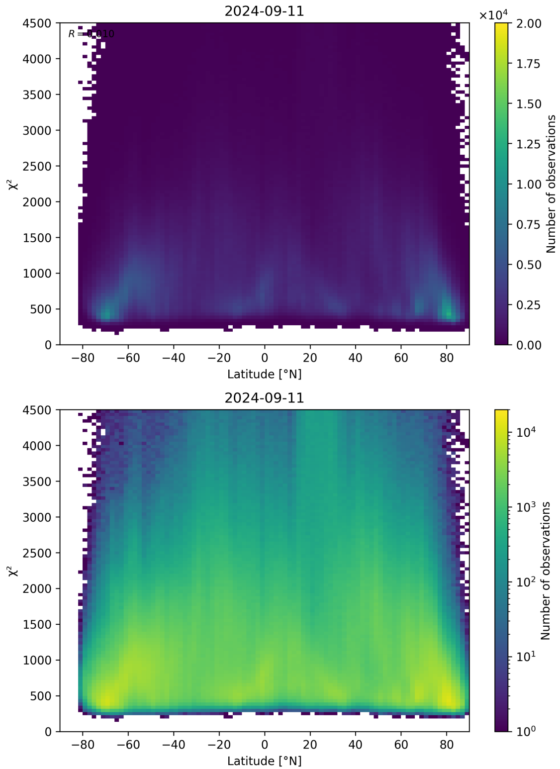
Figure 54: Scatter density plot of “Latitude” against “ \chi^2 ” for 2024-09-10 to 2024-09-12.
