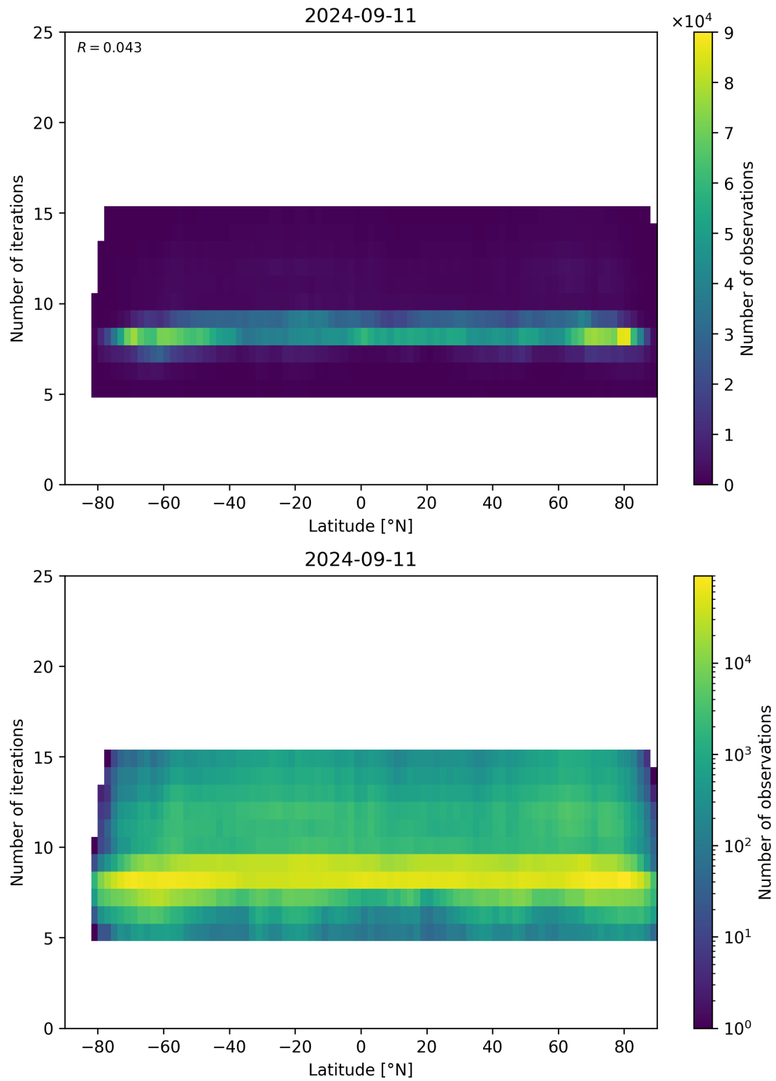
Figure 56: Scatter density plot of “Latitude” against “Number of iterations” for 2024-09-10 to 2024-09-12.
