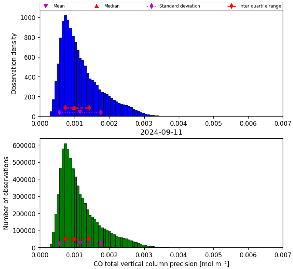
Figure 20: Histogram of “CO total vertical column precision” for 2024-09-10 to 2024-09-12
