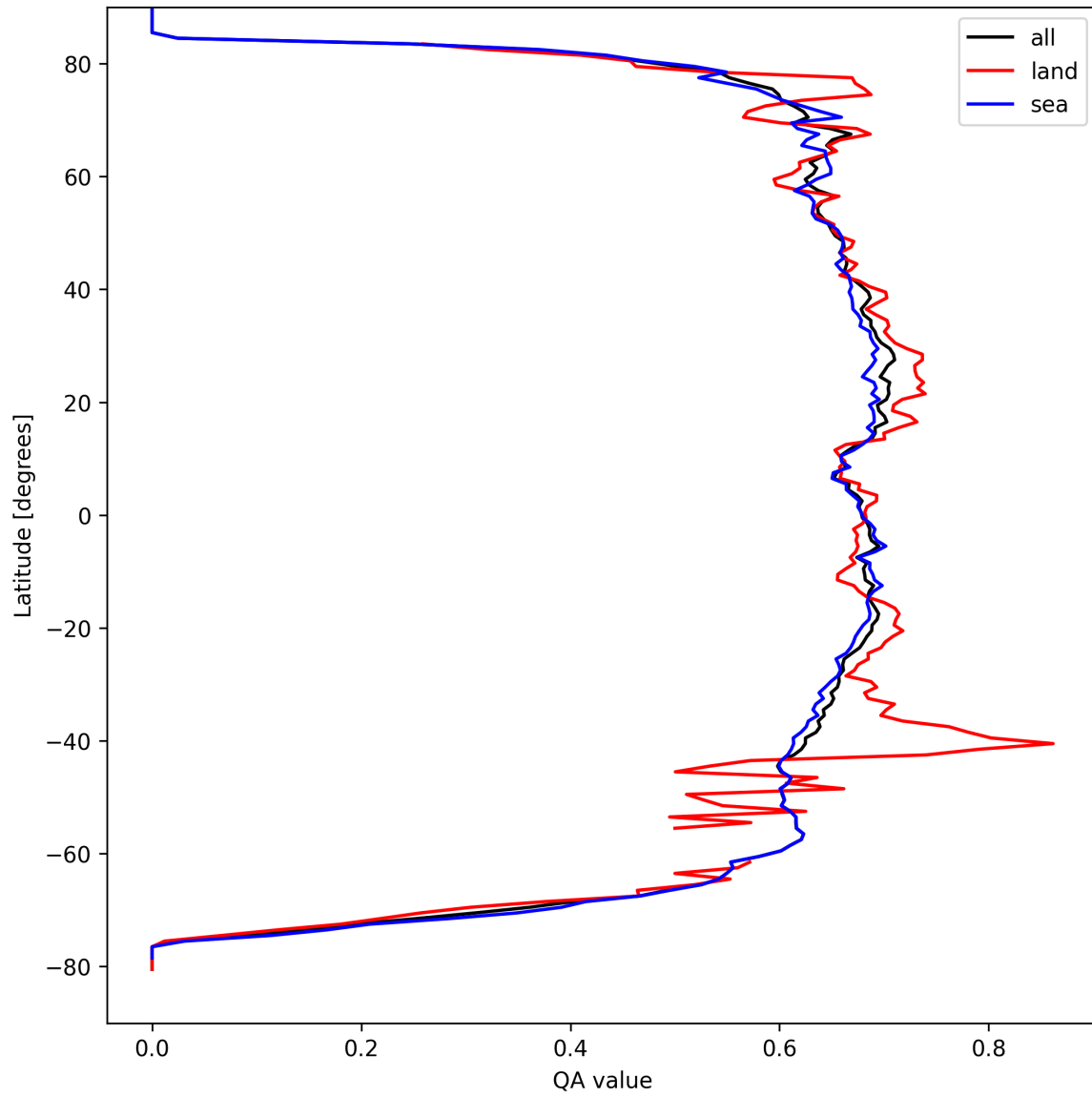
Figure 9: Zonal average of “QA value” for 2024-09-10 to 2024-09-12.
