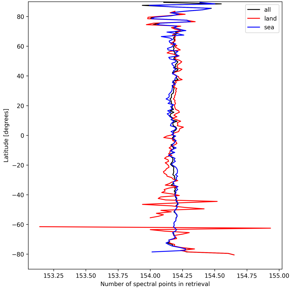
Figure 13: Zonal average of “Number of spectral points in retrieval” for 2024-09-10 to 2024-09-12.
