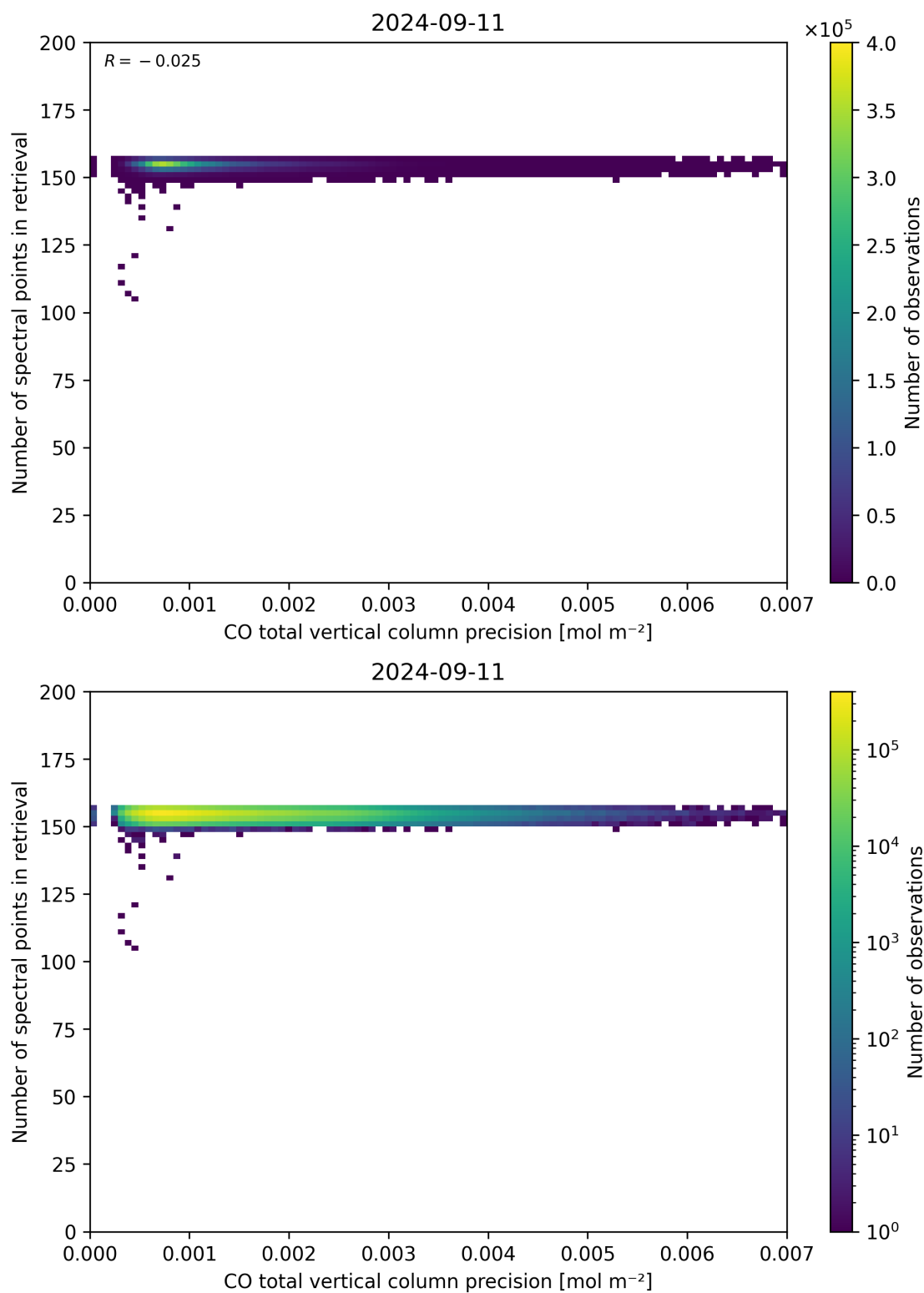
Figure 47: Scatter density plot of “CO total vertical column precision” against “Number of spectral points in retrieval” for 2024-09-10 to 2024-09-12.
