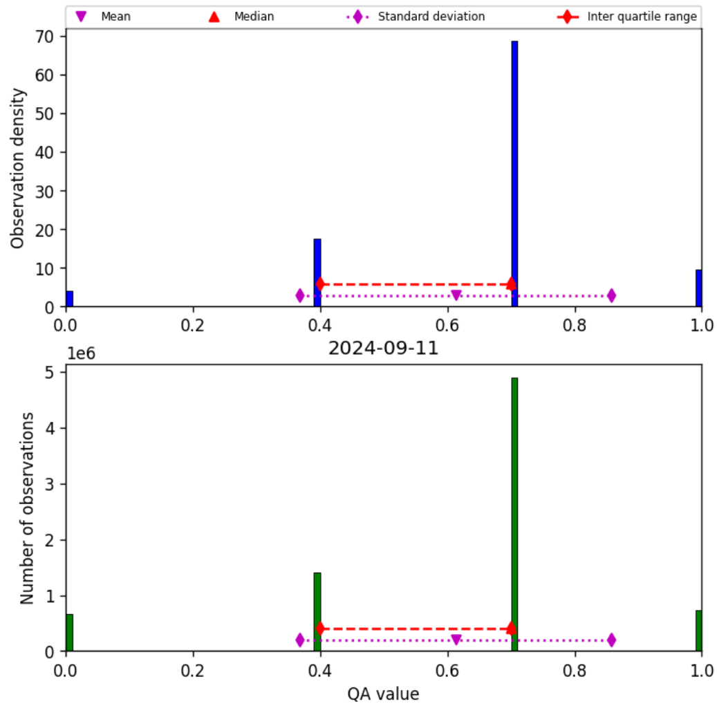
Figure 17: Histogram of “QA value” for 2024-09-10 to 2024-09-12
