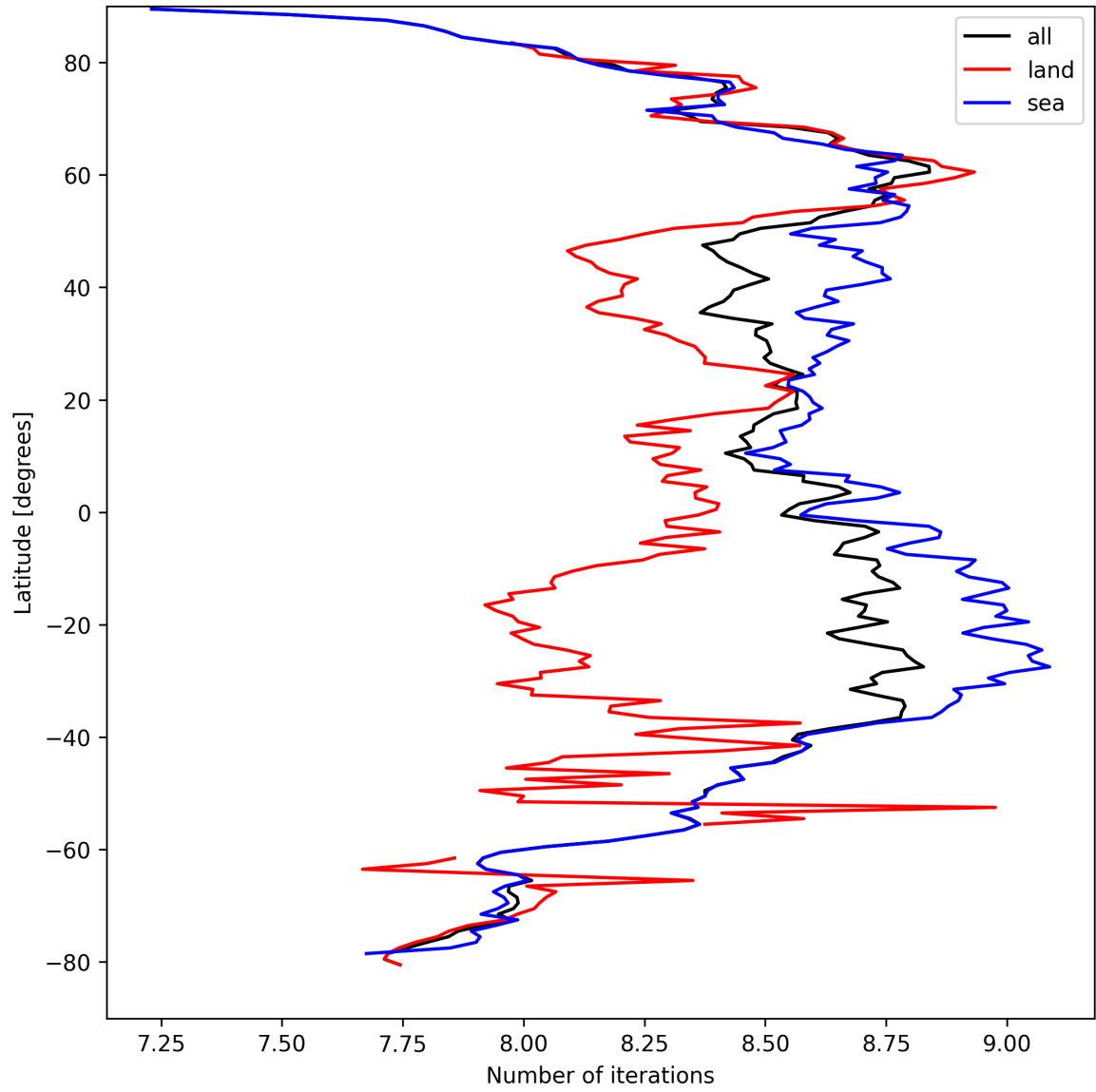
Figure 16: Zonal average of “Number of iterations” for 2024-09-10 to 2024-09-12.
