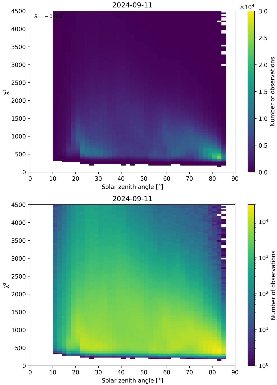
Figure 64: Scatter density plot of “Solar zenith angle” against “ \chi^2 ” for 2024-09-10 to 2024-09-12.
