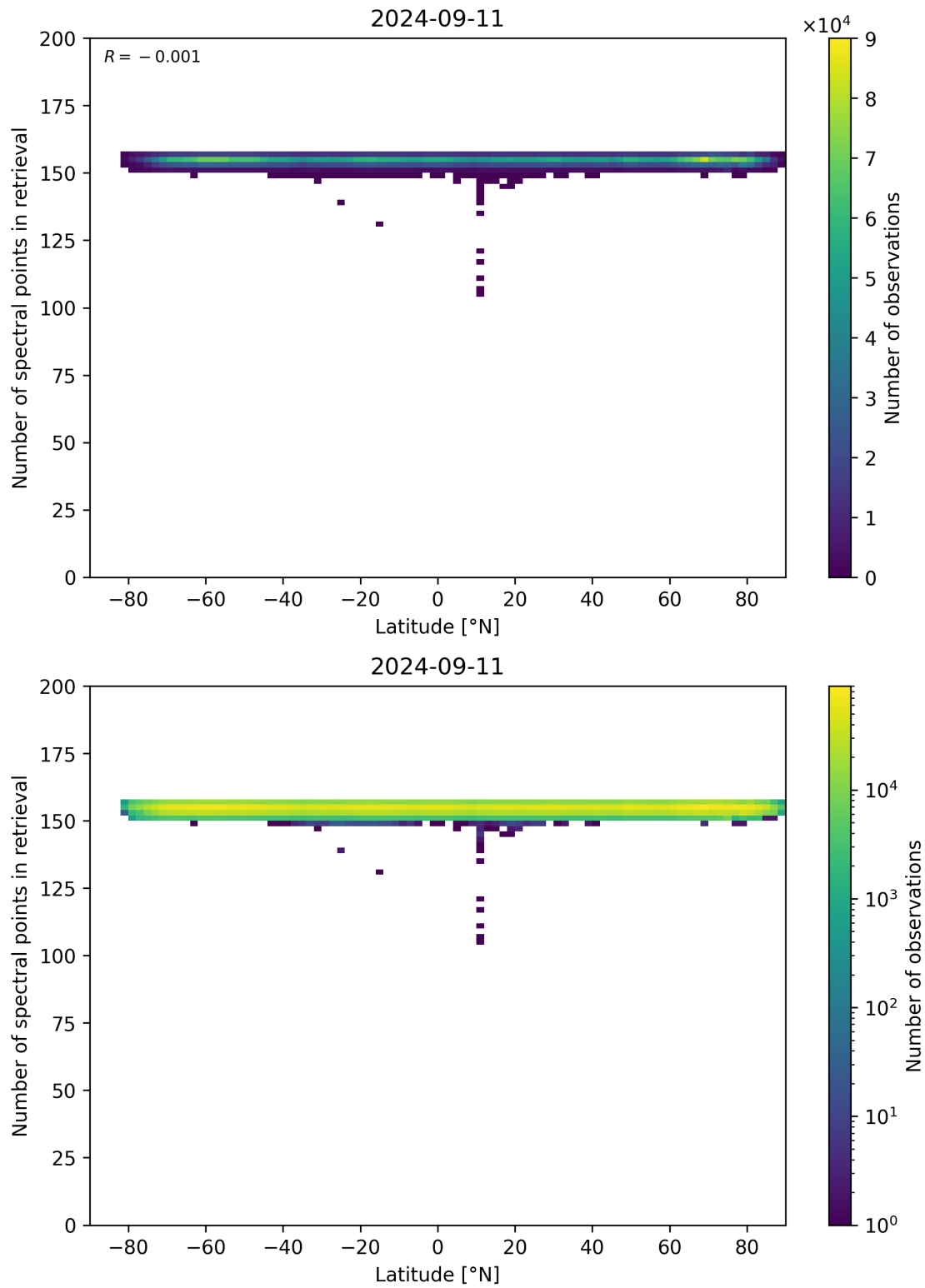
Figure 57: Scatter density plot of “Latitude” against “Number of spectral points in retrieval” for 2024-09-10 to 2024-09-12.
