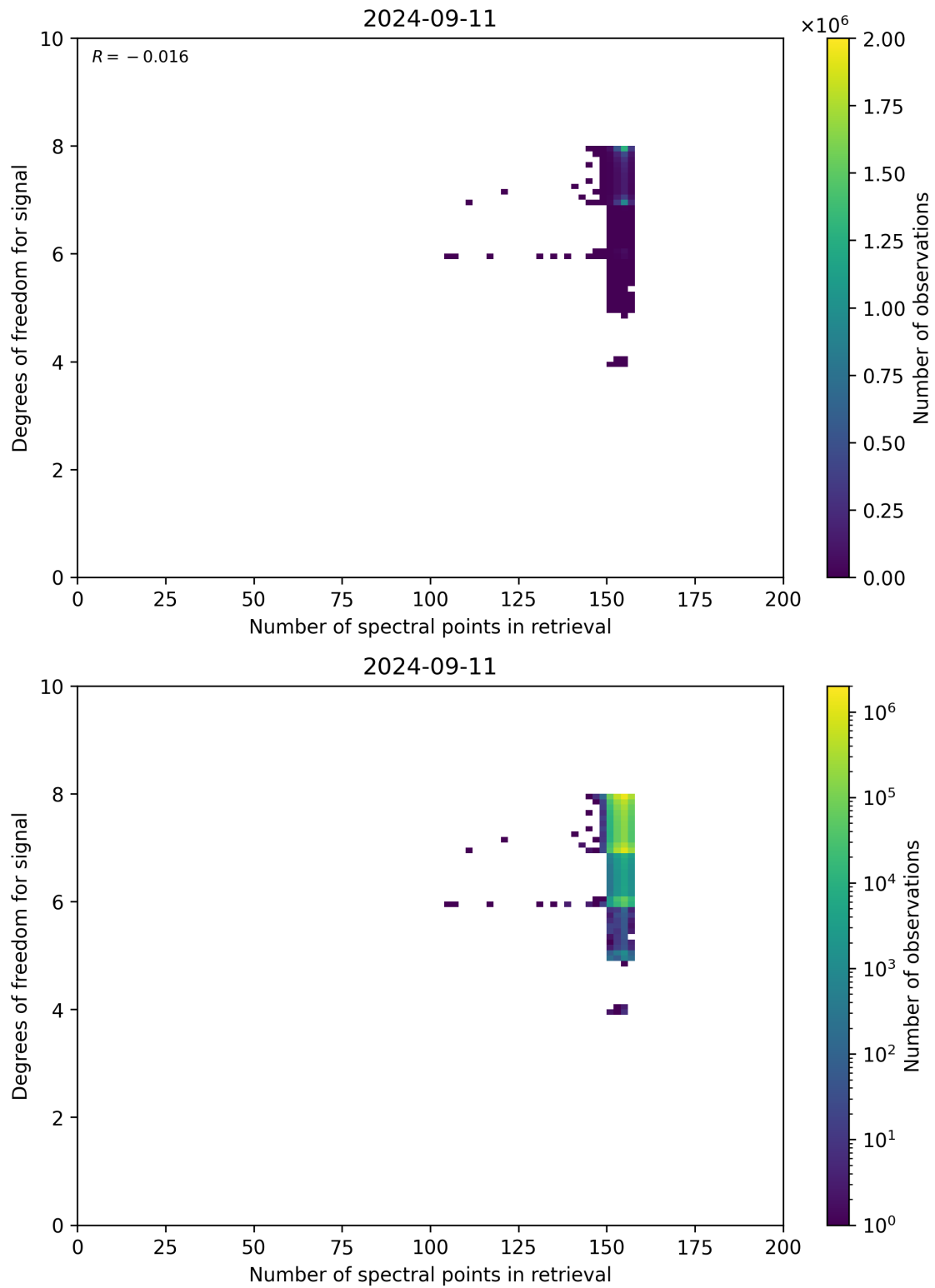
Figure 59: Scatter density plot of “Number of spectral points in retrieval” against “Degrees of freedom for signal” for 2024-09-10 to 2024-09-12.
