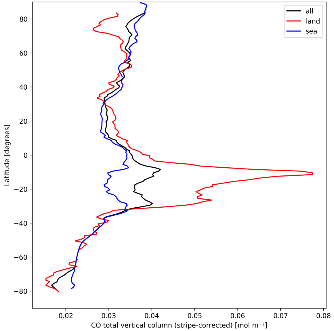
Figure 11: Zonal average of “CO total vertical column (stripe-corrected)” for 2024-09-10 to 2024-09-12.
