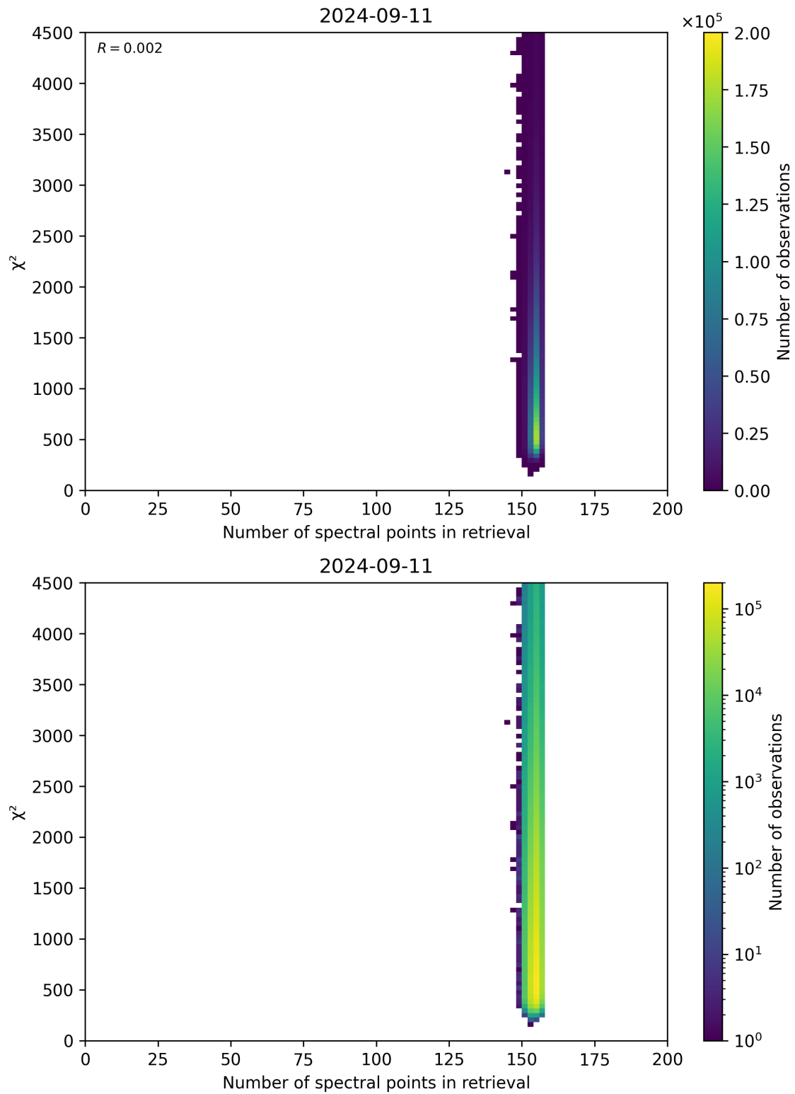
Figure 58: Scatter density plot of “Number of spectral points in retrieval” against “ \chi^2 ” for 2024-09-10 to 2024-09-12.
