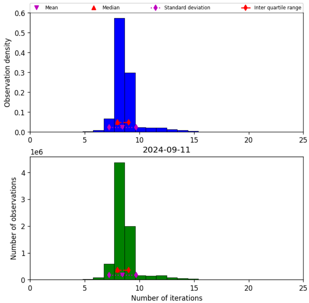
Figure 24: Histogram of “Number of iterations” for 2024-09-10 to 2024-09-12
