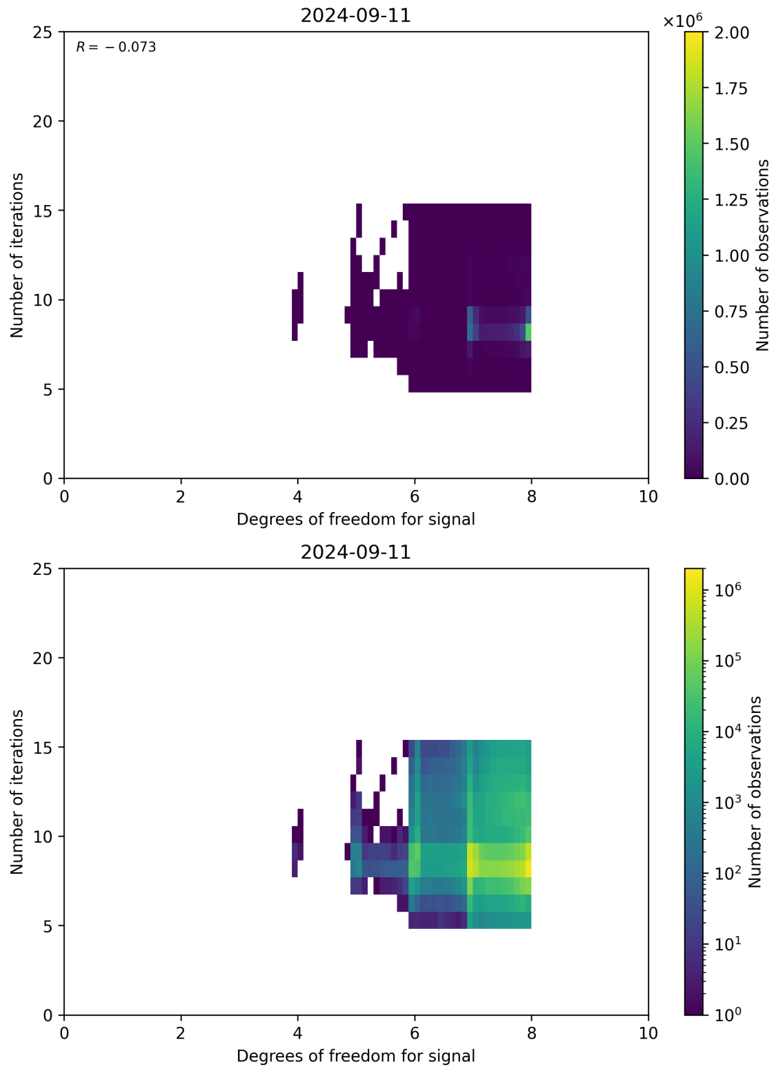
Figure 50: Scatter density plot of “Degrees of freedom for signal” against “Number of iterations” for 2024-09-10 to 2024-09-12.
