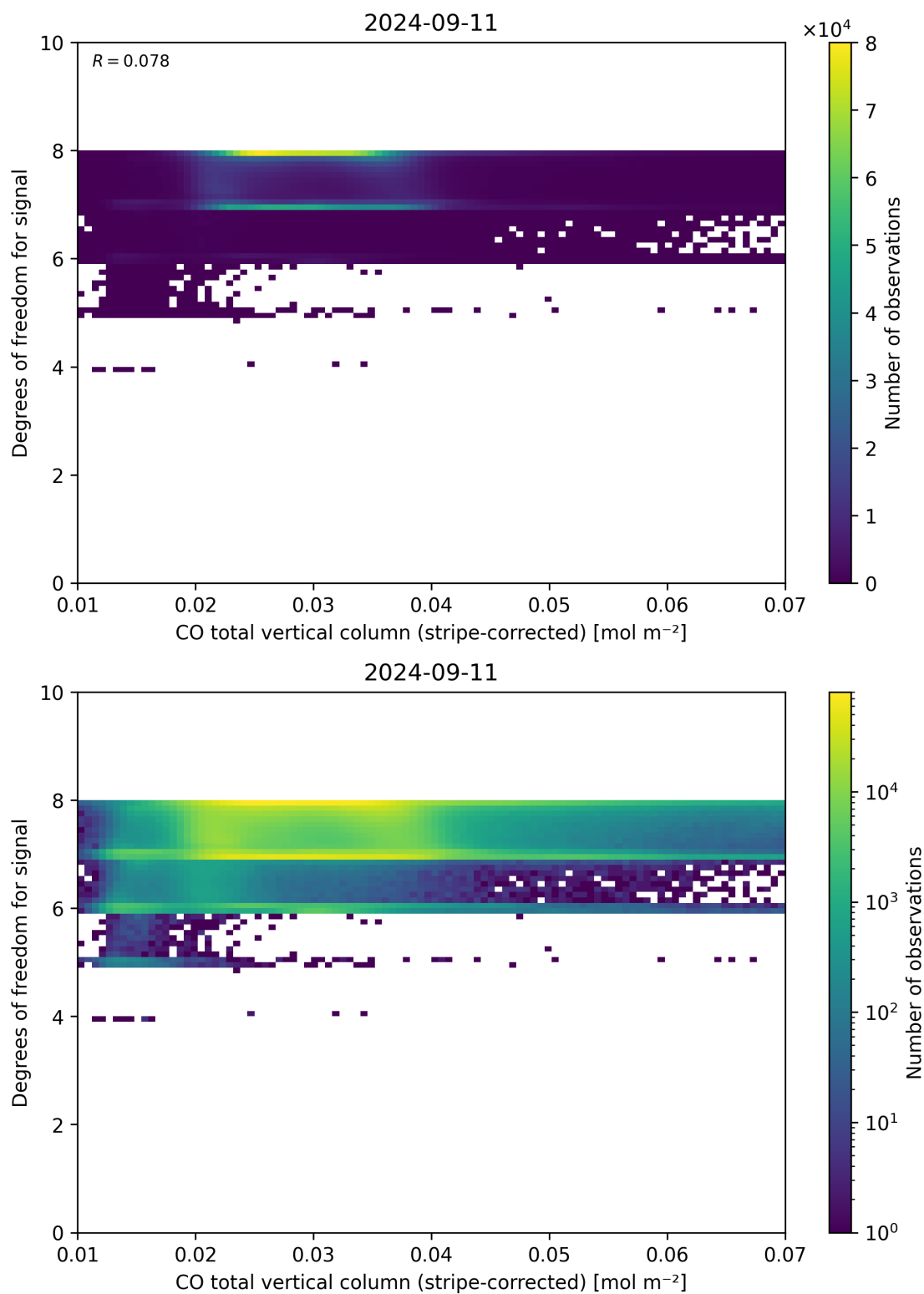
Figure 38: Scatter density plot of “CO total vertical column (stripe-corrected)” against “Degrees of freedom for signal” for 2024-09-10 to 2024-09-12.
