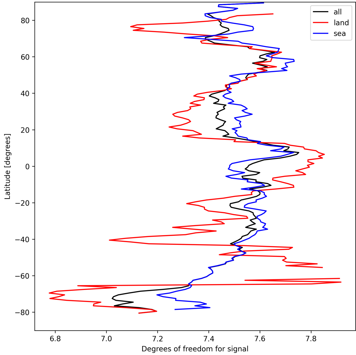
Figure 15: Zonal average of “Degrees of freedom for signal” for 2024-09-10 to 2024-09-12.
