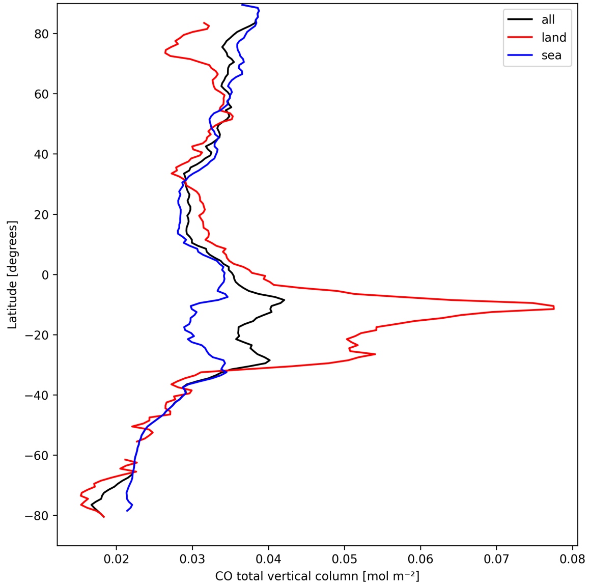
Figure 10: Zonal average of “CO total vertical column” for 2024-09-10 to 2024-09-12.
