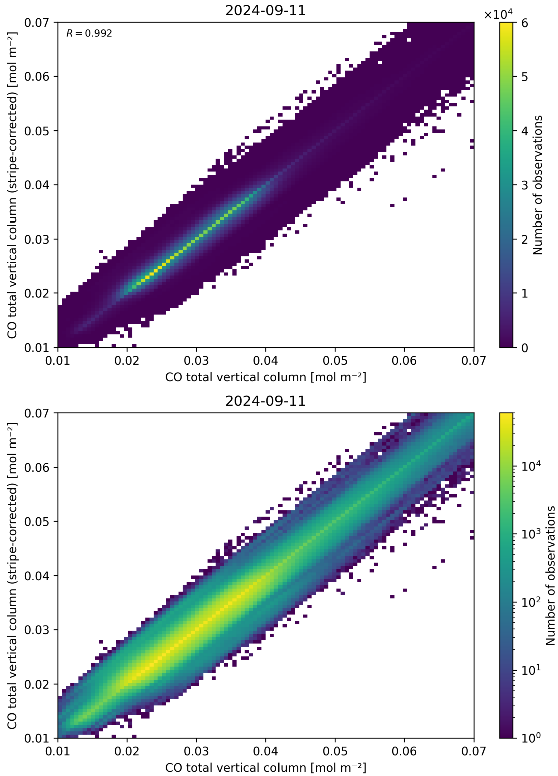
Figure 33: Scatter density plot of “CO total vertical column” against “CO total vertical column (stripe-corrected)” for 2024-09-10 to 2024-09-12.
