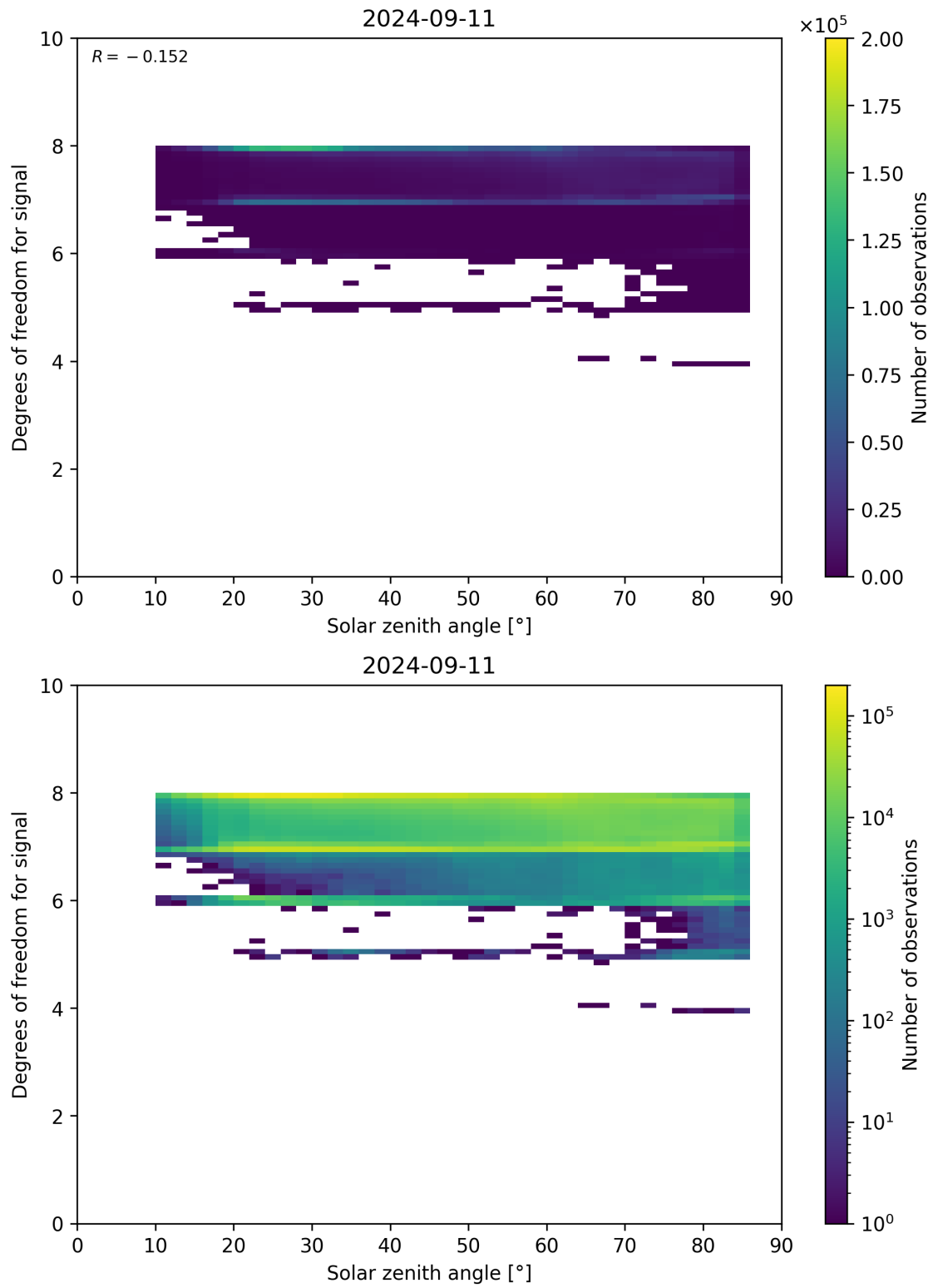
Figure 65: Scatter density plot of “Solar zenith angle” against “Degrees of freedom for signal” for 2024-09-10 to 2024-09-12.
