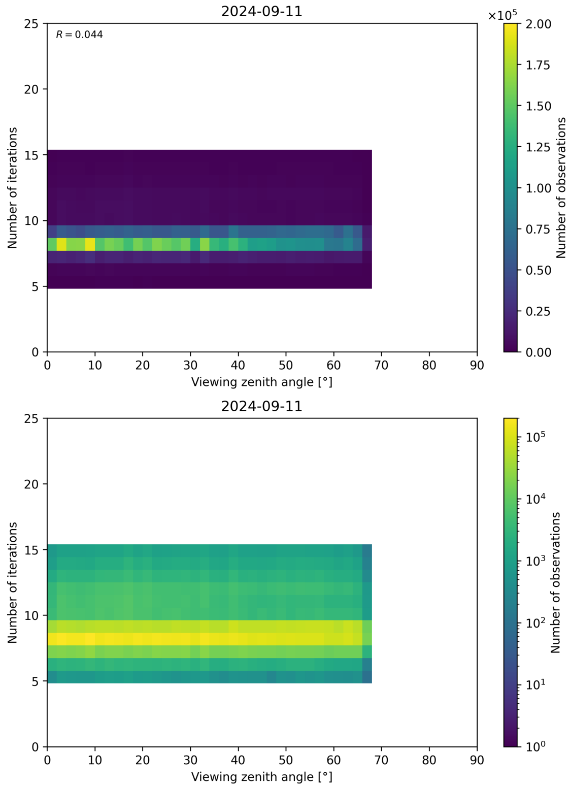
Figure 75: Scatter density plot of “Viewing zenith angle” against “Number of iterations” for 2024-09-10 to 2024-09-12.
