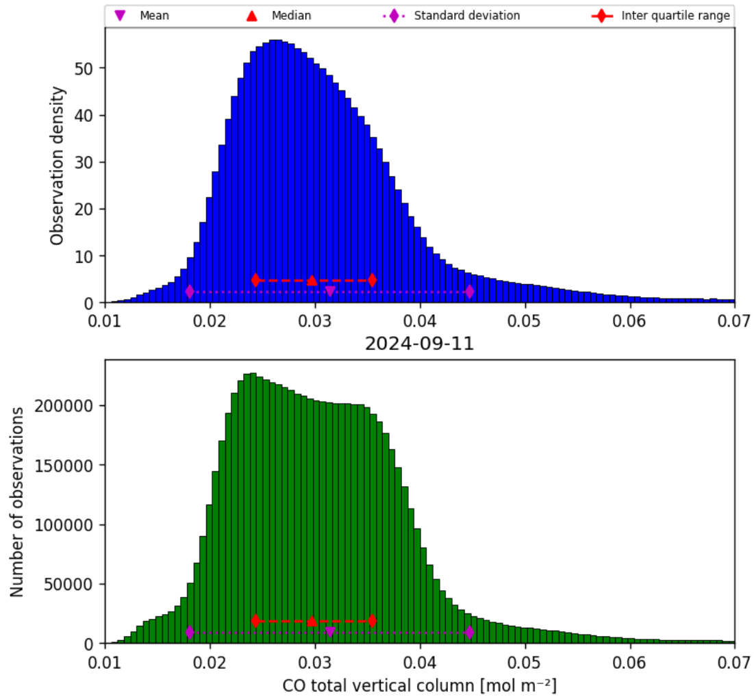
Figure 18: Histogram of “CO total vertical column” for 2024-09-10 to 2024-09-12
