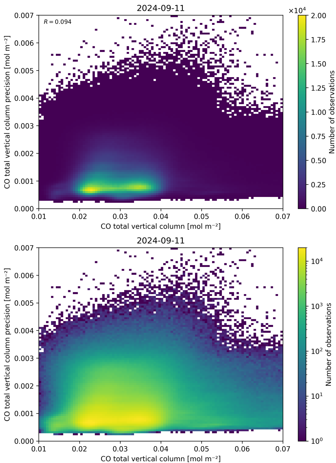
Figure 34: Scatter density plot of “CO total vertical column” against “CO total vertical column precision” for 2024-09-10 to 2024-09-12.
