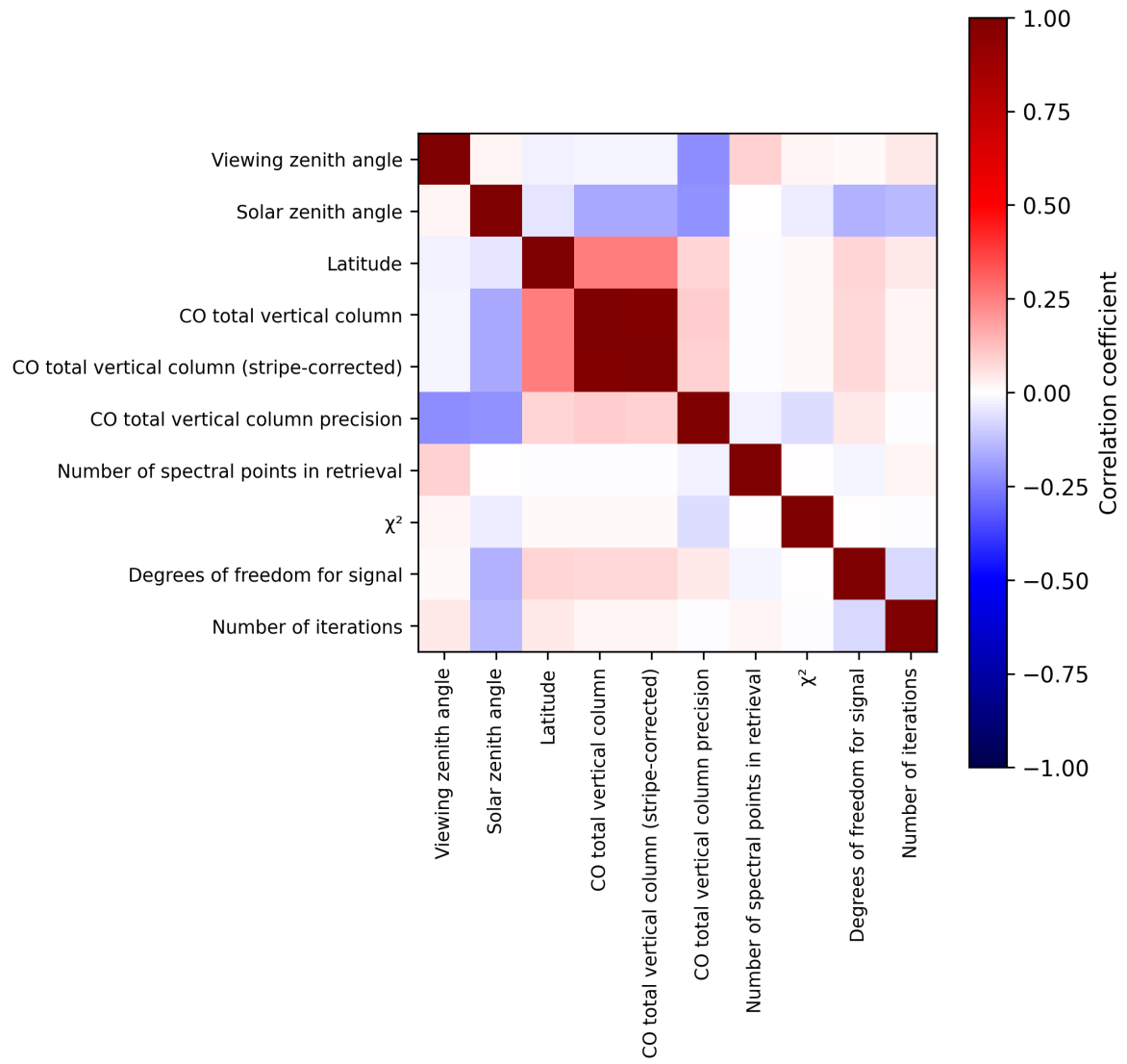
Figure 2: Map of correlation matrix for 2024-09-10 to 2024-09-12.
