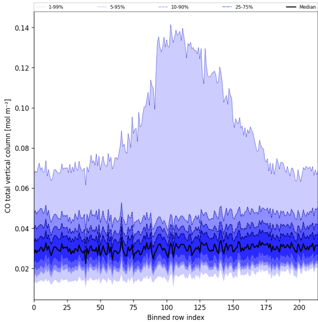
Figure 26: Along track statistics of “CO total vertical column” for 2024-09-10 to 2024-09-12
