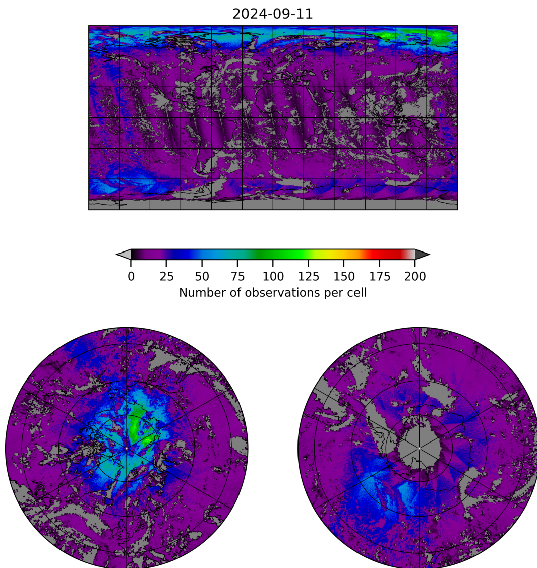
Figure 8: Map of the number of observations for 2024-09-10 to 2024-09-12
