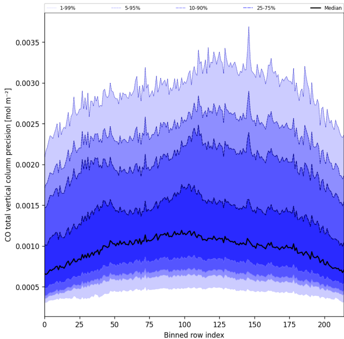
Figure 28: Along track statistics of “CO total vertical column precision” for 2024-09-10 to 2024-09-12
