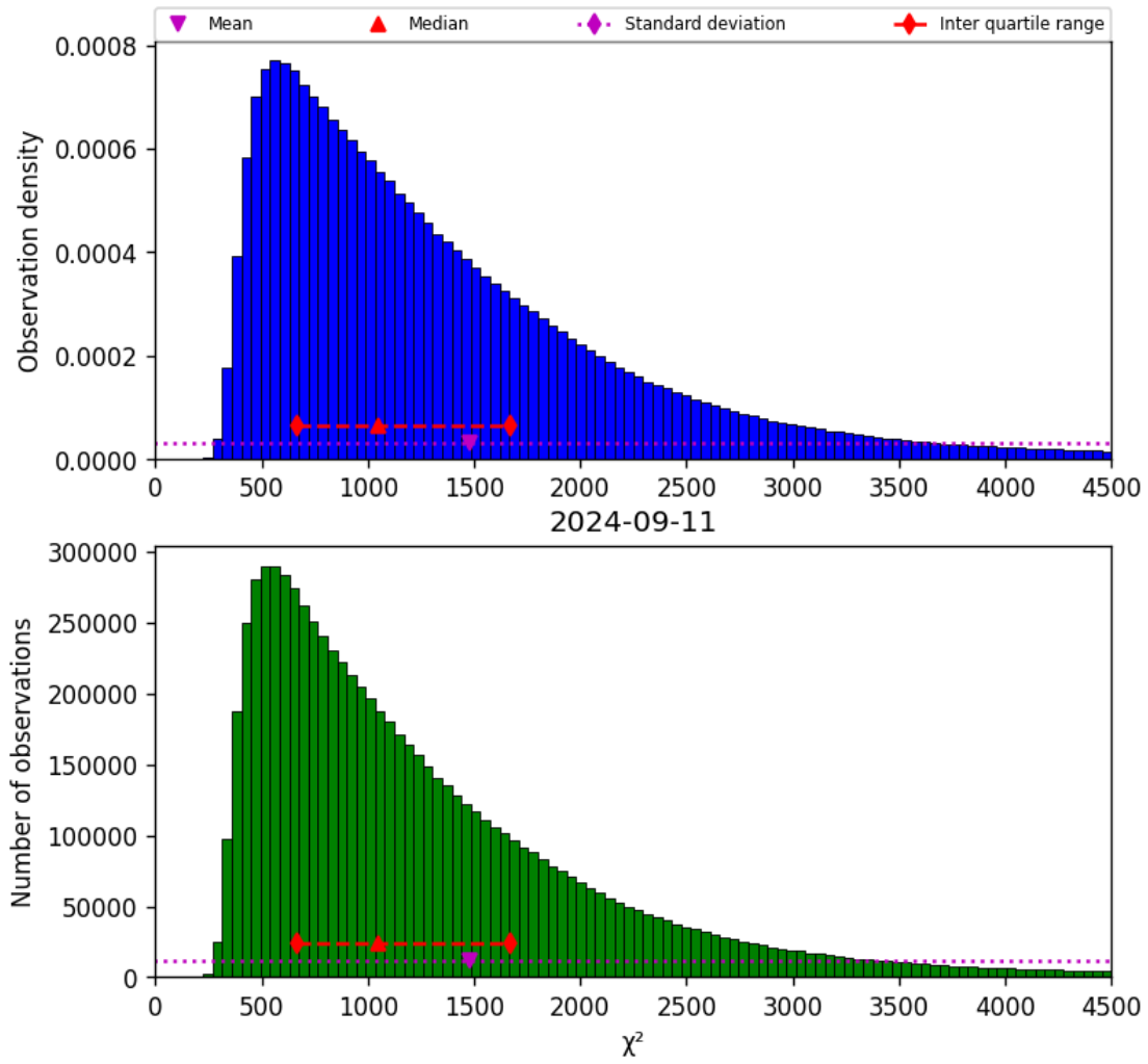
Figure 22: Histogram of “ \chi^2 ” for 2024-09-10 to 2024-09-12
