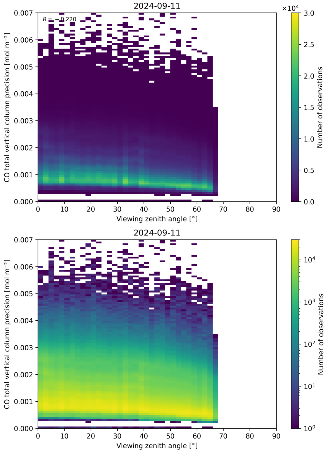
Figure 71: Scatter density plot of “Viewing zenith angle” against “CO total vertical column precision” for 2024-09-10 to 2024-09-12.
