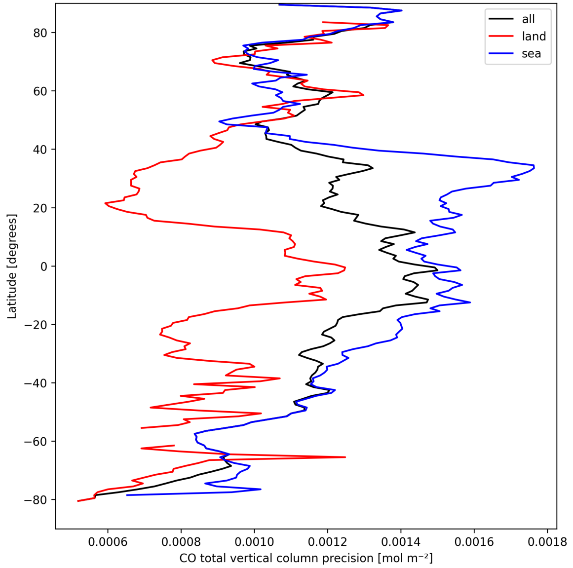
Figure 12: Zonal average of “CO total vertical column precision” for 2024-09-10 to 2024-09-12.
