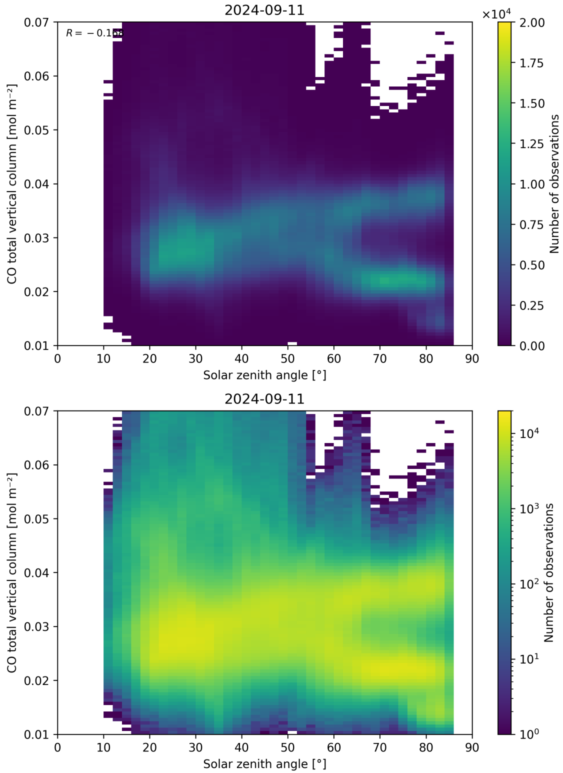
Figure 61: Scatter density plot of “Solar zenith angle” against “CO total vertical column” for 2024-09-10 to 2024-09-12.
