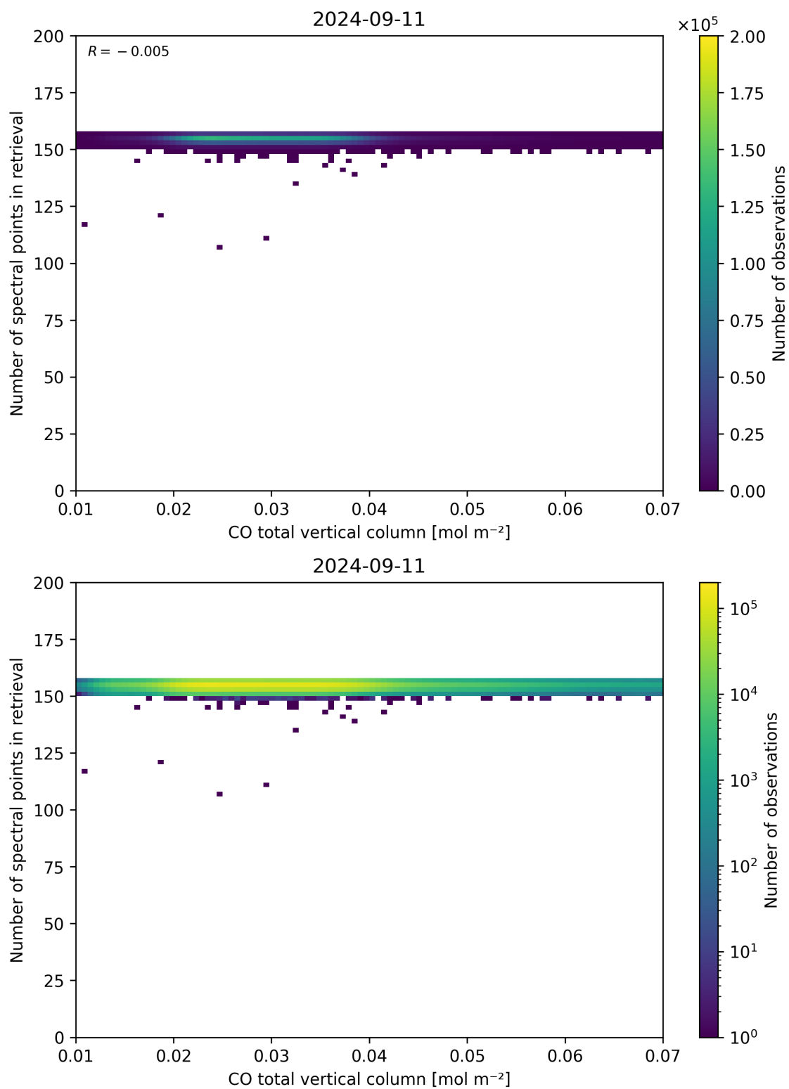
Figure 43: Scatter density plot of “CO total vertical column” against “Number of spectral points in retrieval” for 2024-09-10 to 2024-09-12.
