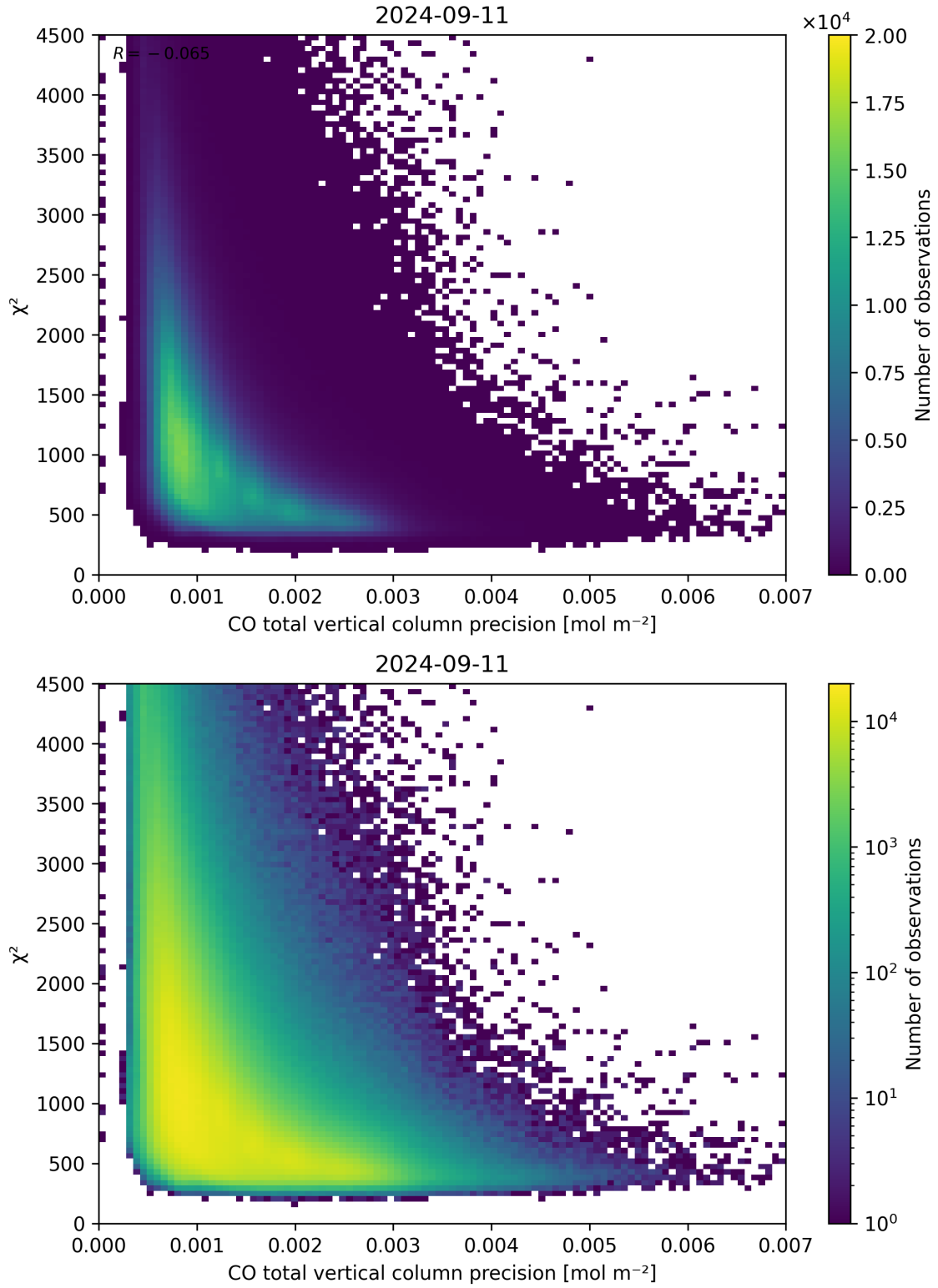
Figure 44: Scatter density plot of “CO total vertical column precision” against “ \chi^2 ” for 2024-09-10 to 2024-09-12.
