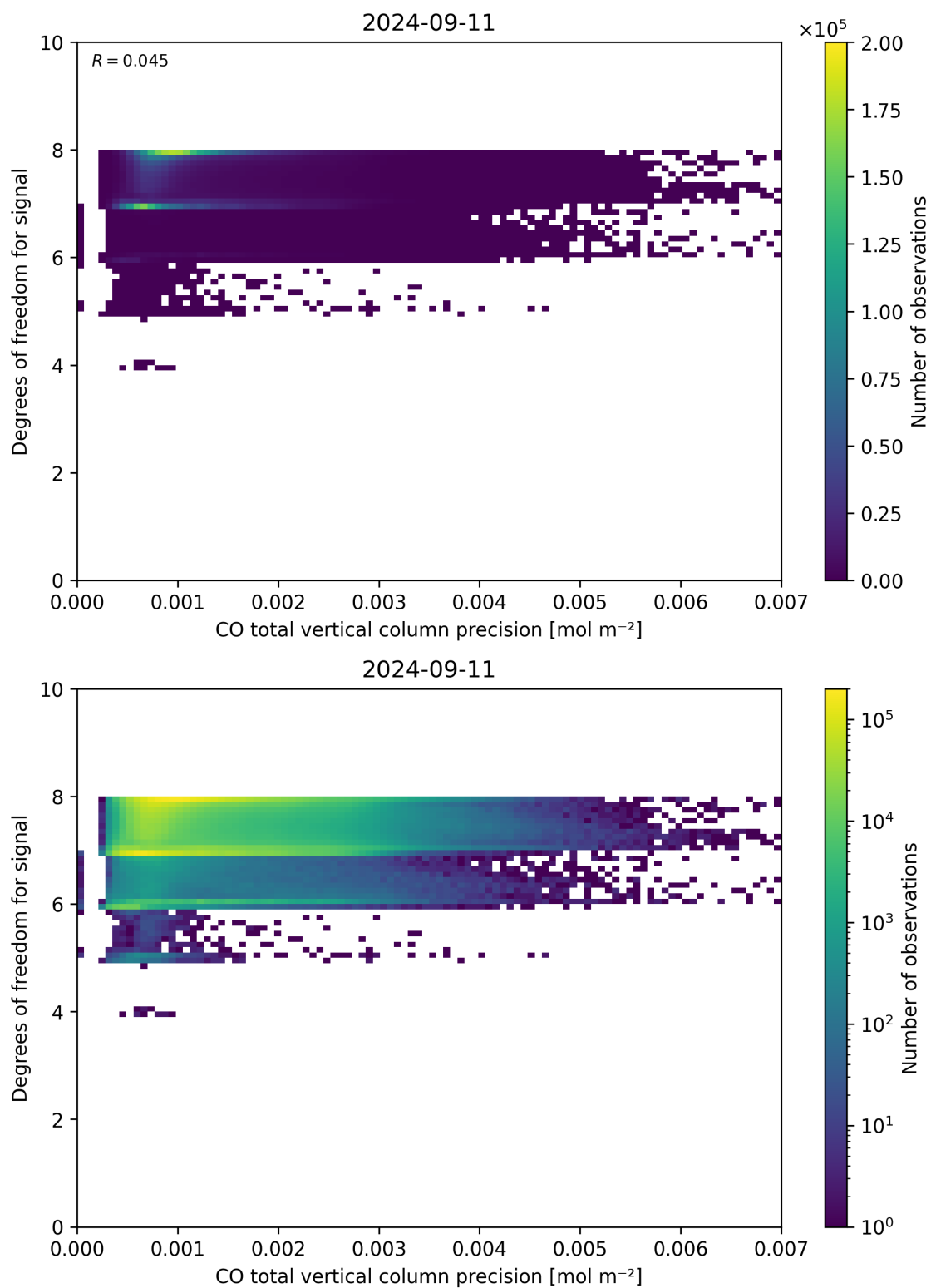
Figure 45: Scatter density plot of “CO total vertical column precision” against “Degrees of freedom for signal” for 2024-09-10 to 2024-09-12.
