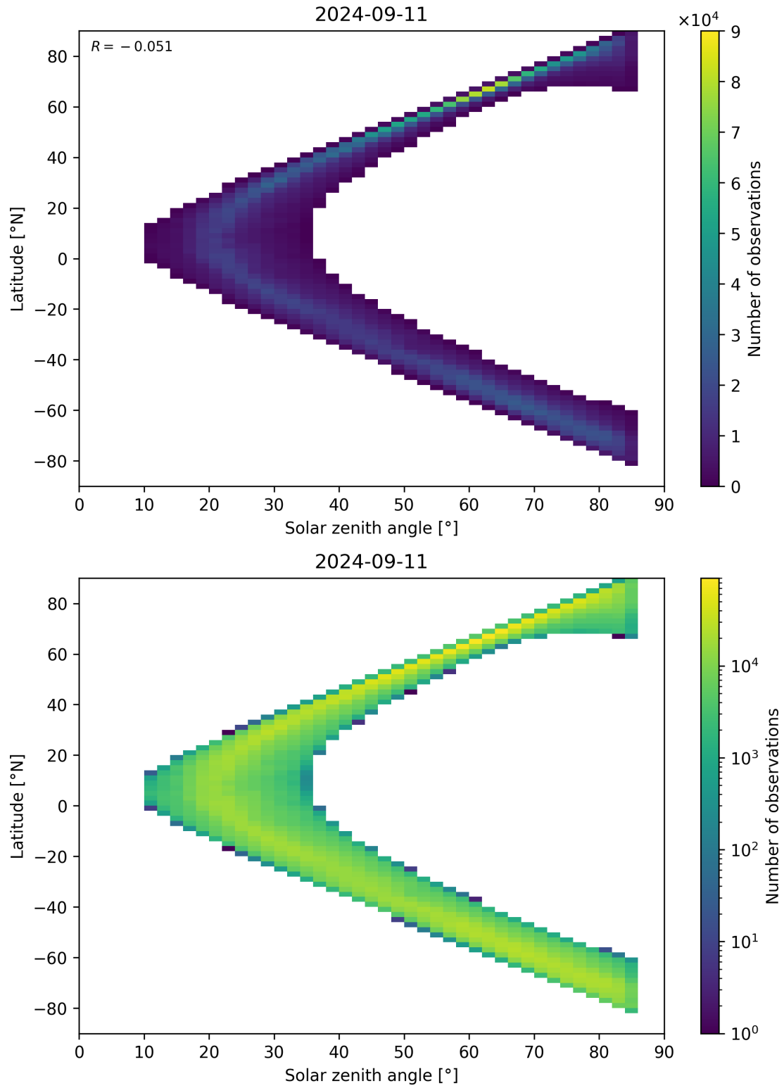
Figure 66: Scatter density plot of “Solar zenith angle” against “Latitude” for 2024-09-10 to 2024-09-12.
