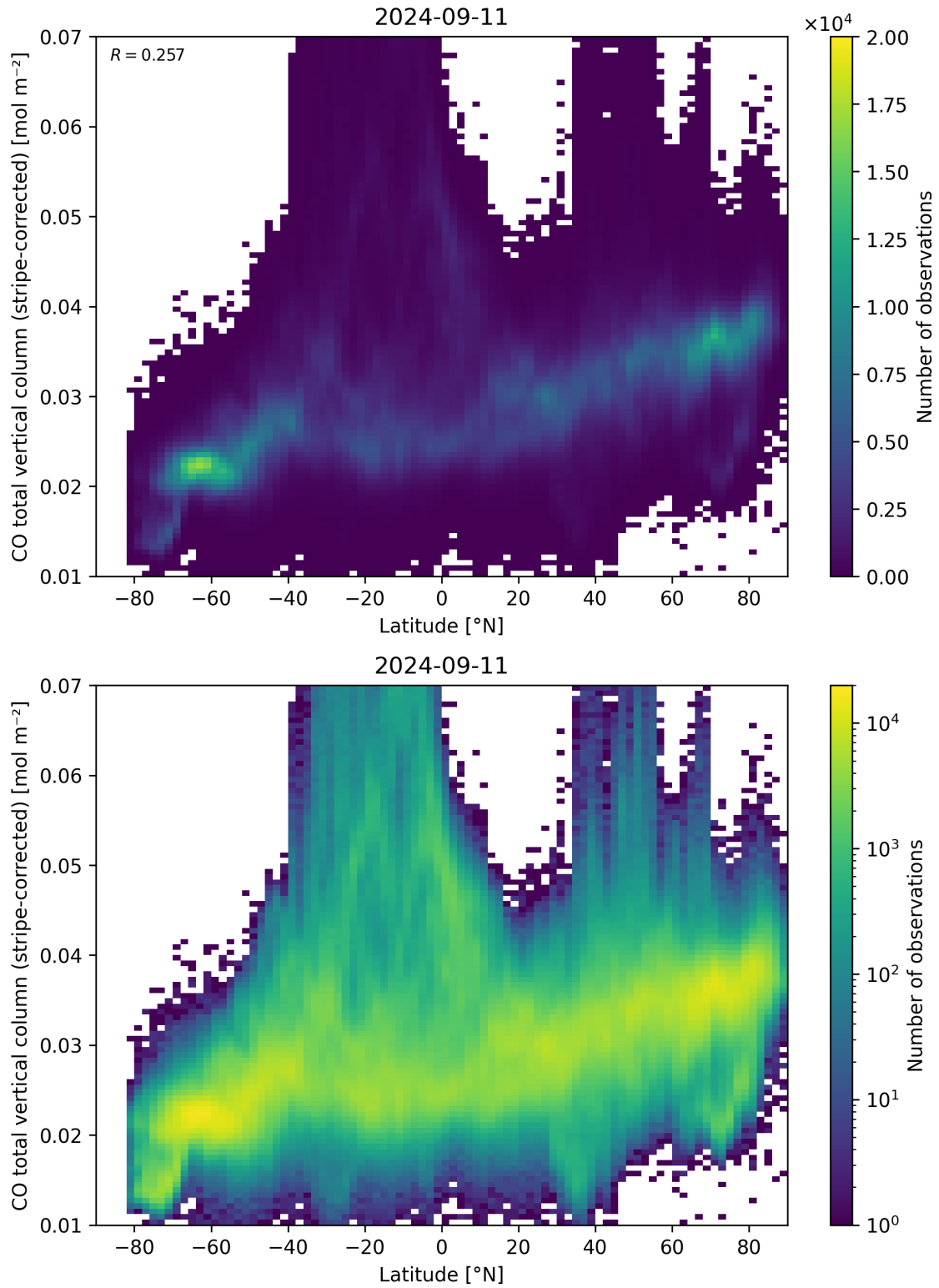
Figure 52: Scatter density plot of “Latitude” against “CO total vertical column (stripe-corrected)” for 2024-09-10 to 2024-09-12.
