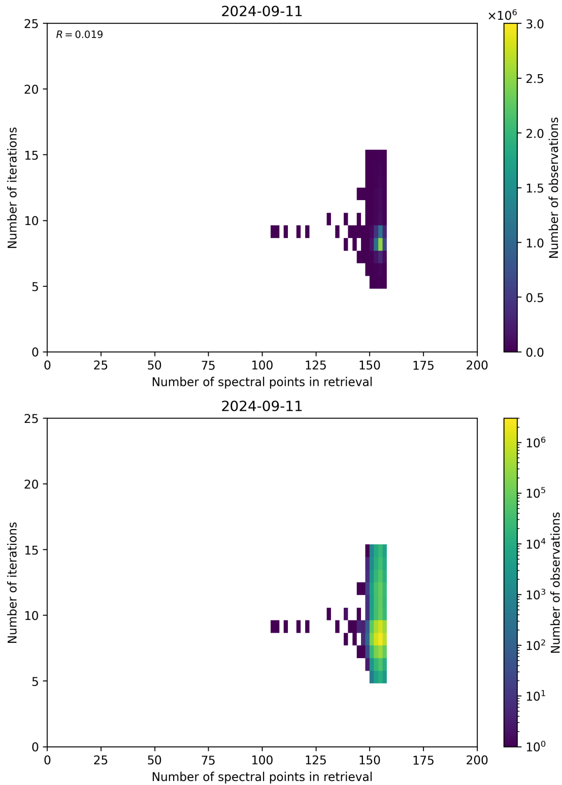
Figure 60: Scatter density plot of “Number of spectral points in retrieval” against “Number of iterations” for 2024-09-10 to 2024-09-12.
