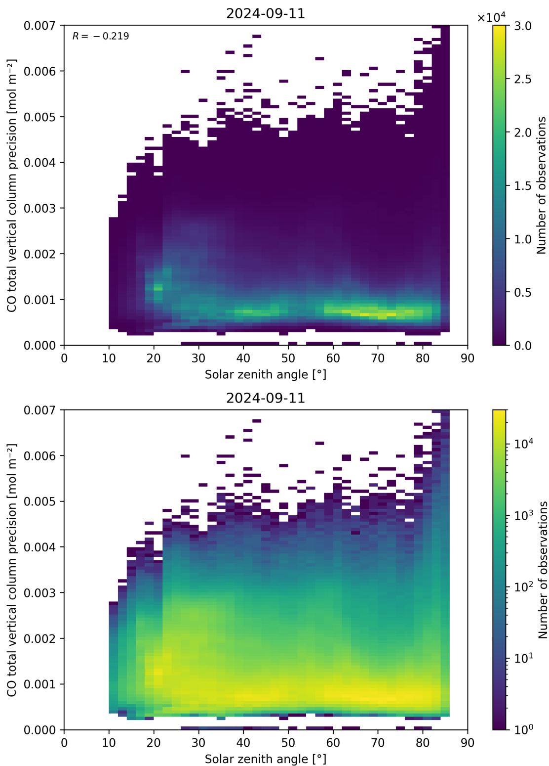
Figure 63: Scatter density plot of “Solar zenith angle” against “CO total vertical column precision” for 2024-09-10 to 2024-09-12.
