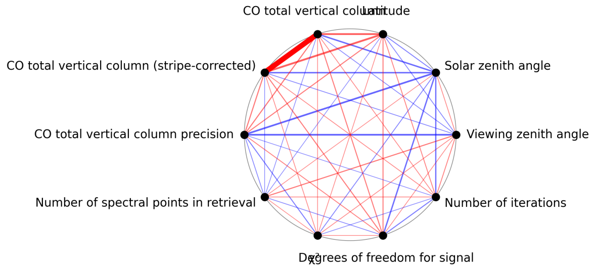
Figure 1: Map of correlation graph for 2024-09-10 to 2024-09-12.
