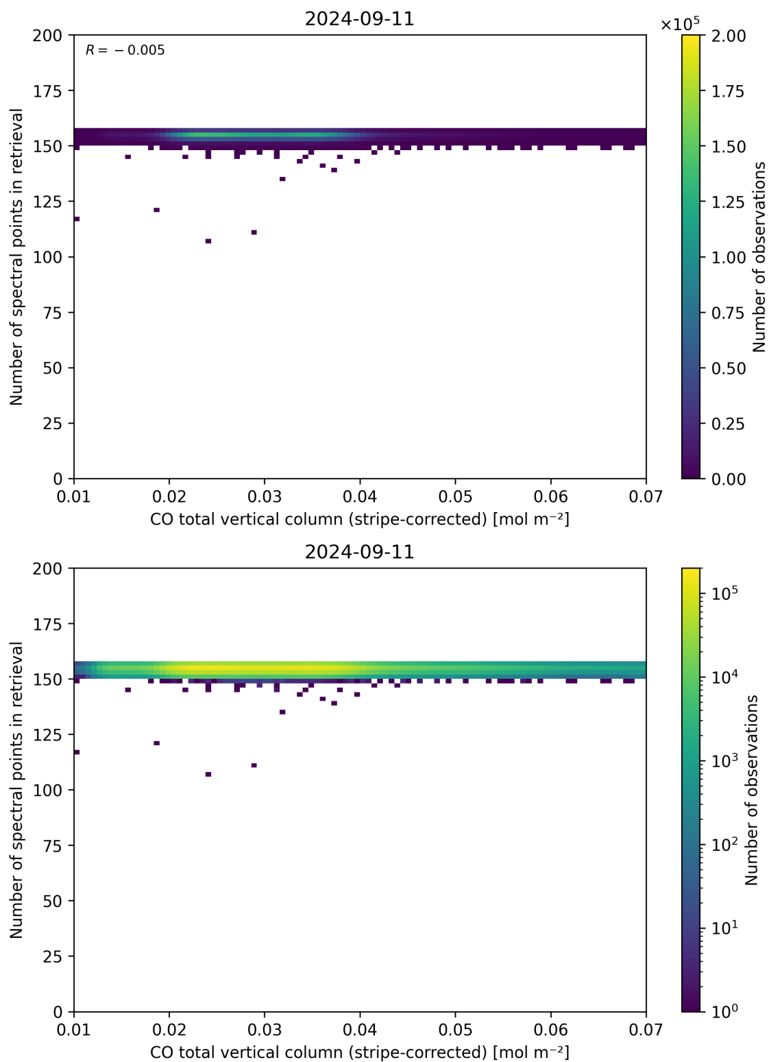
Figure 40: Scatter density plot of “CO total vertical column (stripe-corrected)” against “Number of spectral points in retrieval” for 2024-09-10 to 2024-09-12.
