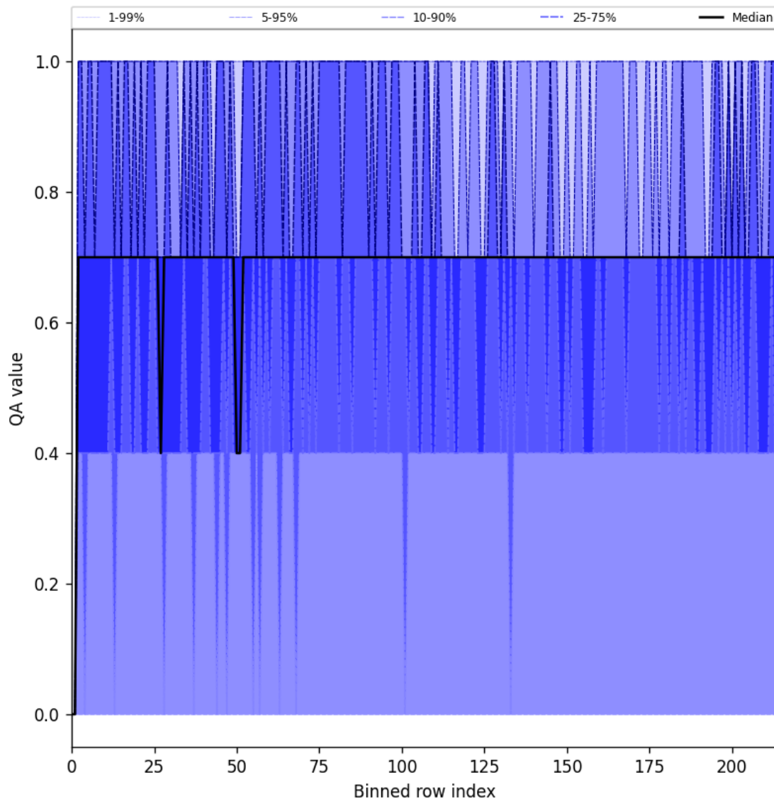
Figure 25: Along track statistics of “QA value” for 2024-09-10 to 2024-09-12
