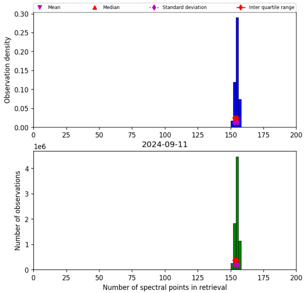
Figure 21: Histogram of “Number of spectral points in retrieval” for 2024-09-10 to 2024-09-12
