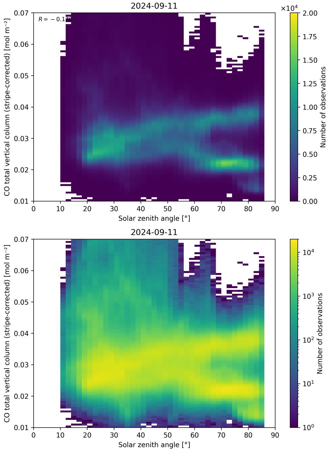
Figure 62: Scatter density plot of “Solar zenith angle” against “CO total vertical column (stripe-corrected)” for 2024-09-10 to 2024-09-12.
