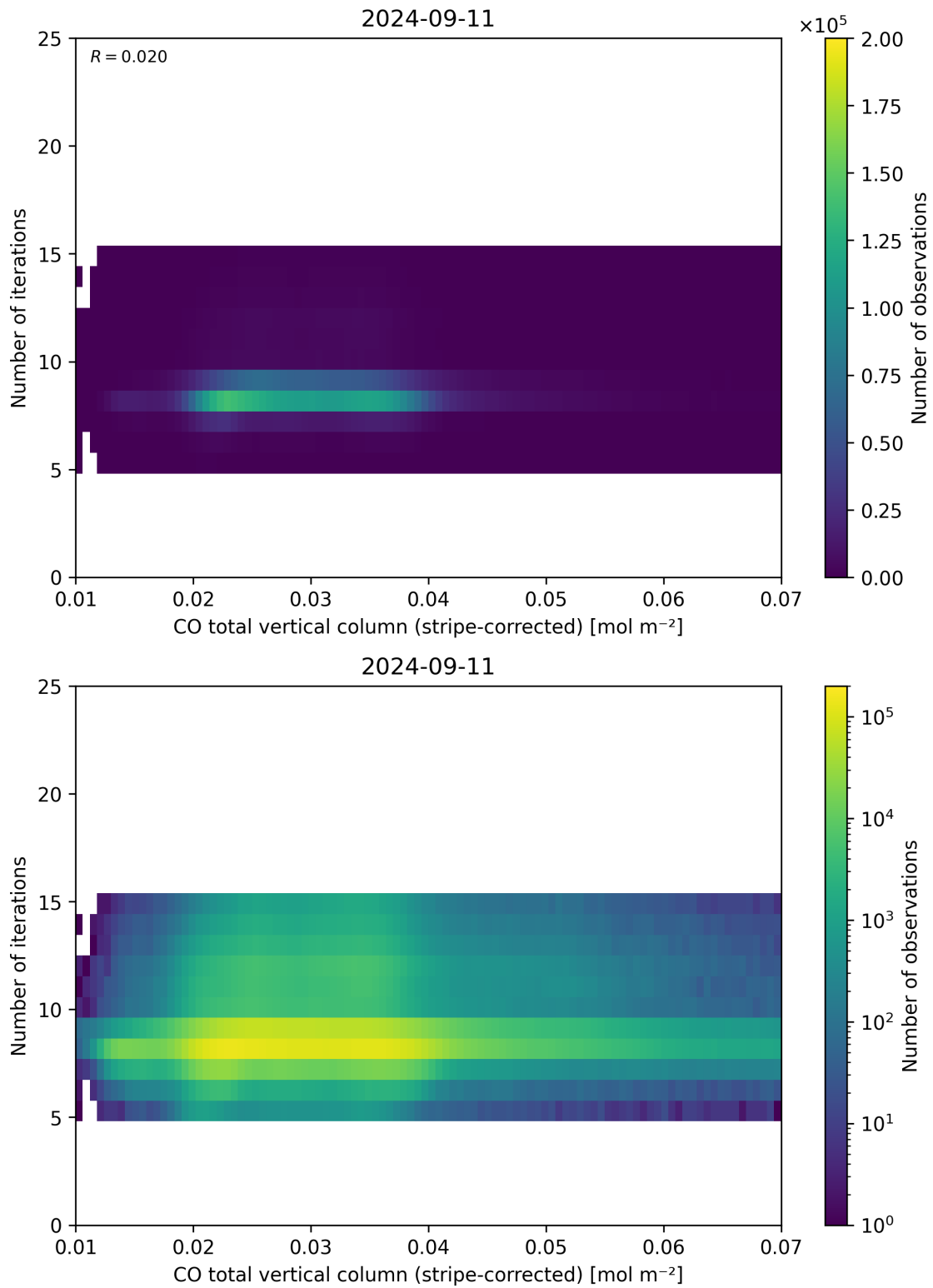
Figure 39: Scatter density plot of “CO total vertical column (stripe-corrected)” against “Number of iterations” for 2024-09-10 to 2024-09-12.
