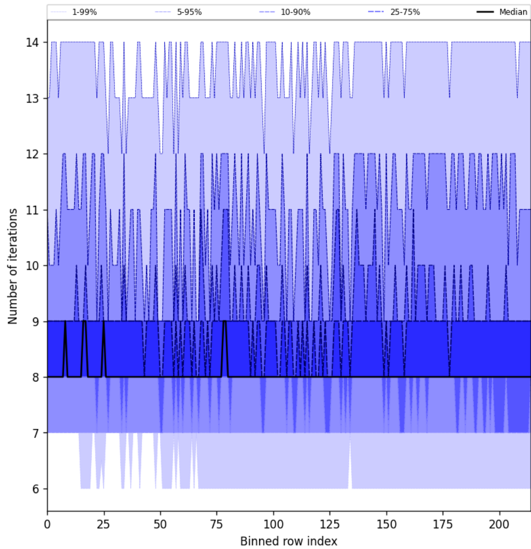
Figure 32: Along track statistics of “Number of iterations” for 2024-09-10 to 2024-09-12
