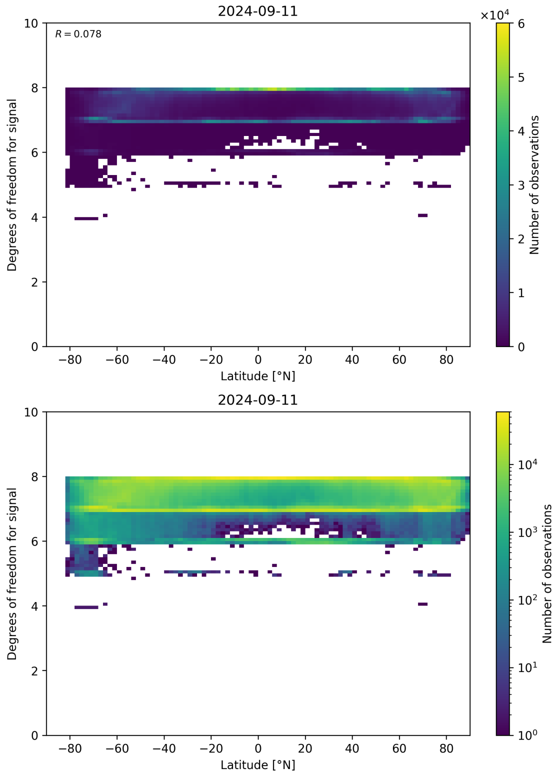
Figure 55: Scatter density plot of “Latitude” against “Degrees of freedom for signal” for 2024-09-10 to 2024-09-12.
