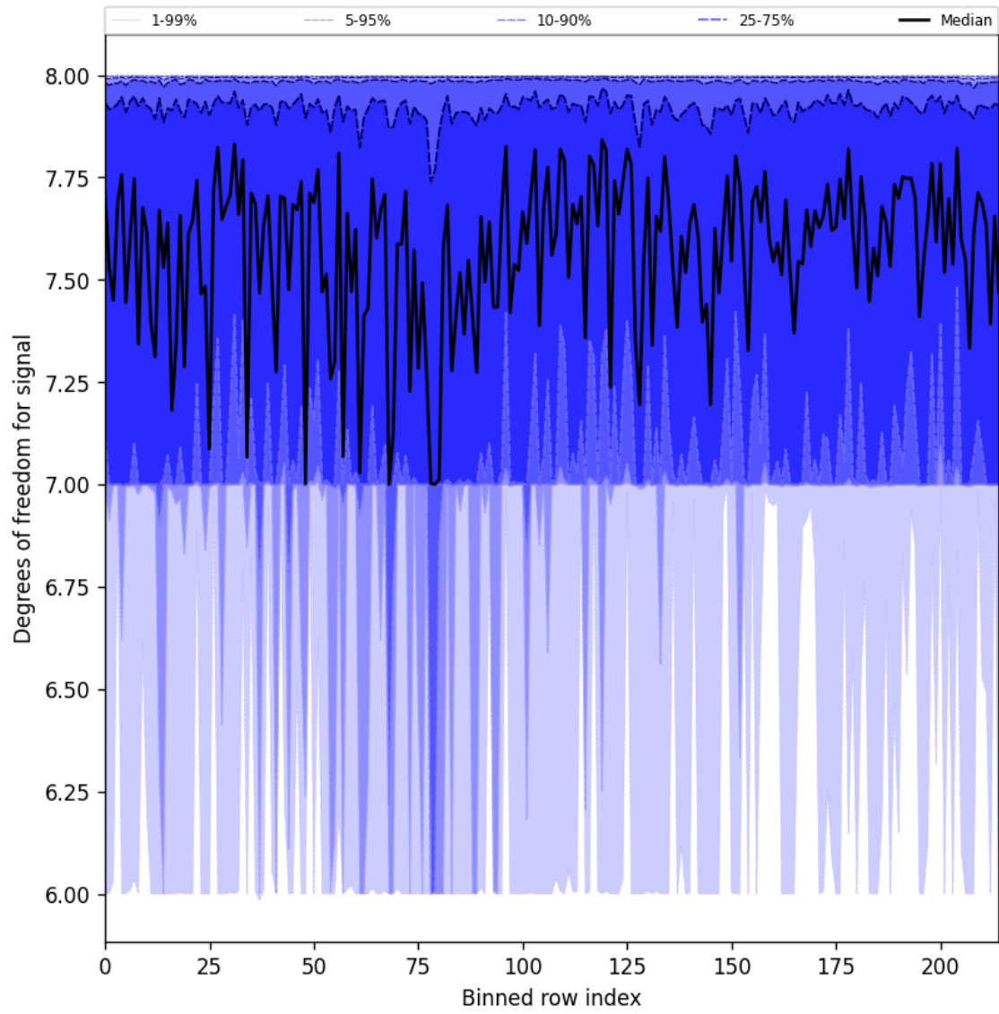
Figure 31: Along track statistics of “Degrees of freedom for signal” for 2024-09-10 to 2024-09-12
