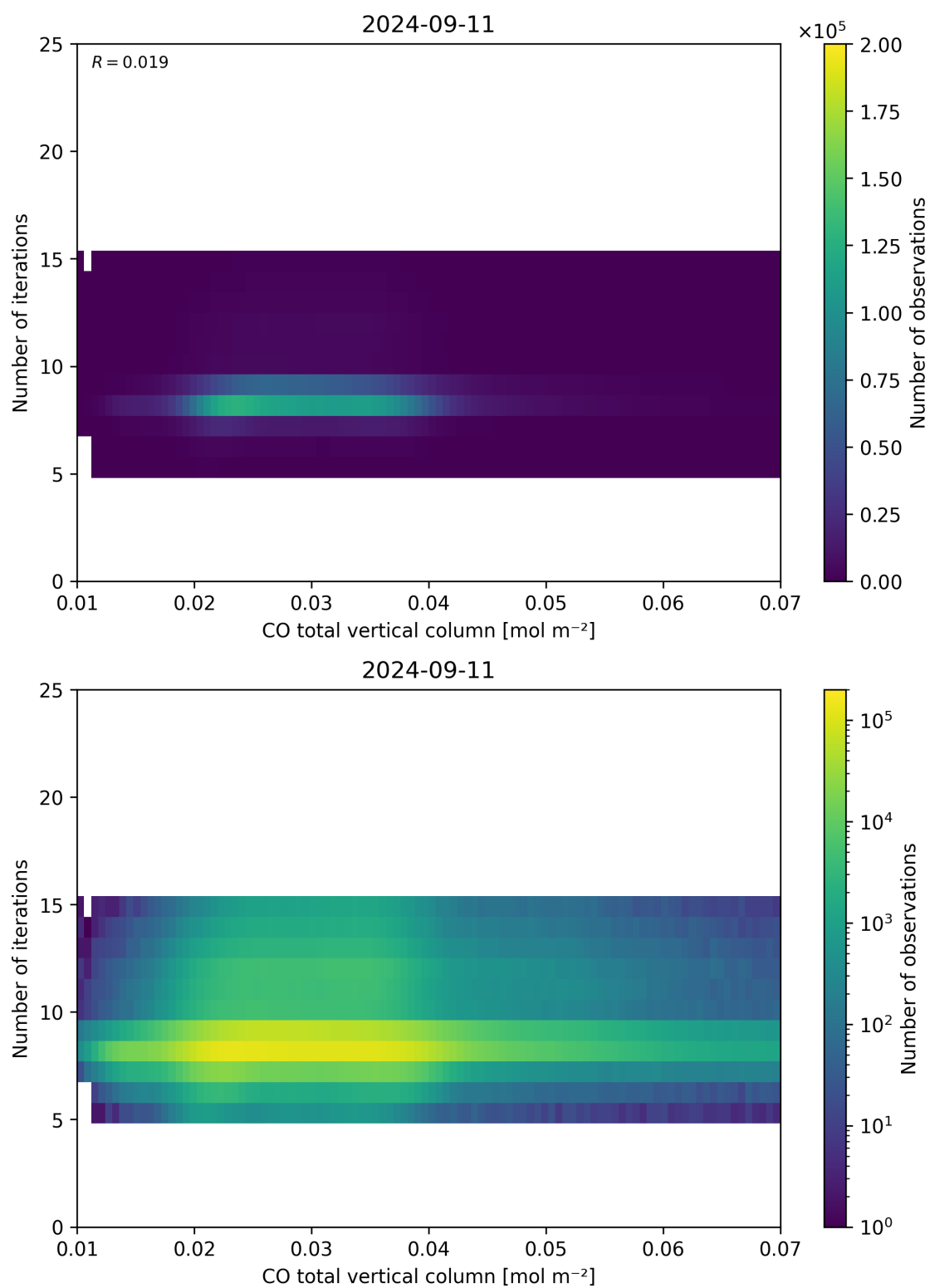
Figure 42: Scatter density plot of “CO total vertical column” against “Number of iterations” for 2024-09-10 to 2024-09-12.
