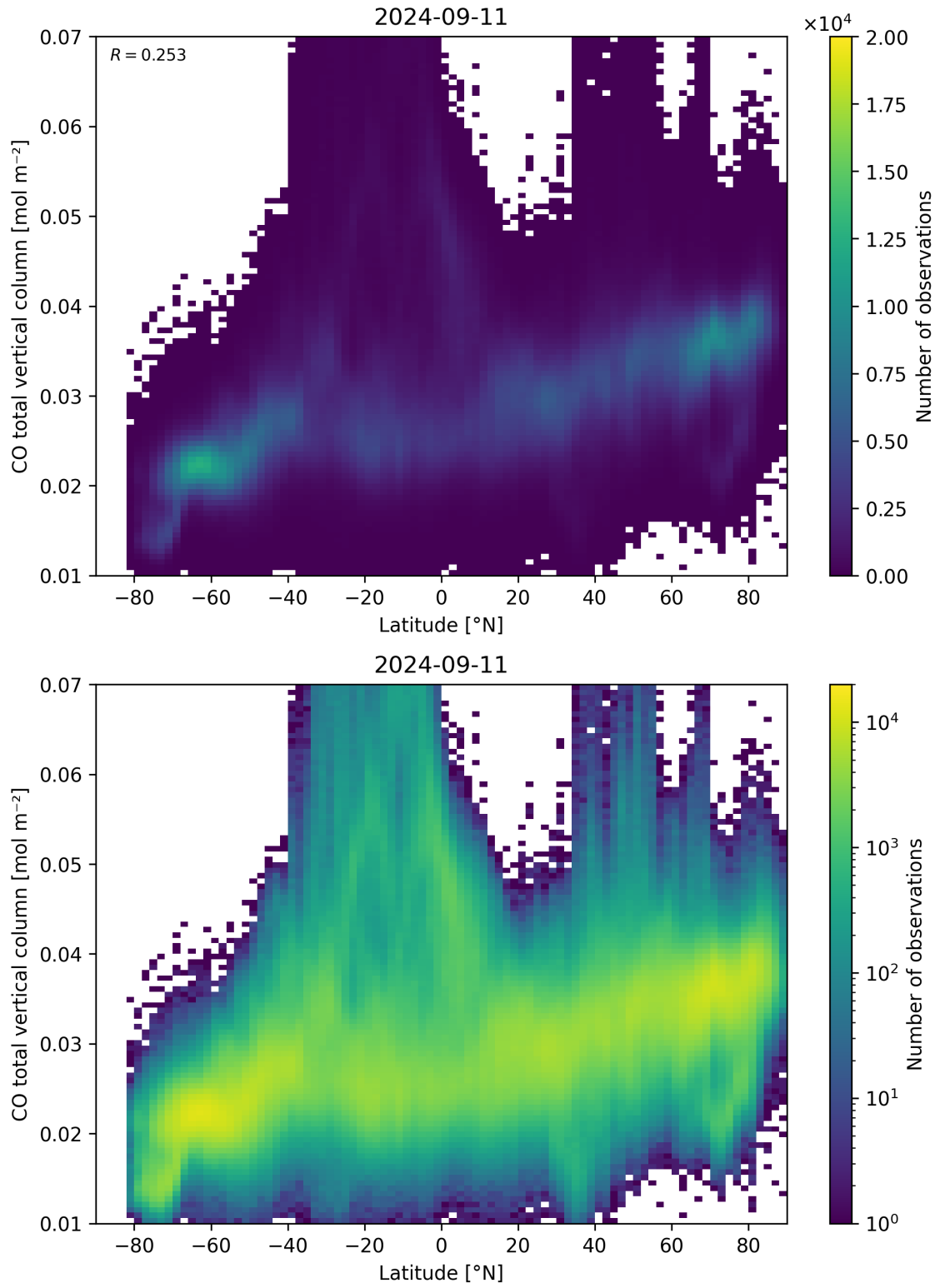
Figure 51: Scatter density plot of “Latitude” against “CO total vertical column” for 2024-09-10 to 2024-09-12.
