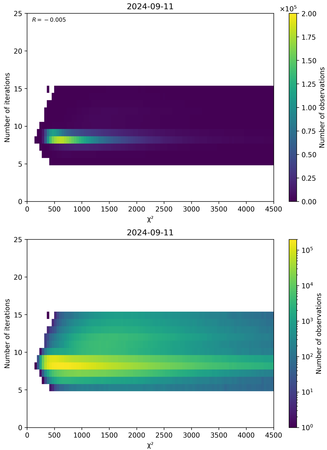
Figure 49: Scatter density plot of “ \chi^2 ” against “Number of iterations” for 2024-09-10 to 2024-09-12.
