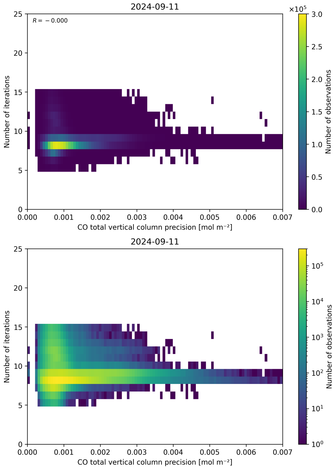
Figure 46: Scatter density plot of “CO total vertical column precision” against “Number of iterations” for 2024-09-10 to 2024-09-12.
