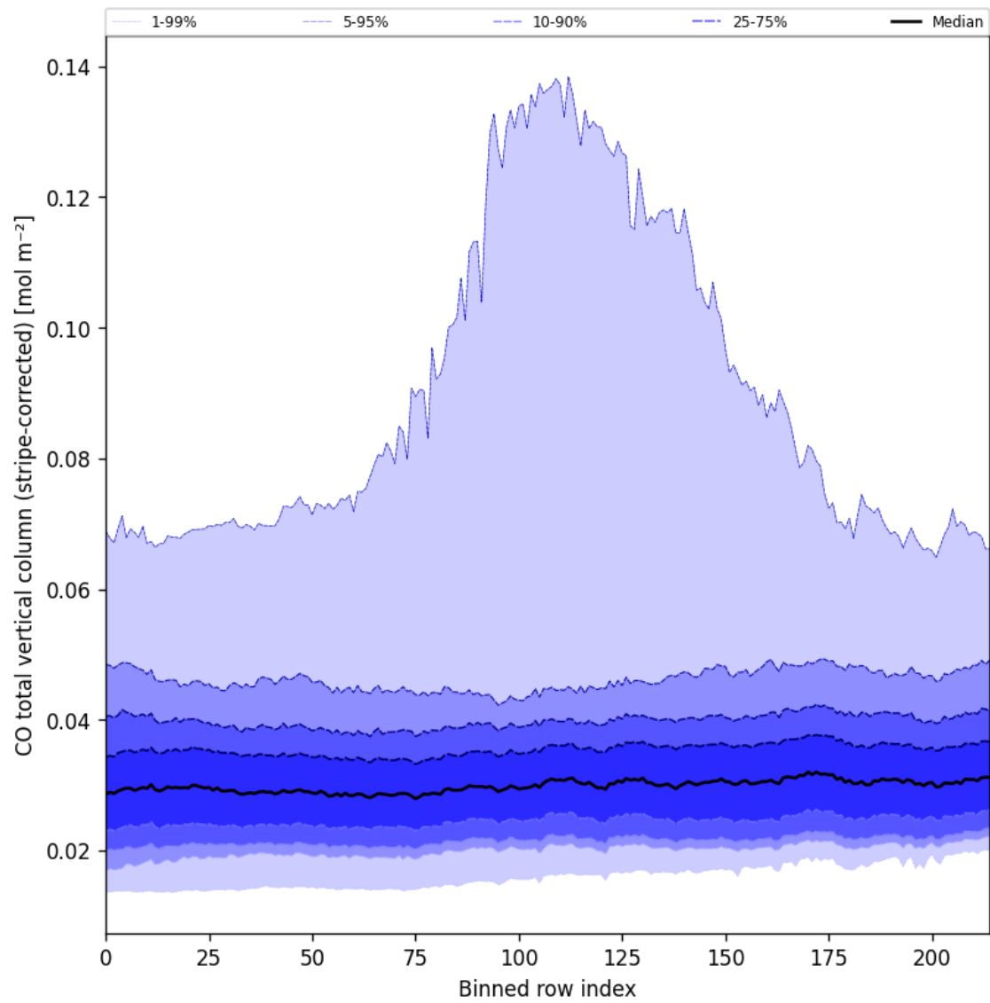
Figure 27: Along track statistics of “CO total vertical column (stripe-corrected)” for 2024-09-10 to 2024-09-12
