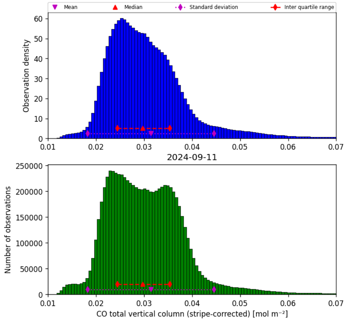
Figure 19: Histogram of “CO total vertical column (stripe-corrected)” for 2024-09-10 to 2024-09-12
