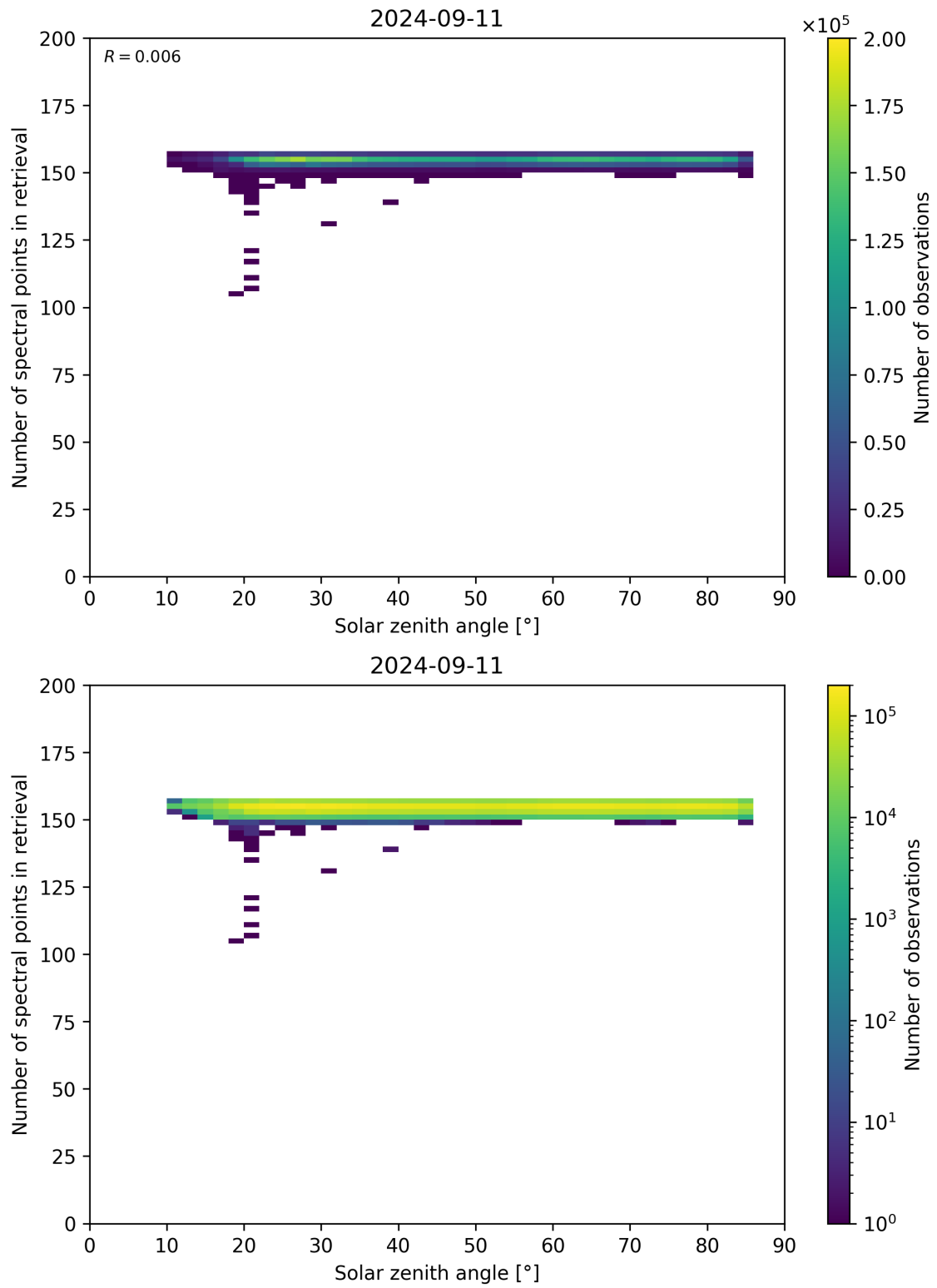
Figure 68: Scatter density plot of “Solar zenith angle” against “Number of spectral points in retrieval” for 2024-09-10 to 2024-09-12.
