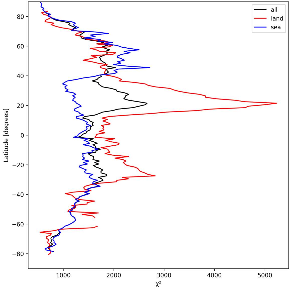
Figure 14: Zonal average of “ \chi^2 ” for 2024-09-10 to 2024-09-12.
