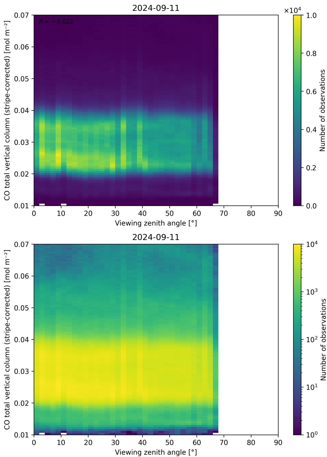
Figure 70: Scatter density plot of “Viewing zenith angle” against “CO total vertical column (stripe-corrected)” for 2024-09-10 to 2024-09-12.
