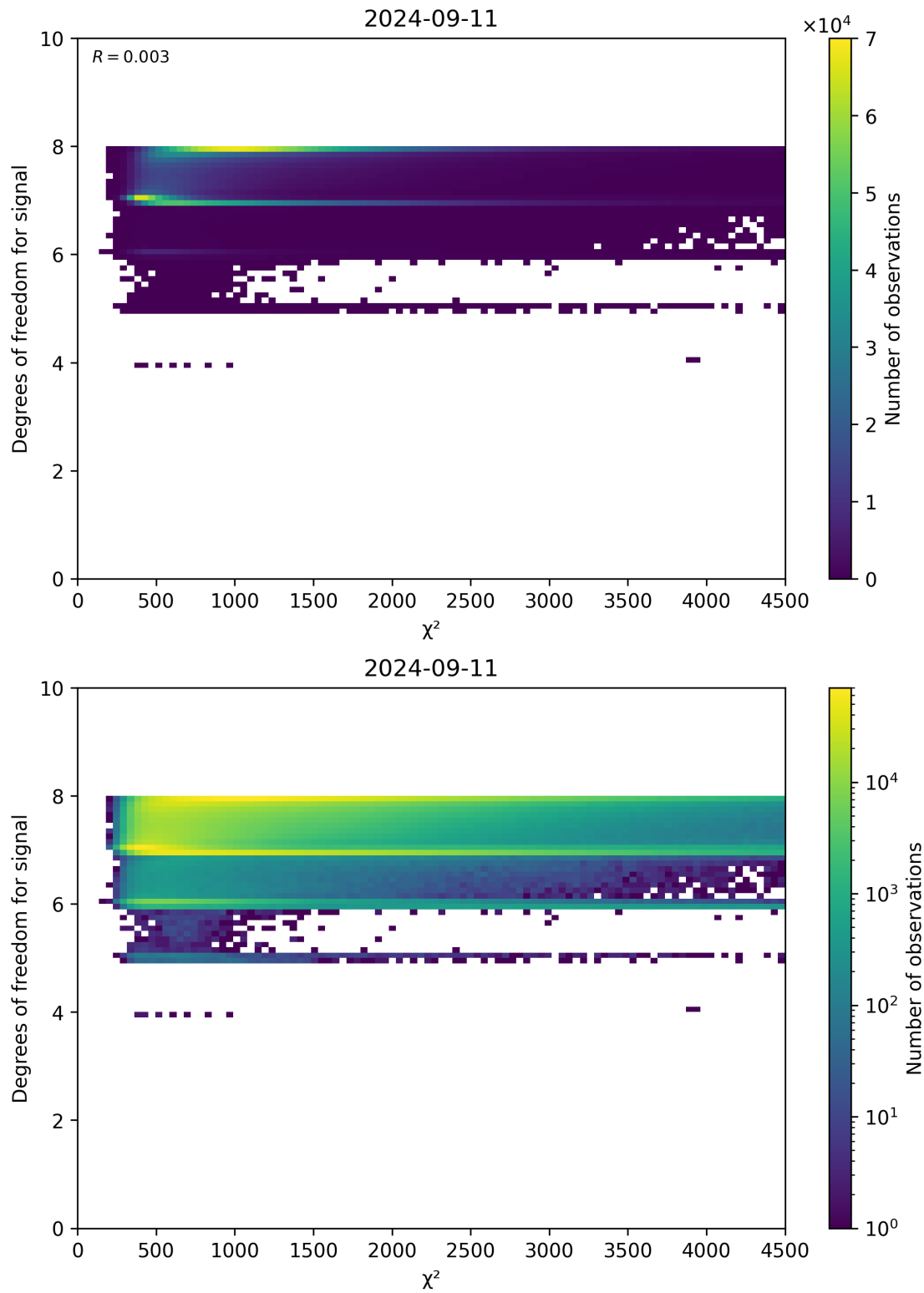
Figure 48: Scatter density plot of “ \chi^2 ” against “Degrees of freedom for signal” for 2024-09-10 to 2024-09-12.
