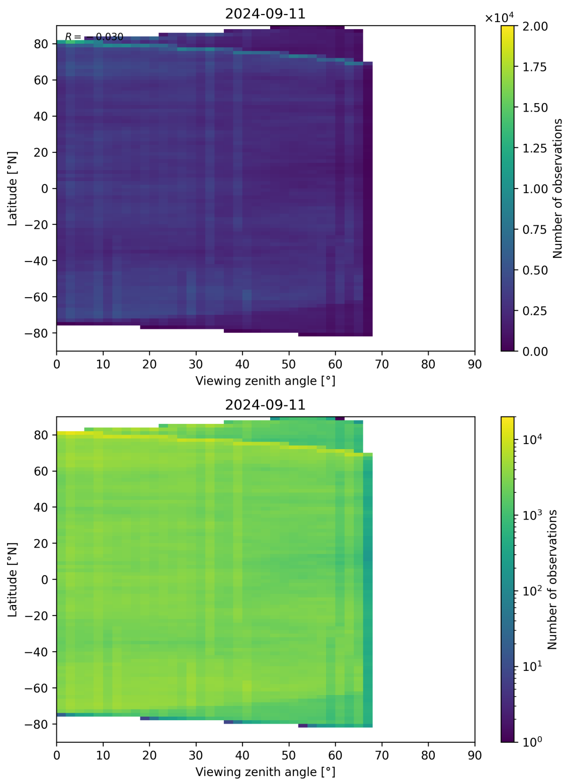
Figure 74: Scatter density plot of “Viewing zenith angle” against “Latitude” for 2024-09-10 to 2024-09-12.
