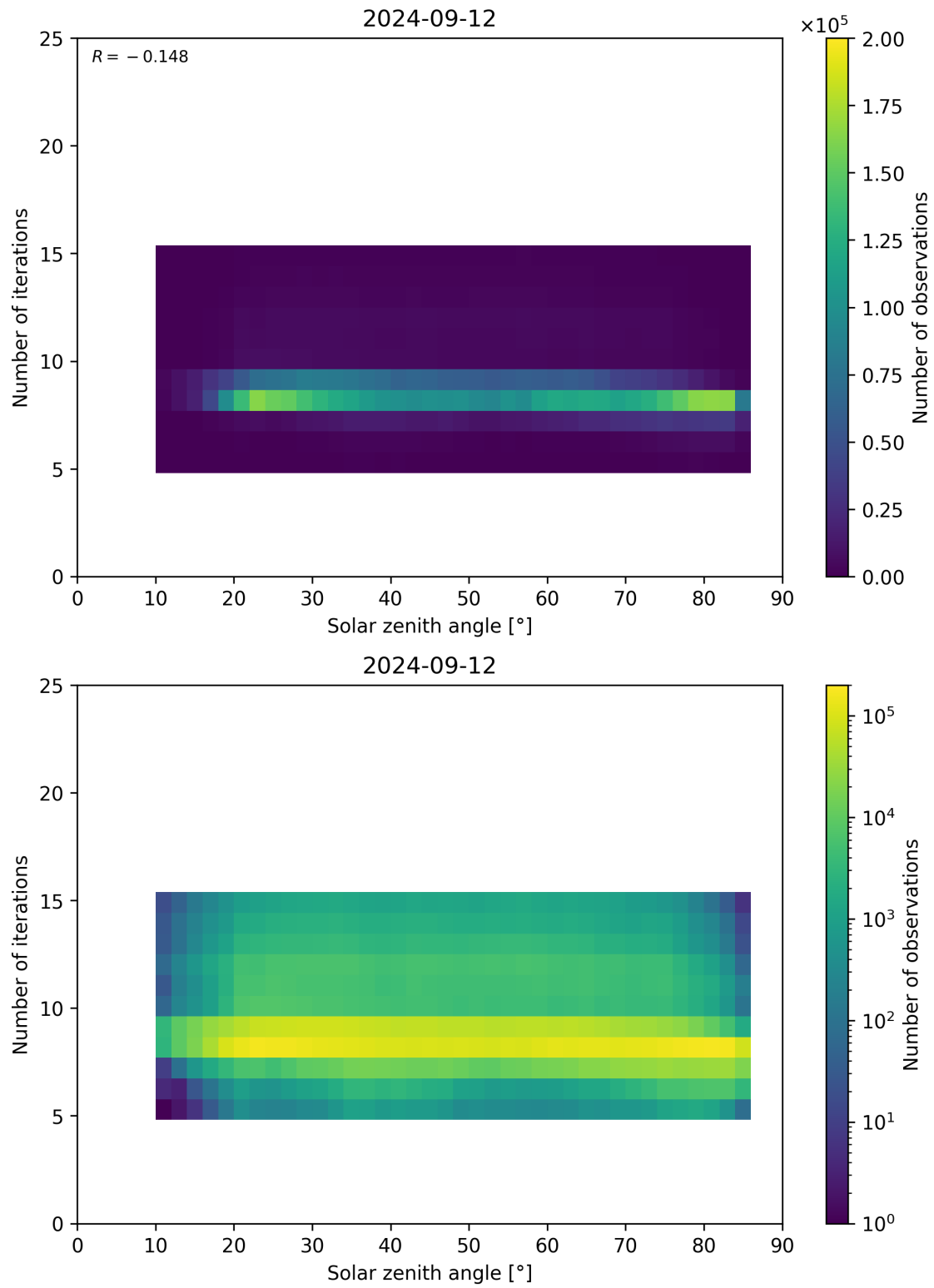
Figure 67: Scatter density plot of “Solar zenith angle” against “Number of iterations” for 2024-09-12 to 2024-09-13.
