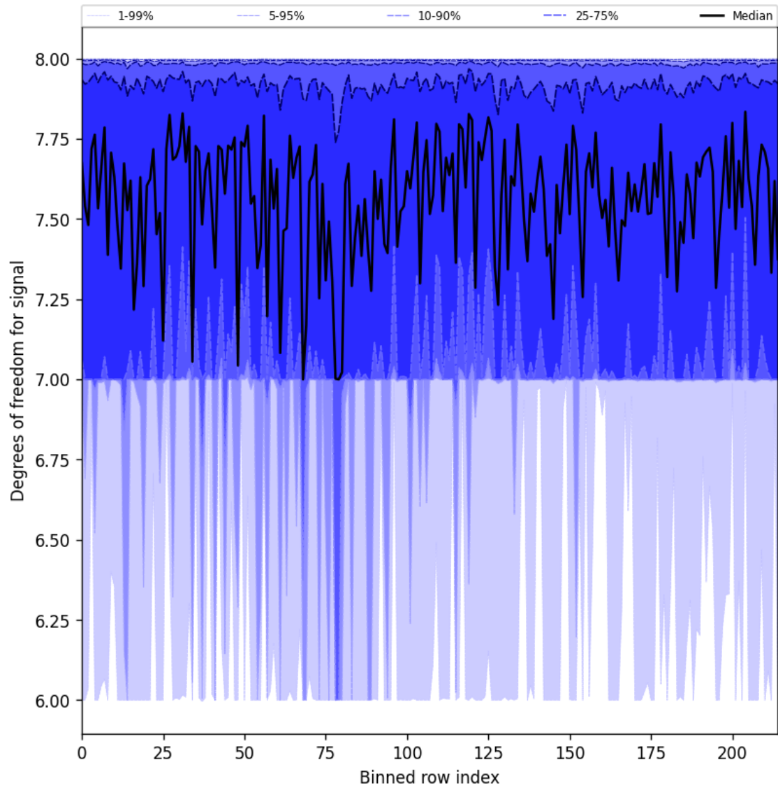
Figure 31: Along track statistics of “Degrees of freedom for signal” for 2024-09-12 to 2024-09-13
