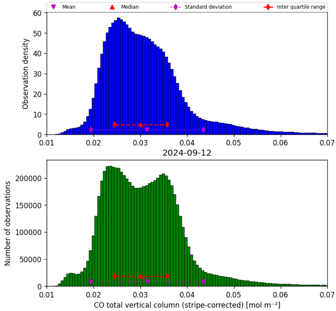
Figure 19: Histogram of “CO total vertical column (stripe-corrected)” for 2024-09-12 to 2024-09-13
