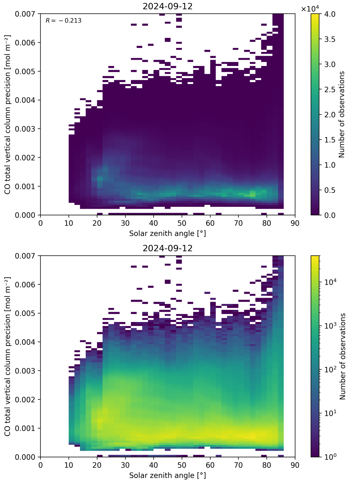
Figure 63: Scatter density plot of “Solar zenith angle” against “CO total vertical column precision” for 2024-09-12 to 2024-09-13.
