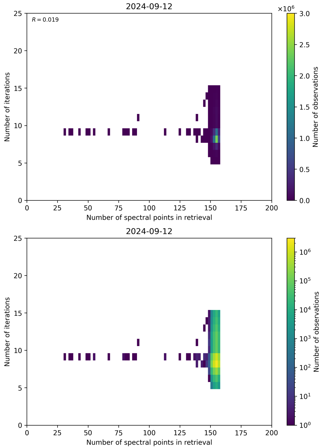
Figure 60: Scatter density plot of “Number of spectral points in retrieval” against “Number of iterations” for 2024-09-12 to 2024-09-13.
