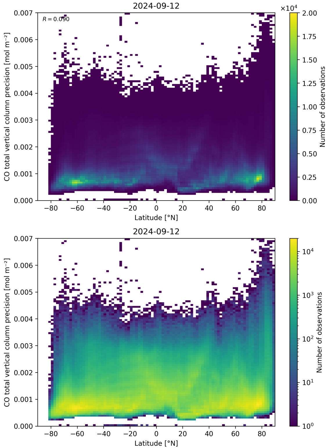
Figure 53: Scatter density plot of “Latitude” against “CO total vertical column precision” for 2024-09-12 to 2024-09-13.
