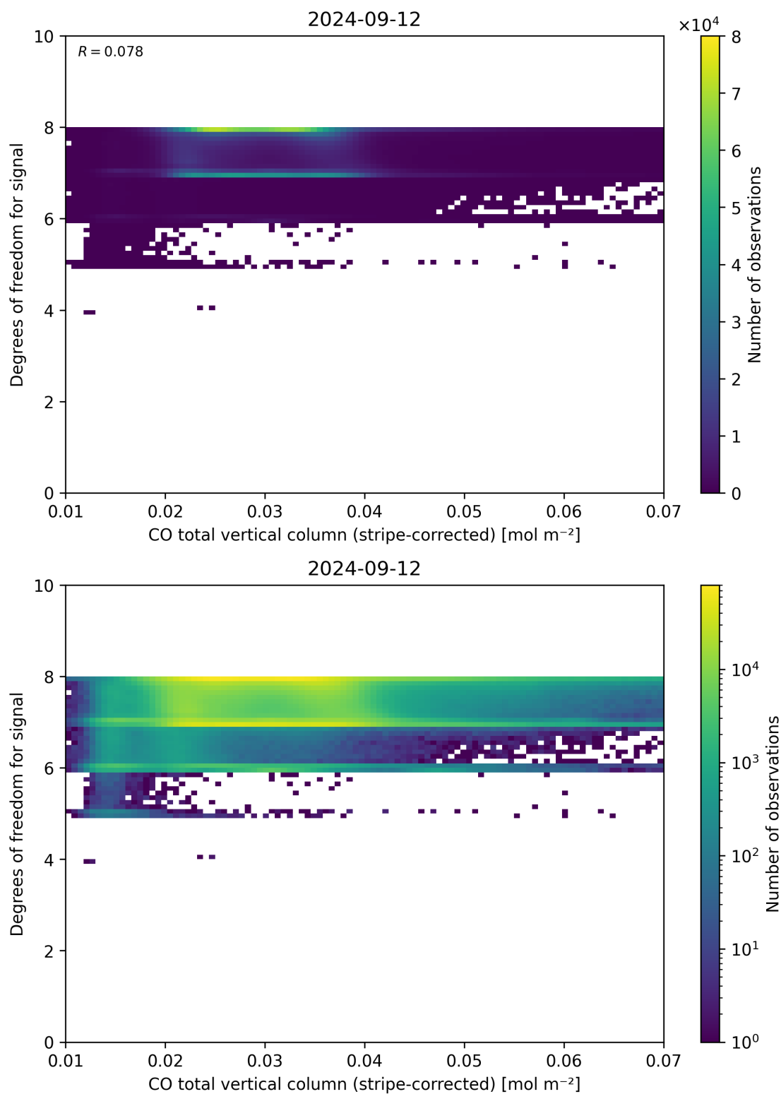
Figure 38: Scatter density plot of “CO total vertical column (stripe-corrected)” against “Degrees of freedom for signal” for 2024-09-12 to 2024-09-13.
