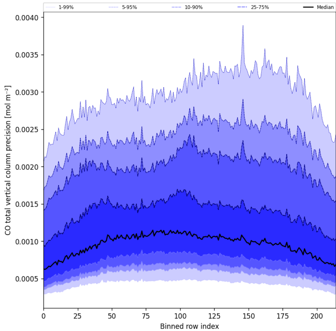
Figure 28: Along track statistics of “CO total vertical column precision” for 2024-09-12 to 2024-09-13
