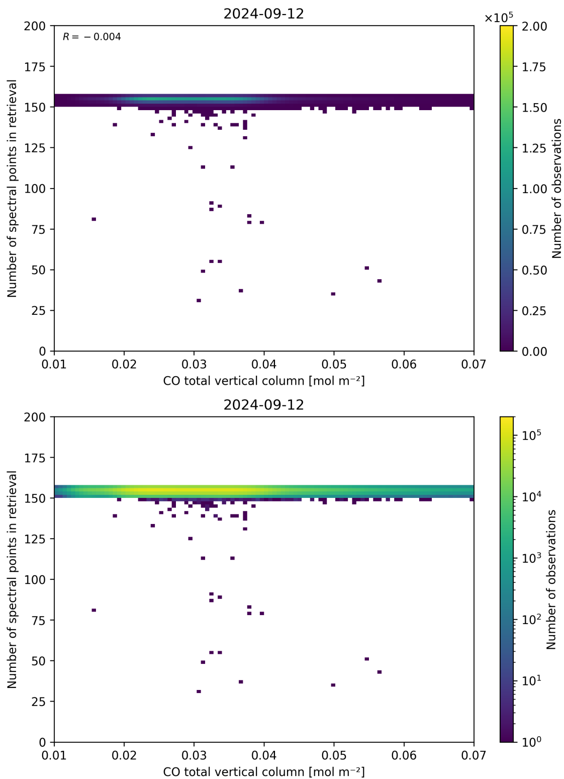
Figure 43: Scatter density plot of “CO total vertical column” against “Number of spectral points in retrieval” for 2024-09-12 to 2024-09-13.
