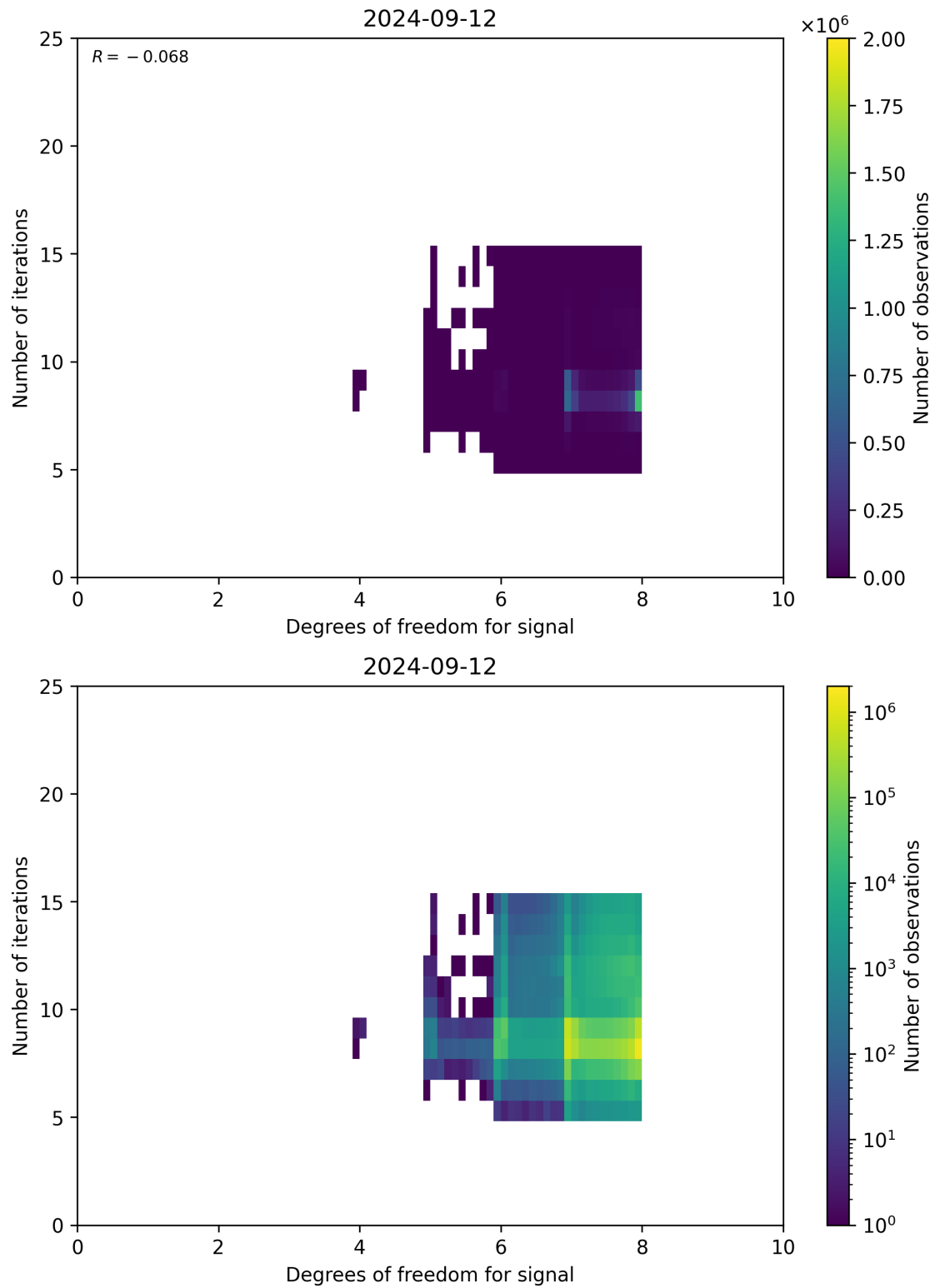
Figure 50: Scatter density plot of “Degrees of freedom for signal” against “Number of iterations” for 2024-09-12 to 2024-09-13.
