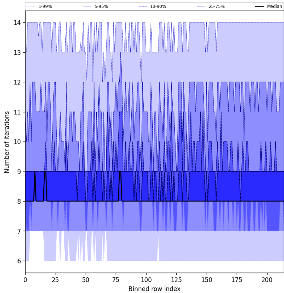
Figure 32: Along track statistics of “Number of iterations” for 2024-09-12 to 2024-09-13
