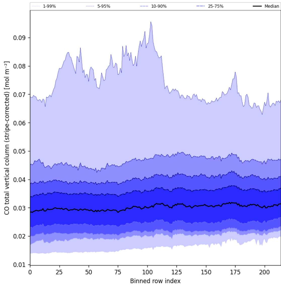
Figure 27: Along track statistics of “CO total vertical column (stripe-corrected)” for 2024-09-12 to 2024-09-13
