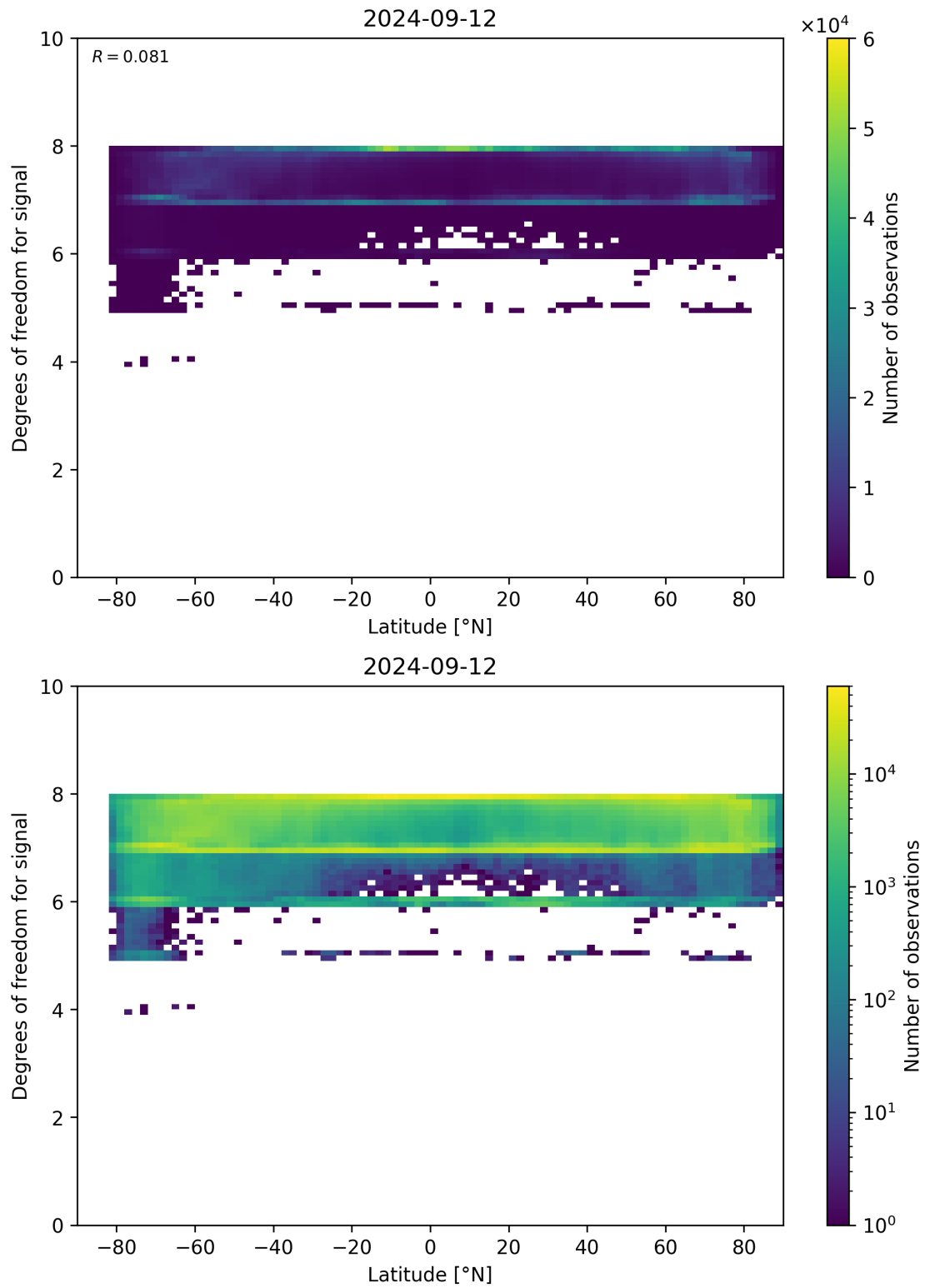
Figure 55: Scatter density plot of “Latitude” against “Degrees of freedom for signal” for 2024-09-12 to 2024-09-13.
