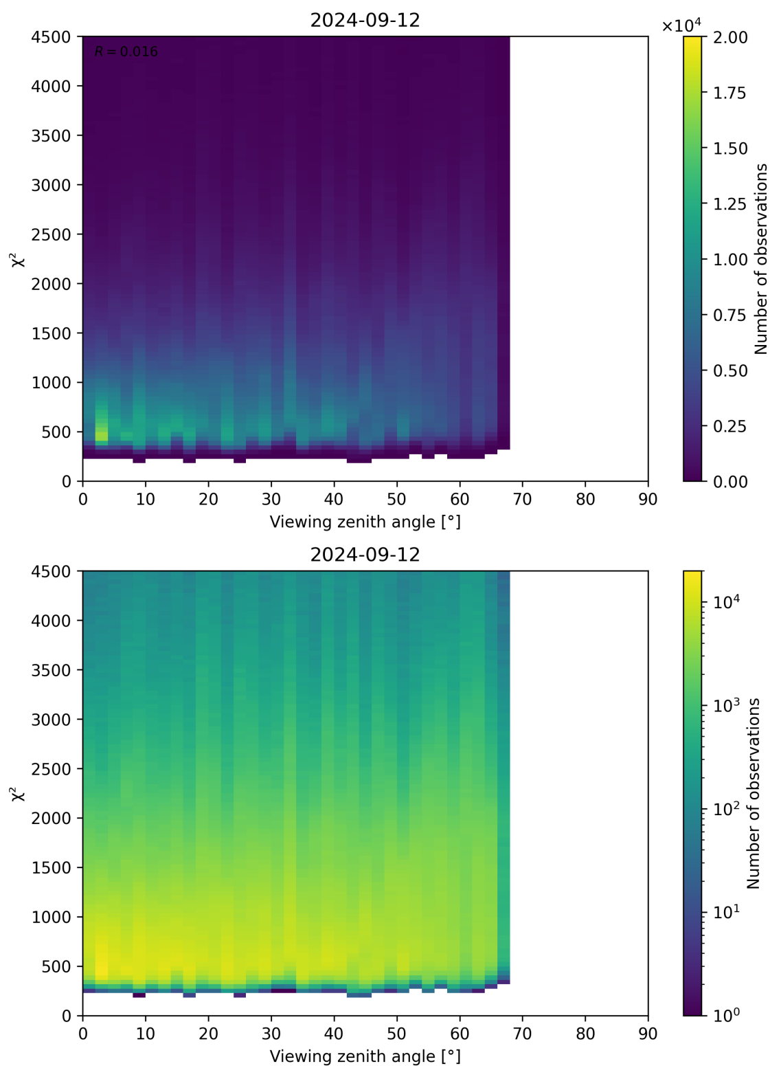
Figure 72: Scatter density plot of “Viewing zenith angle” against “ \chi^2 ” for 2024-09-12 to 2024-09-13.
