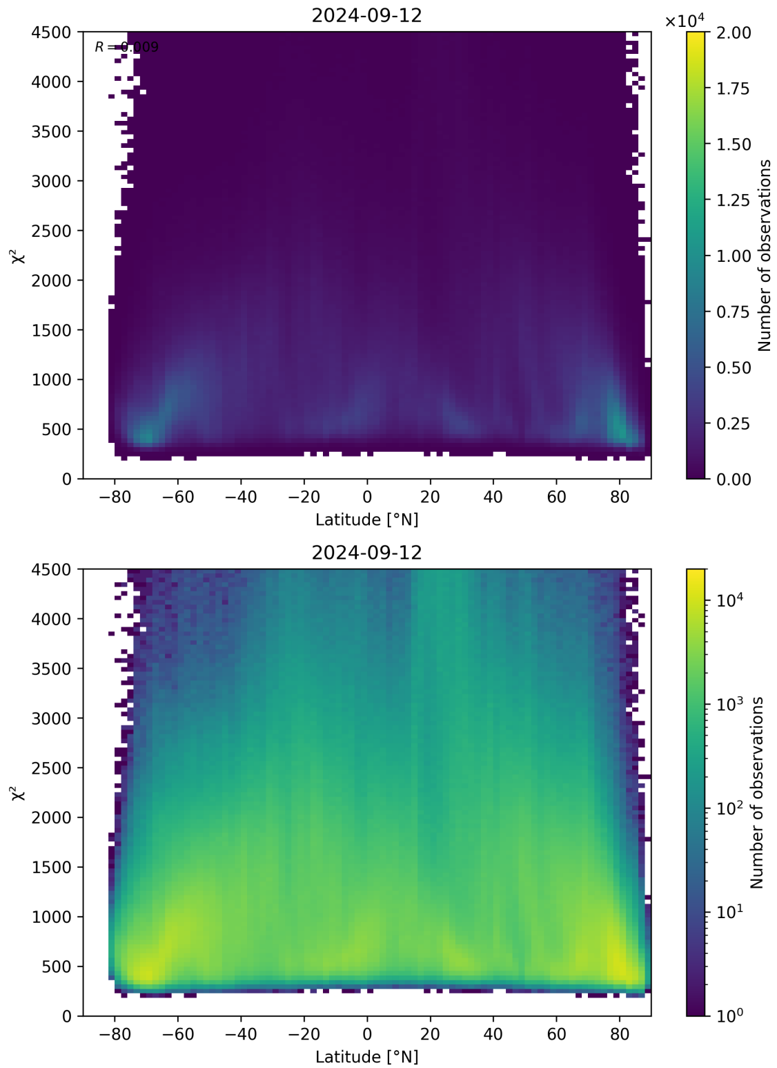
Figure 54: Scatter density plot of “Latitude” against “ \chi^2 ” for 2024-09-12 to 2024-09-13.
