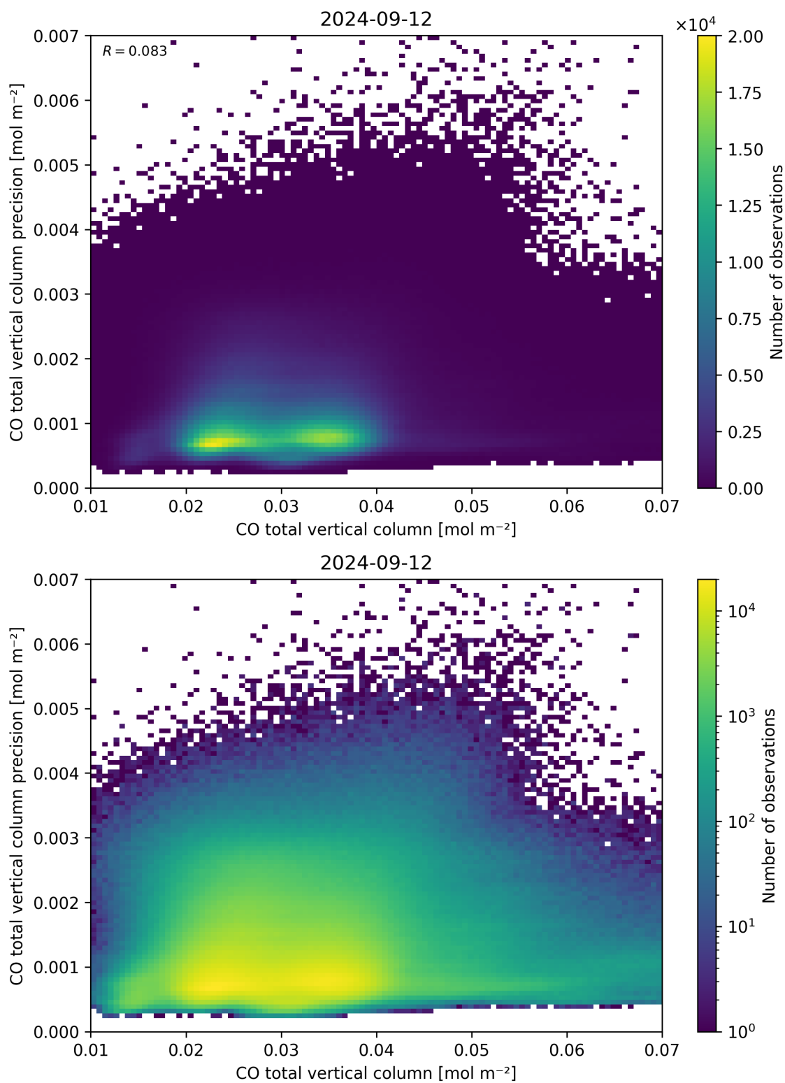
Figure 34: Scatter density plot of “CO total vertical column” against “CO total vertical column precision” for 2024-09-12 to 2024-09-13.
