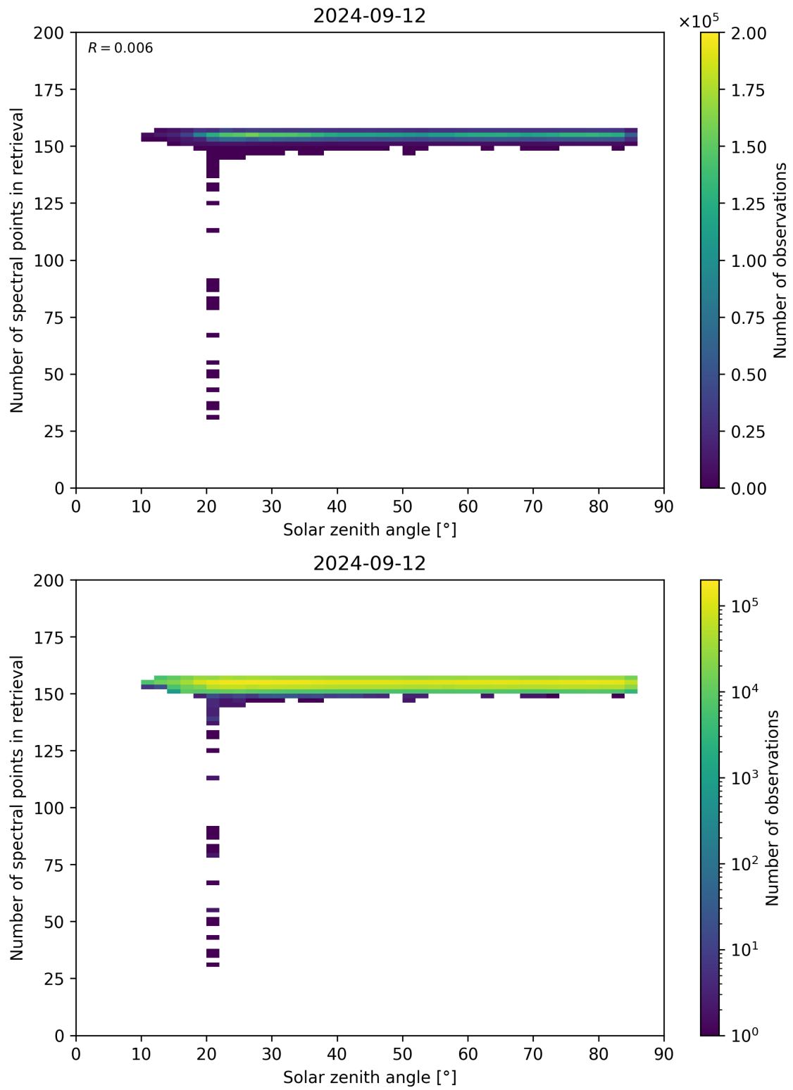
Figure 68: Scatter density plot of “Solar zenith angle” against “Number of spectral points in retrieval” for 2024-09-12 to 2024-09-13.
