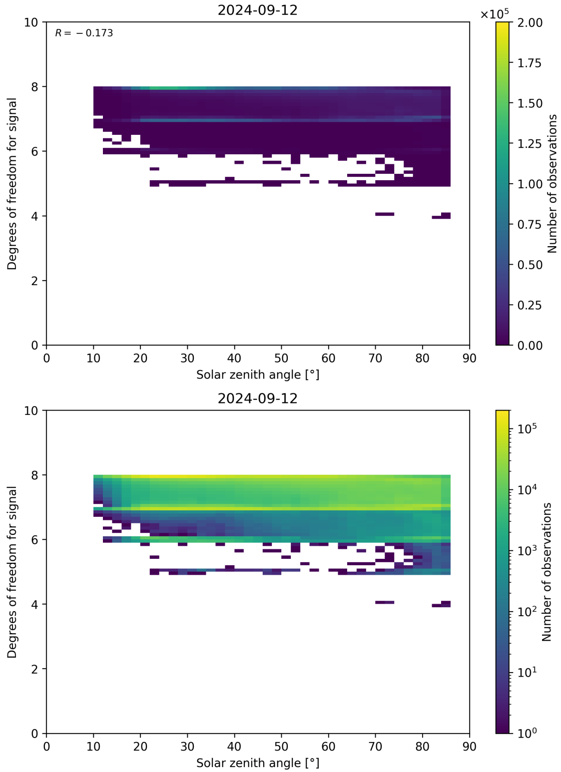
Figure 65: Scatter density plot of “Solar zenith angle” against “Degrees of freedom for signal” for 2024-09-12 to 2024-09-13.
