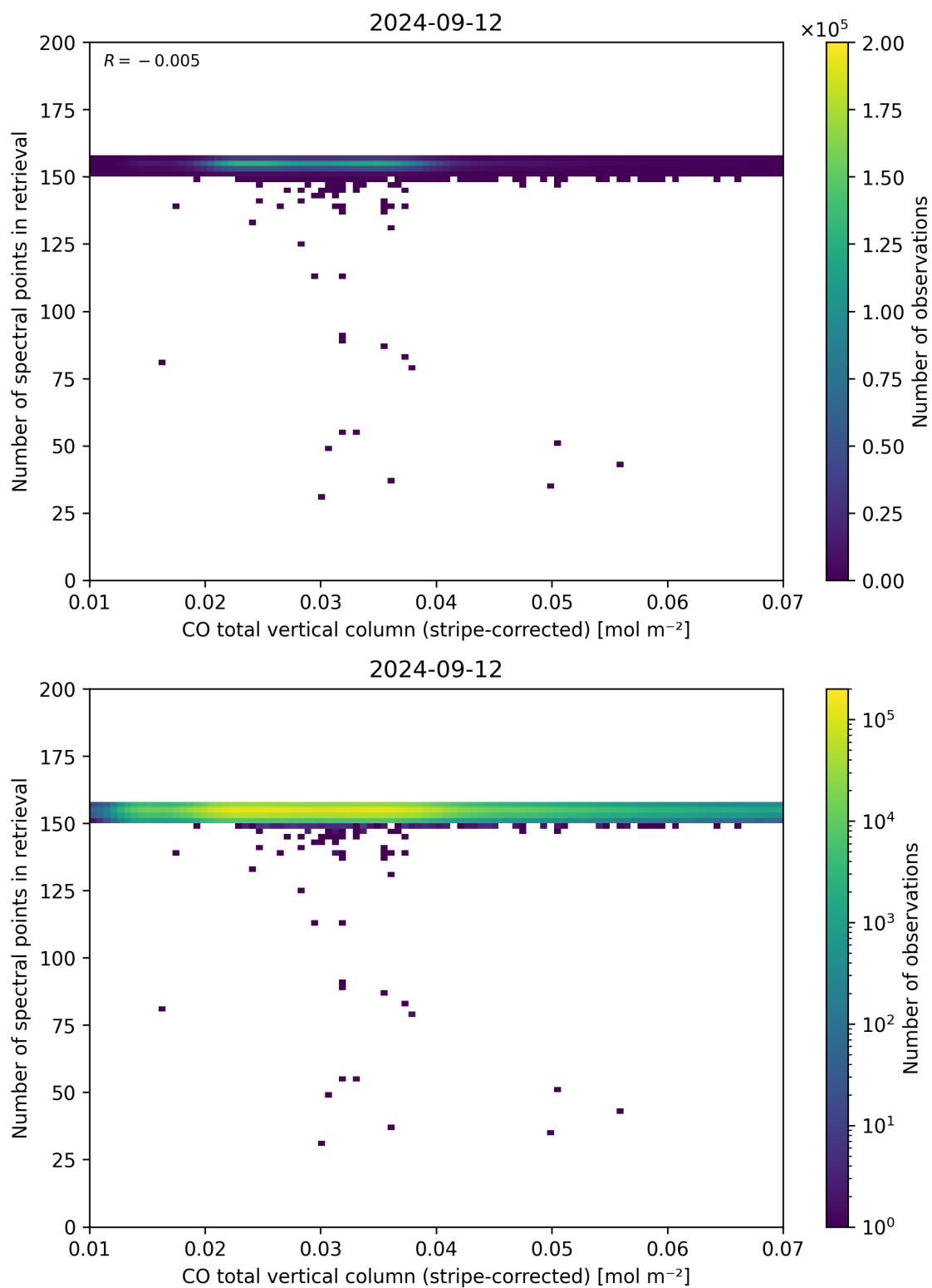
Figure 40: Scatter density plot of “CO total vertical column (stripe-corrected)” against “Number of spectral points in retrieval” for 2024-09-12 to 2024-09-13.
