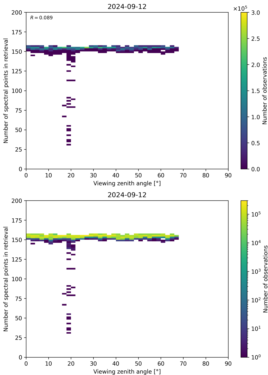
Figure 76: Scatter density plot of “Viewing zenith angle” against “Number of spectral points in retrieval” for 2024-09-12 to 2024-09-13.
