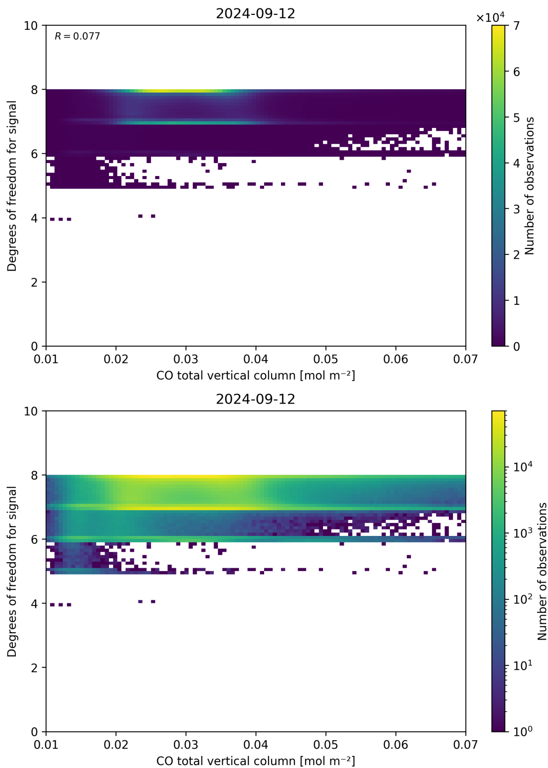
Figure 41: Scatter density plot of “CO total vertical column” against “Degrees of freedom for signal” for 2024-09-12 to 2024-09-13.
