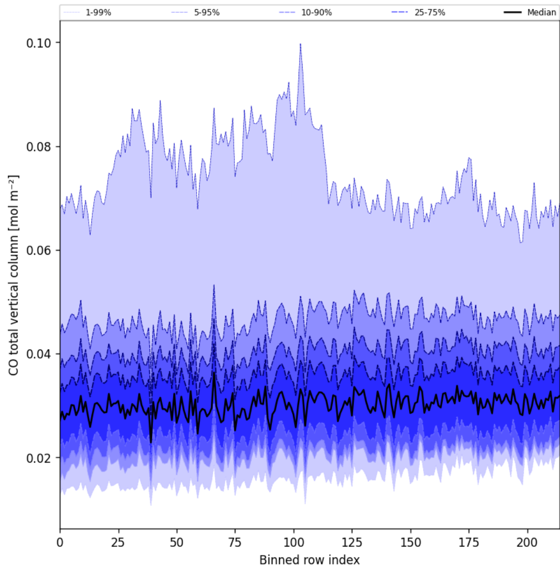
Figure 26: Along track statistics of “CO total vertical column” for 2024-09-12 to 2024-09-13
