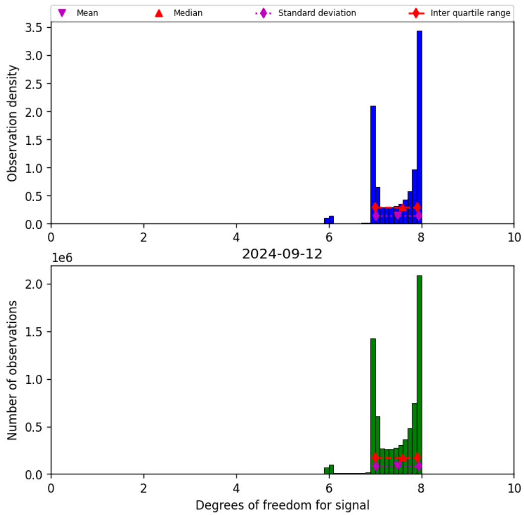
Figure 23: Histogram of “Degrees of freedom for signal” for 2024-09-12 to 2024-09-13
