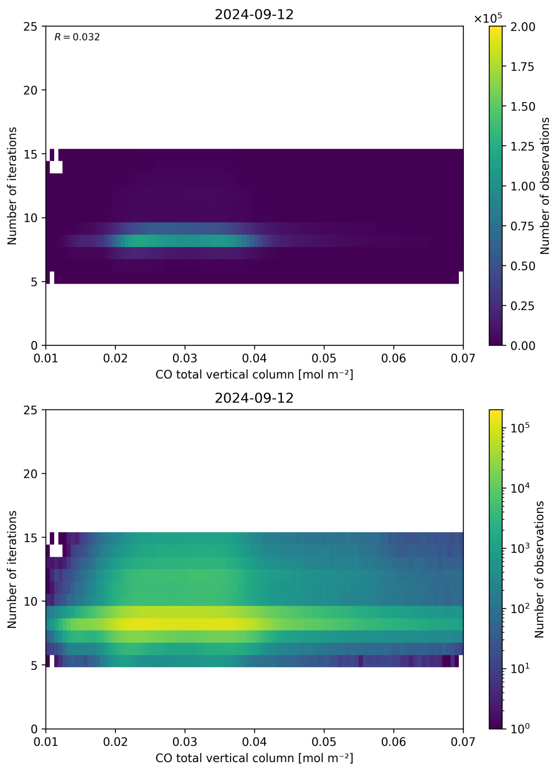
Figure 42: Scatter density plot of “CO total vertical column” against “Number of iterations” for 2024-09-12 to 2024-09-13.
