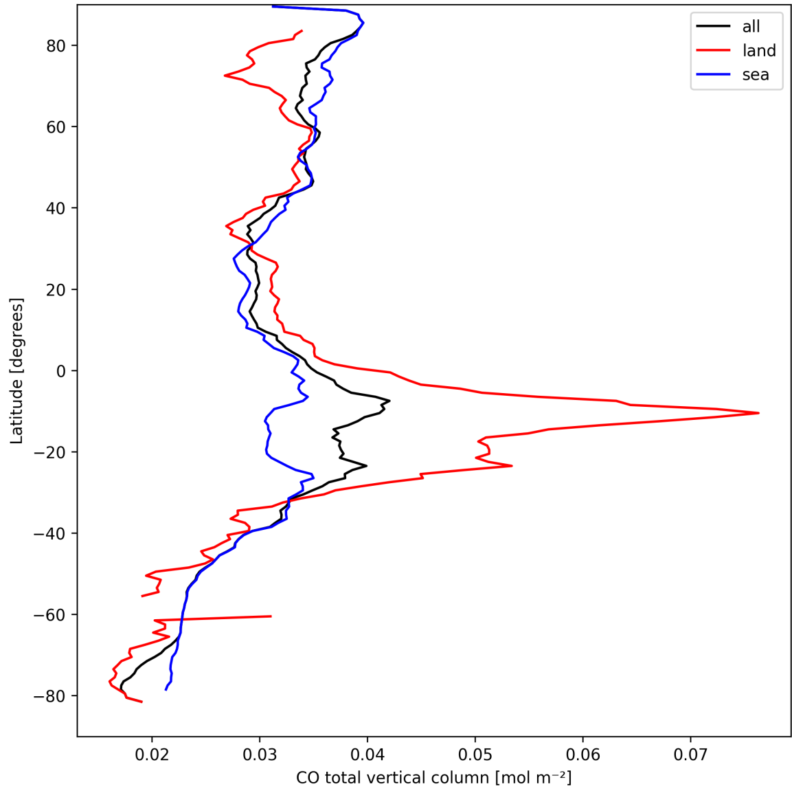
Figure 10: Zonal average of “CO total vertical column” for 2024-09-12 to 2024-09-13.
