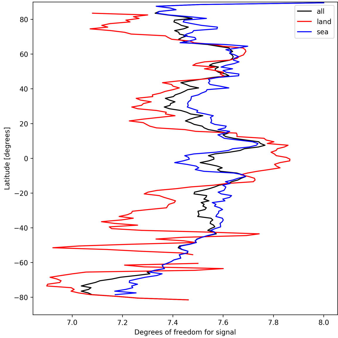
Figure 15: Zonal average of “Degrees of freedom for signal” for 2024-09-12 to 2024-09-13.
