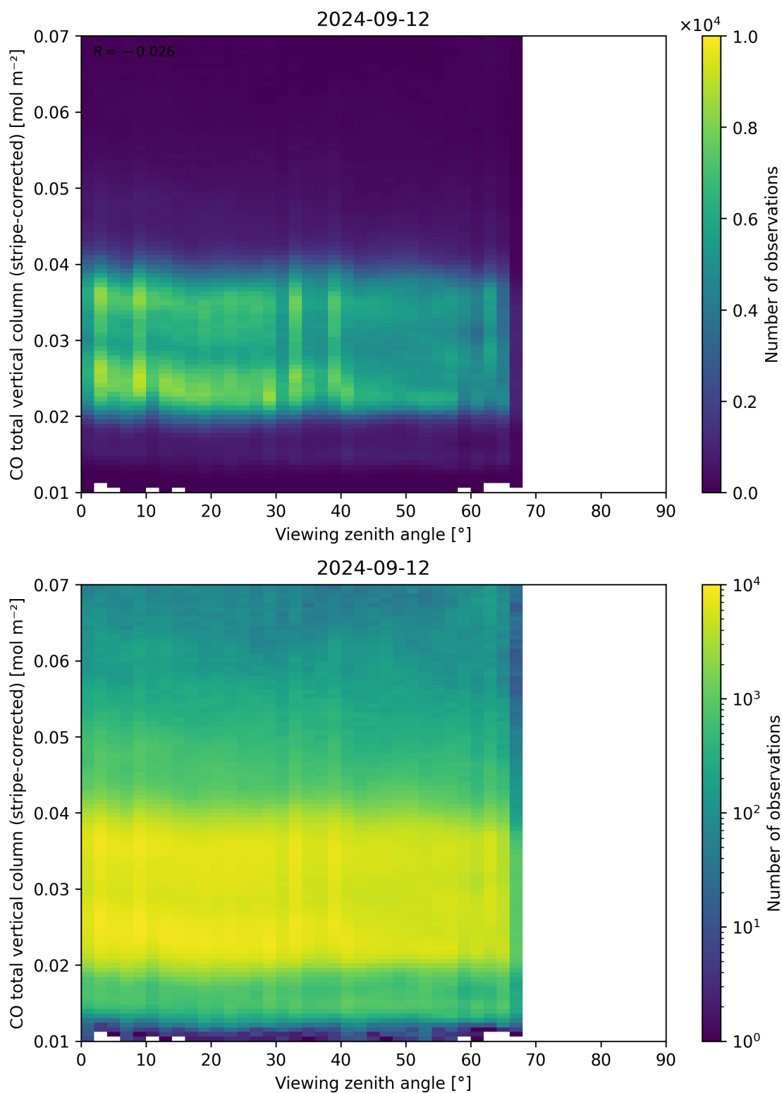
Figure 70: Scatter density plot of “Viewing zenith angle” against “CO total vertical column (stripe-corrected)” for 2024-09-12 to 2024-09-13.
