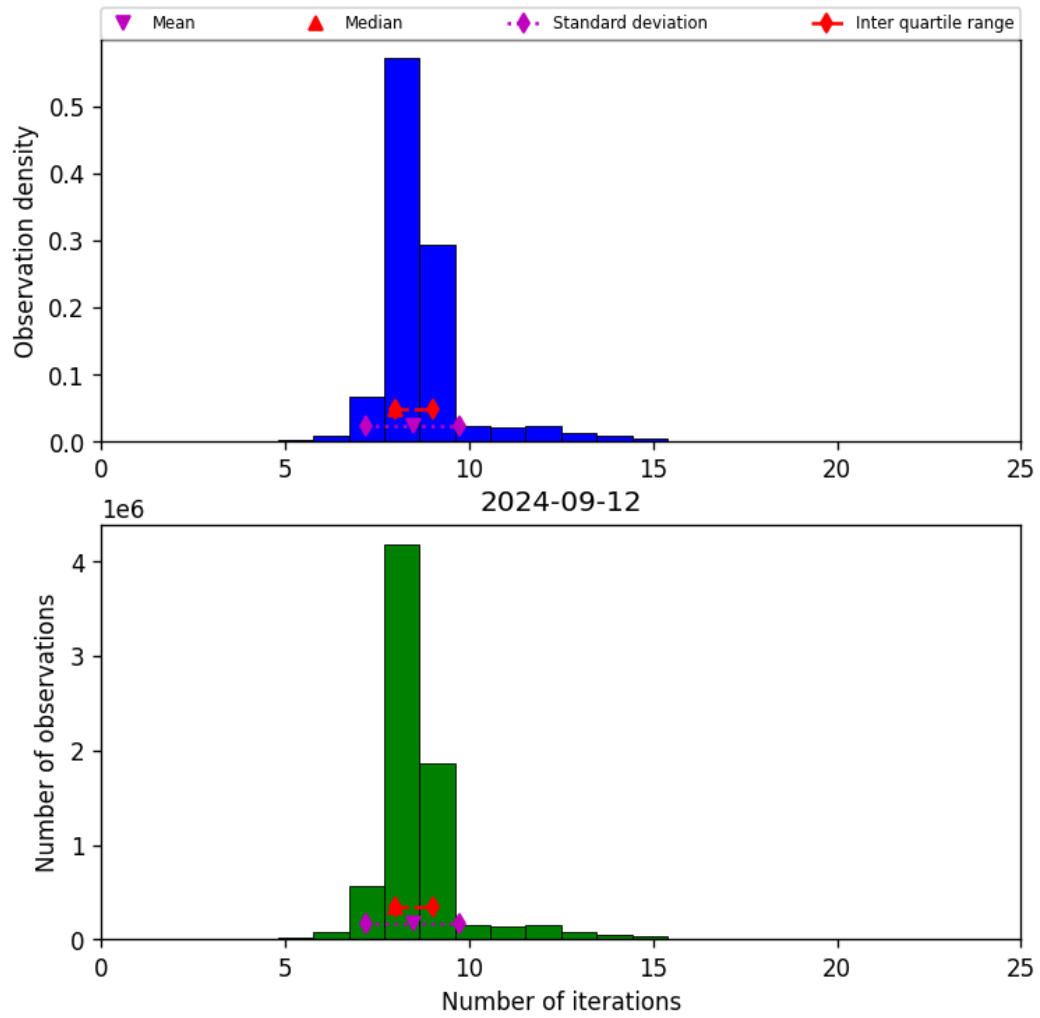
Figure 24: Histogram of “Number of iterations” for 2024-09-12 to 2024-09-13
