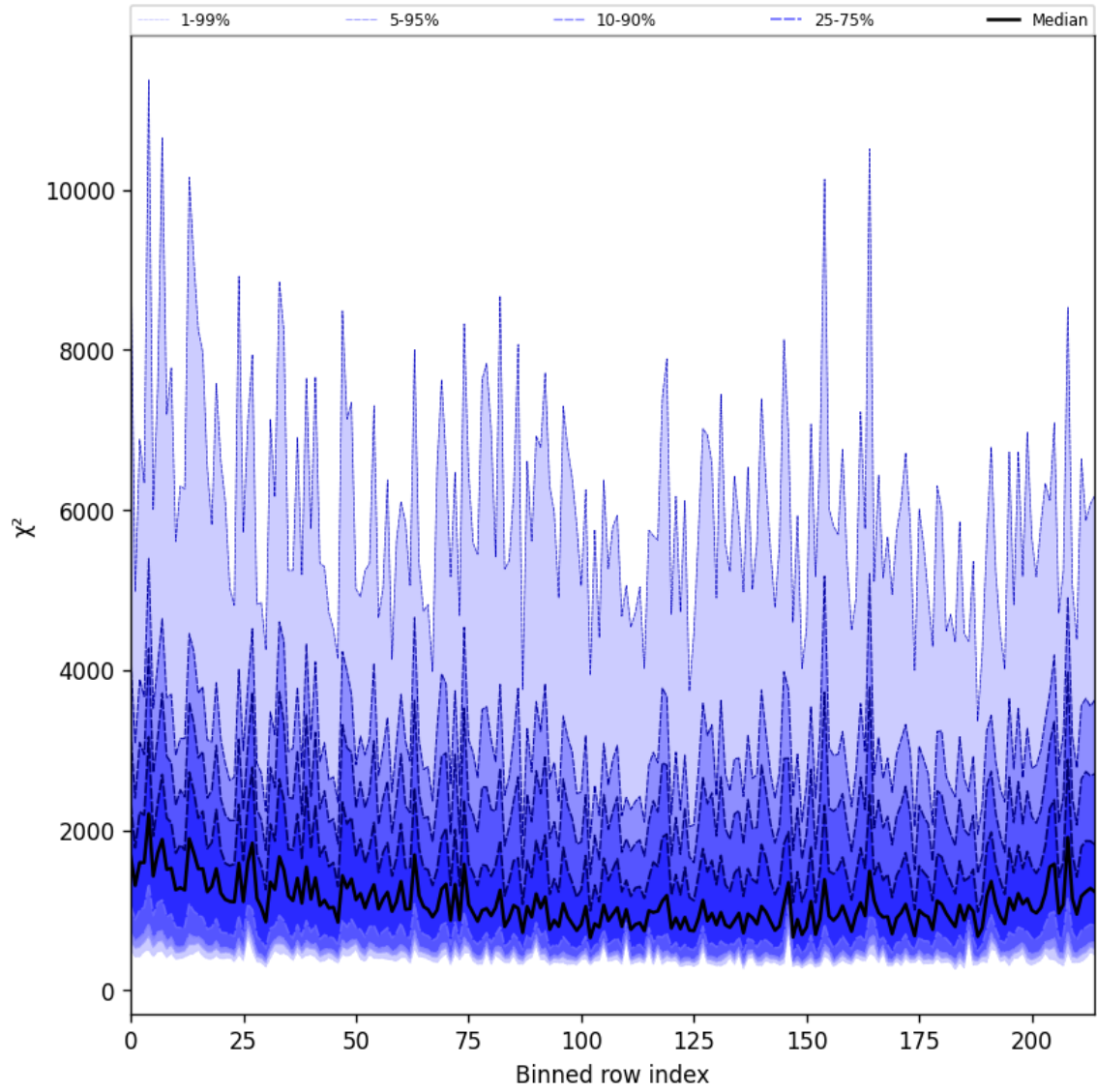
Figure 30: Along track statistics of “ \chi^2 ” for 2024-09-12 to 2024-09-13
