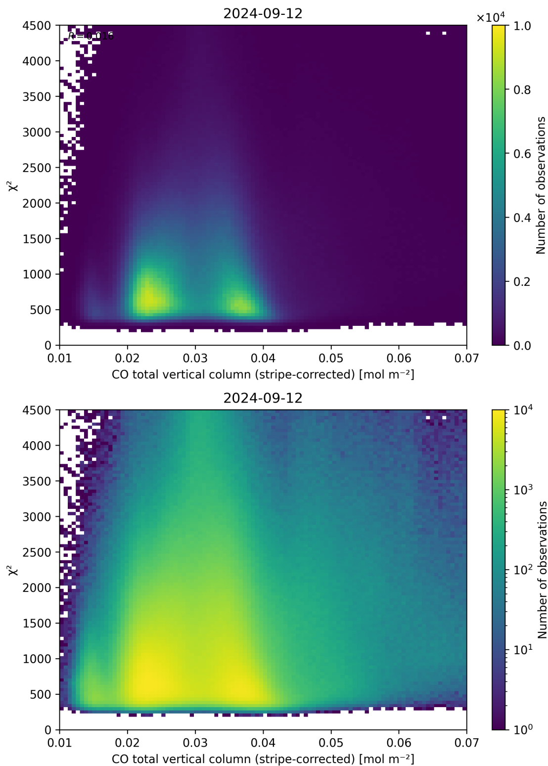
Figure 37: Scatter density plot of “CO total vertical column (stripe-corrected)” against “ \chi^2 ” for 2024-09-12 to 2024-09-13.
