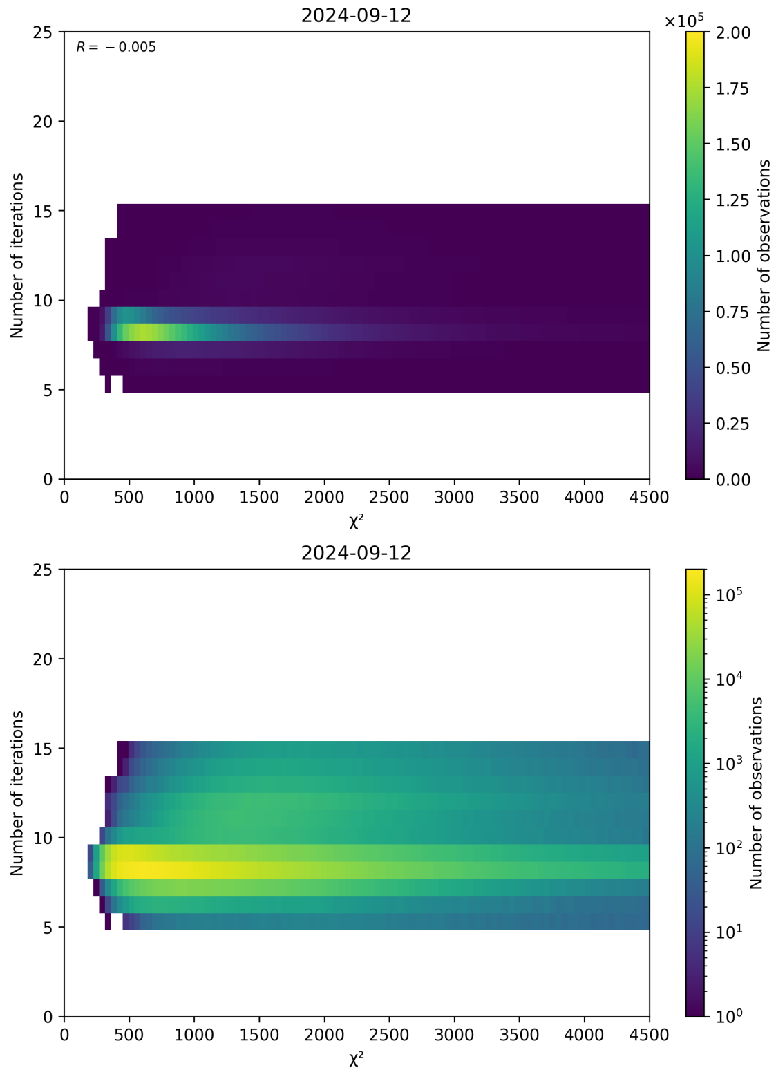
Figure 49: Scatter density plot of “ \chi^2 ” against “Number of iterations” for 2024-09-12 to 2024-09-13.
