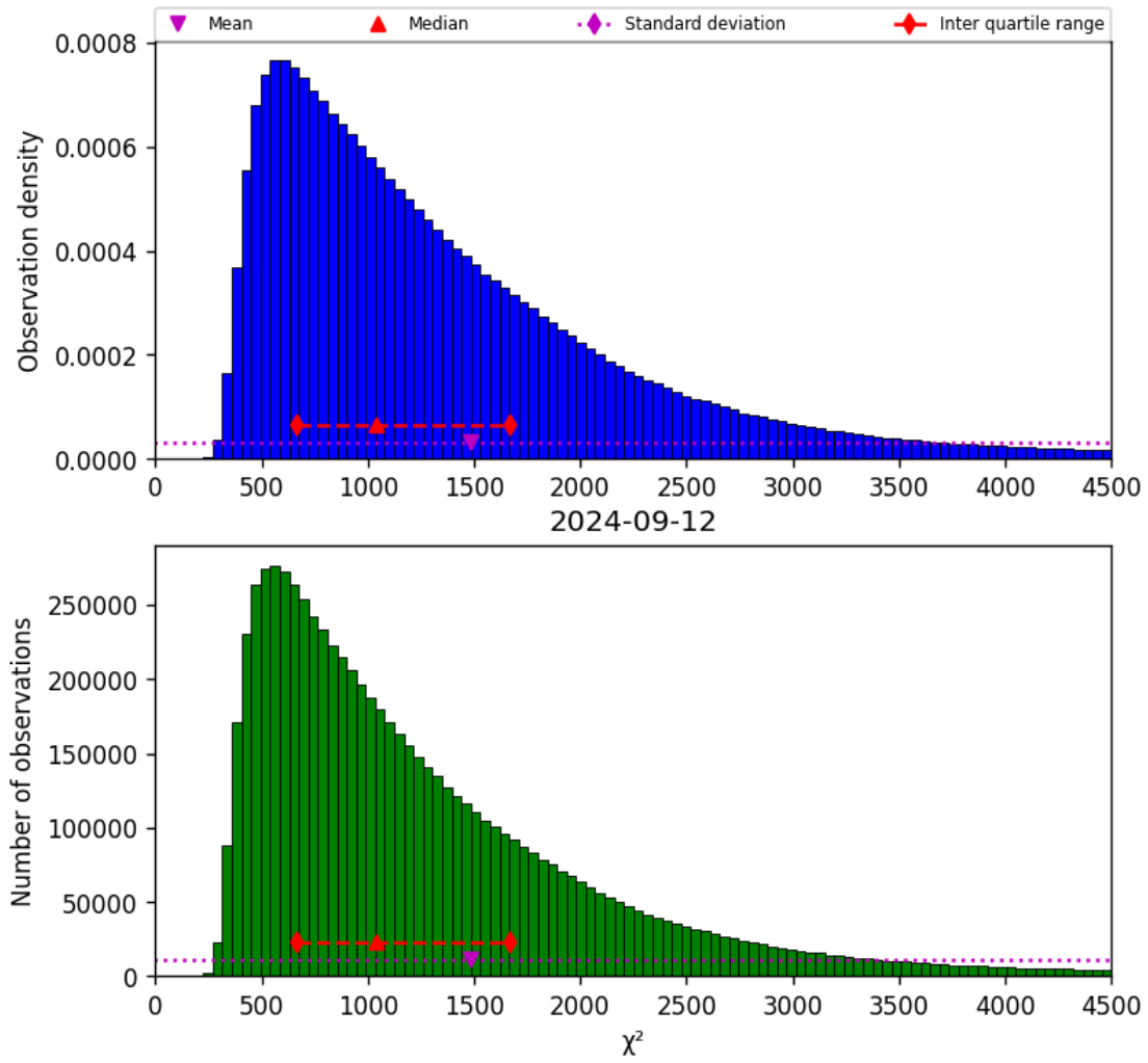
Figure 22: Histogram of “ \chi^2 ” for 2024-09-12 to 2024-09-13
