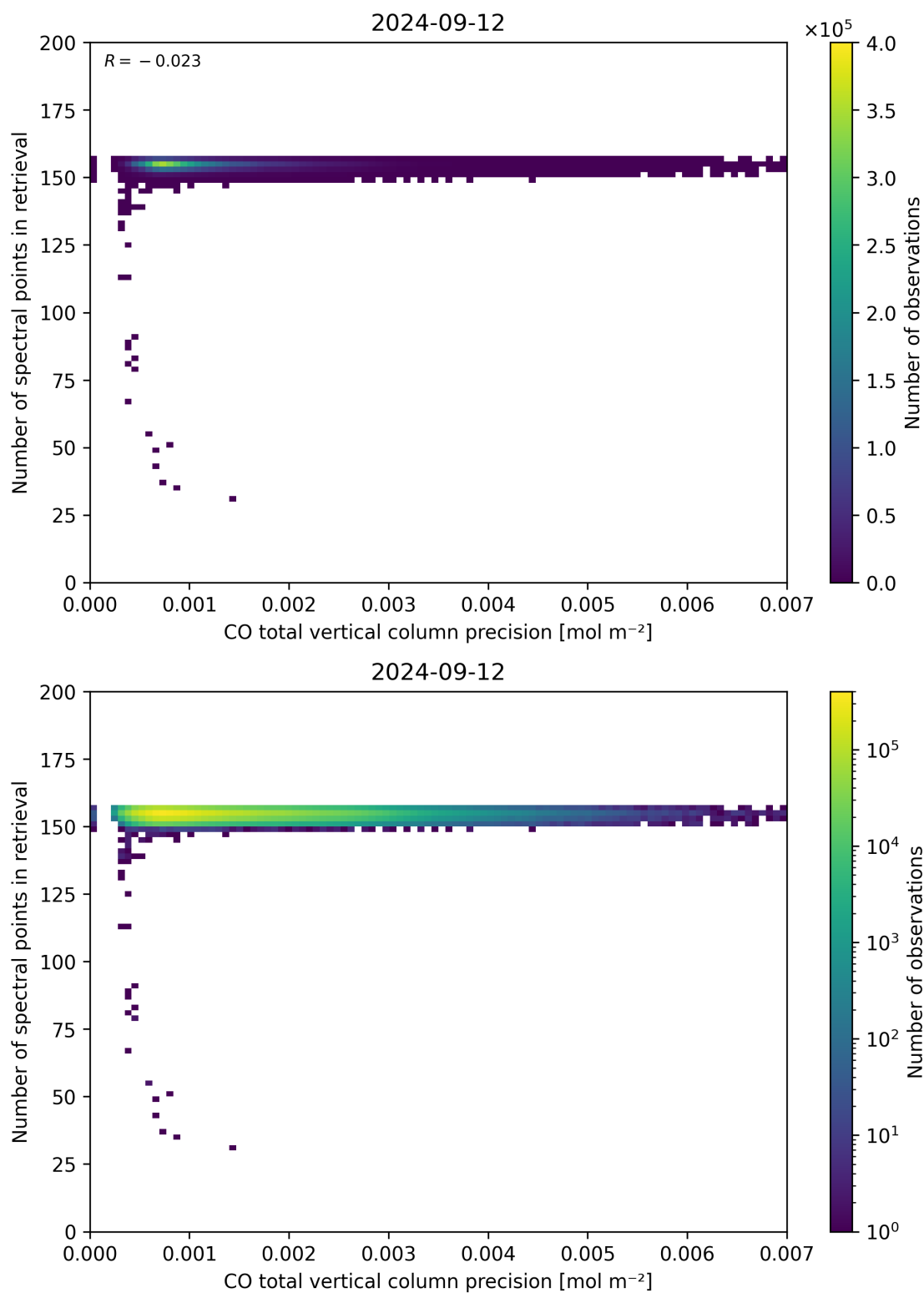
Figure 47: Scatter density plot of “CO total vertical column precision” against “Number of spectral points in retrieval” for 2024-09-12 to 2024-09-13.
