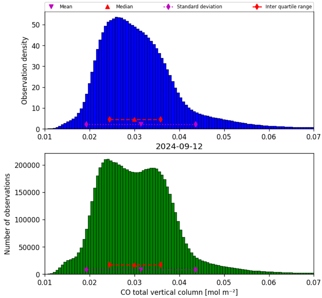
Figure 18: Histogram of “CO total vertical column” for 2024-09-12 to 2024-09-13
