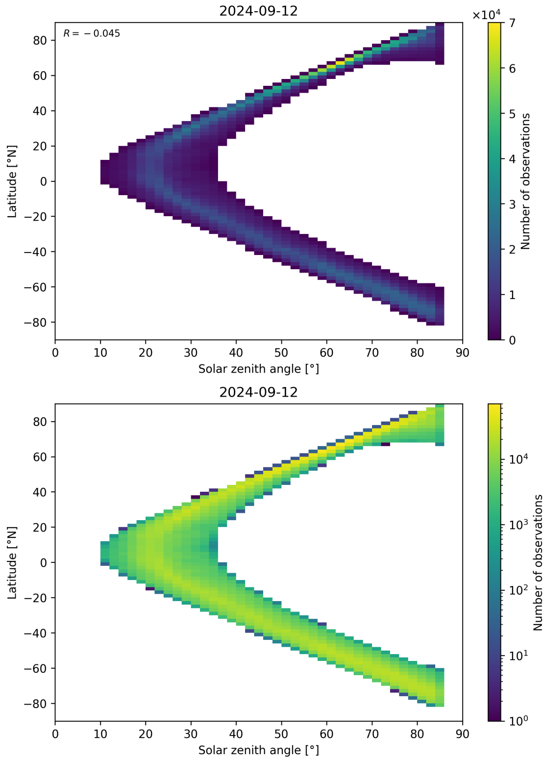
Figure 66: Scatter density plot of “Solar zenith angle” against “Latitude” for 2024-09-12 to 2024-09-13.
