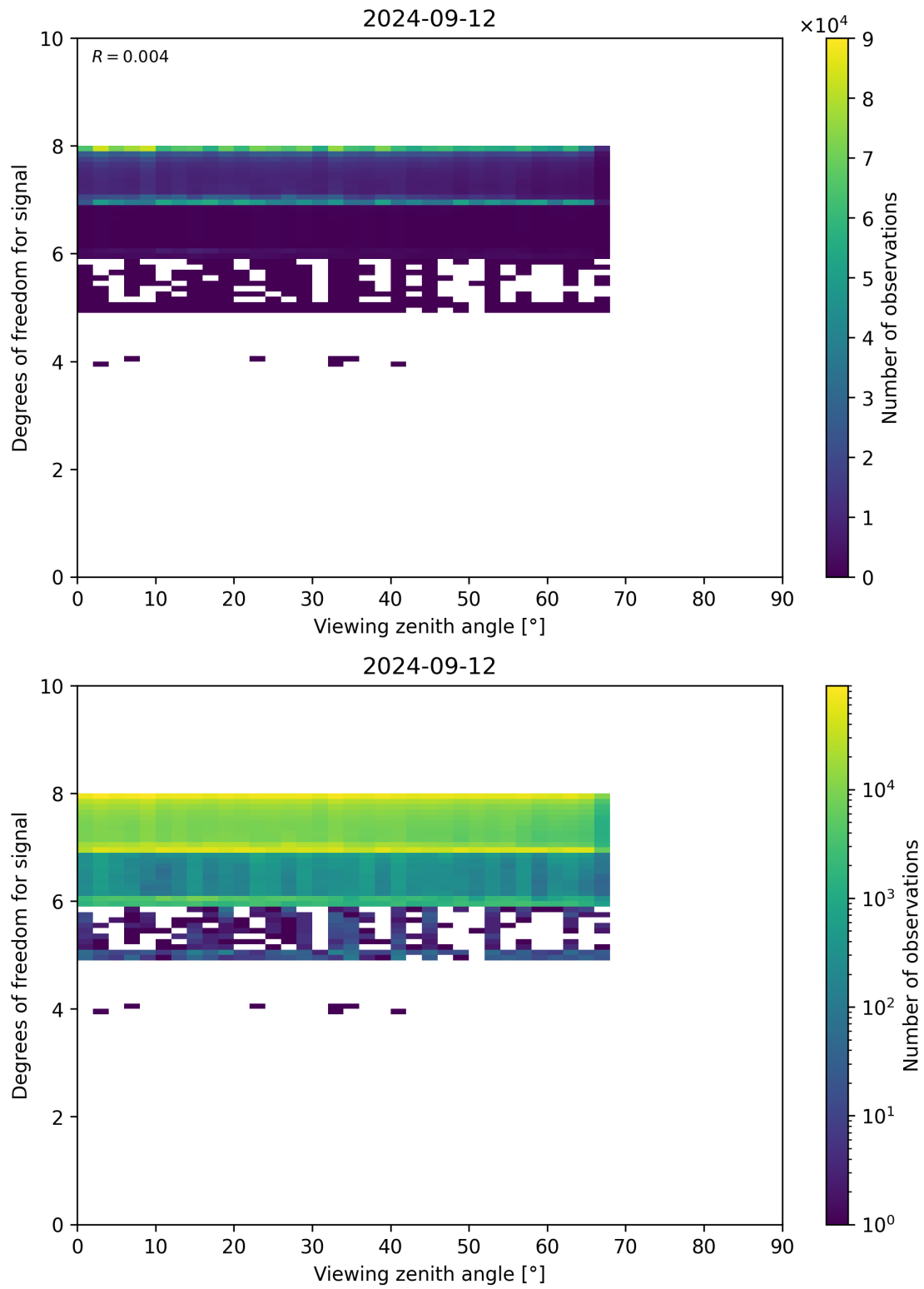
Figure 73: Scatter density plot of “Viewing zenith angle” against “Degrees of freedom for signal” for 2024-09-12 to 2024-09-13.
