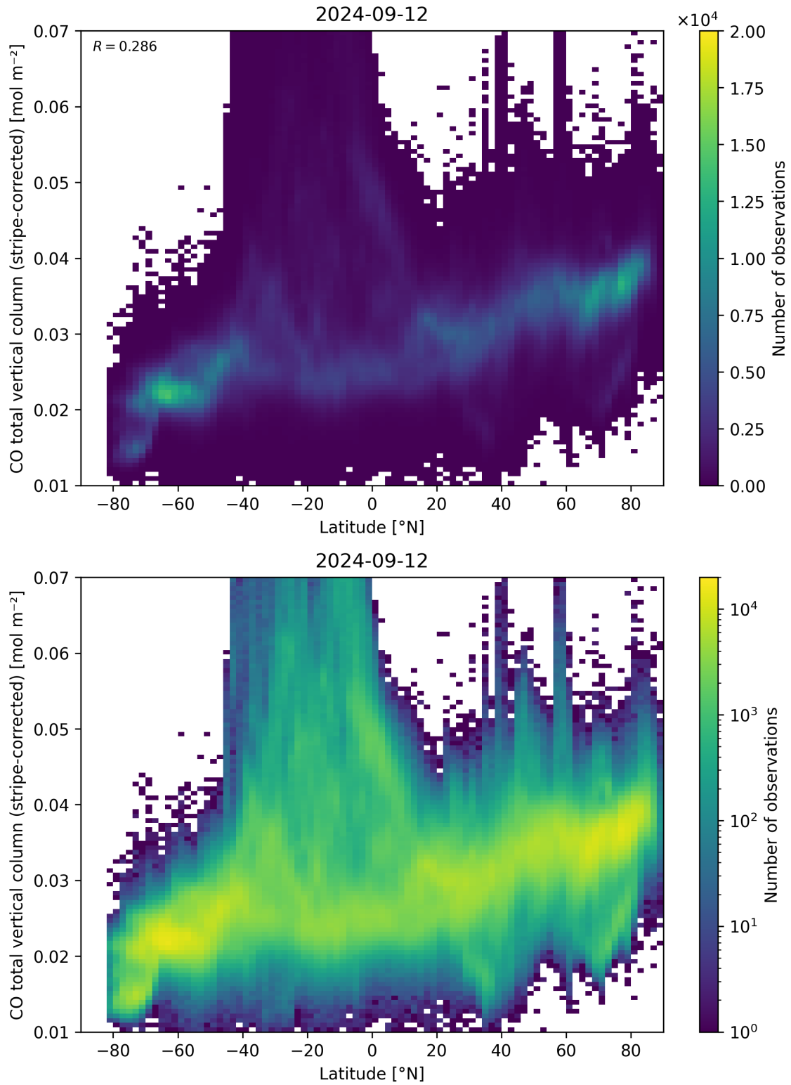
Figure 52: Scatter density plot of “Latitude” against “CO total vertical column (stripe-corrected)” for 2024-09-12 to 2024-09-13.
