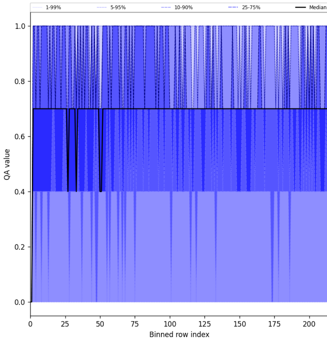
Figure 25: Along track statistics of “QA value” for 2024-09-12 to 2024-09-13
