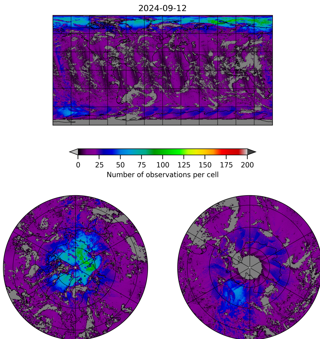
Figure 8: Map of the number of observations for 2024-09-12 to 2024-09-13
