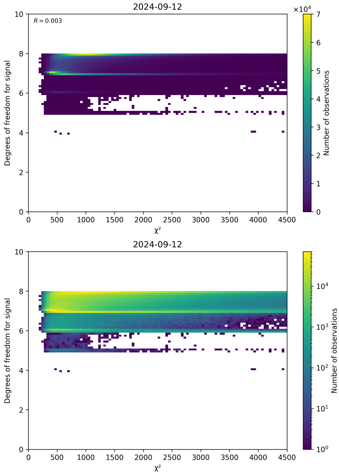
Figure 48: Scatter density plot of “ \chi^2 ” against “Degrees of freedom for signal” for 2024-09-12 to 2024-09-13.
