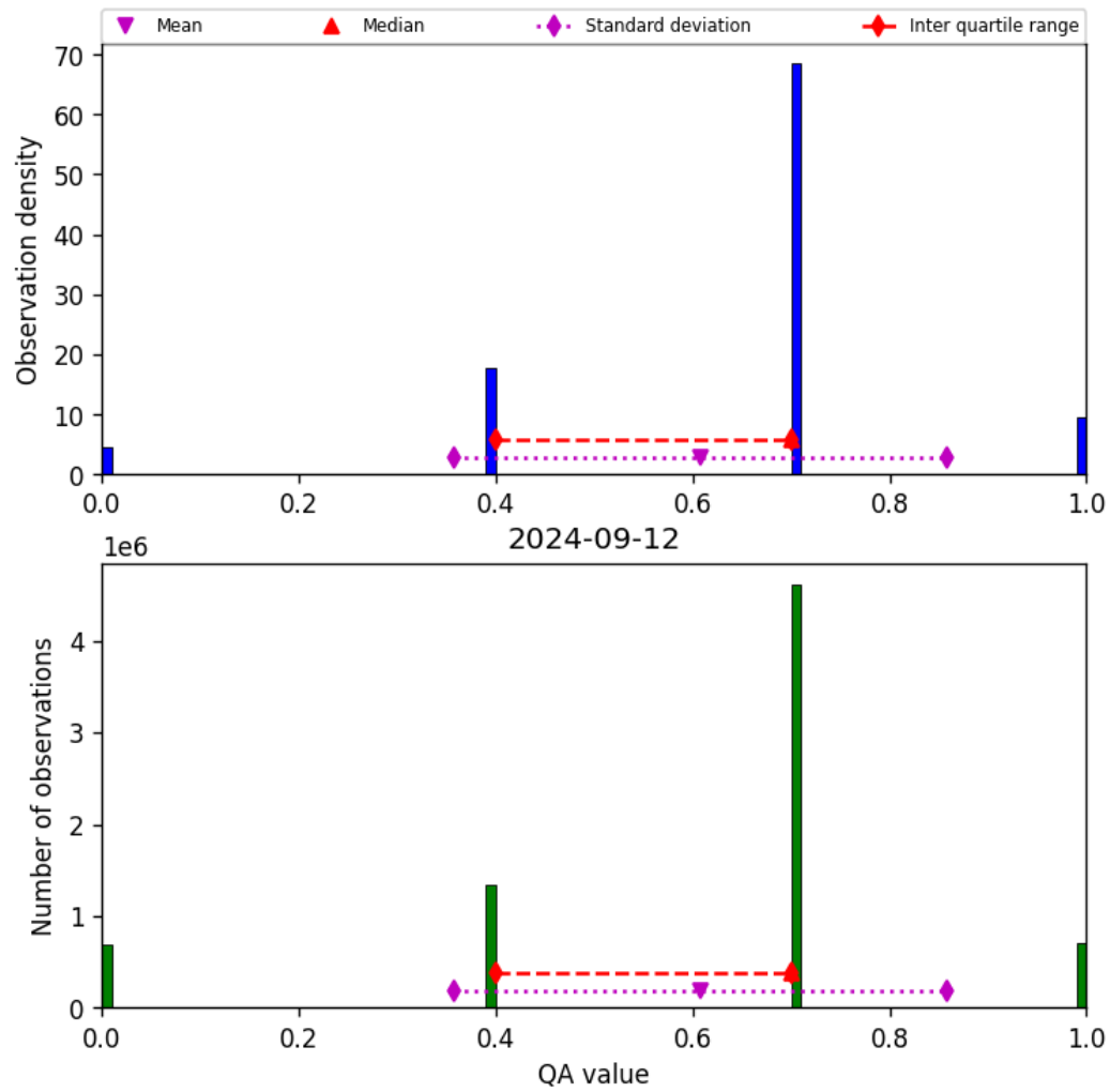
Figure 17: Histogram of “QA value” for 2024-09-12 to 2024-09-13
