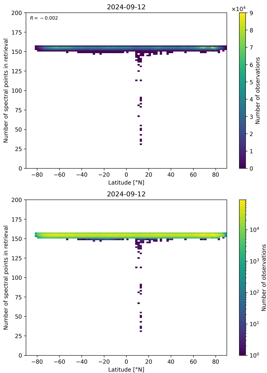
Figure 57: Scatter density plot of “Latitude” against “Number of spectral points in retrieval” for 2024-09-12 to 2024-09-13.
