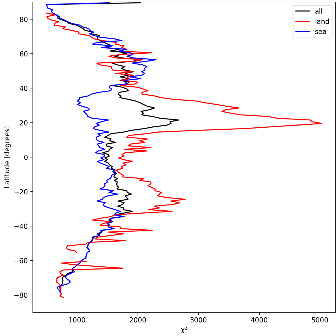
Figure 14: Zonal average of “ \chi^2 ” for 2024-09-12 to 2024-09-13.
