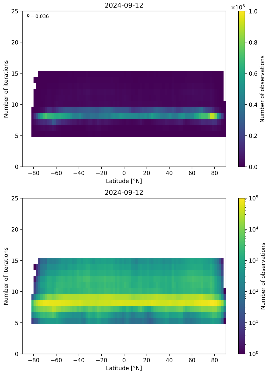
Figure 56: Scatter density plot of “Latitude” against “Number of iterations” for 2024-09-12 to 2024-09-13.
