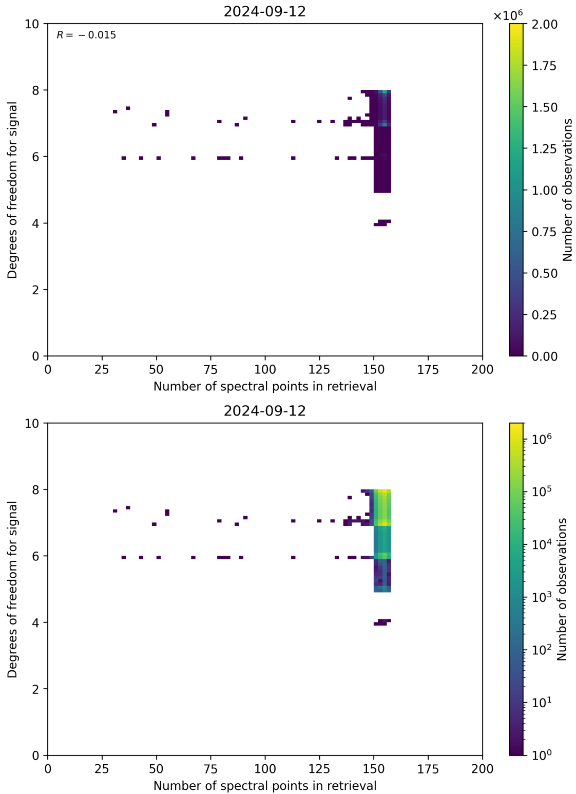
Figure 59: Scatter density plot of “Number of spectral points in retrieval” against “Degrees of freedom for signal” for 2024-09-12 to 2024-09-13.
