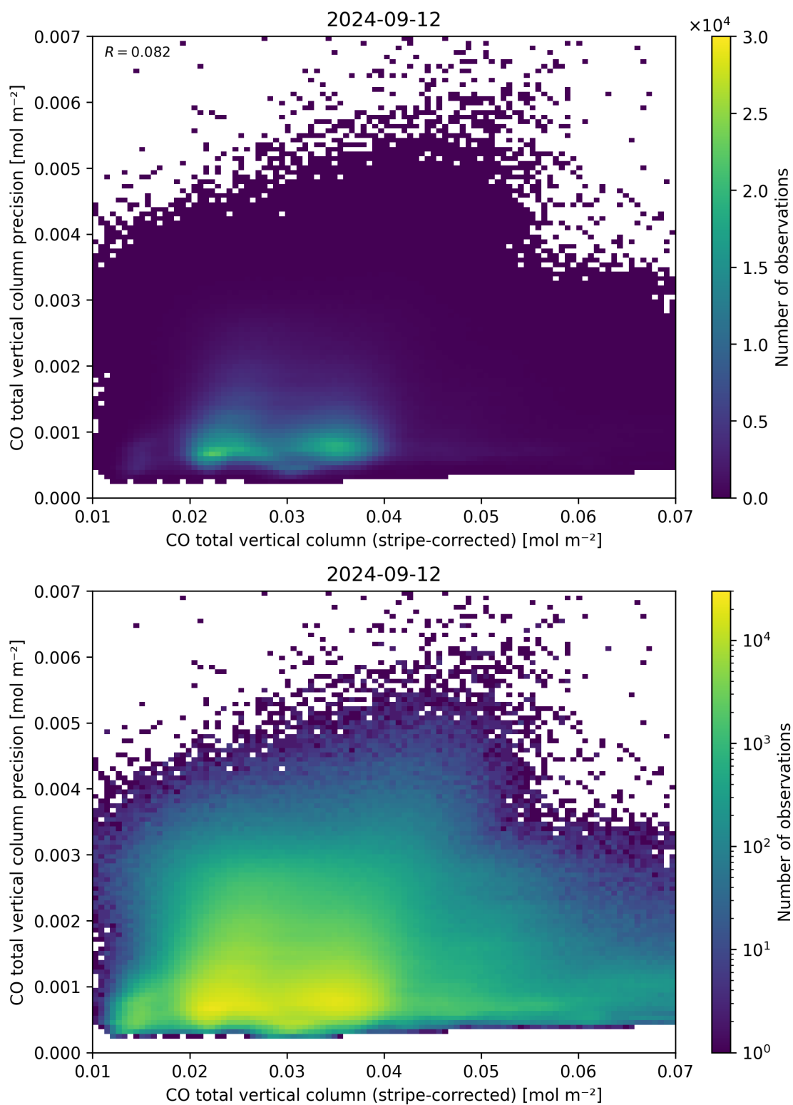
Figure 36: Scatter density plot of “CO total vertical column (stripe-corrected)” against “CO total vertical column precision” for 2024-09-12 to 2024-09-13.
