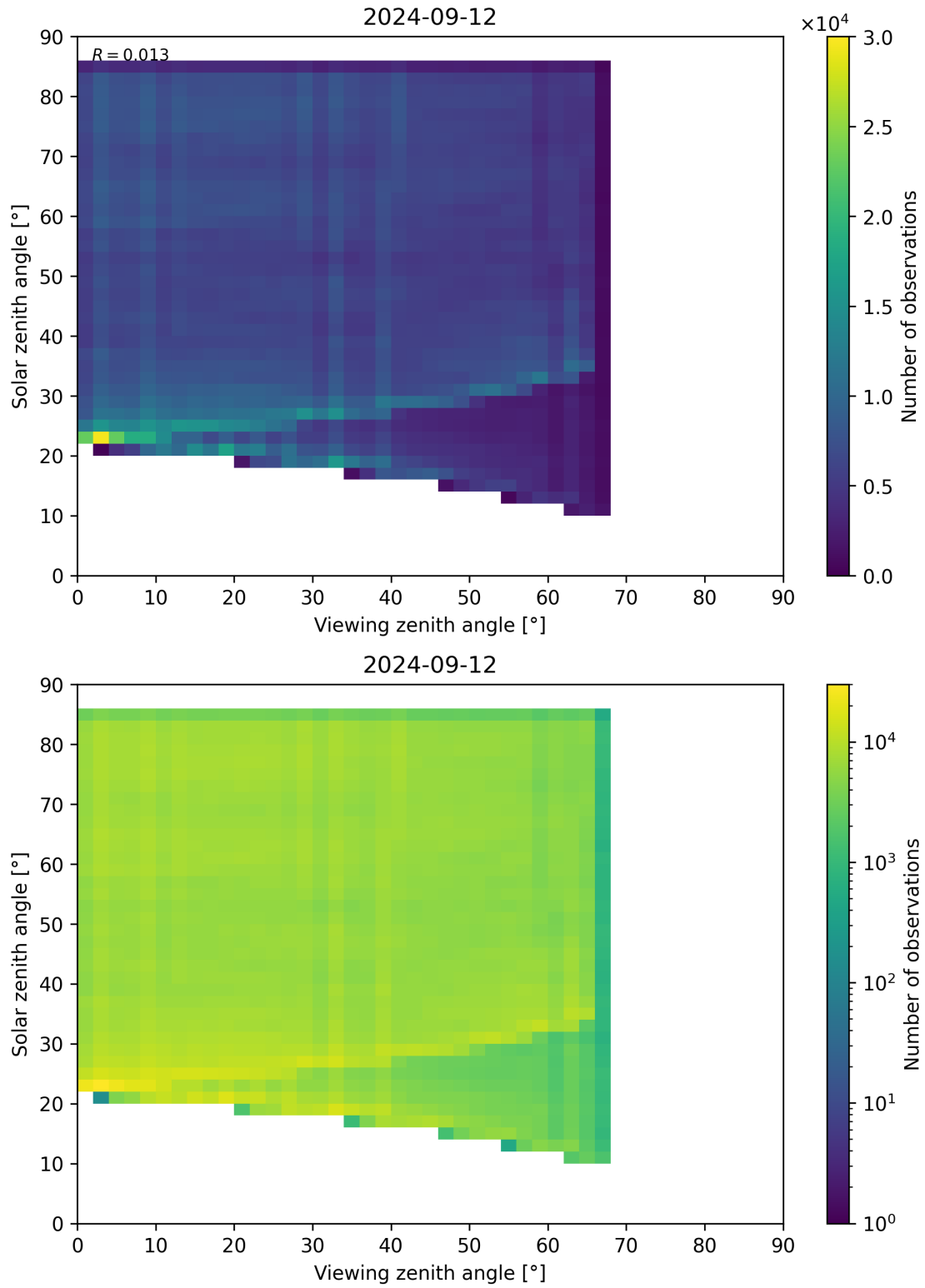
Figure 77: Scatter density plot of “Viewing zenith angle” against “Solar zenith angle” for 2024-09-12 to 2024-09-13.
