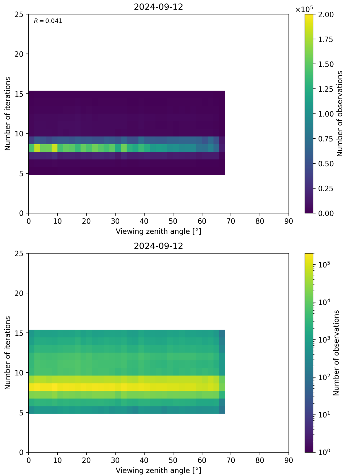
Figure 75: Scatter density plot of “Viewing zenith angle” against “Number of iterations” for 2024-09-12 to 2024-09-13.
