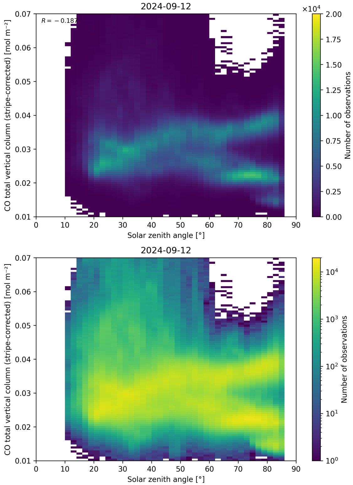
Figure 62: Scatter density plot of “Solar zenith angle” against “CO total vertical column (stripe-corrected)” for 2024-09-12 to 2024-09-13.
