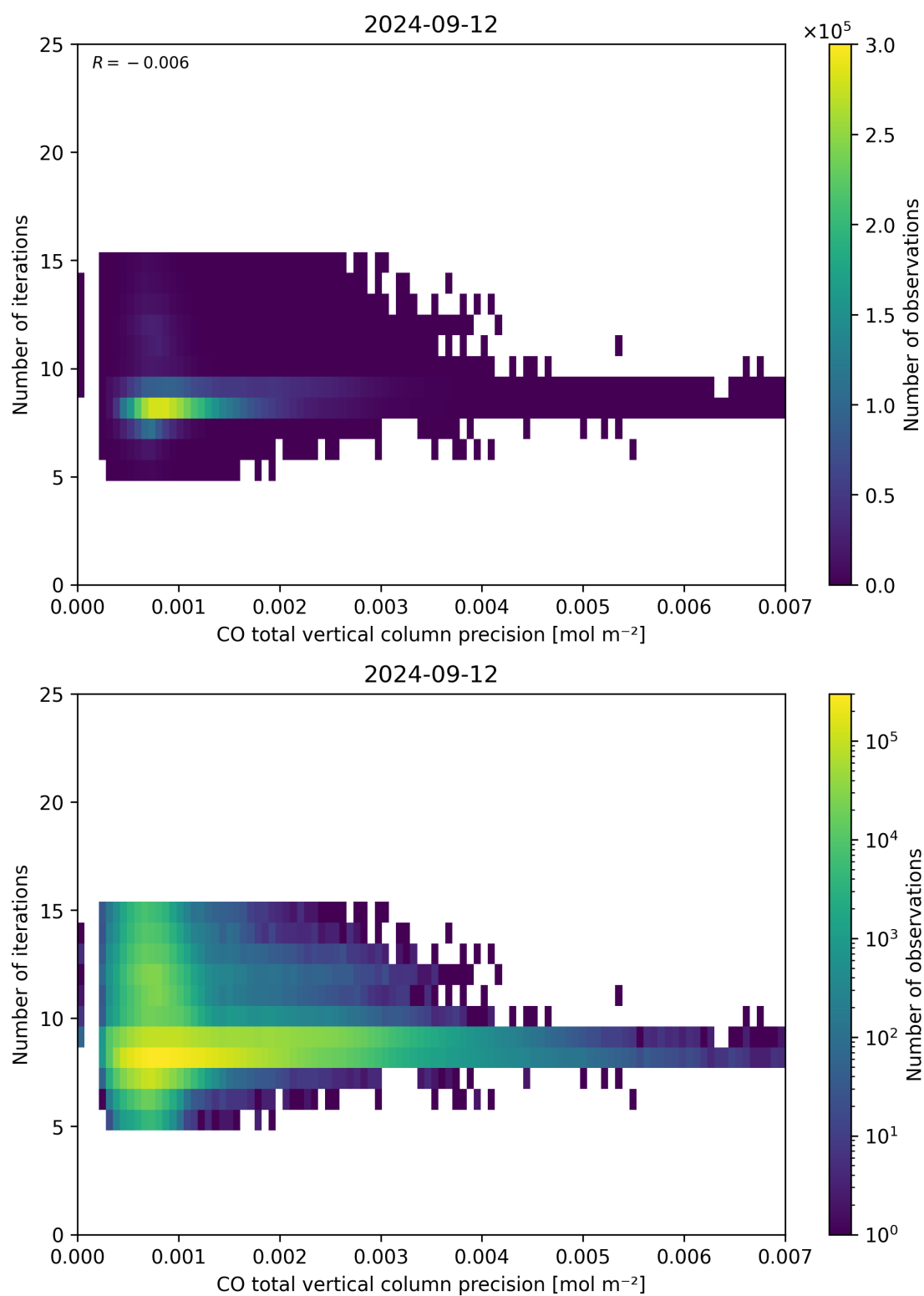
Figure 46: Scatter density plot of “CO total vertical column precision” against “Number of iterations” for 2024-09-12 to 2024-09-13.
