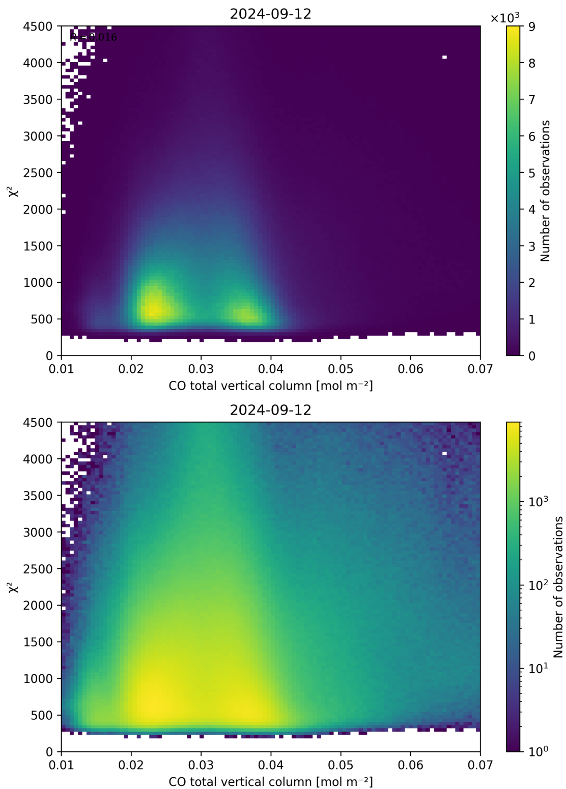
Figure 35: Scatter density plot of “CO total vertical column” against “ \chi^2 ” for 2024-09-12 to 2024-09-13.
