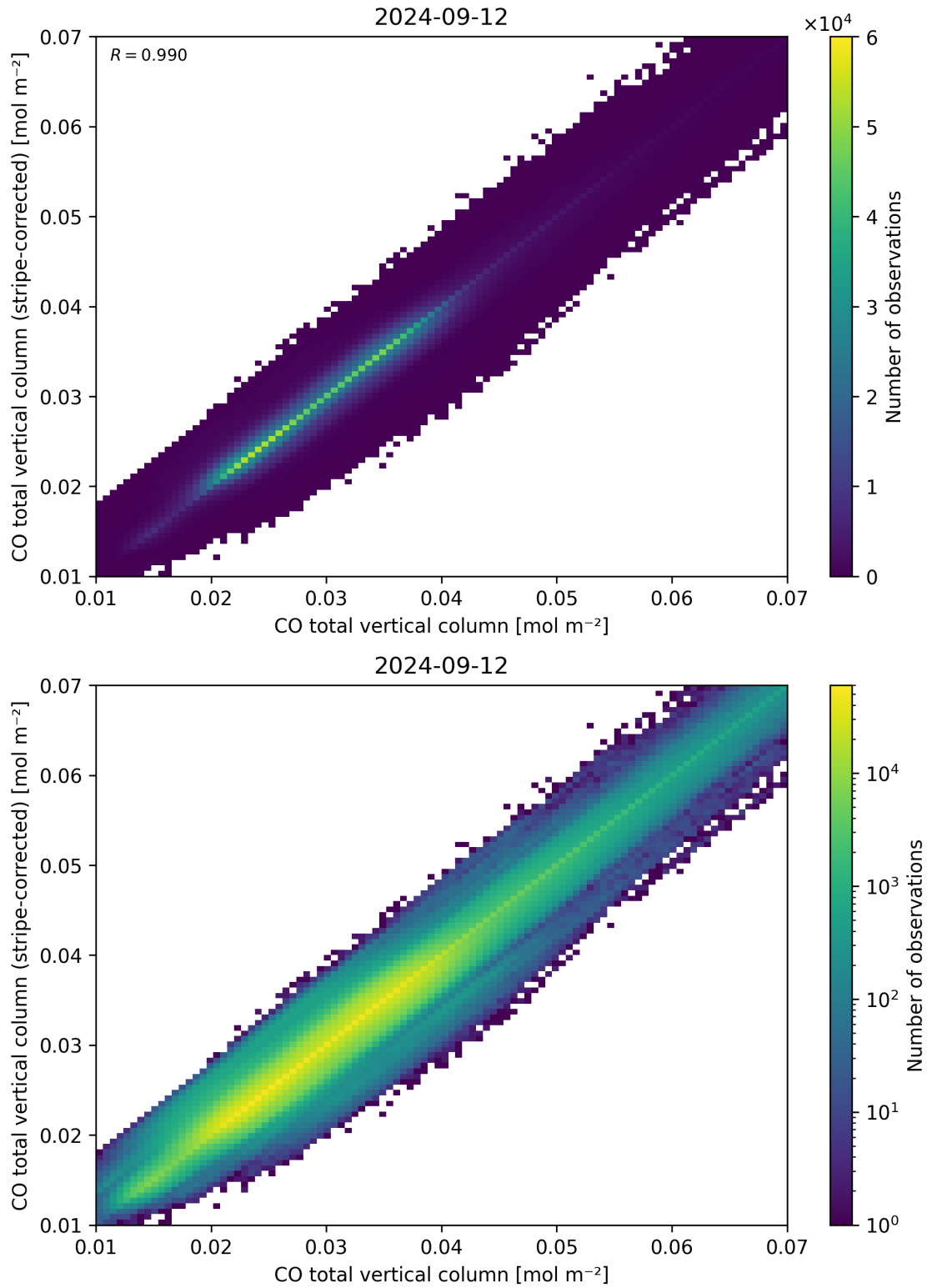
Figure 33: Scatter density plot of “CO total vertical column” against “CO total vertical column (stripe-corrected)” for 2024-09-12 to 2024-09-13.
