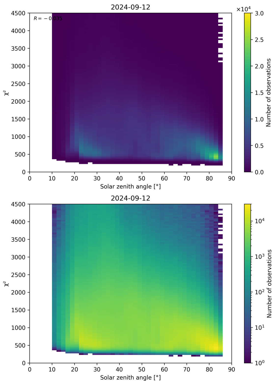
Figure 64: Scatter density plot of “Solar zenith angle” against “ \chi^2 ” for 2024-09-12 to 2024-09-13.
