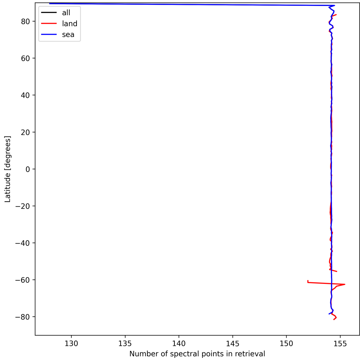
Figure 13: Zonal average of “Number of spectral points in retrieval” for 2024-09-12 to 2024-09-13.
