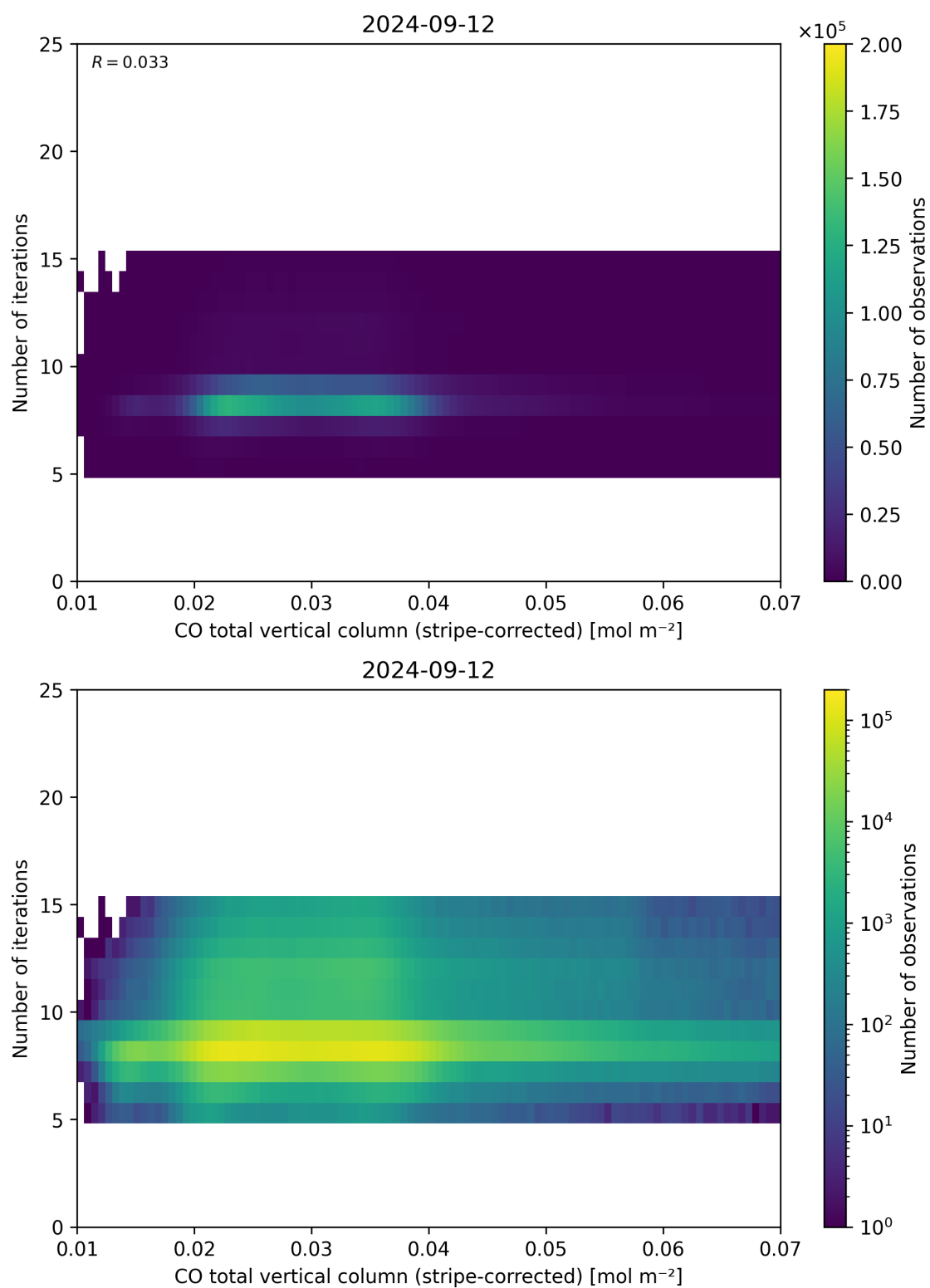
Figure 39: Scatter density plot of “CO total vertical column (stripe-corrected)” against “Number of iterations” for 2024-09-12 to 2024-09-13.
