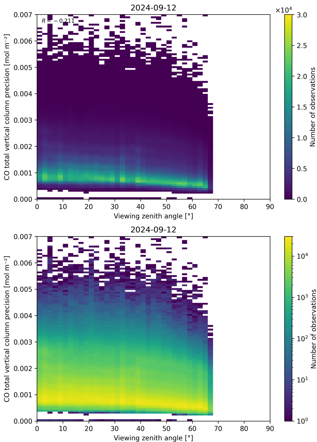
Figure 71: Scatter density plot of “Viewing zenith angle” against “CO total vertical column precision” for 2024-09-12 to 2024-09-13.
