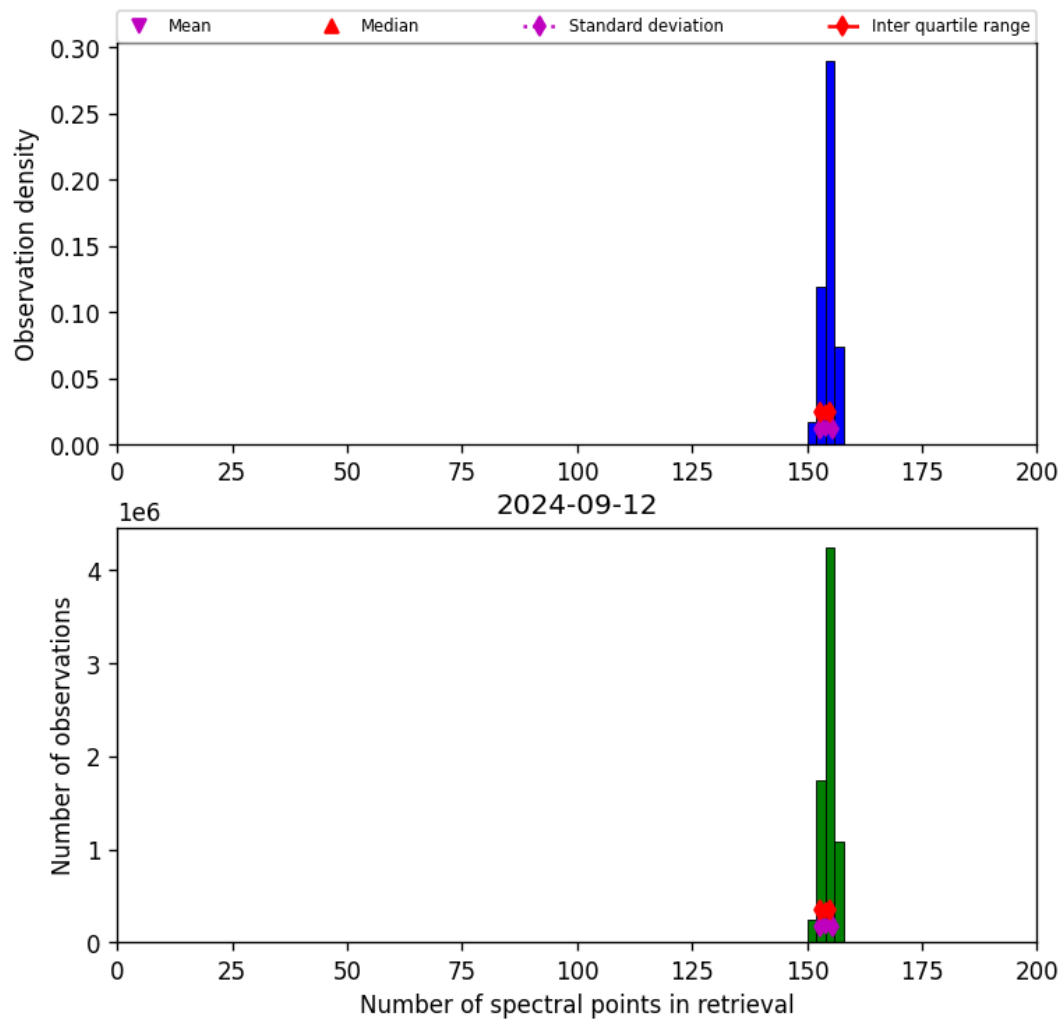
Figure 21: Histogram of “Number of spectral points in retrieval” for 2024-09-12 to 2024-09-13
