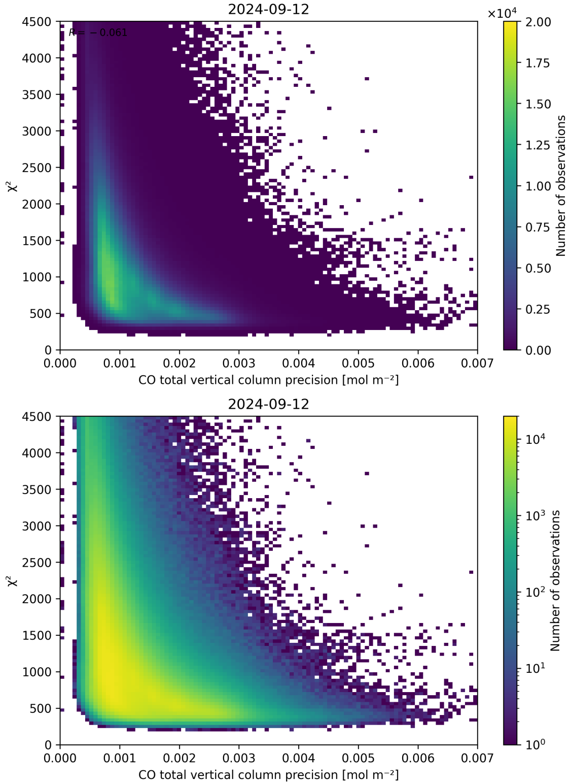
Figure 44: Scatter density plot of “CO total vertical column precision” against “ \chi^2 ” for 2024-09-12 to 2024-09-13.
