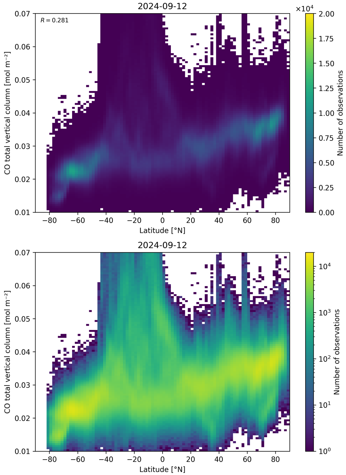
Figure 51: Scatter density plot of “Latitude” against “CO total vertical column” for 2024-09-12 to 2024-09-13.
