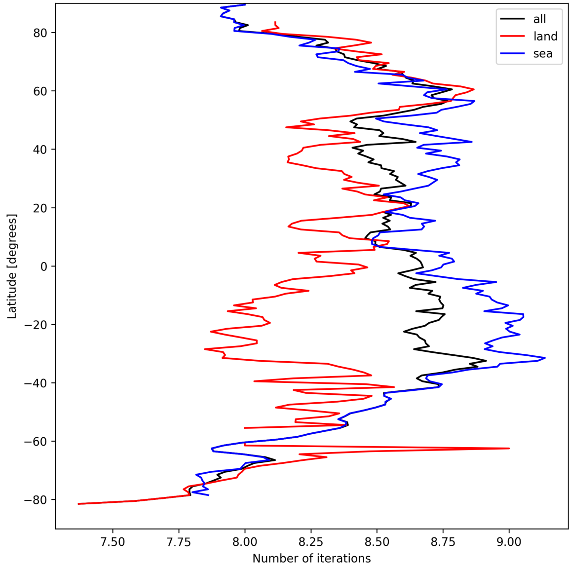
Figure 16: Zonal average of “Number of iterations” for 2024-09-12 to 2024-09-13.
