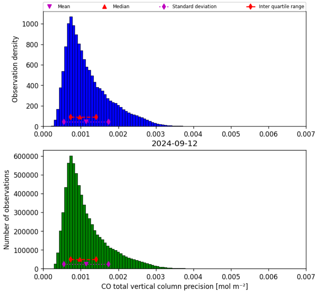
Figure 20: Histogram of “CO total vertical column precision” for 2024-09-12 to 2024-09-13
