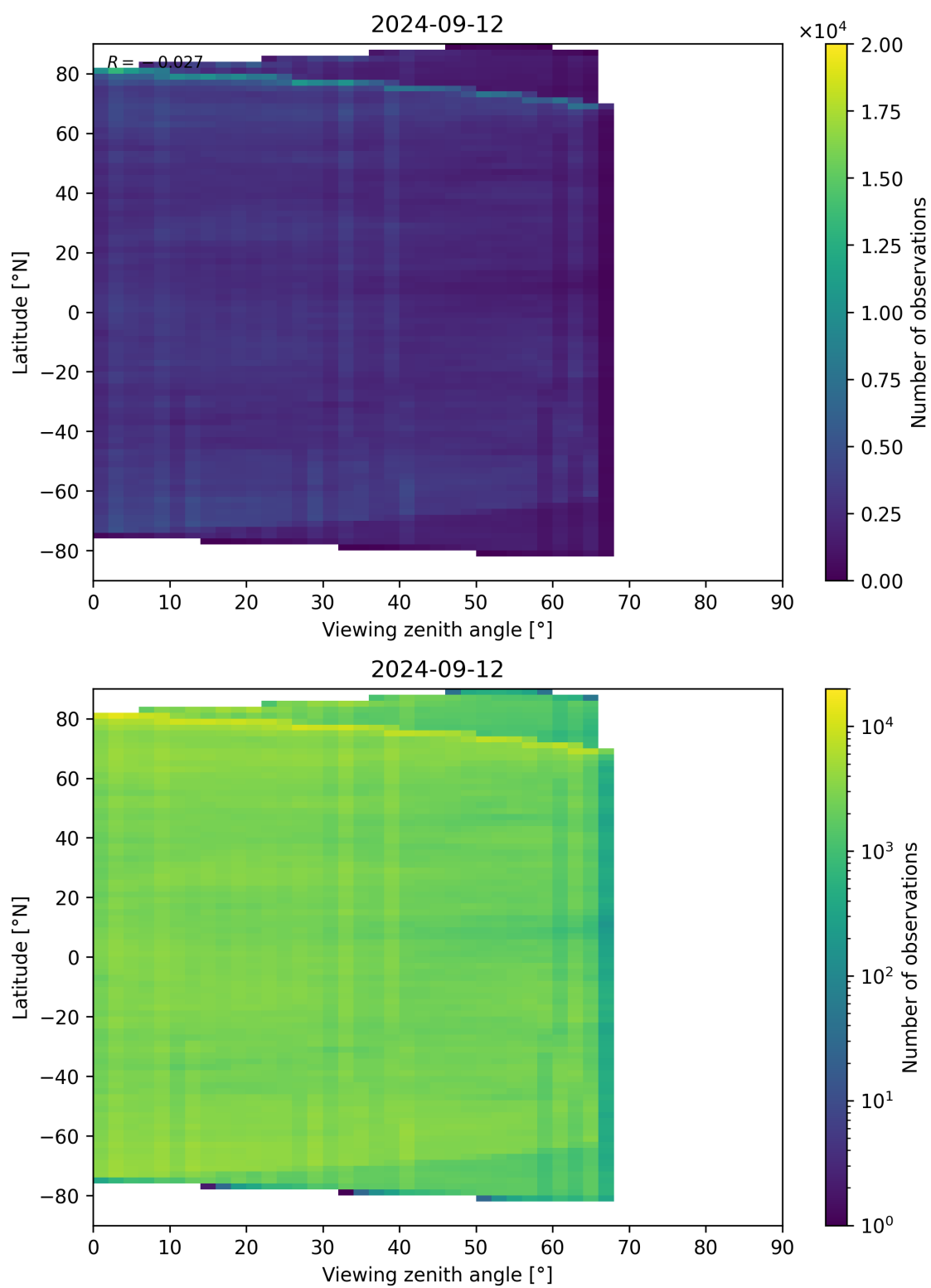
Figure 74: Scatter density plot of “Viewing zenith angle” against “Latitude” for 2024-09-12 to 2024-09-13.
