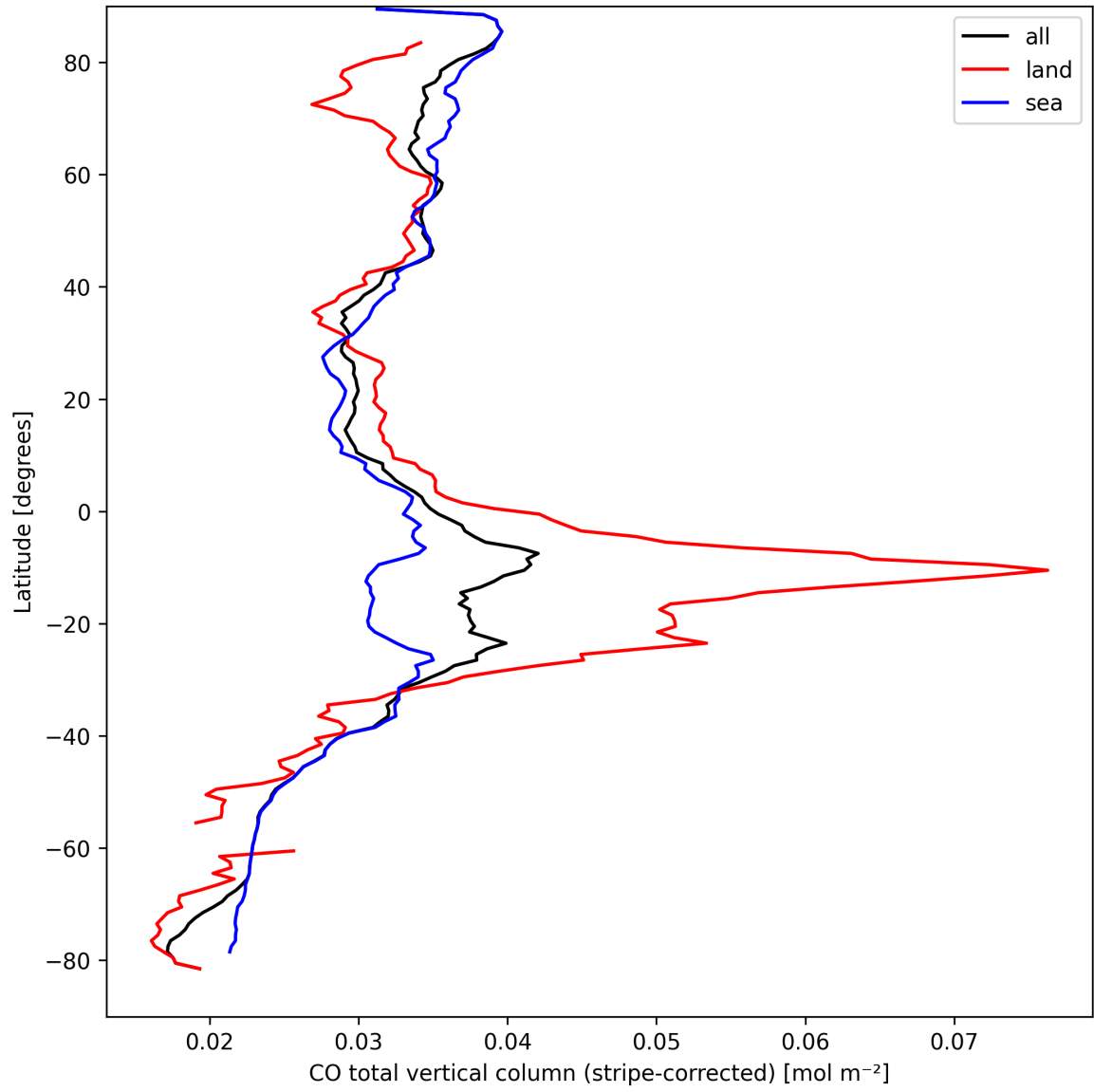
Figure 11: Zonal average of “CO total vertical column (stripe-corrected)” for 2024-09-12 to 2024-09-13.
