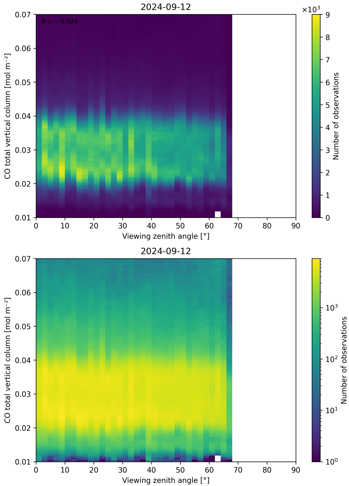
Figure 69: Scatter density plot of “Viewing zenith angle” against “CO total vertical column” for 2024-09-12 to 2024-09-13.
