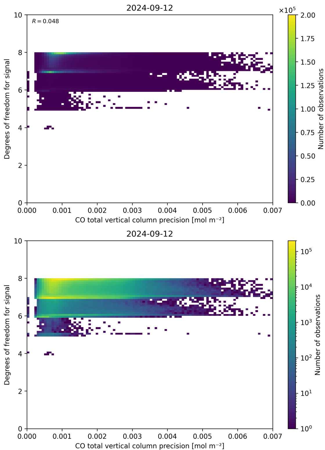
Figure 45: Scatter density plot of “CO total vertical column precision” against “Degrees of freedom for signal” for 2024-09-12 to 2024-09-13.
