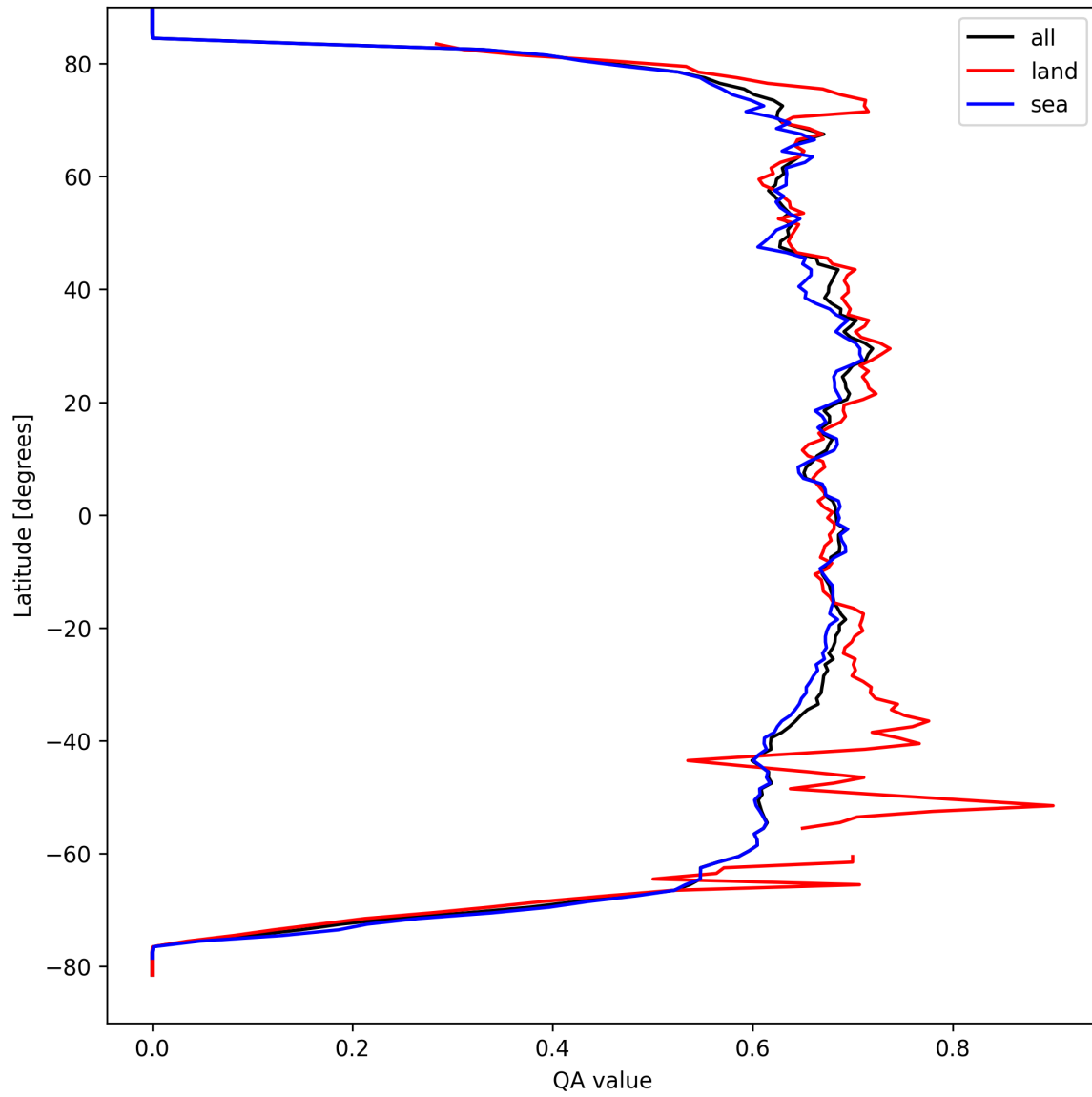
Figure 9: Zonal average of “QA value” for 2024-09-12 to 2024-09-13.
