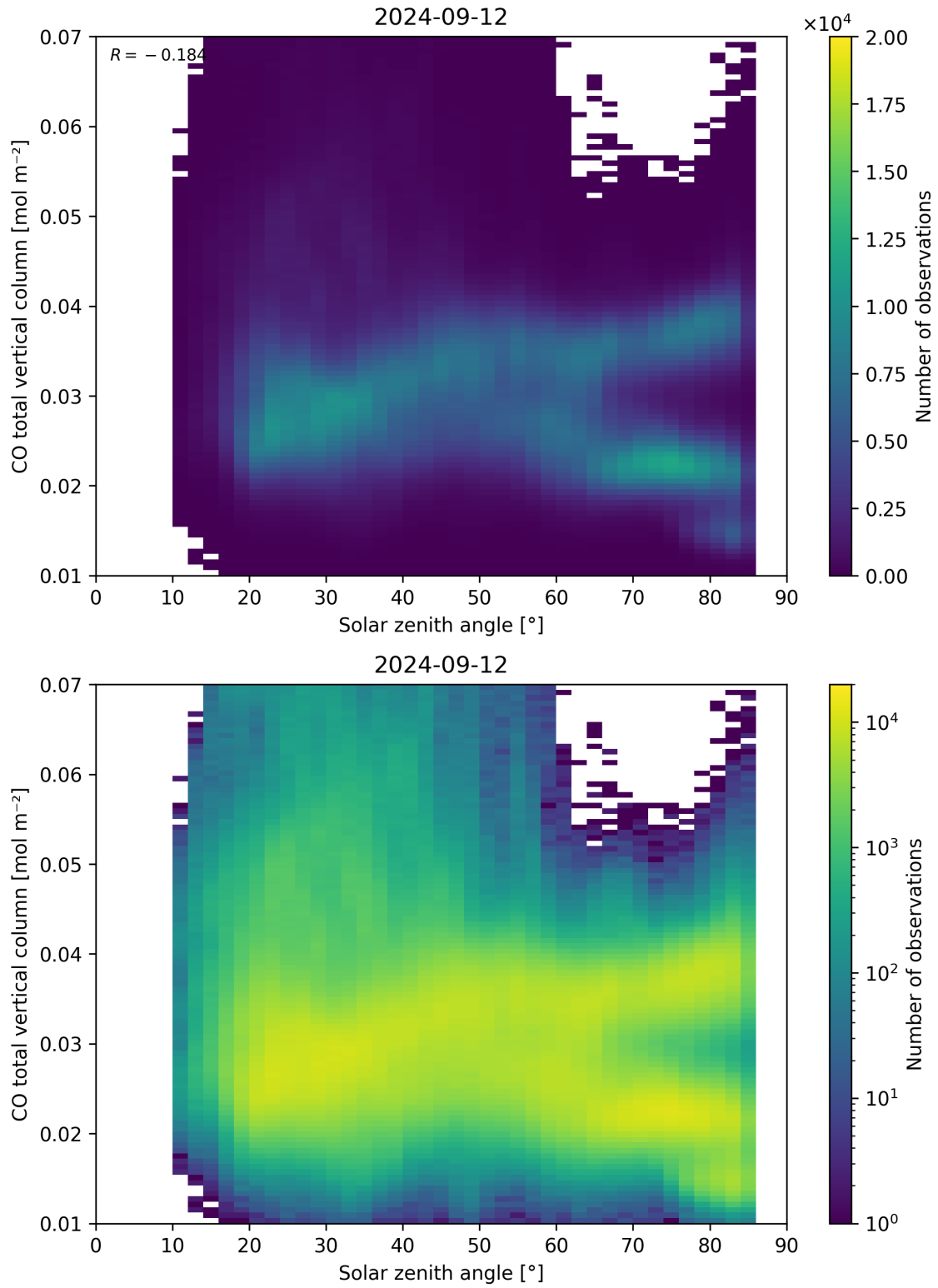
Figure 61: Scatter density plot of “Solar zenith angle” against “CO total vertical column” for 2024-09-12 to 2024-09-13.
