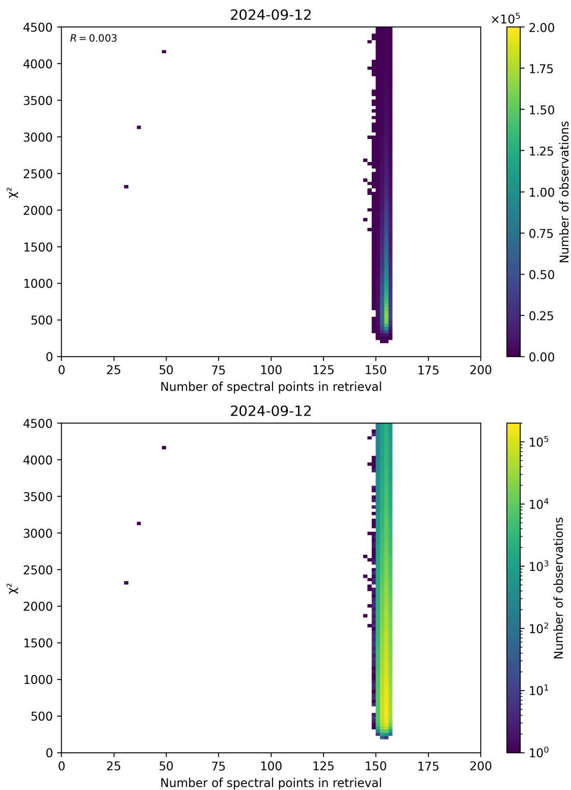
Figure 58: Scatter density plot of “Number of spectral points in retrieval” against “ \chi^2 ” for 2024-09-12 to 2024-09-13.
