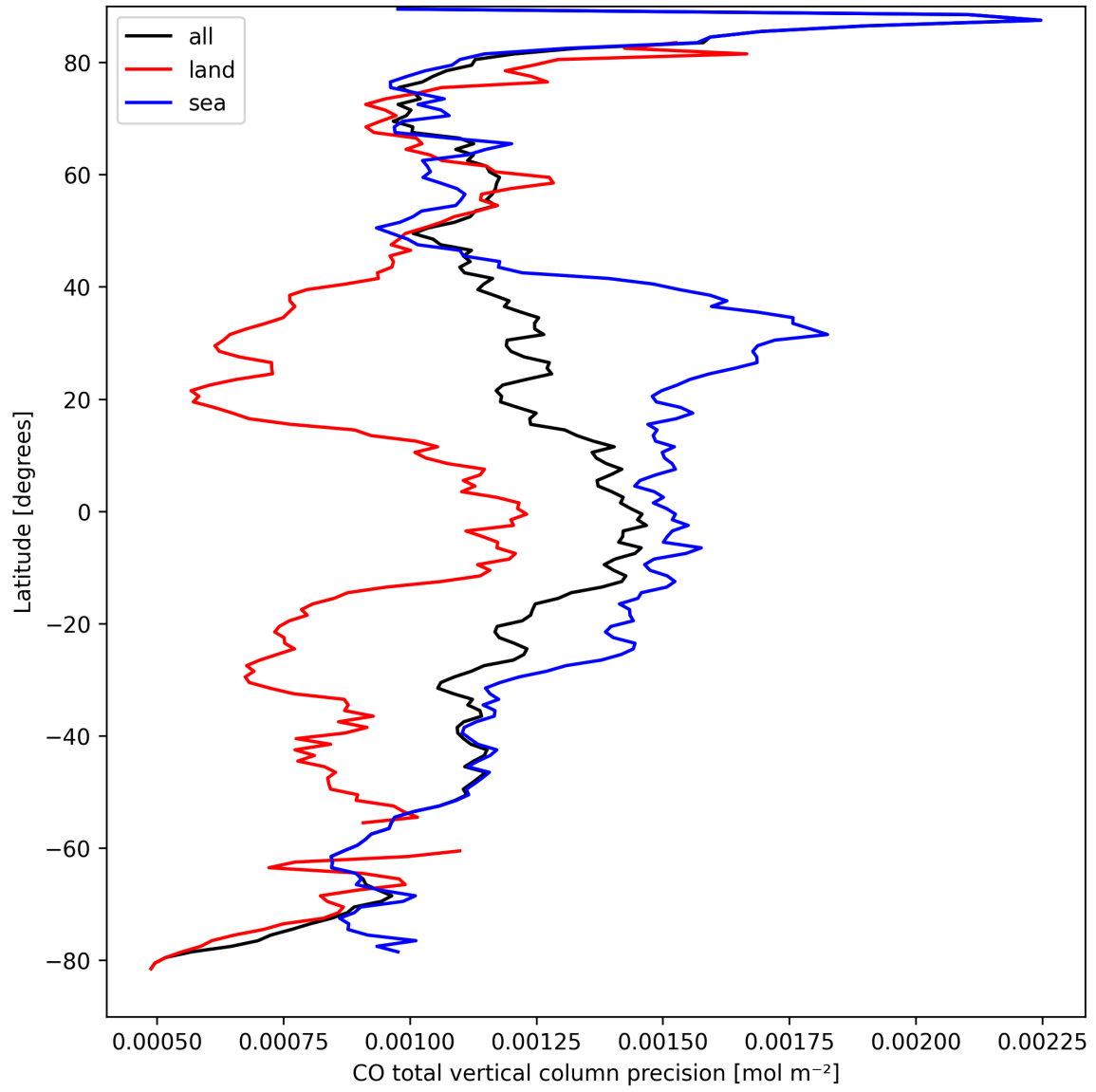
Figure 12: Zonal average of “CO total vertical column precision” for 2024-09-12 to 2024-09-13.
