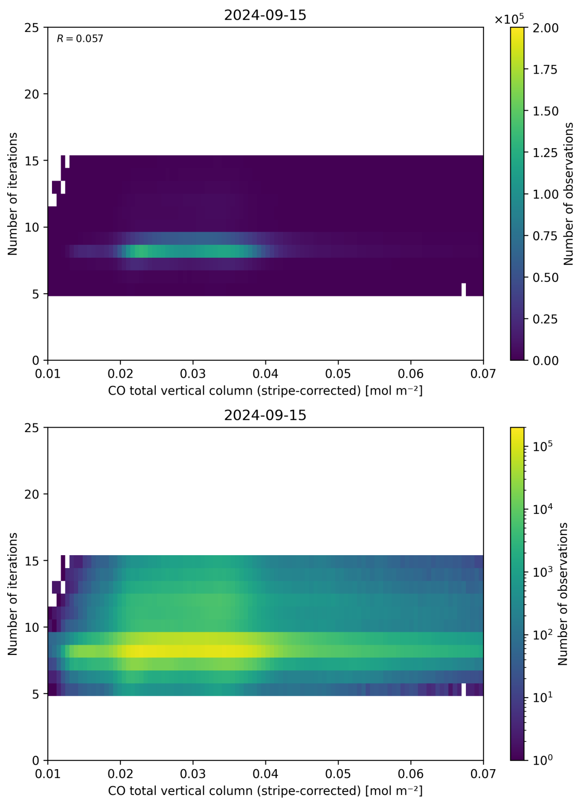
Figure 39: Scatter density plot of “CO total vertical column (stripe-corrected)” against “Number of iterations” for 2024-09-14 to 2024-09-16.
