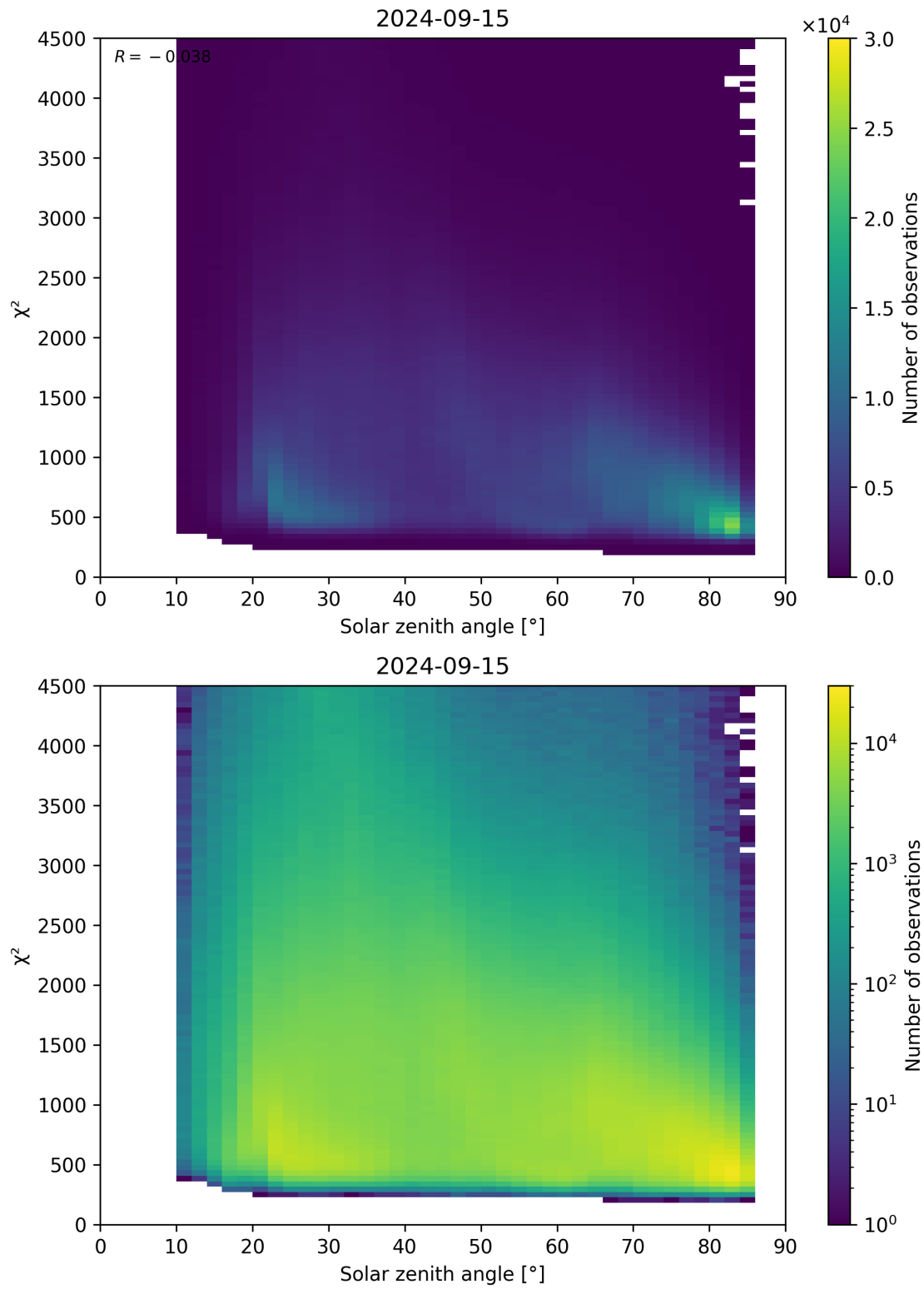
Figure 64: Scatter density plot of “Solar zenith angle” against “ \chi^2 ” for 2024-09-14 to 2024-09-16.
