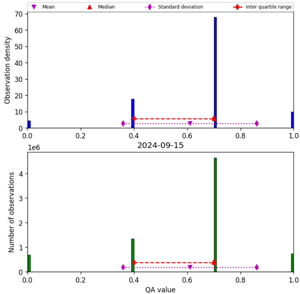
Figure 17: Histogram of “QA value” for 2024-09-14 to 2024-09-16
