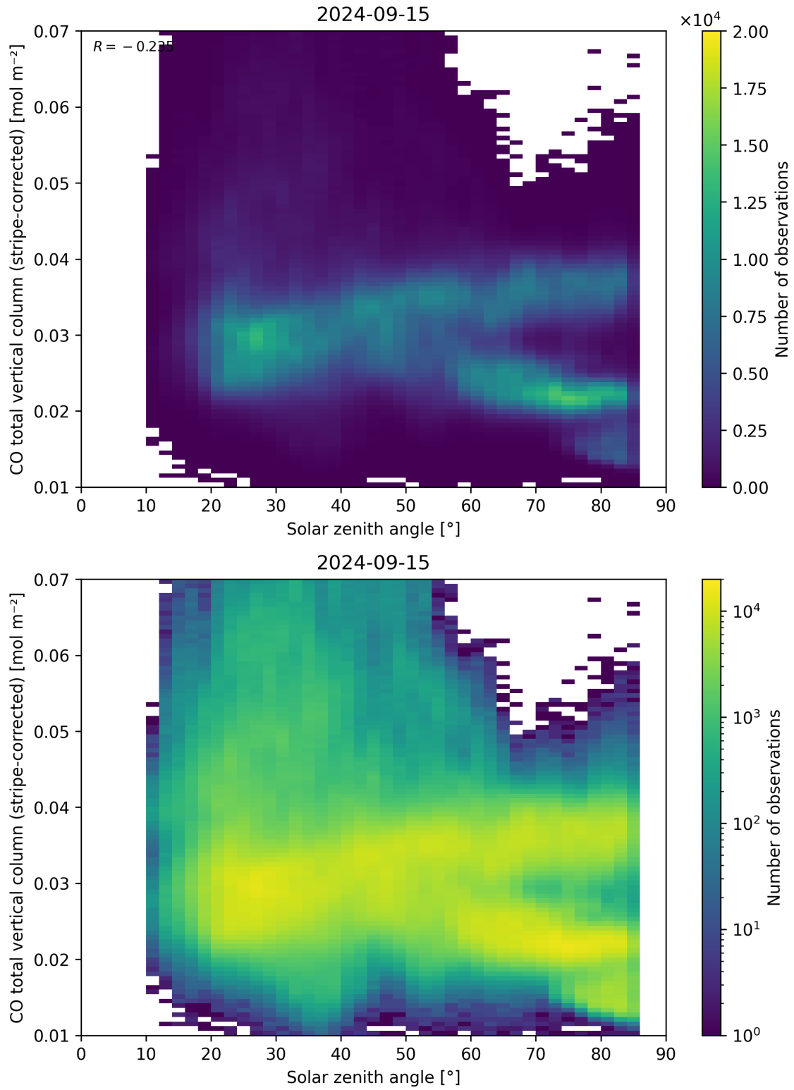
Figure 62: Scatter density plot of “Solar zenith angle” against “CO total vertical column (stripe-corrected)” for 2024-09-14 to 2024-09-16.
