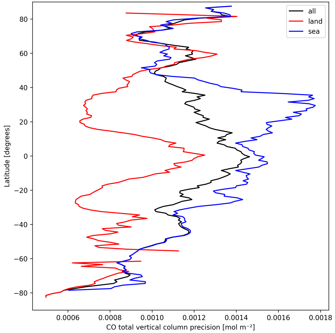
Figure 12: Zonal average of “CO total vertical column precision” for 2024-09-14 to 2024-09-16.
