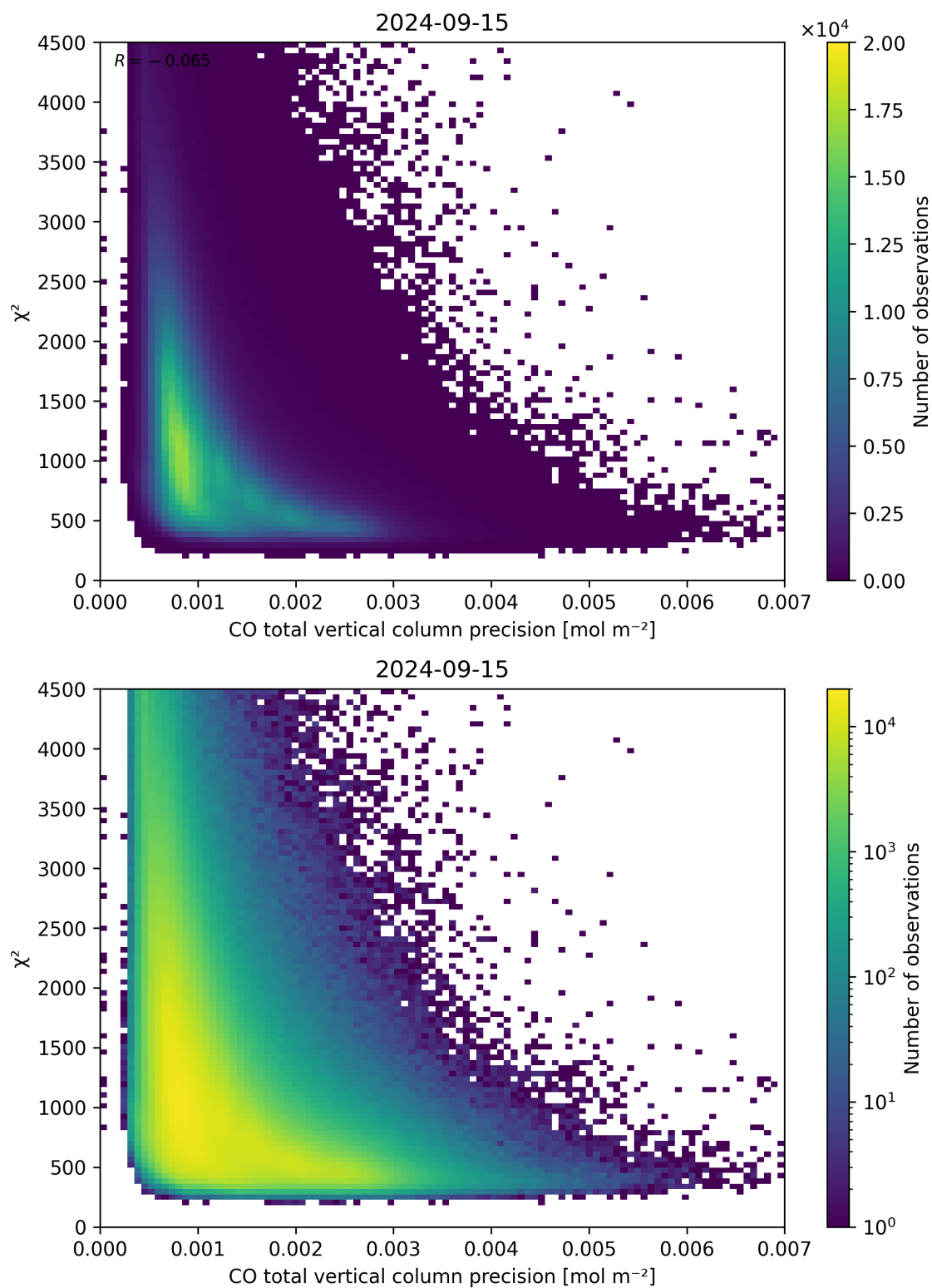
Figure 44: Scatter density plot of “CO total vertical column precision” against “ \chi^2 ” for 2024-09-14 to 2024-09-16.
