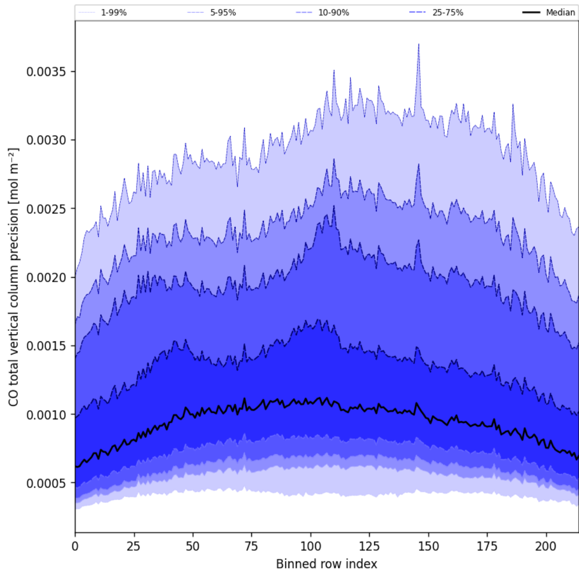
Figure 28: Along track statistics of “CO total vertical column precision” for 2024-09-14 to 2024-09-16
