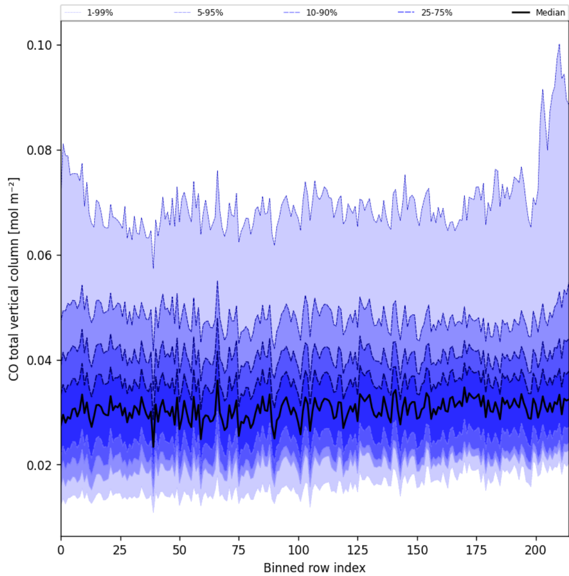
Figure 26: Along track statistics of “CO total vertical column” for 2024-09-14 to 2024-09-16
