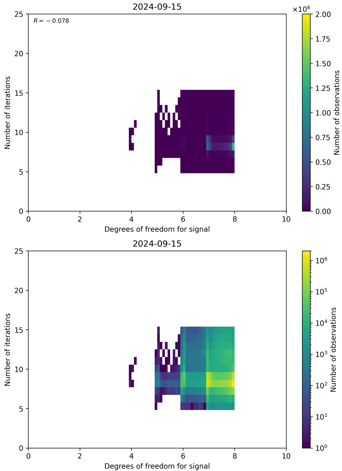
Figure 50: Scatter density plot of “Degrees of freedom for signal” against “Number of iterations” for 2024-09-14 to 2024-09-16.
