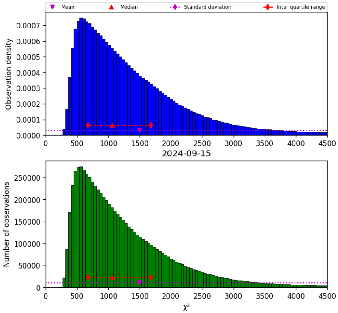
Figure 22: Histogram of “ \chi^2 ” for 2024-09-14 to 2024-09-16
