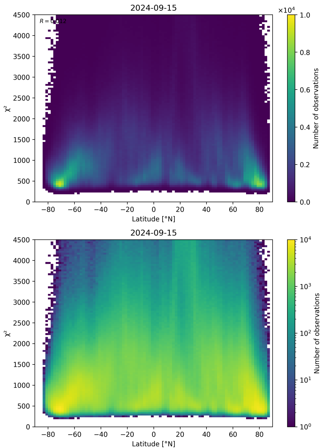
Figure 54: Scatter density plot of “Latitude” against “ \chi^2 ” for 2024-09-14 to 2024-09-16.
