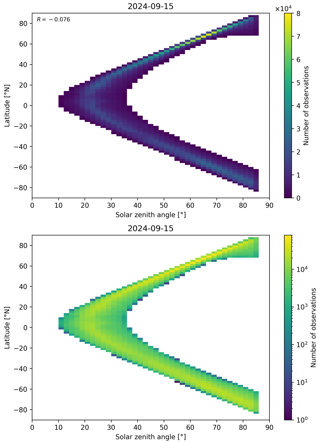
Figure 66: Scatter density plot of “Solar zenith angle” against “Latitude” for 2024-09-14 to 2024-09-16.
