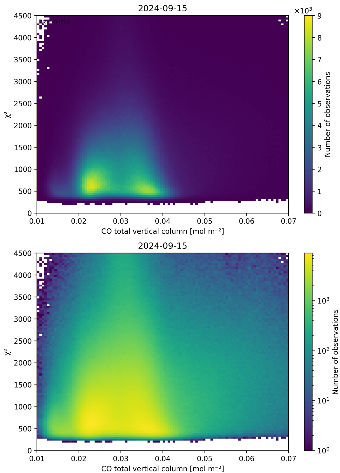
Figure 35: Scatter density plot of “CO total vertical column” against “ \chi^2 ” for 2024-09-14 to 2024-09-16.
