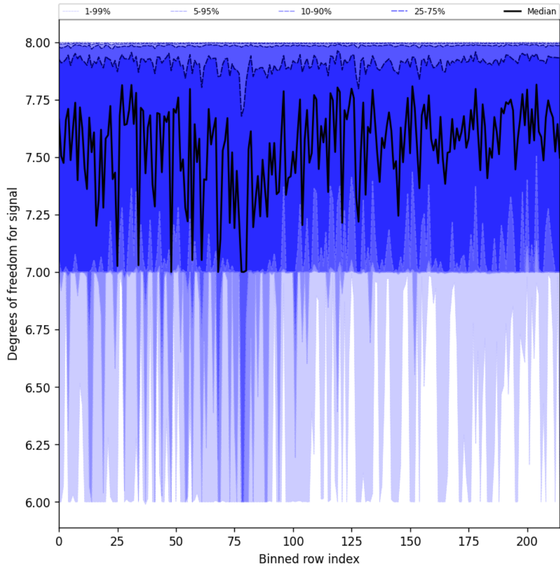
Figure 31: Along track statistics of “Degrees of freedom for signal” for 2024-09-14 to 2024-09-16
