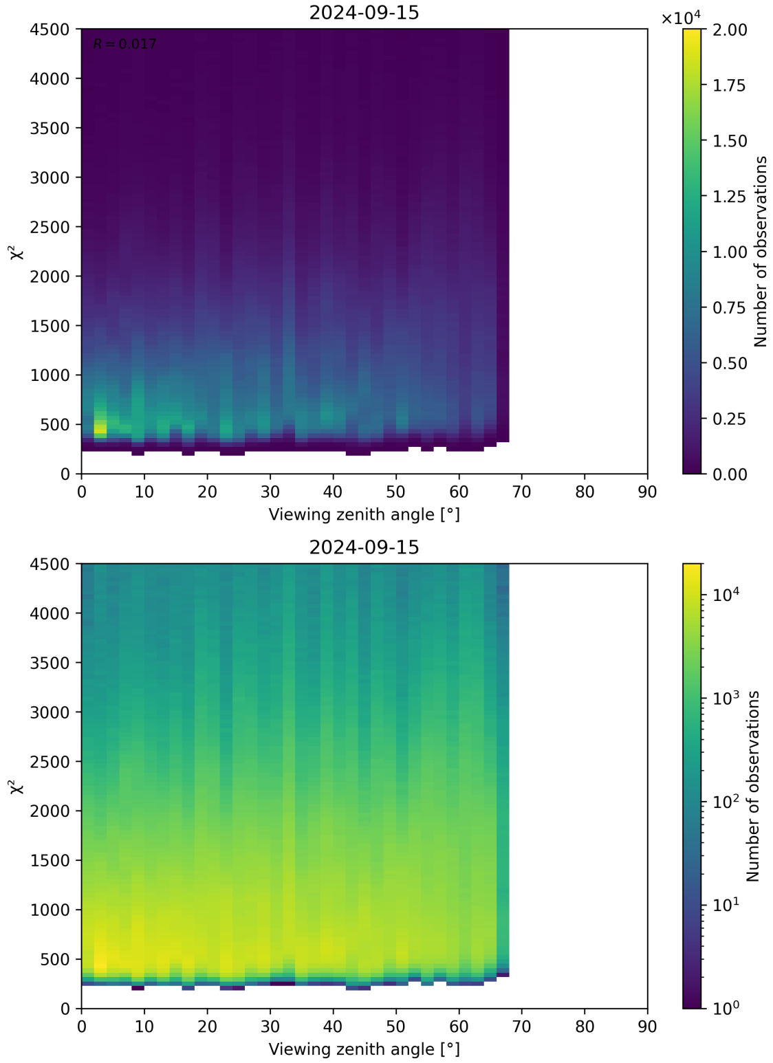
Figure 72: Scatter density plot of “Viewing zenith angle” against “ \chi^2 ” for 2024-09-14 to 2024-09-16.
