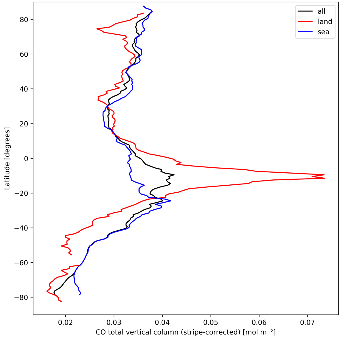
Figure 11: Zonal average of “CO total vertical column (stripe-corrected)” for 2024-09-14 to 2024-09-16.
