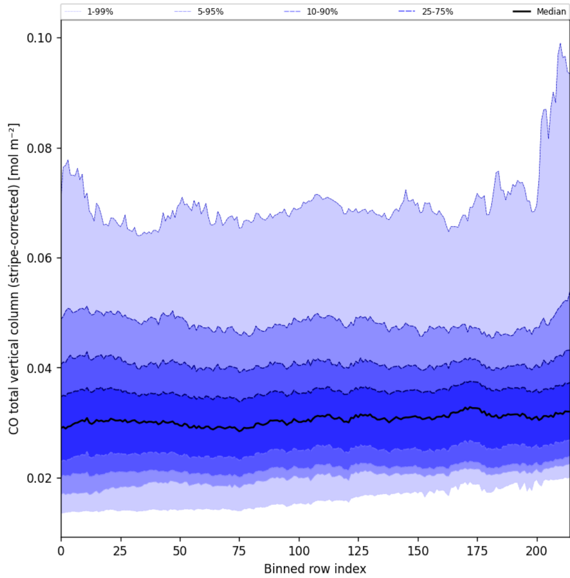
Figure 27: Along track statistics of “CO total vertical column (stripe-corrected)” for 2024-09-14 to 2024-09-16
