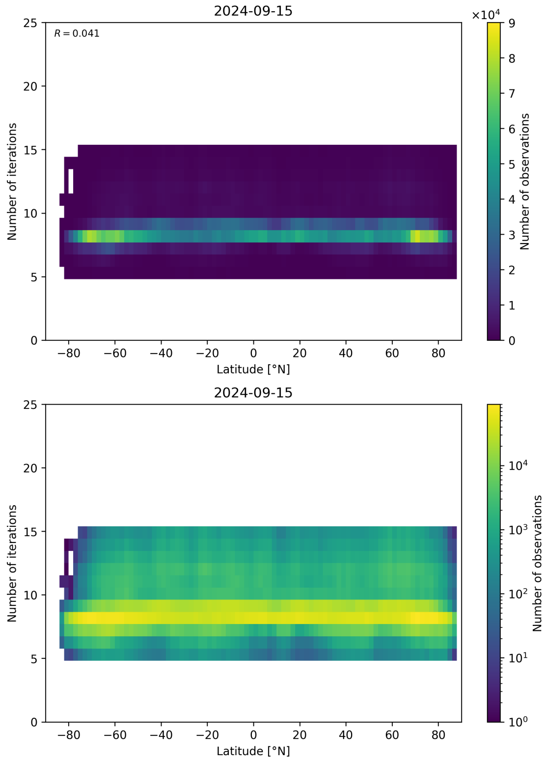
Figure 56: Scatter density plot of “Latitude” against “Number of iterations” for 2024-09-14 to 2024-09-16.
