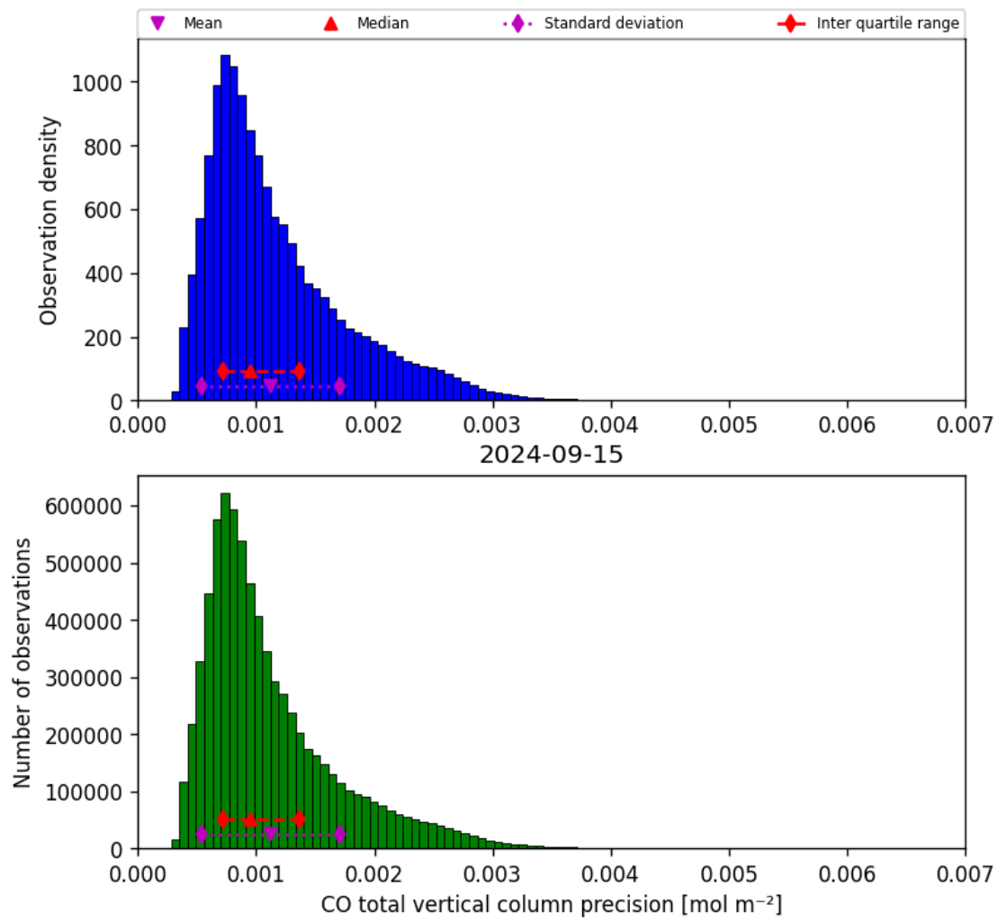
Figure 20: Histogram of “CO total vertical column precision” for 2024-09-14 to 2024-09-16
