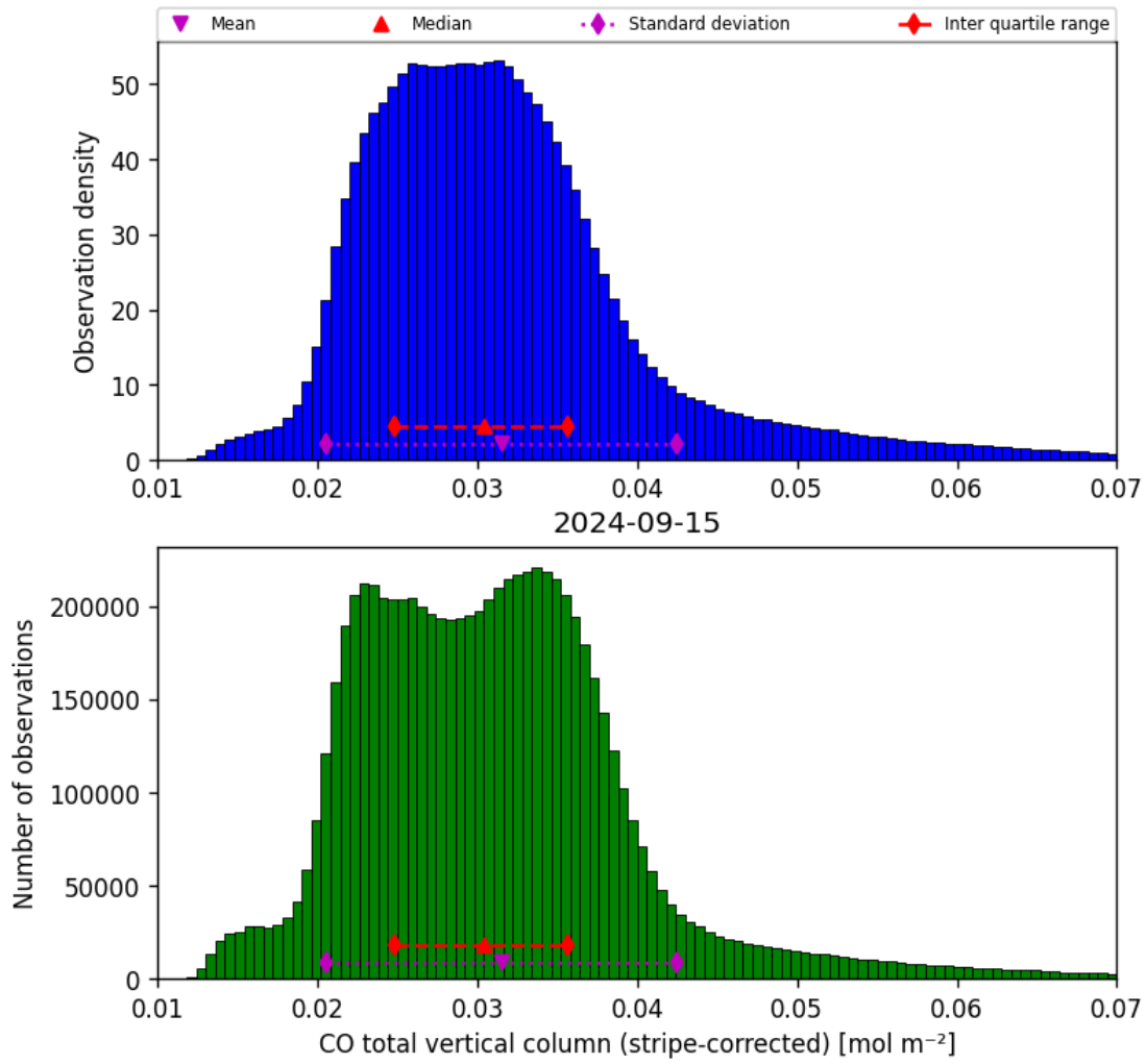
Figure 19: Histogram of “CO total vertical column (stripe-corrected)” for 2024-09-14 to 2024-09-16
