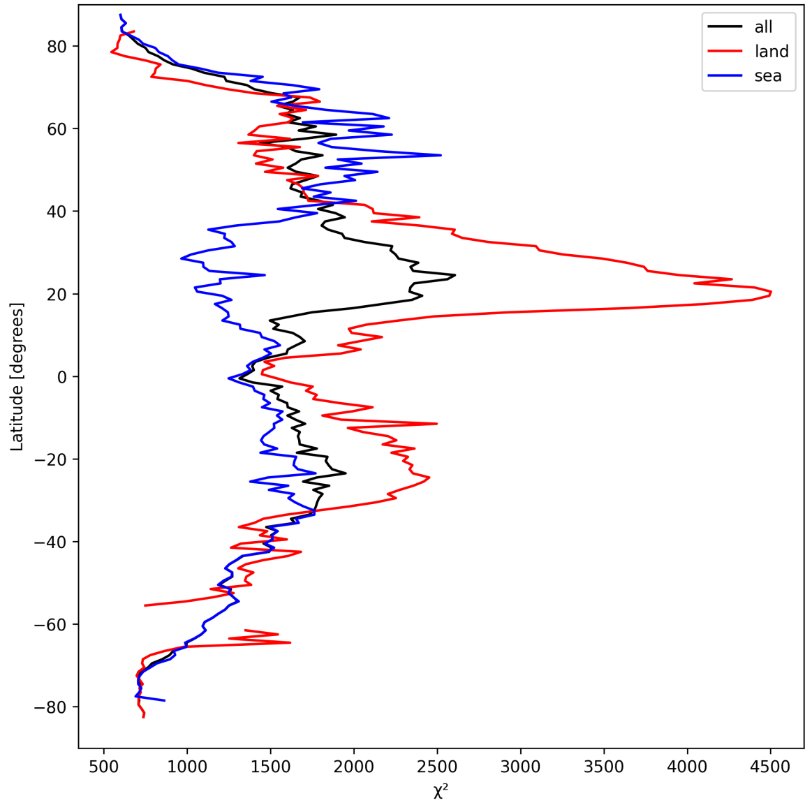
Figure 14: Zonal average of “ \chi^2 ” for 2024-09-14 to 2024-09-16.
