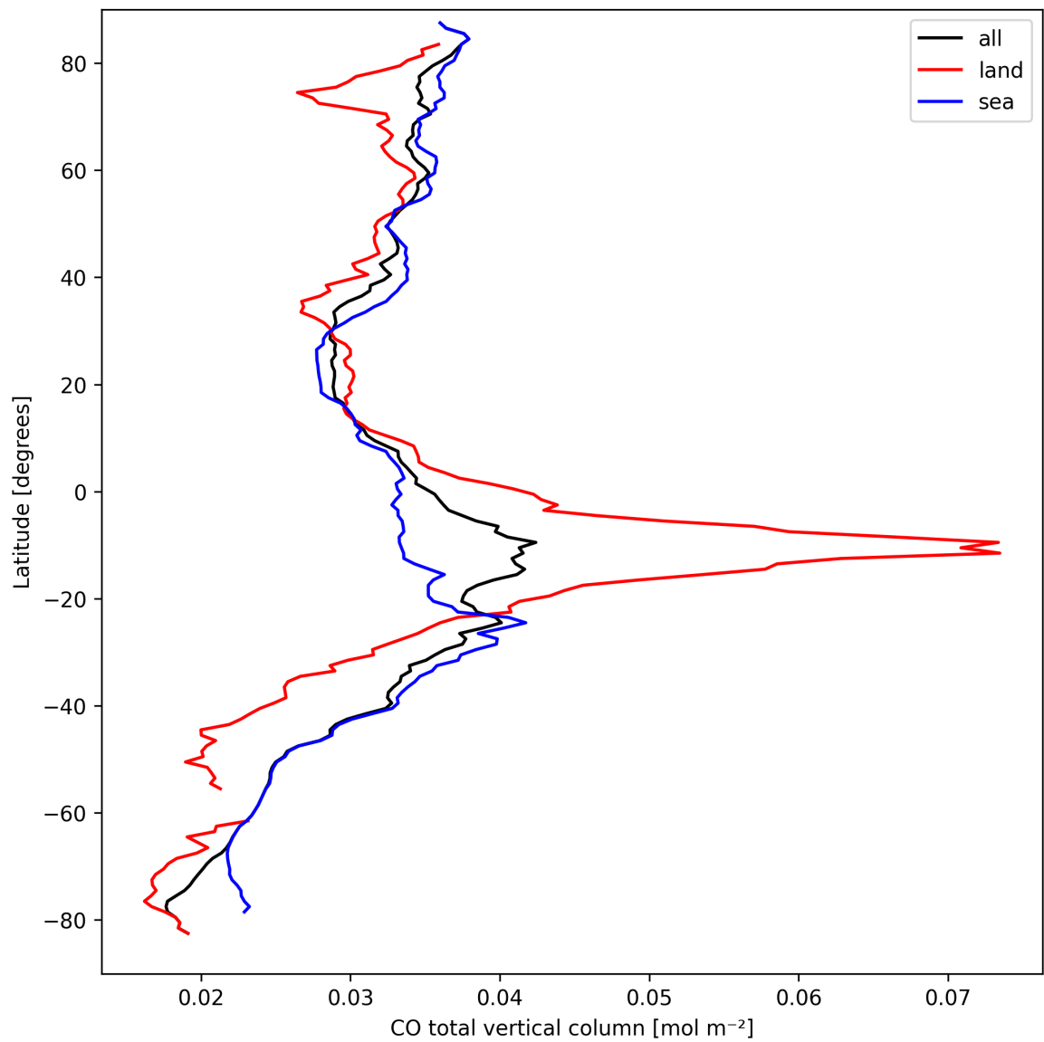
Figure 10: Zonal average of “CO total vertical column” for 2024-09-14 to 2024-09-16.
