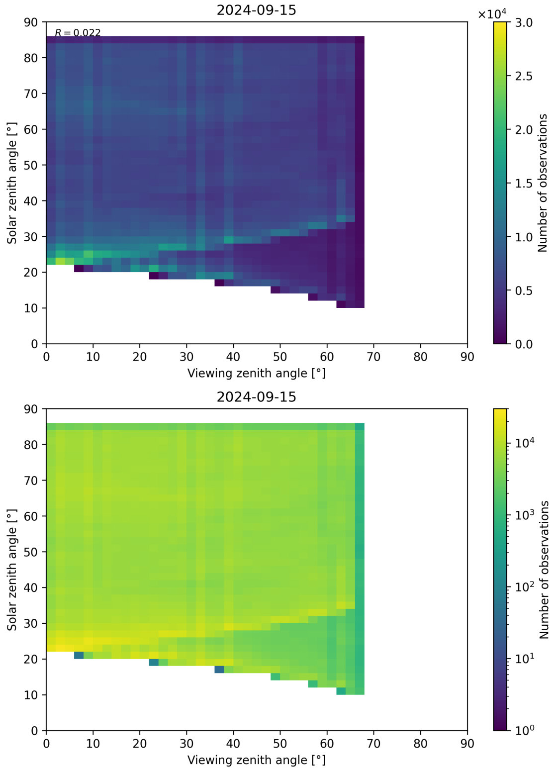
Figure 77: Scatter density plot of “Viewing zenith angle” against “Solar zenith angle” for 2024-09-14 to 2024-09-16.
