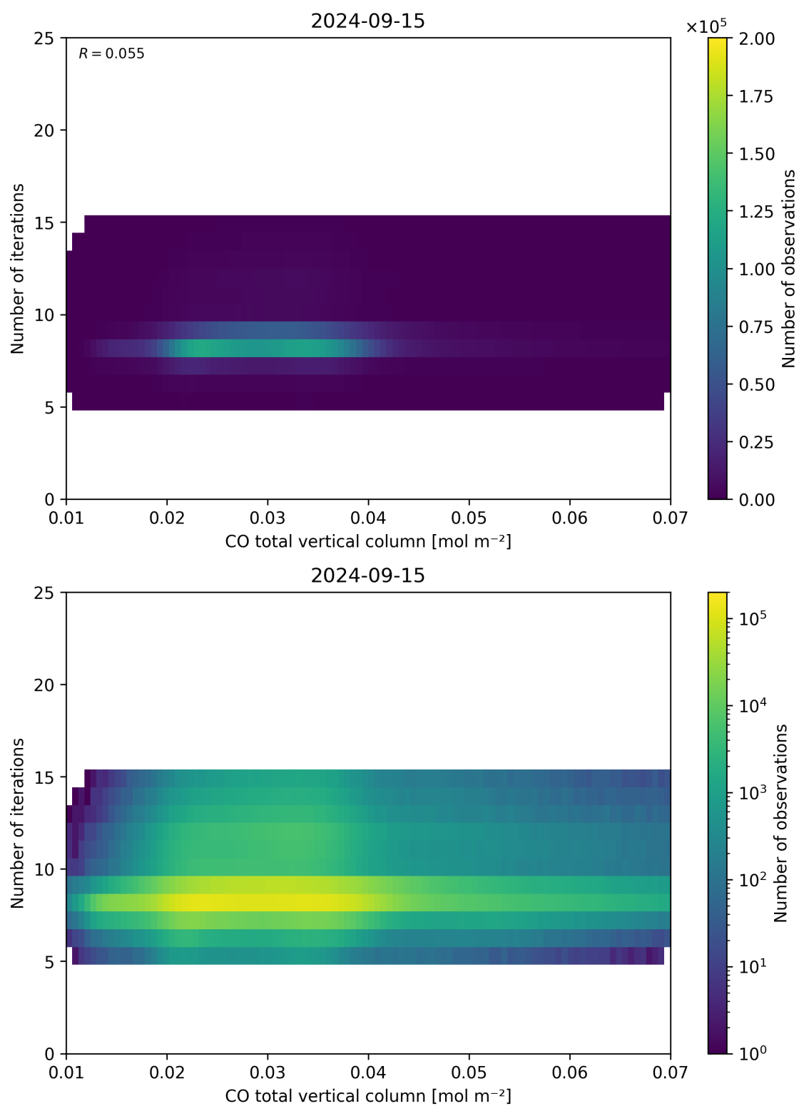
Figure 42: Scatter density plot of “CO total vertical column” against “Number of iterations” for 2024-09-14 to 2024-09-16.
