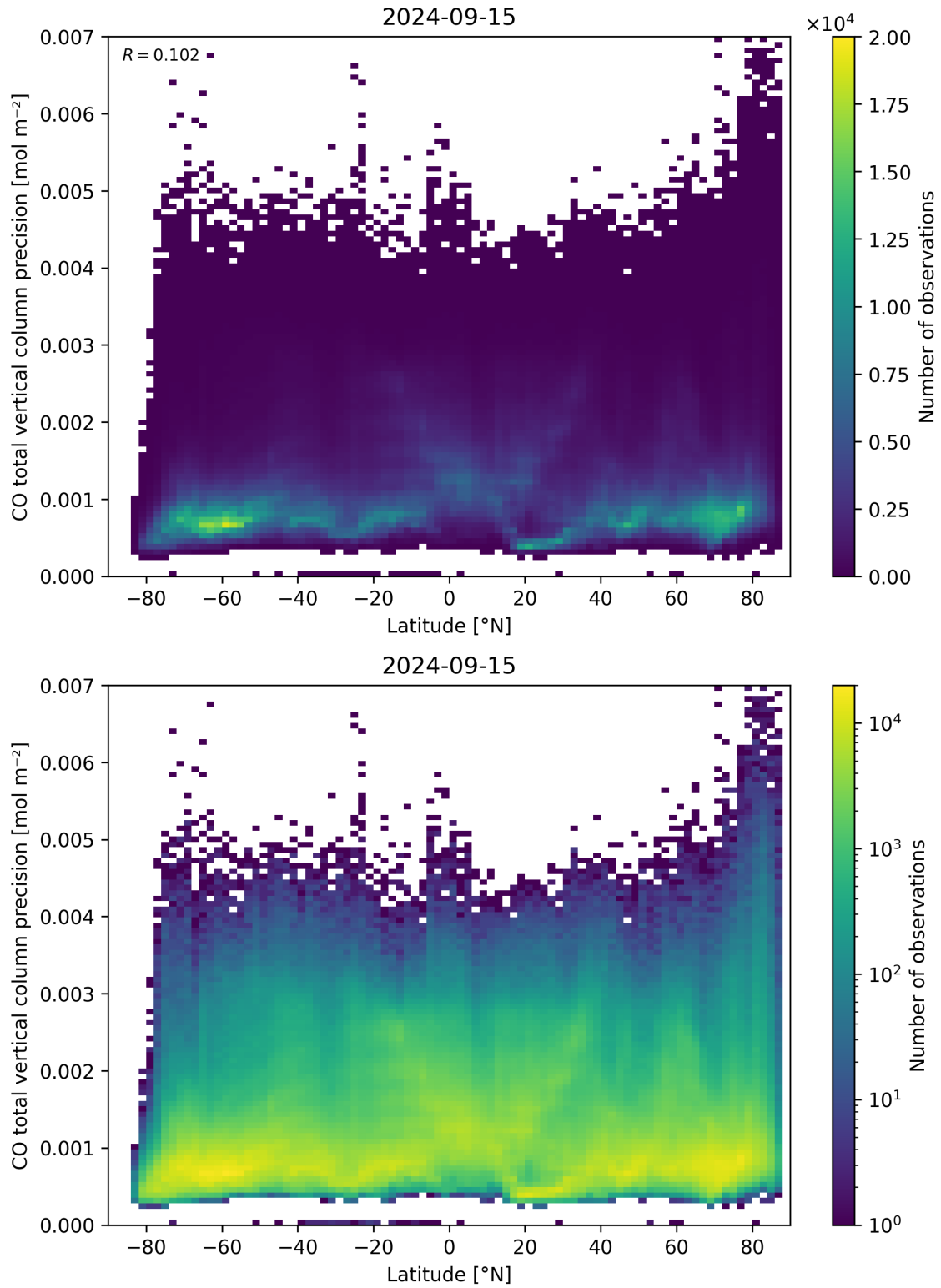
Figure 53: Scatter density plot of “Latitude” against “CO total vertical column precision” for 2024-09-14 to 2024-09-16.
