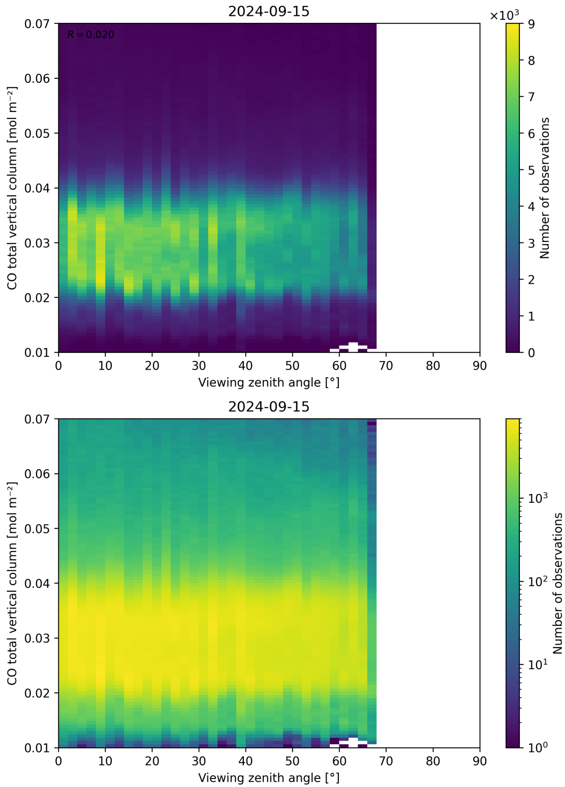
Figure 69: Scatter density plot of “Viewing zenith angle” against “CO total vertical column” for 2024-09-14 to 2024-09-16.
