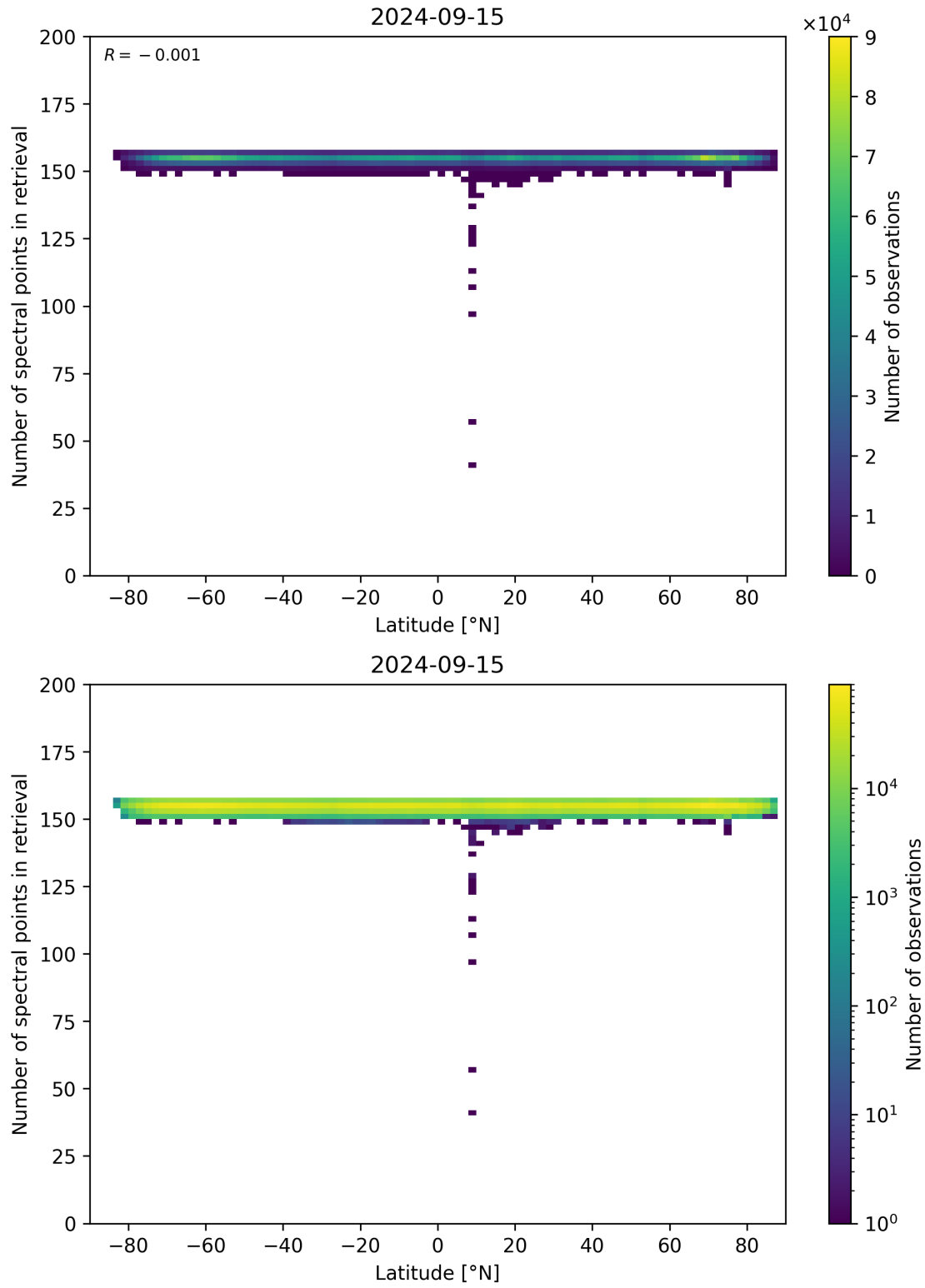
Figure 57: Scatter density plot of “Latitude” against “Number of spectral points in retrieval” for 2024-09-14 to 2024-09-16.
