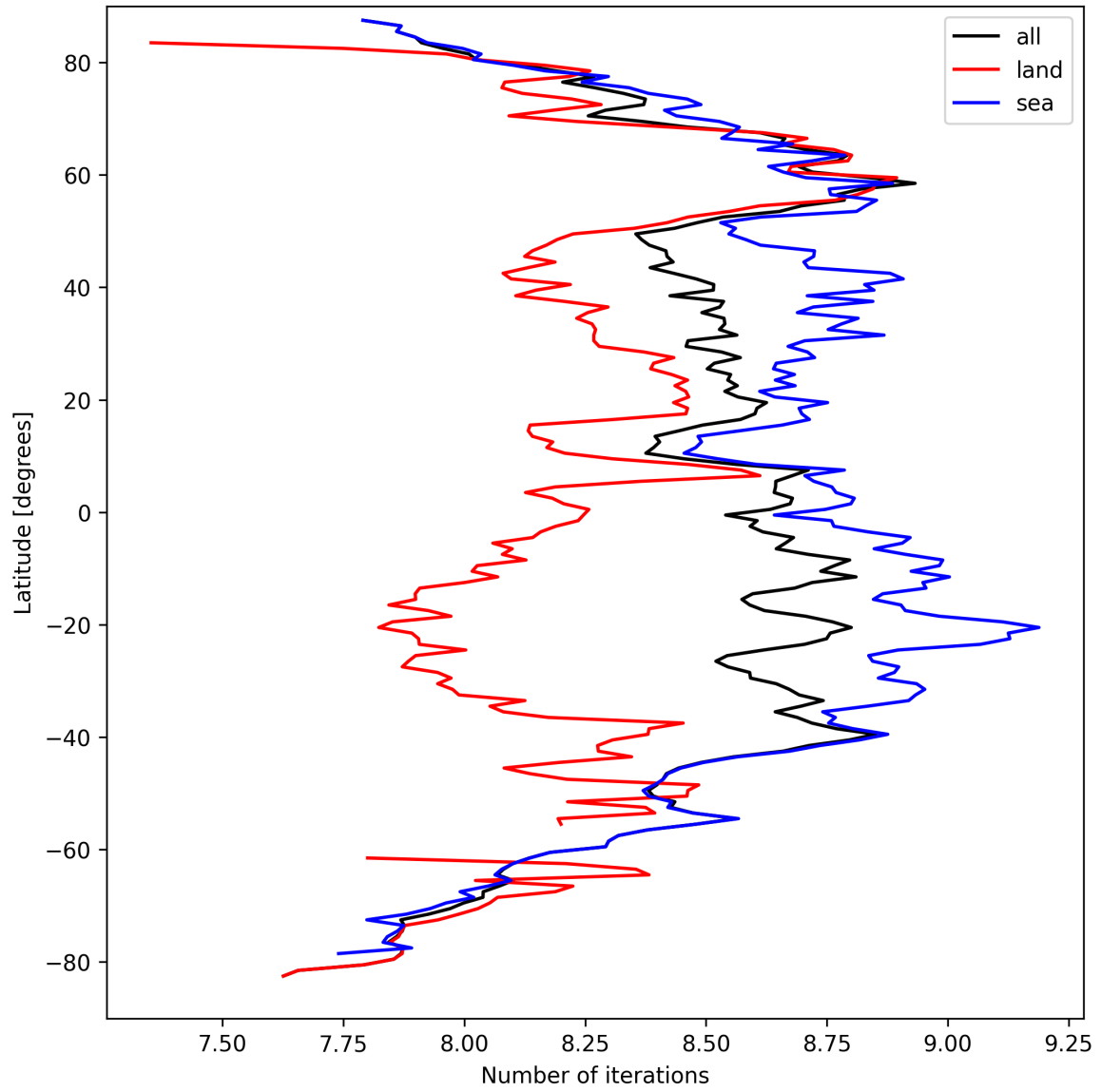
Figure 16: Zonal average of “Number of iterations” for 2024-09-14 to 2024-09-16.
