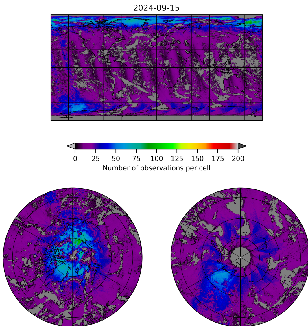
Figure 8: Map of the number of observations for 2024-09-14 to 2024-09-16
