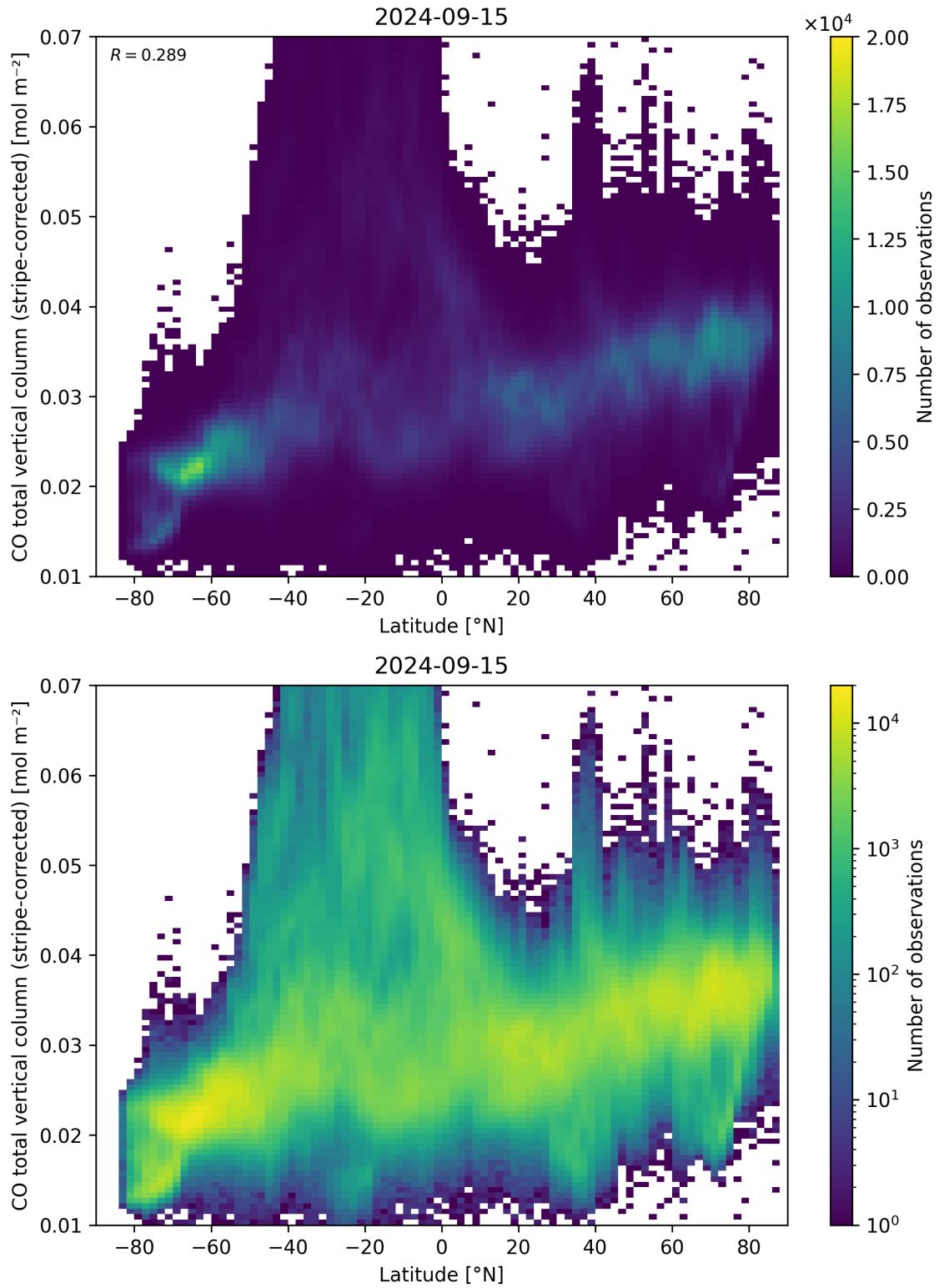
Figure 52: Scatter density plot of “Latitude” against “CO total vertical column (stripe-corrected)” for 2024-09-14 to 2024-09-16.
