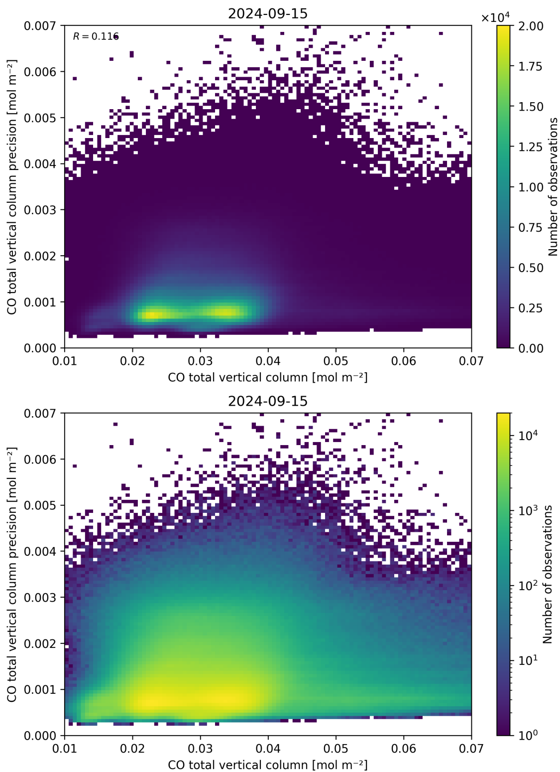
Figure 34: Scatter density plot of “CO total vertical column” against “CO total vertical column precision” for 2024-09-14 to 2024-09-16.
