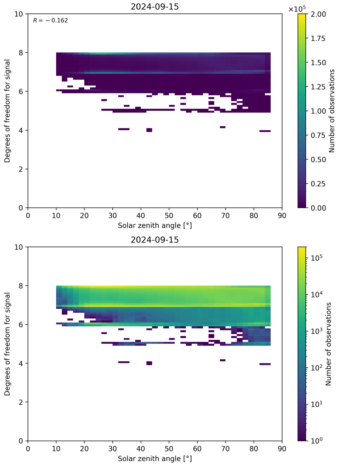
Figure 65: Scatter density plot of “Solar zenith angle” against “Degrees of freedom for signal” for 2024-09-14 to 2024-09-16.
