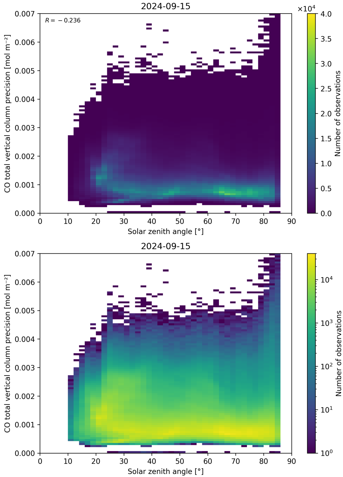
Figure 63: Scatter density plot of “Solar zenith angle” against “CO total vertical column precision” for 2024-09-14 to 2024-09-16.
