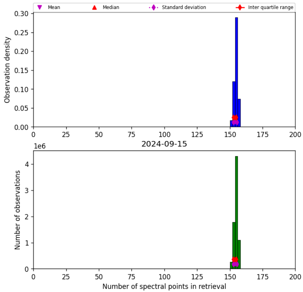
Figure 21: Histogram of “Number of spectral points in retrieval” for 2024-09-14 to 2024-09-16
