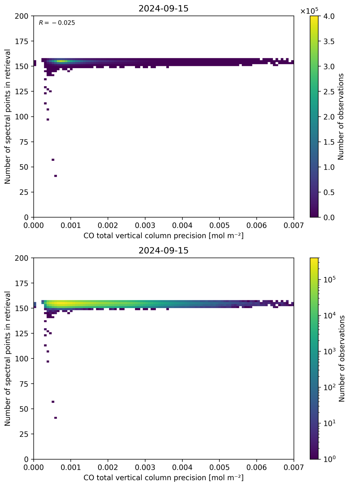
Figure 47: Scatter density plot of “CO total vertical column precision” against “Number of spectral points in retrieval” for 2024-09-14 to 2024-09-16.
