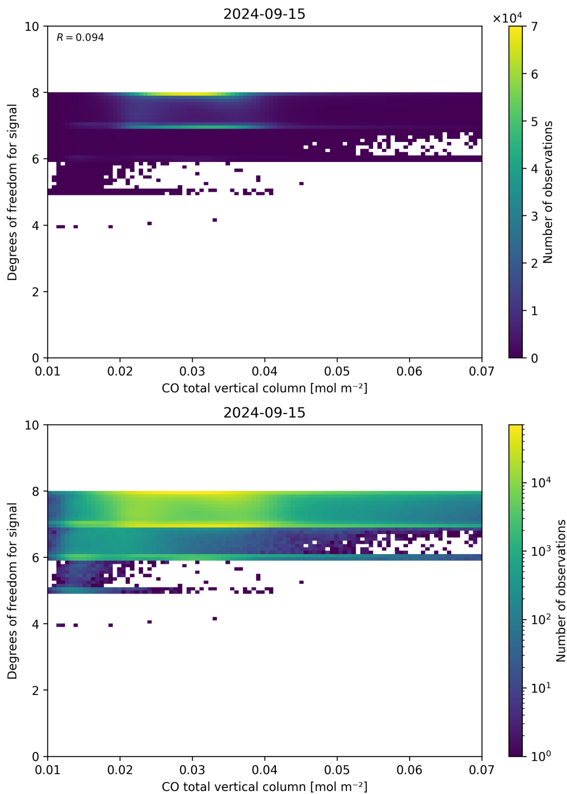
Figure 41: Scatter density plot of “CO total vertical column” against “Degrees of freedom for signal” for 2024-09-14 to 2024-09-16.
