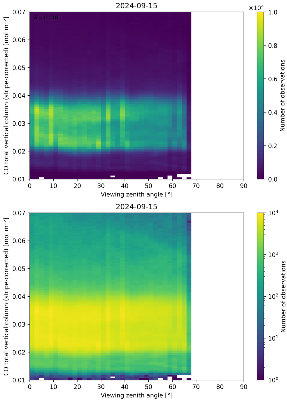
Figure 70: Scatter density plot of “Viewing zenith angle” against “CO total vertical column (stripe-corrected)” for 2024-09-14 to 2024-09-16.
