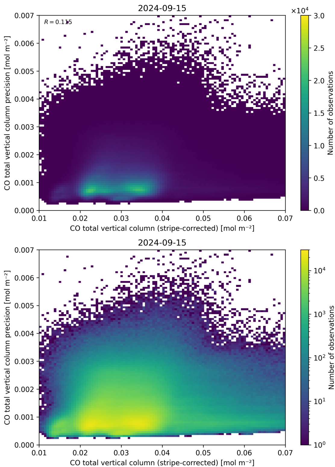
Figure 36: Scatter density plot of “CO total vertical column (stripe-corrected)” against “CO total vertical column precision” for 2024-09-14 to 2024-09-16.
