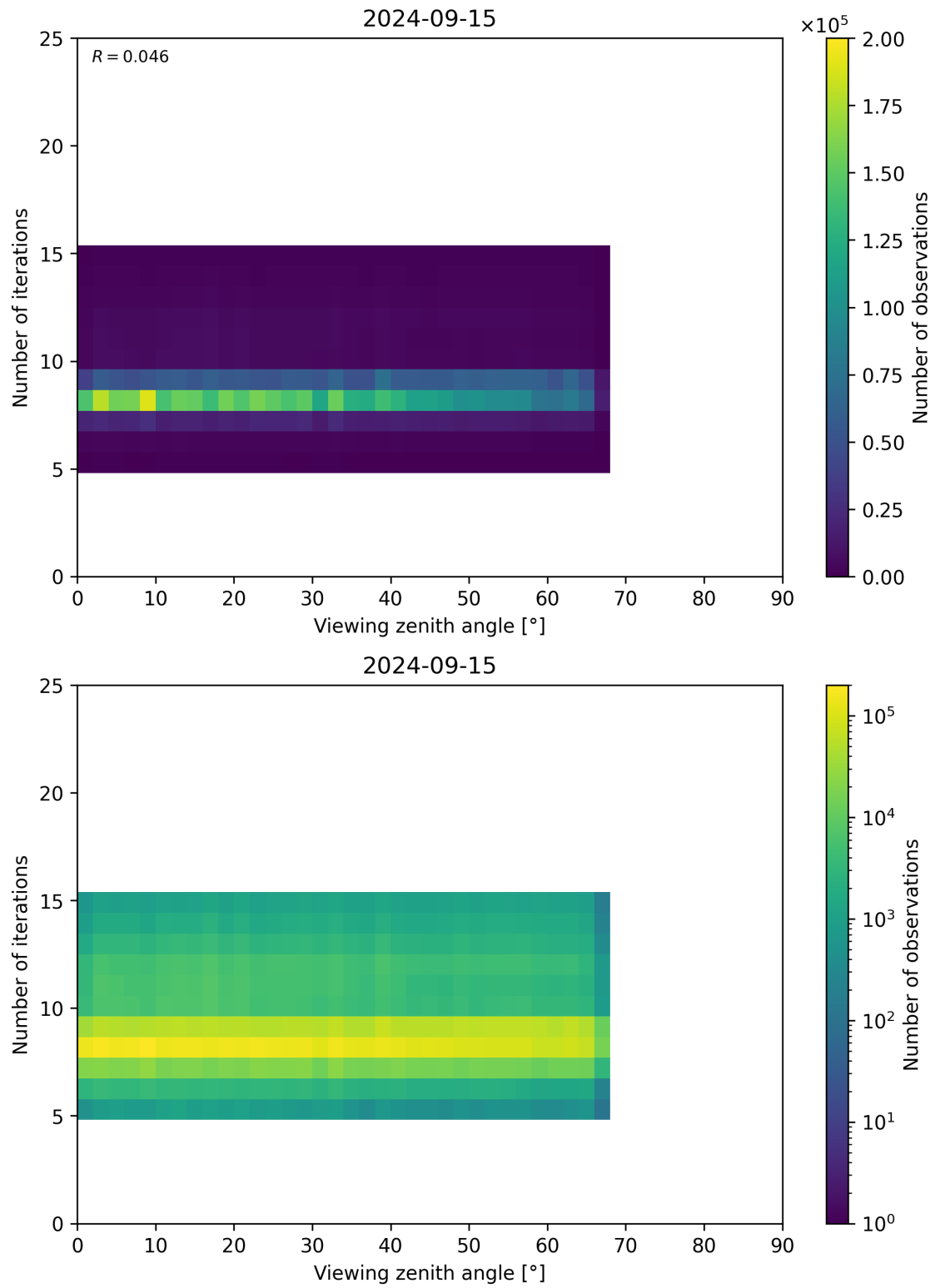
Figure 75: Scatter density plot of “Viewing zenith angle” against “Number of iterations” for 2024-09-14 to 2024-09-16.
