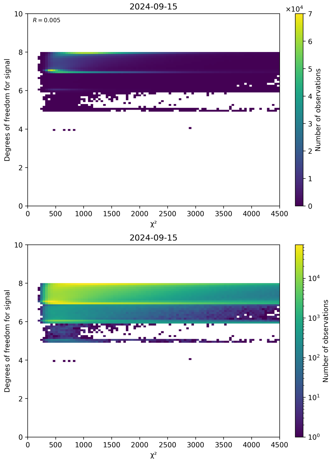
Figure 48: Scatter density plot of “ \chi^2 ” against “Degrees of freedom for signal” for 2024-09-14 to 2024-09-16.
