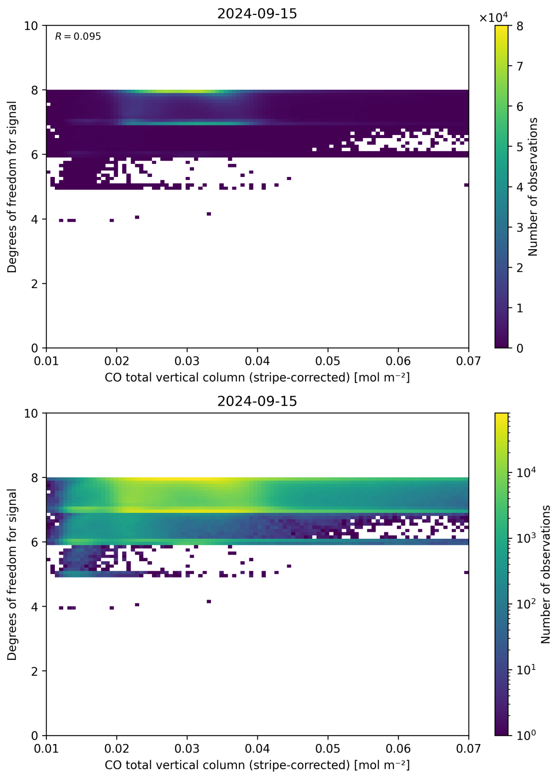
Figure 38: Scatter density plot of “CO total vertical column (stripe-corrected)” against “Degrees of freedom for signal” for 2024-09-14 to 2024-09-16.
