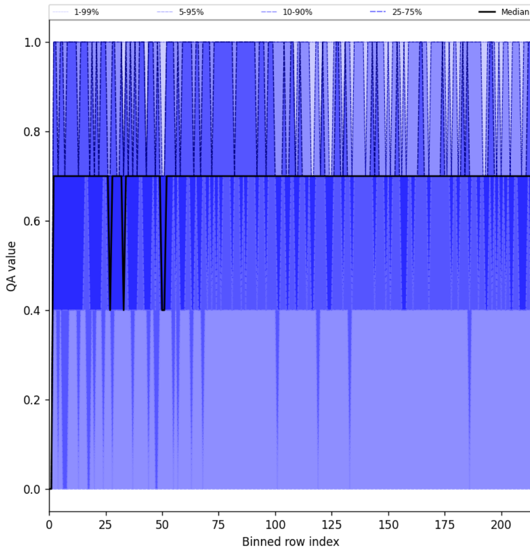
Figure 25: Along track statistics of “QA value” for 2024-09-14 to 2024-09-16
