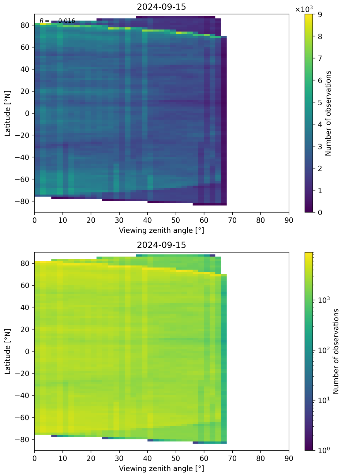
Figure 74: Scatter density plot of “Viewing zenith angle” against “Latitude” for 2024-09-14 to 2024-09-16.
