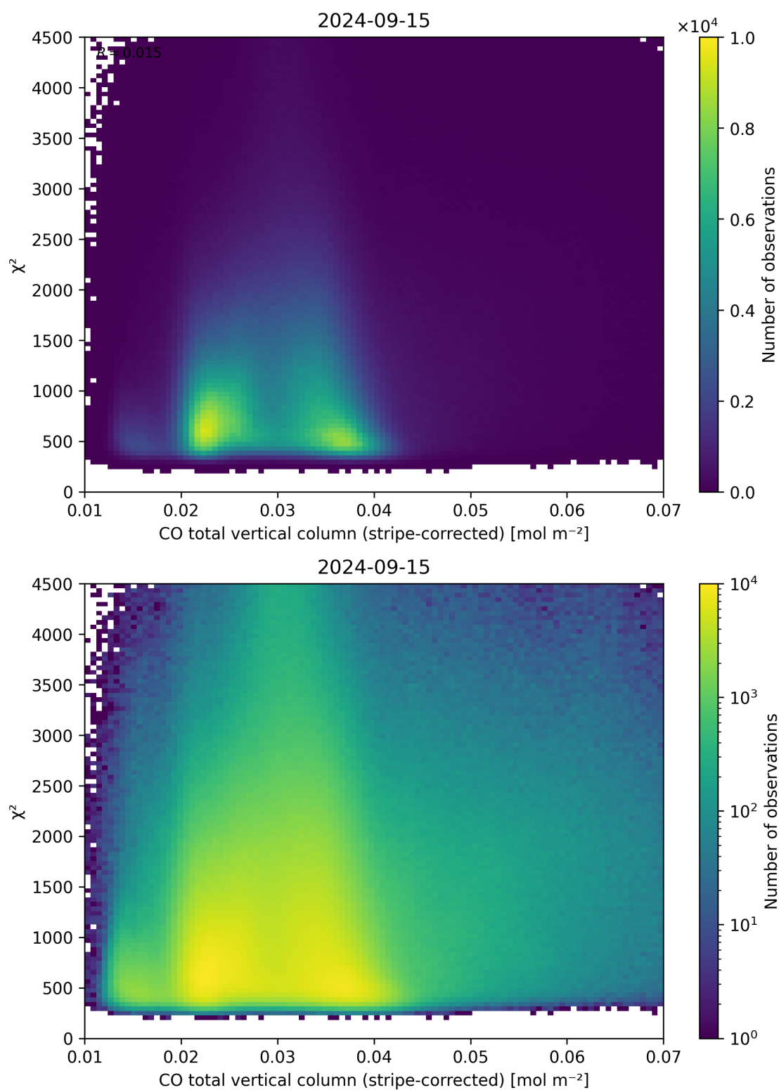
Figure 37: Scatter density plot of “CO total vertical column (stripe-corrected)” against “ \chi^2 ” for 2024-09-14 to 2024-09-16.
