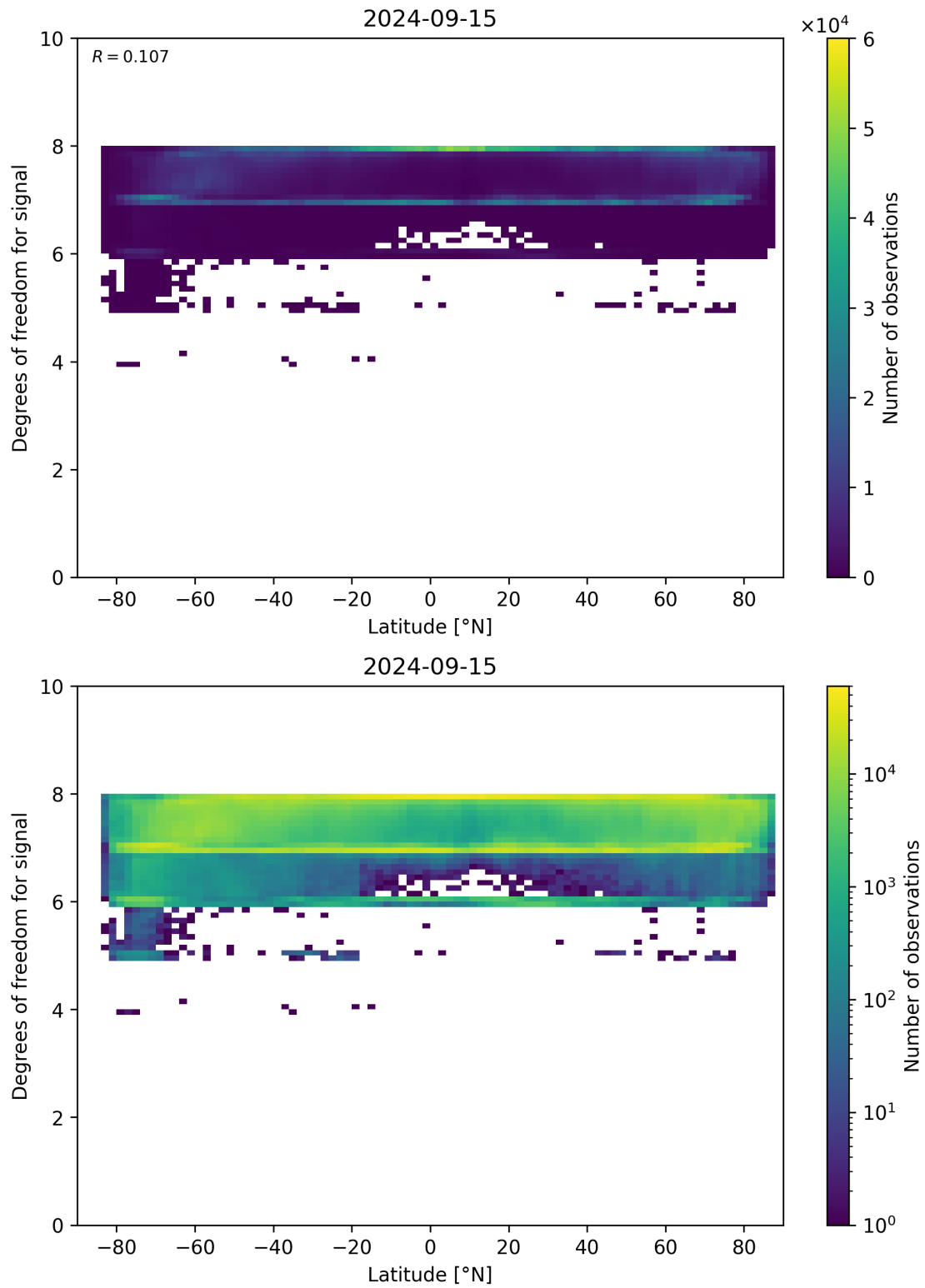
Figure 55: Scatter density plot of “Latitude” against “Degrees of freedom for signal” for 2024-09-14 to 2024-09-16.
