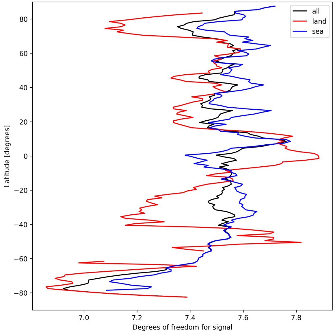
Figure 15: Zonal average of “Degrees of freedom for signal” for 2024-09-14 to 2024-09-16.
