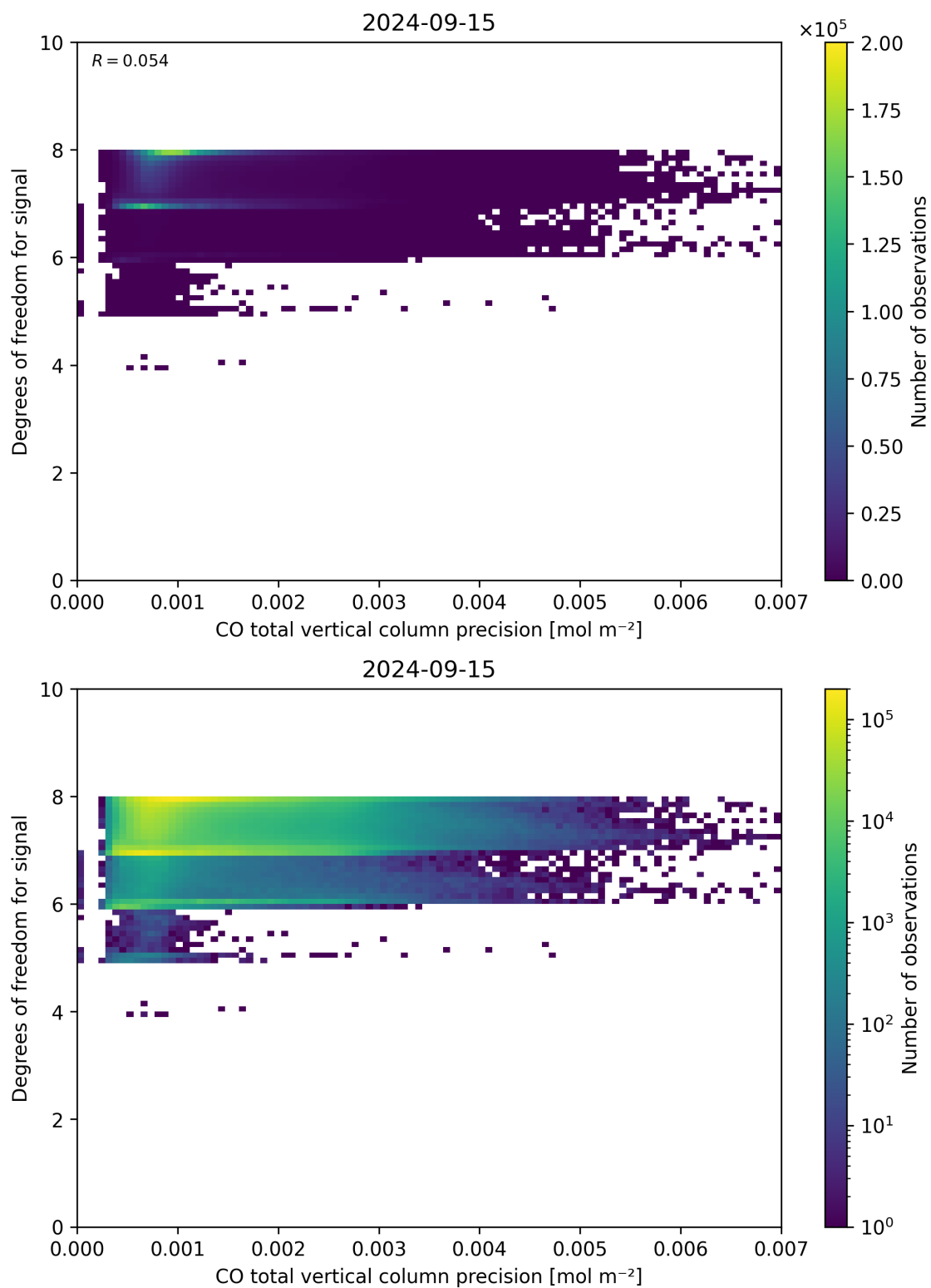
Figure 45: Scatter density plot of “CO total vertical column precision” against “Degrees of freedom for signal” for 2024-09-14 to 2024-09-16.
