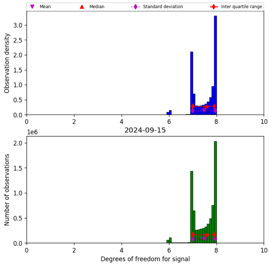
Figure 23: Histogram of “Degrees of freedom for signal” for 2024-09-14 to 2024-09-16
