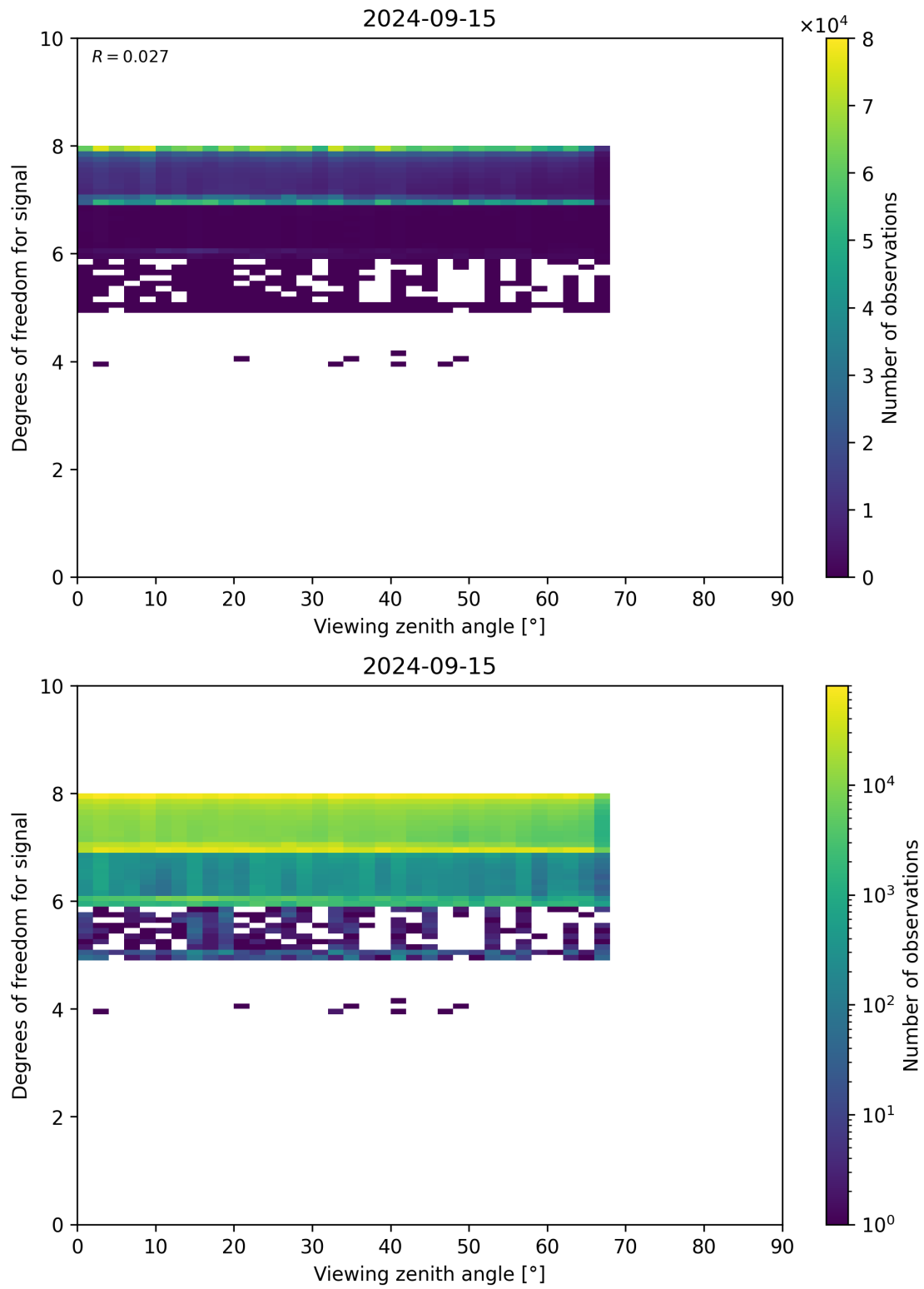
Figure 73: Scatter density plot of “Viewing zenith angle” against “Degrees of freedom for signal” for 2024-09-14 to 2024-09-16.
