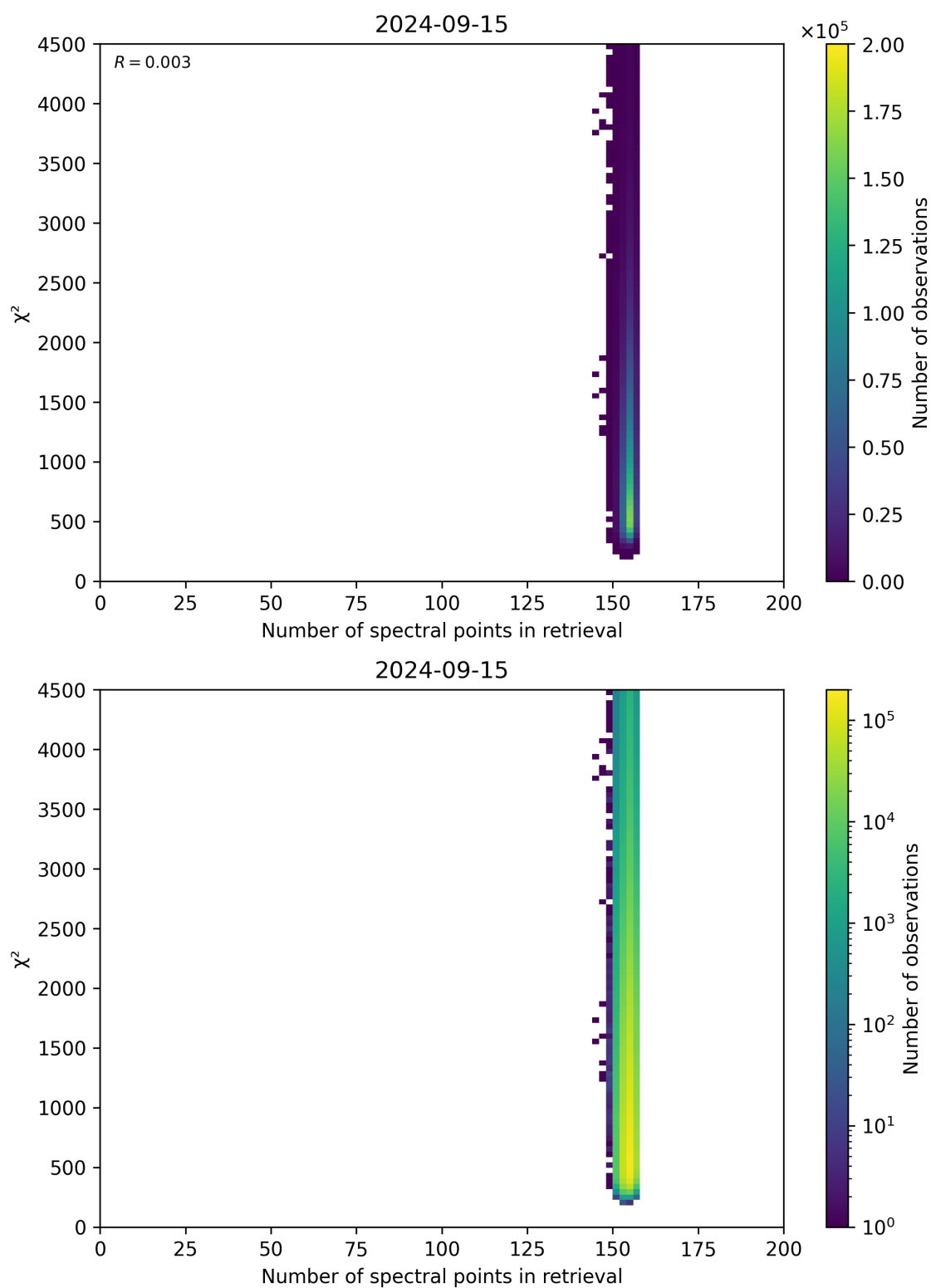
Figure 58: Scatter density plot of “Number of spectral points in retrieval” against “ \chi^2 ” for 2024-09-14 to 2024-09-16.
