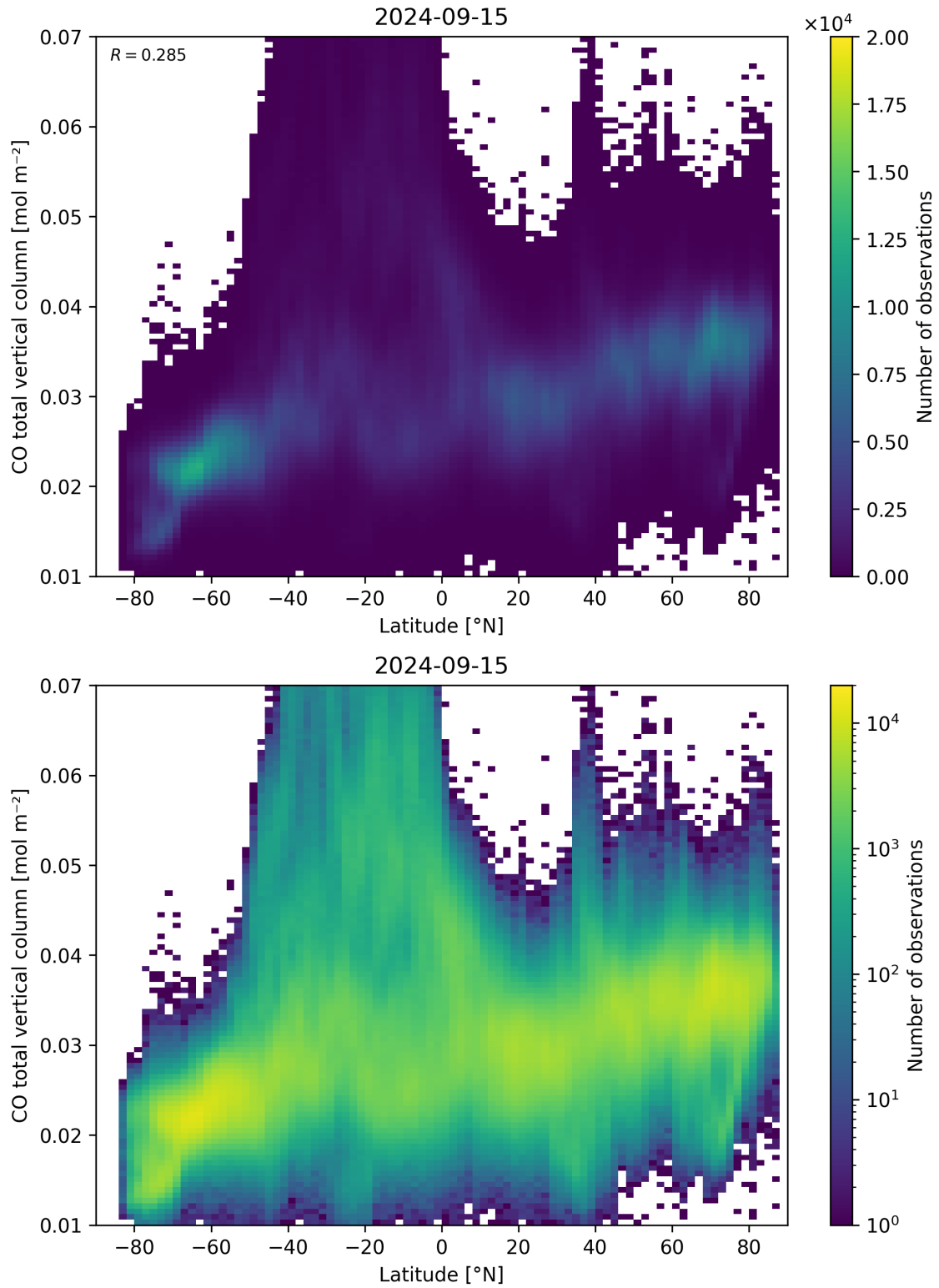
Figure 51: Scatter density plot of “Latitude” against “CO total vertical column” for 2024-09-14 to 2024-09-16.
