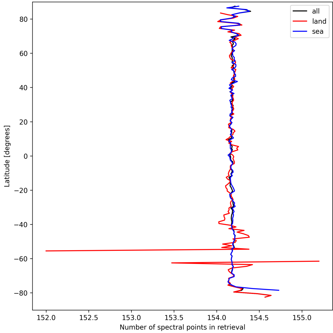
Figure 13: Zonal average of “Number of spectral points in retrieval” for 2024-09-14 to 2024-09-16.
