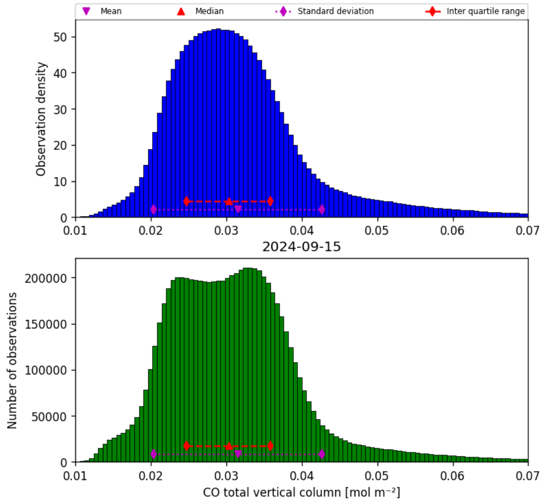
Figure 18: Histogram of “CO total vertical column” for 2024-09-14 to 2024-09-16
