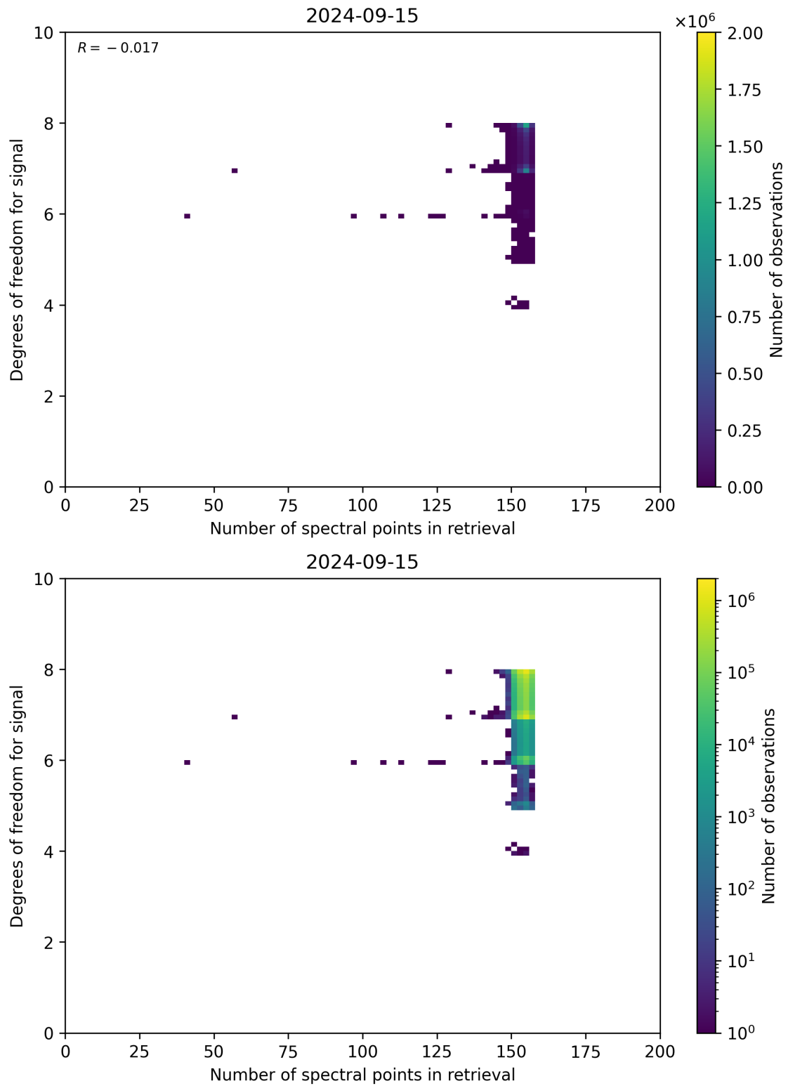
Figure 59: Scatter density plot of “Number of spectral points in retrieval” against “Degrees of freedom for signal” for 2024-09-14 to 2024-09-16.
