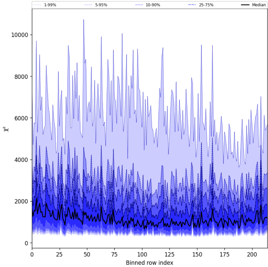
Figure 30: Along track statistics of “ \chi^2 ” for 2024-09-14 to 2024-09-16
