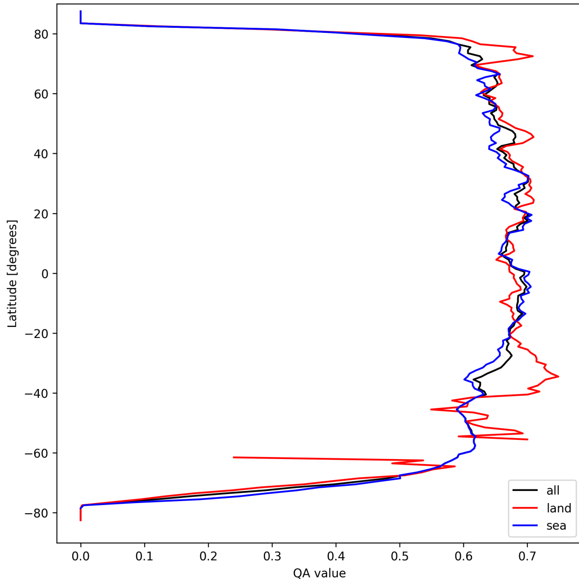
Figure 9: Zonal average of “QA value” for 2024-09-14 to 2024-09-16.
