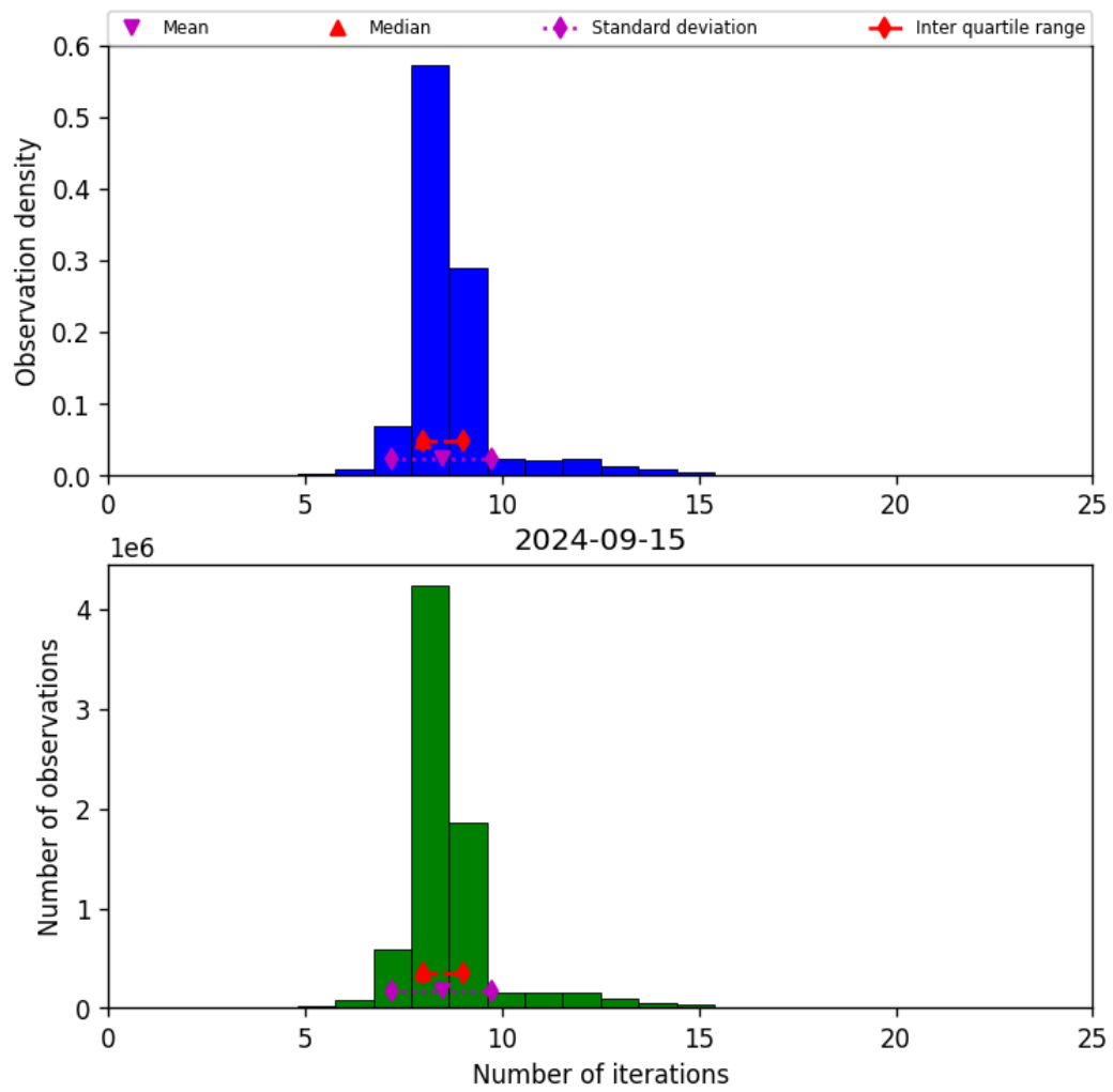
Figure 24: Histogram of “Number of iterations” for 2024-09-14 to 2024-09-16
