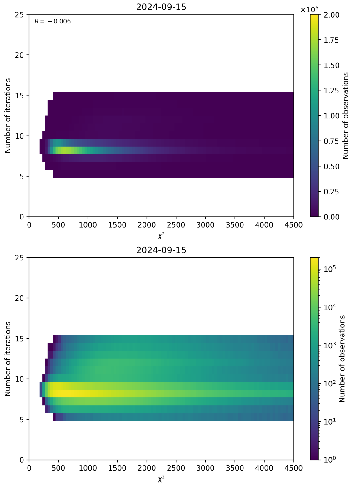
Figure 49: Scatter density plot of “ \chi^2 ” against “Number of iterations” for 2024-09-14 to 2024-09-16.
