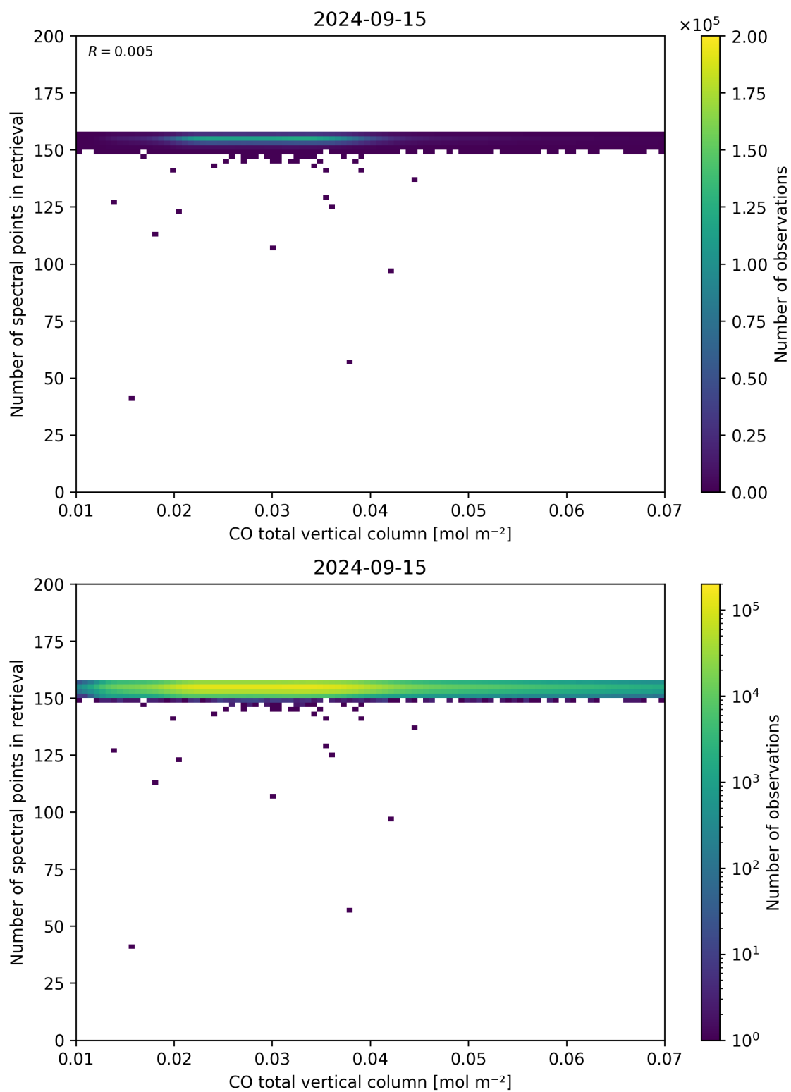
Figure 43: Scatter density plot of “CO total vertical column” against “Number of spectral points in retrieval” for 2024-09-14 to 2024-09-16.
