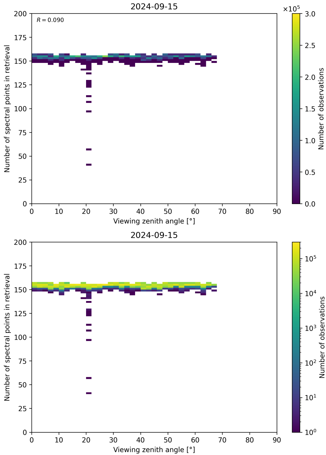
Figure 76: Scatter density plot of “Viewing zenith angle” against “Number of spectral points in retrieval” for 2024-09-14 to 2024-09-16.
