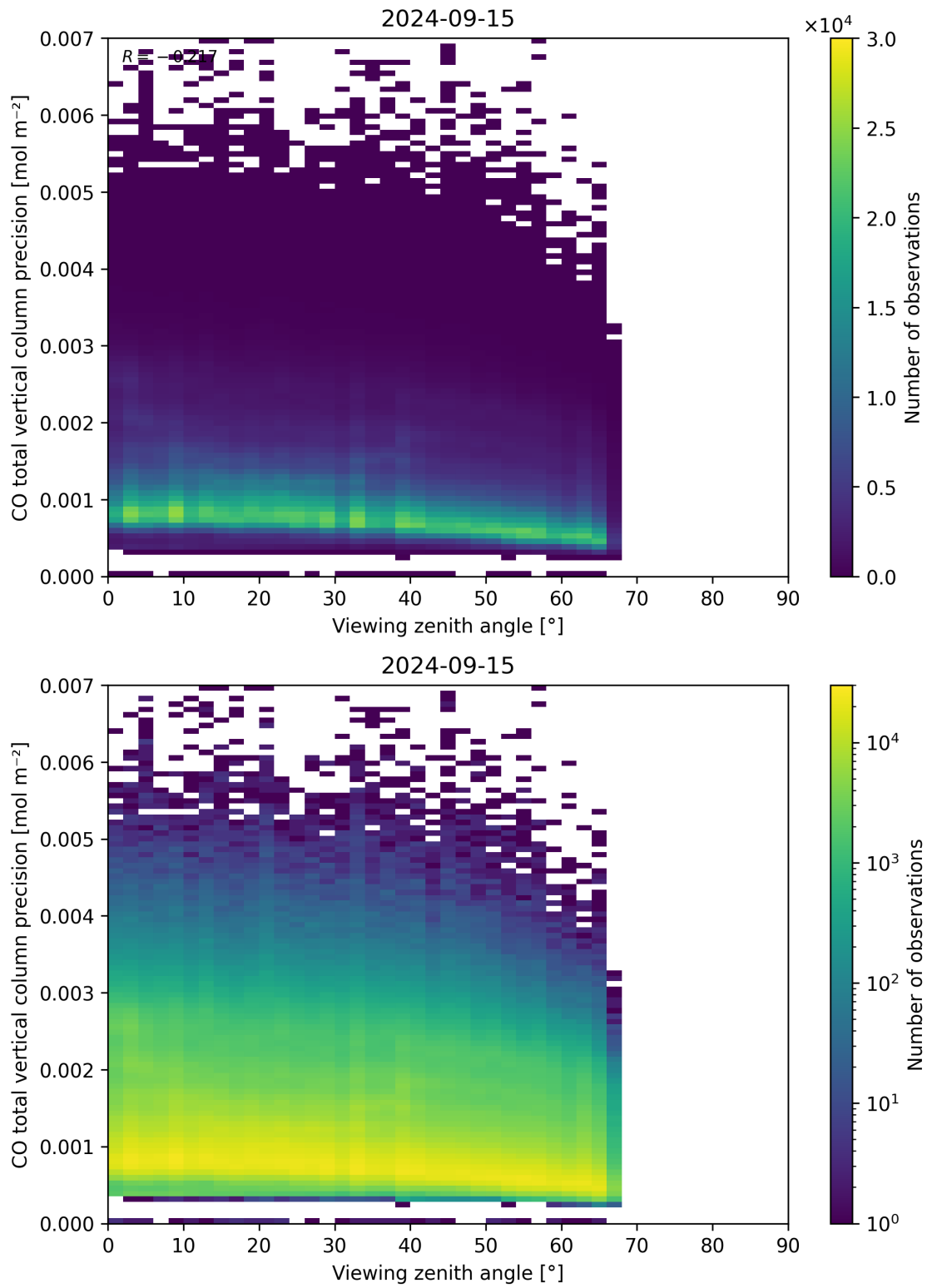
Figure 71: Scatter density plot of “Viewing zenith angle” against “CO total vertical column precision” for 2024-09-14 to 2024-09-16.
