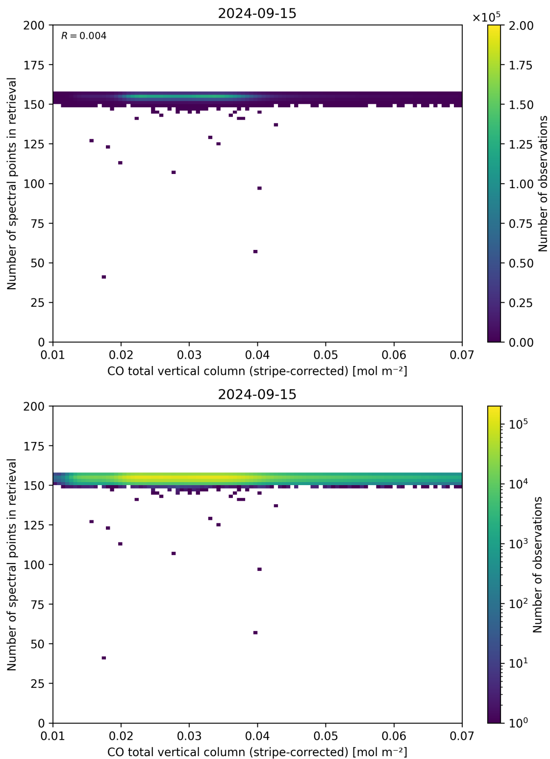
Figure 40: Scatter density plot of “CO total vertical column (stripe-corrected)” against “Number of spectral points in retrieval” for 2024-09-14 to 2024-09-16.
