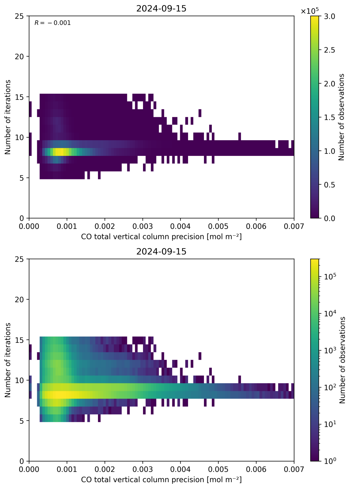
Figure 46: Scatter density plot of “CO total vertical column precision” against “Number of iterations” for 2024-09-14 to 2024-09-16.
