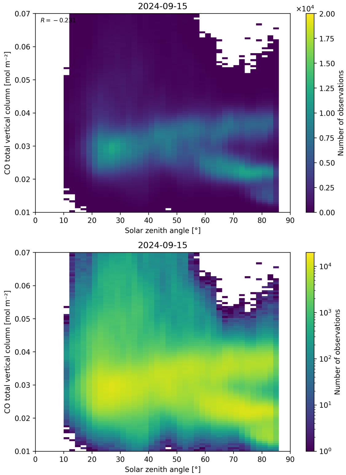
Figure 61: Scatter density plot of “Solar zenith angle” against “CO total vertical column” for 2024-09-14 to 2024-09-16.
