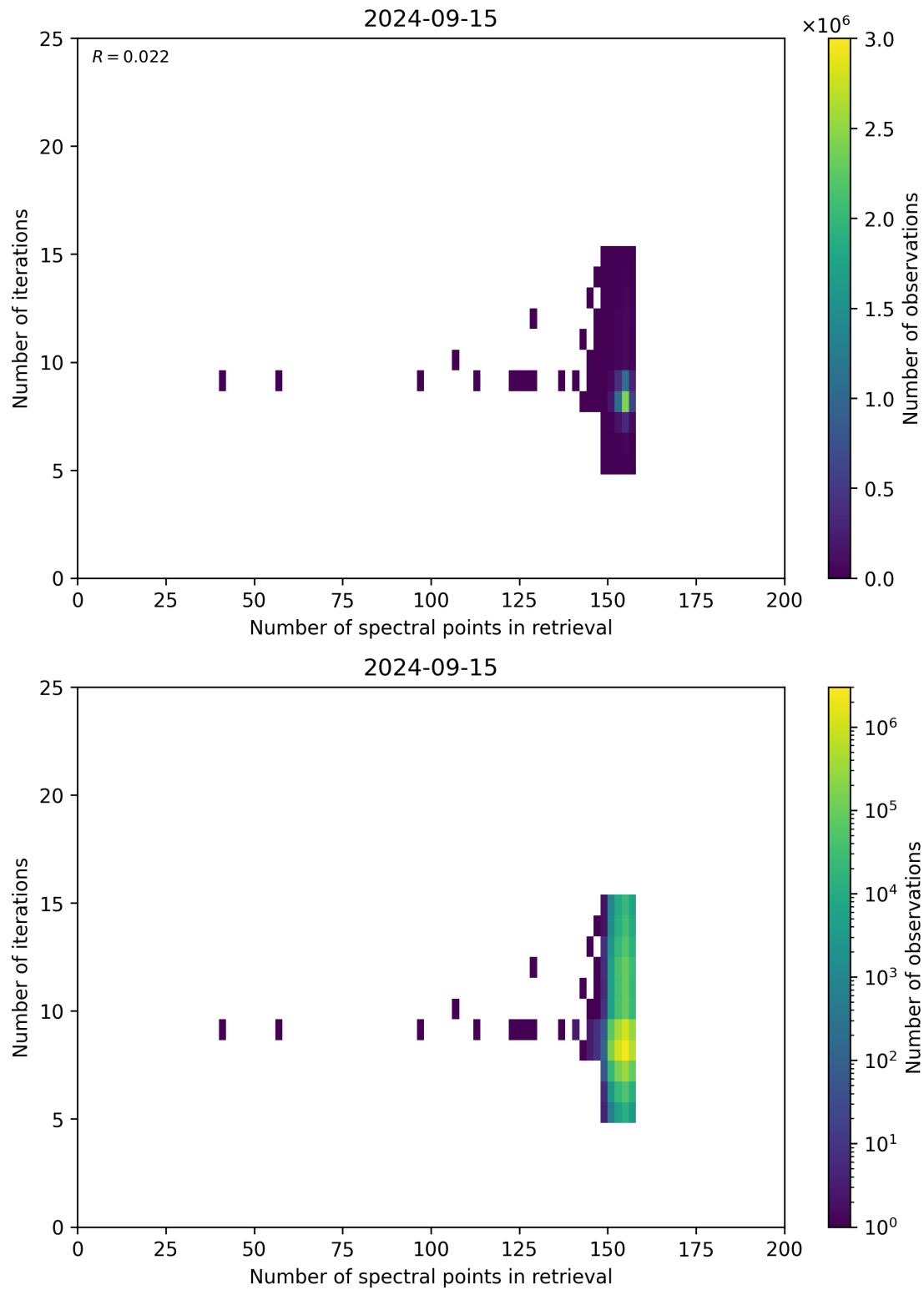
Figure 60: Scatter density plot of “Number of spectral points in retrieval” against “Number of iterations” for 2024-09-14 to 2024-09-16.
