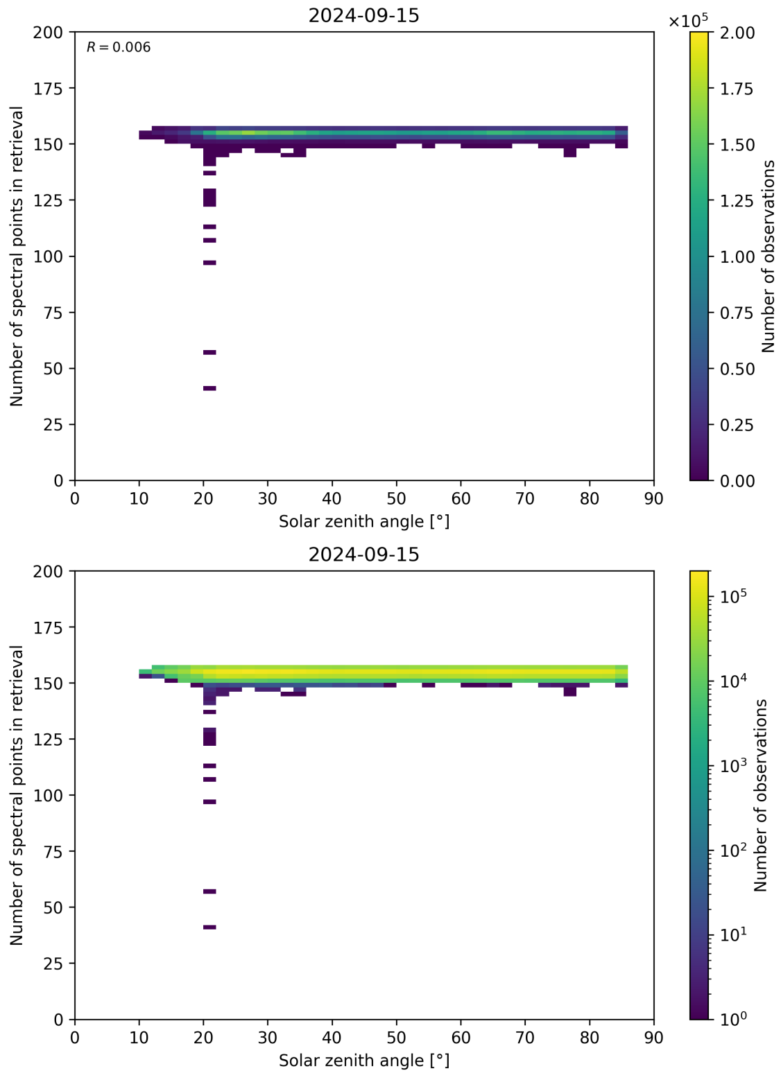
Figure 68: Scatter density plot of “Solar zenith angle” against “Number of spectral points in retrieval” for 2024-09-14 to 2024-09-16.
