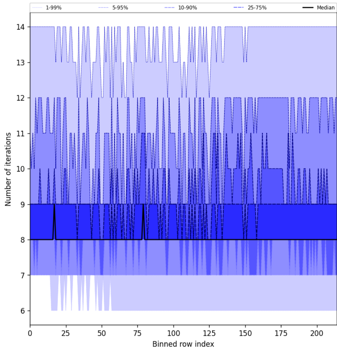
Figure 32: Along track statistics of “Number of iterations” for 2024-09-14 to 2024-09-16
