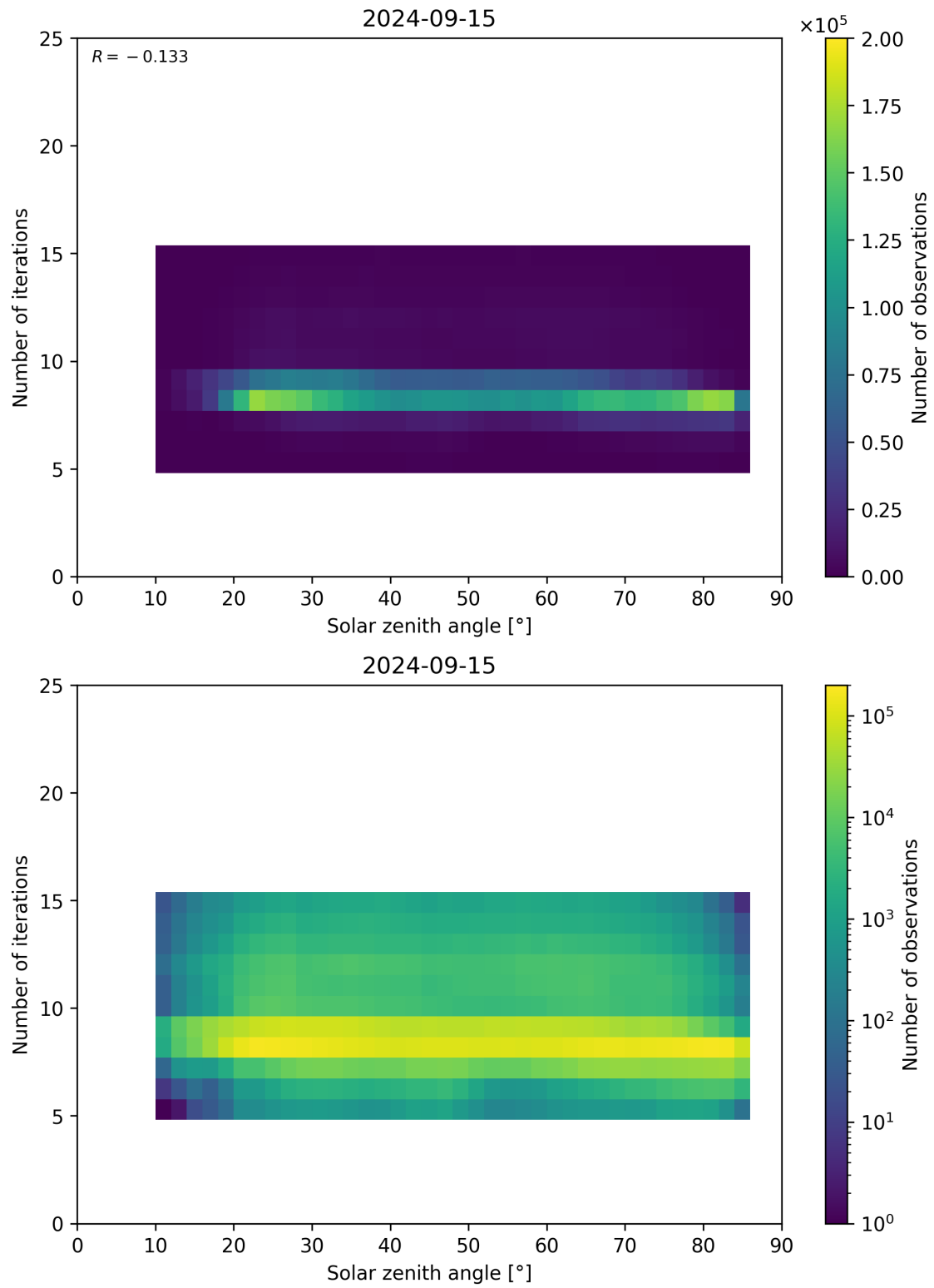
Figure 67: Scatter density plot of “Solar zenith angle” against “Number of iterations” for 2024-09-14 to 2024-09-16.
