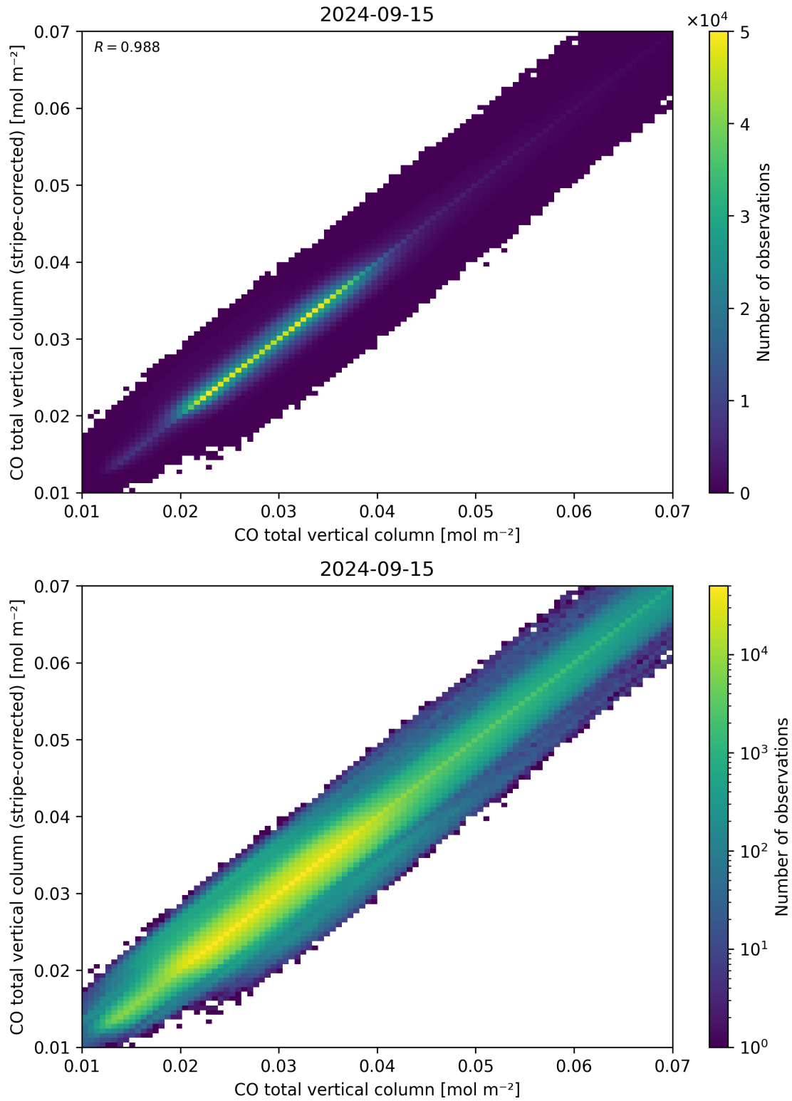
Figure 33: Scatter density plot of “CO total vertical column” against “CO total vertical column (stripe-corrected)” for 2024-09-14 to 2024-09-16.
