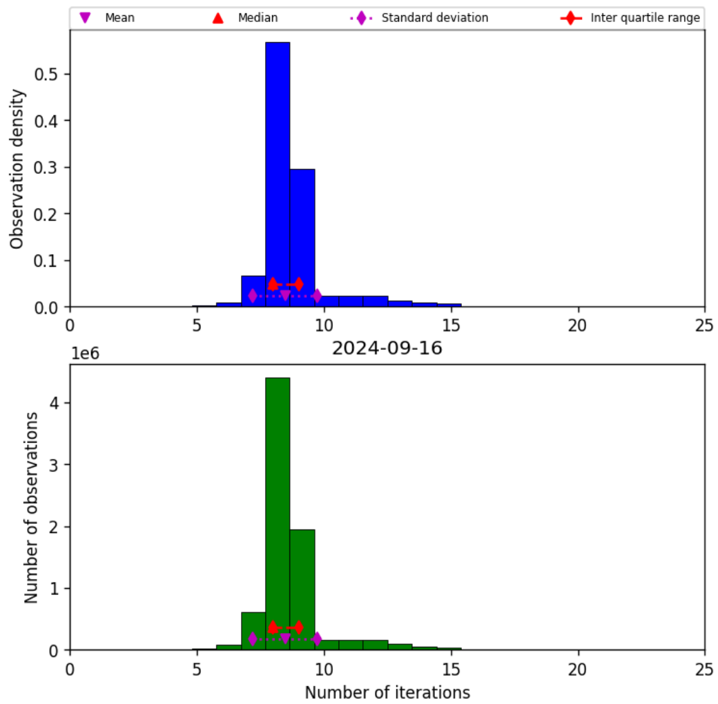
Figure 24: Histogram of “Number of iterations” for 2024-09-15 to 2024-09-17
