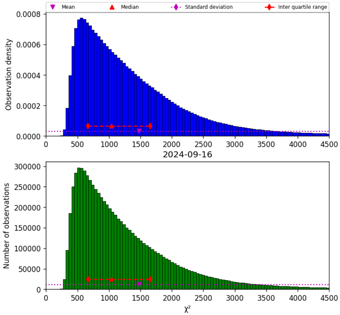
Figure 22: Histogram of “ \chi^2 ” for 2024-09-15 to 2024-09-17
