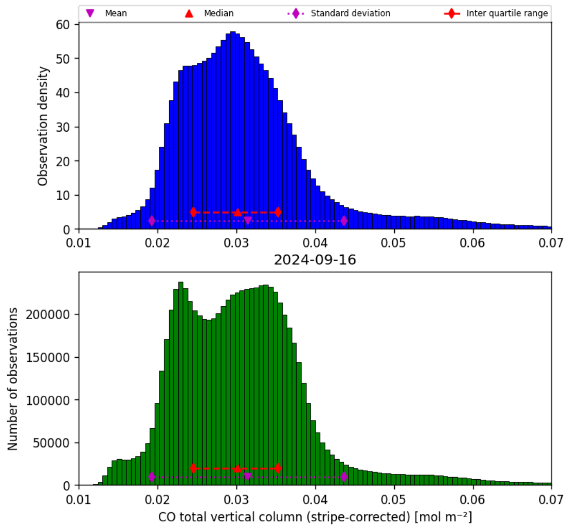
Figure 19: Histogram of “CO total vertical column (stripe-corrected)” for 2024-09-15 to 2024-09-17
