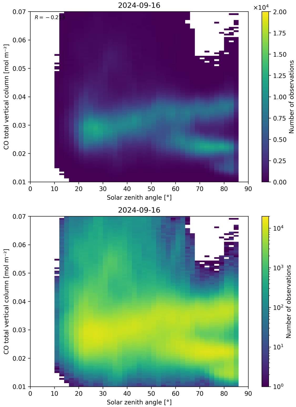
Figure 61: Scatter density plot of “Solar zenith angle” against “CO total vertical column” for 2024-09-15 to 2024-09-17.
