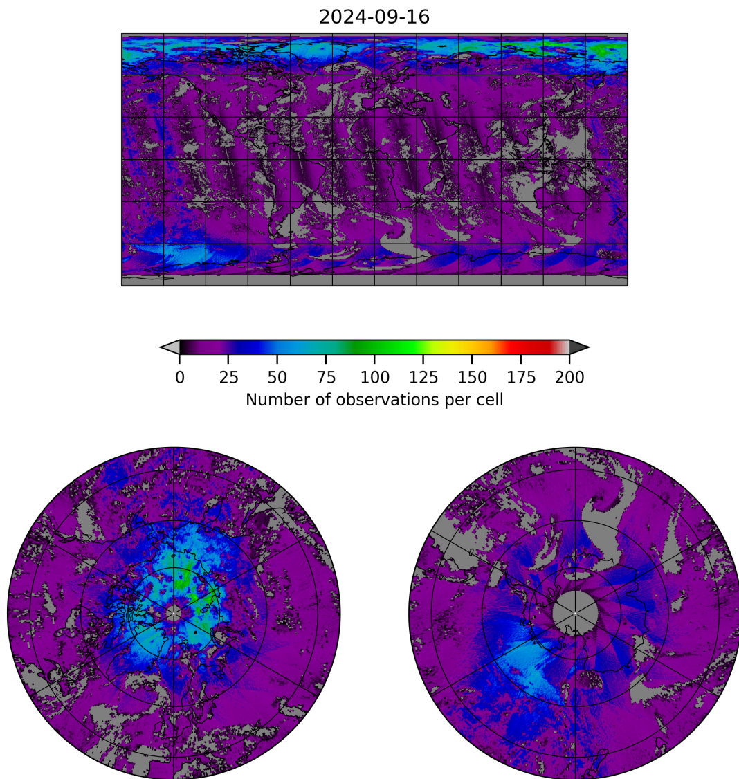
Figure 8: Map of the number of observations for 2024-09-15 to 2024-09-17
