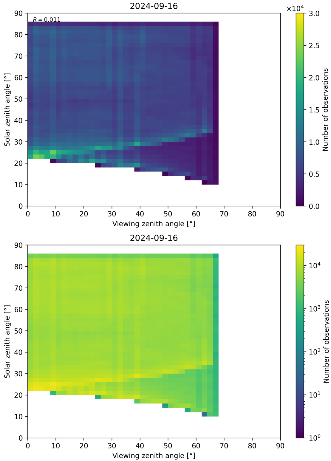
Figure 77: Scatter density plot of “Viewing zenith angle” against “Solar zenith angle” for 2024-09-15 to 2024-09-17.
