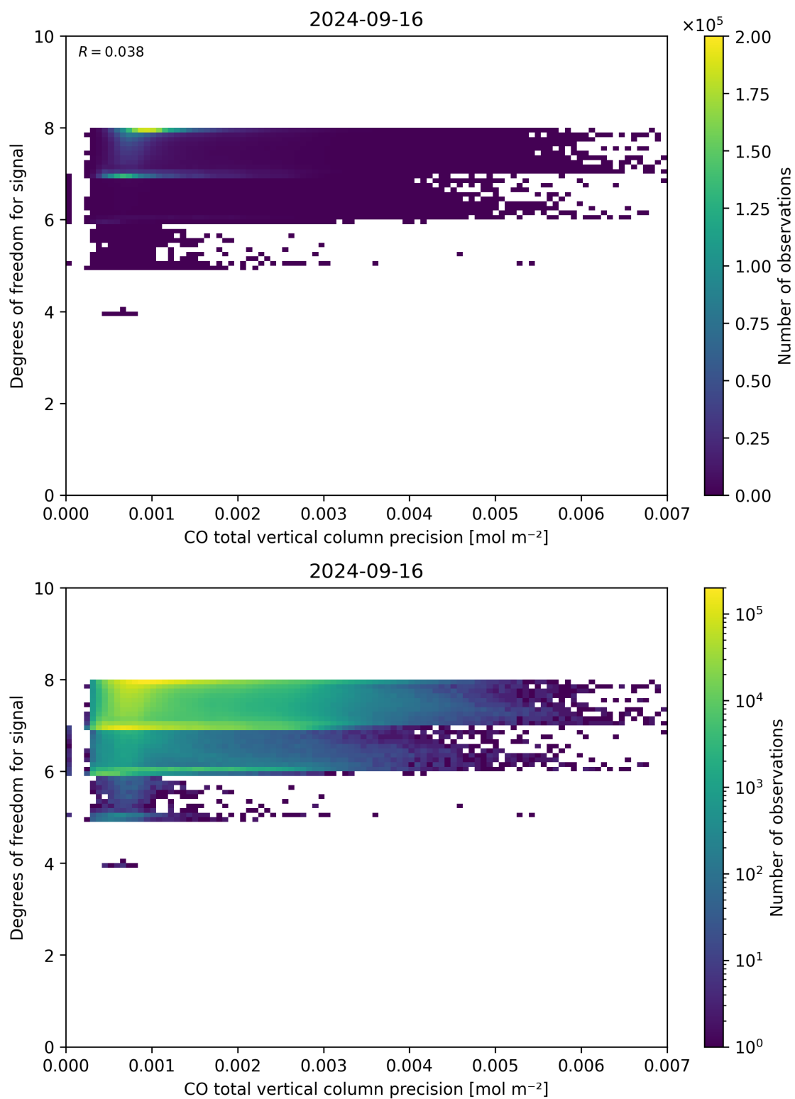
Figure 45: Scatter density plot of “CO total vertical column precision” against “Degrees of freedom for signal” for 2024-09-15 to 2024-09-17.
