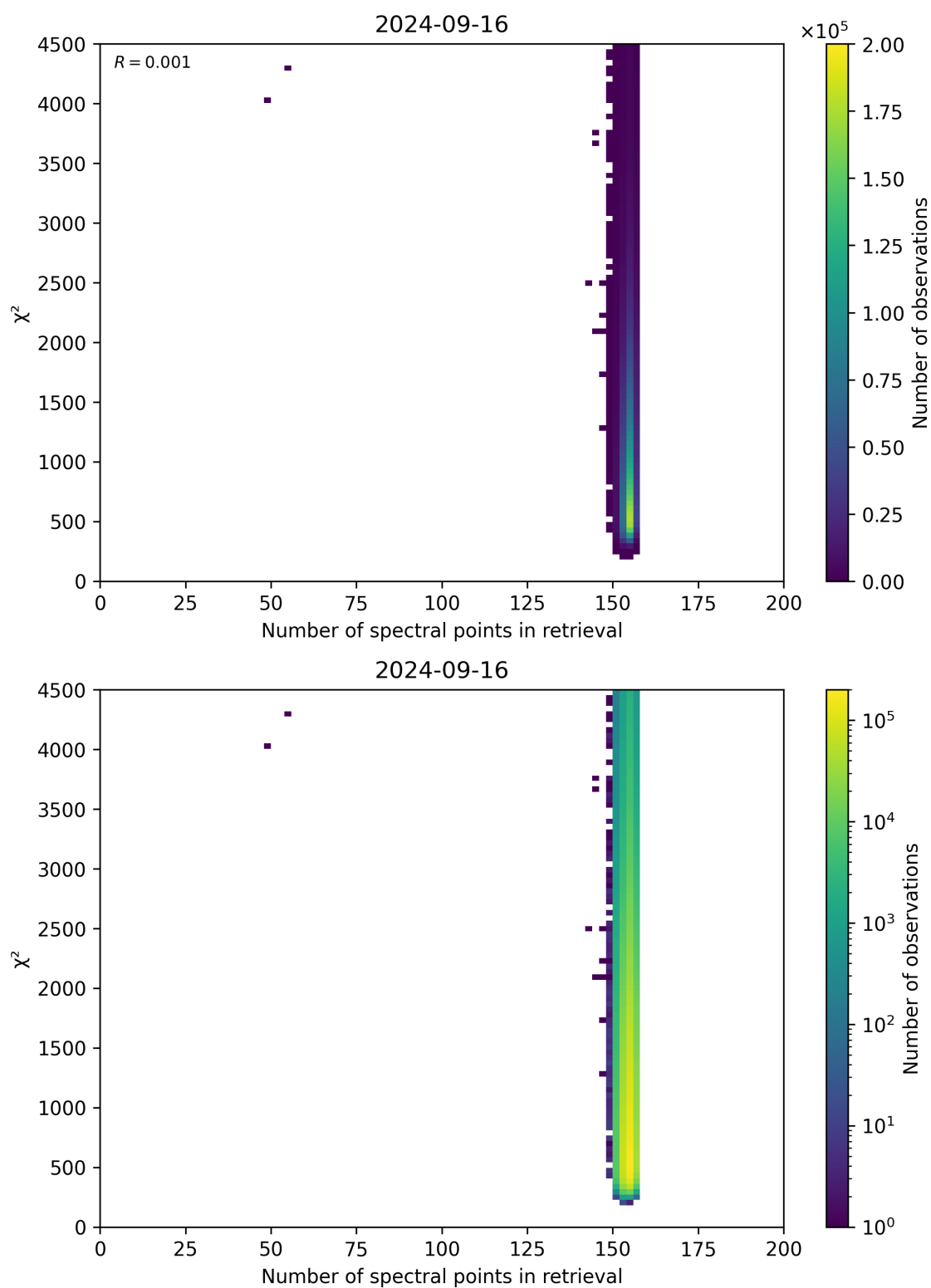
Figure 58: Scatter density plot of “Number of spectral points in retrieval” against “ \chi^2 ” for 2024-09-15 to 2024-09-17.
