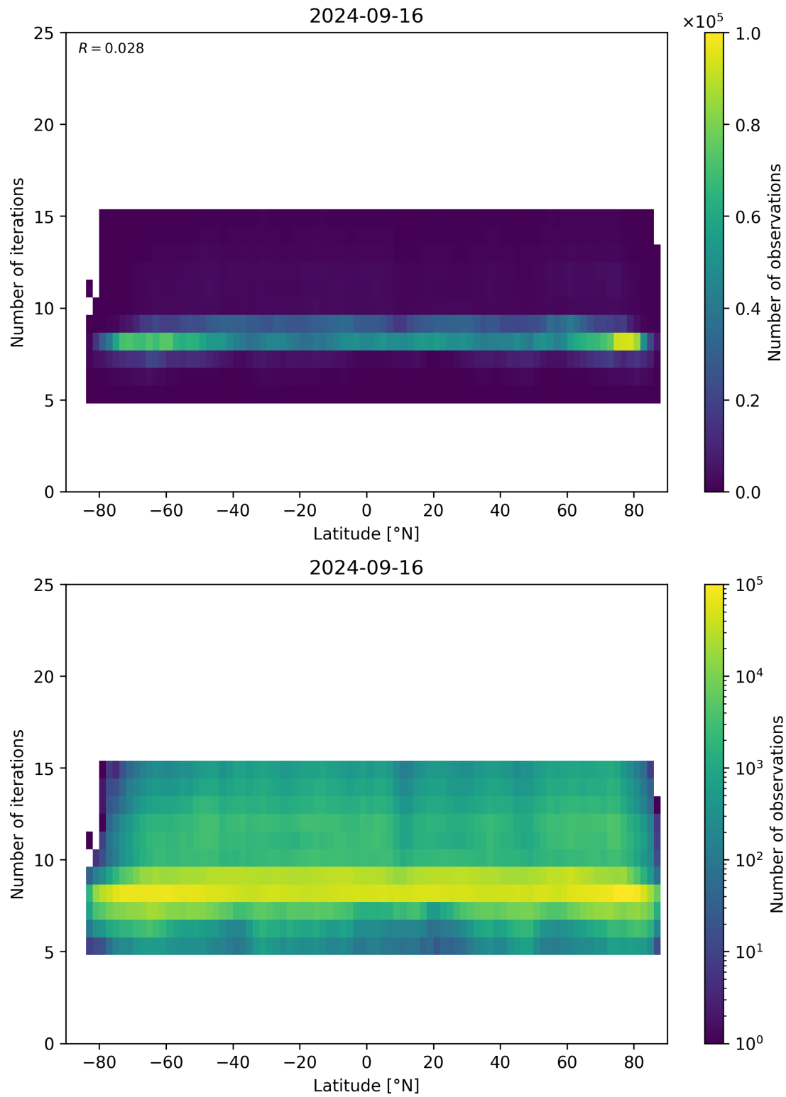
Figure 56: Scatter density plot of “Latitude” against “Number of iterations” for 2024-09-15 to 2024-09-17.
