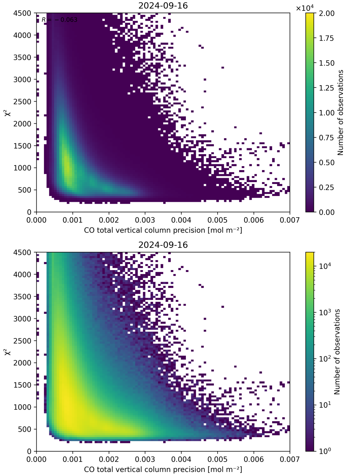
Figure 44: Scatter density plot of “CO total vertical column precision” against “ \chi^2 ” for 2024-09-15 to 2024-09-17.
