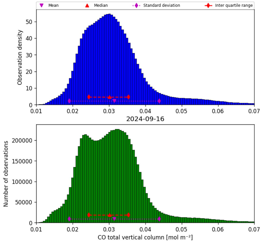
Figure 18: Histogram of “CO total vertical column” for 2024-09-15 to 2024-09-17
