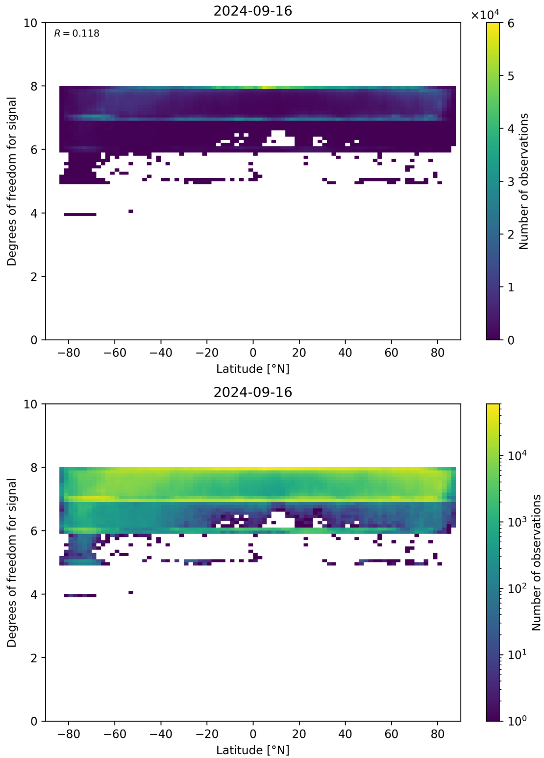
Figure 55: Scatter density plot of “Latitude” against “Degrees of freedom for signal” for 2024-09-15 to 2024-09-17.
