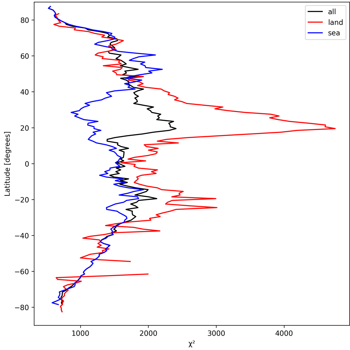
Figure 14: Zonal average of “ \chi^2 ” for 2024-09-15 to 2024-09-17.
