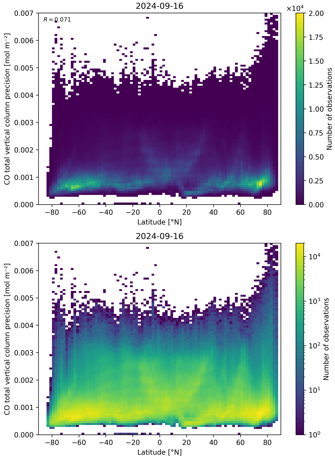
Figure 53: Scatter density plot of “Latitude” against “CO total vertical column precision” for 2024-09-15 to 2024-09-17.
