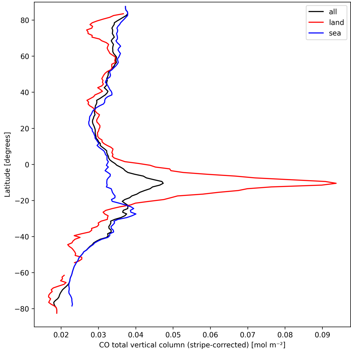
Figure 11: Zonal average of “CO total vertical column (stripe-corrected)” for 2024-09-15 to 2024-09-17.
