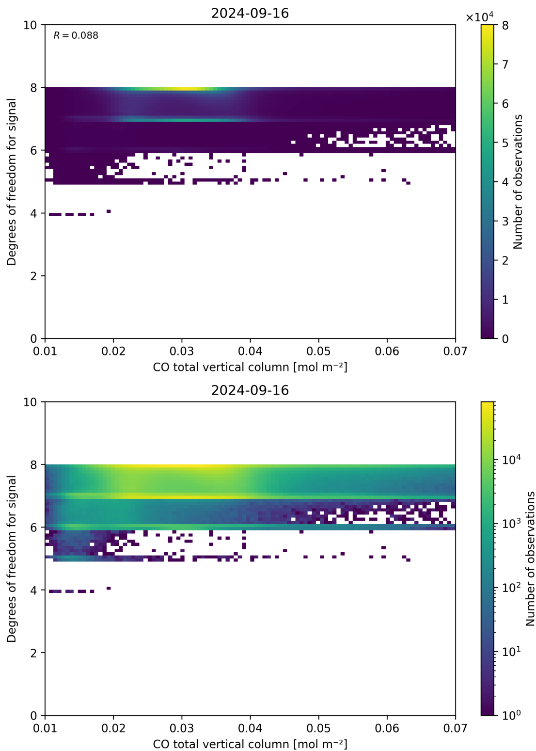
Figure 41: Scatter density plot of “CO total vertical column” against “Degrees of freedom for signal” for 2024-09-15 to 2024-09-17.
