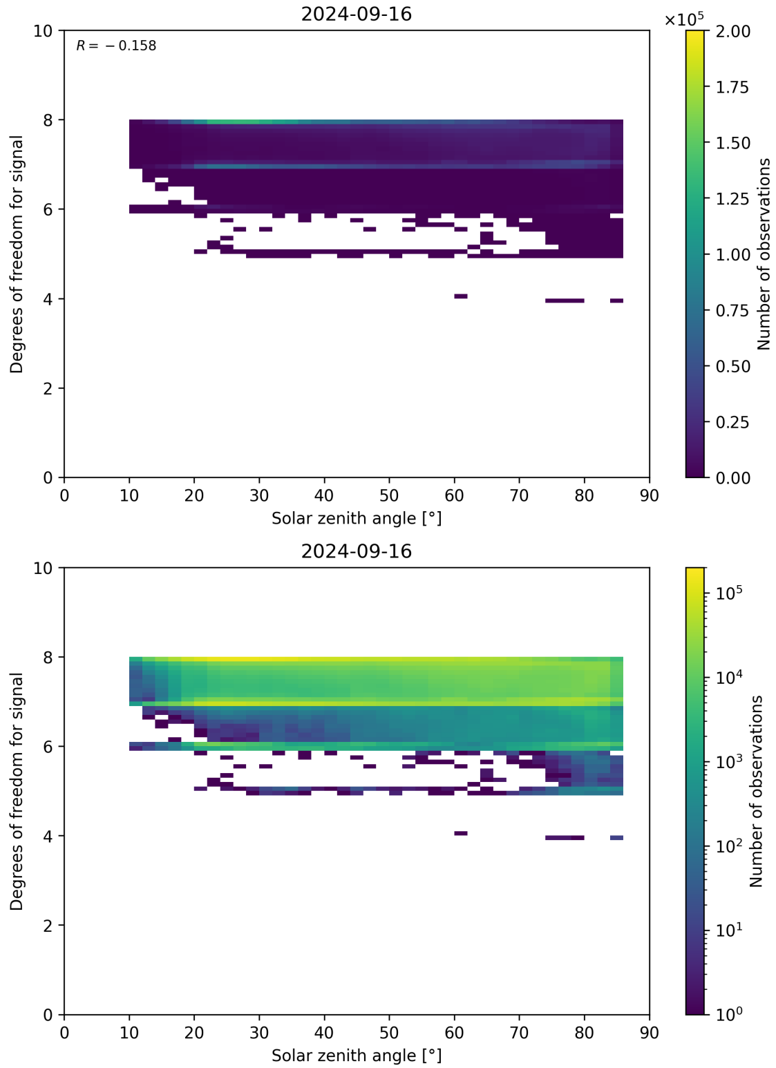
Figure 65: Scatter density plot of “Solar zenith angle” against “Degrees of freedom for signal” for 2024-09-15 to 2024-09-17.
