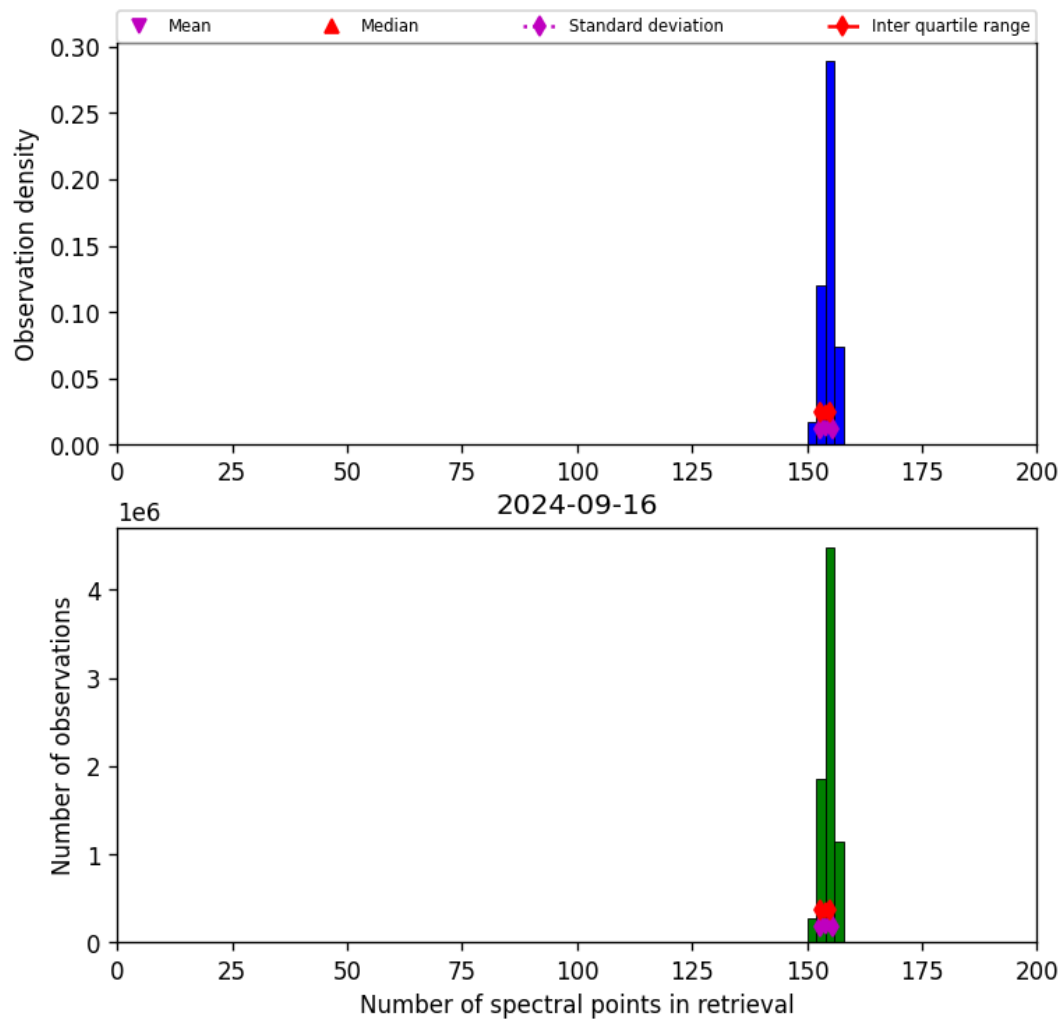
Figure 21: Histogram of “Number of spectral points in retrieval” for 2024-09-15 to 2024-09-17
