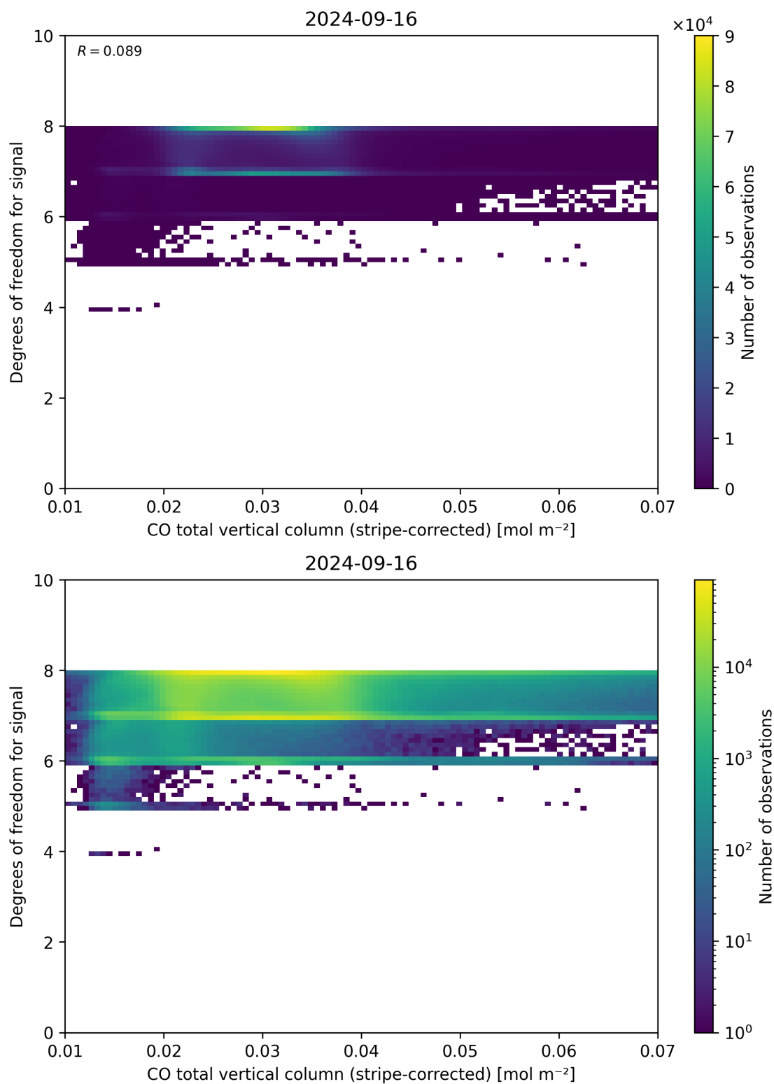
Figure 38: Scatter density plot of “CO total vertical column (stripe-corrected)” against “Degrees of freedom for signal” for 2024-09-15 to 2024-09-17.
