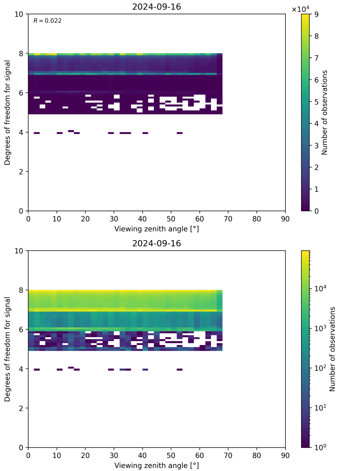
Figure 73: Scatter density plot of “Viewing zenith angle” against “Degrees of freedom for signal” for 2024-09-15 to 2024-09-17.
