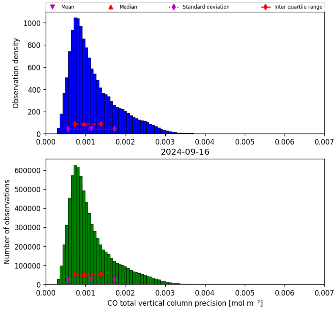
Figure 20: Histogram of “CO total vertical column precision” for 2024-09-15 to 2024-09-17
