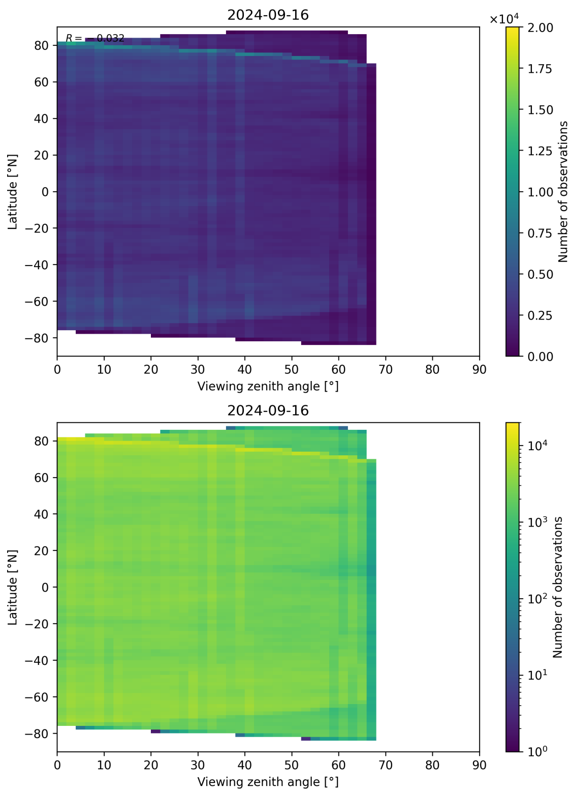
Figure 74: Scatter density plot of “Viewing zenith angle” against “Latitude” for 2024-09-15 to 2024-09-17.
