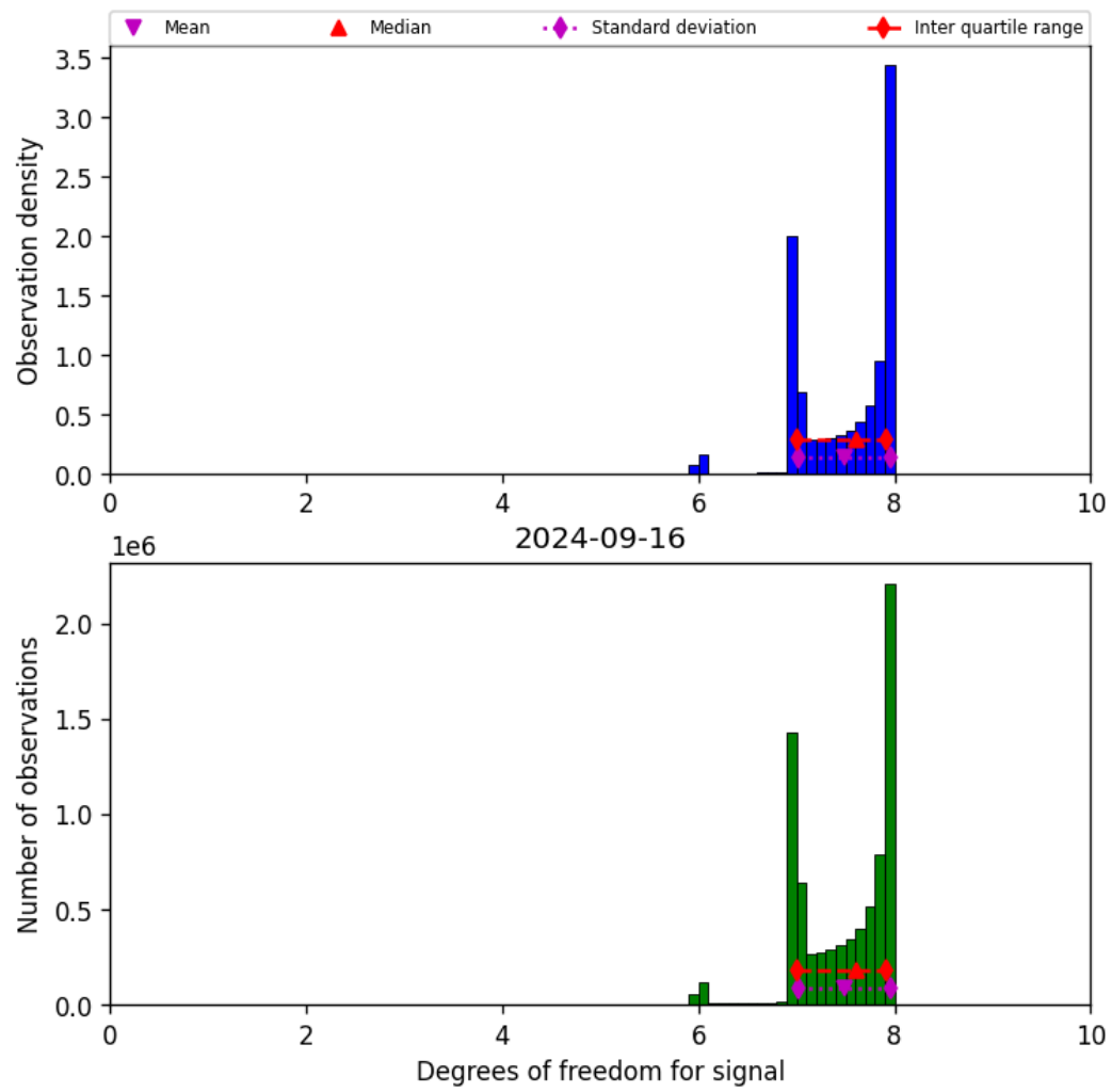
Figure 23: Histogram of “Degrees of freedom for signal” for 2024-09-15 to 2024-09-17
