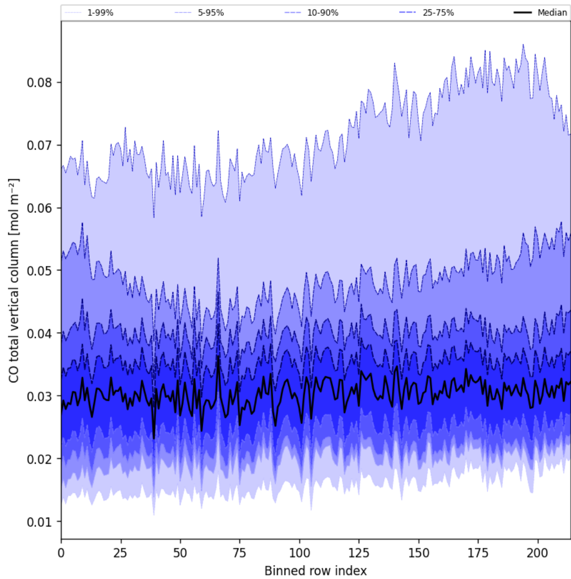
Figure 26: Along track statistics of “CO total vertical column” for 2024-09-15 to 2024-09-17
