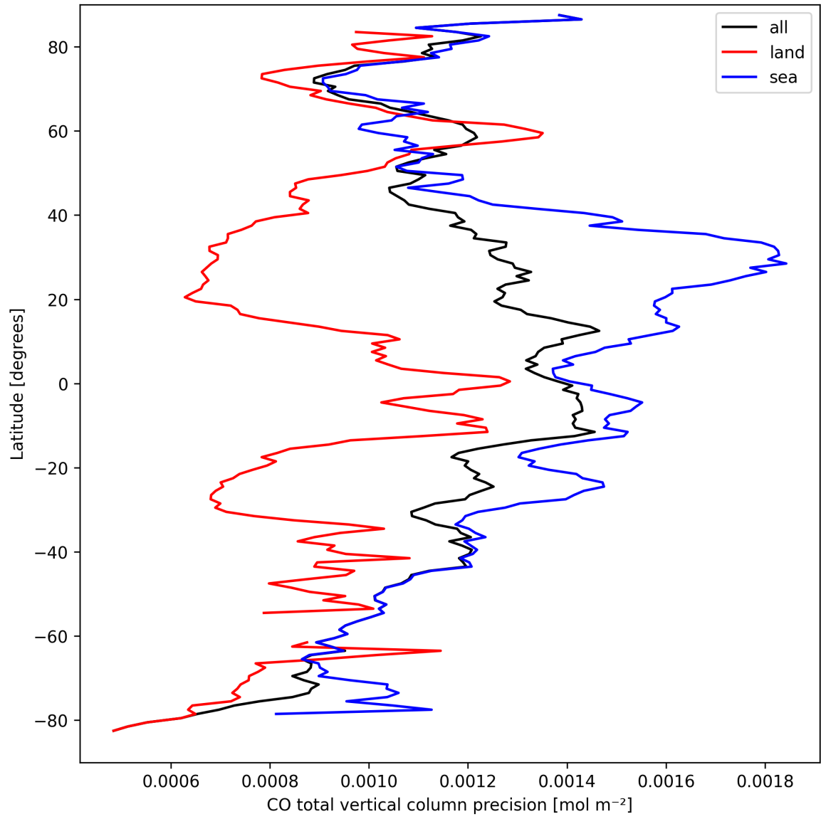
Figure 12: Zonal average of "CO total vertical column precision" for 2024-09-15 to 2024-09-17.
