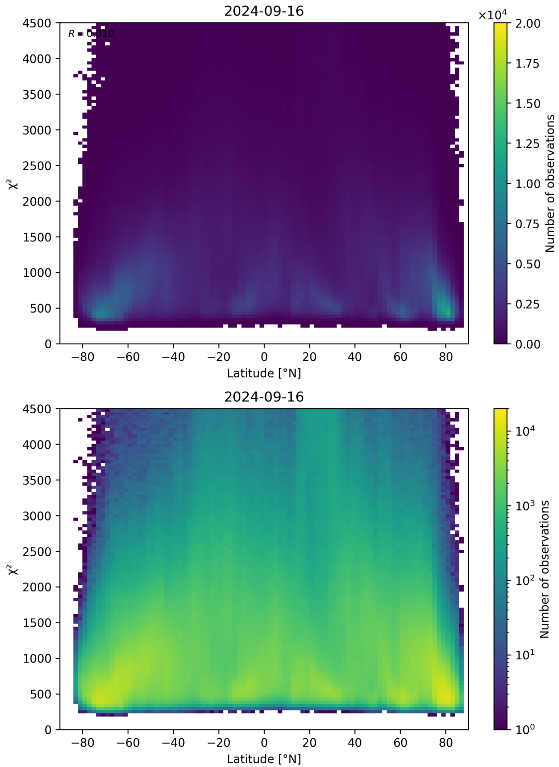
Figure 54: Scatter density plot of “Latitude” against “ \chi^2 ” for 2024-09-15 to 2024-09-17.
