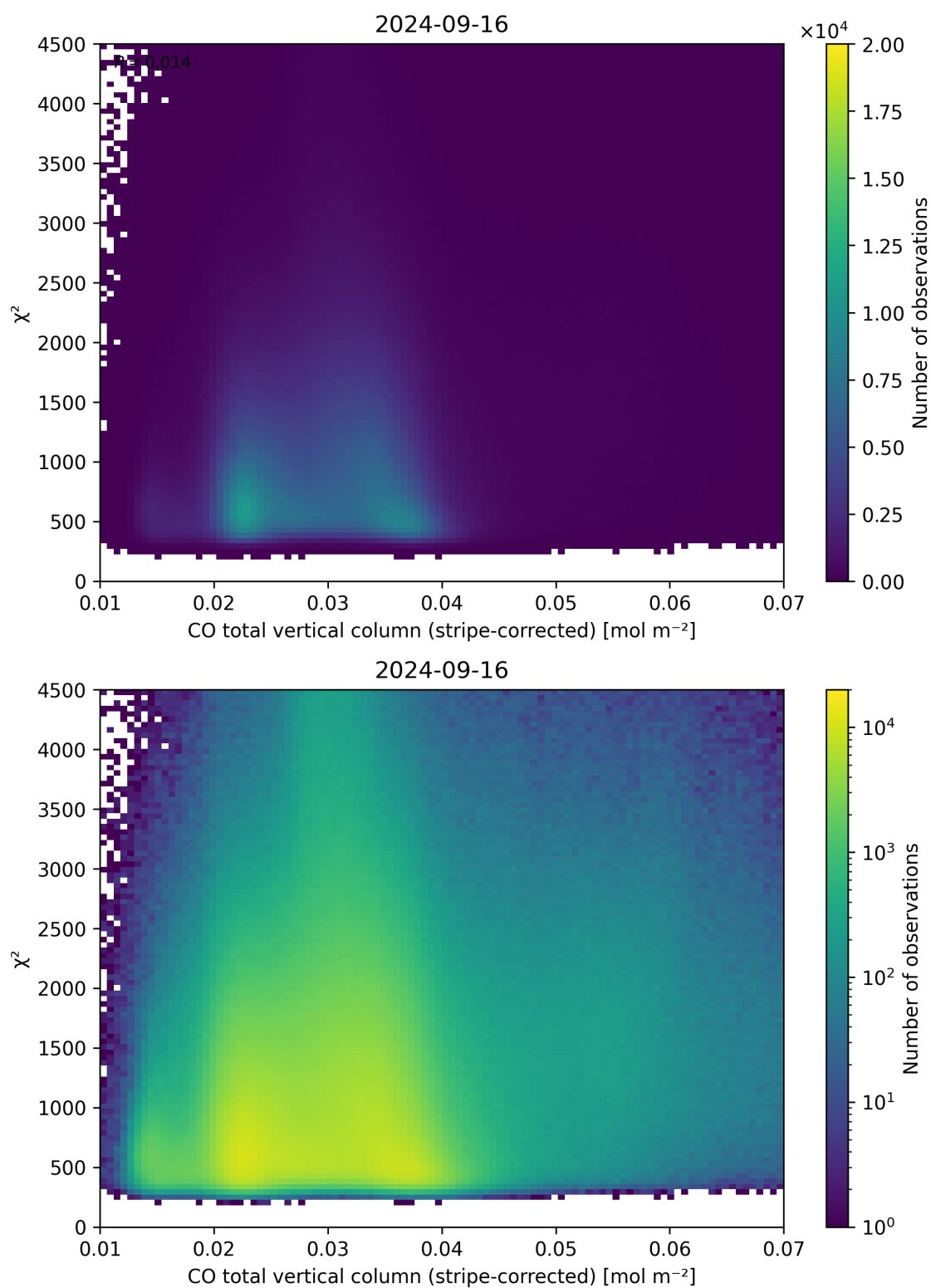
Figure 37: Scatter density plot of “CO total vertical column (stripe-corrected)” against “ \chi^2 ” for 2024-09-15 to 2024-09-17.
