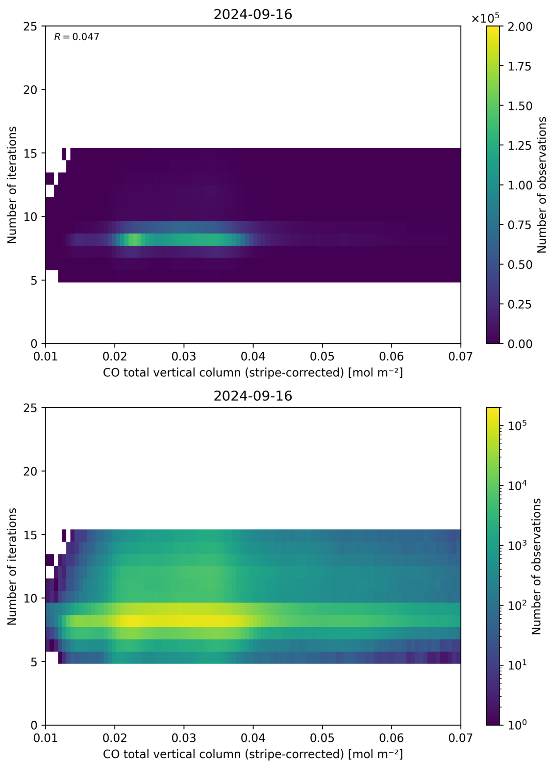
Figure 39: Scatter density plot of “CO total vertical column (stripe-corrected)” against “Number of iterations” for 2024-09-15 to 2024-09-17.
