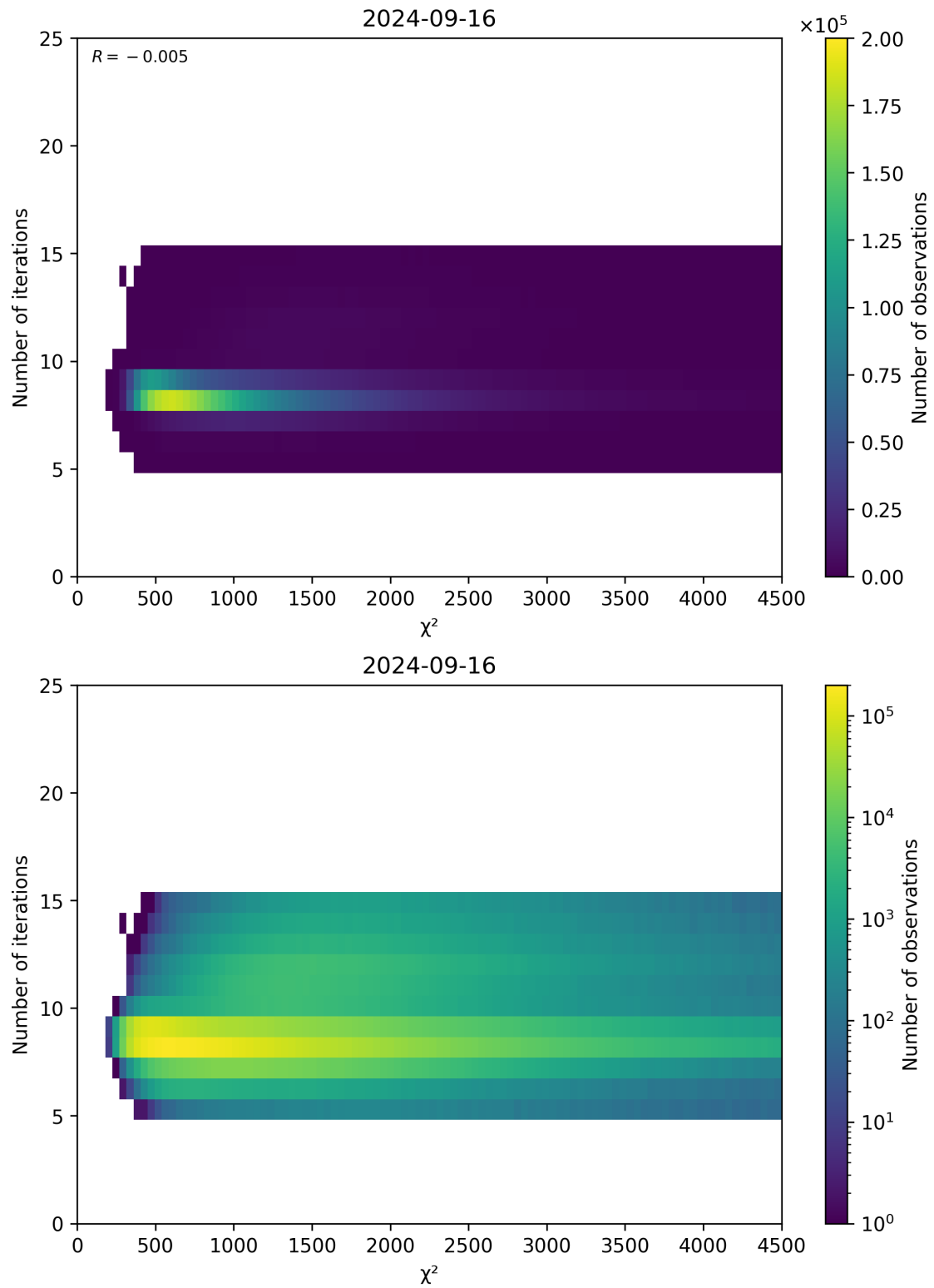
Figure 49: Scatter density plot of “ \chi^2 ” against “Number of iterations” for 2024-09-15 to 2024-09-17.
