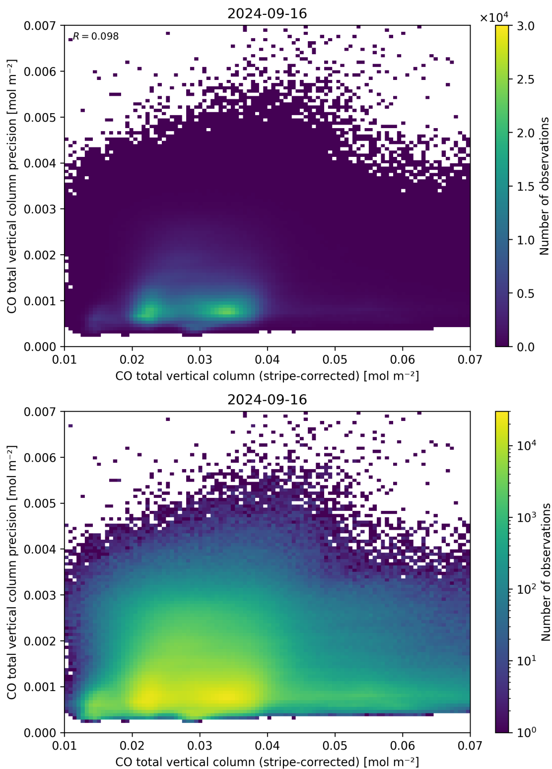
Figure 36: Scatter density plot of “CO total vertical column (stripe-corrected)” against “CO total vertical column precision” for 2024-09-15 to 2024-09-17.
