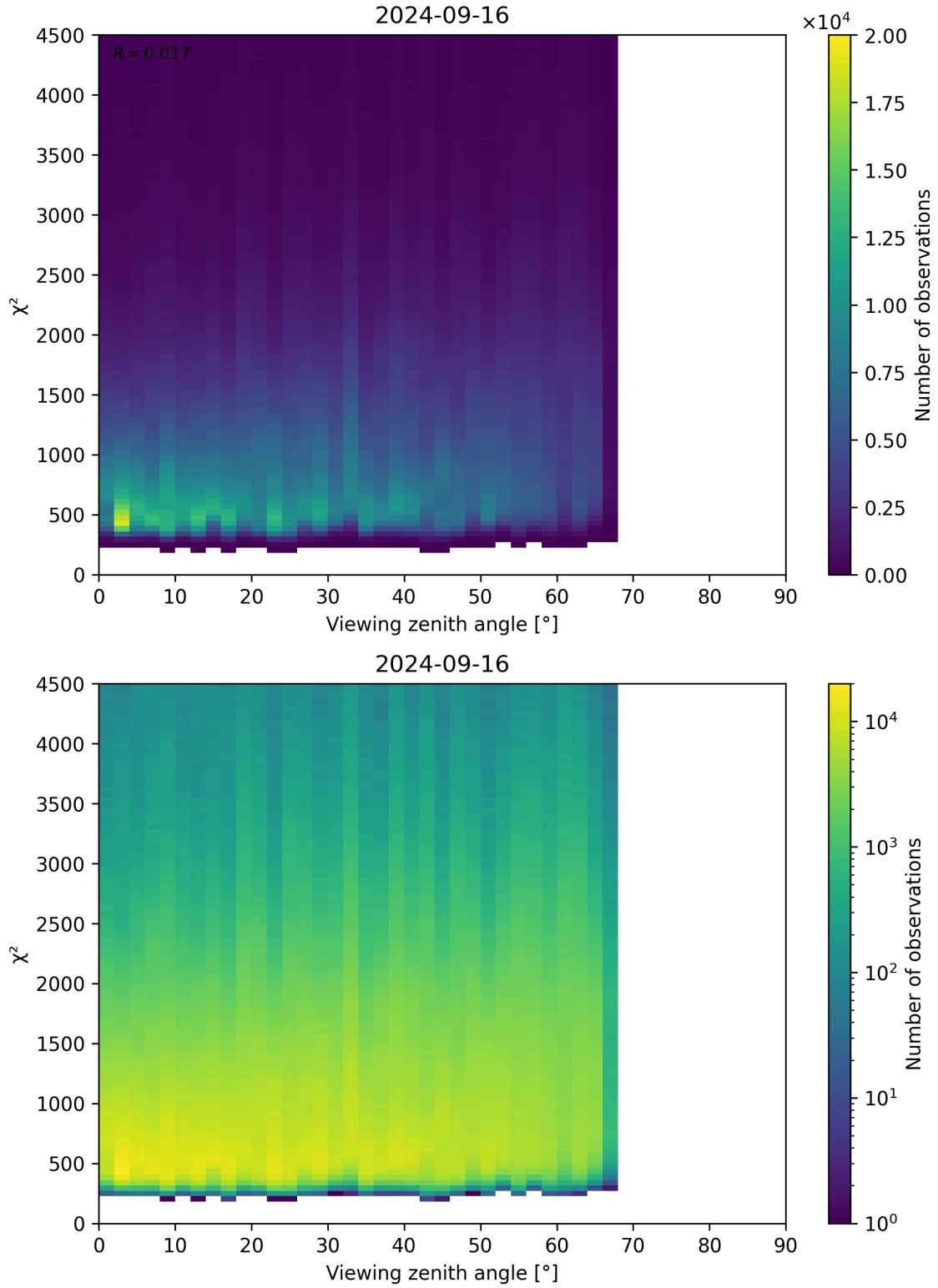
Figure 72: Scatter density plot of “Viewing zenith angle” against “ \chi^2 ” for 2024-09-15 to 2024-09-17.
