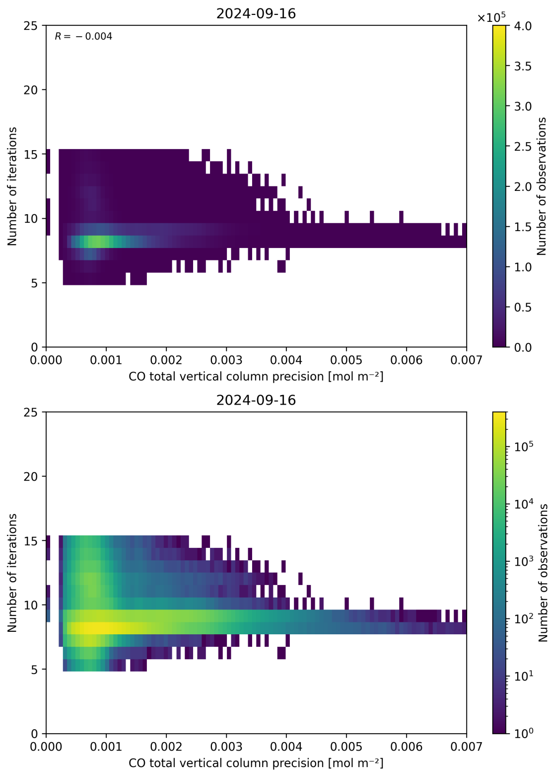
Figure 46: Scatter density plot of “CO total vertical column precision” against “Number of iterations” for 2024-09-15 to 2024-09-17.
