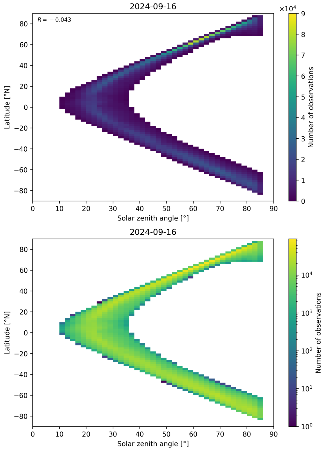
Figure 66: Scatter density plot of “Solar zenith angle” against “Latitude” for 2024-09-15 to 2024-09-17.
