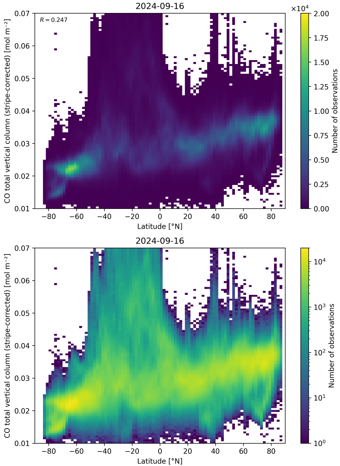
Figure 52: Scatter density plot of “Latitude” against “CO total vertical column (stripe-corrected)” for 2024-09-15 to 2024-09-17.
