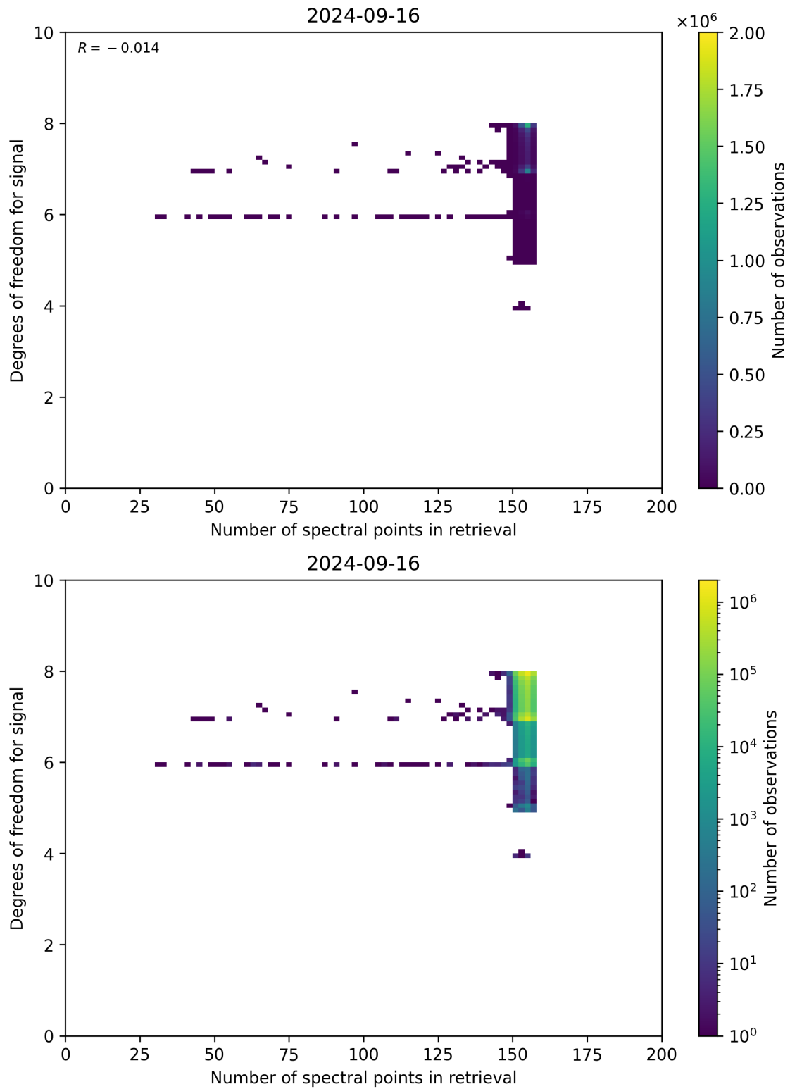
Figure 59: Scatter density plot of “Number of spectral points in retrieval” against “Degrees of freedom for signal” for 2024-09-15 to 2024-09-17.
