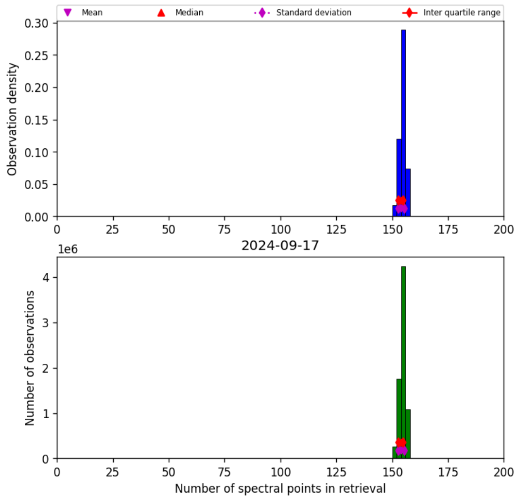
Figure 21: Histogram of “Number of spectral points in retrieval” for 2024-09-17 to 2024-09-18
