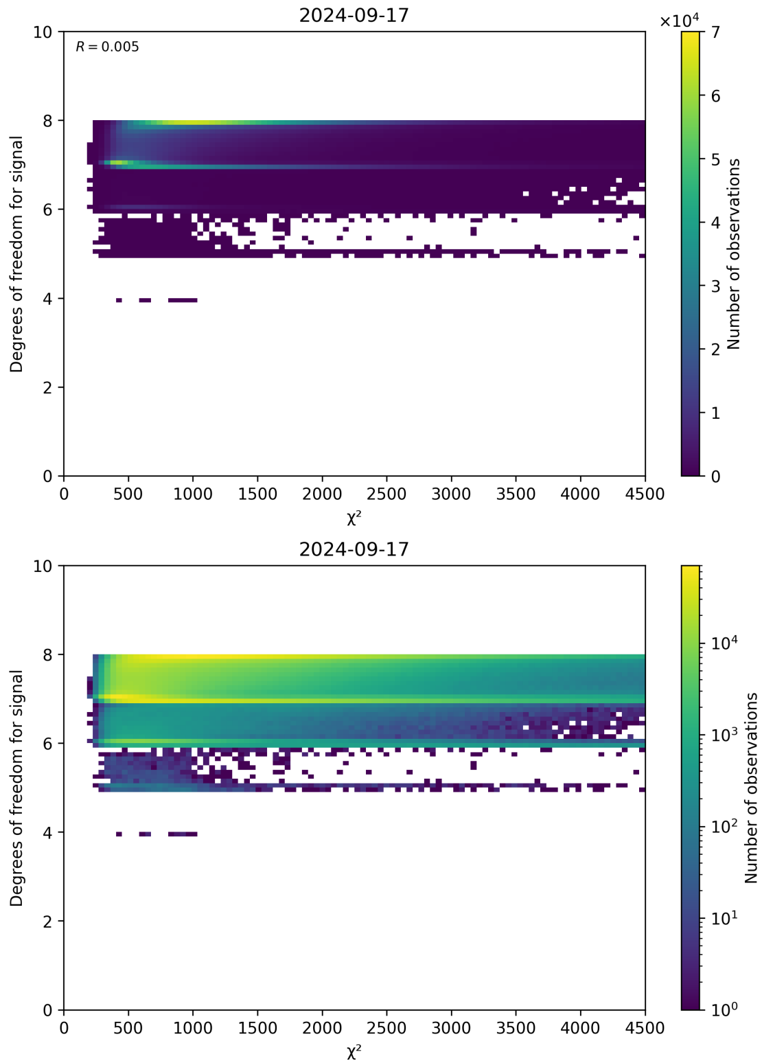
Figure 48: Scatter density plot of “ \chi^2 ” against “Degrees of freedom for signal” for 2024-09-17 to 2024-09-18.
