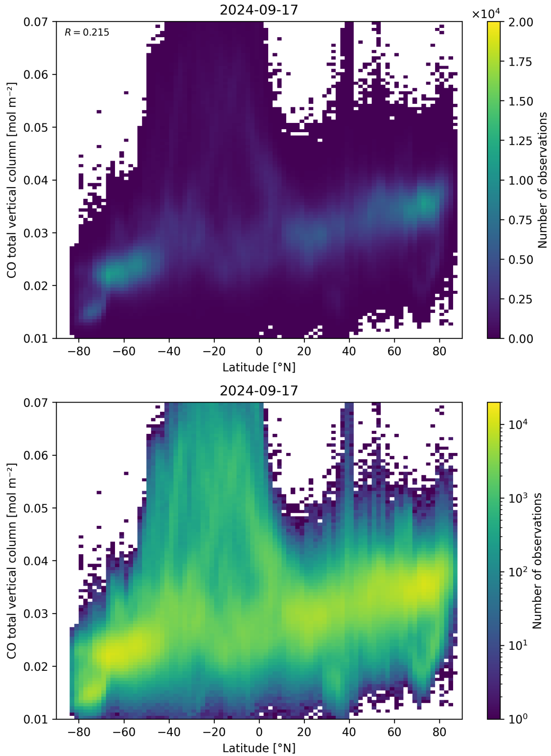
Figure 51: Scatter density plot of “Latitude” against “CO total vertical column” for 2024-09-17 to 2024-09-18.
