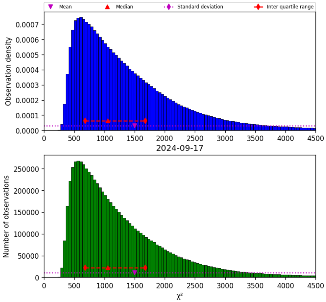
Figure 22: Histogram of “ \chi^2 ” for 2024-09-17 to 2024-09-18
