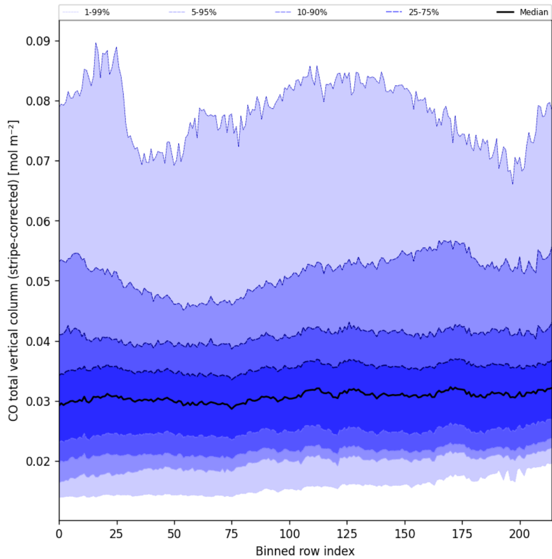
Figure 27: Along track statistics of “CO total vertical column (stripe-corrected)” for 2024-09-17 to 2024-09-18
