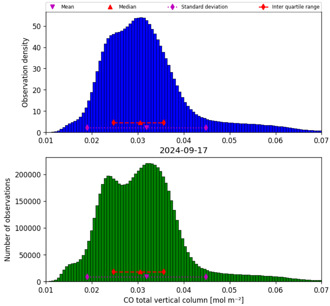
Figure 18: Histogram of “CO total vertical column” for 2024-09-17 to 2024-09-18
