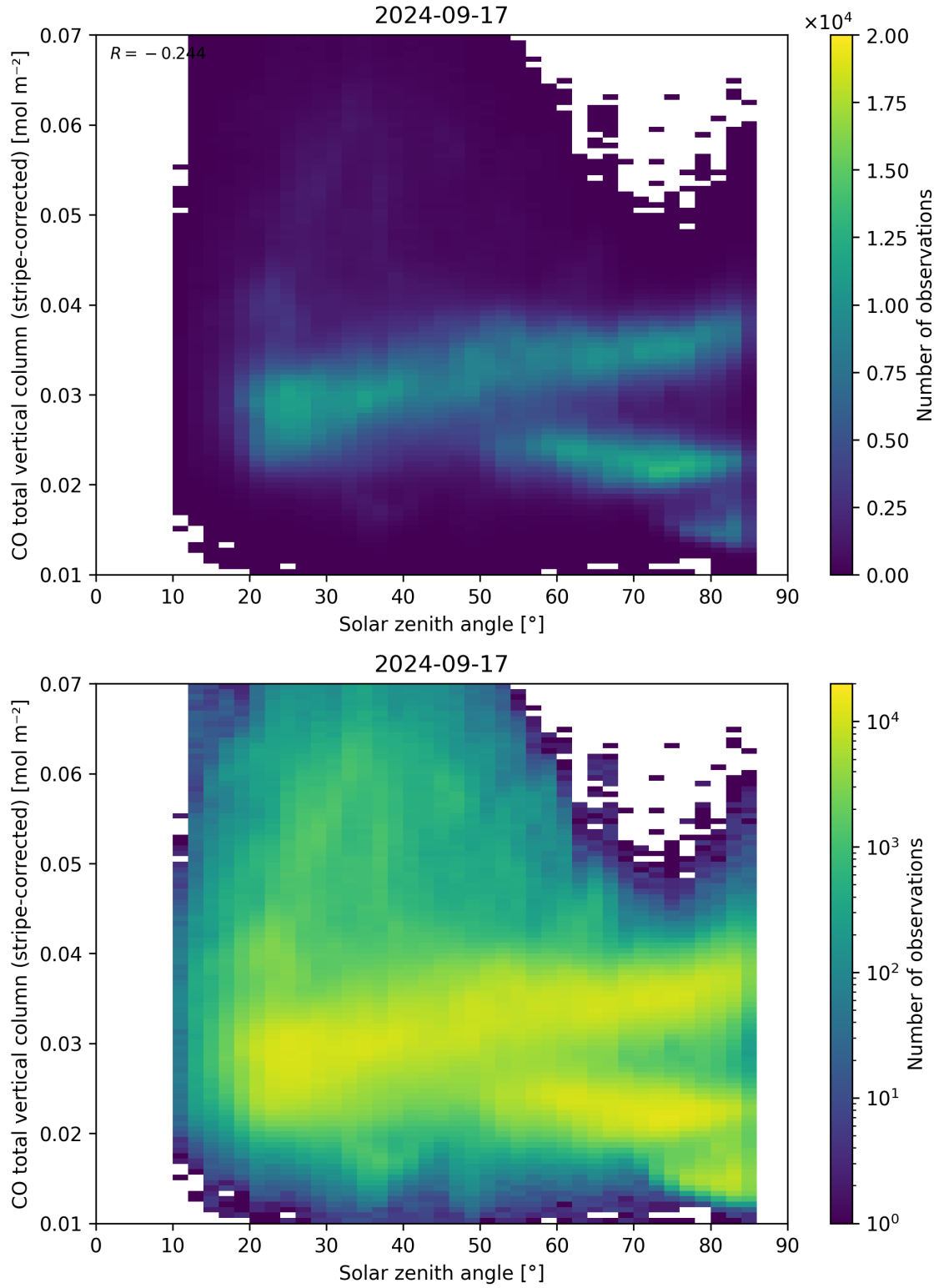
Figure 62: Scatter density plot of “Solar zenith angle” against “CO total vertical column (stripe-corrected)” for 2024-09-17 to 2024-09-18.
