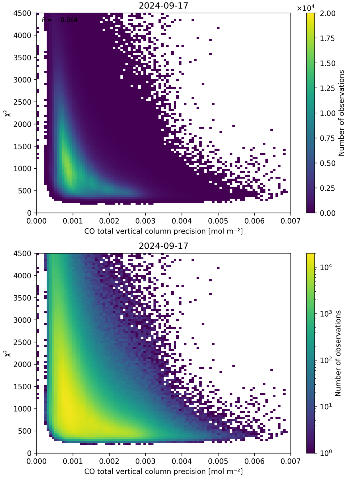
Figure 44: Scatter density plot of “CO total vertical column precision” against “ \chi^2 ” for 2024-09-17 to 2024-09-18.
