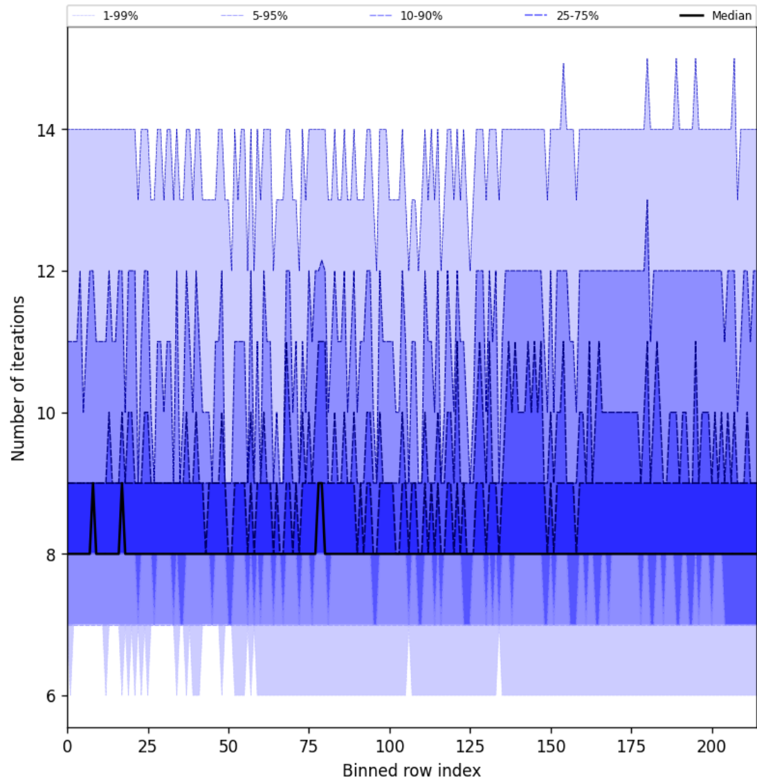
Figure 32: Along track statistics of “Number of iterations” for 2024-09-17 to 2024-09-18
