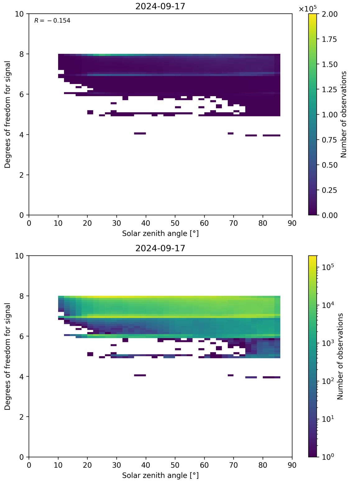
Figure 65: Scatter density plot of “Solar zenith angle” against “Degrees of freedom for signal” for 2024-09-17 to 2024-09-18.
