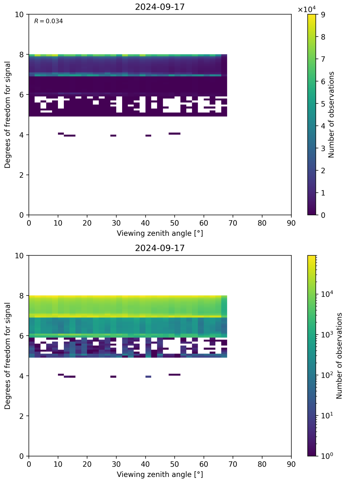
Figure 73: Scatter density plot of “Viewing zenith angle” against “Degrees of freedom for signal” for 2024-09-17 to 2024-09-18.
