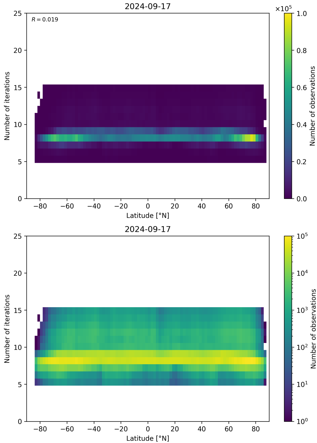
Figure 56: Scatter density plot of “Latitude” against “Number of iterations” for 2024-09-17 to 2024-09-18.
