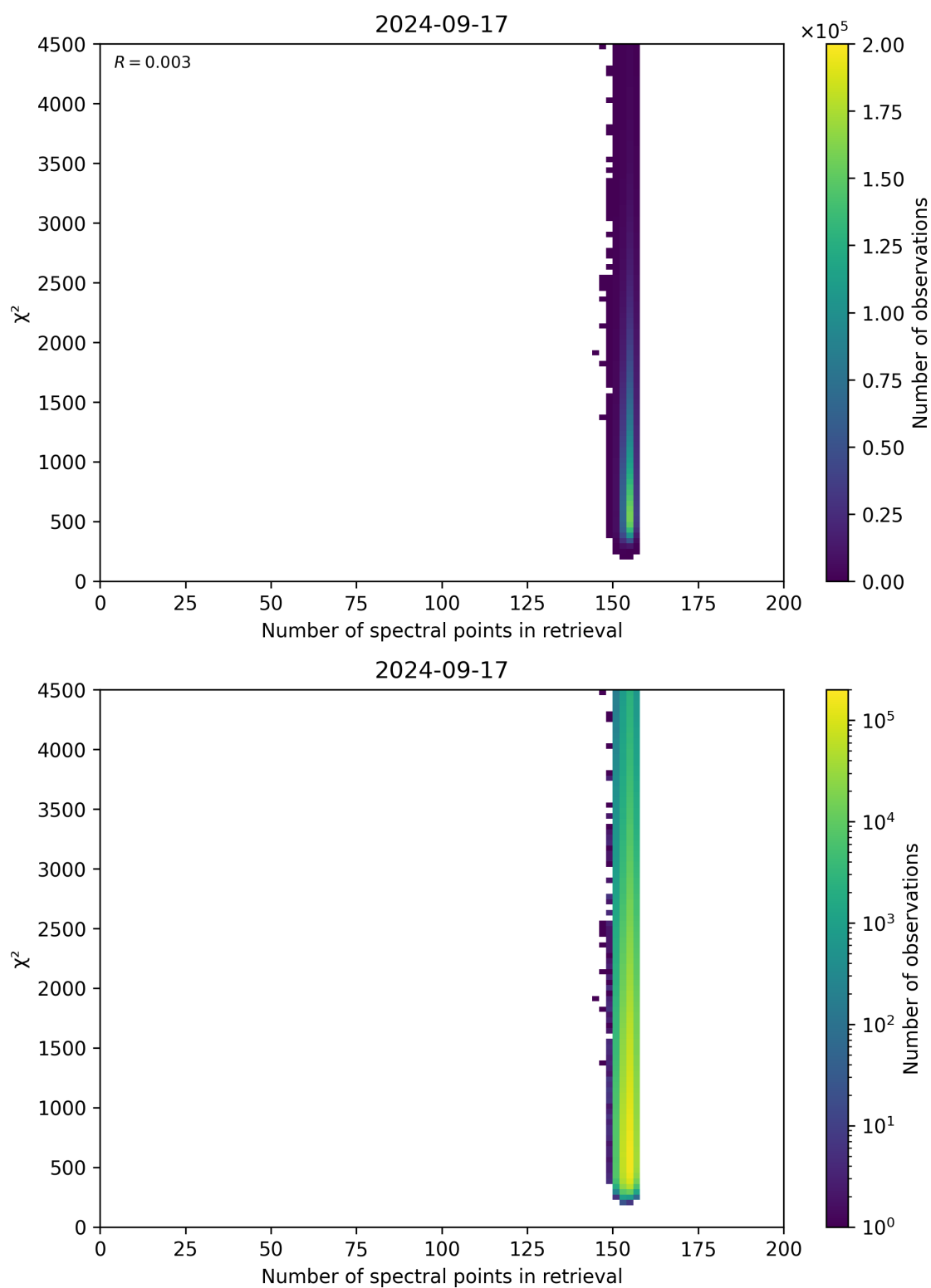
Figure 58: Scatter density plot of “Number of spectral points in retrieval” against “ \chi^2 ” for 2024-09-17 to 2024-09-18.
