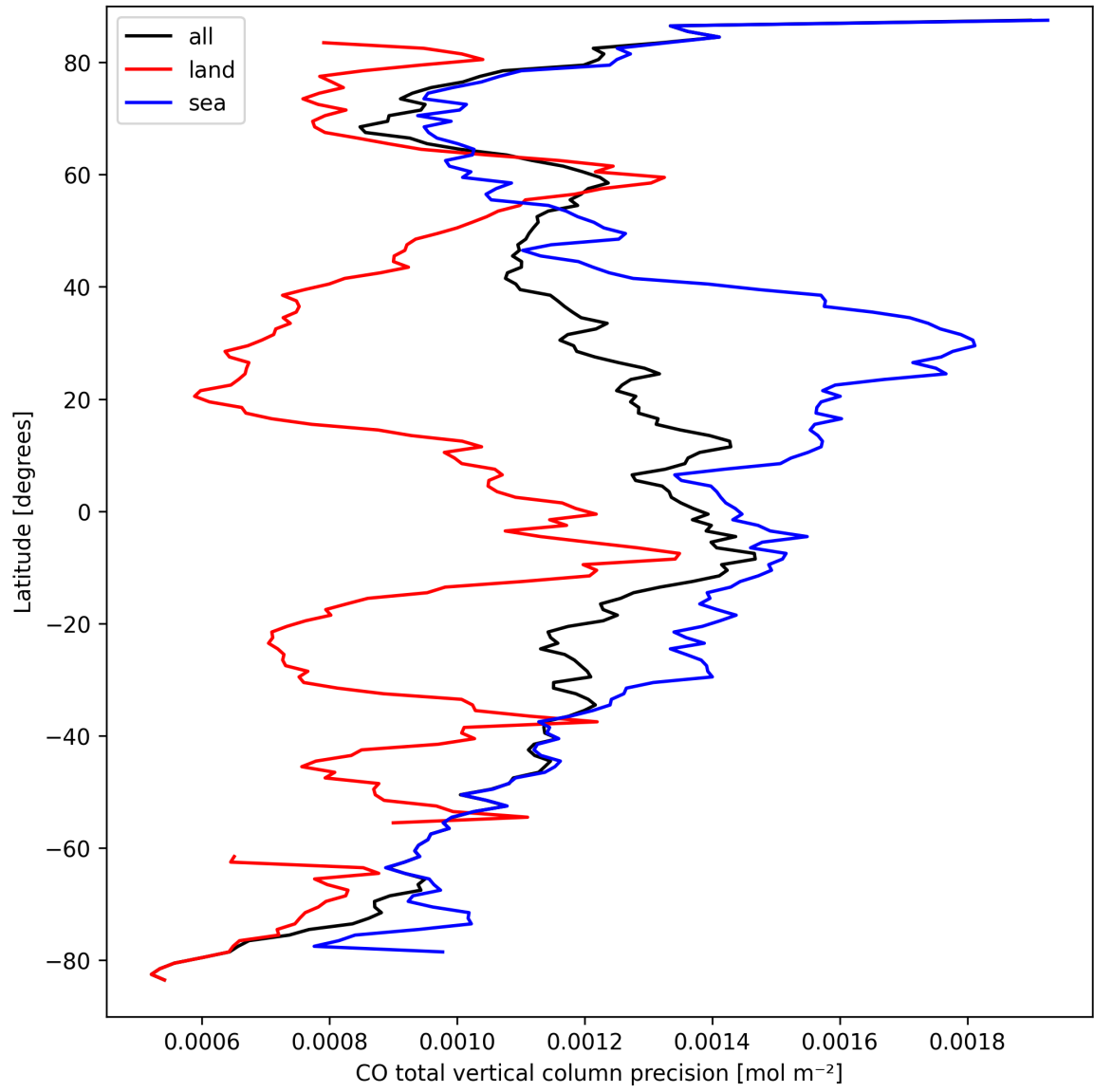
Figure 12: Zonal average of “CO total vertical column precision” for 2024-09-17 to 2024-09-18.
