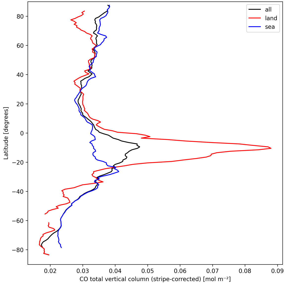
Figure 11: Zonal average of “CO total vertical column (stripe-corrected)” for 2024-09-17 to 2024-09-18.
