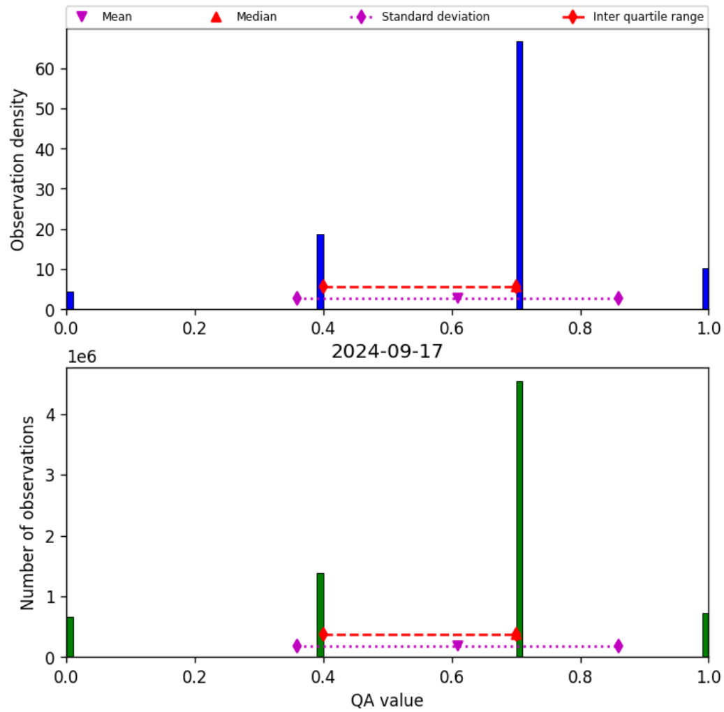
Figure 17: Histogram of “QA value” for 2024-09-17 to 2024-09-18
