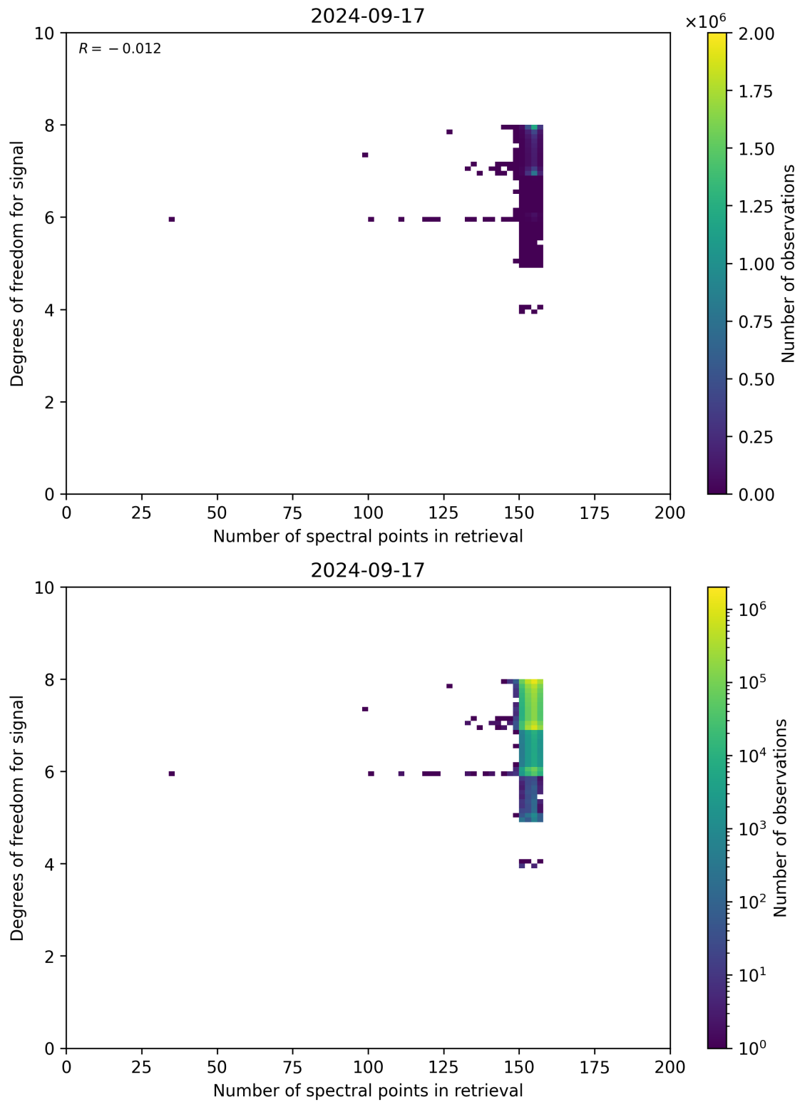
Figure 59: Scatter density plot of “Number of spectral points in retrieval” against “Degrees of freedom for signal” for 2024-09-17 to 2024-09-18.
