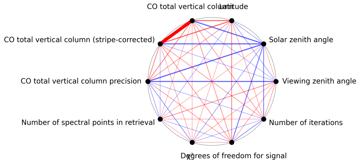
Figure 1: Map of correlation graph for 2024-09-17 to 2024-09-18.
