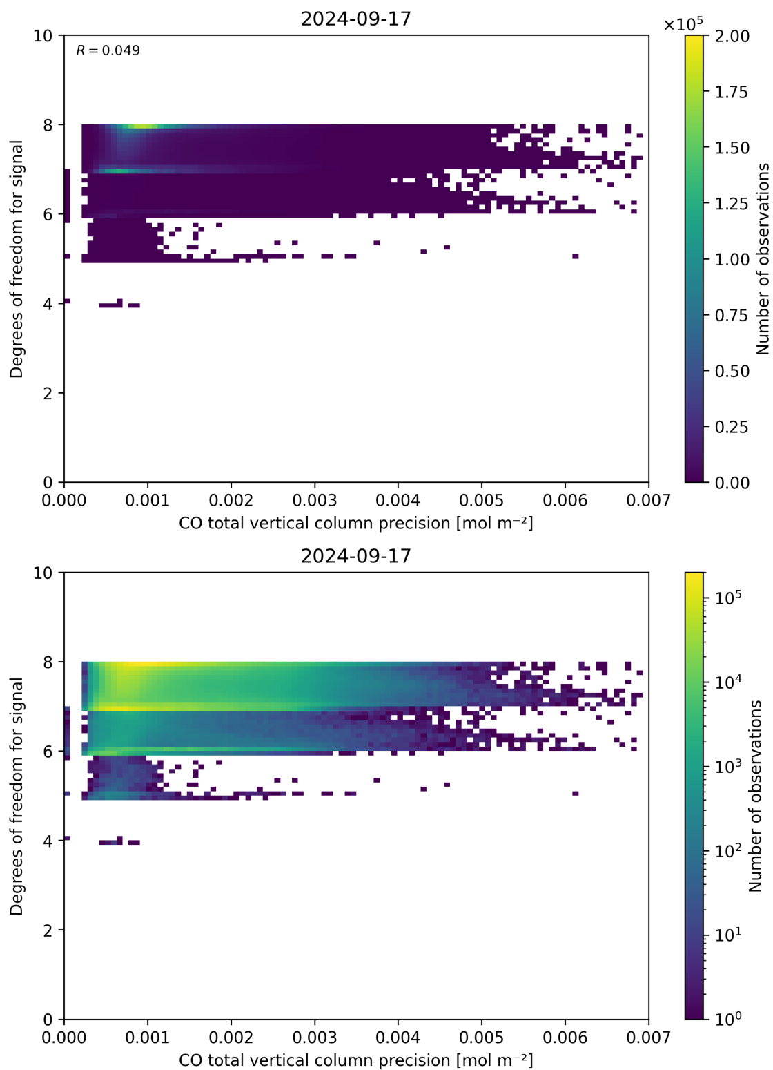
Figure 45: Scatter density plot of “CO total vertical column precision” against “Degrees of freedom for signal” for 2024-09-17 to 2024-09-18.
