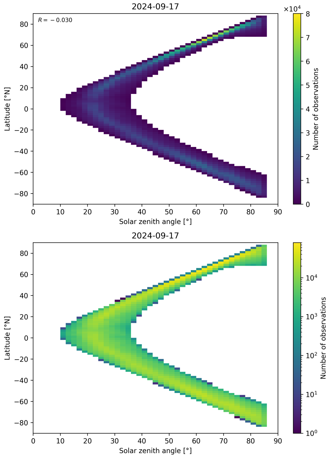
Figure 66: Scatter density plot of “Solar zenith angle” against “Latitude” for 2024-09-17 to 2024-09-18.
