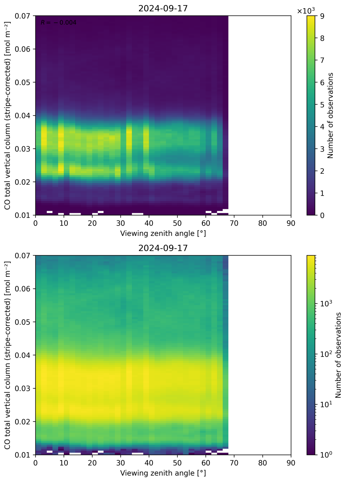
Figure 70: Scatter density plot of “Viewing zenith angle” against “CO total vertical column (stripe-corrected)” for 2024-09-17 to 2024-09-18.
