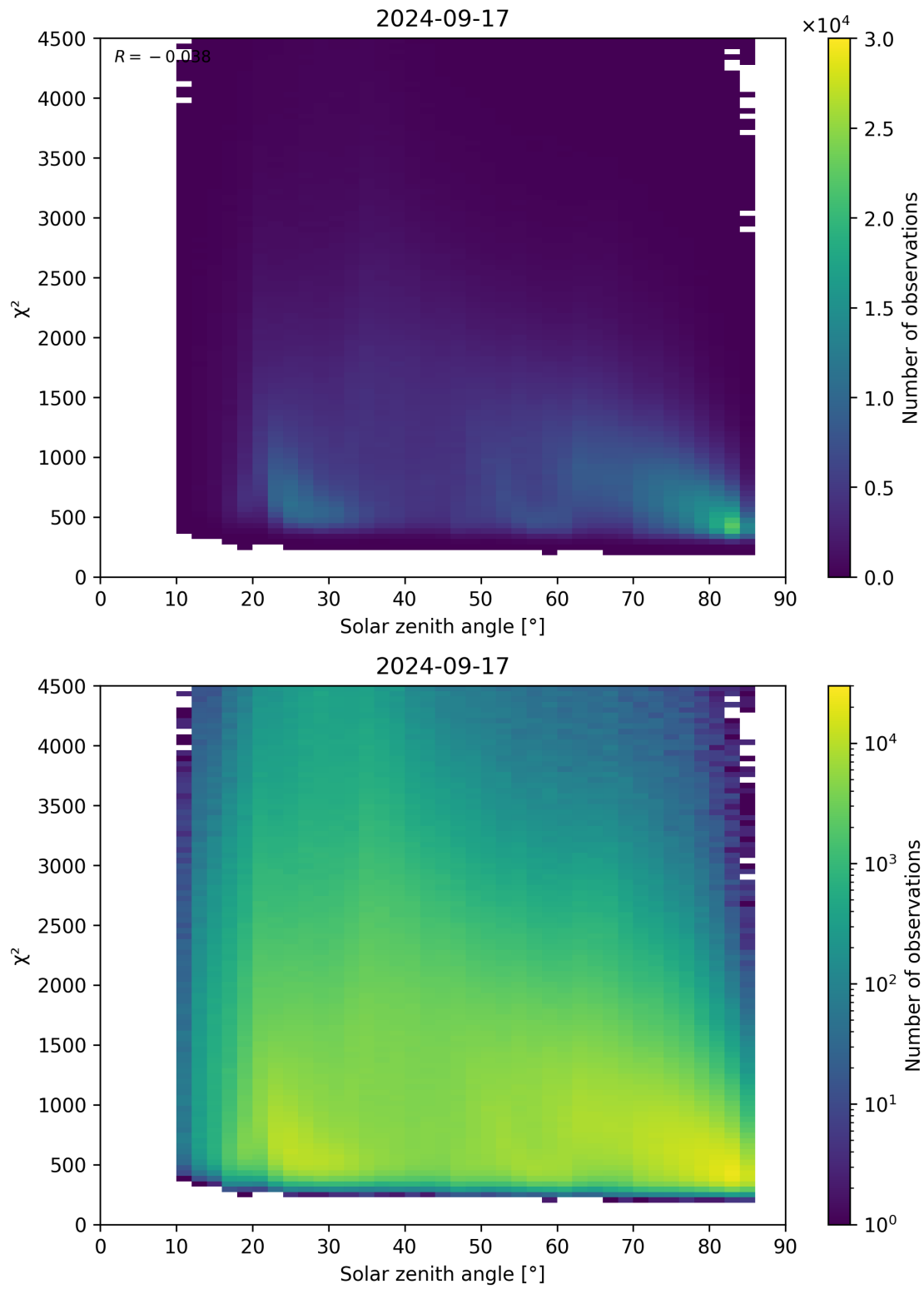
Figure 64: Scatter density plot of “Solar zenith angle” against “ \chi^2 ” for 2024-09-17 to 2024-09-18.
