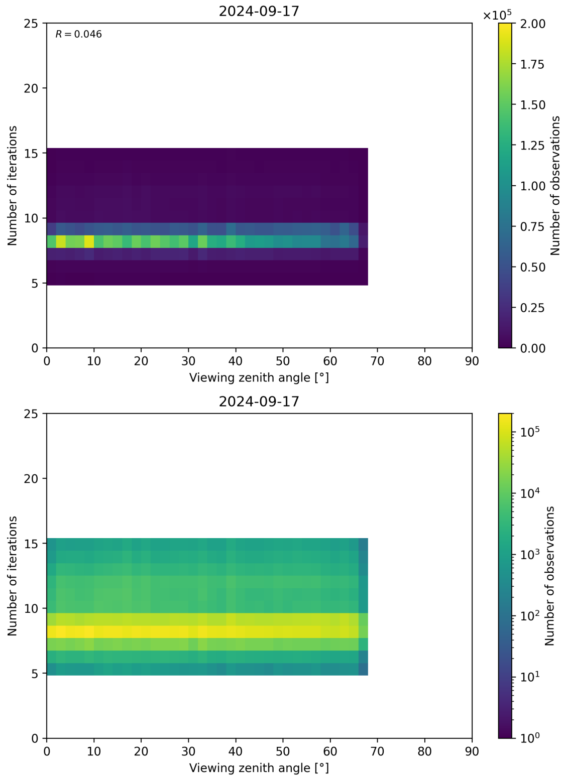
Figure 75: Scatter density plot of “Viewing zenith angle” against “Number of iterations” for 2024-09-17 to 2024-09-18.
