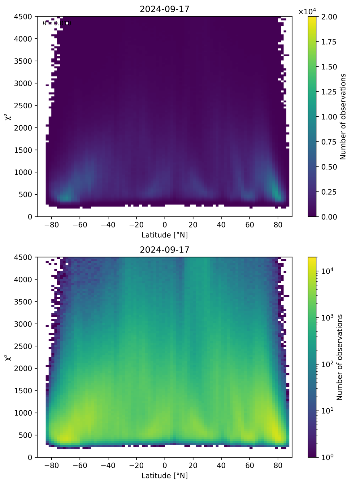
Figure 54: Scatter density plot of “Latitude” against “ \chi^2 ” for 2024-09-17 to 2024-09-18.
