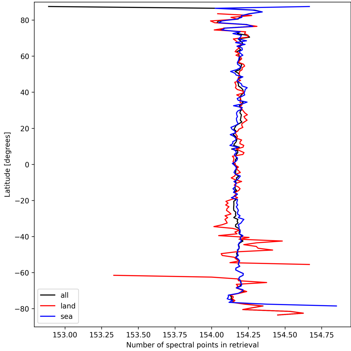
Figure 13: Zonal average of “Number of spectral points in retrieval” for 2024-09-17 to 2024-09-18.
