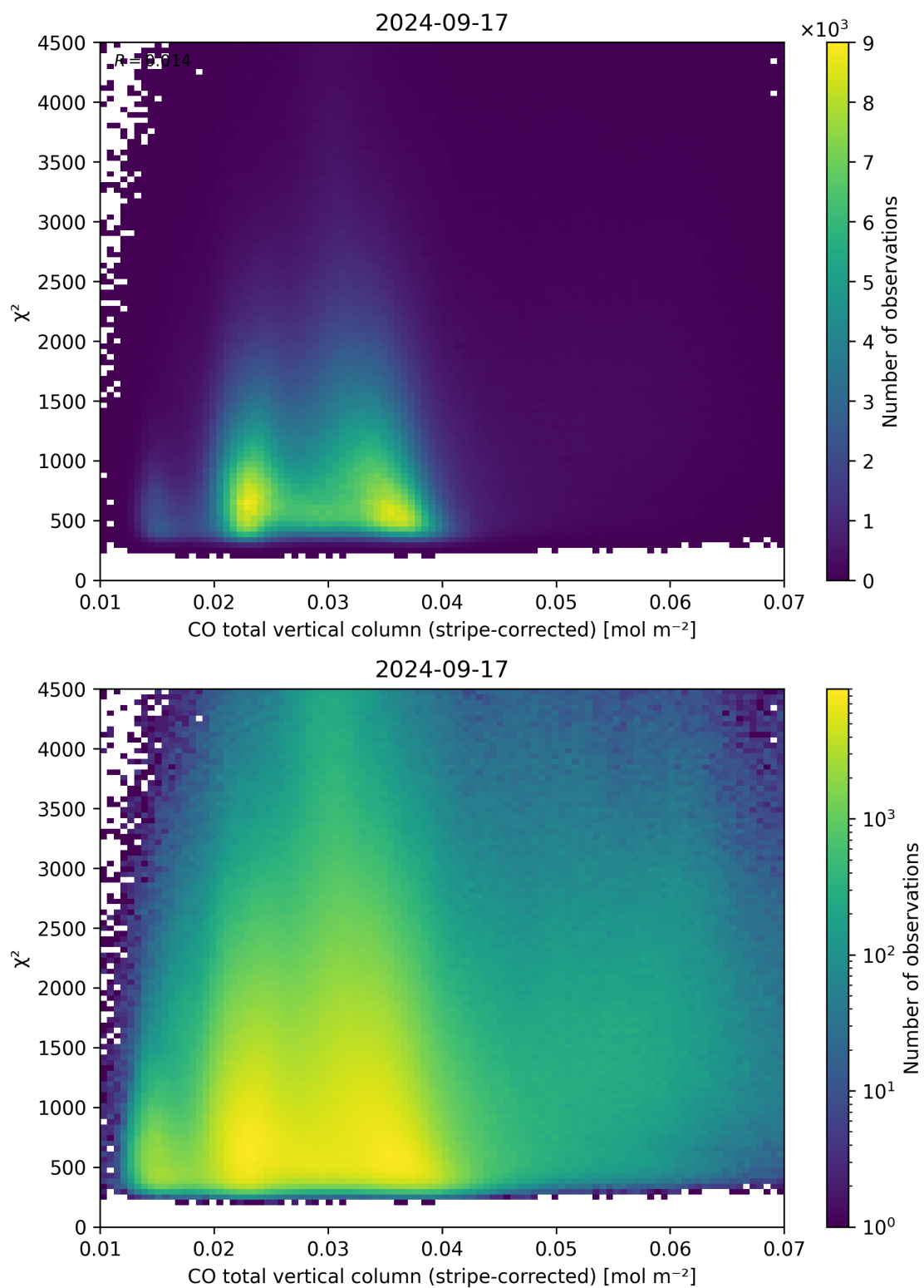
Figure 37: Scatter density plot of “CO total vertical column (stripe-corrected)” against “ \chi^2 ” for 2024-09-17 to 2024-09-18.
