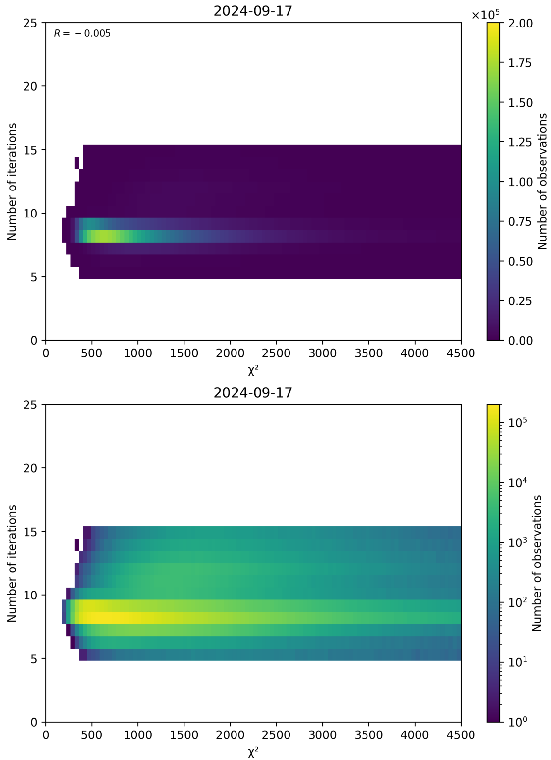
Figure 49: Scatter density plot of “ \chi^2 ” against “Number of iterations” for 2024-09-17 to 2024-09-18.
