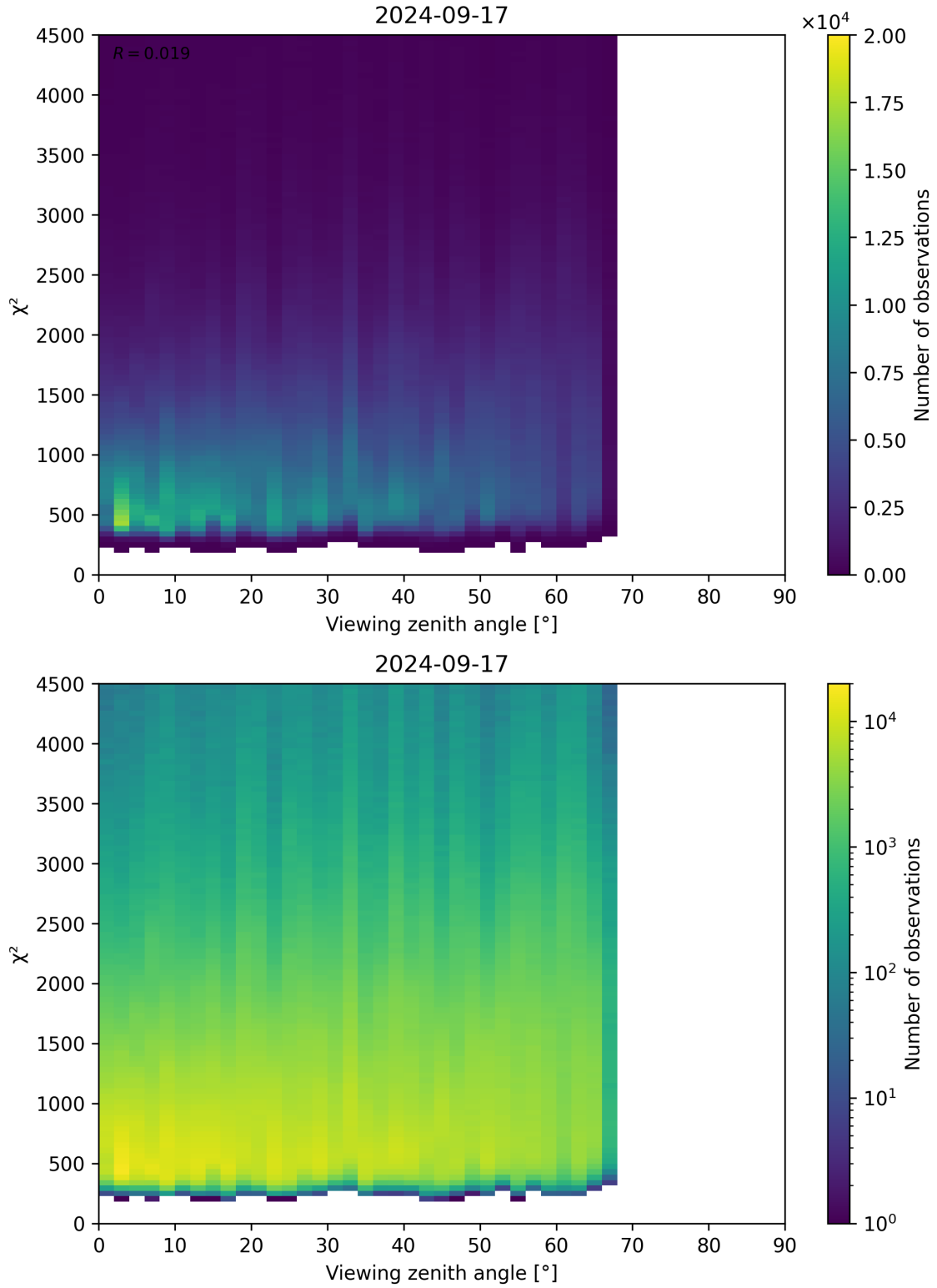
Figure 72: Scatter density plot of “Viewing zenith angle” against “ \chi^2 ” for 2024-09-17 to 2024-09-18.
