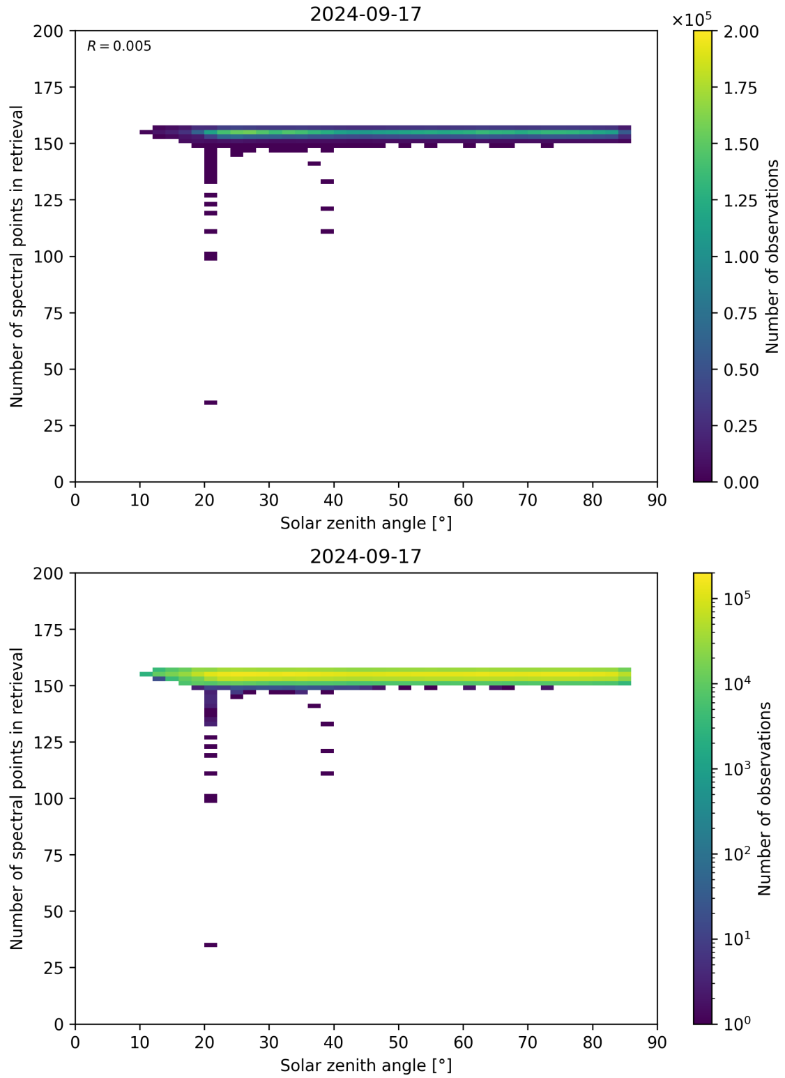
Figure 68: Scatter density plot of “Solar zenith angle” against “Number of spectral points in retrieval” for 2024-09-17 to 2024-09-18.
