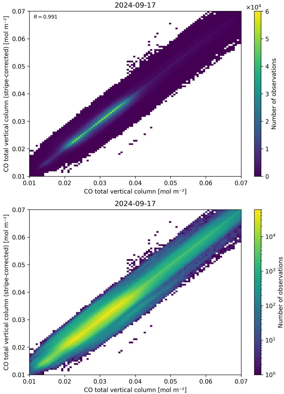
Figure 33: Scatter density plot of “CO total vertical column” against “CO total vertical column (stripe-corrected)” for 2024-09-17 to 2024-09-18.
