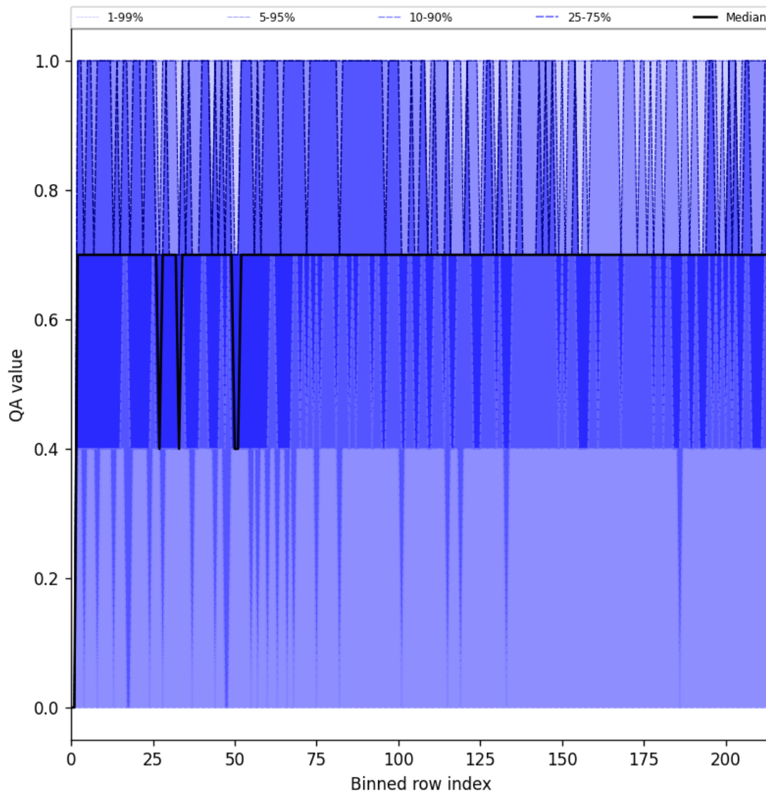
Figure 25: Along track statistics of “QA value” for 2024-09-17 to 2024-09-18
