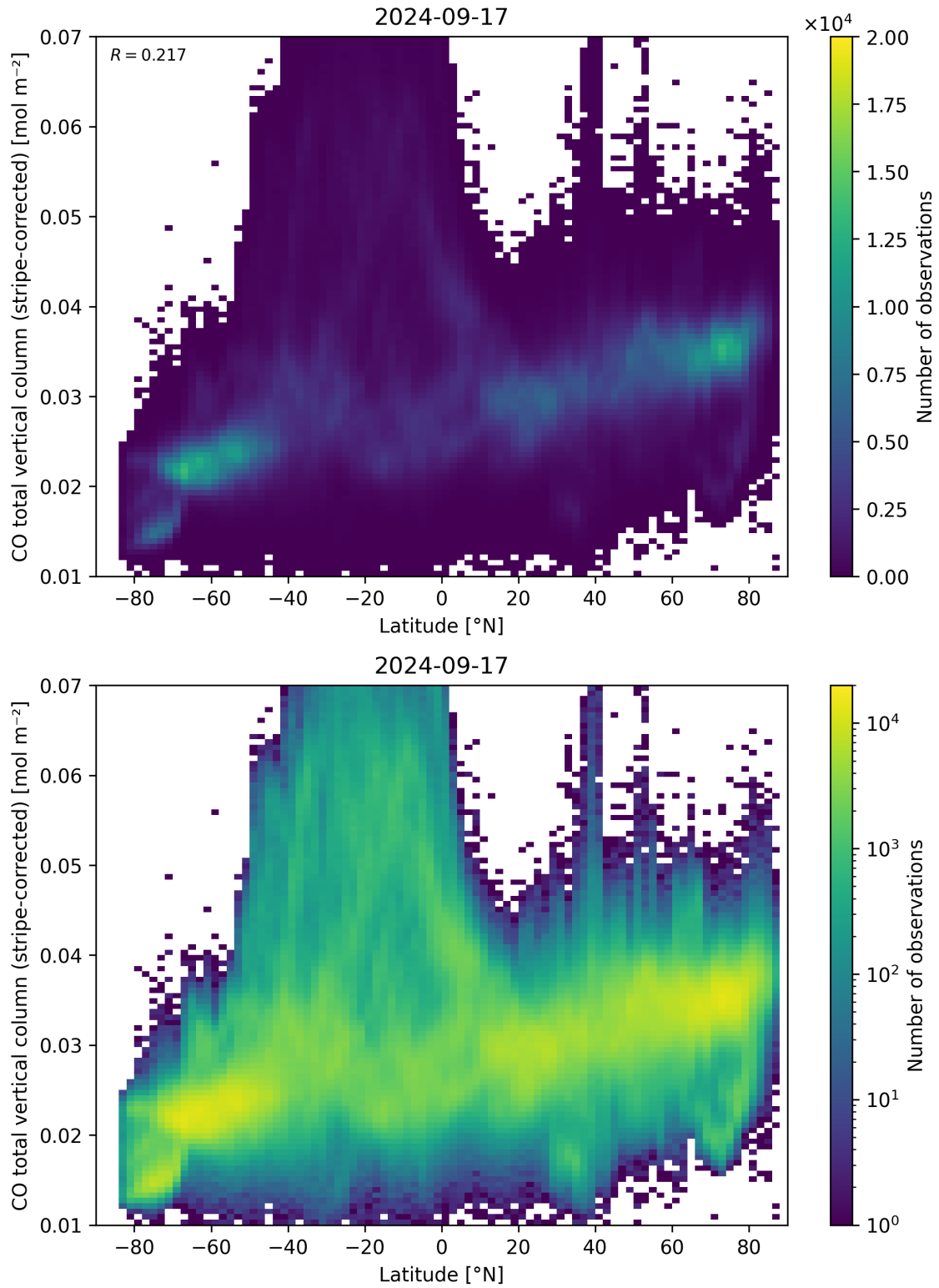
Figure 52: Scatter density plot of “Latitude” against “CO total vertical column (stripe-corrected)” for 2024-09-17 to 2024-09-18.
