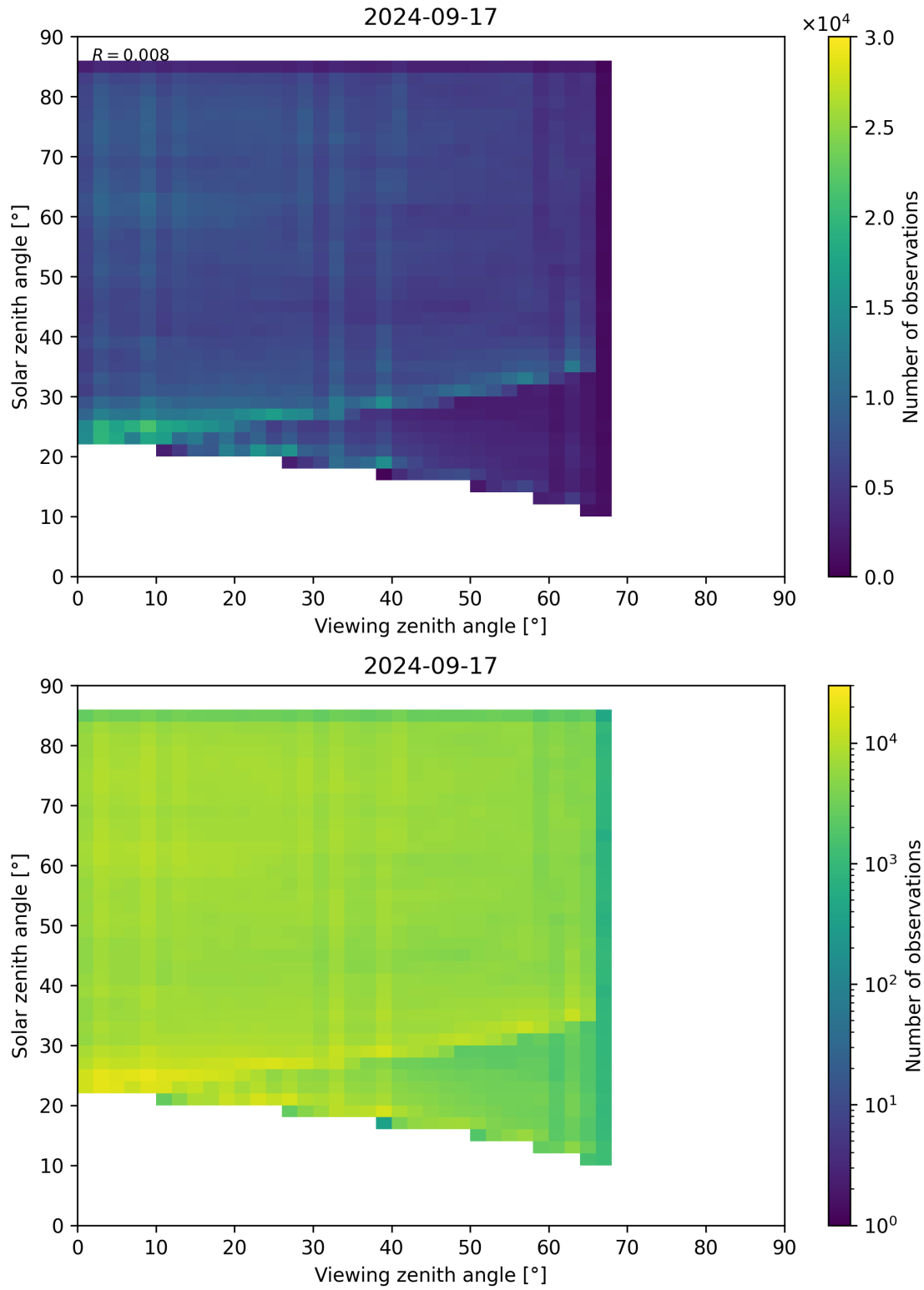
Figure 77: Scatter density plot of “Viewing zenith angle” against “Solar zenith angle” for 2024-09-17 to 2024-09-18.
