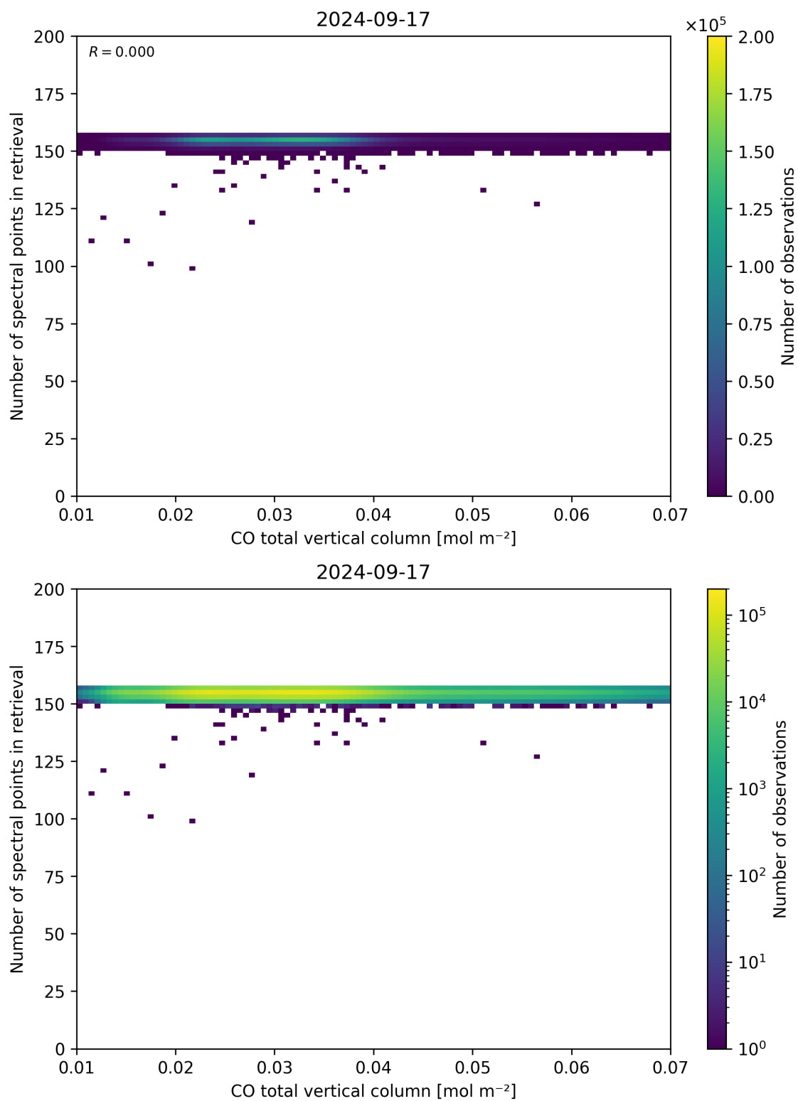
Figure 43: Scatter density plot of “CO total vertical column” against “Number of spectral points in retrieval” for 2024-09-17 to 2024-09-18.
