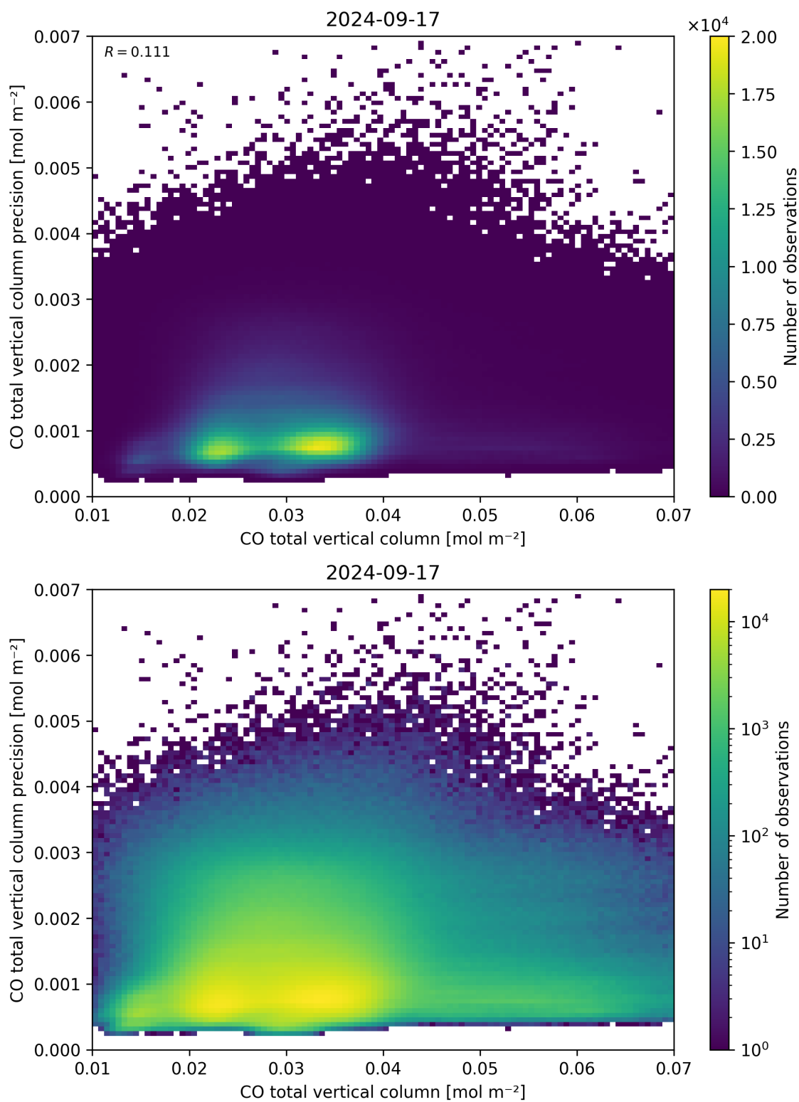
Figure 34: Scatter density plot of “CO total vertical column” against “CO total vertical column precision” for 2024-09-17 to 2024-09-18.
