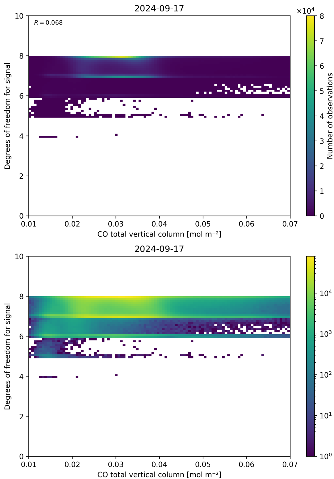
Figure 41: Scatter density plot of “CO total vertical column” against “Degrees of freedom for signal” for 2024-09-17 to 2024-09-18.
