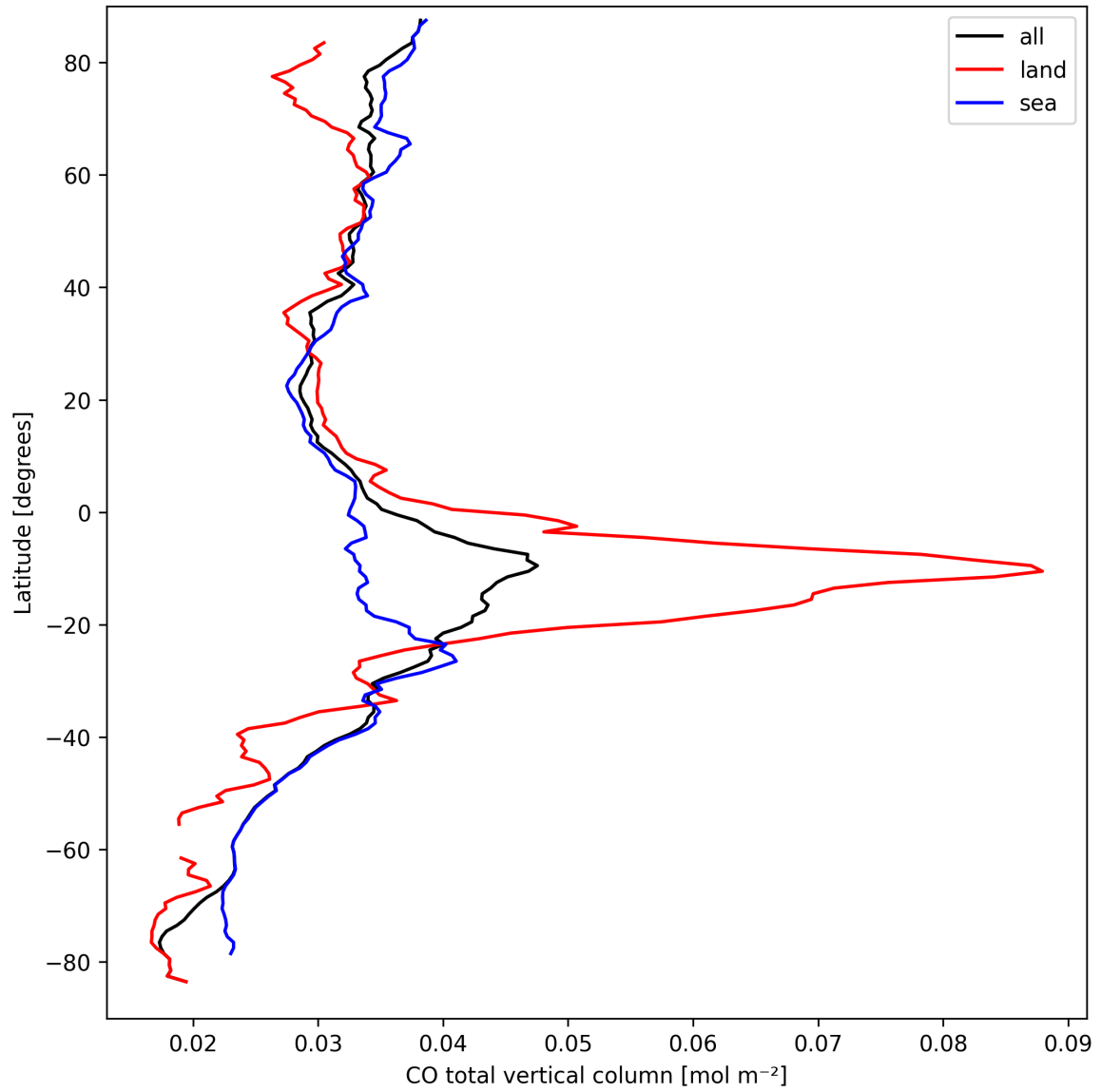
Figure 10: Zonal average of “CO total vertical column” for 2024-09-17 to 2024-09-18.
