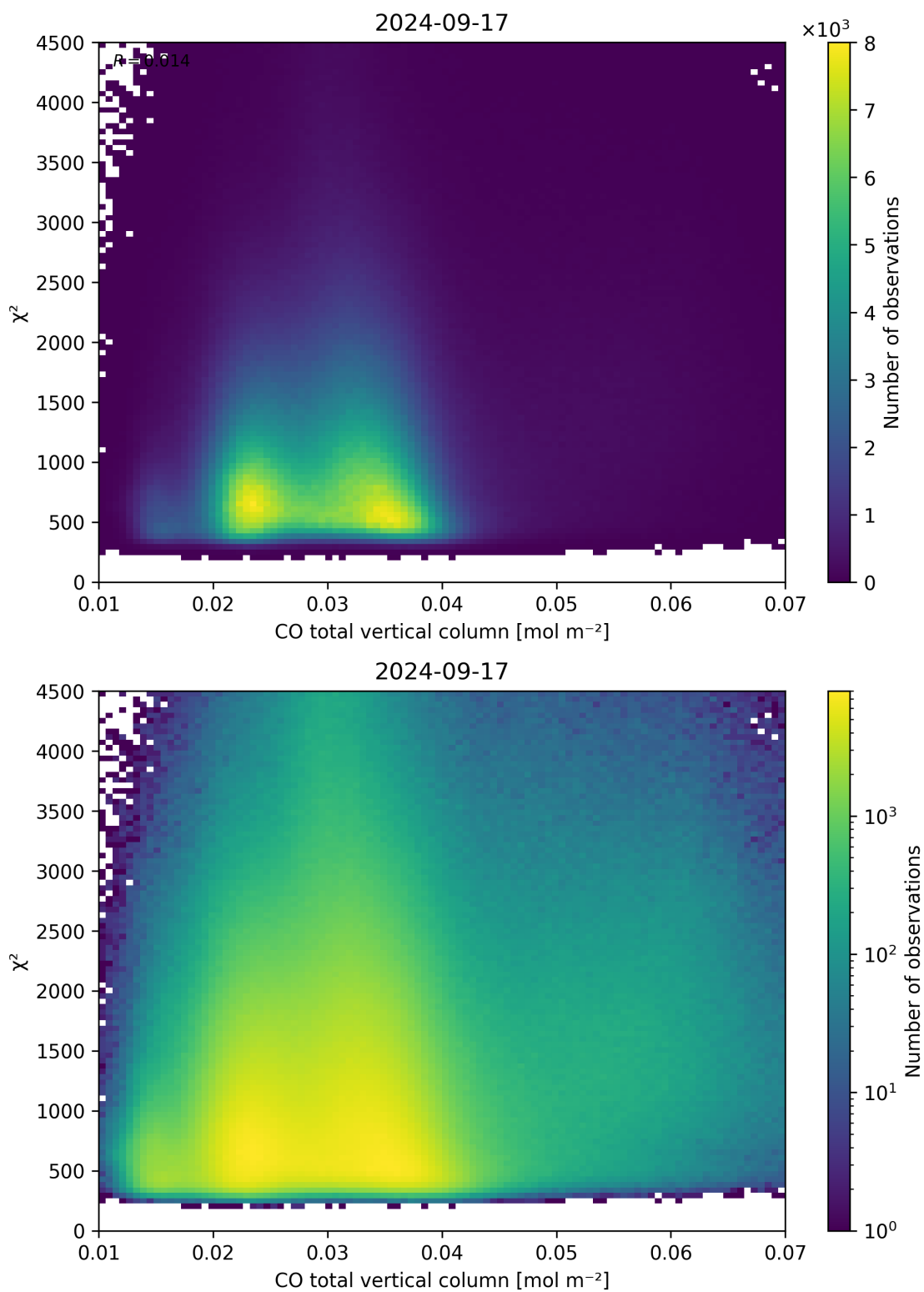
Figure 35: Scatter density plot of “CO total vertical column” against “ \chi^2 ” for 2024-09-17 to 2024-09-18.
