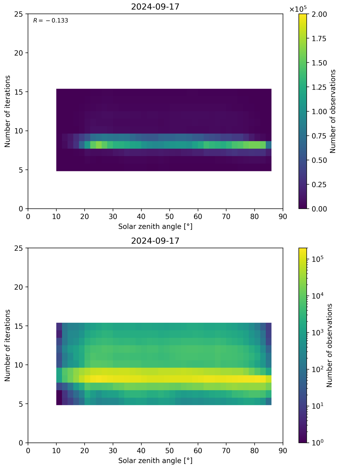
Figure 67: Scatter density plot of “Solar zenith angle” against “Number of iterations” for 2024-09-17 to 2024-09-18.
