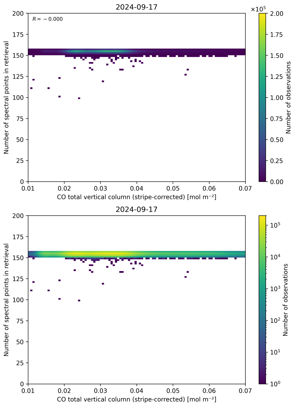
Figure 40: Scatter density plot of “CO total vertical column (stripe-corrected)” against “Number of spectral points in retrieval” for 2024-09-17 to 2024-09-18.
