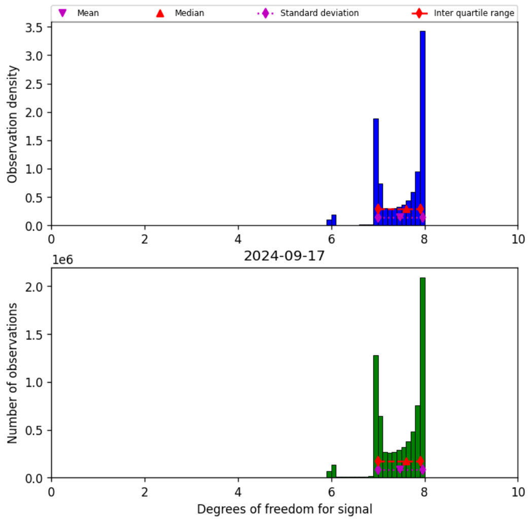
Figure 23: Histogram of “Degrees of freedom for signal” for 2024-09-17 to 2024-09-18
