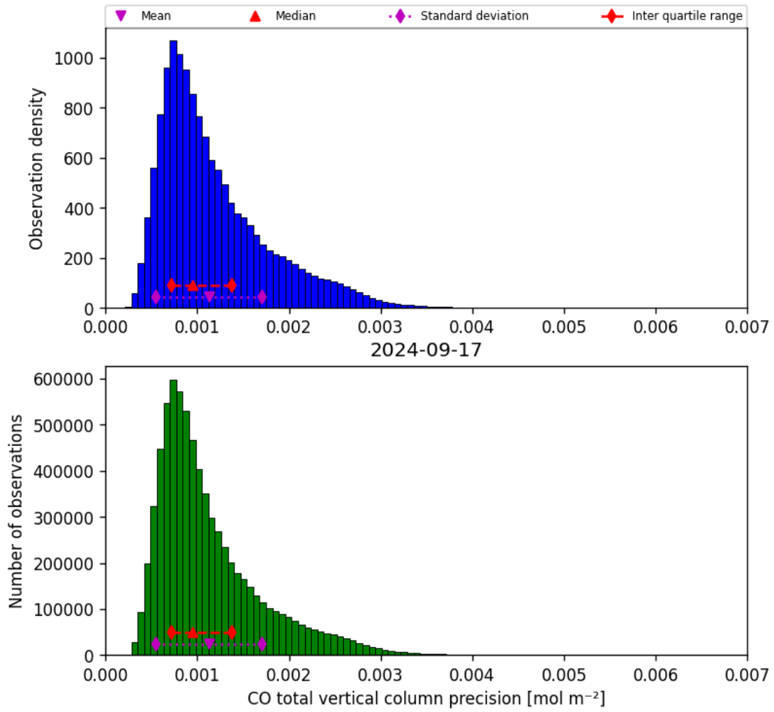
Figure 20: Histogram of “CO total vertical column precision” for 2024-09-17 to 2024-09-18
