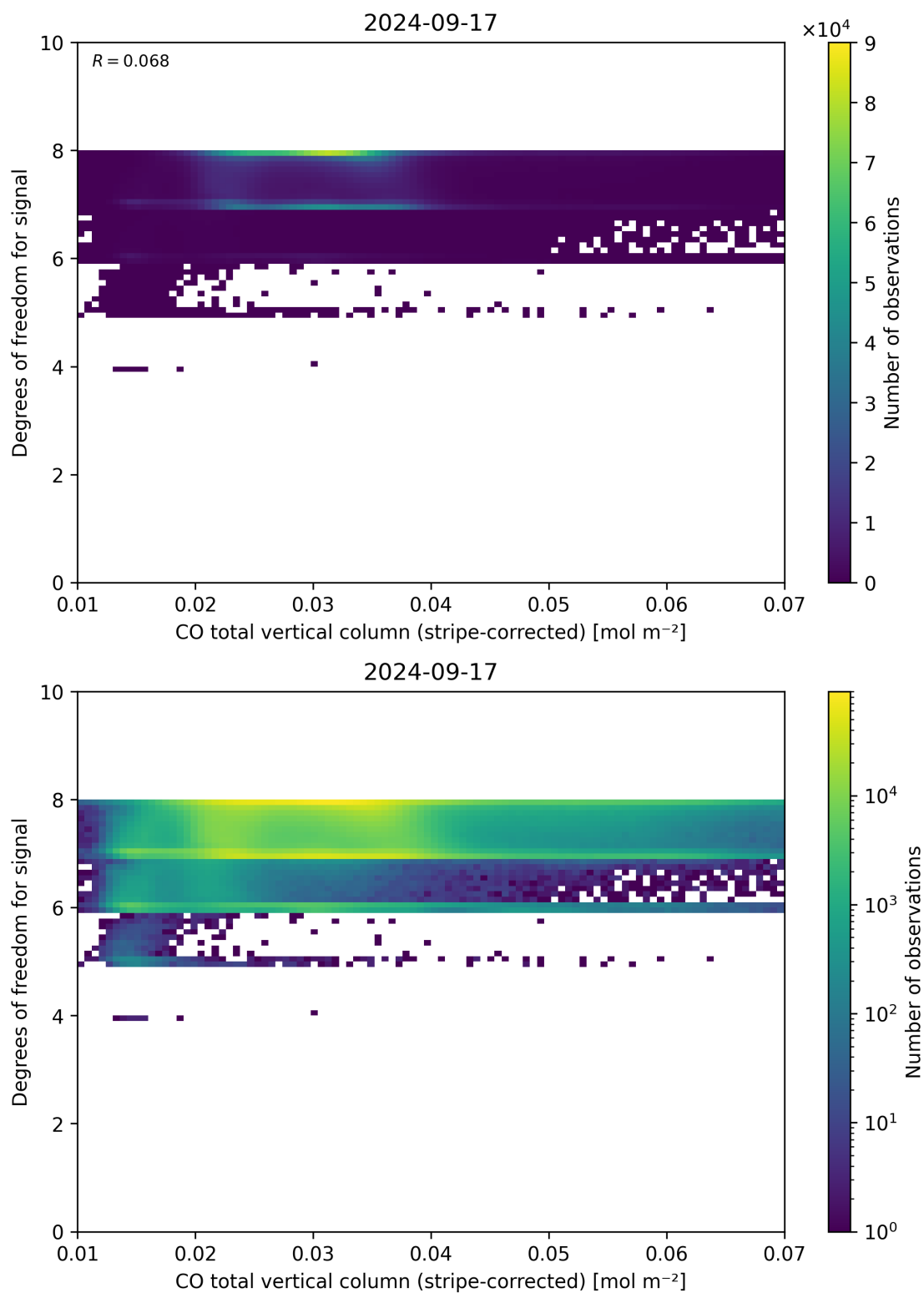
Figure 38: Scatter density plot of “CO total vertical column (stripe-corrected)” against “Degrees of freedom for signal” for 2024-09-17 to 2024-09-18.
