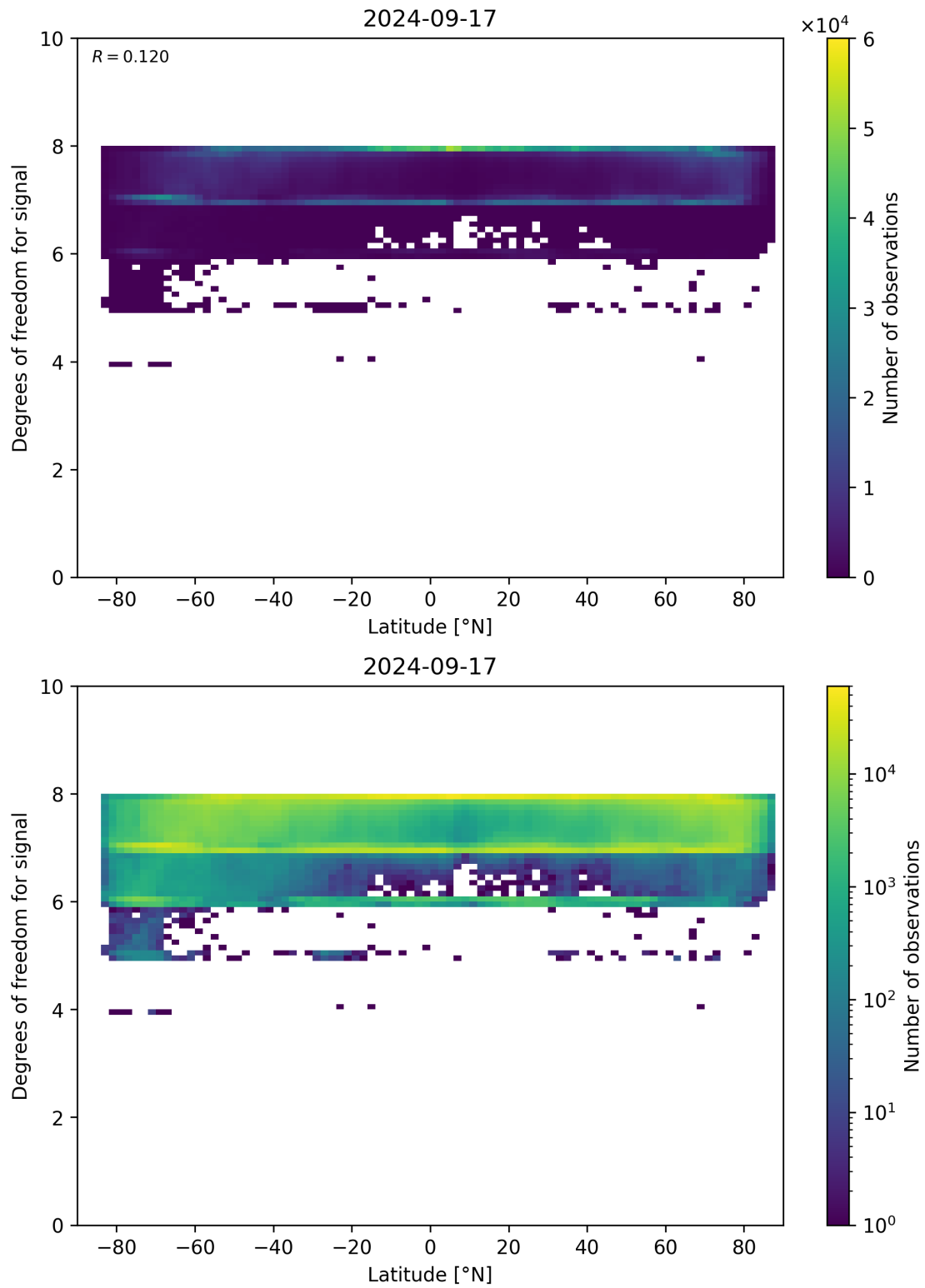
Figure 55: Scatter density plot of “Latitude” against “Degrees of freedom for signal” for 2024-09-17 to 2024-09-18.
