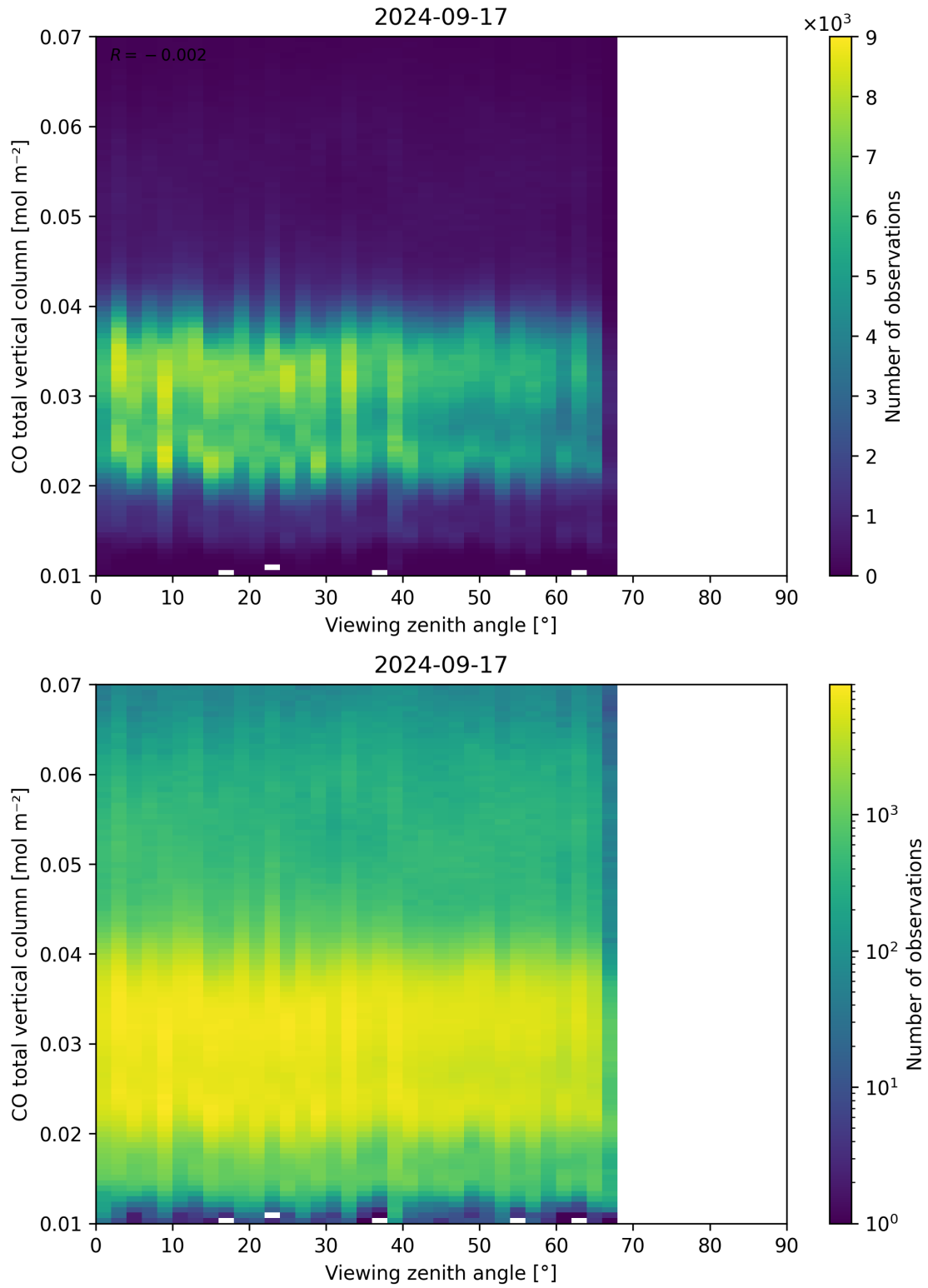
Figure 69: Scatter density plot of “Viewing zenith angle” against “CO total vertical column” for 2024-09-17 to 2024-09-18.
