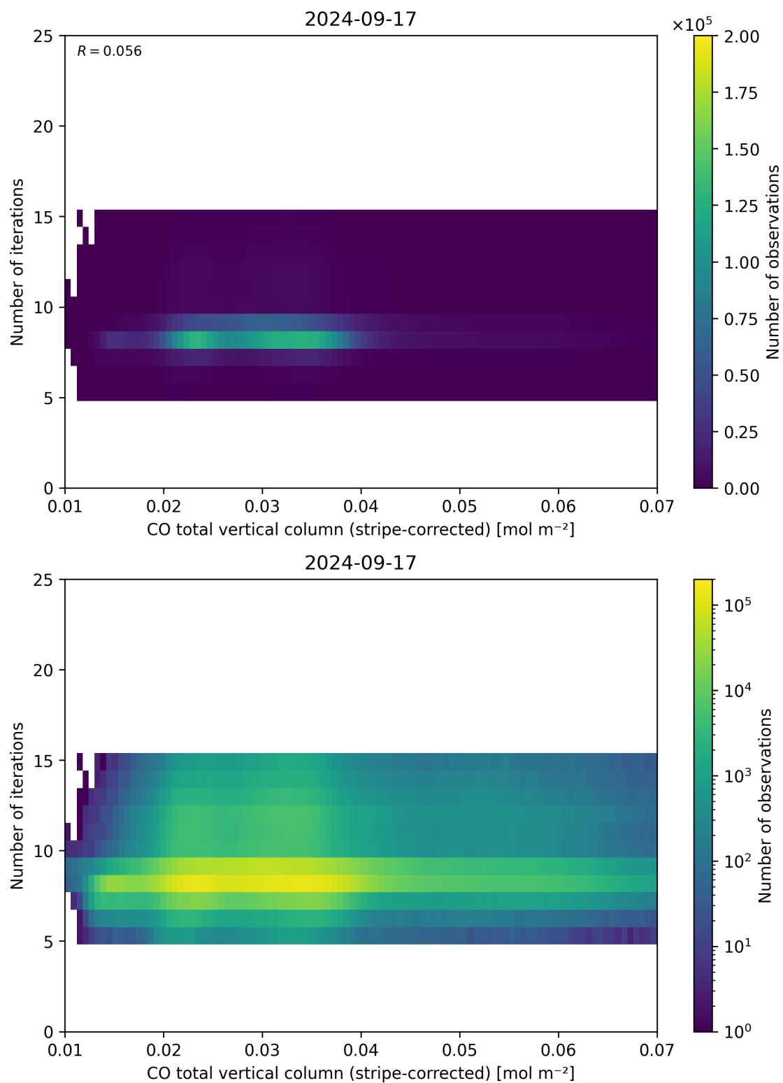
Figure 39: Scatter density plot of “CO total vertical column (stripe-corrected)” against “Number of iterations” for 2024-09-17 to 2024-09-18.
