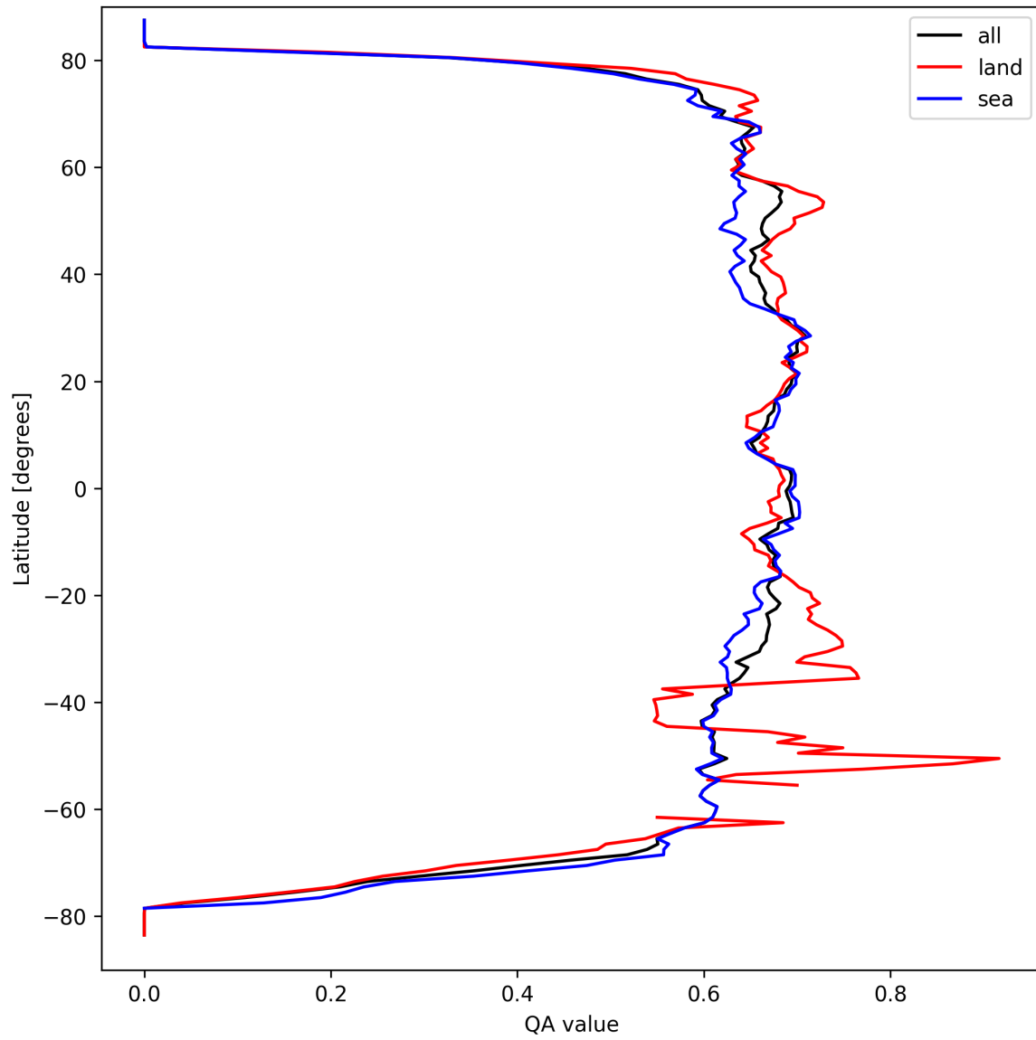
Figure 9: Zonal average of “QA value” for 2024-09-17 to 2024-09-18.
