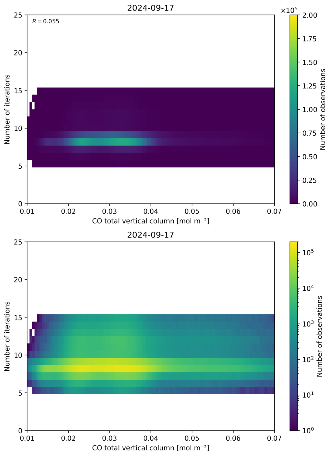
Figure 42: Scatter density plot of “CO total vertical column” against “Number of iterations” for 2024-09-17 to 2024-09-18.
