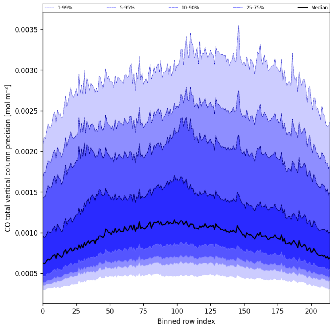
Figure 28: Along track statistics of “CO total vertical column precision” for 2024-09-17 to 2024-09-18
