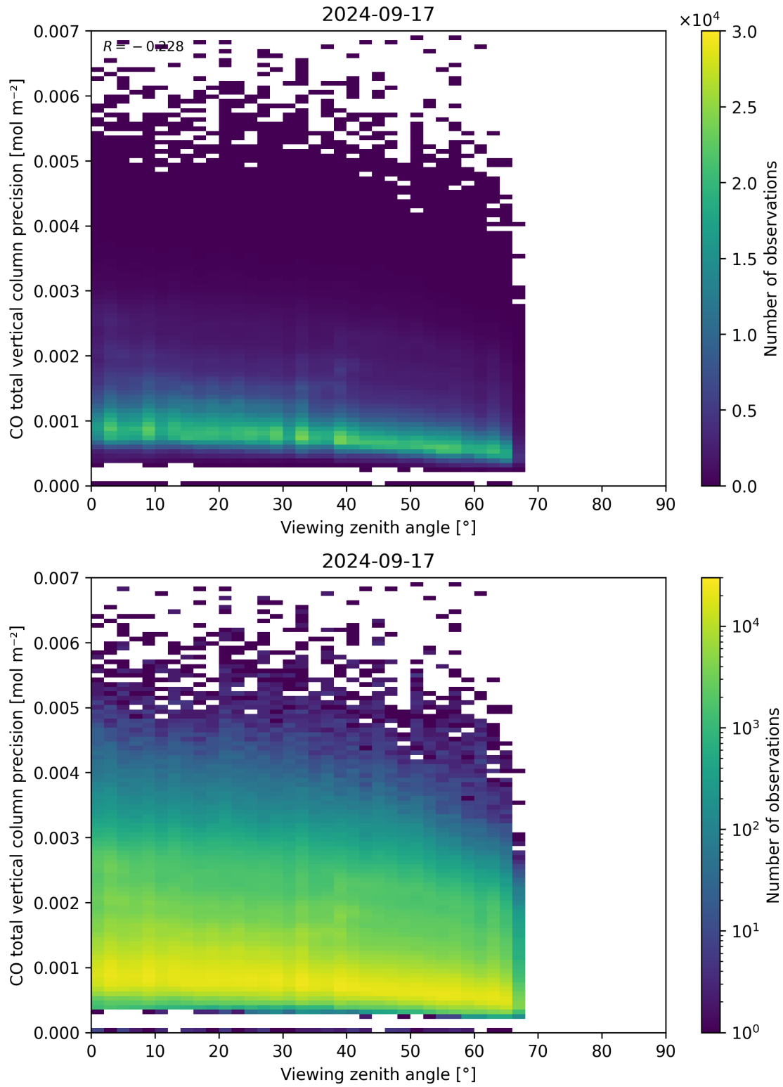
Figure 71: Scatter density plot of “Viewing zenith angle” against “CO total vertical column precision” for 2024-09-17 to 2024-09-18.
