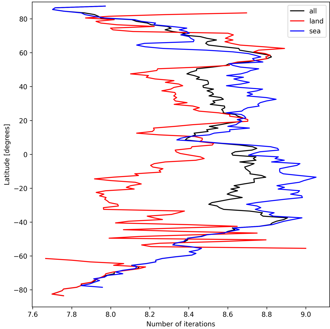
Figure 16: Zonal average of “Number of iterations” for 2024-09-17 to 2024-09-18.
