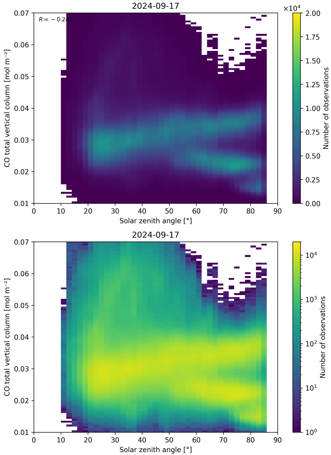
Figure 61: Scatter density plot of “Solar zenith angle” against “CO total vertical column” for 2024-09-17 to 2024-09-18.
