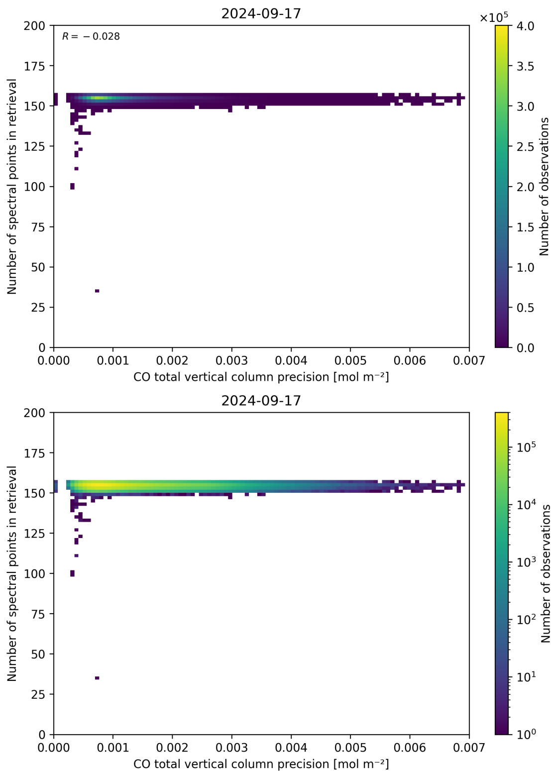
Figure 47: Scatter density plot of “CO total vertical column precision” against “Number of spectral points in retrieval” for 2024-09-17 to 2024-09-18.
