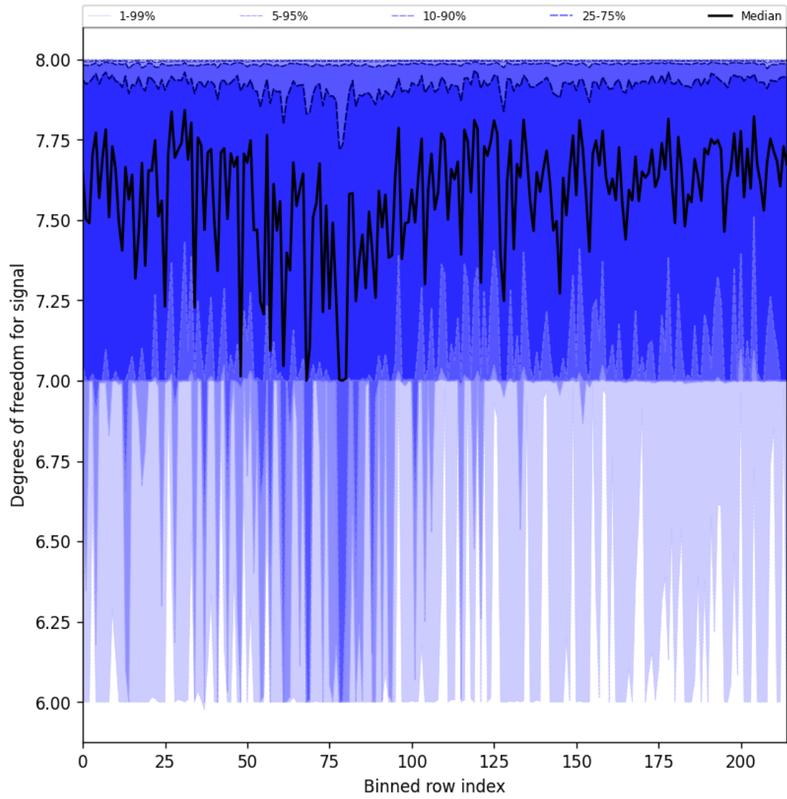
Figure 31: Along track statistics of “Degrees of freedom for signal” for 2024-09-17 to 2024-09-18
