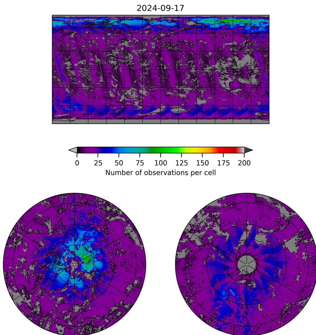
Figure 8: Map of the number of observations for 2024-09-17 to 2024-09-18
