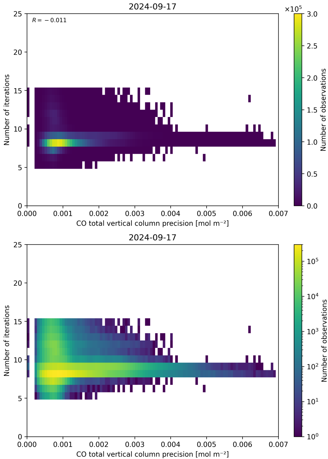
Figure 46: Scatter density plot of “CO total vertical column precision” against “Number of iterations” for 2024-09-17 to 2024-09-18.
