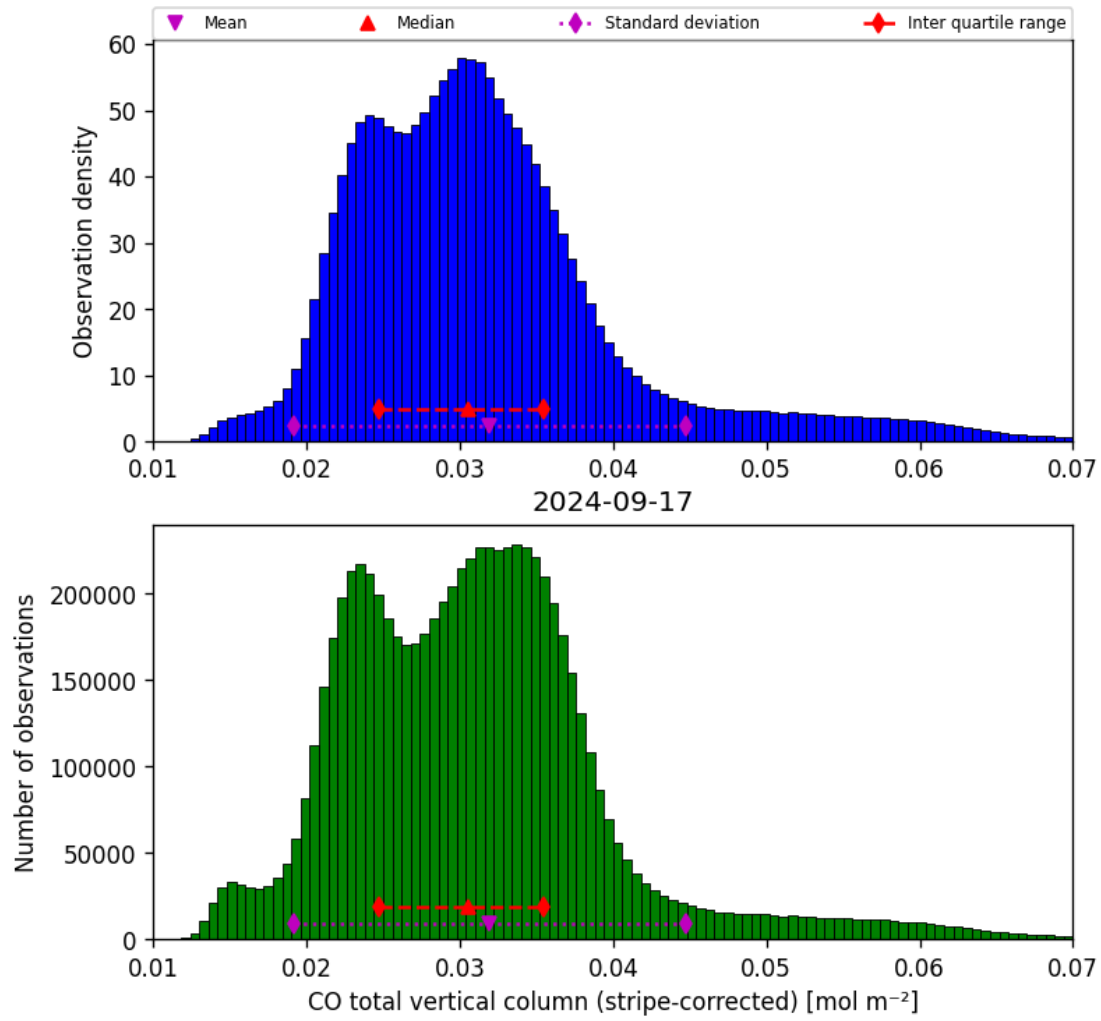
Figure 19: Histogram of “CO total vertical column (stripe-corrected)” for 2024-09-17 to 2024-09-18
