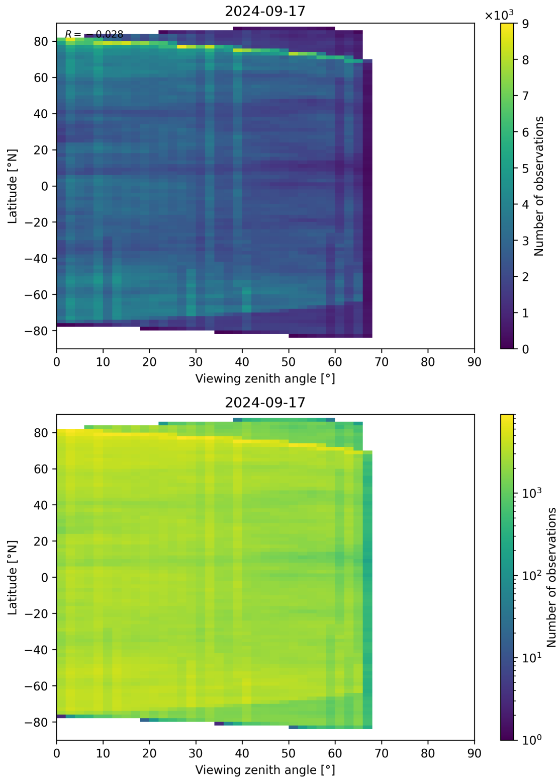
Figure 74: Scatter density plot of “Viewing zenith angle” against “Latitude” for 2024-09-17 to 2024-09-18.
