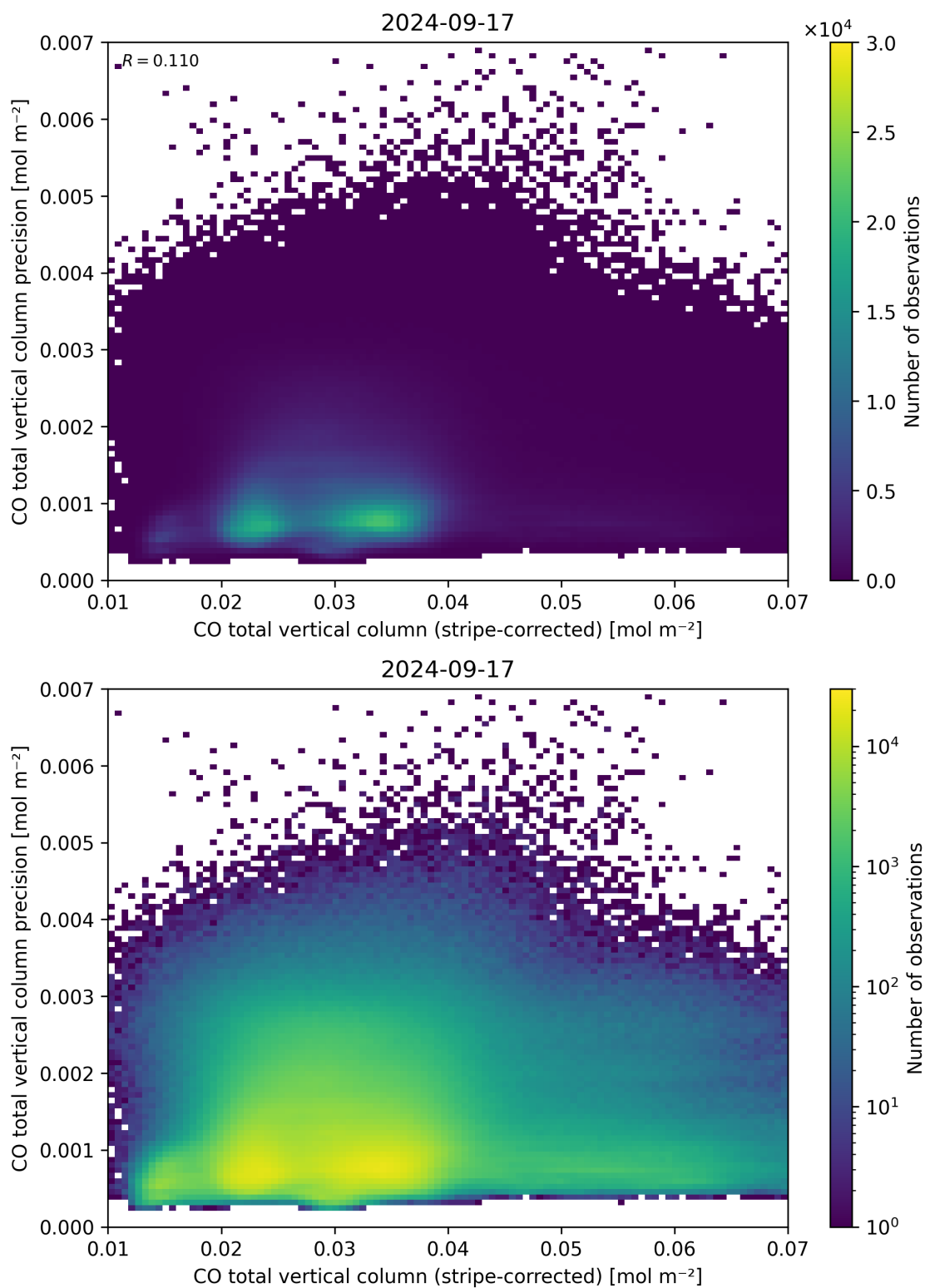
Figure 36: Scatter density plot of “CO total vertical column (stripe-corrected)” against “CO total vertical column precision” for 2024-09-17 to 2024-09-18.
