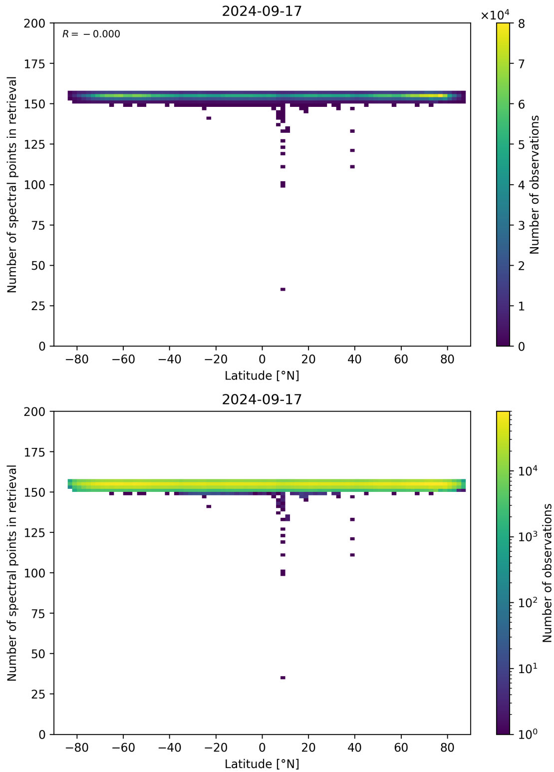
Figure 57: Scatter density plot of “Latitude” against “Number of spectral points in retrieval” for 2024-09-17 to 2024-09-18.
