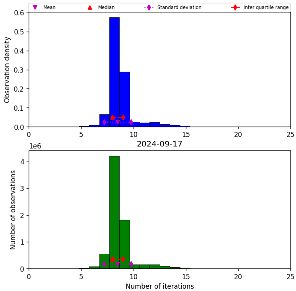
Figure 24: Histogram of “Number of iterations” for 2024-09-17 to 2024-09-18
