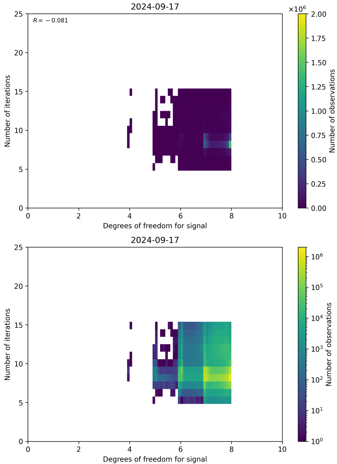
Figure 50: Scatter density plot of “Degrees of freedom for signal” against “Number of iterations” for 2024-09-17 to 2024-09-18.
