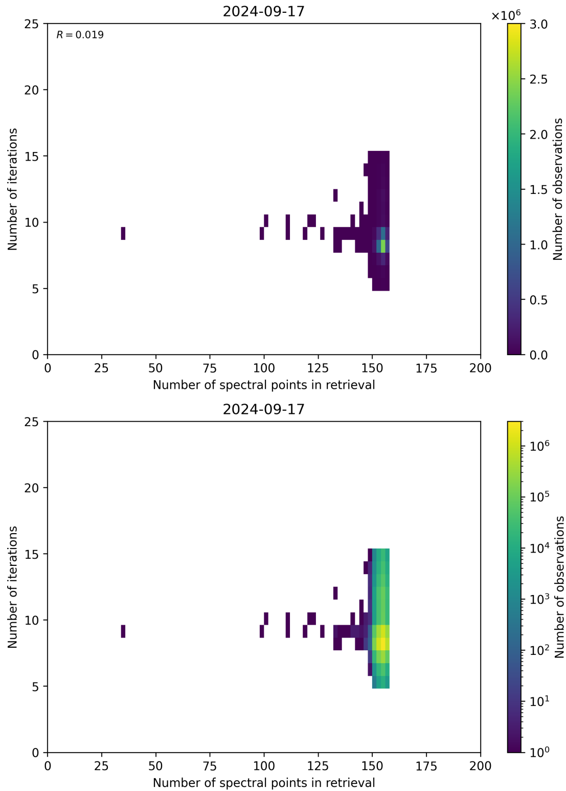
Figure 60: Scatter density plot of “Number of spectral points in retrieval” against “Number of iterations” for 2024-09-17 to 2024-09-18.
