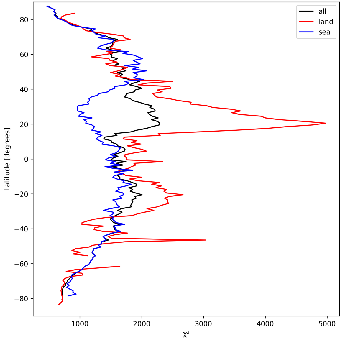
Figure 14: Zonal average of “ \chi^2 ” for 2024-09-17 to 2024-09-18.
