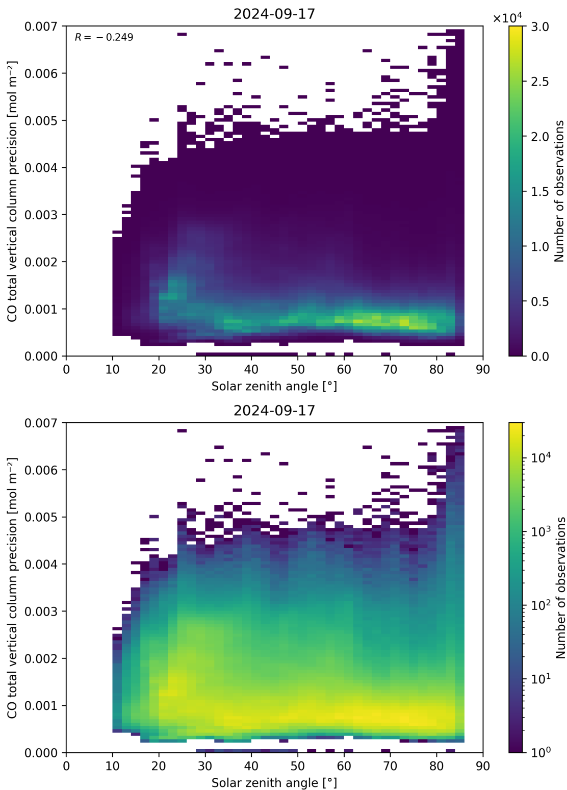
Figure 63: Scatter density plot of “Solar zenith angle” against “CO total vertical column precision” for 2024-09-17 to 2024-09-18.
