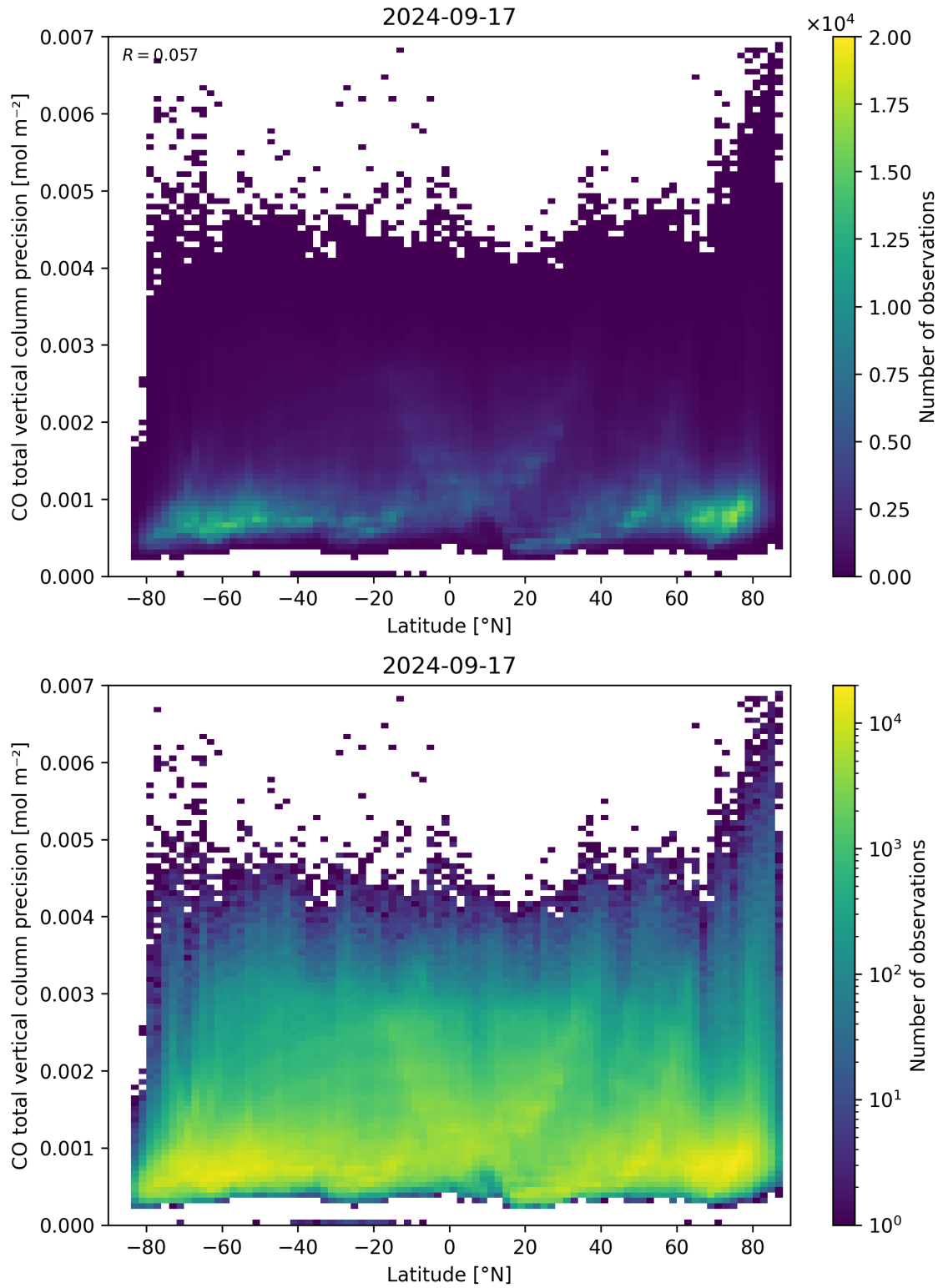
Figure 53: Scatter density plot of “Latitude” against “CO total vertical column precision” for 2024-09-17 to 2024-09-18.
