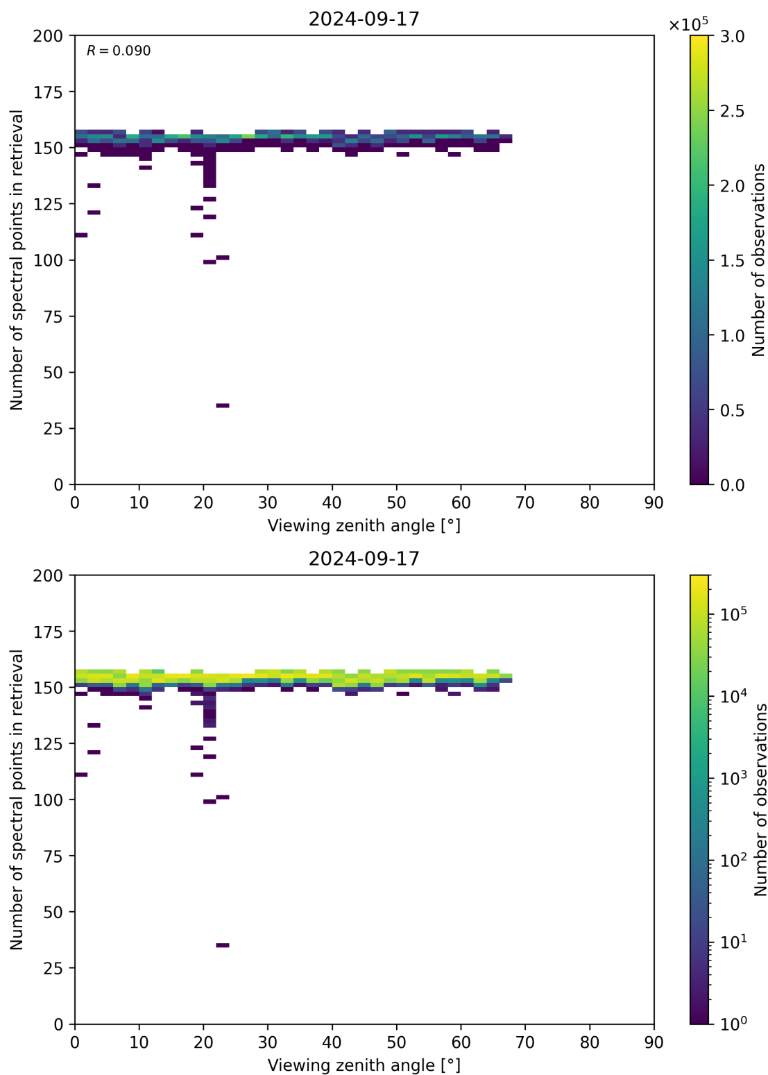
Figure 76: Scatter density plot of “Viewing zenith angle” against “Number of spectral points in retrieval” for 2024-09-17 to 2024-09-18.
