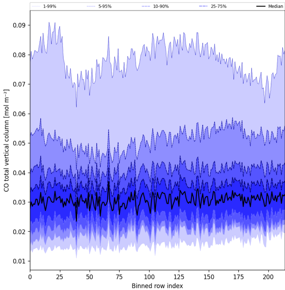
Figure 26: Along track statistics of “CO total vertical column” for 2024-09-17 to 2024-09-18
