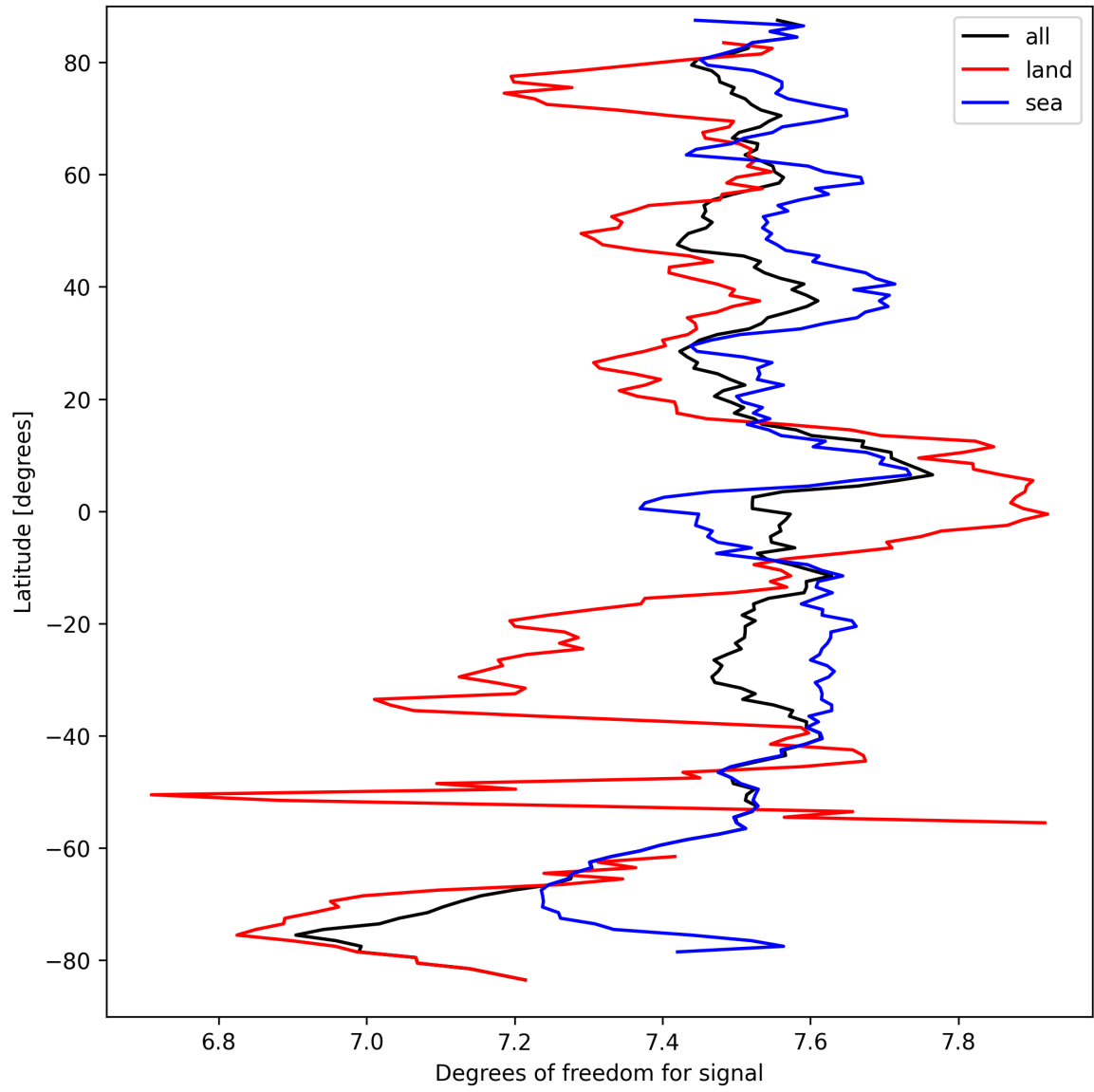
Figure 15: Zonal average of “Degrees of freedom for signal” for 2024-09-17 to 2024-09-18.
