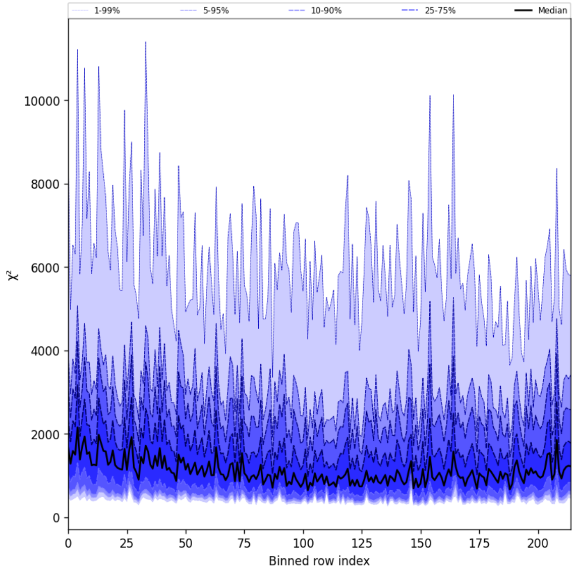
Figure 30: Along track statistics of “ \chi^2 ” for 2024-09-17 to 2024-09-18
