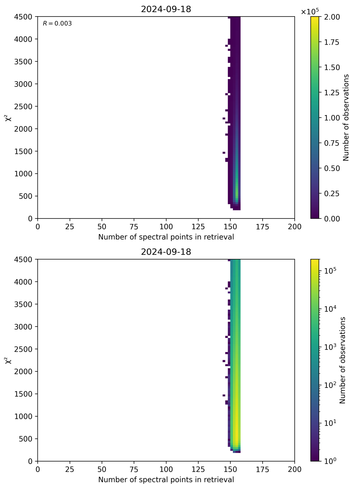
Figure 58: Scatter density plot of “Number of spectral points in retrieval” against “ \chi^2 ” for 2024-09-17 to 2024-09-19.
