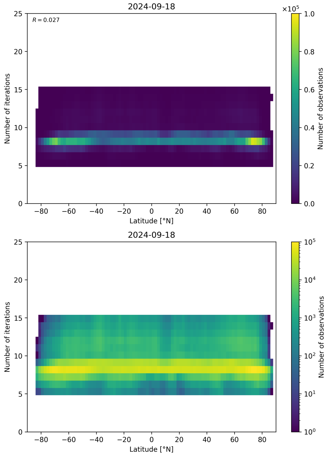
Figure 56: Scatter density plot of “Latitude” against “Number of iterations” for 2024-09-17 to 2024-09-19.
