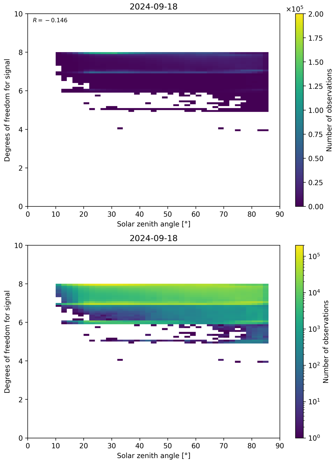
Figure 65: Scatter density plot of “Solar zenith angle” against “Degrees of freedom for signal” for 2024-09-17 to 2024-09-19.
