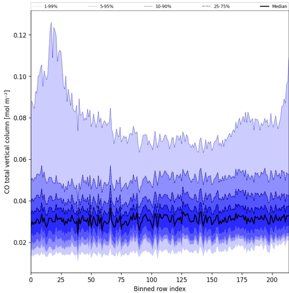
Figure 26: Along track statistics of “CO total vertical column” for 2024-09-17 to 2024-09-19
