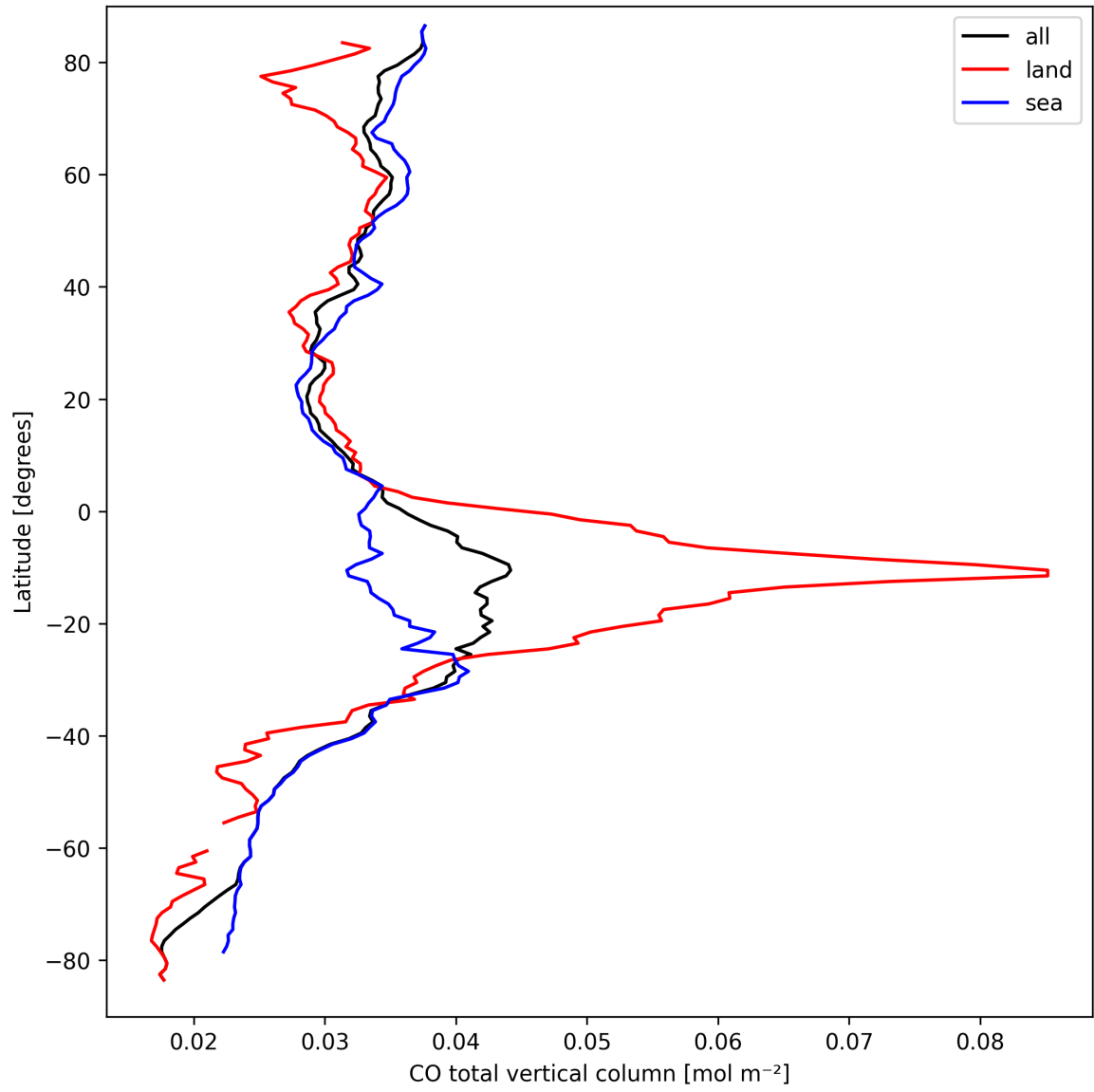
Figure 10: Zonal average of “CO total vertical column” for 2024-09-17 to 2024-09-19.
