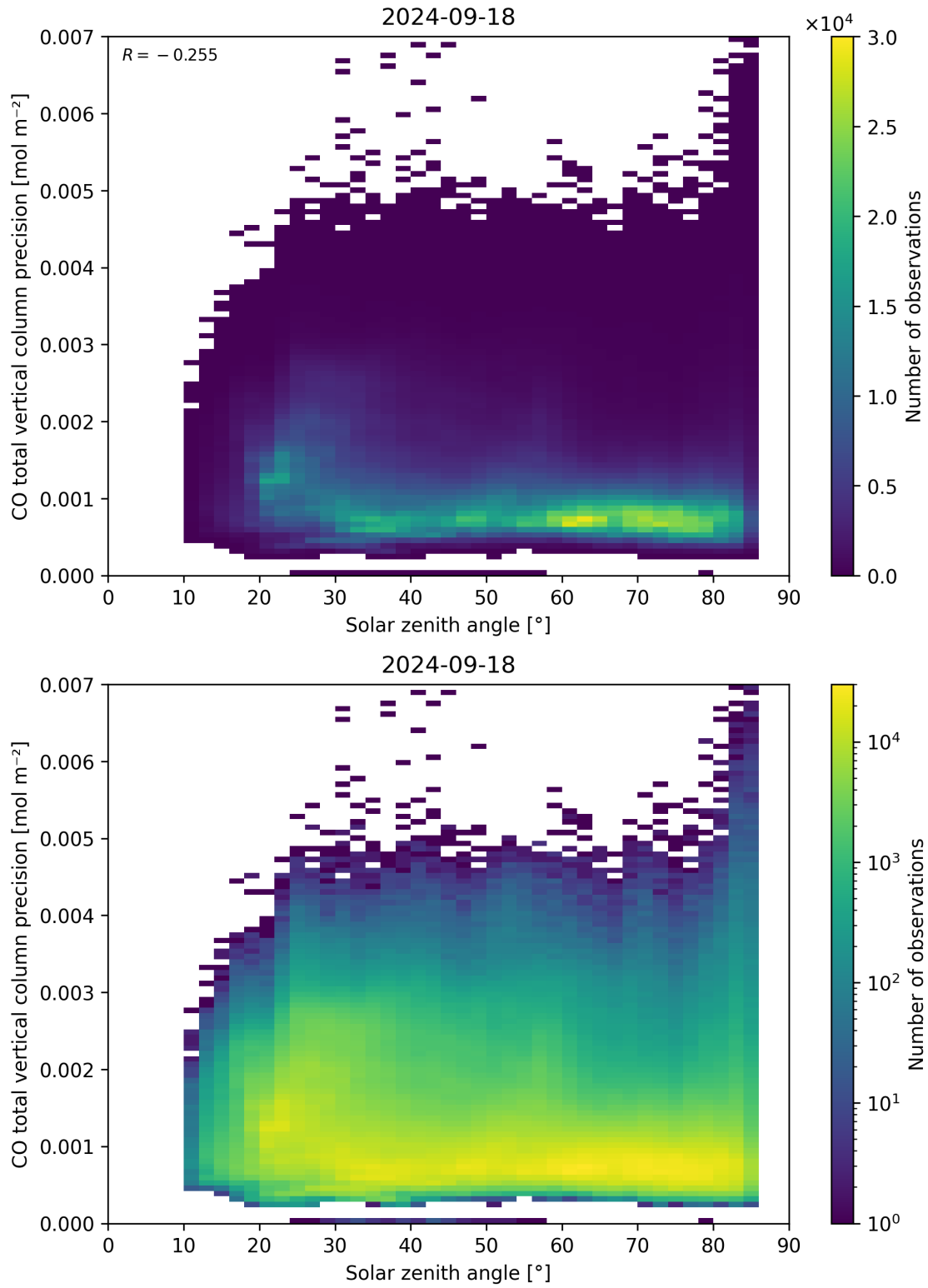
Figure 63: Scatter density plot of “Solar zenith angle” against “CO total vertical column precision” for 2024-09-17 to 2024-09-19.
