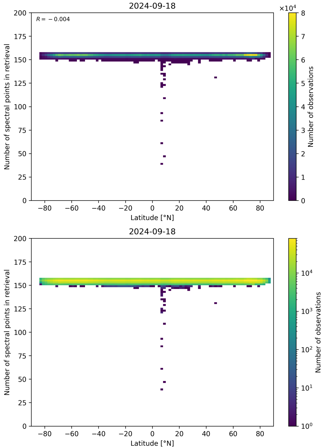
Figure 57: Scatter density plot of “Latitude” against “Number of spectral points in retrieval” for 2024-09-17 to 2024-09-19.
