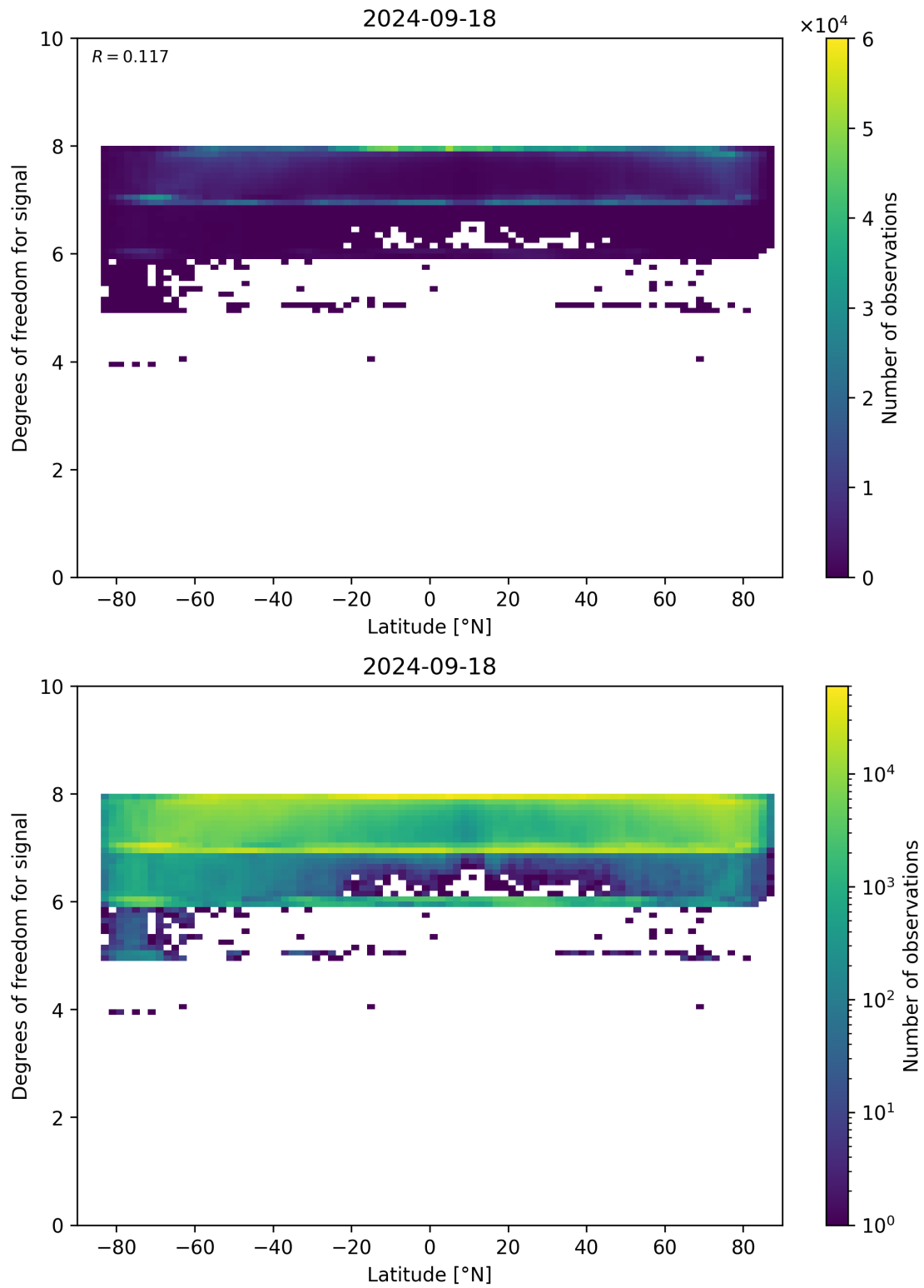
Figure 55: Scatter density plot of “Latitude” against “Degrees of freedom for signal” for 2024-09-17 to 2024-09-19.
