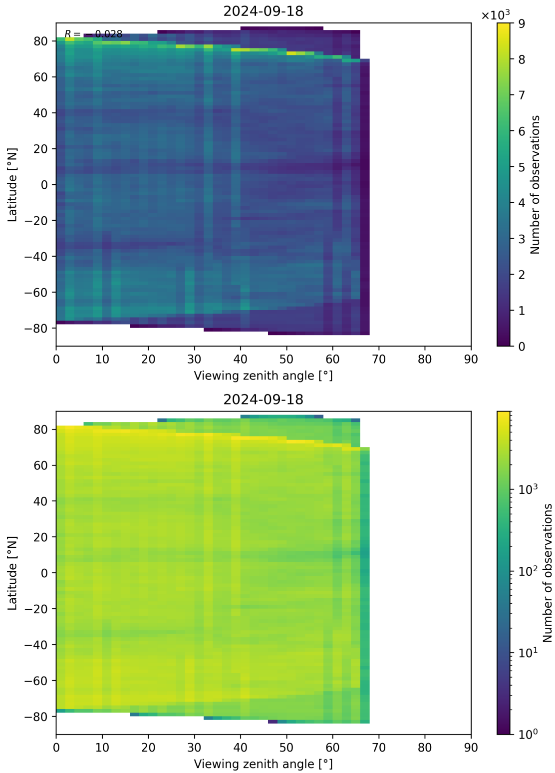
Figure 74: Scatter density plot of “Viewing zenith angle” against “Latitude” for 2024-09-17 to 2024-09-19.
