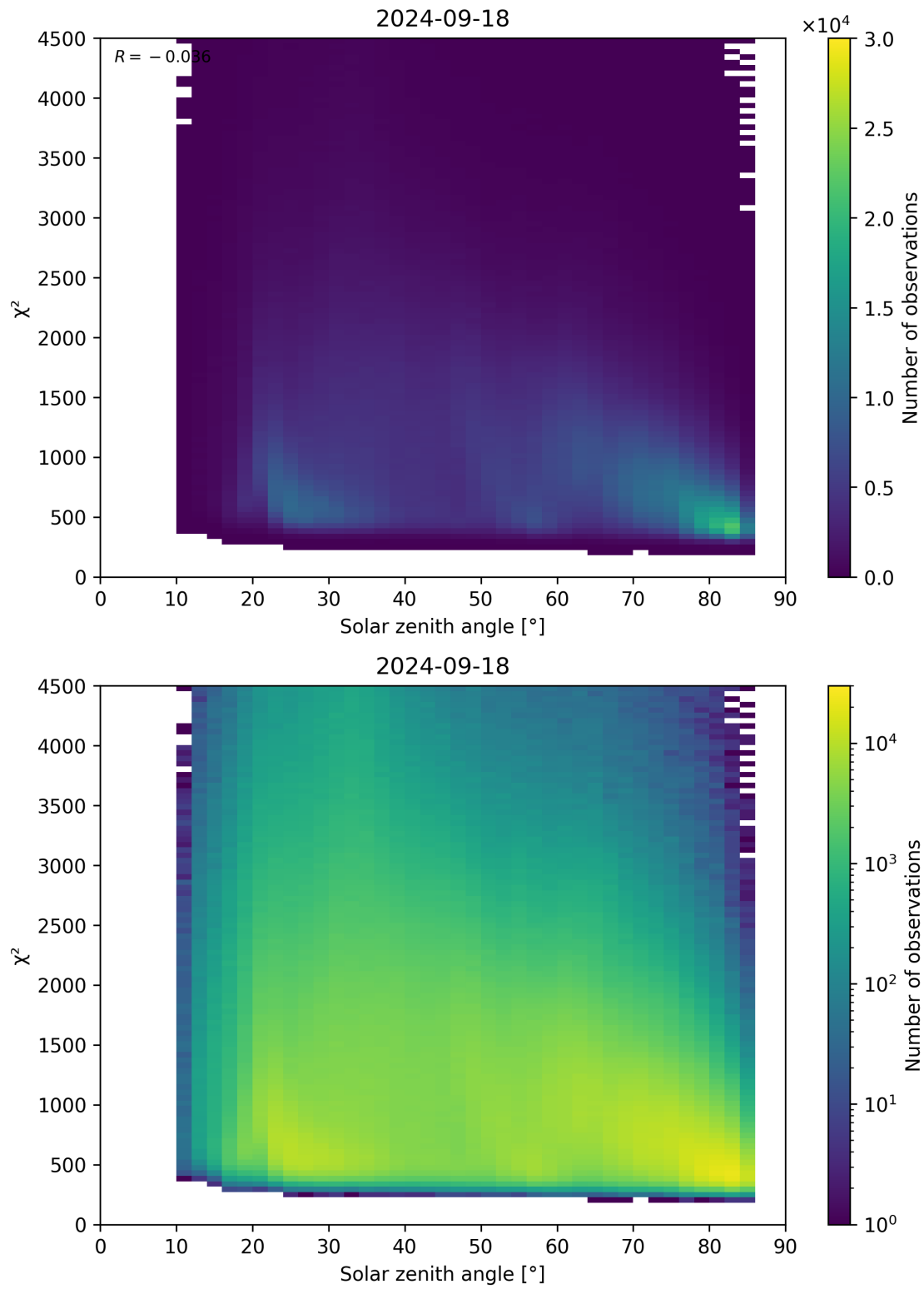
Figure 64: Scatter density plot of “Solar zenith angle” against “ \chi^2 ” for 2024-09-17 to 2024-09-19.
