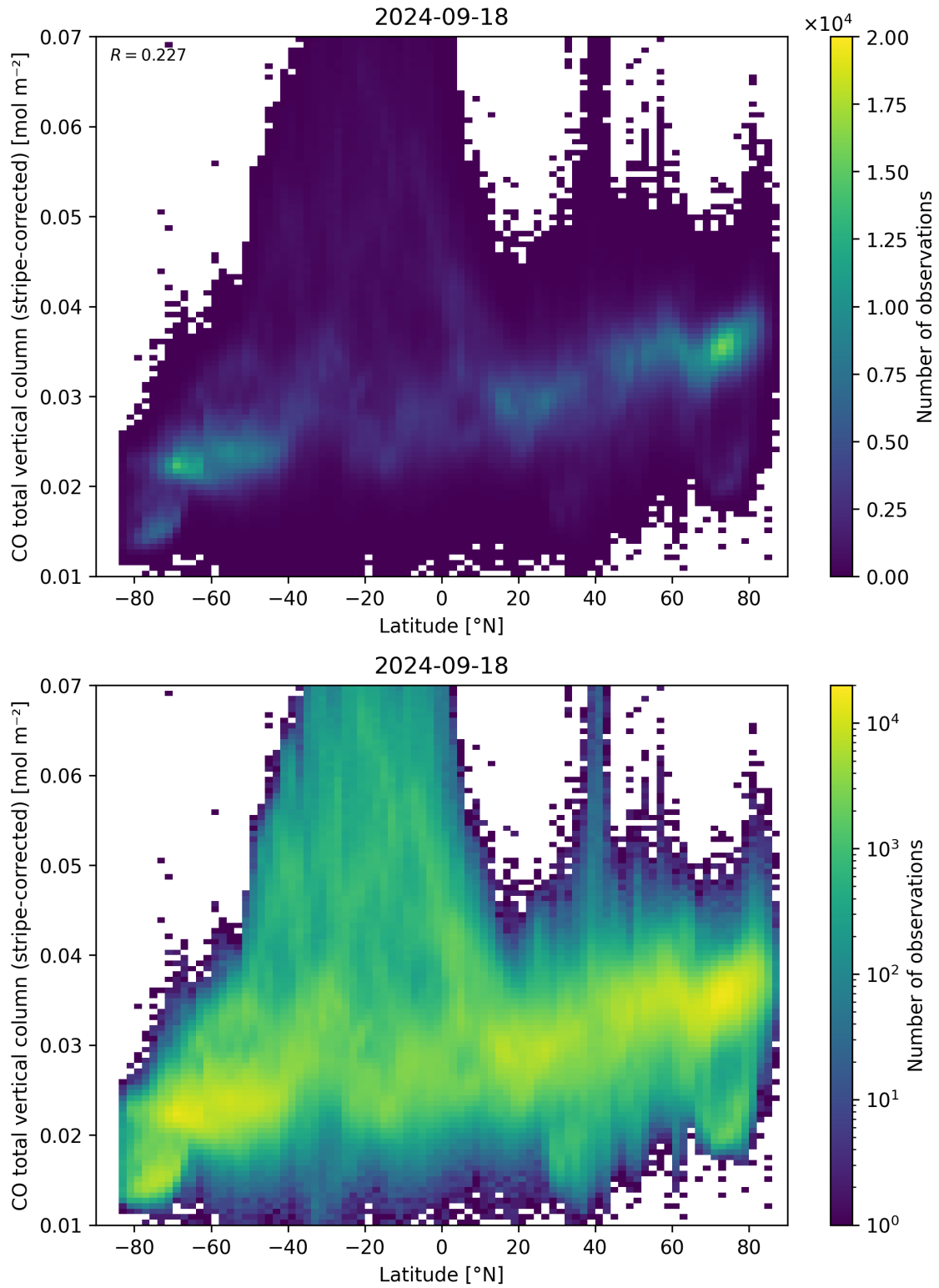
Figure 52: Scatter density plot of “Latitude” against “CO total vertical column (stripe-corrected)” for 2024-09-17 to 2024-09-19.
