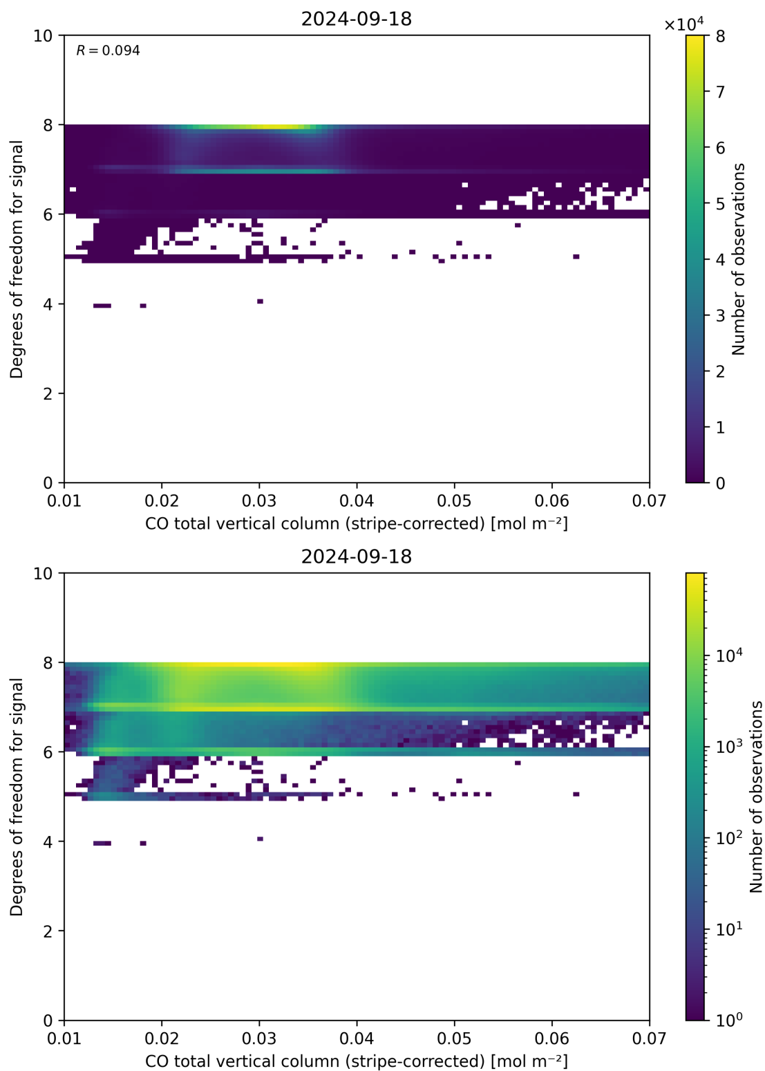
Figure 38: Scatter density plot of “CO total vertical column (stripe-corrected)” against “Degrees of freedom for signal” for 2024-09-17 to 2024-09-19.
