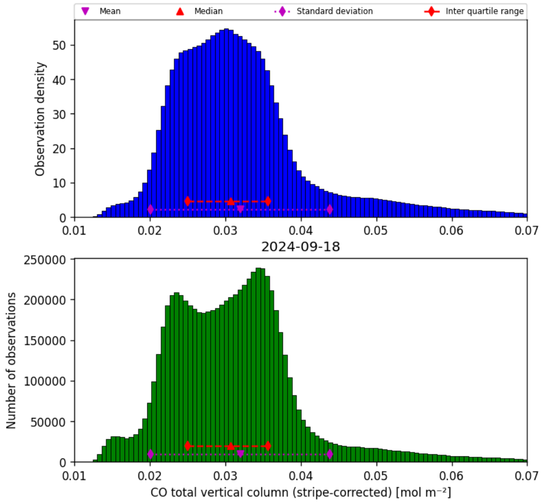
Figure 19: Histogram of “CO total vertical column (stripe-corrected)” for 2024-09-17 to 2024-09-19
