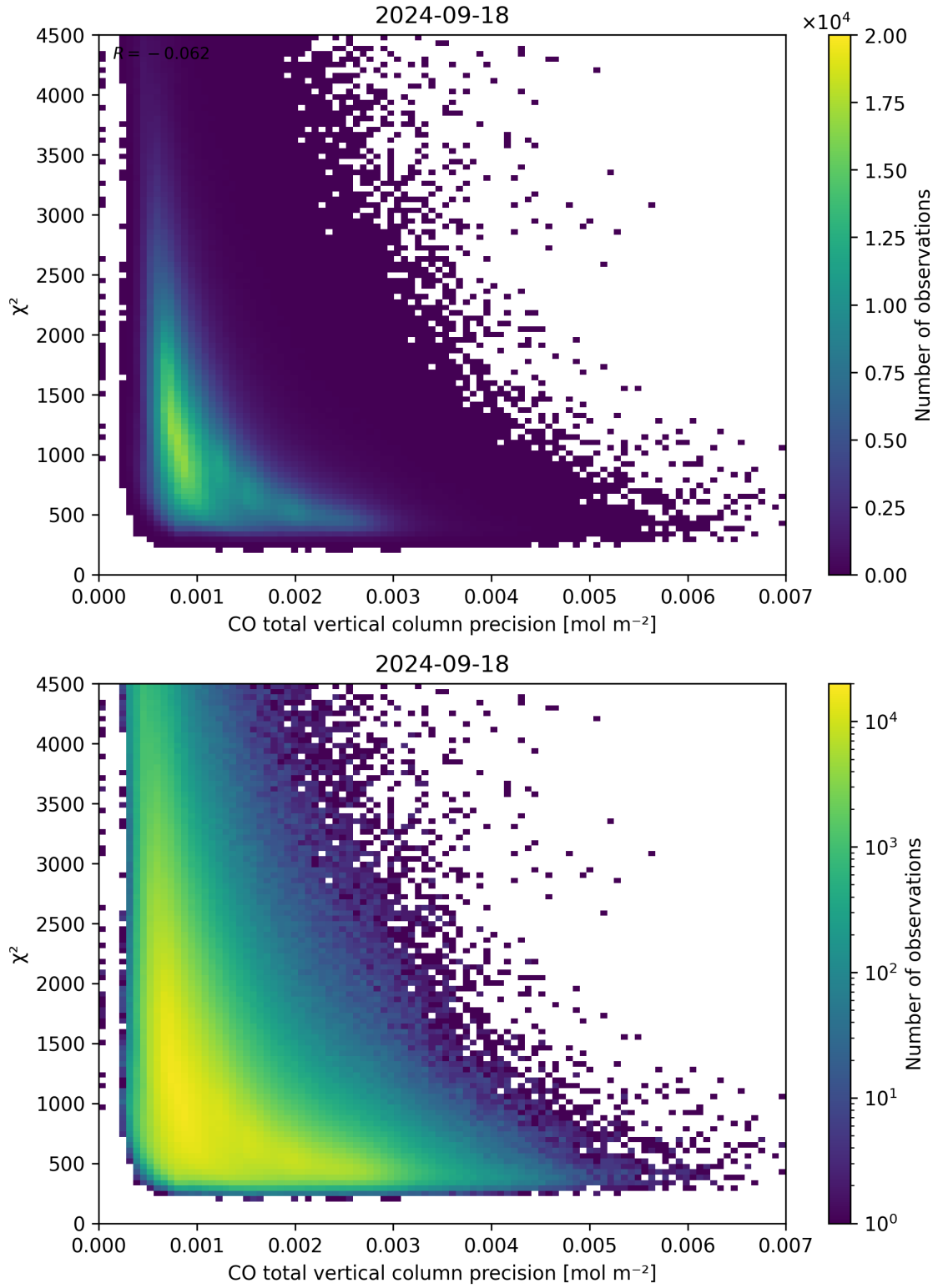
Figure 44: Scatter density plot of “CO total vertical column precision” against “ \chi^2 ” for 2024-09-17 to 2024-09-19.
