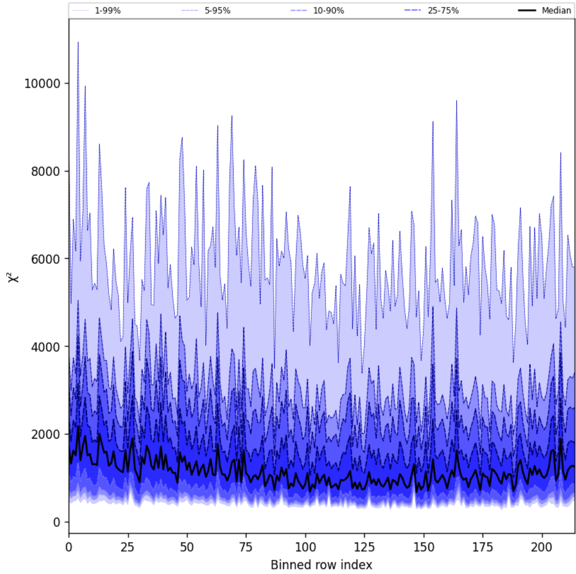
Figure 30: Along track statistics of “ \chi^2 ” for 2024-09-17 to 2024-09-19
