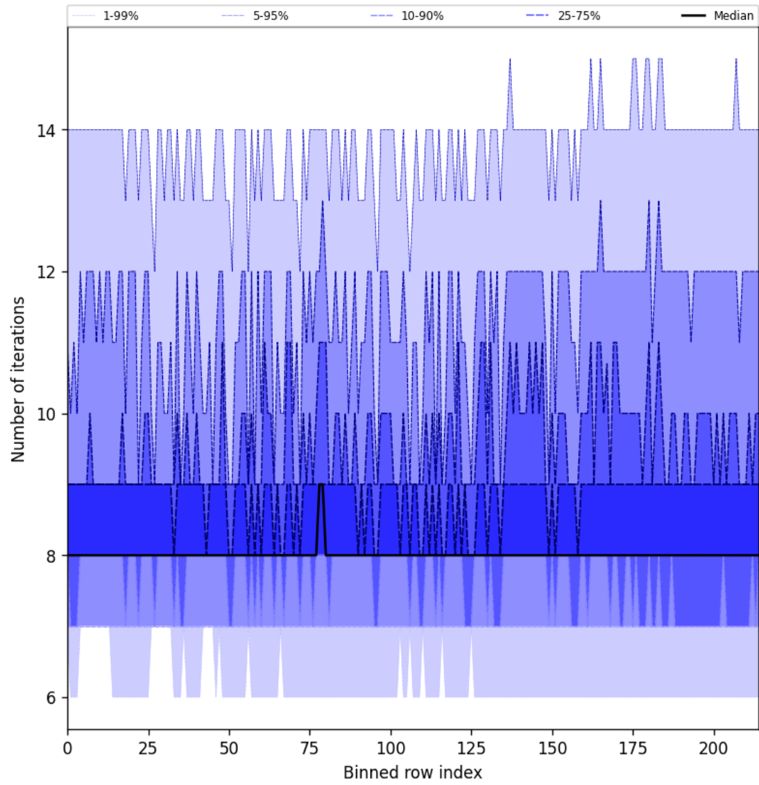
Figure 32: Along track statistics of “Number of iterations” for 2024-09-17 to 2024-09-19
