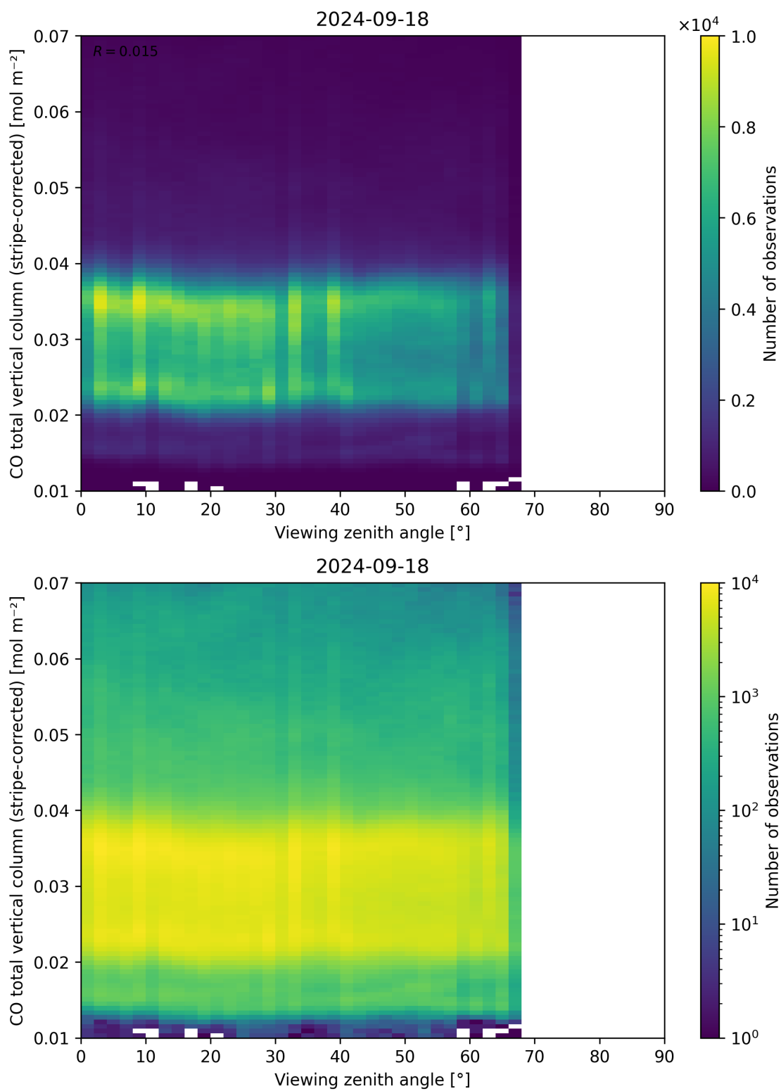
Figure 70: Scatter density plot of “Viewing zenith angle” against “CO total vertical column (stripe-corrected)” for 2024-09-17 to 2024-09-19.
