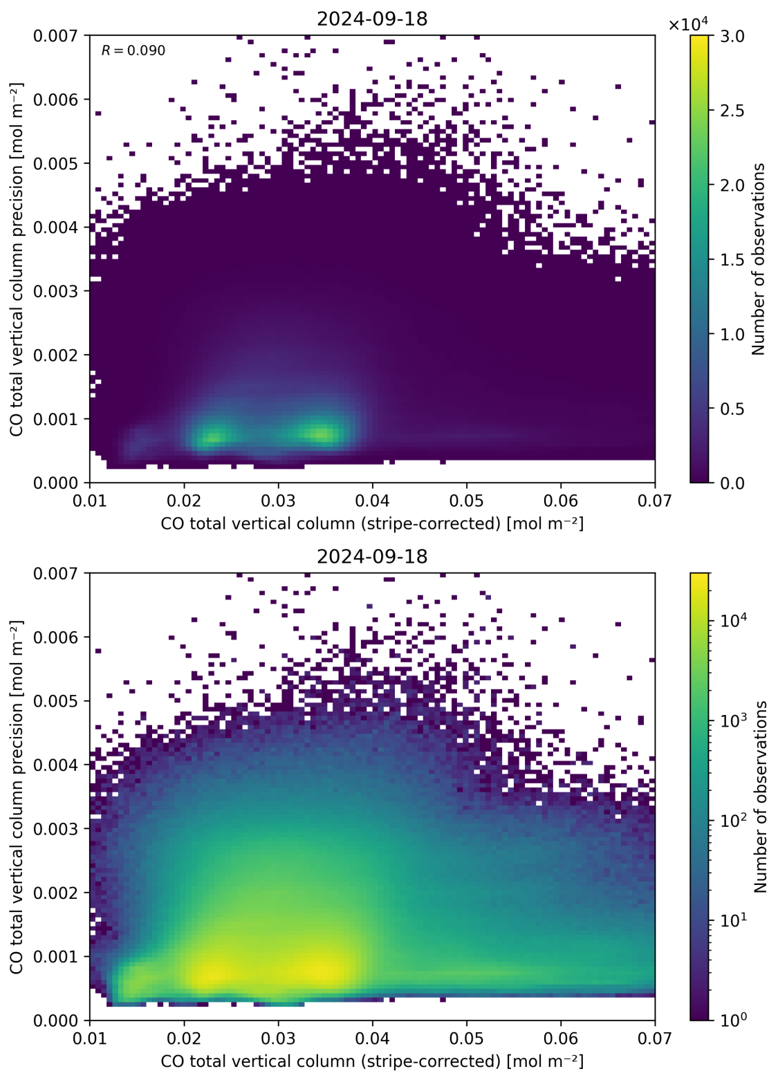
Figure 36: Scatter density plot of “CO total vertical column (stripe-corrected)” against “CO total vertical column precision” for 2024-09-17 to 2024-09-19.
