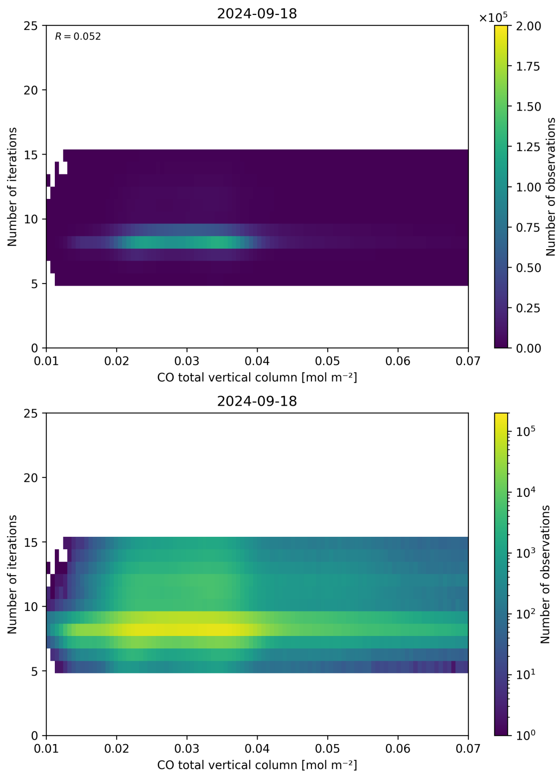
Figure 42: Scatter density plot of “CO total vertical column” against “Number of iterations” for 2024-09-17 to 2024-09-19.
