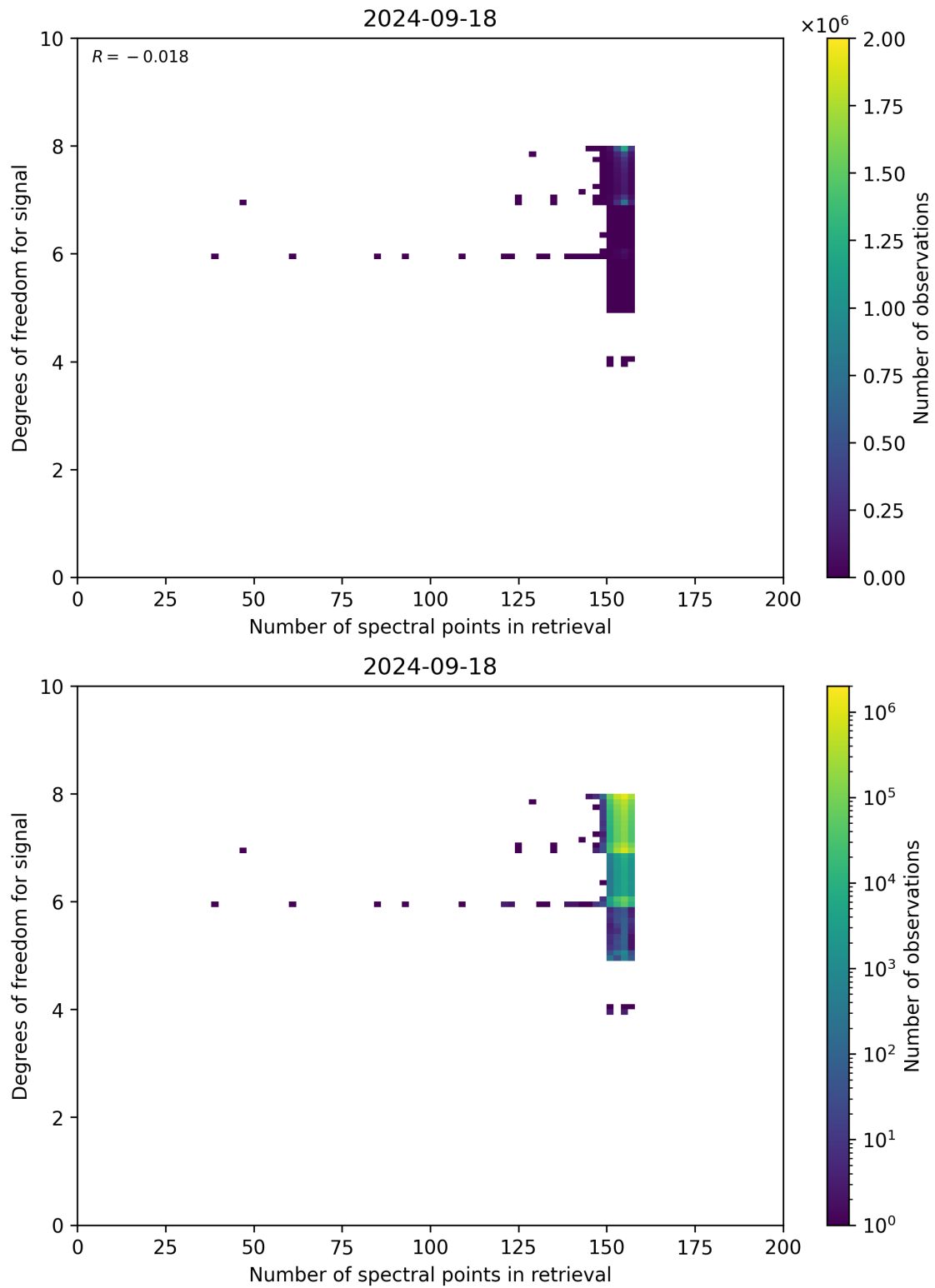
Figure 59: Scatter density plot of “Number of spectral points in retrieval” against “Degrees of freedom for signal” for 2024-09-17 to 2024-09-19.
