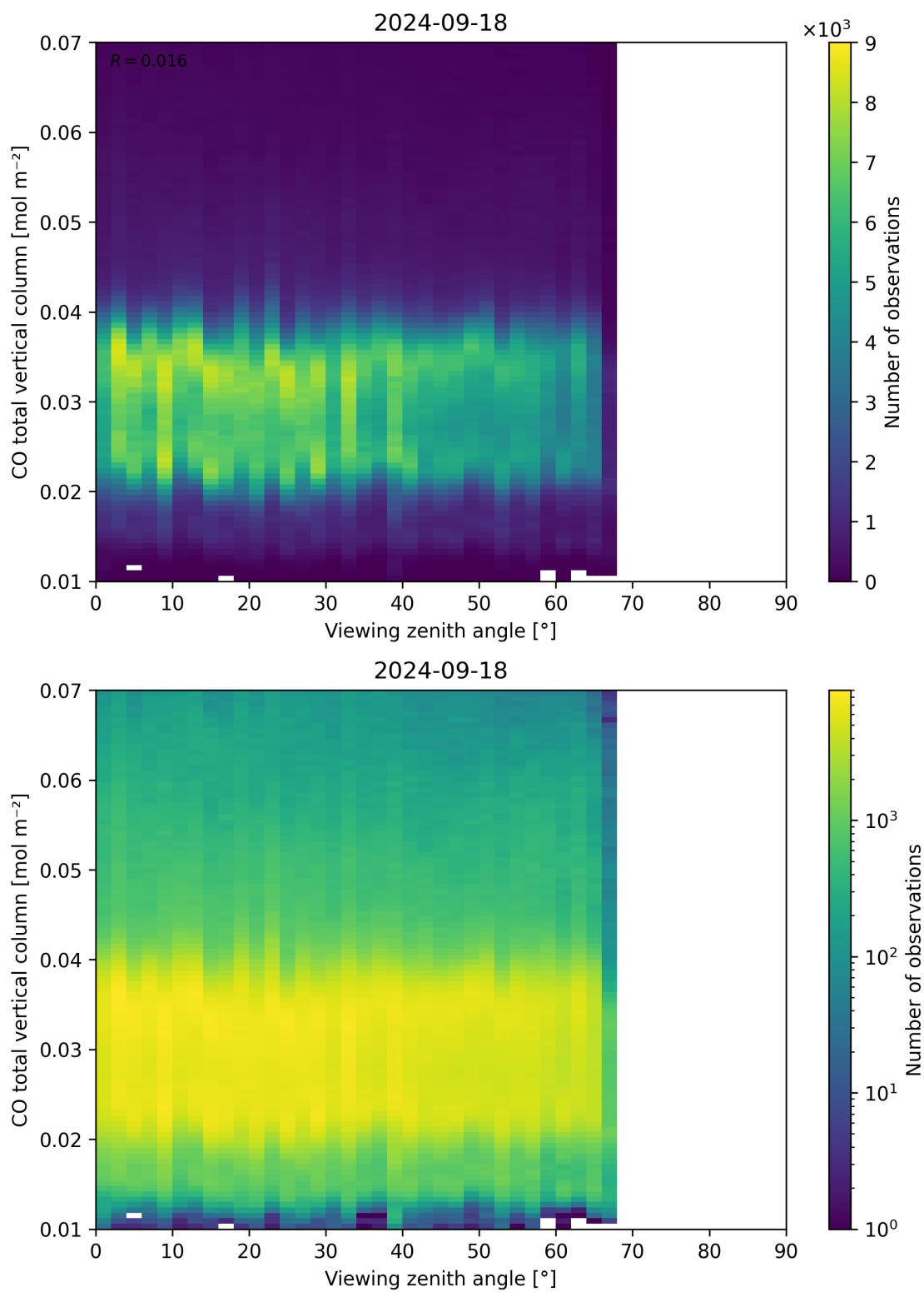
Figure 69: Scatter density plot of “Viewing zenith angle” against “CO total vertical column” for 2024-09-17 to 2024-09-19.
