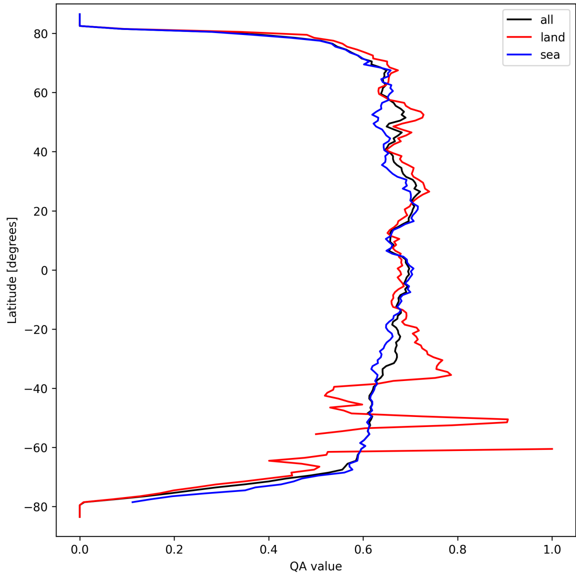
Figure 9: Zonal average of “QA value” for 2024-09-17 to 2024-09-19.
