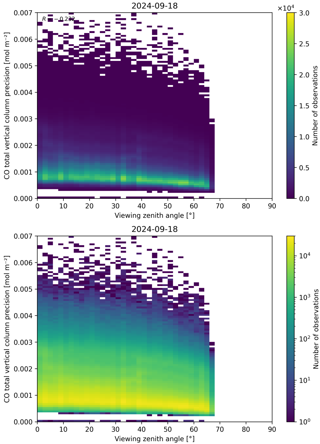
Figure 71: Scatter density plot of “Viewing zenith angle” against “CO total vertical column precision” for 2024-09-17 to 2024-09-19.
