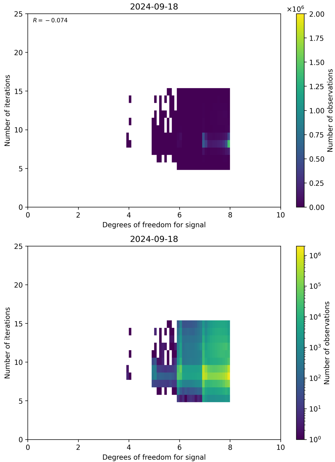
Figure 50: Scatter density plot of “Degrees of freedom for signal” against “Number of iterations” for 2024-09-17 to 2024-09-19.
