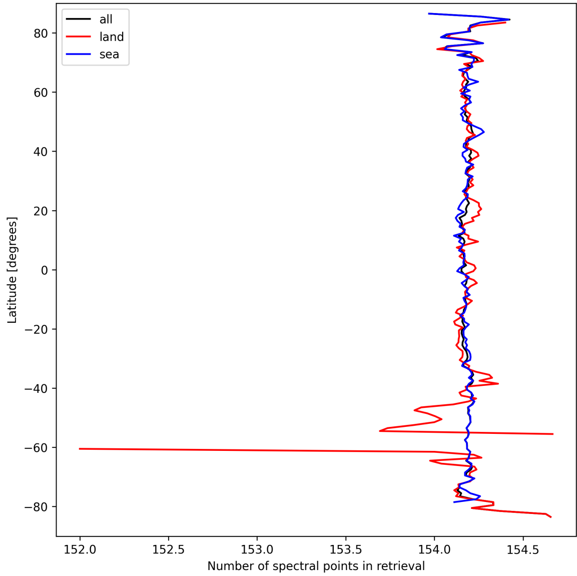
Figure 13: Zonal average of “Number of spectral points in retrieval” for 2024-09-17 to 2024-09-19.
