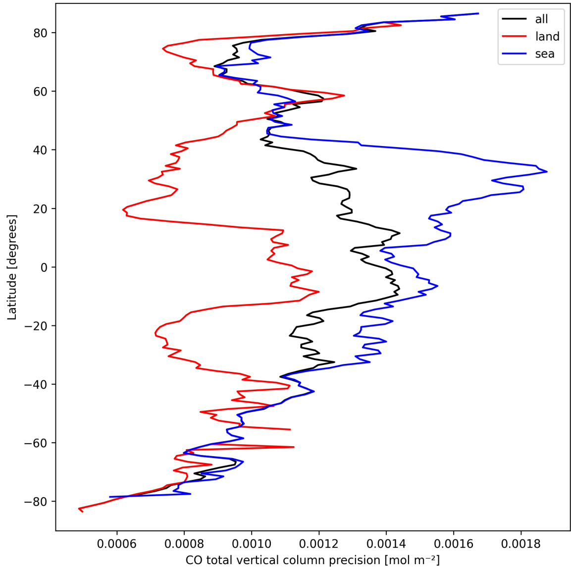
Figure 12: Zonal average of “CO total vertical column precision” for 2024-09-17 to 2024-09-19.
