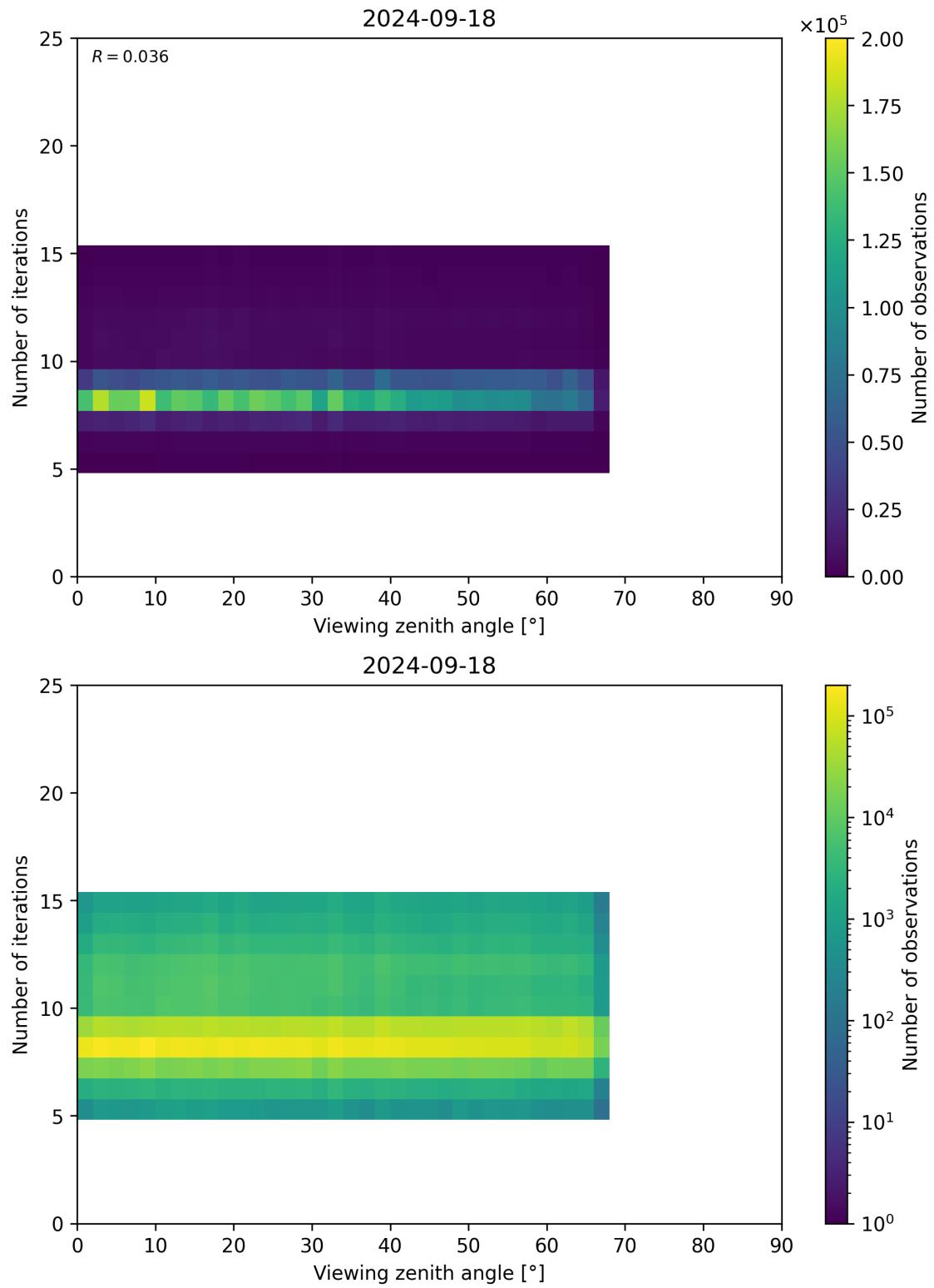
Figure 75: Scatter density plot of “Viewing zenith angle” against “Number of iterations” for 2024-09-17 to 2024-09-19.
