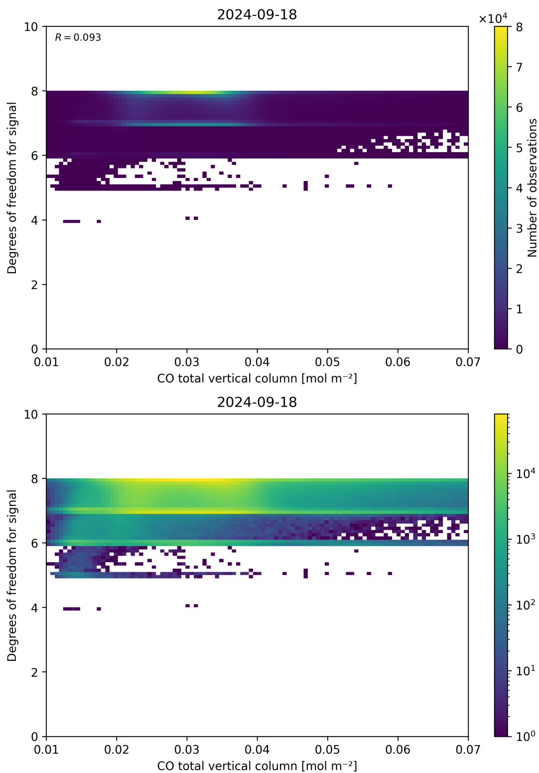
Figure 41: Scatter density plot of “CO total vertical column” against “Degrees of freedom for signal” for 2024-09-17 to 2024-09-19.
