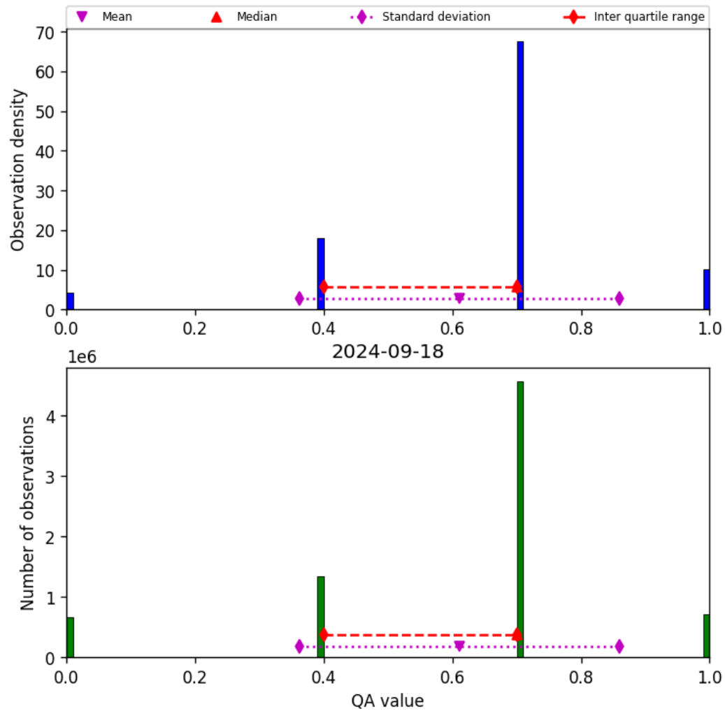
Figure 17: Histogram of “QA value” for 2024-09-17 to 2024-09-19
