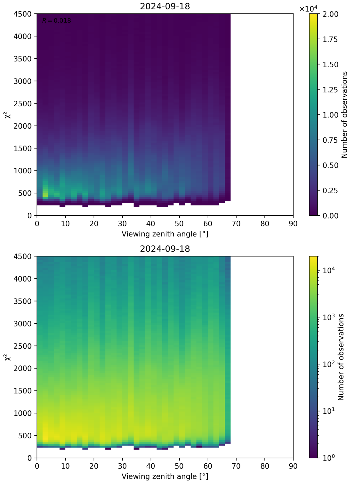
Figure 72: Scatter density plot of “Viewing zenith angle” against “ \chi^2 ” for 2024-09-17 to 2024-09-19.
