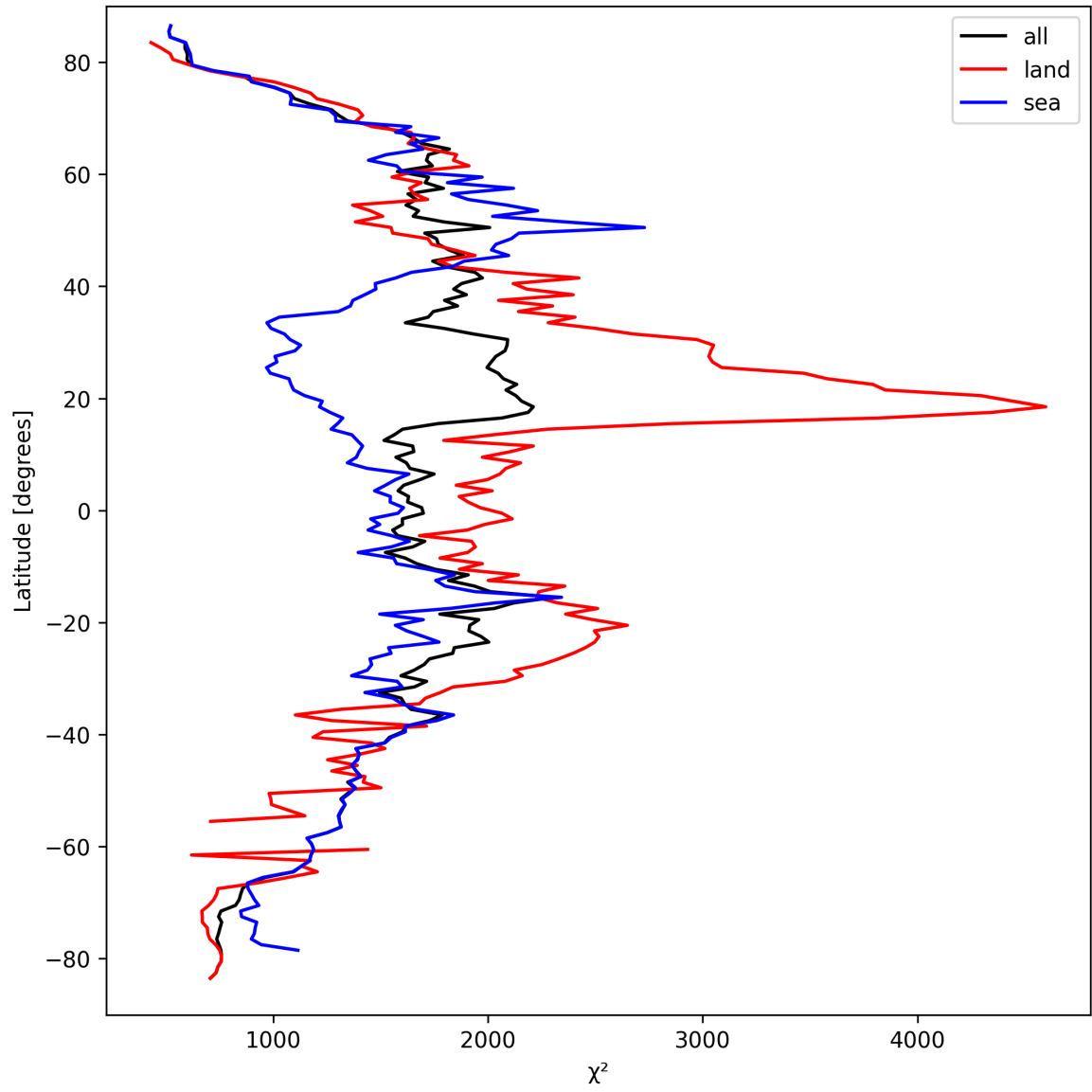
Figure 14: Zonal average of “ \chi^2 ” for 2024-09-17 to 2024-09-19.
