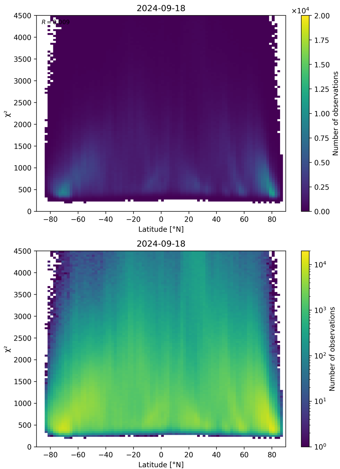
Figure 54: Scatter density plot of “Latitude” against “ \chi^2 ” for 2024-09-17 to 2024-09-19.
