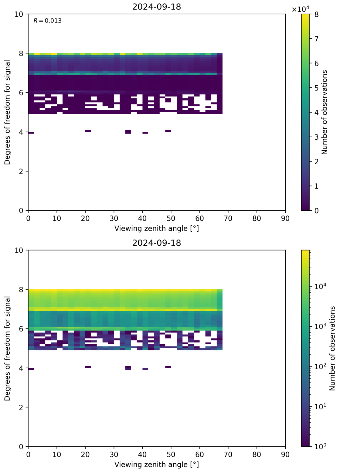
Figure 73: Scatter density plot of “Viewing zenith angle” against “Degrees of freedom for signal” for 2024-09-17 to 2024-09-19.
