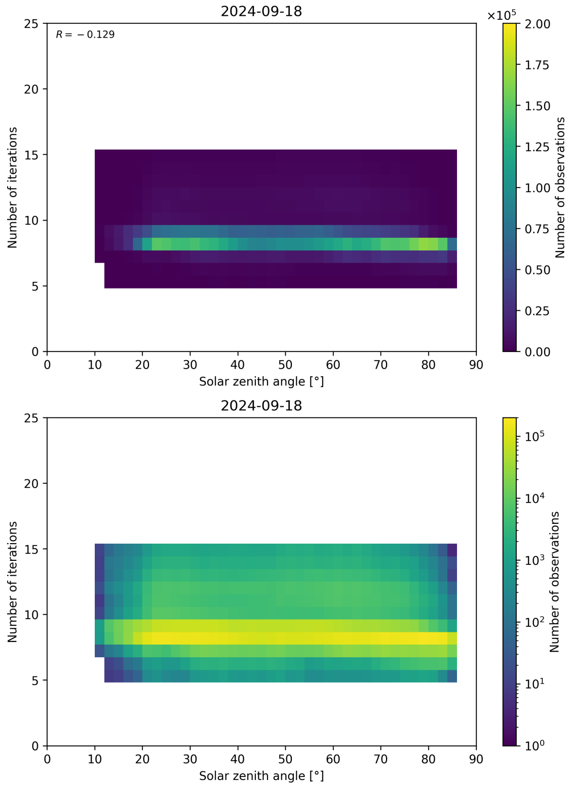
Figure 67: Scatter density plot of “Solar zenith angle” against “Number of iterations” for 2024-09-17 to 2024-09-19.
