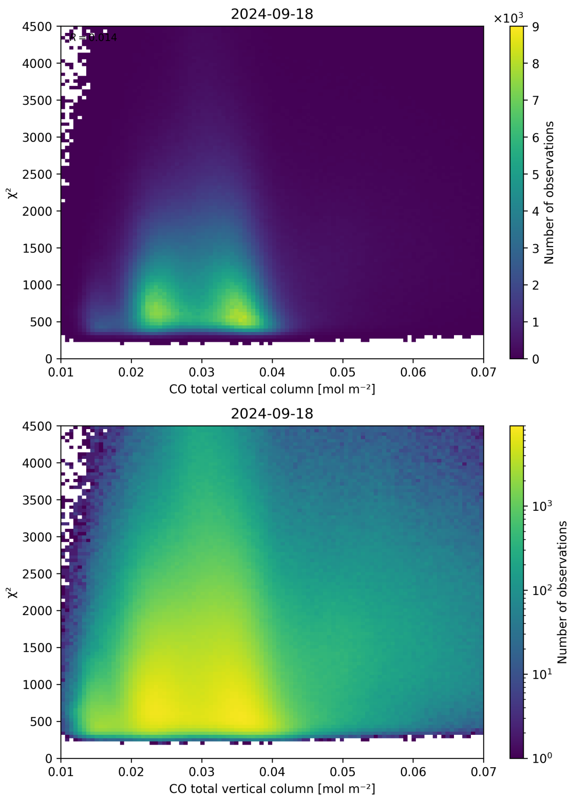
Figure 35: Scatter density plot of “CO total vertical column” against “ \chi^2 ” for 2024-09-17 to 2024-09-19.
