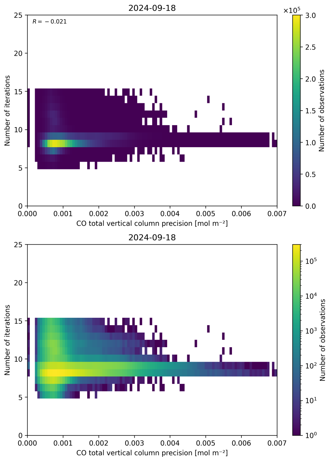
Figure 46: Scatter density plot of “CO total vertical column precision” against “Number of iterations” for 2024-09-17 to 2024-09-19.
