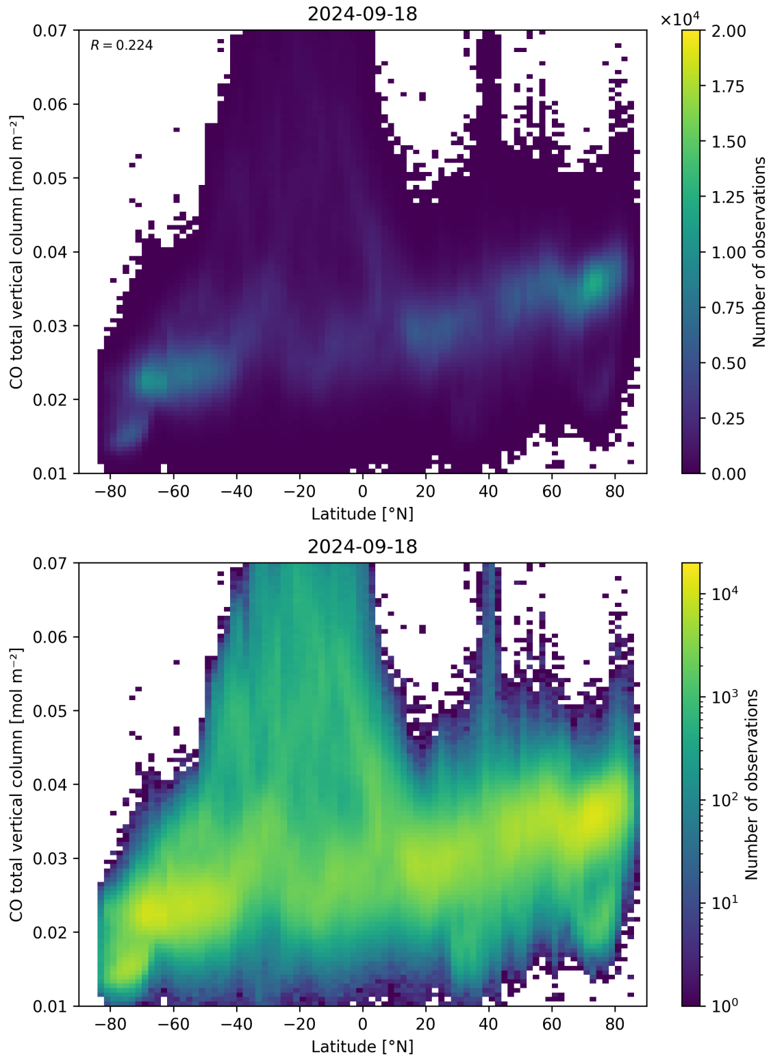
Figure 51: Scatter density plot of “Latitude” against “CO total vertical column” for 2024-09-17 to 2024-09-19.
