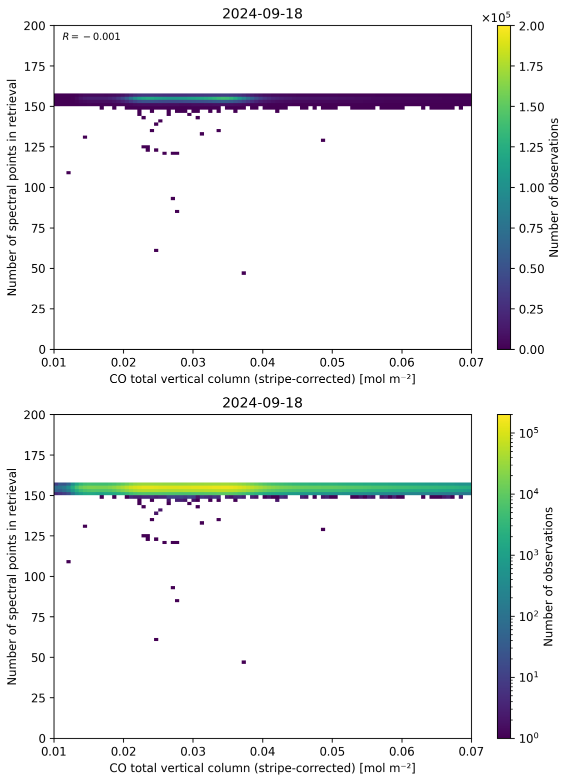
Figure 40: Scatter density plot of “CO total vertical column (stripe-corrected)” against “Number of spectral points in retrieval” for 2024-09-17 to 2024-09-19.
