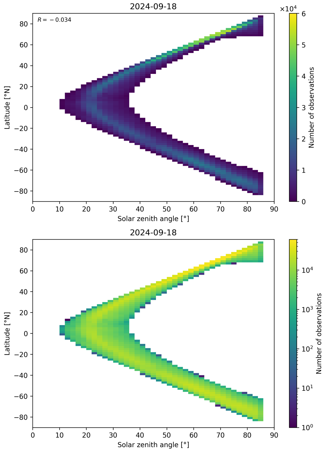
Figure 66: Scatter density plot of “Solar zenith angle” against “Latitude” for 2024-09-17 to 2024-09-19.
