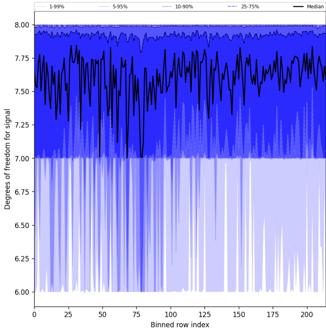
Figure 31: Along track statistics of “Degrees of freedom for signal” for 2024-09-17 to 2024-09-19
