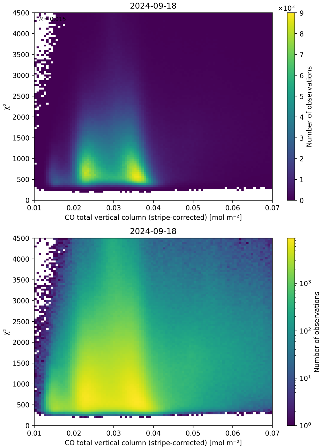
Figure 37: Scatter density plot of “CO total vertical column (stripe-corrected)” against “ \chi^2 ” for 2024-09-17 to 2024-09-19.
