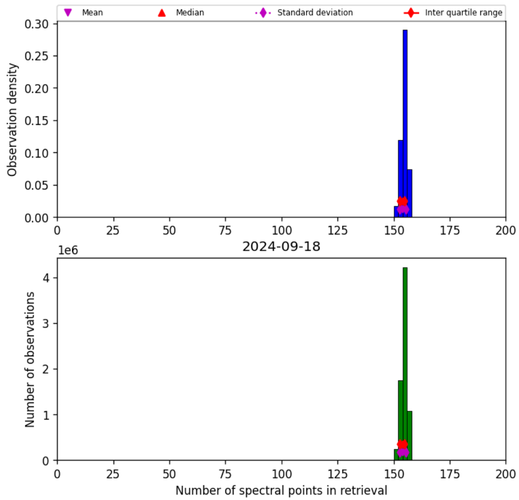
Figure 21: Histogram of “Number of spectral points in retrieval” for 2024-09-17 to 2024-09-19
