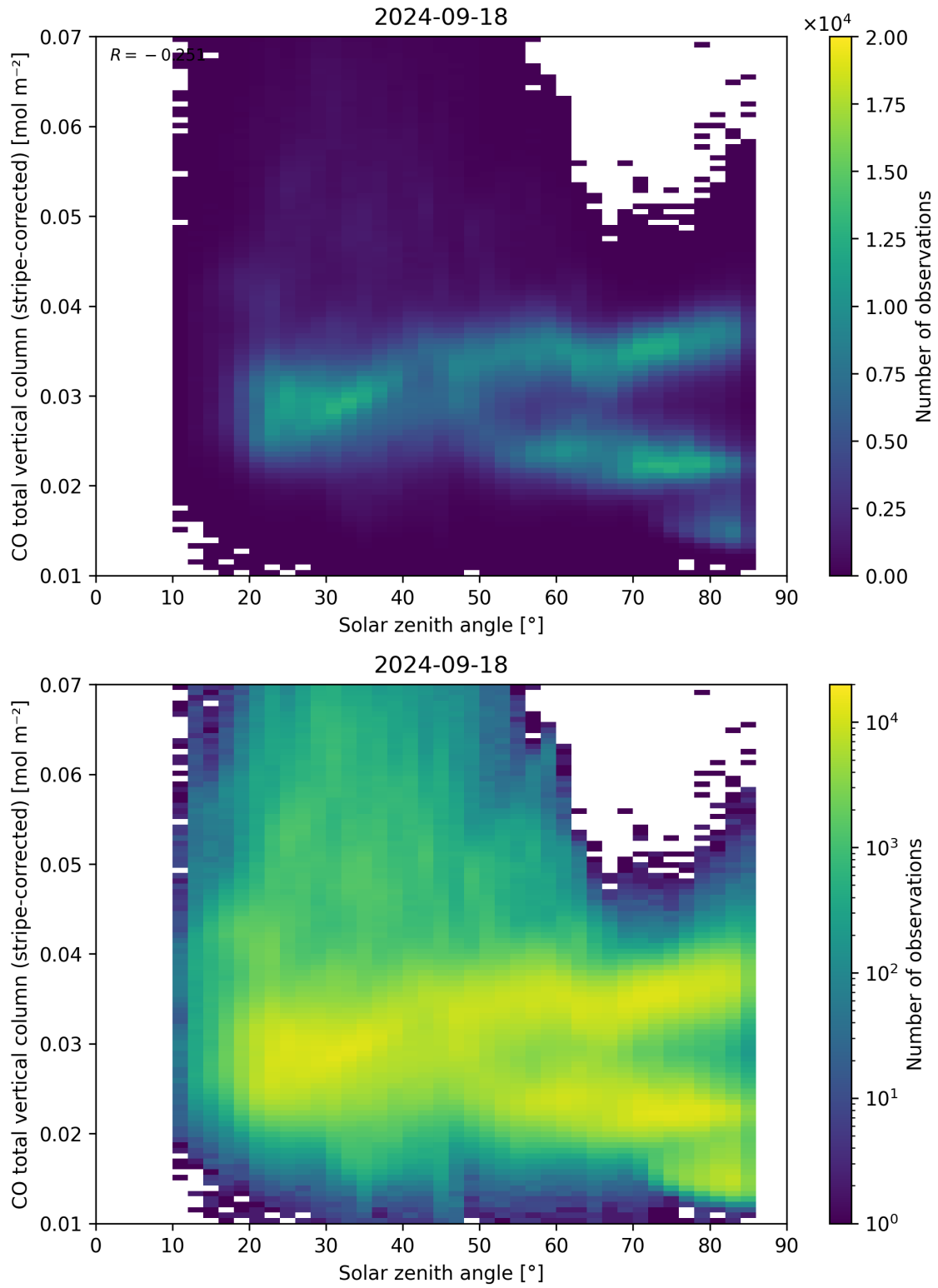
Figure 62: Scatter density plot of “Solar zenith angle” against “CO total vertical column (stripe-corrected)” for 2024-09-17 to 2024-09-19.
