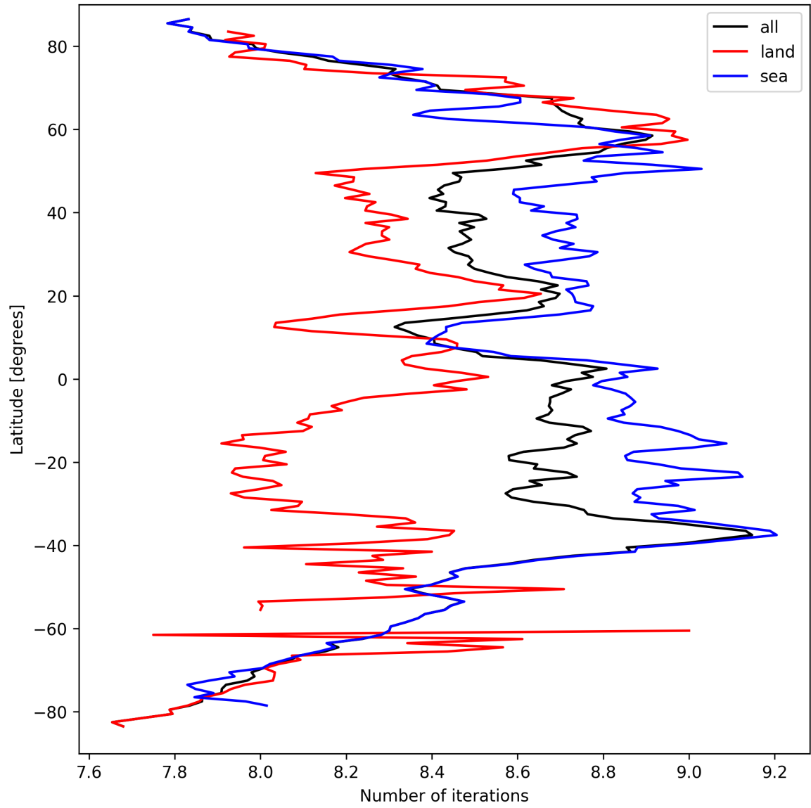
Figure 16: Zonal average of “Number of iterations” for 2024-09-17 to 2024-09-19.
