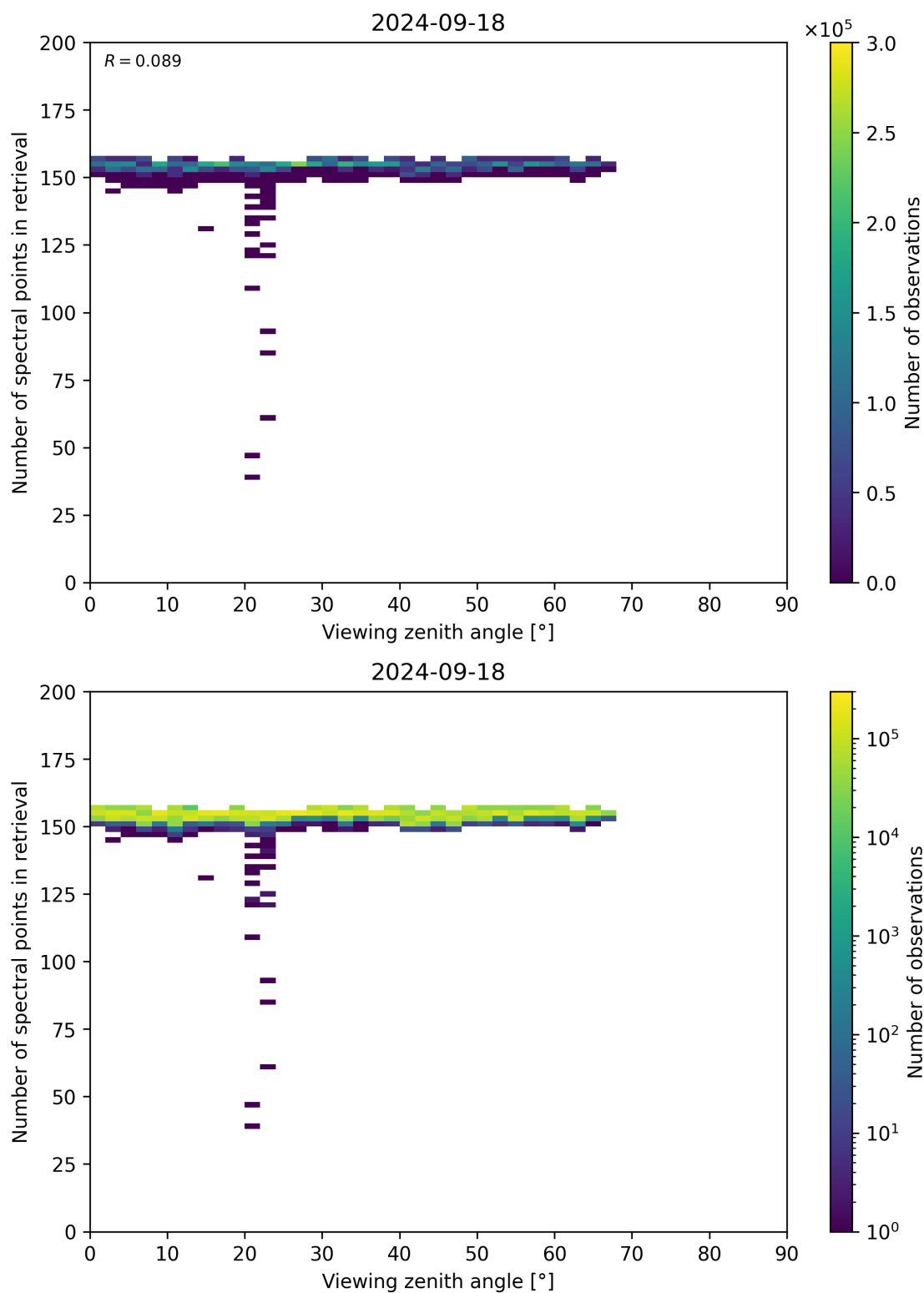
Figure 76: Scatter density plot of “Viewing zenith angle” against “Number of spectral points in retrieval” for 2024-09-17 to 2024-09-19.
