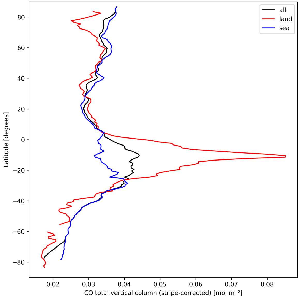
Figure 11: Zonal average of “CO total vertical column (stripe-corrected)” for 2024-09-17 to 2024-09-19.
