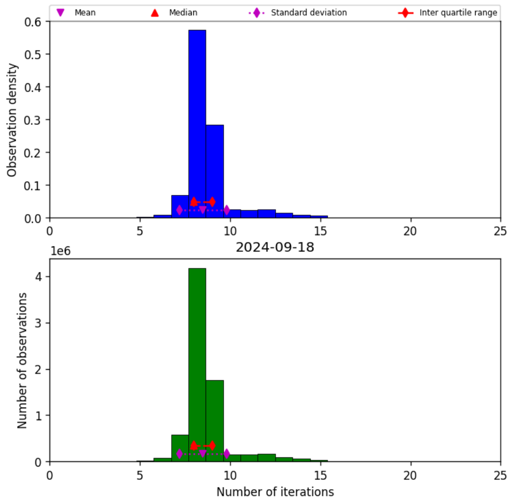
Figure 24: Histogram of “Number of iterations” for 2024-09-17 to 2024-09-19
