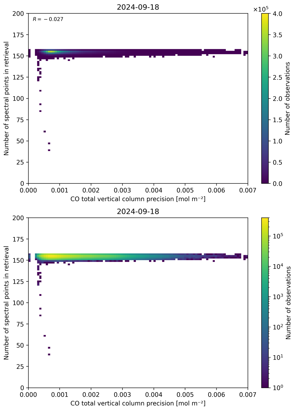
Figure 47: Scatter density plot of “CO total vertical column precision” against “Number of spectral points in retrieval” for 2024-09-17 to 2024-09-19.
