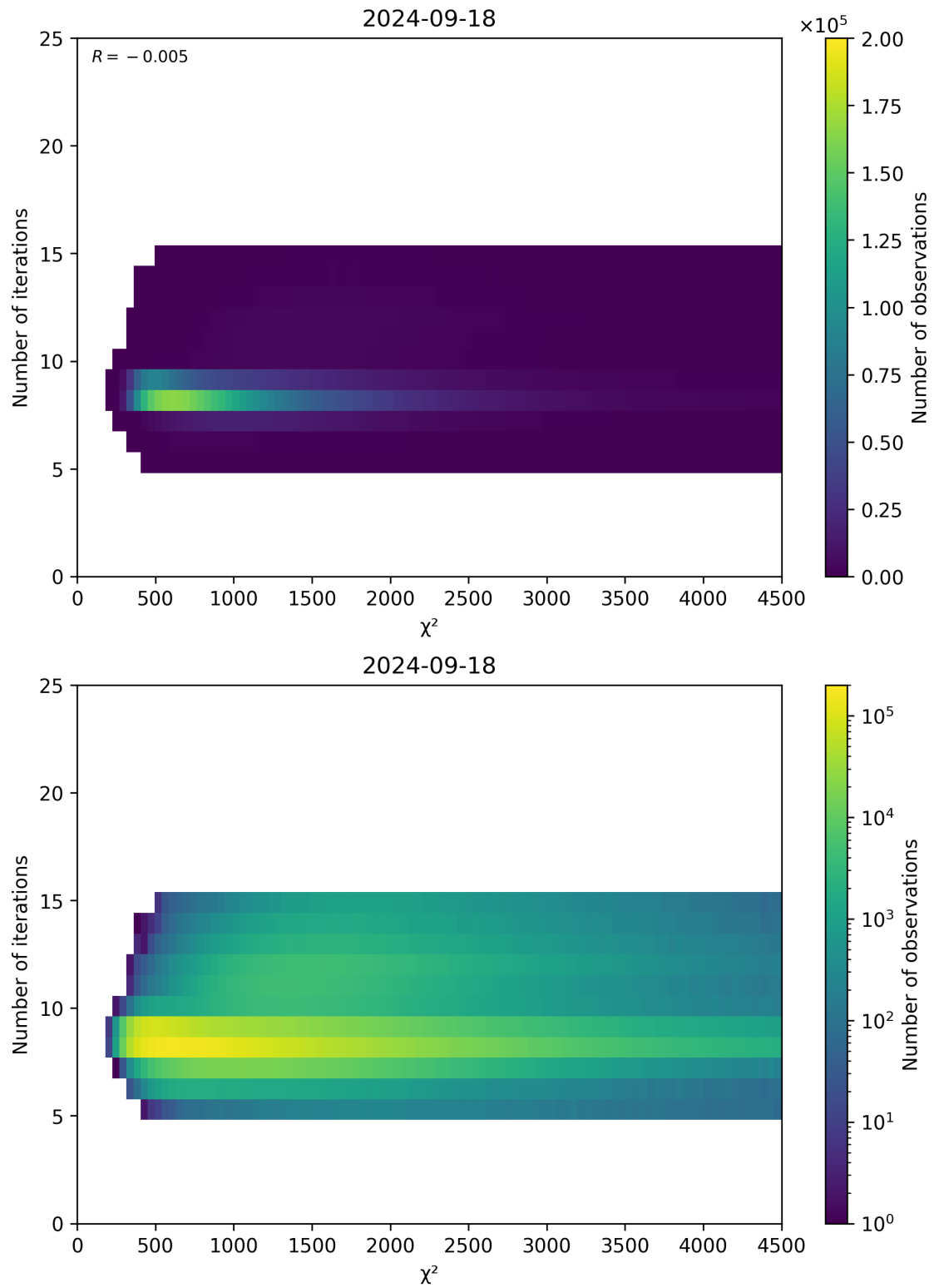
Figure 49: Scatter density plot of “ \chi^2 ” against “Number of iterations” for 2024-09-17 to 2024-09-19.
