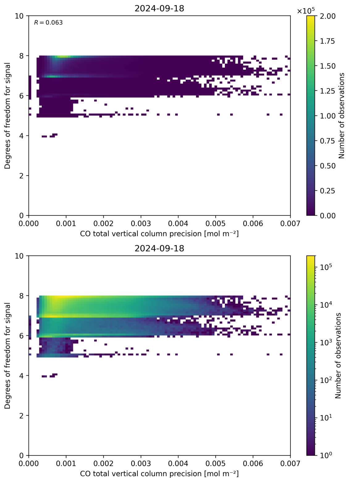
Figure 45: Scatter density plot of “CO total vertical column precision” against “Degrees of freedom for signal” for 2024-09-17 to 2024-09-19.
