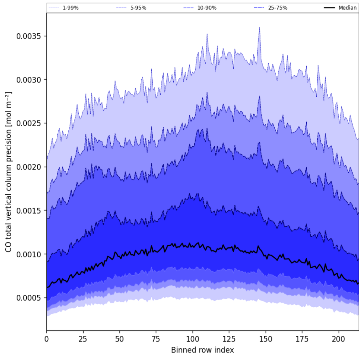
Figure 28: Along track statistics of “CO total vertical column precision” for 2024-09-17 to 2024-09-19
