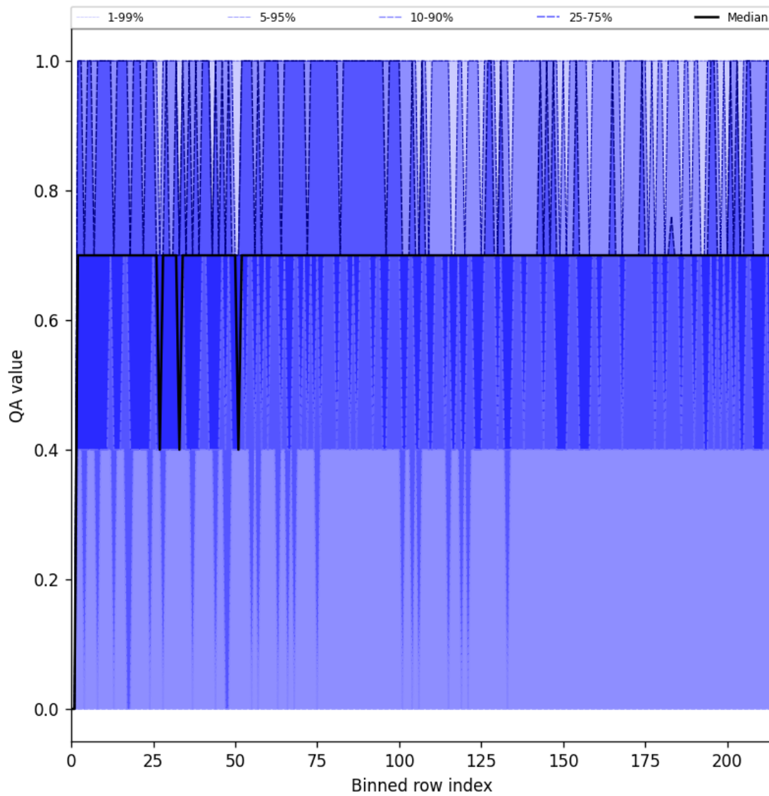
Figure 25: Along track statistics of “QA value” for 2024-09-17 to 2024-09-19
