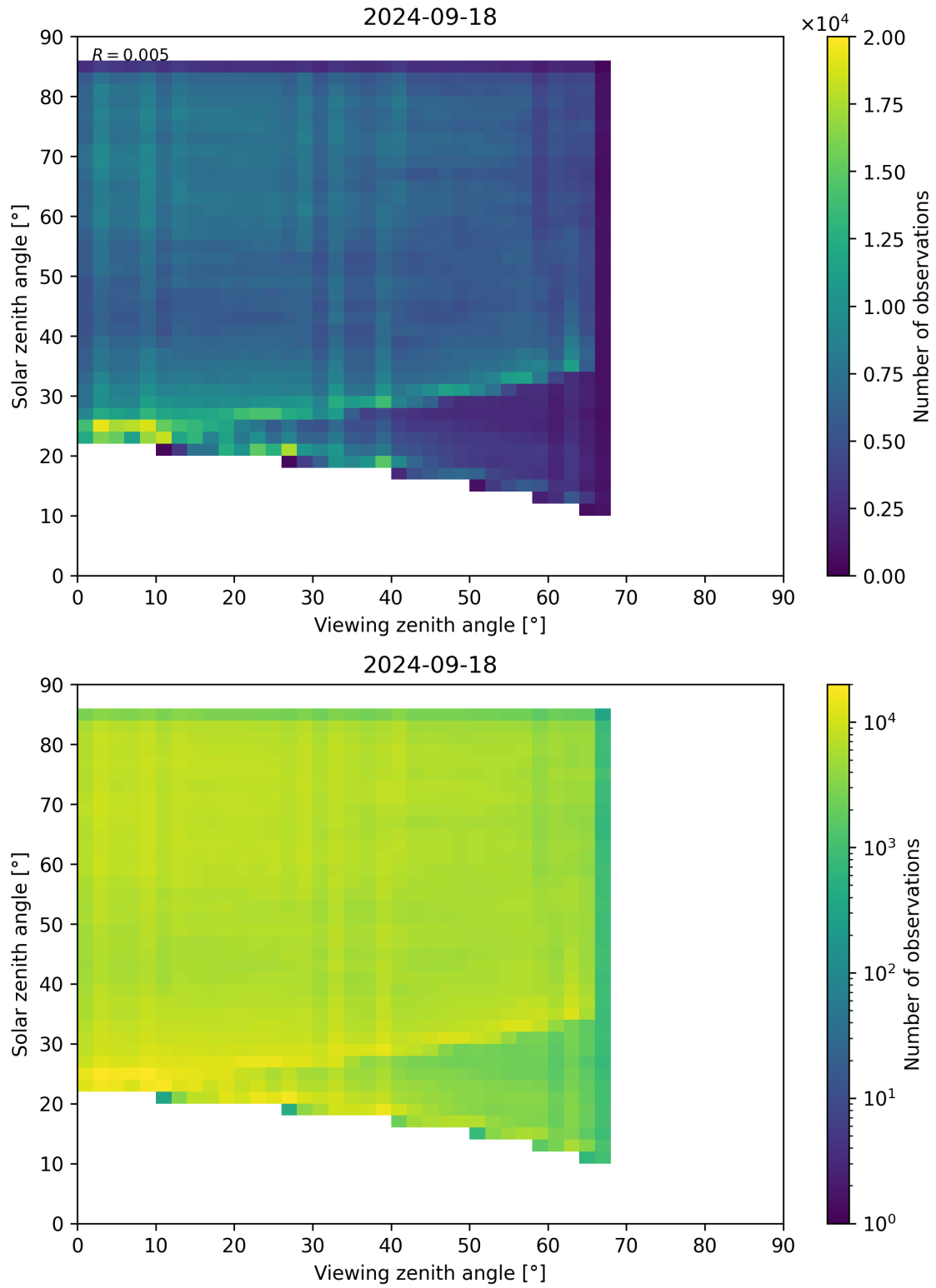
Figure 77: Scatter density plot of “Viewing zenith angle” against “Solar zenith angle” for 2024-09-17 to 2024-09-19.
