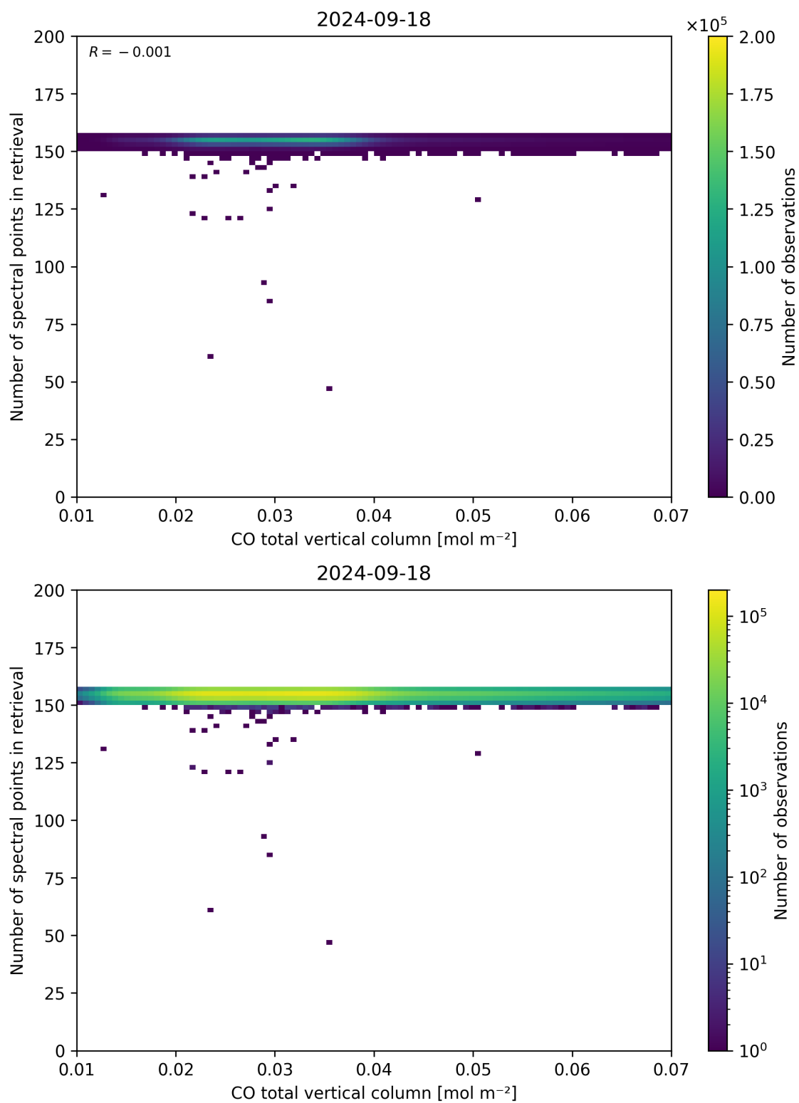
Figure 43: Scatter density plot of “CO total vertical column” against “Number of spectral points in retrieval” for 2024-09-17 to 2024-09-19.
