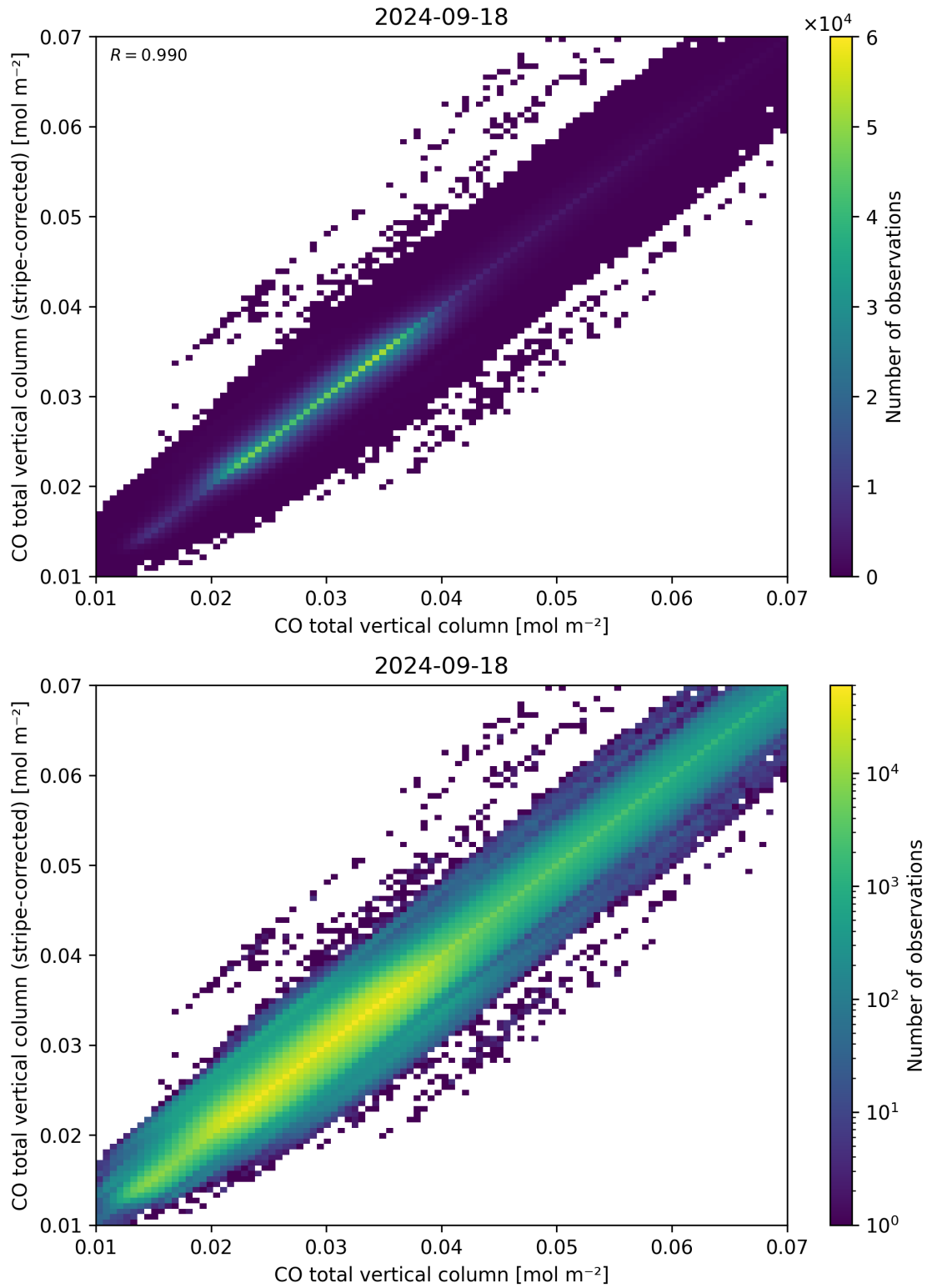
Figure 33: Scatter density plot of “CO total vertical column” against “CO total vertical column (stripe-corrected)” for 2024-09-17 to 2024-09-19.
