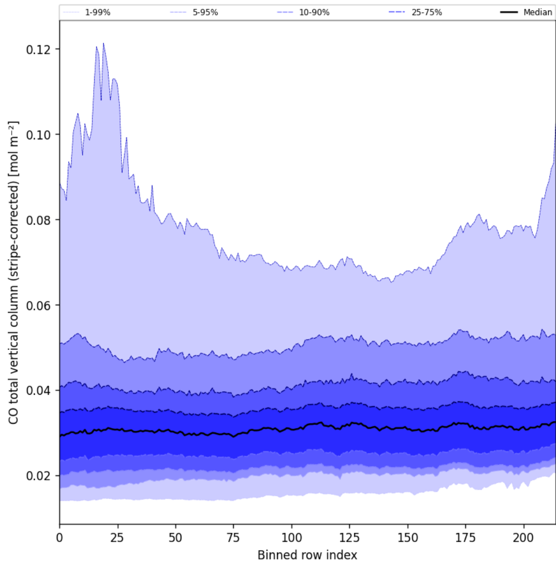
Figure 27: Along track statistics of “CO total vertical column (stripe-corrected)” for 2024-09-17 to 2024-09-19
