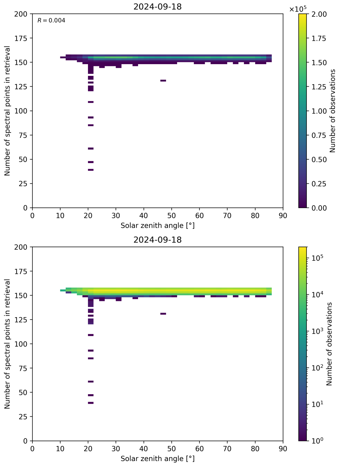
Figure 68: Scatter density plot of “Solar zenith angle” against “Number of spectral points in retrieval” for 2024-09-17 to 2024-09-19.
