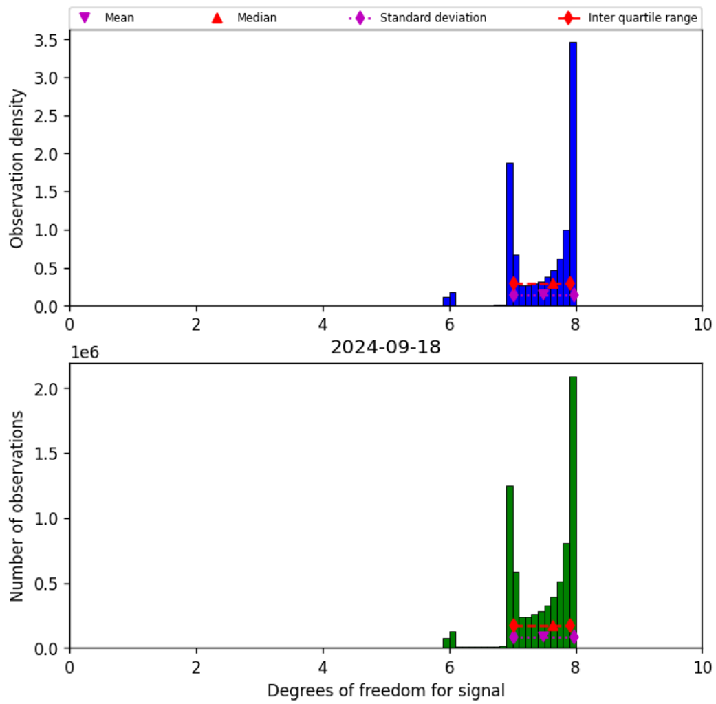
Figure 23: Histogram of “Degrees of freedom for signal” for 2024-09-17 to 2024-09-19
