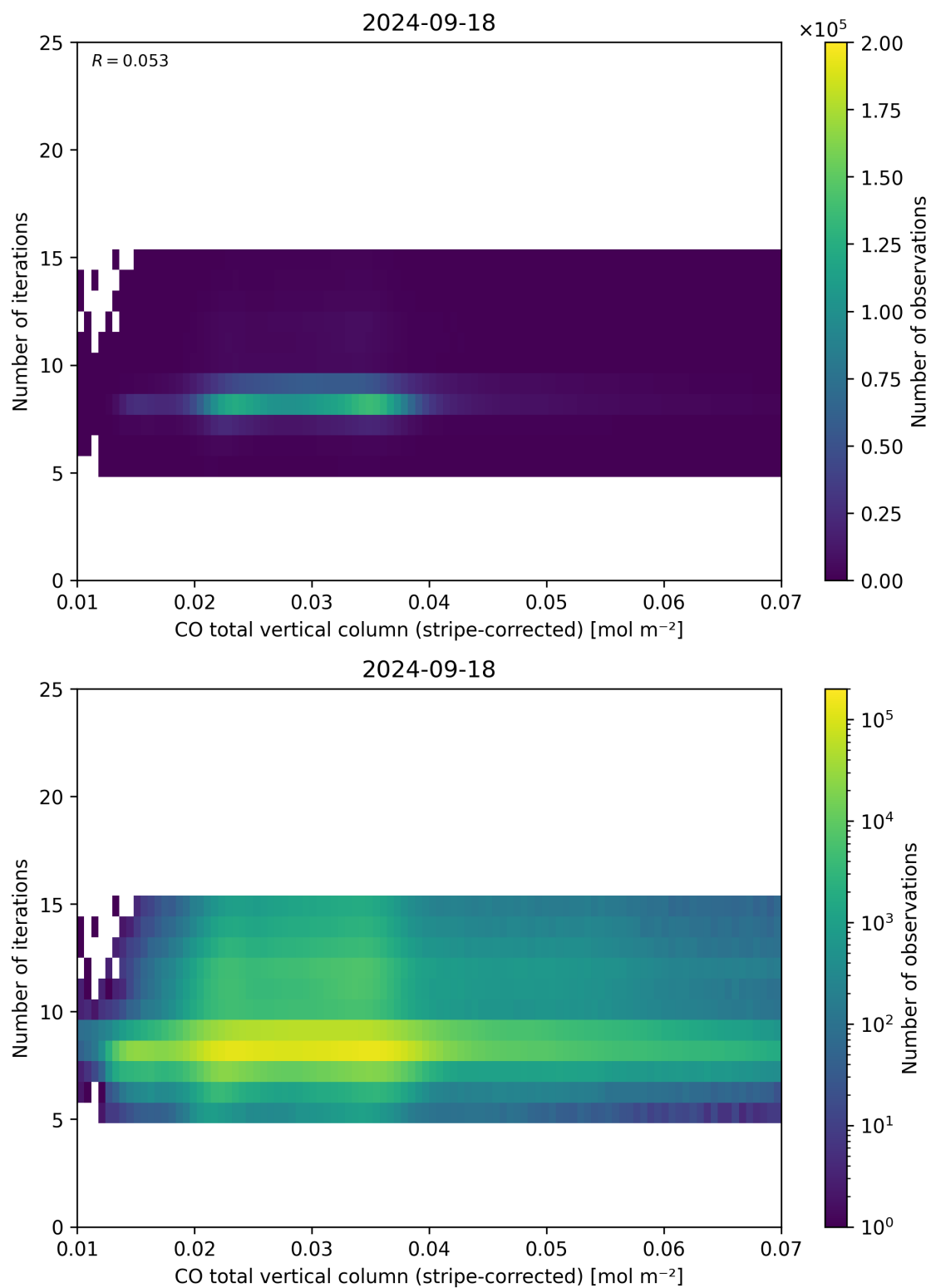
Figure 39: Scatter density plot of “CO total vertical column (stripe-corrected)” against “Number of iterations” for 2024-09-17 to 2024-09-19.
