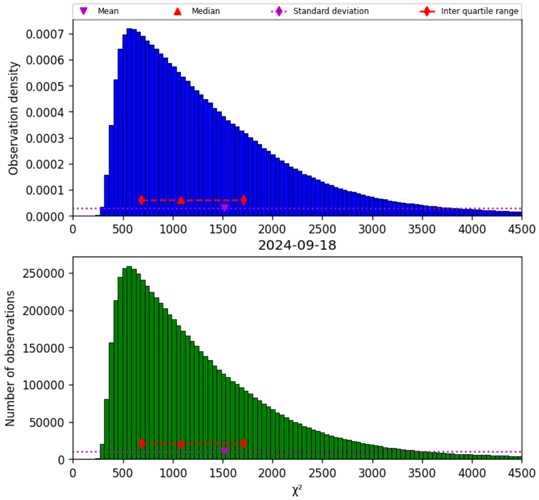
Figure 22: Histogram of “ \chi^2 ” for 2024-09-17 to 2024-09-19
