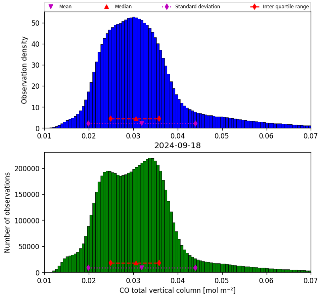
Figure 18: Histogram of “CO total vertical column” for 2024-09-17 to 2024-09-19
