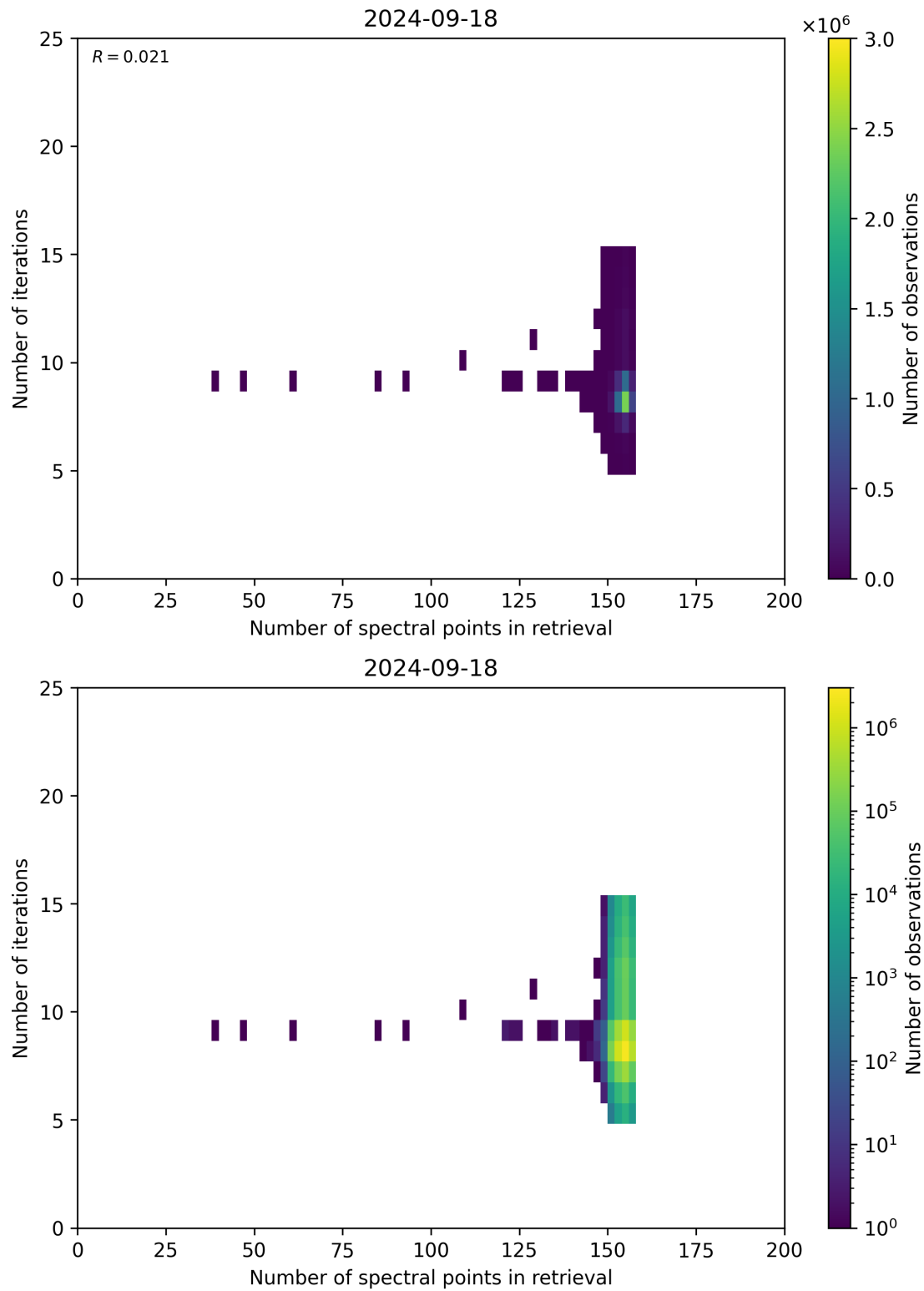
Figure 60: Scatter density plot of “Number of spectral points in retrieval” against “Number of iterations” for 2024-09-17 to 2024-09-19.
