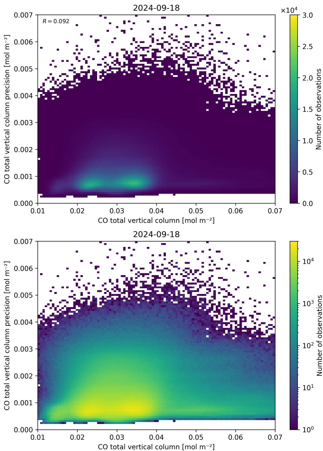
Figure 34: Scatter density plot of “CO total vertical column” against “CO total vertical column precision” for 2024-09-17 to 2024-09-19.
