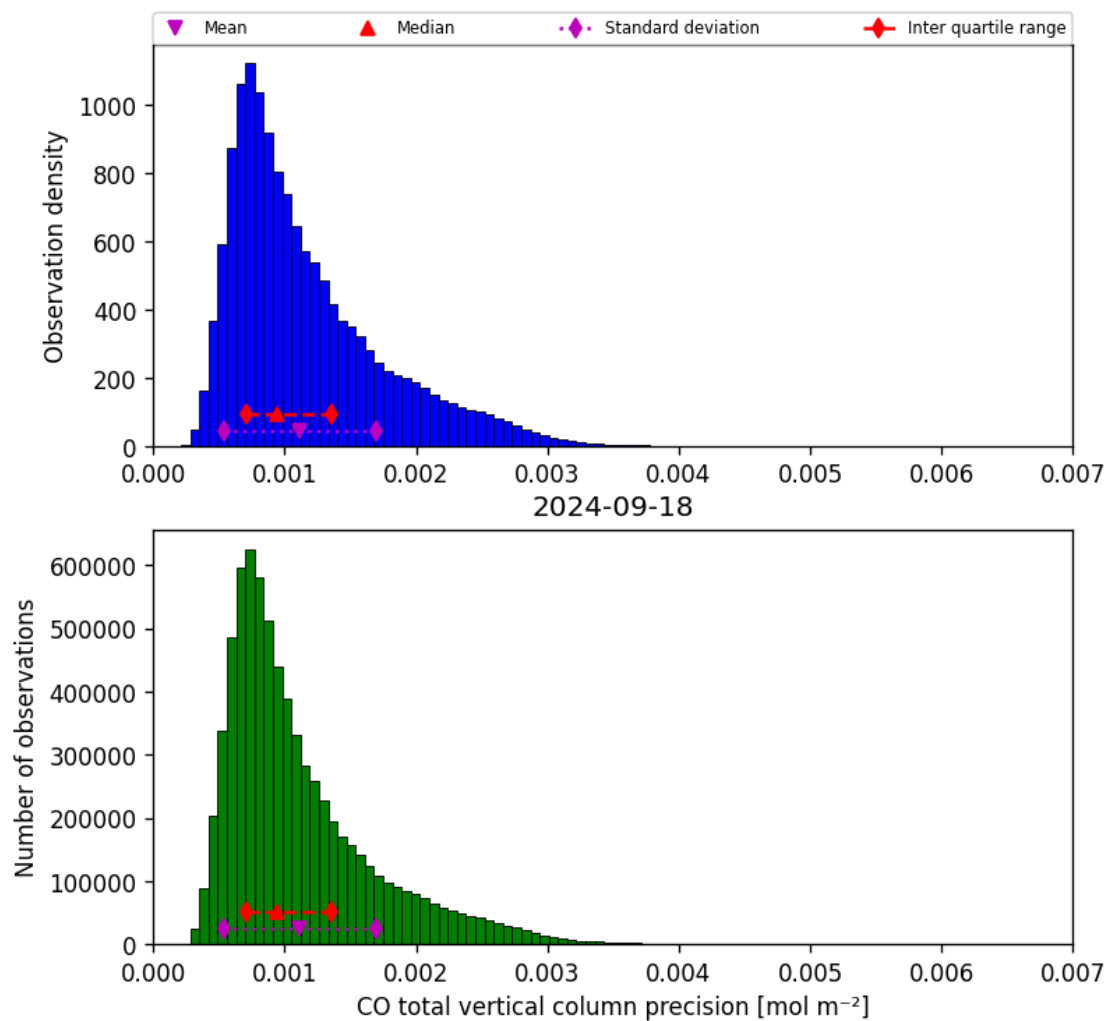
Figure 20: Histogram of “CO total vertical column precision” for 2024-09-17 to 2024-09-19
