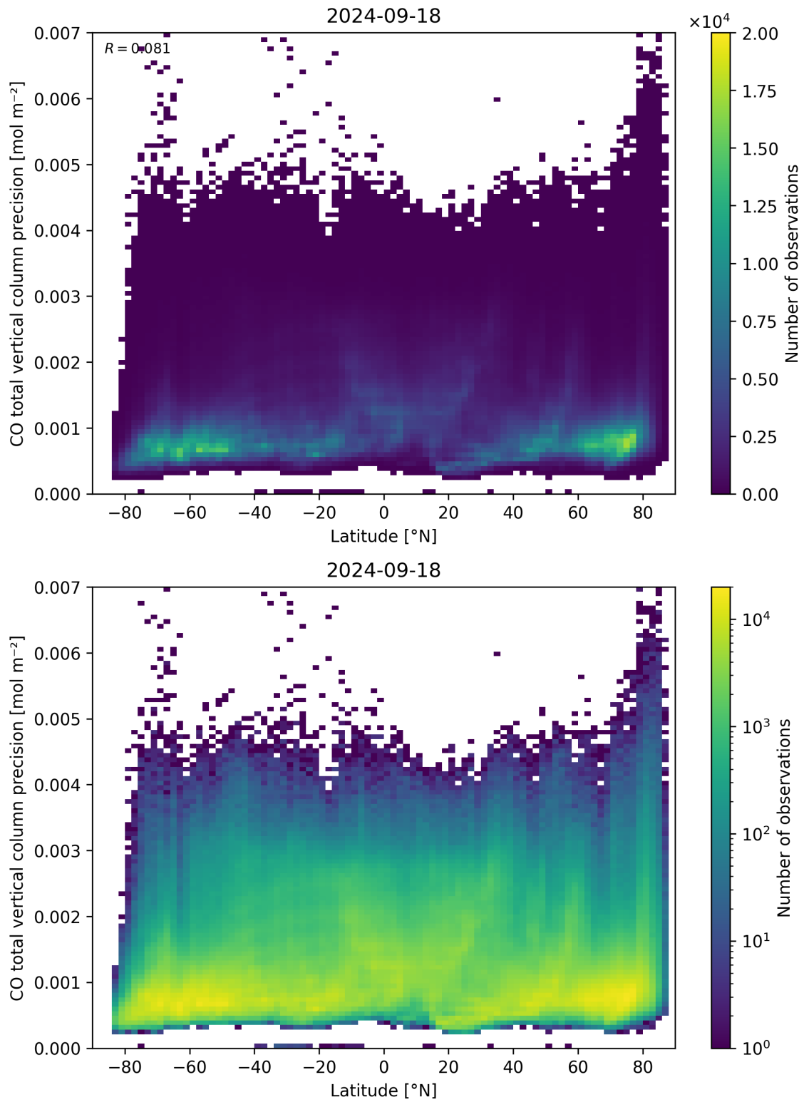
Figure 53: Scatter density plot of “Latitude” against “CO total vertical column precision” for 2024-09-17 to 2024-09-19.
