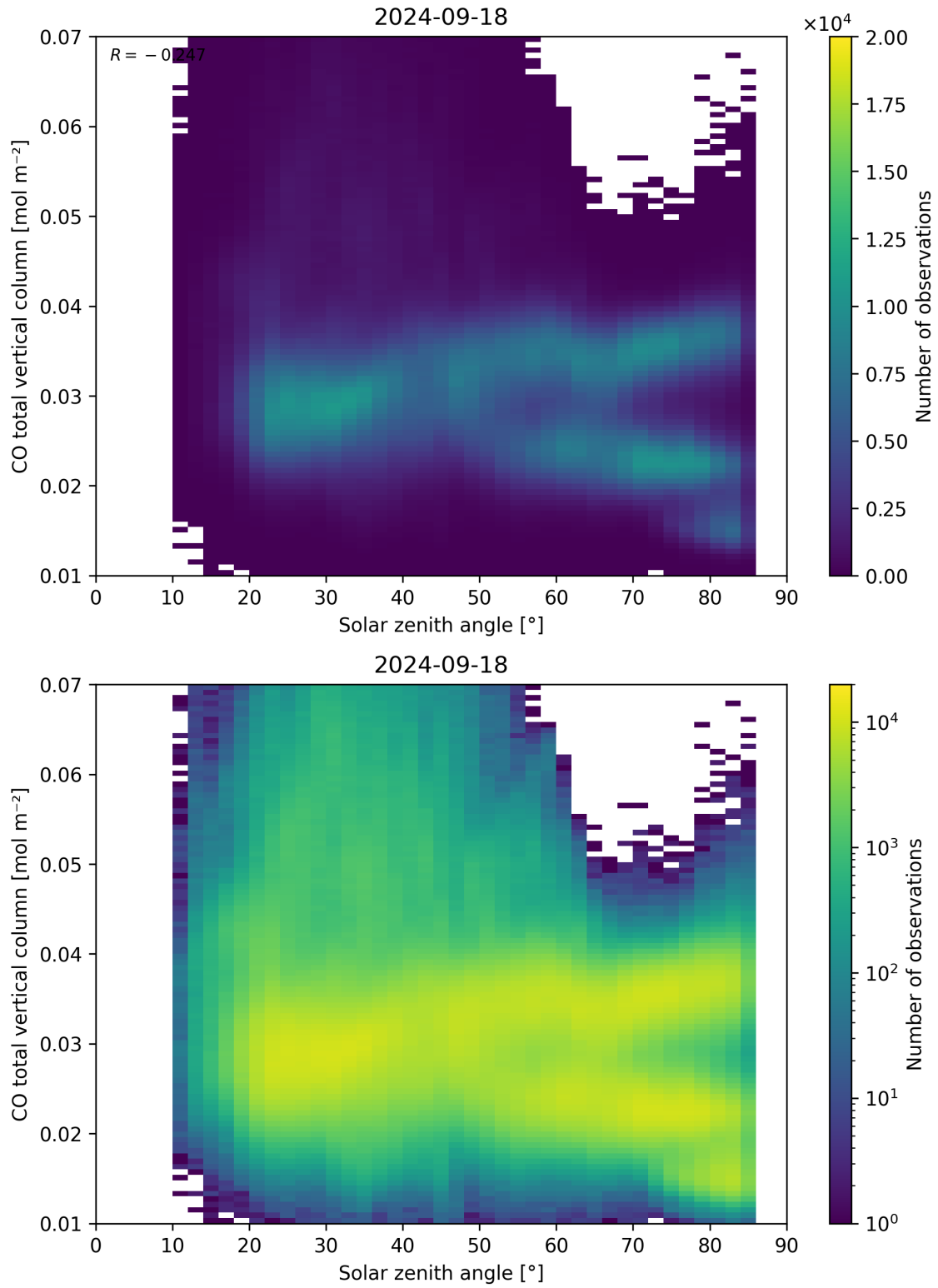
Figure 61: Scatter density plot of “Solar zenith angle” against “CO total vertical column” for 2024-09-17 to 2024-09-19.
