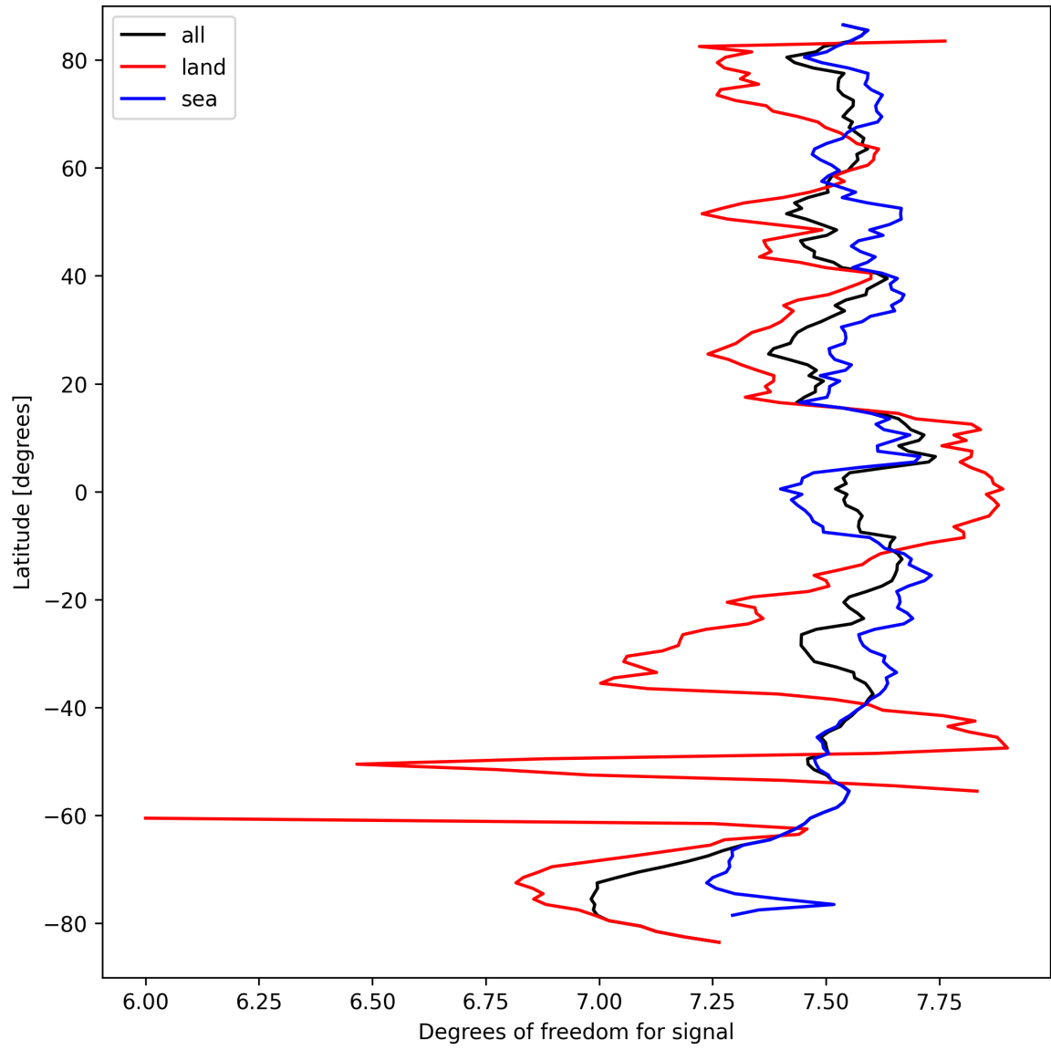
Figure 15: Zonal average of “Degrees of freedom for signal” for 2024-09-17 to 2024-09-19.
