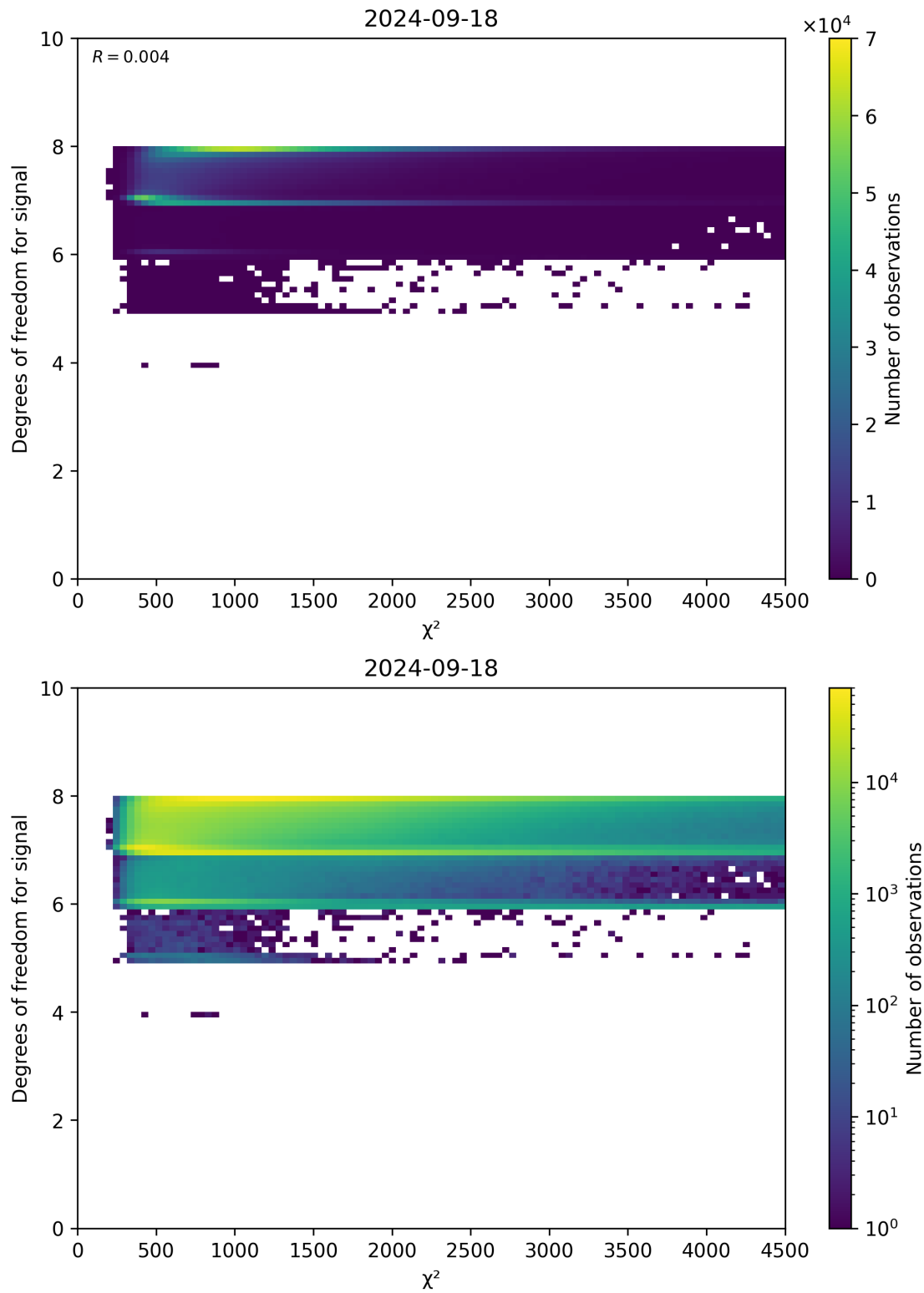
Figure 48: Scatter density plot of “ \chi^2 ” against “Degrees of freedom for signal” for 2024-09-17 to 2024-09-19.
