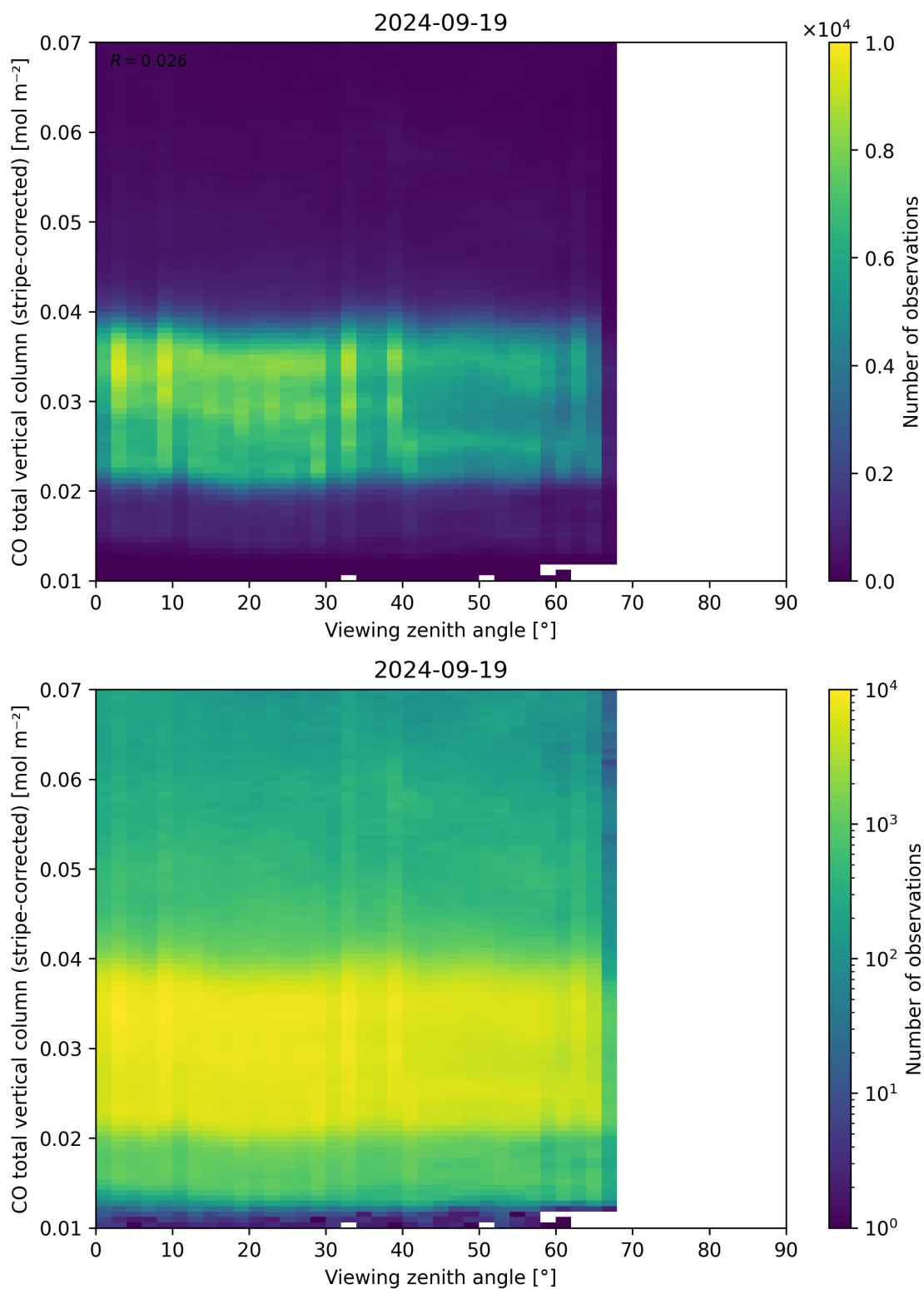
Figure 70: Scatter density plot of “Viewing zenith angle” against “CO total vertical column (stripe-corrected)” for 2024-09-18 to 2024-09-20.
