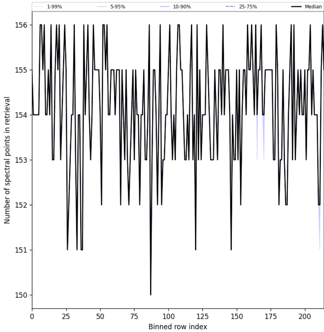
Figure 29: Along track statistics of “Number of spectral points in retrieval” for 2024-09-18 to 2024-09-20
