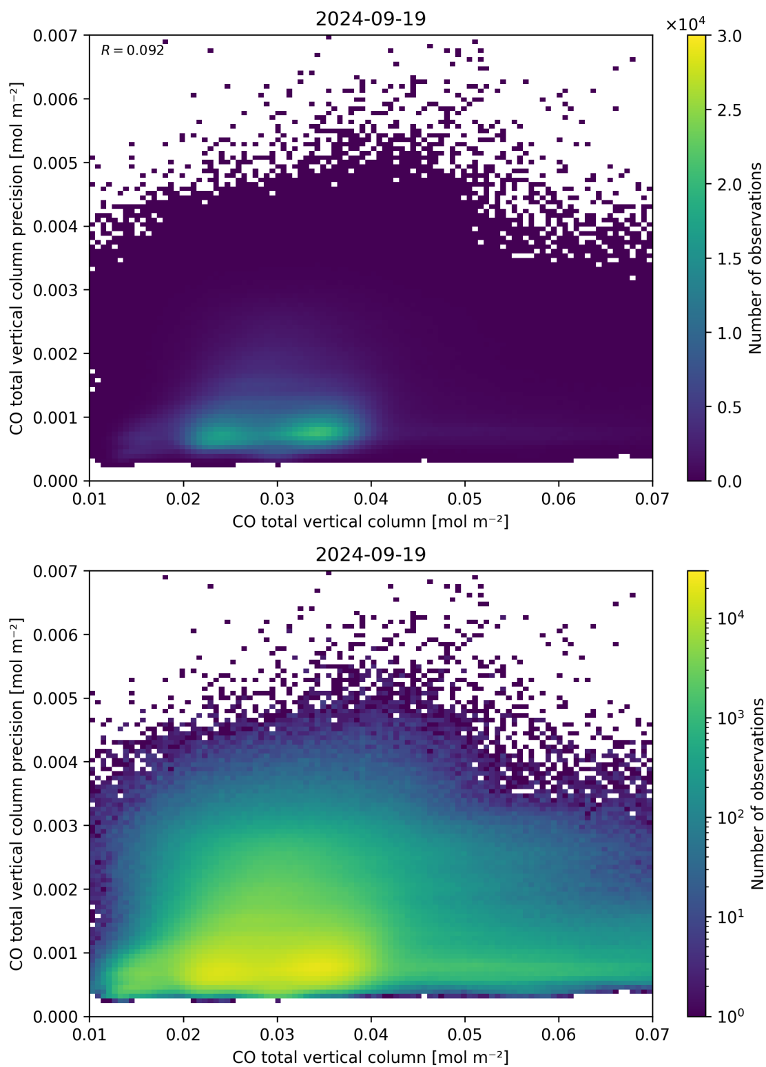
Figure 34: Scatter density plot of “CO total vertical column” against “CO total vertical column precision” for 2024-09-18 to 2024-09-20.
