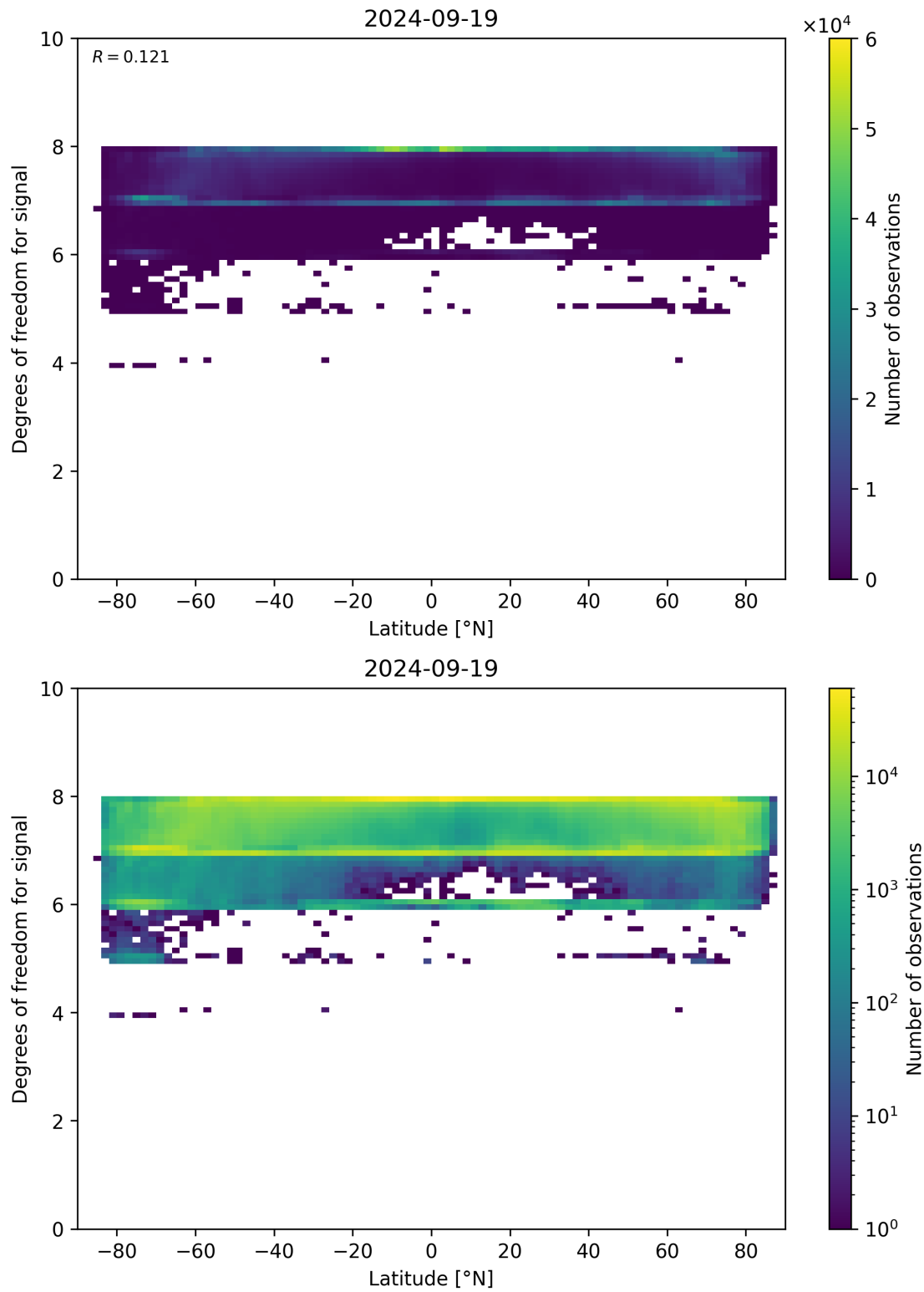
Figure 55: Scatter density plot of “Latitude” against “Degrees of freedom for signal” for 2024-09-18 to 2024-09-20.
