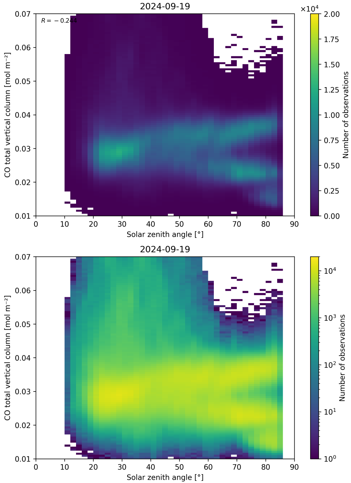
Figure 61: Scatter density plot of “Solar zenith angle” against “CO total vertical column” for 2024-09-18 to 2024-09-20.
