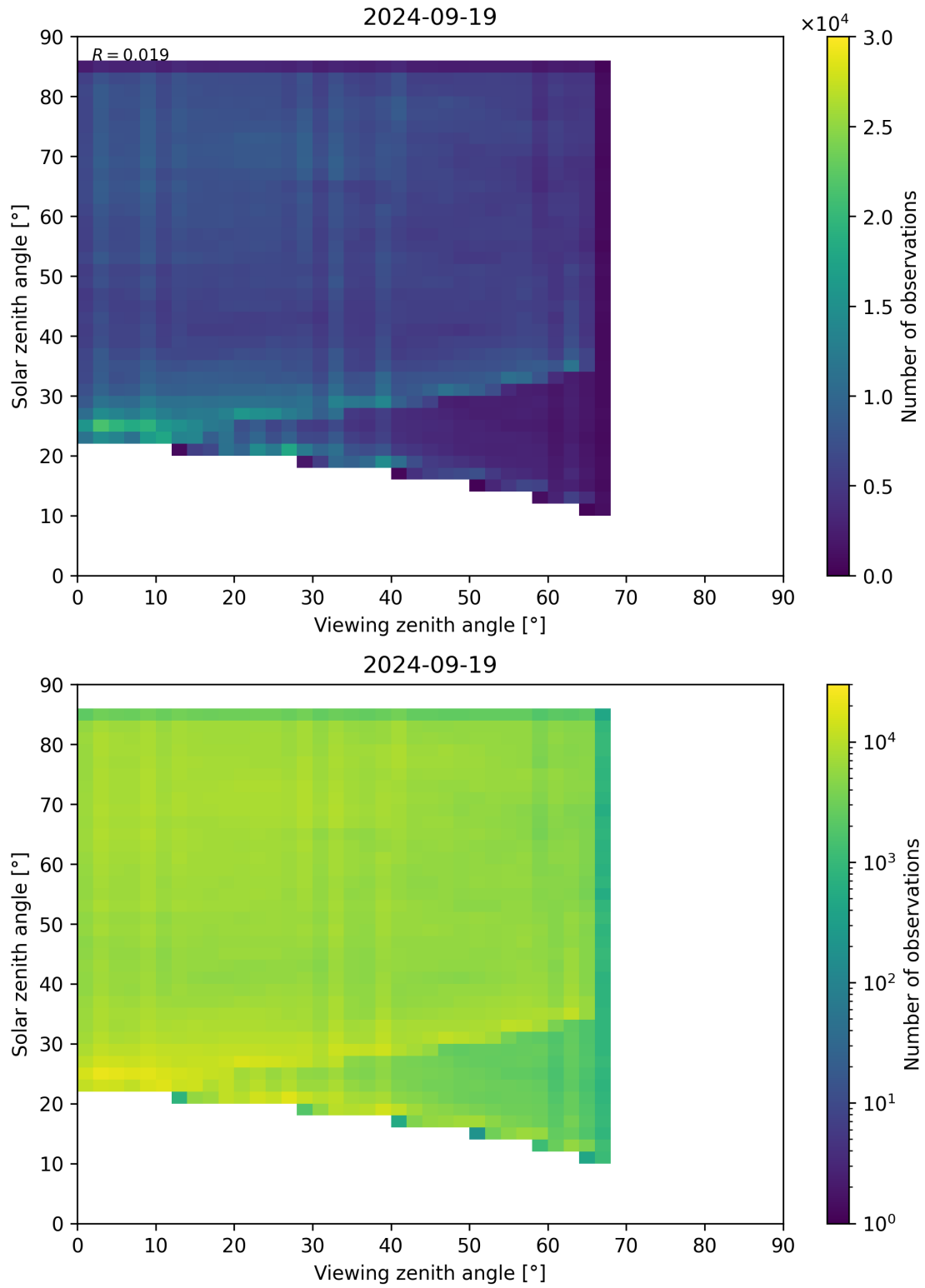
Figure 77: Scatter density plot of “Viewing zenith angle” against “Solar zenith angle” for 2024-09-18 to 2024-09-20.
