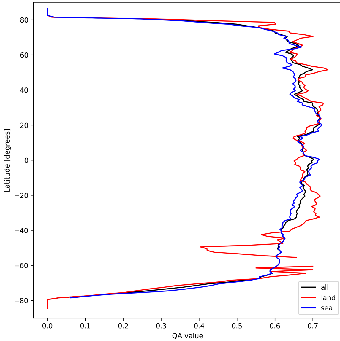
Figure 9: Zonal average of “QA value” for 2024-09-18 to 2024-09-20.
