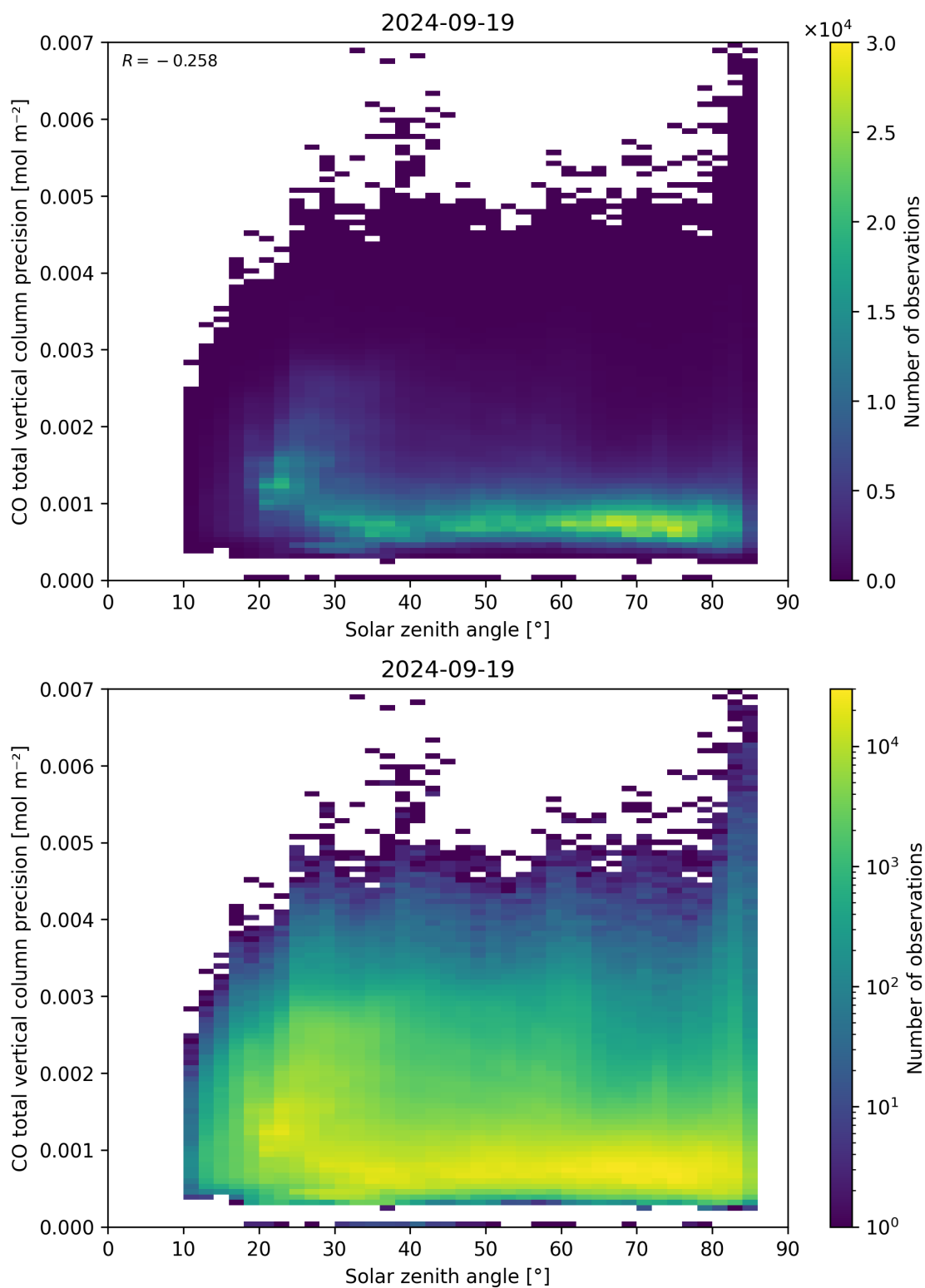
Figure 63: Scatter density plot of “Solar zenith angle” against “CO total vertical column precision” for 2024-09-18 to 2024-09-20.
