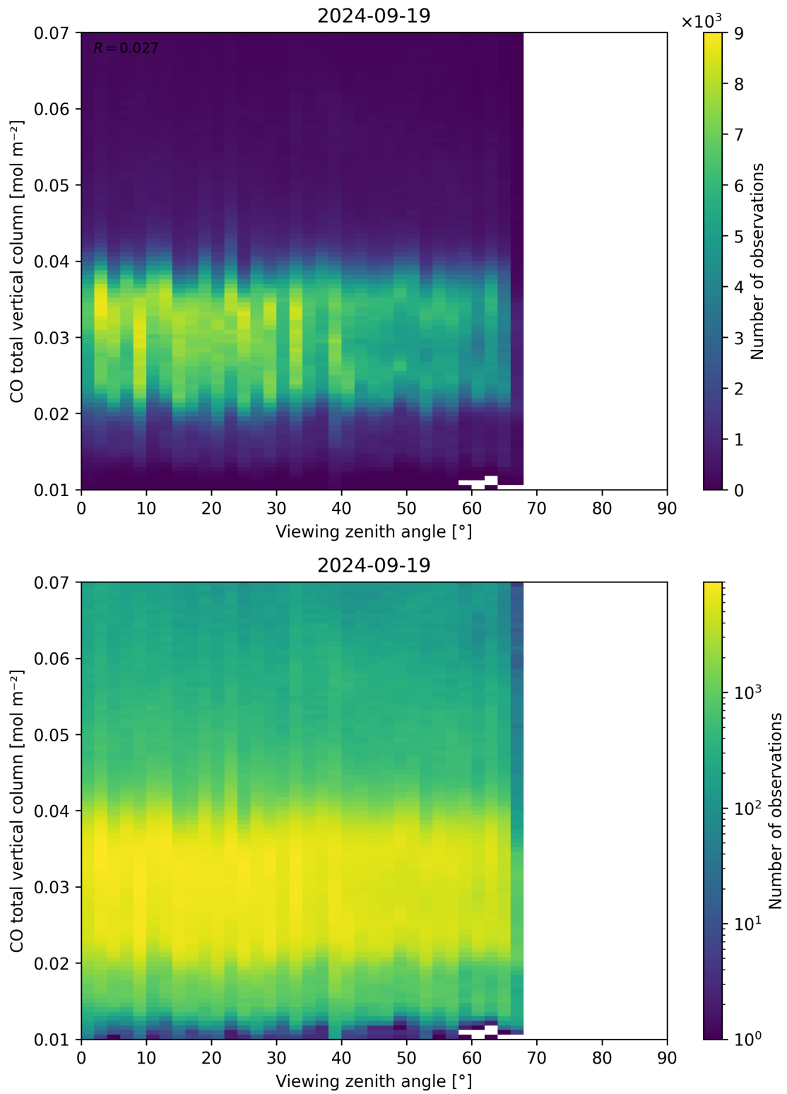
Figure 69: Scatter density plot of “Viewing zenith angle” against “CO total vertical column” for 2024-09-18 to 2024-09-20.
