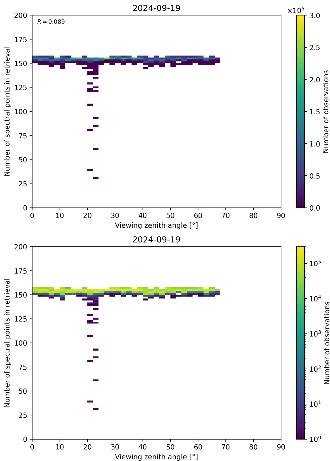
Figure 76: Scatter density plot of “Viewing zenith angle” against “Number of spectral points in retrieval” for 2024-09-18 to 2024-09-20.
