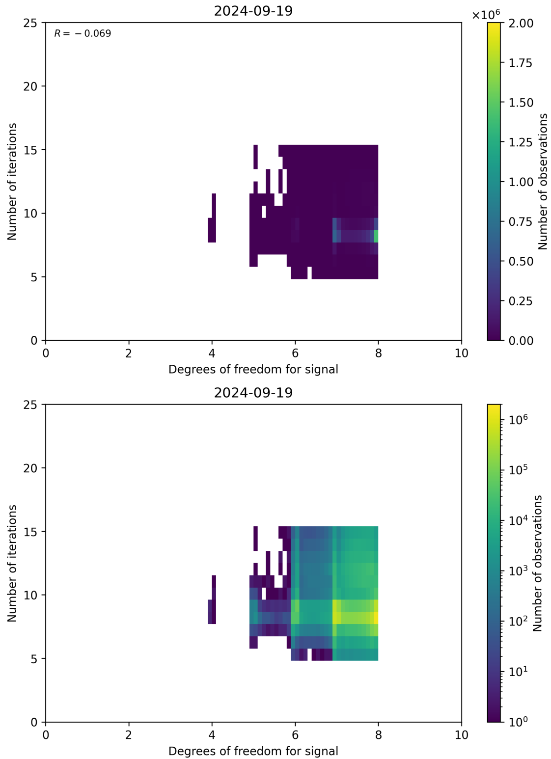
Figure 50: Scatter density plot of “Degrees of freedom for signal” against “Number of iterations” for 2024-09-18 to 2024-09-20.
