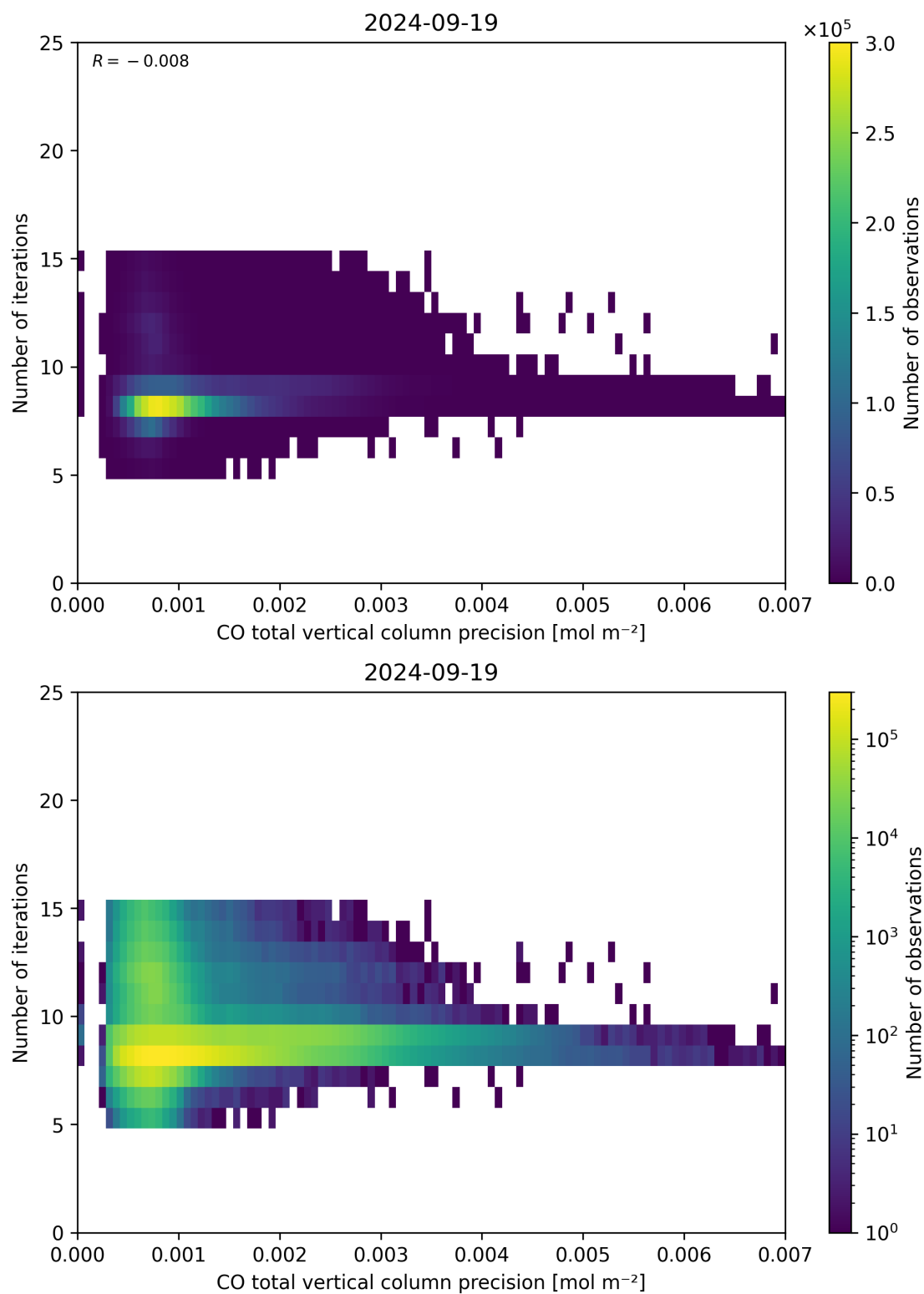
Figure 46: Scatter density plot of “CO total vertical column precision” against “Number of iterations” for 2024-09-18 to 2024-09-20.
