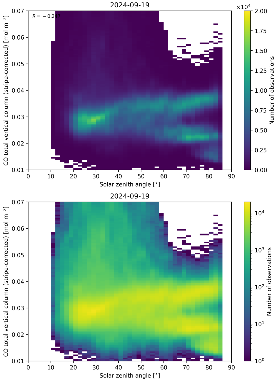
Figure 62: Scatter density plot of “Solar zenith angle” against “CO total vertical column (stripe-corrected)” for 2024-09-18 to 2024-09-20.
