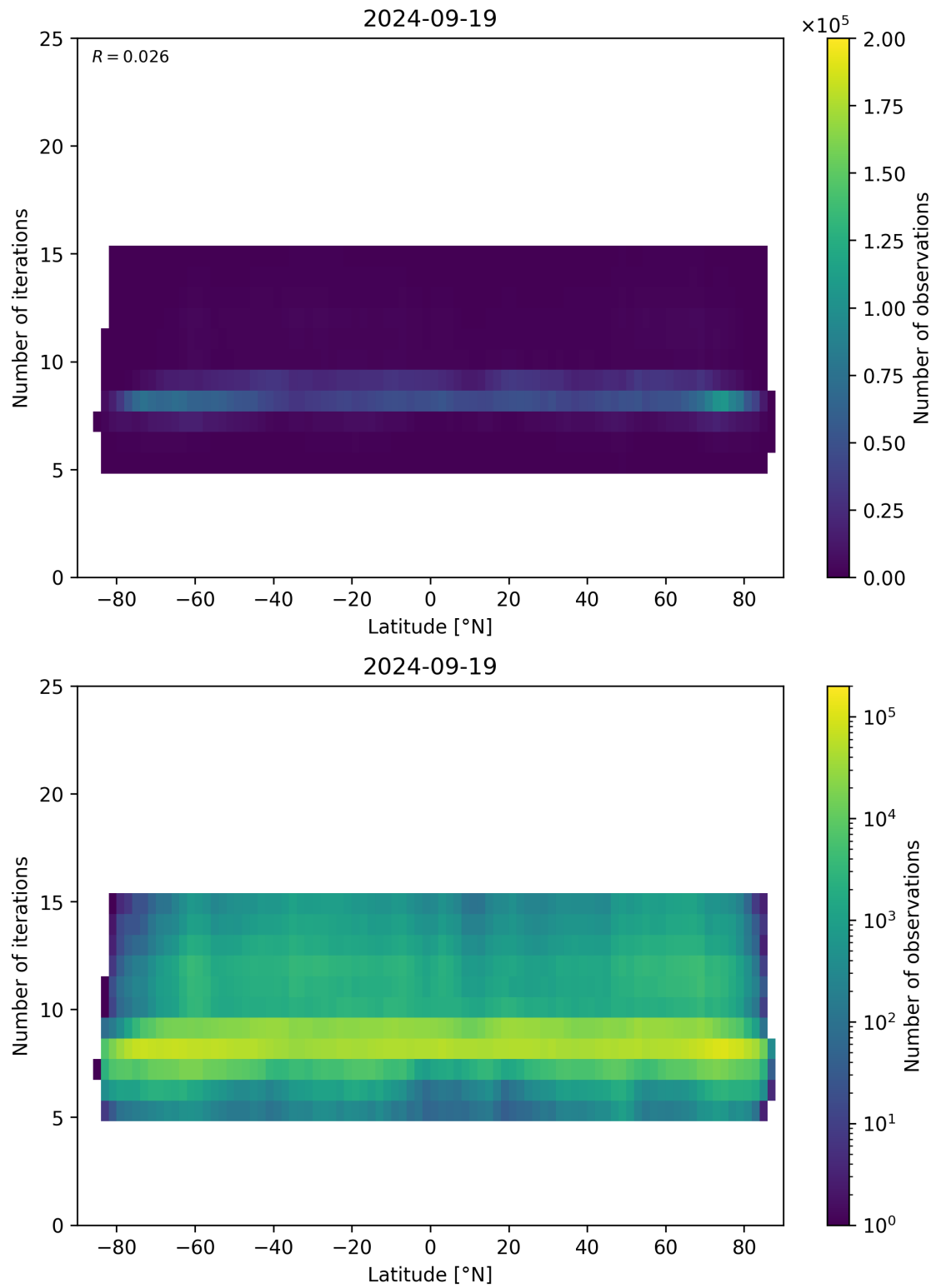
Figure 56: Scatter density plot of “Latitude” against “Number of iterations” for 2024-09-18 to 2024-09-20.
