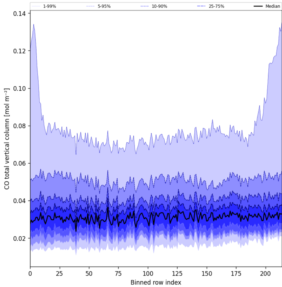
Figure 26: Along track statistics of “CO total vertical column” for 2024-09-18 to 2024-09-20
