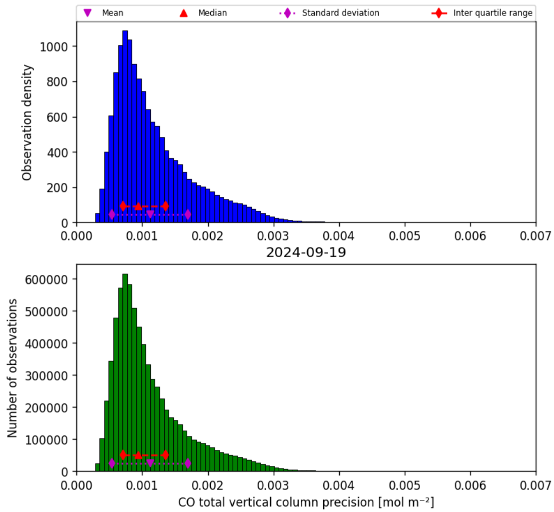
Figure 20: Histogram of “CO total vertical column precision” for 2024-09-18 to 2024-09-20
