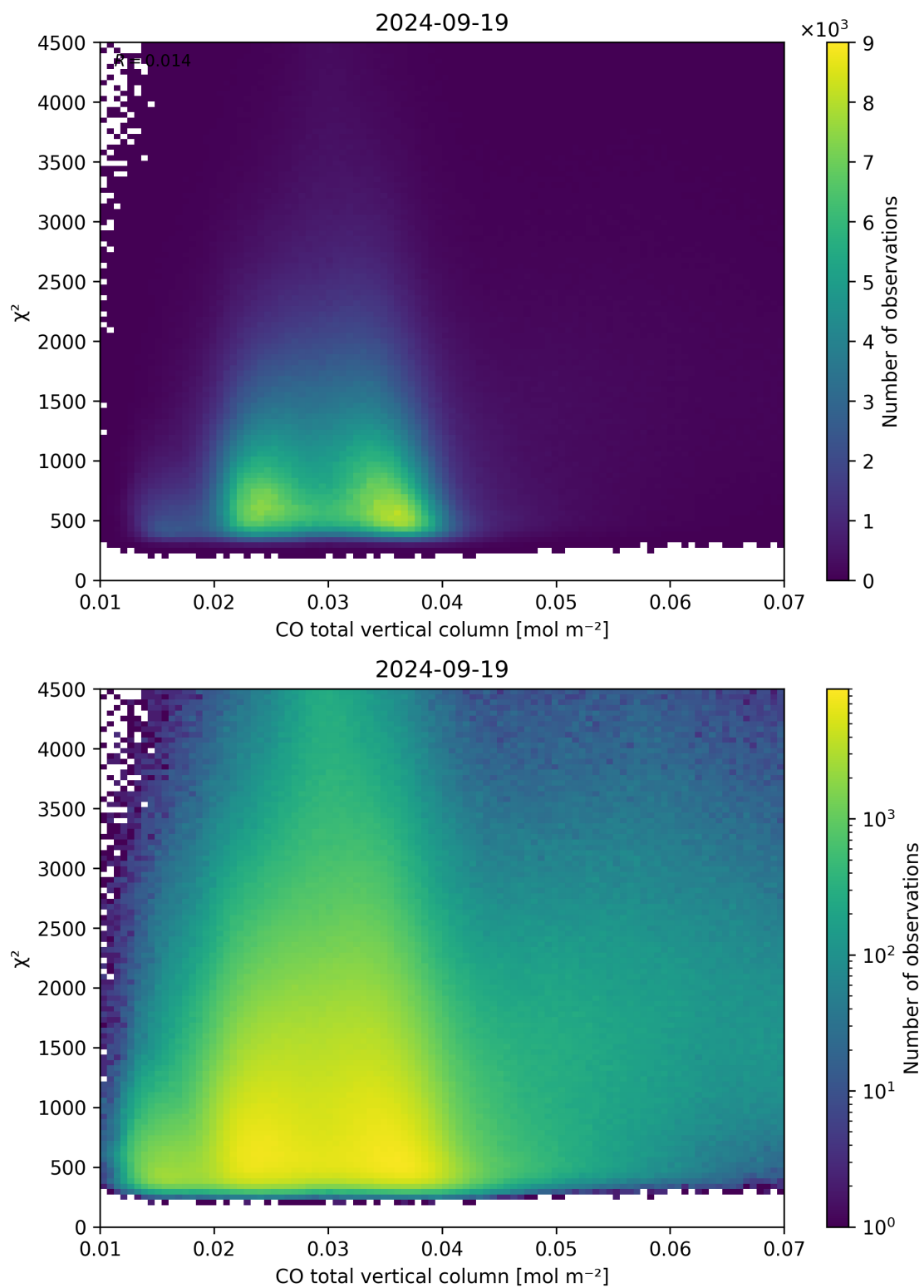
Figure 35: Scatter density plot of “CO total vertical column” against “ \chi^2 ” for 2024-09-18 to 2024-09-20.
