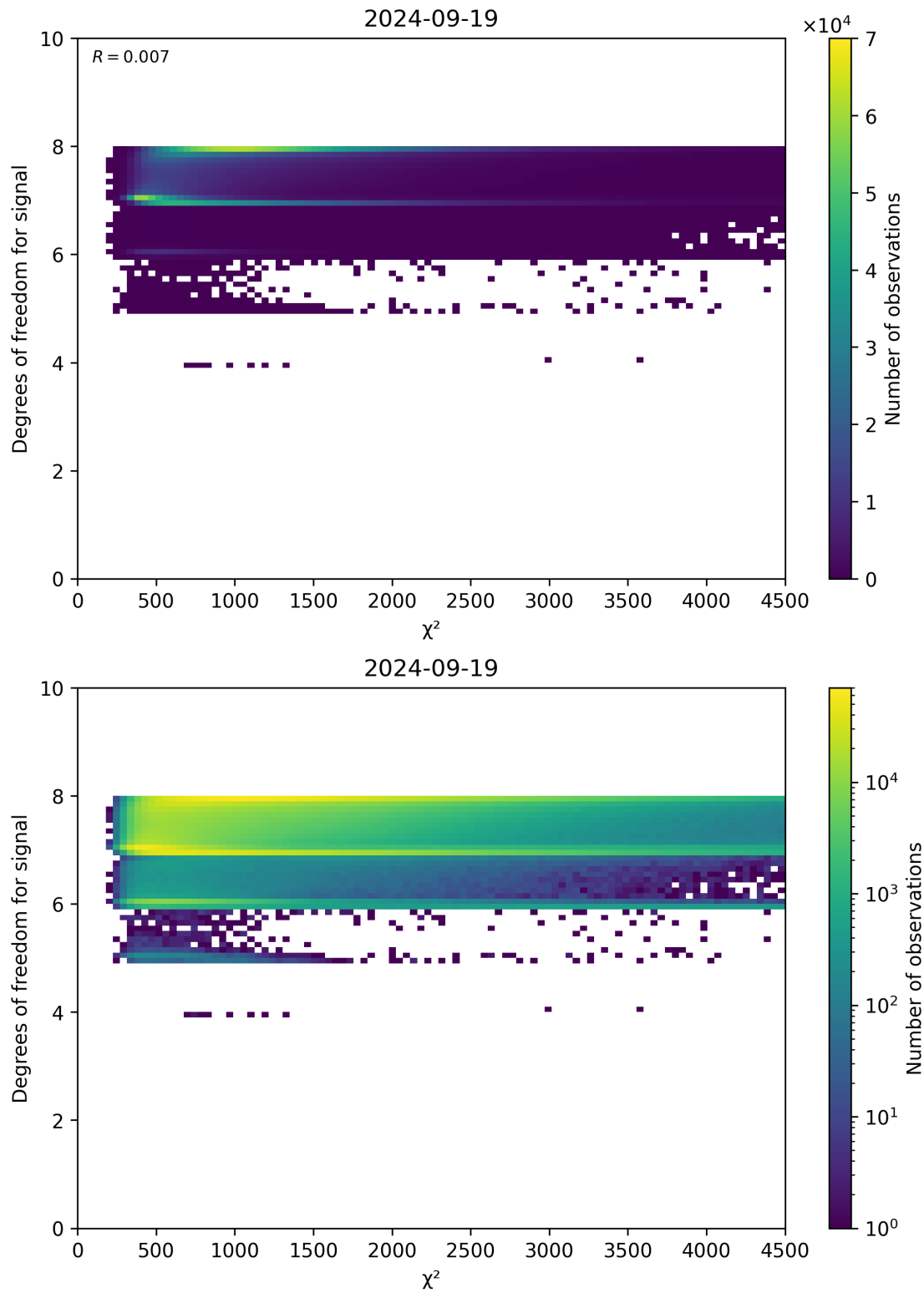
Figure 48: Scatter density plot of “ \chi^2 ” against “Degrees of freedom for signal” for 2024-09-18 to 2024-09-20.
