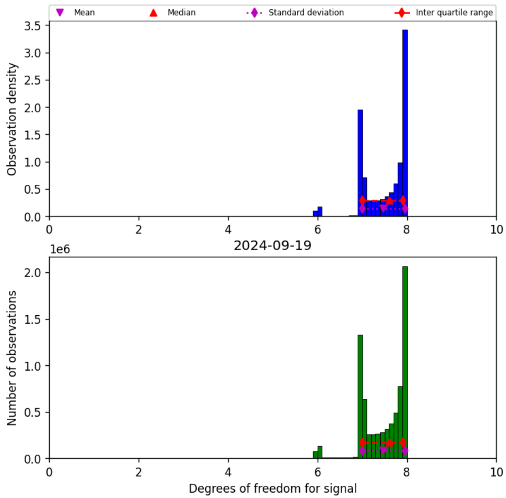
Figure 23: Histogram of “Degrees of freedom for signal” for 2024-09-18 to 2024-09-20
