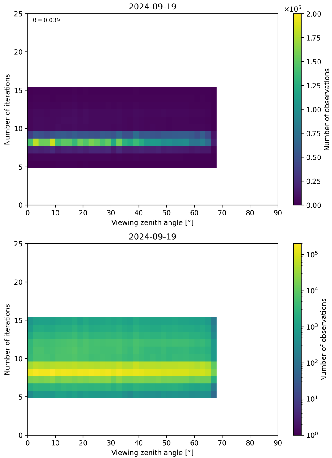
Figure 75: Scatter density plot of “Viewing zenith angle” against “Number of iterations” for 2024-09-18 to 2024-09-20.
