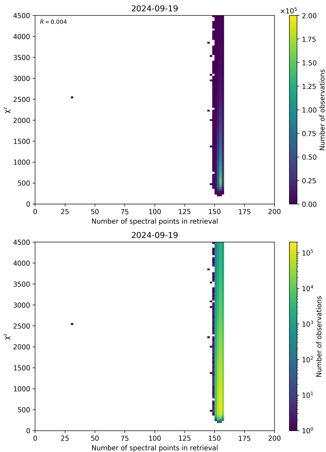
Figure 58: Scatter density plot of “Number of spectral points in retrieval” against “ \chi^2 ” for 2024-09-18 to 2024-09-20.
