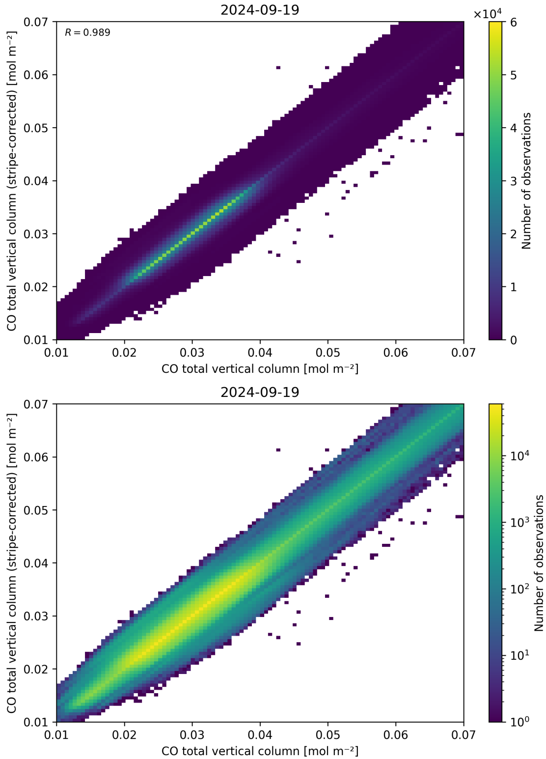
Figure 33: Scatter density plot of “CO total vertical column” against “CO total vertical column (stripe-corrected)” for 2024-09-18 to 2024-09-20.
