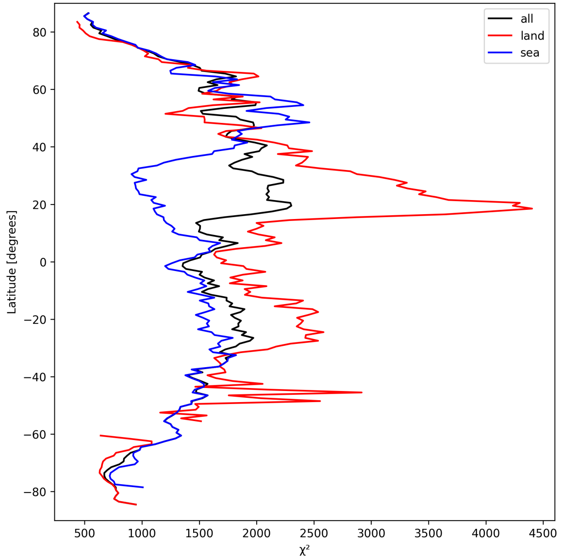
Figure 14: Zonal average of “ \chi^2 ” for 2024-09-18 to 2024-09-20.
