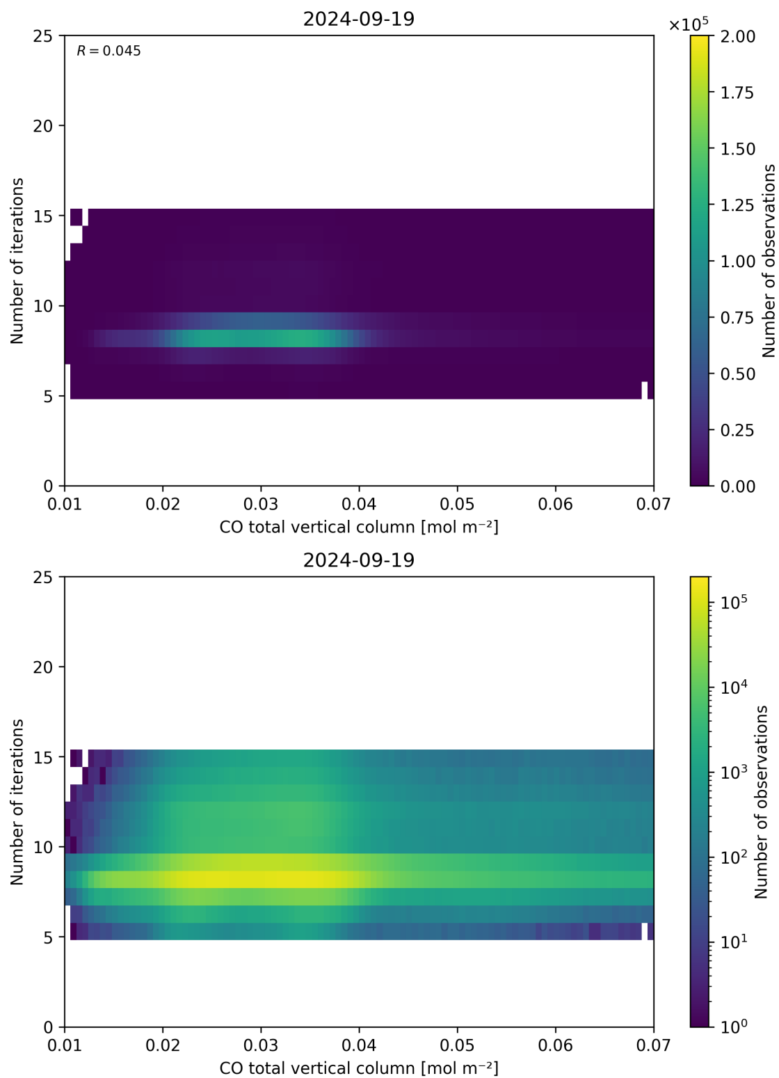
Figure 42: Scatter density plot of “CO total vertical column” against “Number of iterations” for 2024-09-18 to 2024-09-20.
