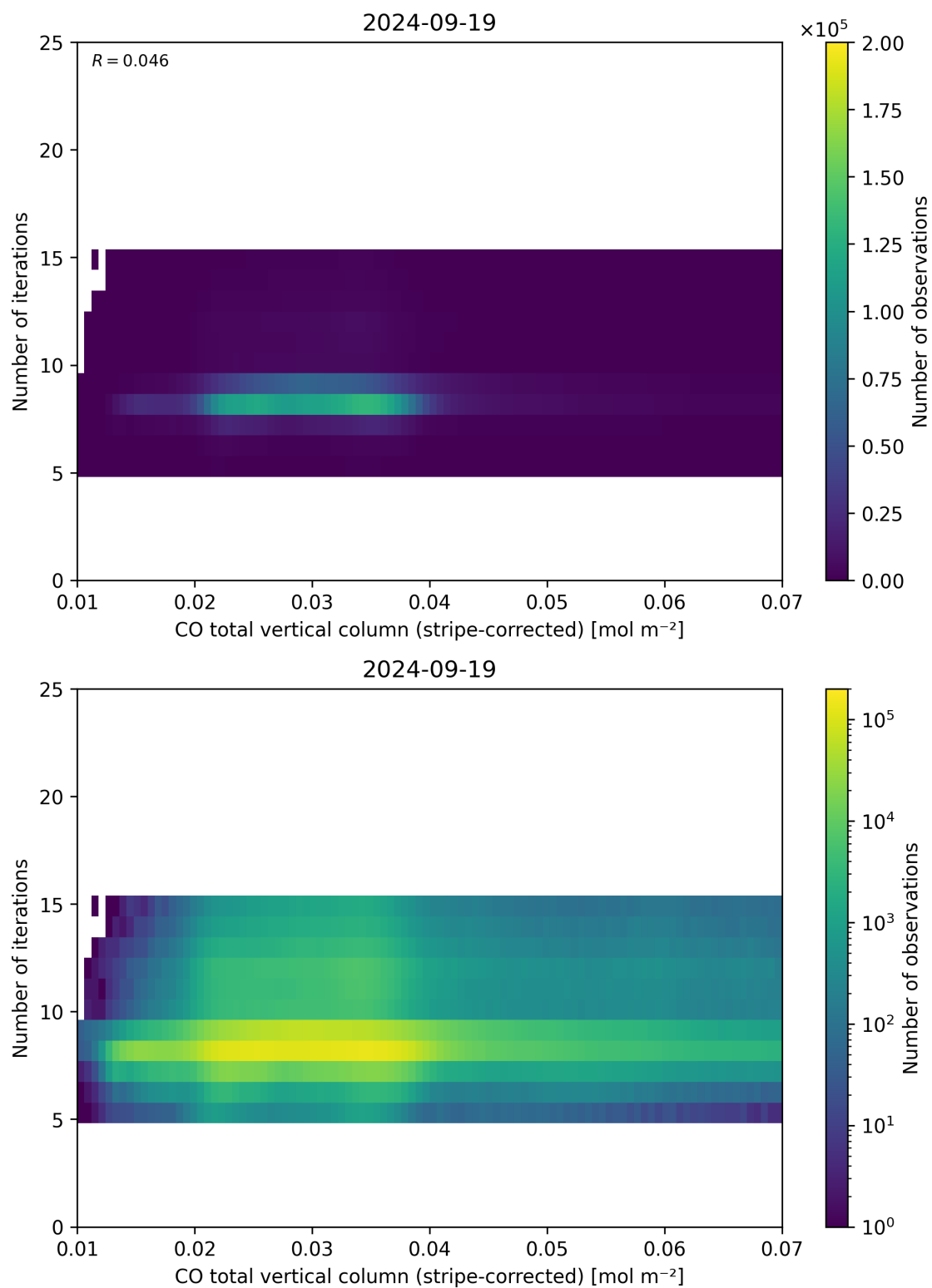
Figure 39: Scatter density plot of “CO total vertical column (stripe-corrected)” against “Number of iterations” for 2024-09-18 to 2024-09-20.
