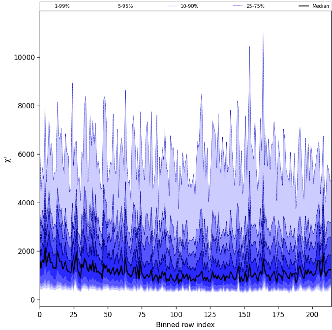
Figure 30: Along track statistics of “ \chi^2 ” for 2024-09-18 to 2024-09-20
