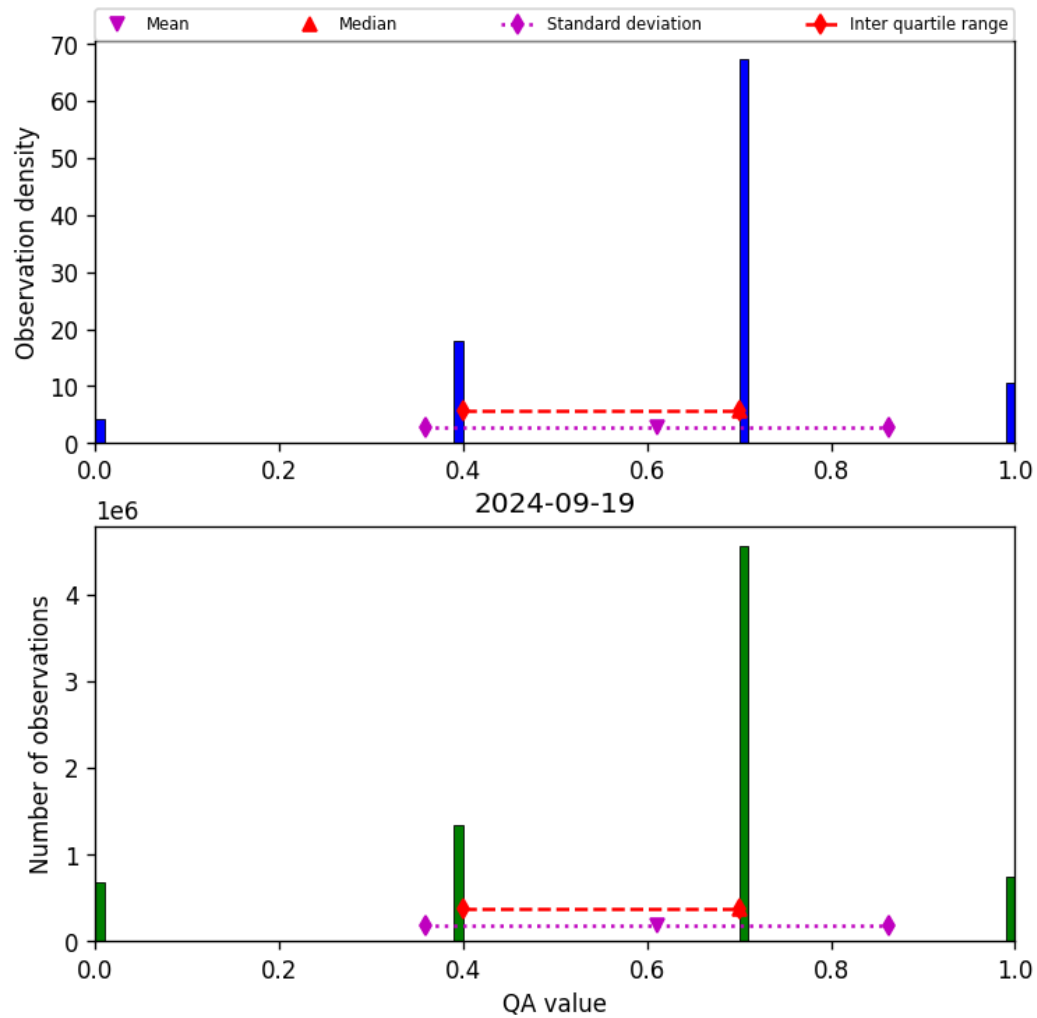
Figure 17: Histogram of “QA value” for 2024-09-18 to 2024-09-20
