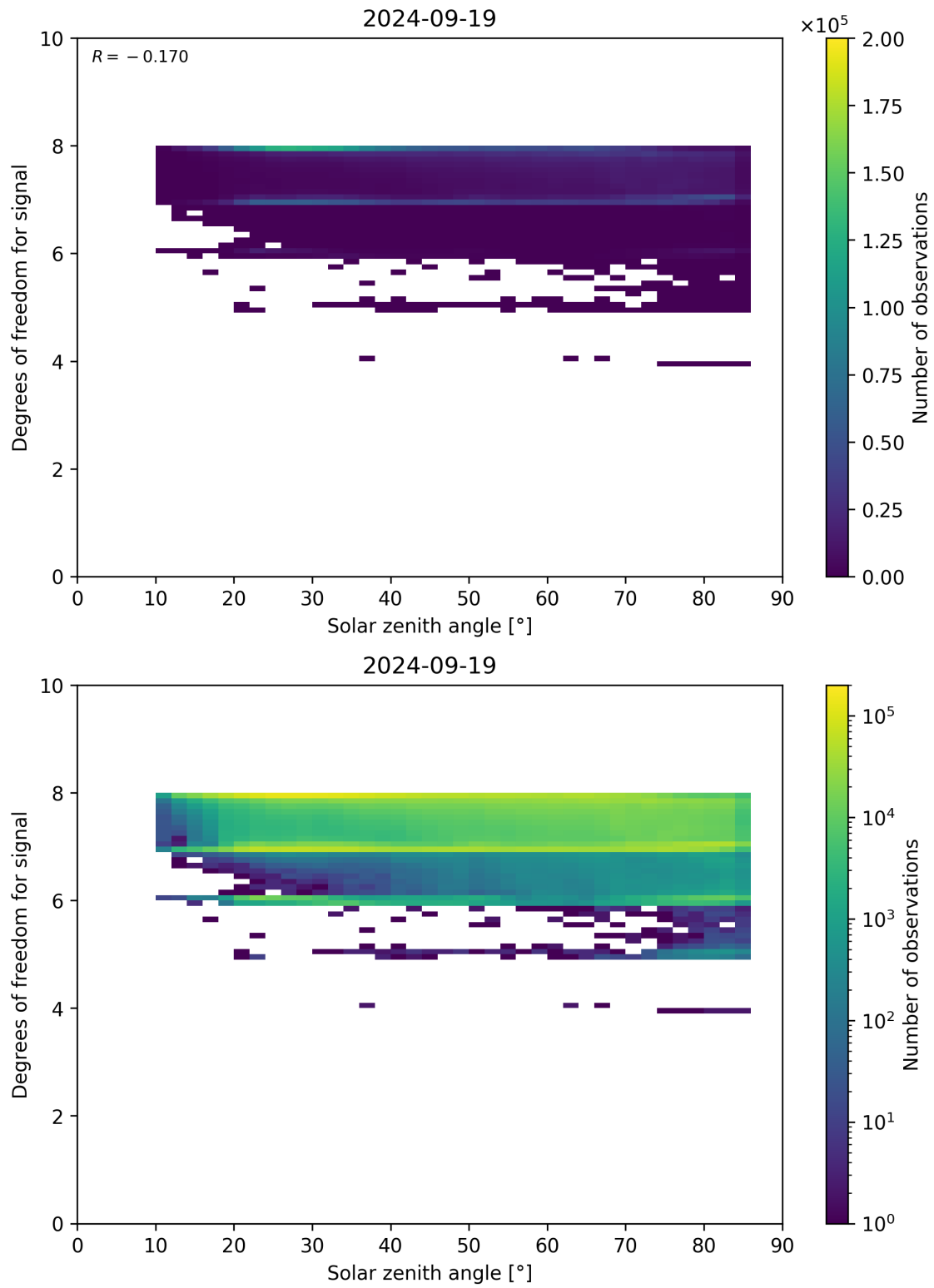
Figure 65: Scatter density plot of “Solar zenith angle” against “Degrees of freedom for signal” for 2024-09-18 to 2024-09-20.
