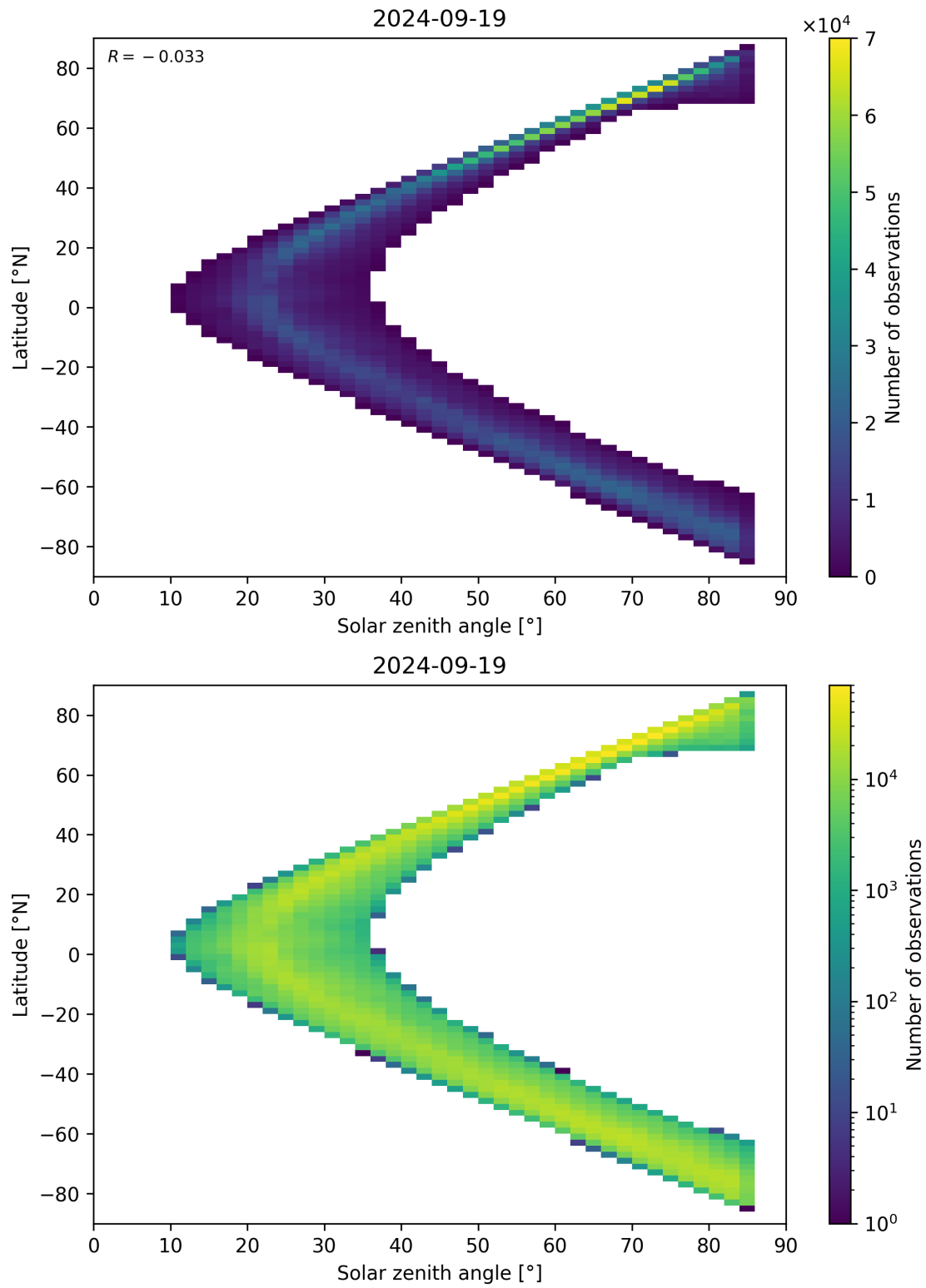
Figure 66: Scatter density plot of “Solar zenith angle” against “Latitude” for 2024-09-18 to 2024-09-20.
