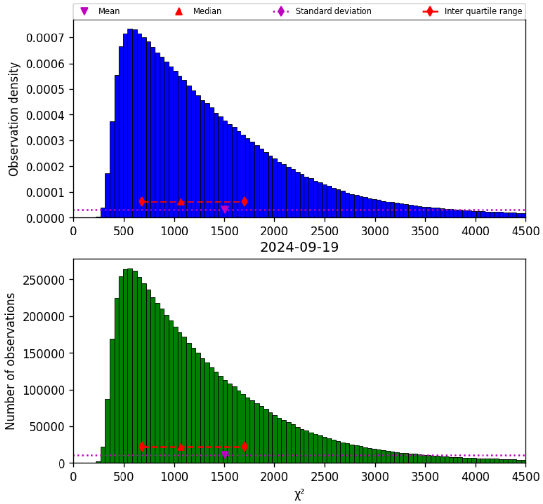
Figure 22: Histogram of “ \chi^2 ” for 2024-09-18 to 2024-09-20
