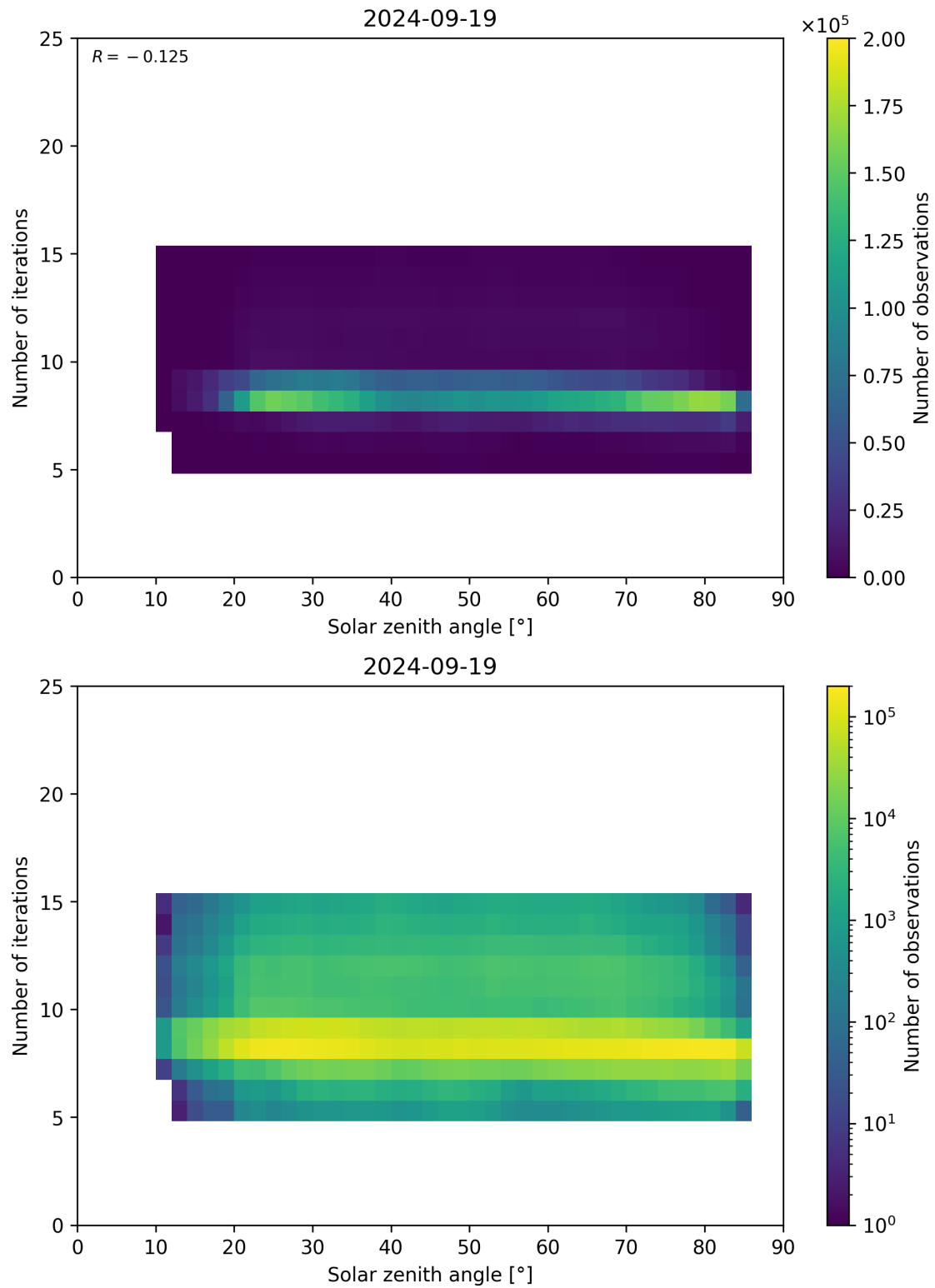
Figure 67: Scatter density plot of “Solar zenith angle” against “Number of iterations” for 2024-09-18 to 2024-09-20.
