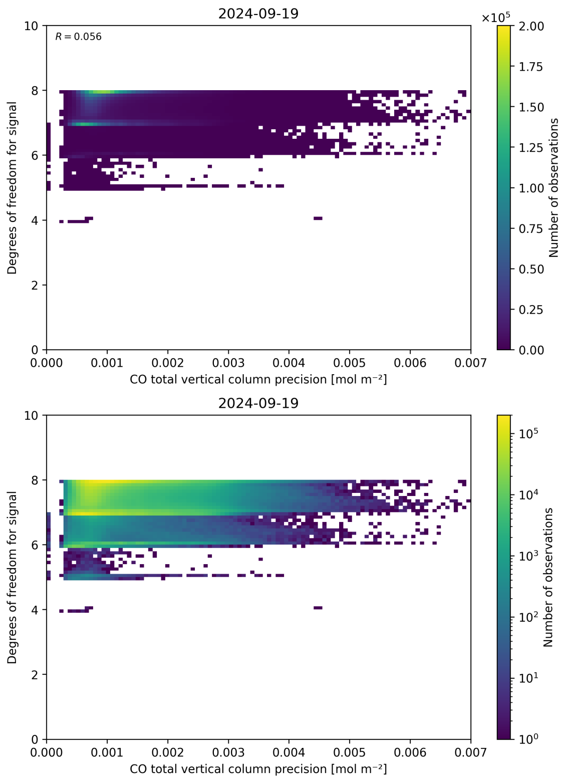
Figure 45: Scatter density plot of “CO total vertical column precision” against “Degrees of freedom for signal” for 2024-09-18 to 2024-09-20.
