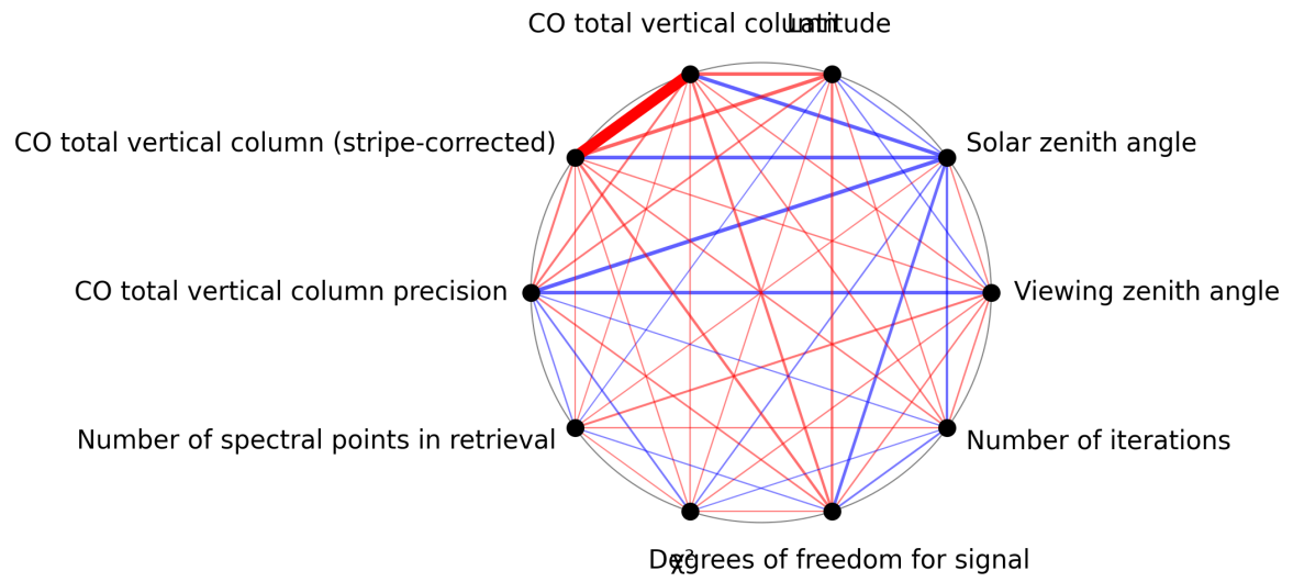
Figure 1: Map of correlation graph for 2024-09-18 to 2024-09-20.
