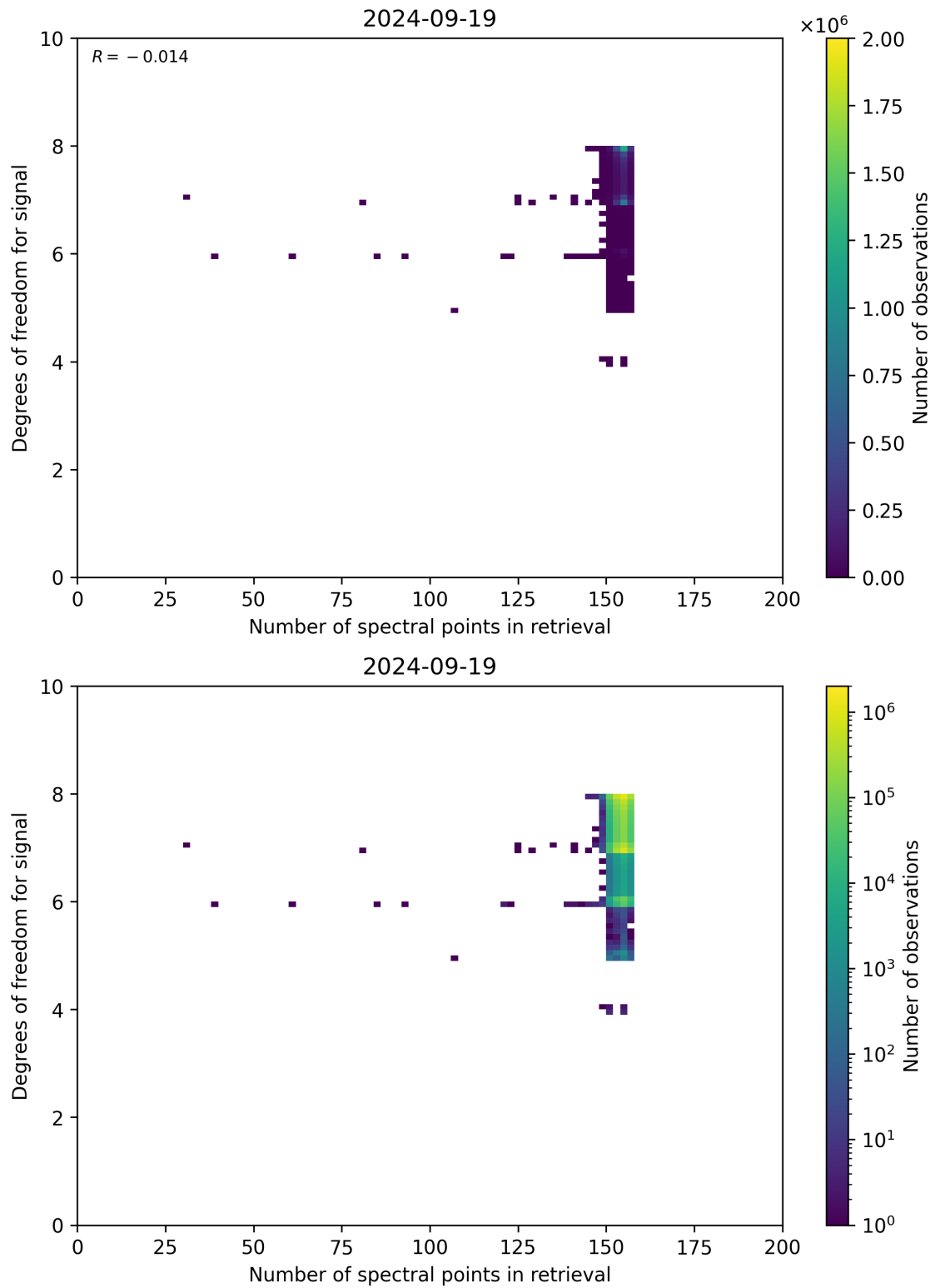
Figure 59: Scatter density plot of “Number of spectral points in retrieval” against “Degrees of freedom for signal” for 2024-09-18 to 2024-09-20.
