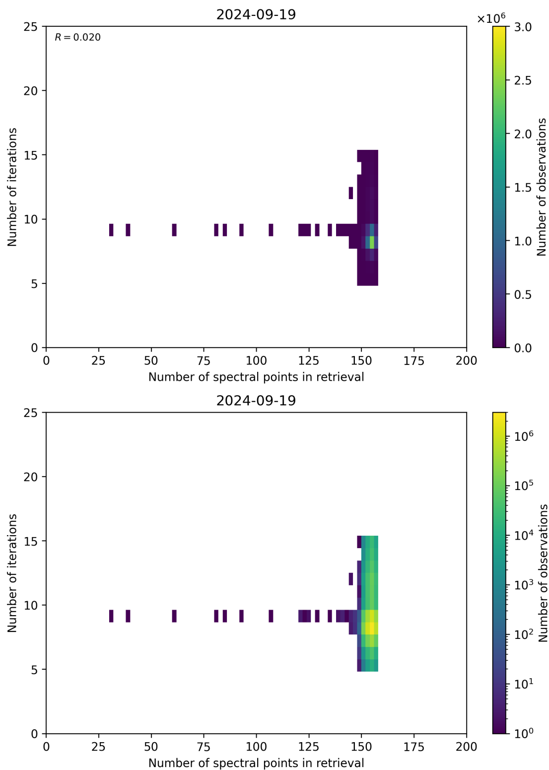
Figure 60: Scatter density plot of “Number of spectral points in retrieval” against “Number of iterations” for 2024-09-18 to 2024-09-20.
