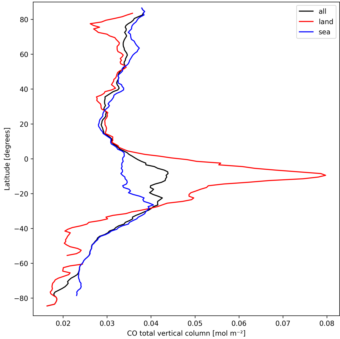
Figure 10: Zonal average of “CO total vertical column” for 2024-09-18 to 2024-09-20.
