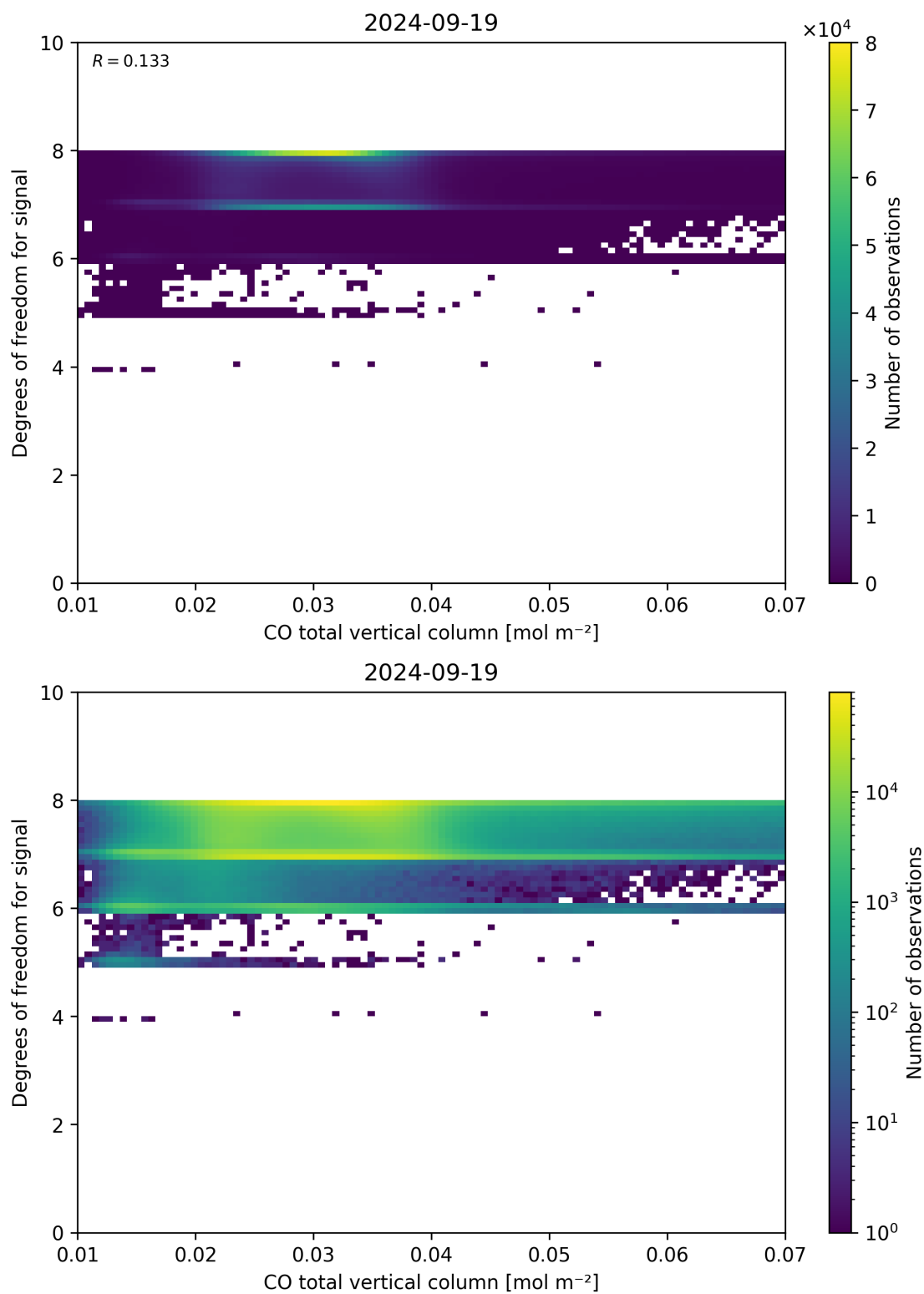
Figure 41: Scatter density plot of “CO total vertical column” against “Degrees of freedom for signal” for 2024-09-18 to 2024-09-20.
