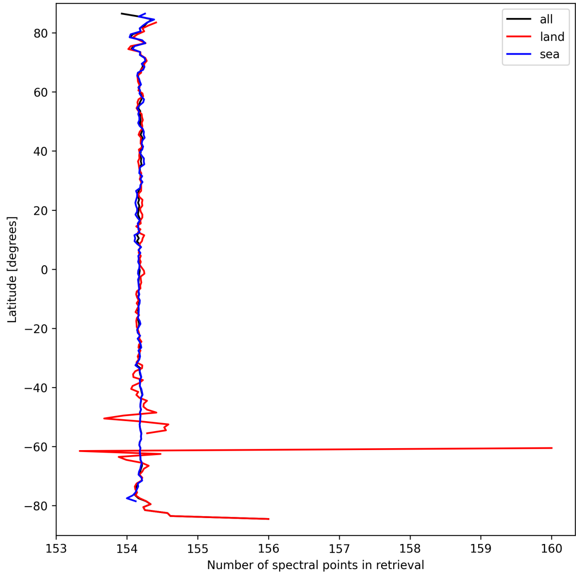
Figure 13: Zonal average of “Number of spectral points in retrieval” for 2024-09-18 to 2024-09-20.
