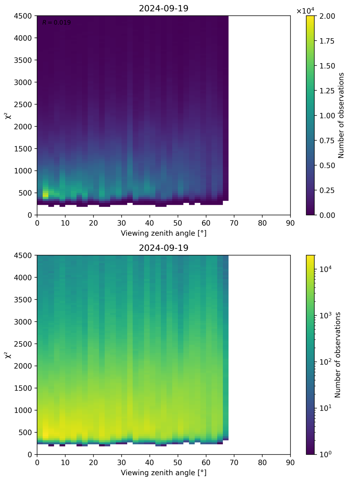
Figure 72: Scatter density plot of “Viewing zenith angle” against “ \chi^2 ” for 2024-09-18 to 2024-09-20.
