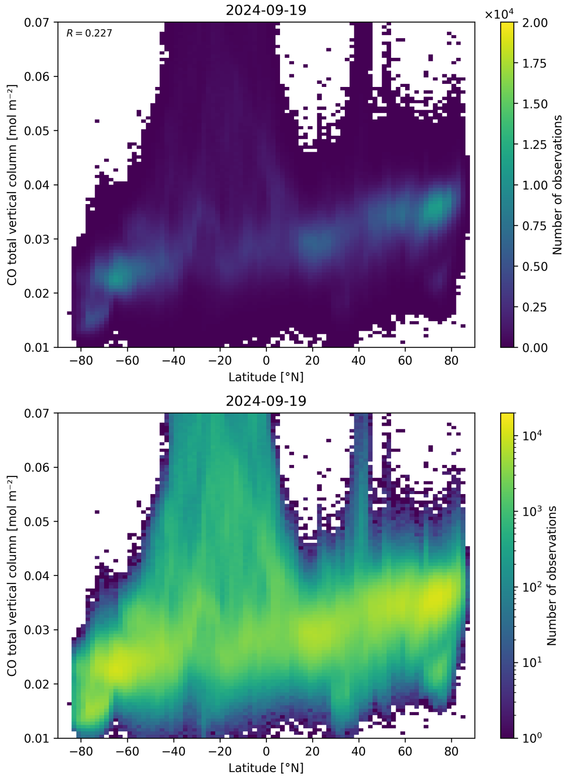
Figure 51: Scatter density plot of “Latitude” against “CO total vertical column” for 2024-09-18 to 2024-09-20.
