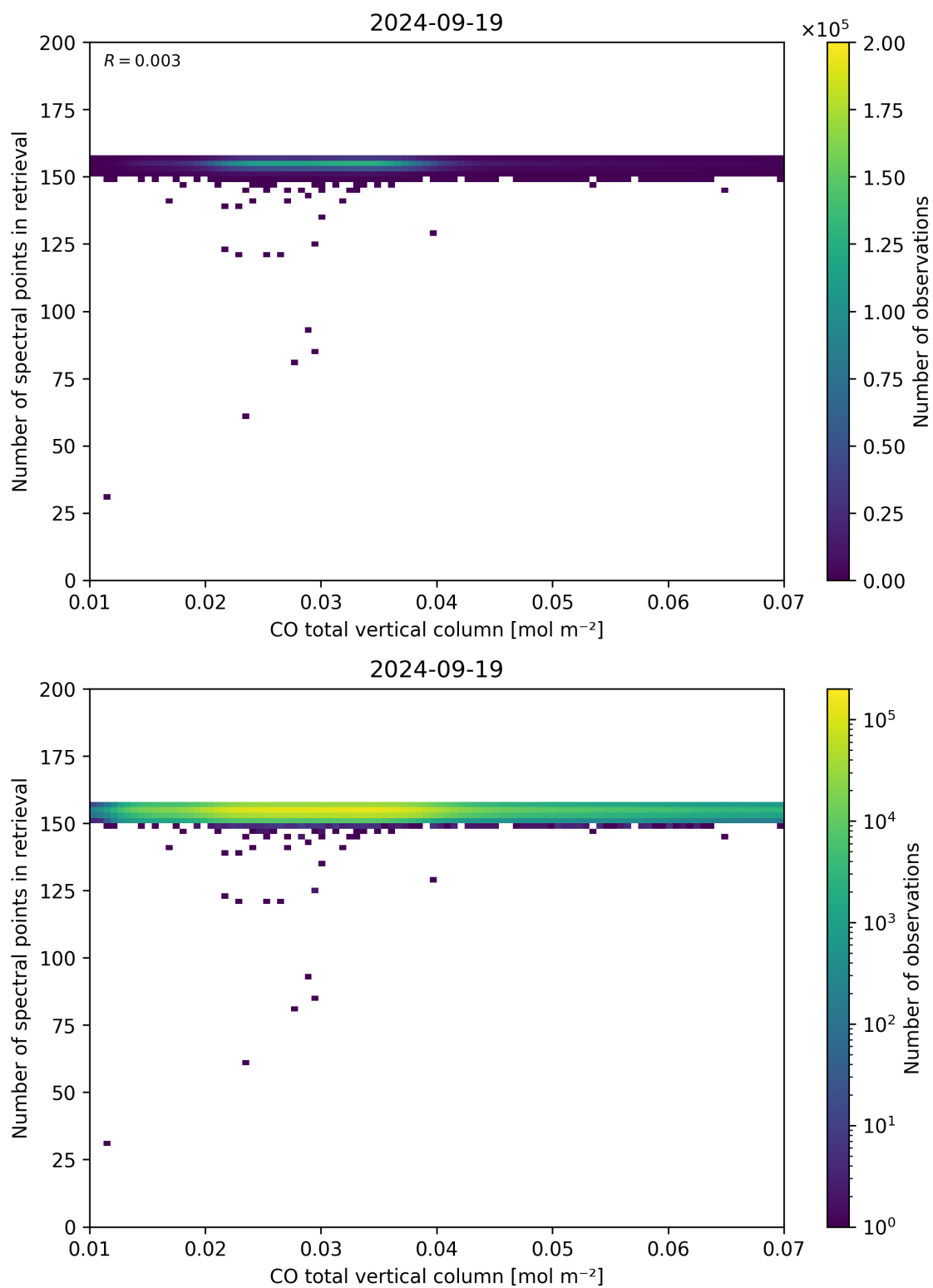
Figure 43: Scatter density plot of “CO total vertical column” against “Number of spectral points in retrieval” for 2024-09-18 to 2024-09-20.
