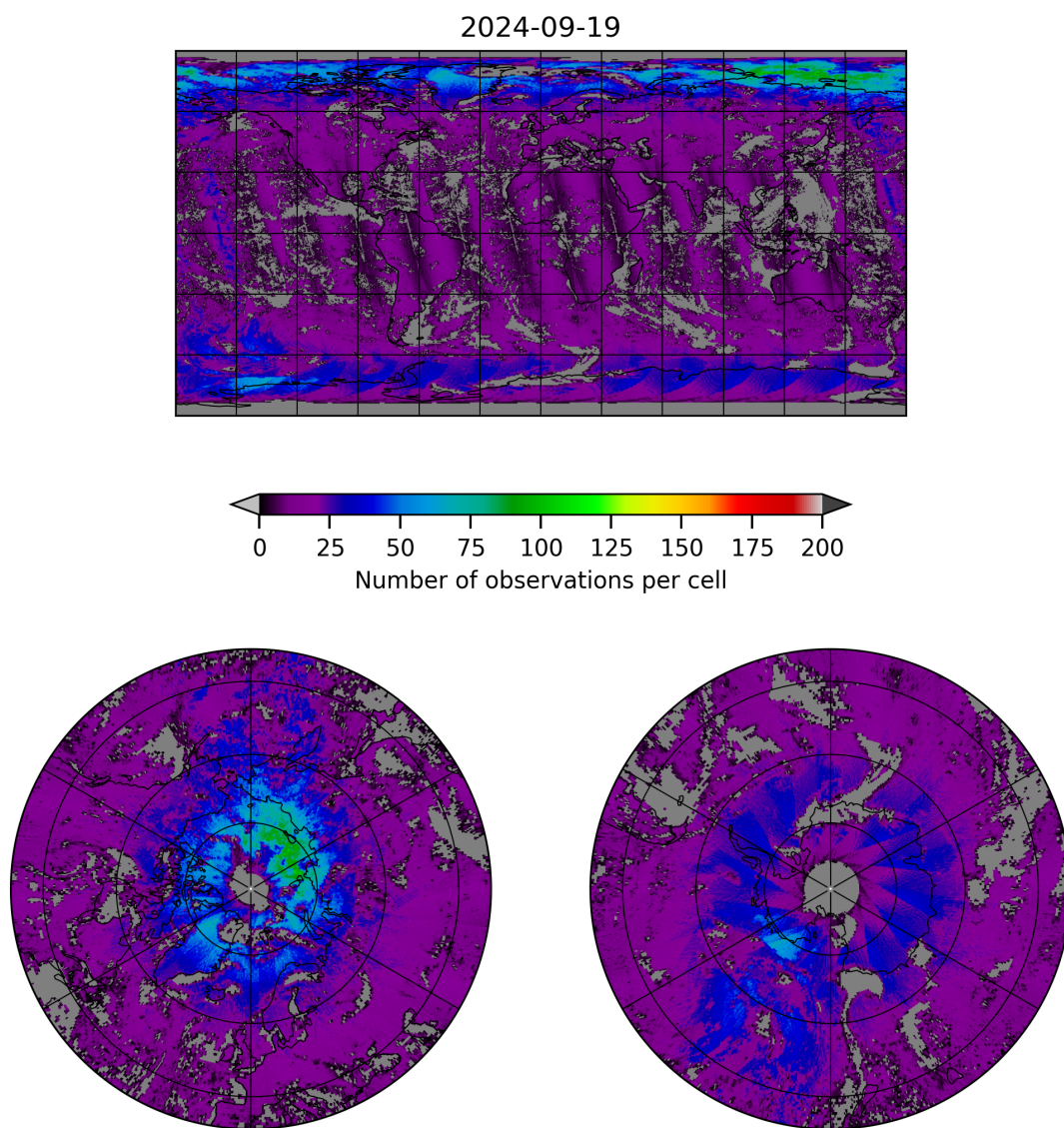
Figure 8: Map of the number of observations for 2024-09-18 to 2024-09-20
