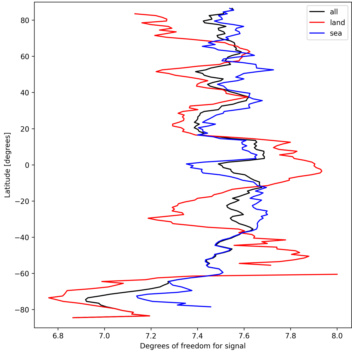
Figure 15: Zonal average of “Degrees of freedom for signal” for 2024-09-18 to 2024-09-20.
