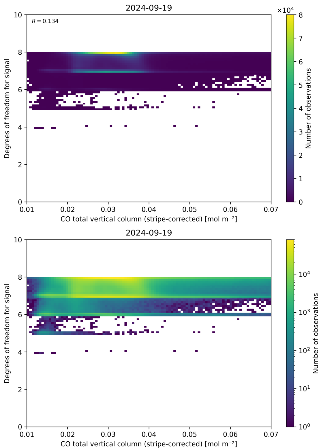
Figure 38: Scatter density plot of “CO total vertical column (stripe-corrected)” against “Degrees of freedom for signal” for 2024-09-18 to 2024-09-20.
