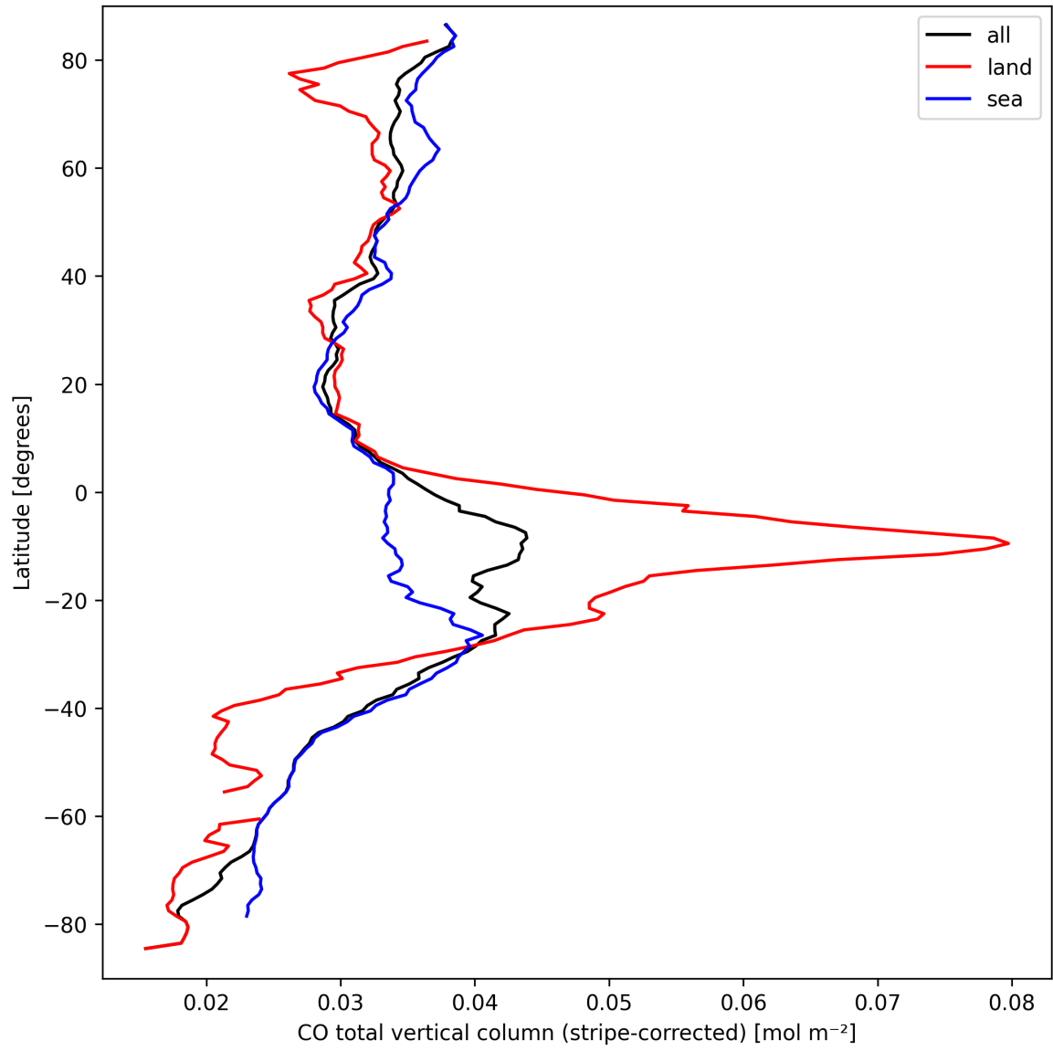
Figure 11: Zonal average of “CO total vertical column (stripe-corrected)” for 2024-09-18 to 2024-09-20.
