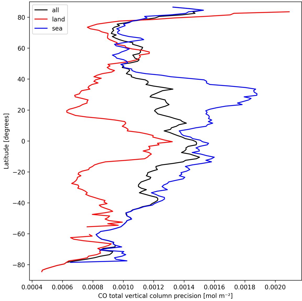
Figure 12: Zonal average of “CO total vertical column precision” for 2024-09-18 to 2024-09-20.
