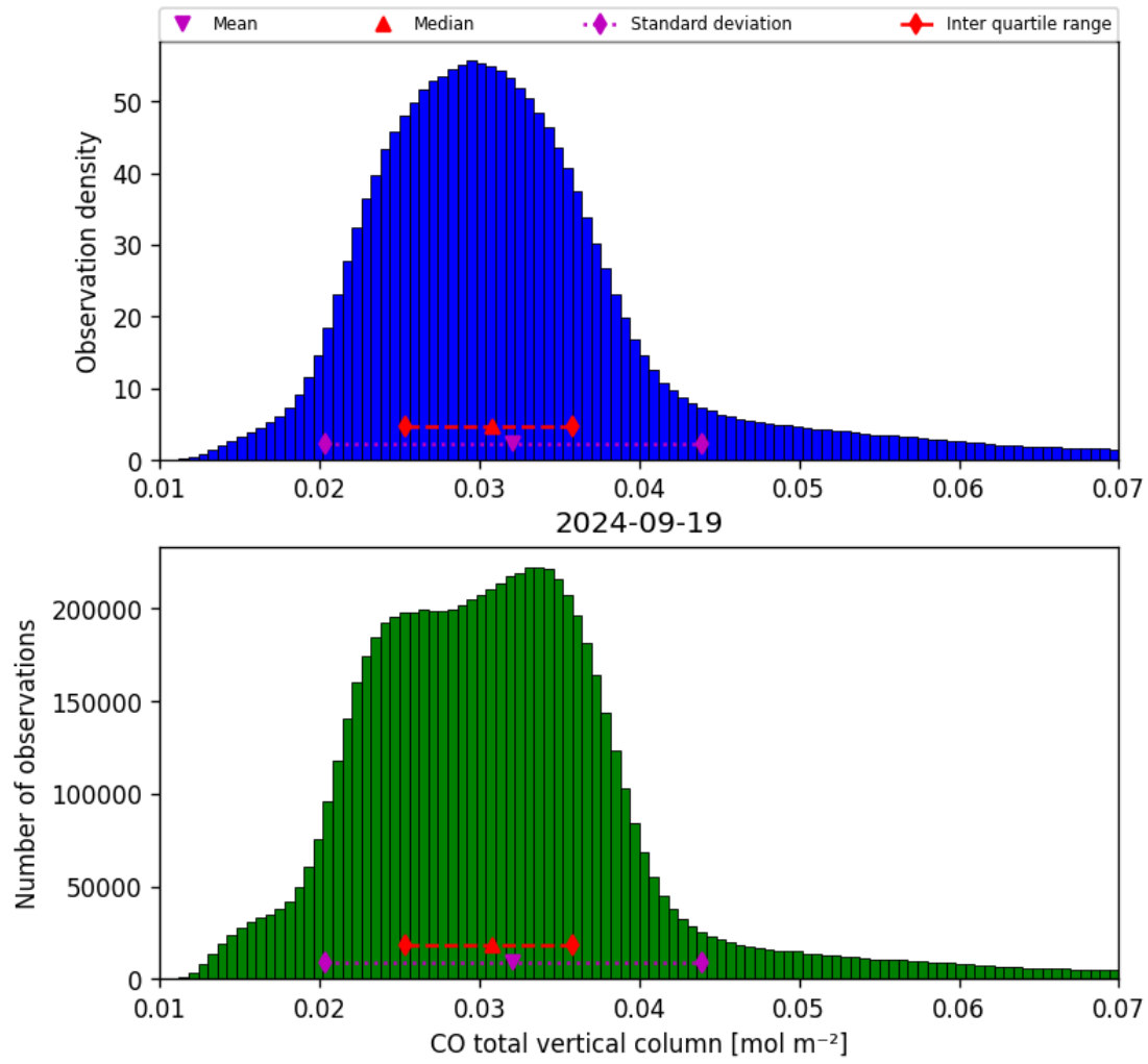
Figure 18: Histogram of “CO total vertical column” for 2024-09-18 to 2024-09-20
