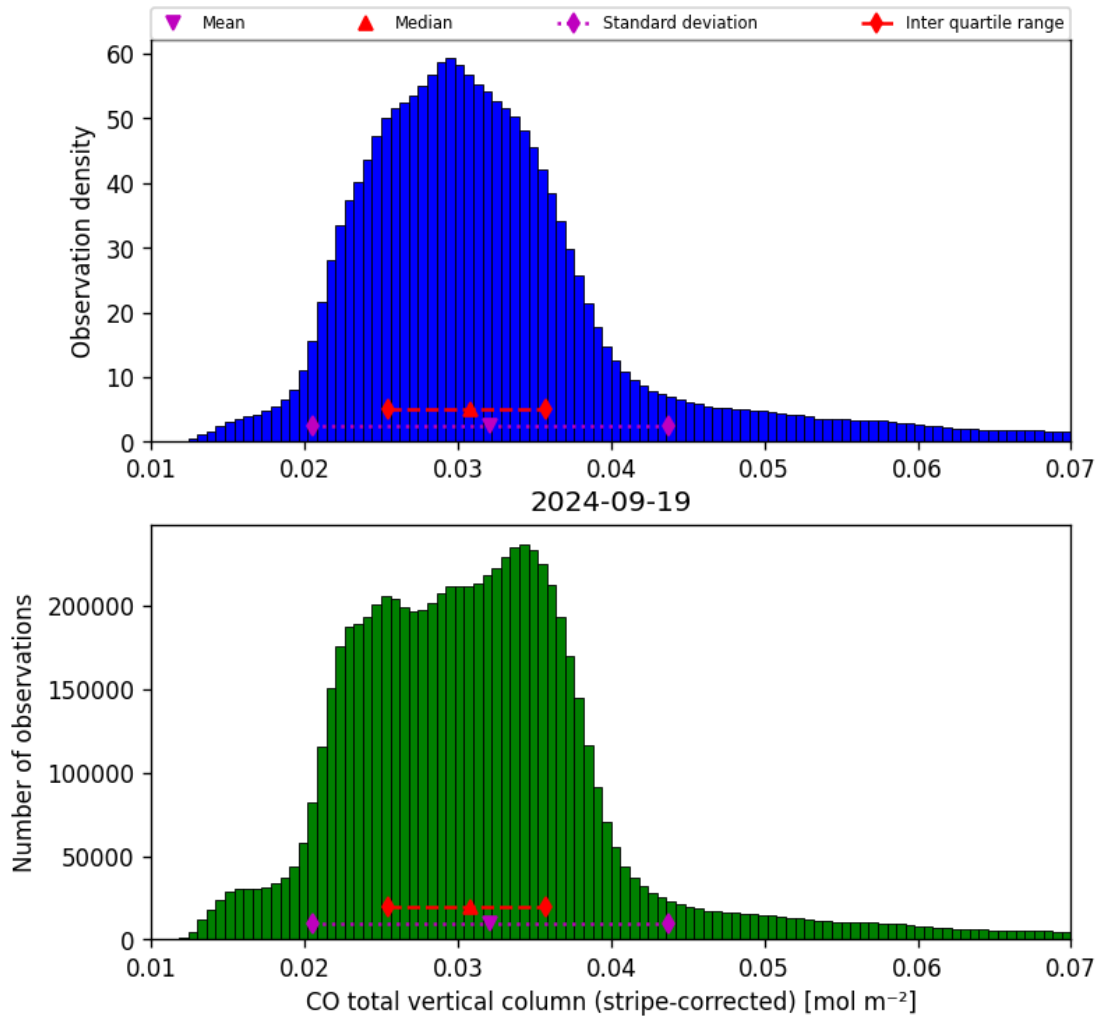
Figure 19: Histogram of “CO total vertical column (stripe-corrected)” for 2024-09-18 to 2024-09-20
