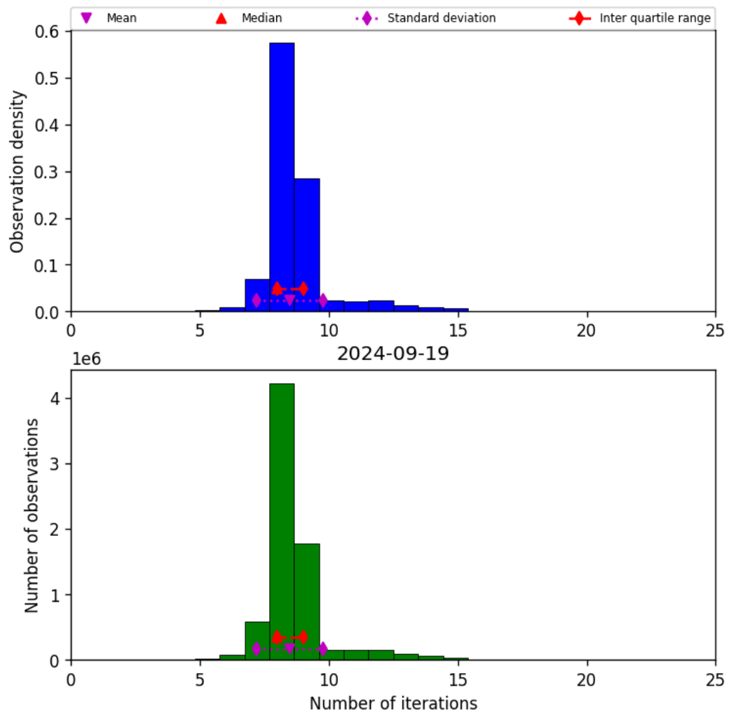
Figure 24: Histogram of “Number of iterations” for 2024-09-18 to 2024-09-20
