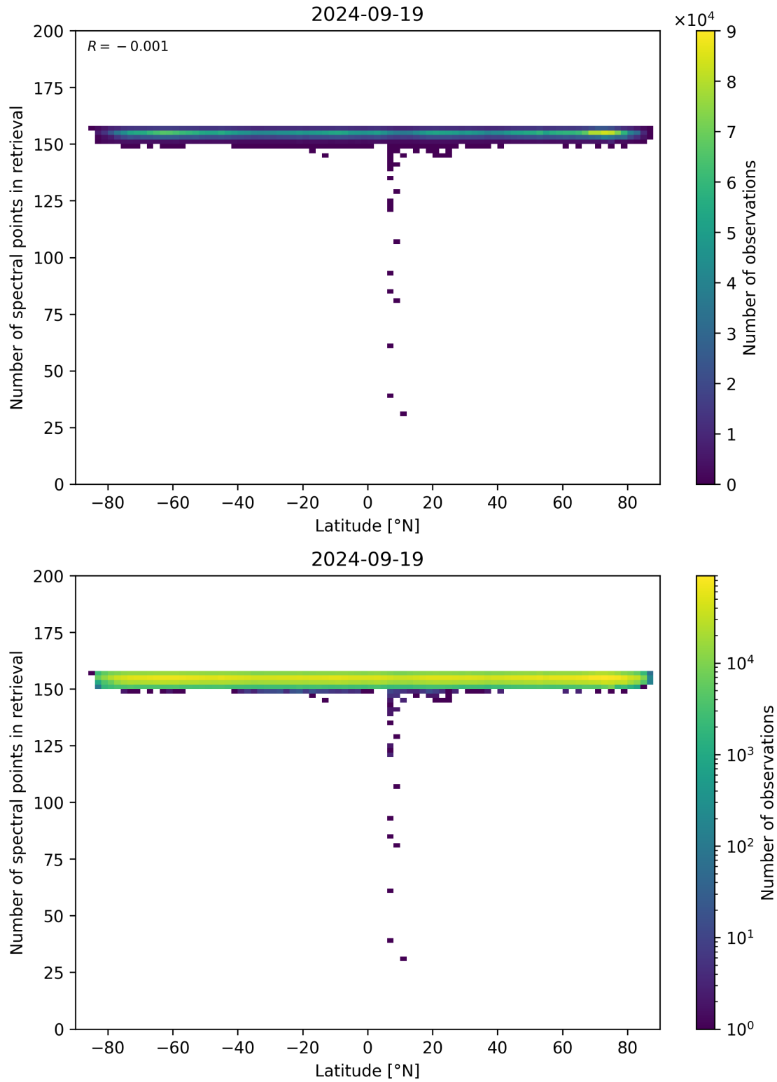
Figure 57: Scatter density plot of “Latitude” against “Number of spectral points in retrieval” for 2024-09-18 to 2024-09-20.
