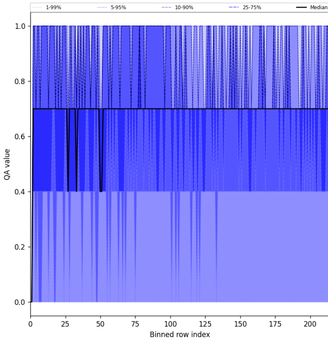
Figure 25: Along track statistics of “QA value” for 2024-09-18 to 2024-09-20
