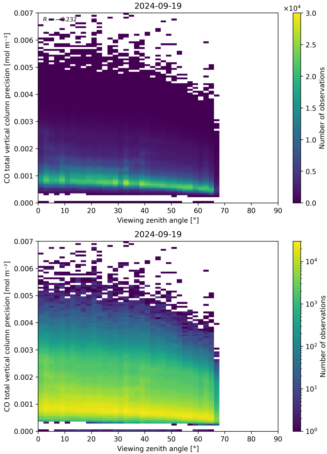
Figure 71: Scatter density plot of “Viewing zenith angle” against “CO total vertical column precision” for 2024-09-18 to 2024-09-20.
