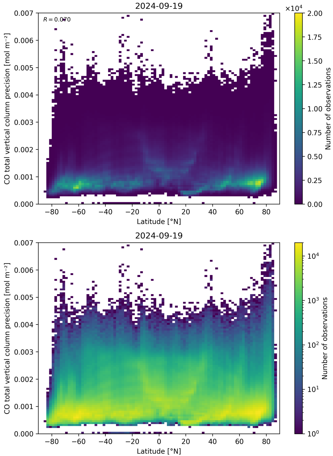
Figure 53: Scatter density plot of “Latitude” against “CO total vertical column precision” for 2024-09-18 to 2024-09-20.
