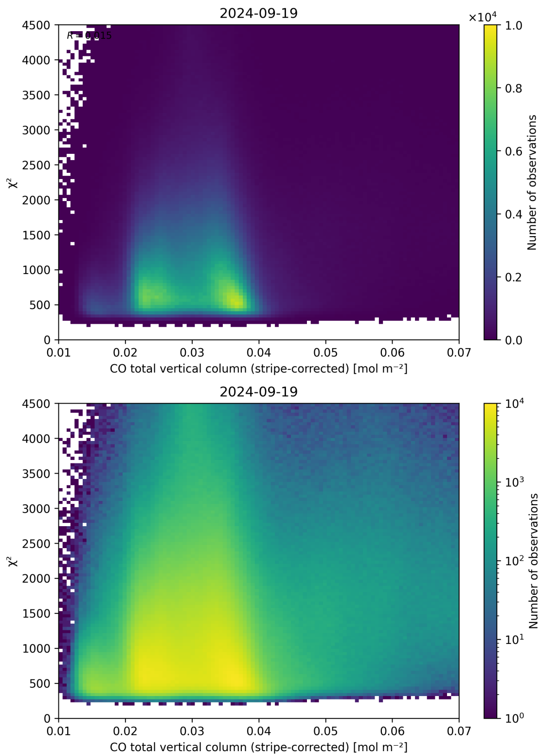
Figure 37: Scatter density plot of “CO total vertical column (stripe-corrected)” against “ \chi^2 ” for 2024-09-18 to 2024-09-20.
