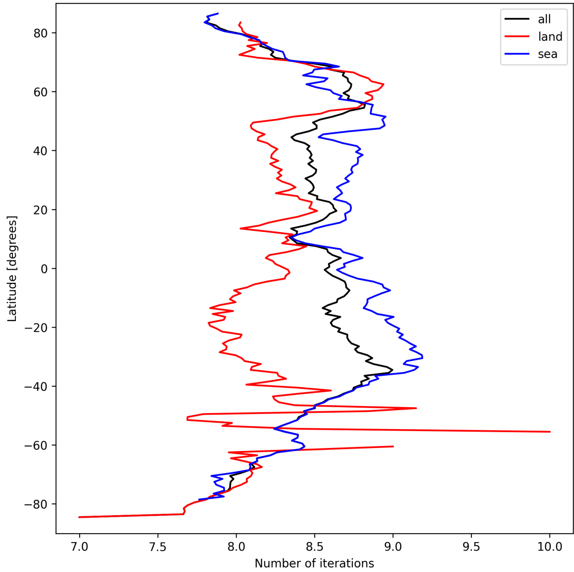
Figure 16: Zonal average of “Number of iterations” for 2024-09-18 to 2024-09-20.
