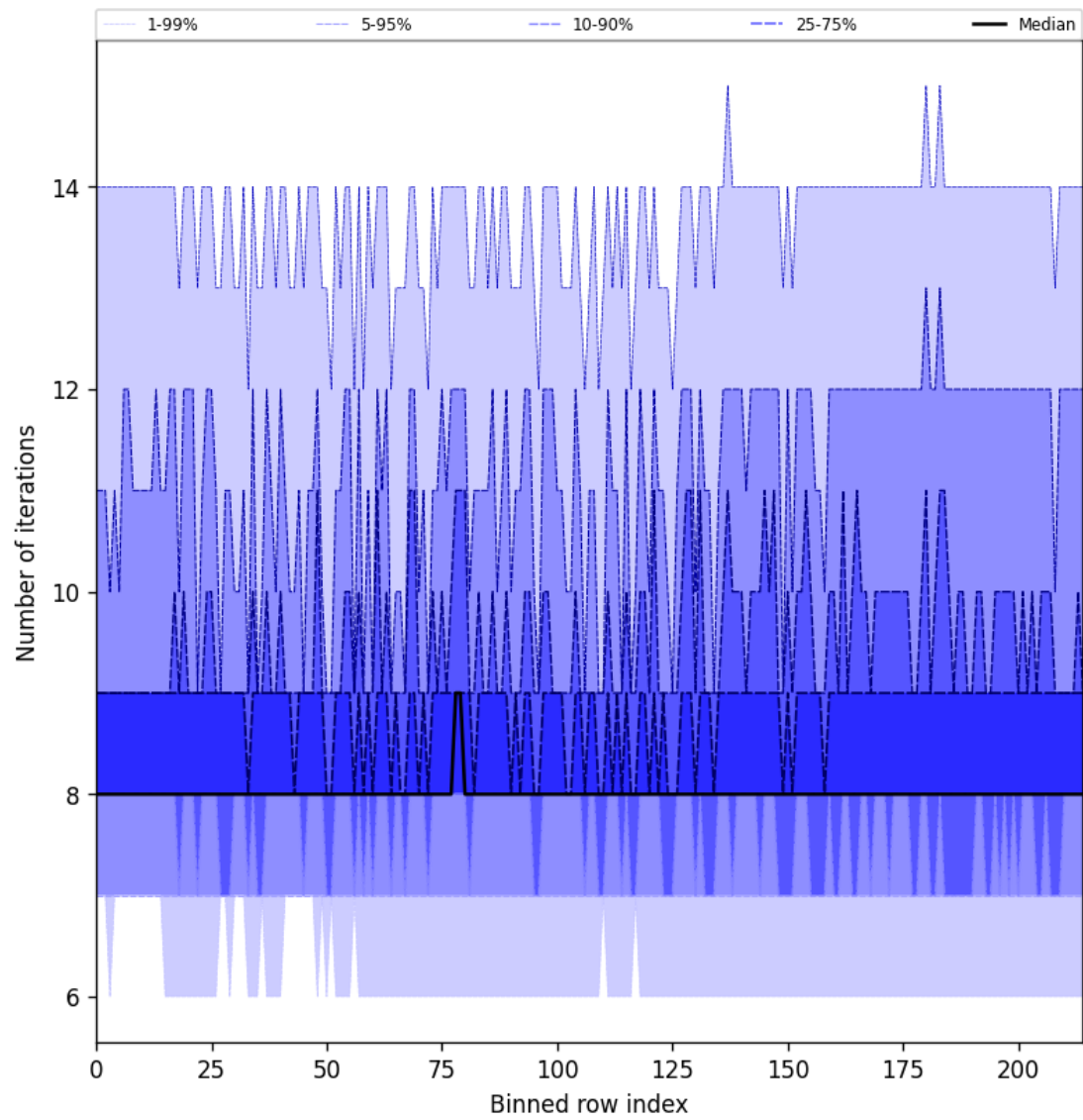
Figure 32: Along track statistics of “Number of iterations” for 2024-09-18 to 2024-09-20
