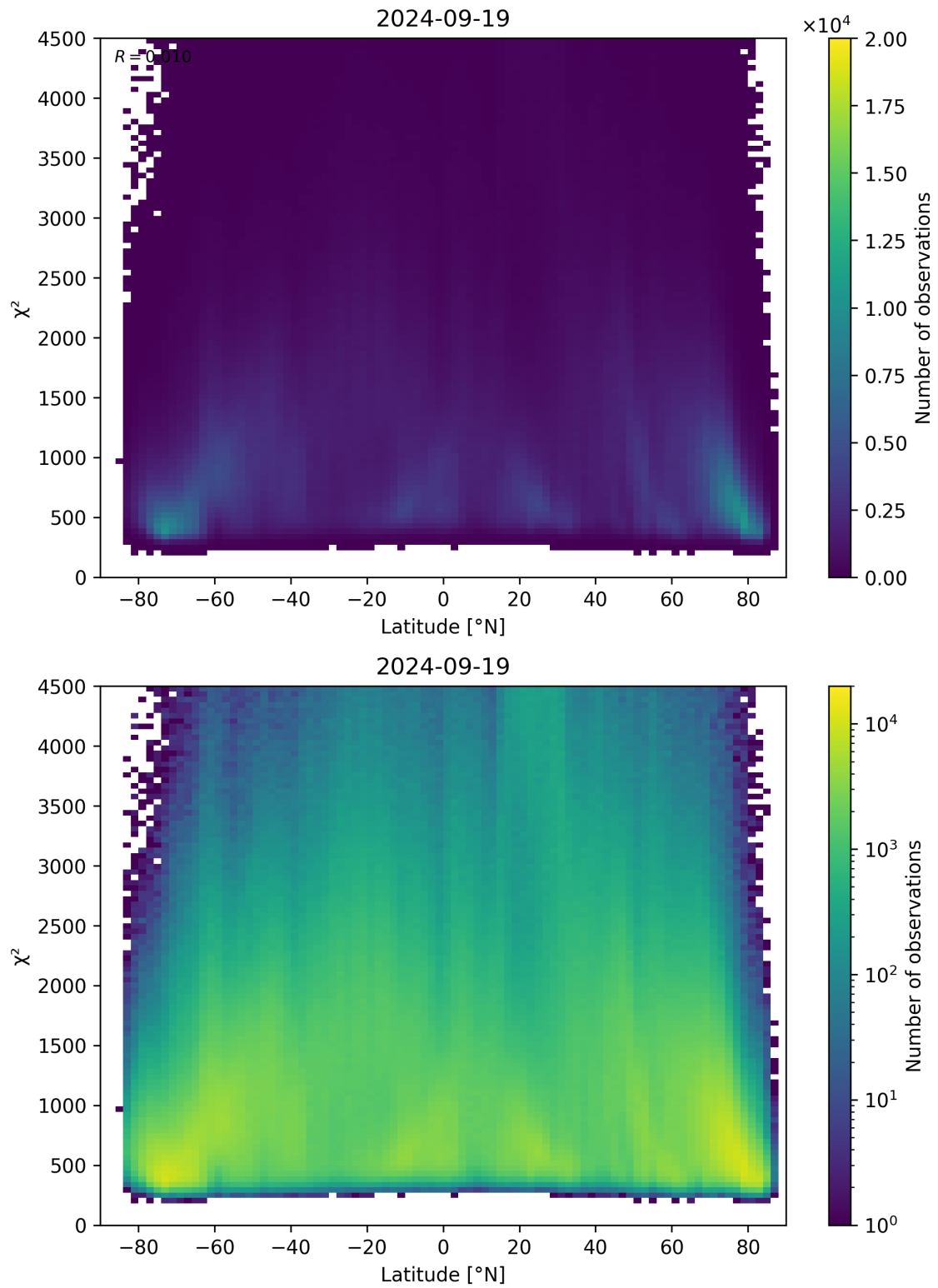
Figure 54: Scatter density plot of “Latitude” against “ \chi^2 ” for 2024-09-18 to 2024-09-20.
