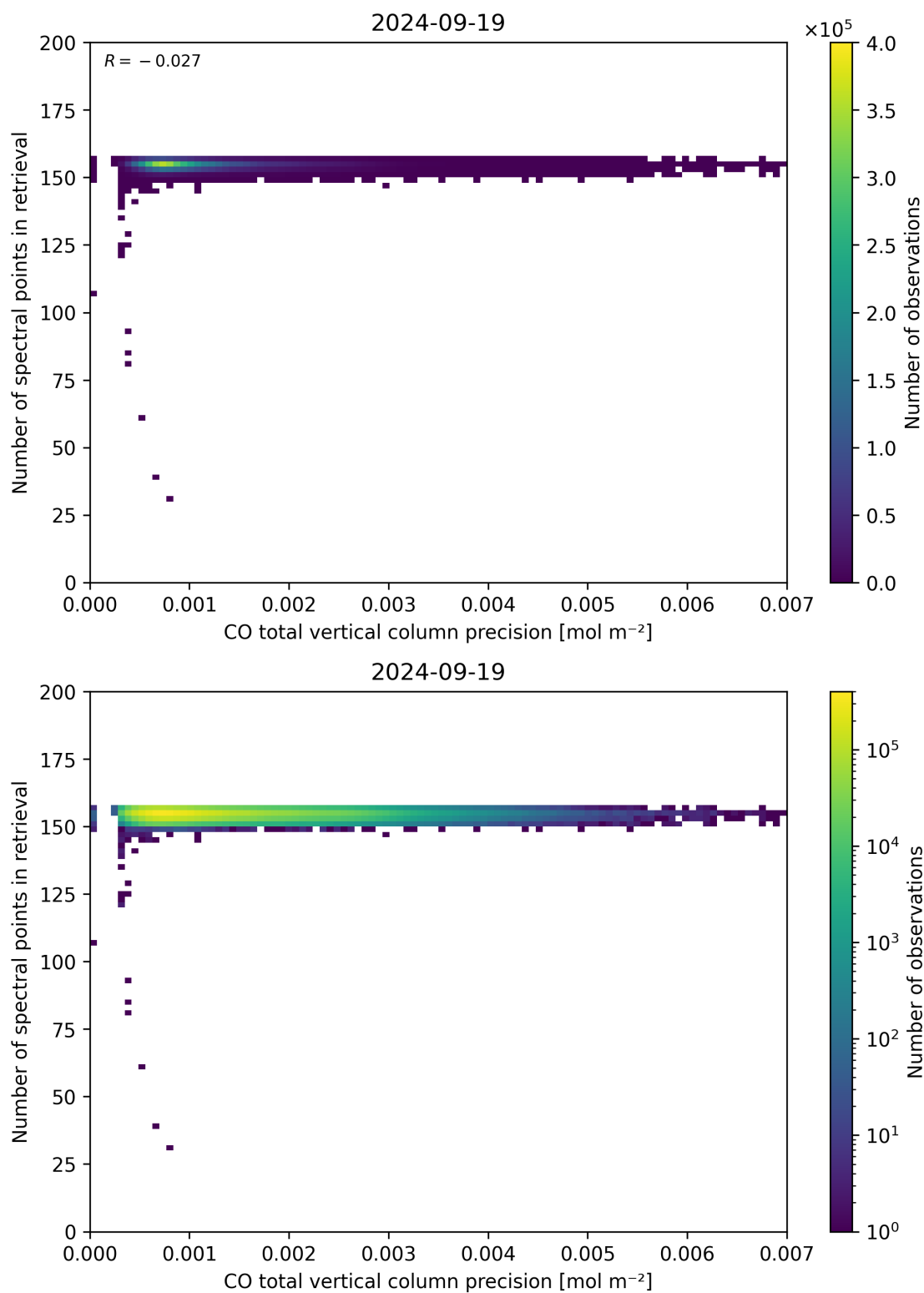
Figure 47: Scatter density plot of “CO total vertical column precision” against “Number of spectral points in retrieval” for 2024-09-18 to 2024-09-20.
