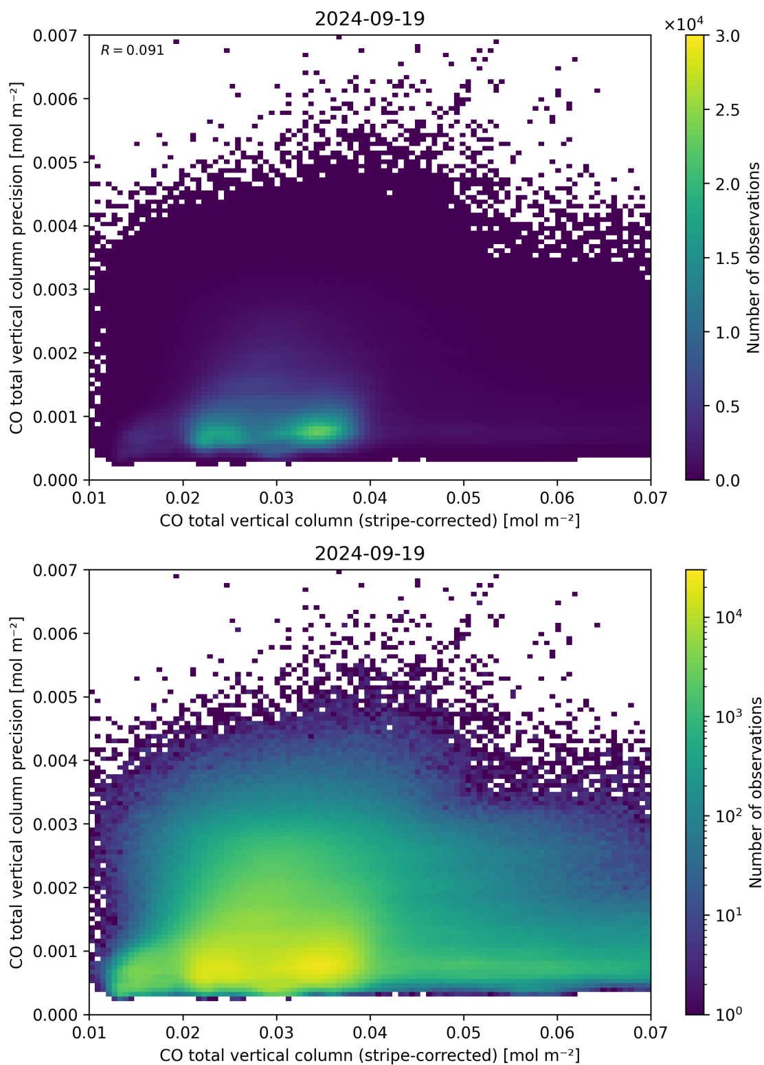
Figure 36: Scatter density plot of “CO total vertical column (stripe-corrected)” against “CO total vertical column precision” for 2024-09-18 to 2024-09-20.
