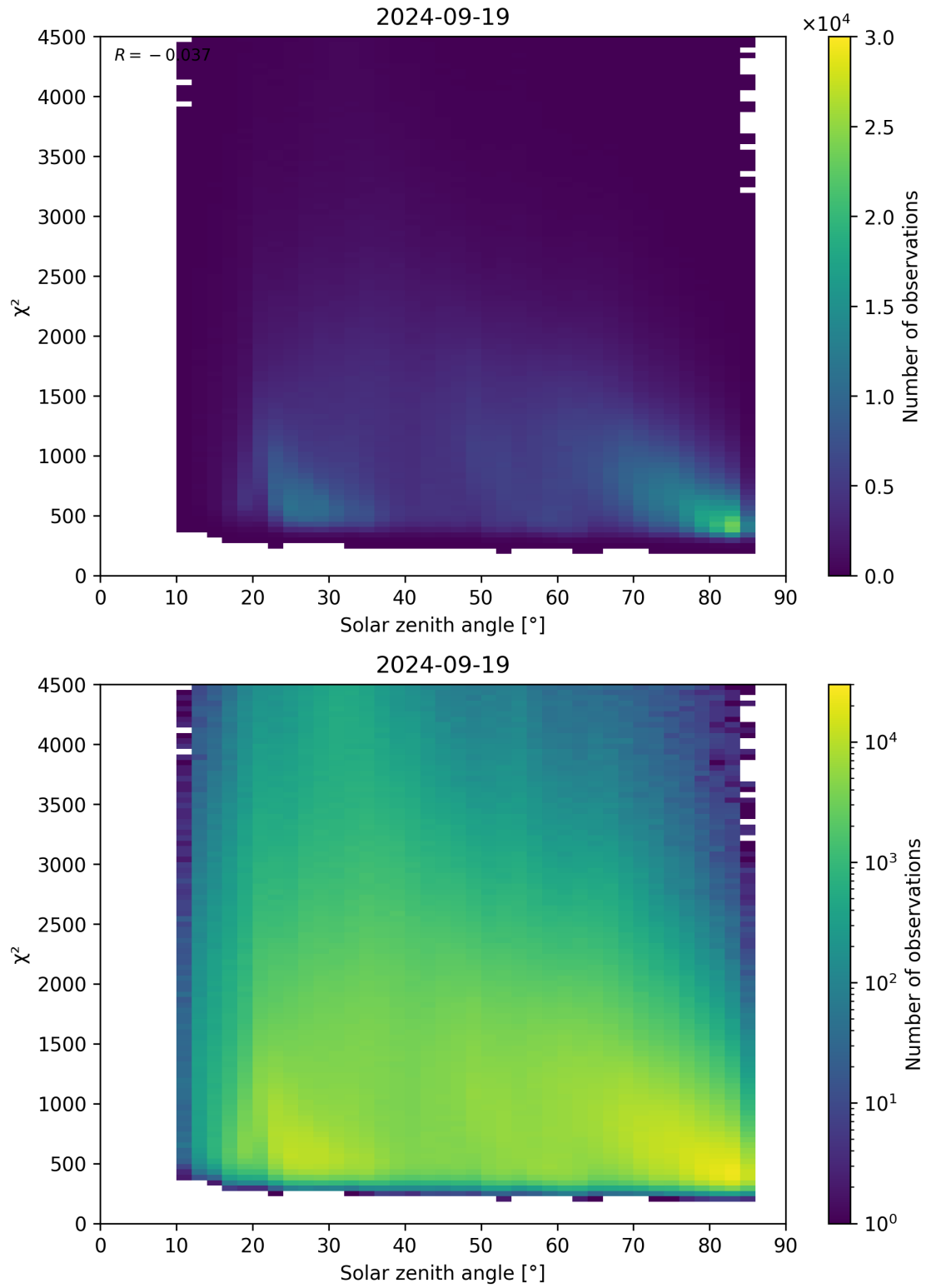
Figure 64: Scatter density plot of “Solar zenith angle” against “ \chi^2 ” for 2024-09-18 to 2024-09-20.
