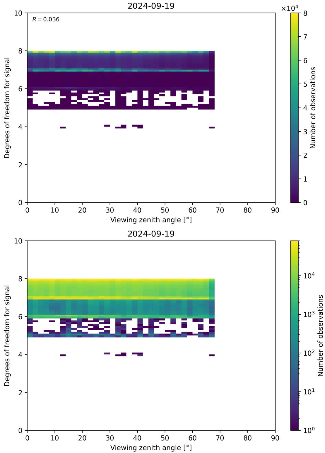
Figure 73: Scatter density plot of “Viewing zenith angle” against “Degrees of freedom for signal” for 2024-09-18 to 2024-09-20.
