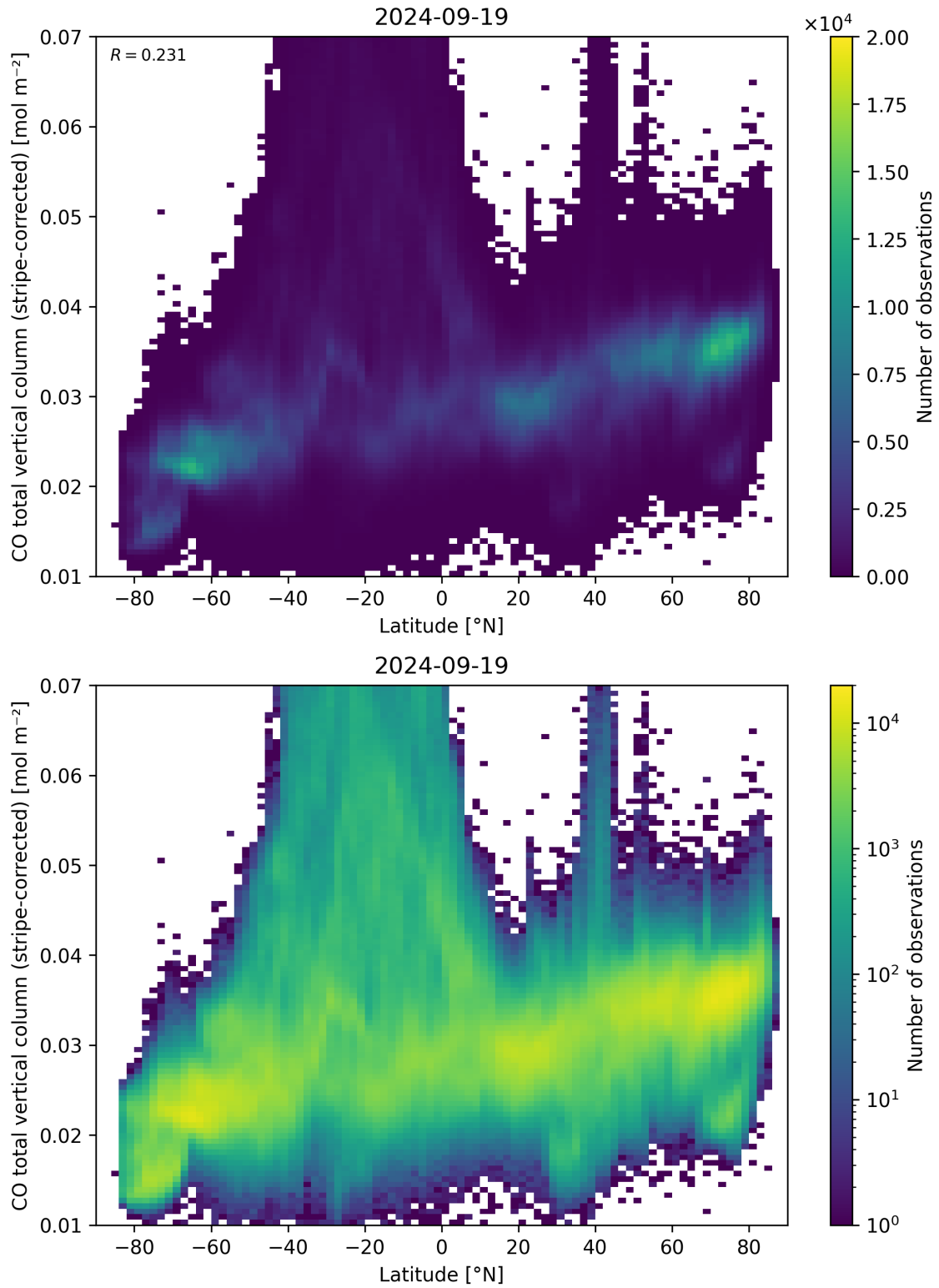
Figure 52: Scatter density plot of “Latitude” against “CO total vertical column (stripe-corrected)” for 2024-09-18 to 2024-09-20.
