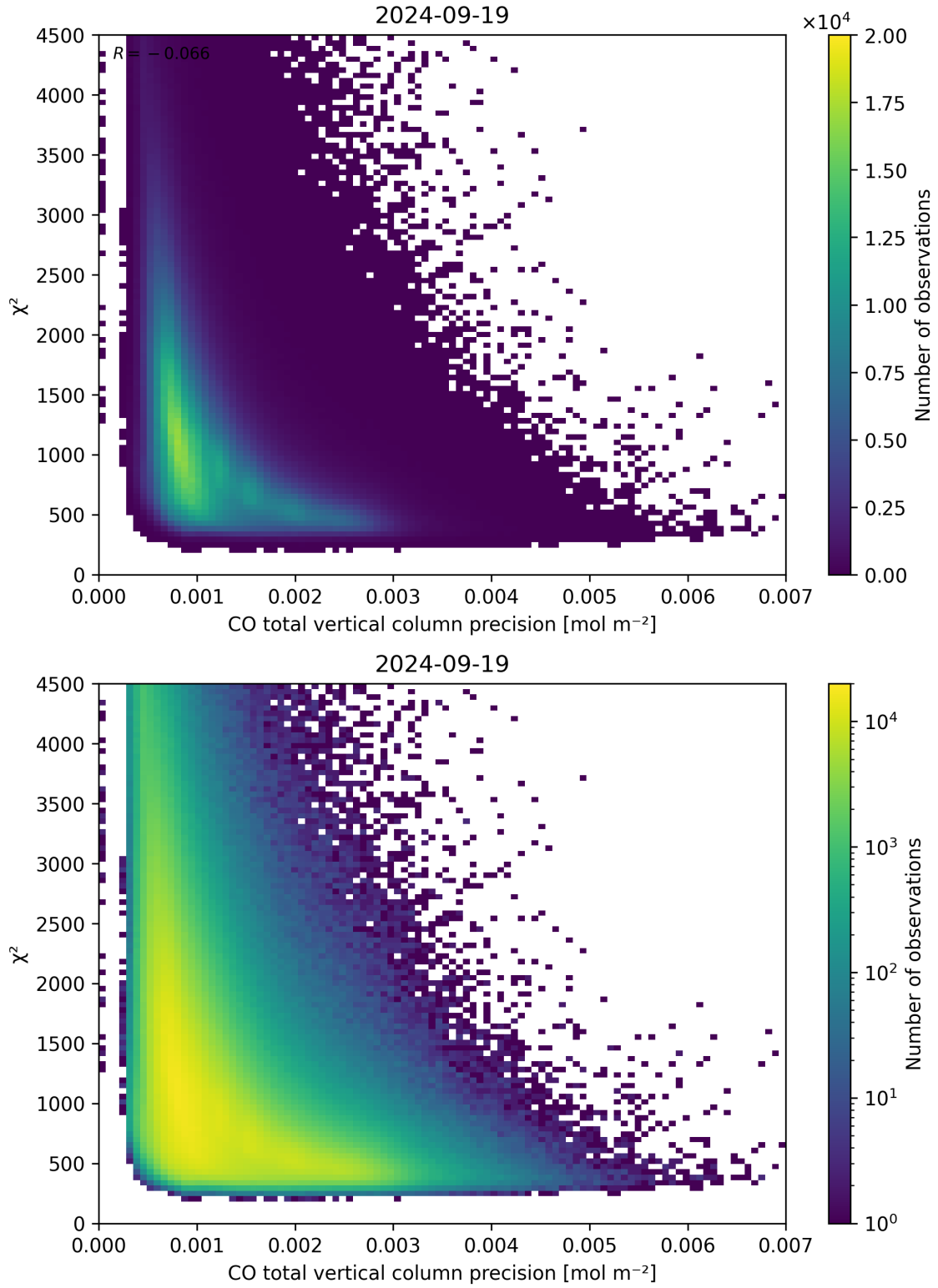
Figure 44: Scatter density plot of “CO total vertical column precision” against “ \chi^2 ” for 2024-09-18 to 2024-09-20.
