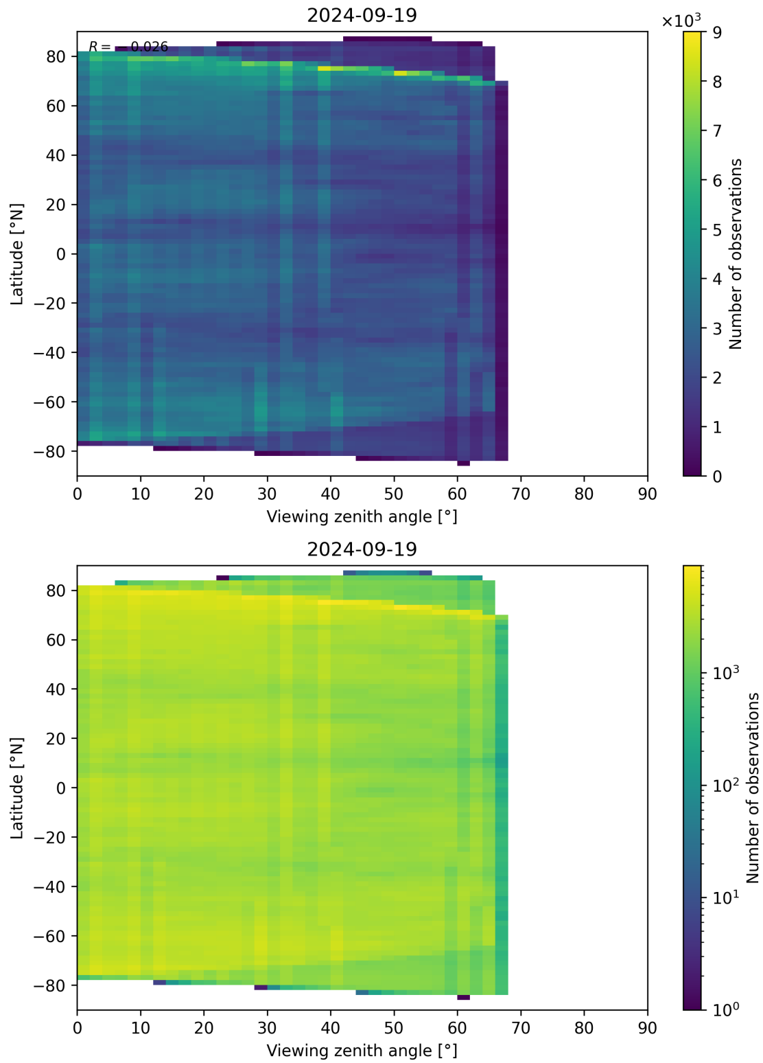
Figure 74: Scatter density plot of “Viewing zenith angle” against “Latitude” for 2024-09-18 to 2024-09-20.
