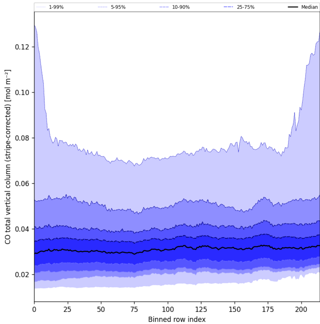
Figure 27: Along track statistics of “CO total vertical column (stripe-corrected)” for 2024-09-18 to 2024-09-20
