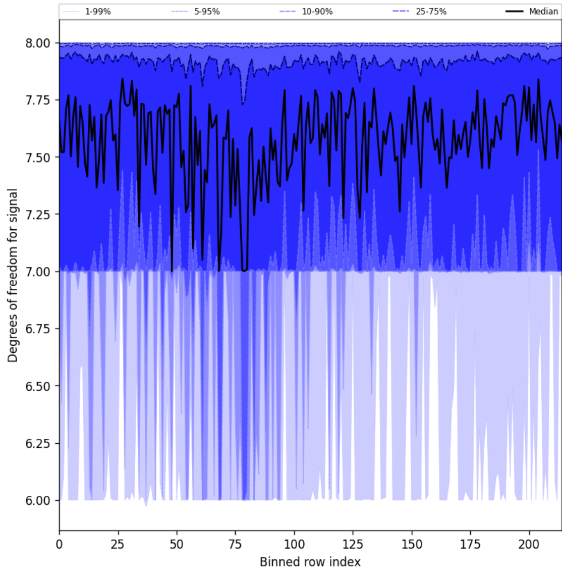
Figure 31: Along track statistics of “Degrees of freedom for signal” for 2024-09-18 to 2024-09-20
