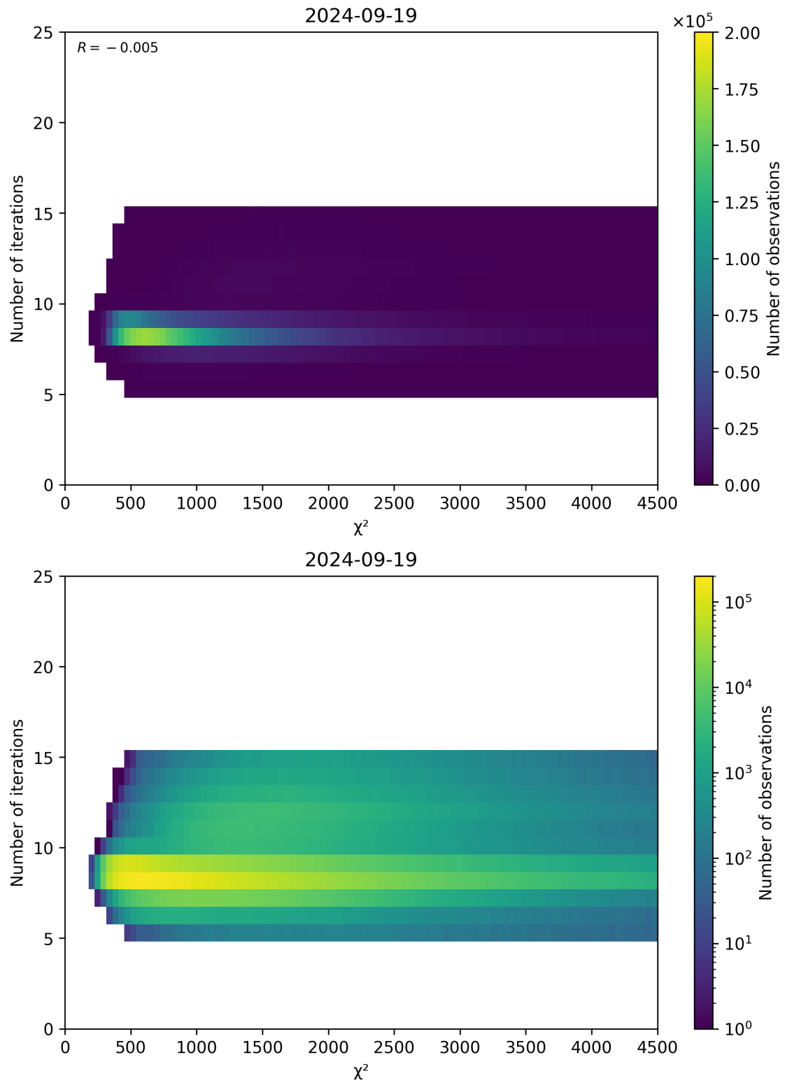
Figure 49: Scatter density plot of “ \chi^2 ” against “Number of iterations” for 2024-09-18 to 2024-09-20.
