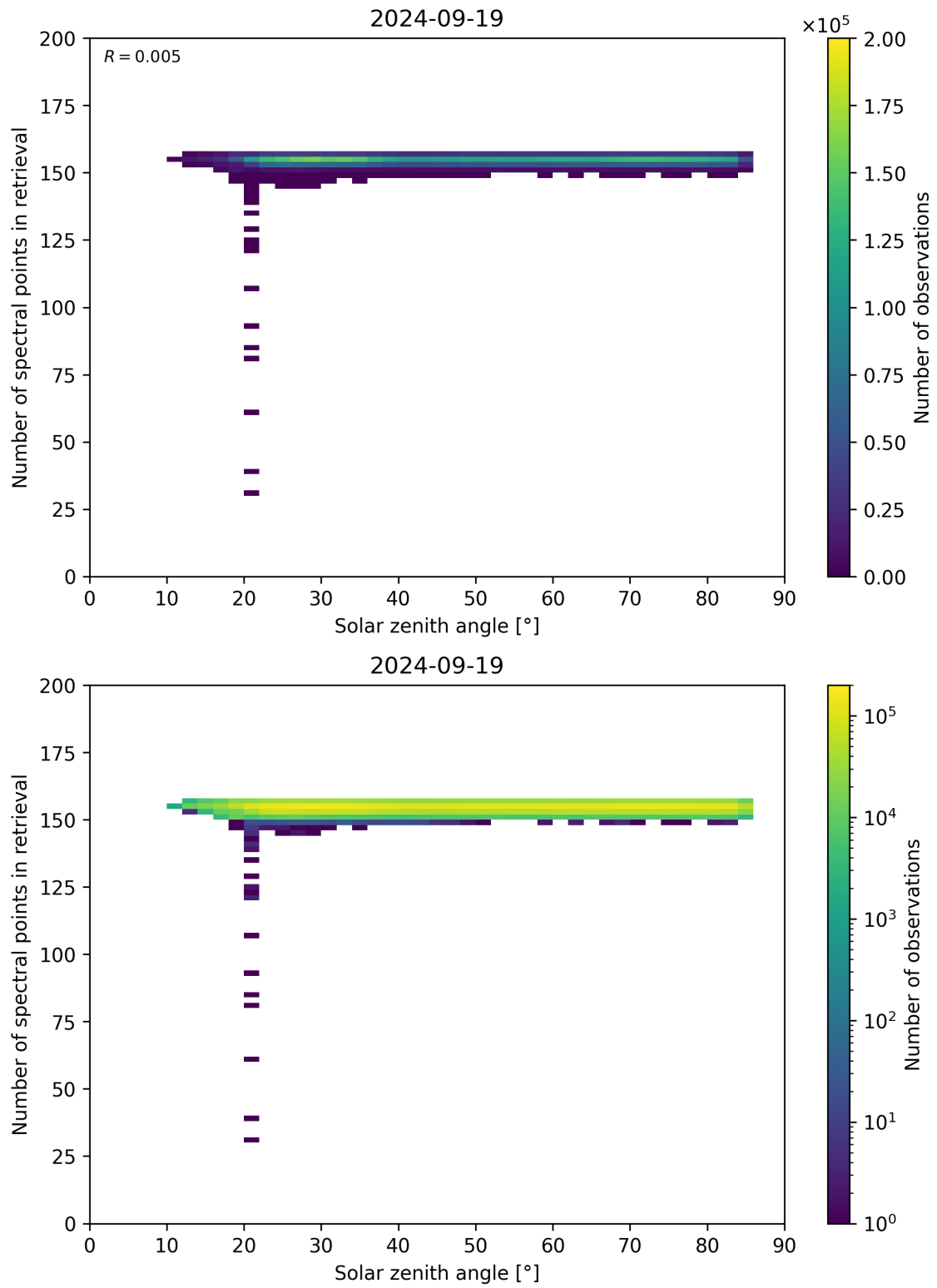
Figure 68: Scatter density plot of “Solar zenith angle” against “Number of spectral points in retrieval” for 2024-09-18 to 2024-09-20.
