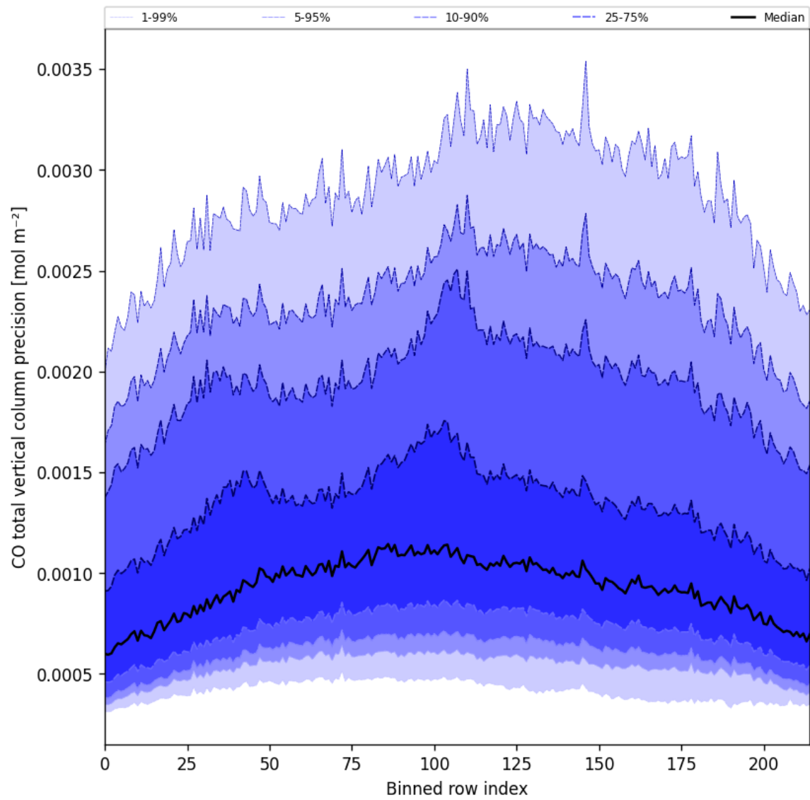
Figure 28: Along track statistics of “CO total vertical column precision” for 2024-09-18 to 2024-09-20
