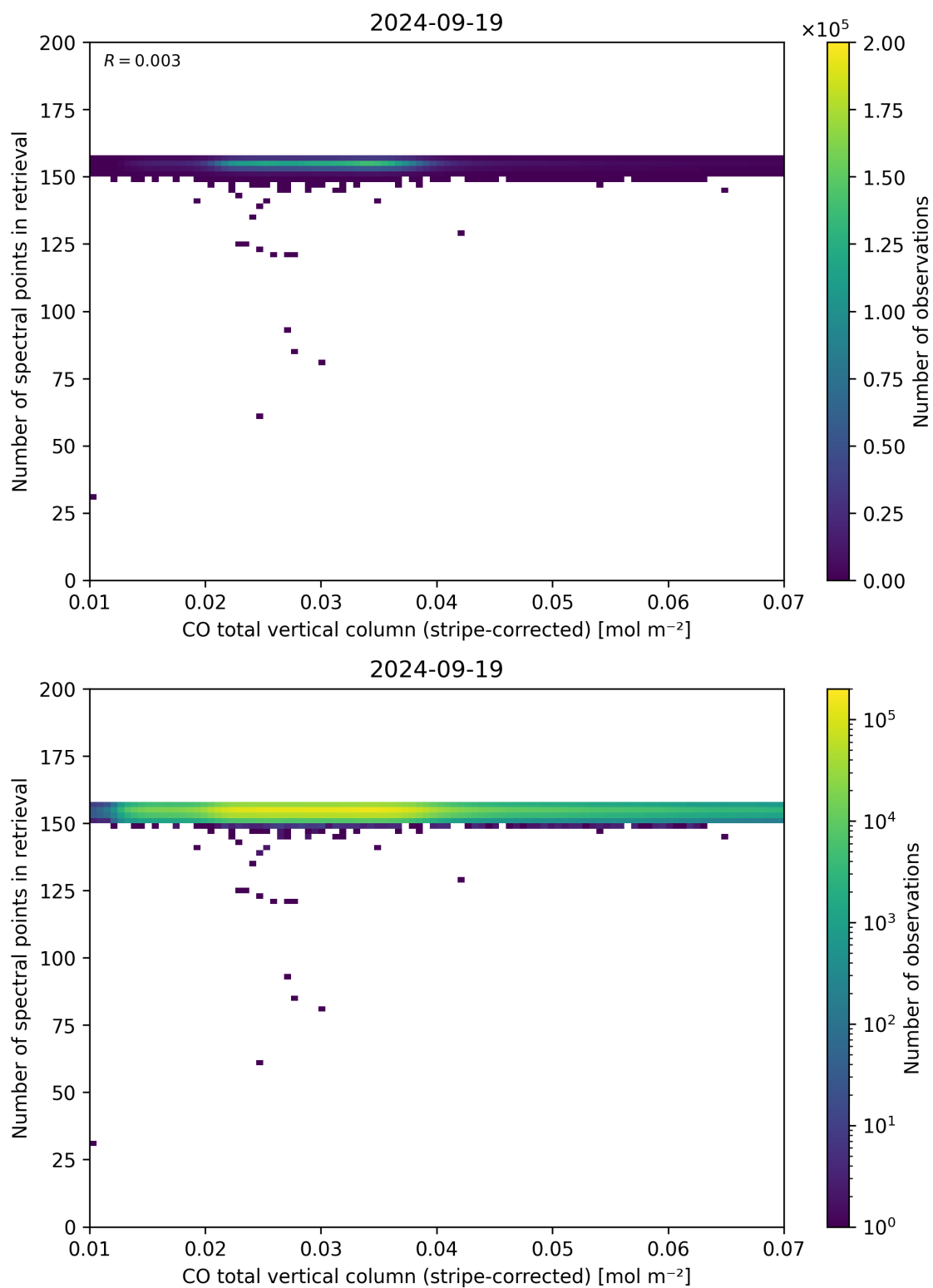
Figure 40: Scatter density plot of “CO total vertical column (stripe-corrected)” against “Number of spectral points in retrieval” for 2024-09-18 to 2024-09-20.
