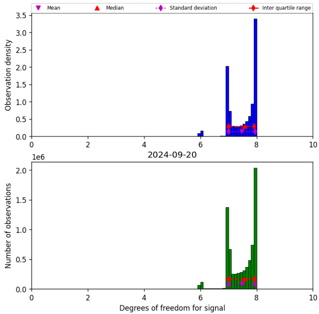
Figure 23: Histogram of “Degrees of freedom for signal” for 2024-09-19 to 2024-09-21
