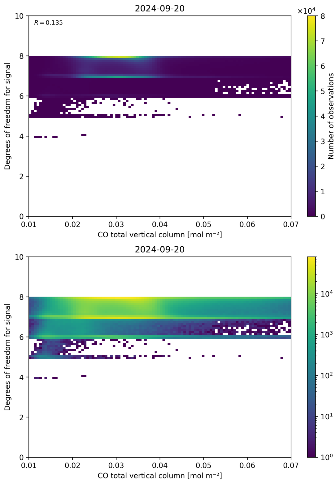
Figure 41: Scatter density plot of “CO total vertical column” against “Degrees of freedom for signal” for 2024-09-19 to 2024-09-21.
