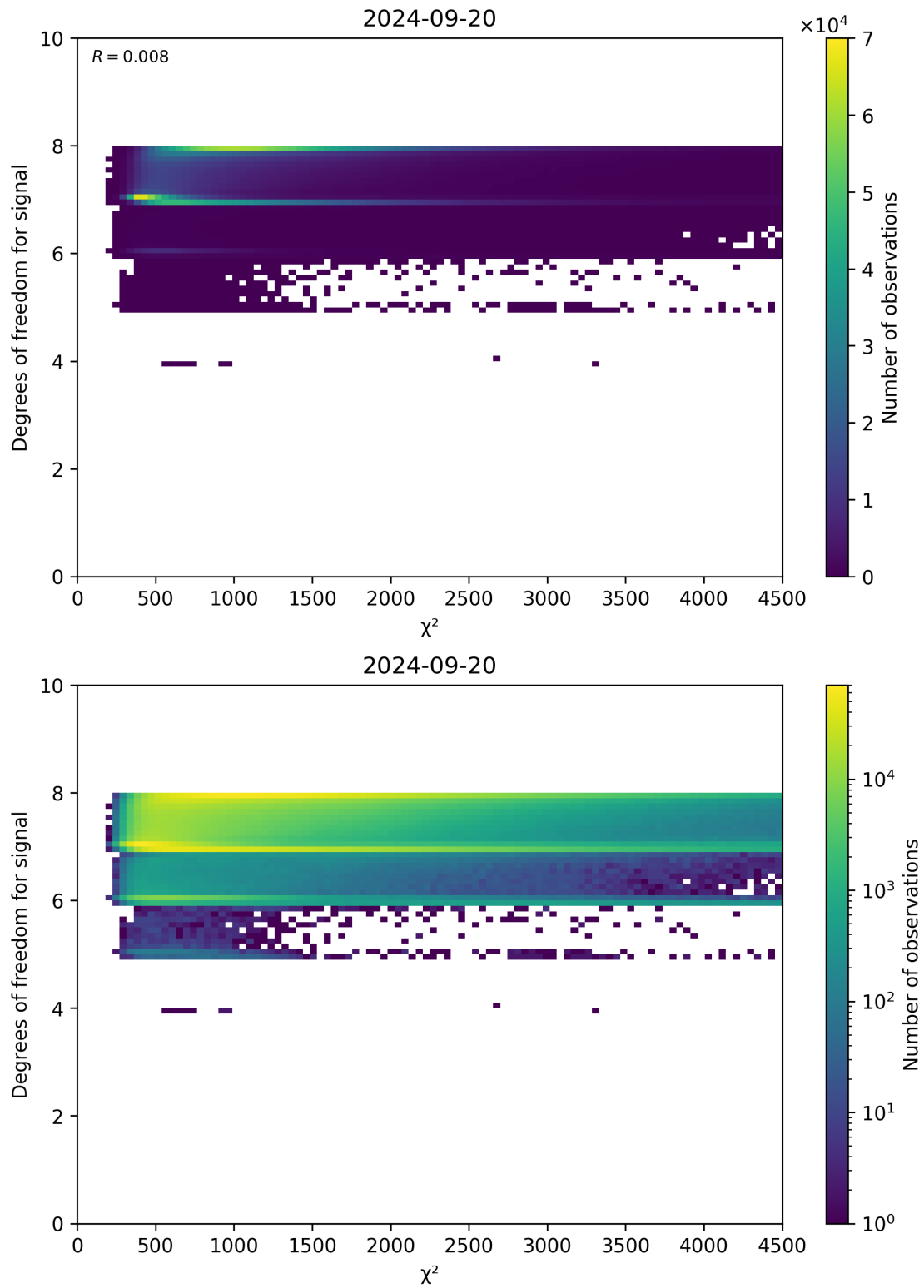
Figure 48: Scatter density plot of “ \chi^2 ” against “Degrees of freedom for signal” for 2024-09-19 to 2024-09-21.
