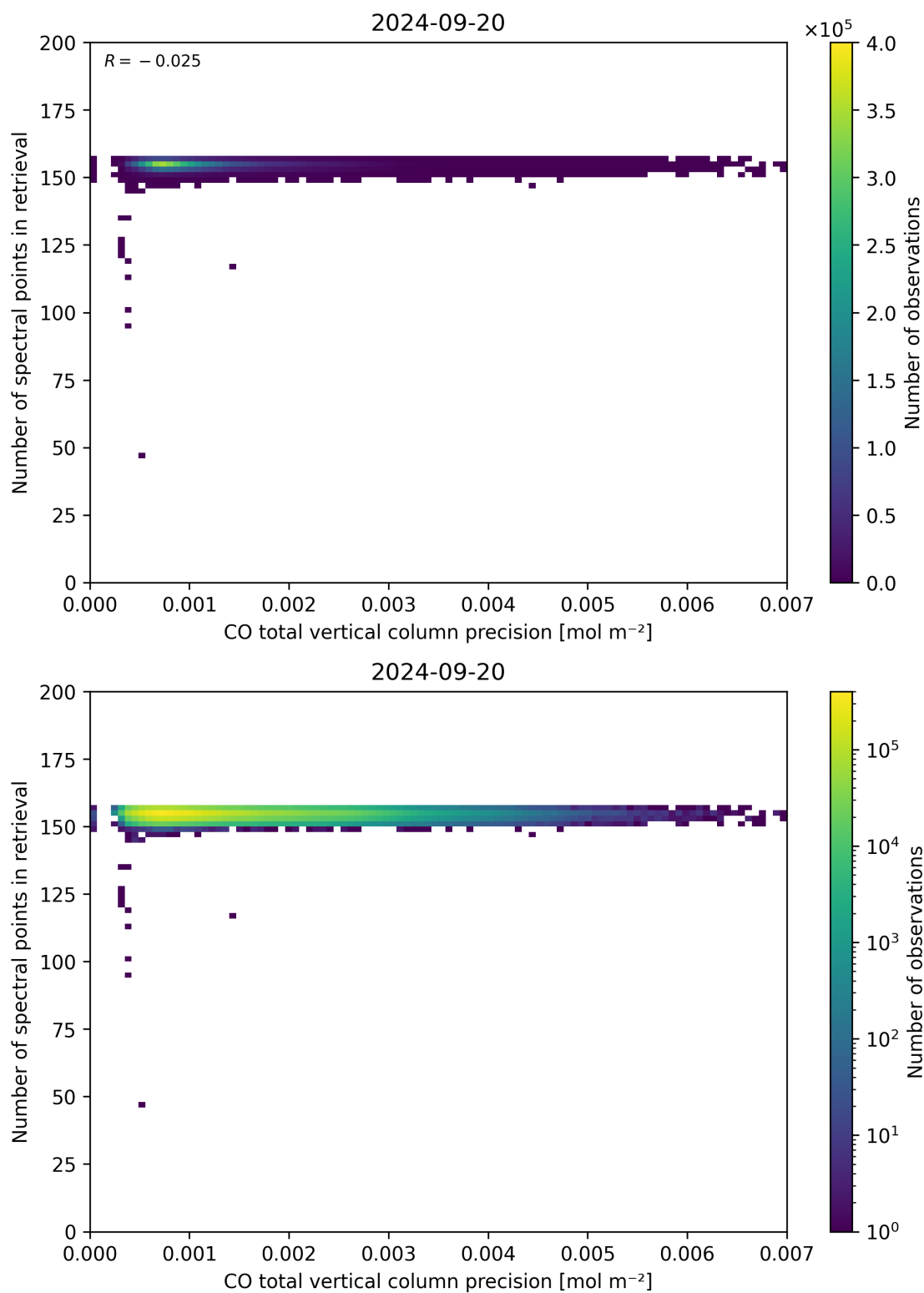
Figure 47: Scatter density plot of “CO total vertical column precision” against “Number of spectral points in retrieval” for 2024-09-19 to 2024-09-21.
