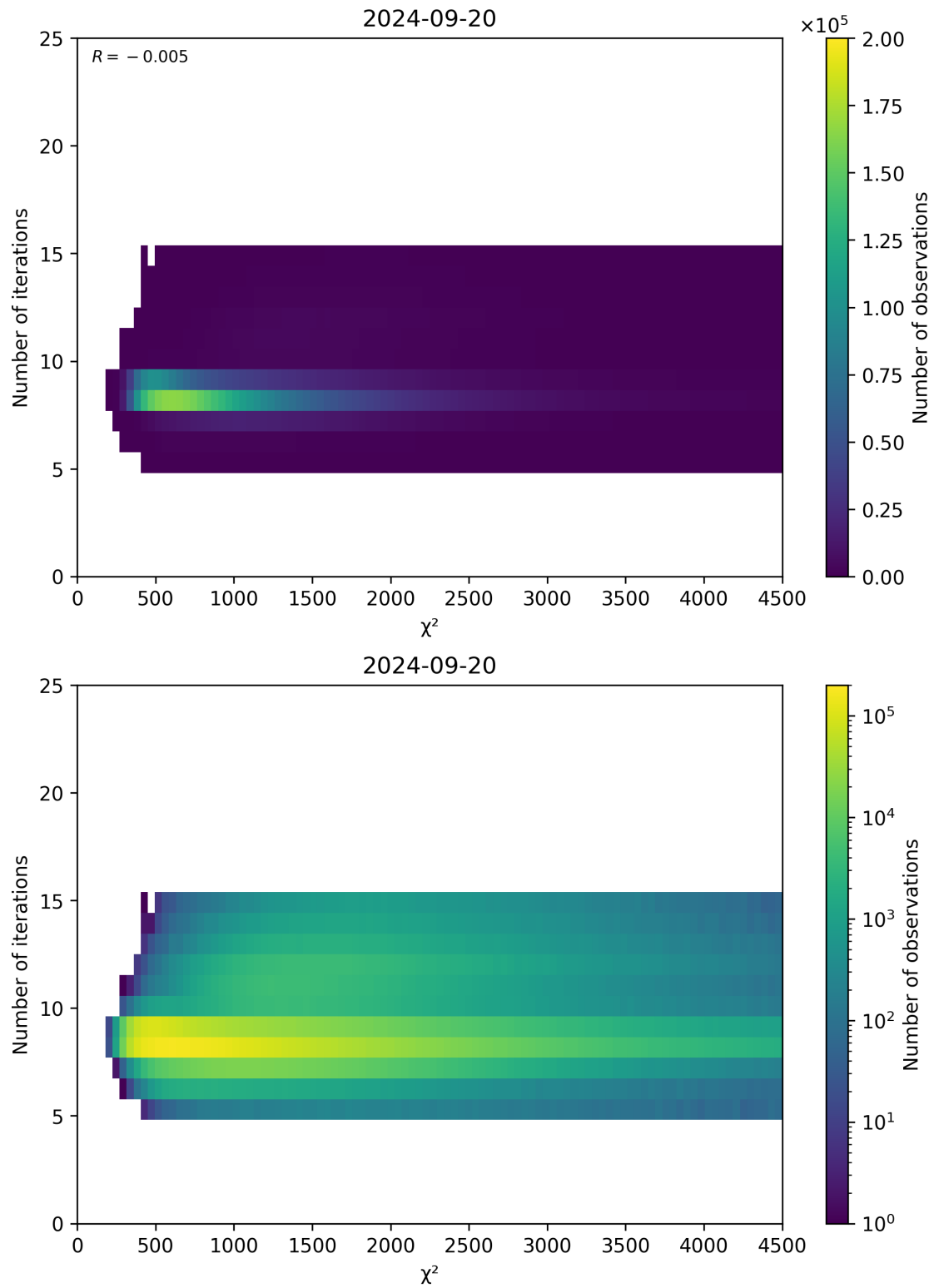
Figure 49: Scatter density plot of “ \chi^2 ” against “Number of iterations” for 2024-09-19 to 2024-09-21.
