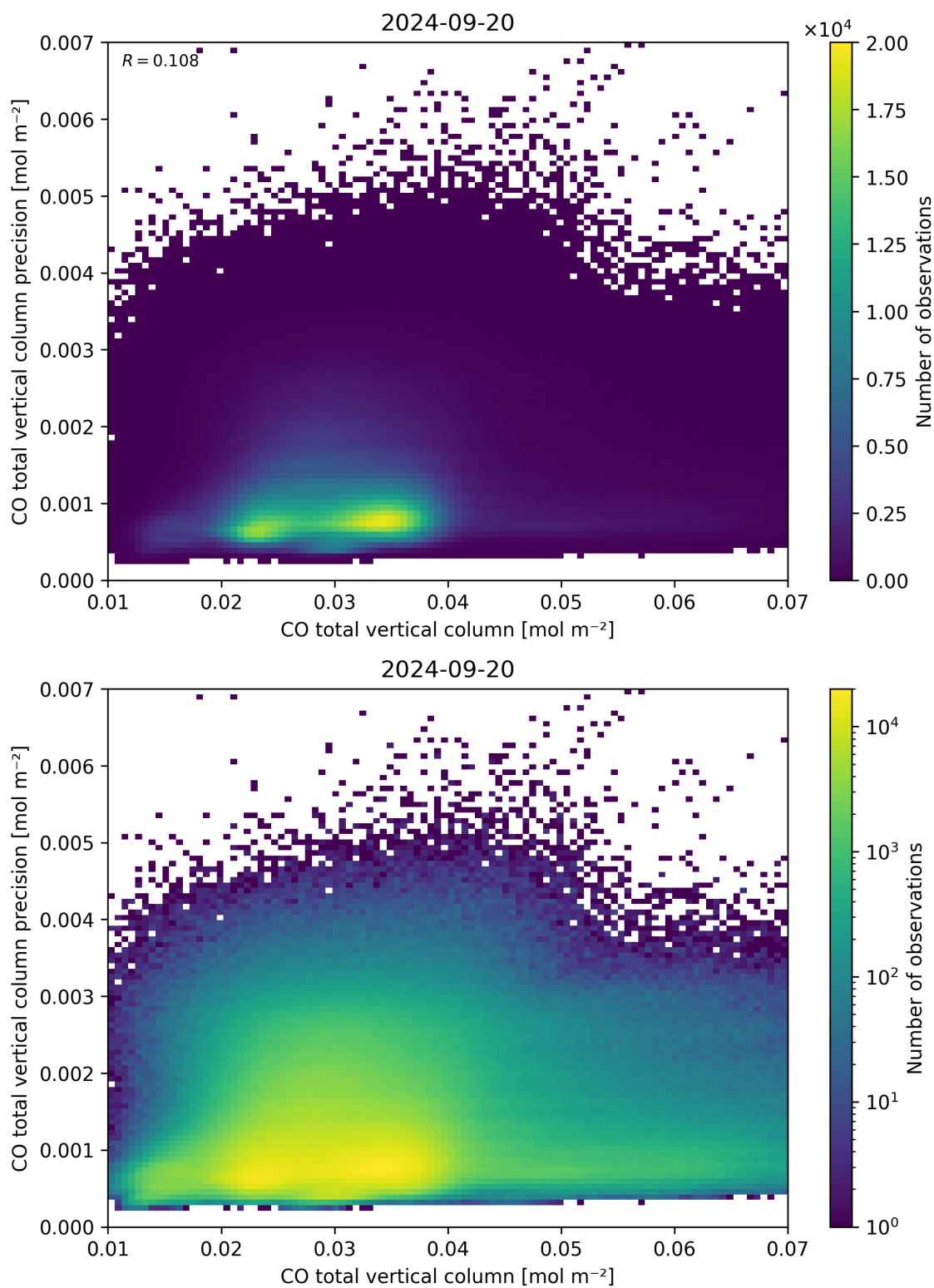
Figure 34: Scatter density plot of “CO total vertical column” against “CO total vertical column precision” for 2024-09-19 to 2024-09-21.
