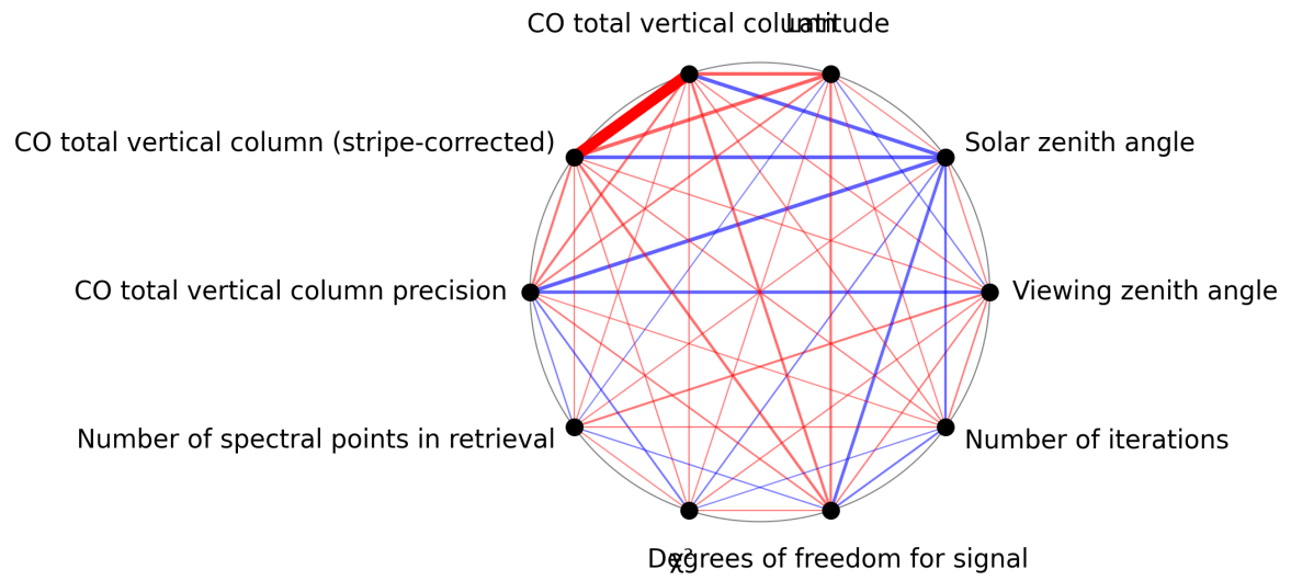
Figure 1: Map of correlation graph for 2024-09-19 to 2024-09-21.
