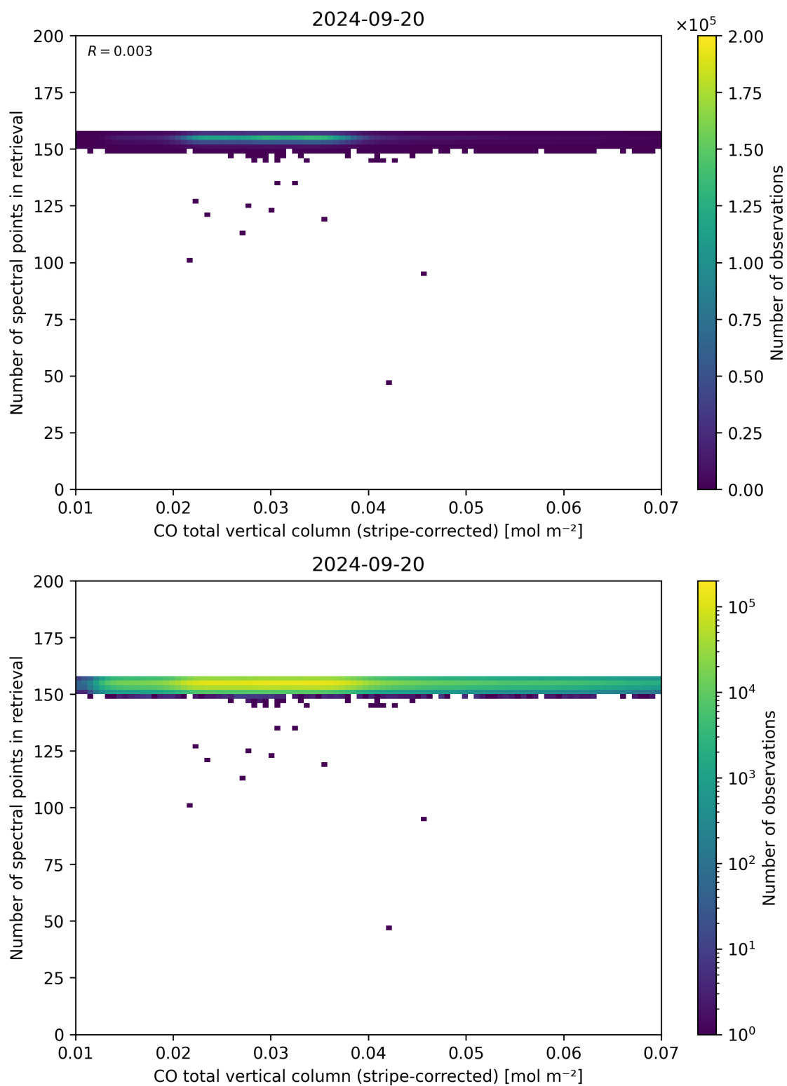
Figure 40: Scatter density plot of “CO total vertical column (stripe-corrected)” against “Number of spectral points in retrieval” for 2024-09-19 to 2024-09-21.
