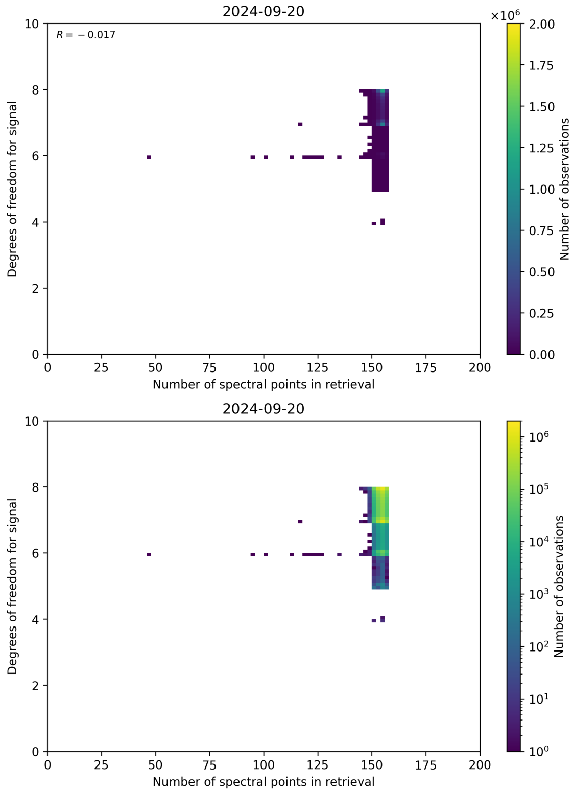
Figure 59: Scatter density plot of “Number of spectral points in retrieval” against “Degrees of freedom for signal” for 2024-09-19 to 2024-09-21.
