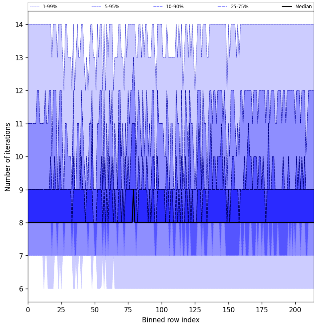
Figure 32: Along track statistics of “Number of iterations” for 2024-09-19 to 2024-09-21
