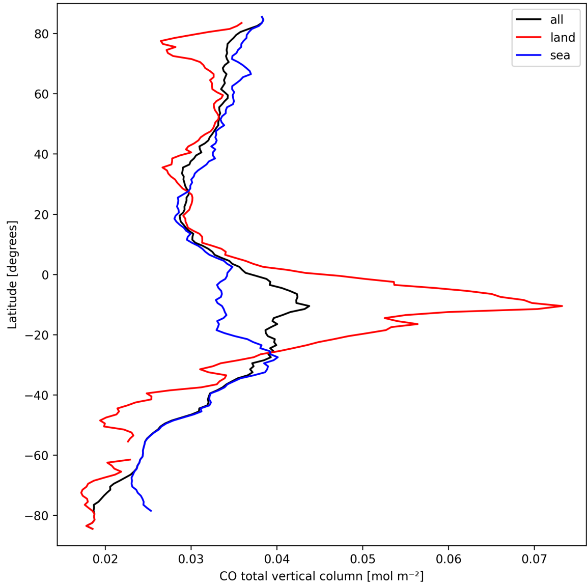
Figure 10: Zonal average of “CO total vertical column” for 2024-09-19 to 2024-09-21.
