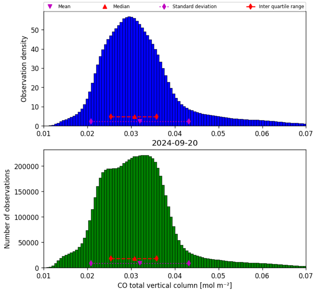
Figure 18: Histogram of “CO total vertical column” for 2024-09-19 to 2024-09-21
