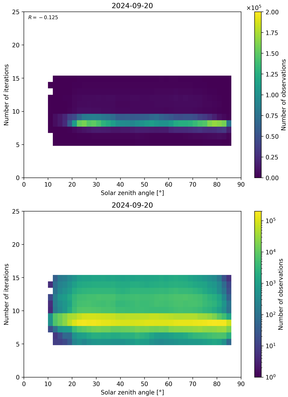
Figure 67: Scatter density plot of “Solar zenith angle” against “Number of iterations” for 2024-09-19 to 2024-09-21.
