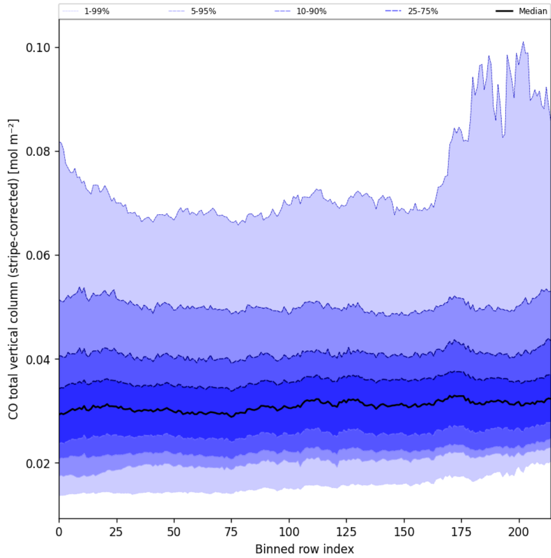
Figure 27: Along track statistics of “CO total vertical column (stripe-corrected)” for 2024-09-19 to 2024-09-21
