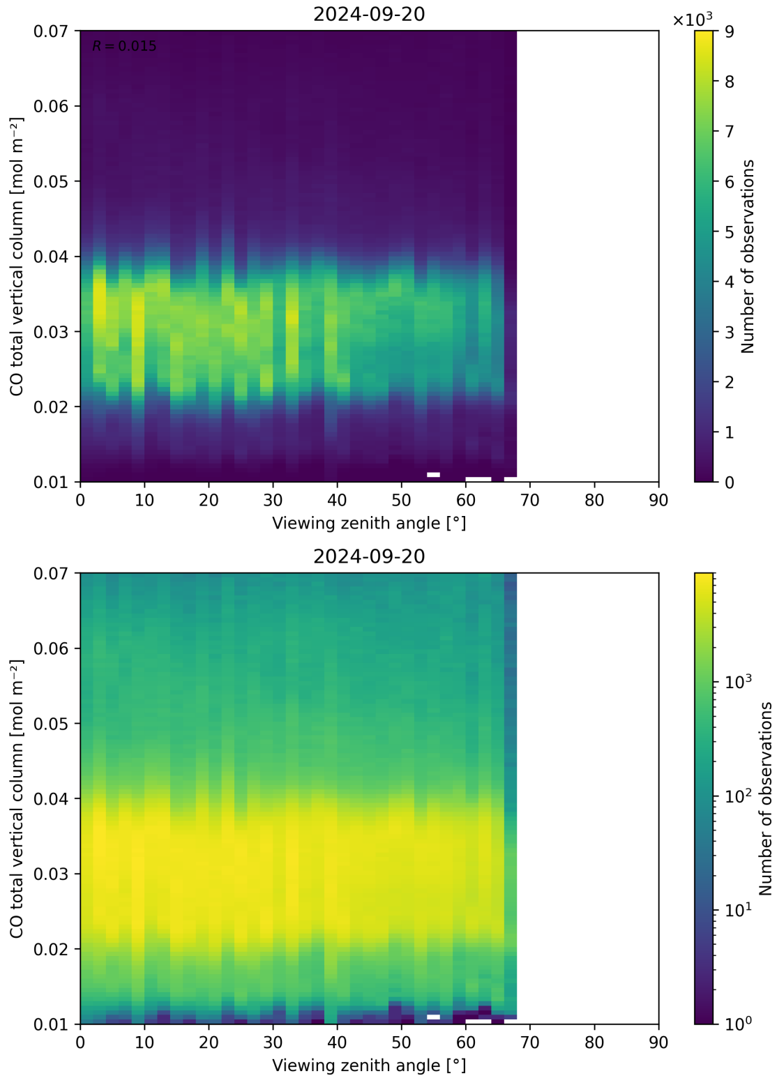
Figure 69: Scatter density plot of “Viewing zenith angle” against “CO total vertical column” for 2024-09-19 to 2024-09-21.
