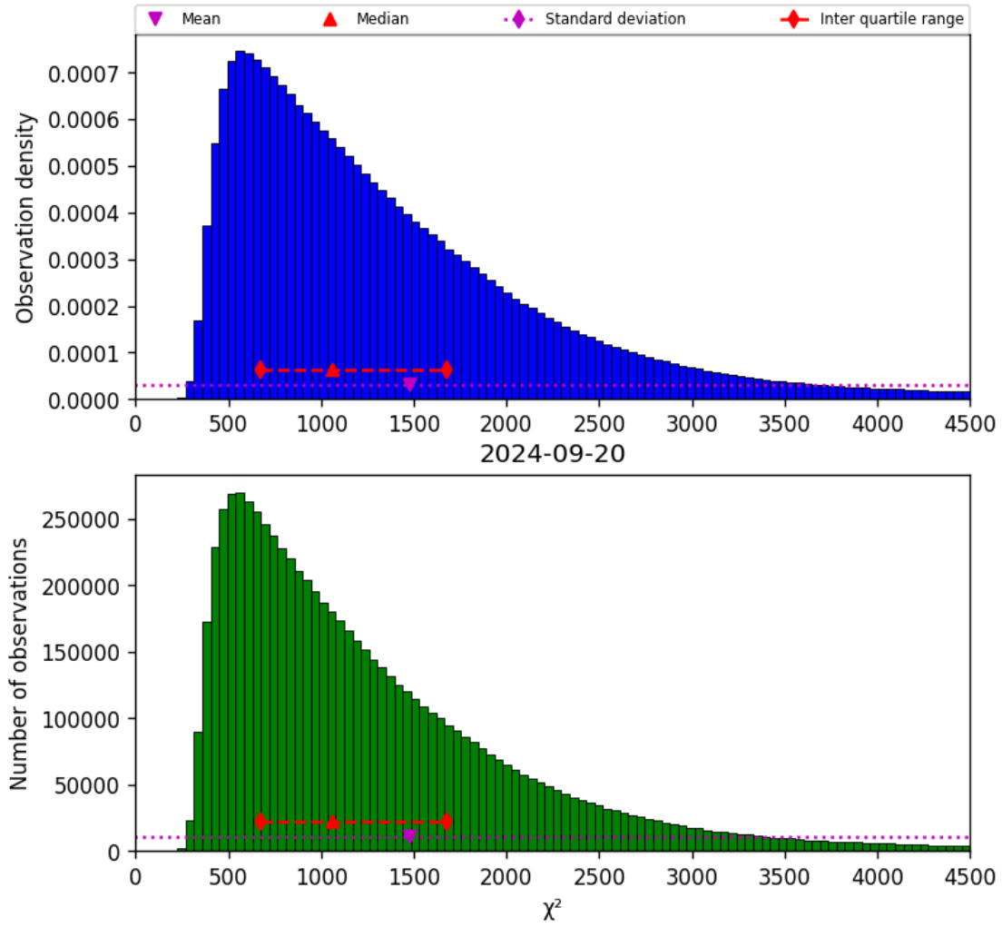
Figure 22: Histogram of “ \chi^2 ” for 2024-09-19 to 2024-09-21
