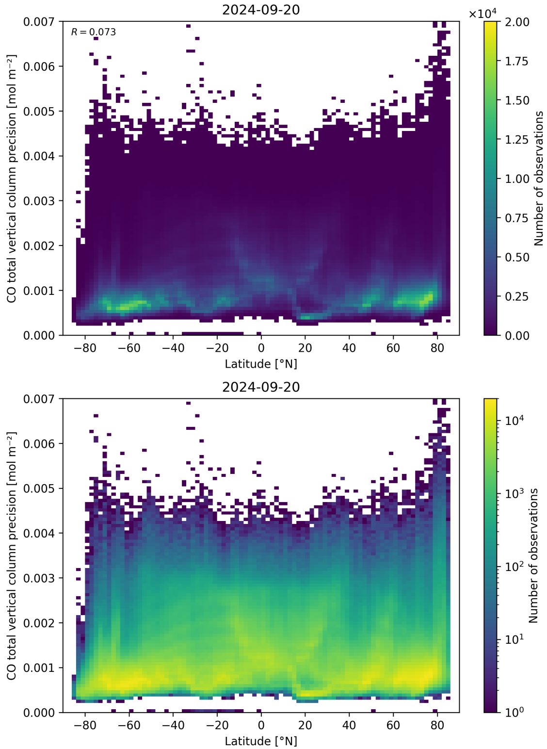
Figure 53: Scatter density plot of “Latitude” against “CO total vertical column precision” for 2024-09-19 to 2024-09-21.
