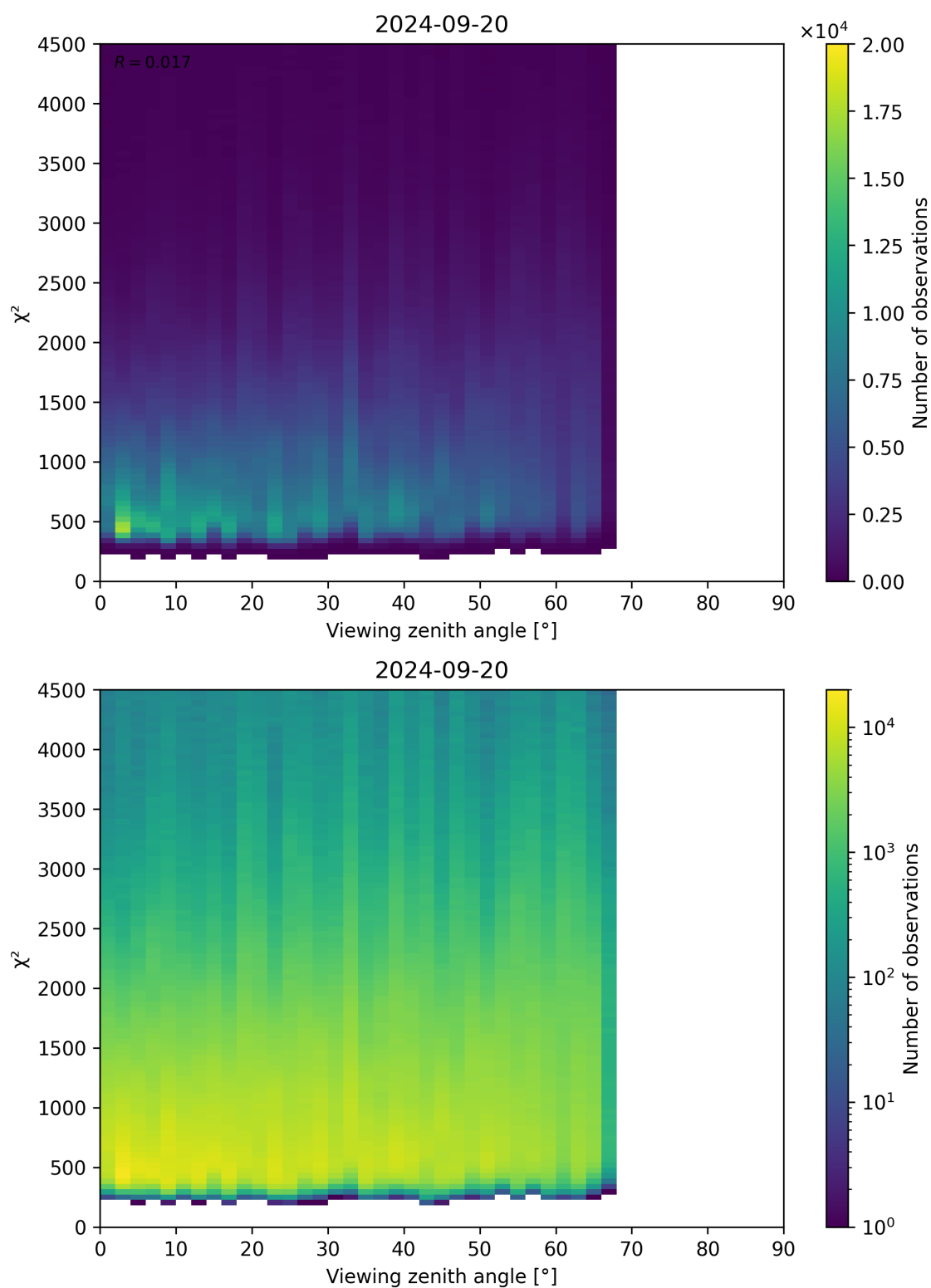
Figure 72: Scatter density plot of “Viewing zenith angle” against “ \chi^2 ” for 2024-09-19 to 2024-09-21.
