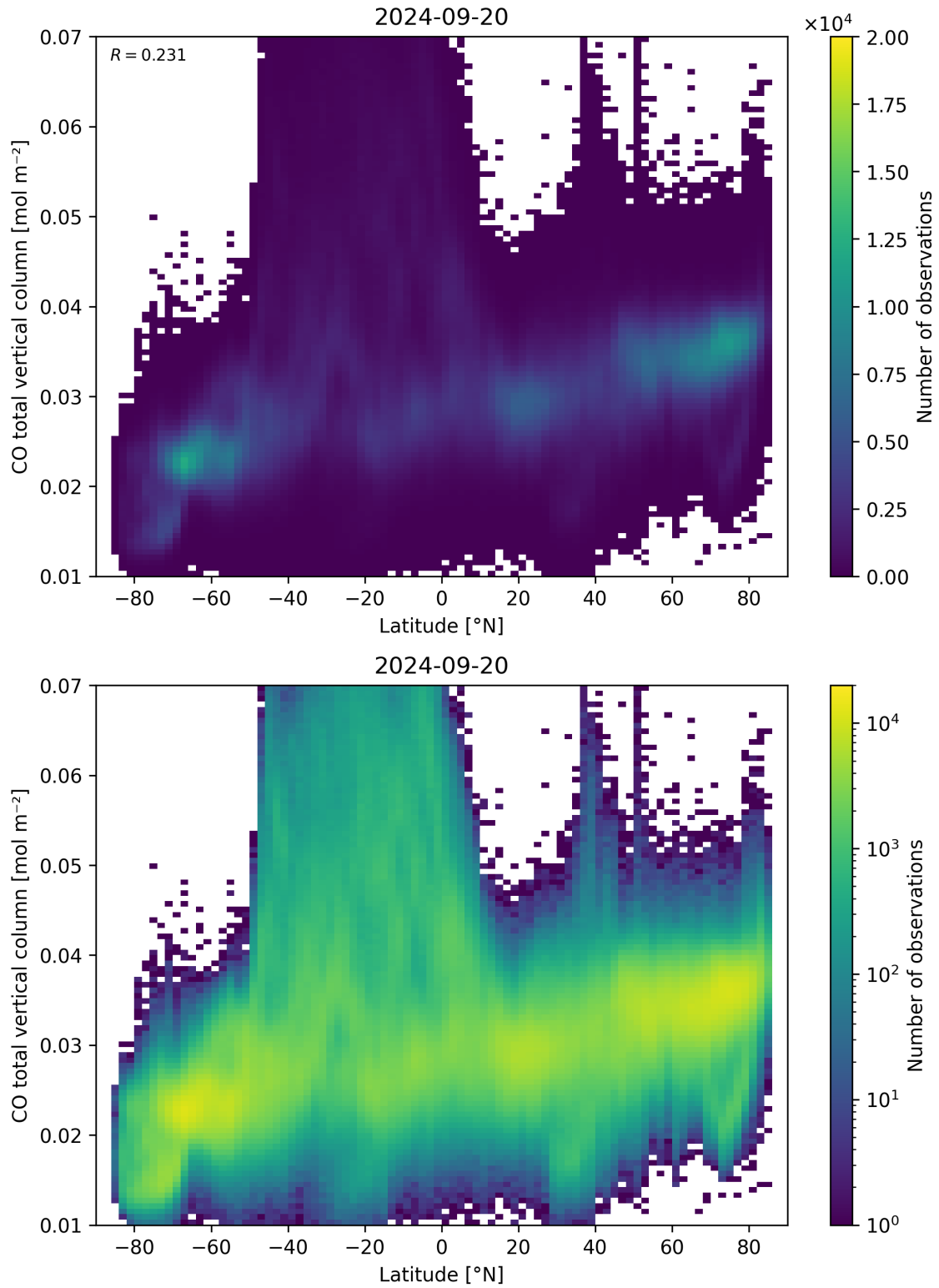
Figure 51: Scatter density plot of “Latitude” against “CO total vertical column” for 2024-09-19 to 2024-09-21.
