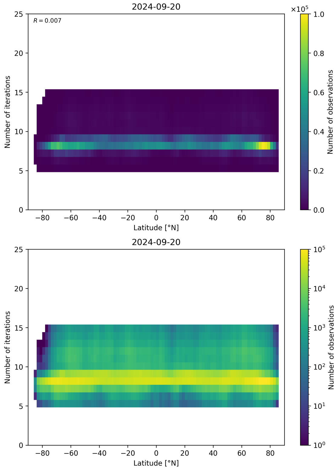
Figure 56: Scatter density plot of “Latitude” against “Number of iterations” for 2024-09-19 to 2024-09-21.
