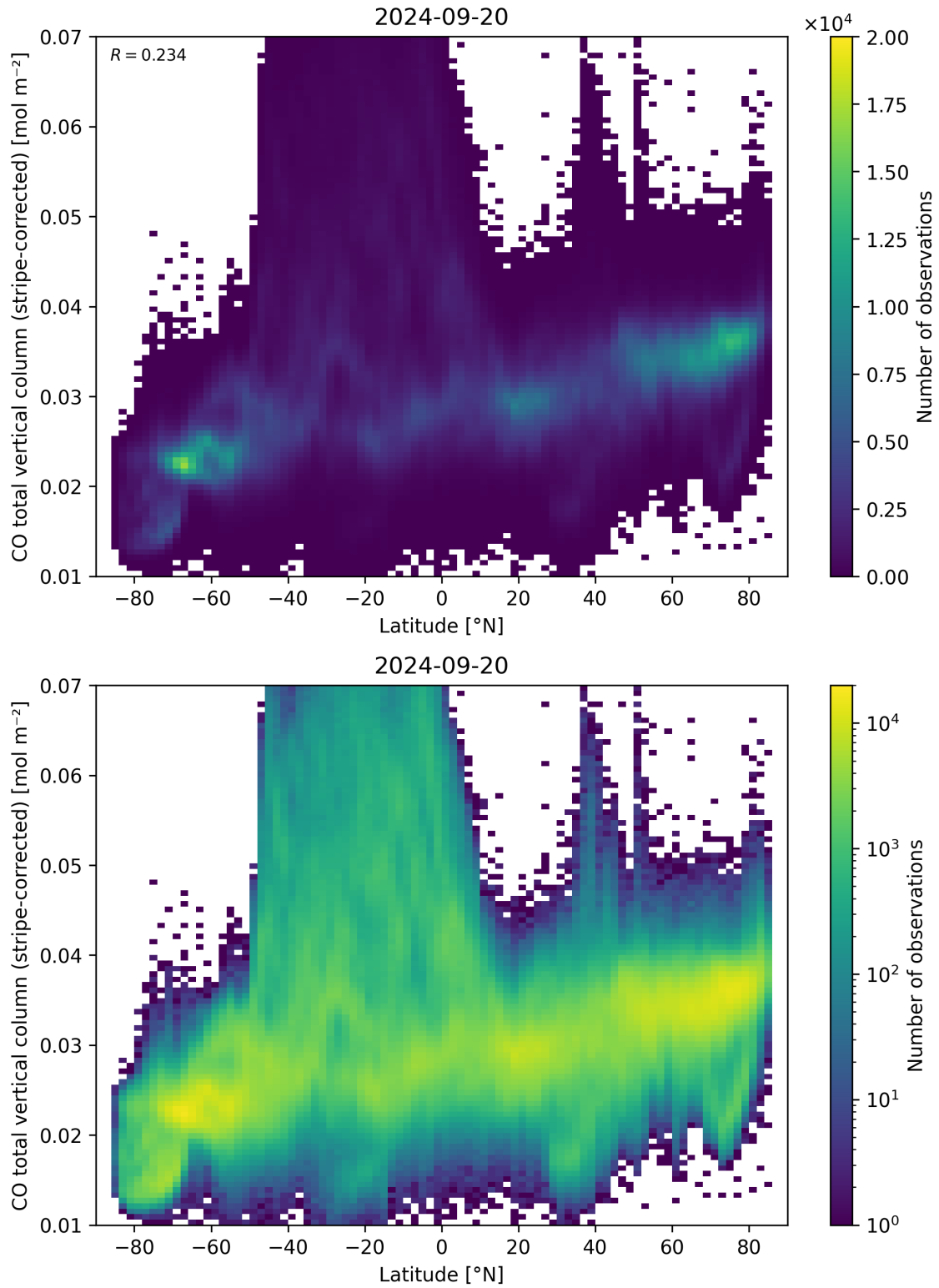
Figure 52: Scatter density plot of “Latitude” against “CO total vertical column (stripe-corrected)” for 2024-09-19 to 2024-09-21.
