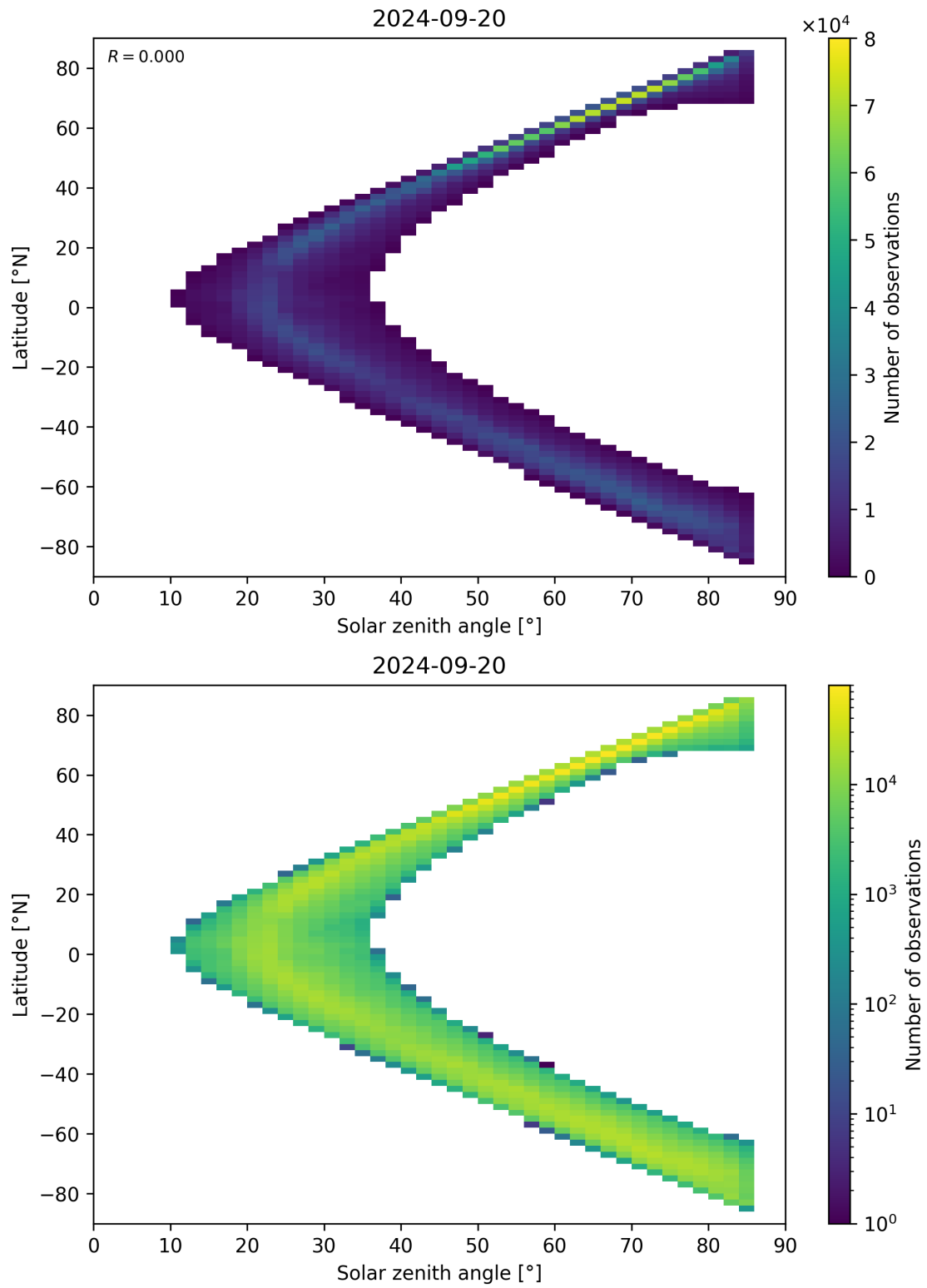
Figure 66: Scatter density plot of “Solar zenith angle” against “Latitude” for 2024-09-19 to 2024-09-21.
