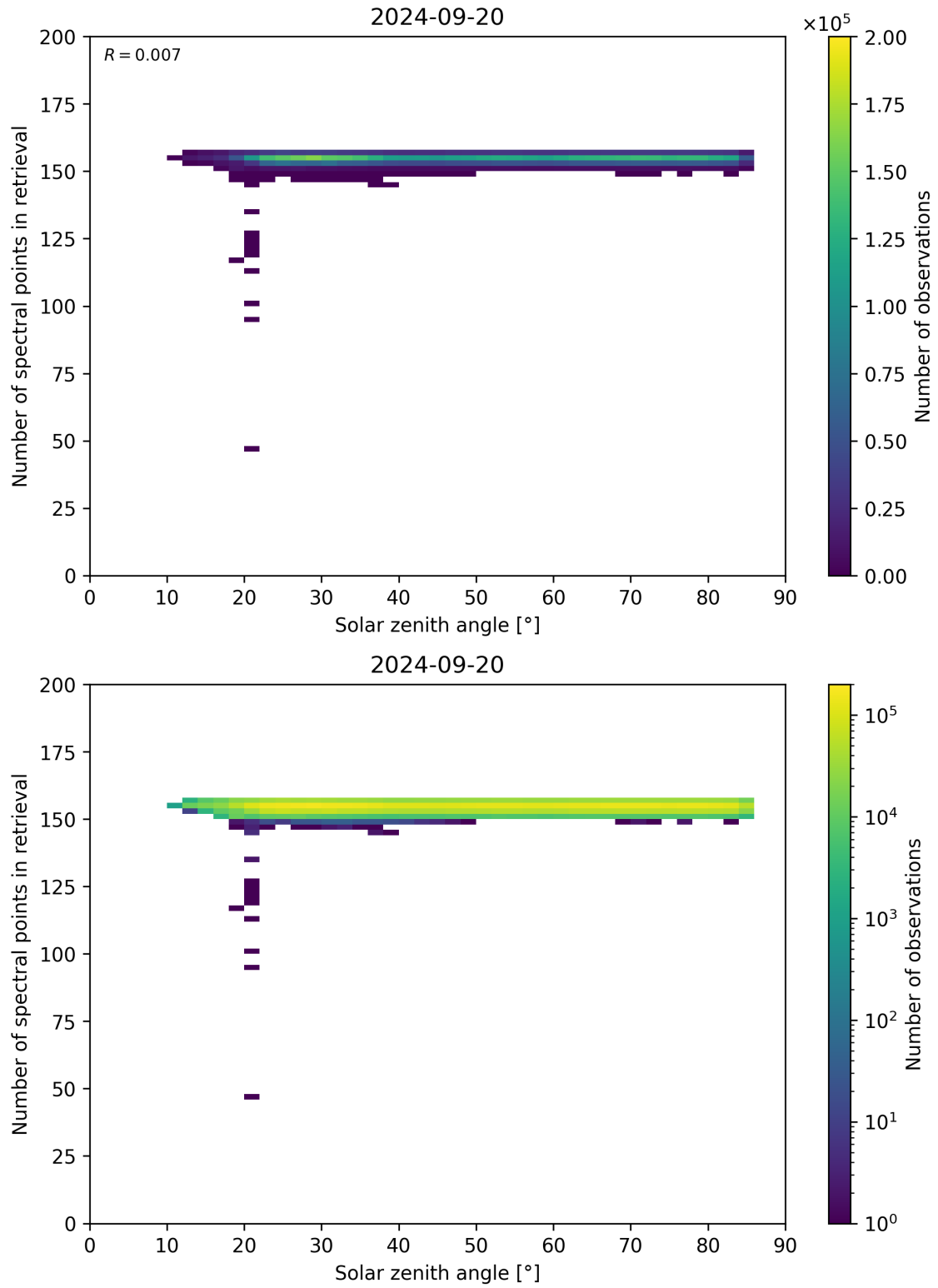
Figure 68: Scatter density plot of “Solar zenith angle” against “Number of spectral points in retrieval” for 2024-09-19 to 2024-09-21.
