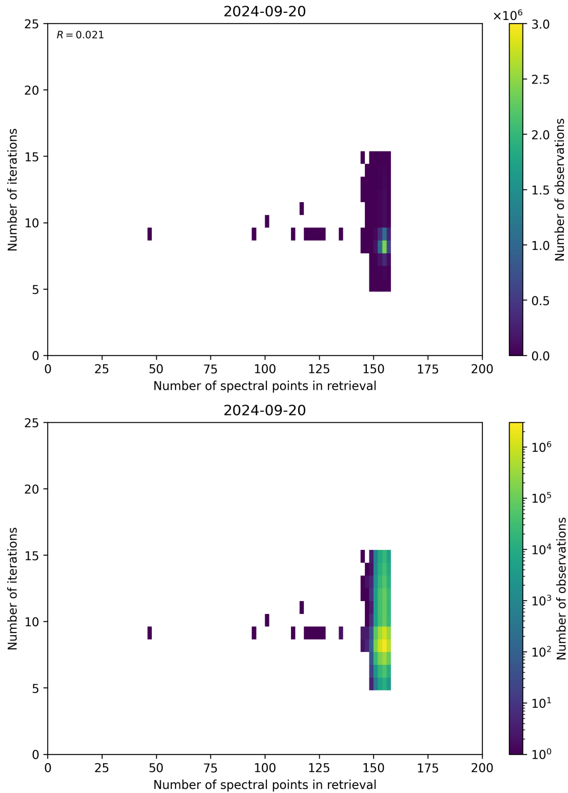
Figure 60: Scatter density plot of “Number of spectral points in retrieval” against “Number of iterations” for 2024-09-19 to 2024-09-21.
