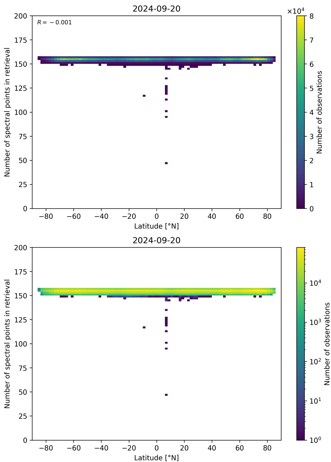
Figure 57: Scatter density plot of “Latitude” against “Number of spectral points in retrieval” for 2024-09-19 to 2024-09-21.
