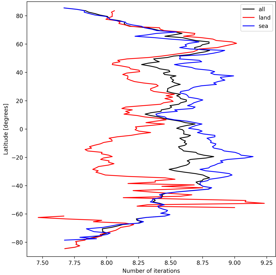
Figure 16: Zonal average of “Number of iterations” for 2024-09-19 to 2024-09-21.
