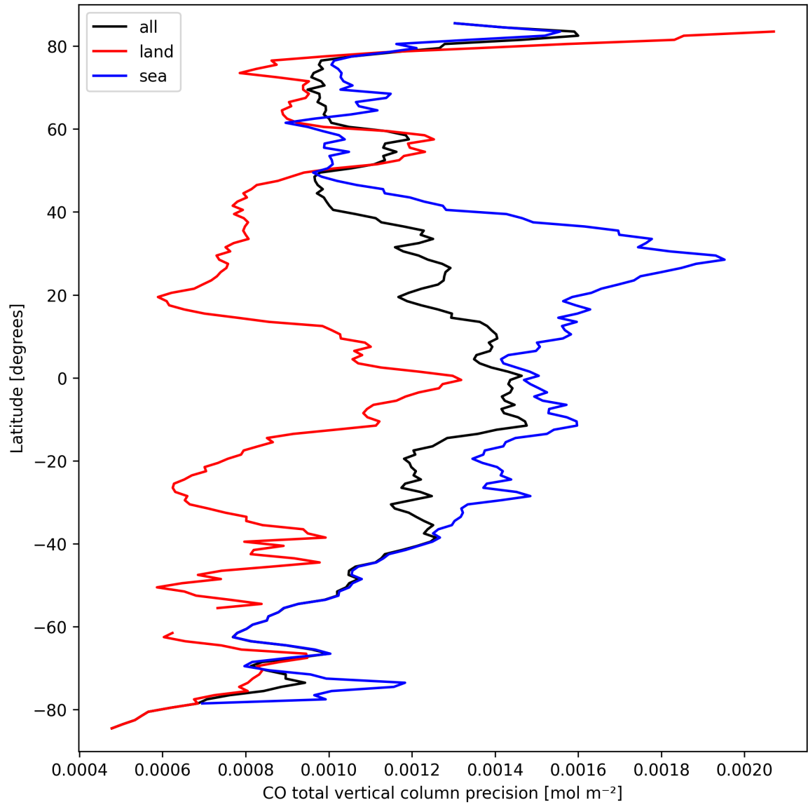
Figure 12: Zonal average of “CO total vertical column precision” for 2024-09-19 to 2024-09-21.
