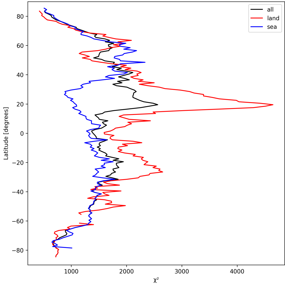
Figure 14: Zonal average of “ \chi^2 ” for 2024-09-19 to 2024-09-21.
