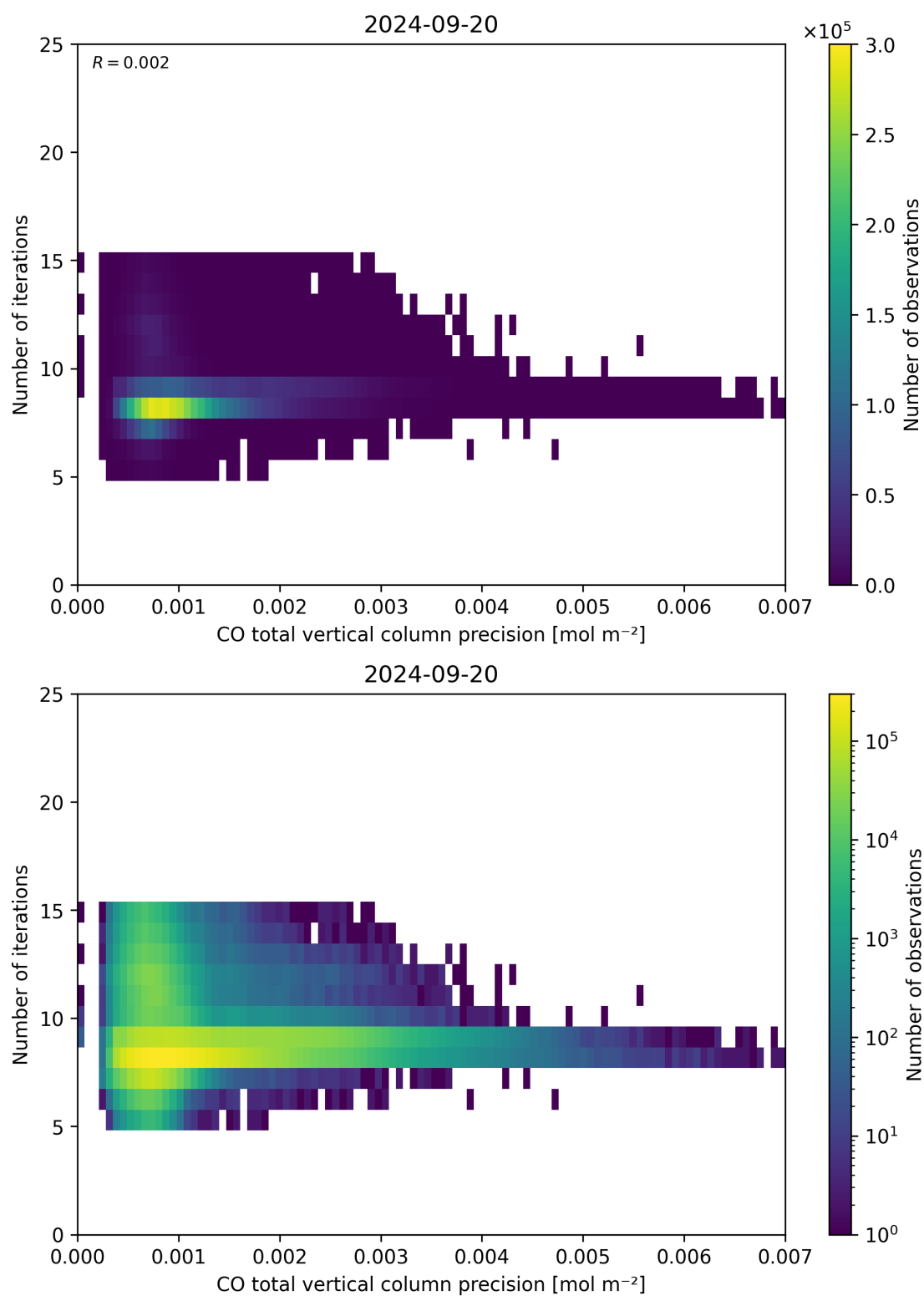
Figure 46: Scatter density plot of “CO total vertical column precision” against “Number of iterations” for 2024-09-19 to 2024-09-21.
