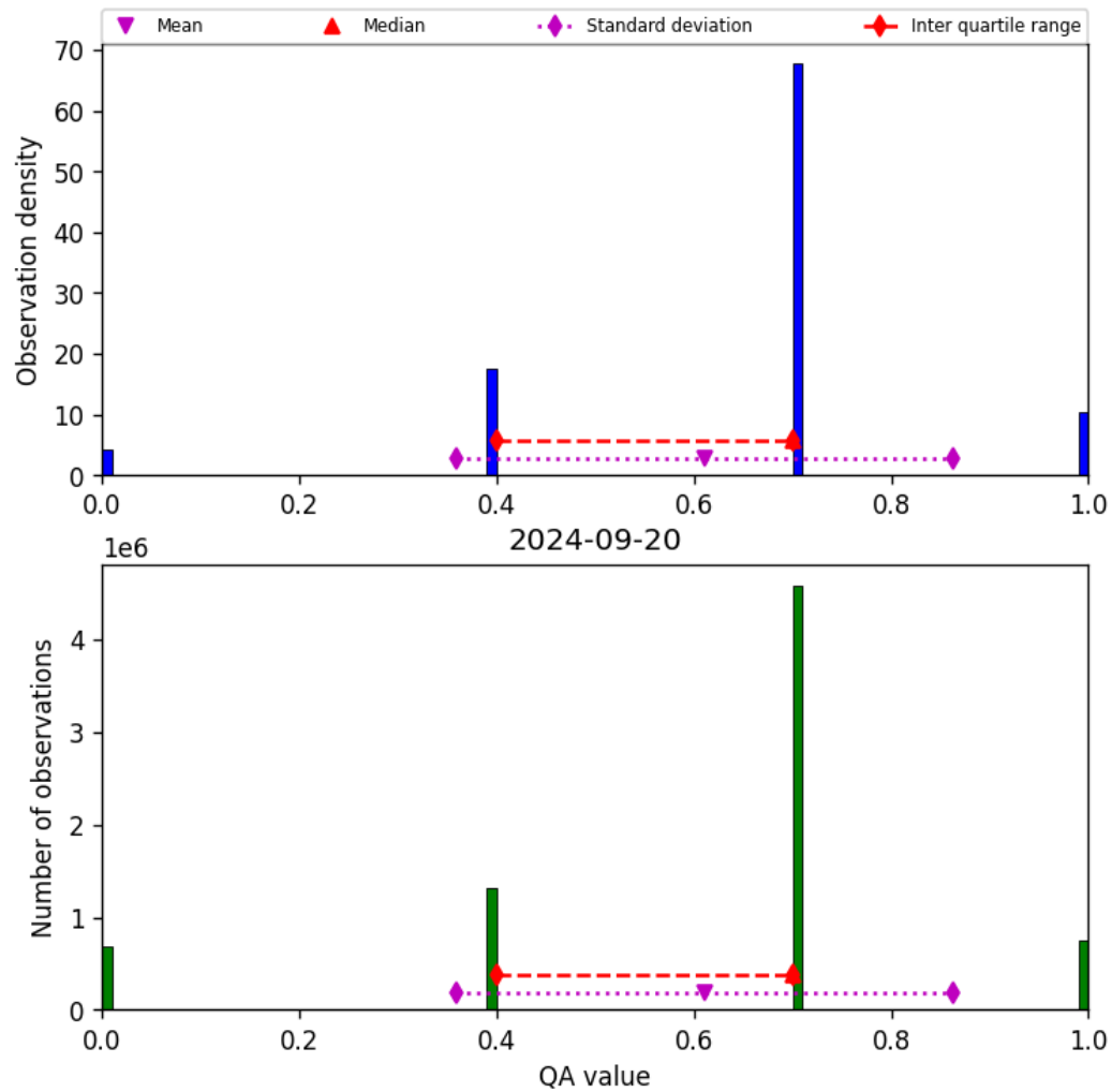
Figure 17: Histogram of “QA value” for 2024-09-19 to 2024-09-21
