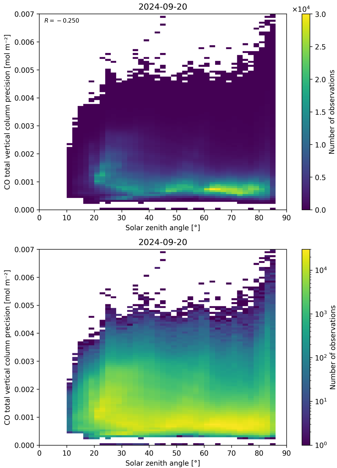
Figure 63: Scatter density plot of “Solar zenith angle” against “CO total vertical column precision” for 2024-09-19 to 2024-09-21.
