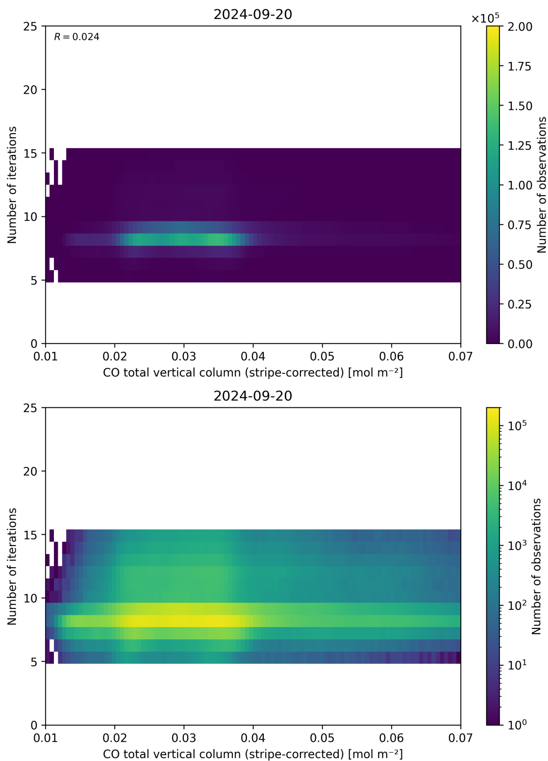
Figure 39: Scatter density plot of “CO total vertical column (stripe-corrected)” against “Number of iterations” for 2024-09-19 to 2024-09-21.
