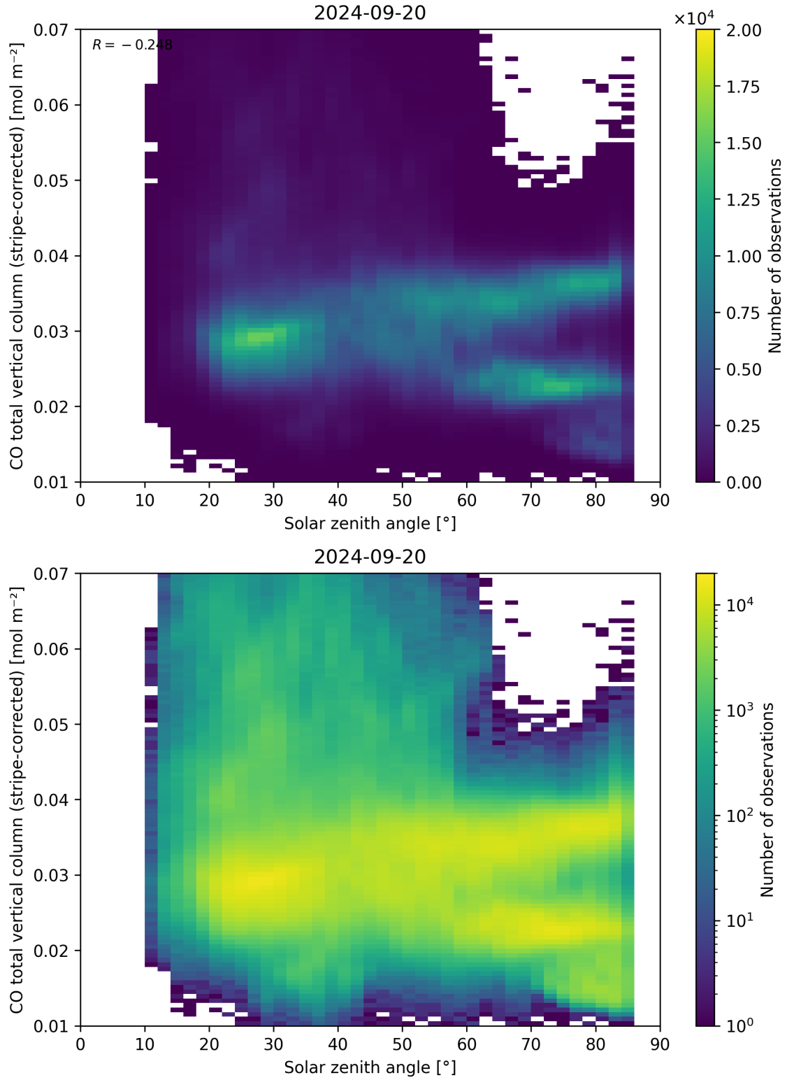
Figure 62: Scatter density plot of “Solar zenith angle” against “CO total vertical column (stripe-corrected)” for 2024-09-19 to 2024-09-21.
