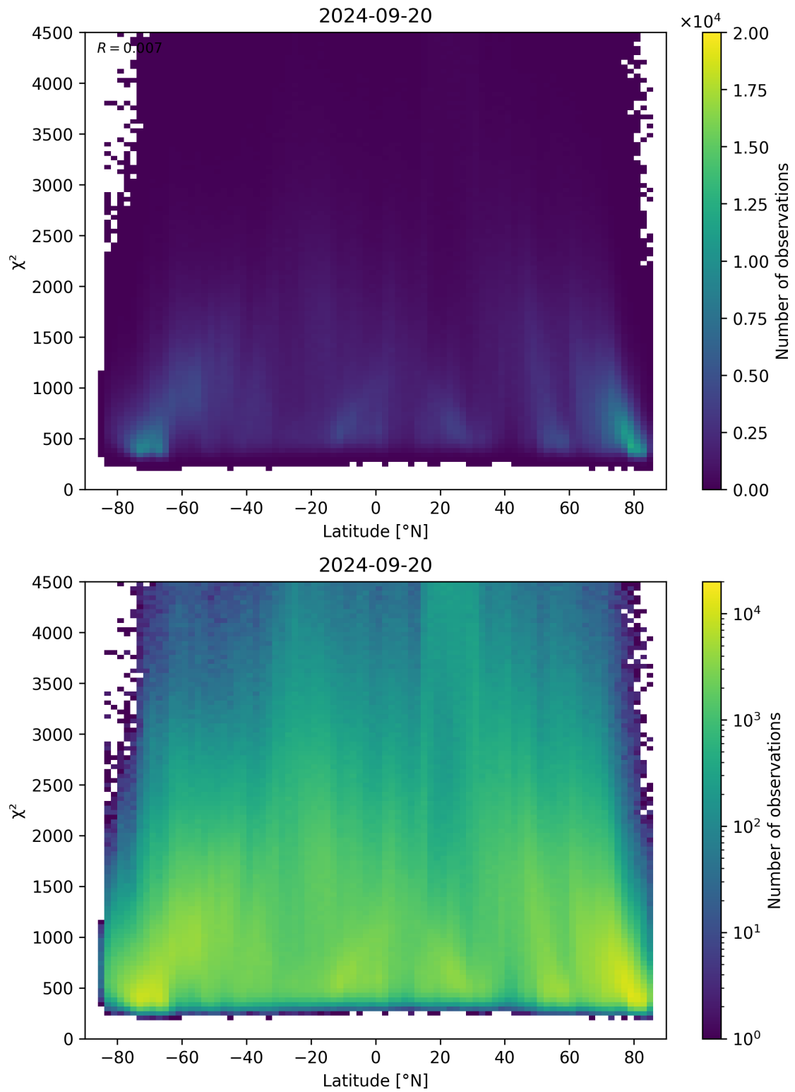
Figure 54: Scatter density plot of “Latitude” against “ \chi^2 ” for 2024-09-19 to 2024-09-21.
