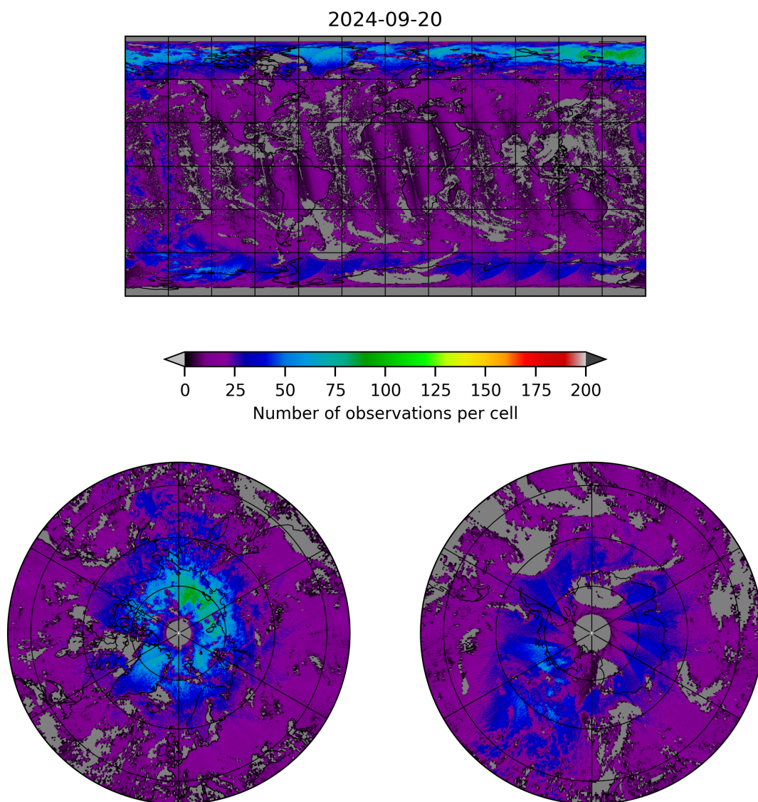
Figure 8: Map of the number of observations for 2024-09-19 to 2024-09-21
