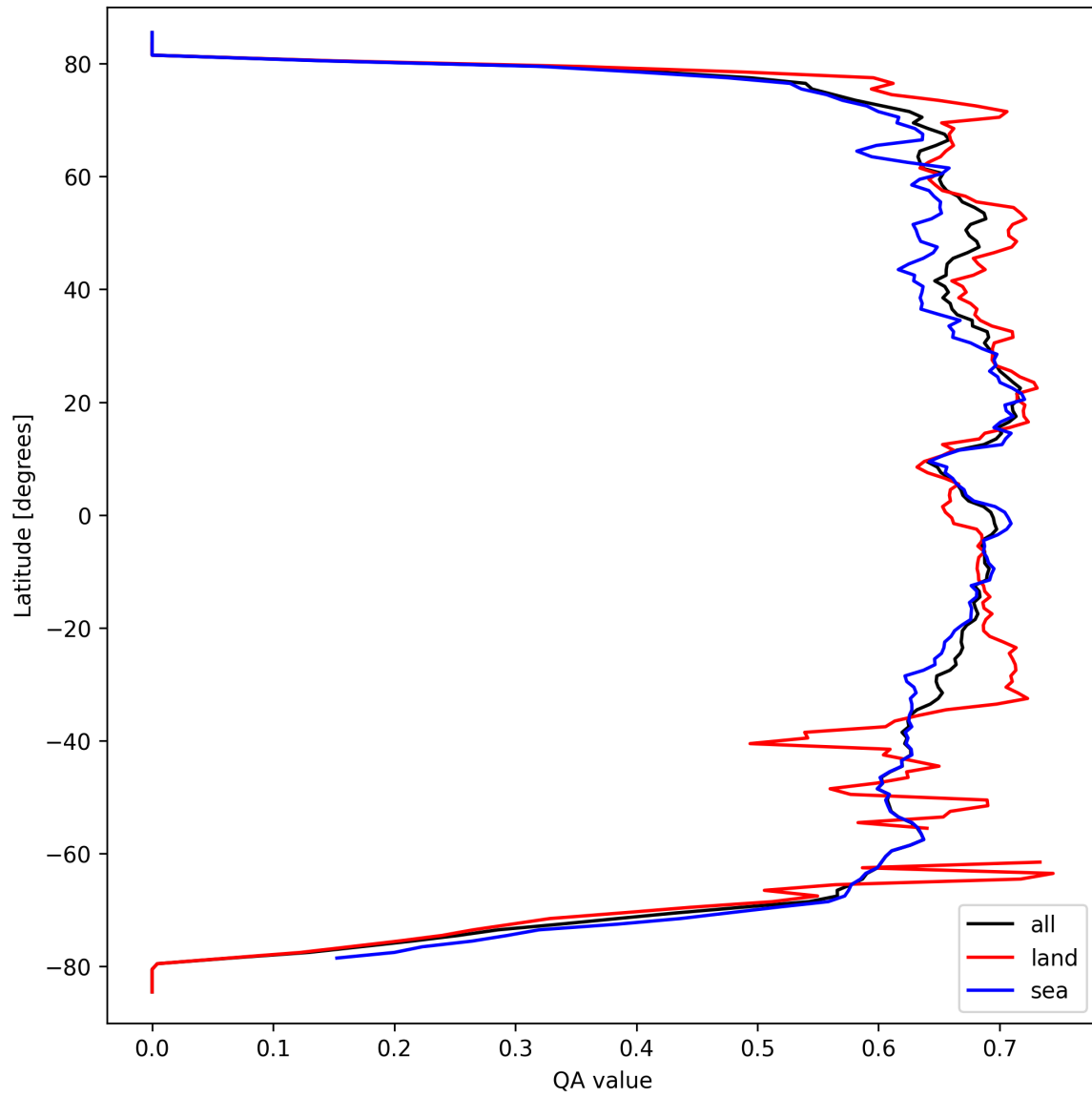
Figure 9: Zonal average of “QA value” for 2024-09-19 to 2024-09-21.
