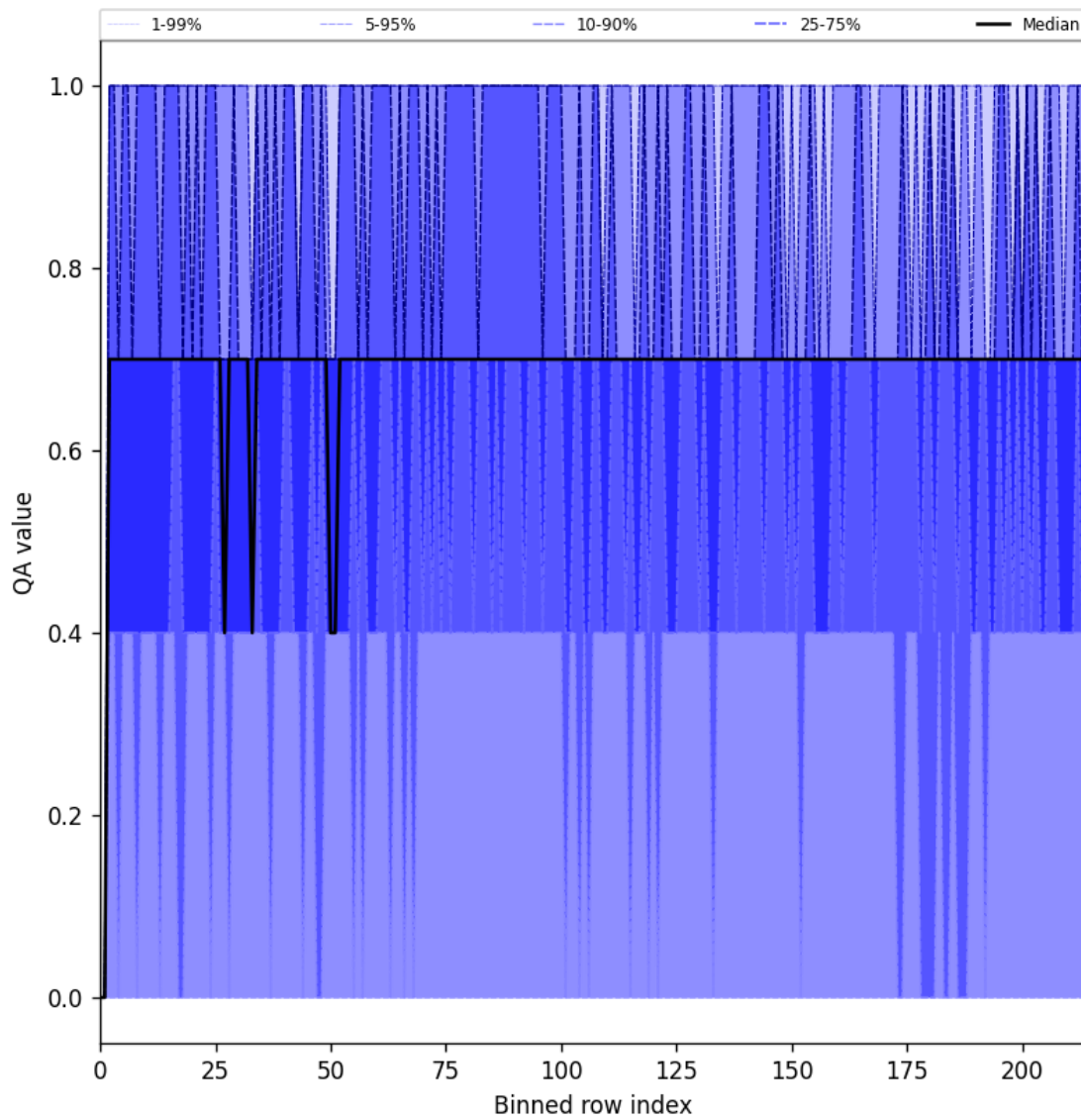
Figure 25: Along track statistics of “QA value” for 2024-09-19 to 2024-09-21
