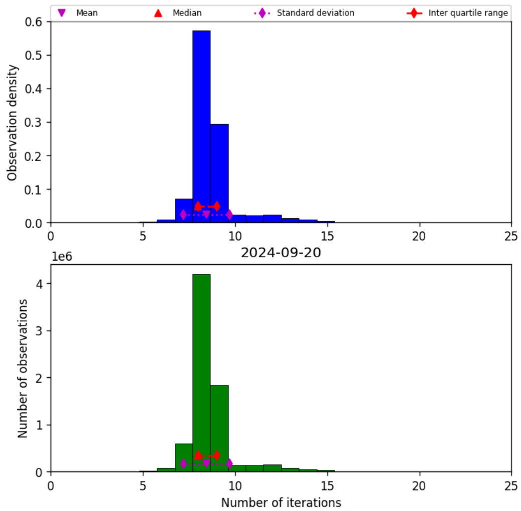
Figure 24: Histogram of “Number of iterations” for 2024-09-19 to 2024-09-21
