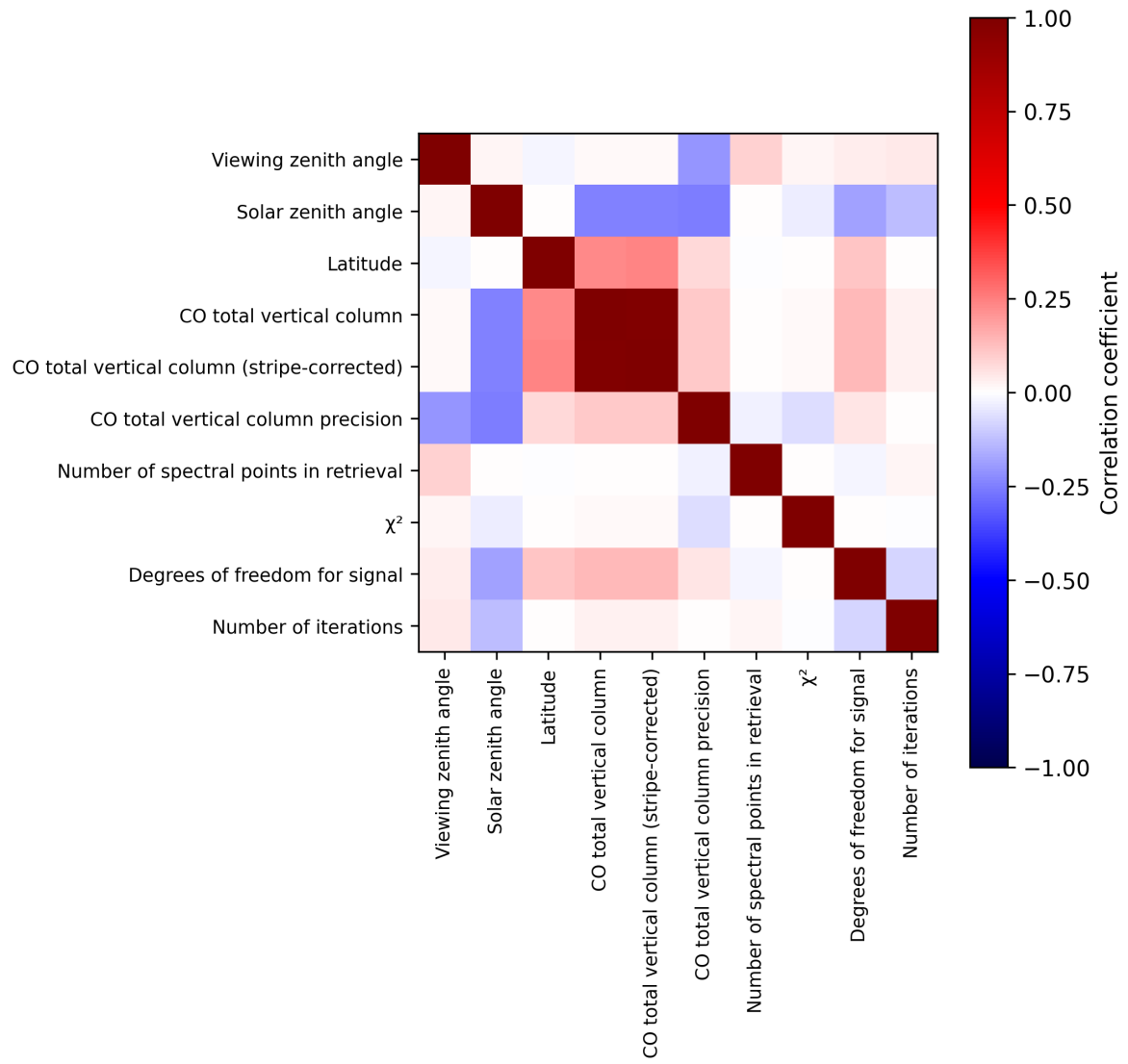
Figure 2: Map of correlation matrix for 2024-09-19 to 2024-09-21.
