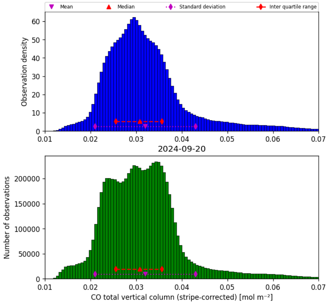
Figure 19: Histogram of “CO total vertical column (stripe-corrected)” for 2024-09-19 to 2024-09-21
