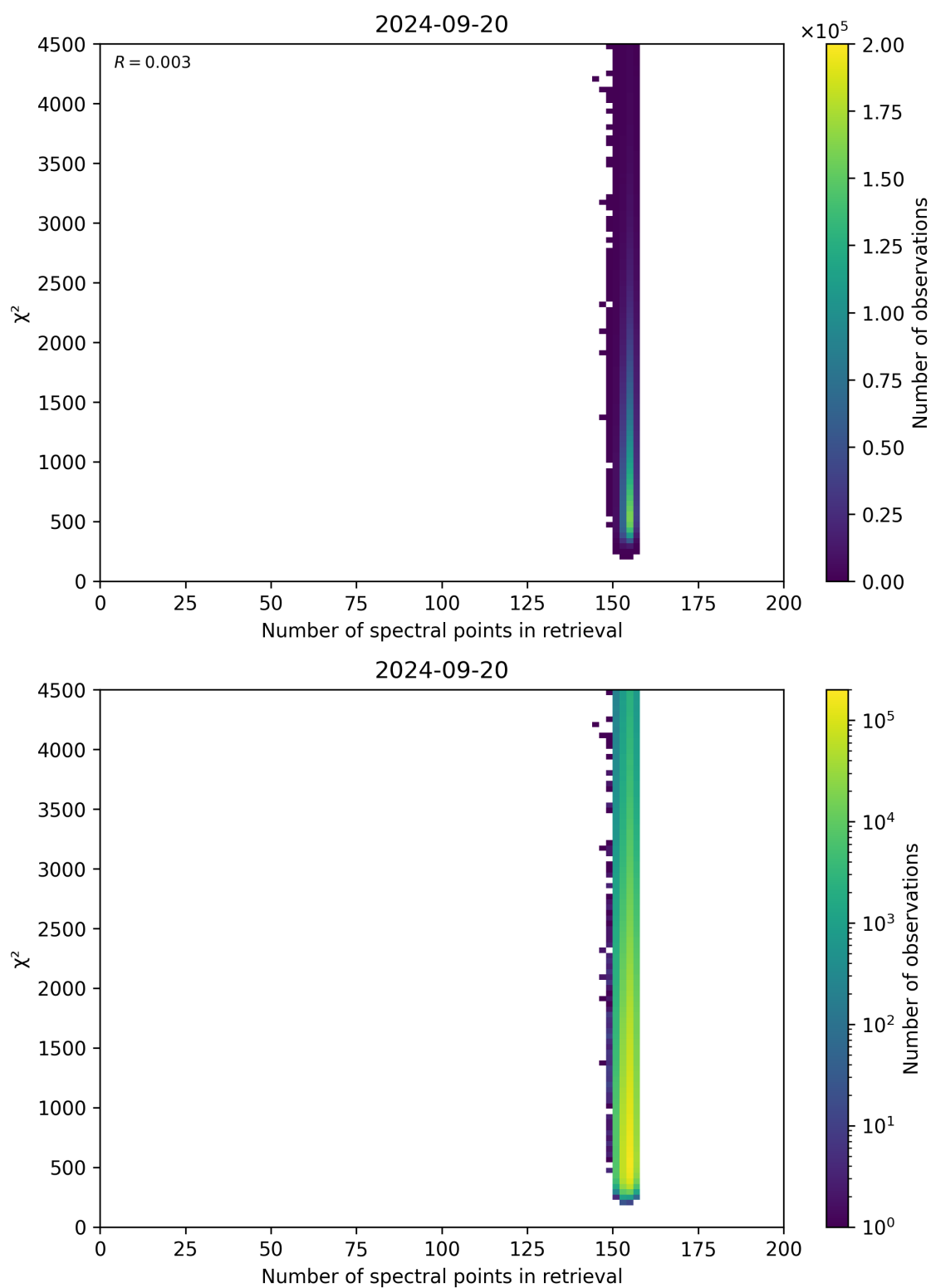
Figure 58: Scatter density plot of “Number of spectral points in retrieval” against “ \chi^2 ” for 2024-09-19 to 2024-09-21.
