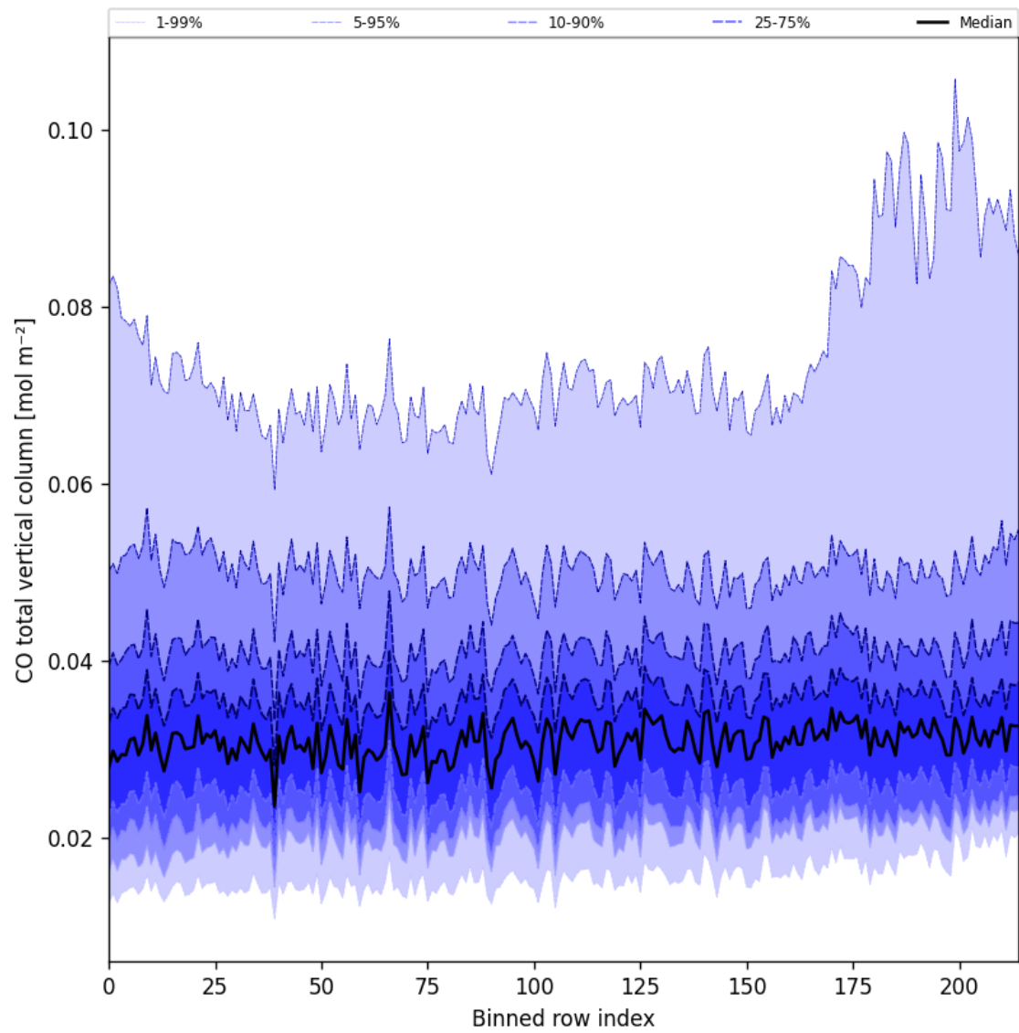
Figure 26: Along track statistics of “CO total vertical column” for 2024-09-19 to 2024-09-21
