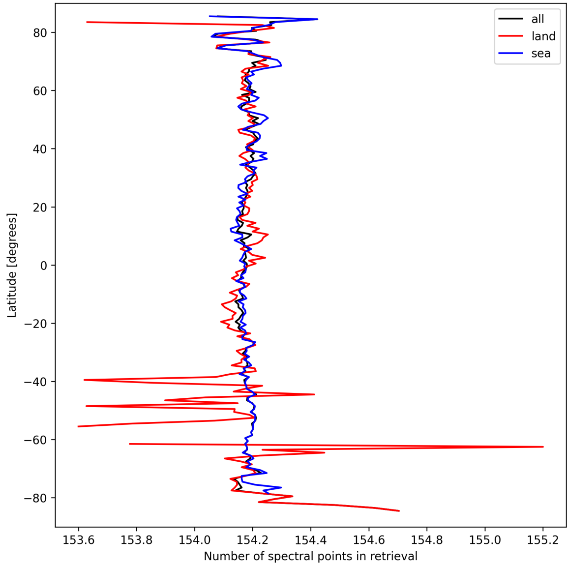
Figure 13: Zonal average of “Number of spectral points in retrieval” for 2024-09-19 to 2024-09-21.
