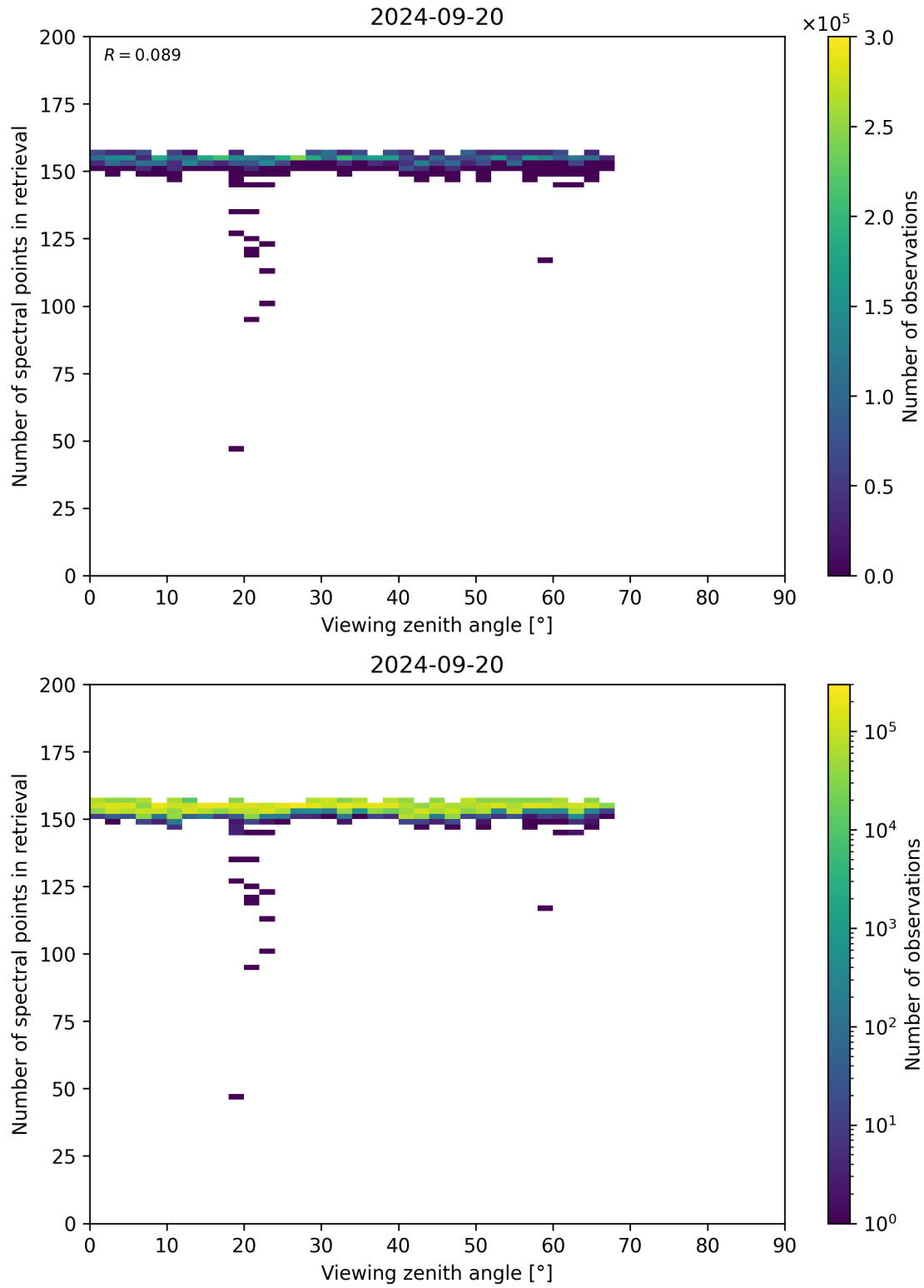
Figure 76: Scatter density plot of “Viewing zenith angle” against “Number of spectral points in retrieval” for 2024-09-19 to 2024-09-21.
