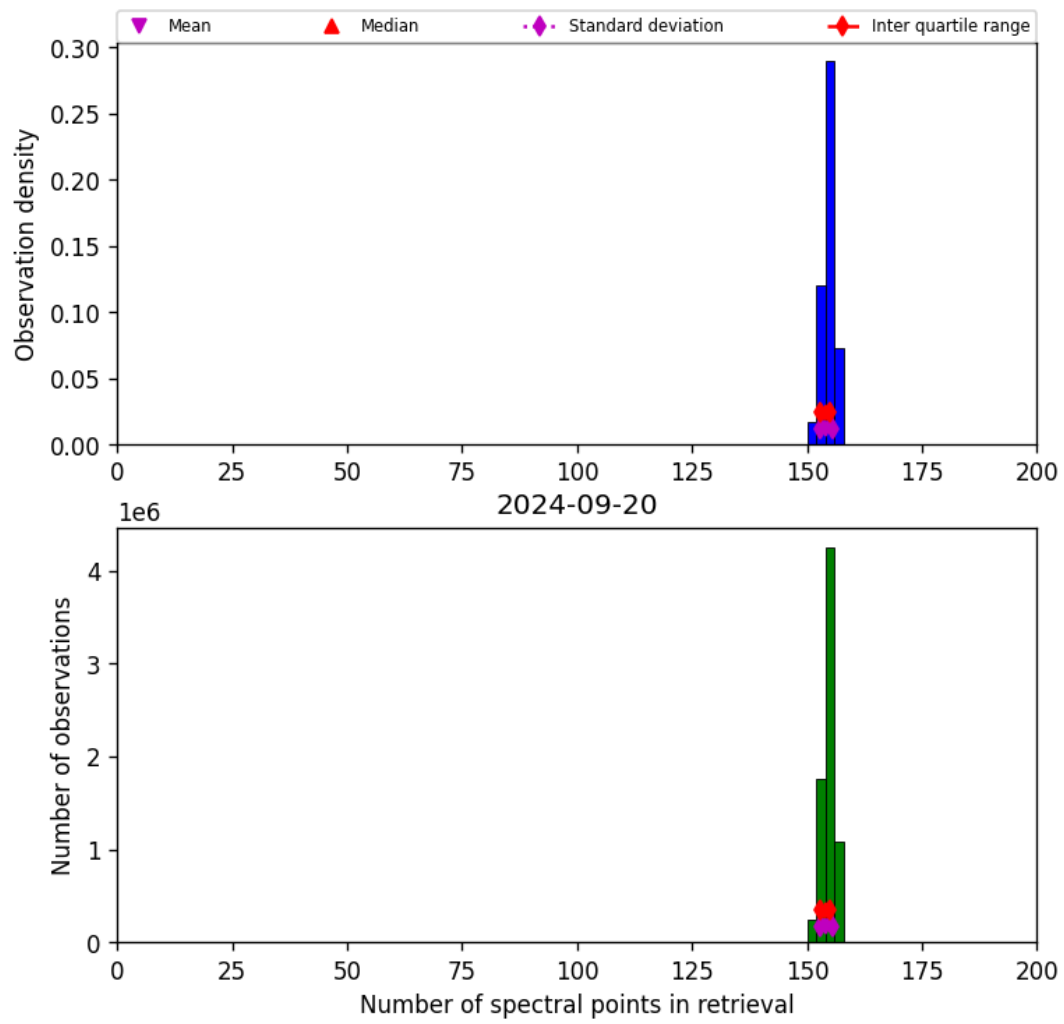
Figure 21: Histogram of “Number of spectral points in retrieval” for 2024-09-19 to 2024-09-21
