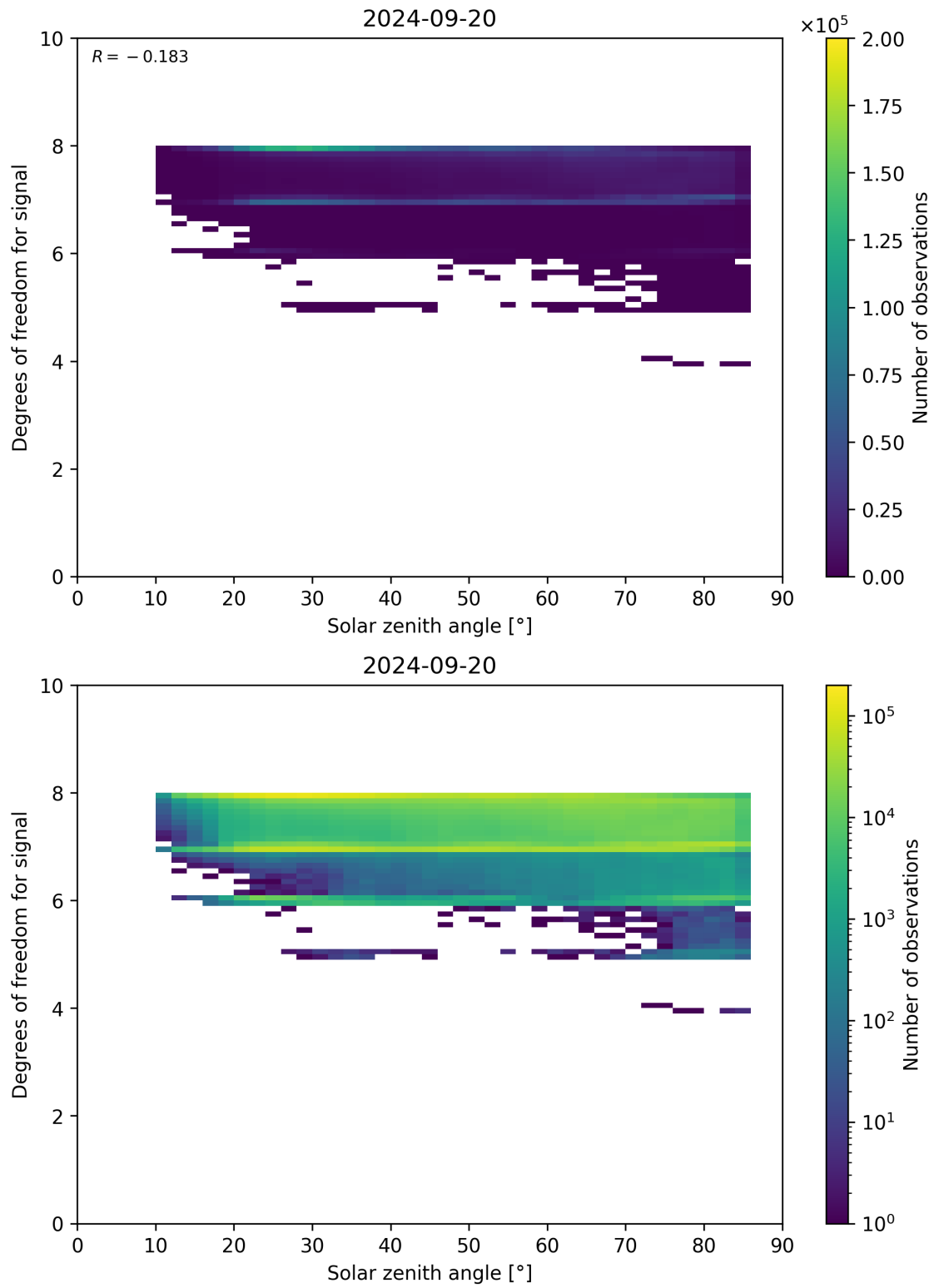
Figure 65: Scatter density plot of “Solar zenith angle” against “Degrees of freedom for signal” for 2024-09-19 to 2024-09-21.
