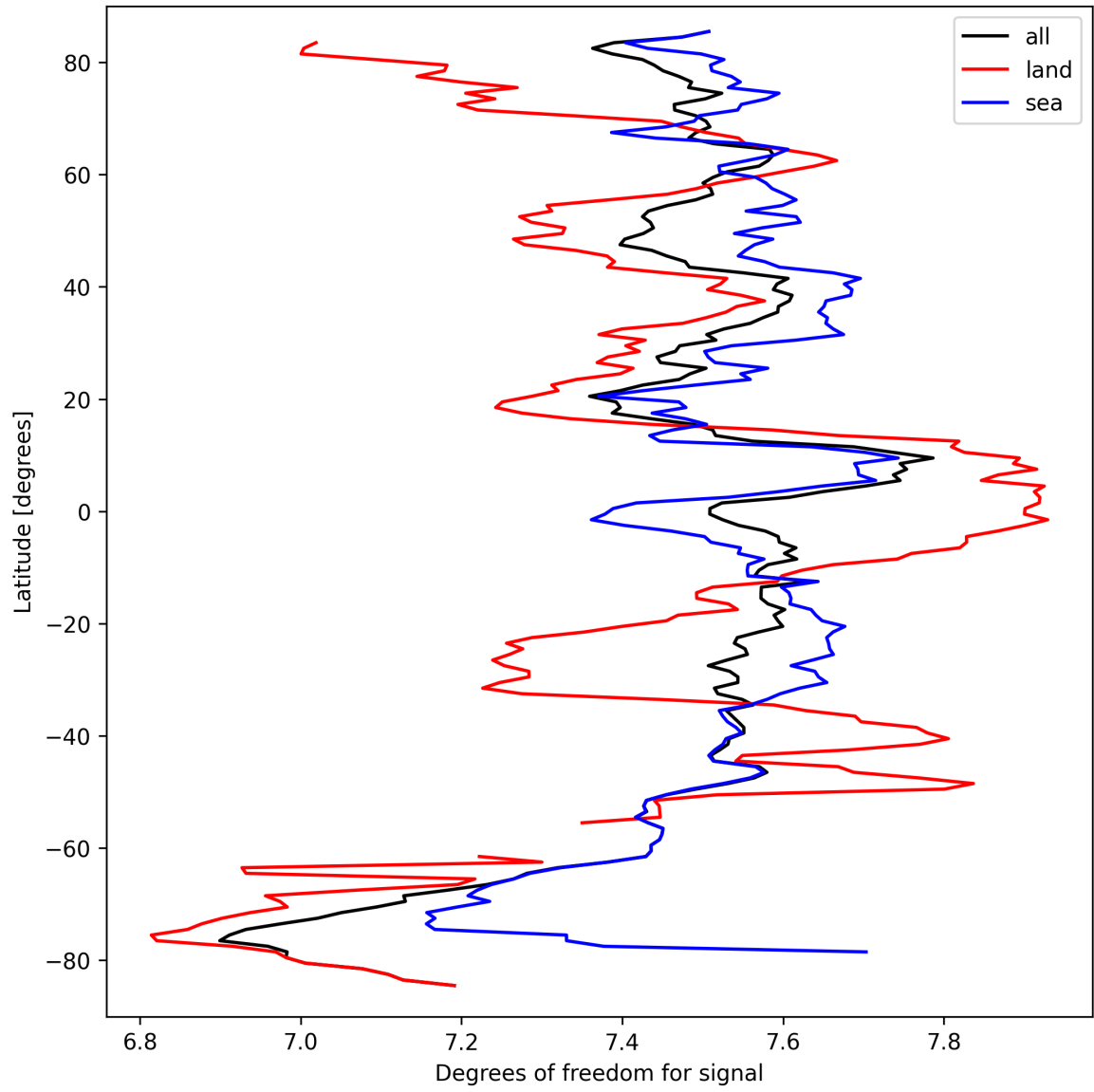
Figure 15: Zonal average of “Degrees of freedom for signal” for 2024-09-19 to 2024-09-21.
