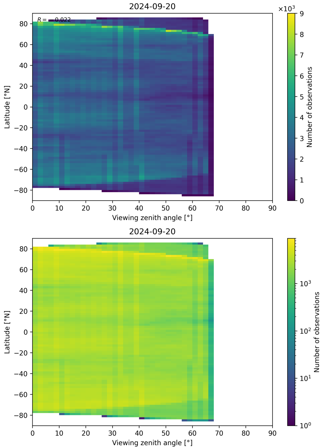
Figure 74: Scatter density plot of “Viewing zenith angle” against “Latitude” for 2024-09-19 to 2024-09-21.
