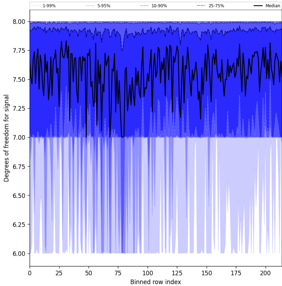
Figure 31: Along track statistics of “Degrees of freedom for signal” for 2024-09-19 to 2024-09-21
