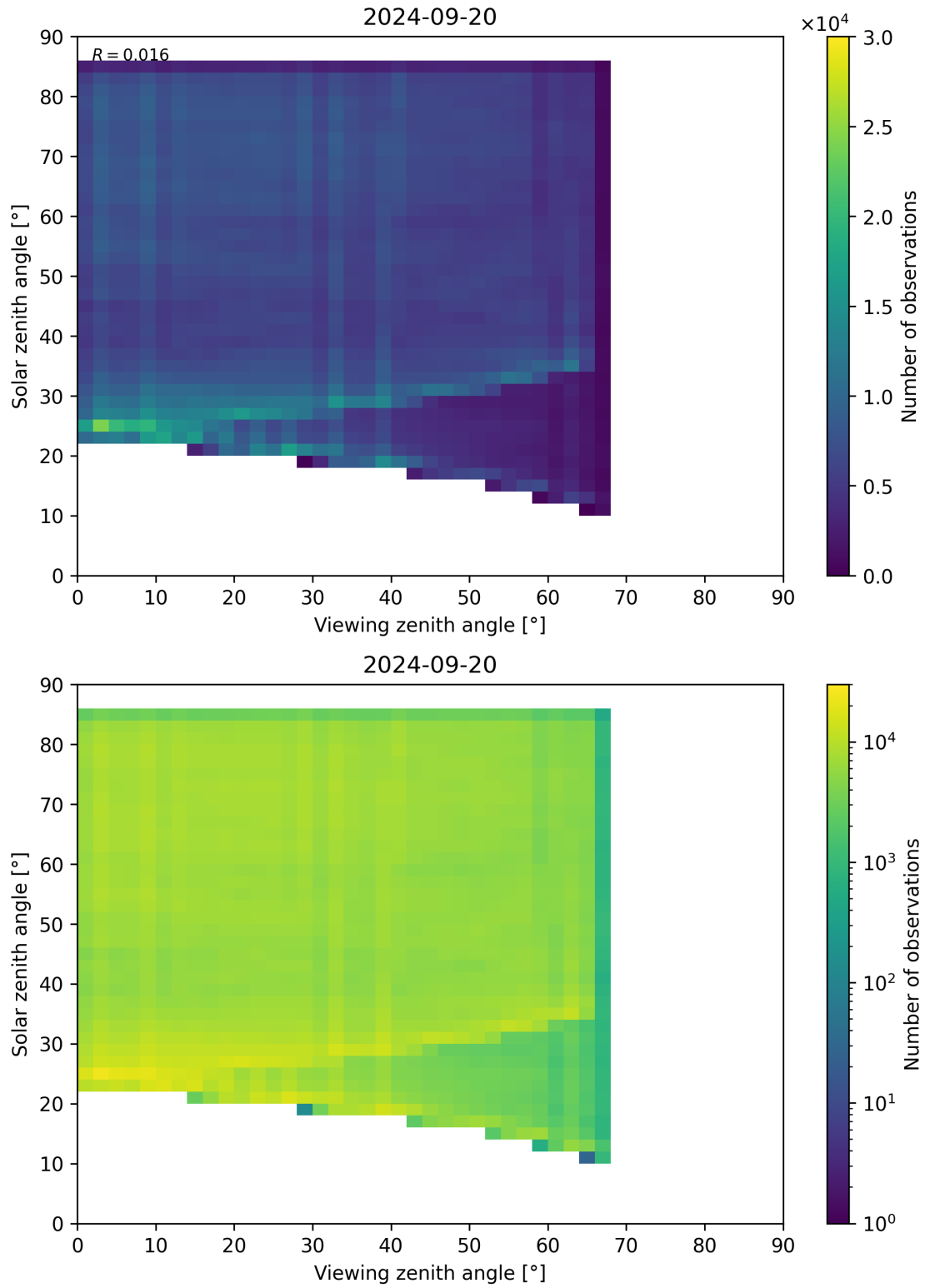
Figure 77: Scatter density plot of “Viewing zenith angle” against “Solar zenith angle” for 2024-09-19 to 2024-09-21.
