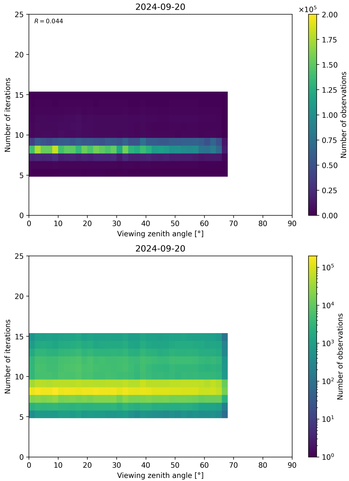
Figure 75: Scatter density plot of “Viewing zenith angle” against “Number of iterations” for 2024-09-19 to 2024-09-21.
