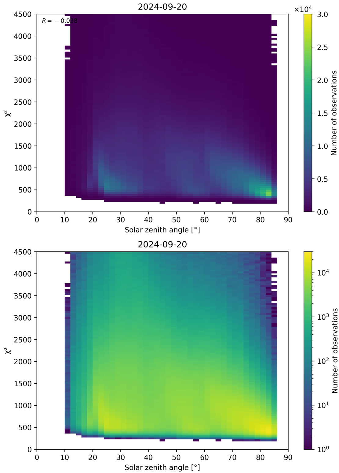
Figure 64: Scatter density plot of “Solar zenith angle” against “ \chi^2 ” for 2024-09-19 to 2024-09-21.
