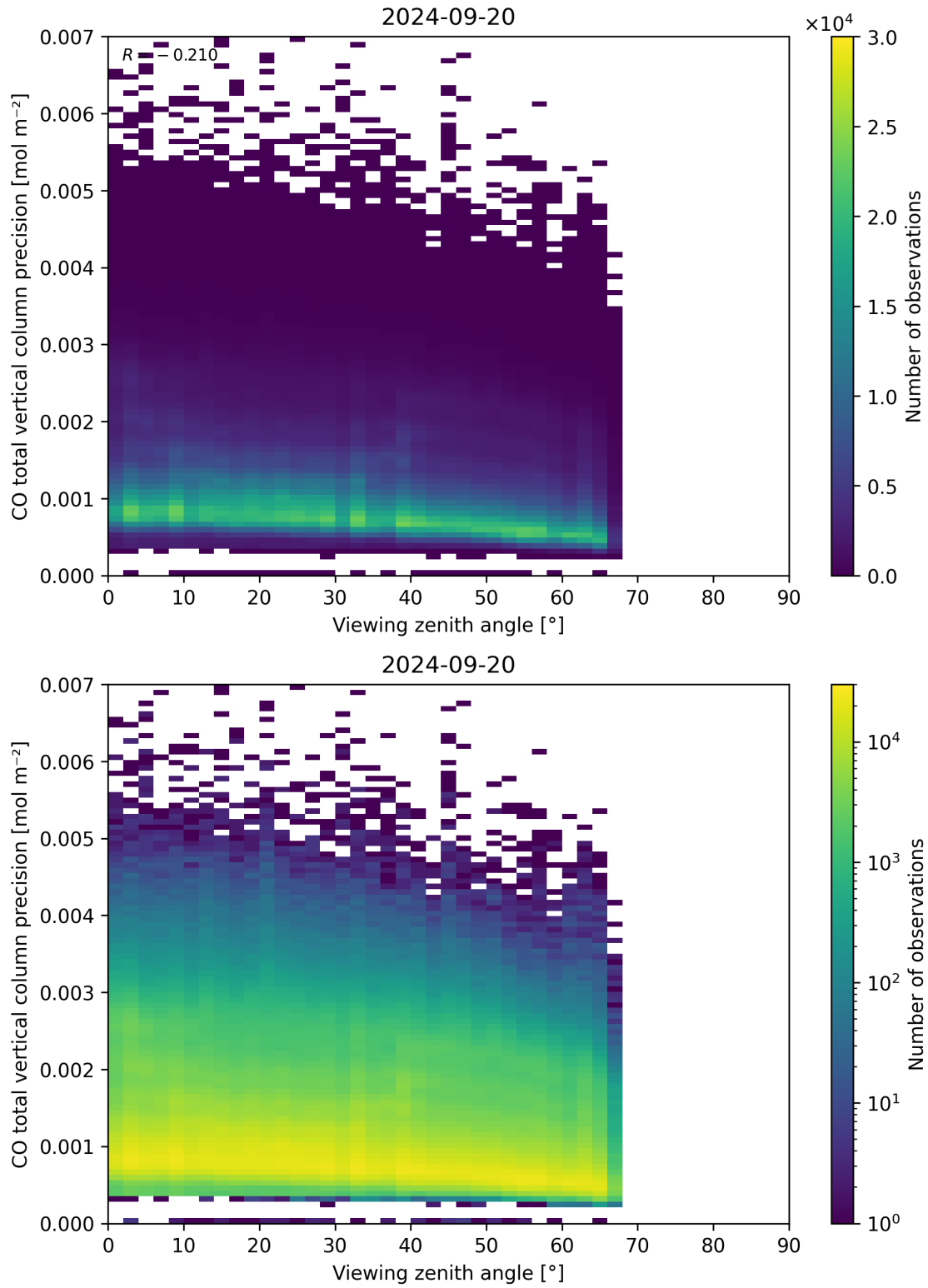
Figure 71: Scatter density plot of “Viewing zenith angle” against “CO total vertical column precision” for 2024-09-19 to 2024-09-21.
