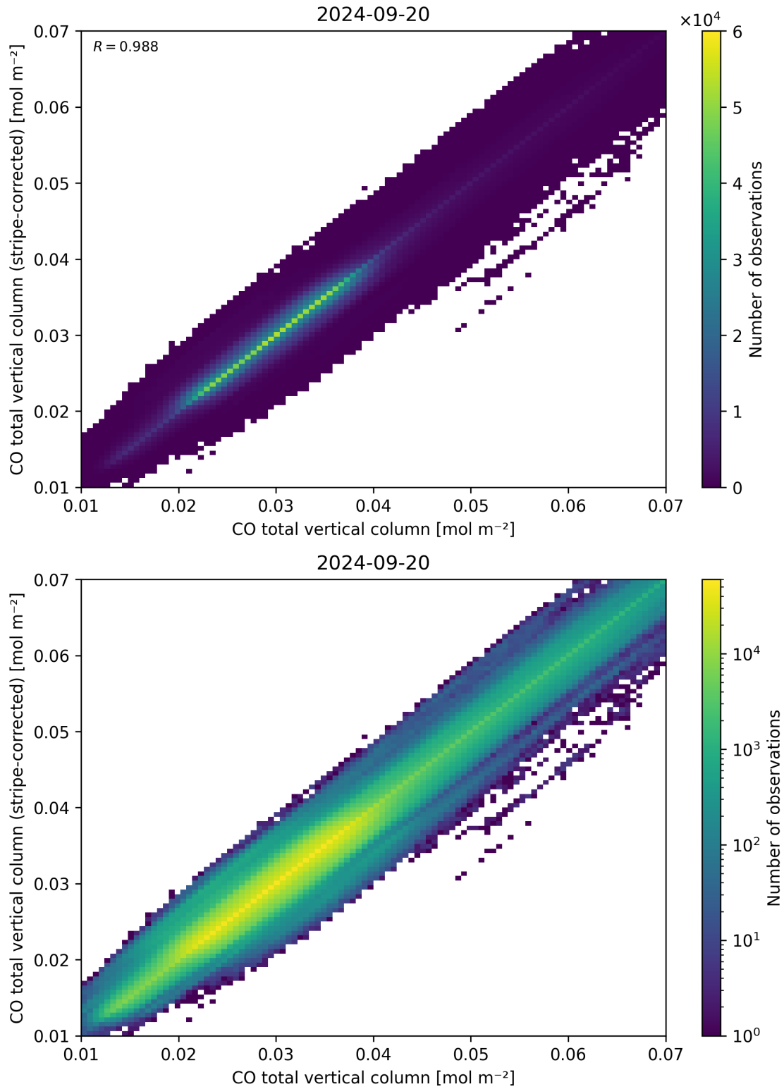
Figure 33: Scatter density plot of “CO total vertical column” against “CO total vertical column (stripe-corrected)” for 2024-09-19 to 2024-09-21.
