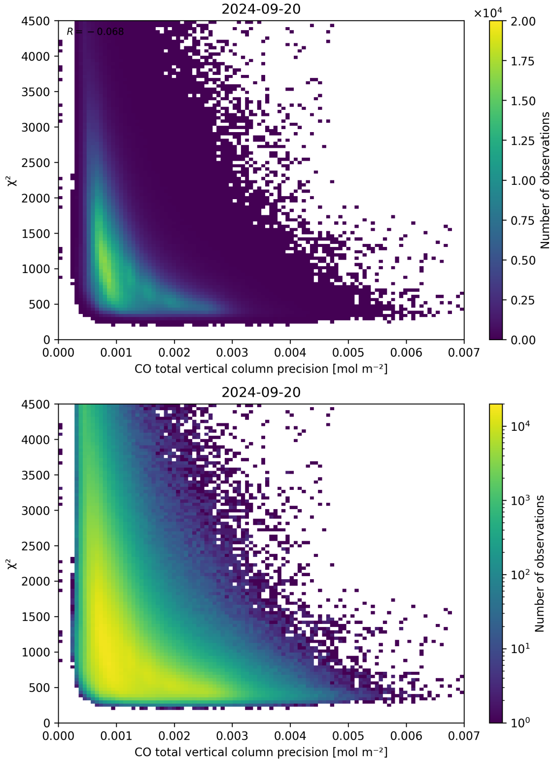
Figure 44: Scatter density plot of “CO total vertical column precision” against “ \chi^2 ” for 2024-09-19 to 2024-09-21.
