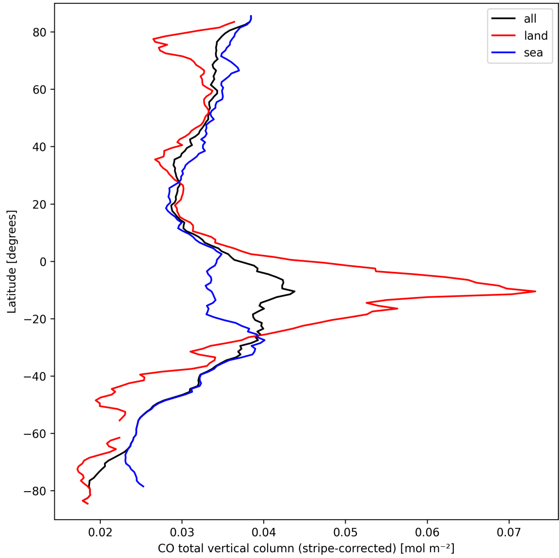
Figure 11: Zonal average of “CO total vertical column (stripe-corrected)” for 2024-09-19 to 2024-09-21.
