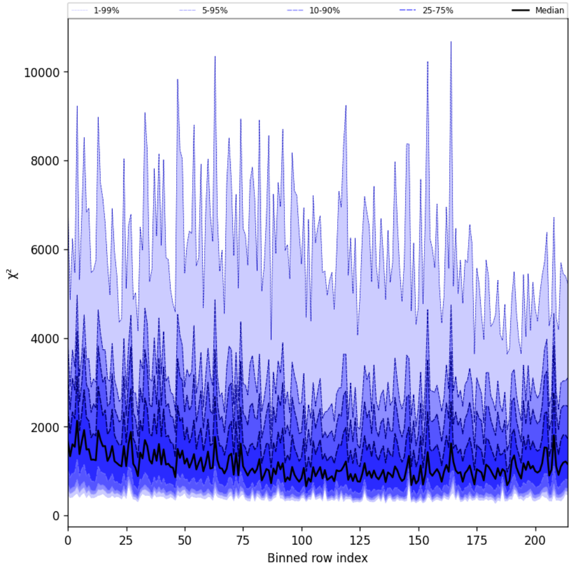
Figure 30: Along track statistics of “ \chi^2 ” for 2024-09-19 to 2024-09-21
