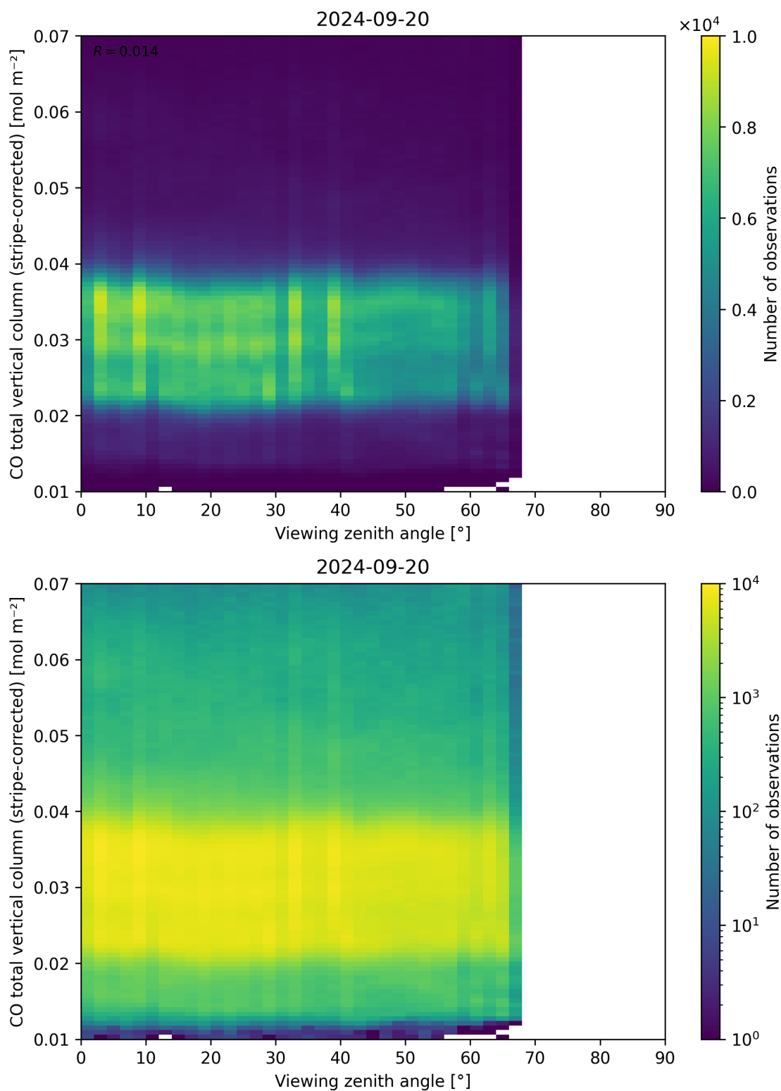
Figure 70: Scatter density plot of “Viewing zenith angle” against “CO total vertical column (stripe-corrected)” for 2024-09-19 to 2024-09-21.
