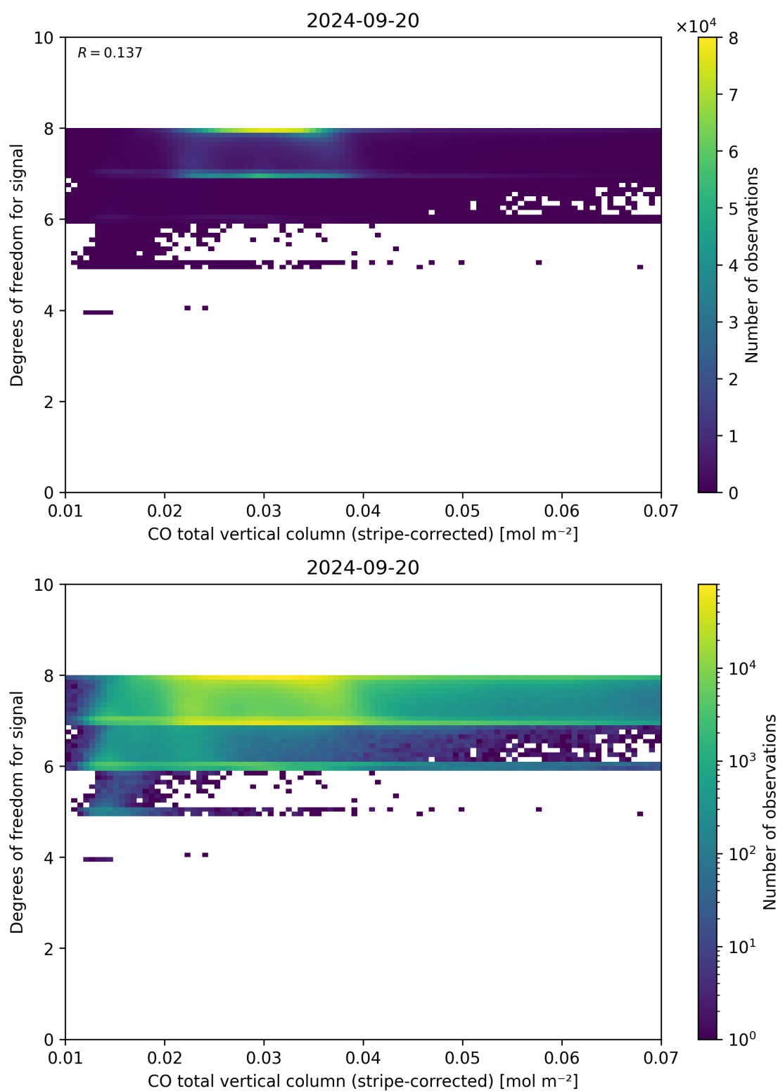
Figure 38: Scatter density plot of “CO total vertical column (stripe-corrected)” against “Degrees of freedom for signal” for 2024-09-19 to 2024-09-21.
