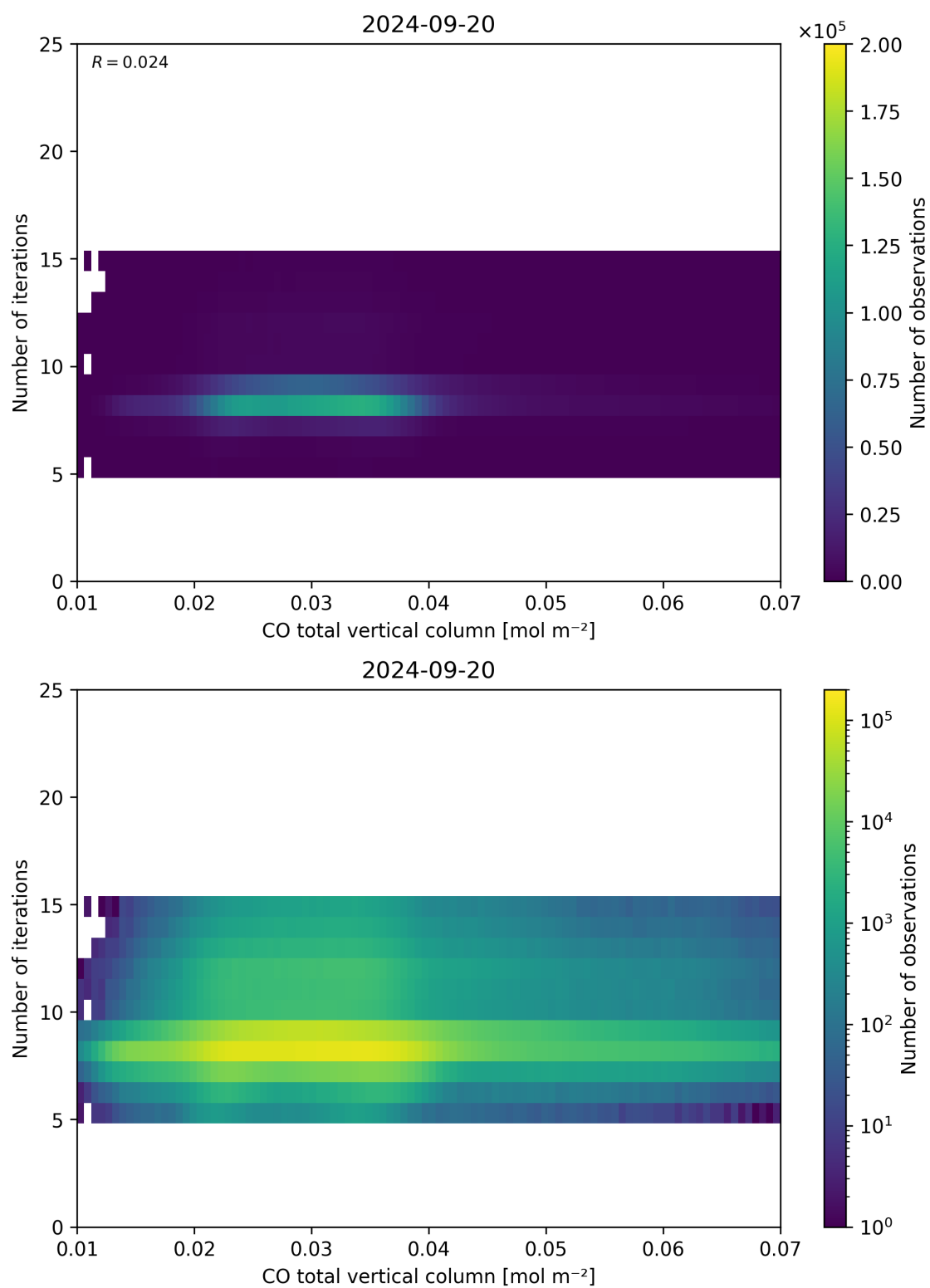
Figure 42: Scatter density plot of “CO total vertical column” against “Number of iterations” for 2024-09-19 to 2024-09-21.
