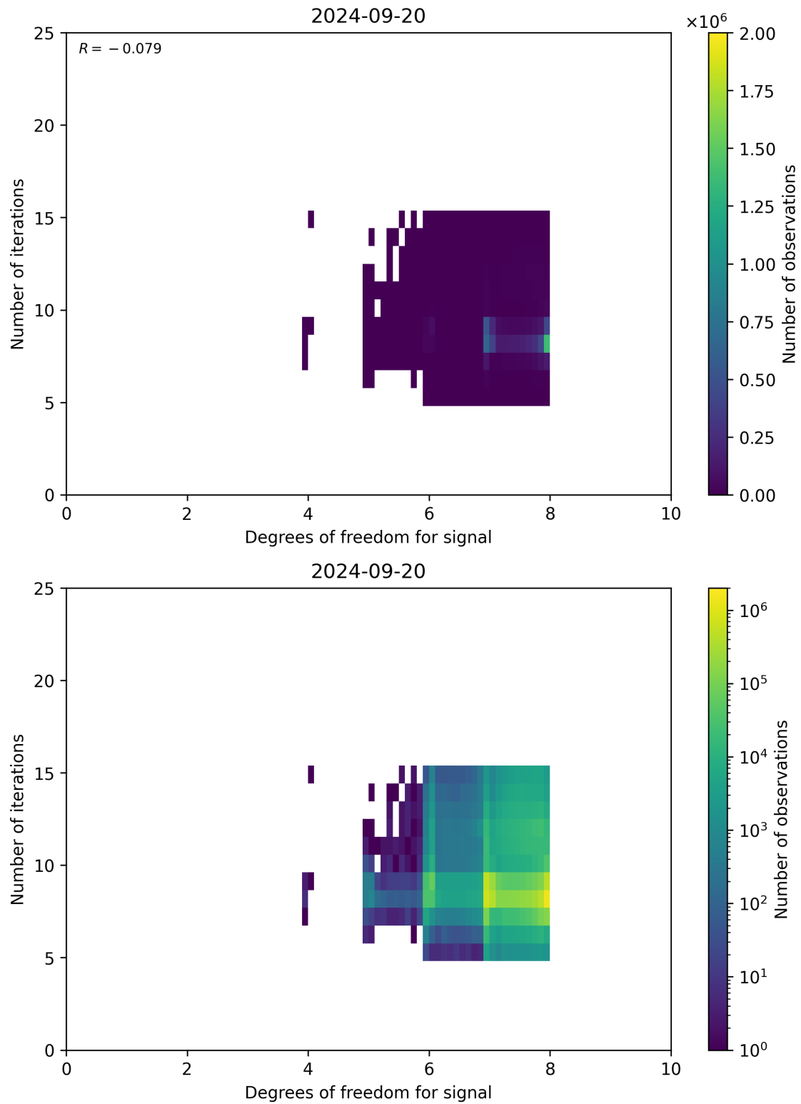
Figure 50: Scatter density plot of “Degrees of freedom for signal” against “Number of iterations” for 2024-09-19 to 2024-09-21.
