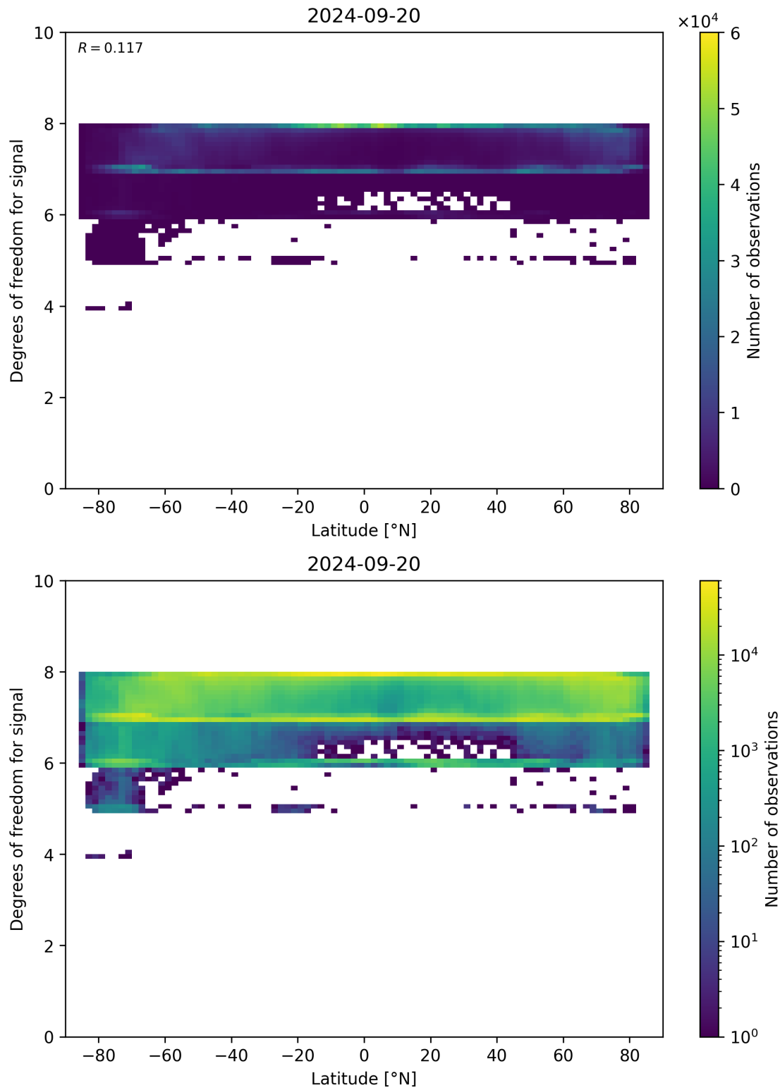
Figure 55: Scatter density plot of “Latitude” against “Degrees of freedom for signal” for 2024-09-19 to 2024-09-21.
