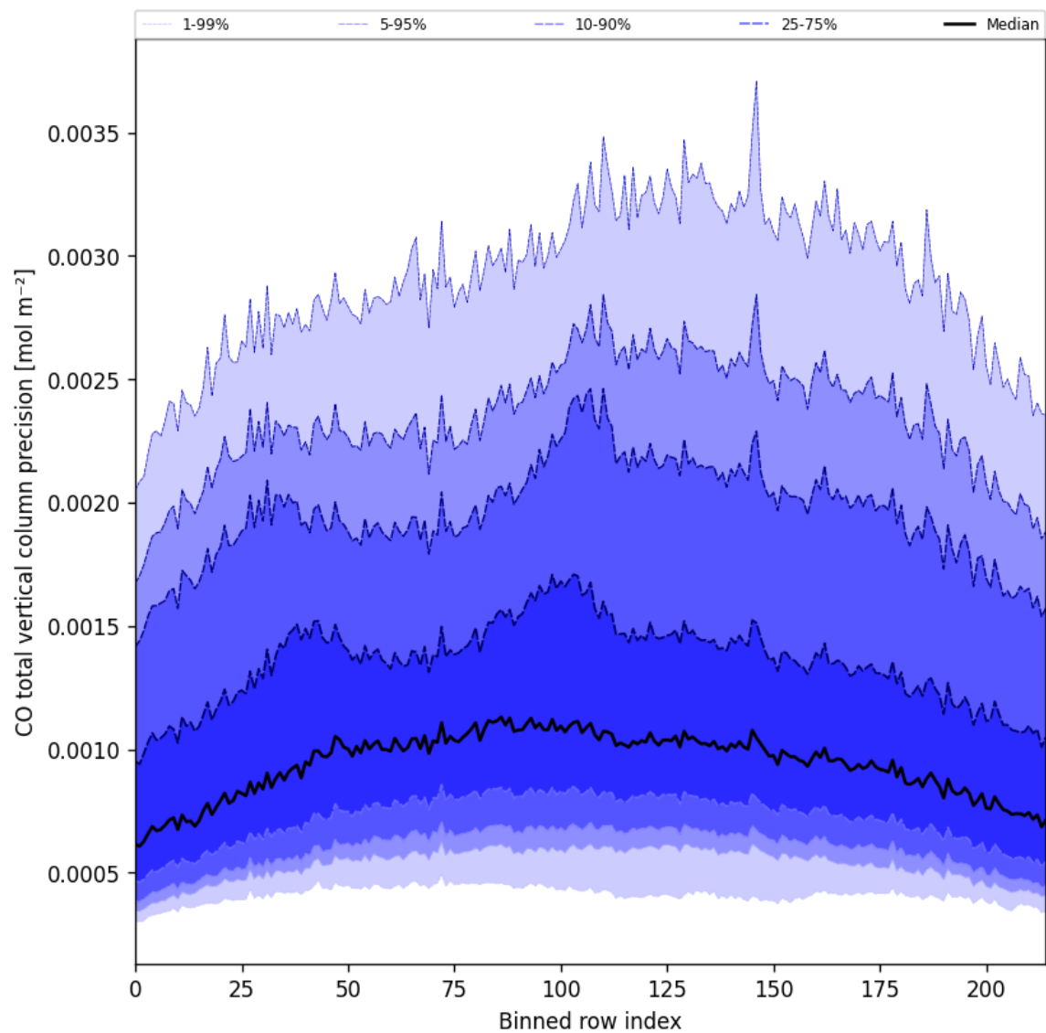
Figure 28: Along track statistics of “CO total vertical column precision” for 2024-09-19 to 2024-09-21
