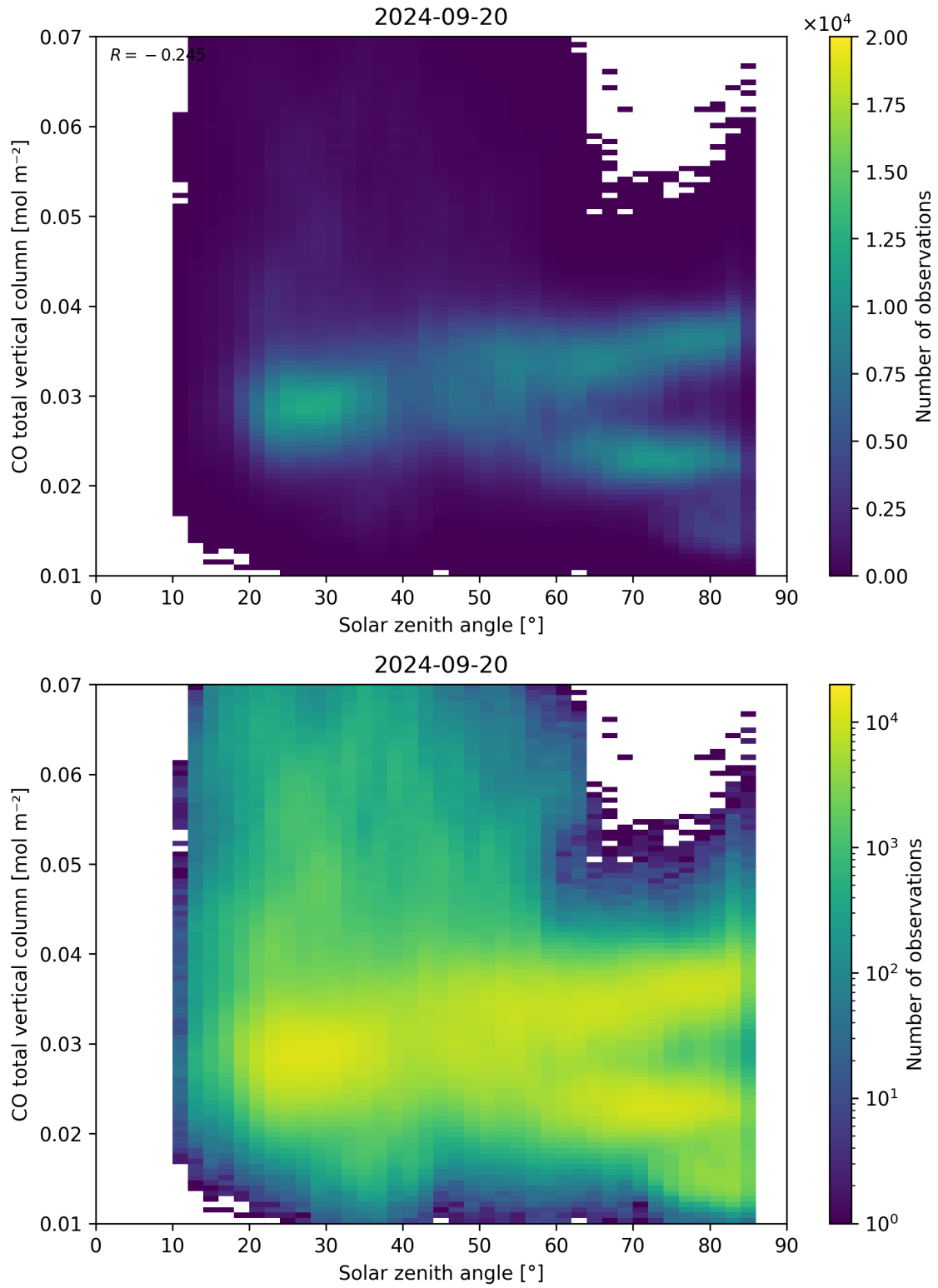
Figure 61: Scatter density plot of “Solar zenith angle” against “CO total vertical column” for 2024-09-19 to 2024-09-21.
