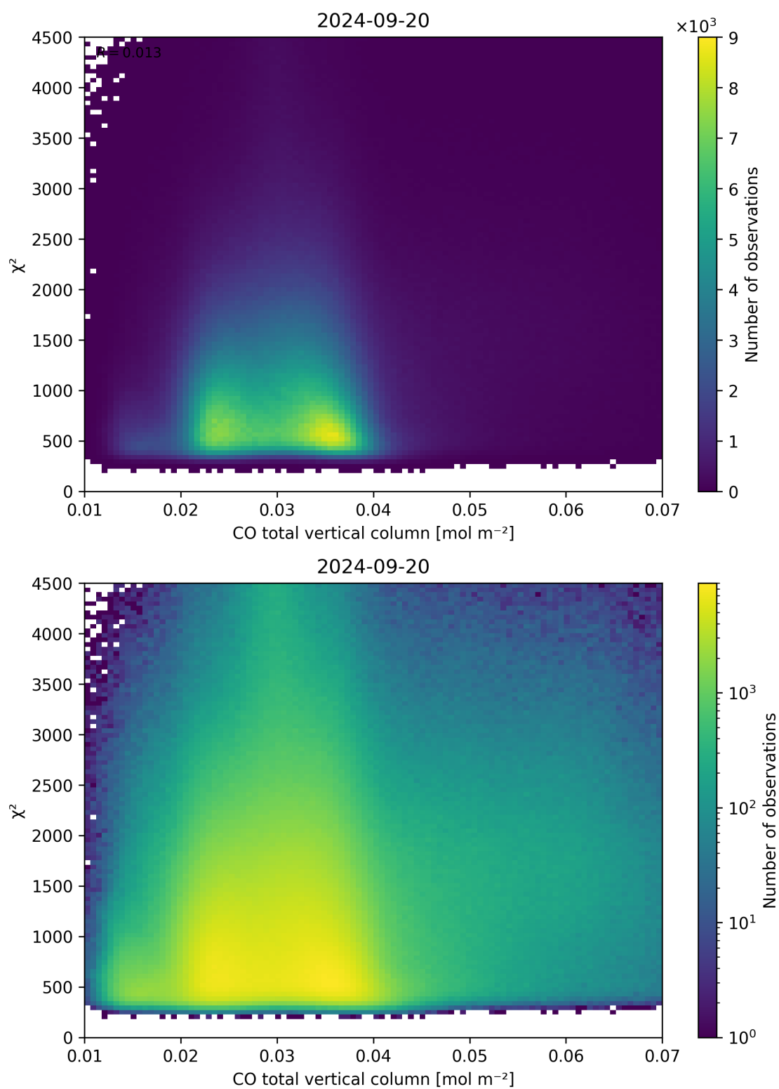
Figure 35: Scatter density plot of “CO total vertical column” against “ \chi^2 ” for 2024-09-19 to 2024-09-21.
