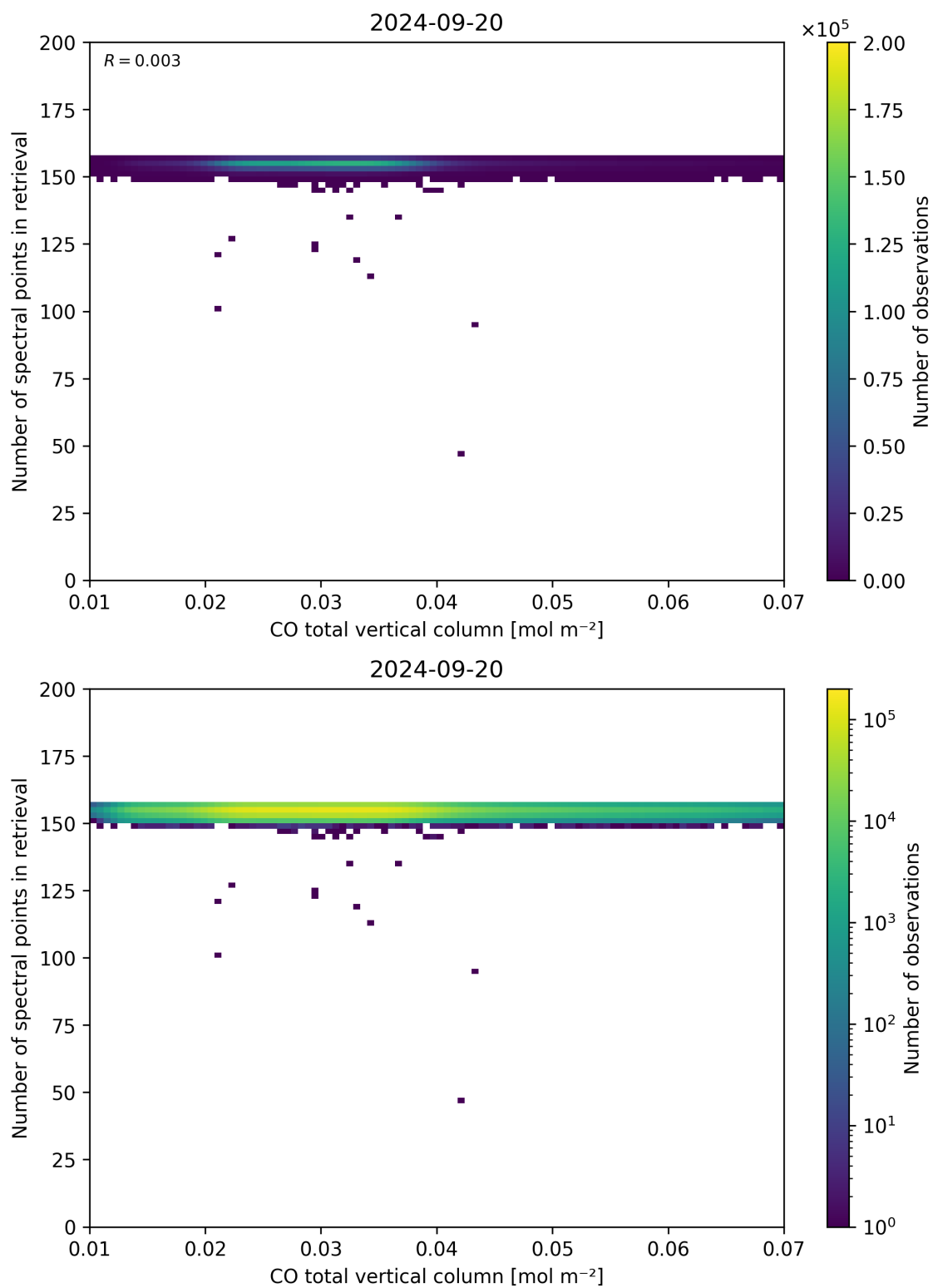
Figure 43: Scatter density plot of “CO total vertical column” against “Number of spectral points in retrieval” for 2024-09-19 to 2024-09-21.
