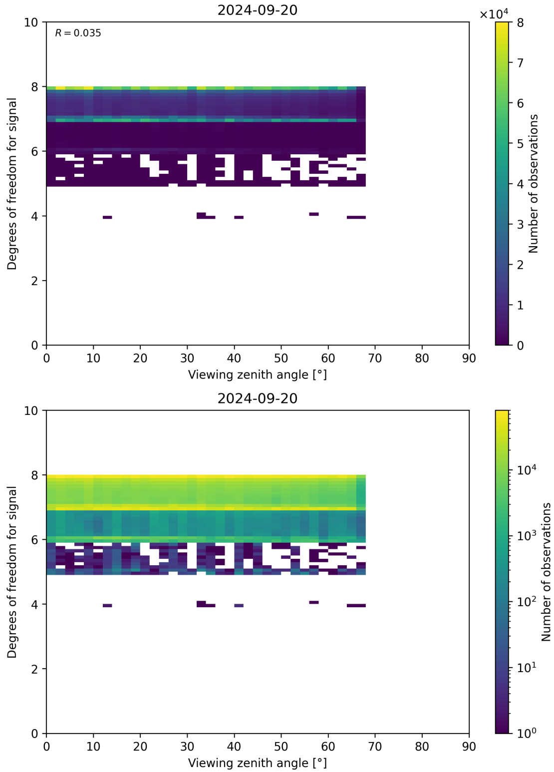
Figure 73: Scatter density plot of “Viewing zenith angle” against “Degrees of freedom for signal” for 2024-09-19 to 2024-09-21.
