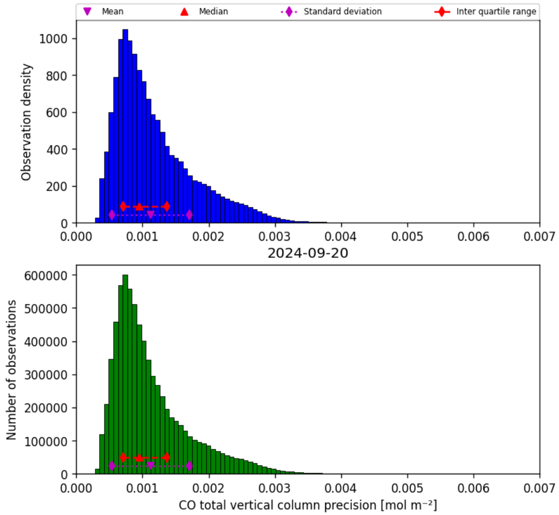
Figure 20: Histogram of “CO total vertical column precision” for 2024-09-19 to 2024-09-21
