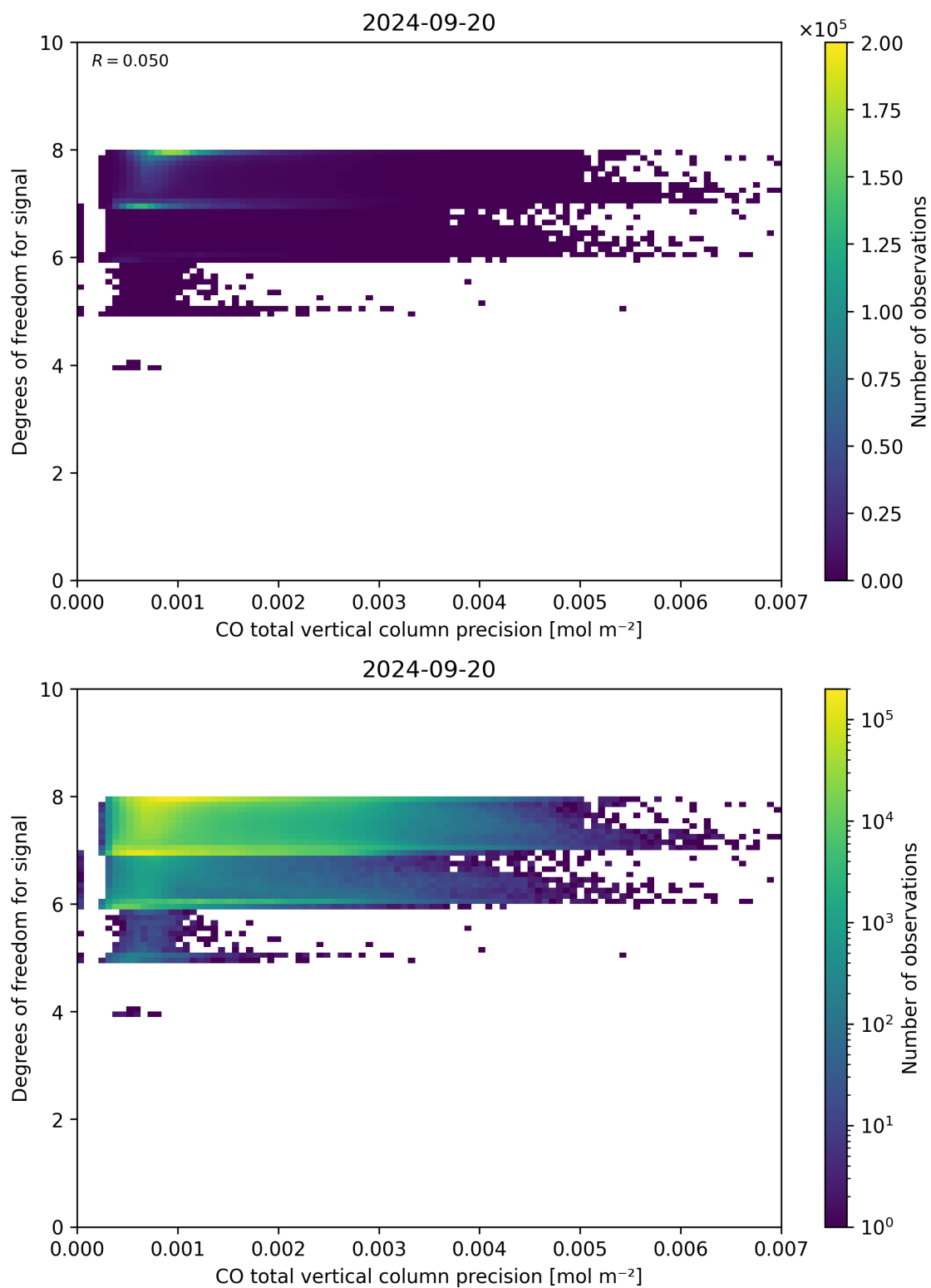
Figure 45: Scatter density plot of “CO total vertical column precision” against “Degrees of freedom for signal” for 2024-09-19 to 2024-09-21.
