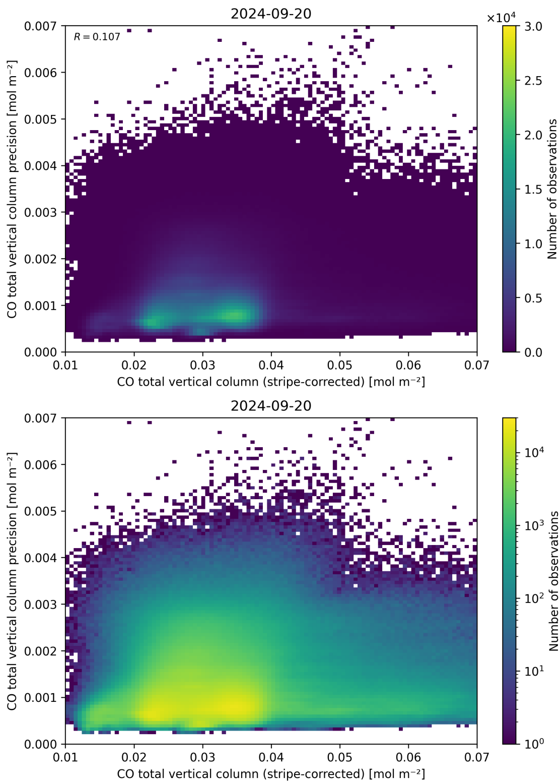
Figure 36: Scatter density plot of “CO total vertical column (stripe-corrected)” against “CO total vertical column precision” for 2024-09-19 to 2024-09-21.
