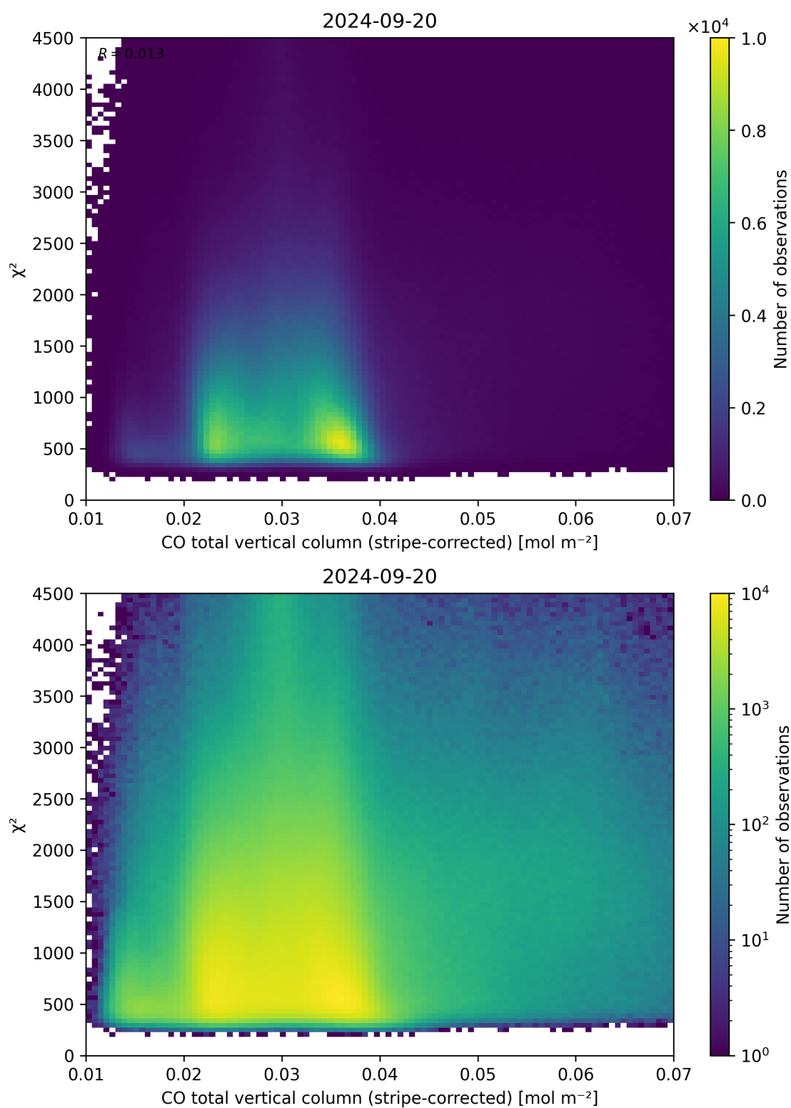
Figure 37: Scatter density plot of “CO total vertical column (stripe-corrected)” against “ \chi^2 ” for 2024-09-19 to 2024-09-21.
