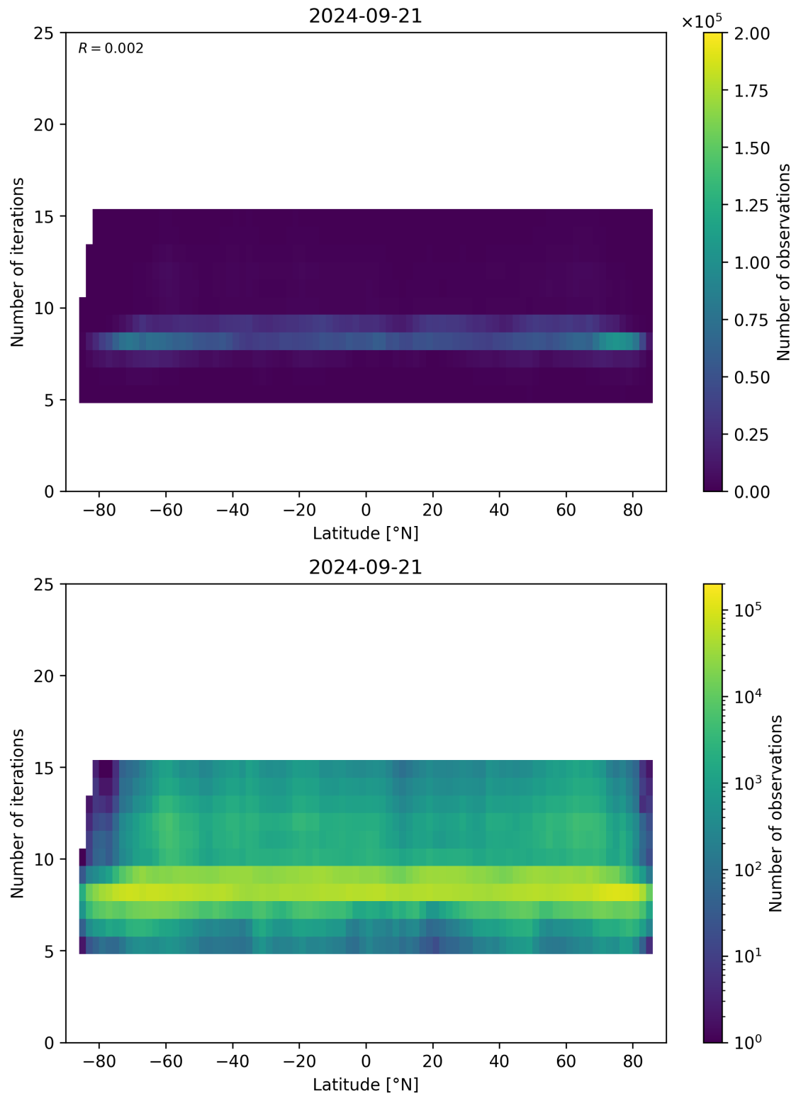
Figure 56: Scatter density plot of “Latitude” against “Number of iterations” for 2024-09-20 to 2024-09-22.
