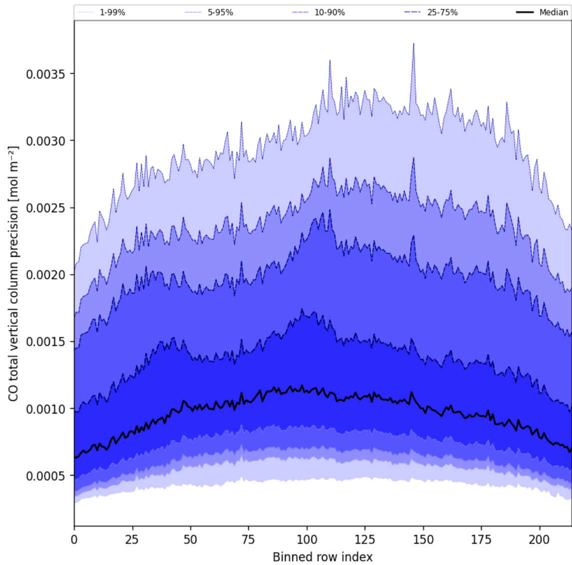
Figure 28: Along track statistics of “CO total vertical column precision” for 2024-09-20 to 2024-09-22
