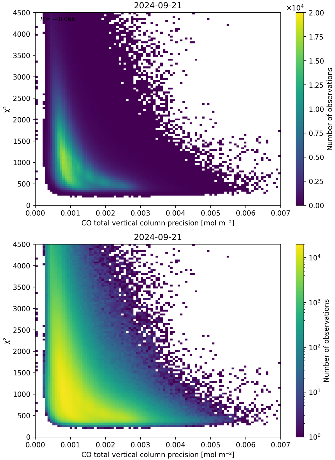
Figure 44: Scatter density plot of “CO total vertical column precision” against “ \chi^2 ” for 2024-09-20 to 2024-09-22.
