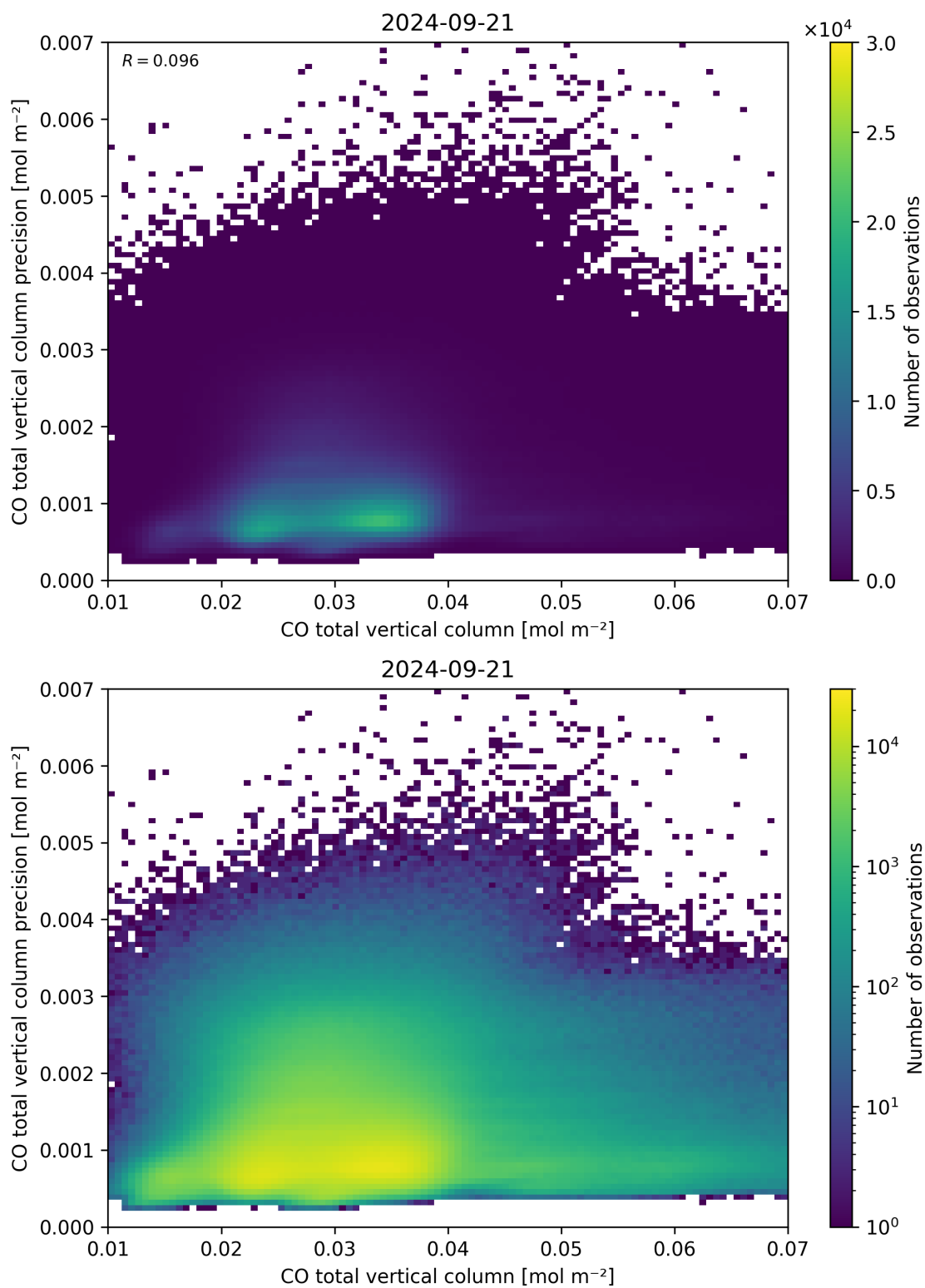
Figure 34: Scatter density plot of “CO total vertical column” against “CO total vertical column precision” for 2024-09-20 to 2024-09-22.
