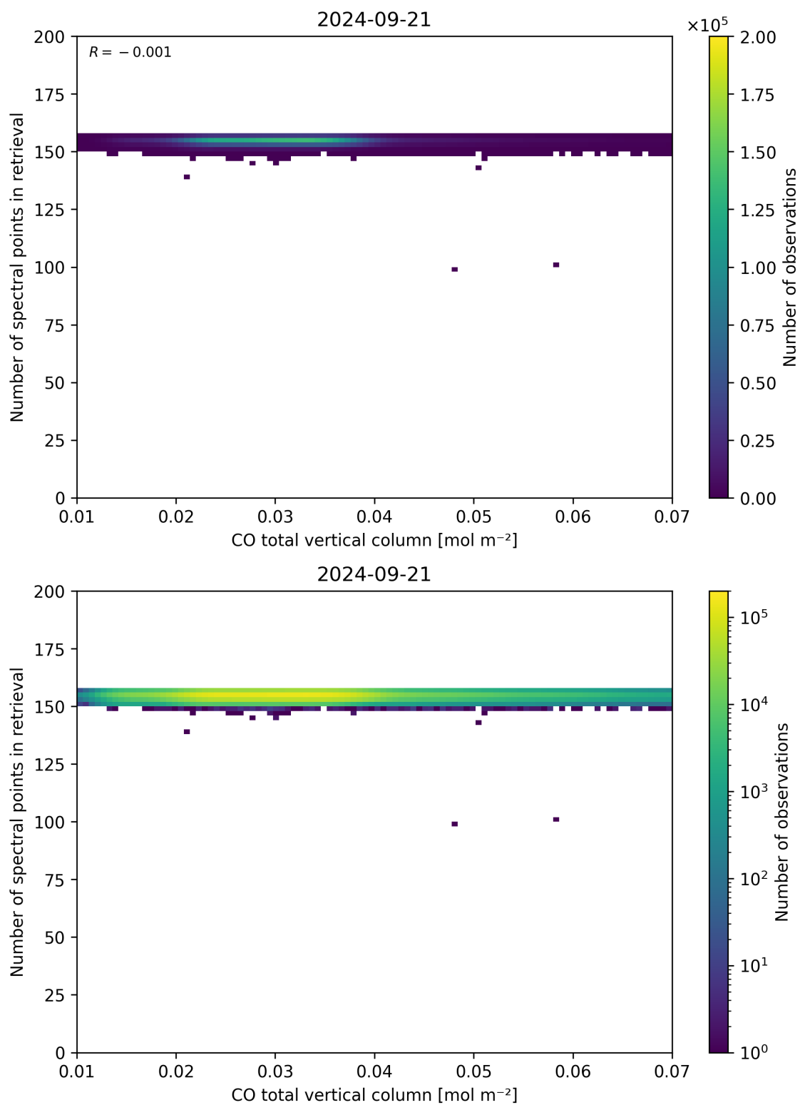
Figure 43: Scatter density plot of “CO total vertical column” against “Number of spectral points in retrieval” for 2024-09-20 to 2024-09-22.
