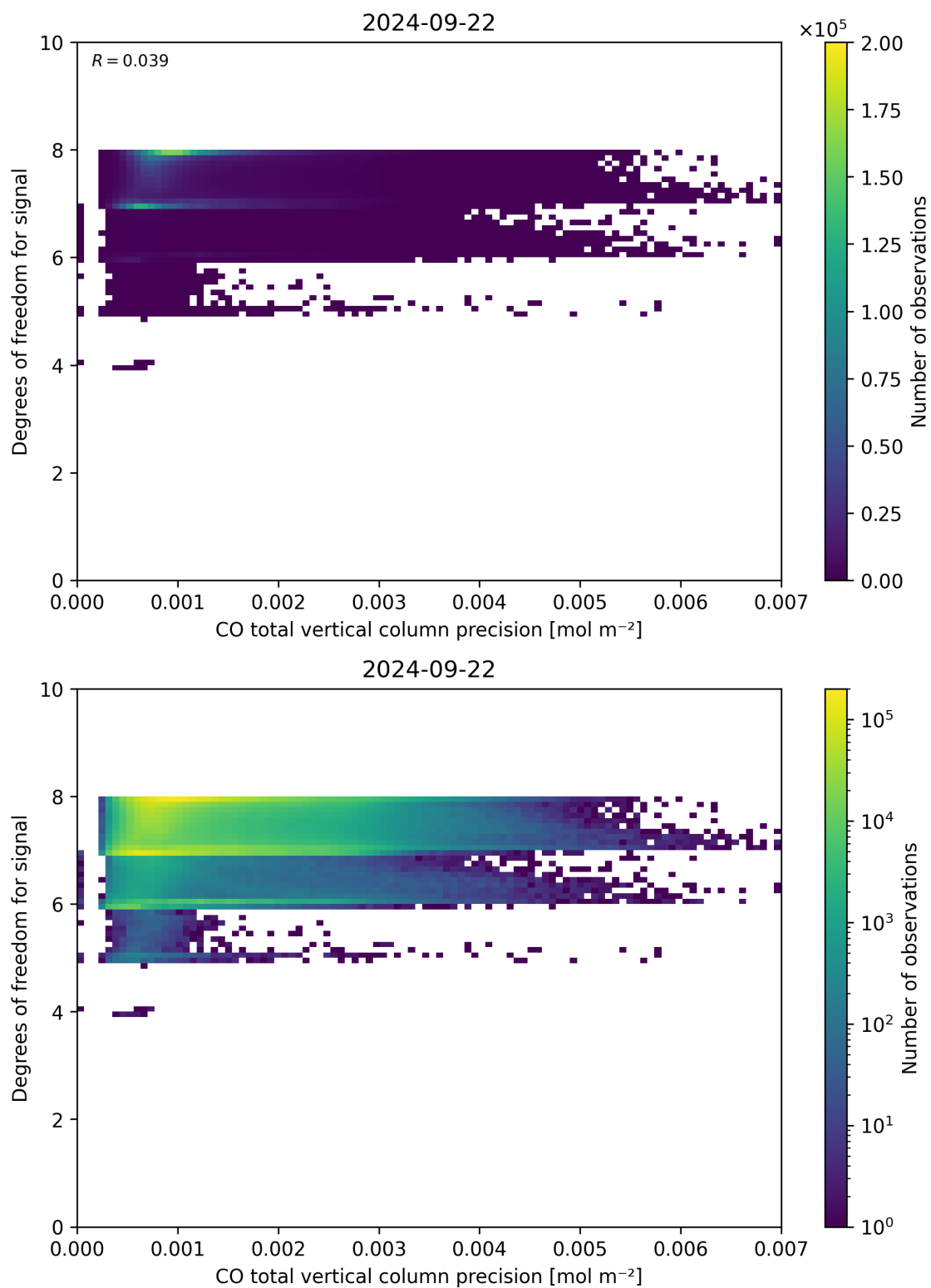
Figure 45: Scatter density plot of “CO total vertical column precision” against “Degrees of freedom for signal” for 2024-09-22 to 2024-09-23.
