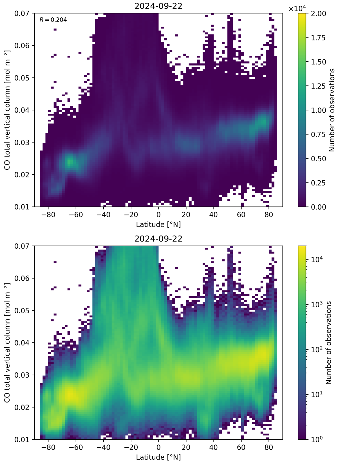
Figure 51: Scatter density plot of “Latitude” against “CO total vertical column” for 2024-09-22 to 2024-09-23.
