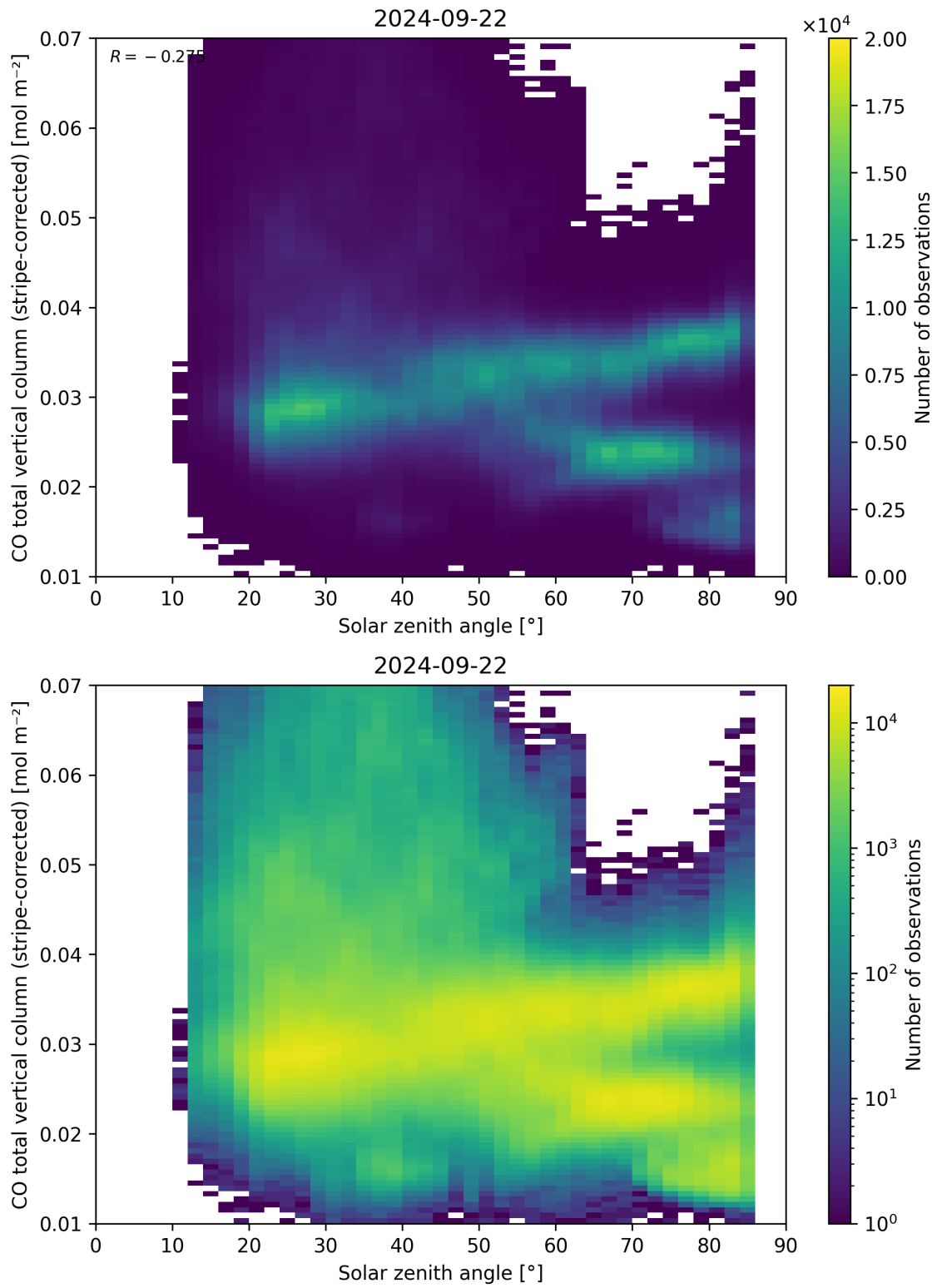
Figure 62: Scatter density plot of “Solar zenith angle” against “CO total vertical column (stripe-corrected)” for 2024-09-22 to 2024-09-23.
