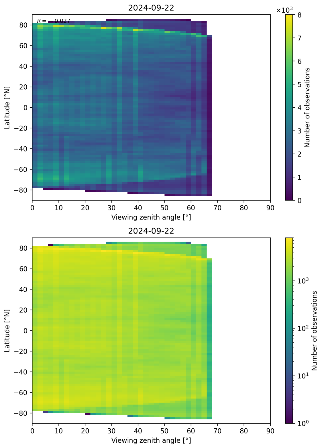
Figure 74: Scatter density plot of “Viewing zenith angle” against “Latitude” for 2024-09-22 to 2024-09-23.
