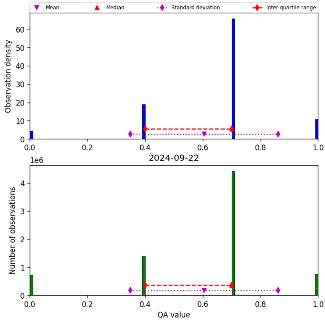
Figure 17: Histogram of “QA value” for 2024-09-22 to 2024-09-23
