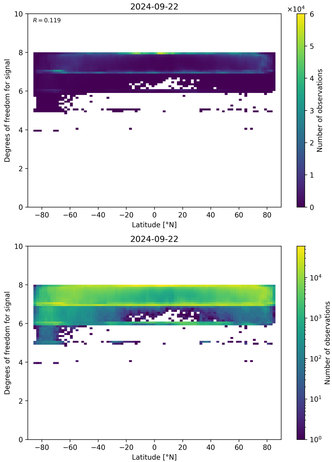
Figure 55: Scatter density plot of “Latitude” against “Degrees of freedom for signal” for 2024-09-22 to 2024-09-23.
