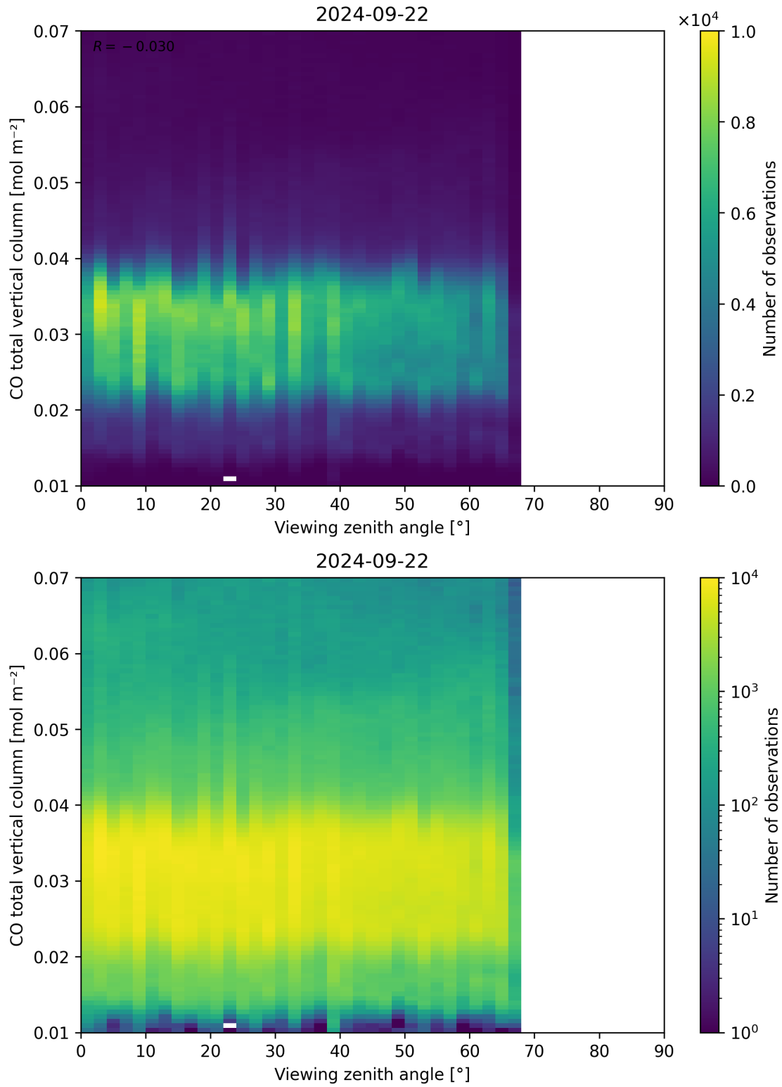
Figure 69: Scatter density plot of “Viewing zenith angle” against “CO total vertical column” for 2024-09-22 to 2024-09-23.
