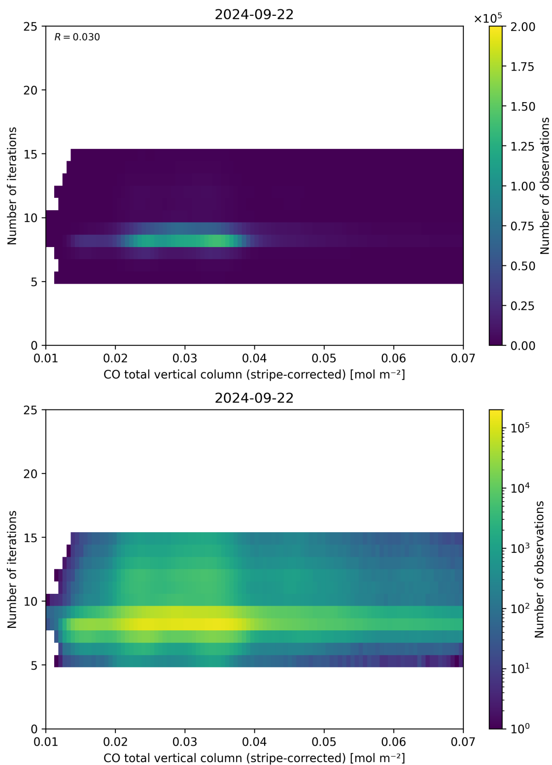
Figure 39: Scatter density plot of “CO total vertical column (stripe-corrected)” against “Number of iterations” for 2024-09-22 to 2024-09-23.
