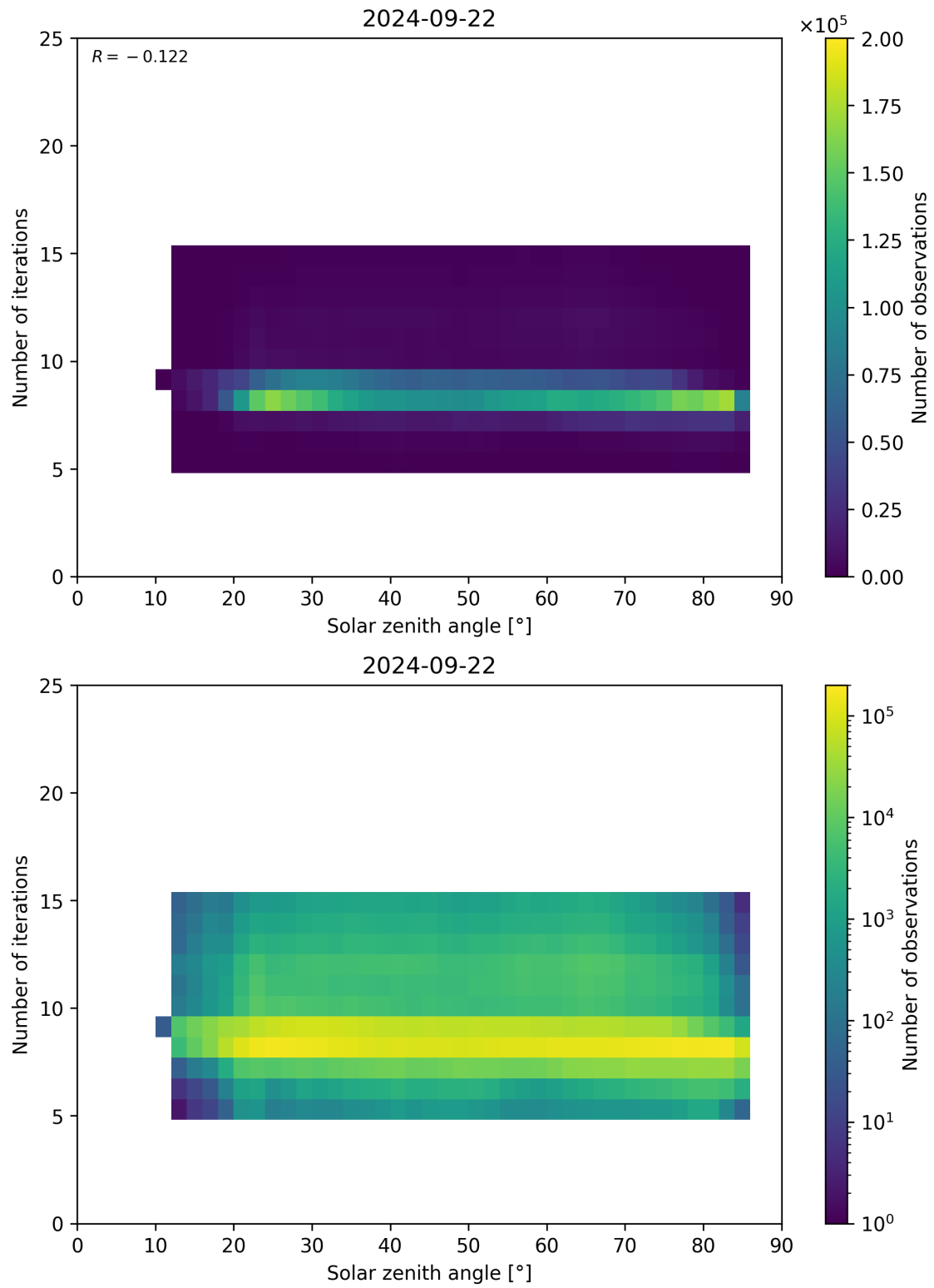
Figure 67: Scatter density plot of “Solar zenith angle” against “Number of iterations” for 2024-09-22 to 2024-09-23.
