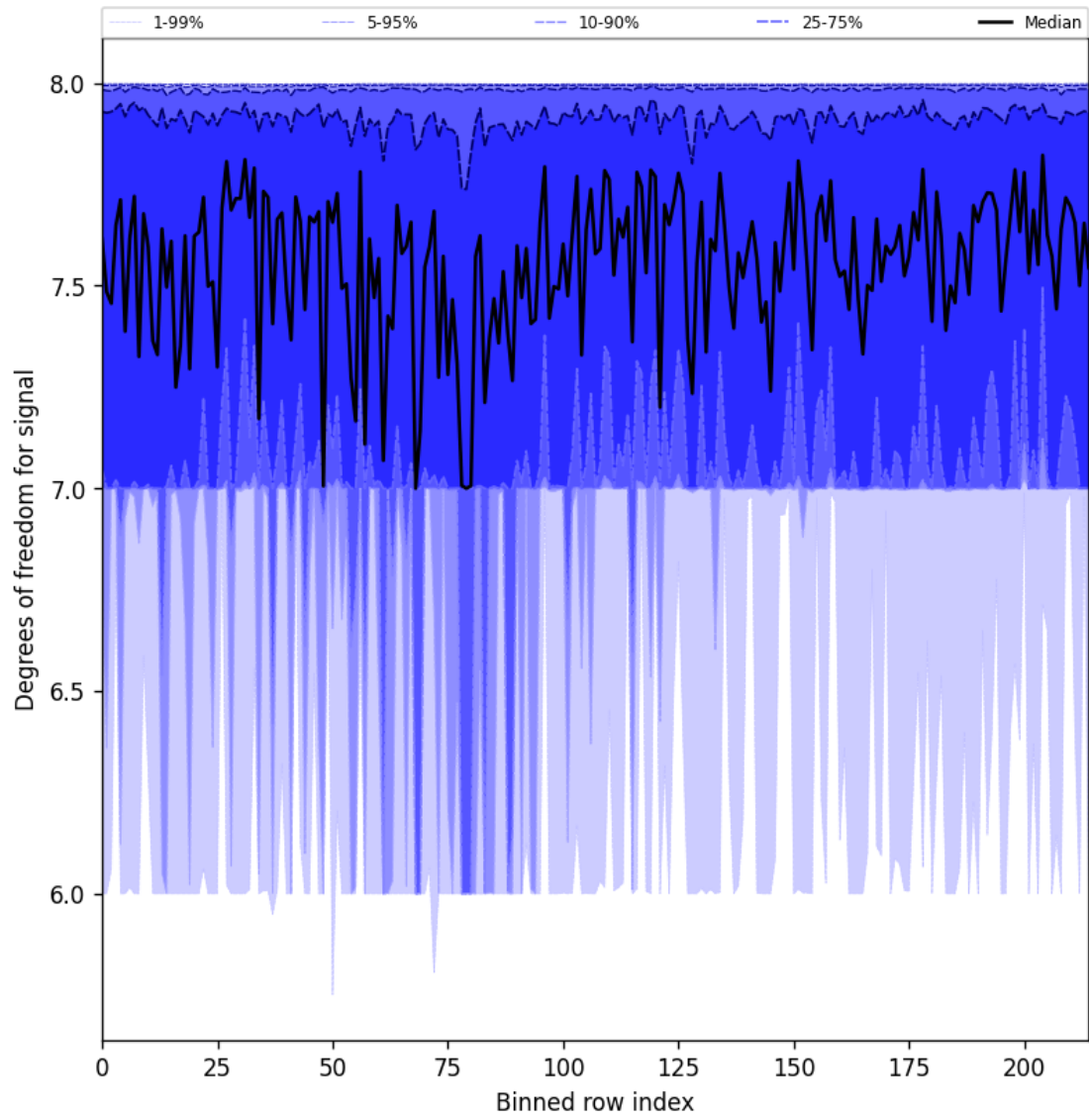
Figure 31: Along track statistics of “Degrees of freedom for signal” for 2024-09-22 to 2024-09-23
