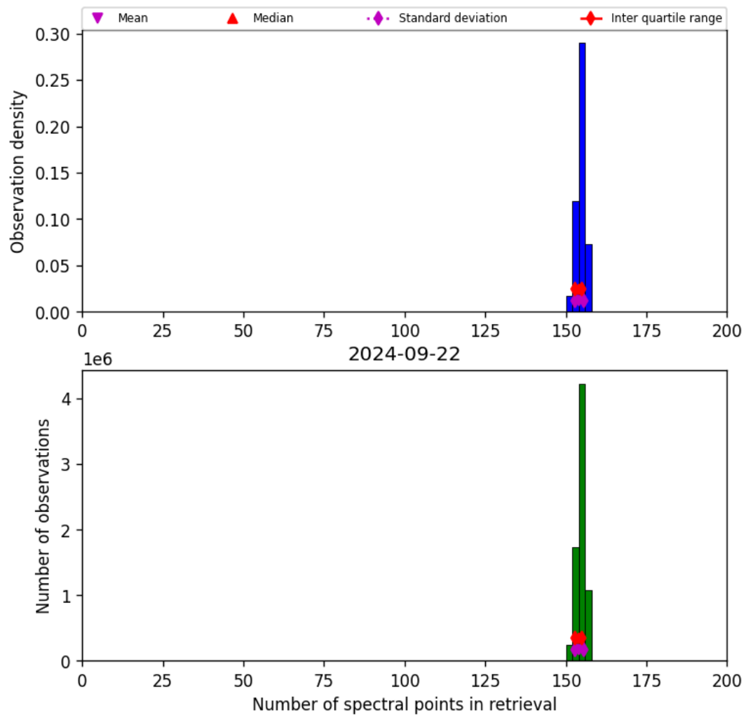
Figure 21: Histogram of “Number of spectral points in retrieval” for 2024-09-22 to 2024-09-23
