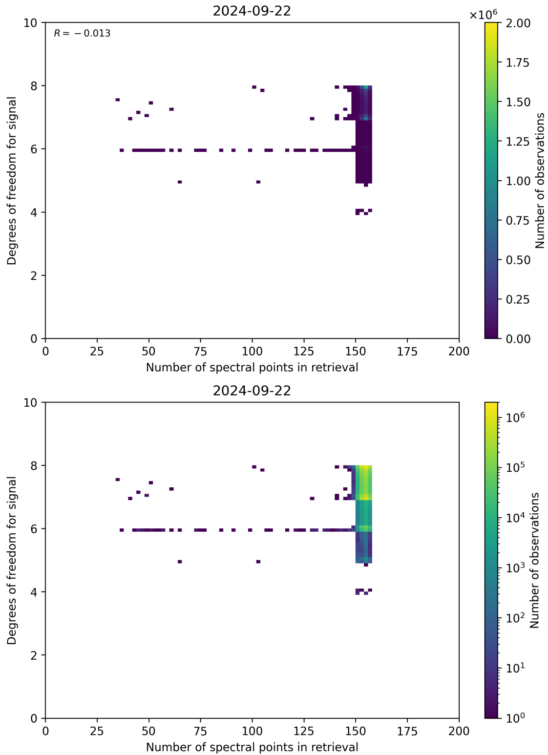
Figure 59: Scatter density plot of “Number of spectral points in retrieval” against “Degrees of freedom for signal” for 2024-09-22 to 2024-09-23.
