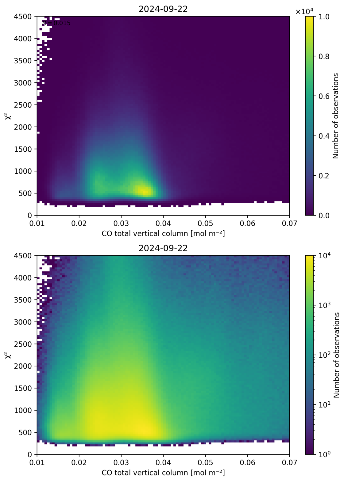
Figure 35: Scatter density plot of “CO total vertical column” against “ \chi^2 ” for 2024-09-22 to 2024-09-23.
