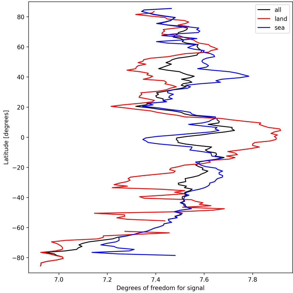
Figure 15: Zonal average of “Degrees of freedom for signal” for 2024-09-22 to 2024-09-23.
