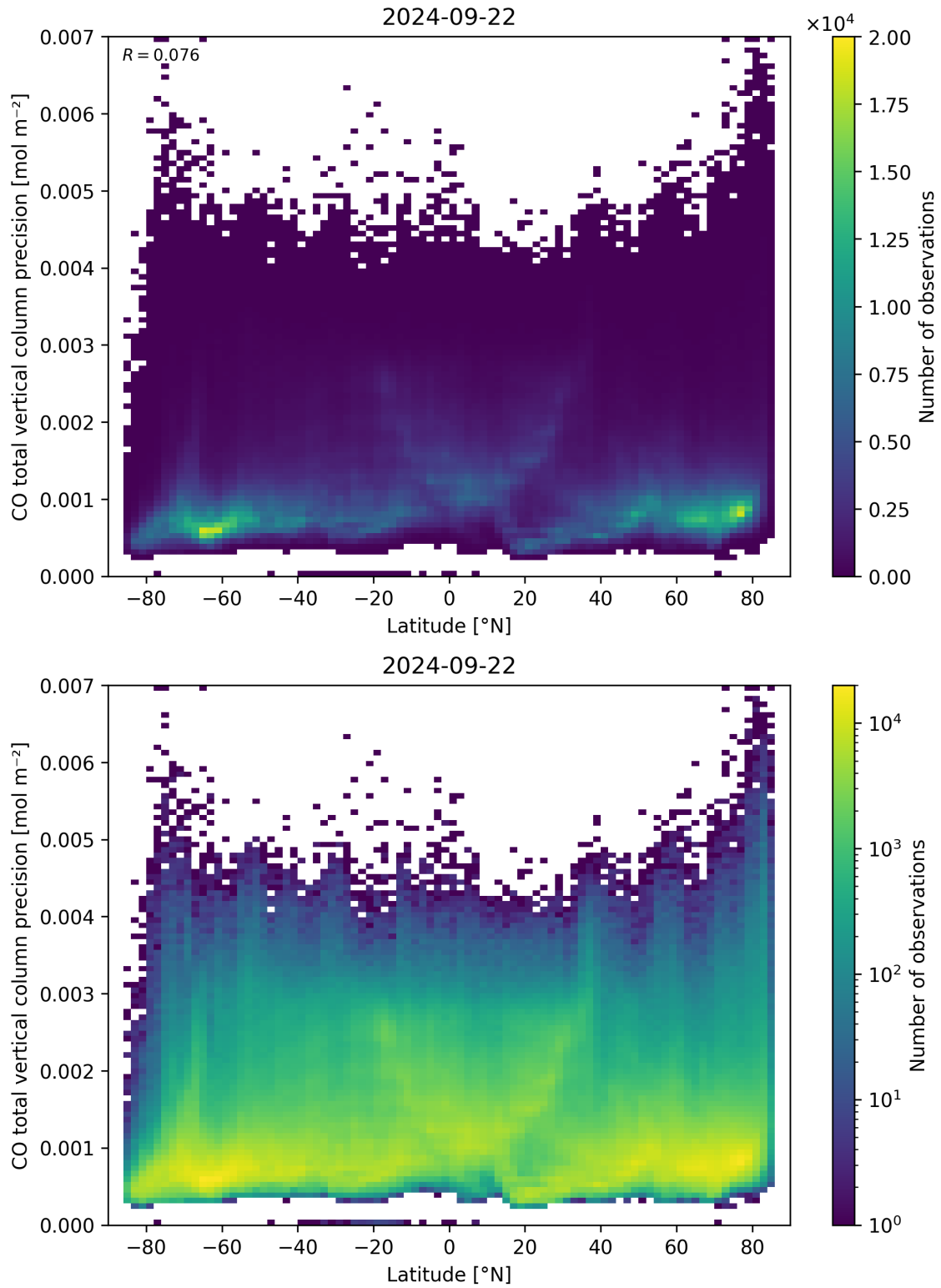
Figure 53: Scatter density plot of “Latitude” against “CO total vertical column precision” for 2024-09-22 to 2024-09-23.
