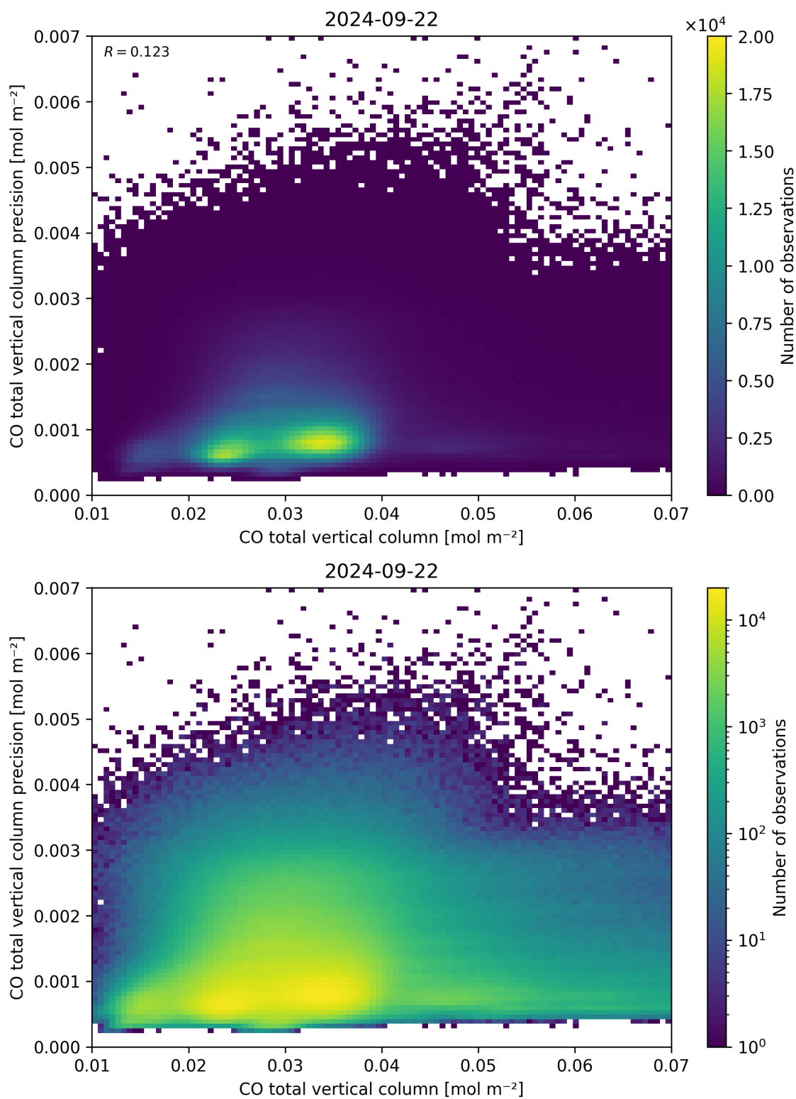
Figure 34: Scatter density plot of “CO total vertical column” against “CO total vertical column precision” for 2024-09-22 to 2024-09-23.
