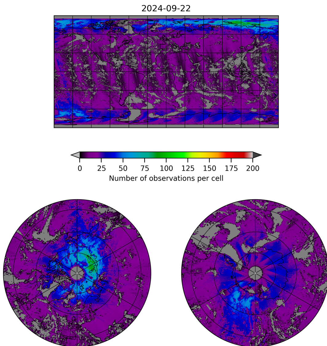
Figure 8: Map of the number of observations for 2024-09-22 to 2024-09-23
