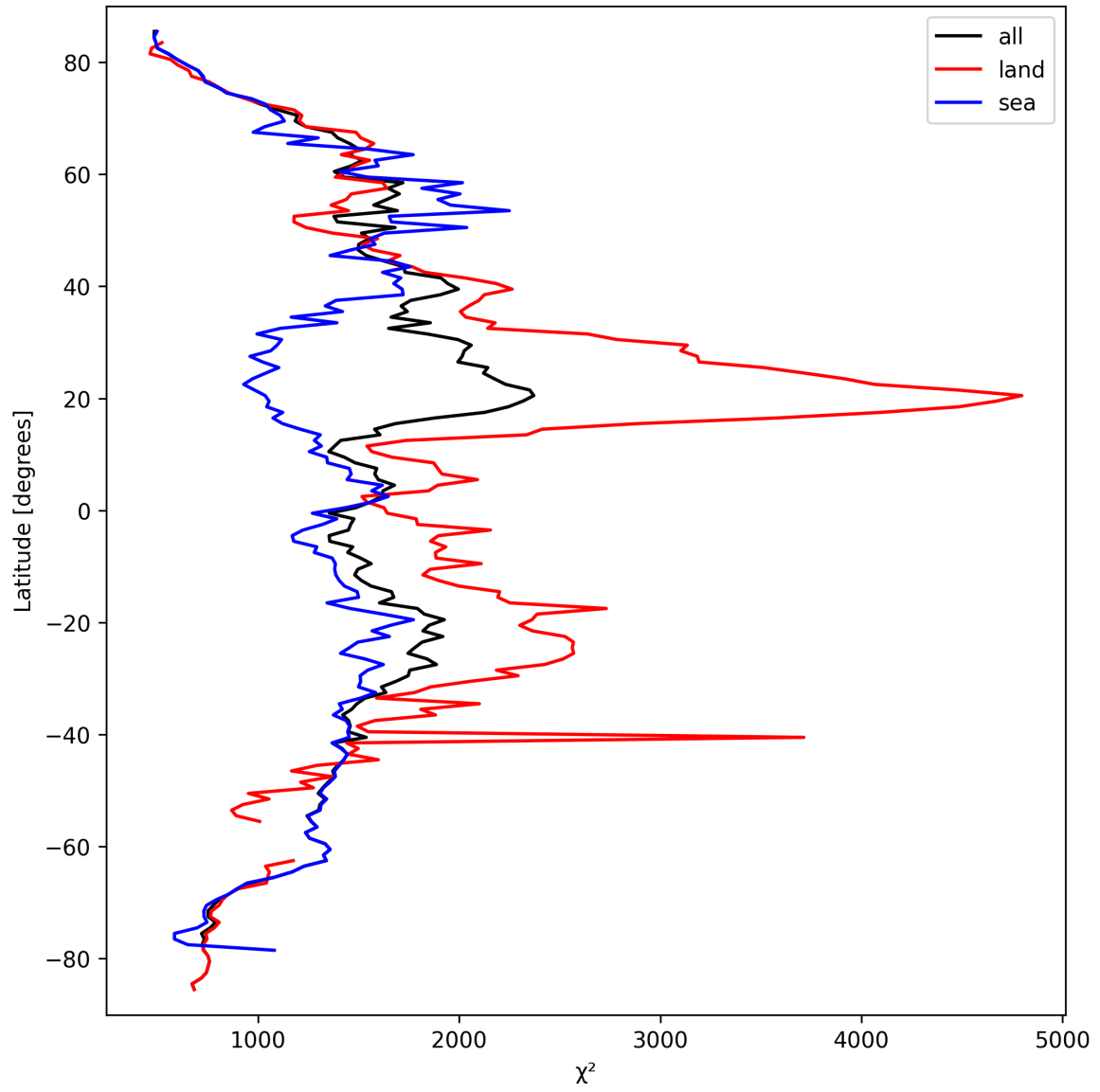
Figure 14: Zonal average of “ \chi^2 ” for 2024-09-22 to 2024-09-23.
