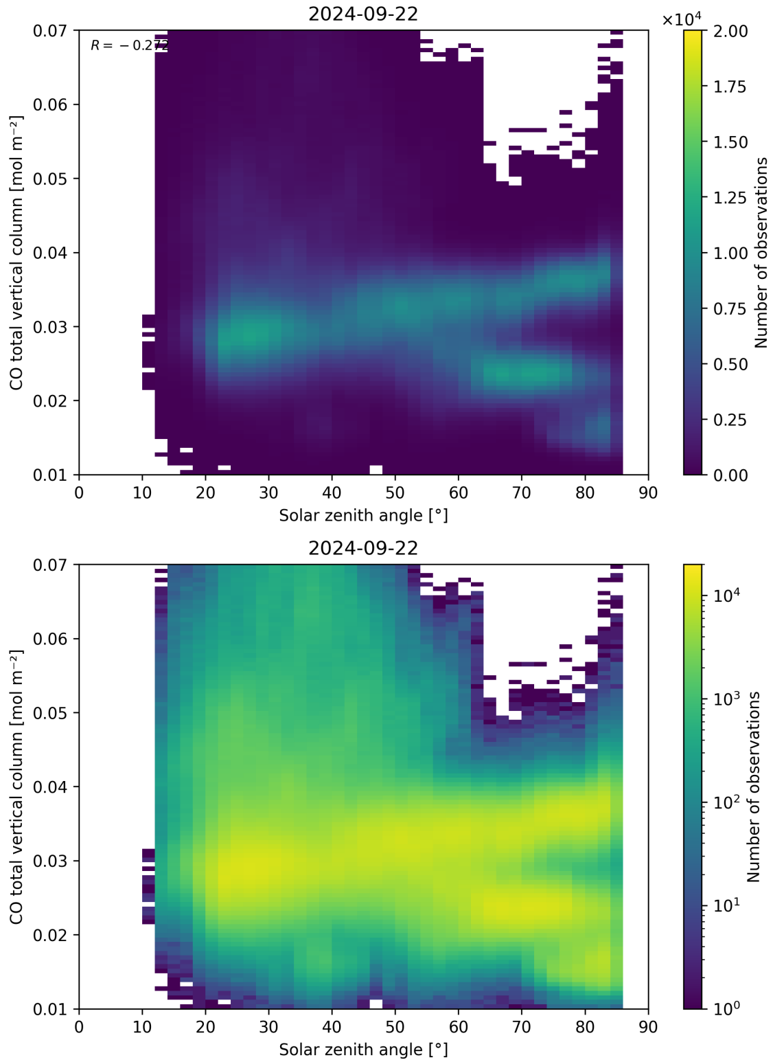
Figure 61: Scatter density plot of “Solar zenith angle” against “CO total vertical column” for 2024-09-22 to 2024-09-23.
