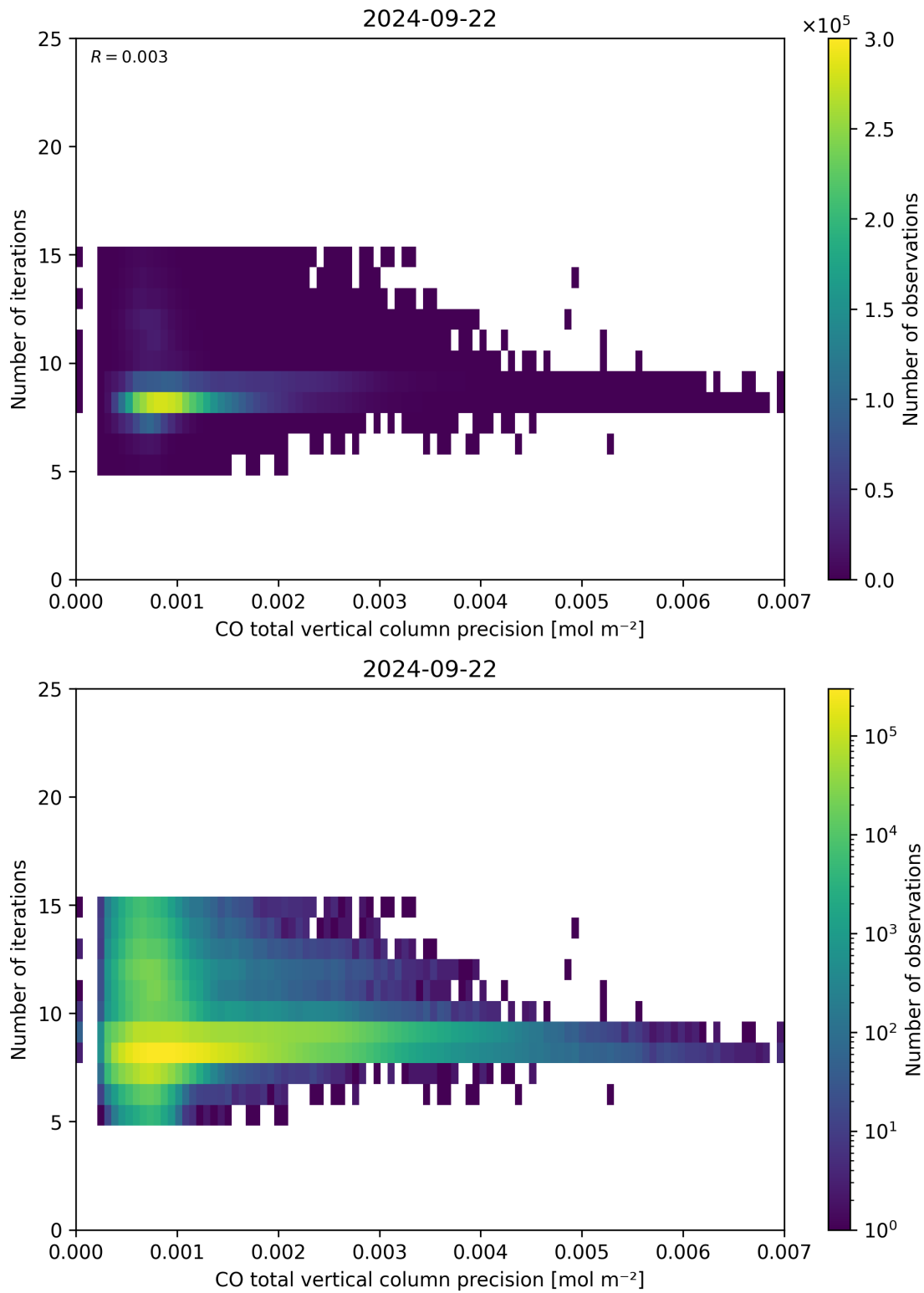
Figure 46: Scatter density plot of “CO total vertical column precision” against “Number of iterations” for 2024-09-22 to 2024-09-23.
