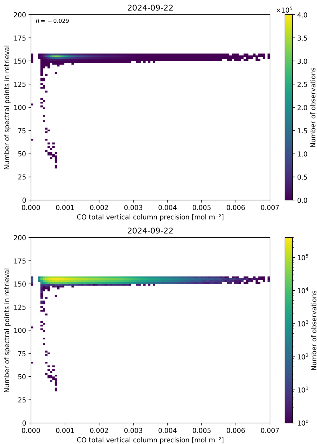
Figure 47: Scatter density plot of “CO total vertical column precision” against “Number of spectral points in retrieval” for 2024-09-22 to 2024-09-23.
