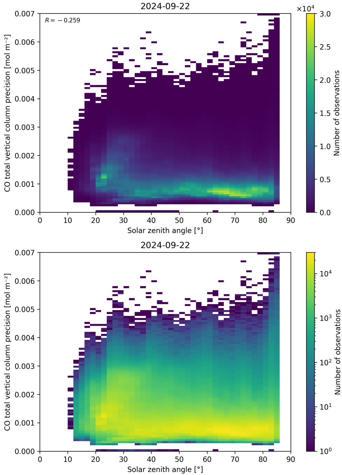
Figure 63: Scatter density plot of “Solar zenith angle” against “CO total vertical column precision” for 2024-09-22 to 2024-09-23.
