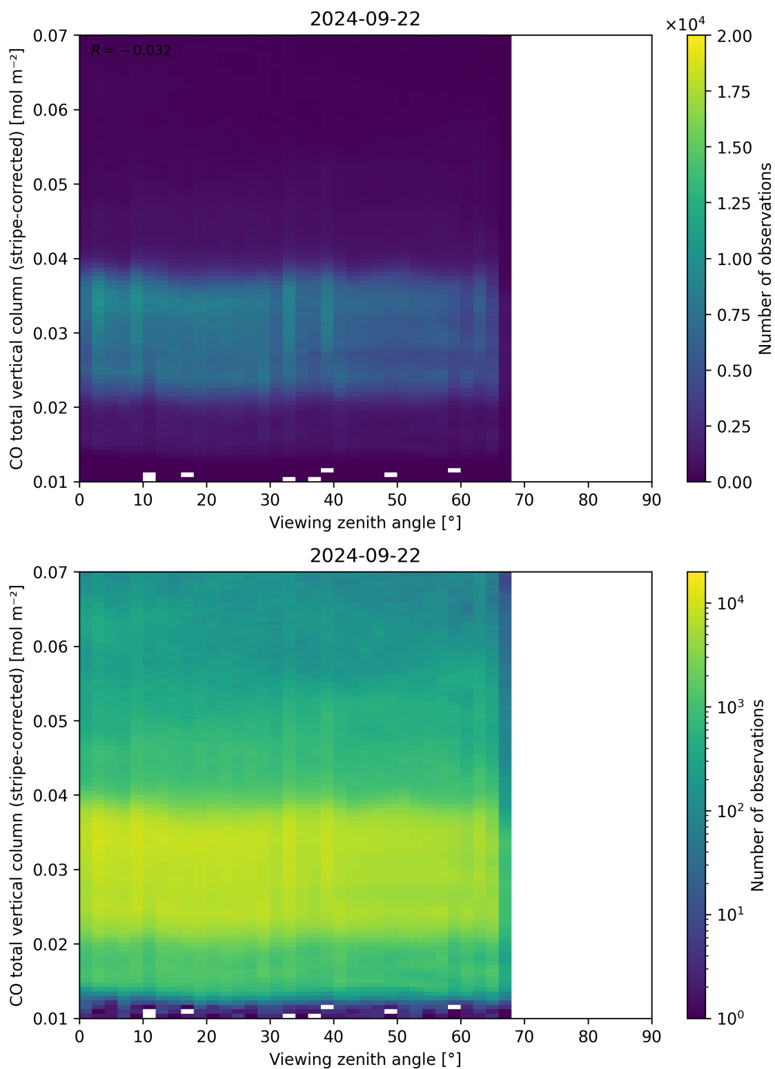
Figure 70: Scatter density plot of “Viewing zenith angle” against “CO total vertical column (stripe-corrected)” for 2024-09-22 to 2024-09-23.
