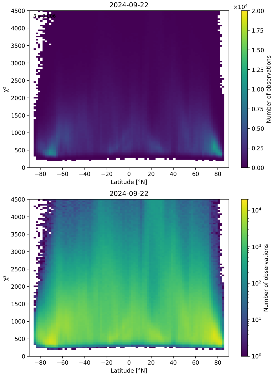
Figure 54: Scatter density plot of “Latitude” against “ \chi^2 ” for 2024-09-22 to 2024-09-23.
