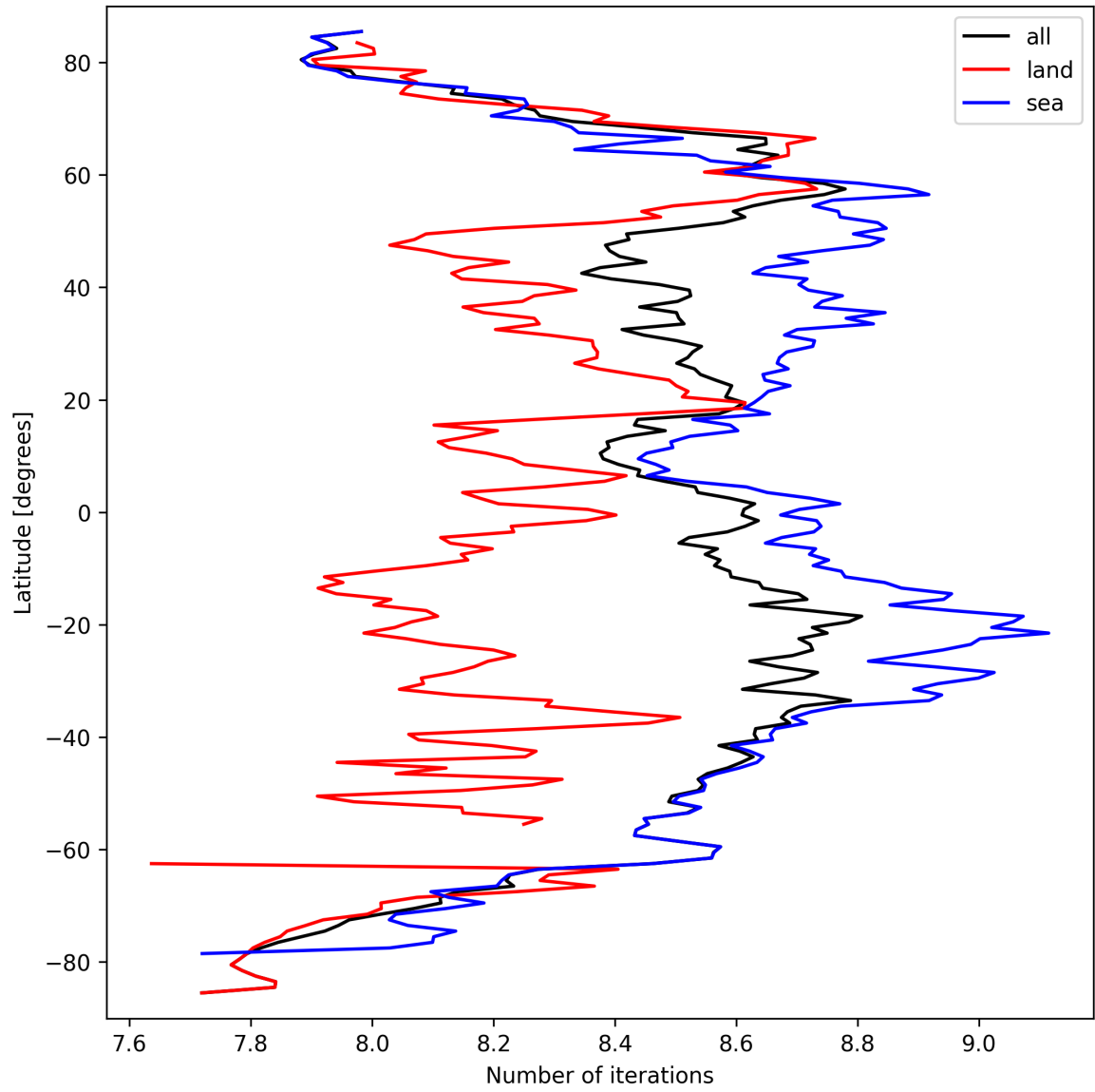
Figure 16: Zonal average of “Number of iterations” for 2024-09-22 to 2024-09-23.
