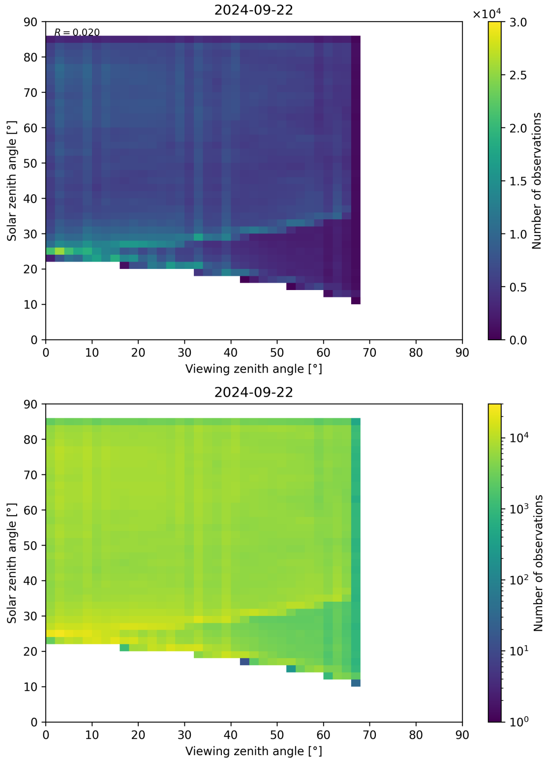
Figure 77: Scatter density plot of “Viewing zenith angle” against “Solar zenith angle” for 2024-09-22 to 2024-09-23.
