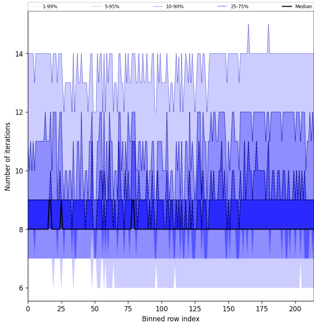
Figure 32: Along track statistics of “Number of iterations” for 2024-09-22 to 2024-09-23
