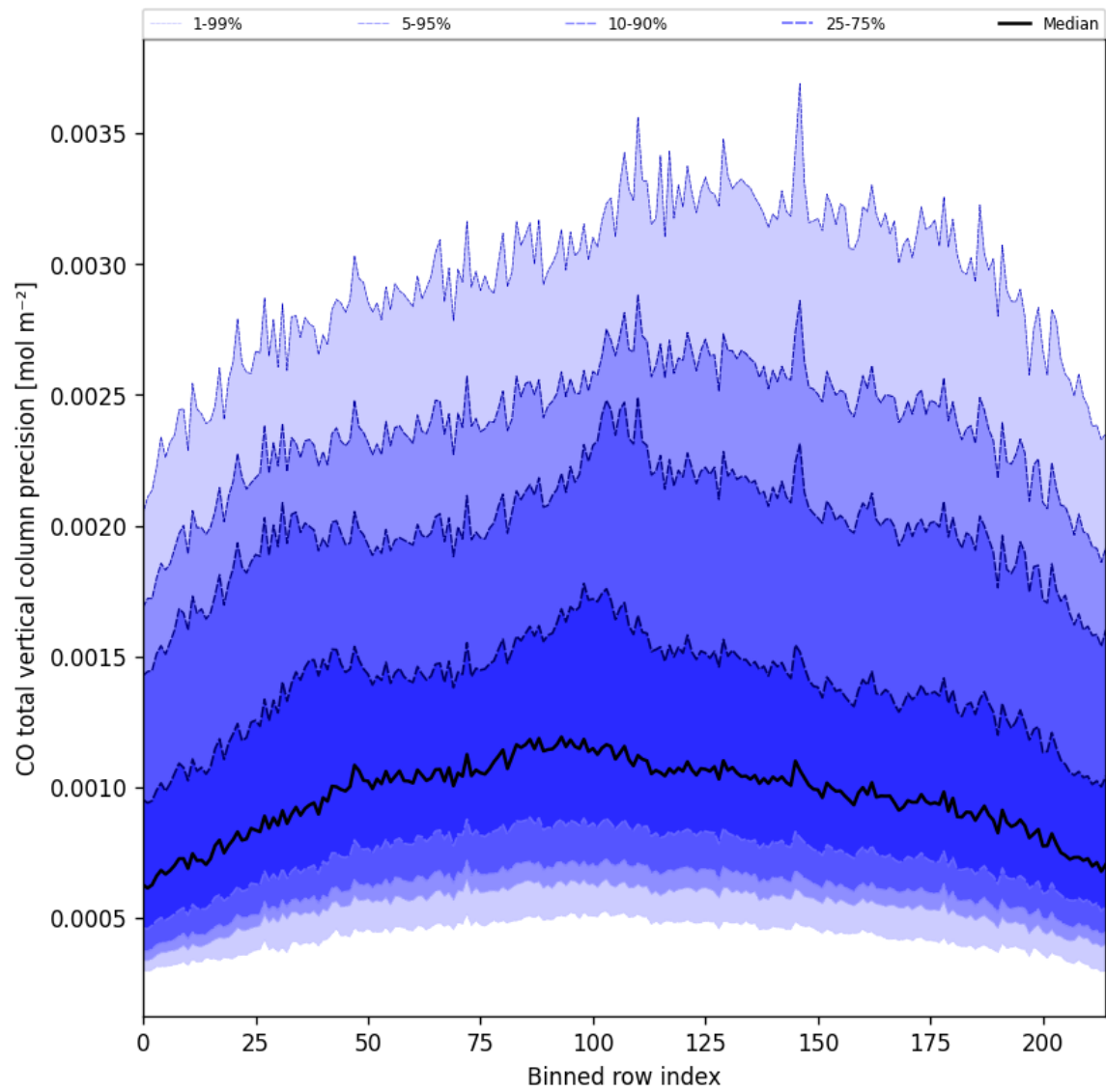
Figure 28: Along track statistics of “CO total vertical column precision” for 2024-09-22 to 2024-09-23
