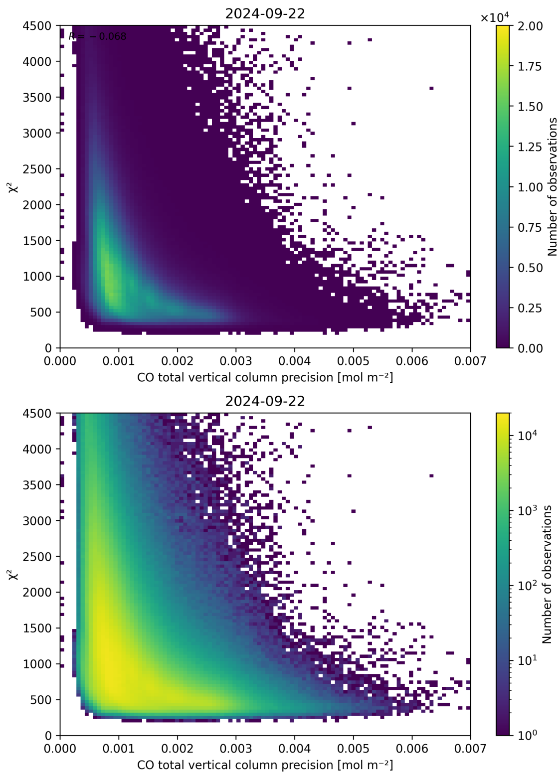
Figure 44: Scatter density plot of “CO total vertical column precision” against “ \chi^2 ” for 2024-09-22 to 2024-09-23.
