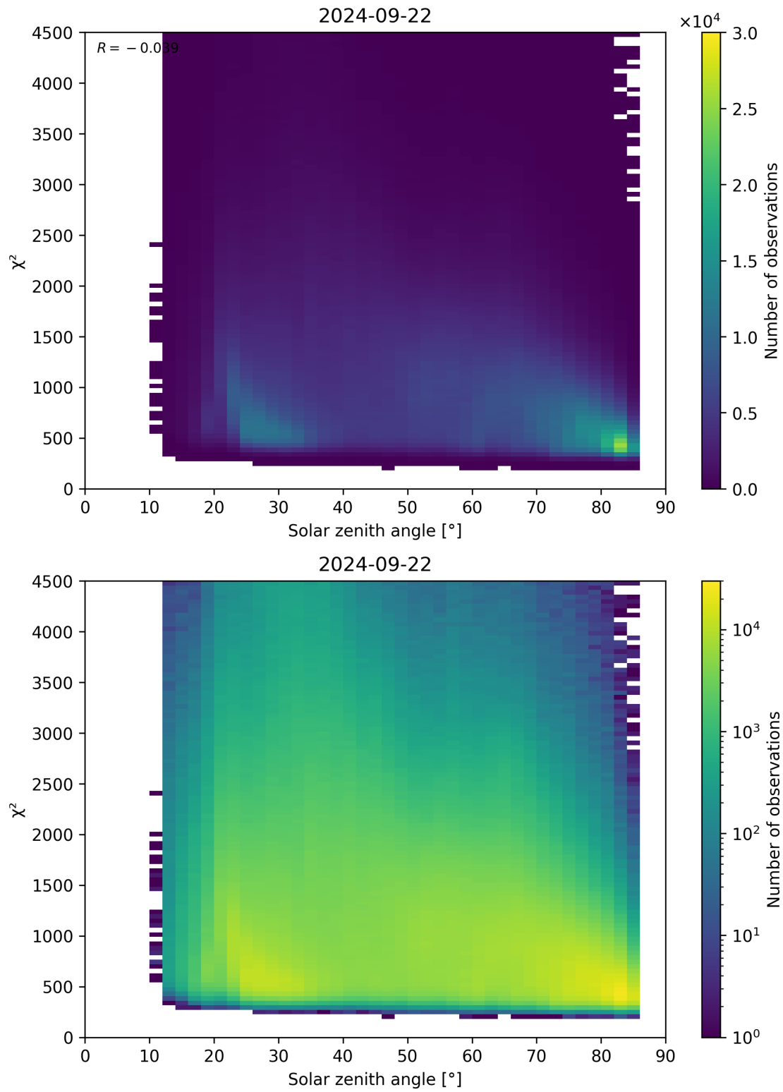
Figure 64: Scatter density plot of “Solar zenith angle” against “ \chi^2 ” for 2024-09-22 to 2024-09-23.
