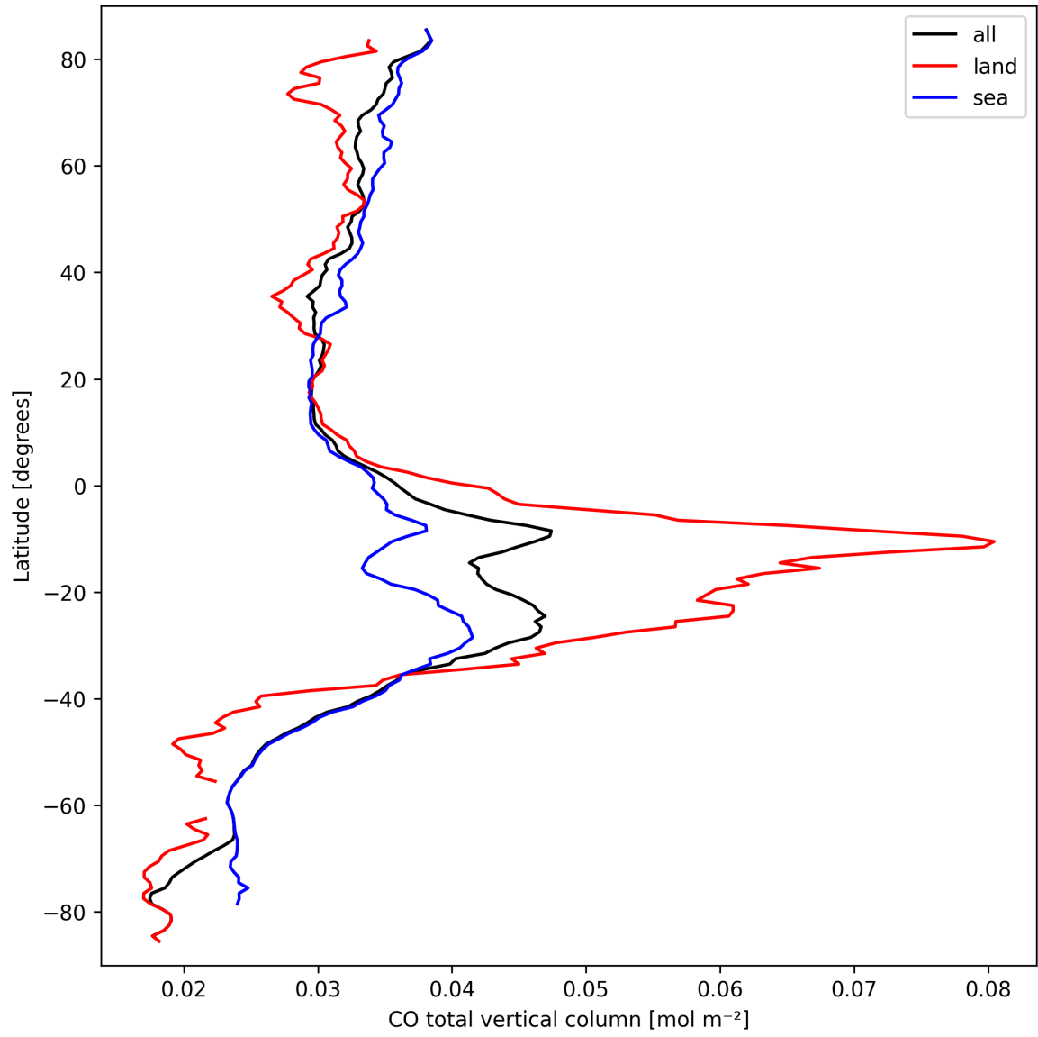
Figure 10: Zonal average of “CO total vertical column” for 2024-09-22 to 2024-09-23.
