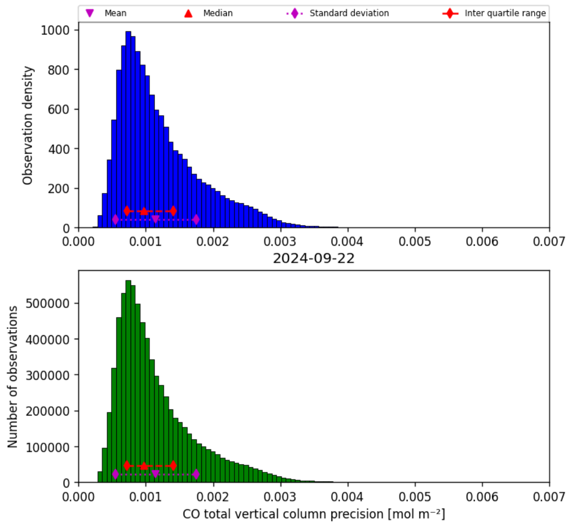
Figure 20: Histogram of “CO total vertical column precision” for 2024-09-22 to 2024-09-23
