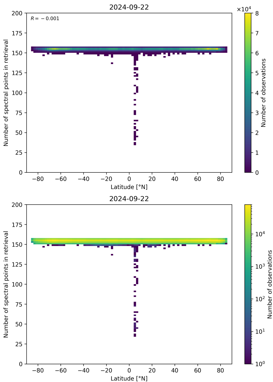
Figure 57: Scatter density plot of “Latitude” against “Number of spectral points in retrieval” for 2024-09-22 to 2024-09-23.
