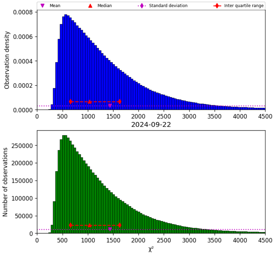
Figure 22: Histogram of " \chi^2 " for 2024-09-22 to 2024-09-23
