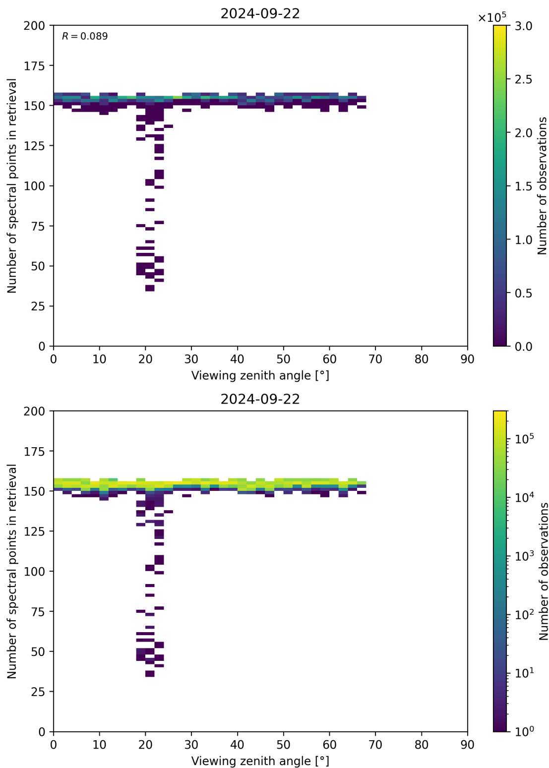
Figure 76: Scatter density plot of “Viewing zenith angle” against “Number of spectral points in retrieval” for 2024-09-22 to 2024-09-23.
