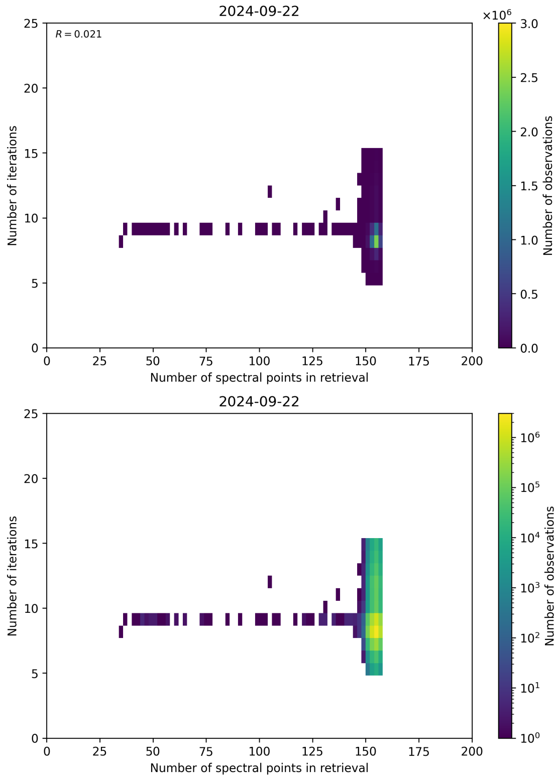
Figure 60: Scatter density plot of “Number of spectral points in retrieval” against “Number of iterations” for 2024-09-22 to 2024-09-23.
