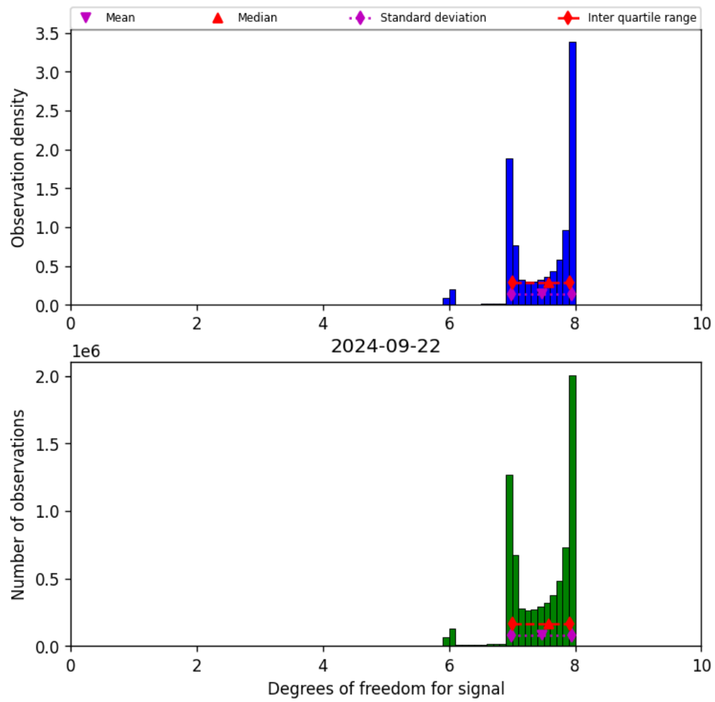
Figure 23: Histogram of “Degrees of freedom for signal” for 2024-09-22 to 2024-09-23
