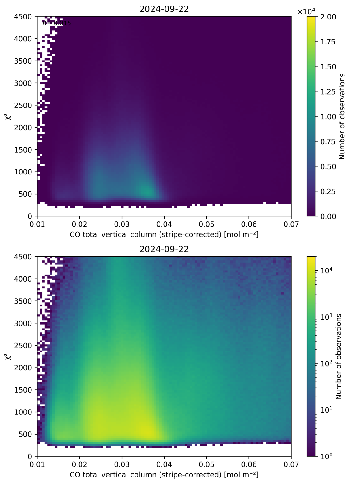
Figure 37: Scatter density plot of “CO total vertical column (stripe-corrected)” against “ \chi^2 ” for 2024-09-22 to 2024-09-23.
