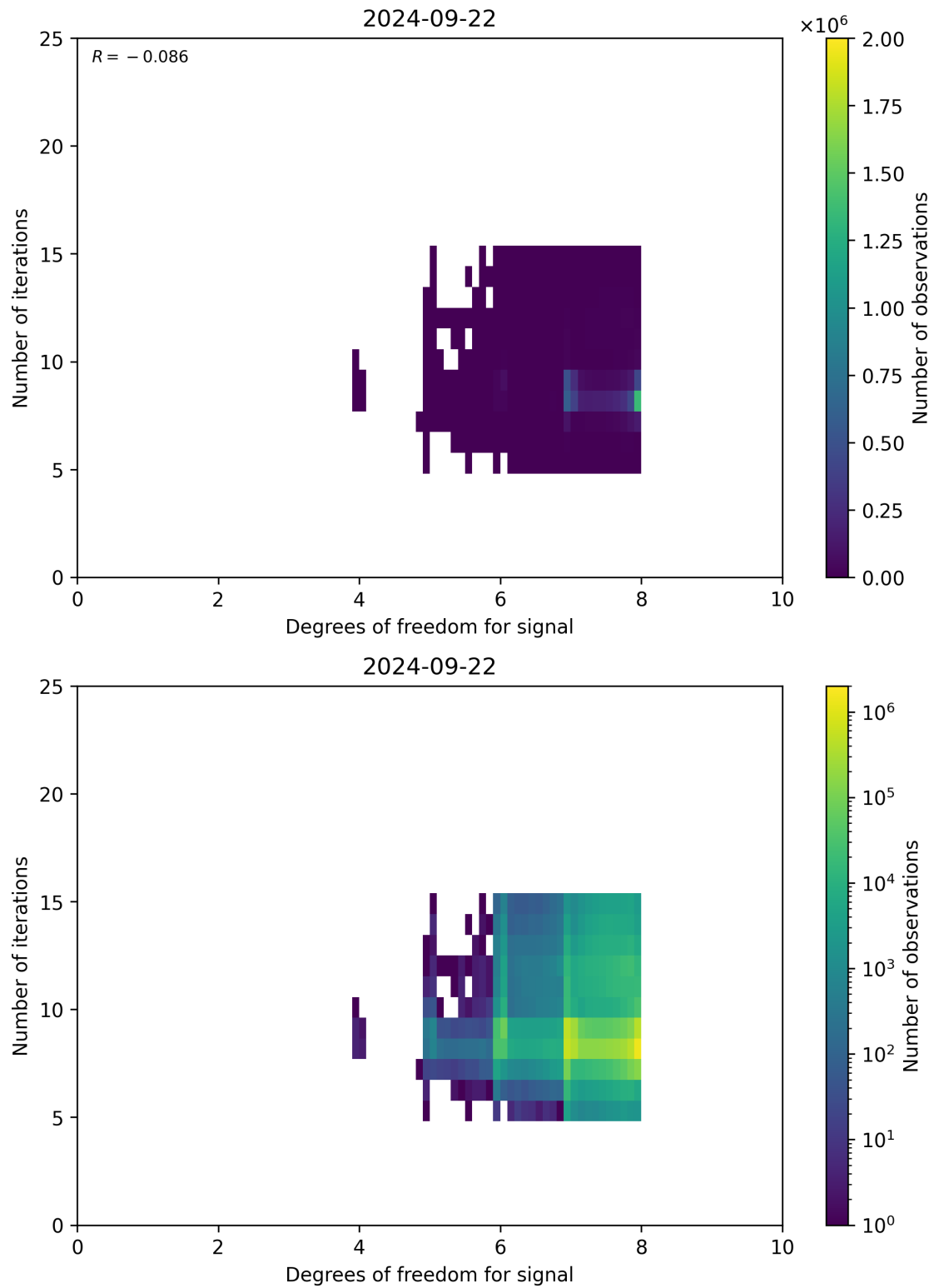
Figure 50: Scatter density plot of “Degrees of freedom for signal” against “Number of iterations” for 2024-09-22 to 2024-09-23.
