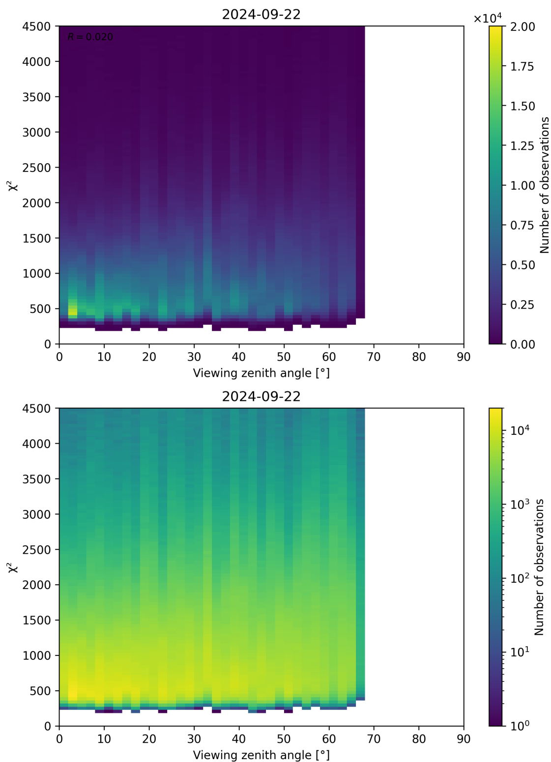
Figure 72: Scatter density plot of “Viewing zenith angle” against “ \chi^2 ” for 2024-09-22 to 2024-09-23.
