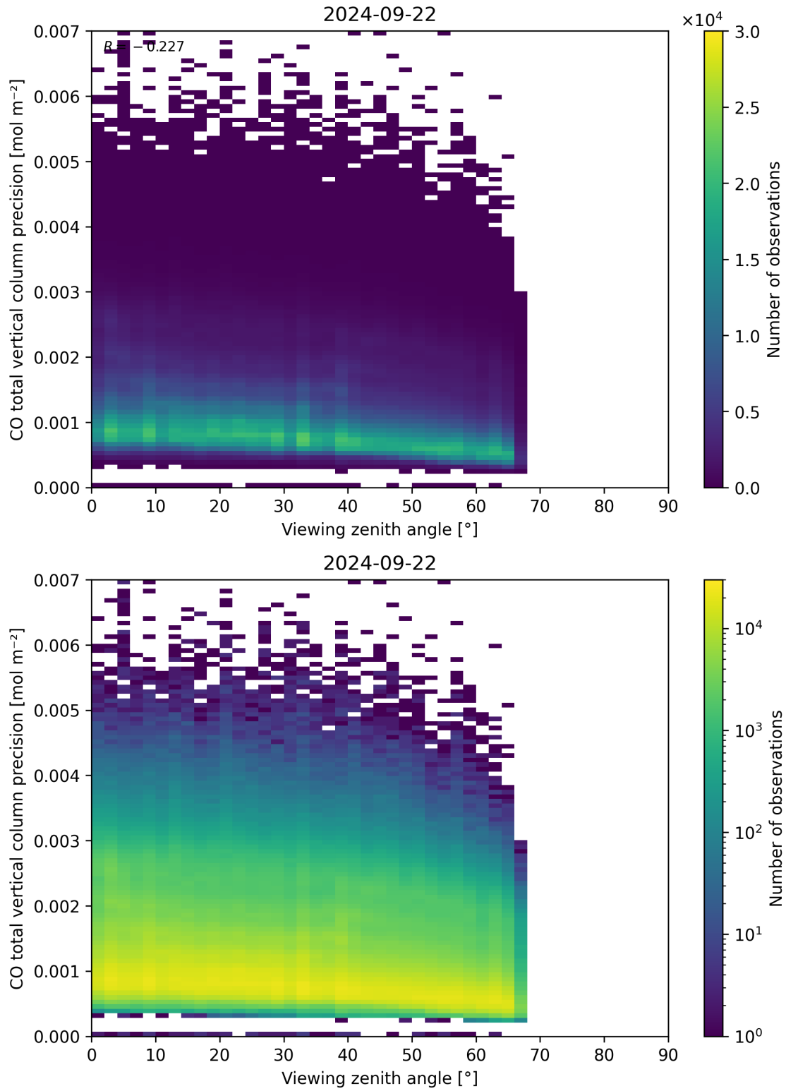
Figure 71: Scatter density plot of “Viewing zenith angle” against “CO total vertical column precision” for 2024-09-22 to 2024-09-23.
