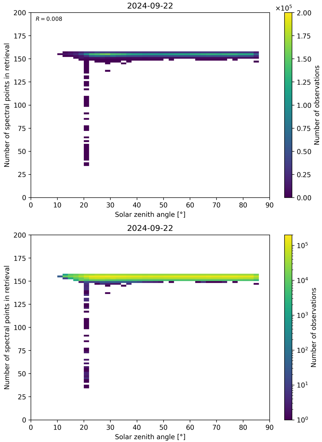
Figure 68: Scatter density plot of “Solar zenith angle” against “Number of spectral points in retrieval” for 2024-09-22 to 2024-09-23.
