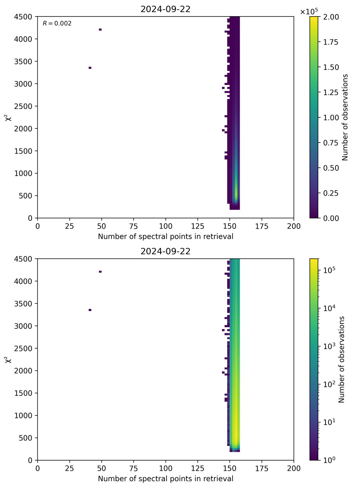
Figure 58: Scatter density plot of “Number of spectral points in retrieval” against “ \chi^2 ” for 2024-09-22 to 2024-09-23.
