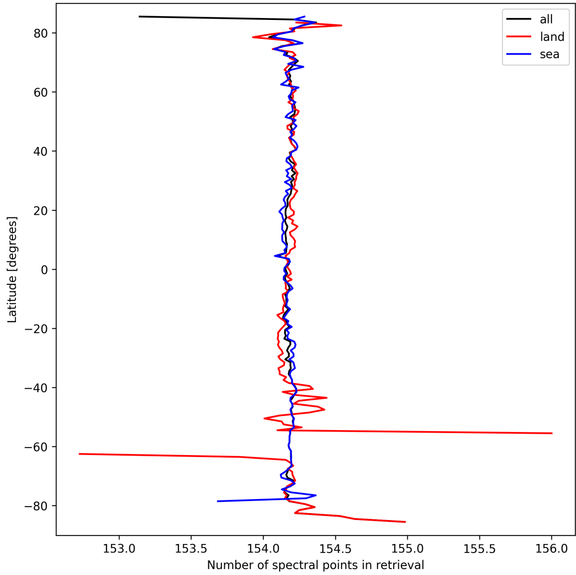
Figure 13: Zonal average of “Number of spectral points in retrieval” for 2024-09-22 to 2024-09-23.
