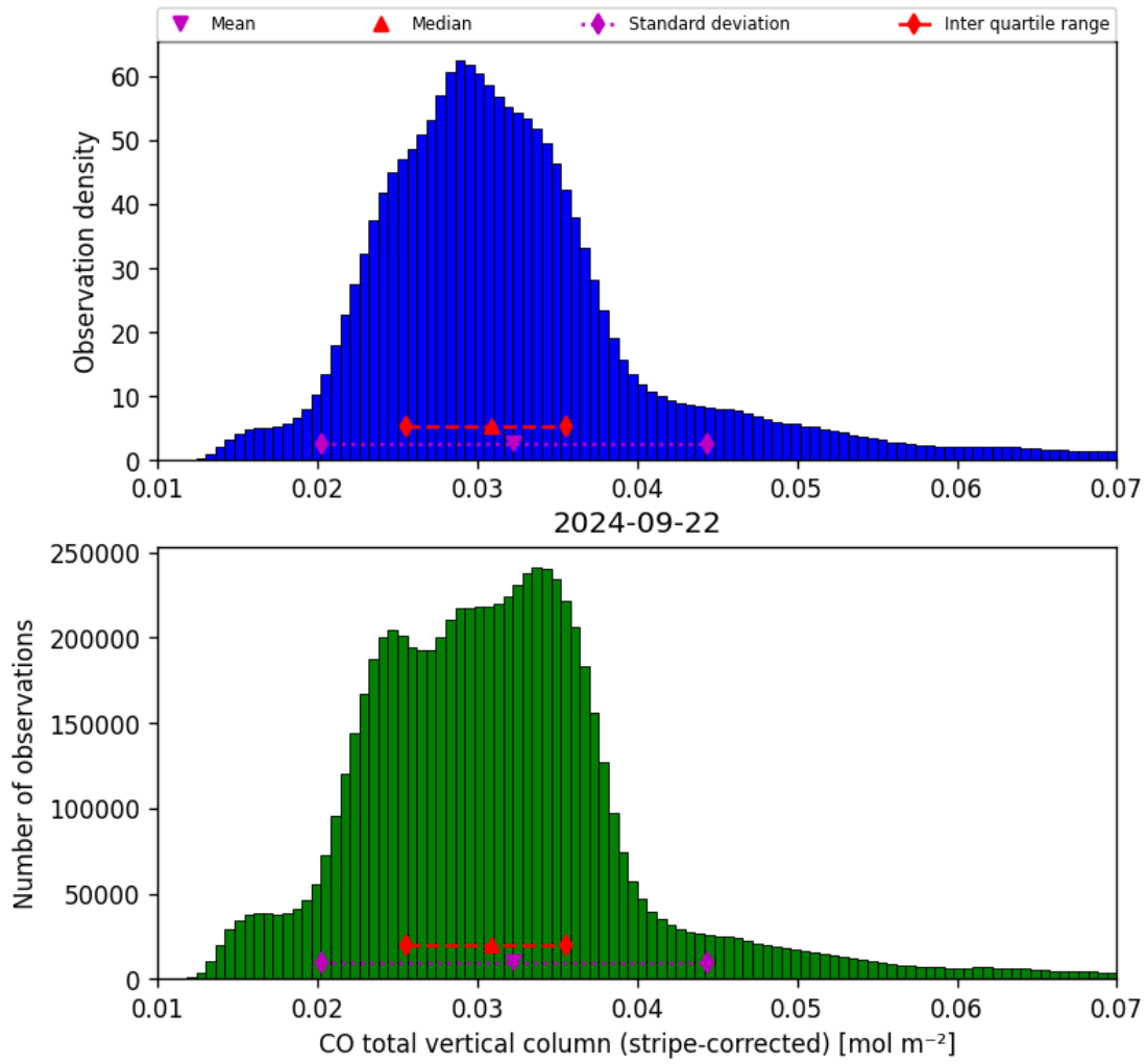
Figure 19: Histogram of “CO total vertical column (stripe-corrected)” for 2024-09-22 to 2024-09-23
