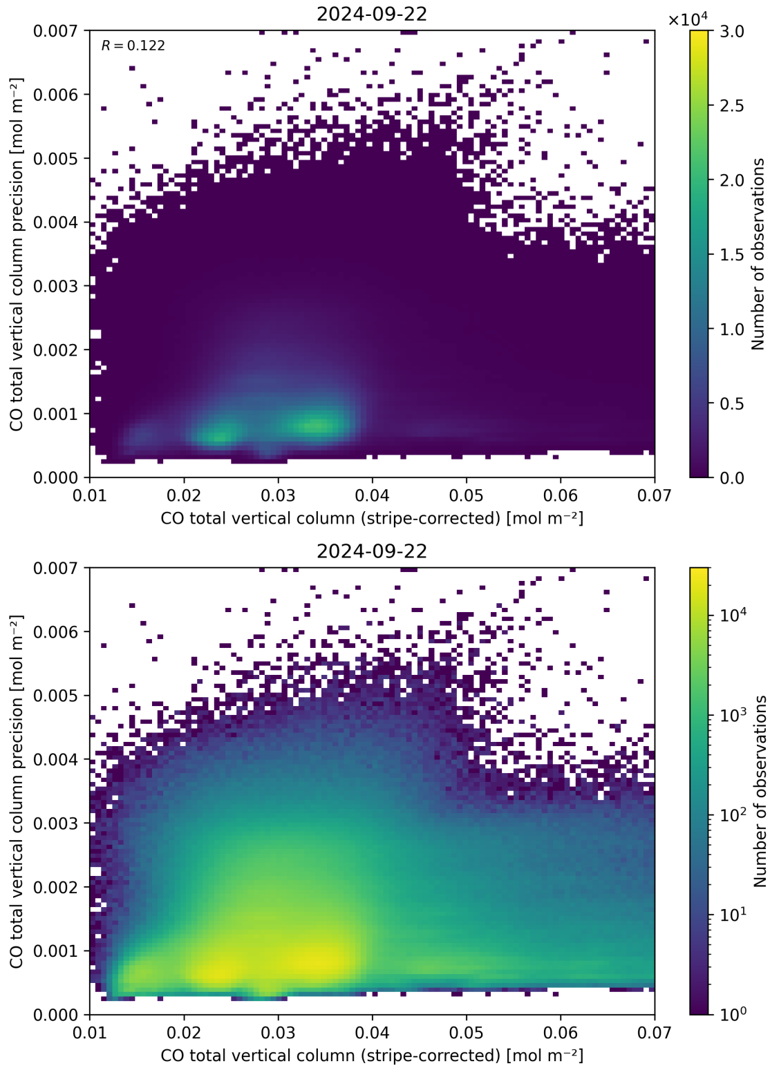
Figure 36: Scatter density plot of “CO total vertical column (stripe-corrected)” against “CO total vertical column precision” for 2024-09-22 to 2024-09-23.
