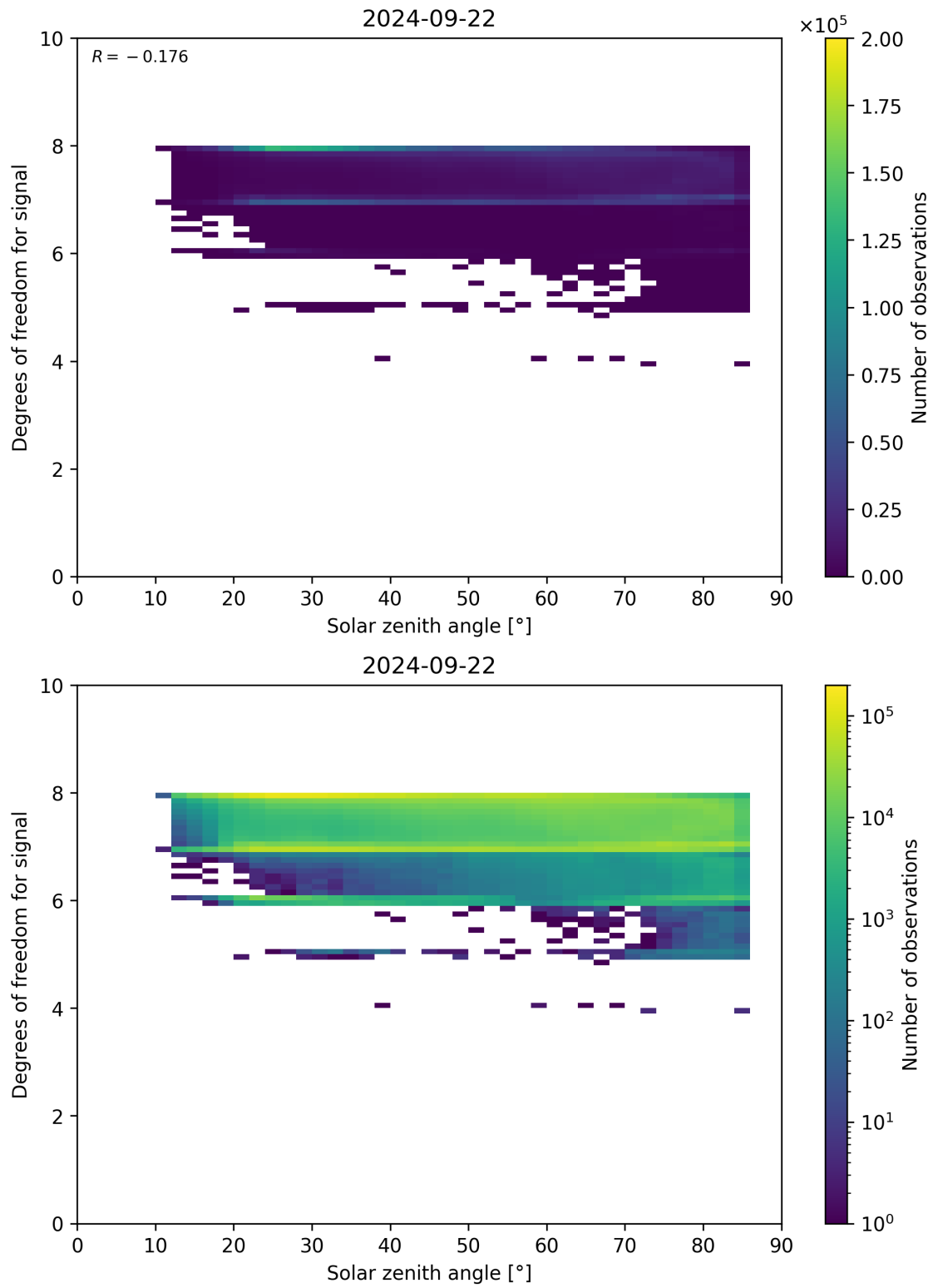
Figure 65: Scatter density plot of “Solar zenith angle” against “Degrees of freedom for signal” for 2024-09-22 to 2024-09-23.
