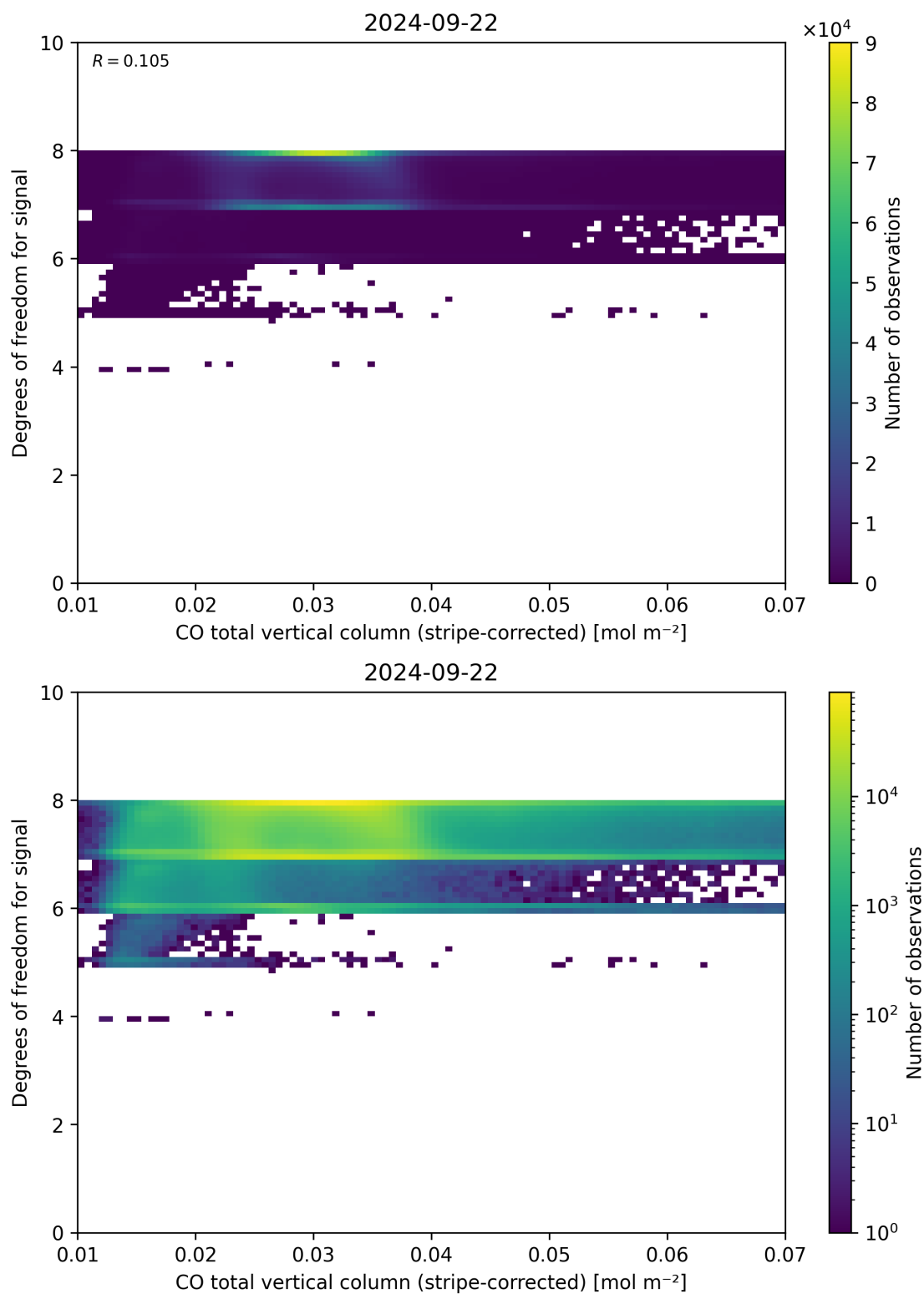
Figure 38: Scatter density plot of “CO total vertical column (stripe-corrected)” against “Degrees of freedom for signal” for 2024-09-22 to 2024-09-23.
