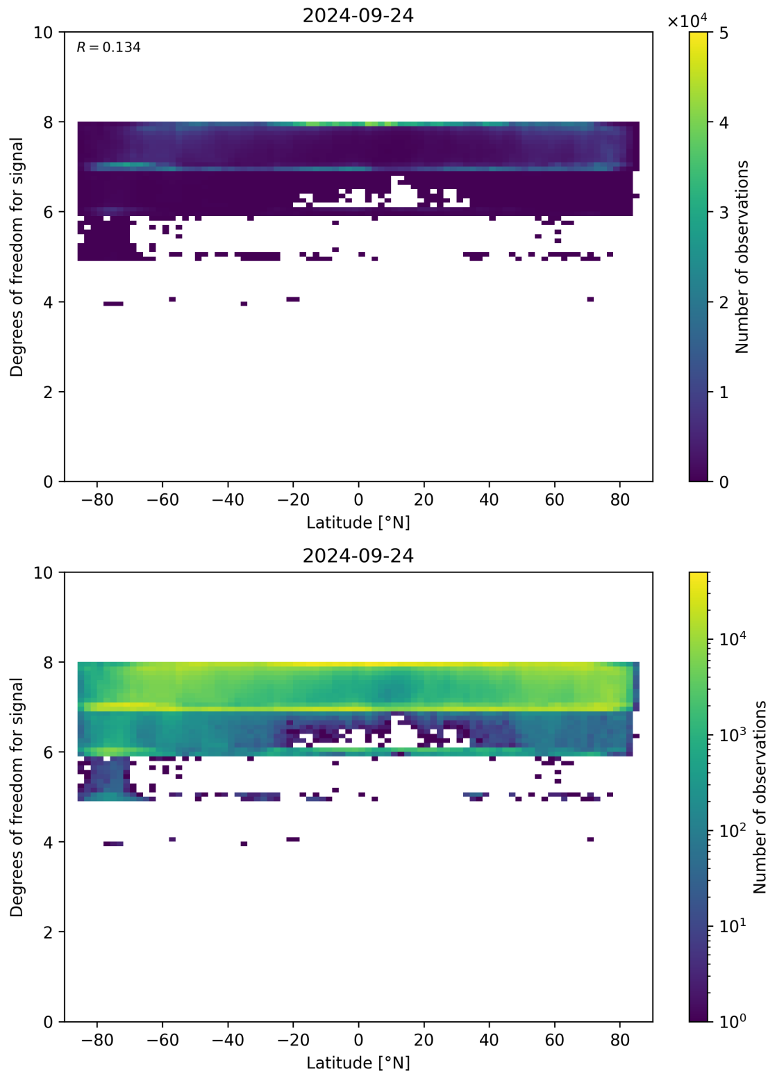
Figure 55: Scatter density plot of “Latitude” against “Degrees of freedom for signal” for 2024-09-23 to 2024-09-25.
