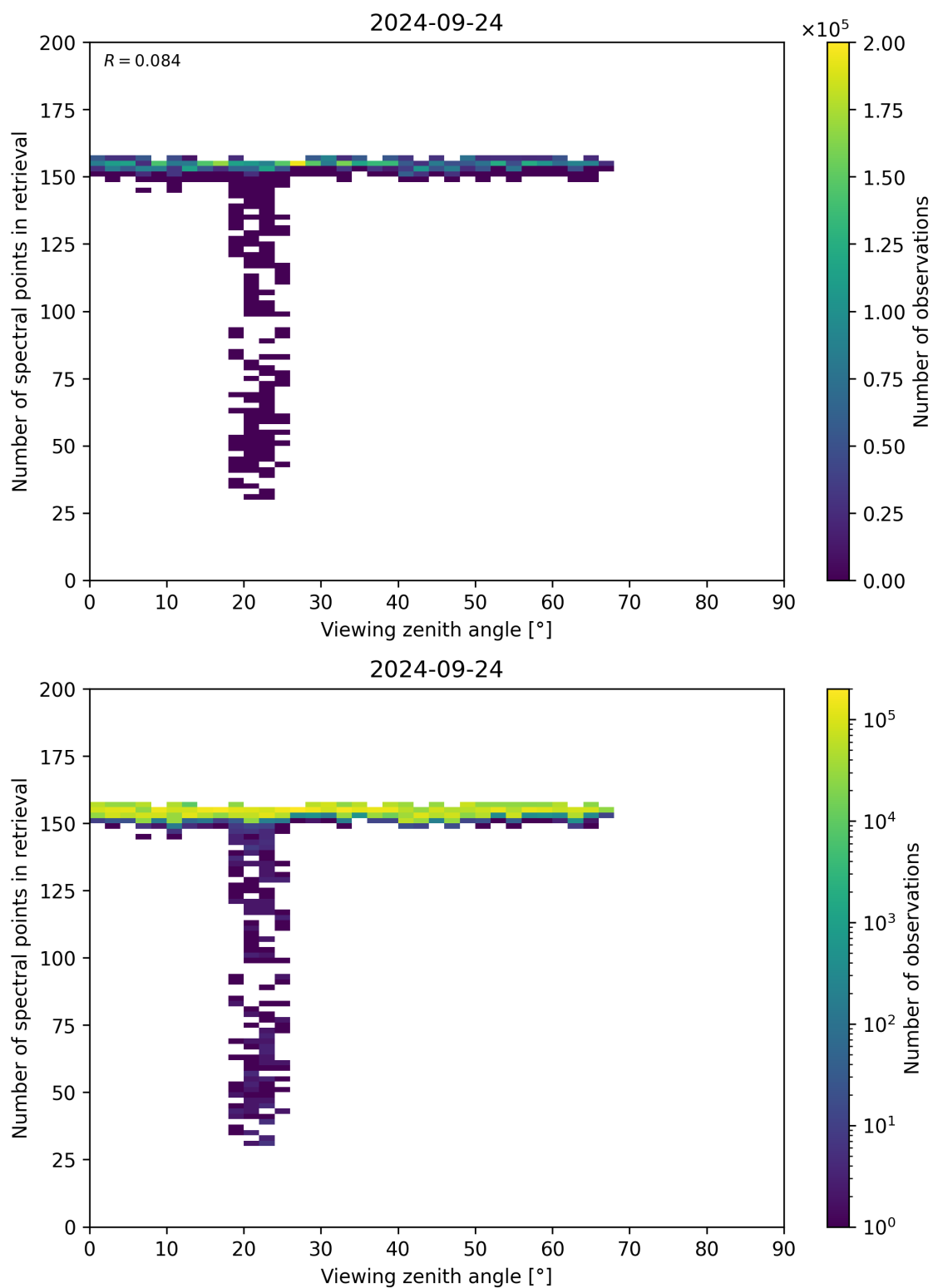
Figure 76: Scatter density plot of “Viewing zenith angle” against “Number of spectral points in retrieval” for 2024-09-23 to 2024-09-25.
