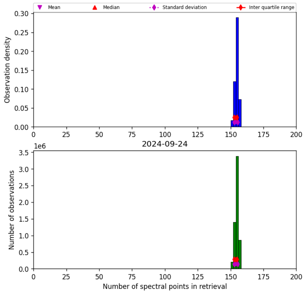
Figure 21: Histogram of “Number of spectral points in retrieval” for 2024-09-23 to 2024-09-25
