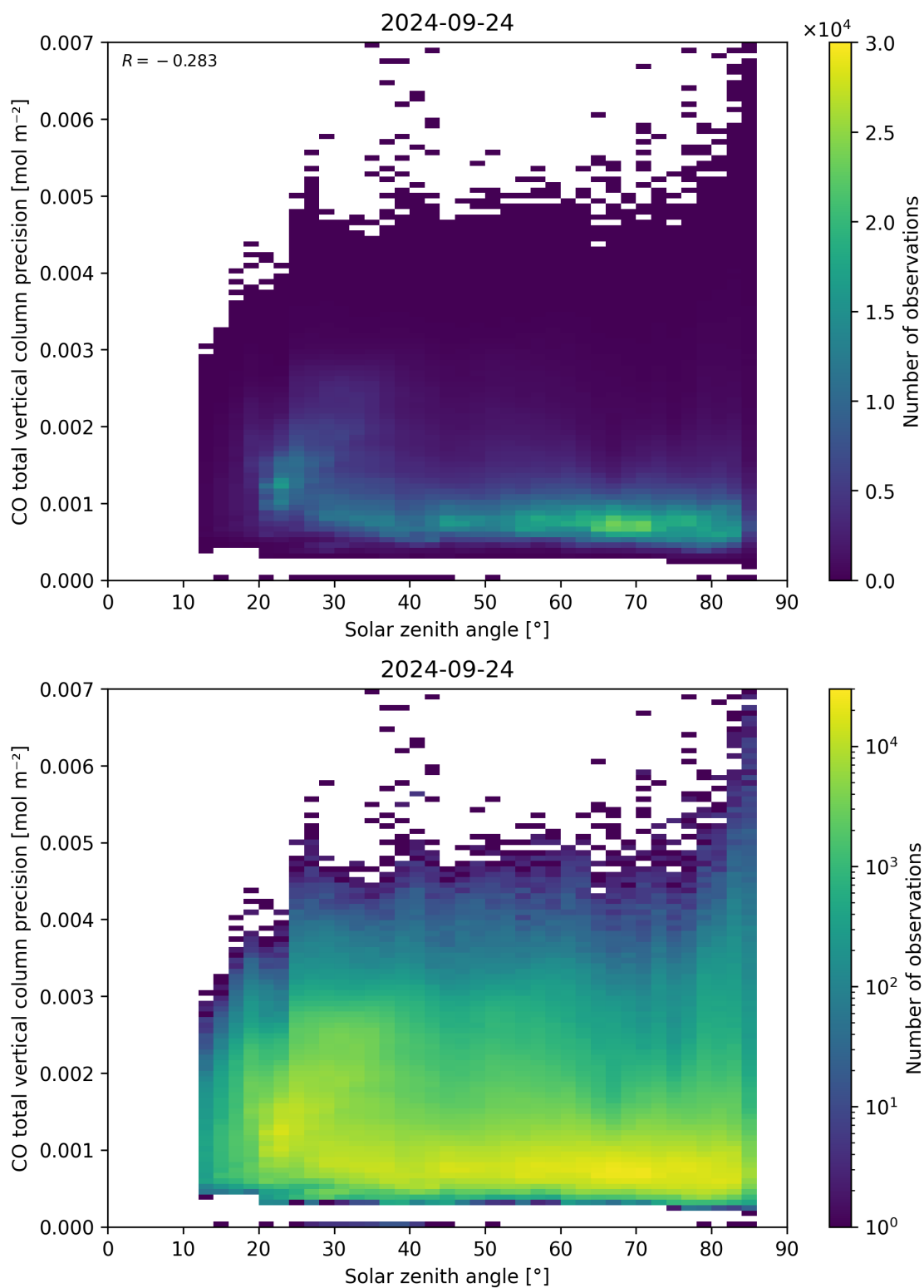
Figure 63: Scatter density plot of “Solar zenith angle” against “CO total vertical column precision” for 2024-09-23 to 2024-09-25.
