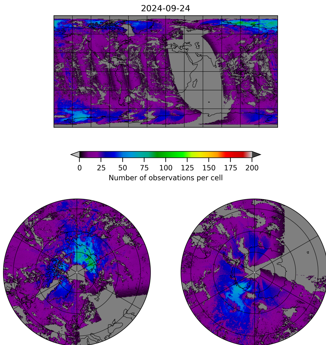
Figure 8: Map of the number of observations for 2024-09-23 to 2024-09-25
