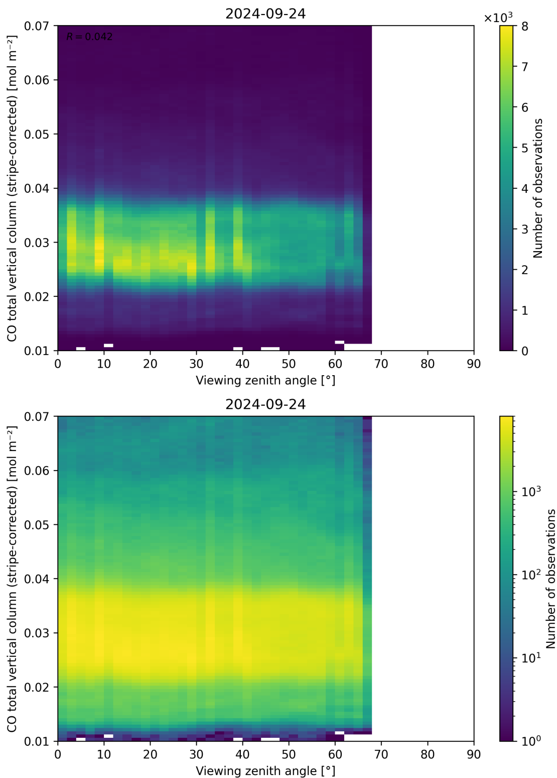
Figure 70: Scatter density plot of “Viewing zenith angle” against “CO total vertical column (stripe-corrected)” for 2024-09-23 to 2024-09-25.
