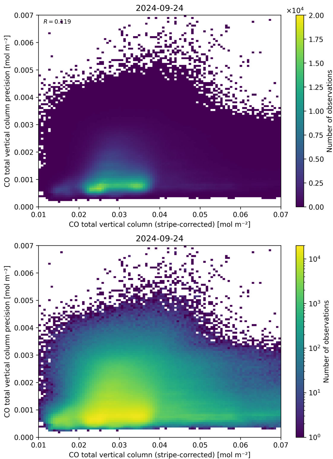
Figure 36: Scatter density plot of “CO total vertical column (stripe-corrected)” against “CO total vertical column precision” for 2024-09-23 to 2024-09-25.
