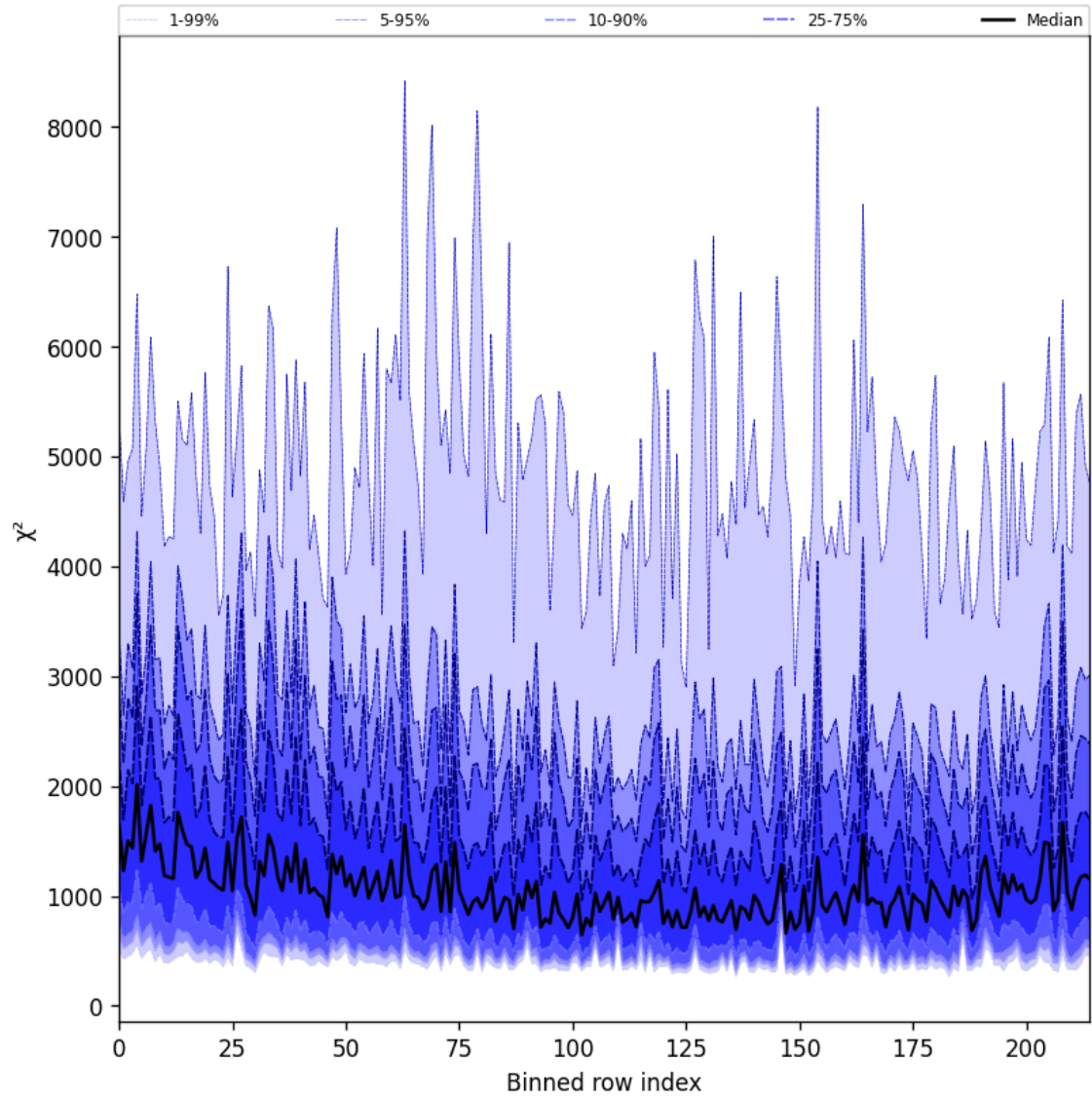
Figure 30: Along track statistics of “ \chi^2 ” for 2024-09-23 to 2024-09-25
