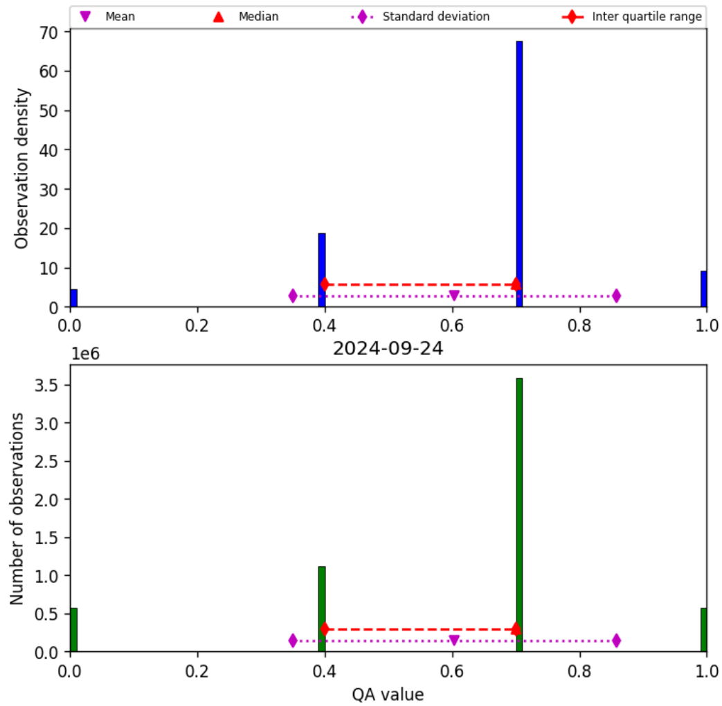
Figure 17: Histogram of “QA value” for 2024-09-23 to 2024-09-25
