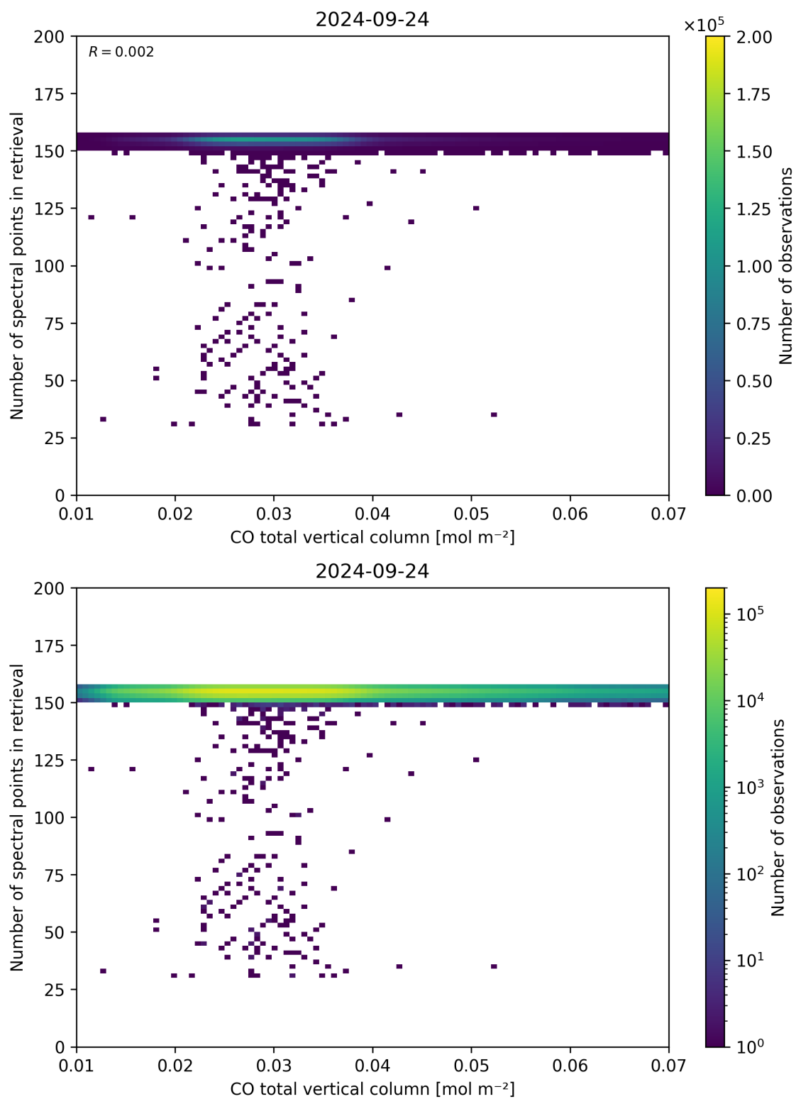
Figure 43: Scatter density plot of “CO total vertical column” against “Number of spectral points in retrieval” for 2024-09-23 to 2024-09-25.
