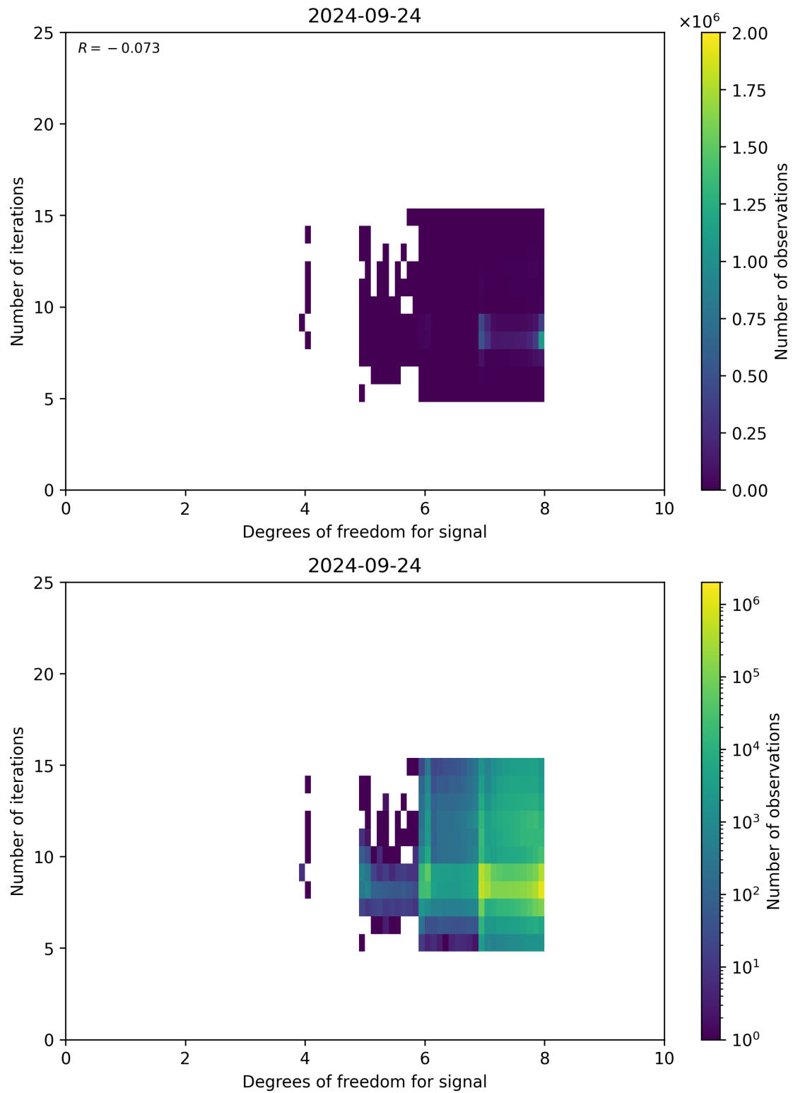
Figure 50: Scatter density plot of “Degrees of freedom for signal” against “Number of iterations” for 2024-09-23 to 2024-09-25.
