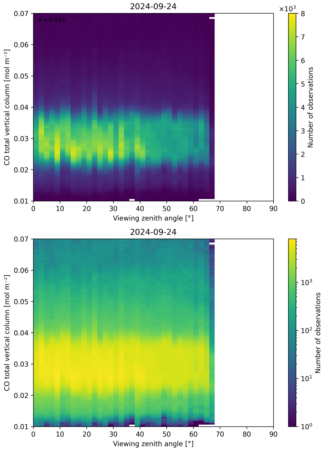
Figure 69: Scatter density plot of “Viewing zenith angle” against “CO total vertical column” for 2024-09-23 to 2024-09-25.
