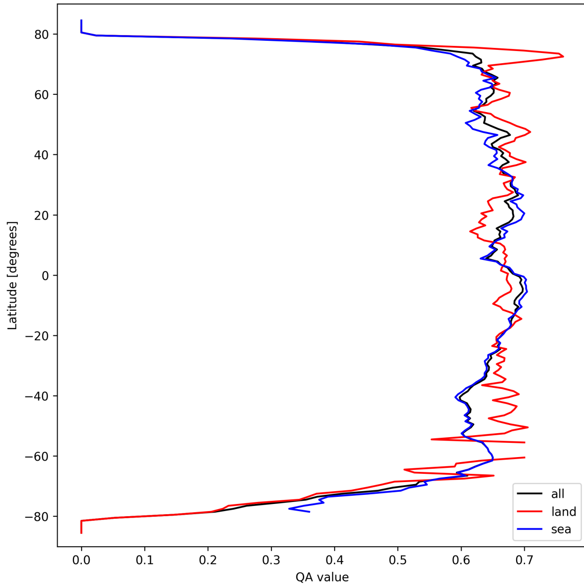
Figure 9: Zonal average of “QA value” for 2024-09-23 to 2024-09-25.
