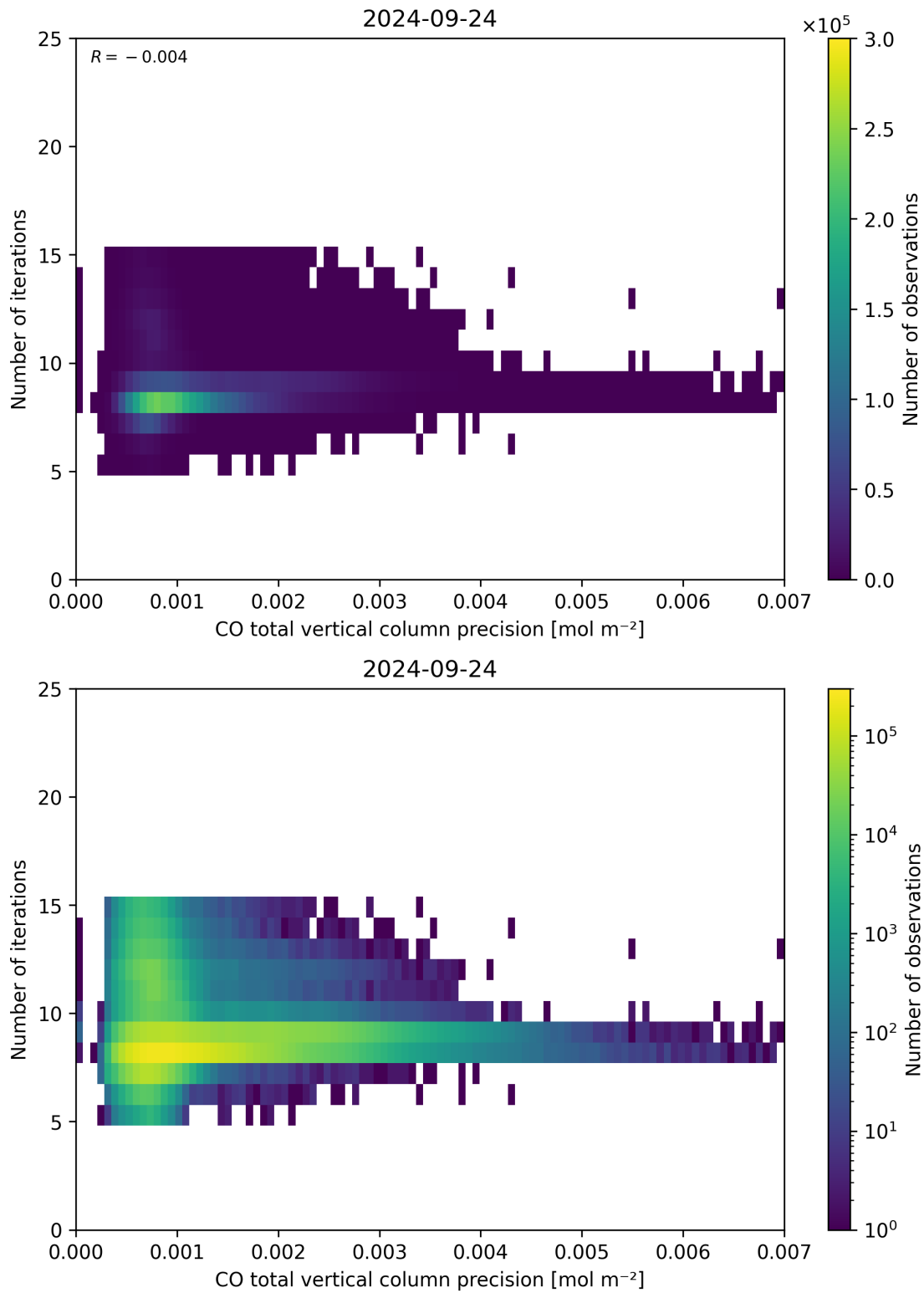
Figure 46: Scatter density plot of “CO total vertical column precision” against “Number of iterations” for 2024-09-23 to 2024-09-25.
