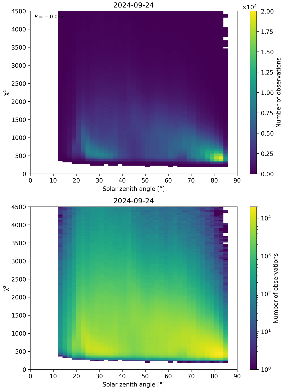
Figure 64: Scatter density plot of “Solar zenith angle” against “ \chi^2 ” for 2024-09-23 to 2024-09-25.
