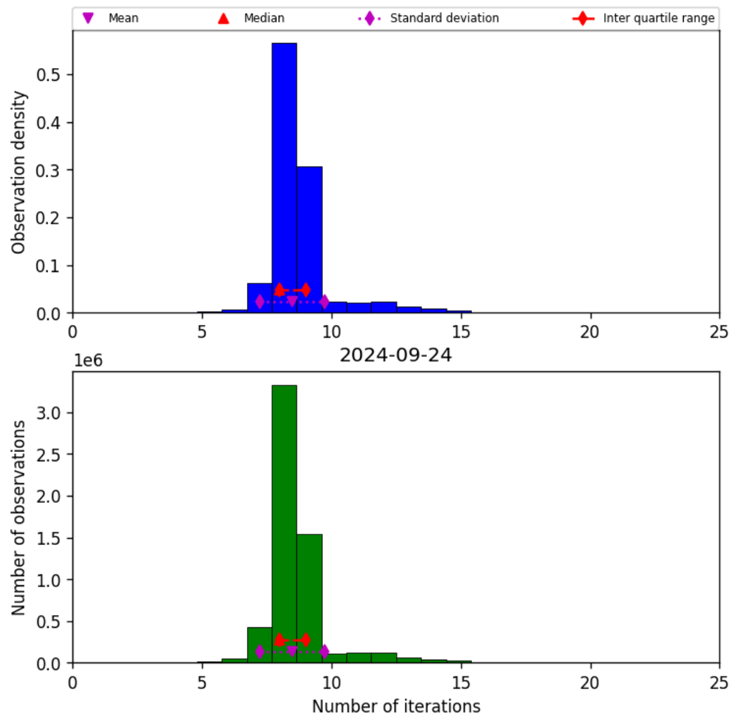
Figure 24: Histogram of “Number of iterations” for 2024-09-23 to 2024-09-25
