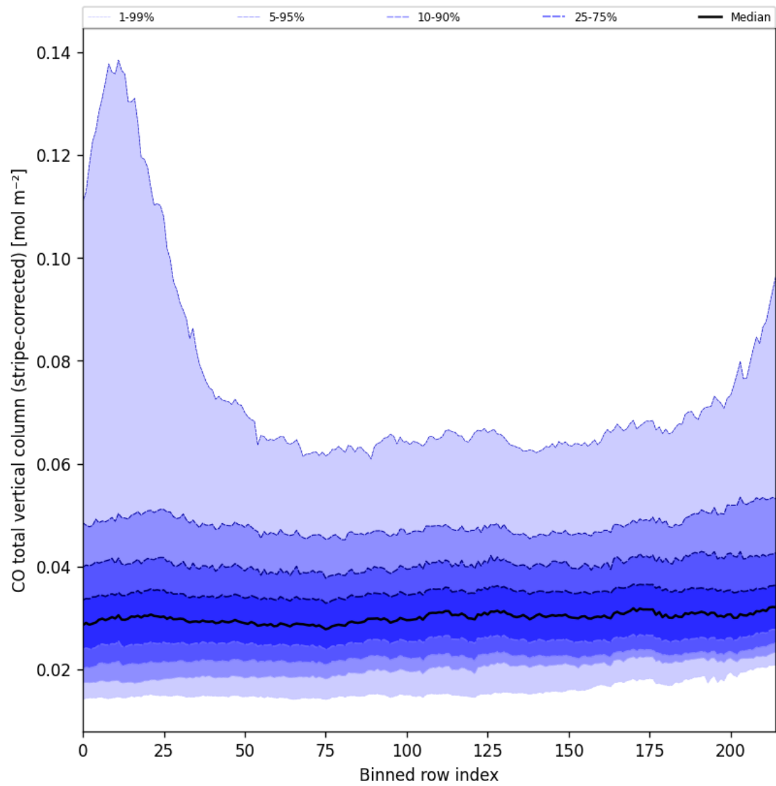
Figure 27: Along track statistics of “CO total vertical column (stripe-corrected)” for 2024-09-23 to 2024-09-25
