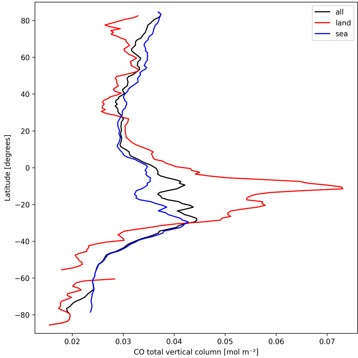
Figure 10: Zonal average of “CO total vertical column” for 2024-09-23 to 2024-09-25.
