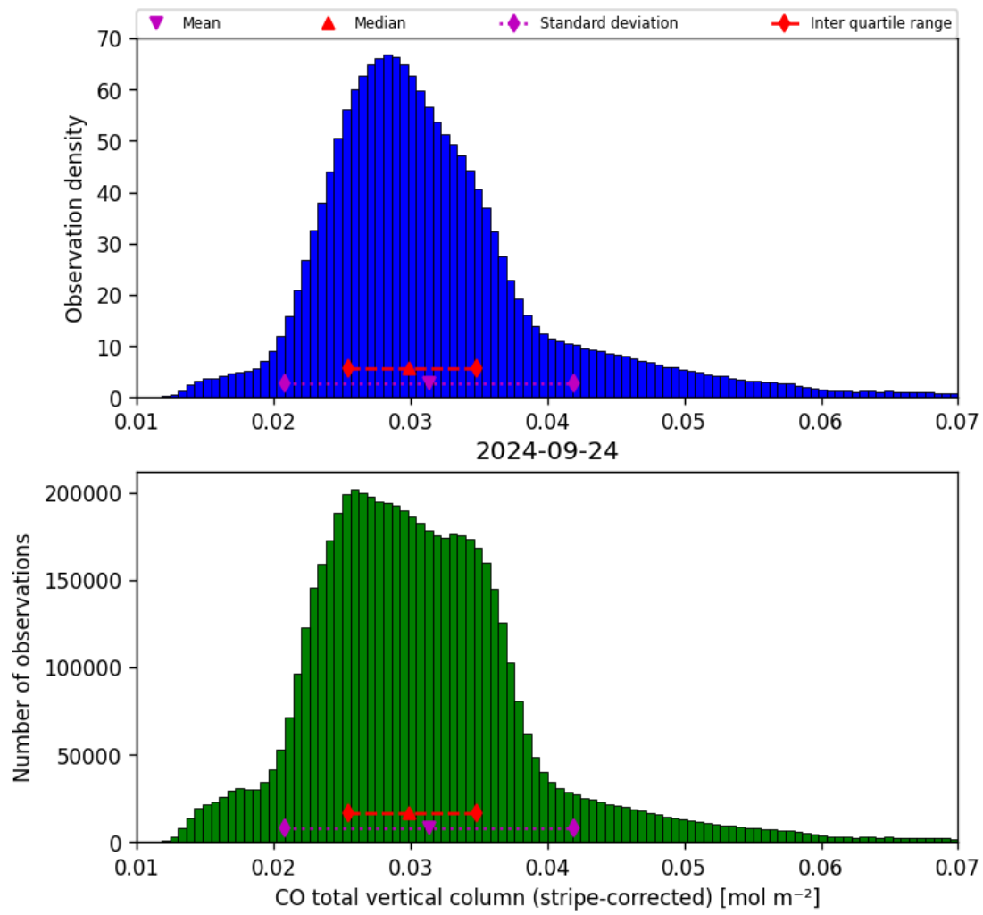
Figure 19: Histogram of “CO total vertical column (stripe-corrected)” for 2024-09-23 to 2024-09-25
