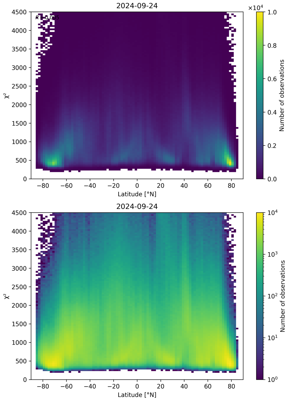
Figure 54: Scatter density plot of “Latitude” against “ \chi^2 ” for 2024-09-23 to 2024-09-25.
