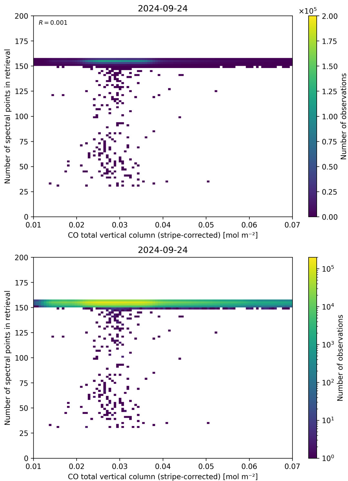
Figure 40: Scatter density plot of “CO total vertical column (stripe-corrected)” against “Number of spectral points in retrieval” for 2024-09-23 to 2024-09-25.
