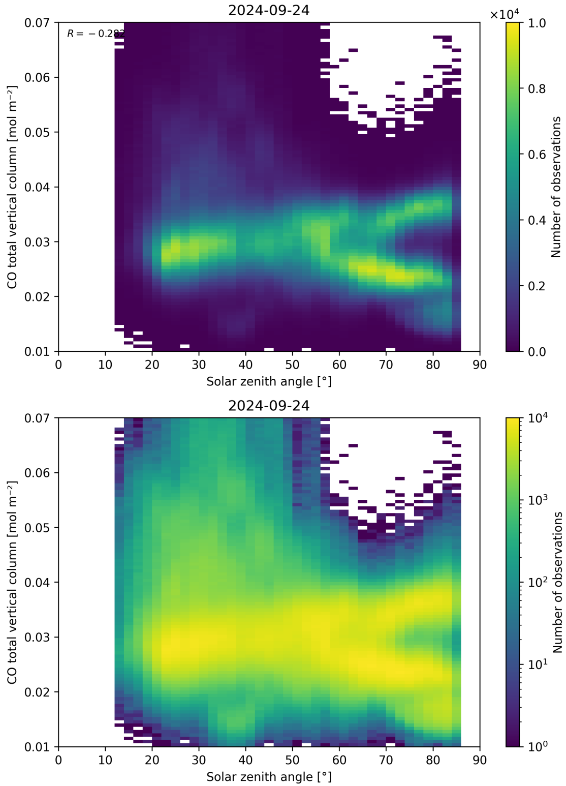
Figure 61: Scatter density plot of “Solar zenith angle” against “CO total vertical column” for 2024-09-23 to 2024-09-25.
