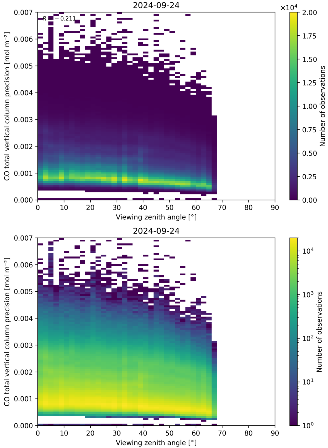
Figure 71: Scatter density plot of “Viewing zenith angle” against “CO total vertical column precision” for 2024-09-23 to 2024-09-25.
