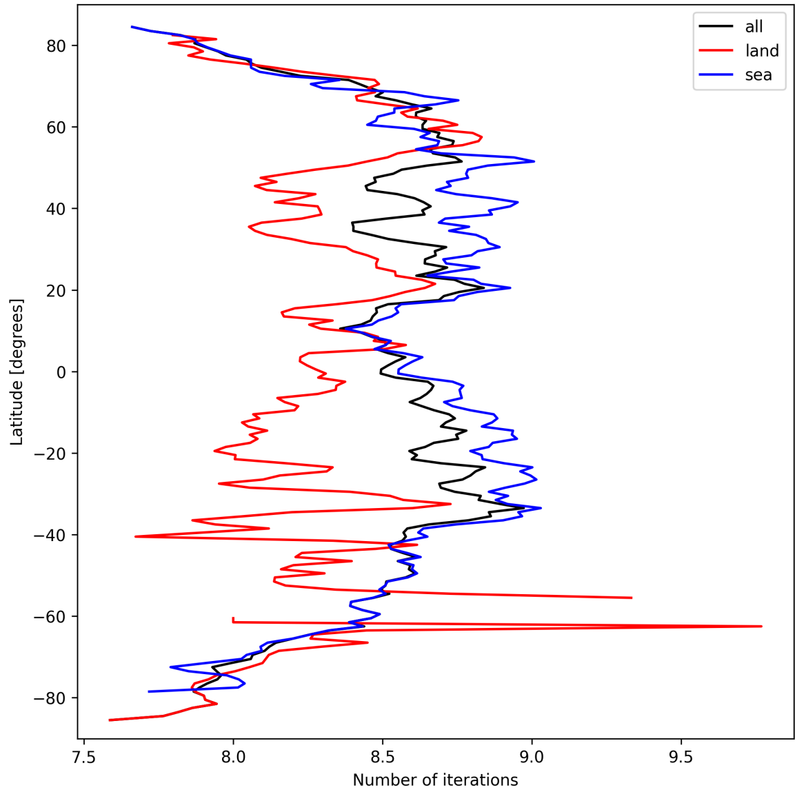
Figure 16: Zonal average of “Number of iterations” for 2024-09-23 to 2024-09-25.
