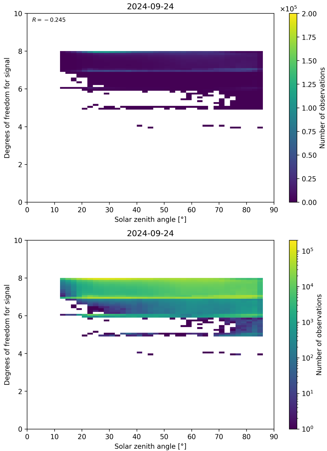
Figure 65: Scatter density plot of “Solar zenith angle” against “Degrees of freedom for signal” for 2024-09-23 to 2024-09-25.
