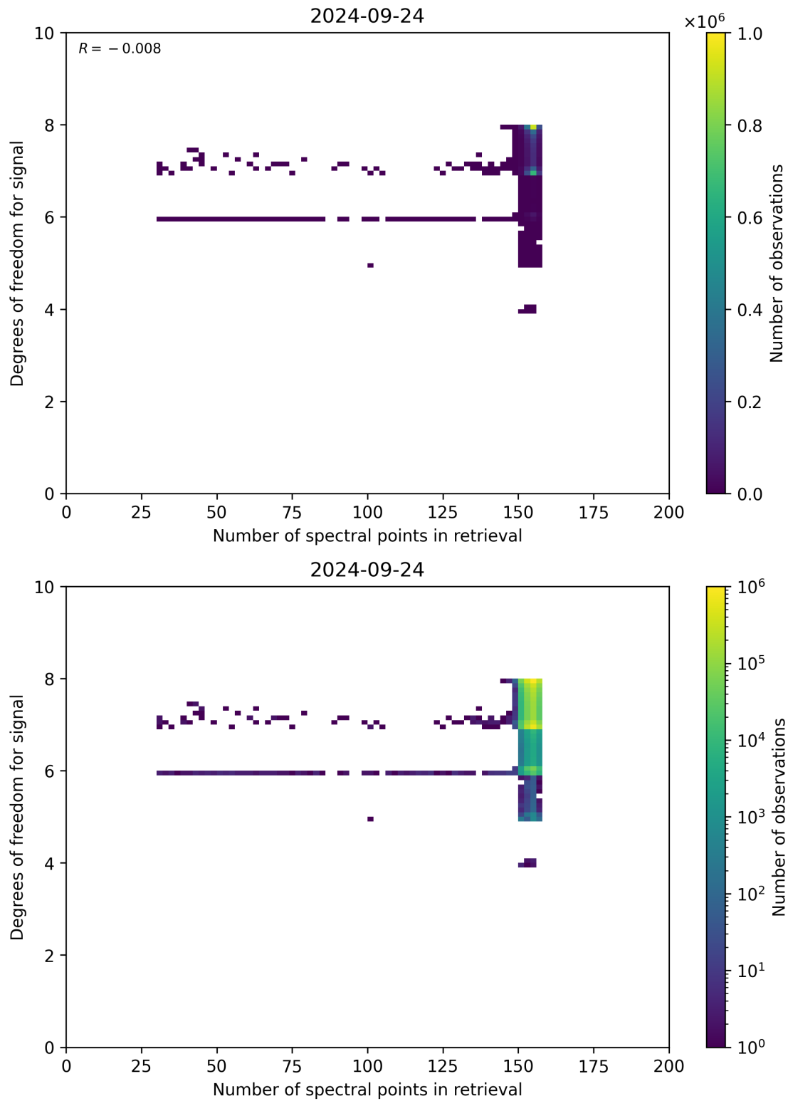
Figure 59: Scatter density plot of “Number of spectral points in retrieval” against “Degrees of freedom for signal” for 2024-09-23 to 2024-09-25.
