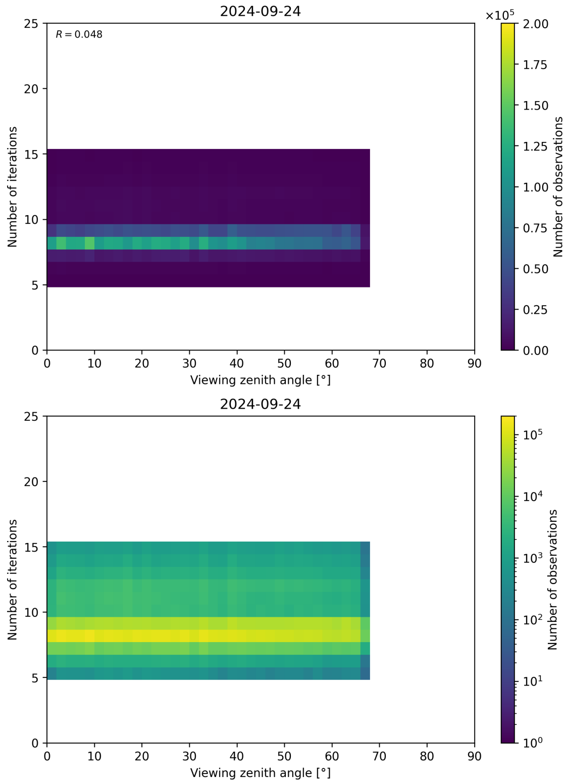
Figure 75: Scatter density plot of “Viewing zenith angle” against “Number of iterations” for 2024-09-23 to 2024-09-25.
