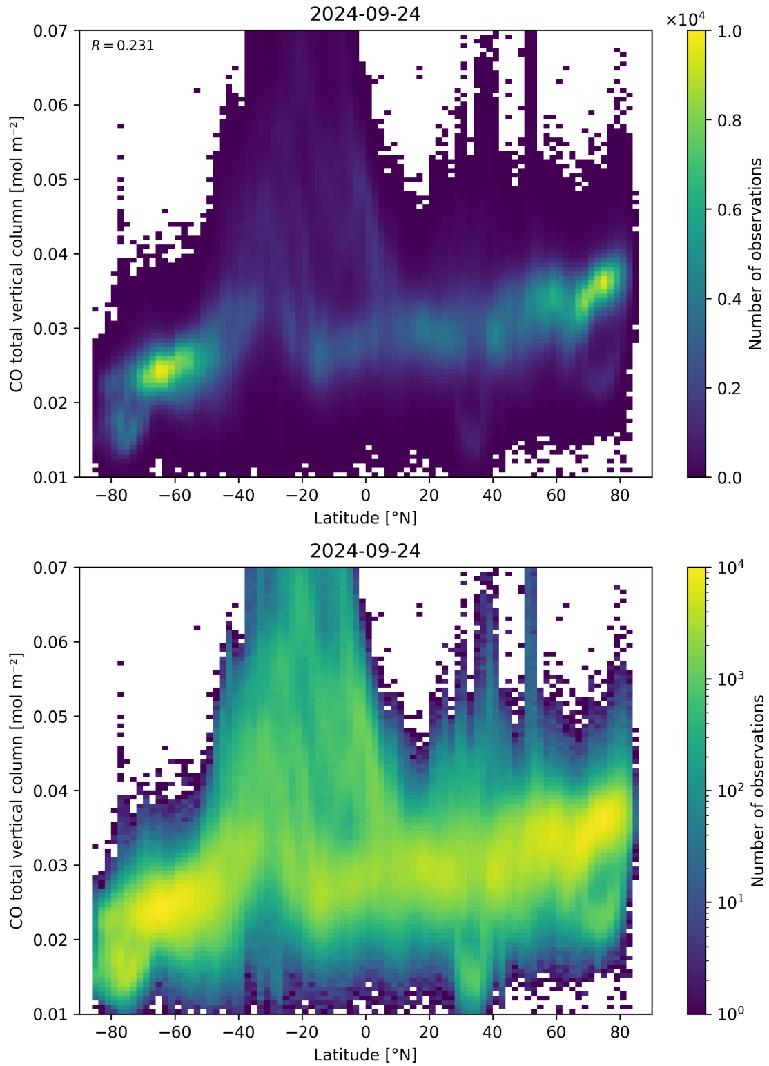
Figure 51: Scatter density plot of “Latitude” against “CO total vertical column” for 2024-09-23 to 2024-09-25.
