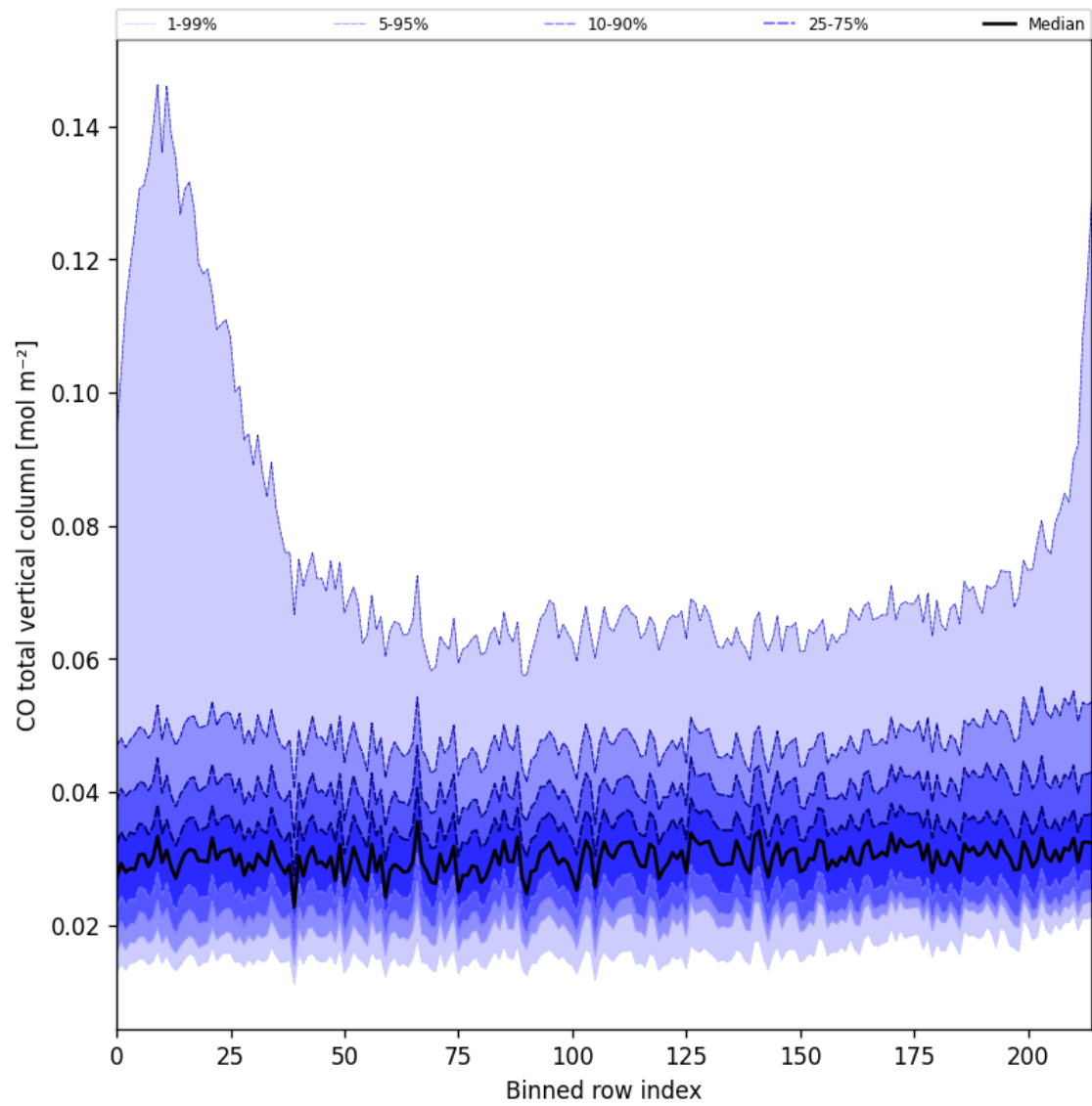
Figure 26: Along track statistics of “CO total vertical column” for 2024-09-23 to 2024-09-25
