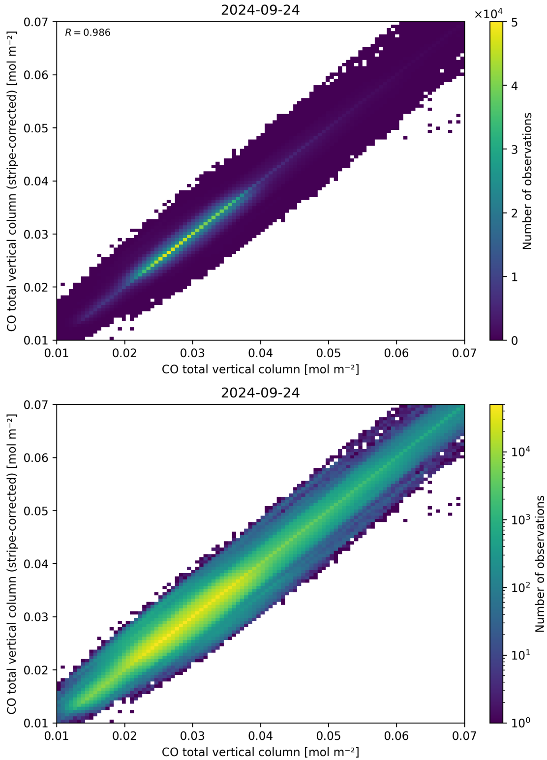
Figure 33: Scatter density plot of “CO total vertical column” against “CO total vertical column (stripe-corrected)” for 2024-09-23 to 2024-09-25.
