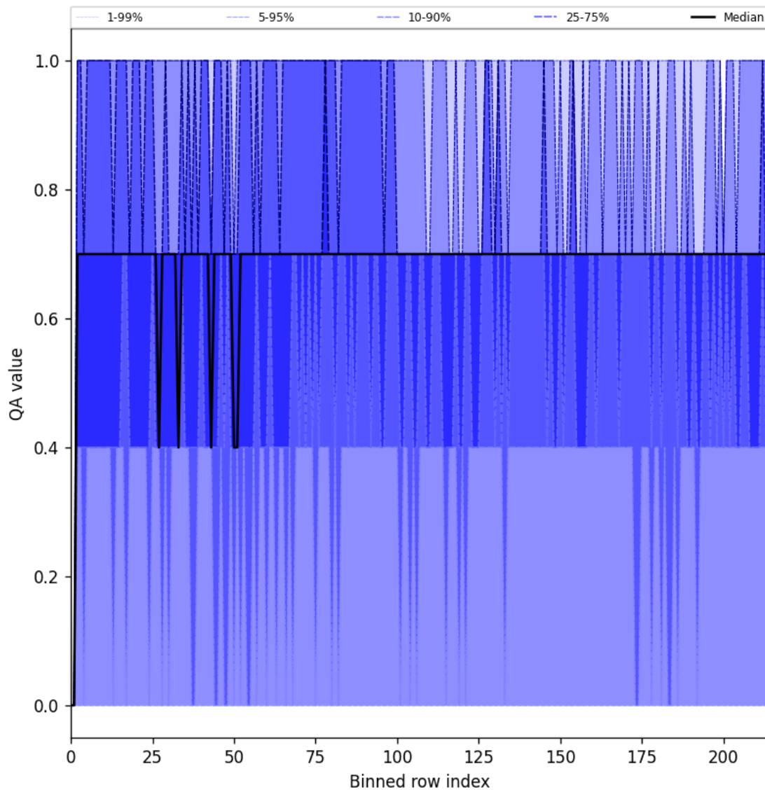
Figure 25: Along track statistics of “QA value” for 2024-09-23 to 2024-09-25
