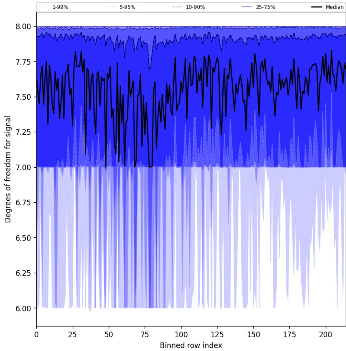
Figure 31: Along track statistics of “Degrees of freedom for signal” for 2024-09-23 to 2024-09-25
