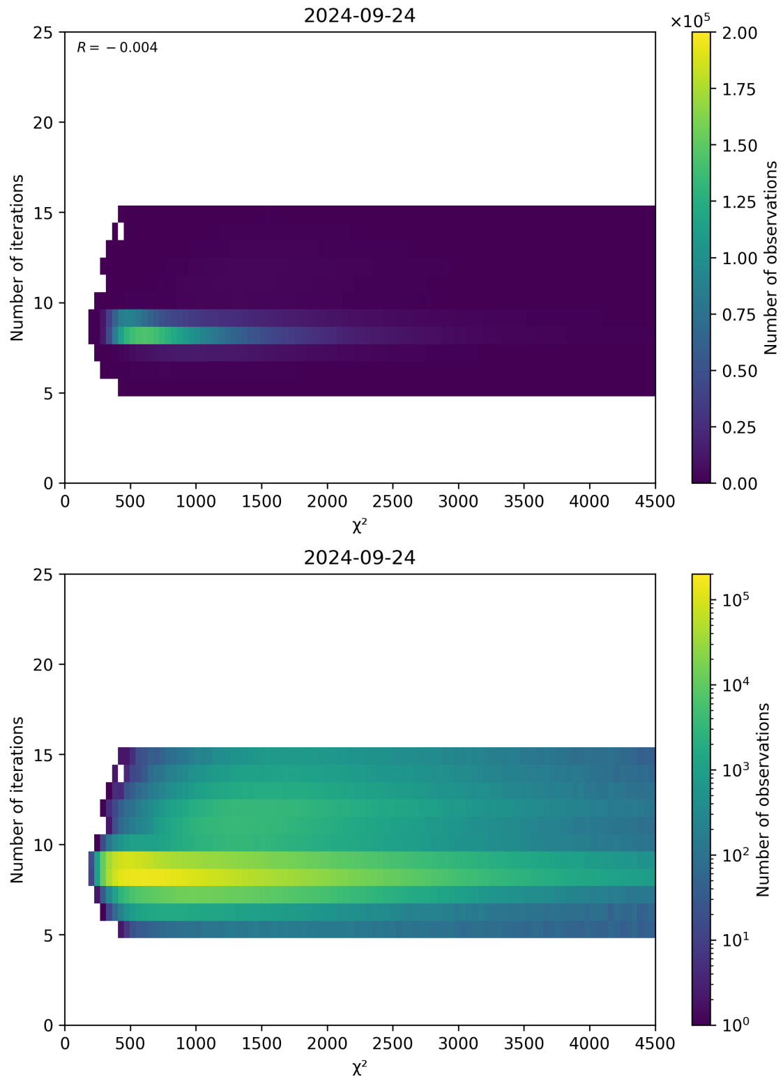
Figure 49: Scatter density plot of “ \chi^2 ” against “Number of iterations” for 2024-09-23 to 2024-09-25.
