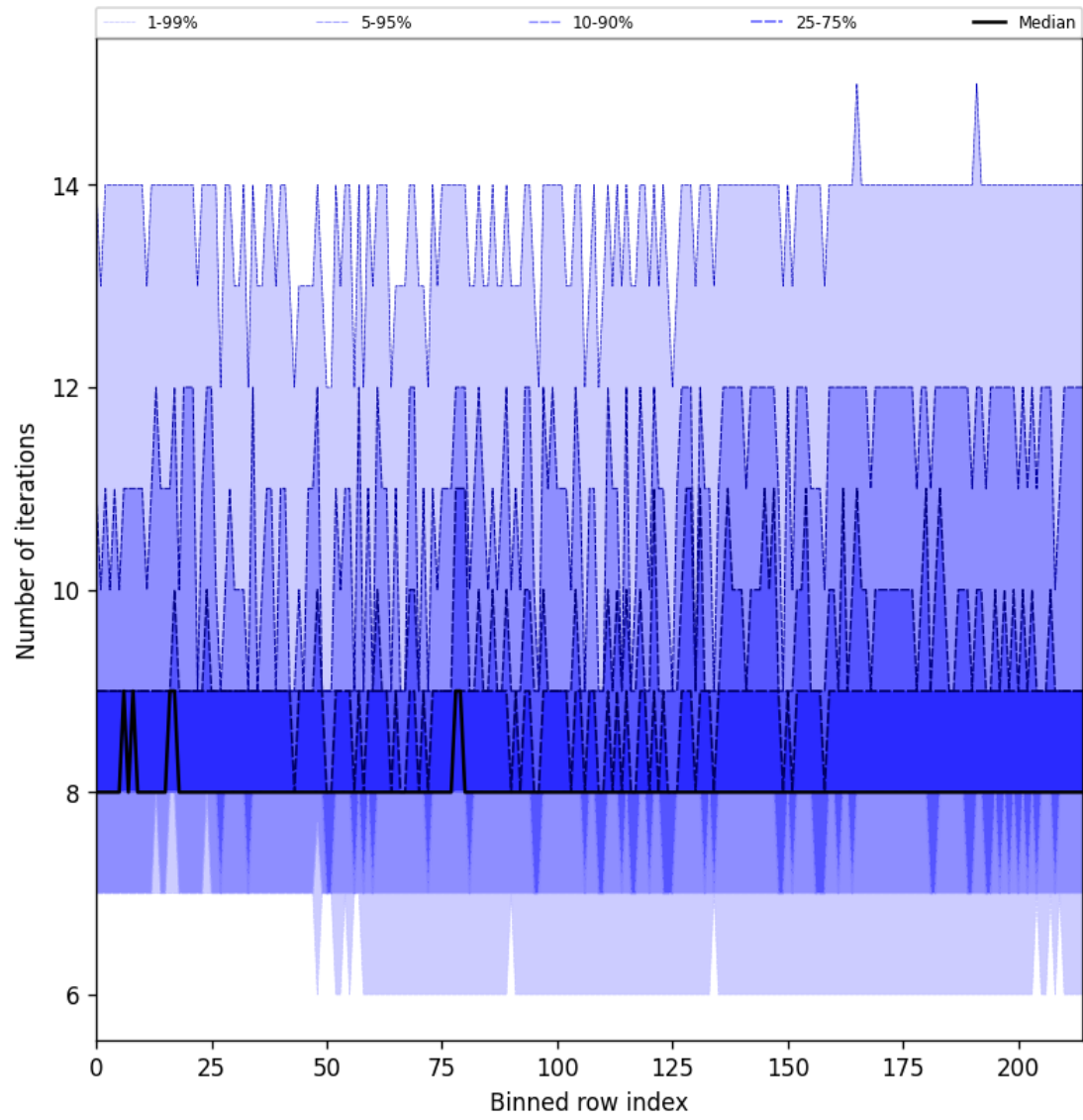
Figure 32: Along track statistics of “Number of iterations” for 2024-09-23 to 2024-09-25
