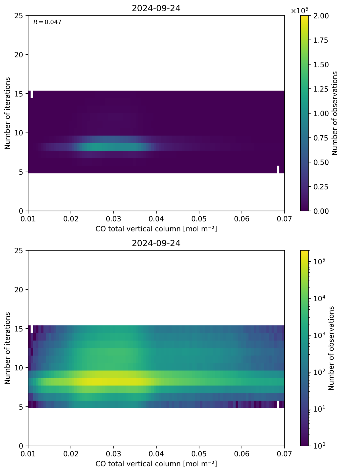
Figure 42: Scatter density plot of “CO total vertical column” against “Number of iterations” for 2024-09-23 to 2024-09-25.
