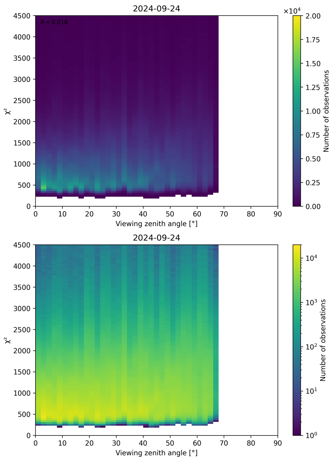
Figure 72: Scatter density plot of “Viewing zenith angle” against “ \chi^2 ” for 2024-09-23 to 2024-09-25.
