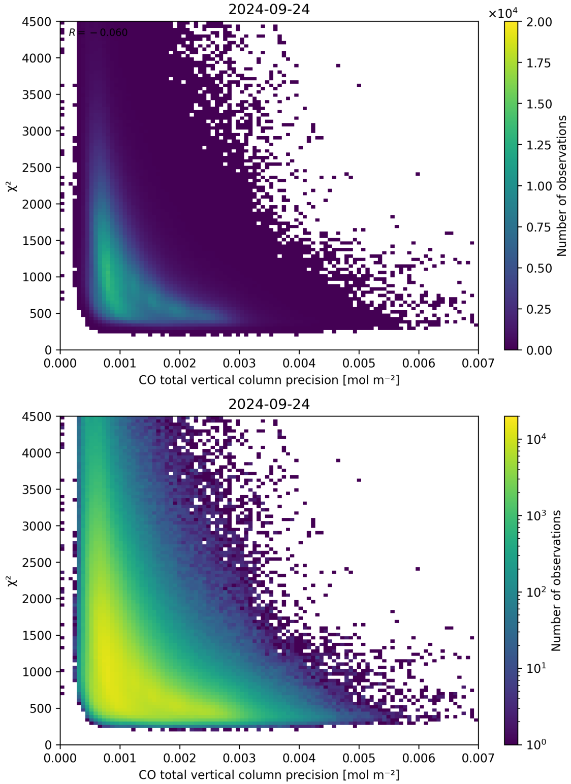
Figure 44: Scatter density plot of “CO total vertical column precision” against “ \chi^2 ” for 2024-09-23 to 2024-09-25.
