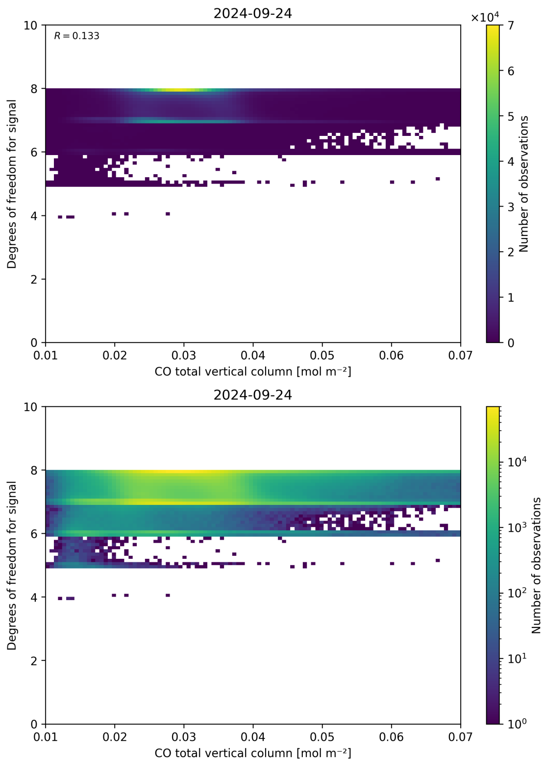
Figure 41: Scatter density plot of “CO total vertical column” against “Degrees of freedom for signal” for 2024-09-23 to 2024-09-25.
