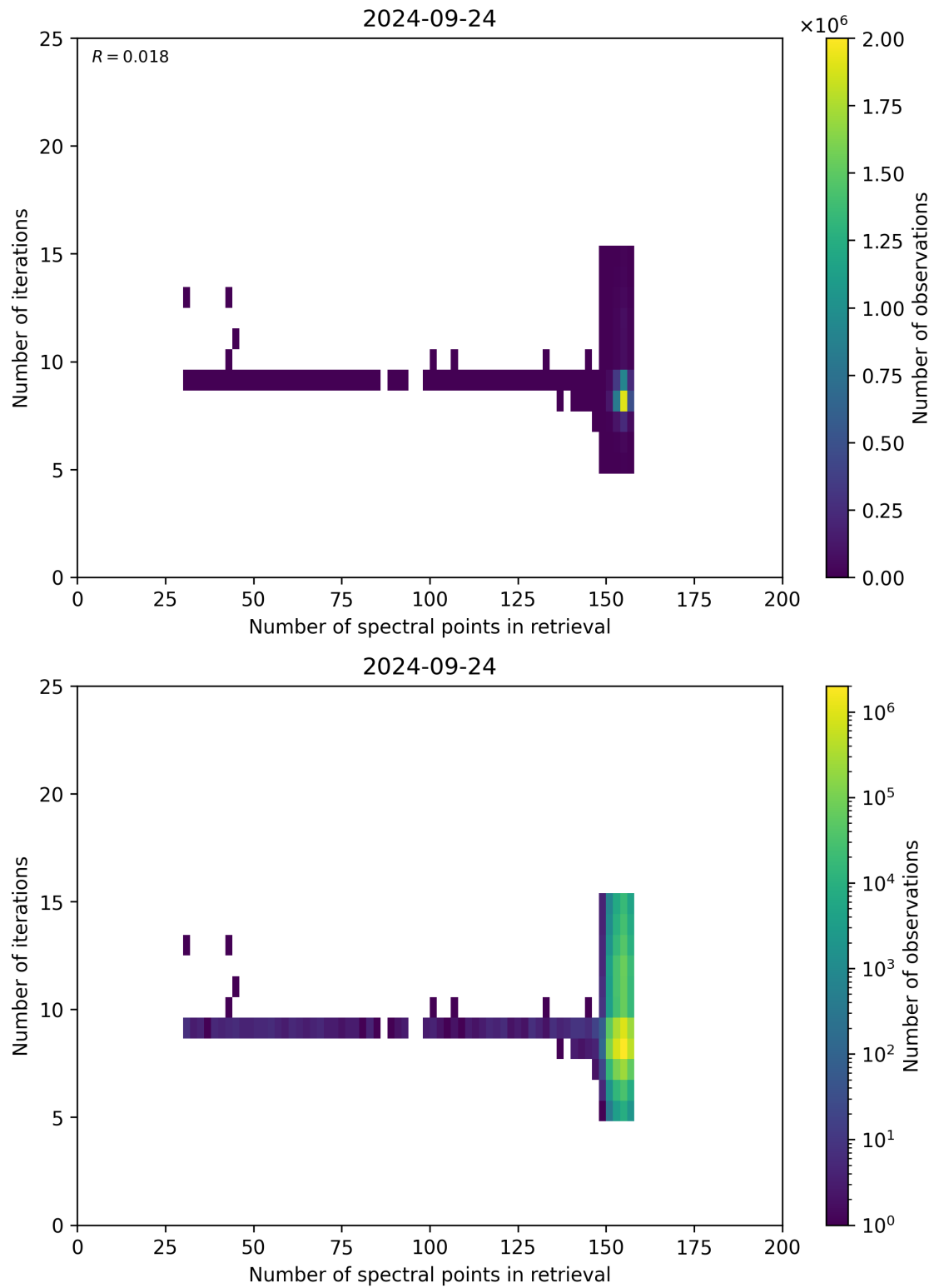
Figure 60: Scatter density plot of “Number of spectral points in retrieval” against “Number of iterations” for 2024-09-23 to 2024-09-25.
