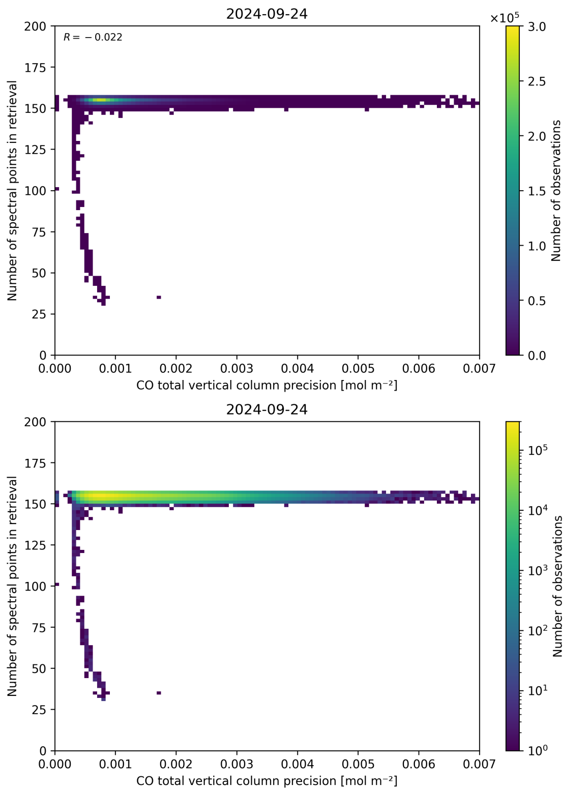
Figure 47: Scatter density plot of “CO total vertical column precision” against “Number of spectral points in retrieval” for 2024-09-23 to 2024-09-25.
