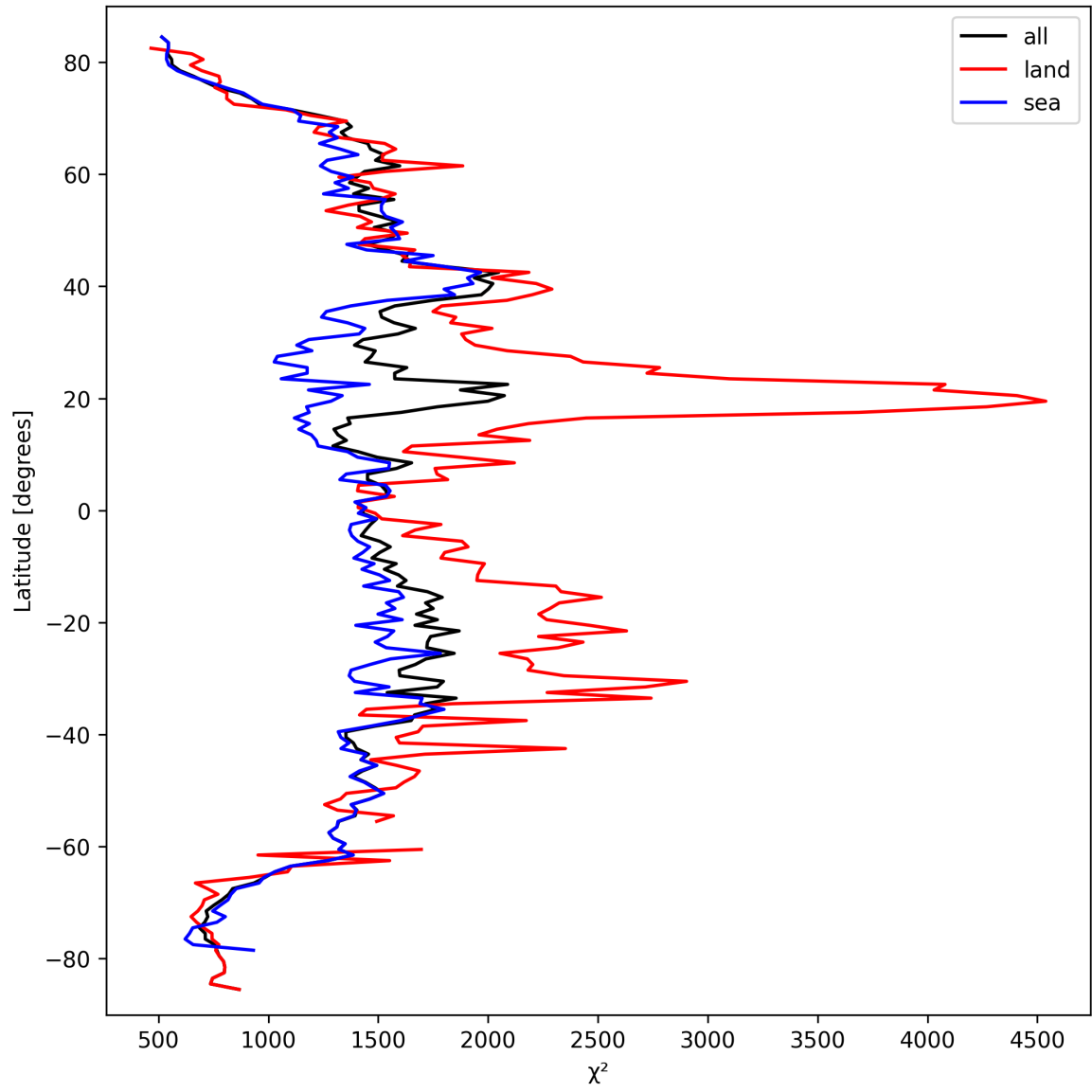
Figure 14: Zonal average of “ \chi^2 ” for 2024-09-23 to 2024-09-25.
