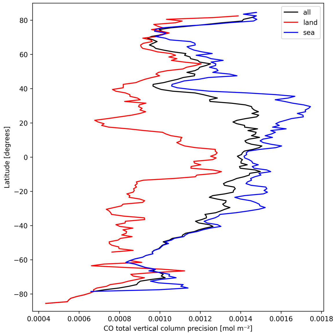
Figure 12: Zonal average of “CO total vertical column precision” for 2024-09-23 to 2024-09-25.
