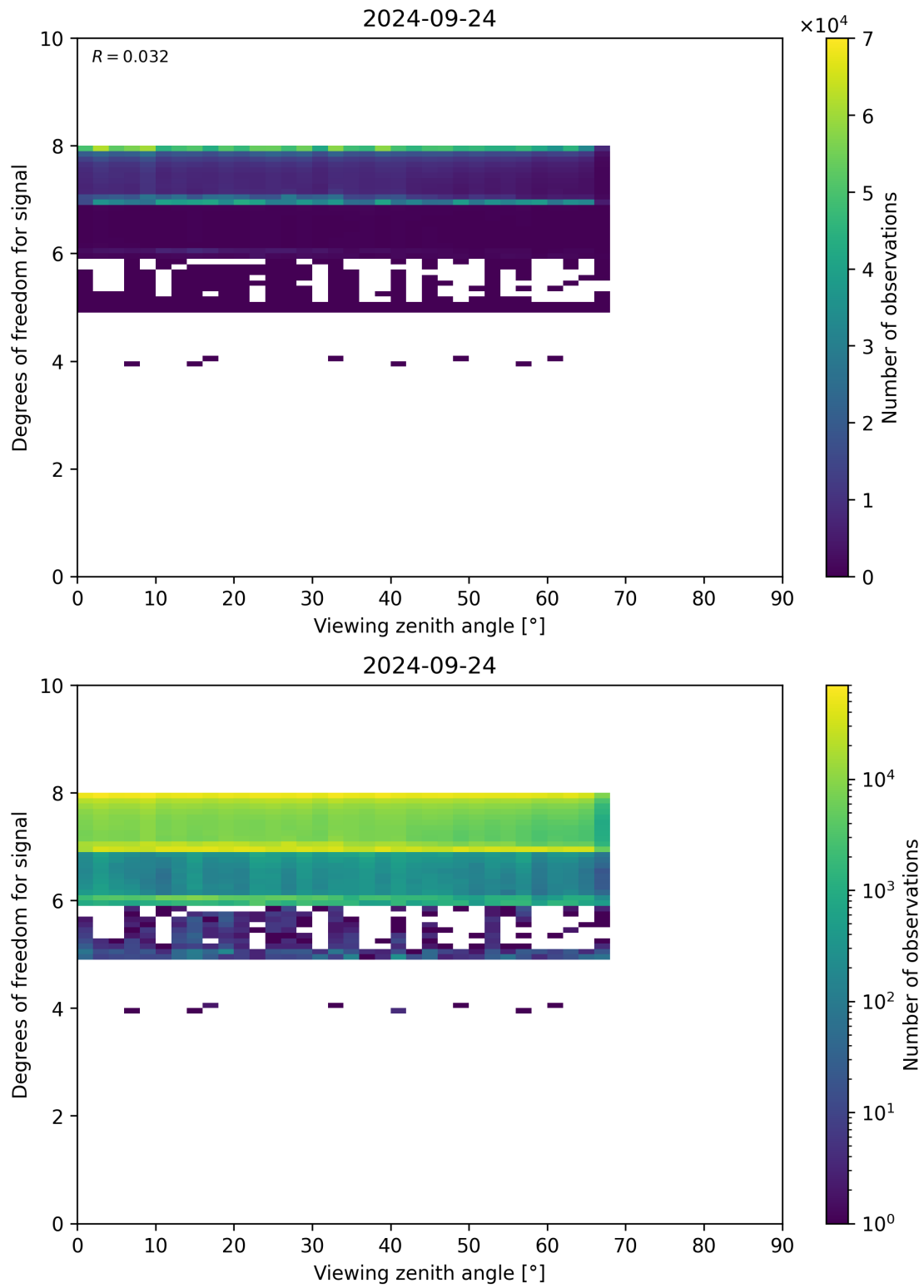
Figure 73: Scatter density plot of “Viewing zenith angle” against “Degrees of freedom for signal” for 2024-09-23 to 2024-09-25.
