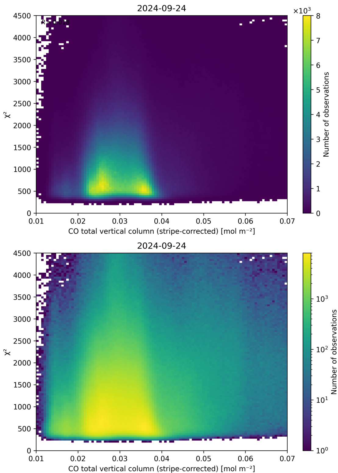
Figure 37: Scatter density plot of “CO total vertical column (stripe-corrected)” against “ \chi^2 ” for 2024-09-23 to 2024-09-25.
