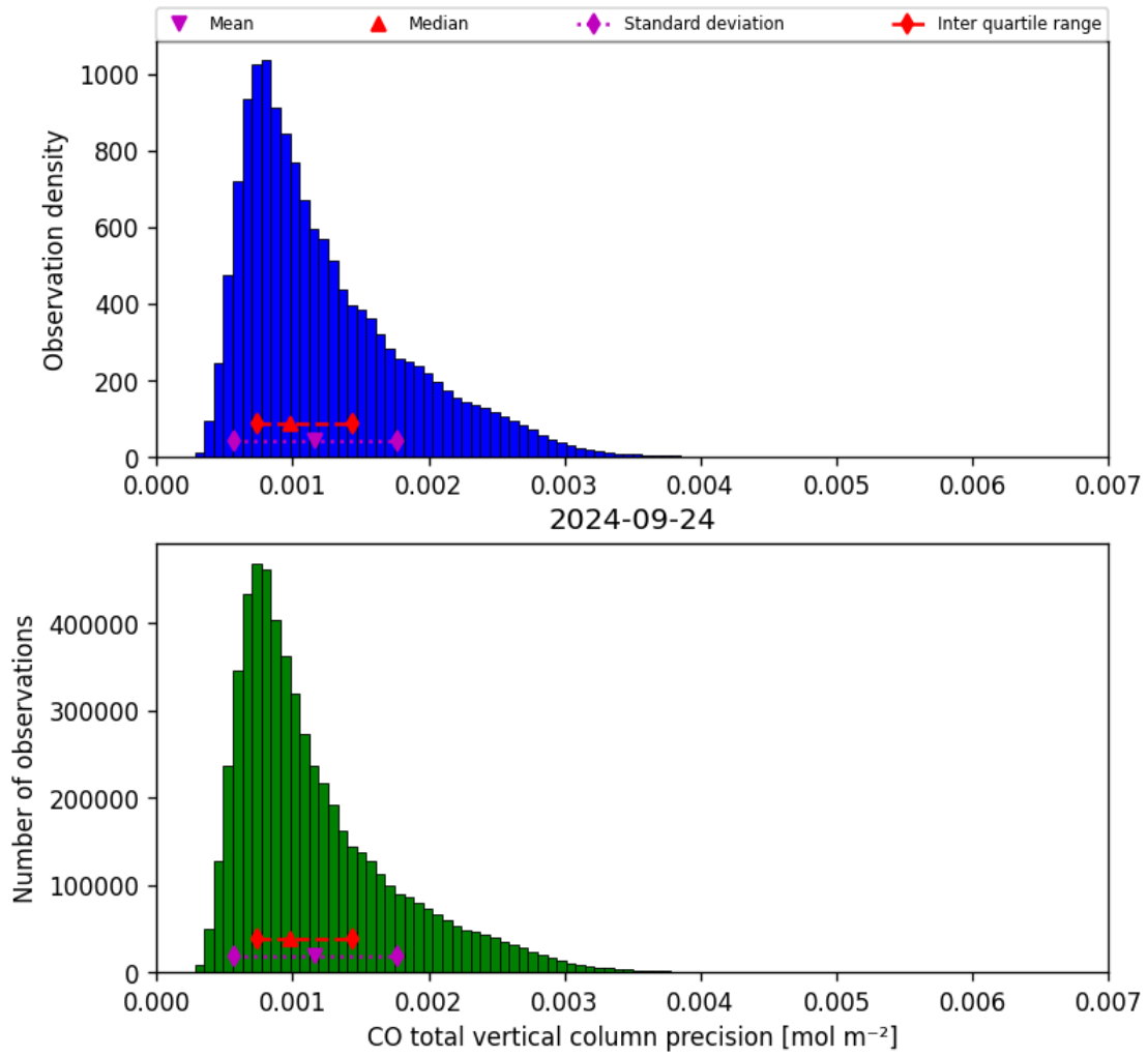
Figure 20: Histogram of “CO total vertical column precision” for 2024-09-23 to 2024-09-25
