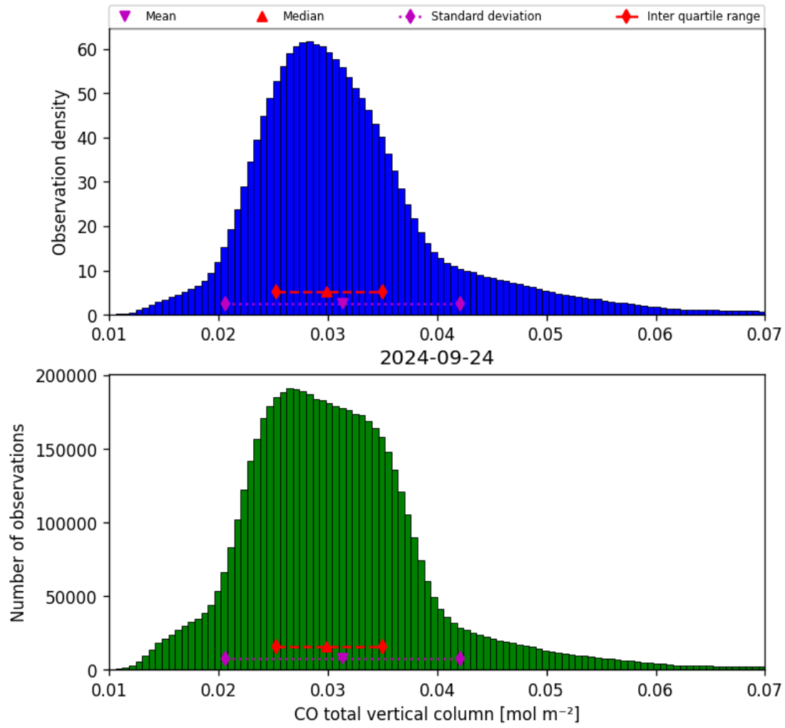
Figure 18: Histogram of “CO total vertical column” for 2024-09-23 to 2024-09-25
