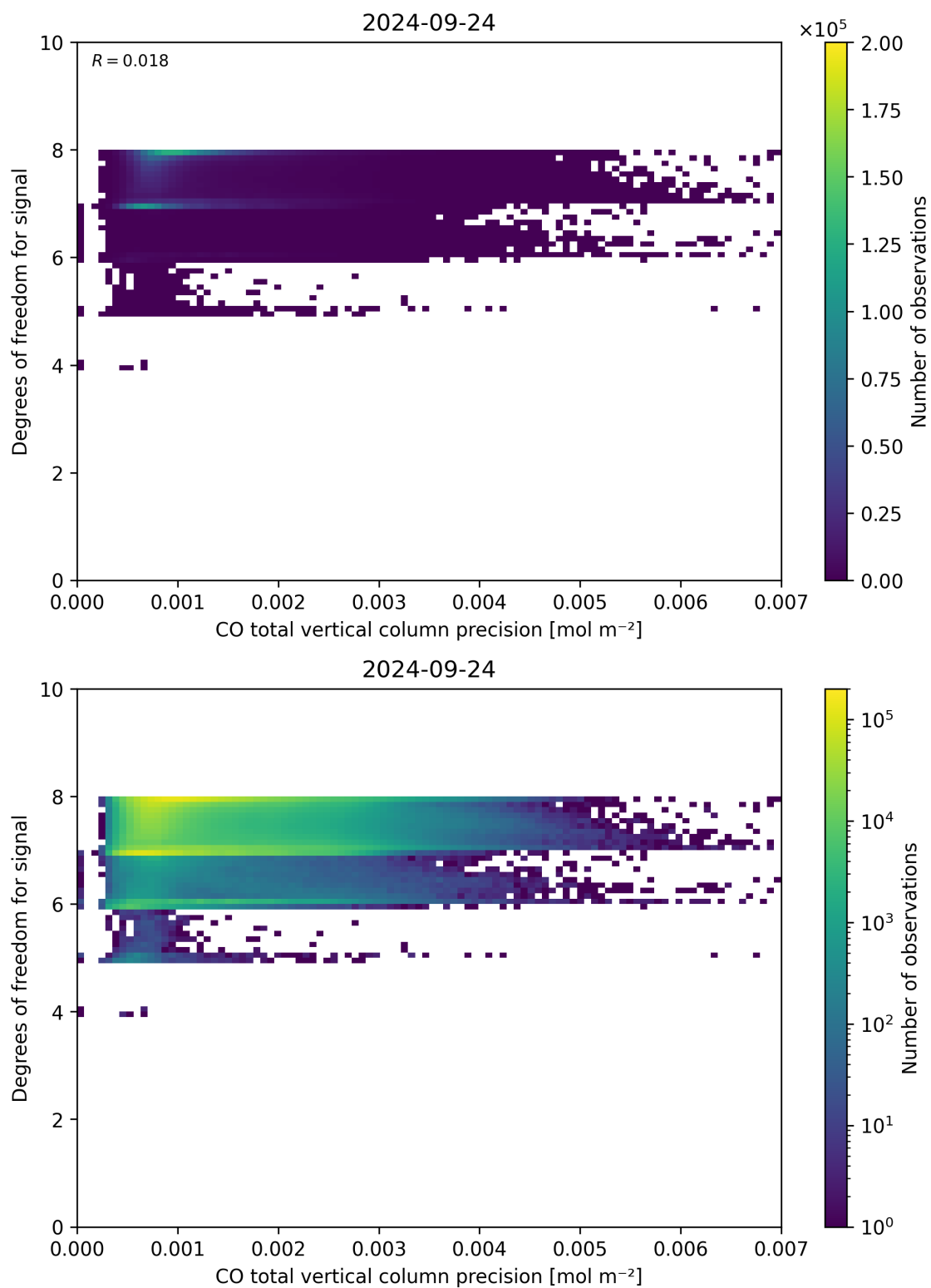
Figure 45: Scatter density plot of “CO total vertical column precision” against “Degrees of freedom for signal” for 2024-09-23 to 2024-09-25.
