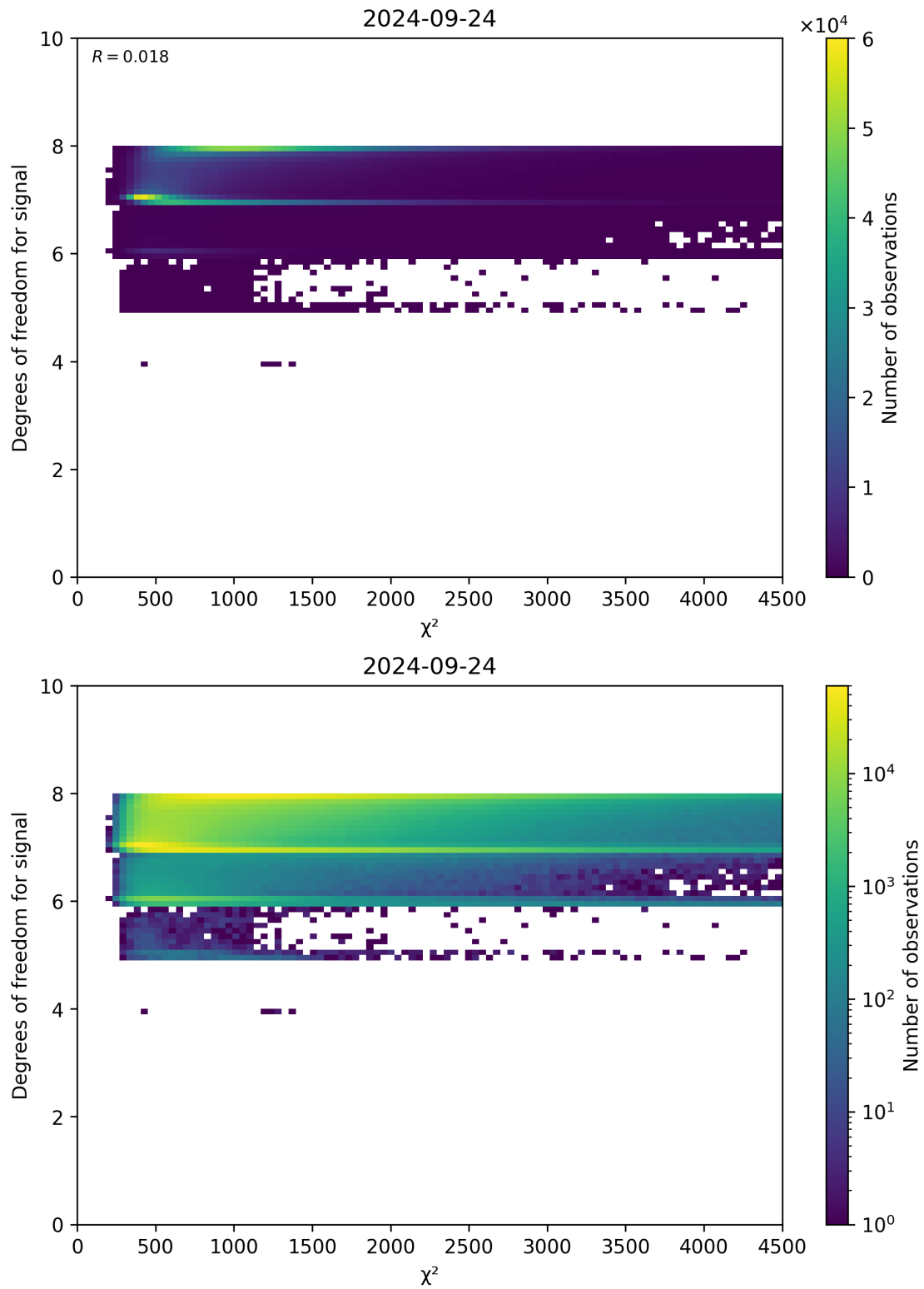
Figure 48: Scatter density plot of “ \chi^2 ” against “Degrees of freedom for signal” for 2024-09-23 to 2024-09-25.
