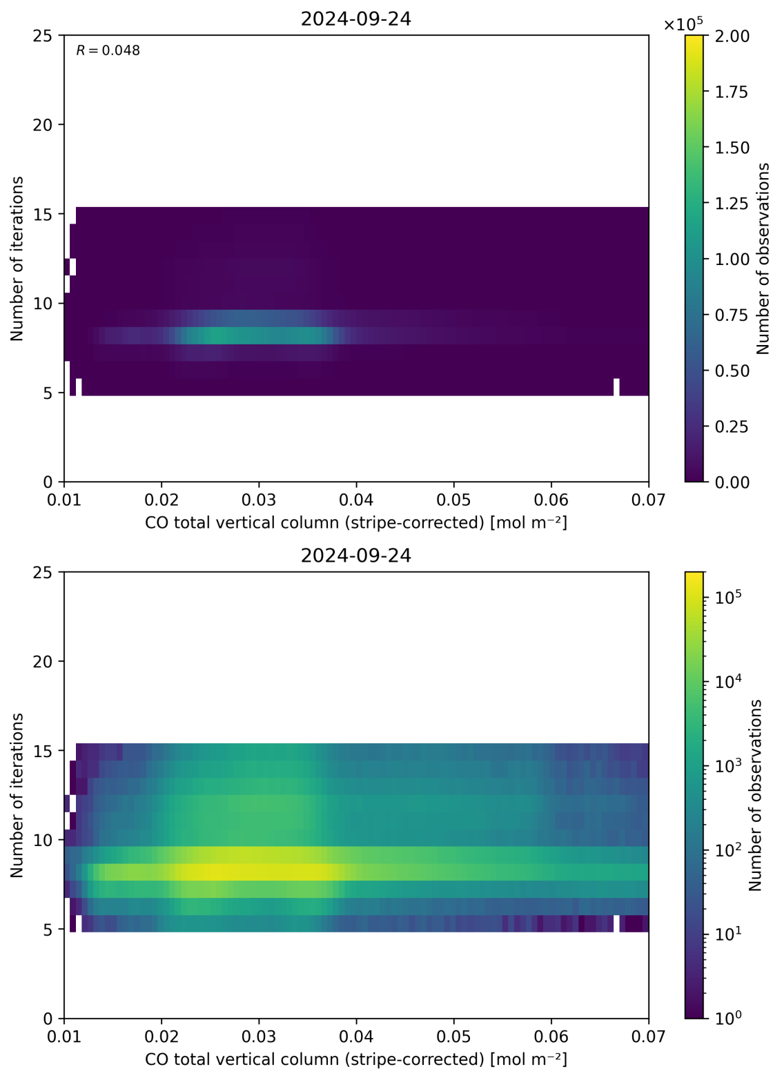
Figure 39: Scatter density plot of “CO total vertical column (stripe-corrected)” against “Number of iterations” for 2024-09-23 to 2024-09-25.
