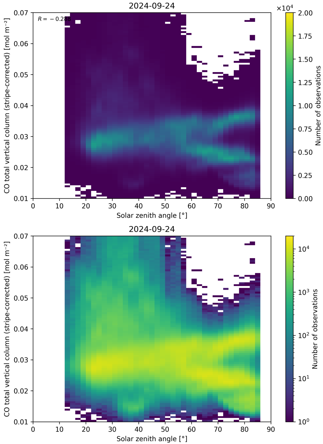
Figure 62: Scatter density plot of “Solar zenith angle” against “CO total vertical column (stripe-corrected)” for 2024-09-23 to 2024-09-25.
