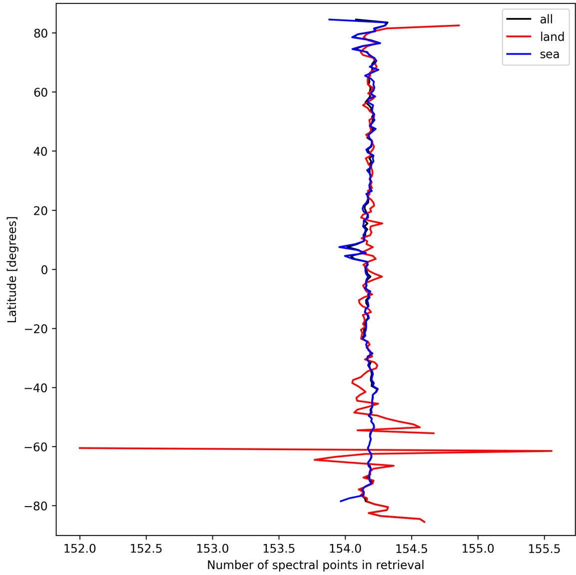
Figure 13: Zonal average of “Number of spectral points in retrieval” for 2024-09-23 to 2024-09-25.
