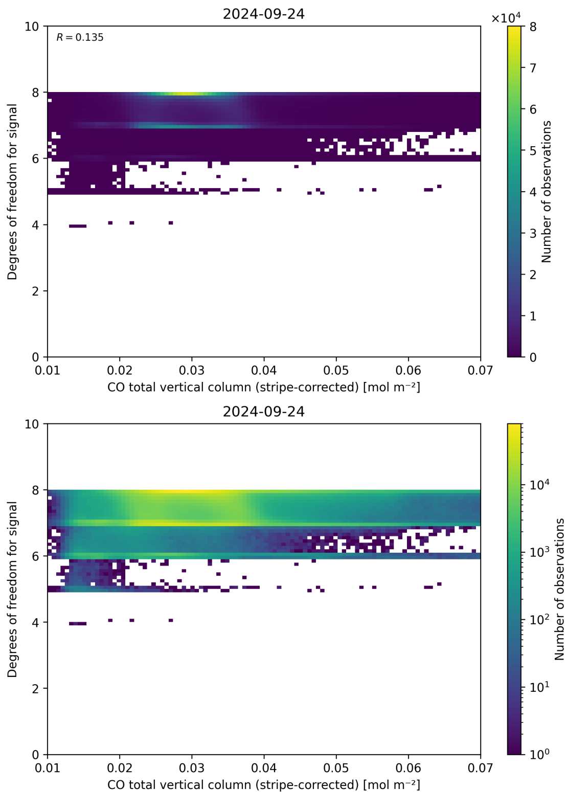
Figure 38: Scatter density plot of “CO total vertical column (stripe-corrected)” against “Degrees of freedom for signal” for 2024-09-23 to 2024-09-25.
