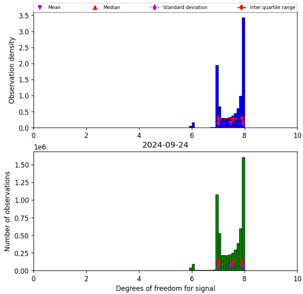
Figure 23: Histogram of “Degrees of freedom for signal” for 2024-09-23 to 2024-09-25
