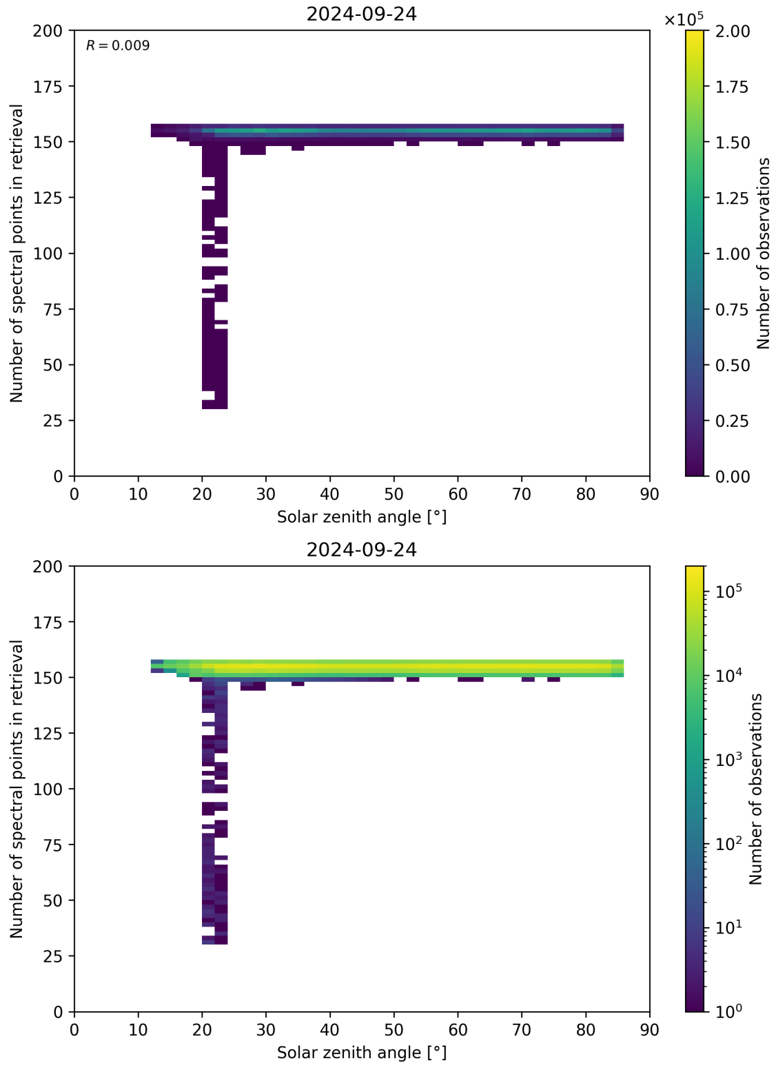
Figure 68: Scatter density plot of “Solar zenith angle” against “Number of spectral points in retrieval” for 2024-09-23 to 2024-09-25.
