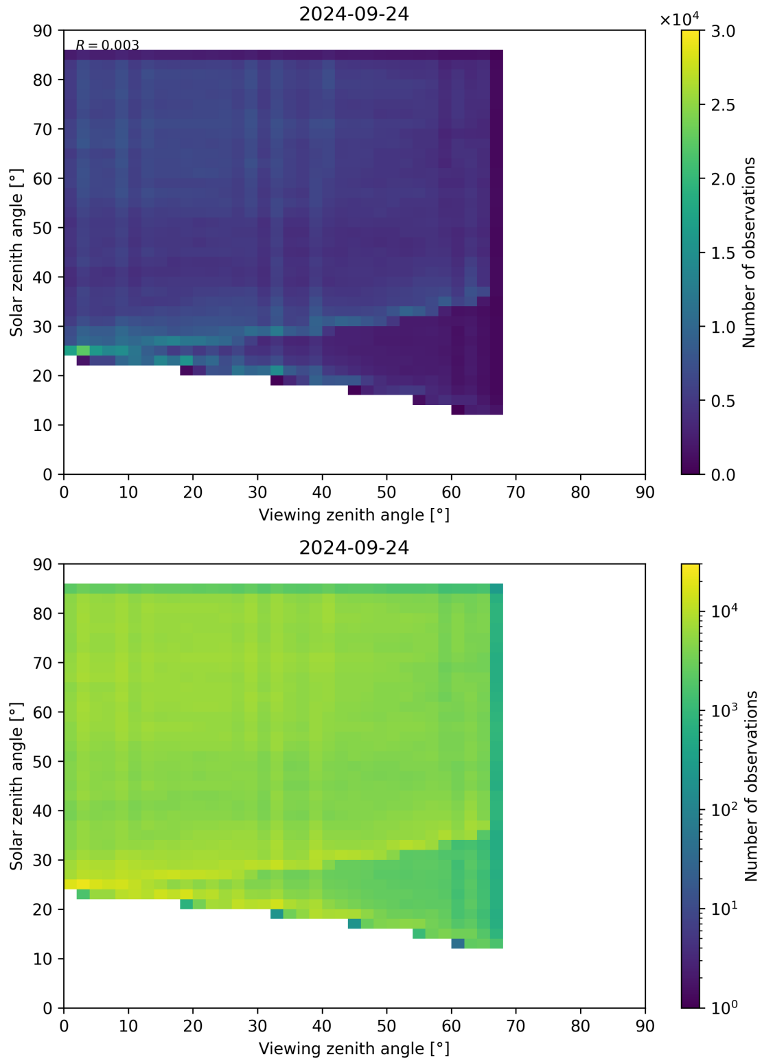
Figure 77: Scatter density plot of “Viewing zenith angle” against “Solar zenith angle” for 2024-09-23 to 2024-09-25.
