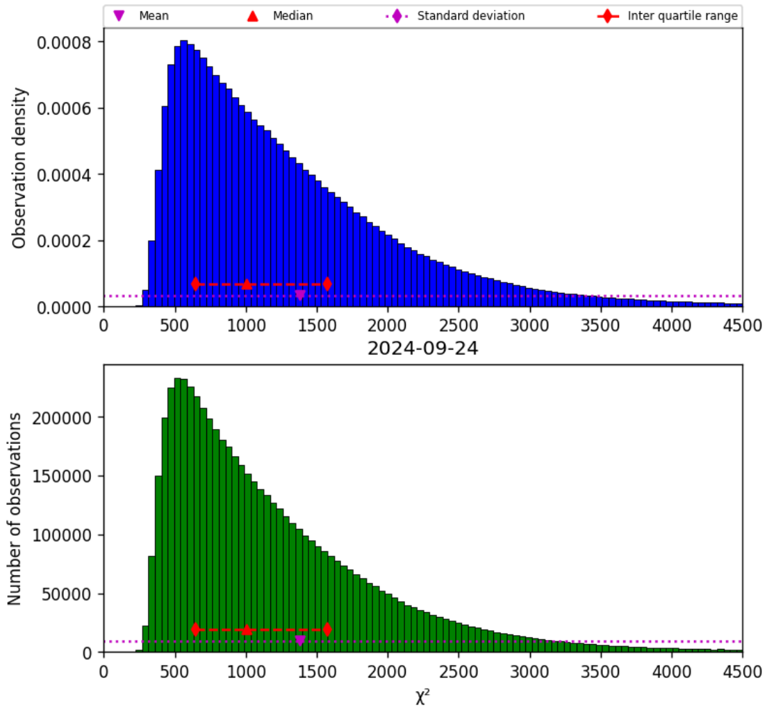
Figure 22: Histogram of “ \chi^2 ” for 2024-09-23 to 2024-09-25
