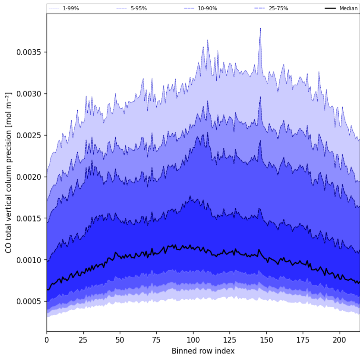
Figure 28: Along track statistics of “CO total vertical column precision” for 2024-09-23 to 2024-09-25
