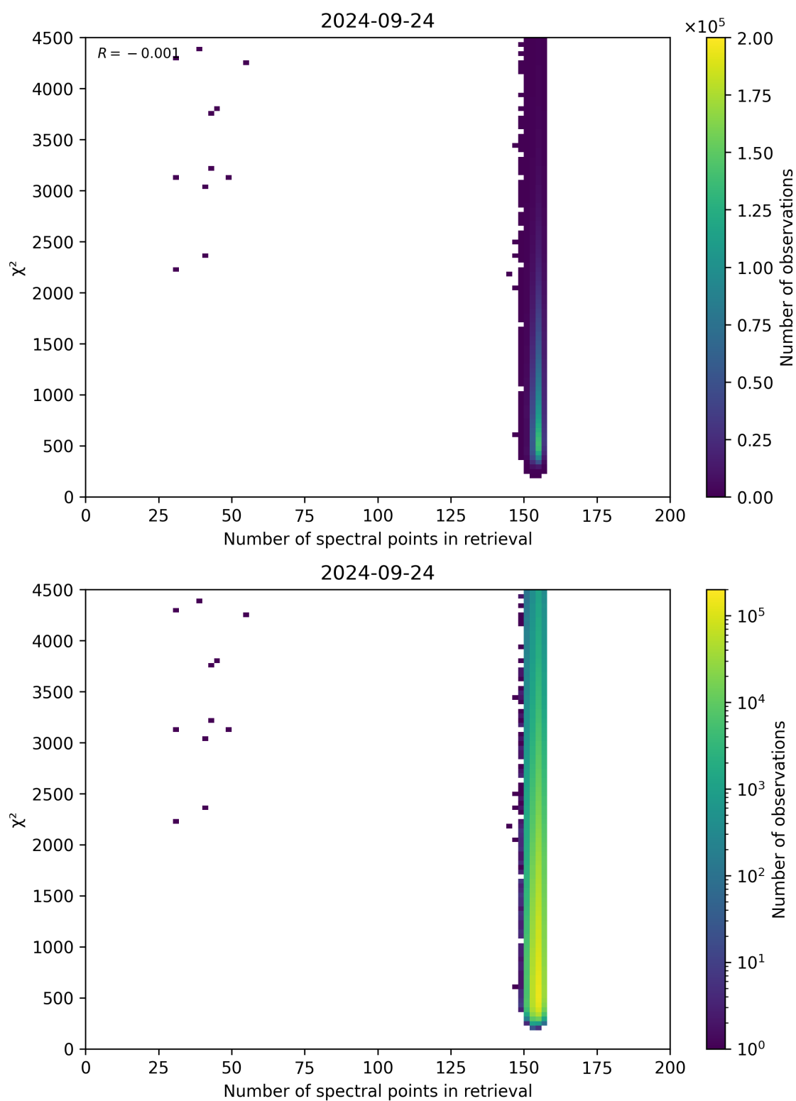
Figure 58: Scatter density plot of “Number of spectral points in retrieval” against “ \chi^2 ” for 2024-09-23 to 2024-09-25.
