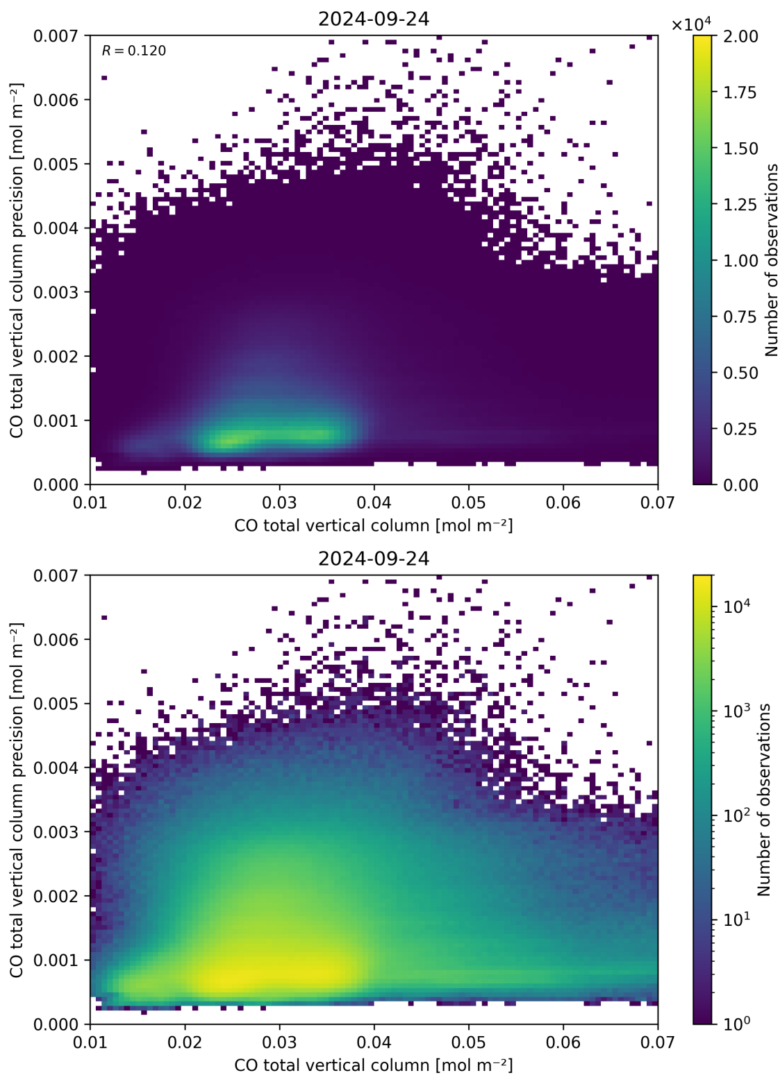
Figure 34: Scatter density plot of “CO total vertical column” against “CO total vertical column precision” for 2024-09-23 to 2024-09-25.
