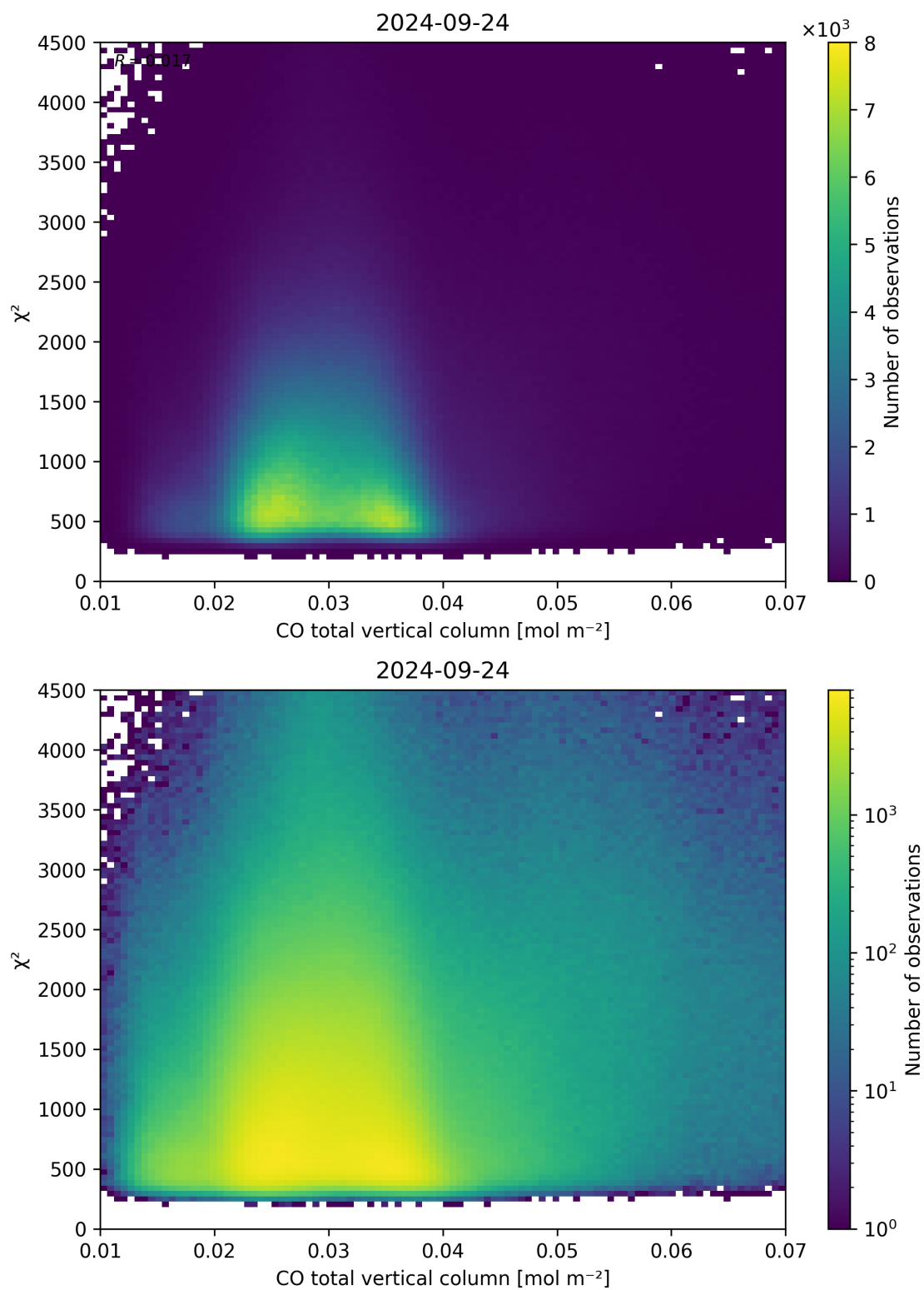
Figure 35: Scatter density plot of “CO total vertical column” against “ \chi^2 ” for 2024-09-23 to 2024-09-25.
