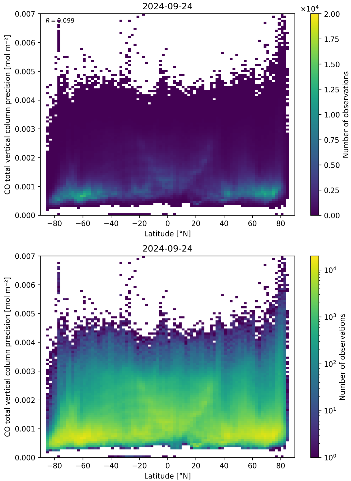
Figure 53: Scatter density plot of “Latitude” against “CO total vertical column precision” for 2024-09-23 to 2024-09-25.
