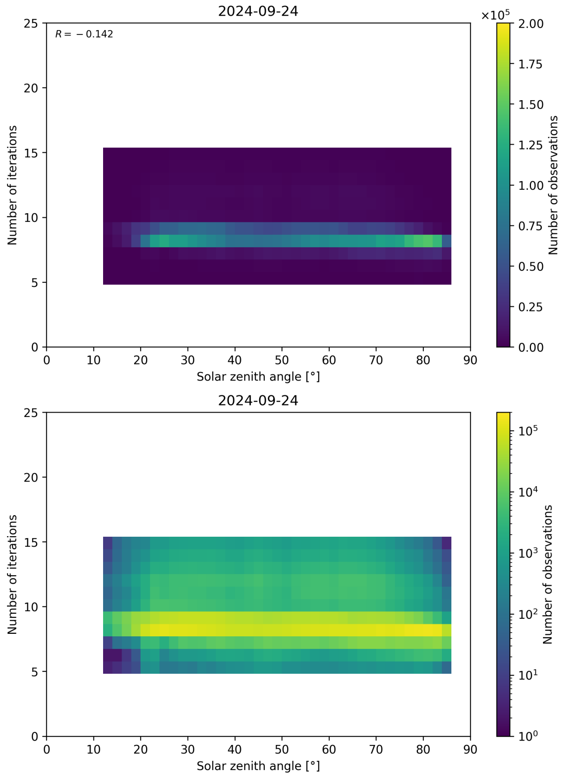
Figure 67: Scatter density plot of “Solar zenith angle” against “Number of iterations” for 2024-09-23 to 2024-09-25.
