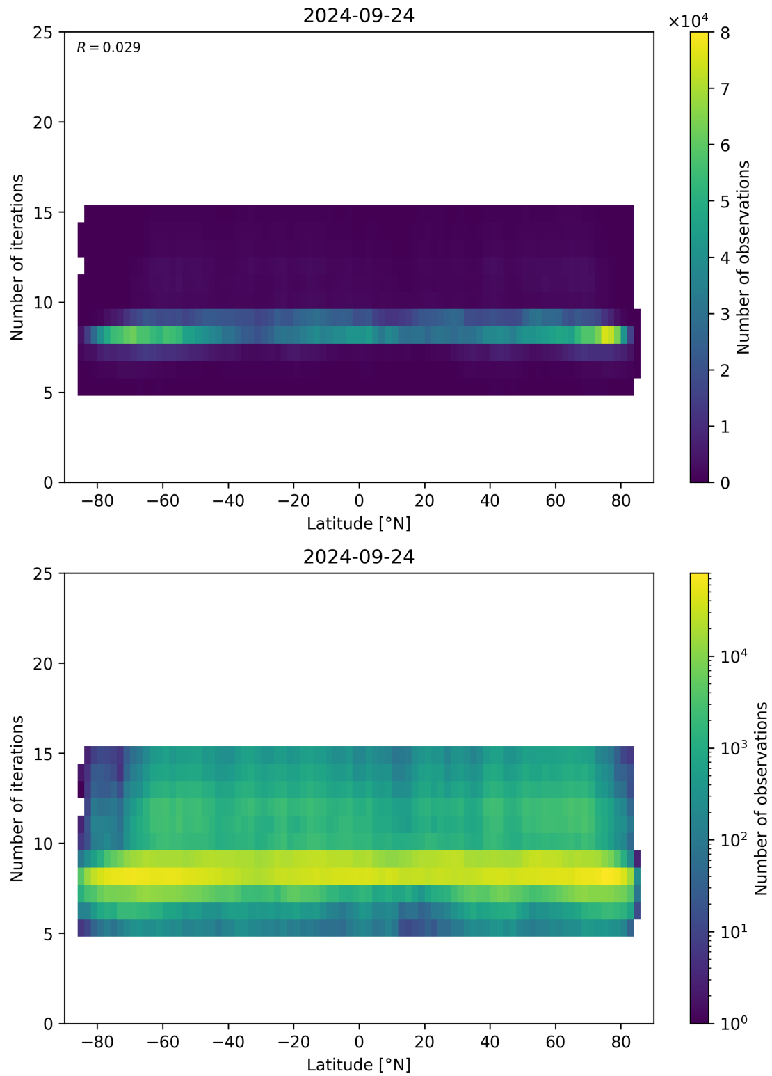
Figure 56: Scatter density plot of “Latitude” against “Number of iterations” for 2024-09-23 to 2024-09-25.
