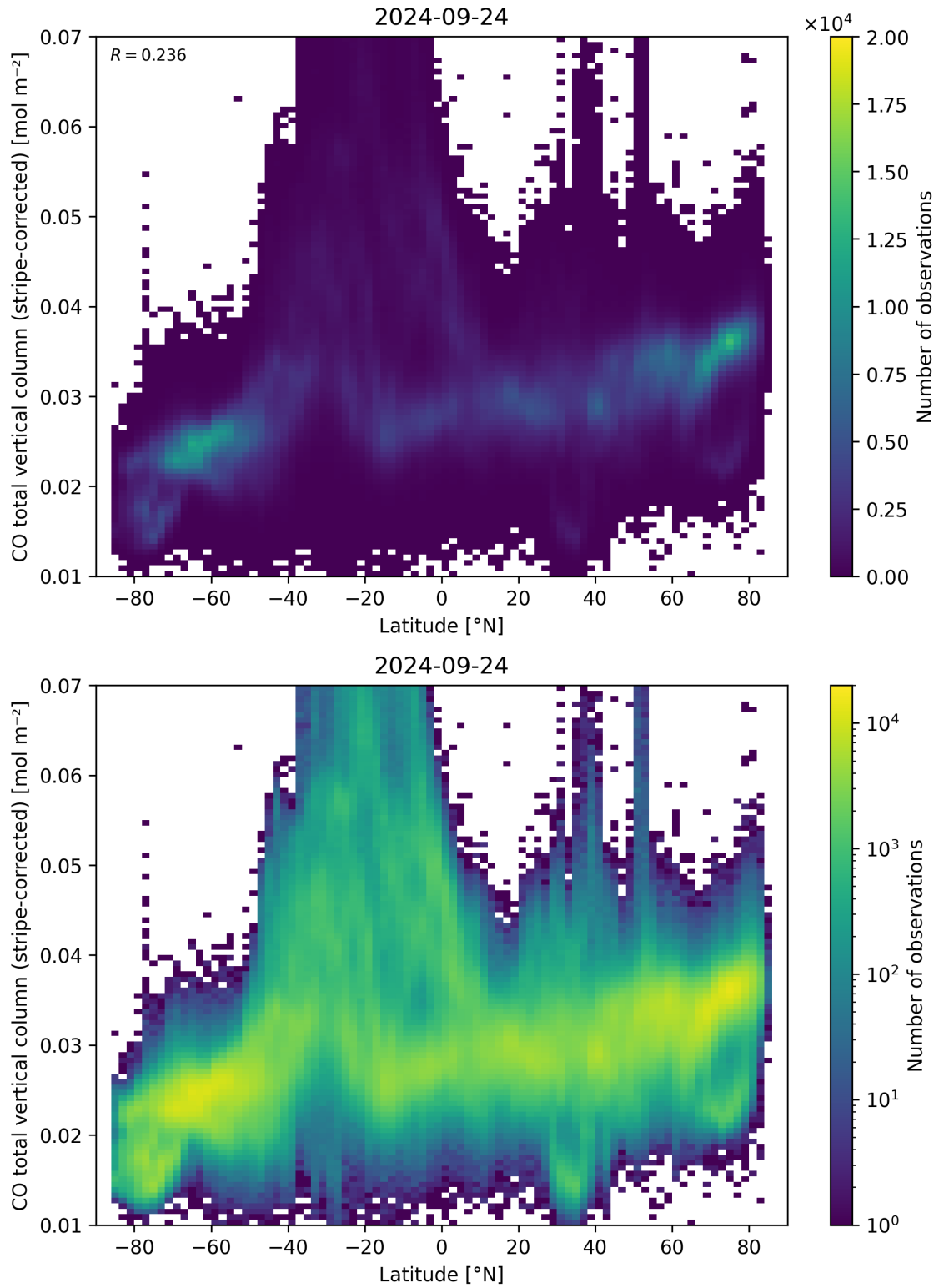
Figure 52: Scatter density plot of “Latitude” against “CO total vertical column (stripe-corrected)” for 2024-09-23 to 2024-09-25.
