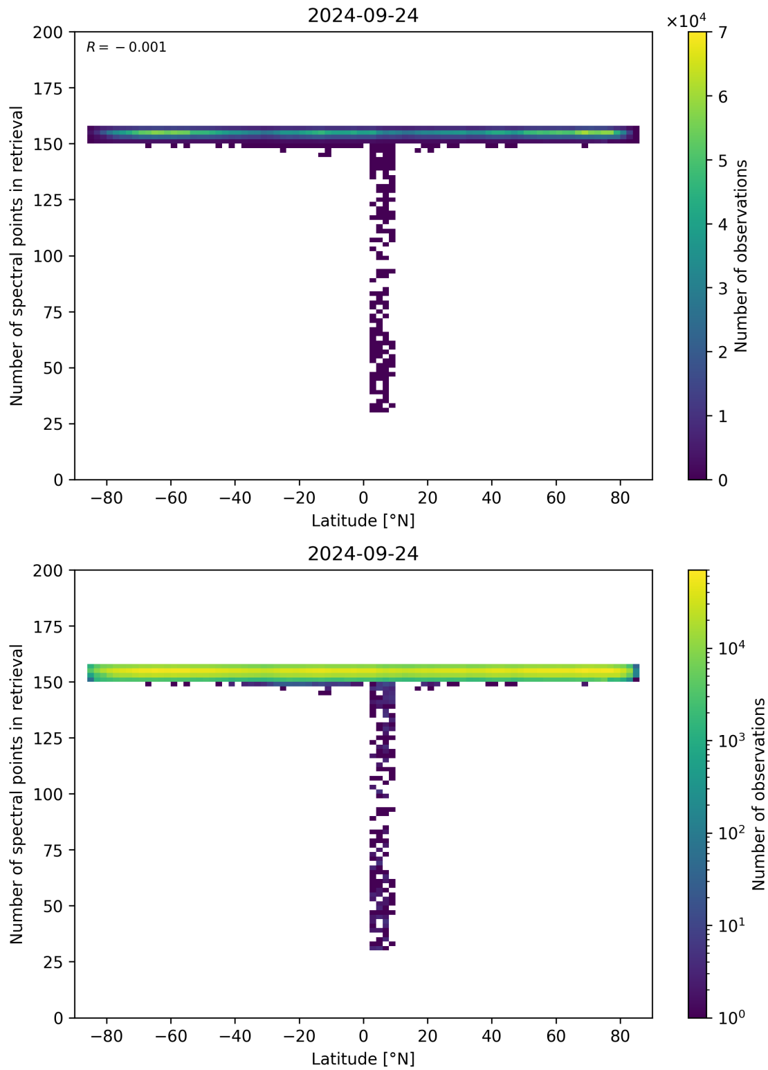
Figure 57: Scatter density plot of “Latitude” against “Number of spectral points in retrieval” for 2024-09-23 to 2024-09-25.
