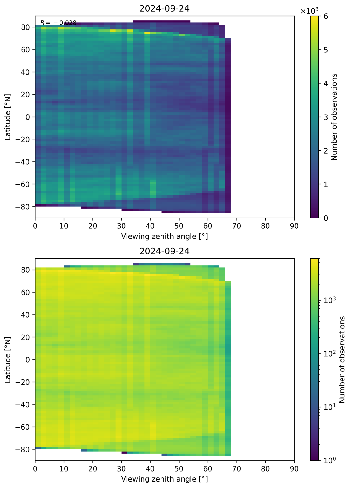
Figure 74: Scatter density plot of “Viewing zenith angle” against “Latitude” for 2024-09-23 to 2024-09-25.
