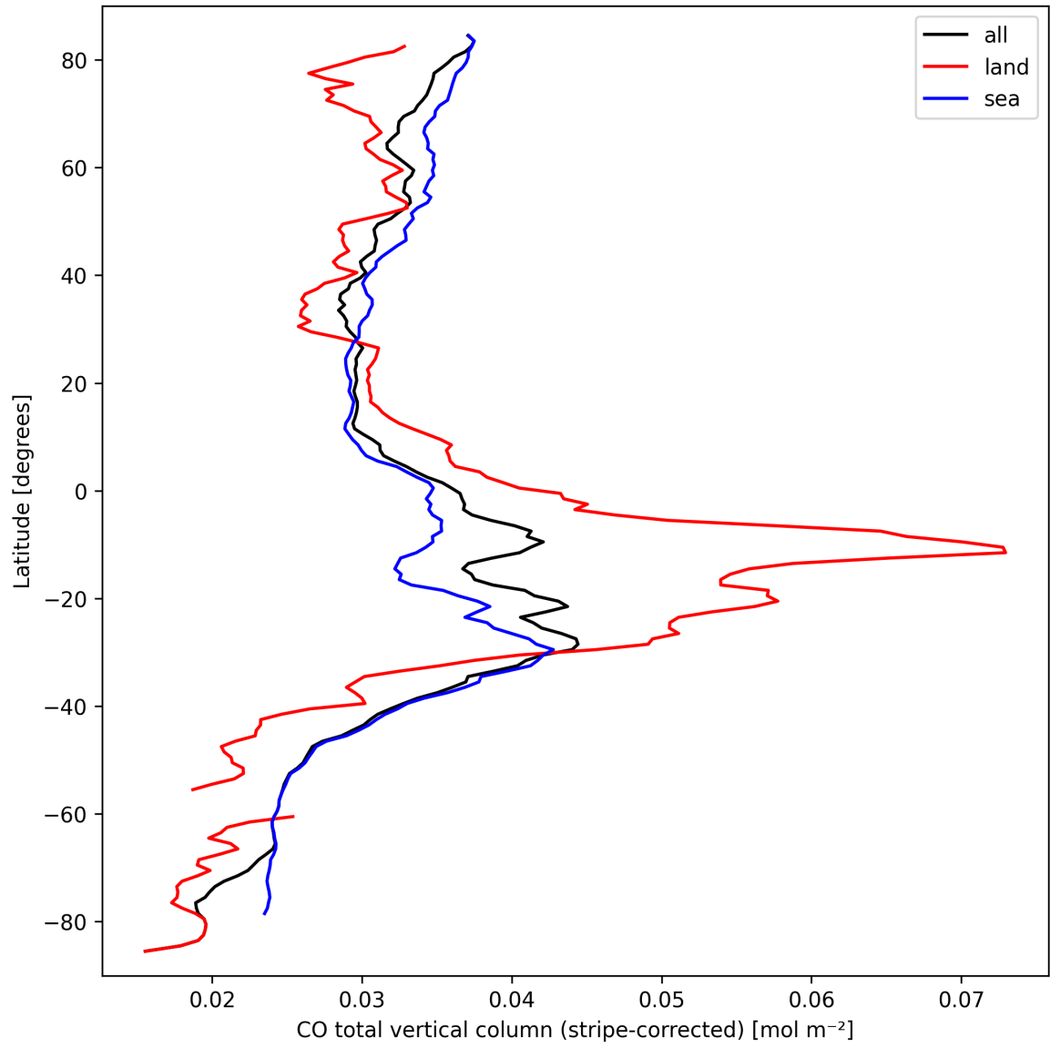
Figure 11: Zonal average of “CO total vertical column (stripe-corrected)” for 2024-09-23 to 2024-09-25.
