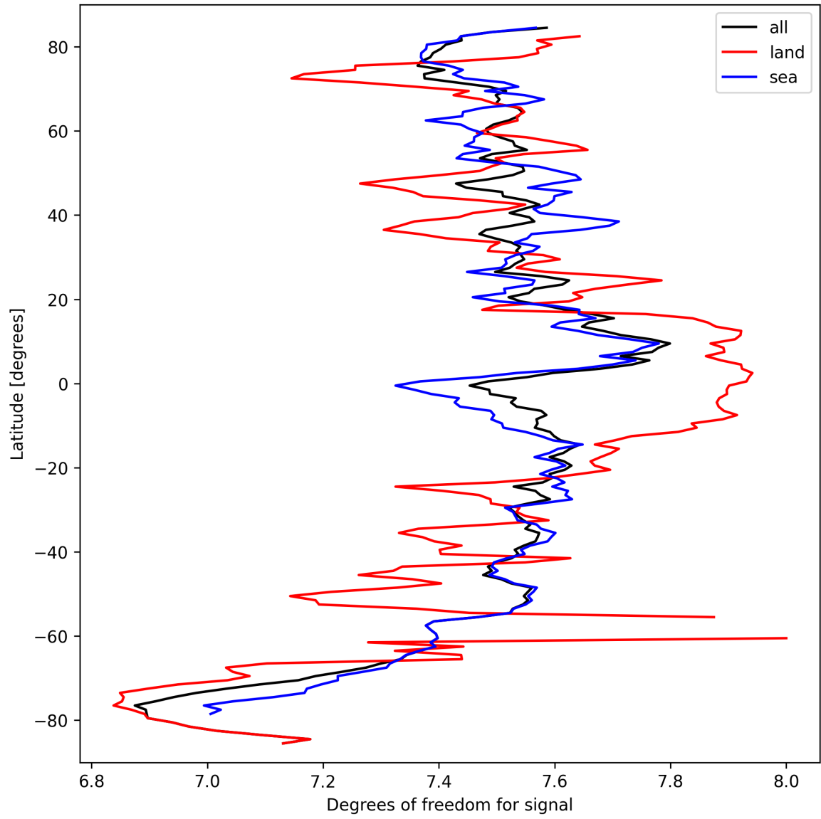
Figure 15: Zonal average of “Degrees of freedom for signal” for 2024-09-23 to 2024-09-25.
