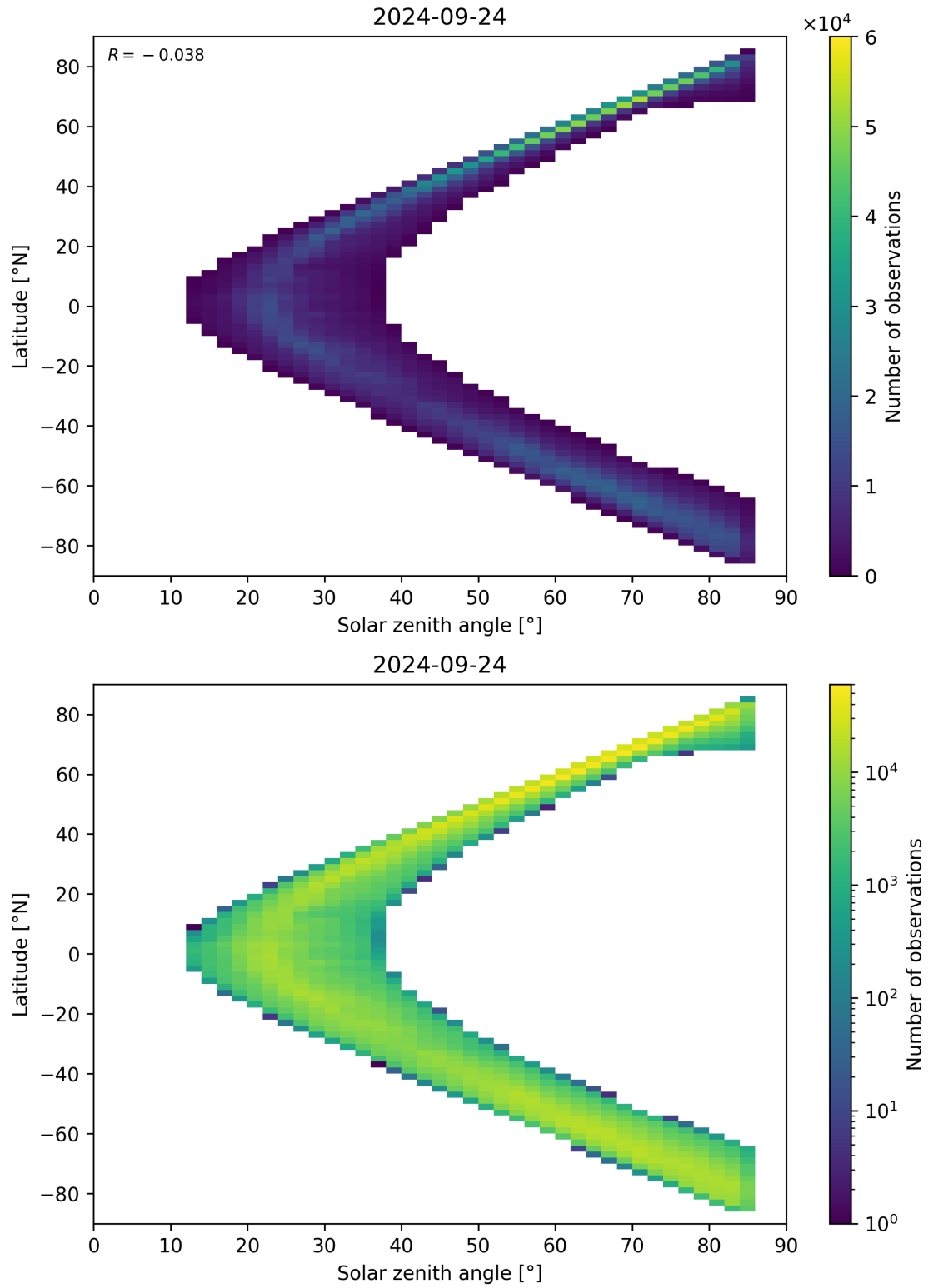
Figure 66: Scatter density plot of “Solar zenith angle” against “Latitude” for 2024-09-23 to 2024-09-25.
