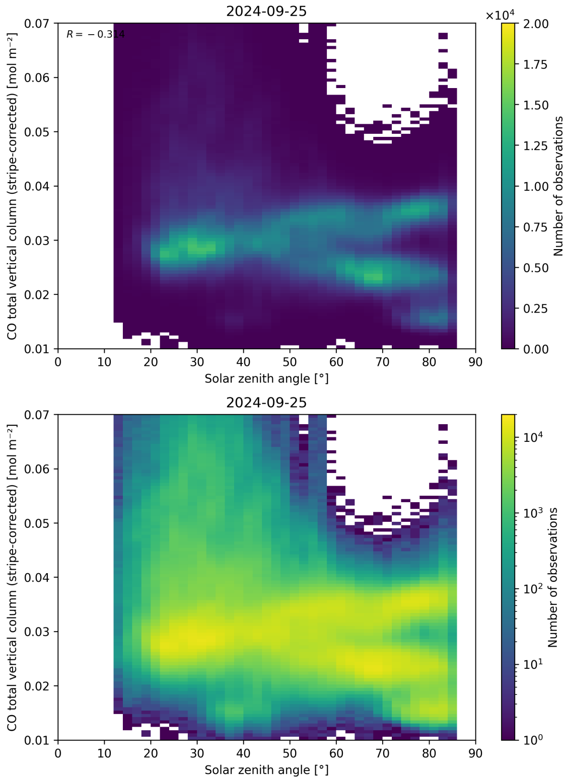
Figure 62: Scatter density plot of “Solar zenith angle” against “CO total vertical column (stripe-corrected)” for 2024-09-24 to 2024-09-26.
