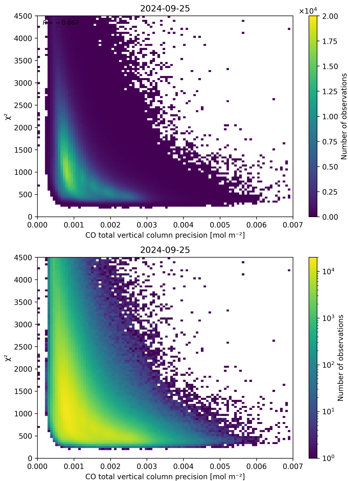
Figure 44: Scatter density plot of “CO total vertical column precision” against “ \chi^2 ” for 2024-09-24 to 2024-09-26.
