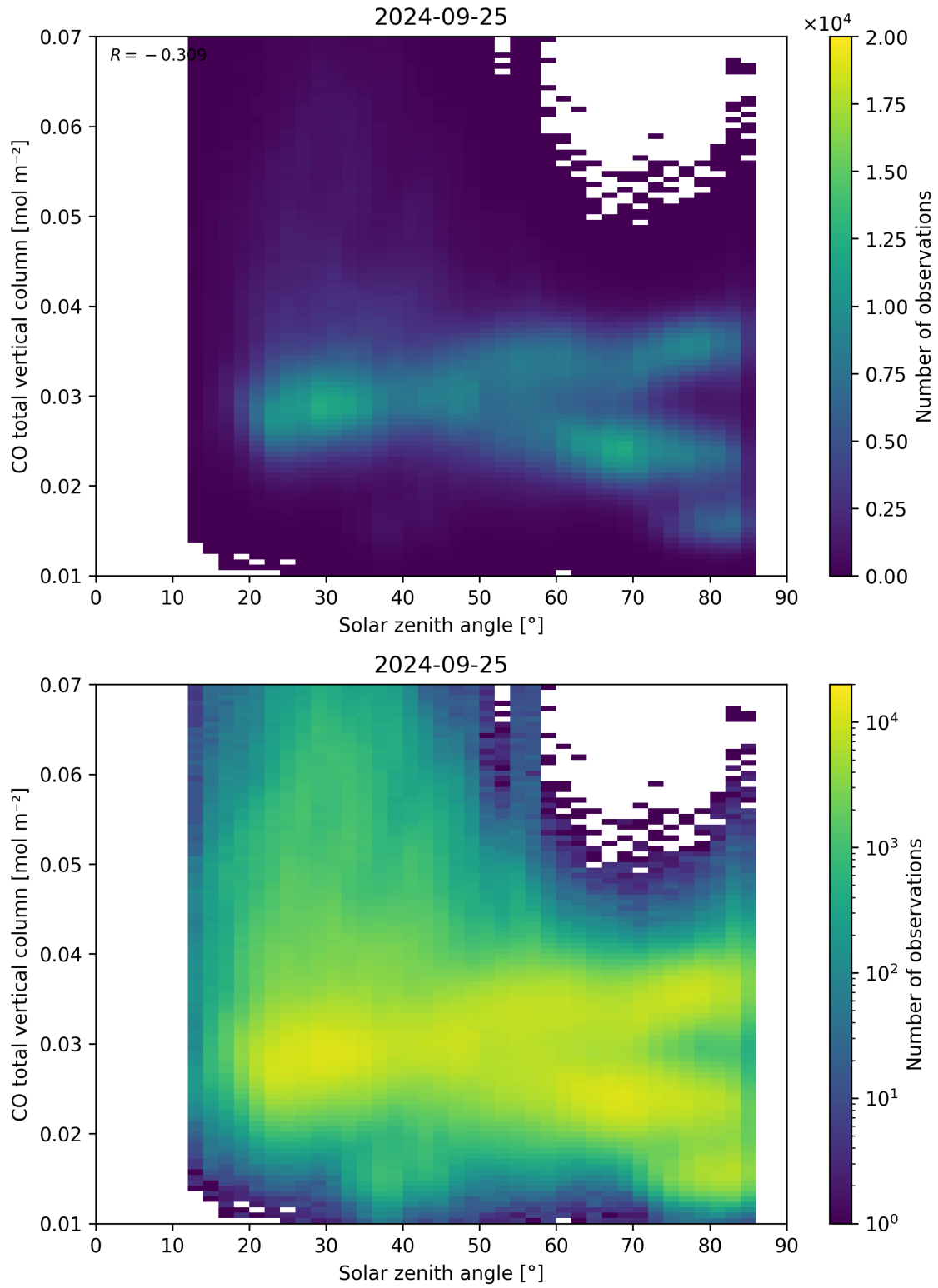
Figure 61: Scatter density plot of “Solar zenith angle” against “CO total vertical column” for 2024-09-24 to 2024-09-26.
