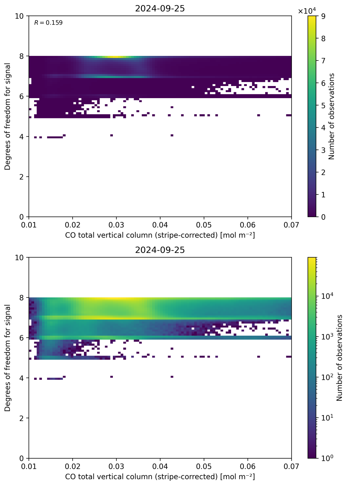
Figure 38: Scatter density plot of “CO total vertical column (stripe-corrected)” against “Degrees of freedom for signal” for 2024-09-24 to 2024-09-26.
