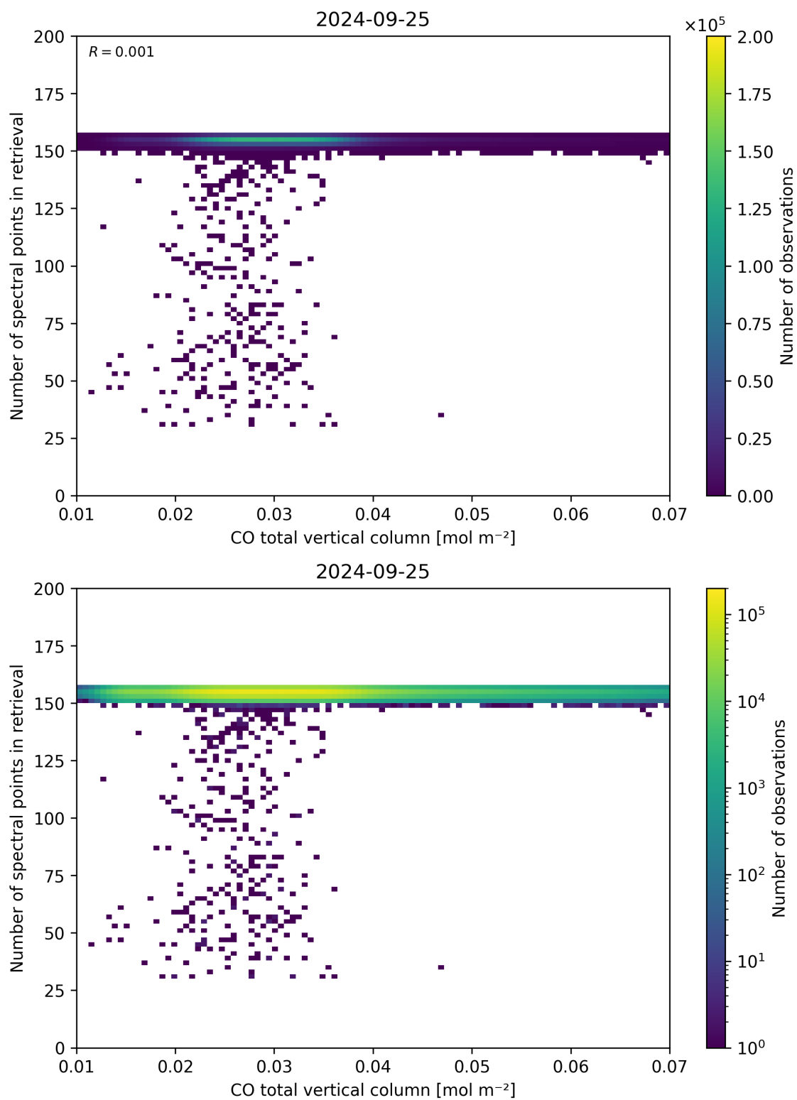
Figure 43: Scatter density plot of “CO total vertical column” against “Number of spectral points in retrieval” for 2024-09-24 to 2024-09-26.
