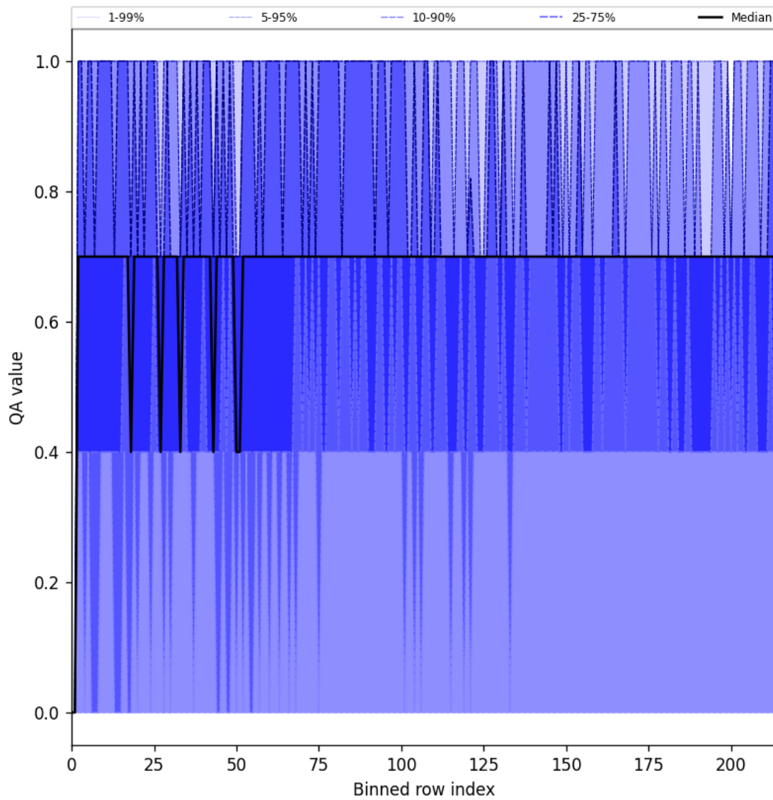
Figure 25: Along track statistics of “QA value” for 2024-09-24 to 2024-09-26
