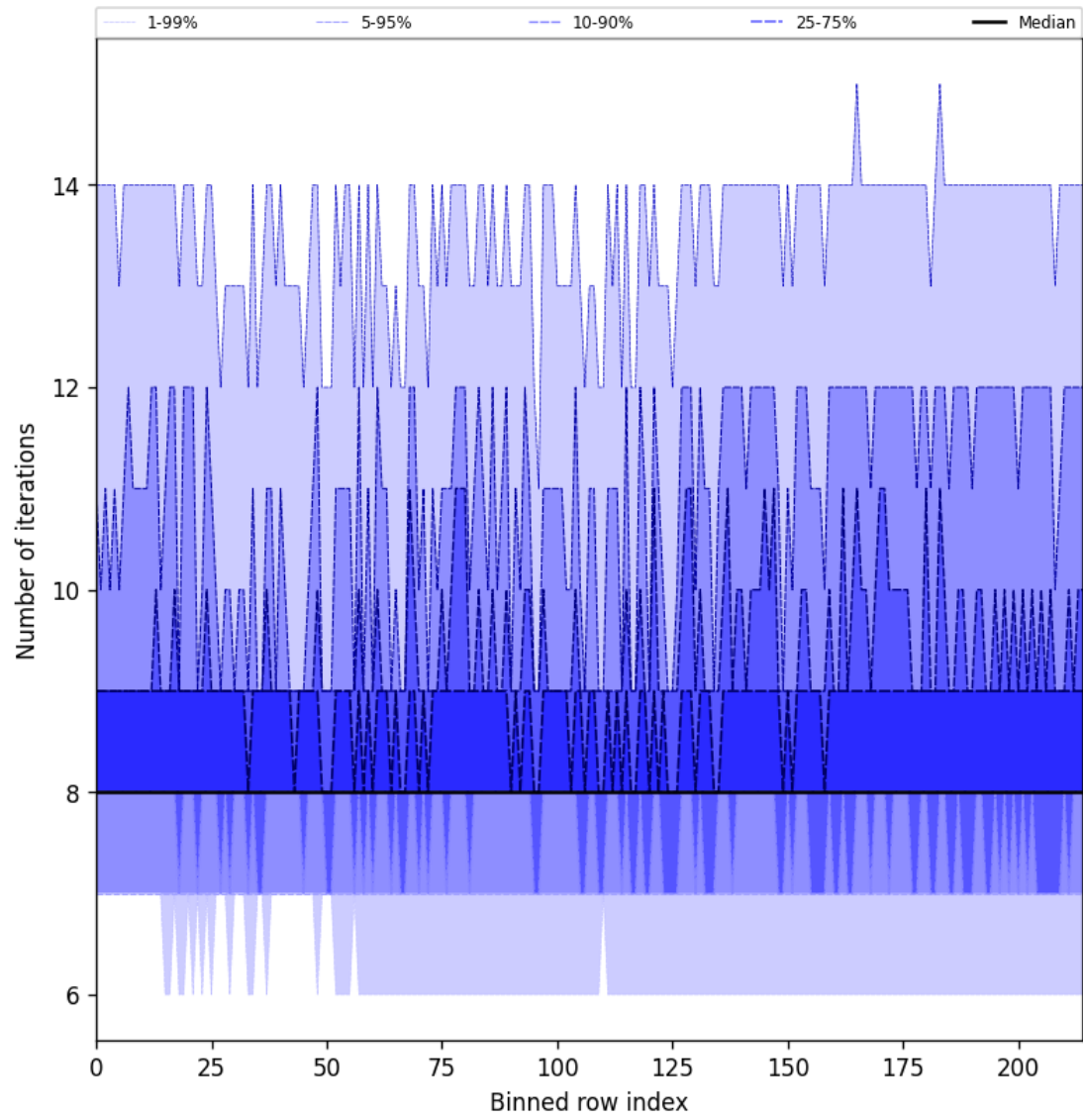
Figure 32: Along track statistics of “Number of iterations” for 2024-09-24 to 2024-09-26
