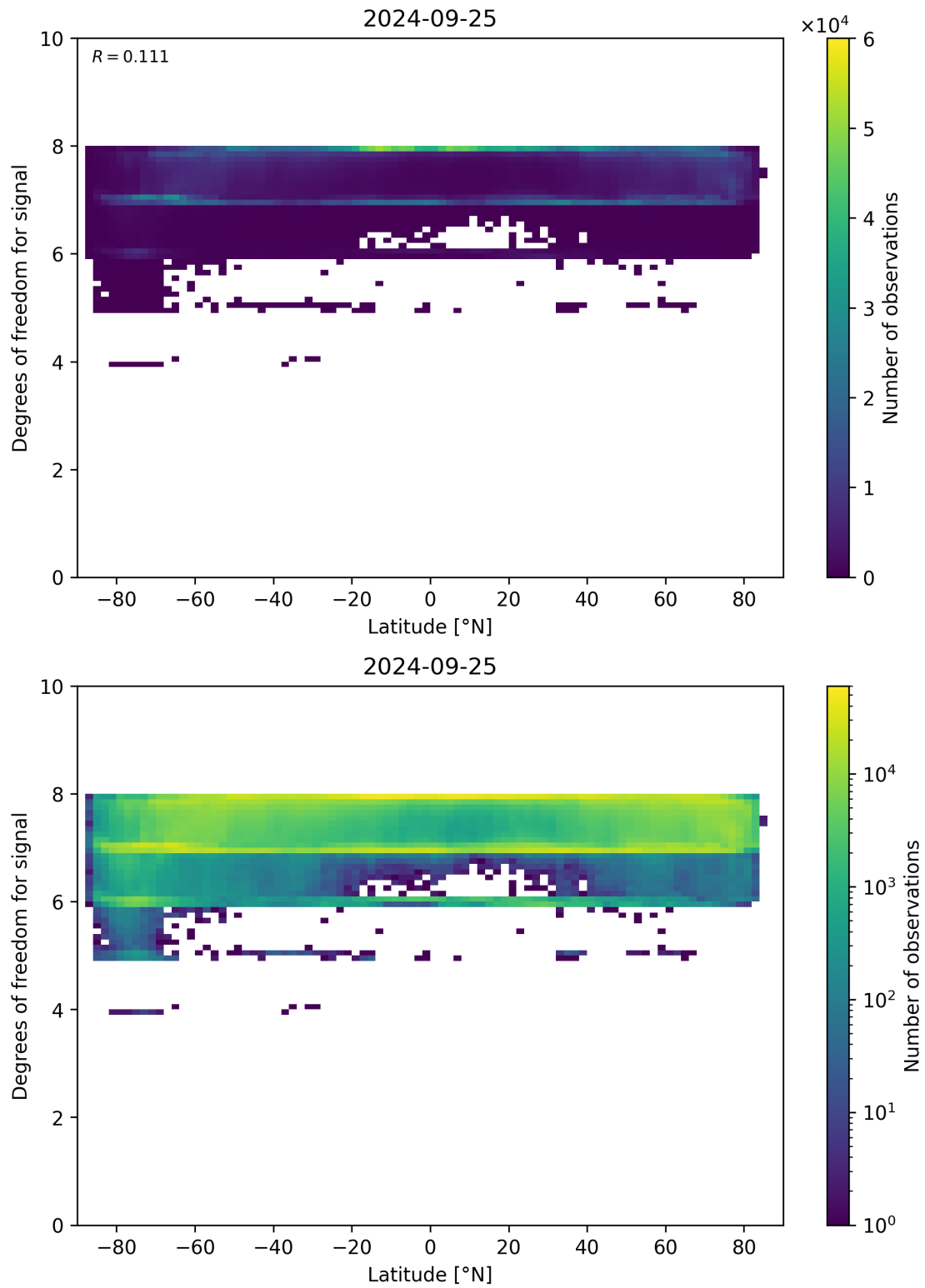
Figure 55: Scatter density plot of “Latitude” against “Degrees of freedom for signal” for 2024-09-24 to 2024-09-26.
