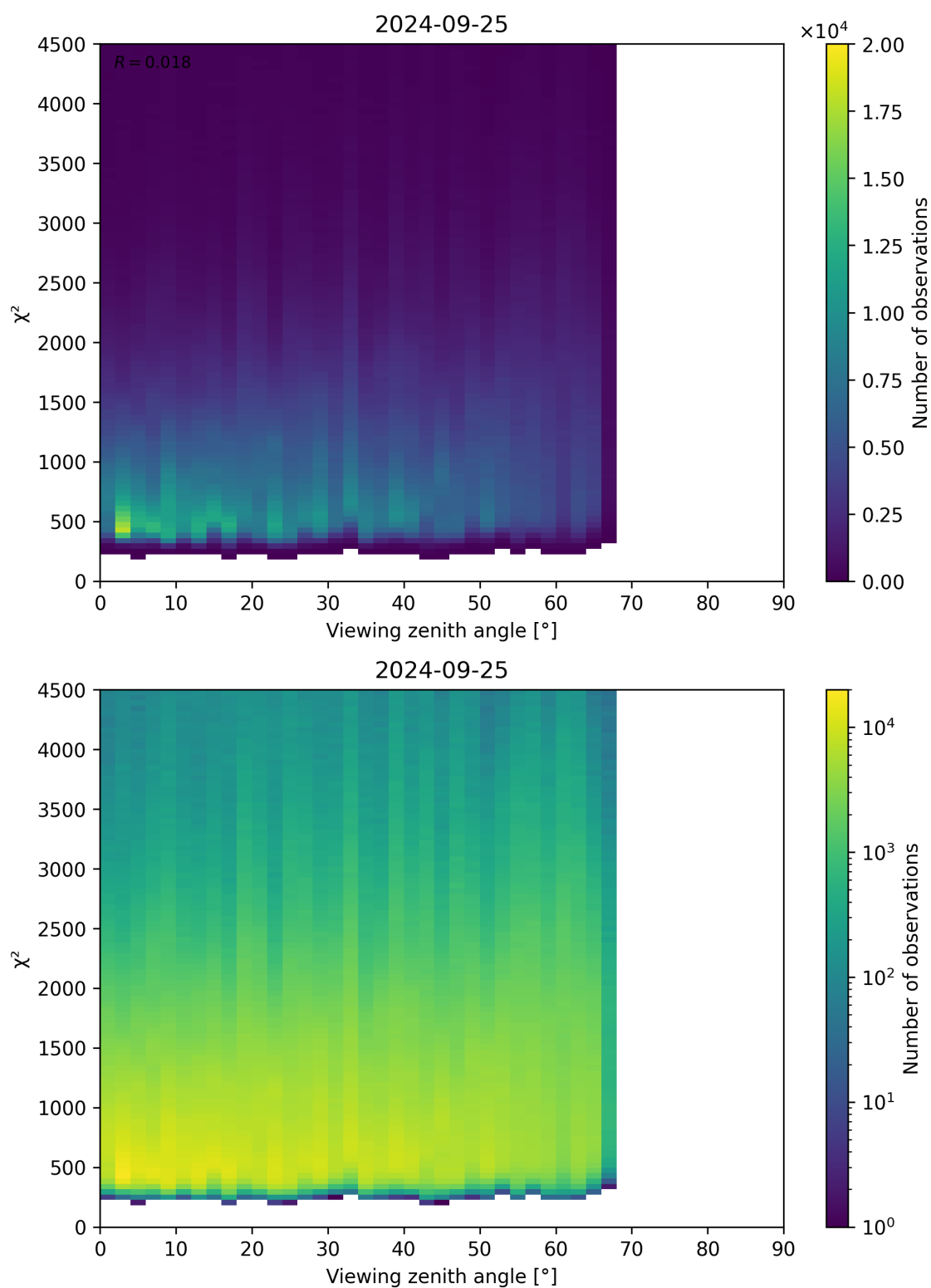
Figure 72: Scatter density plot of “Viewing zenith angle” against “ \chi^2 ” for 2024-09-24 to 2024-09-26.
