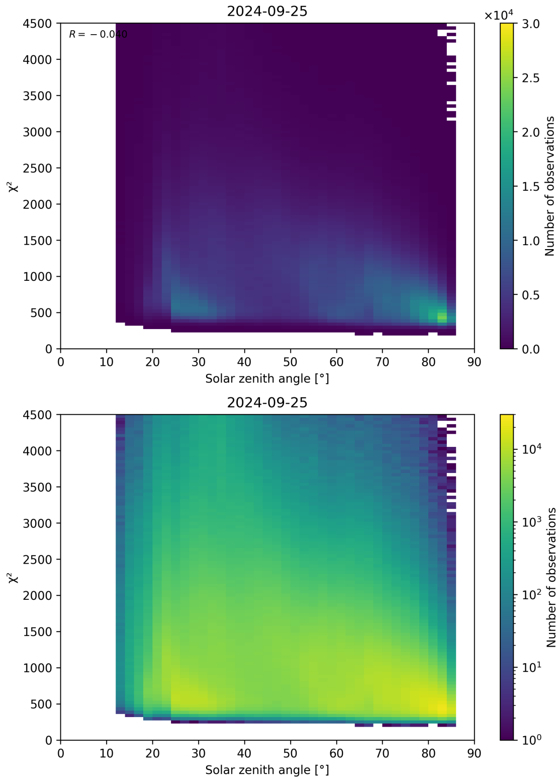
Figure 64: Scatter density plot of “Solar zenith angle” against “ \chi^2 ” for 2024-09-24 to 2024-09-26.
