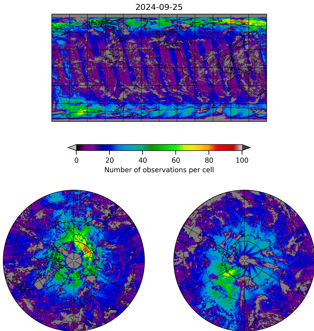
Figure 8: Map of the number of observations for 2024-09-24 to 2024-09-26
