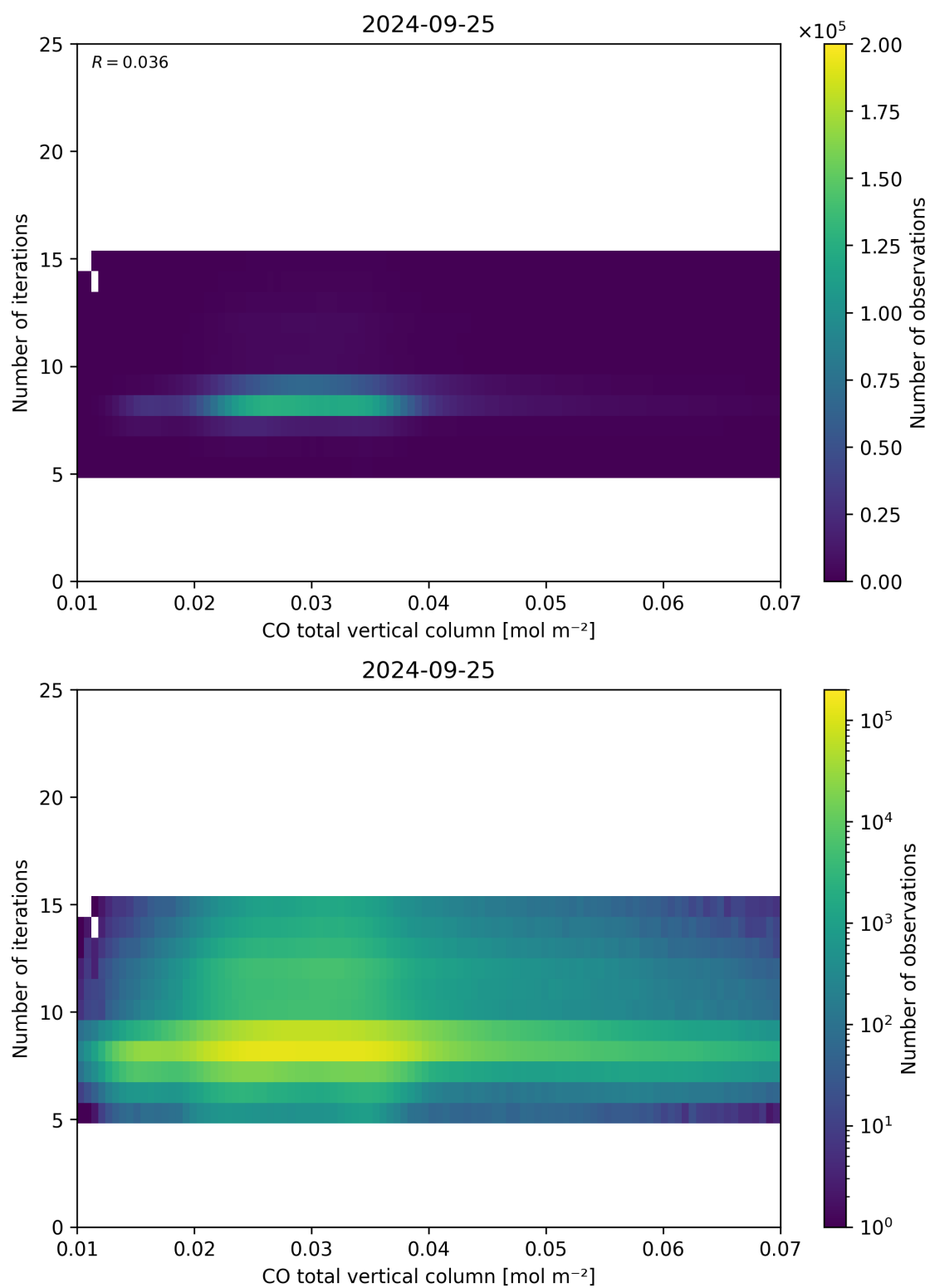
Figure 42: Scatter density plot of “CO total vertical column” against “Number of iterations” for 2024-09-24 to 2024-09-26.
