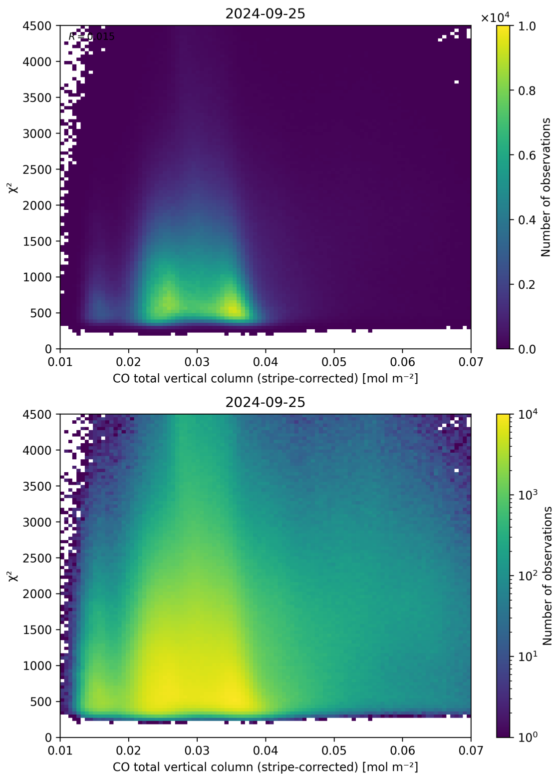
Figure 37: Scatter density plot of “CO total vertical column (stripe-corrected)” against “ \chi^2 ” for 2024-09-24 to 2024-09-26.
