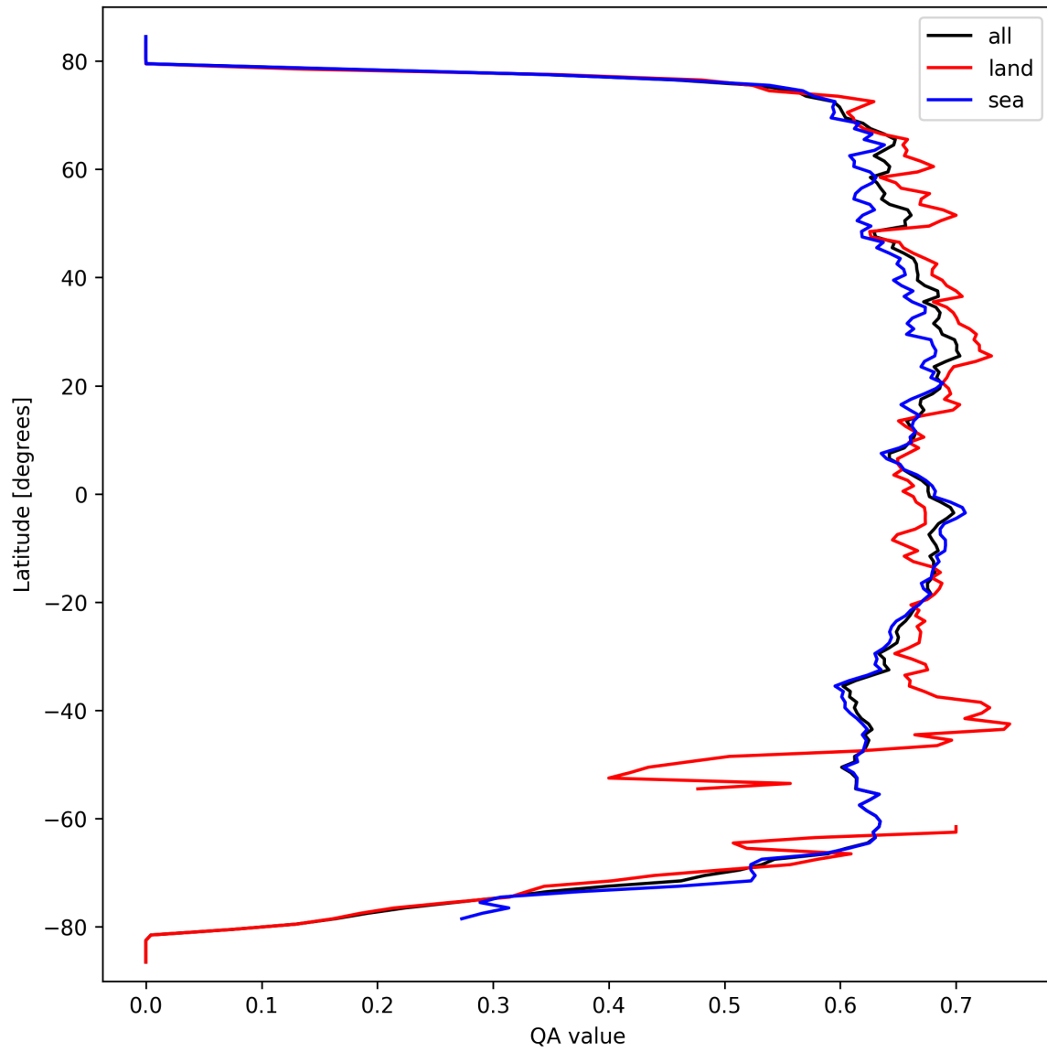
Figure 9: Zonal average of “QA value” for 2024-09-24 to 2024-09-26.
