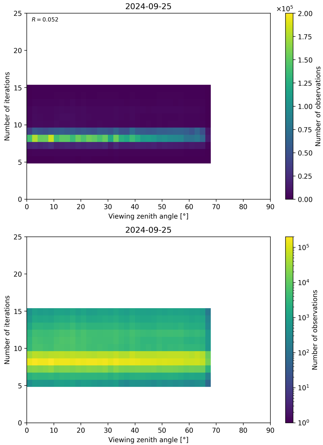
Figure 75: Scatter density plot of “Viewing zenith angle” against “Number of iterations” for 2024-09-24 to 2024-09-26.
