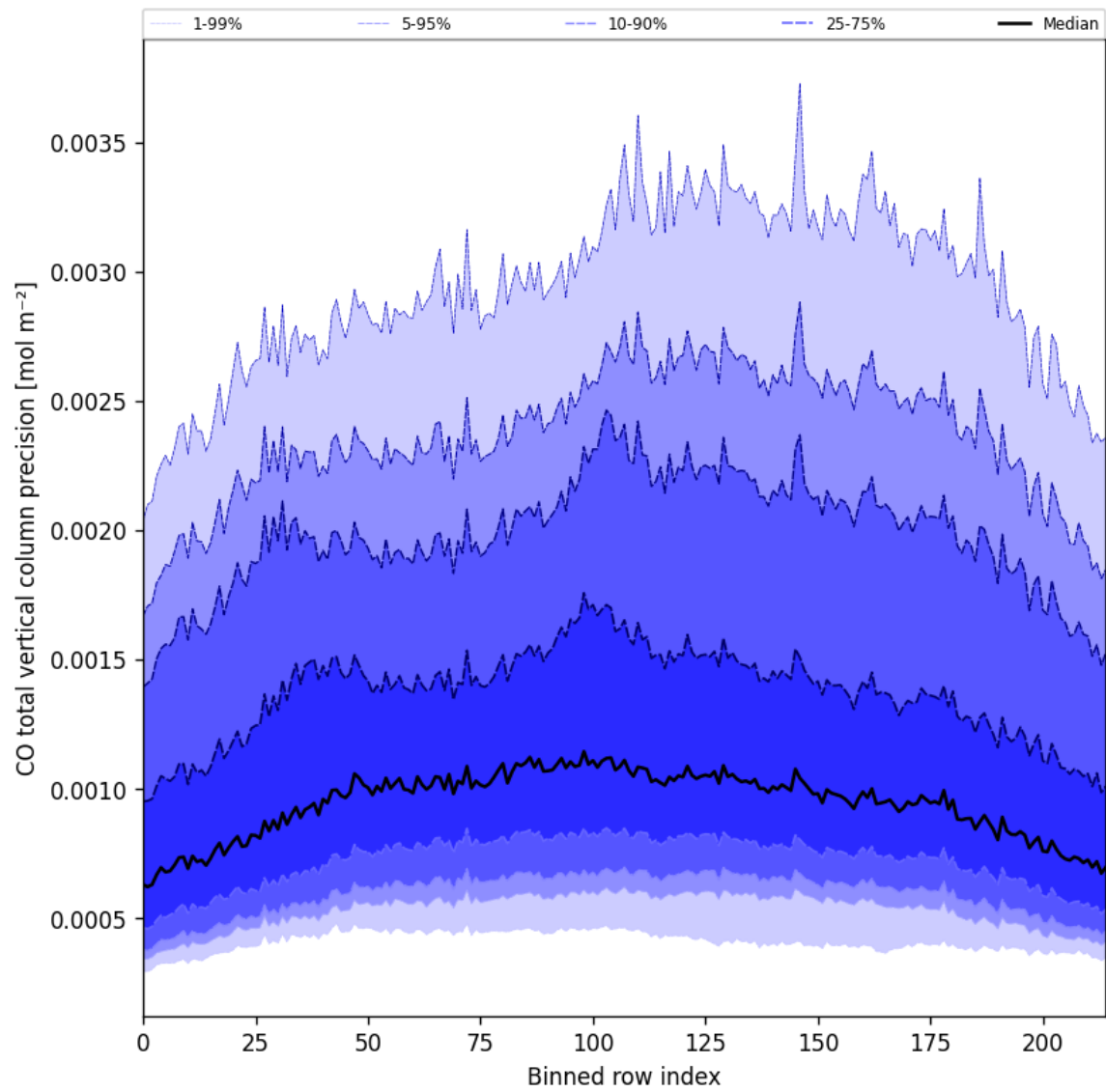
Figure 28: Along track statistics of “CO total vertical column precision” for 2024-09-24 to 2024-09-26
