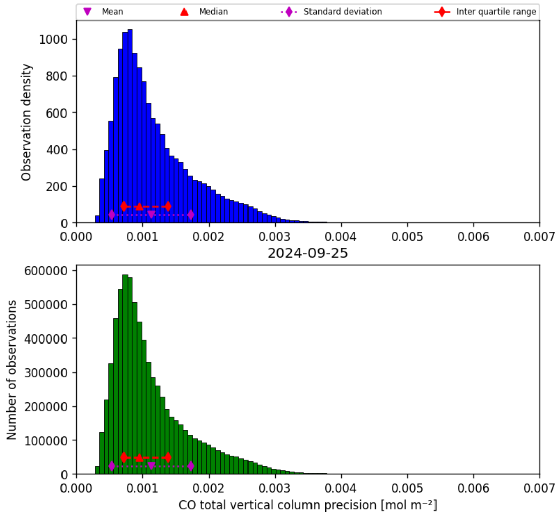
Figure 20: Histogram of “CO total vertical column precision” for 2024-09-24 to 2024-09-26
