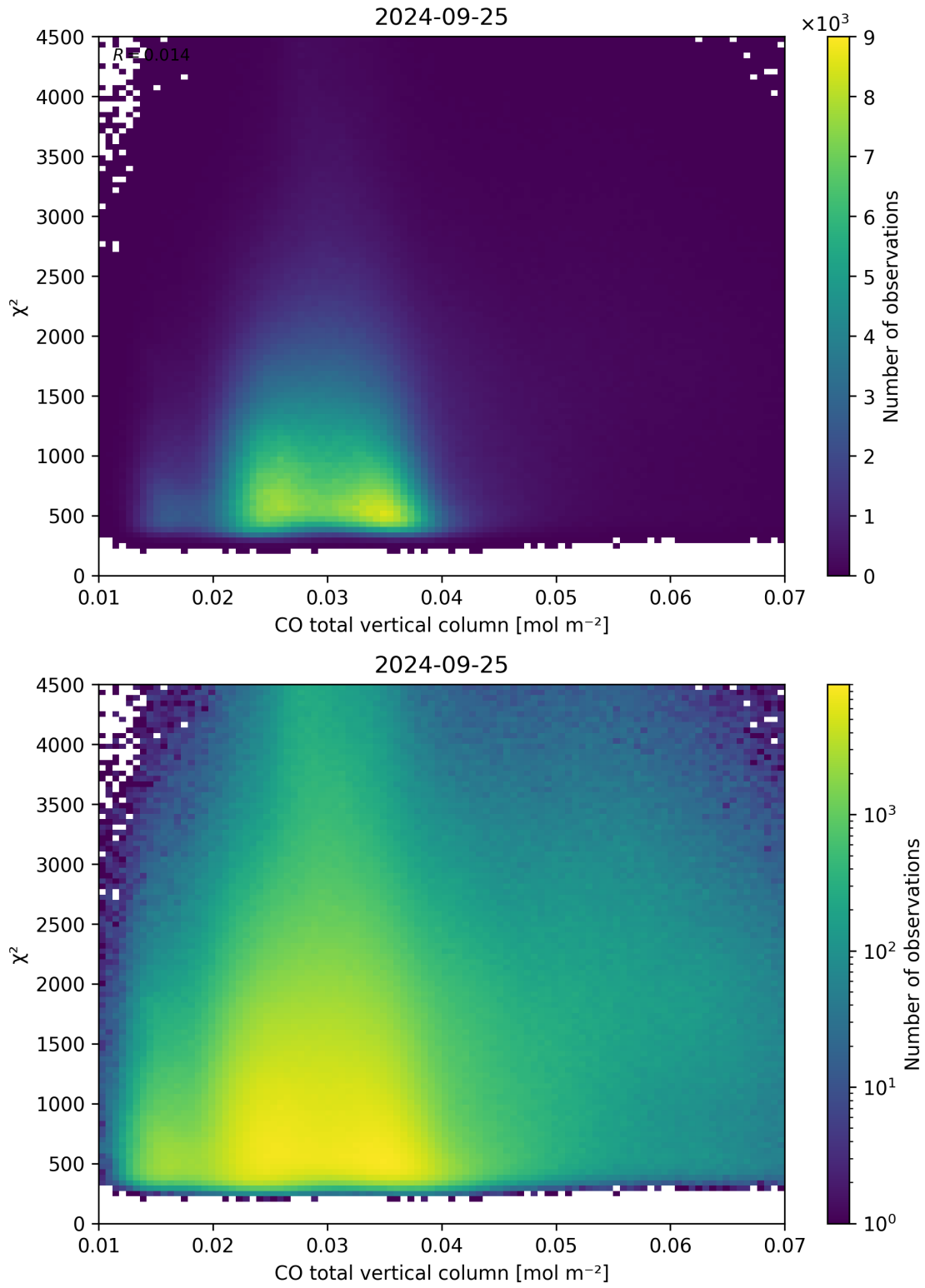
Figure 35: Scatter density plot of “CO total vertical column” against “ \chi^2 ” for 2024-09-24 to 2024-09-26.
