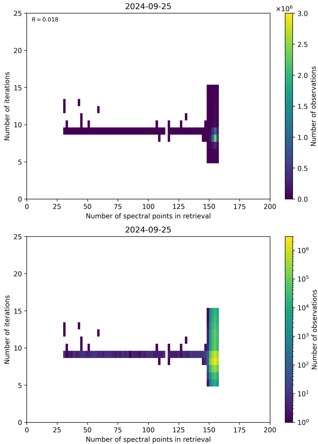
Figure 60: Scatter density plot of “Number of spectral points in retrieval” against “Number of iterations” for 2024-09-24 to 2024-09-26.
