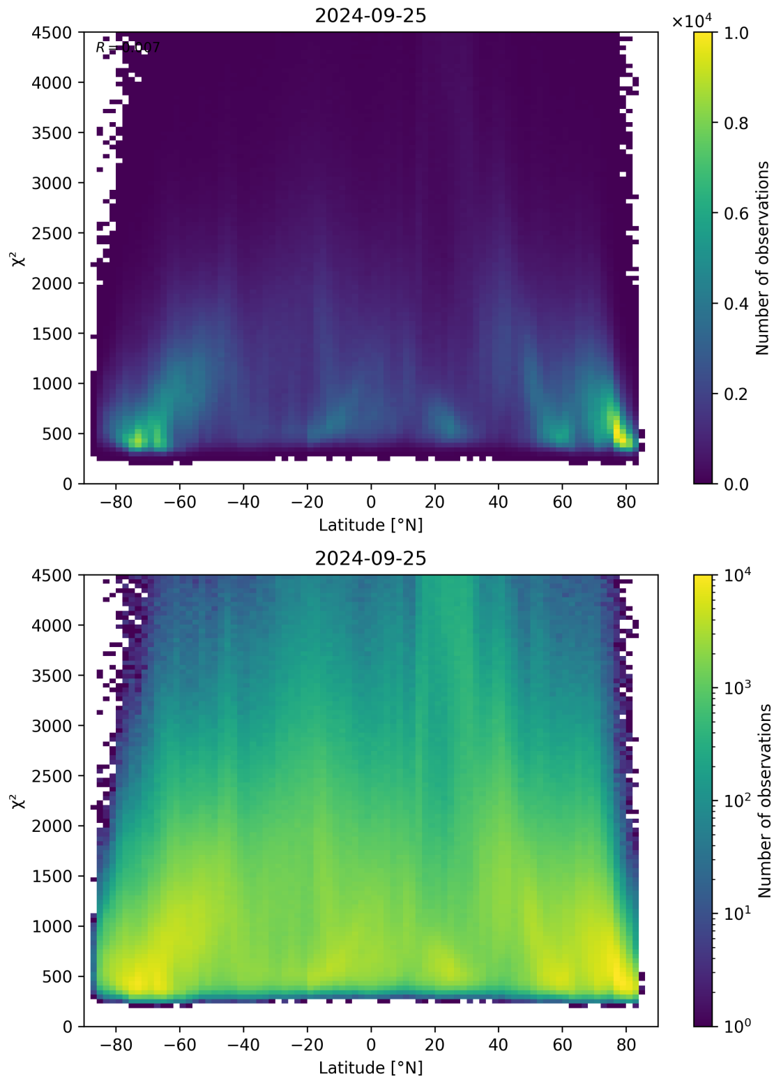
Figure 54: Scatter density plot of “Latitude” against “ \chi^2 ” for 2024-09-24 to 2024-09-26.
