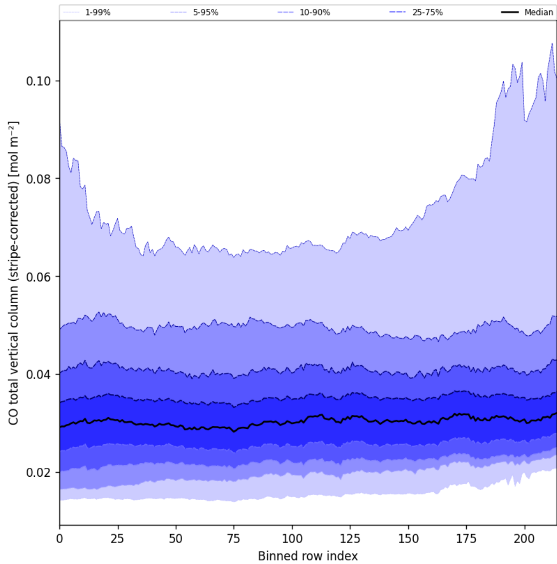
Figure 27: Along track statistics of “CO total vertical column (stripe-corrected)” for 2024-09-24 to 2024-09-26
