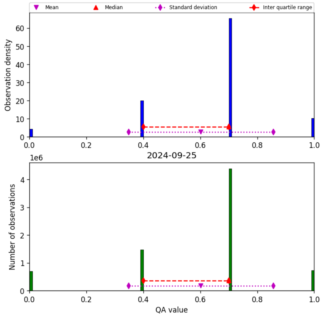
Figure 17: Histogram of “QA value” for 2024-09-24 to 2024-09-26
