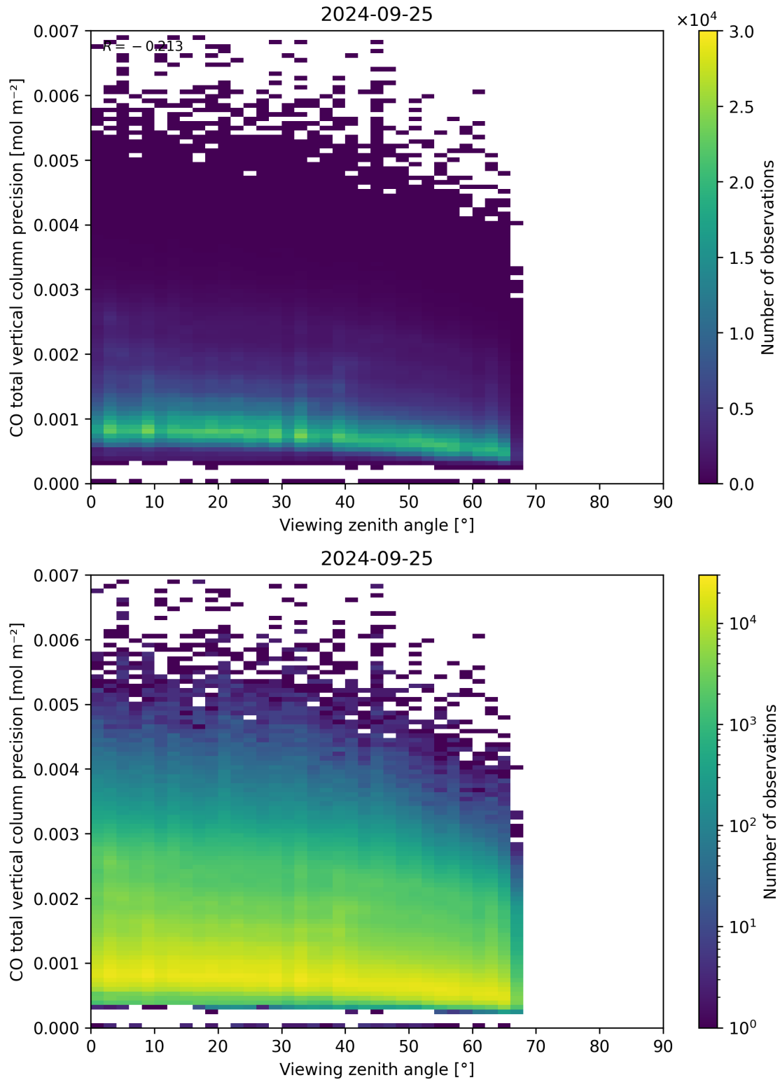
Figure 71: Scatter density plot of “Viewing zenith angle” against “CO total vertical column precision” for 2024-09-24 to 2024-09-26.
