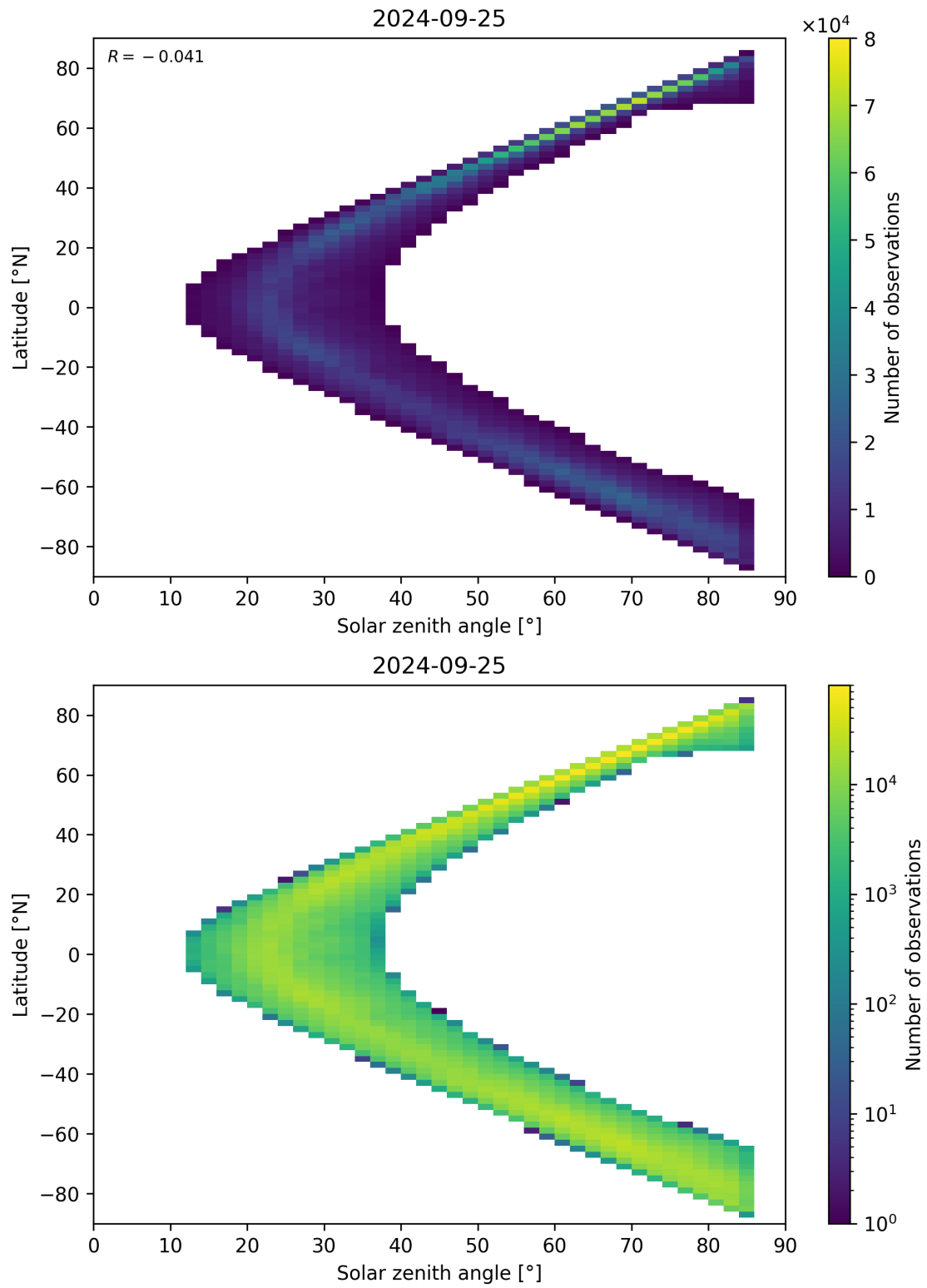
Figure 66: Scatter density plot of “Solar zenith angle” against “Latitude” for 2024-09-24 to 2024-09-26.
