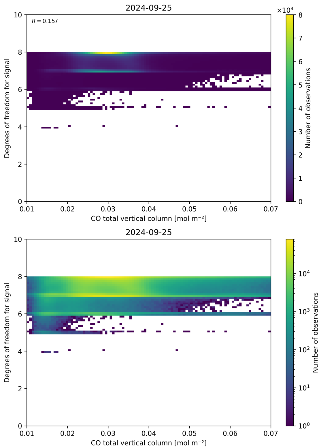
Figure 41: Scatter density plot of “CO total vertical column” against “Degrees of freedom for signal” for 2024-09-24 to 2024-09-26.
