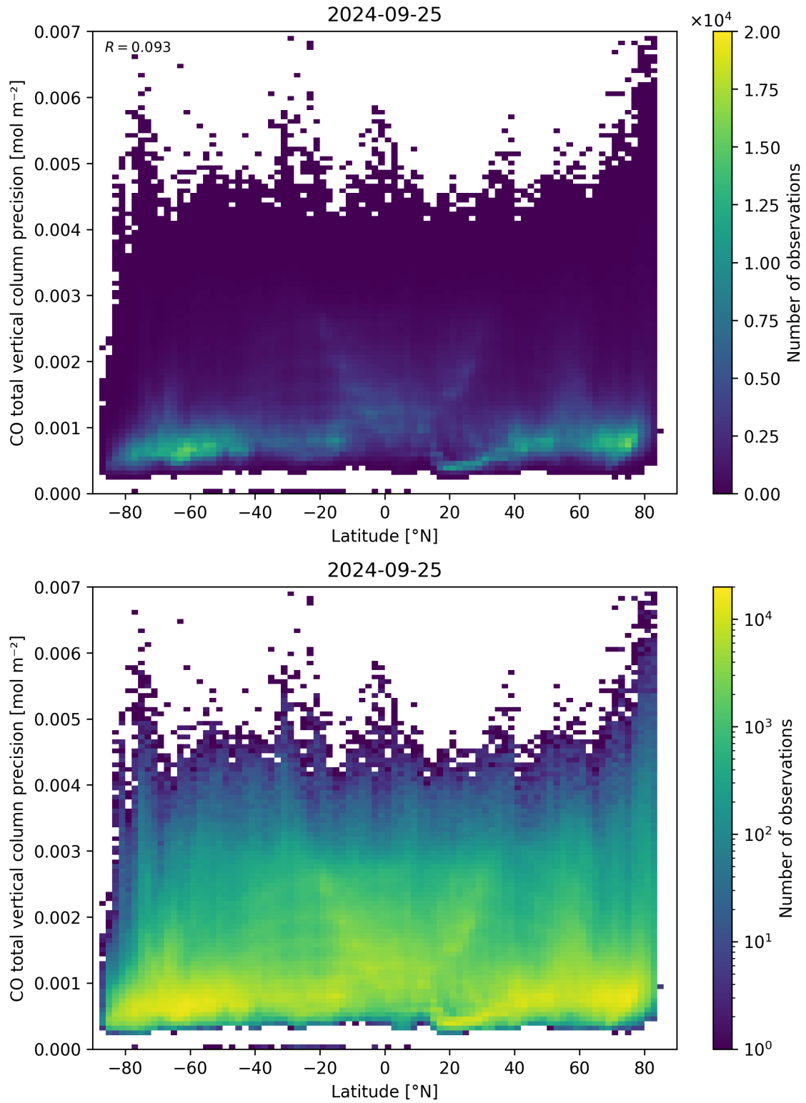
Figure 53: Scatter density plot of “Latitude” against “CO total vertical column precision” for 2024-09-24 to 2024-09-26.
