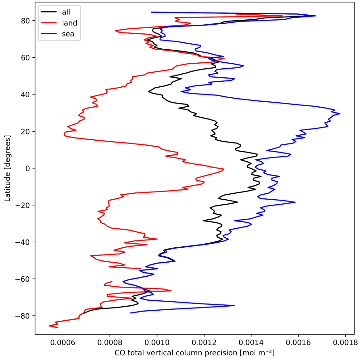
Figure 12: Zonal average of “CO total vertical column precision” for 2024-09-24 to 2024-09-26.
