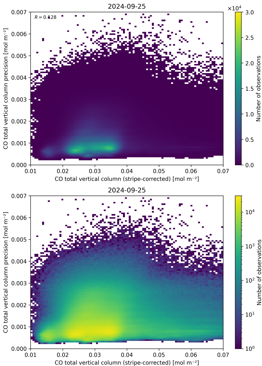
Figure 36: Scatter density plot of “CO total vertical column (stripe-corrected)” against “CO total vertical column precision” for 2024-09-24 to 2024-09-26.
