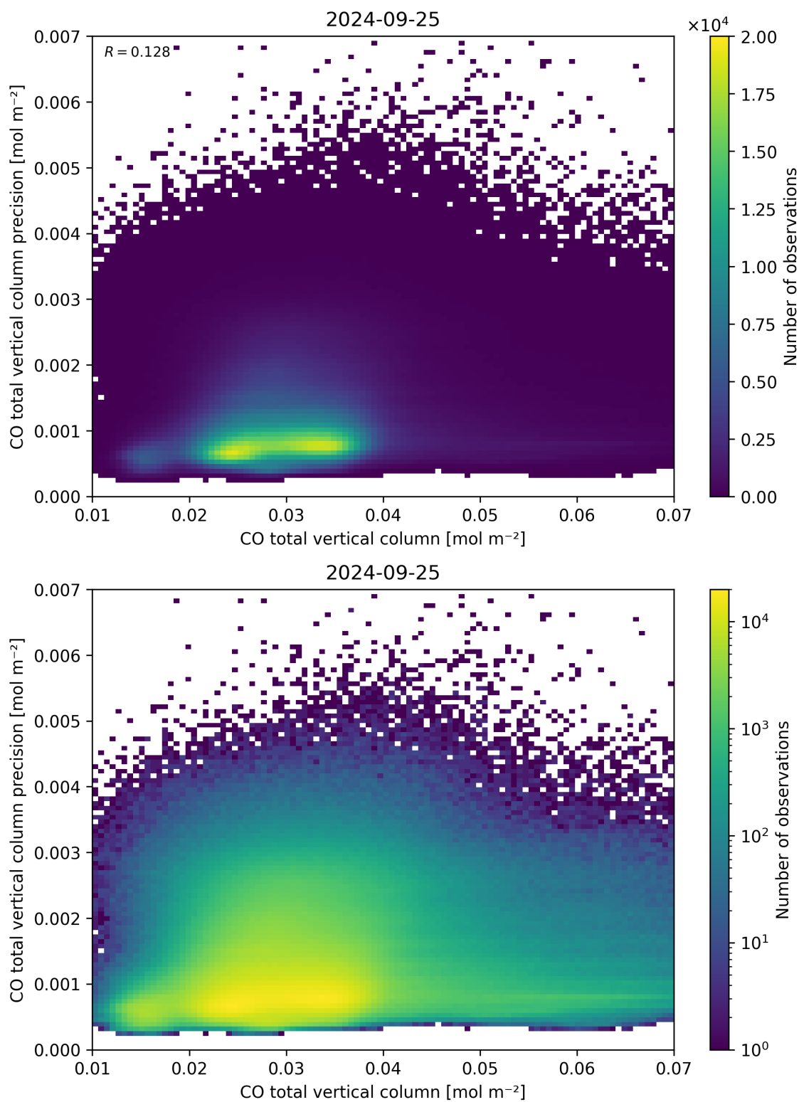
Figure 34: Scatter density plot of “CO total vertical column” against “CO total vertical column precision” for 2024-09-24 to 2024-09-26.
