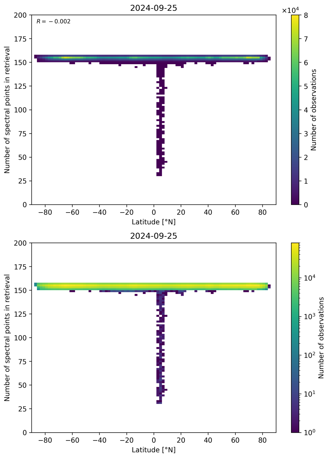
Figure 57: Scatter density plot of “Latitude” against “Number of spectral points in retrieval” for 2024-09-24 to 2024-09-26.
