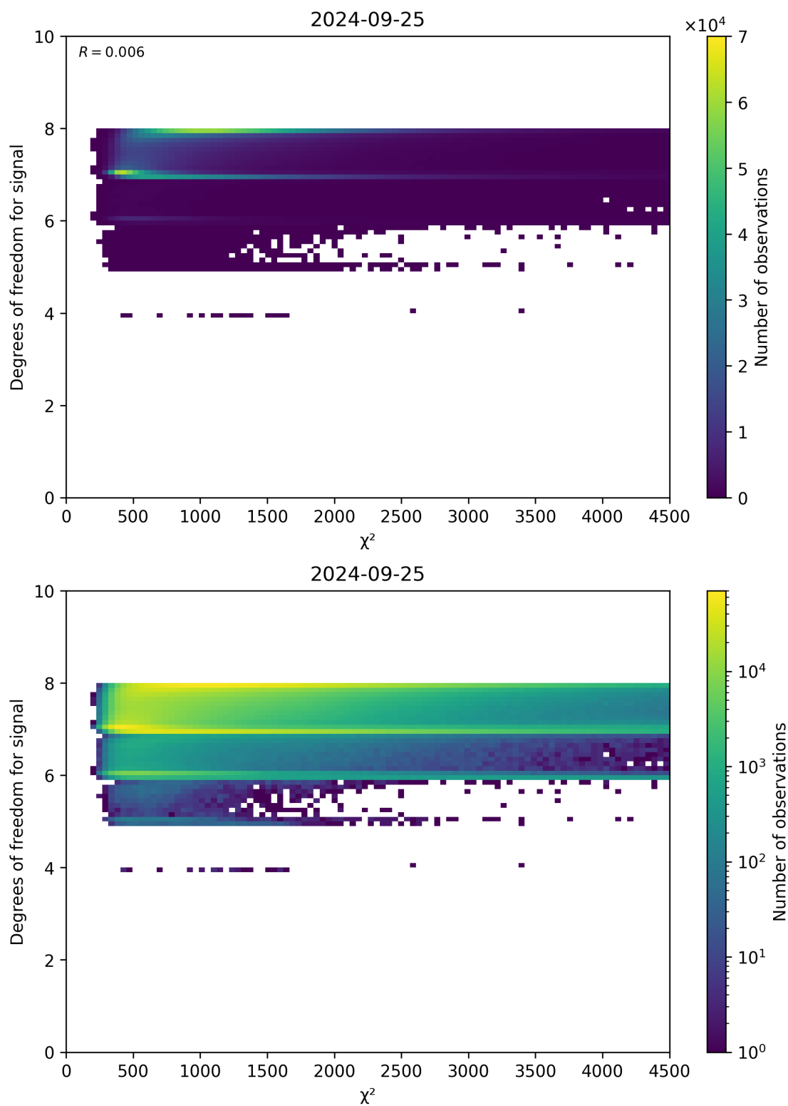
Figure 48: Scatter density plot of “ \chi^2 ” against “Degrees of freedom for signal” for 2024-09-24 to 2024-09-26.
