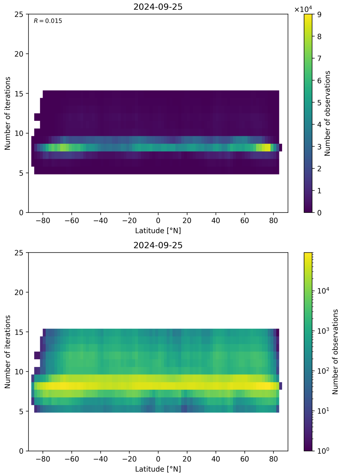
Figure 56: Scatter density plot of “Latitude” against “Number of iterations” for 2024-09-24 to 2024-09-26.
