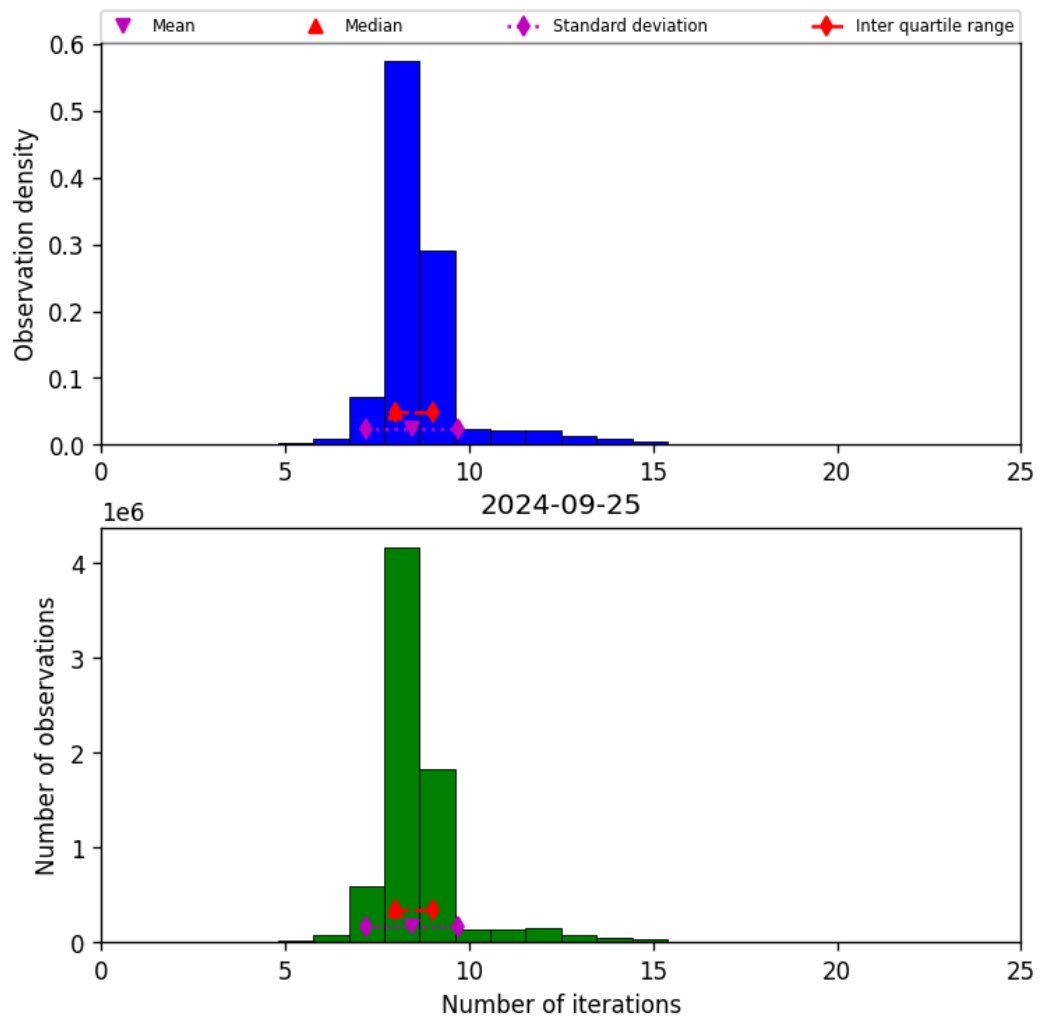
Figure 24: Histogram of “Number of iterations” for 2024-09-24 to 2024-09-26
