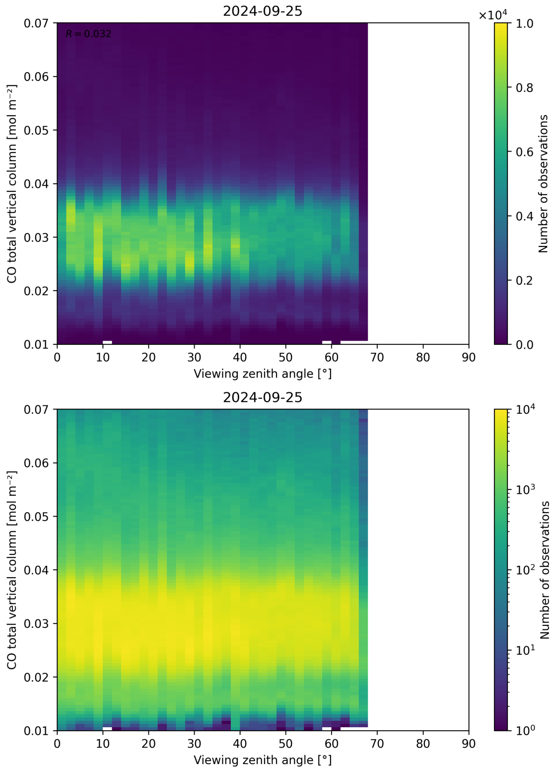
Figure 69: Scatter density plot of “Viewing zenith angle” against “CO total vertical column” for 2024-09-24 to 2024-09-26.
