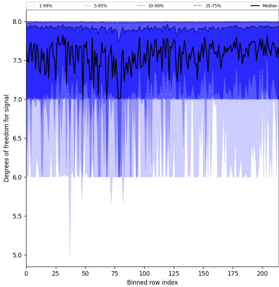
Figure 31: Along track statistics of “Degrees of freedom for signal” for 2024-09-24 to 2024-09-26
