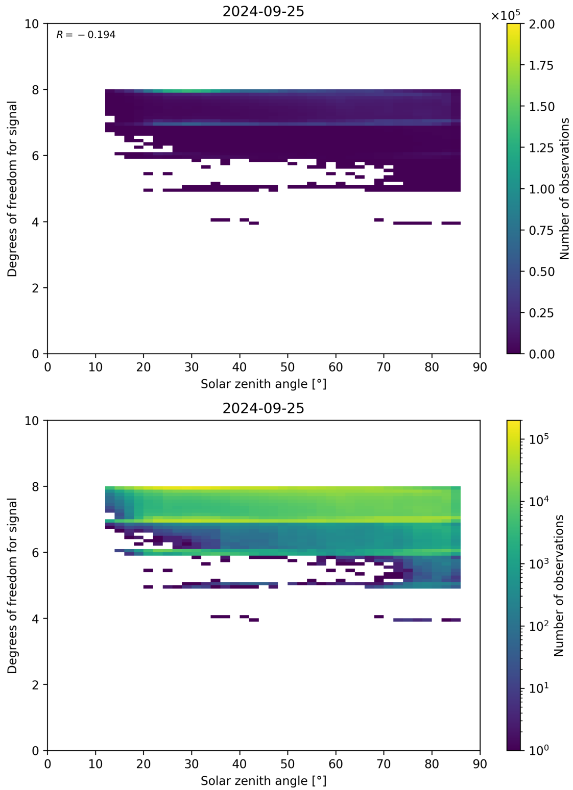
Figure 65: Scatter density plot of “Solar zenith angle” against “Degrees of freedom for signal” for 2024-09-24 to 2024-09-26.
