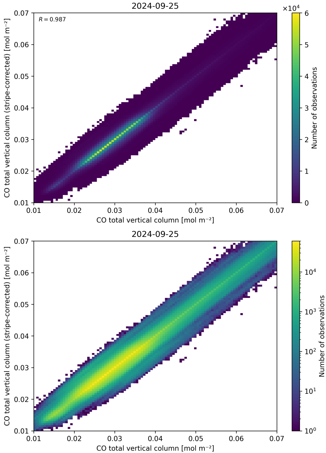
Figure 33: Scatter density plot of “CO total vertical column” against “CO total vertical column (stripe-corrected)” for 2024-09-24 to 2024-09-26.
