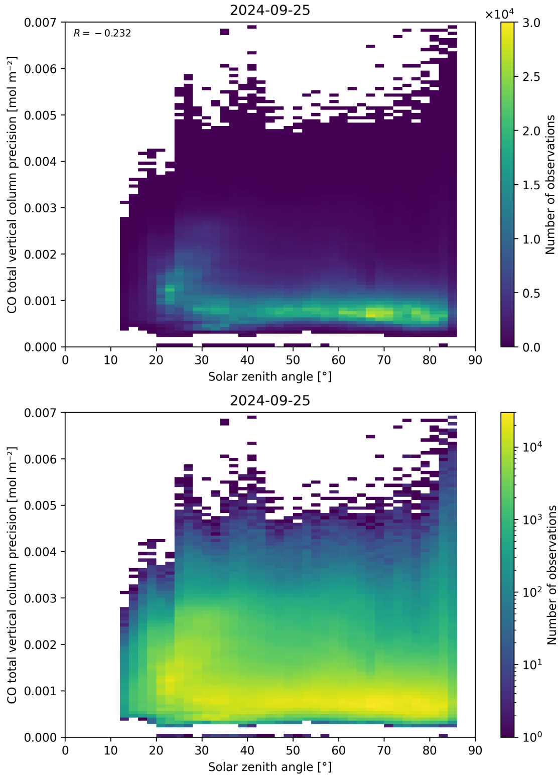
Figure 63: Scatter density plot of “Solar zenith angle” against “CO total vertical column precision” for 2024-09-24 to 2024-09-26.
