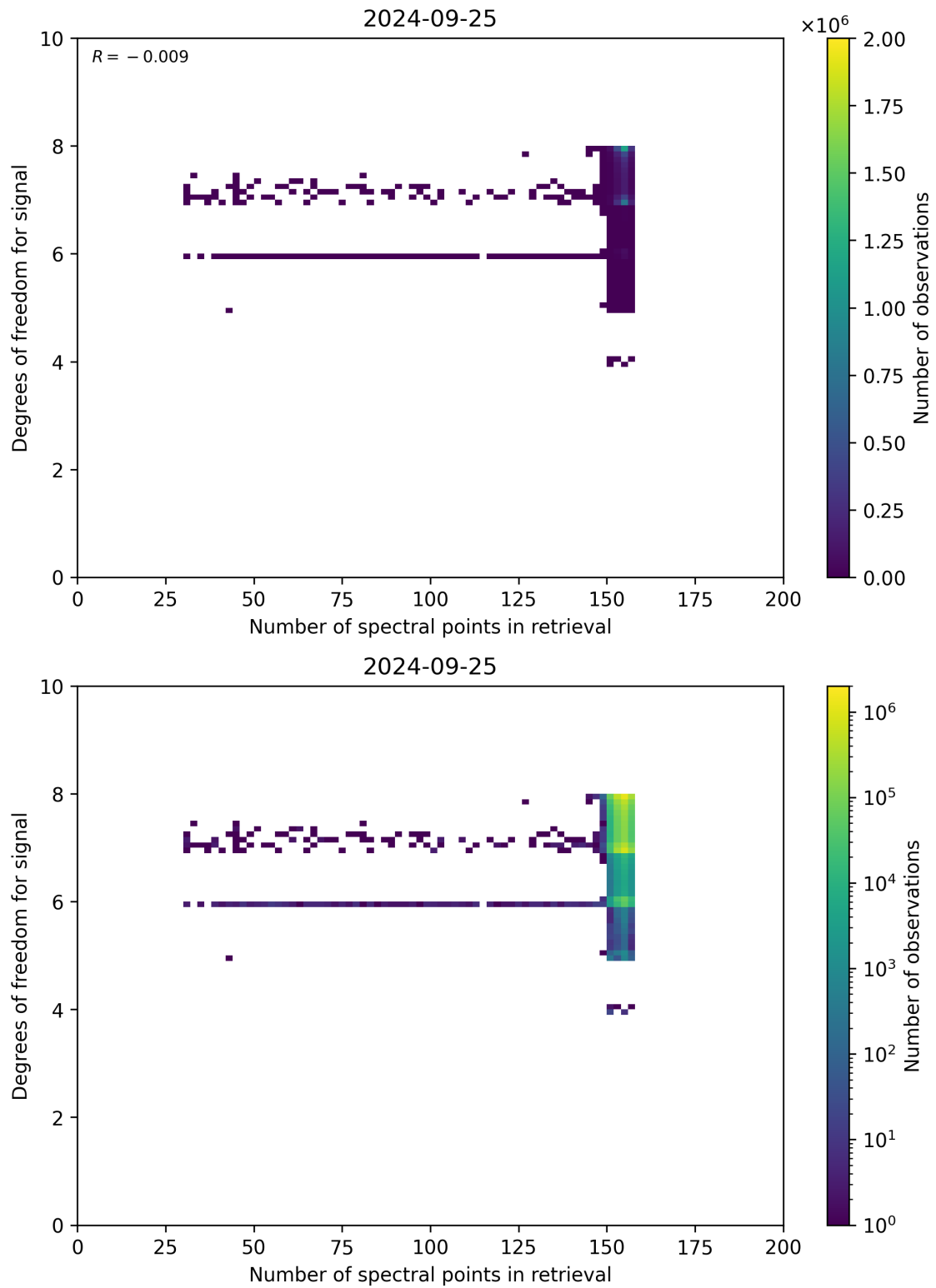
Figure 59: Scatter density plot of “Number of spectral points in retrieval” against “Degrees of freedom for signal” for 2024-09-24 to 2024-09-26.
