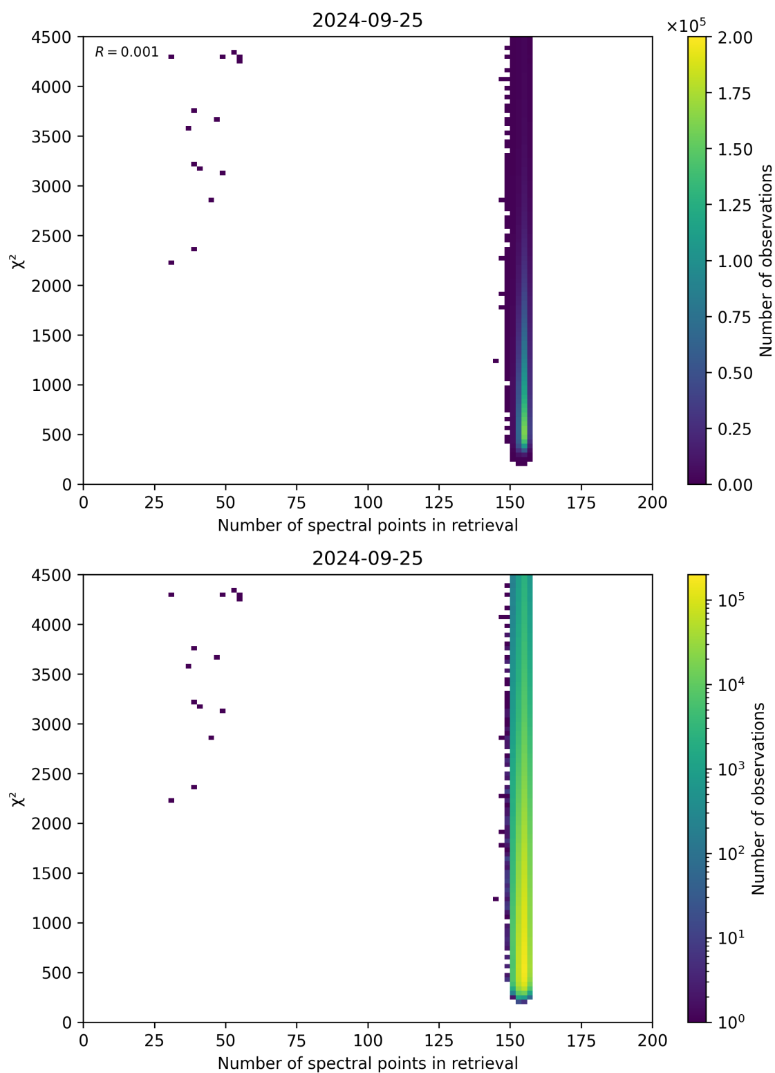
Figure 58: Scatter density plot of “Number of spectral points in retrieval” against “ \chi^2 ” for 2024-09-24 to 2024-09-26.
