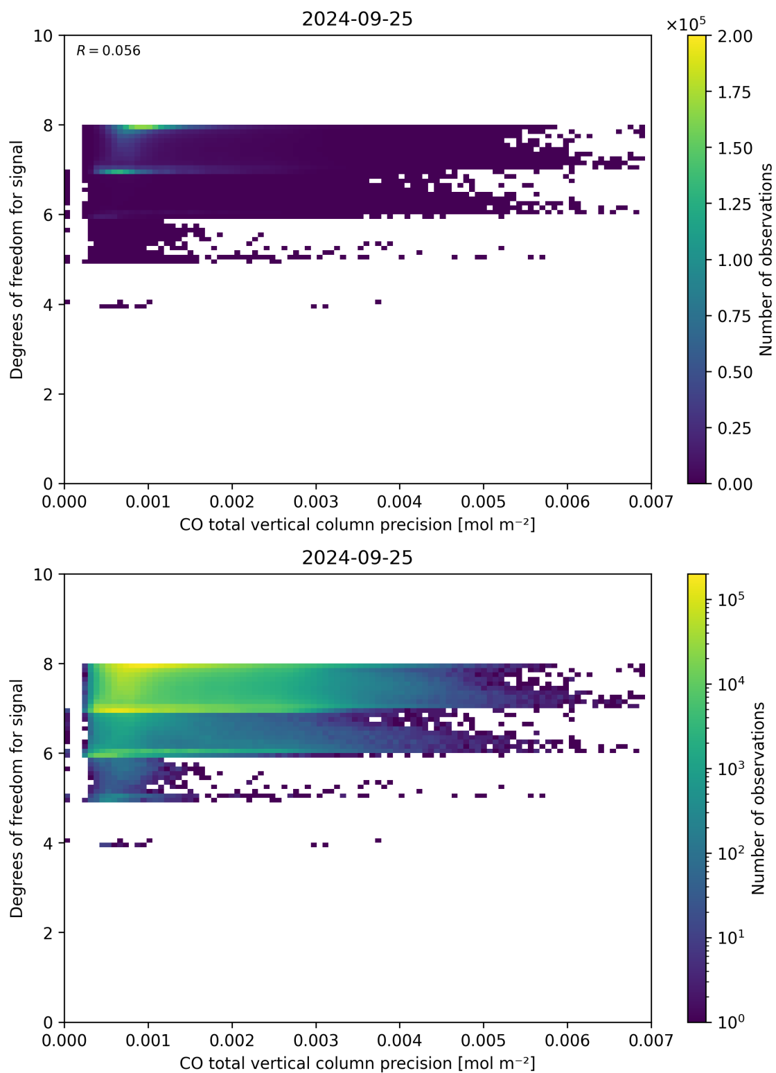
Figure 45: Scatter density plot of “CO total vertical column precision” against “Degrees of freedom for signal” for 2024-09-24 to 2024-09-26.
