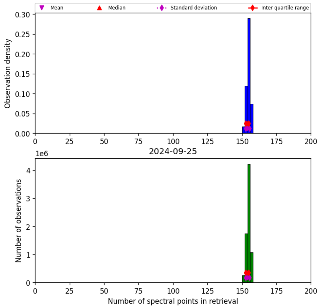
Figure 21: Histogram of “Number of spectral points in retrieval” for 2024-09-24 to 2024-09-26
