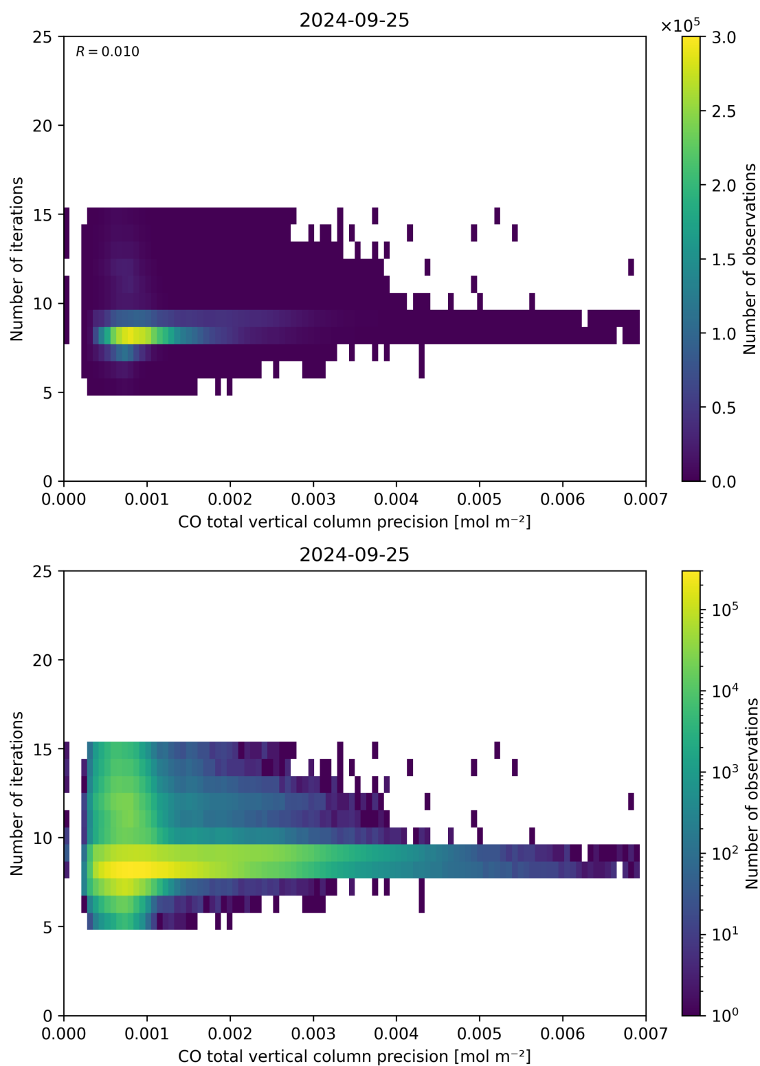
Figure 46: Scatter density plot of “CO total vertical column precision” against “Number of iterations” for 2024-09-24 to 2024-09-26.
