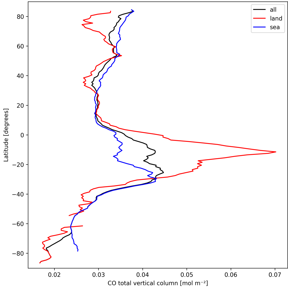
Figure 10: Zonal average of “CO total vertical column” for 2024-09-24 to 2024-09-26.
