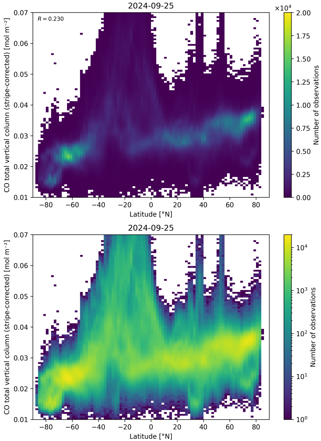
Figure 52: Scatter density plot of “Latitude” against “CO total vertical column (stripe-corrected)” for 2024-09-24 to 2024-09-26.
