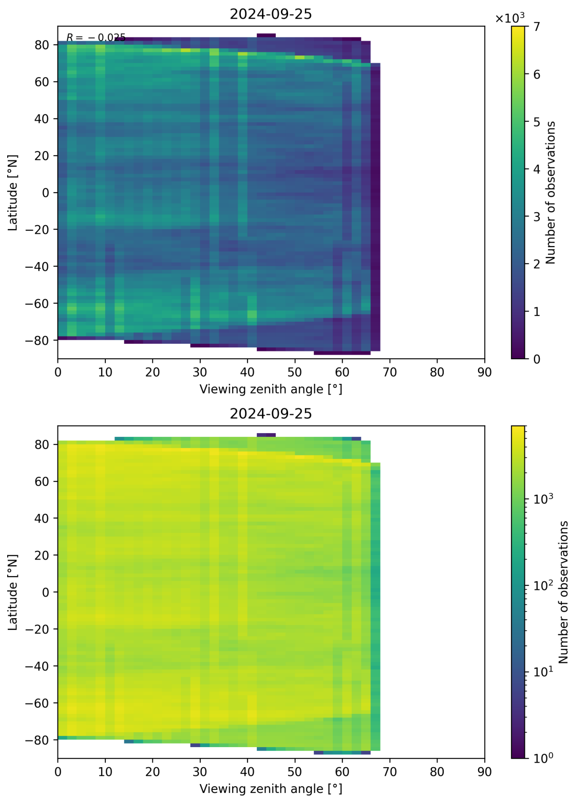
Figure 74: Scatter density plot of “Viewing zenith angle” against “Latitude” for 2024-09-24 to 2024-09-26.
