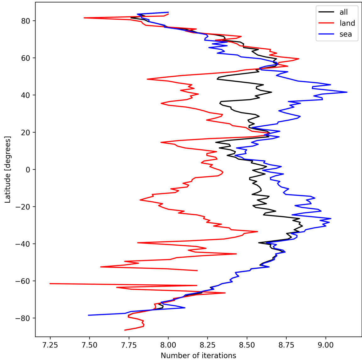
Figure 16: Zonal average of “Number of iterations” for 2024-09-24 to 2024-09-26.
