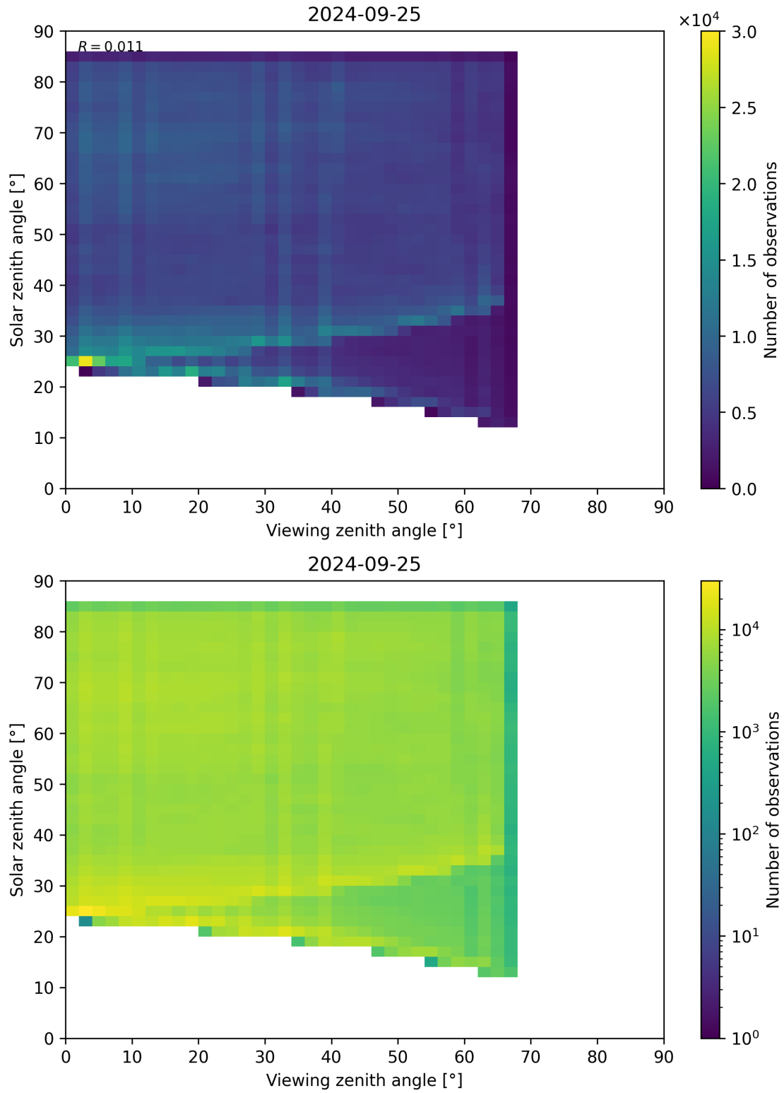
Figure 77: Scatter density plot of “Viewing zenith angle” against “Solar zenith angle” for 2024-09-24 to 2024-09-26.
