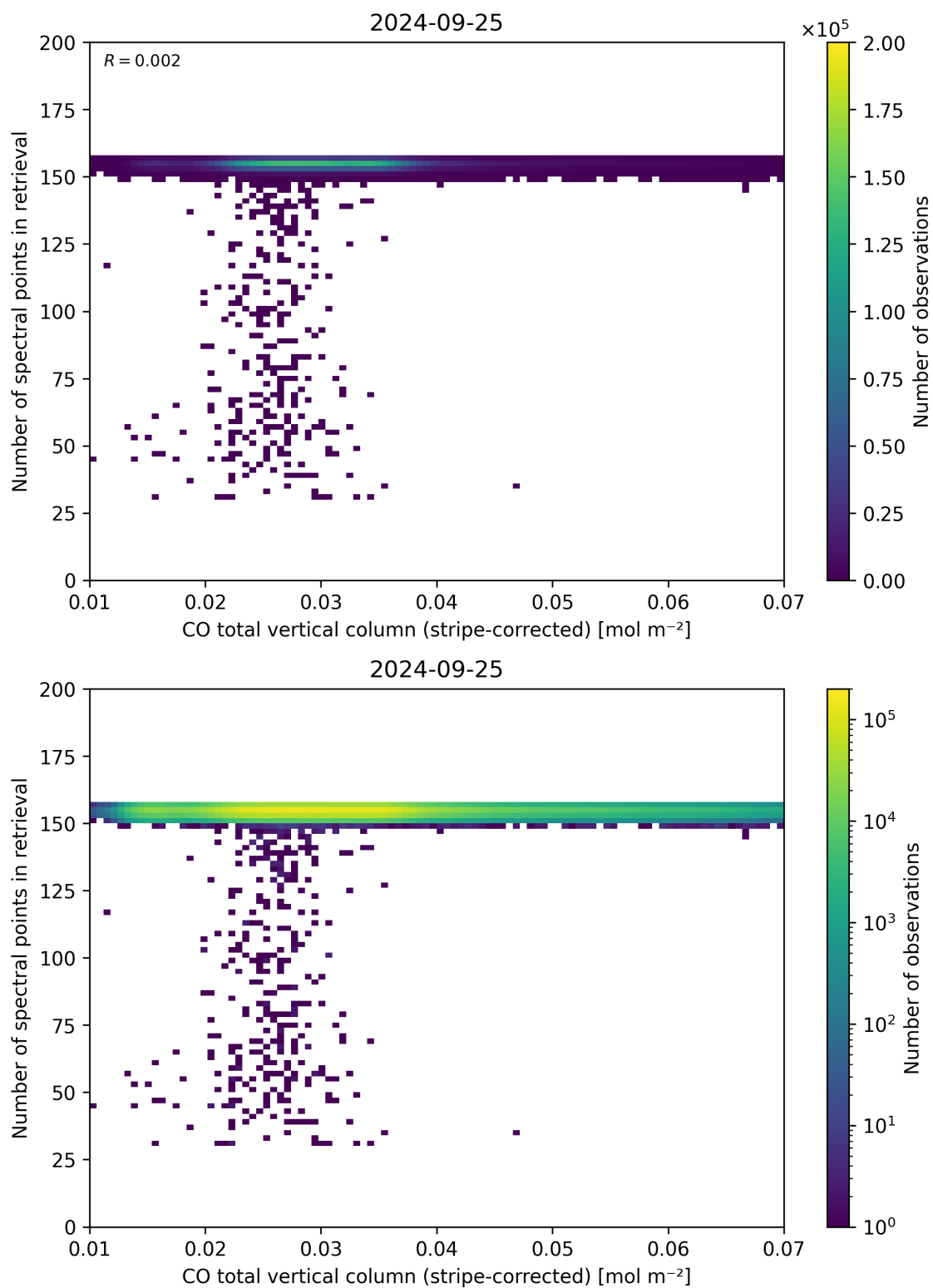
Figure 40: Scatter density plot of “CO total vertical column (stripe-corrected)” against “Number of spectral points in retrieval” for 2024-09-24 to 2024-09-26.
