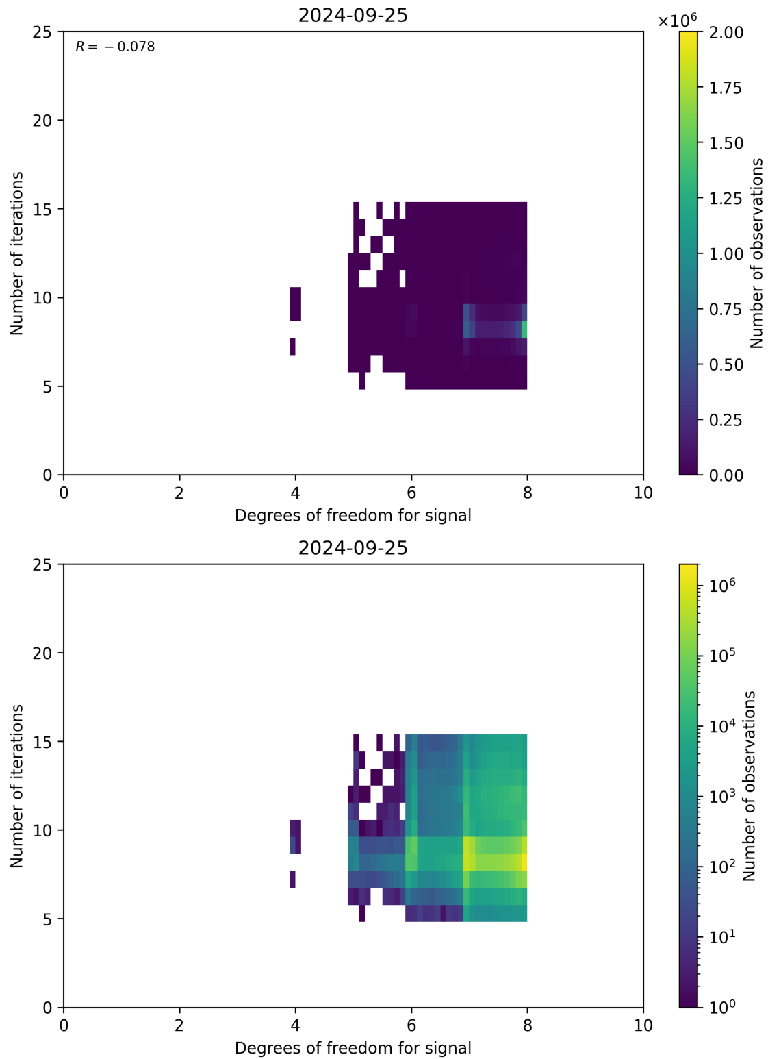
Figure 50: Scatter density plot of “Degrees of freedom for signal” against “Number of iterations” for 2024-09-24 to 2024-09-26.
