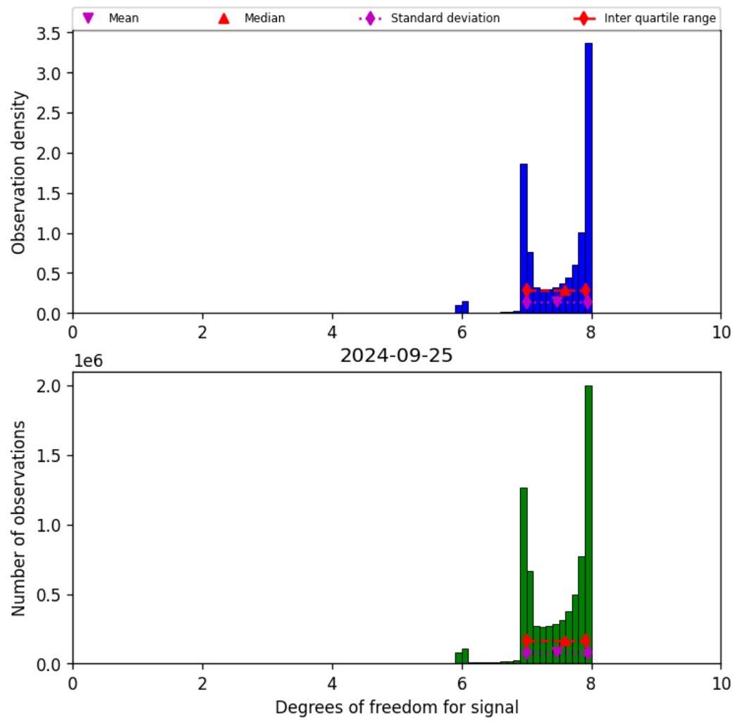
Figure 23: Histogram of “Degrees of freedom for signal” for 2024-09-24 to 2024-09-26
