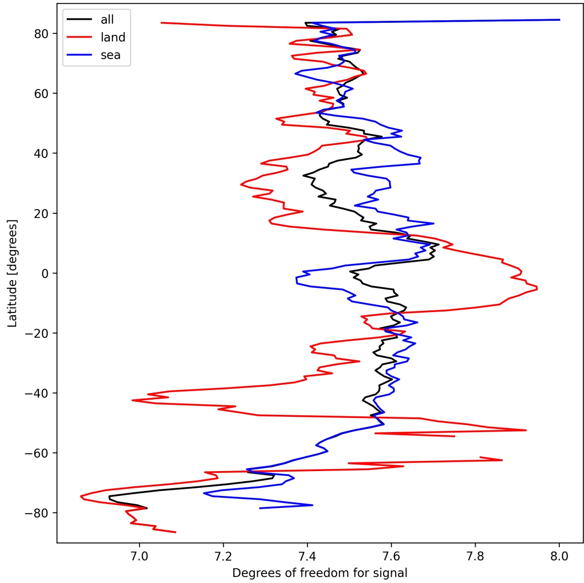
Figure 15: Zonal average of “Degrees of freedom for signal” for 2024-09-24 to 2024-09-26.
