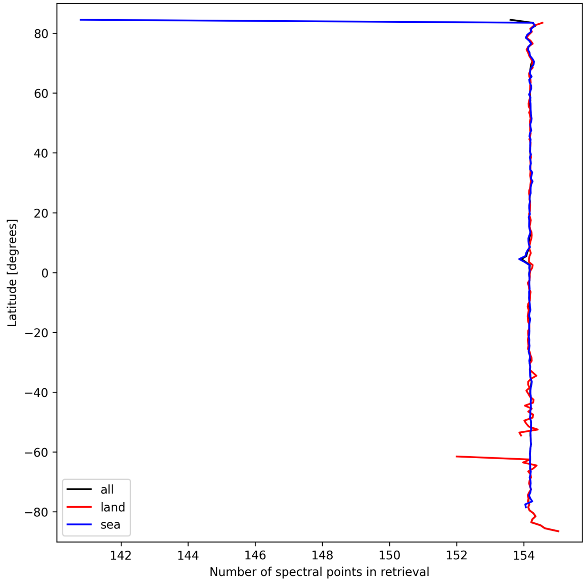
Figure 13: Zonal average of “Number of spectral points in retrieval” for 2024-09-24 to 2024-09-26.
