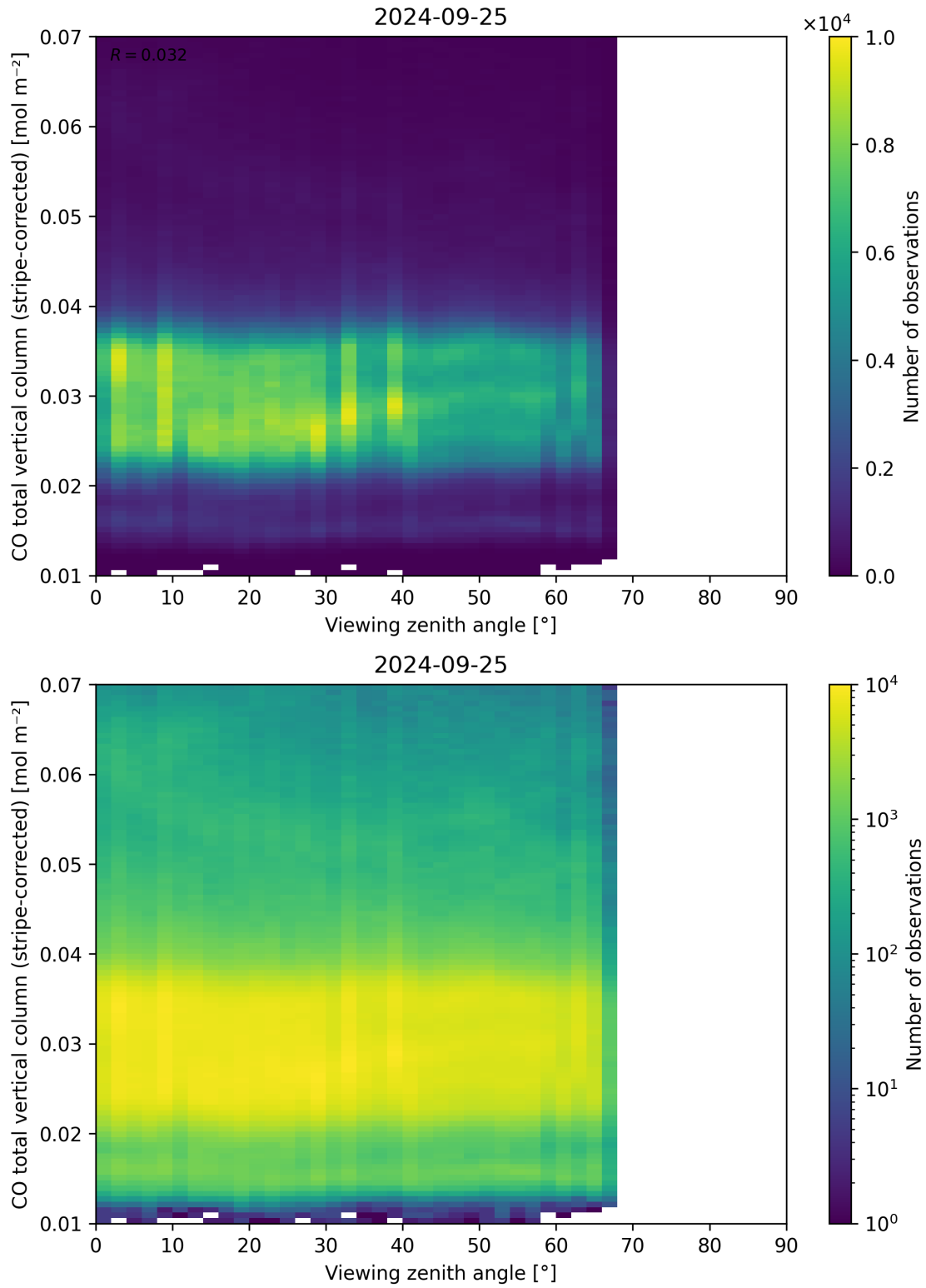
Figure 70: Scatter density plot of “Viewing zenith angle” against “CO total vertical column (stripe-corrected)” for 2024-09-24 to 2024-09-26.
