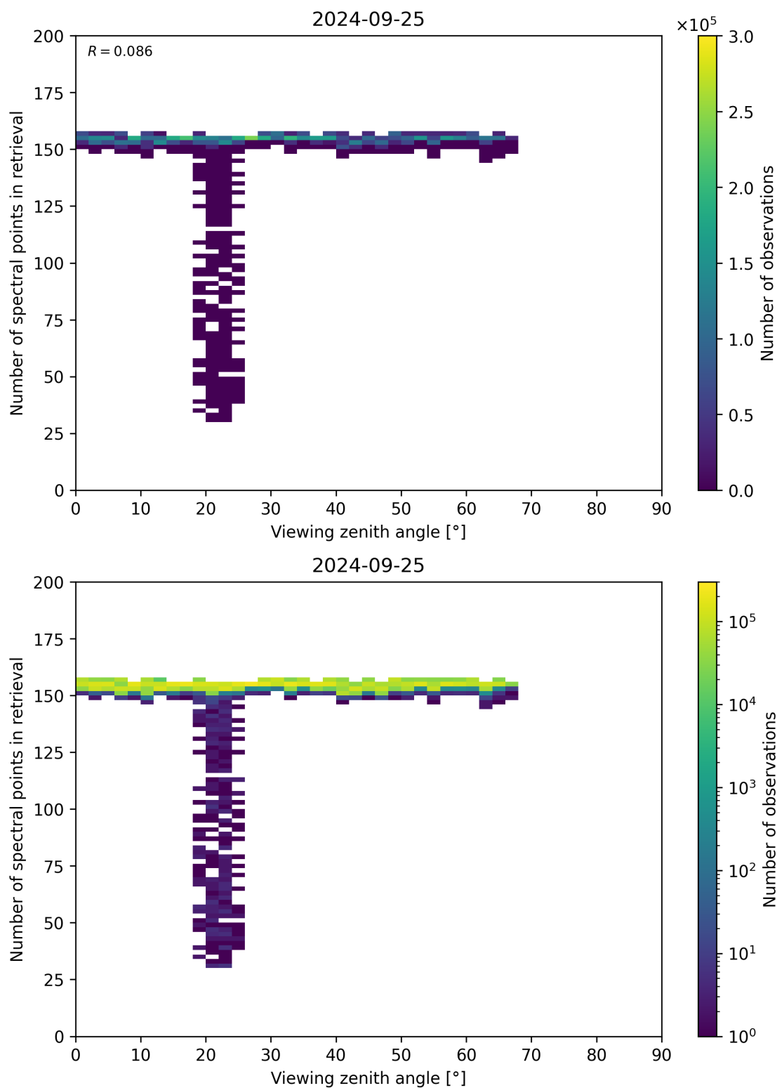
Figure 76: Scatter density plot of “Viewing zenith angle” against “Number of spectral points in retrieval” for 2024-09-24 to 2024-09-26.
