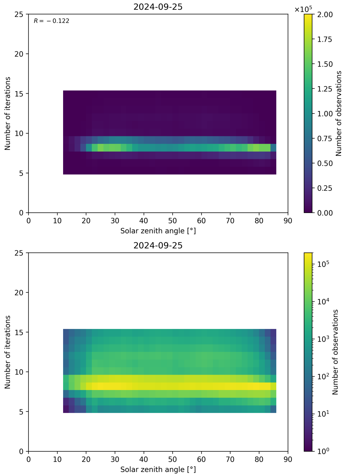
Figure 67: Scatter density plot of “Solar zenith angle” against “Number of iterations” for 2024-09-24 to 2024-09-26.
