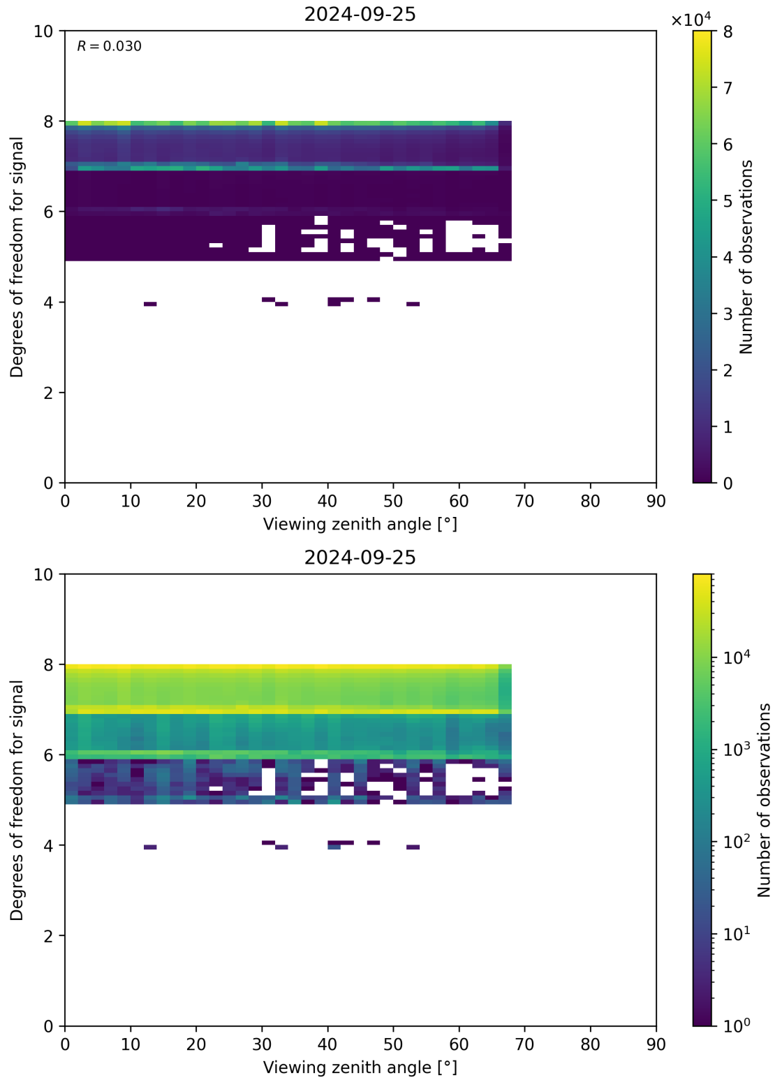
Figure 73: Scatter density plot of “Viewing zenith angle” against “Degrees of freedom for signal” for 2024-09-24 to 2024-09-26.
