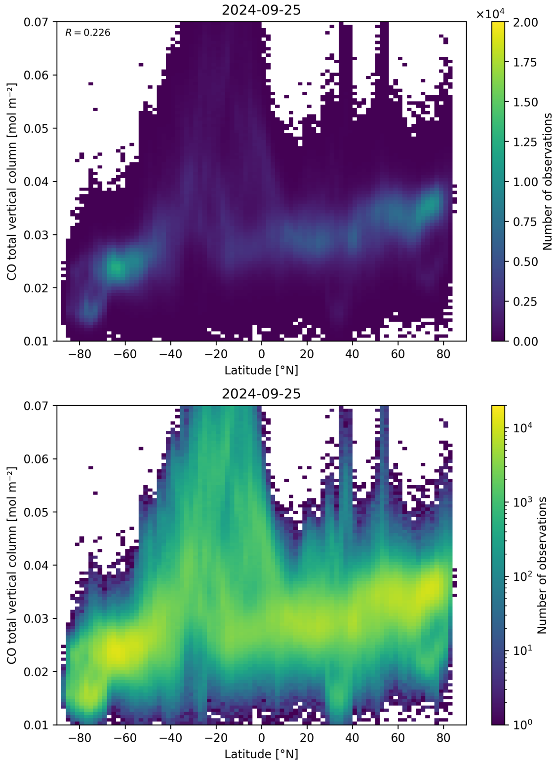
Figure 51: Scatter density plot of “Latitude” against “CO total vertical column” for 2024-09-24 to 2024-09-26.
