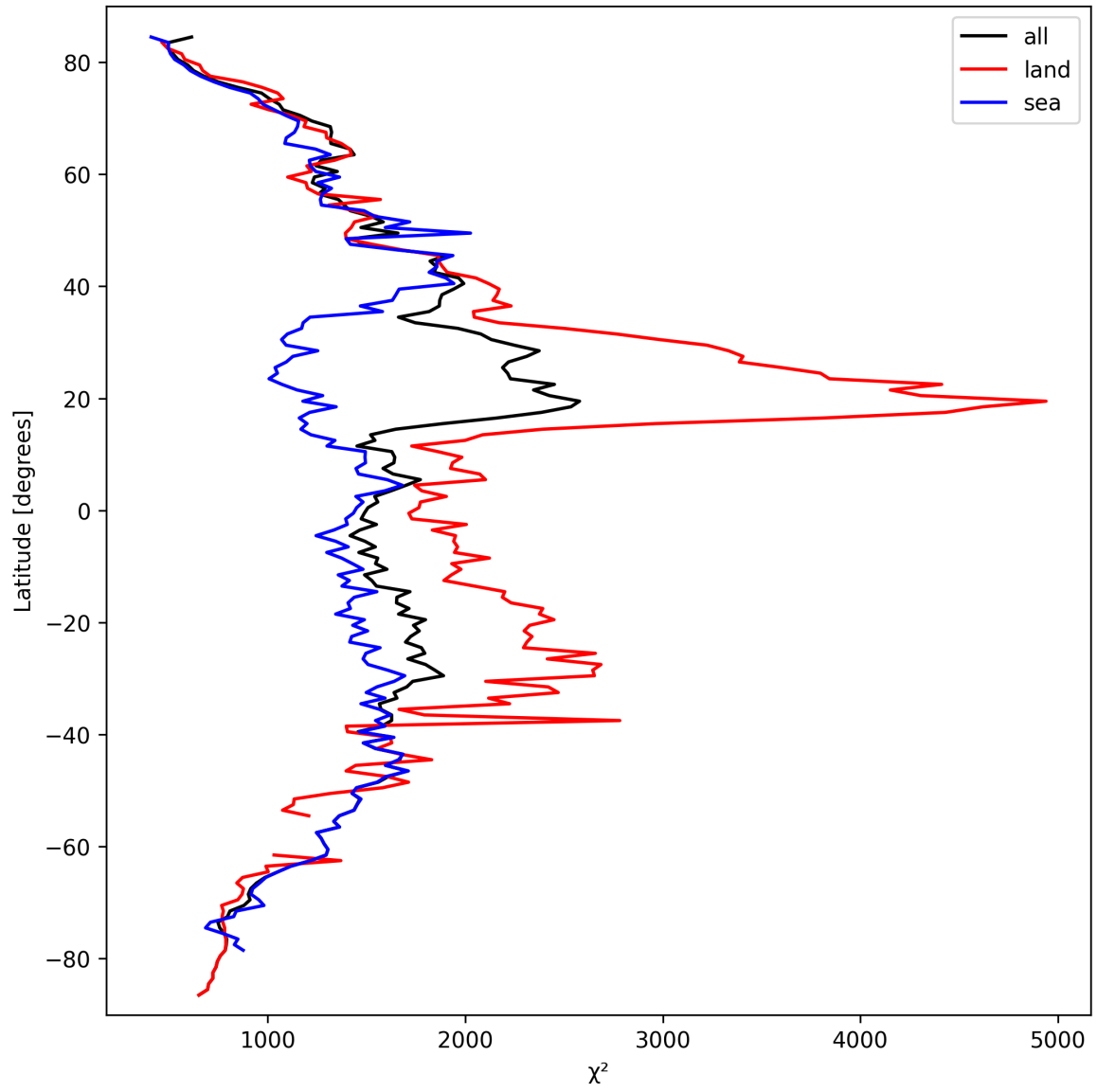
Figure 14: Zonal average of “ \chi^2 ” for 2024-09-24 to 2024-09-26.
