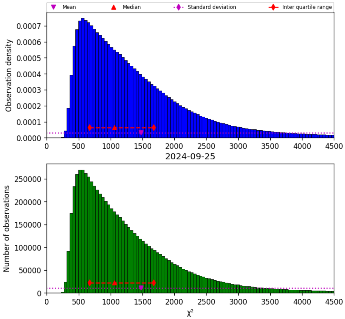
Figure 22: Histogram of “ \chi^2 ” for 2024-09-24 to 2024-09-26
