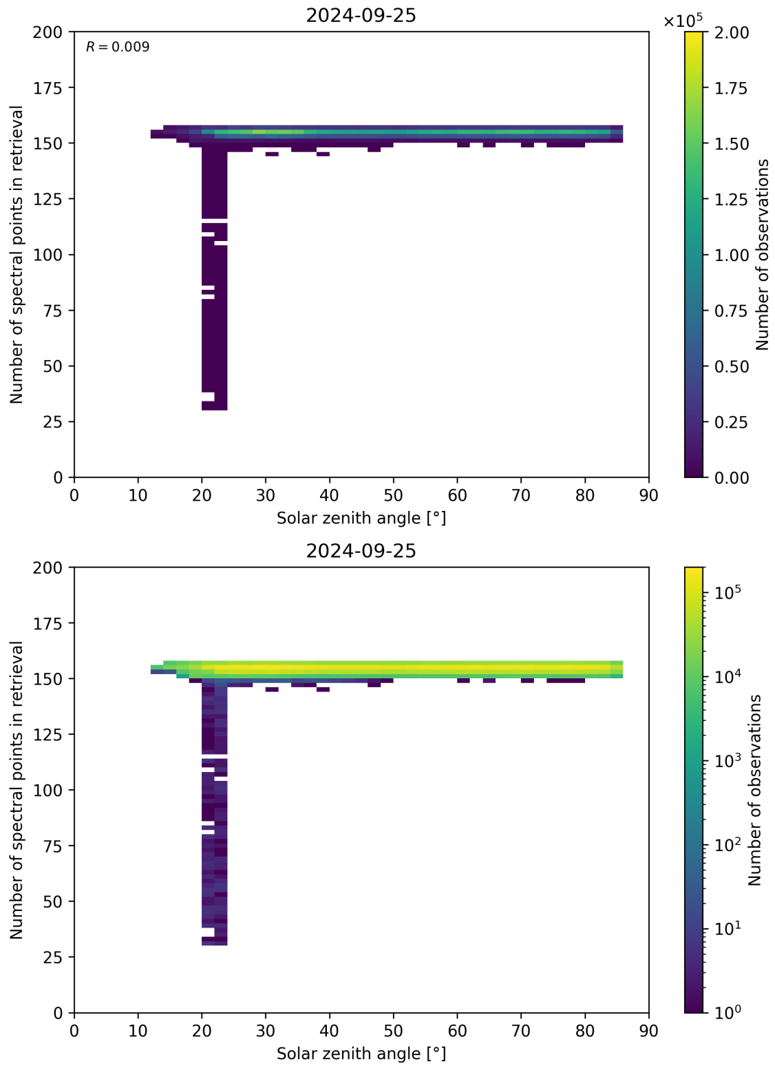
Figure 68: Scatter density plot of “Solar zenith angle” against “Number of spectral points in retrieval” for 2024-09-24 to 2024-09-26.
