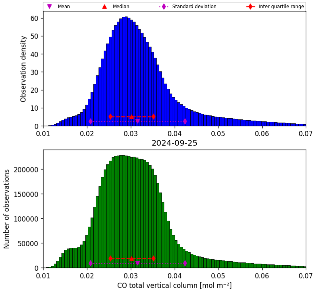
Figure 18: Histogram of “CO total vertical column” for 2024-09-24 to 2024-09-26
