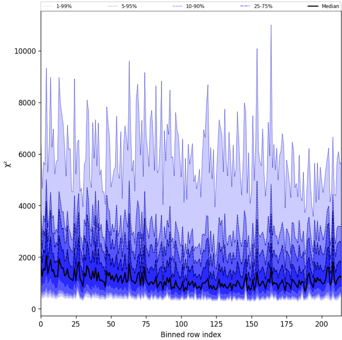
Figure 30: Along track statistics of “ \chi^2 ” for 2024-09-24 to 2024-09-26
