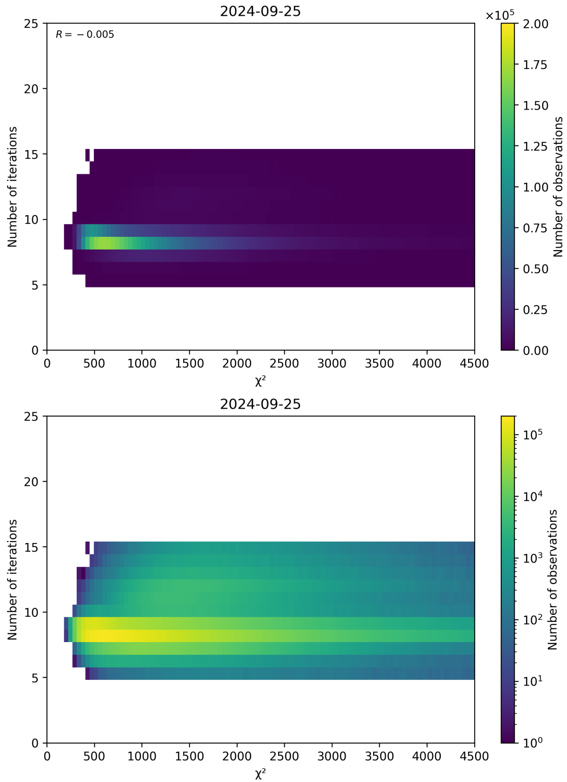
Figure 49: Scatter density plot of “ \chi^2 ” against “Number of iterations” for 2024-09-24 to 2024-09-26.
