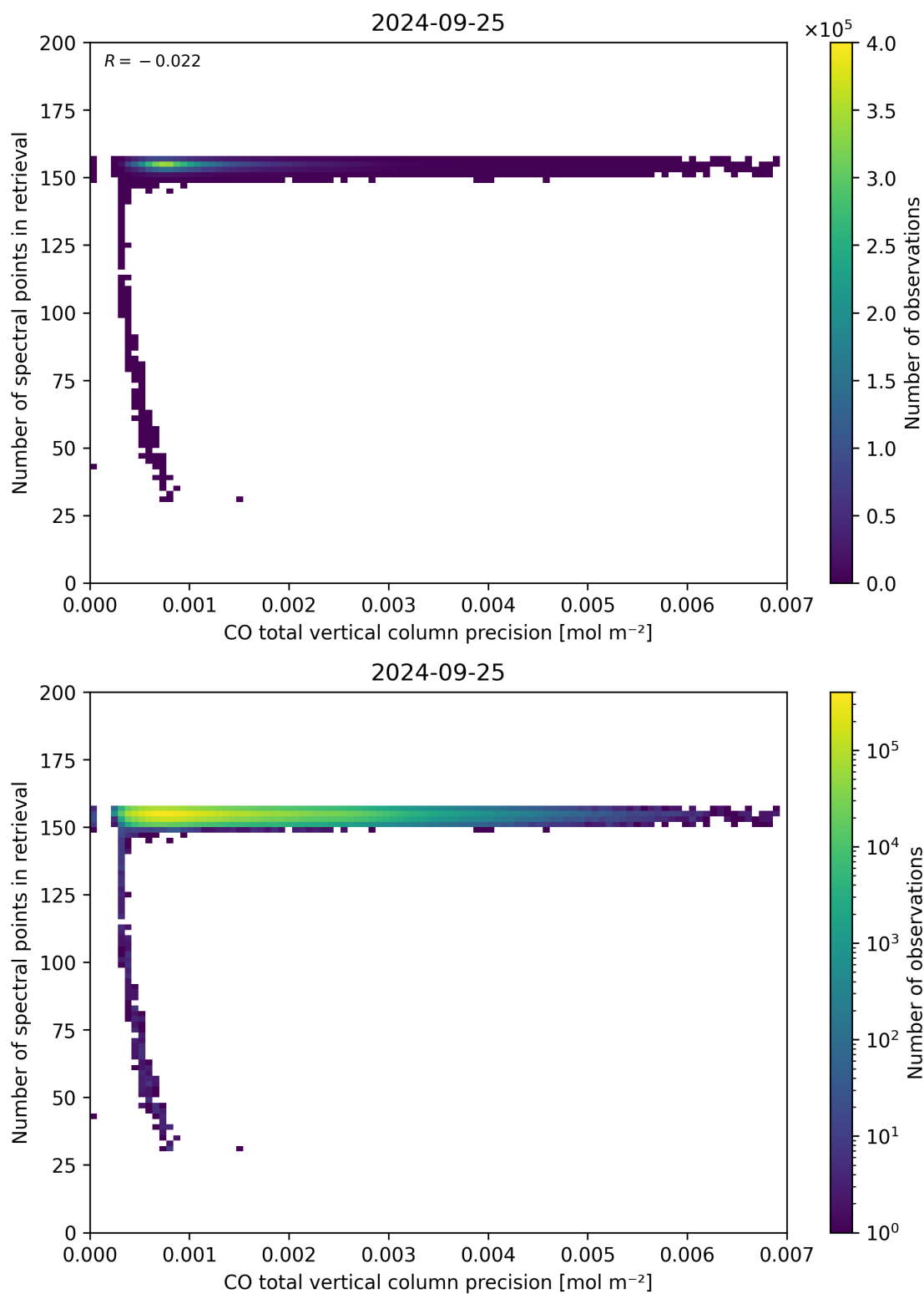
Figure 47: Scatter density plot of “CO total vertical column precision” against “Number of spectral points in retrieval” for 2024-09-24 to 2024-09-26.
