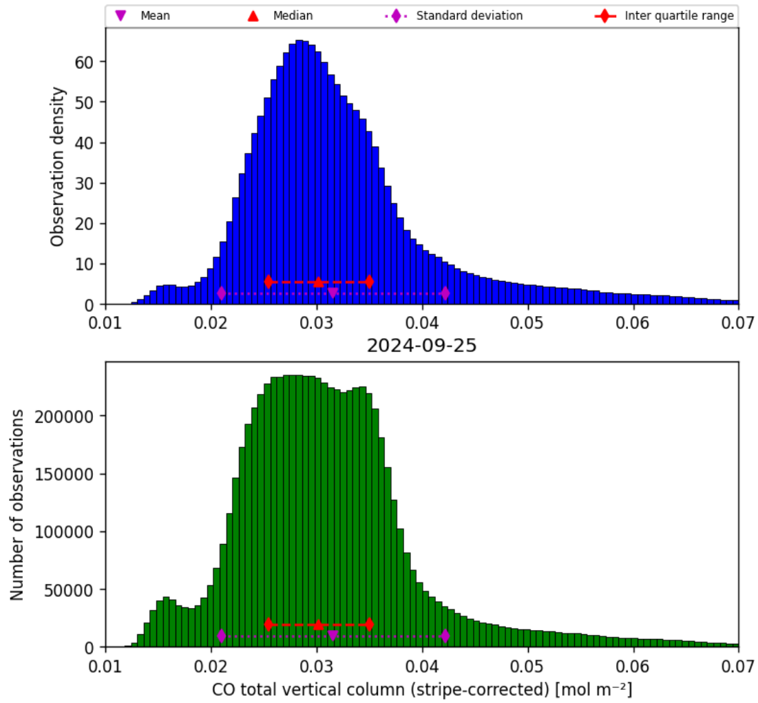
Figure 19: Histogram of “CO total vertical column (stripe-corrected)” for 2024-09-24 to 2024-09-26
