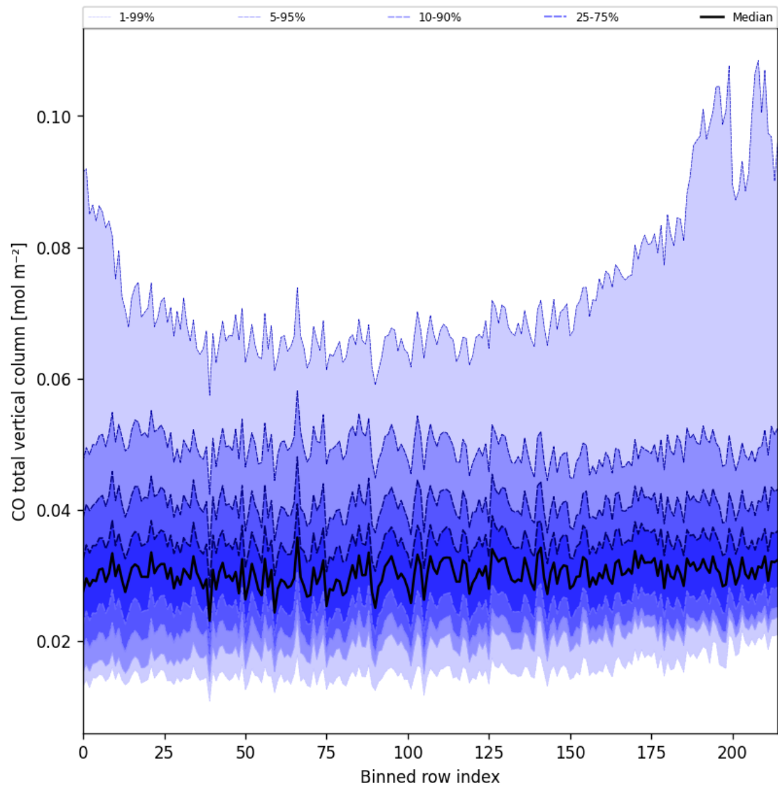
Figure 26: Along track statistics of “CO total vertical column” for 2024-09-24 to 2024-09-26
