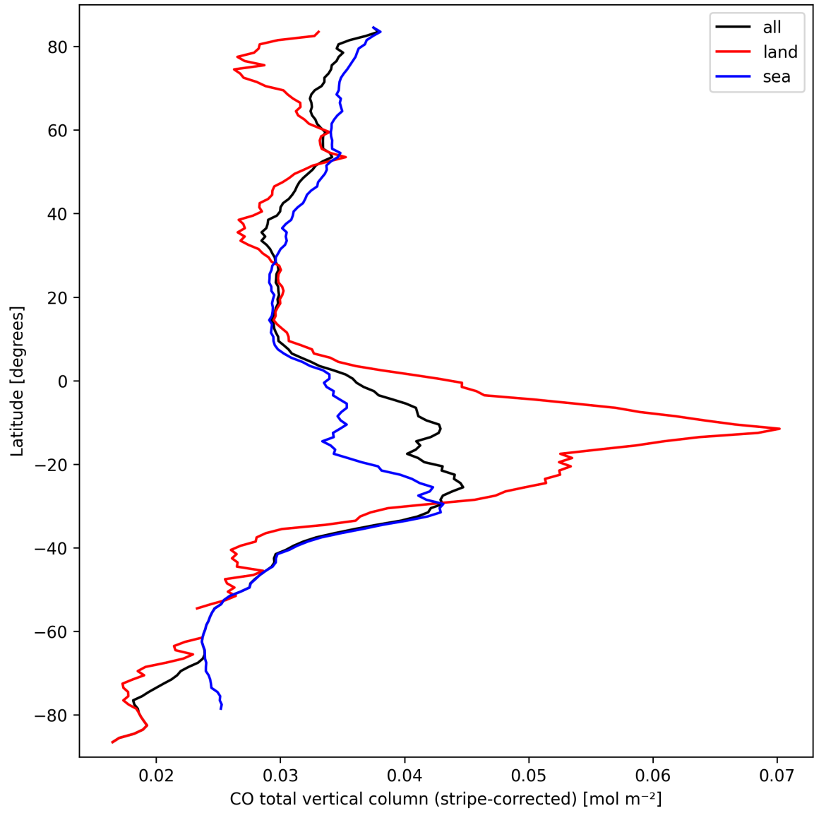
Figure 11: Zonal average of “CO total vertical column (stripe-corrected)” for 2024-09-24 to 2024-09-26.
