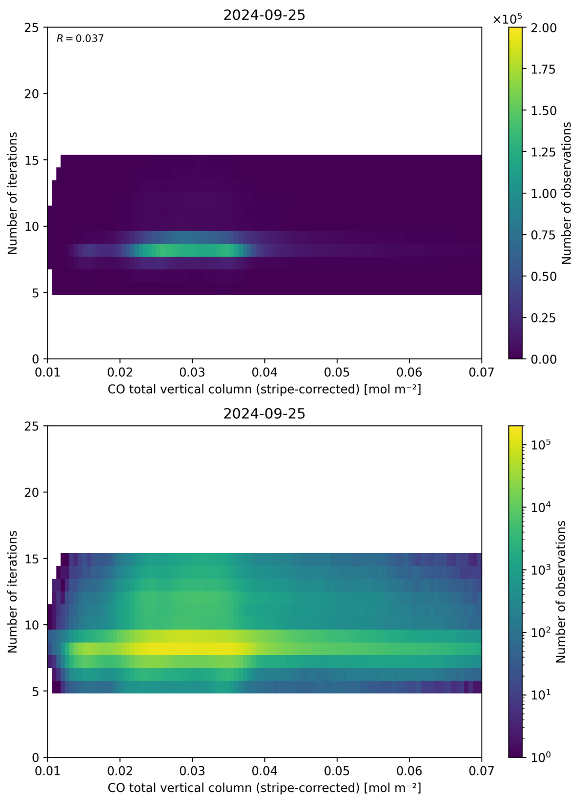
Figure 39: Scatter density plot of “CO total vertical column (stripe-corrected)” against “Number of iterations” for 2024-09-24 to 2024-09-26.
