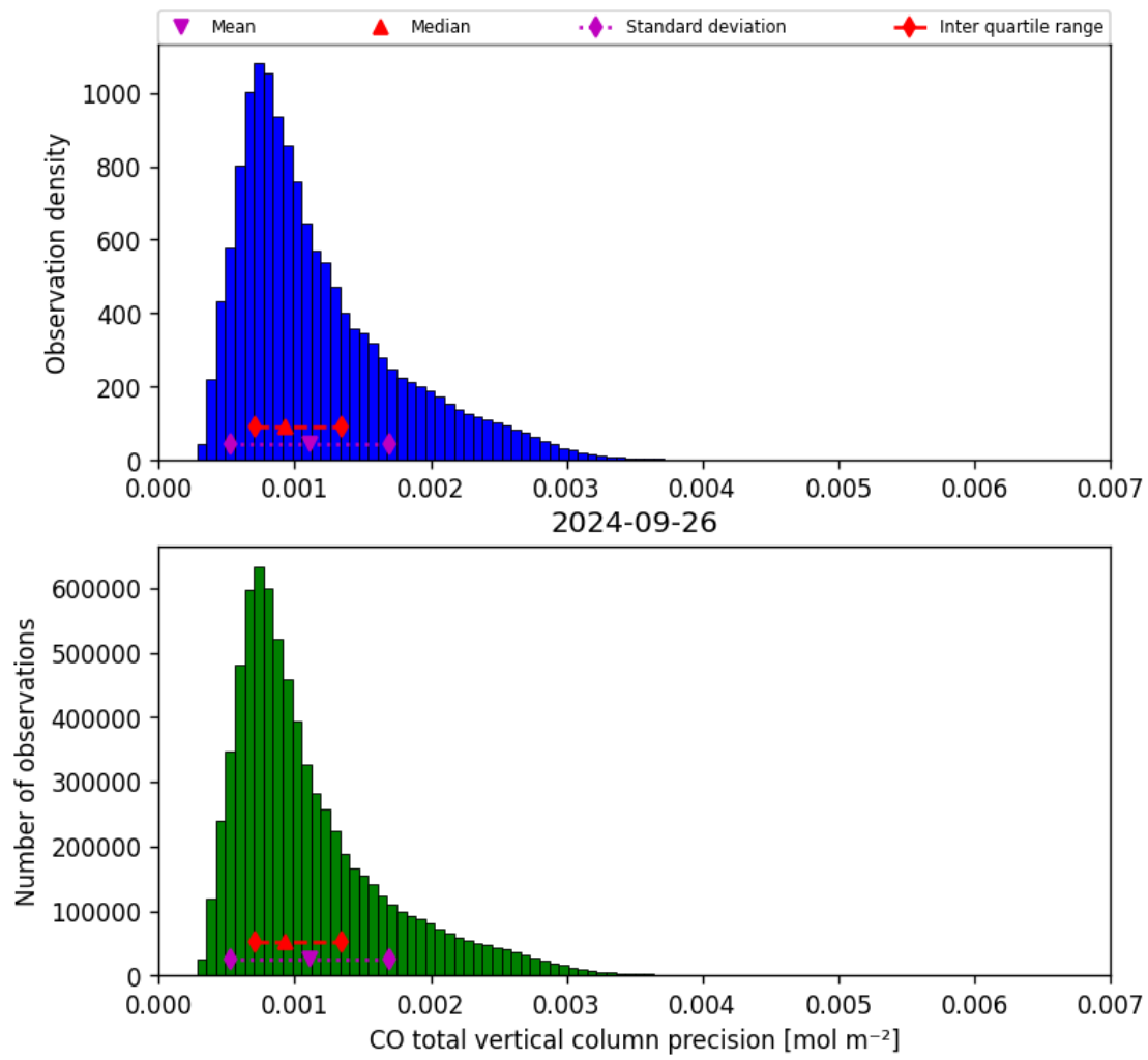
Figure 20: Histogram of “CO total vertical column precision” for 2024-09-25 to 2024-09-27
