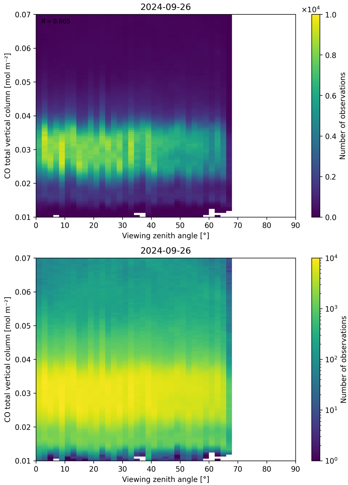
Figure 69: Scatter density plot of “Viewing zenith angle” against “CO total vertical column” for 2024-09-25 to 2024-09-27.
