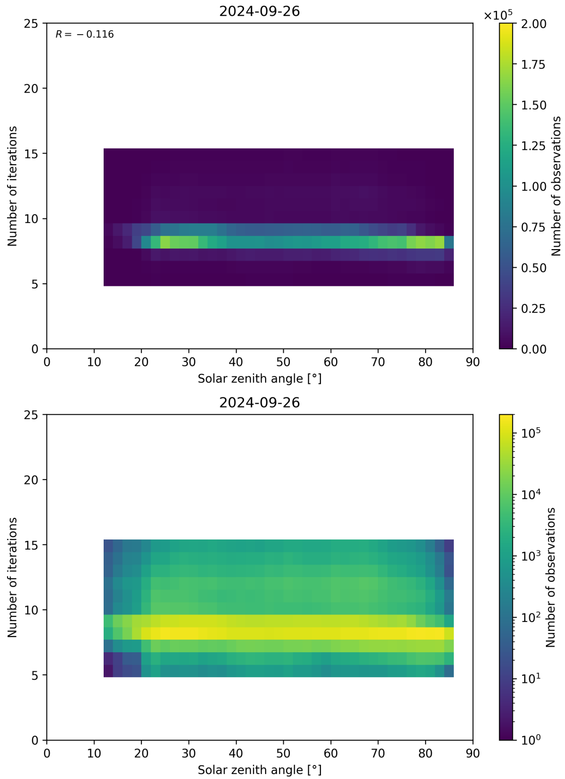
Figure 67: Scatter density plot of “Solar zenith angle” against “Number of iterations” for 2024-09-25 to 2024-09-27.
