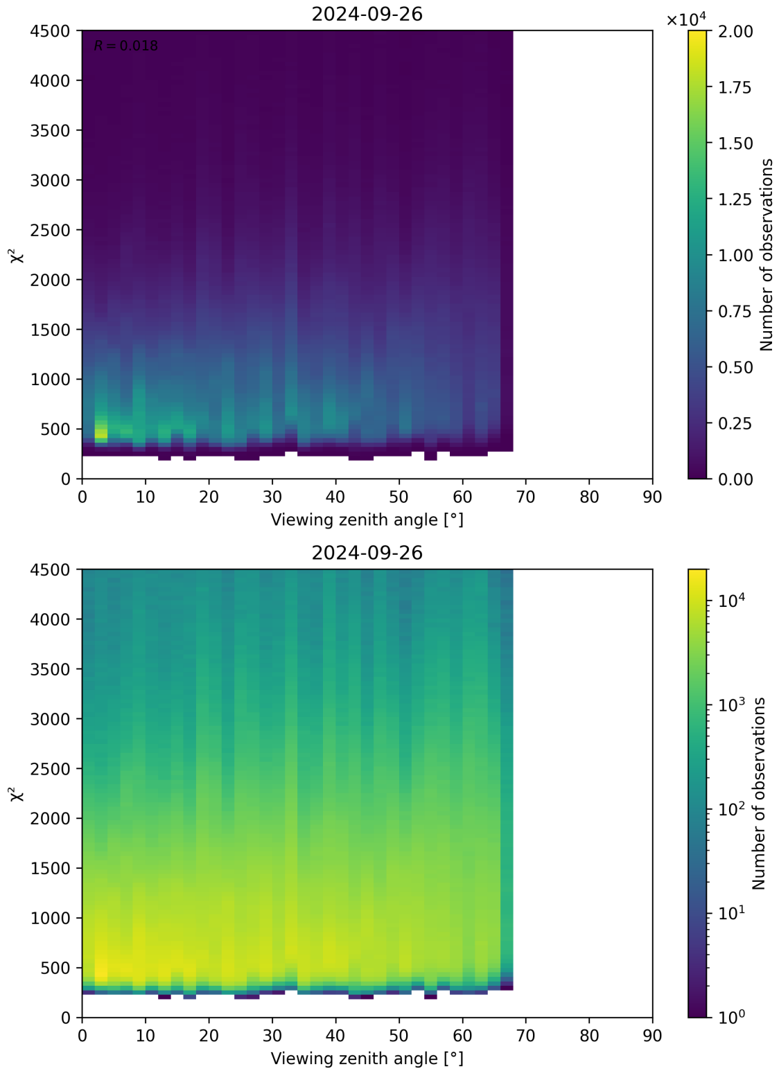
Figure 72: Scatter density plot of “Viewing zenith angle” against “ \chi^2 ” for 2024-09-25 to 2024-09-27.
