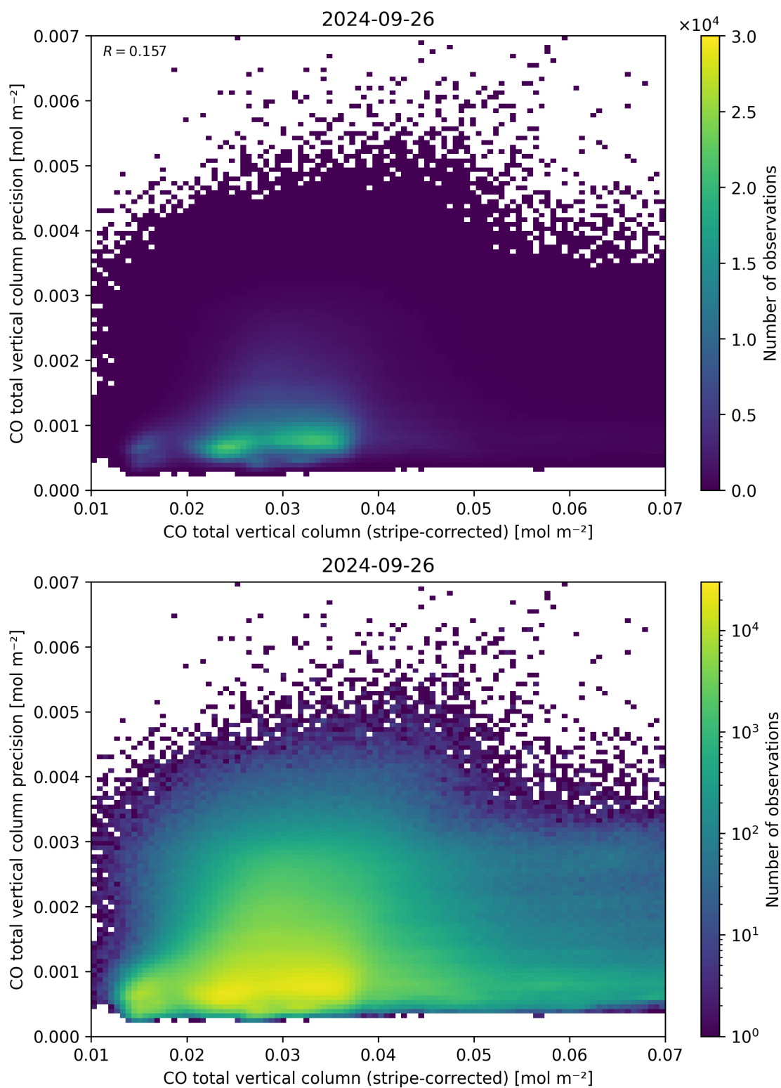
Figure 36: Scatter density plot of “CO total vertical column (stripe-corrected)” against “CO total vertical column precision” for 2024-09-25 to 2024-09-27.
