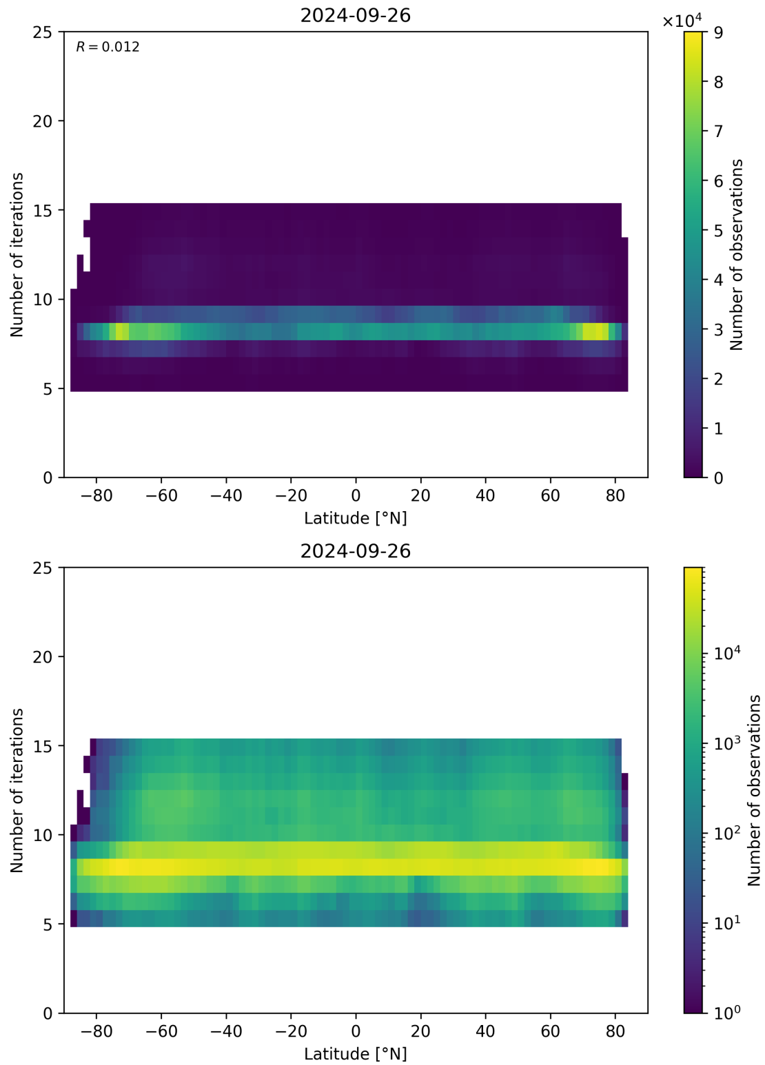
Figure 56: Scatter density plot of “Latitude” against “Number of iterations” for 2024-09-25 to 2024-09-27.
