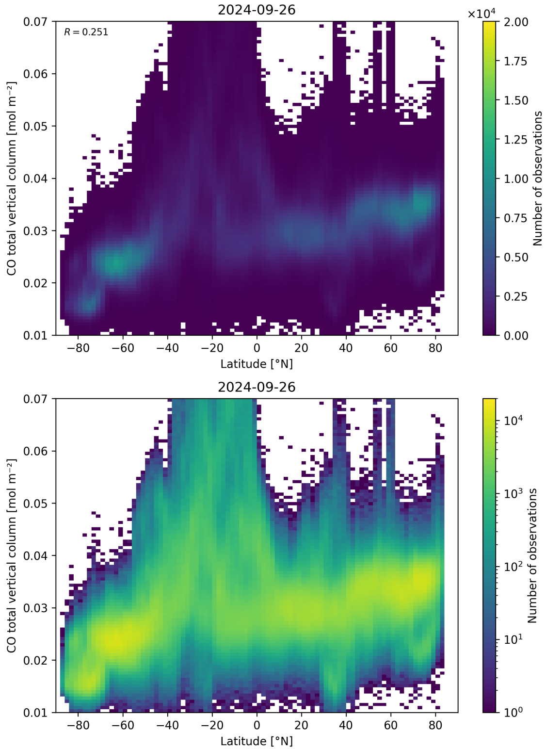
Figure 51: Scatter density plot of “Latitude” against “CO total vertical column” for 2024-09-25 to 2024-09-27.
