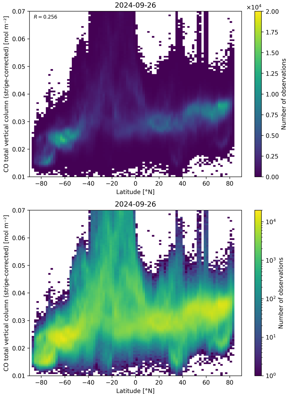
Figure 52: Scatter density plot of “Latitude” against “CO total vertical column (stripe-corrected)” for 2024-09-25 to 2024-09-27.
