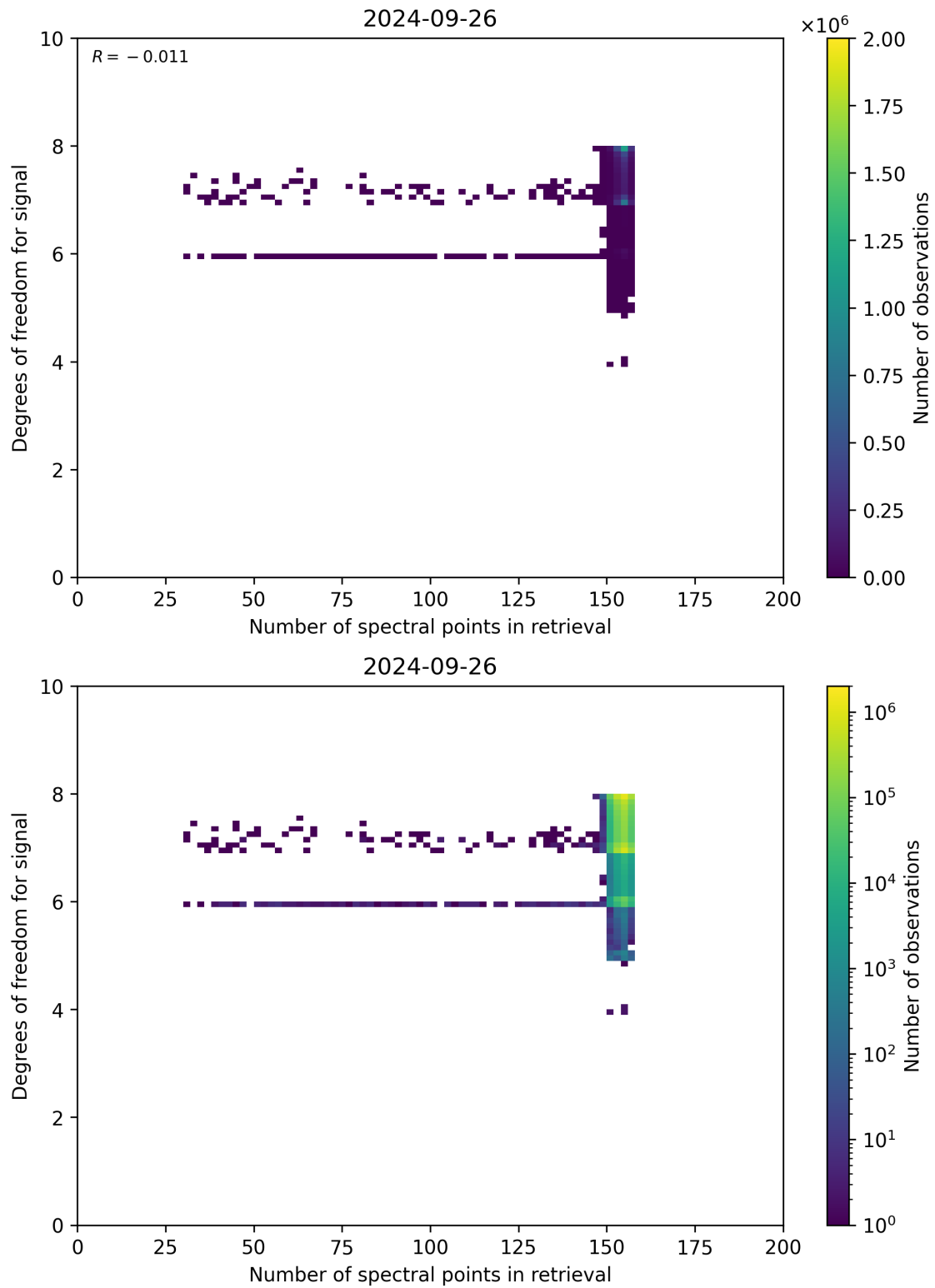
Figure 59: Scatter density plot of “Number of spectral points in retrieval” against “Degrees of freedom for signal” for 2024-09-25 to 2024-09-27.
