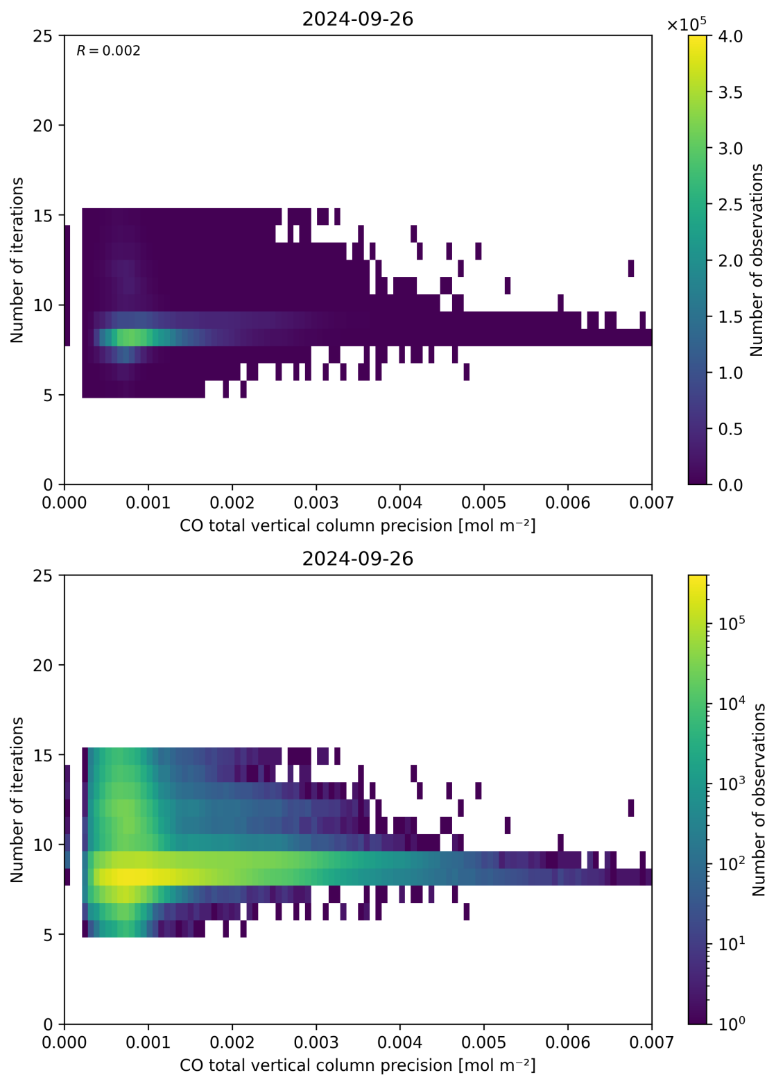
Figure 46: Scatter density plot of “CO total vertical column precision” against “Number of iterations” for 2024-09-25 to 2024-09-27.
