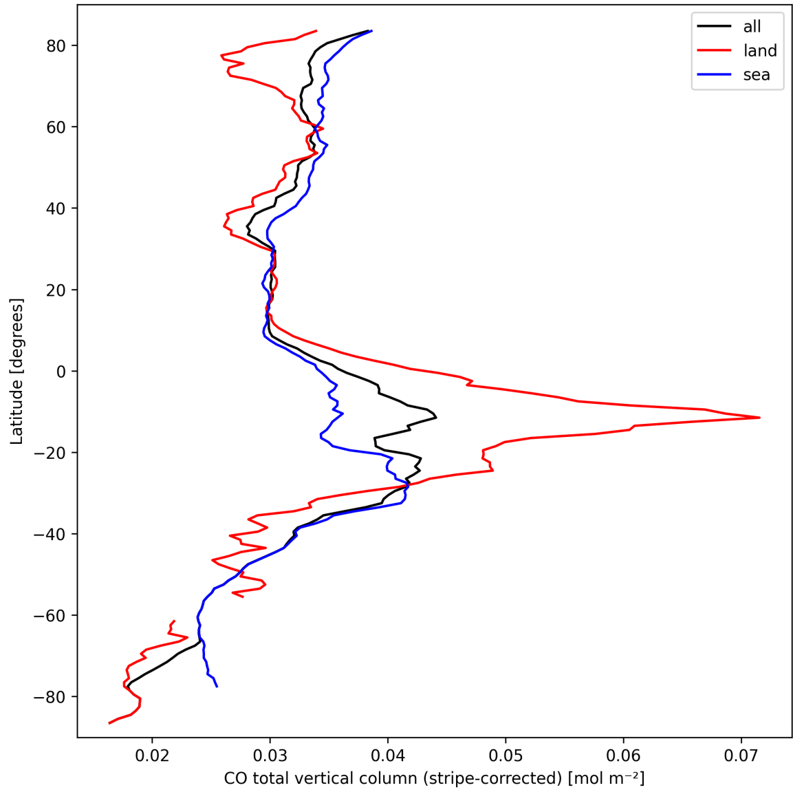
Figure 11: Zonal average of “CO total vertical column (stripe-corrected)” for 2024-09-25 to 2024-09-27.
