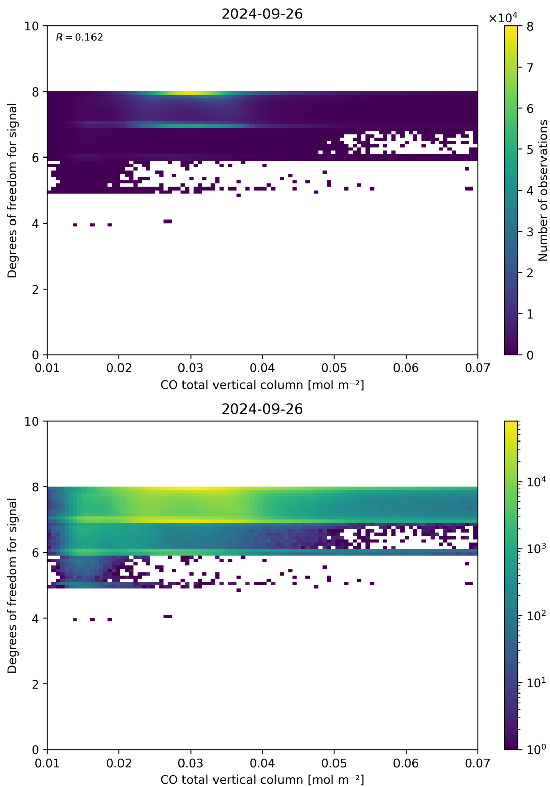
Figure 41: Scatter density plot of “CO total vertical column” against “Degrees of freedom for signal” for 2024-09-25 to 2024-09-27.
