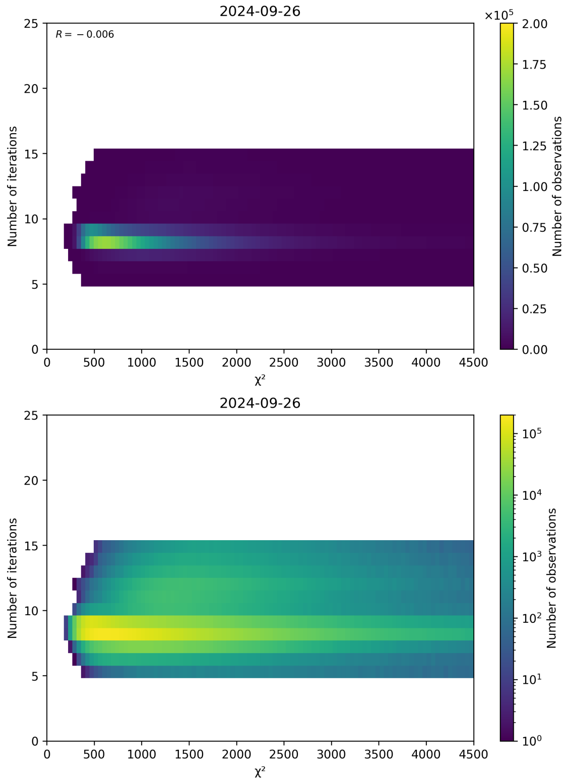
Figure 49: Scatter density plot of “ \chi^2 ” against “Number of iterations” for 2024-09-25 to 2024-09-27.
