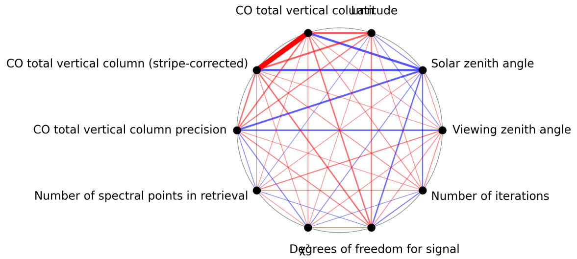
Figure 1: Map of correlation graph for 2024-09-25 to 2024-09-27.
