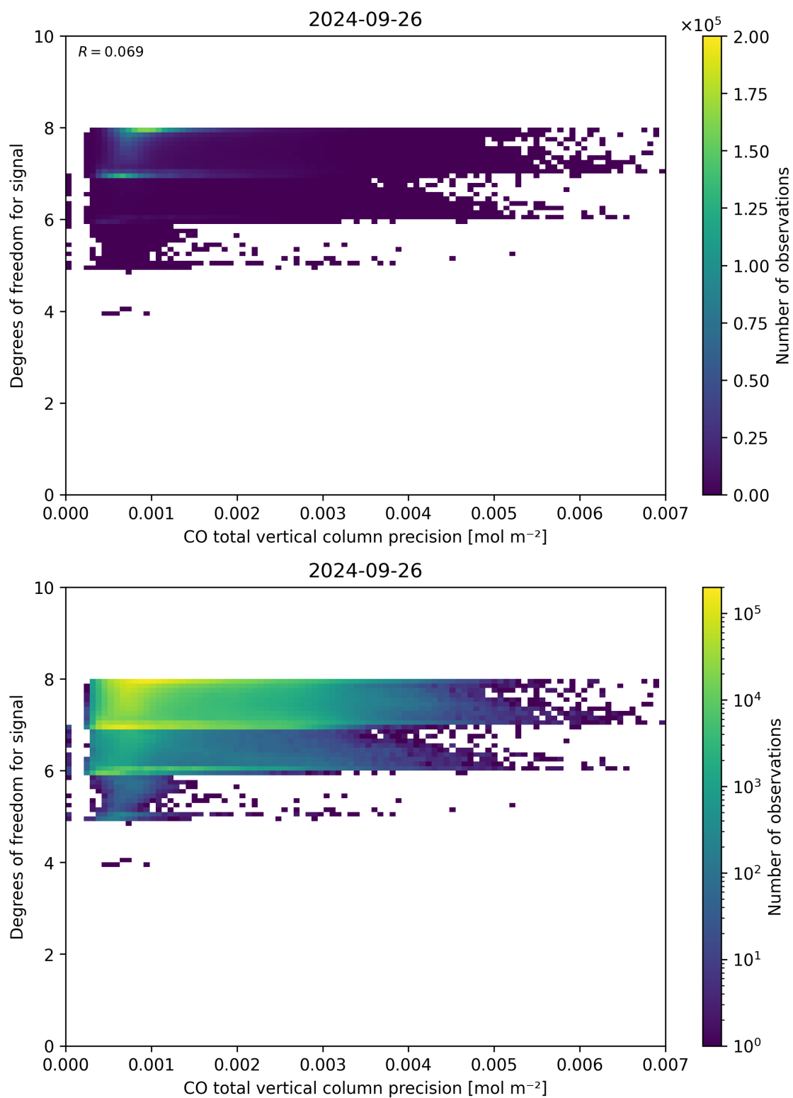
Figure 45: Scatter density plot of “CO total vertical column precision” against “Degrees of freedom for signal” for 2024-09-25 to 2024-09-27.
