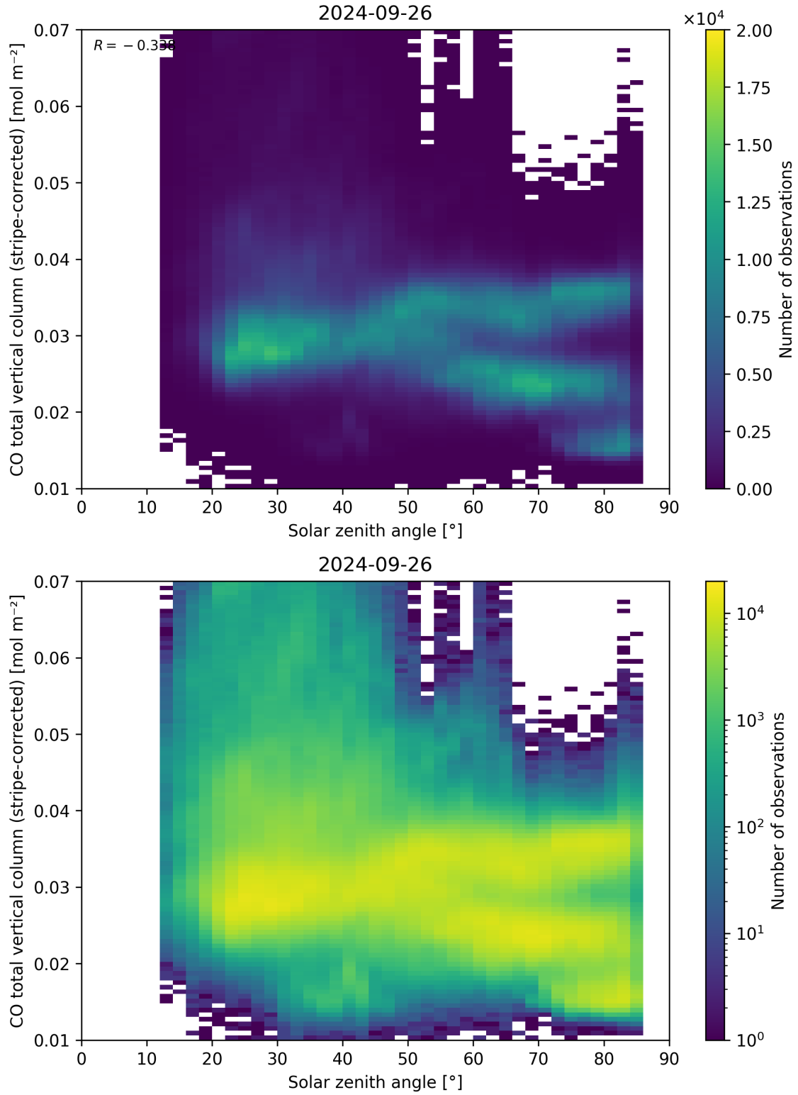
Figure 62: Scatter density plot of “Solar zenith angle” against “CO total vertical column (stripe-corrected)” for 2024-09-25 to 2024-09-27.
