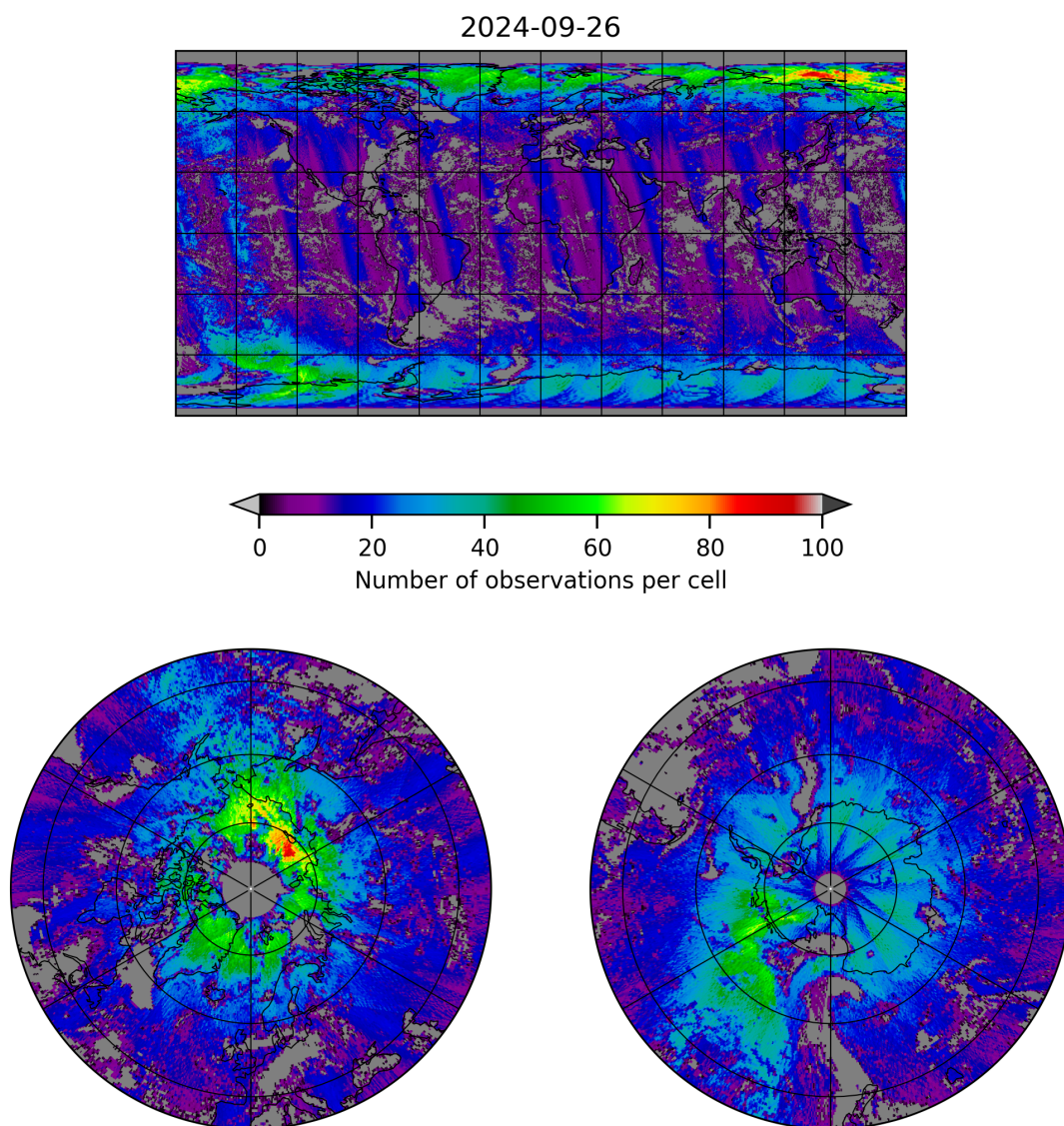
Figure 8: Map of the number of observations for 2024-09-25 to 2024-09-27
