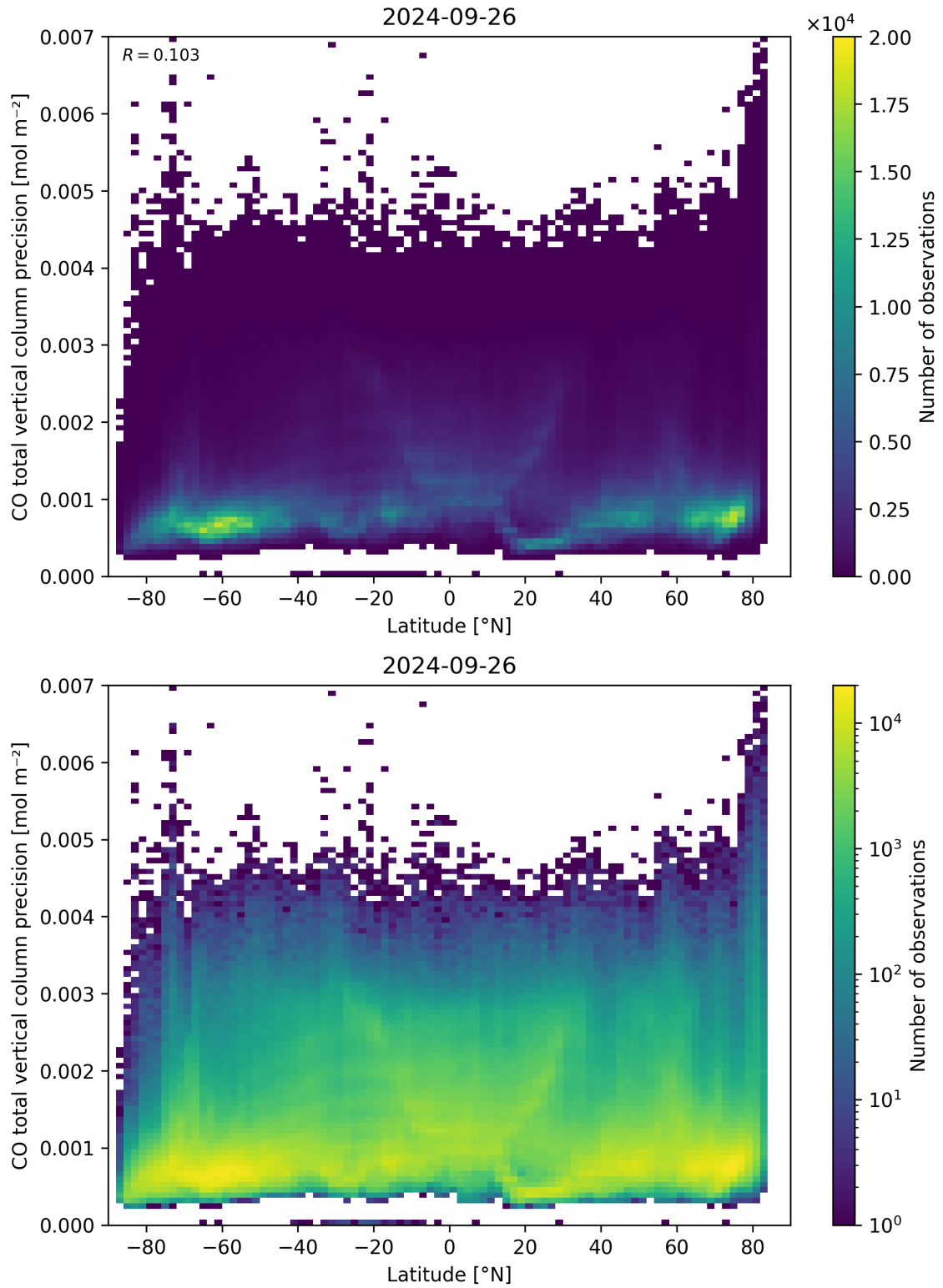
Figure 53: Scatter density plot of “Latitude” against “CO total vertical column precision” for 2024-09-25 to 2024-09-27.
