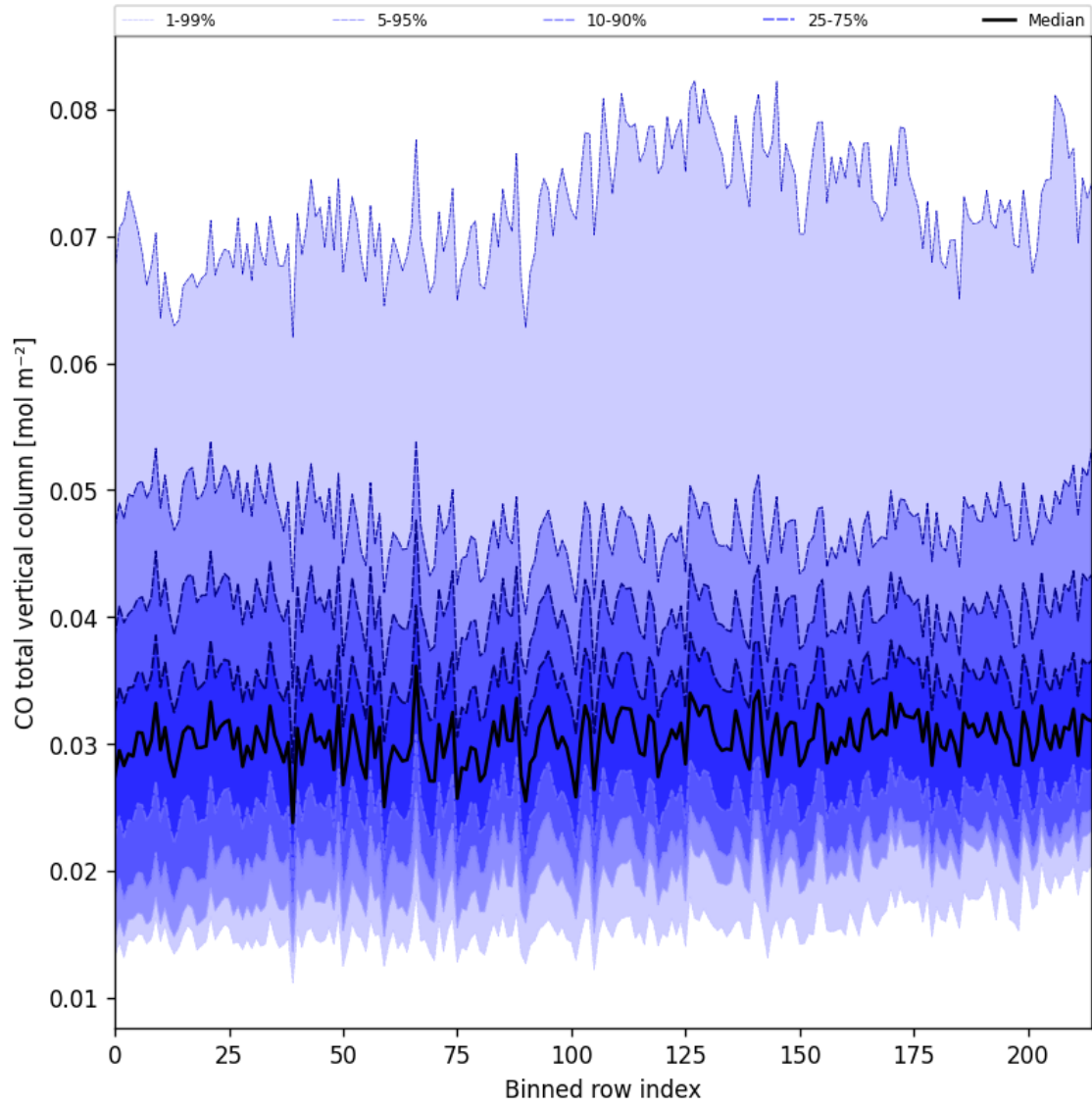
Figure 26: Along track statistics of “CO total vertical column” for 2024-09-25 to 2024-09-27
