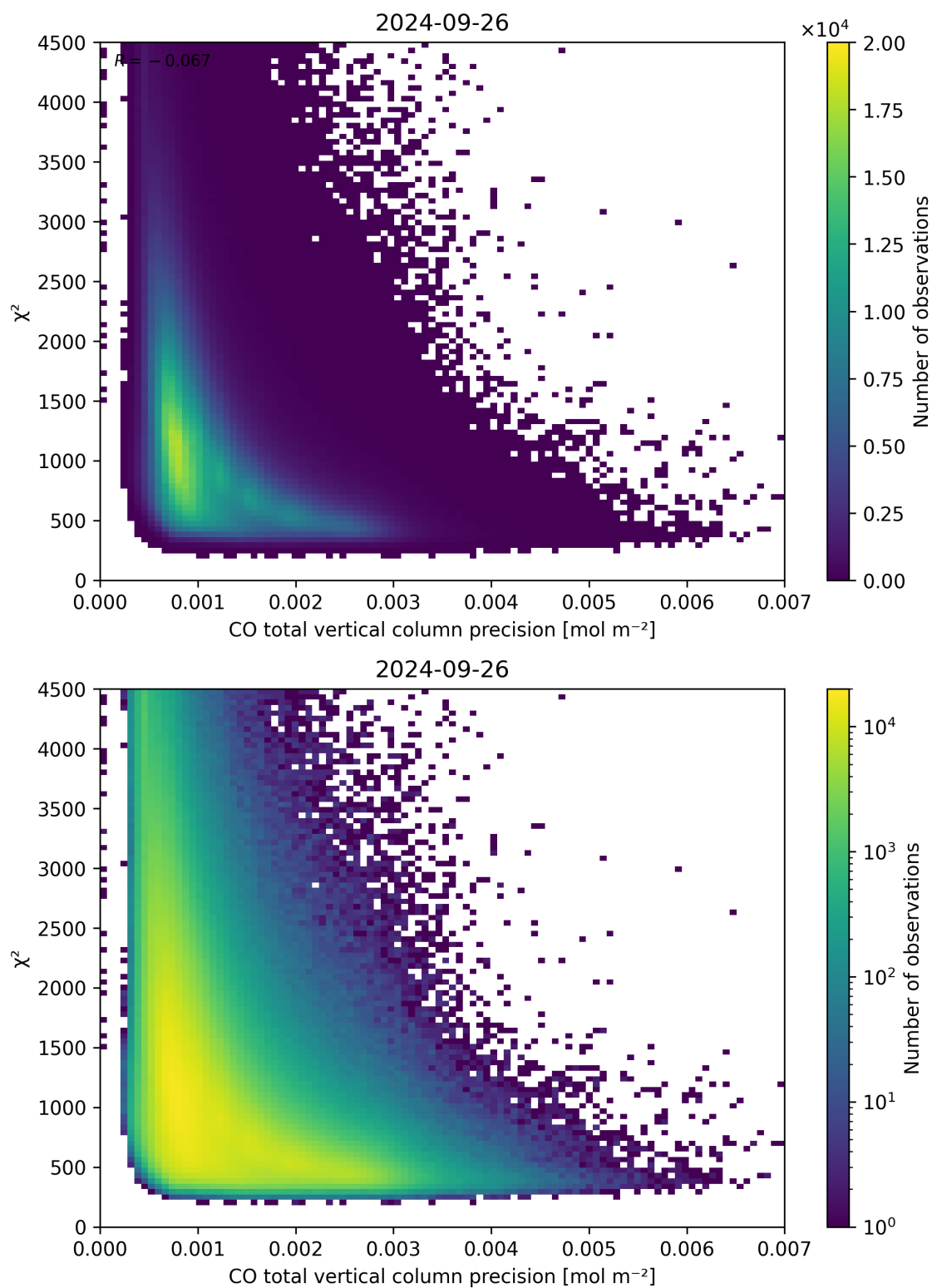
Figure 44: Scatter density plot of “CO total vertical column precision” against “ \chi^2 ” for 2024-09-25 to 2024-09-27.
