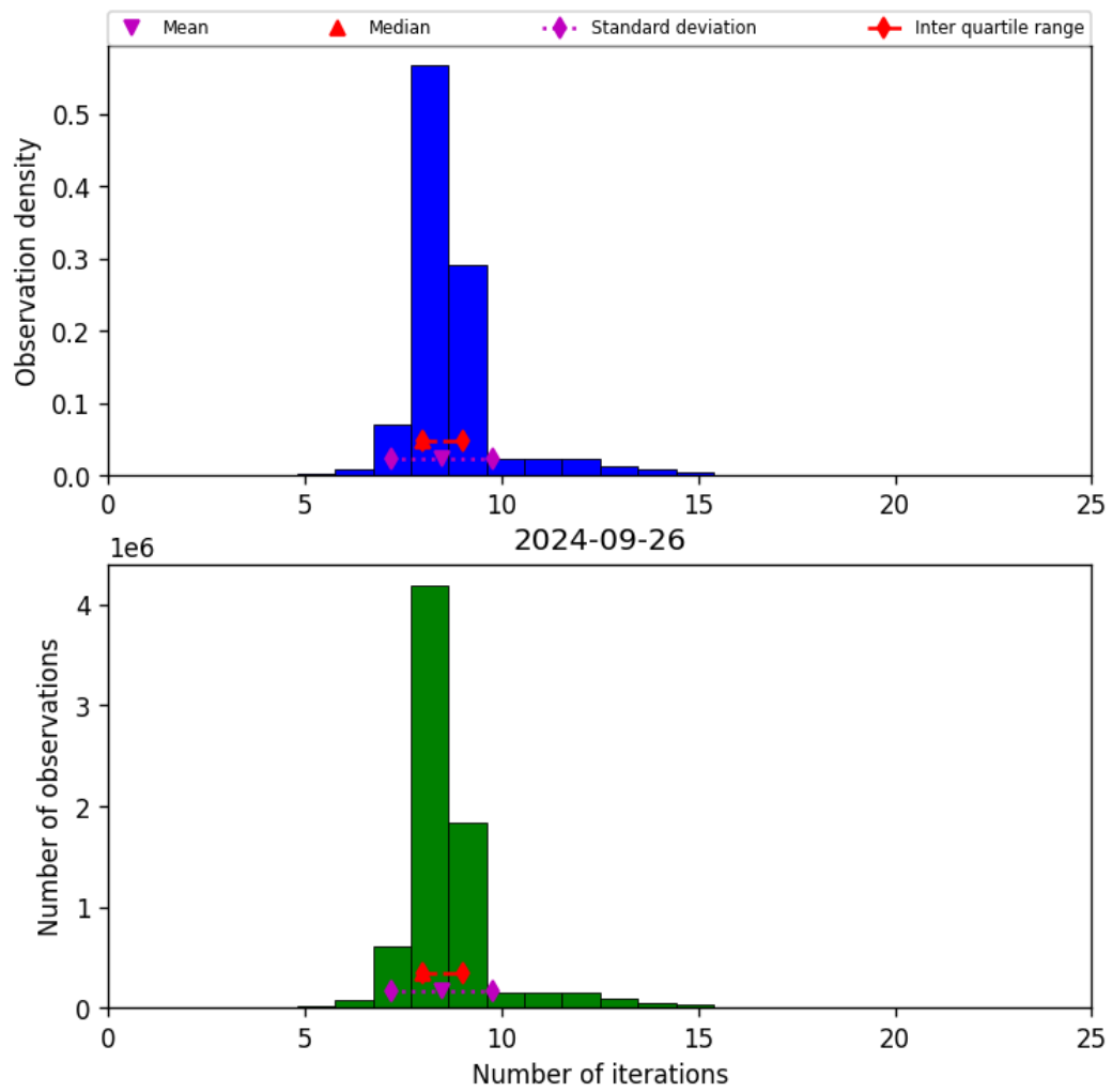
Figure 24: Histogram of “Number of iterations” for 2024-09-25 to 2024-09-27
