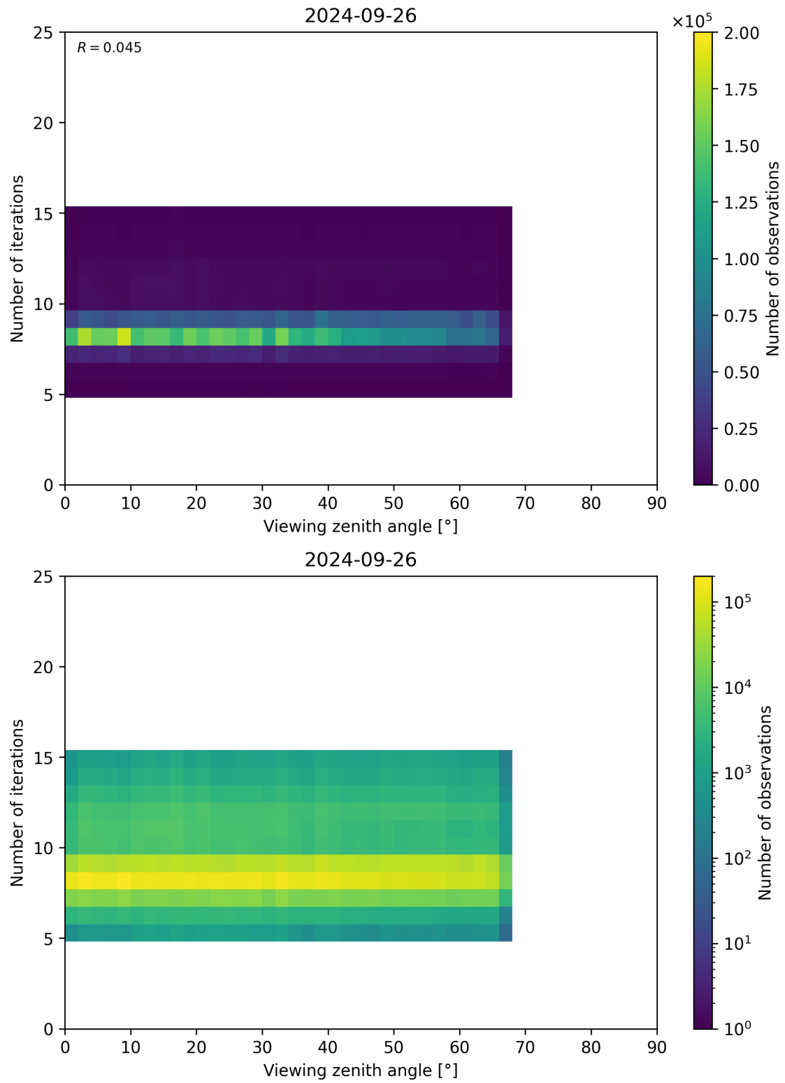
Figure 75: Scatter density plot of “Viewing zenith angle” against “Number of iterations” for 2024-09-25 to 2024-09-27.
