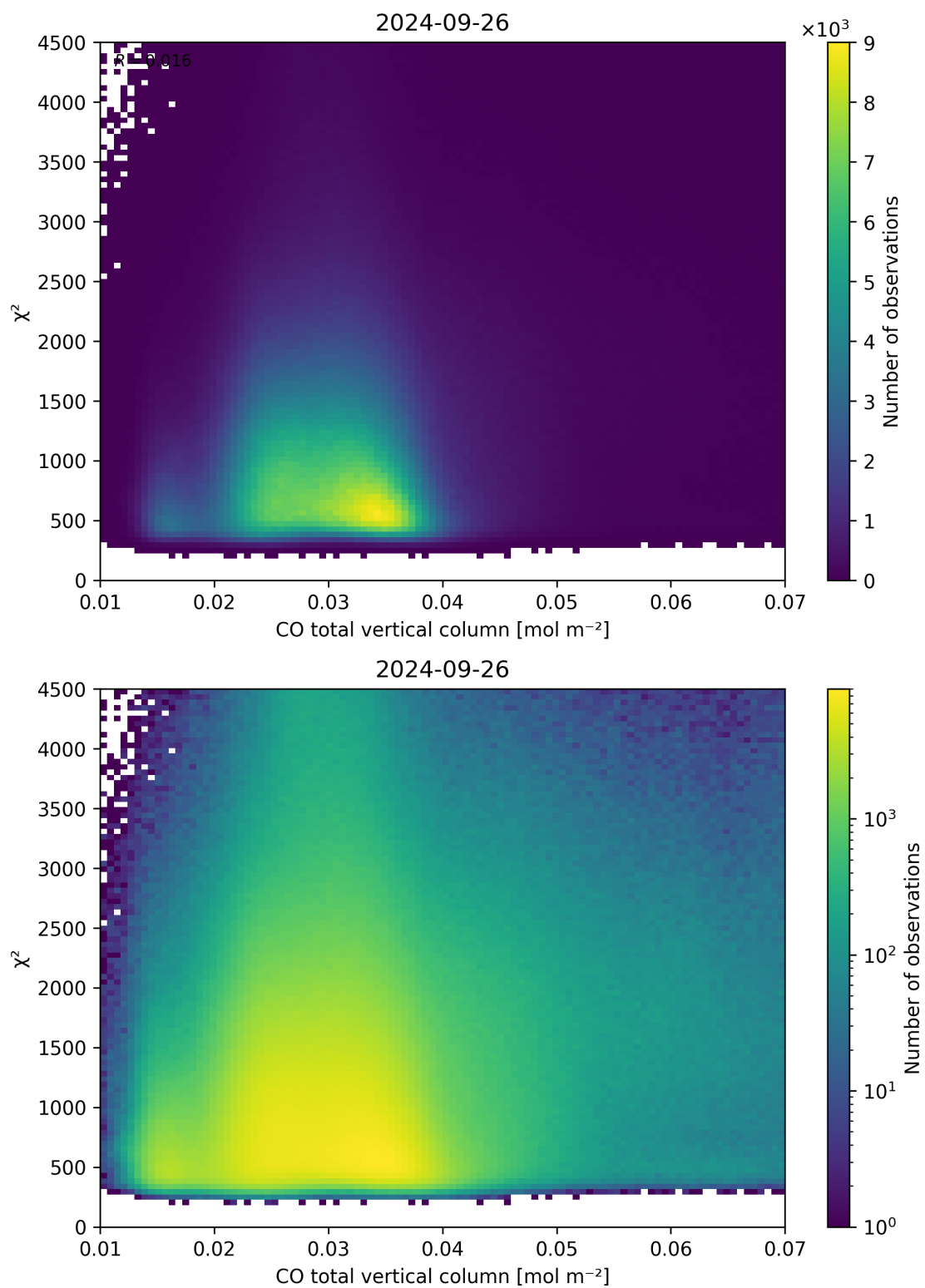
Figure 35: Scatter density plot of “CO total vertical column” against “ \chi^2 ” for 2024-09-25 to 2024-09-27.
