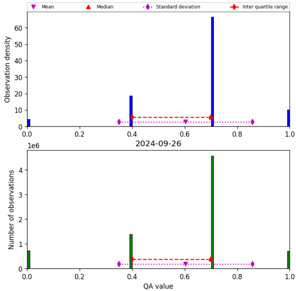
Figure 17: Histogram of “QA value” for 2024-09-25 to 2024-09-27
