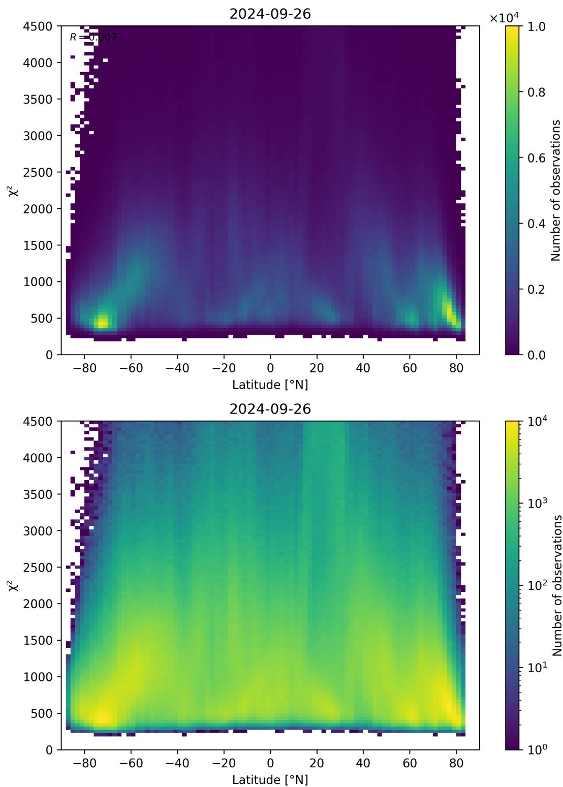
Figure 54: Scatter density plot of “Latitude” against “ \chi^2 ” for 2024-09-25 to 2024-09-27.
