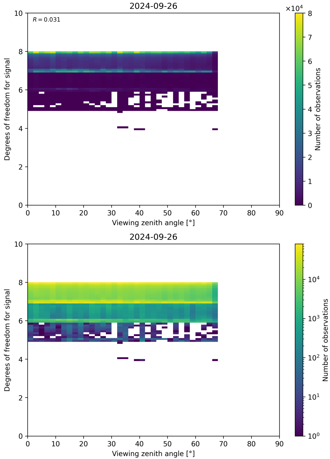
Figure 73: Scatter density plot of “Viewing zenith angle” against “Degrees of freedom for signal” for 2024-09-25 to 2024-09-27.
