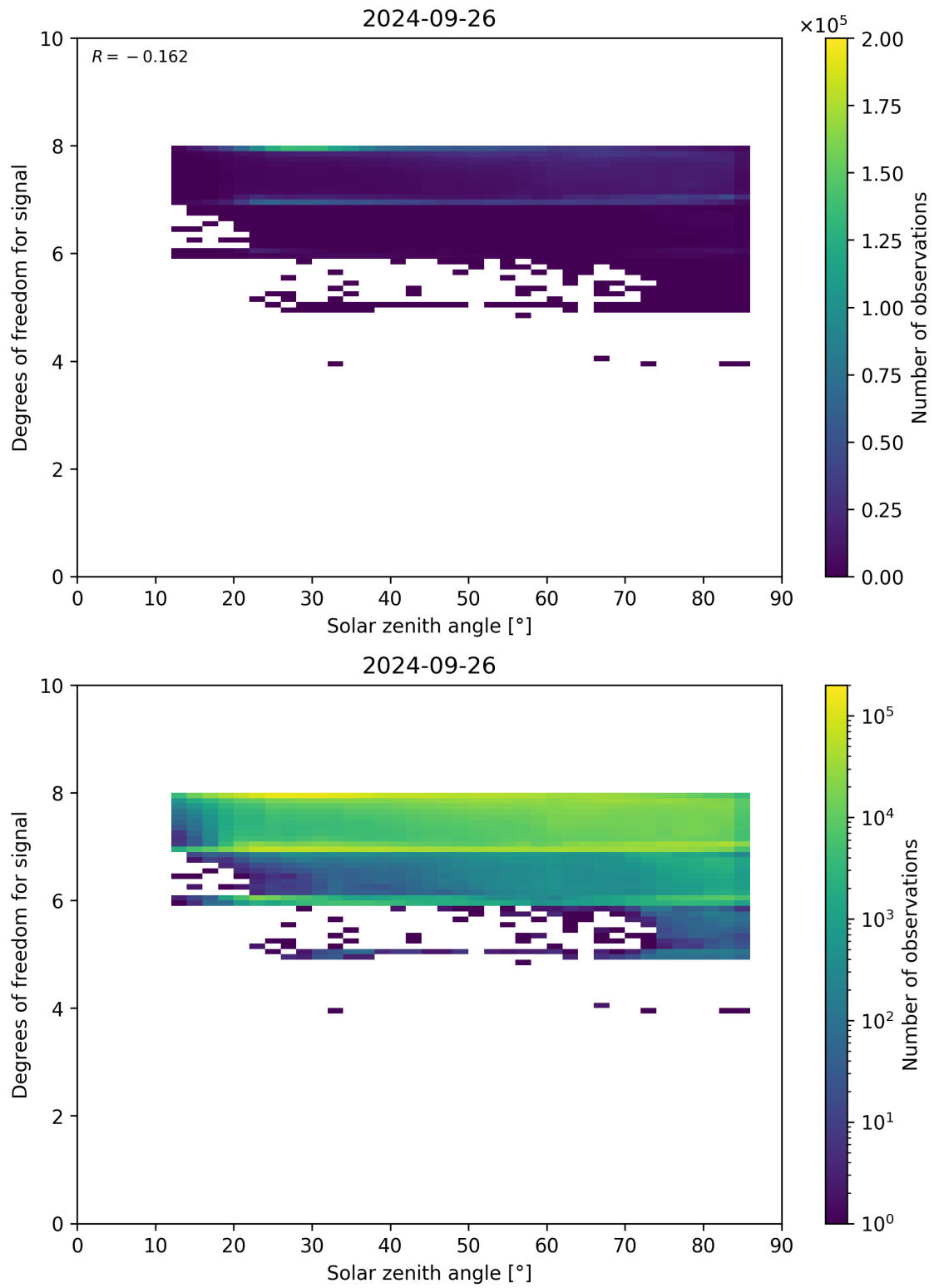
Figure 65: Scatter density plot of “Solar zenith angle” against “Degrees of freedom for signal” for 2024-09-25 to 2024-09-27.
