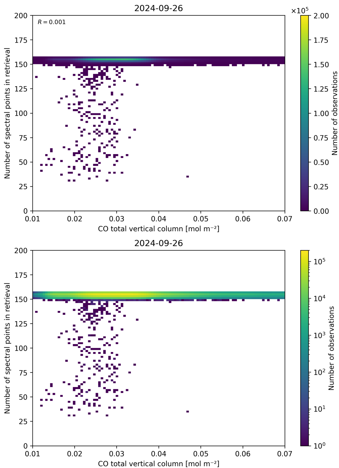
Figure 43: Scatter density plot of “CO total vertical column” against “Number of spectral points in retrieval” for 2024-09-25 to 2024-09-27.
