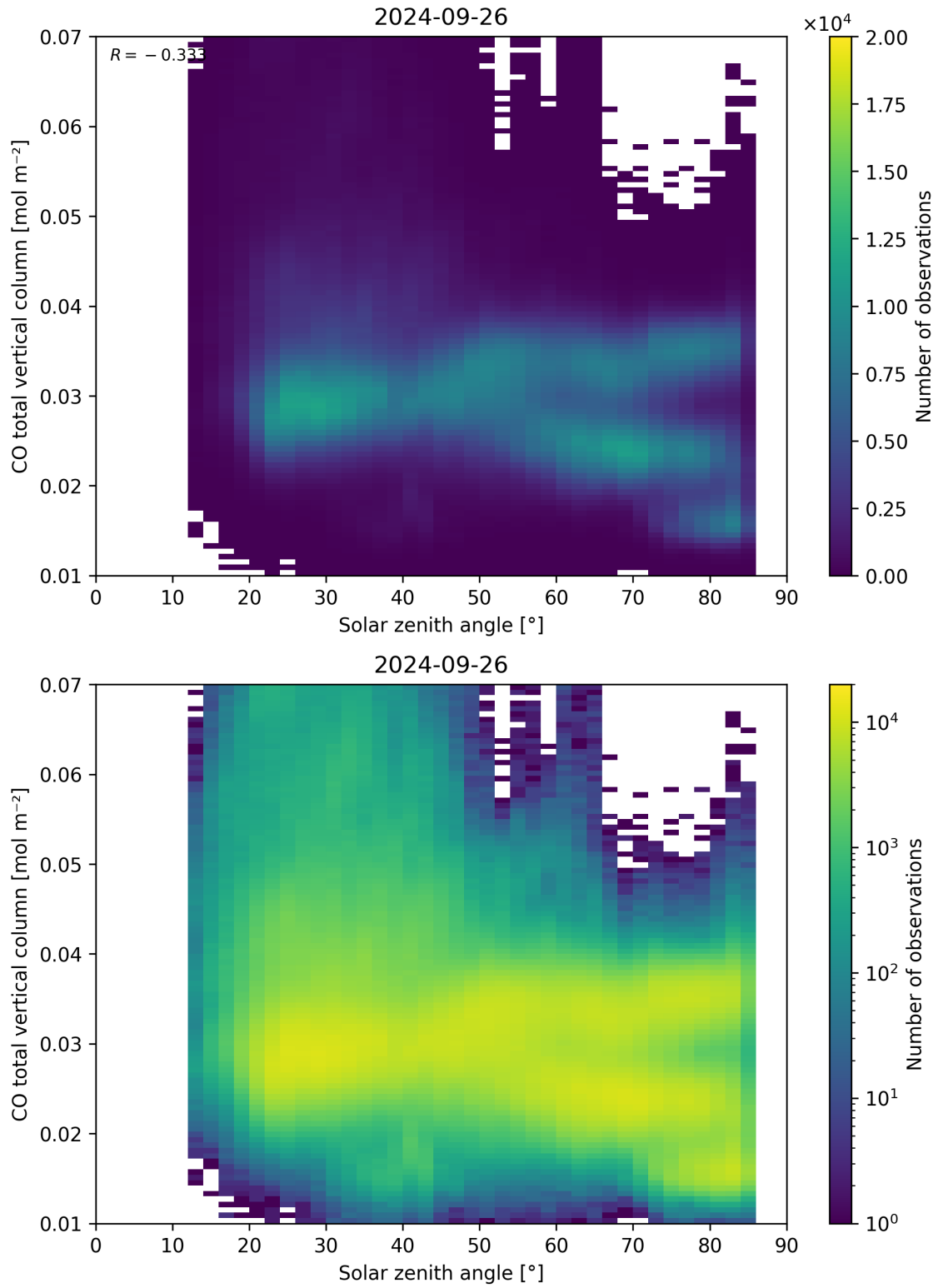
Figure 61: Scatter density plot of “Solar zenith angle” against “CO total vertical column” for 2024-09-25 to 2024-09-27.
