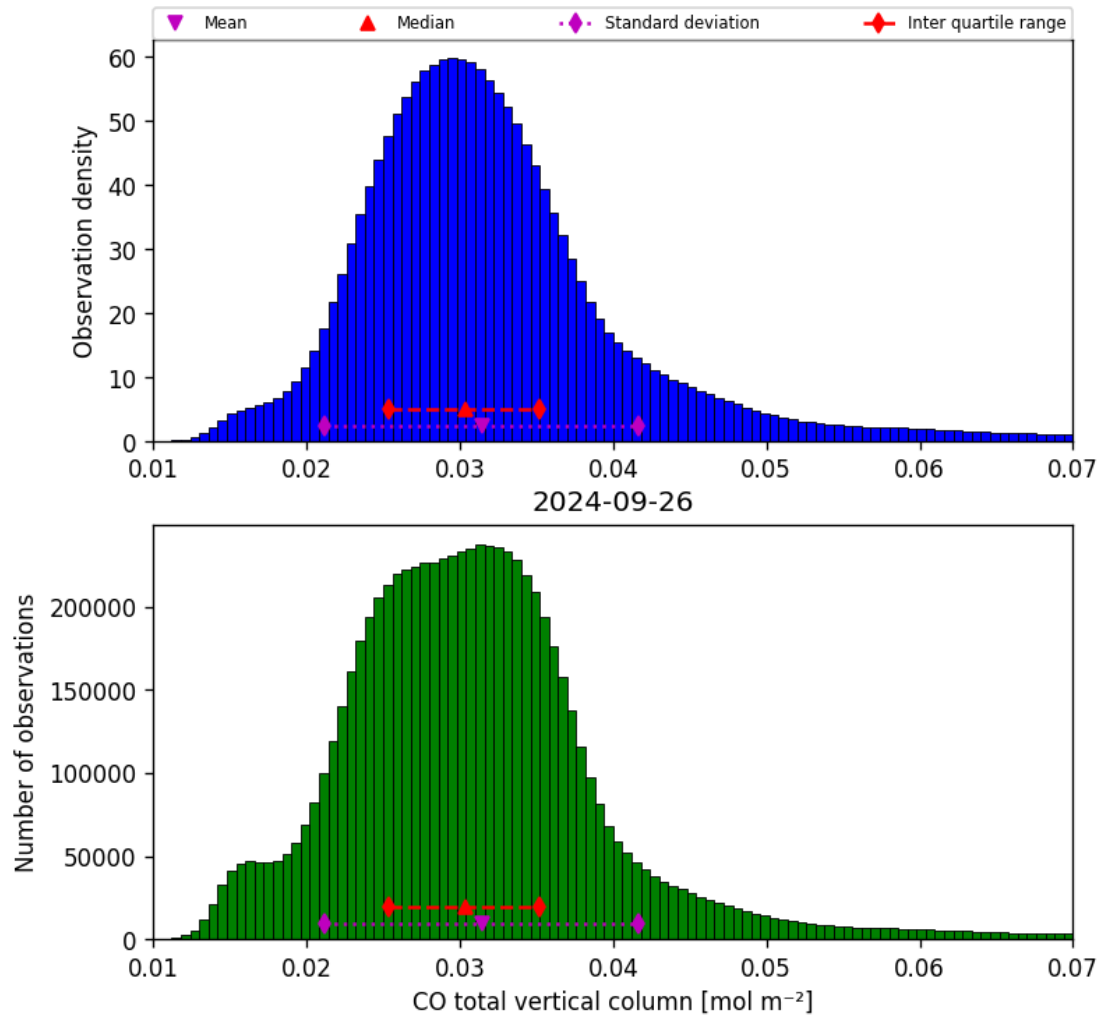
Figure 18: Histogram of “CO total vertical column” for 2024-09-25 to 2024-09-27
