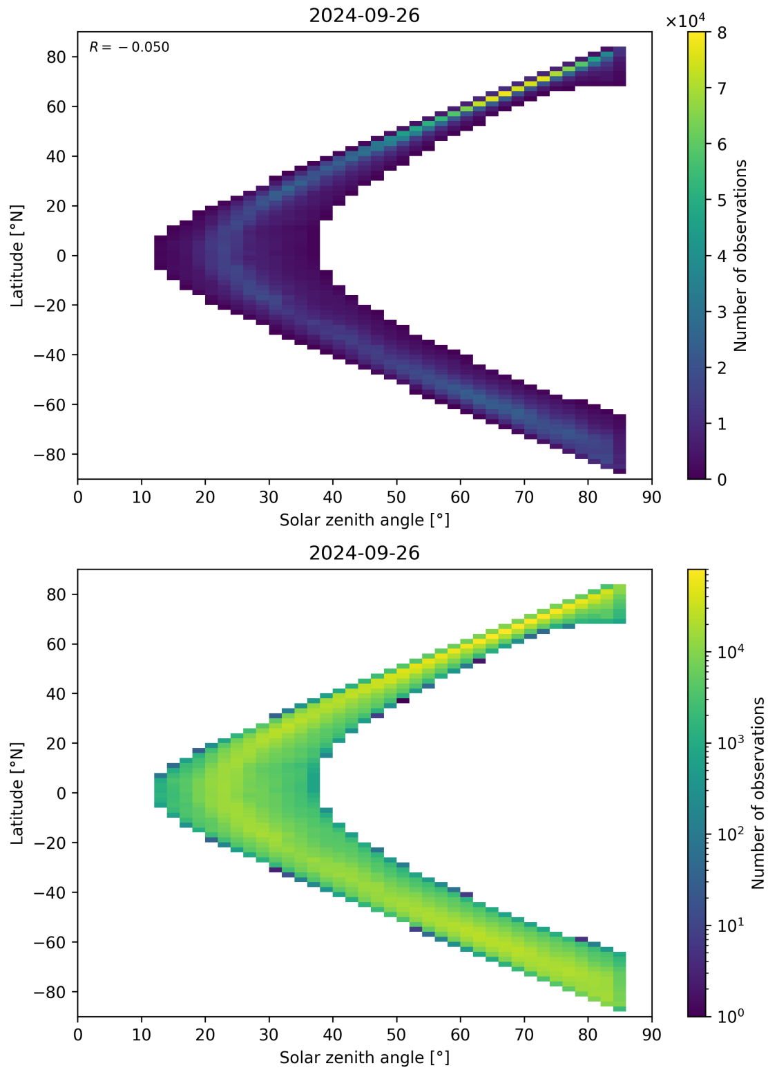
Figure 66: Scatter density plot of “Solar zenith angle” against “Latitude” for 2024-09-25 to 2024-09-27.
