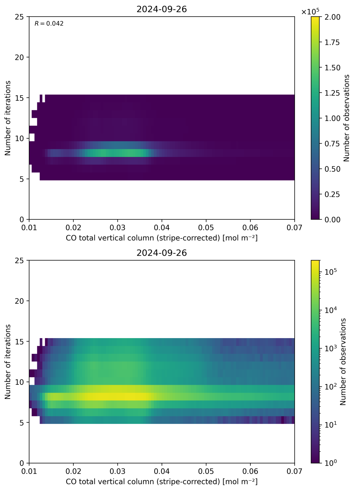
Figure 39: Scatter density plot of “CO total vertical column (stripe-corrected)” against “Number of iterations” for 2024-09-25 to 2024-09-27.
