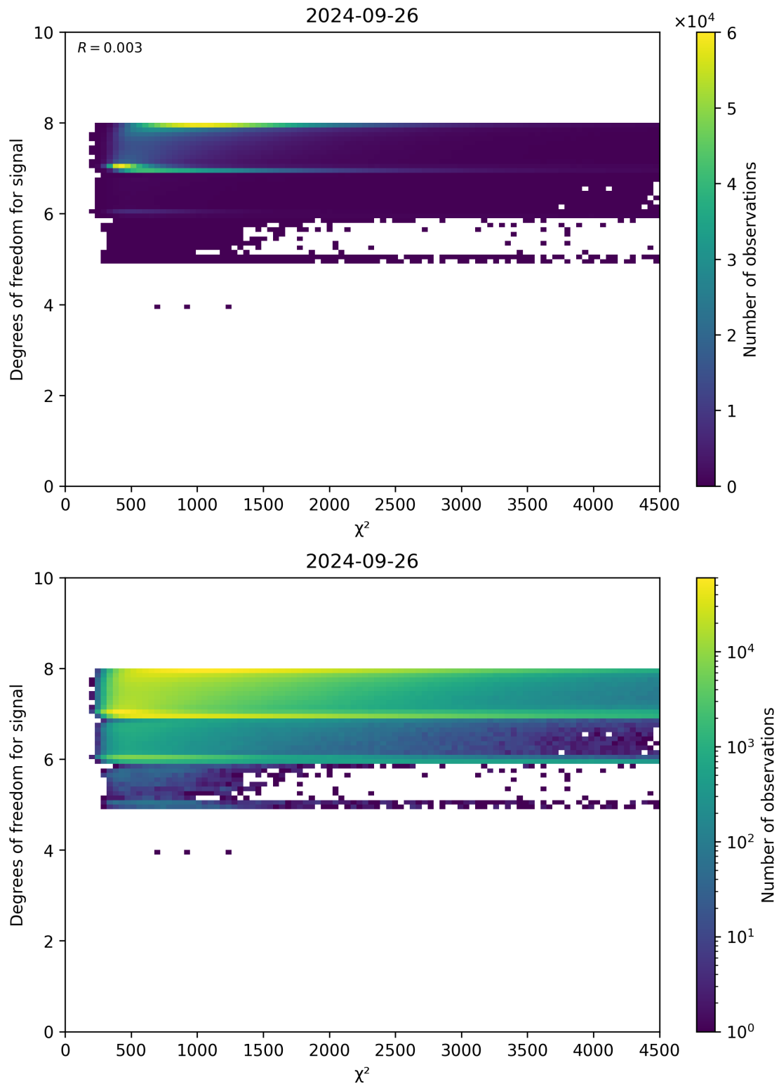
Figure 48: Scatter density plot of “ \chi^2 ” against “Degrees of freedom for signal” for 2024-09-25 to 2024-09-27.
