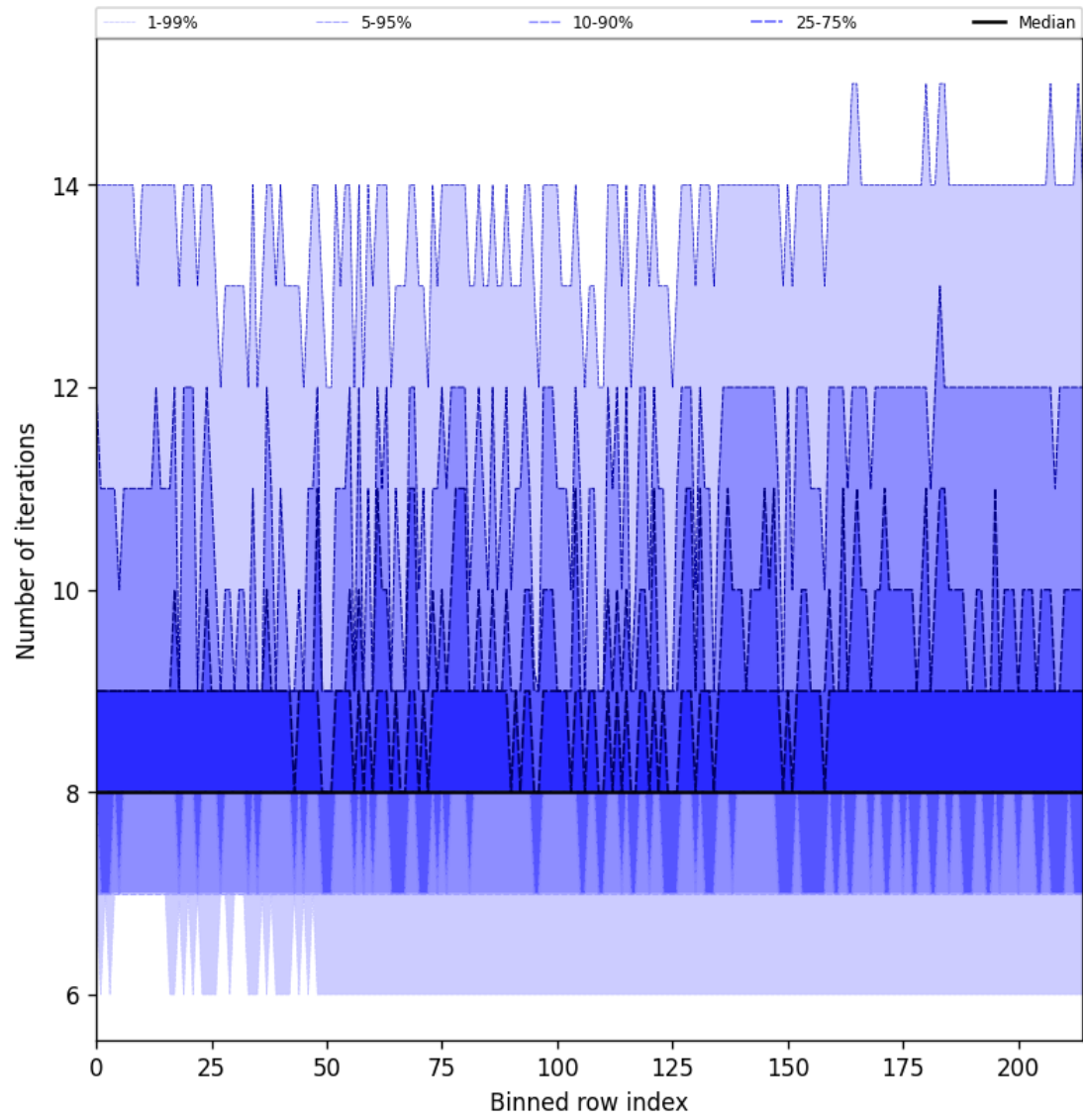
Figure 32: Along track statistics of “Number of iterations” for 2024-09-25 to 2024-09-27
