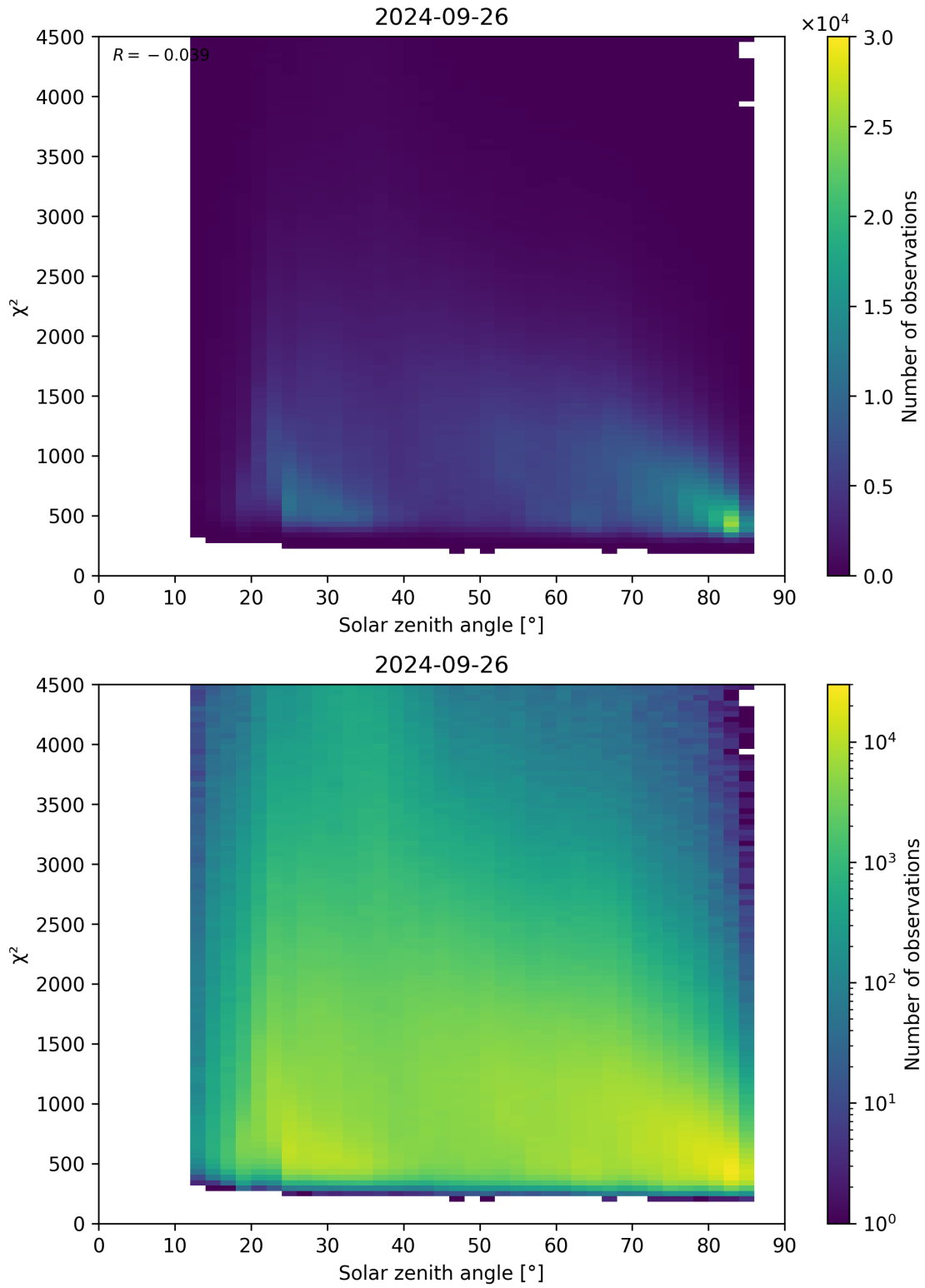
Figure 64: Scatter density plot of “Solar zenith angle” against “ \chi^2 ” for 2024-09-25 to 2024-09-27.
