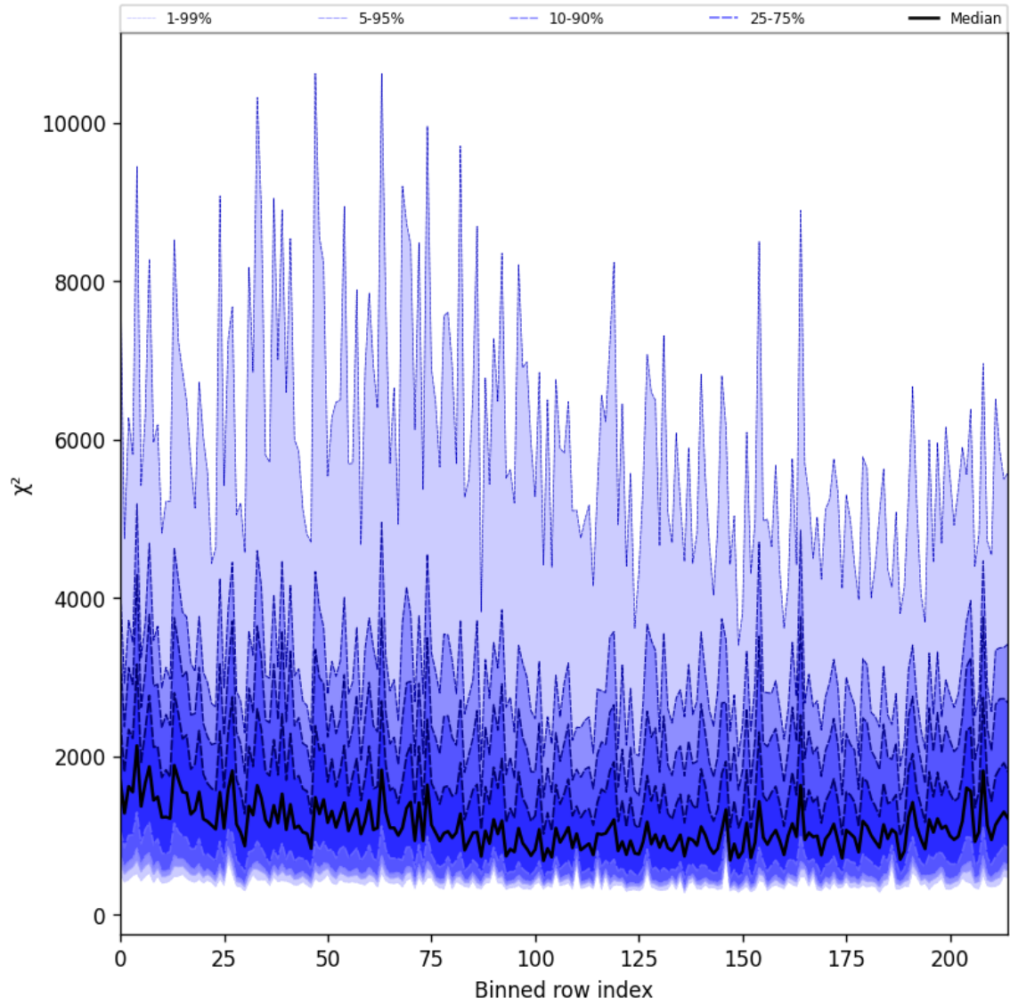
Figure 30: Along track statistics of “ \chi^2 ” for 2024-09-25 to 2024-09-27
