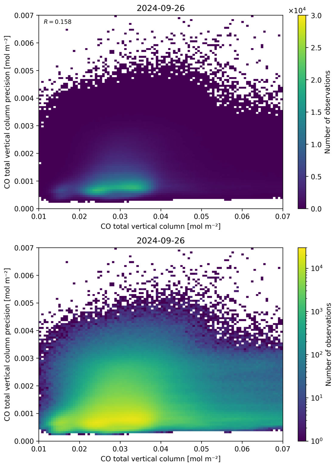
Figure 34: Scatter density plot of “CO total vertical column” against “CO total vertical column precision” for 2024-09-25 to 2024-09-27.
