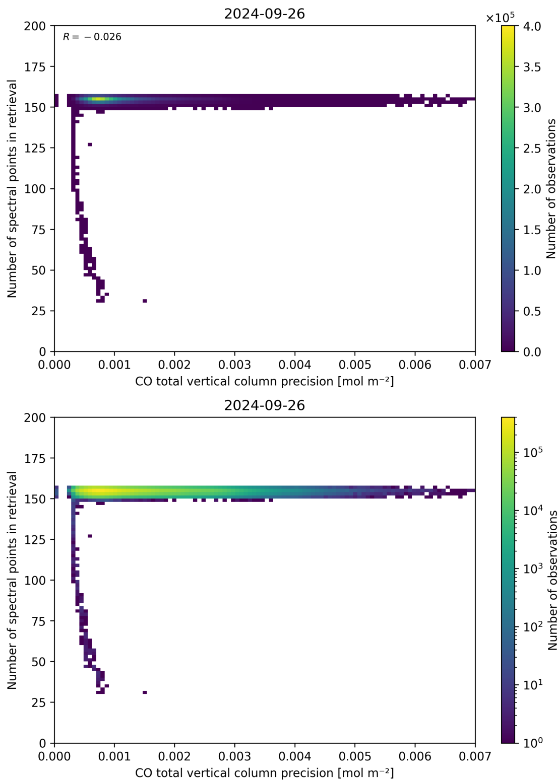
Figure 47: Scatter density plot of “CO total vertical column precision” against “Number of spectral points in retrieval” for 2024-09-25 to 2024-09-27.
