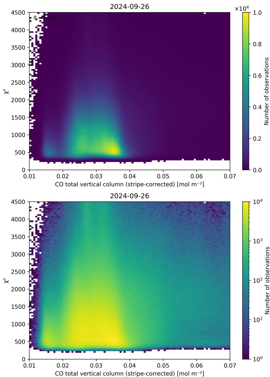
Figure 37: Scatter density plot of “CO total vertical column (stripe-corrected)” against “ \chi^2 ” for 2024-09-25 to 2024-09-27.
