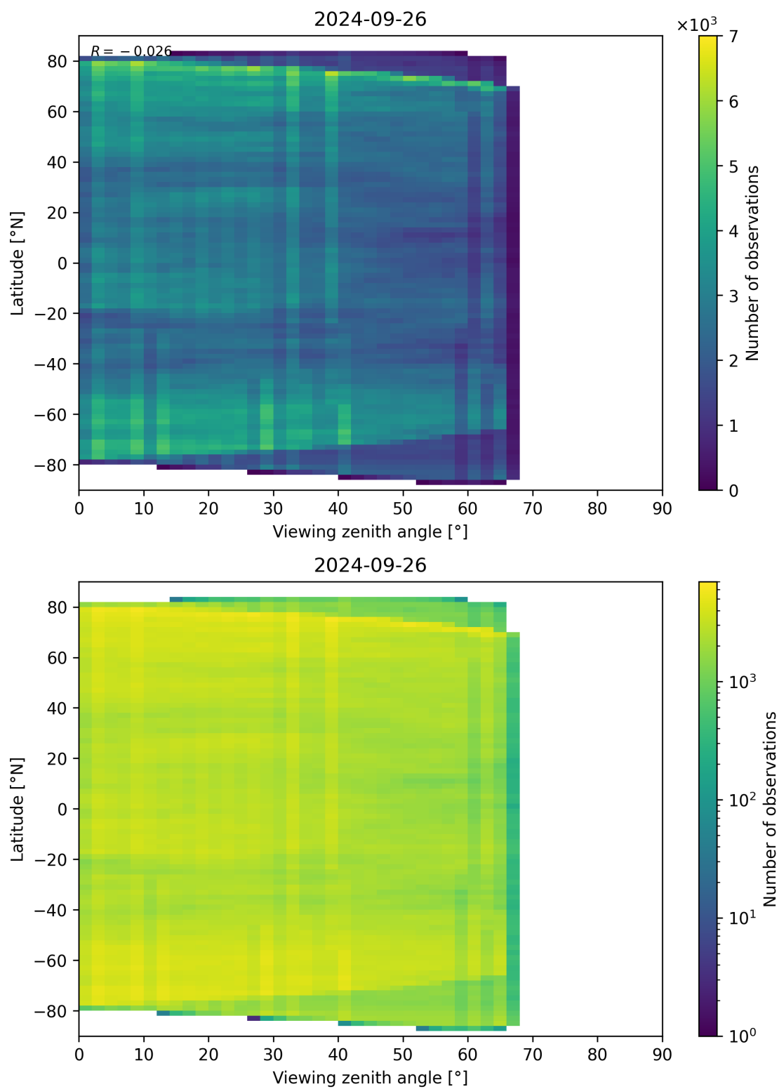
Figure 74: Scatter density plot of “Viewing zenith angle” against “Latitude” for 2024-09-25 to 2024-09-27.
