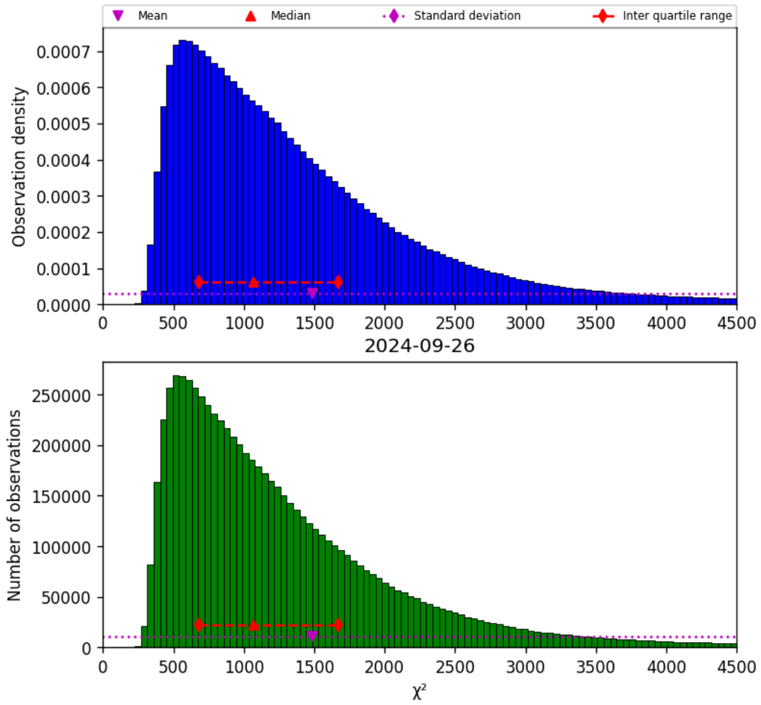
Figure 22: Histogram of “ \chi^2 ” for 2024-09-25 to 2024-09-27
