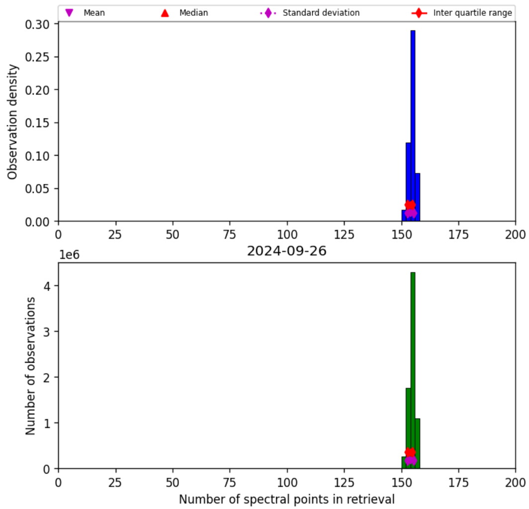
Figure 21: Histogram of “Number of spectral points in retrieval” for 2024-09-25 to 2024-09-27
