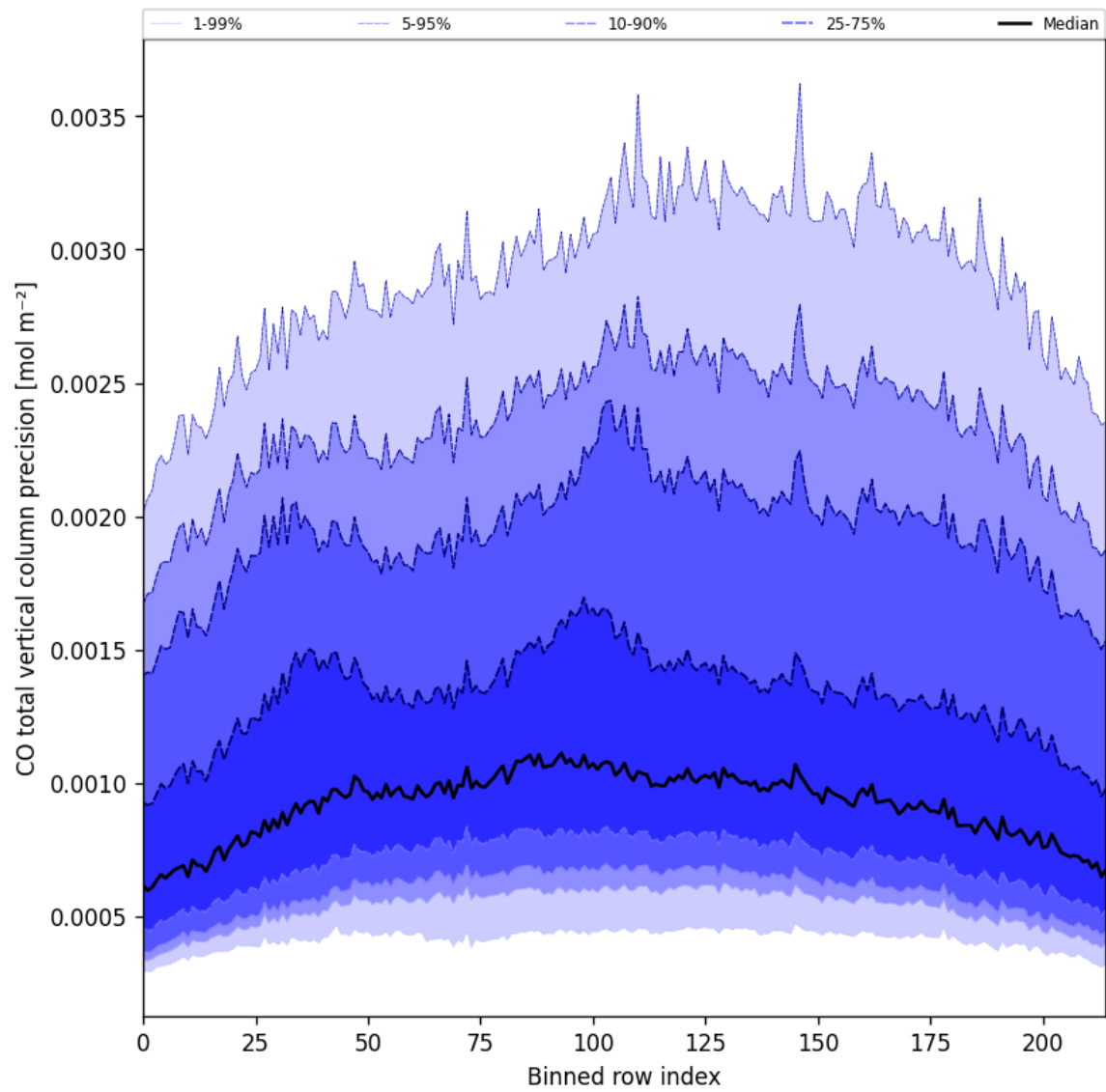
Figure 28: Along track statistics of “CO total vertical column precision” for 2024-09-25 to 2024-09-27
