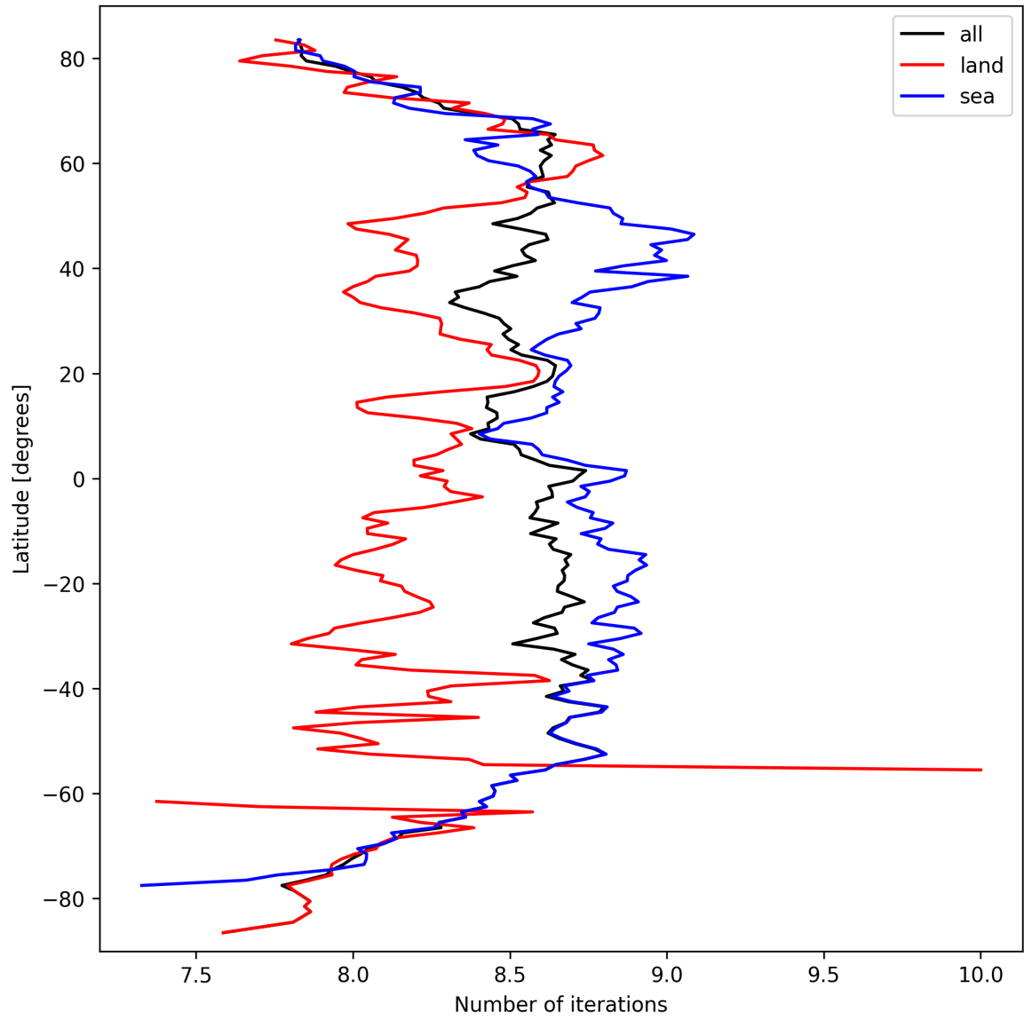
Figure 16: Zonal average of “Number of iterations” for 2024-09-25 to 2024-09-27.
