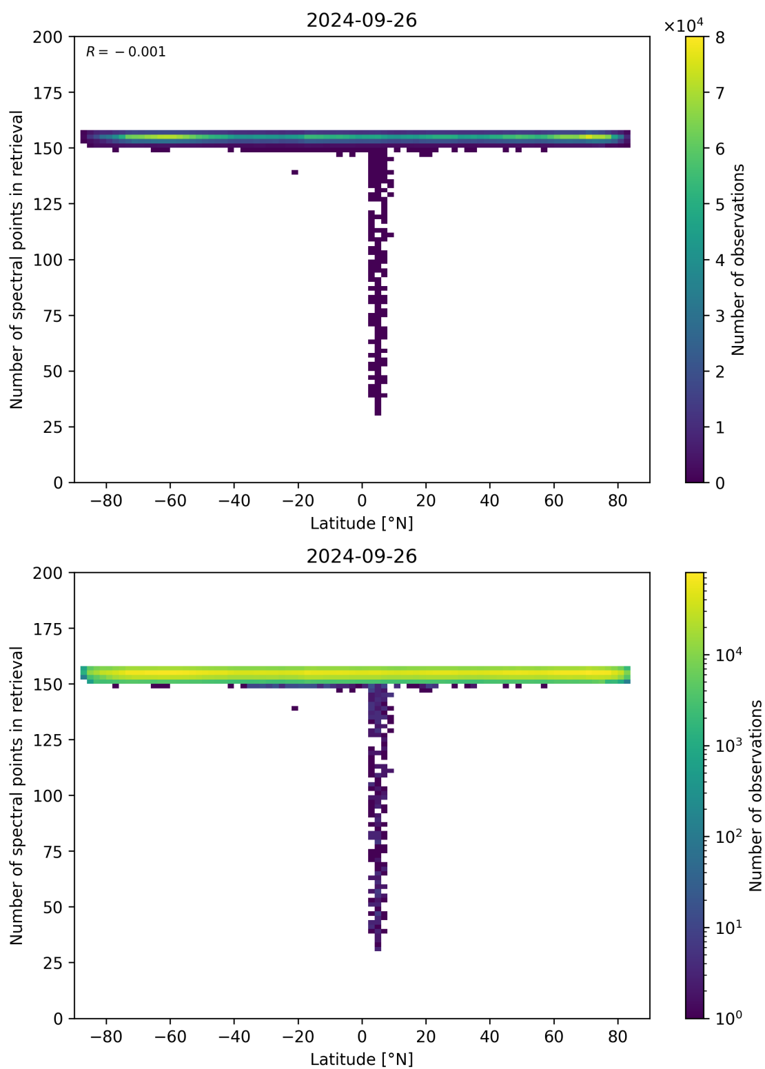
Figure 57: Scatter density plot of “Latitude” against “Number of spectral points in retrieval” for 2024-09-25 to 2024-09-27.
