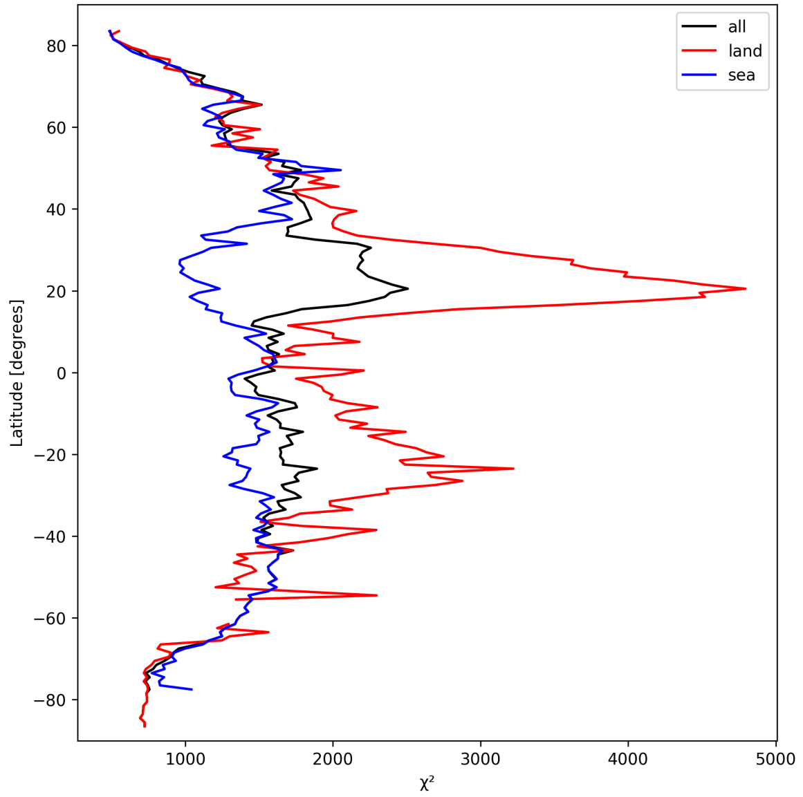
Figure 14: Zonal average of “ \chi^2 ” for 2024-09-25 to 2024-09-27.
