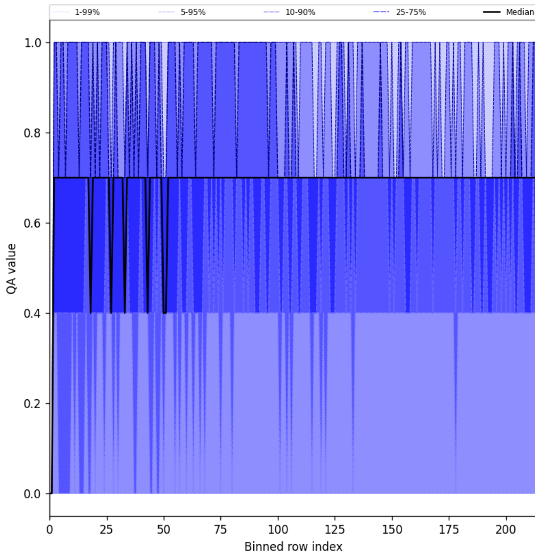
Figure 25: Along track statistics of “QA value” for 2024-09-25 to 2024-09-27
