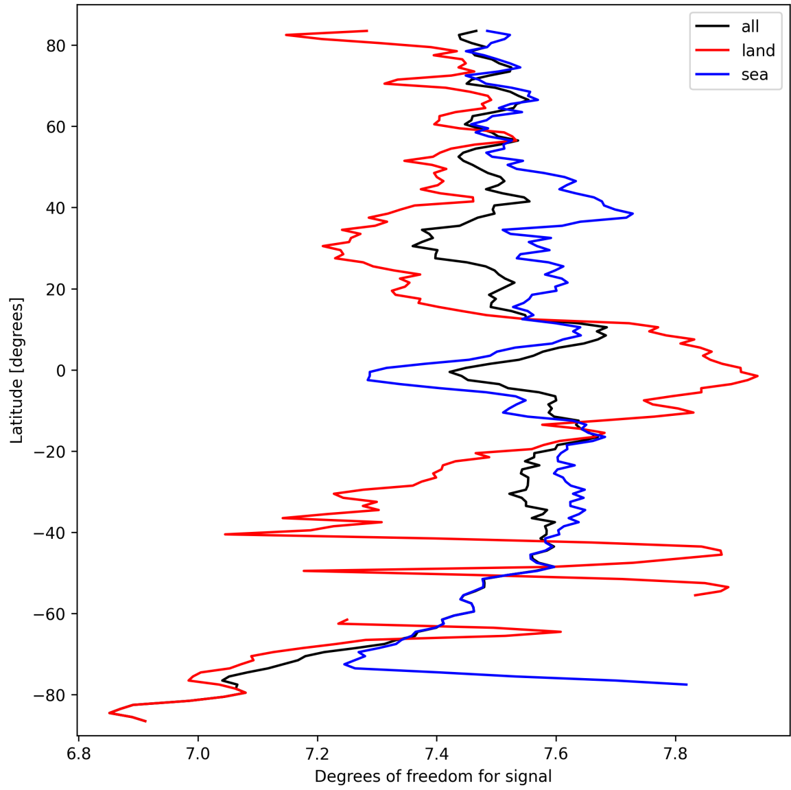
Figure 15: Zonal average of “Degrees of freedom for signal” for 2024-09-25 to 2024-09-27.
