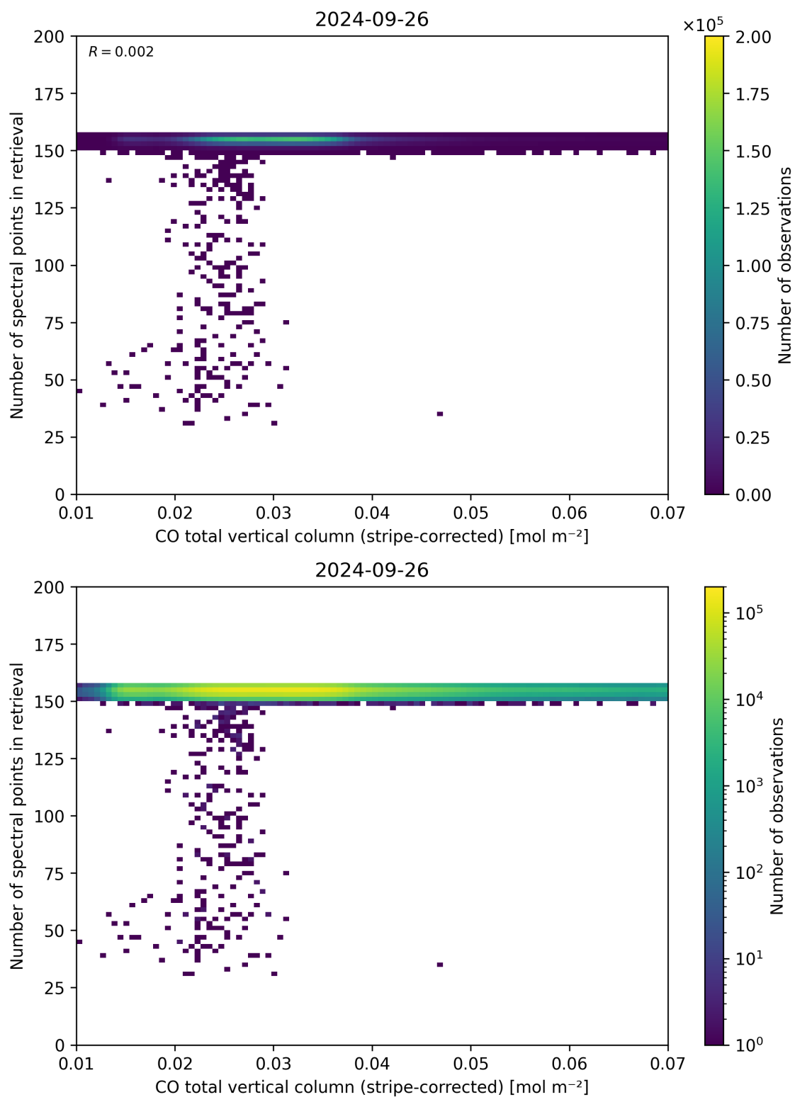
Figure 40: Scatter density plot of “CO total vertical column (stripe-corrected)” against “Number of spectral points in retrieval” for 2024-09-25 to 2024-09-27.
