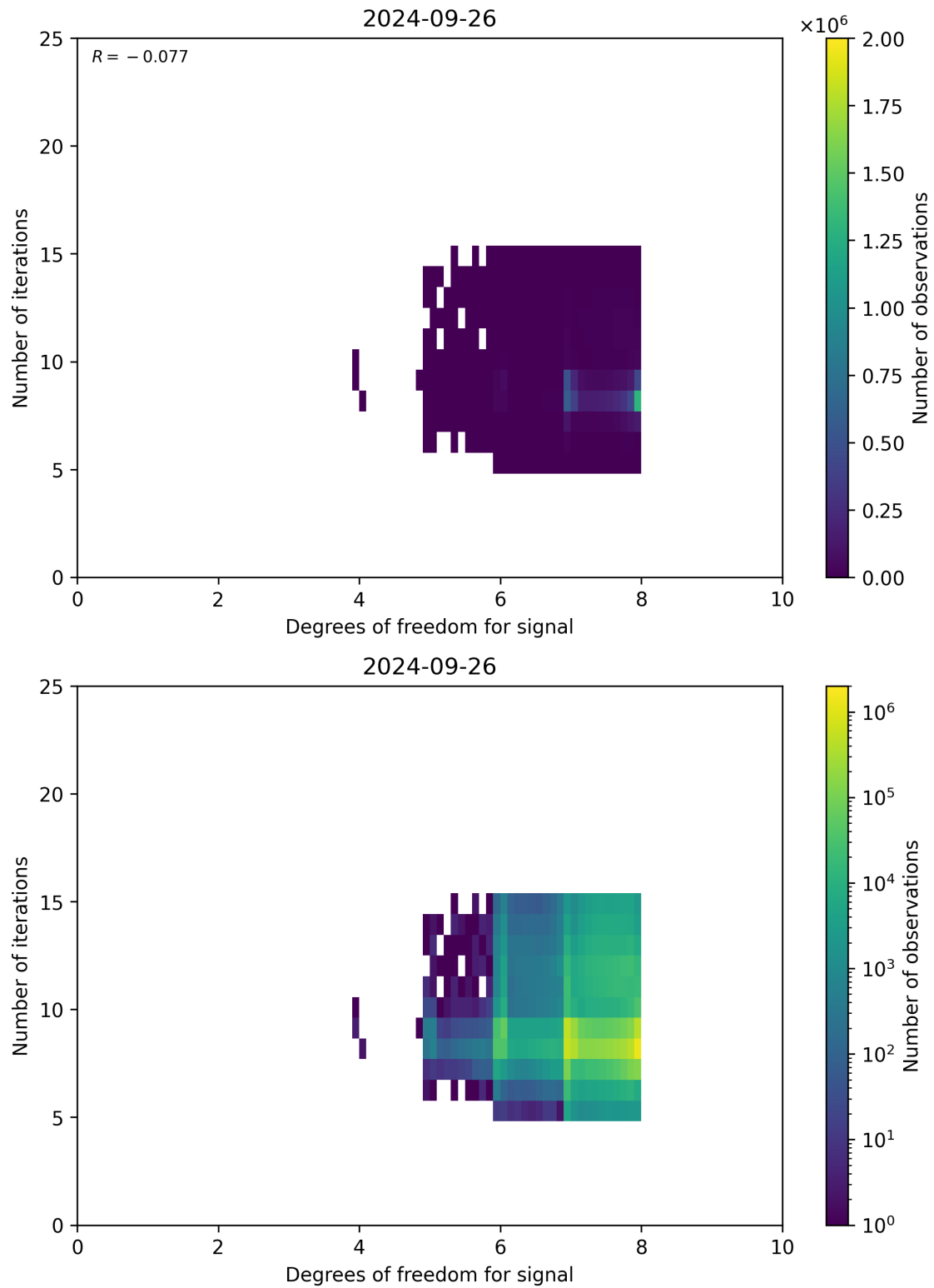
Figure 50: Scatter density plot of “Degrees of freedom for signal” against “Number of iterations” for 2024-09-25 to 2024-09-27.
