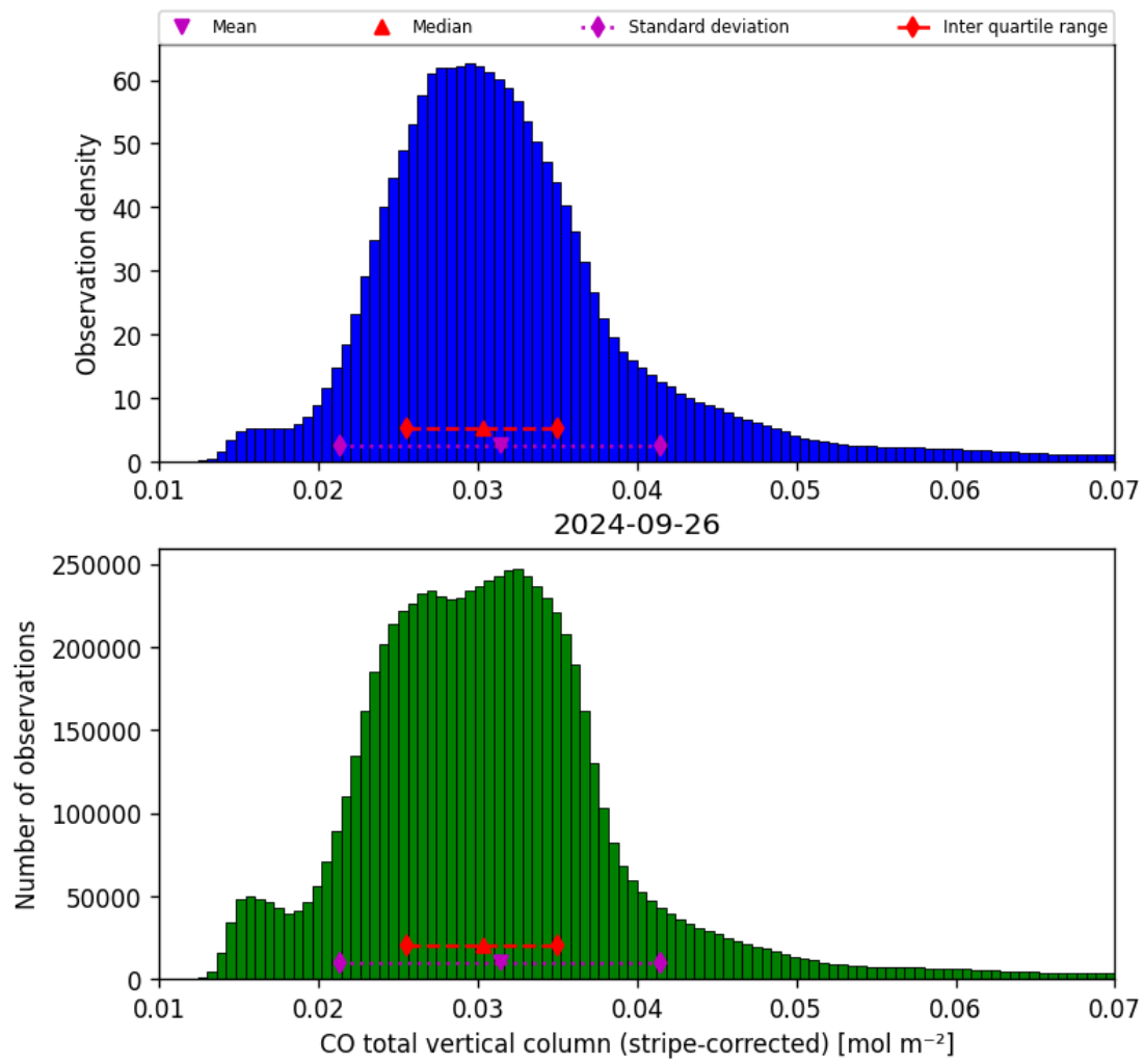
Figure 19: Histogram of “CO total vertical column (stripe-corrected)” for 2024-09-25 to 2024-09-27
