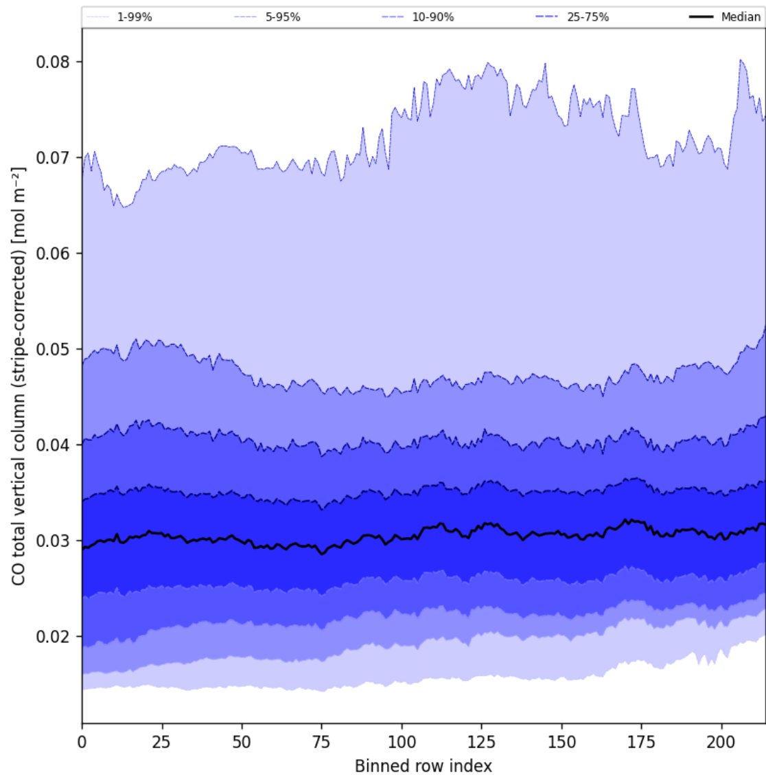
Figure 27: Along track statistics of “CO total vertical column (stripe-corrected)” for 2024-09-25 to 2024-09-27
