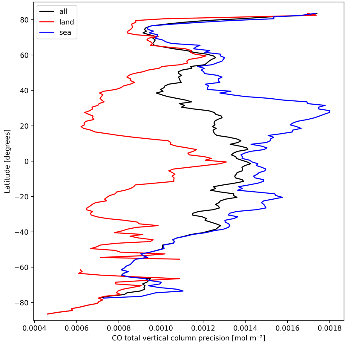
Figure 12: Zonal average of “CO total vertical column precision” for 2024-09-25 to 2024-09-27.
