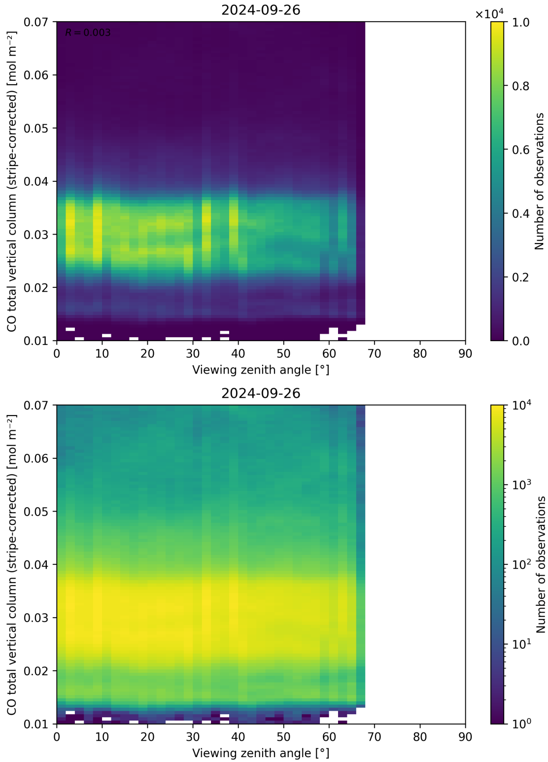
Figure 70: Scatter density plot of “Viewing zenith angle” against “CO total vertical column (stripe-corrected)” for 2024-09-25 to 2024-09-27.
