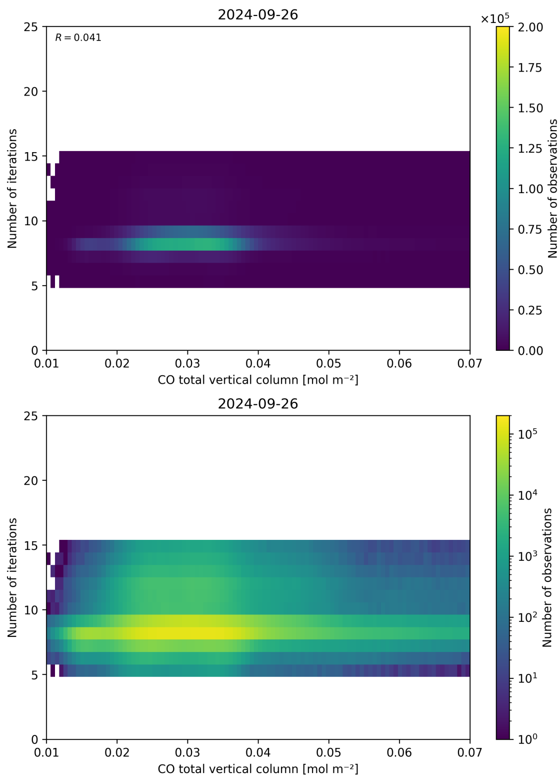
Figure 42: Scatter density plot of “CO total vertical column” against “Number of iterations” for 2024-09-25 to 2024-09-27.
