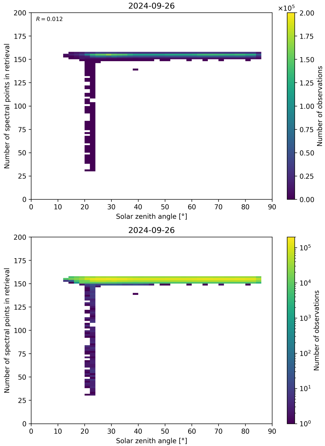
Figure 68: Scatter density plot of “Solar zenith angle” against “Number of spectral points in retrieval” for 2024-09-25 to 2024-09-27.
