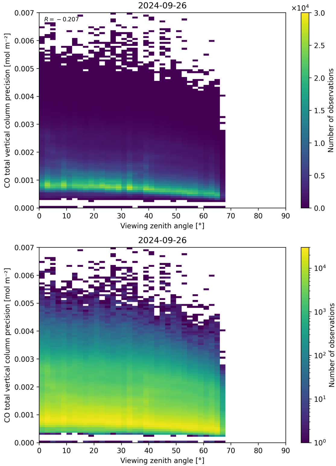
Figure 71: Scatter density plot of “Viewing zenith angle” against “CO total vertical column precision” for 2024-09-25 to 2024-09-27.
