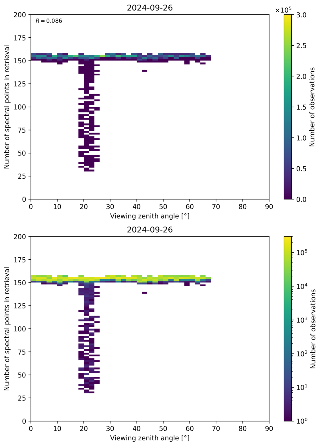
Figure 76: Scatter density plot of “Viewing zenith angle” against “Number of spectral points in retrieval” for 2024-09-25 to 2024-09-27.
