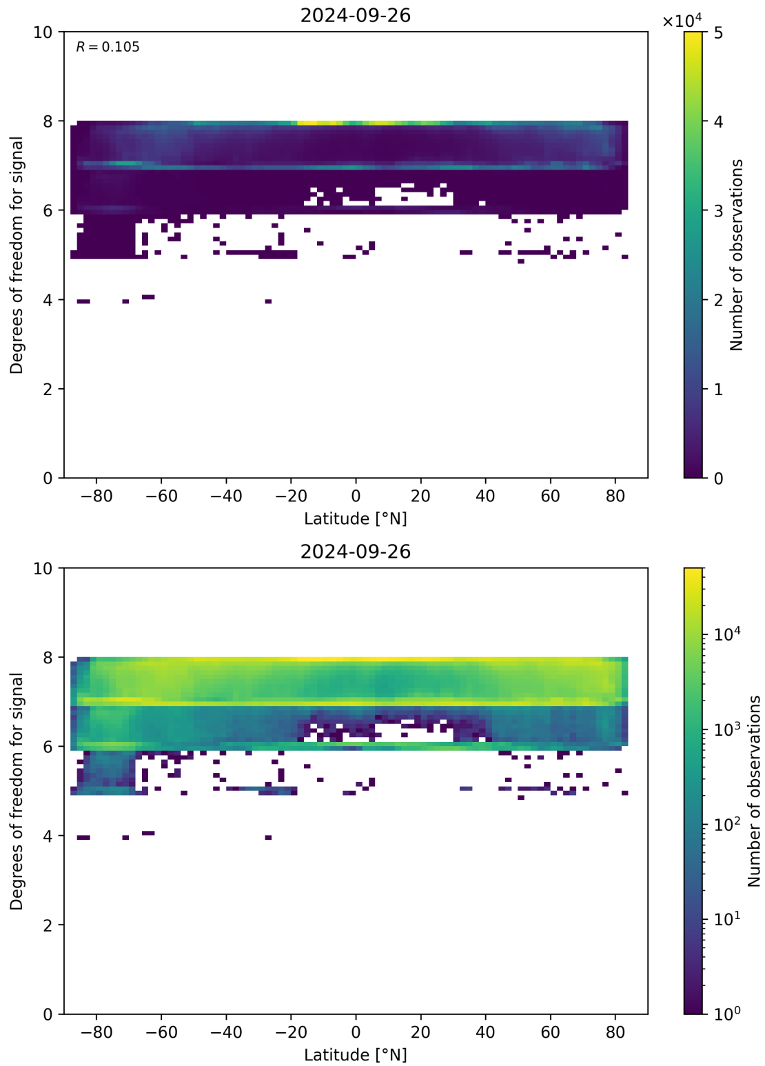
Figure 55: Scatter density plot of “Latitude” against “Degrees of freedom for signal” for 2024-09-25 to 2024-09-27.
