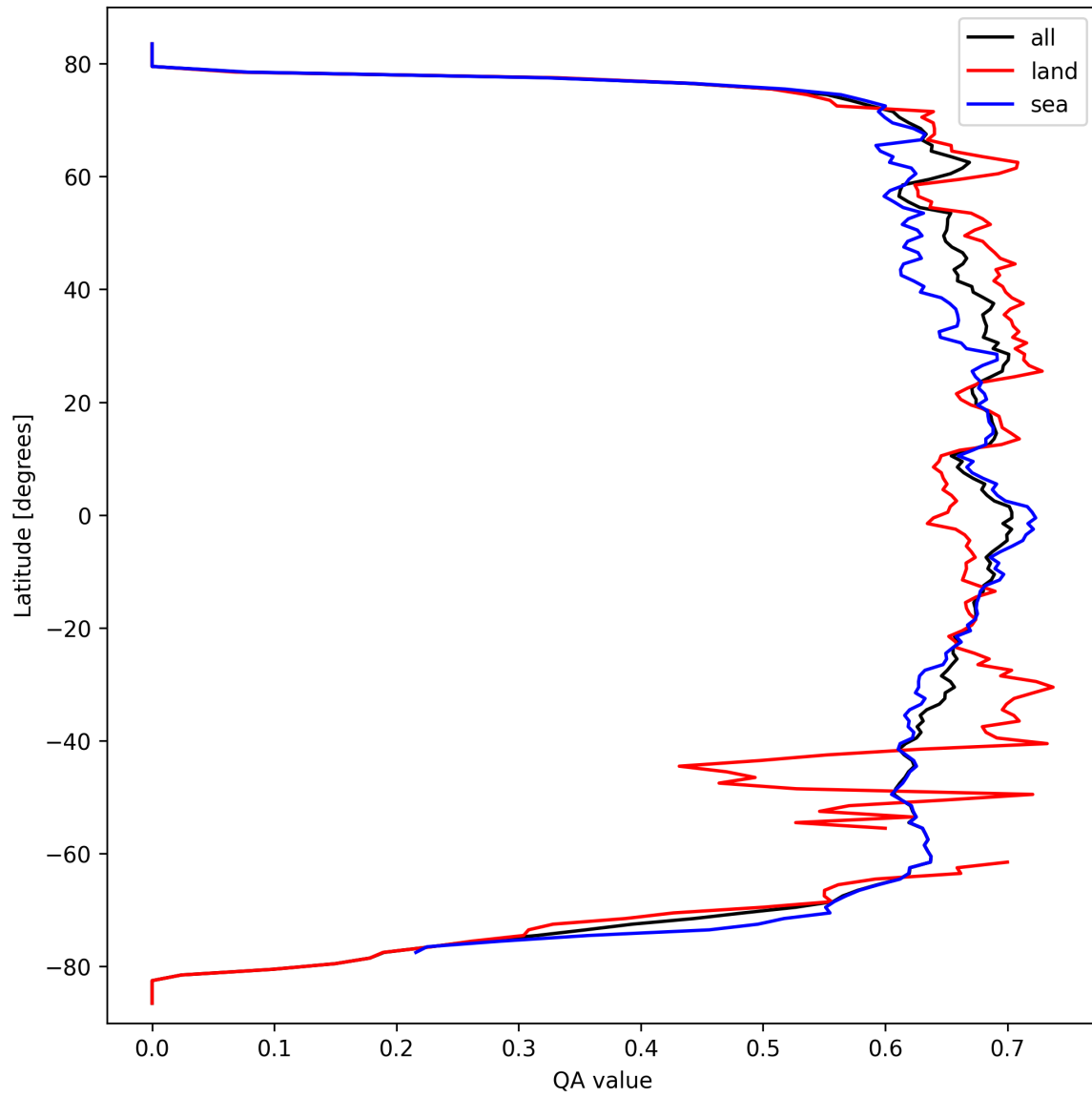
Figure 9: Zonal average of “QA value” for 2024-09-25 to 2024-09-27.
