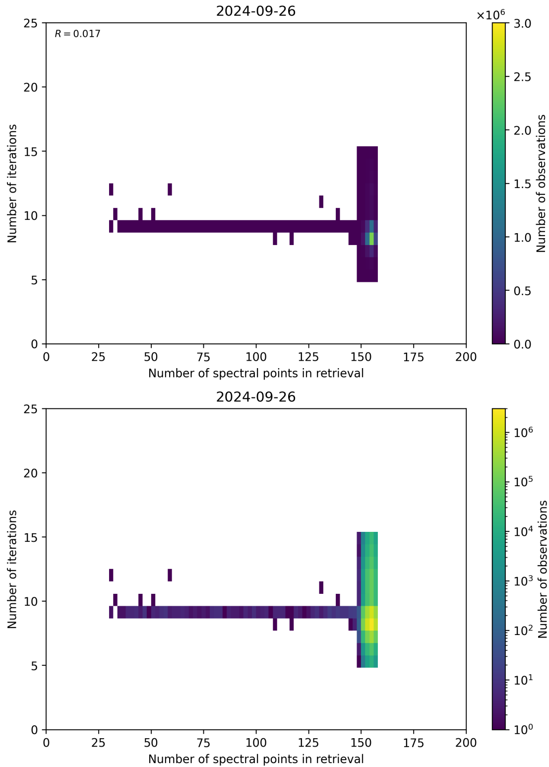
Figure 60: Scatter density plot of “Number of spectral points in retrieval” against “Number of iterations” for 2024-09-25 to 2024-09-27.
