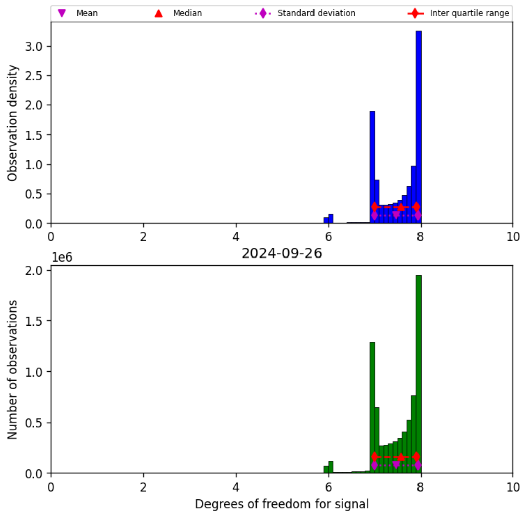
Figure 23: Histogram of “Degrees of freedom for signal” for 2024-09-25 to 2024-09-27
