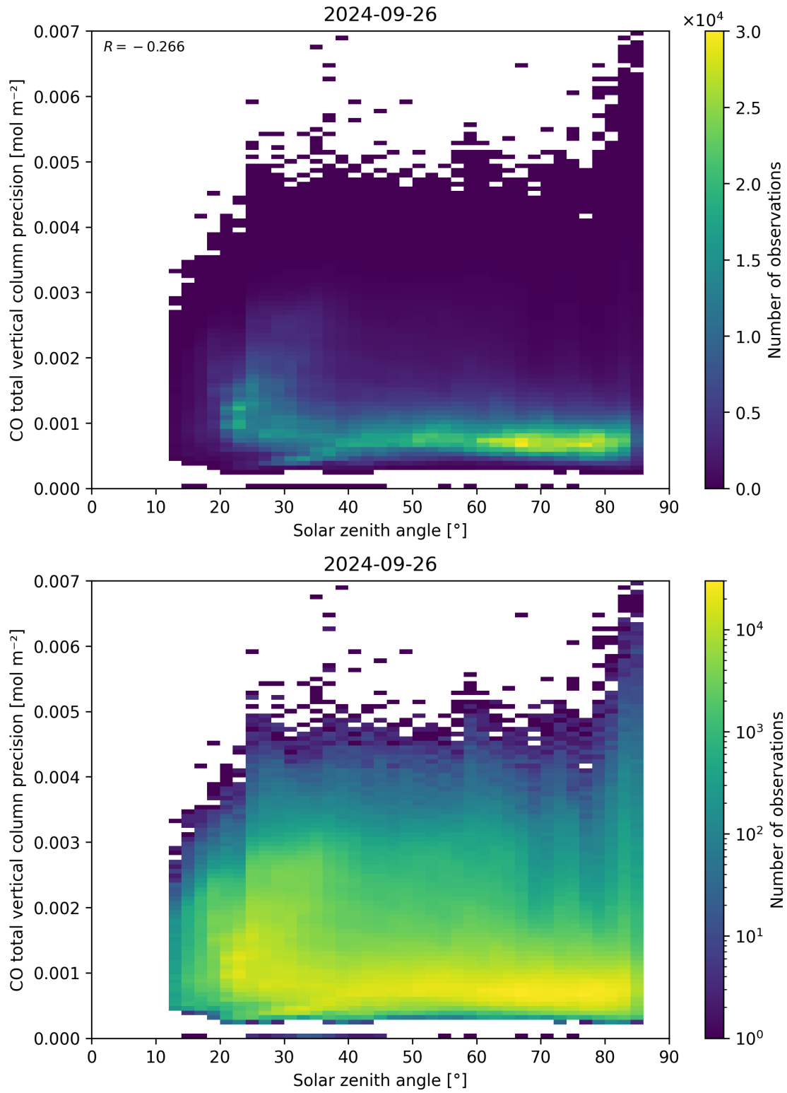
Figure 63: Scatter density plot of “Solar zenith angle” against “CO total vertical column precision” for 2024-09-25 to 2024-09-27.
