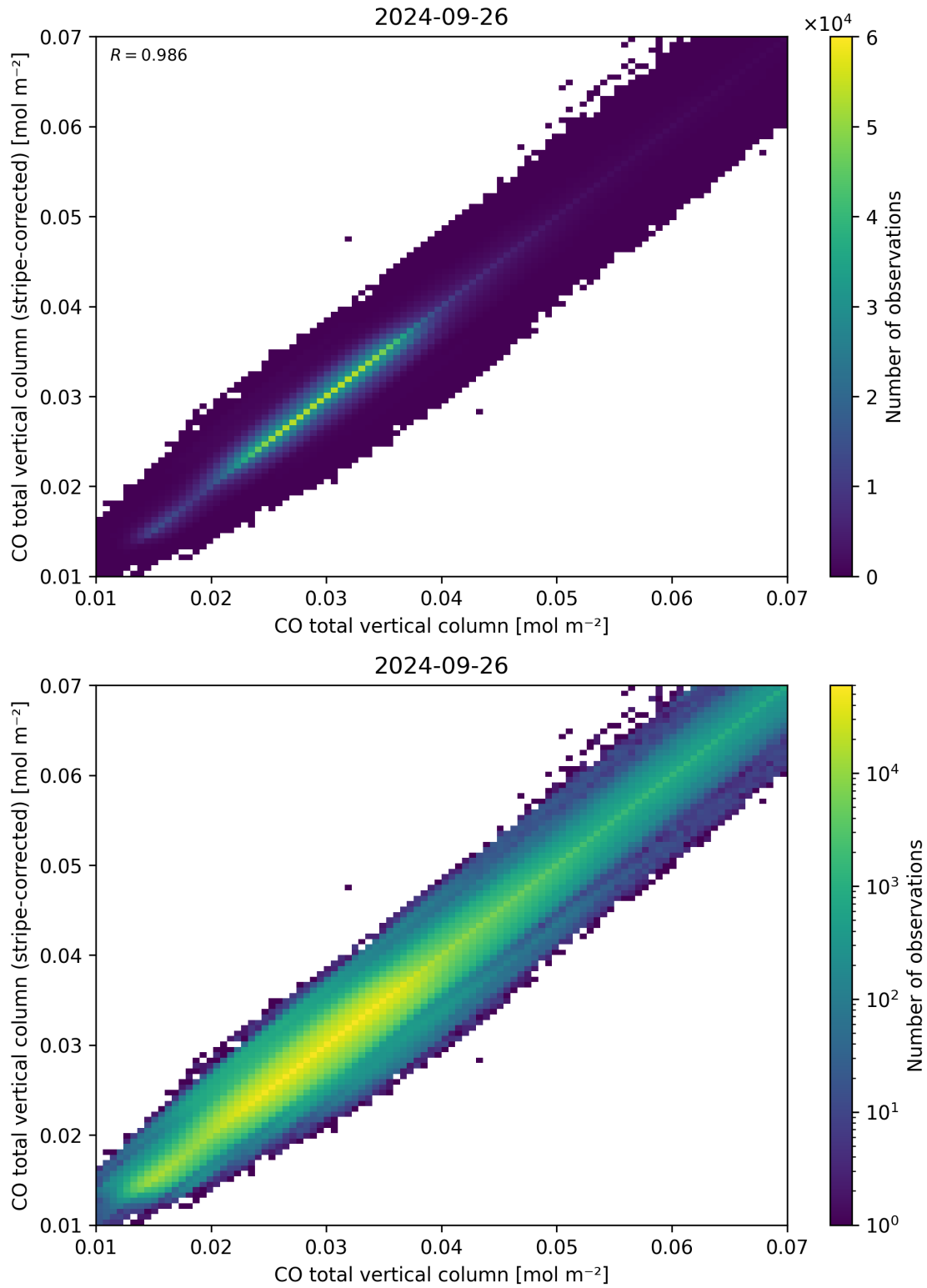
Figure 33: Scatter density plot of “CO total vertical column” against “CO total vertical column (stripe-corrected)” for 2024-09-25 to 2024-09-27.
