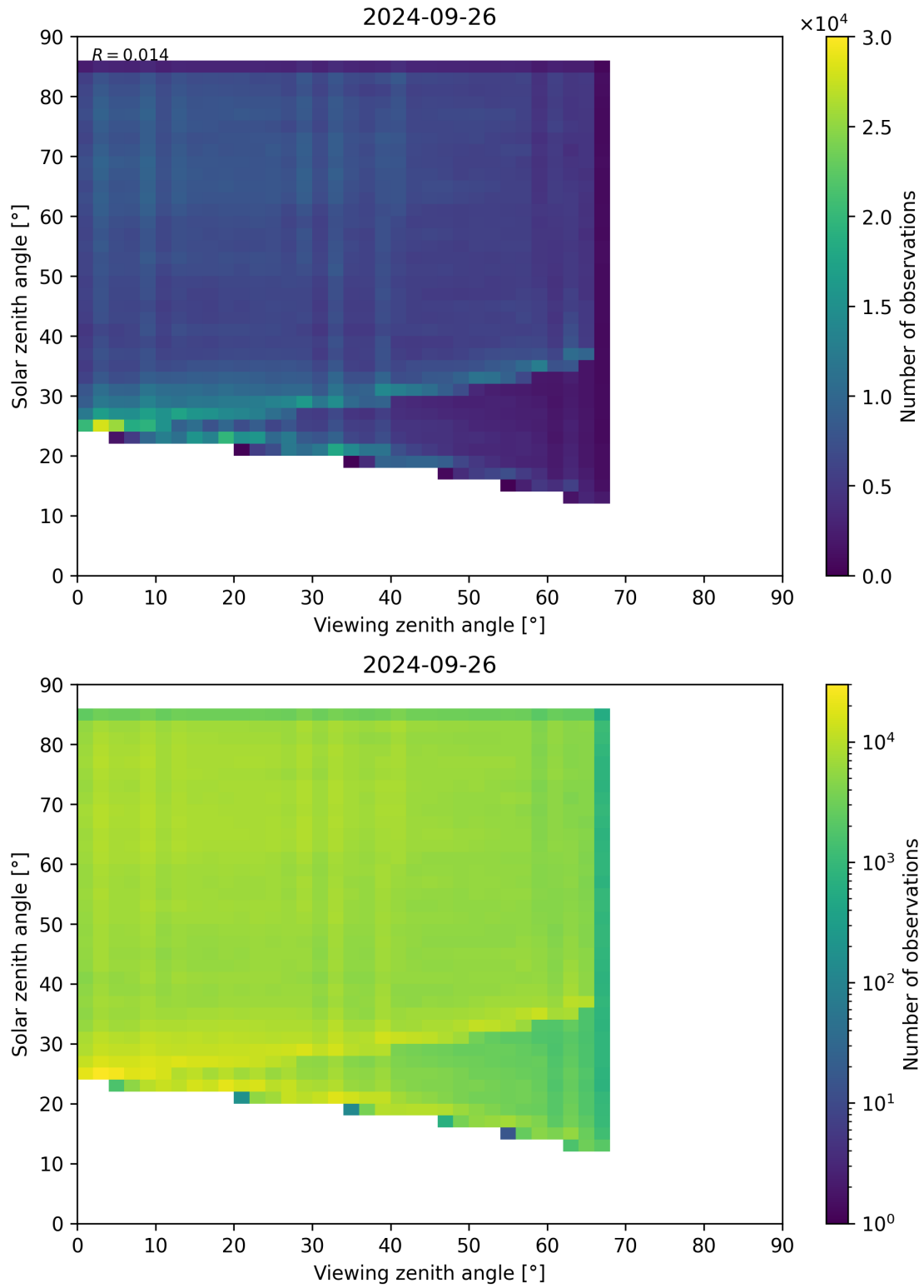
Figure 77: Scatter density plot of “Viewing zenith angle” against “Solar zenith angle” for 2024-09-25 to 2024-09-27.
