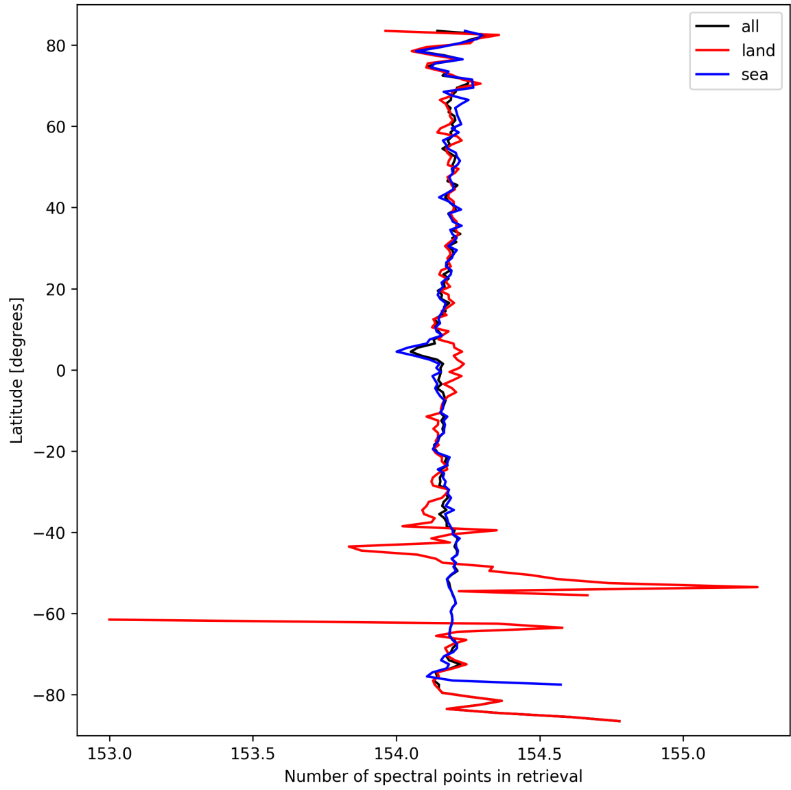
Figure 13: Zonal average of “Number of spectral points in retrieval” for 2024-09-25 to 2024-09-27.
