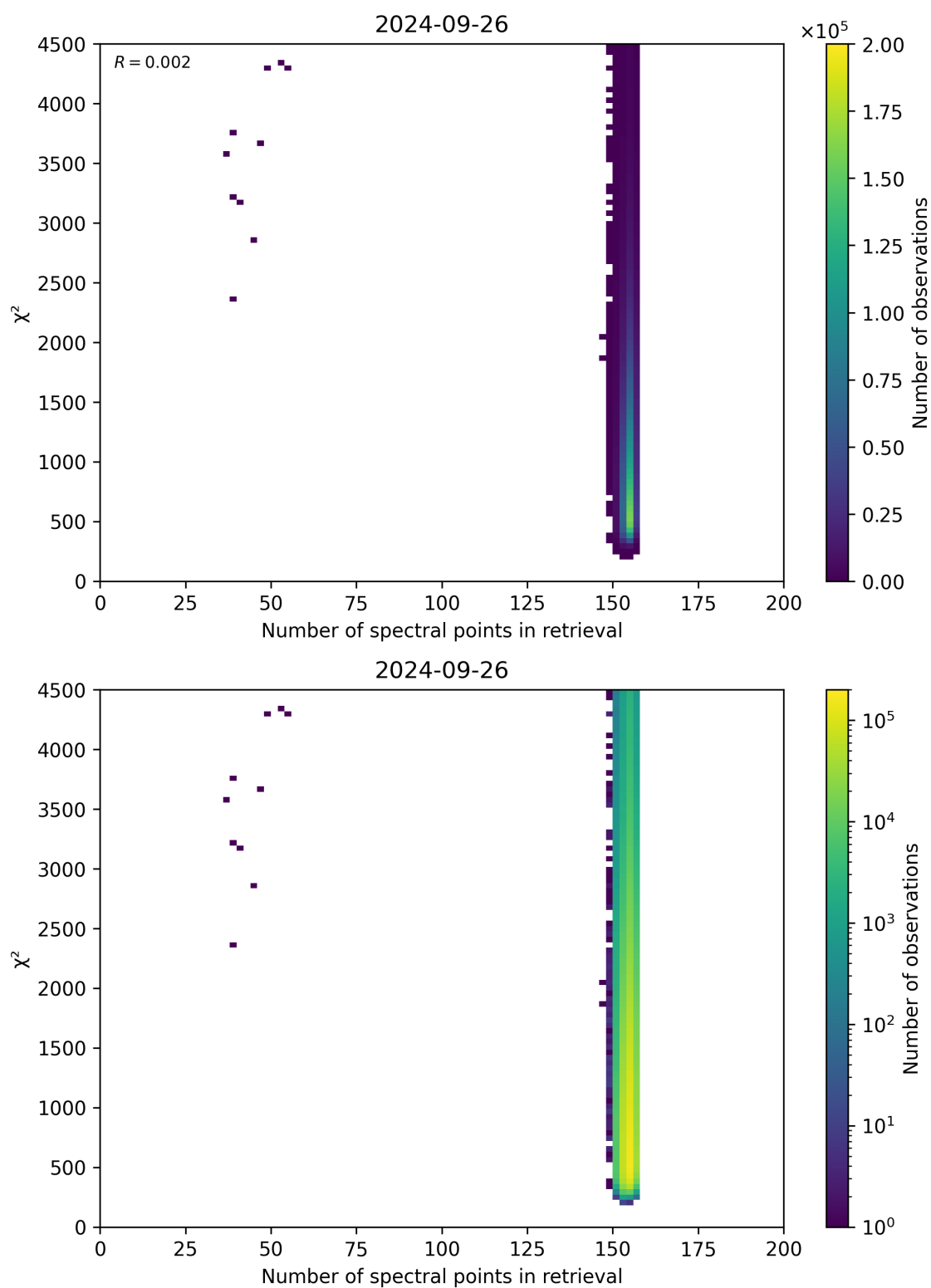
Figure 58: Scatter density plot of “Number of spectral points in retrieval” against “ \chi^2 ” for 2024-09-25 to 2024-09-27.
