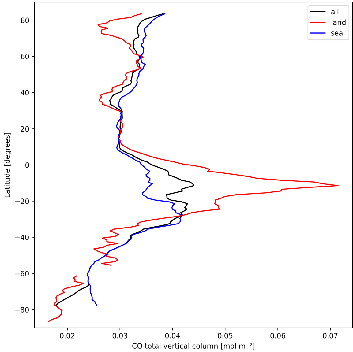
Figure 10: Zonal average of “CO total vertical column” for 2024-09-25 to 2024-09-27.
