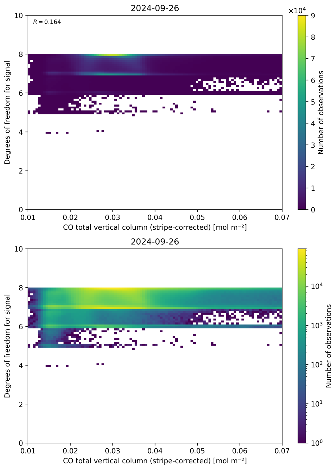
Figure 38: Scatter density plot of “CO total vertical column (stripe-corrected)” against “Degrees of freedom for signal” for 2024-09-25 to 2024-09-27.
