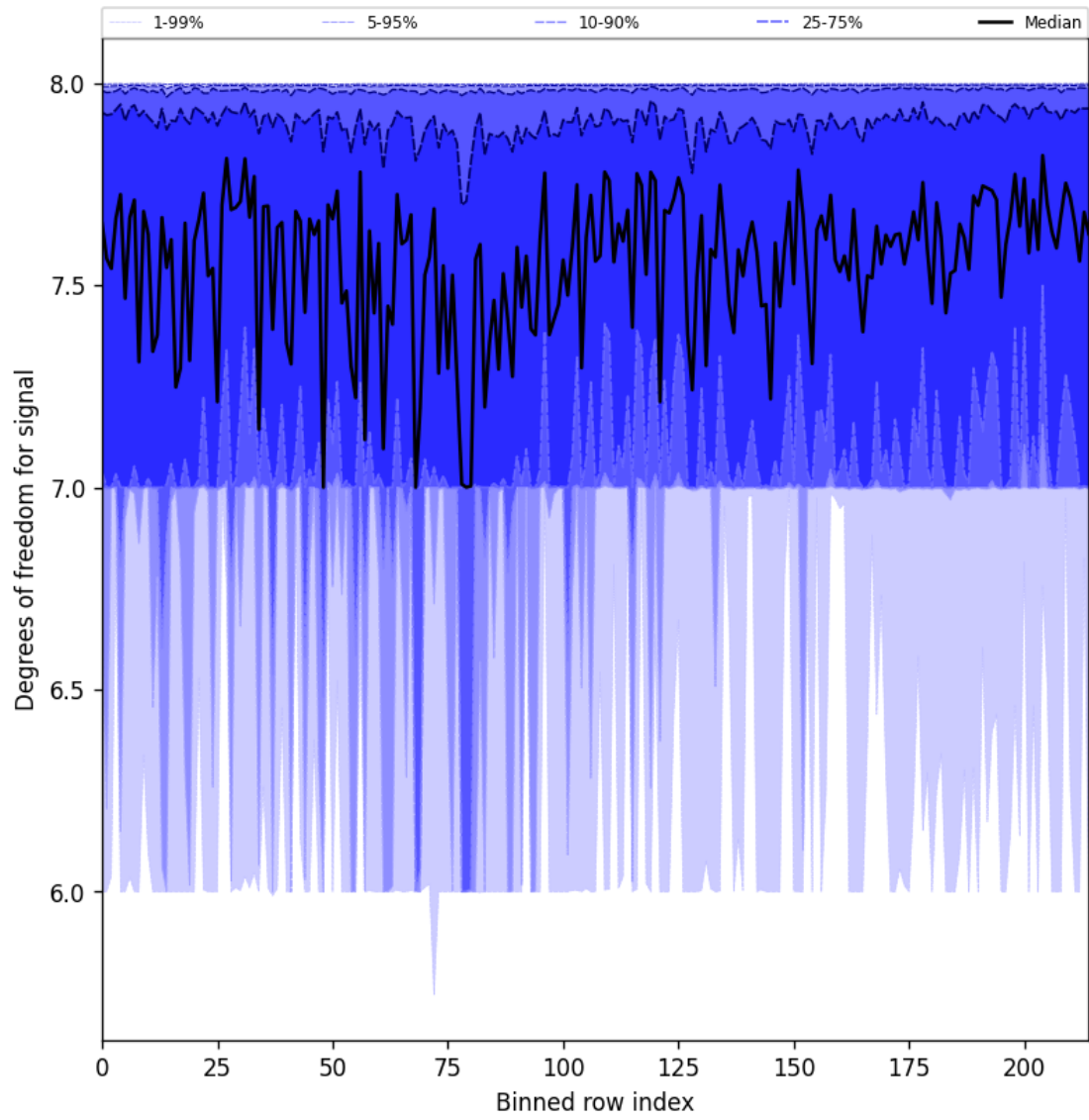
Figure 31: Along track statistics of “Degrees of freedom for signal” for 2024-09-25 to 2024-09-27
