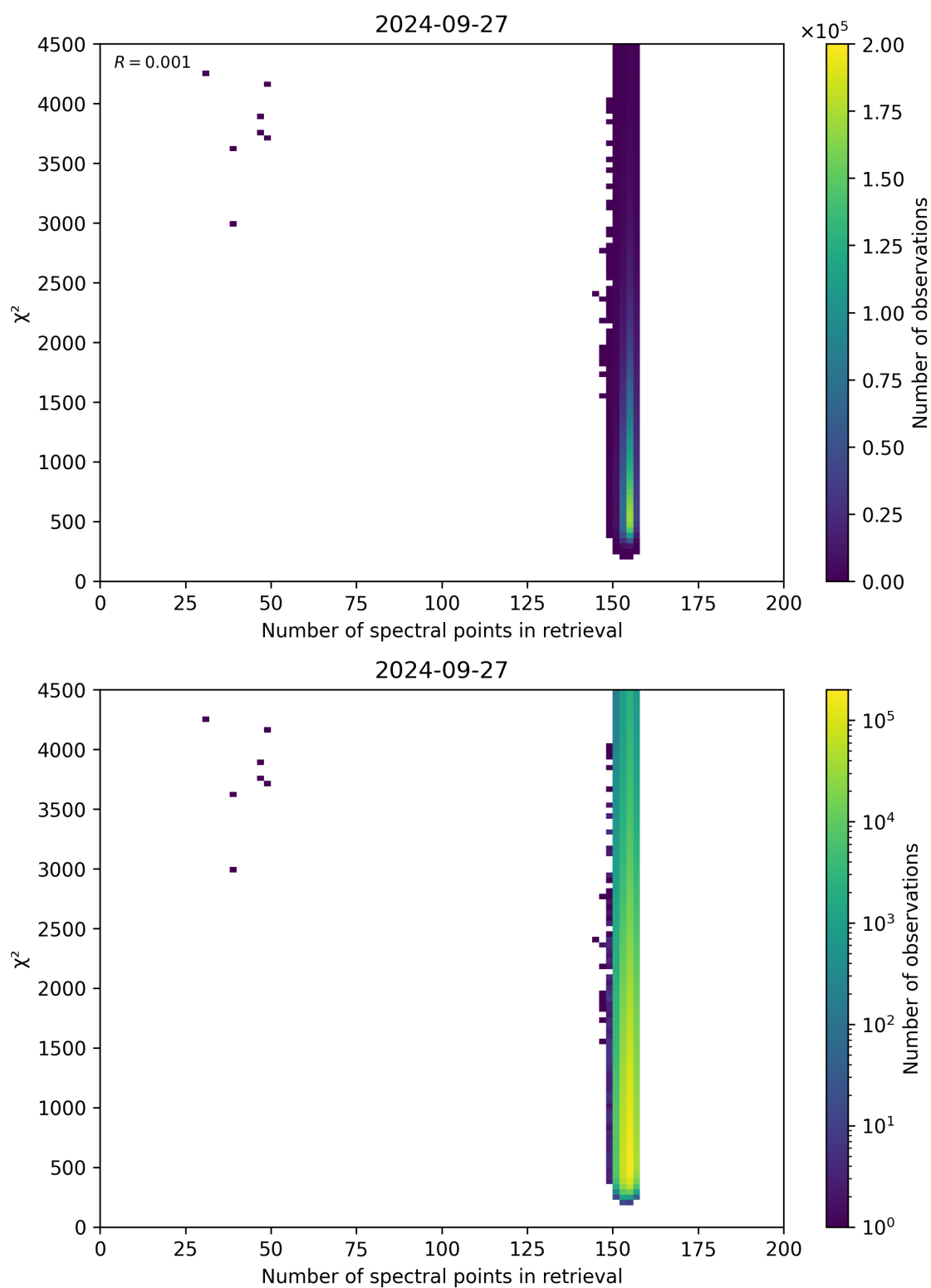
Figure 58: Scatter density plot of “Number of spectral points in retrieval” against “ \chi^2 ” for 2024-09-26 to 2024-09-28.
