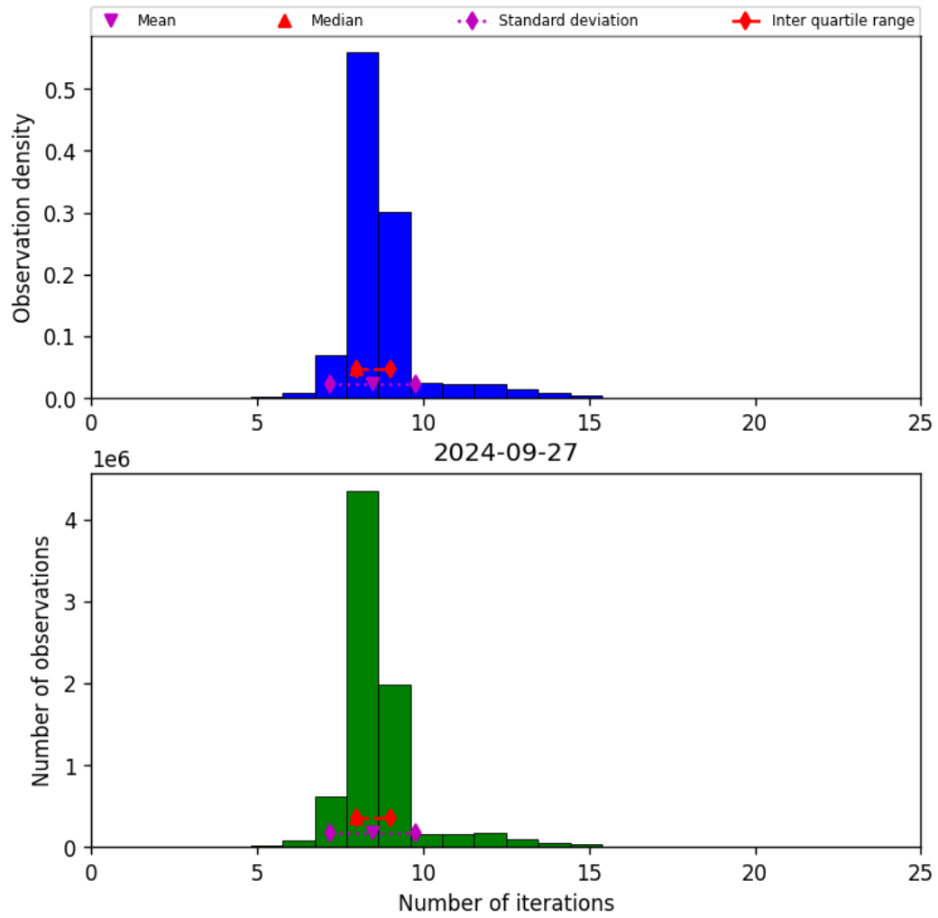
Figure 24: Histogram of “Number of iterations” for 2024-09-26 to 2024-09-28
