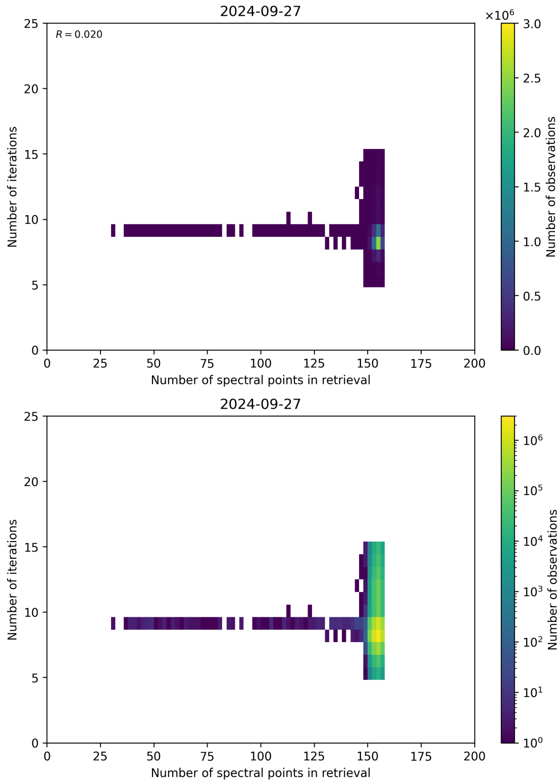
Figure 60: Scatter density plot of “Number of spectral points in retrieval” against “Number of iterations” for 2024-09-26 to 2024-09-28.
