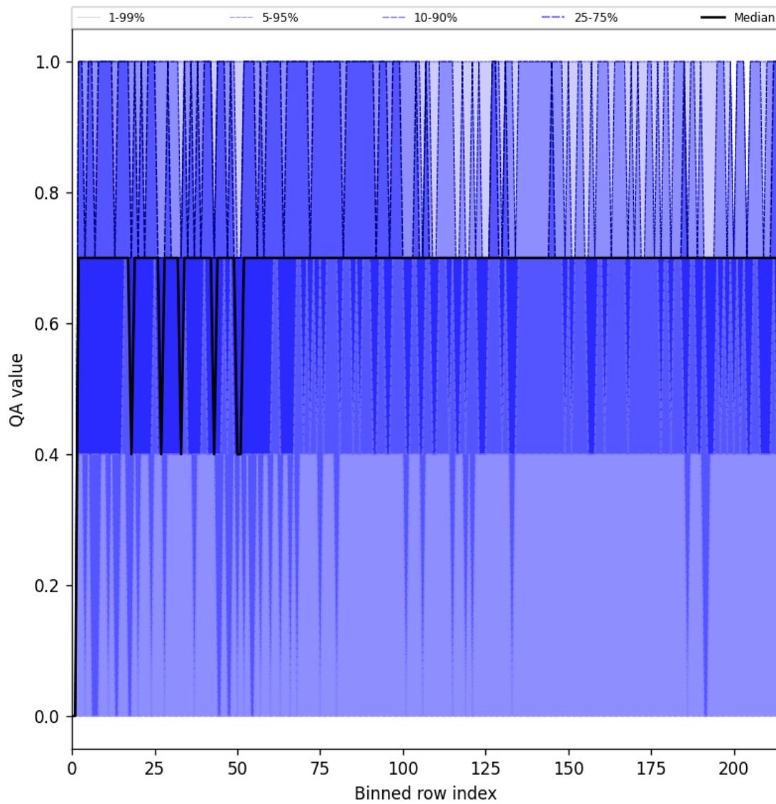
Figure 25: Along track statistics of “QA value” for 2024-09-26 to 2024-09-28
