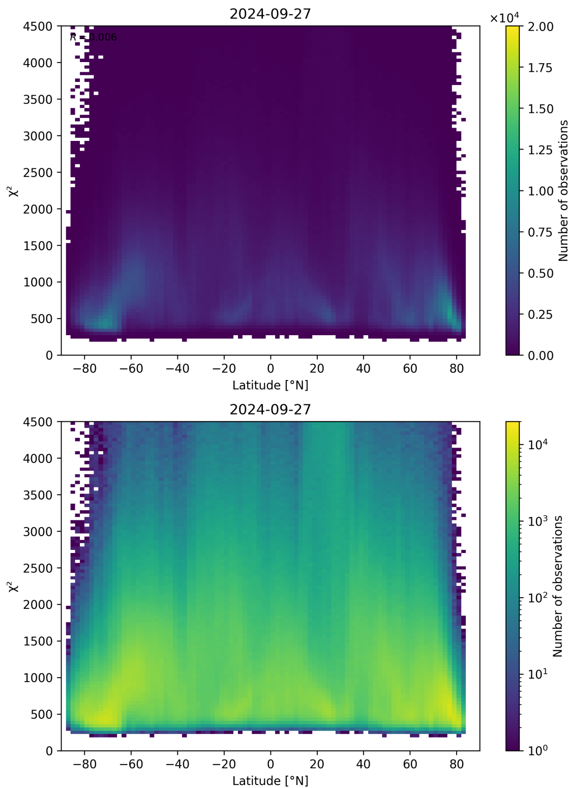
Figure 54: Scatter density plot of “Latitude” against “ \chi^2 ” for 2024-09-26 to 2024-09-28.
