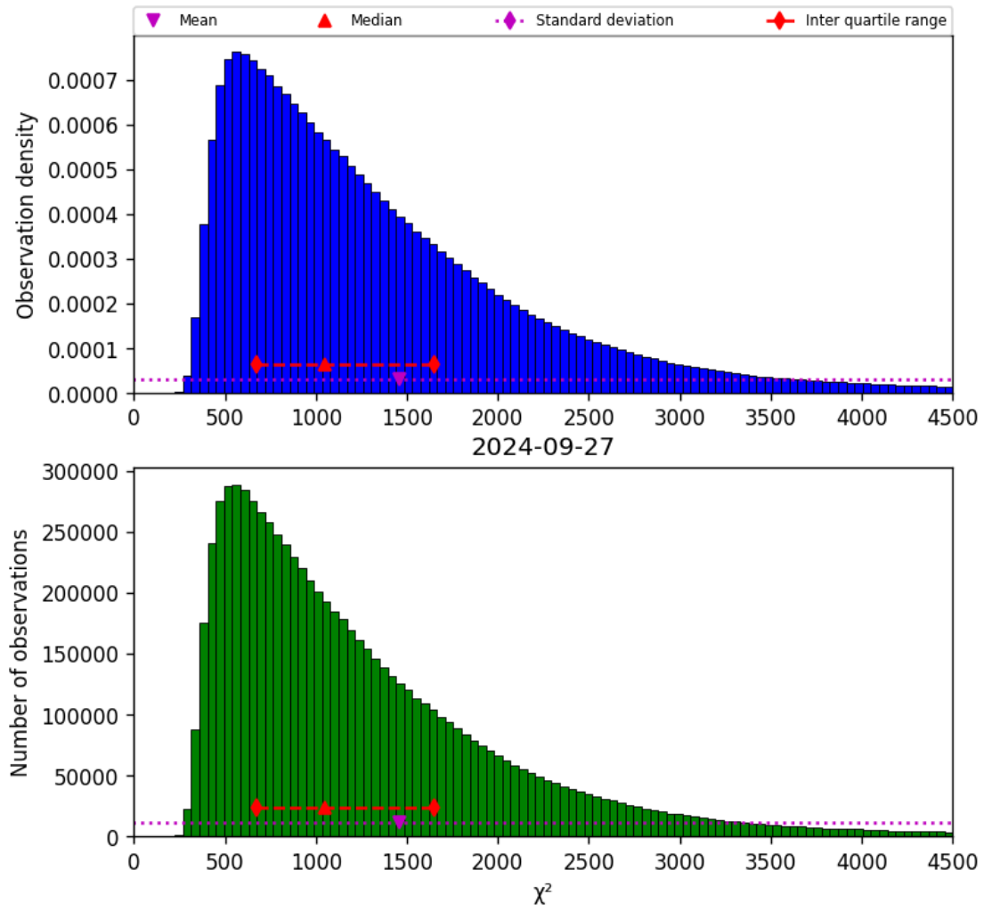
Figure 22: Histogram of “ \chi^2 ” for 2024-09-26 to 2024-09-28
