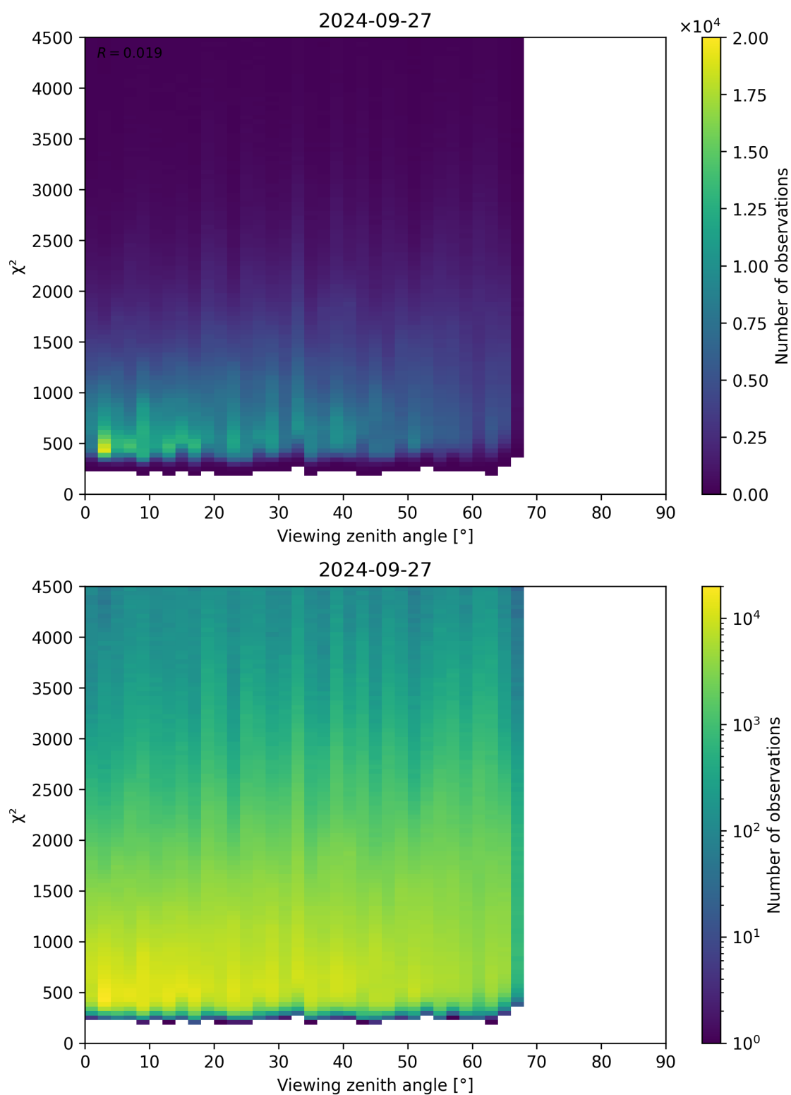
Figure 72: Scatter density plot of “Viewing zenith angle” against “ \chi^2 ” for 2024-09-26 to 2024-09-28.
