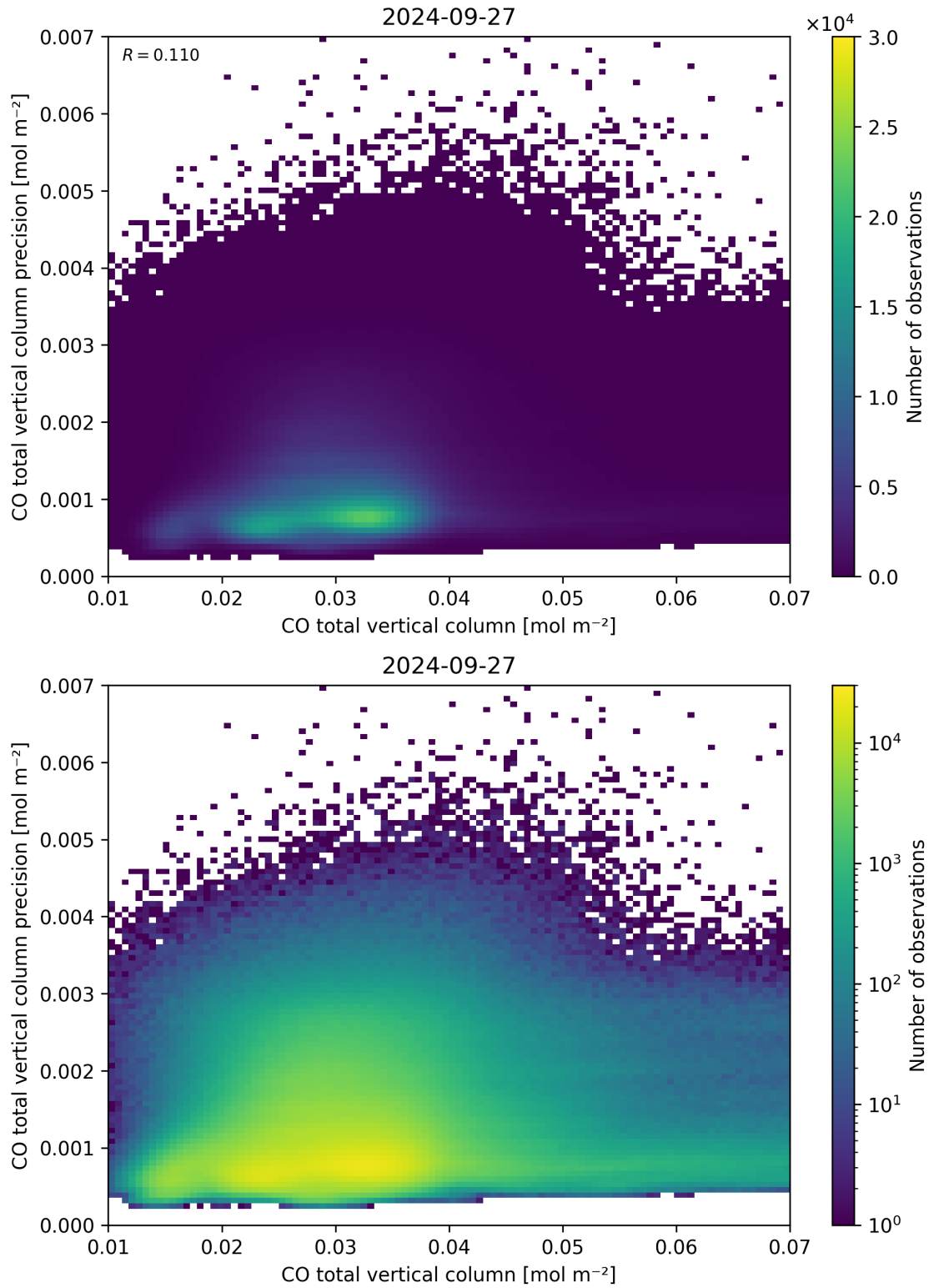
Figure 34: Scatter density plot of “CO total vertical column” against “CO total vertical column precision” for 2024-09-26 to 2024-09-28.
