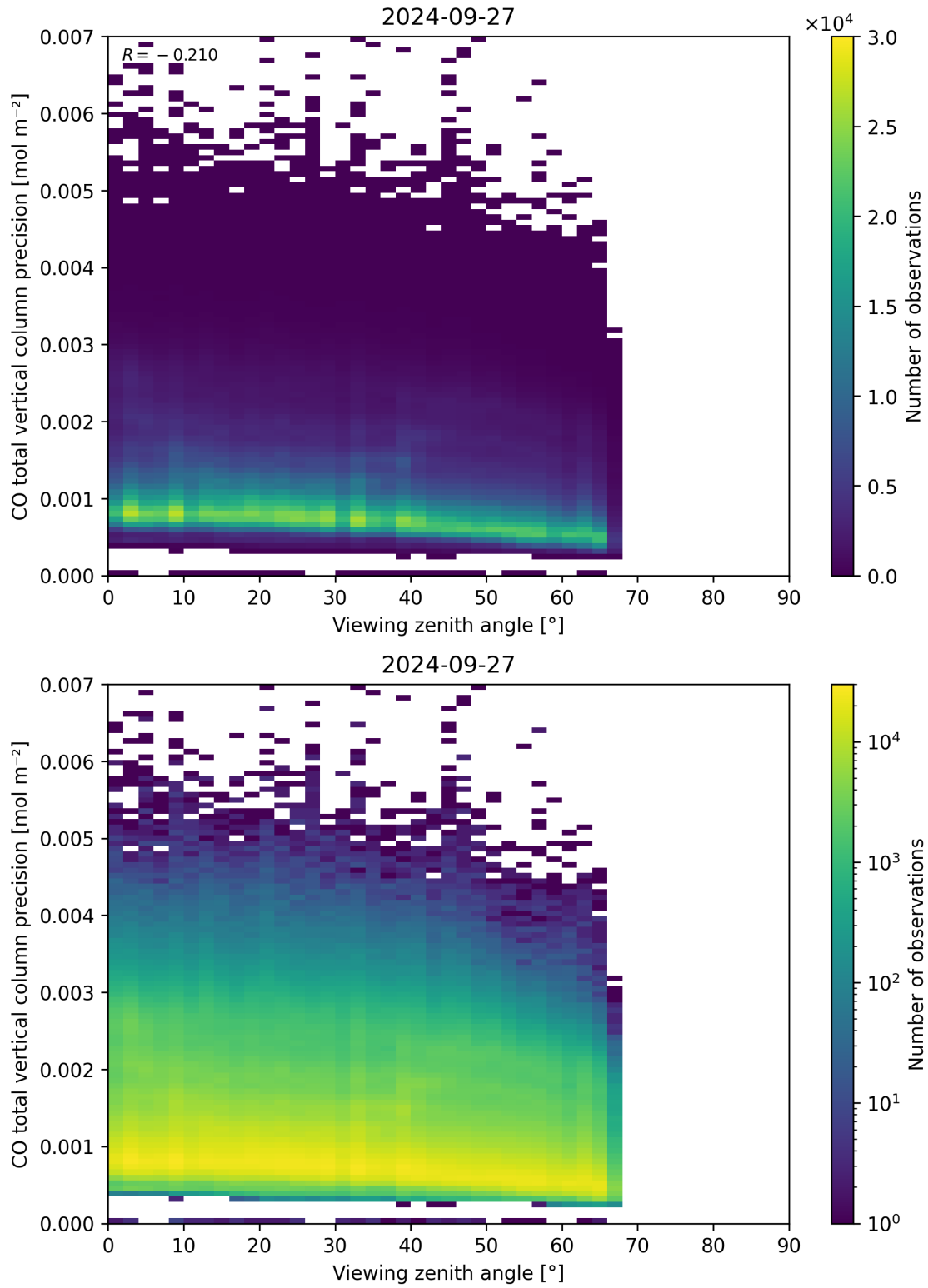
Figure 71: Scatter density plot of “Viewing zenith angle” against “CO total vertical column precision” for 2024-09-26 to 2024-09-28.
