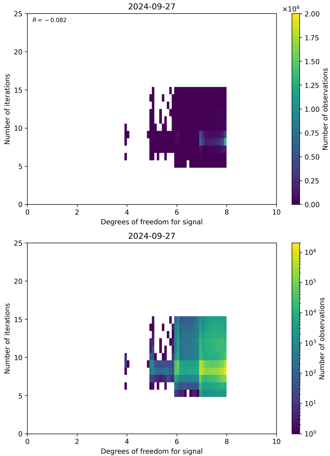
Figure 50: Scatter density plot of “Degrees of freedom for signal” against “Number of iterations” for 2024-09-26 to 2024-09-28.
