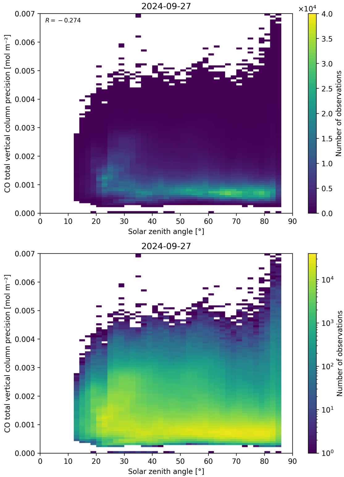
Figure 63: Scatter density plot of “Solar zenith angle” against “CO total vertical column precision” for 2024-09-26 to 2024-09-28.
