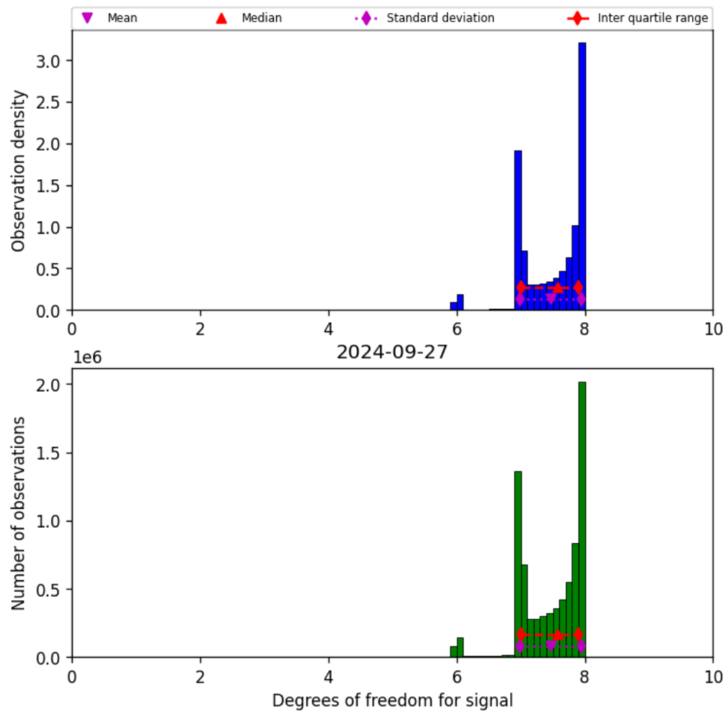
Figure 23: Histogram of “Degrees of freedom for signal” for 2024-09-26 to 2024-09-28
