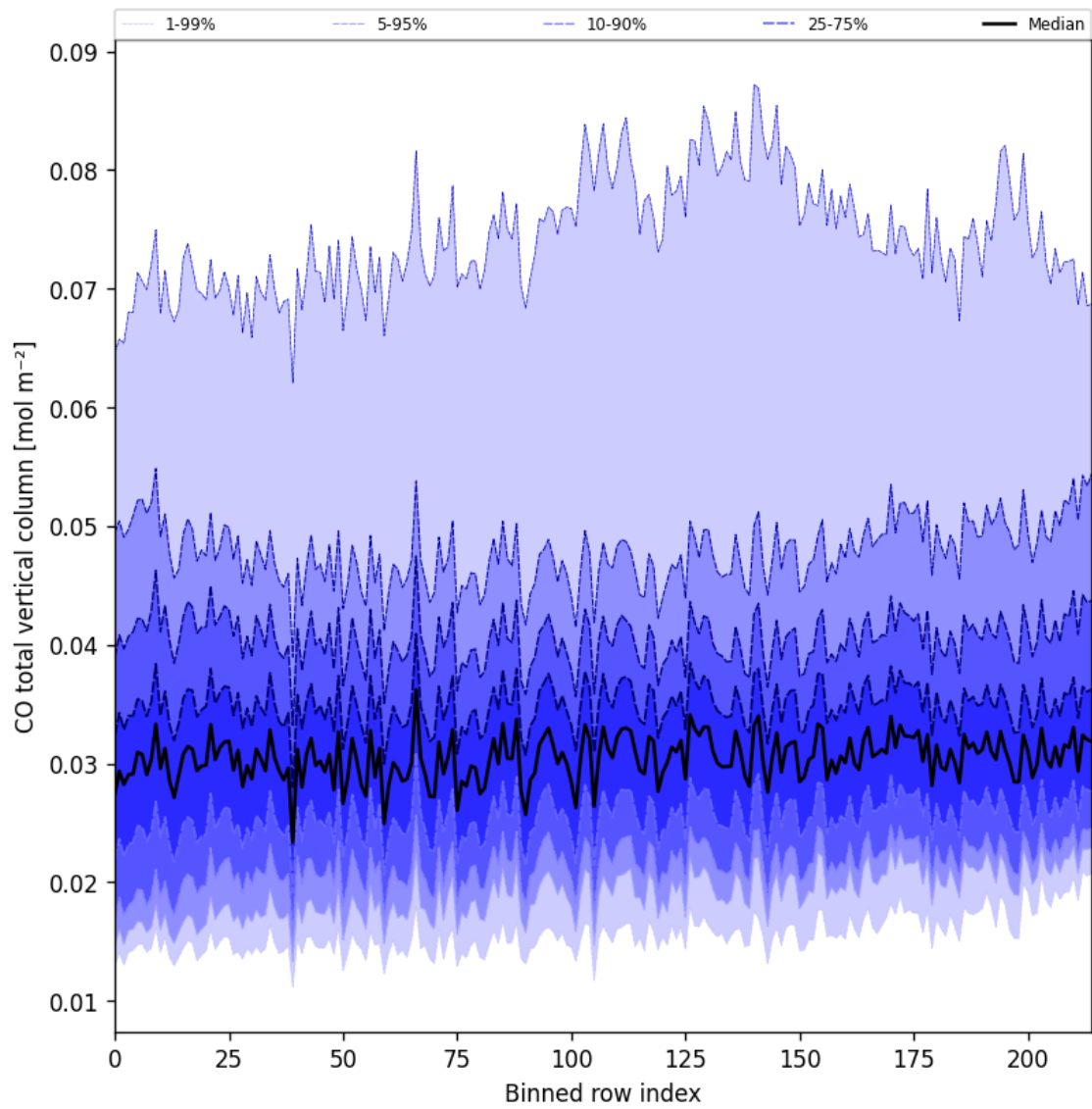
Figure 26: Along track statistics of “CO total vertical column” for 2024-09-26 to 2024-09-28
