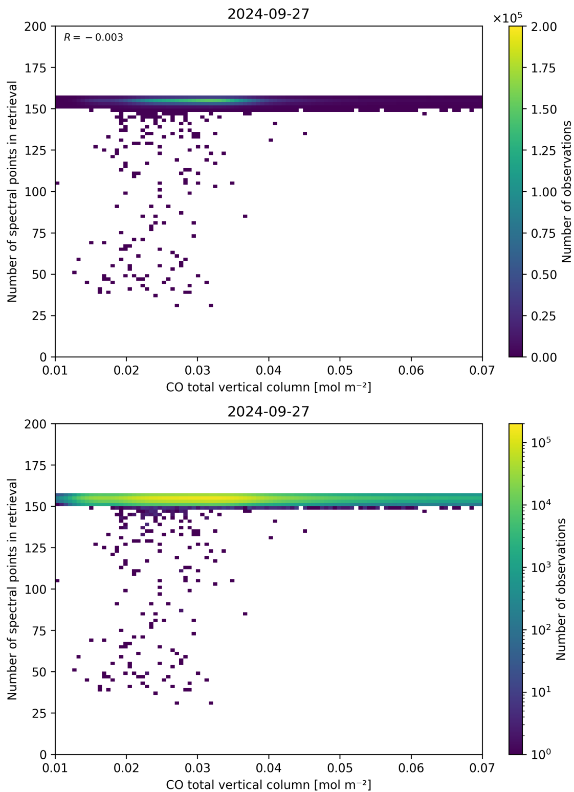
Figure 43: Scatter density plot of “CO total vertical column” against “Number of spectral points in retrieval” for 2024-09-26 to 2024-09-28.
