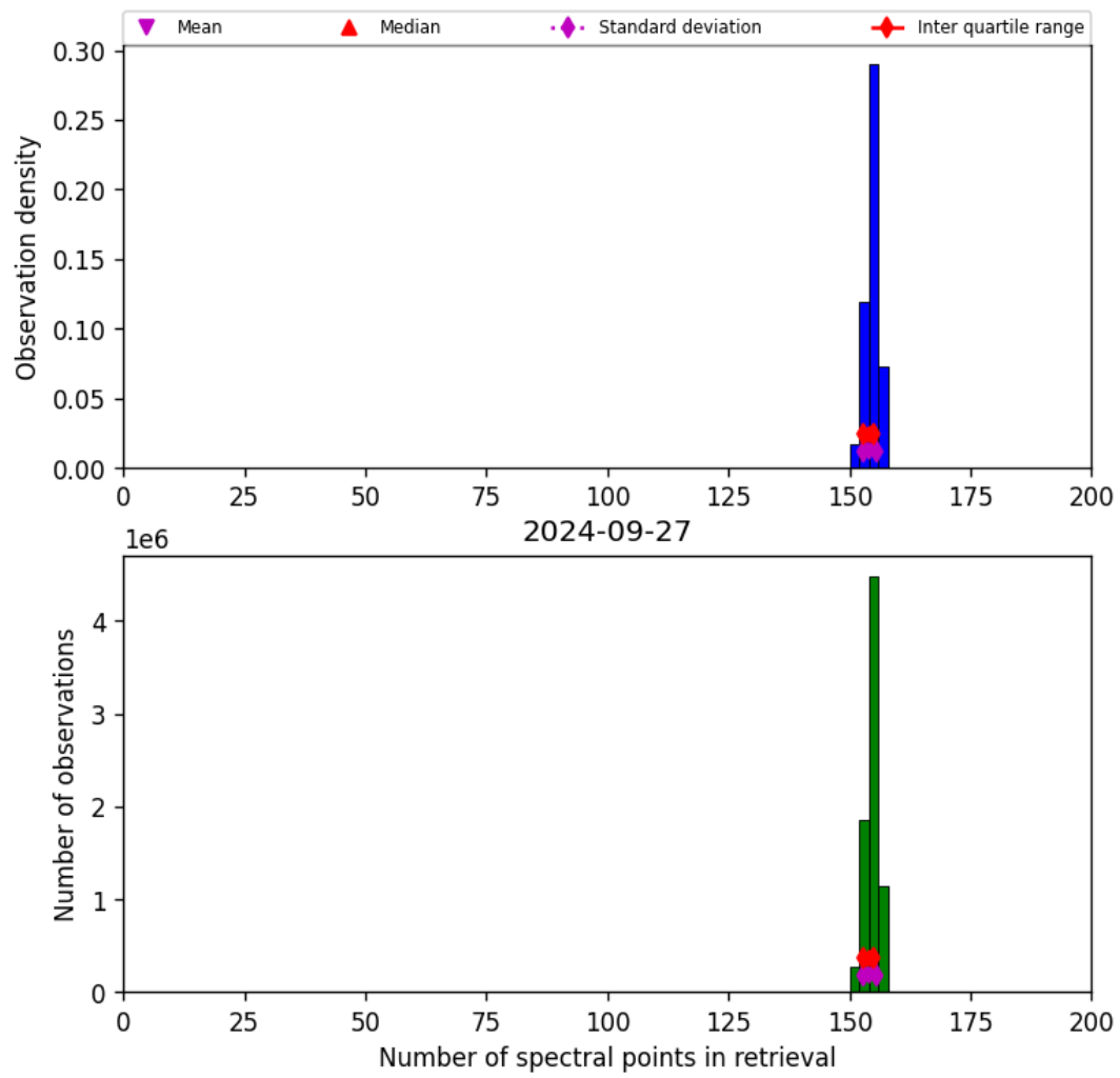
Figure 21: Histogram of “Number of spectral points in retrieval” for 2024-09-26 to 2024-09-28
