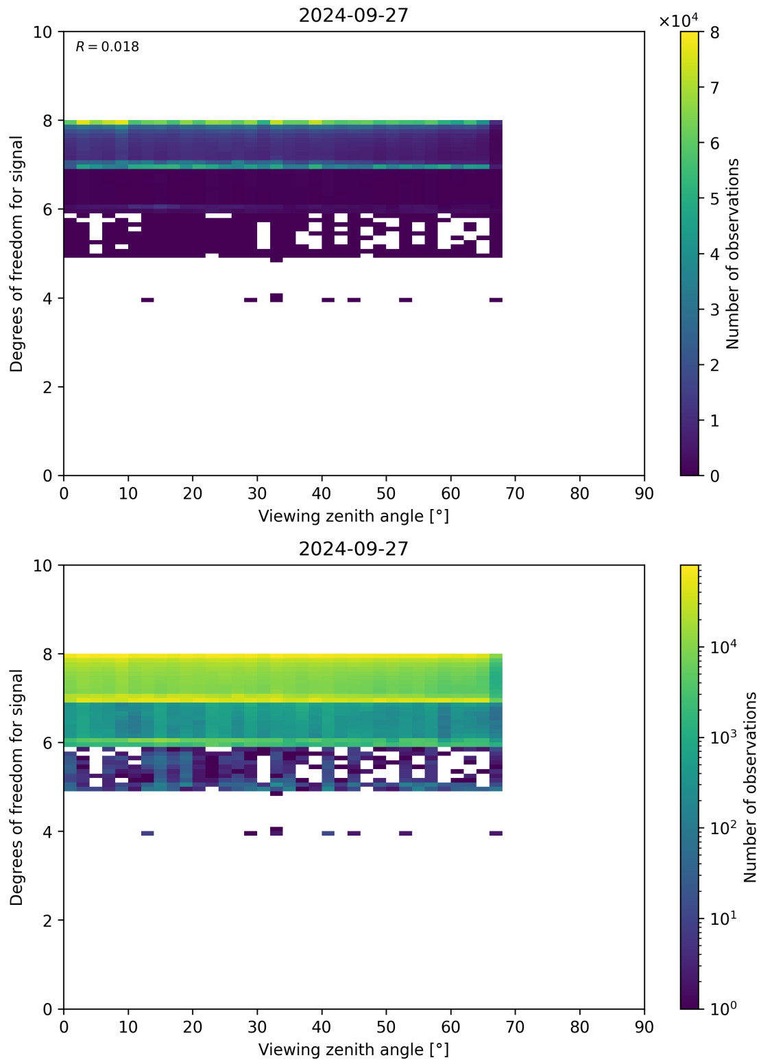
Figure 73: Scatter density plot of “Viewing zenith angle” against “Degrees of freedom for signal” for 2024-09-26 to 2024-09-28.
