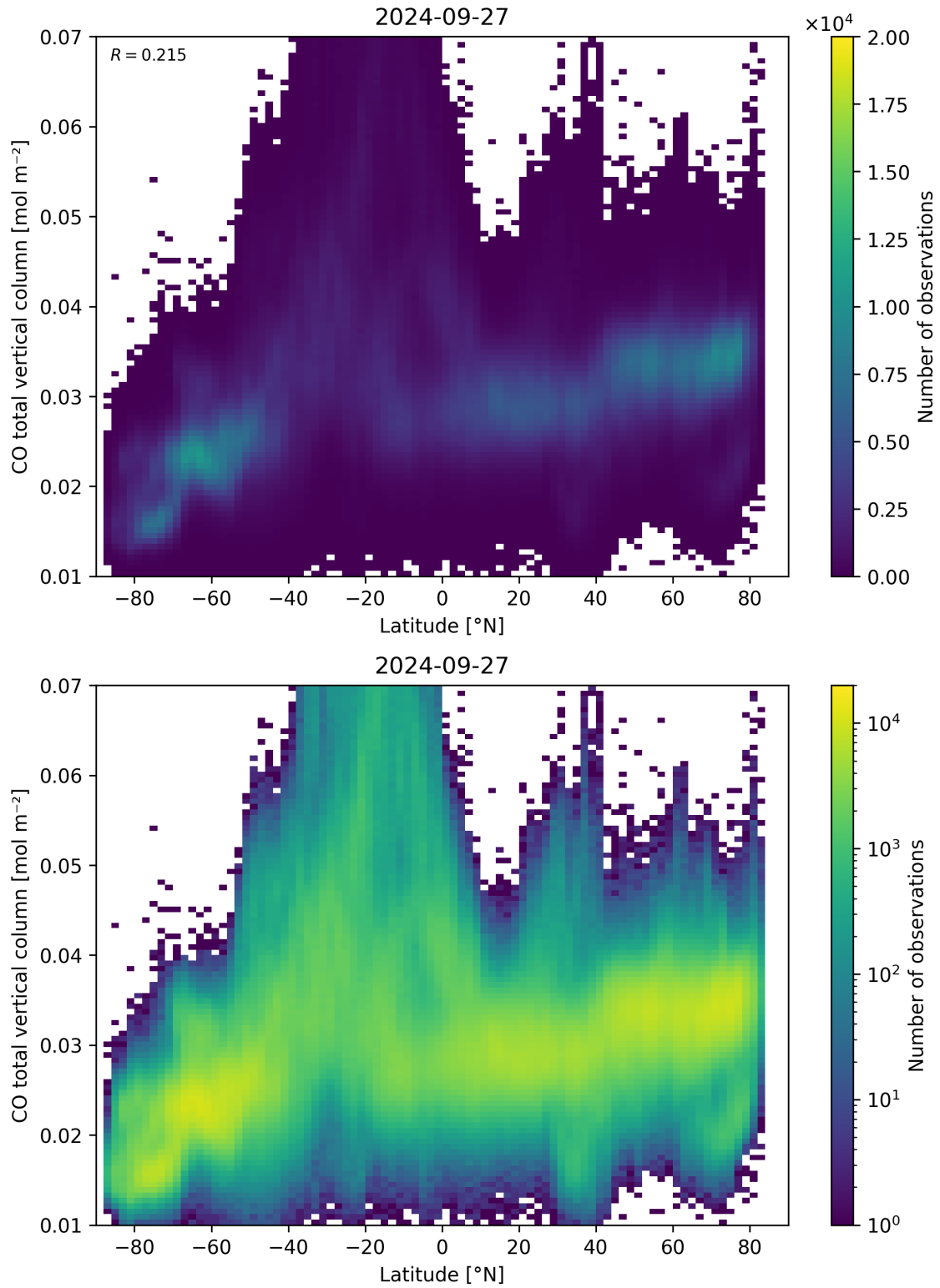
Figure 51: Scatter density plot of “Latitude” against “CO total vertical column” for 2024-09-26 to 2024-09-28.
