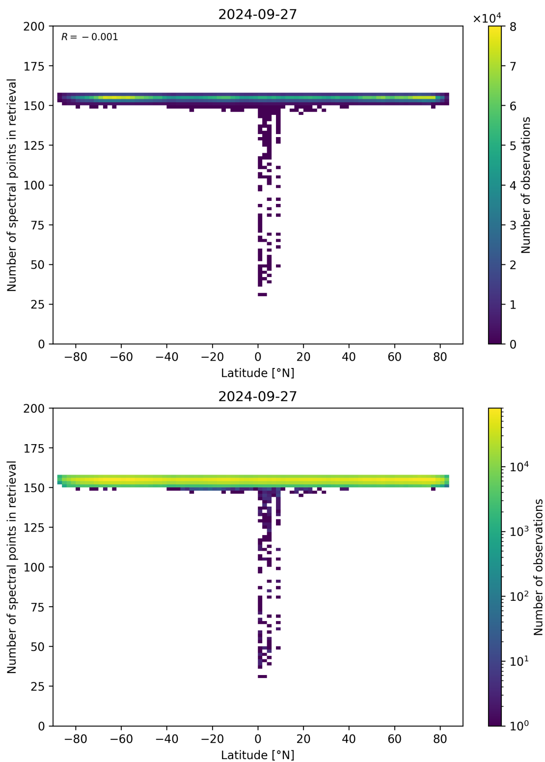
Figure 57: Scatter density plot of “Latitude” against “Number of spectral points in retrieval” for 2024-09-26 to 2024-09-28.
