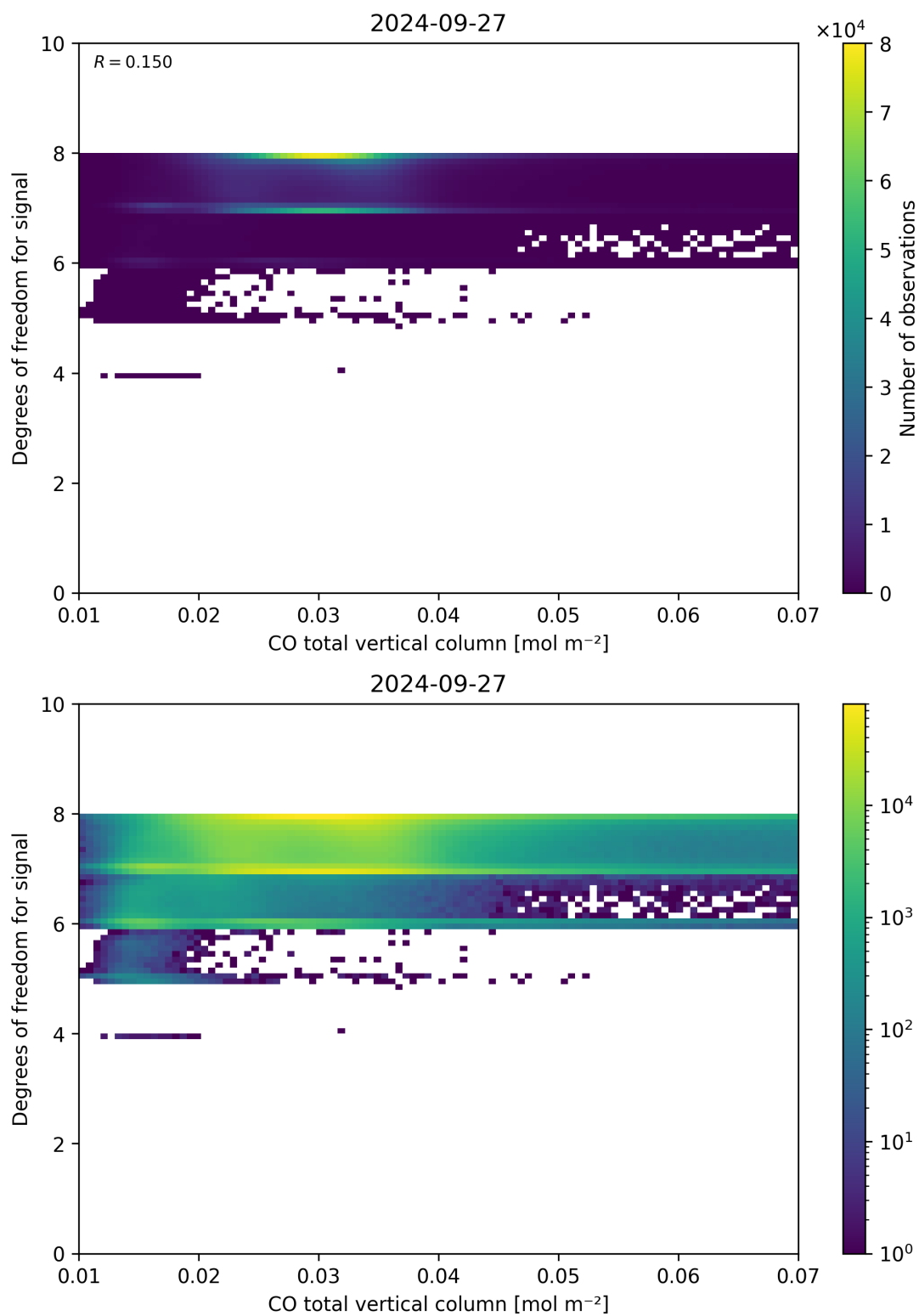
Figure 41: Scatter density plot of “CO total vertical column” against “Degrees of freedom for signal” for 2024-09-26 to 2024-09-28.
