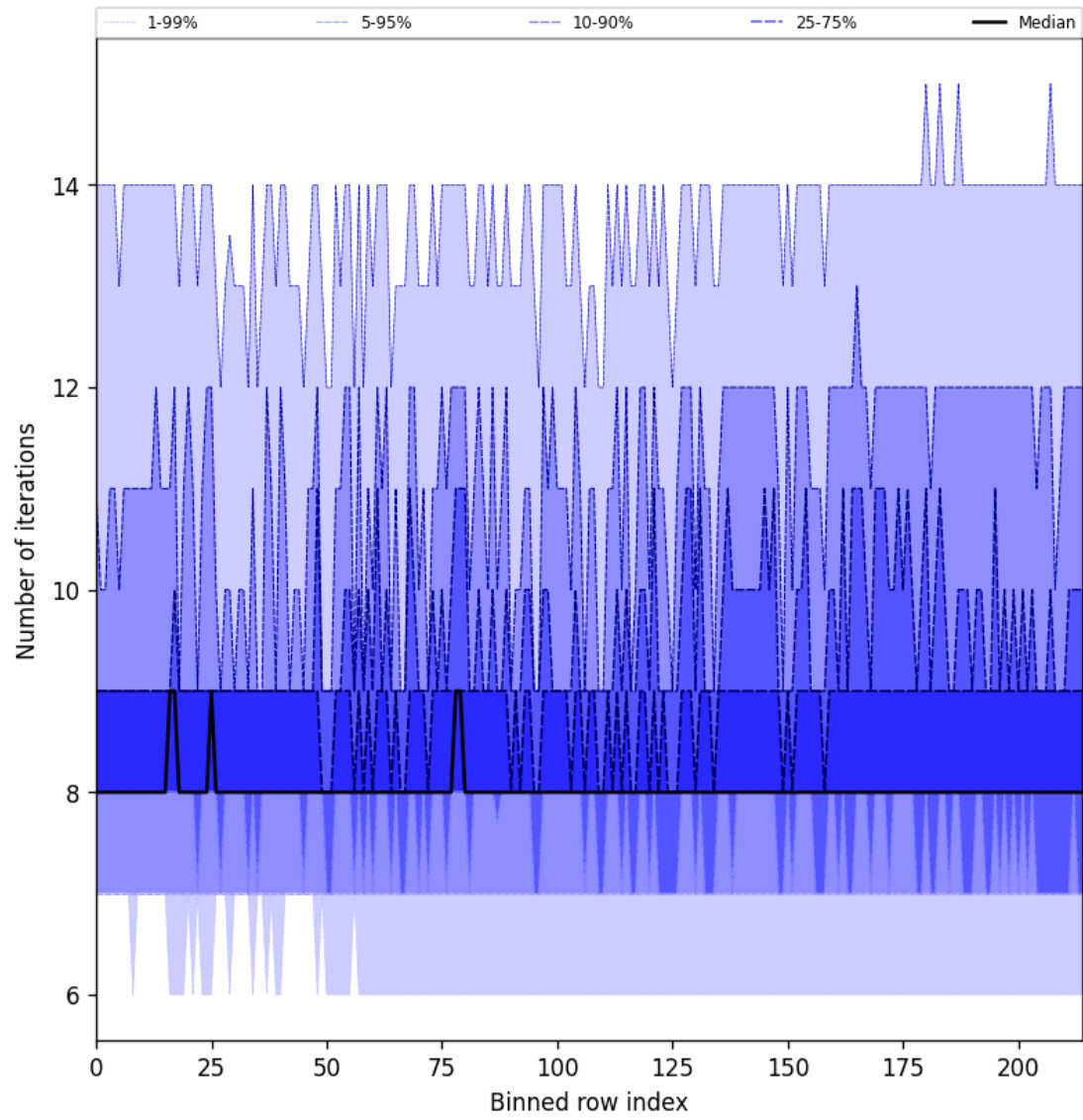
Figure 32: Along track statistics of “Number of iterations” for 2024-09-26 to 2024-09-28
