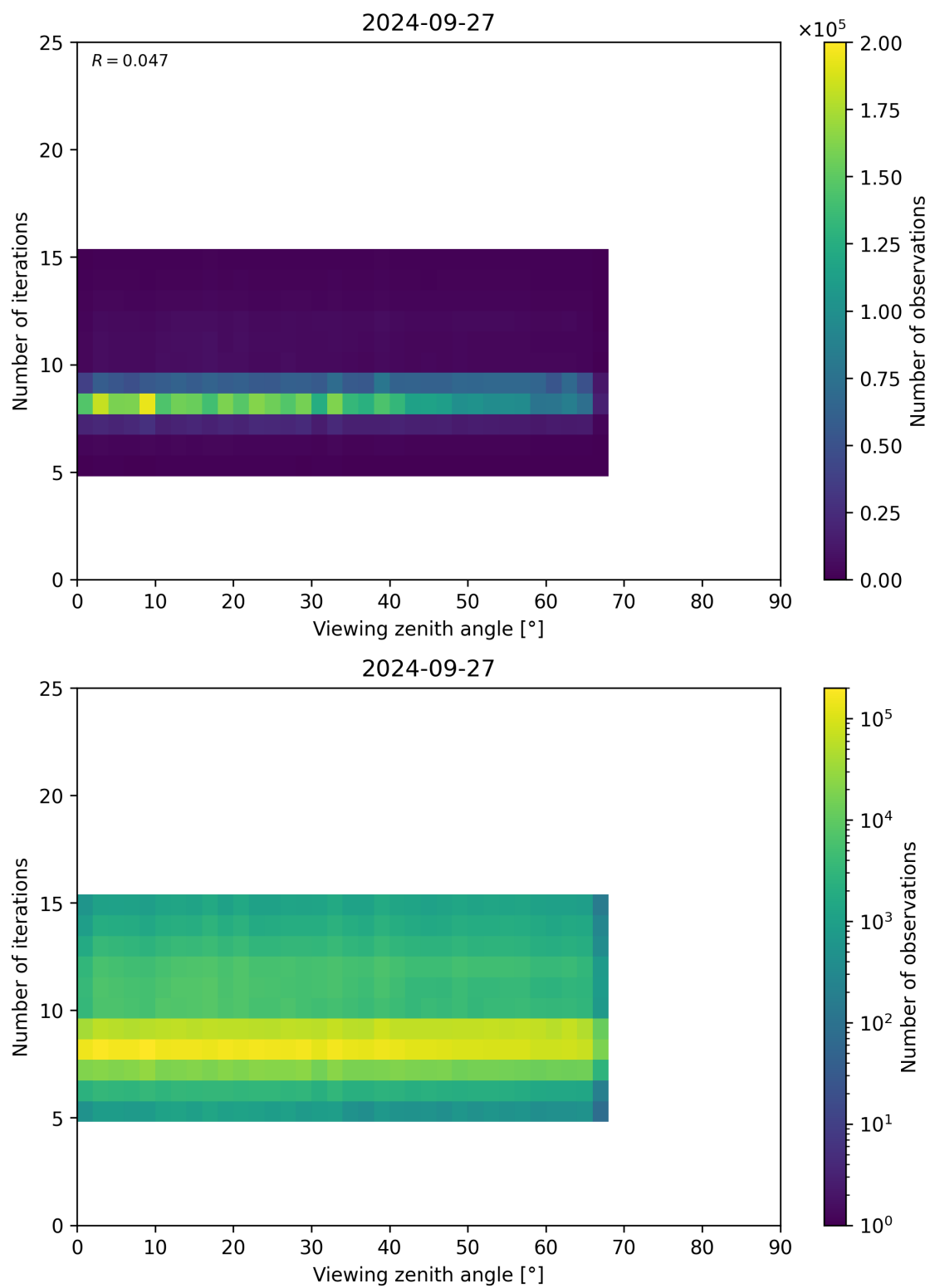
Figure 75: Scatter density plot of “Viewing zenith angle” against “Number of iterations” for 2024-09-26 to 2024-09-28.
