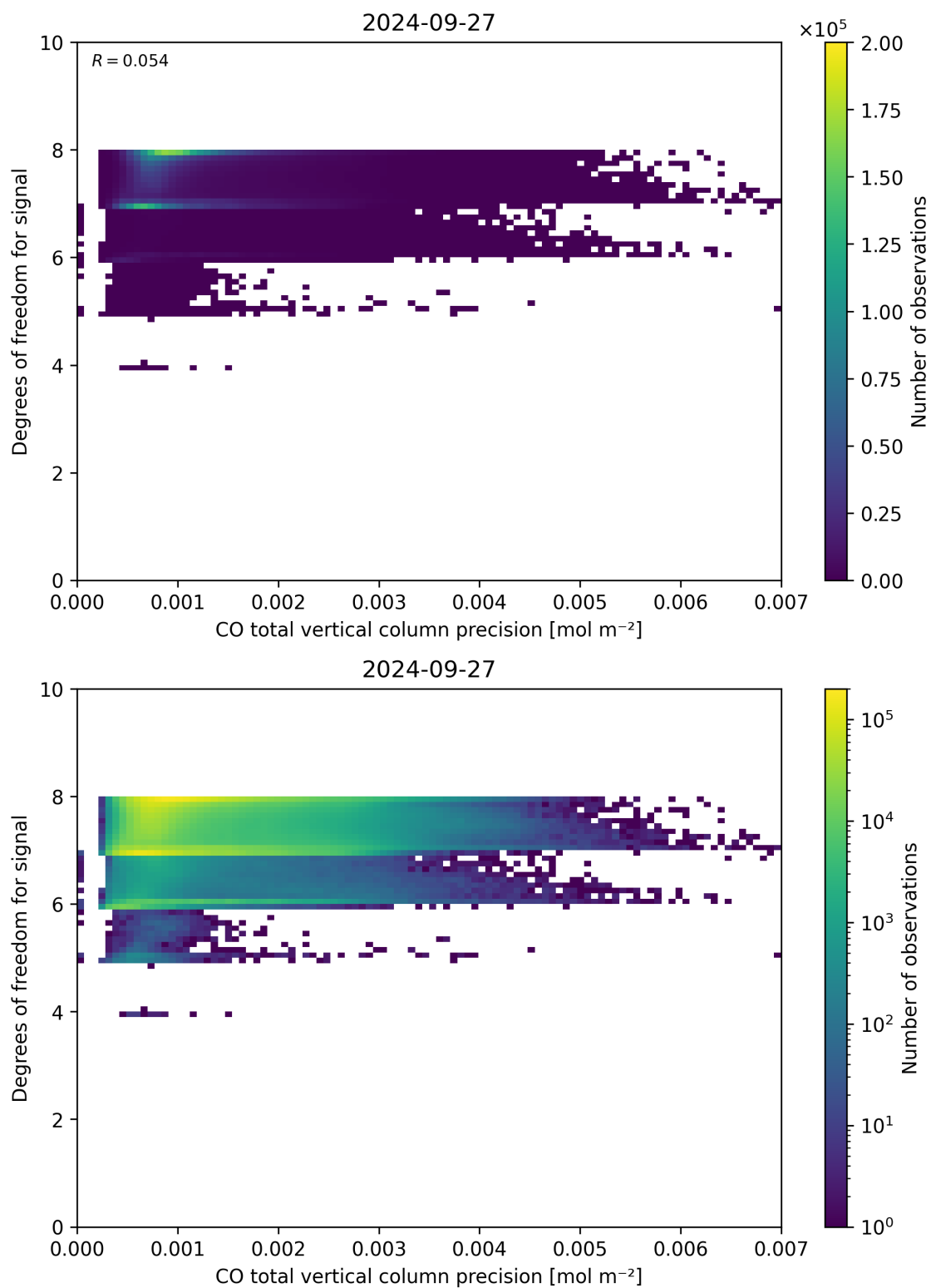
Figure 45: Scatter density plot of “CO total vertical column precision” against “Degrees of freedom for signal” for 2024-09-26 to 2024-09-28.
