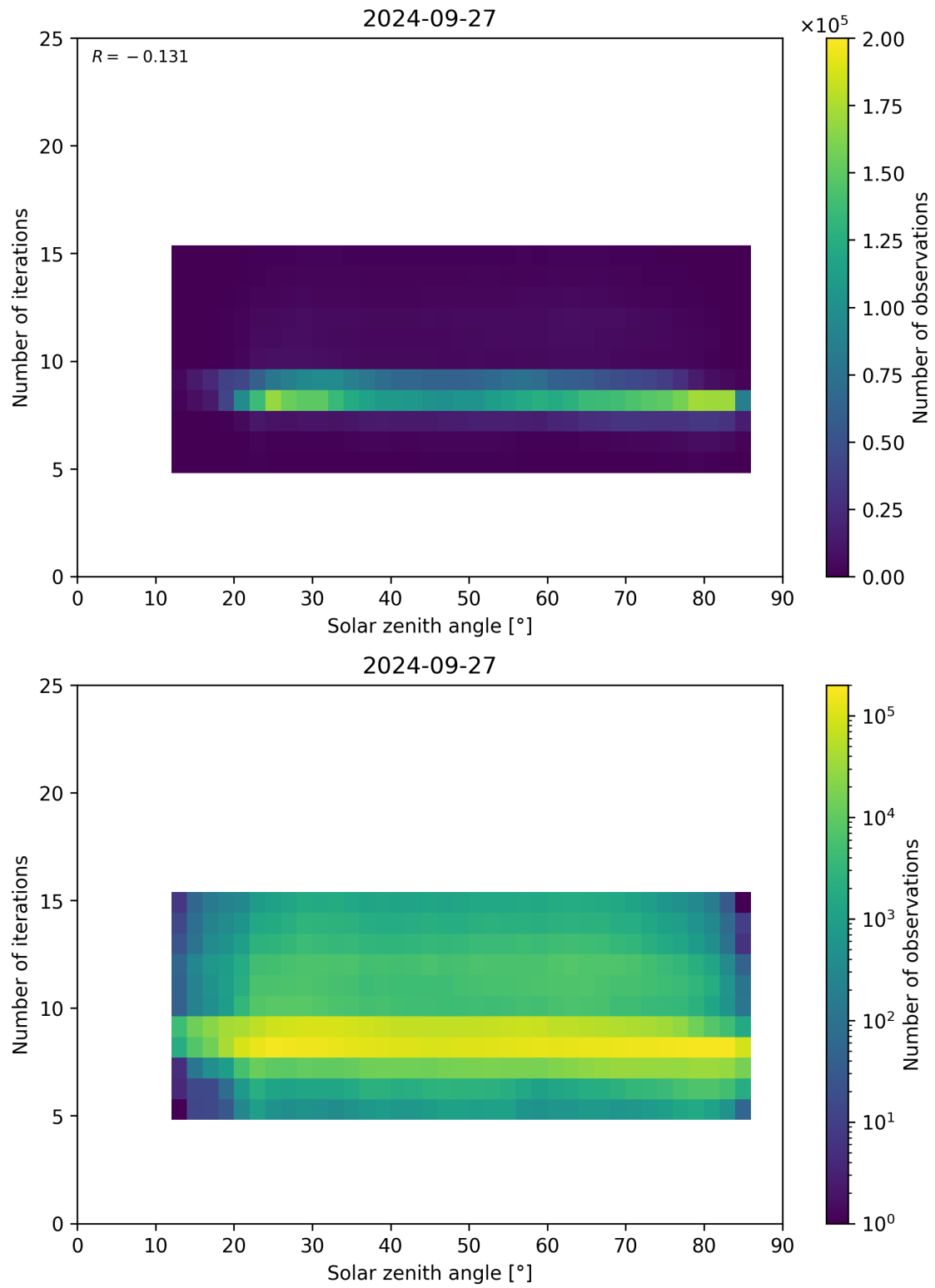
Figure 67: Scatter density plot of “Solar zenith angle” against “Number of iterations” for 2024-09-26 to 2024-09-28.
