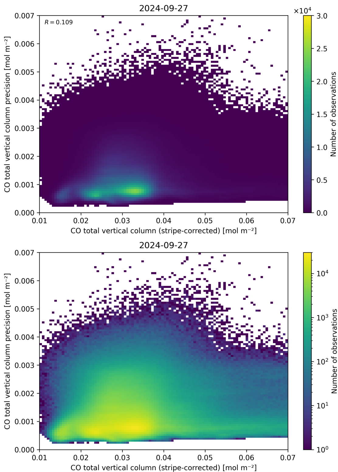
Figure 36: Scatter density plot of “CO total vertical column (stripe-corrected)” against “CO total vertical column precision” for 2024-09-26 to 2024-09-28.
