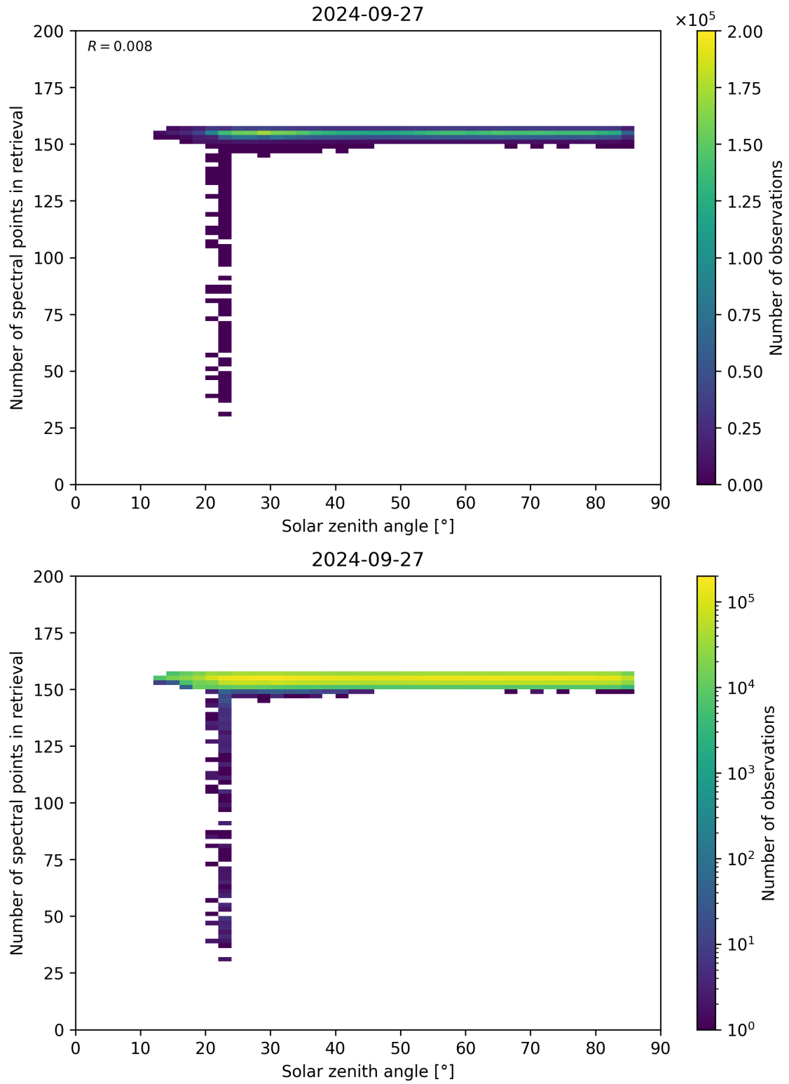
Figure 68: Scatter density plot of “Solar zenith angle” against “Number of spectral points in retrieval” for 2024-09-26 to 2024-09-28.
