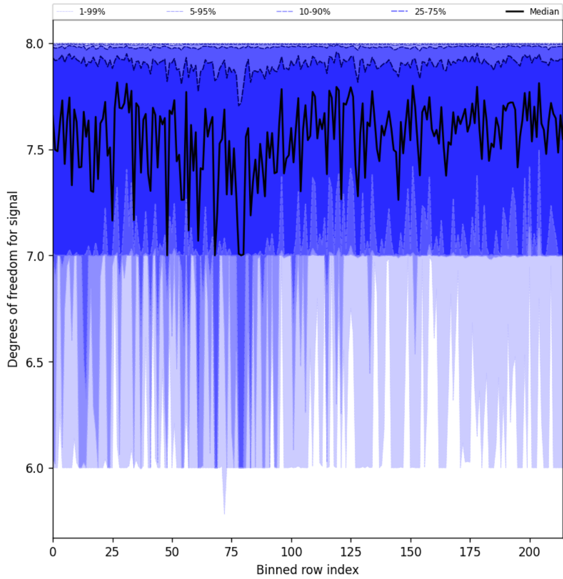
Figure 31: Along track statistics of “Degrees of freedom for signal” for 2024-09-26 to 2024-09-28
