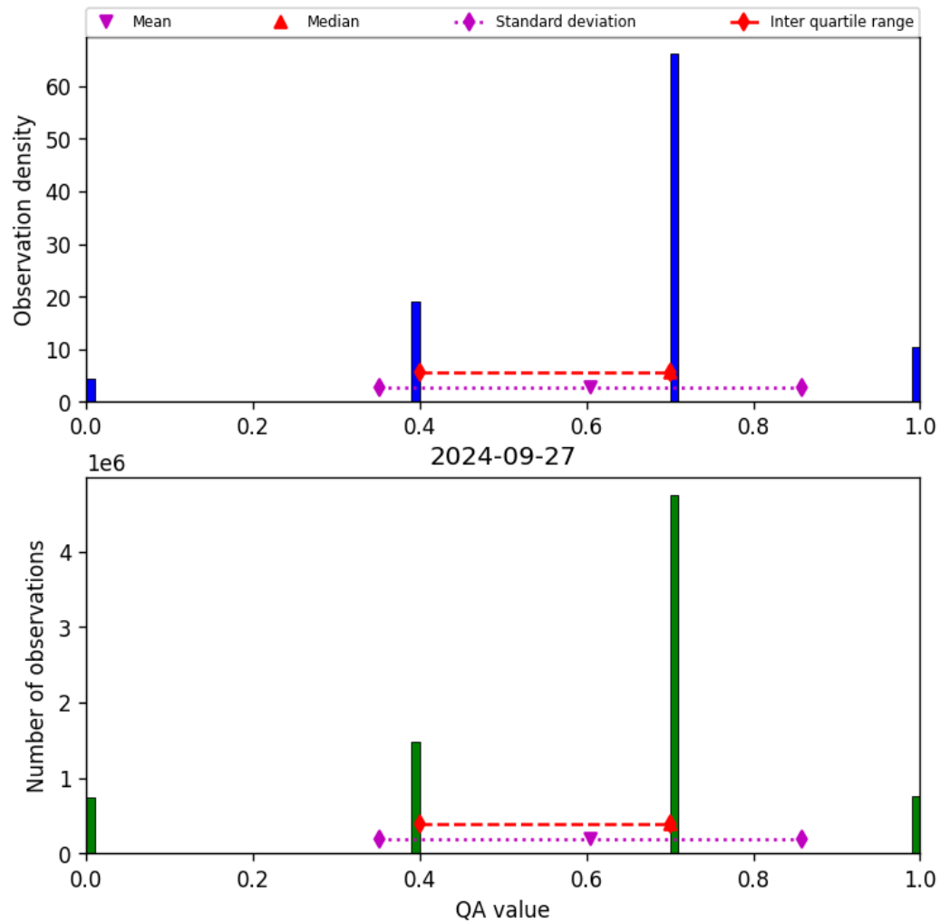
Figure 17: Histogram of “QA value” for 2024-09-26 to 2024-09-28
