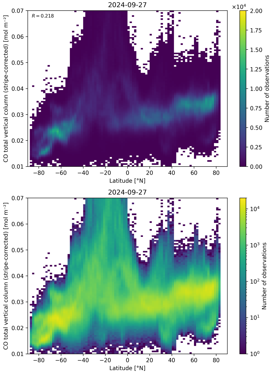
Figure 52: Scatter density plot of “Latitude” against “CO total vertical column (stripe-corrected)” for 2024-09-26 to 2024-09-28.
