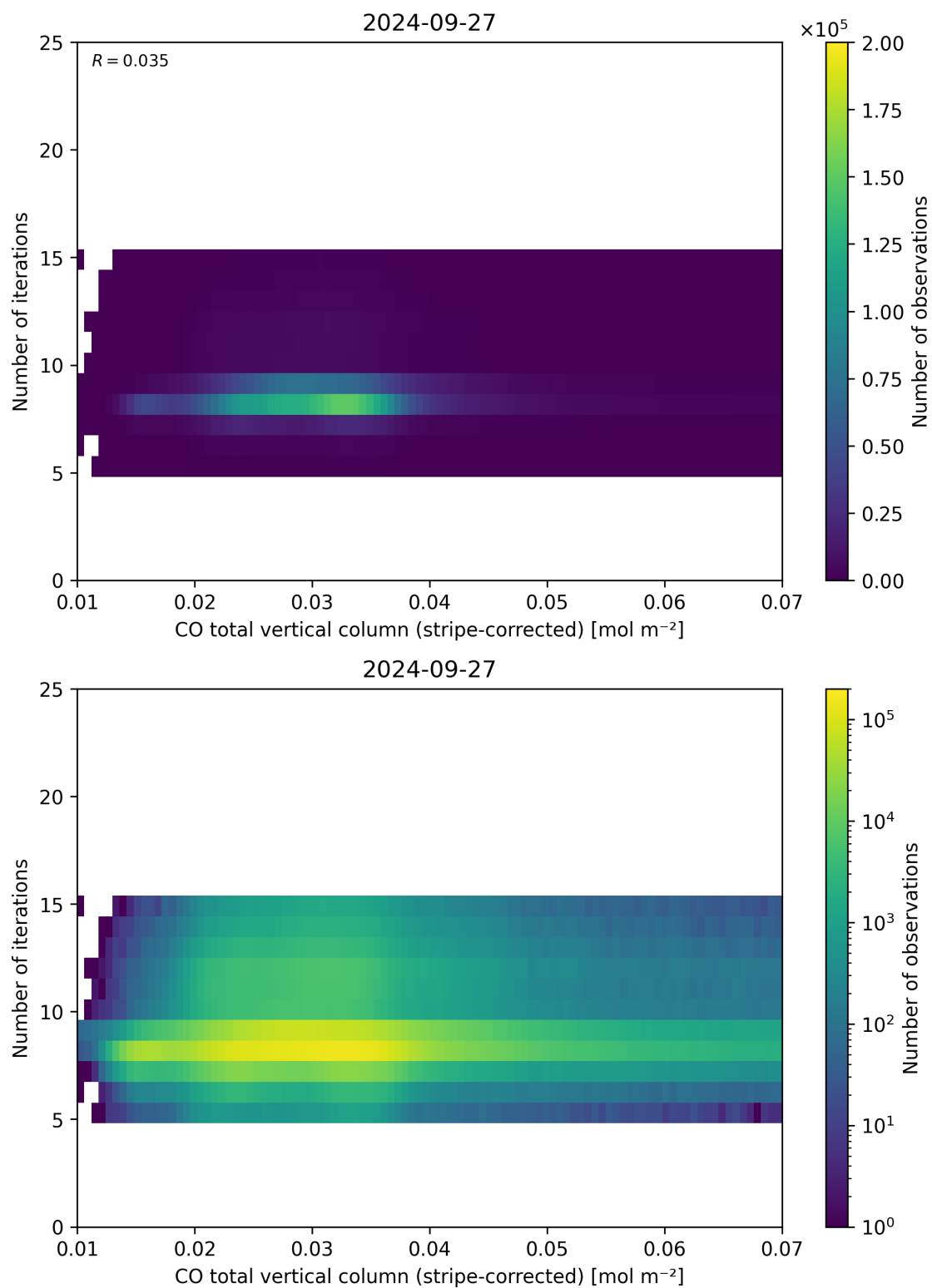
Figure 39: Scatter density plot of “CO total vertical column (stripe-corrected)” against “Number of iterations” for 2024-09-26 to 2024-09-28.
