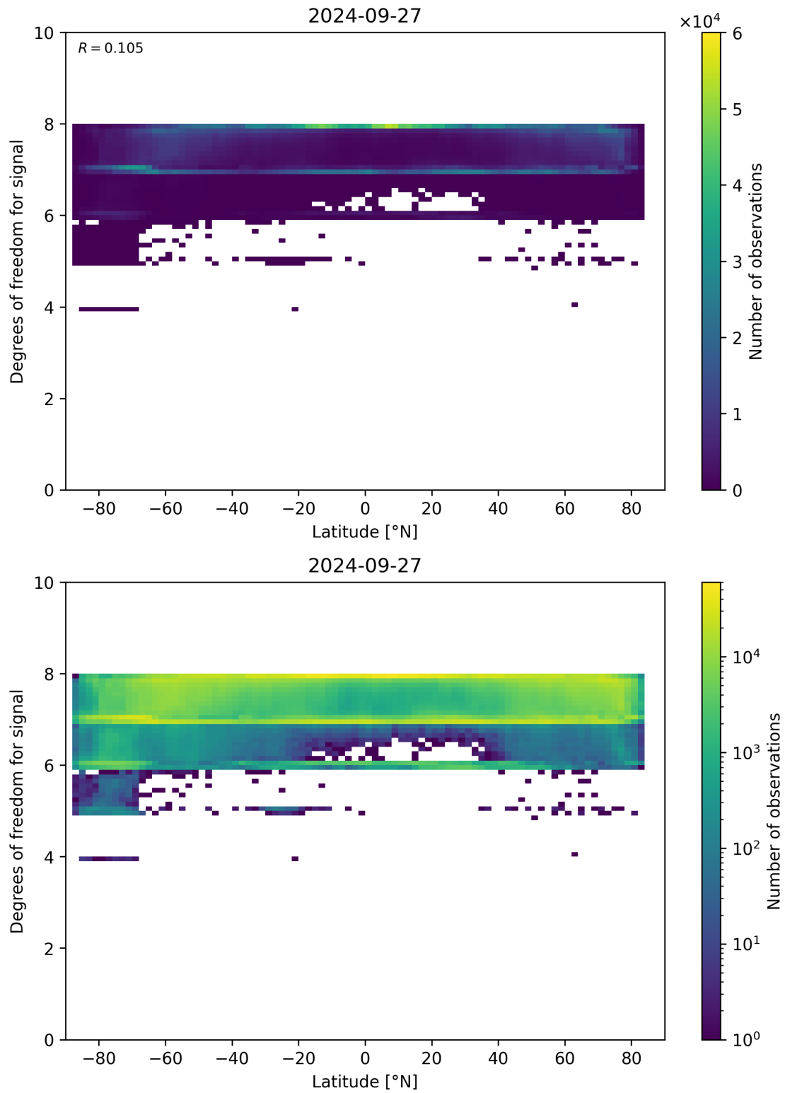
Figure 55: Scatter density plot of “Latitude” against “Degrees of freedom for signal” for 2024-09-26 to 2024-09-28.
