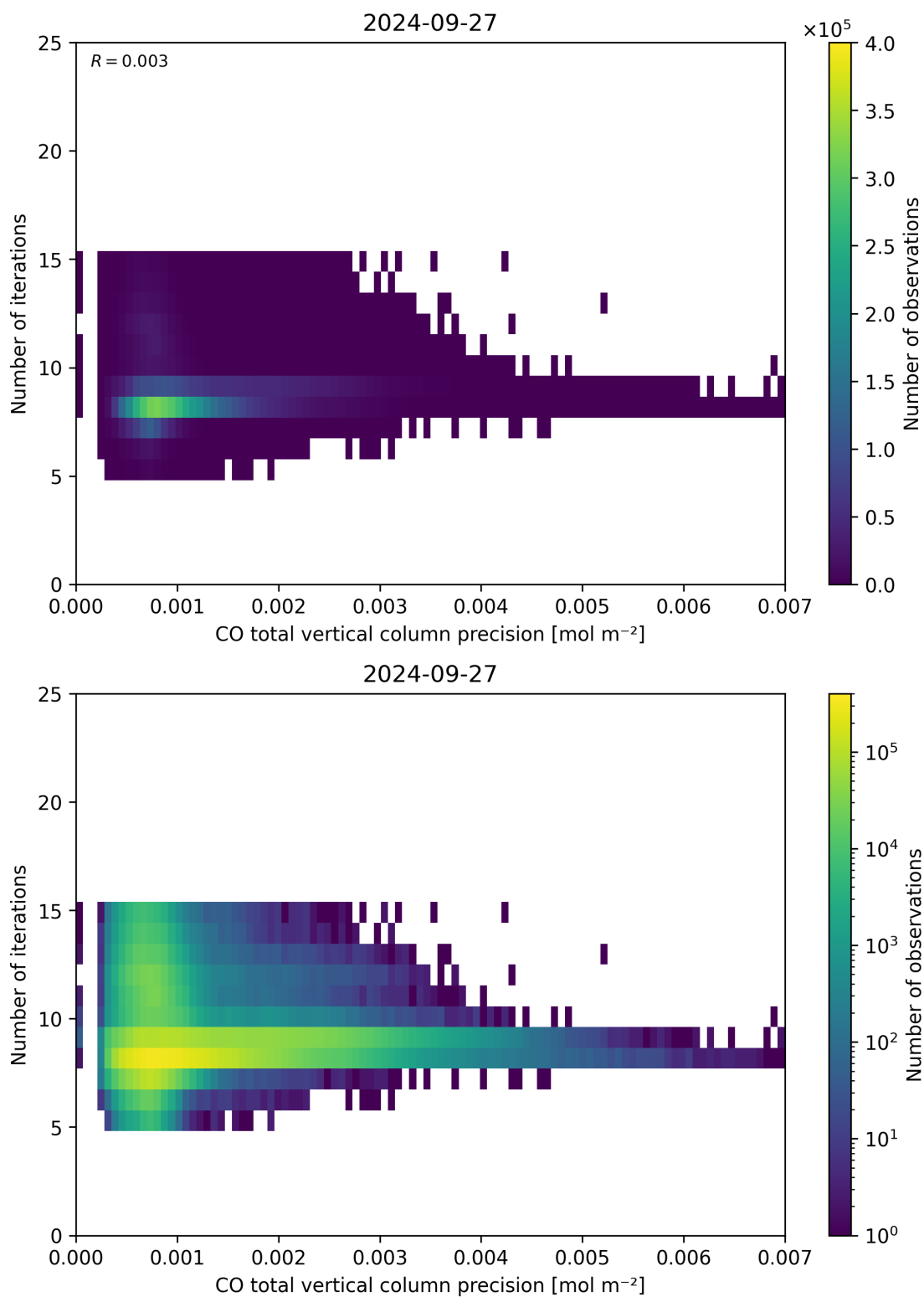
Figure 46: Scatter density plot of “CO total vertical column precision” against “Number of iterations” for 2024-09-26 to 2024-09-28.
