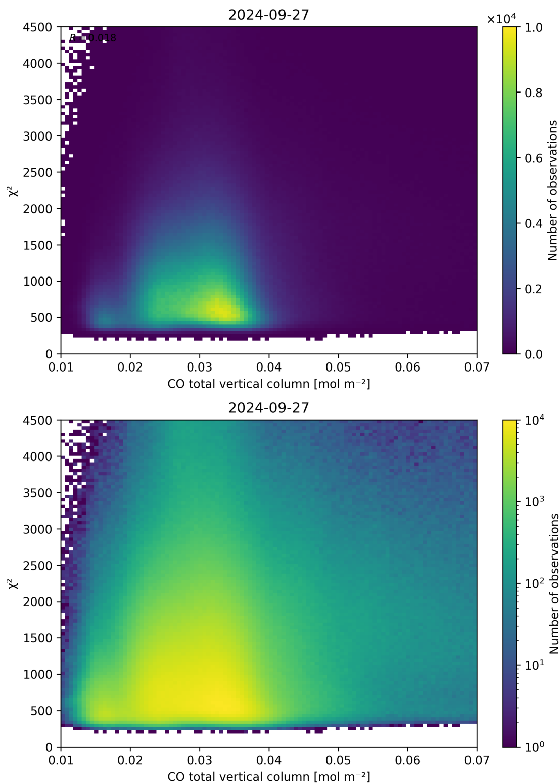
Figure 35: Scatter density plot of “CO total vertical column” against “ \chi^2 ” for 2024-09-26 to 2024-09-28.
