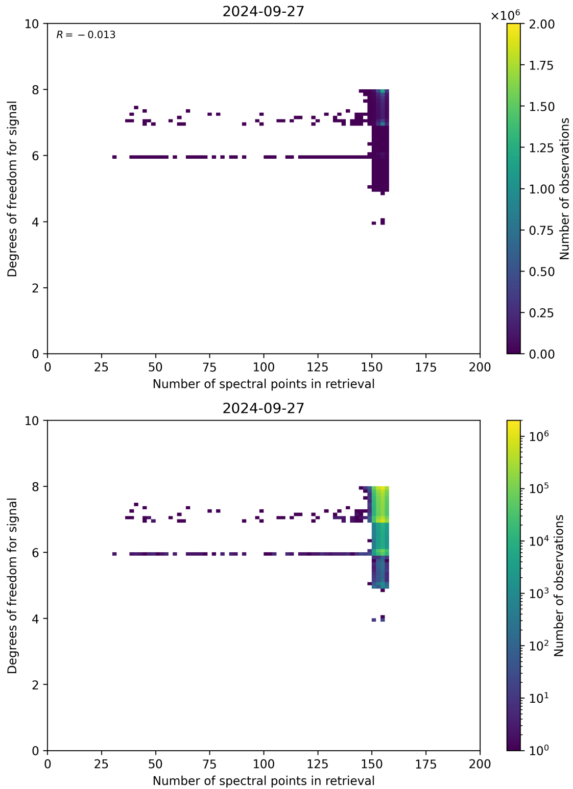
Figure 59: Scatter density plot of “Number of spectral points in retrieval” against “Degrees of freedom for signal” for 2024-09-26 to 2024-09-28.
