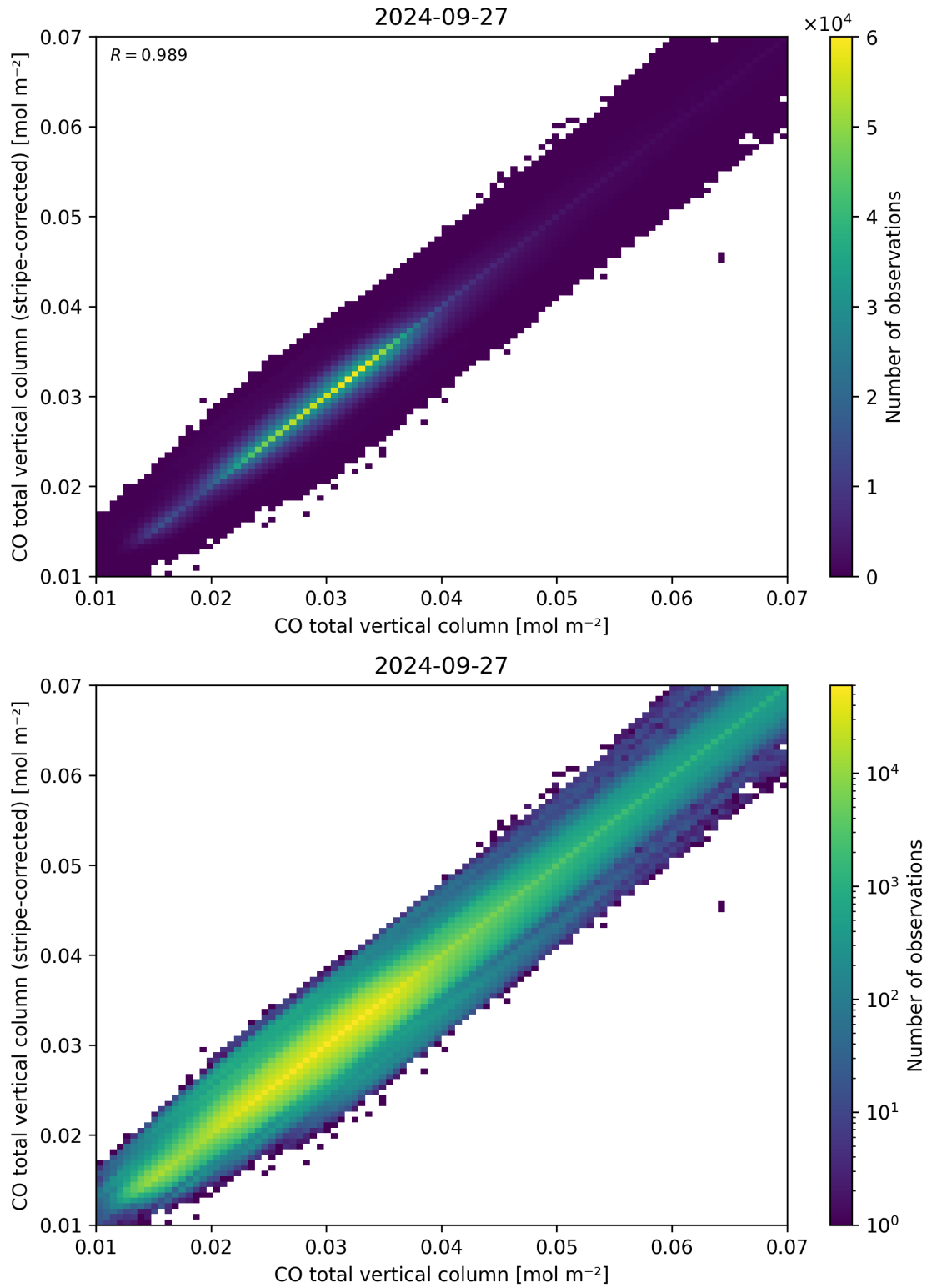
Figure 33: Scatter density plot of “CO total vertical column” against “CO total vertical column (stripe-corrected)” for 2024-09-26 to 2024-09-28.
