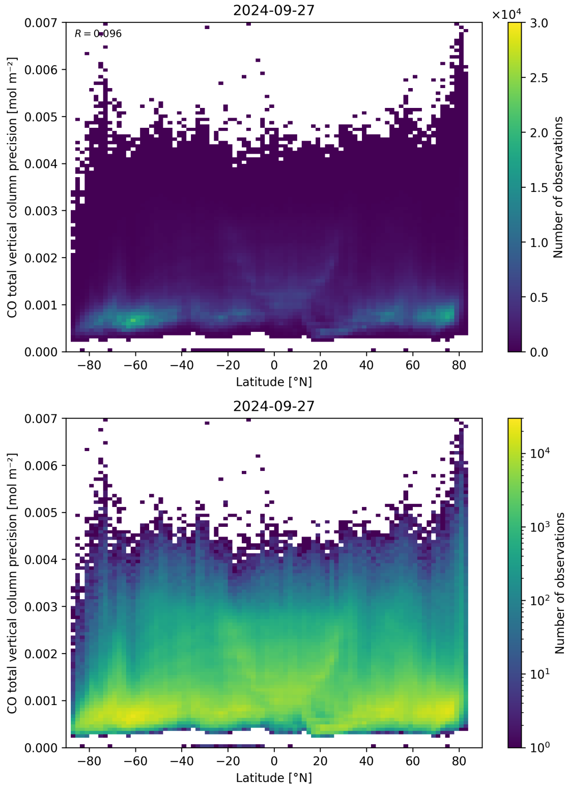
Figure 53: Scatter density plot of “Latitude” against “CO total vertical column precision” for 2024-09-26 to 2024-09-28.
