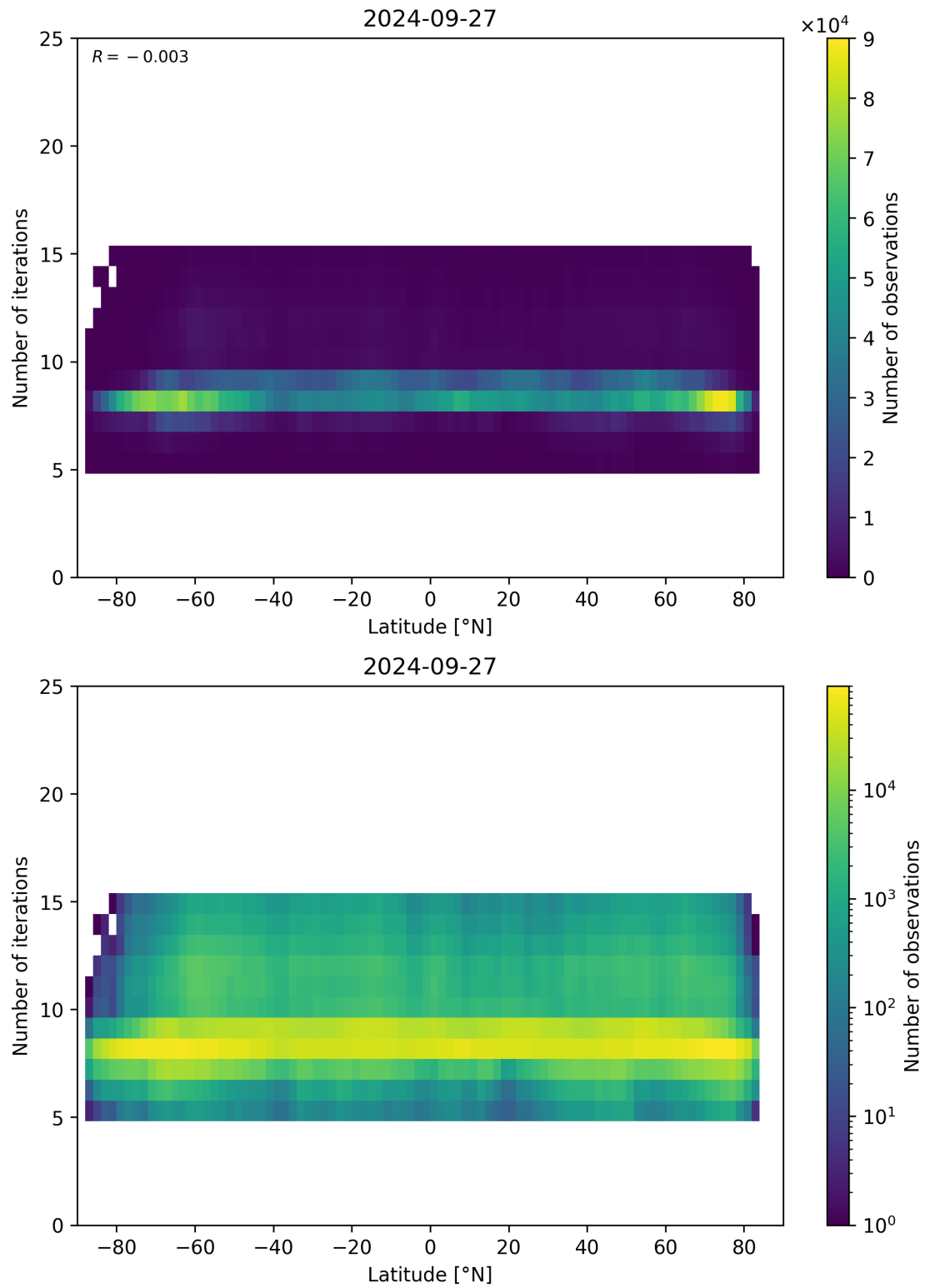
Figure 56: Scatter density plot of “Latitude” against “Number of iterations” for 2024-09-26 to 2024-09-28.
