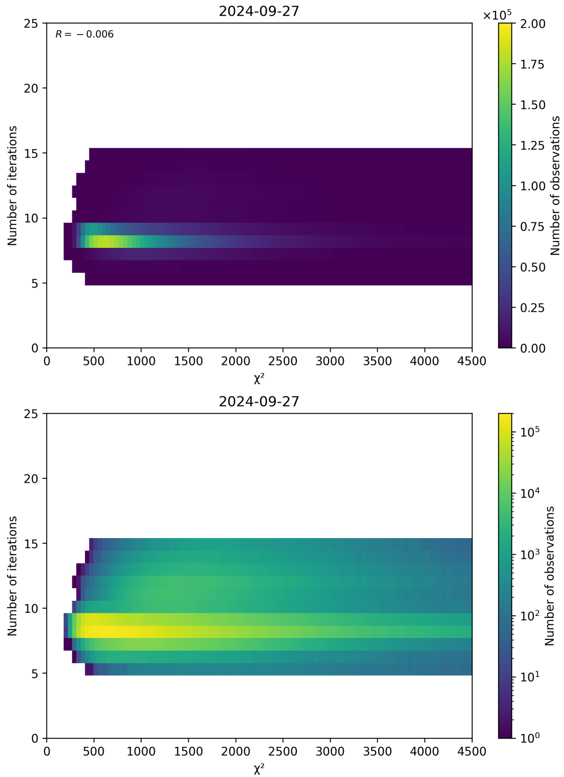
Figure 49: Scatter density plot of “ \chi^2 ” against “Number of iterations” for 2024-09-26 to 2024-09-28.
