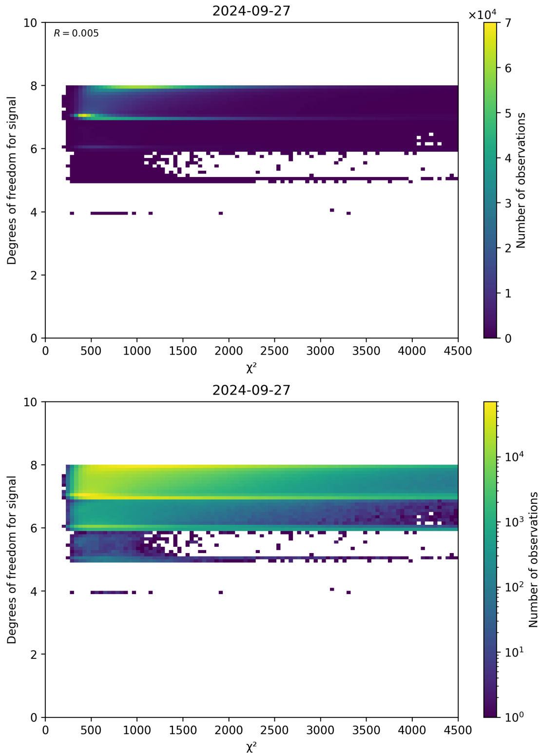
Figure 48: Scatter density plot of “ \chi^2 ” against “Degrees of freedom for signal” for 2024-09-26 to 2024-09-28.
