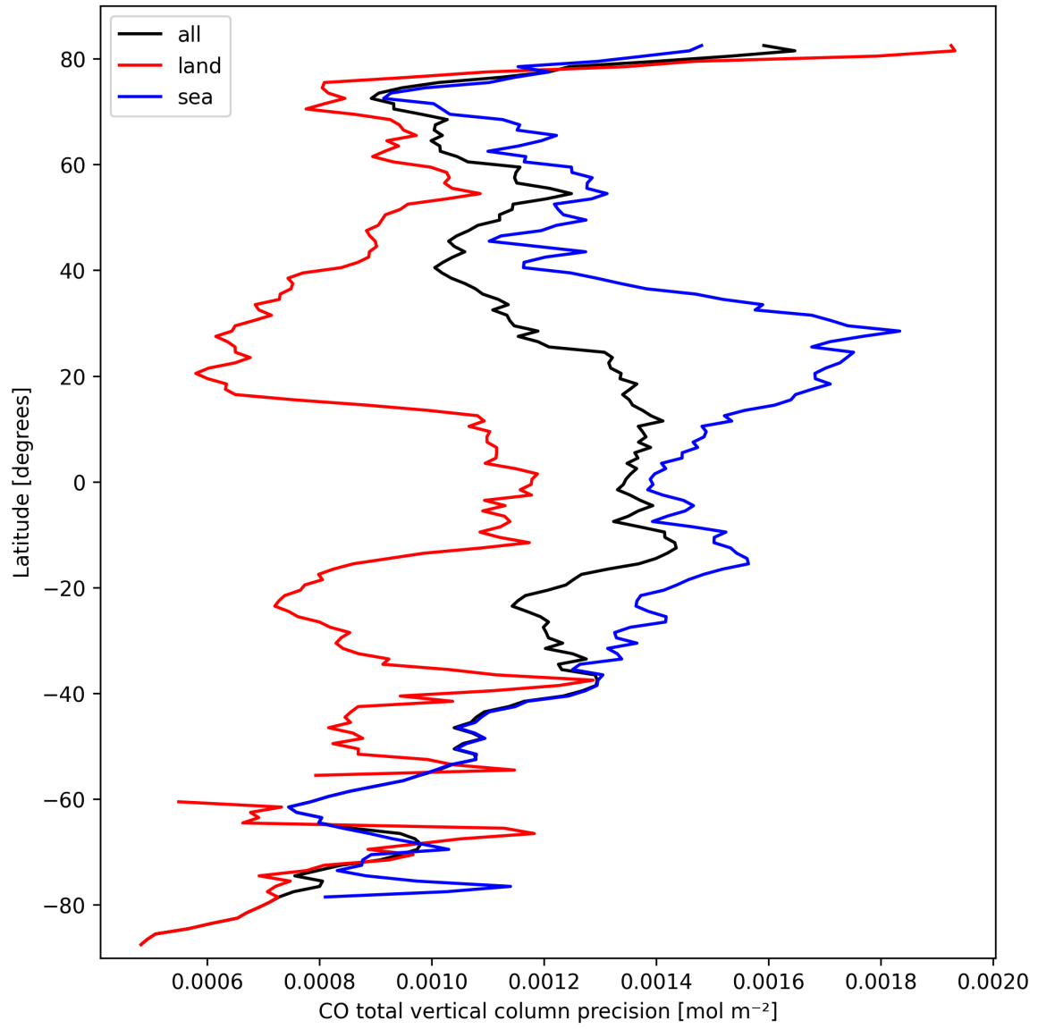
Figure 12: Zonal average of “CO total vertical column precision” for 2024-09-28 to 2024-09-29.
