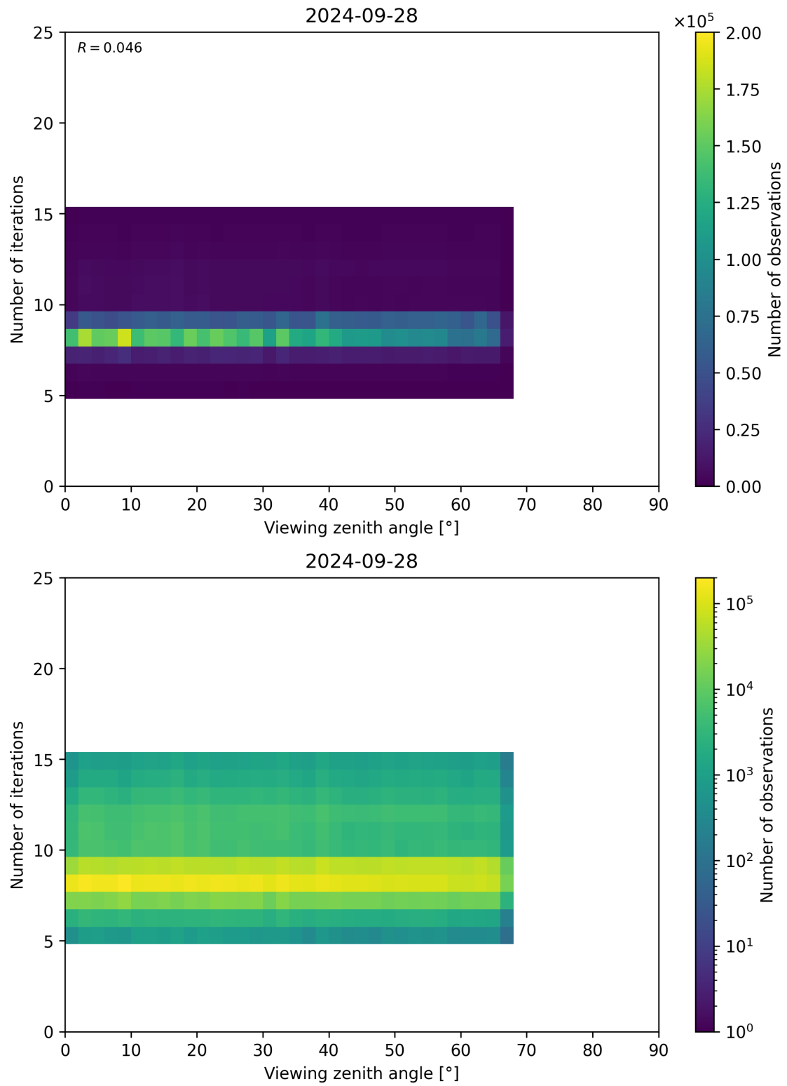
Figure 75: Scatter density plot of “Viewing zenith angle” against “Number of iterations” for 2024-09-28 to 2024-09-29.
