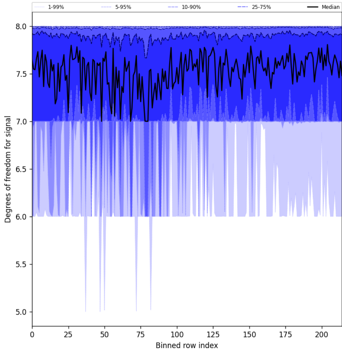
Figure 31: Along track statistics of “Degrees of freedom for signal” for 2024-09-28 to 2024-09-29
