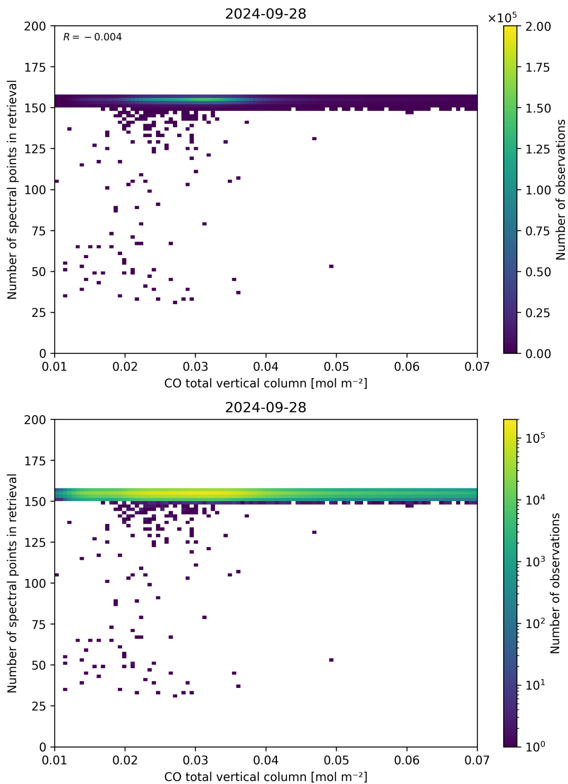
Figure 43: Scatter density plot of “CO total vertical column” against “Number of spectral points in retrieval” for 2024-09-28 to 2024-09-29.
