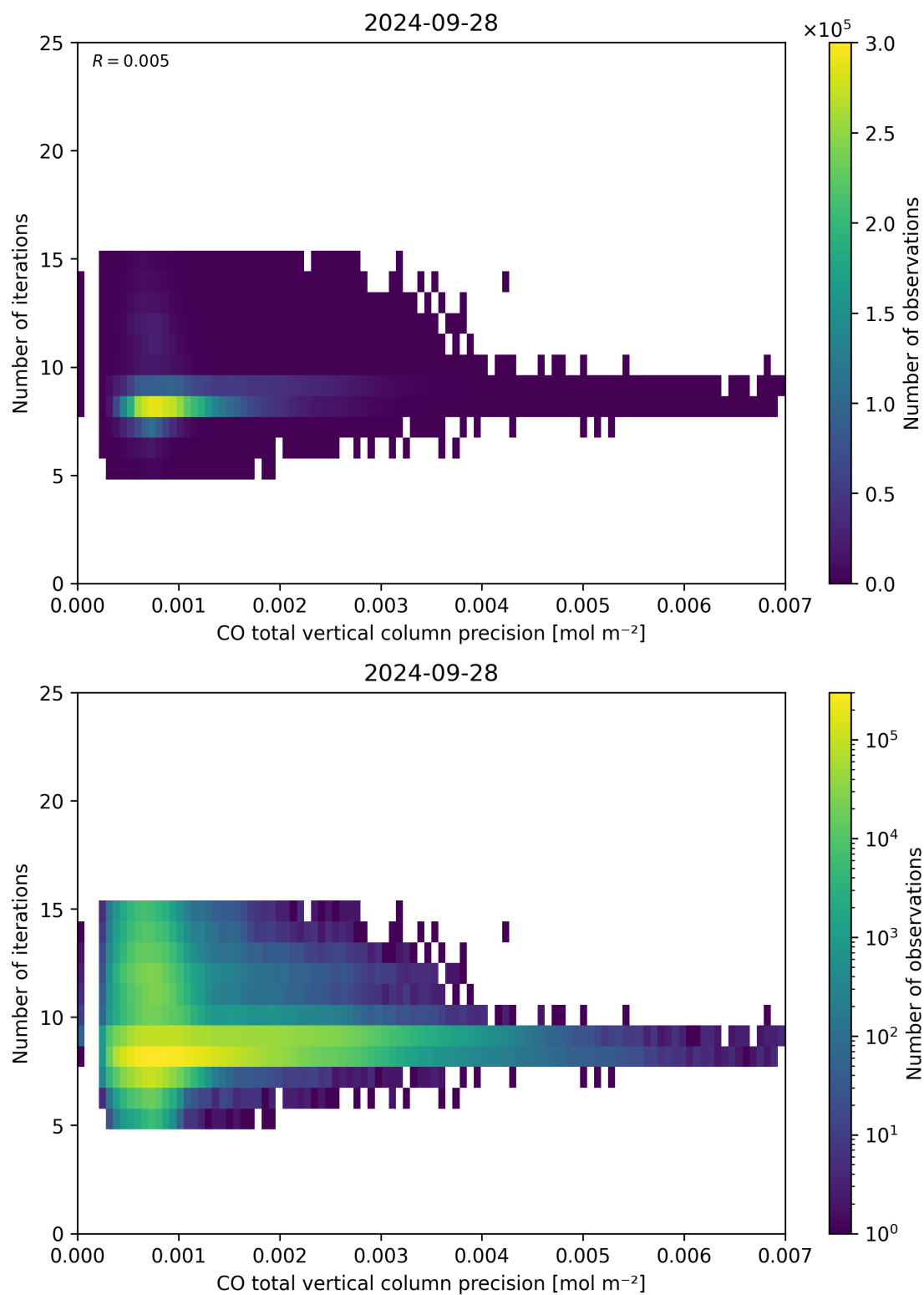
Figure 46: Scatter density plot of “CO total vertical column precision” against “Number of iterations” for 2024-09-28 to 2024-09-29.
