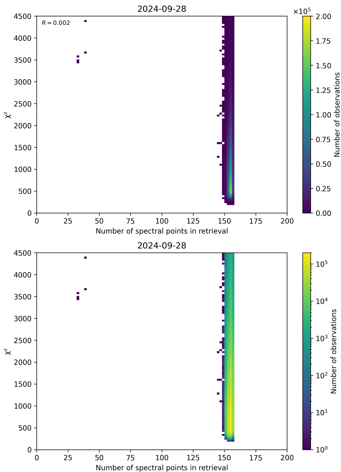
Figure 58: Scatter density plot of “Number of spectral points in retrieval” against “ \chi^2 ” for 2024-09-28 to 2024-09-29.
