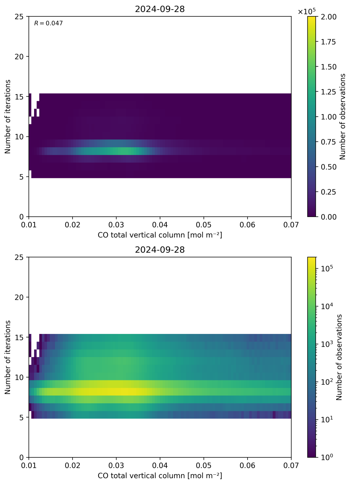
Figure 42: Scatter density plot of “CO total vertical column” against “Number of iterations” for 2024-09-28 to 2024-09-29.
