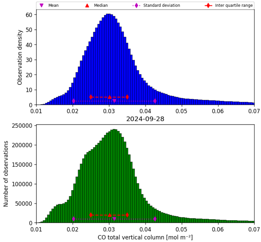
Figure 18: Histogram of “CO total vertical column” for 2024-09-28 to 2024-09-29
