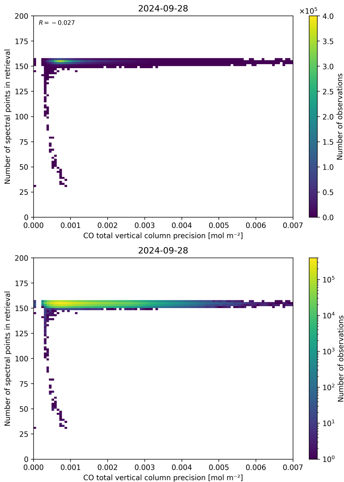
Figure 47: Scatter density plot of “CO total vertical column precision” against “Number of spectral points in retrieval” for 2024-09-28 to 2024-09-29.
