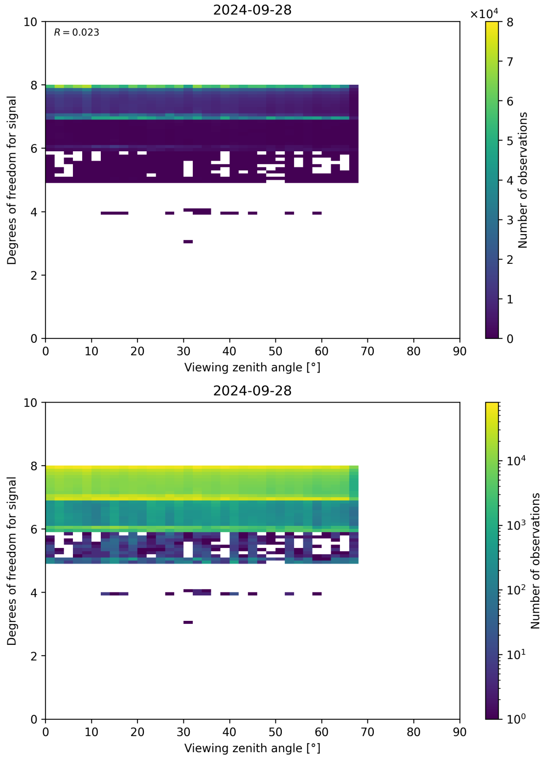
Figure 73: Scatter density plot of “Viewing zenith angle” against “Degrees of freedom for signal” for 2024-09-28 to 2024-09-29.
