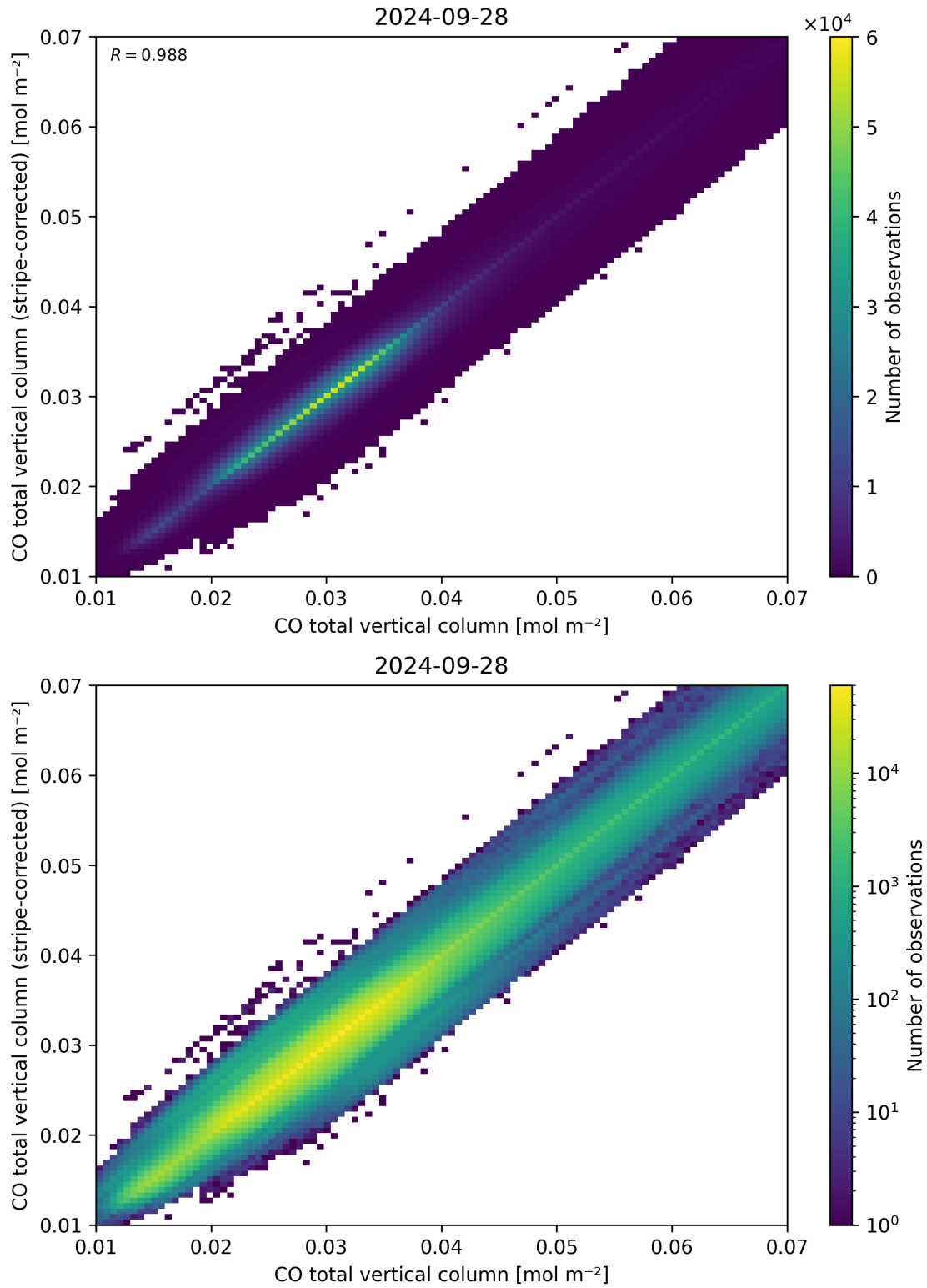
Figure 33: Scatter density plot of “CO total vertical column” against “CO total vertical column (stripe-corrected)” for 2024-09-28 to 2024-09-29.
