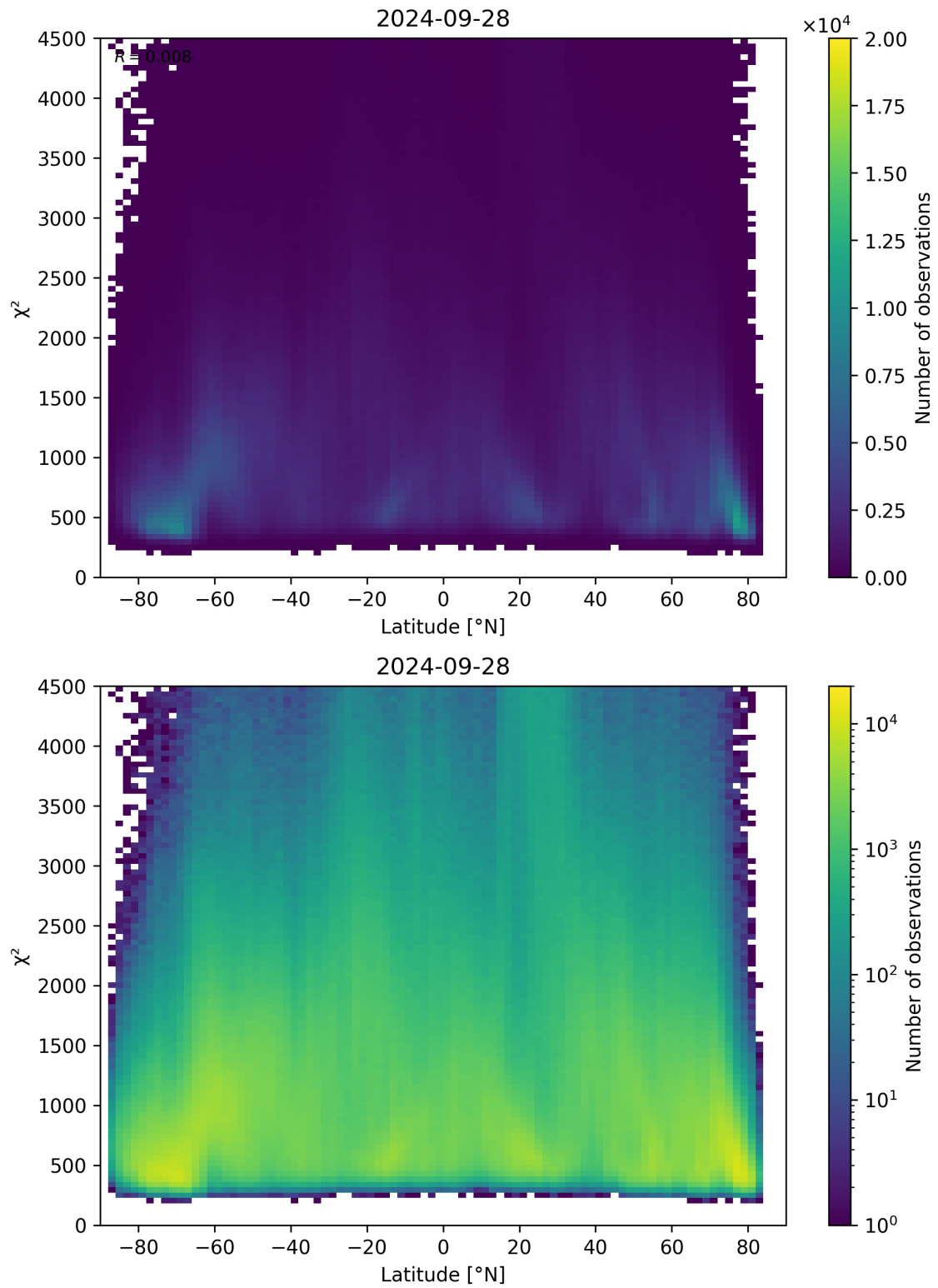
Figure 54: Scatter density plot of “Latitude” against “ \chi^2 ” for 2024-09-28 to 2024-09-29.
