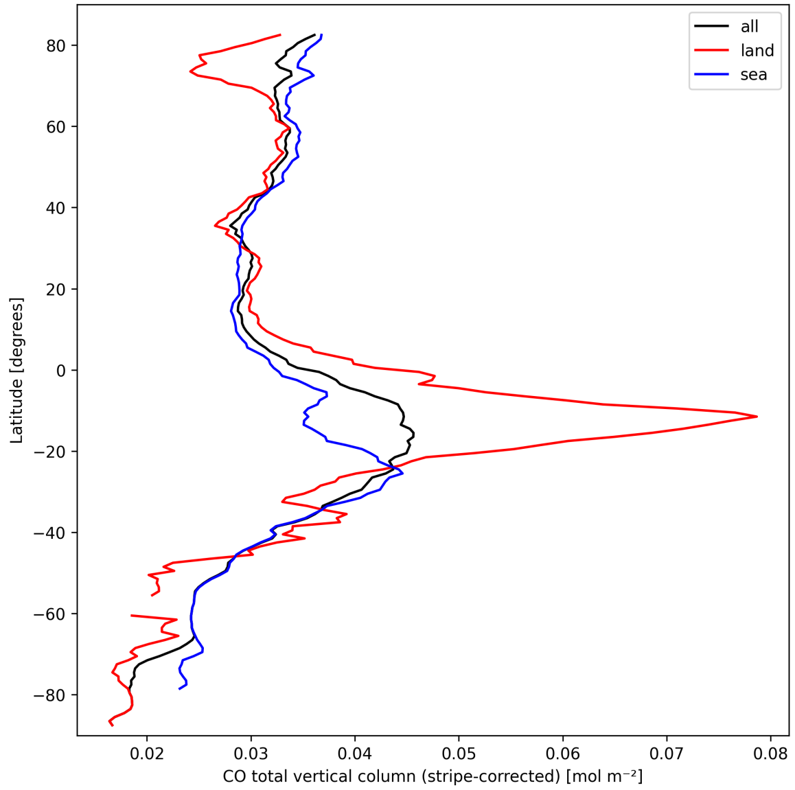
Figure 11: Zonal average of “CO total vertical column (stripe-corrected)” for 2024-09-28 to 2024-09-29.
