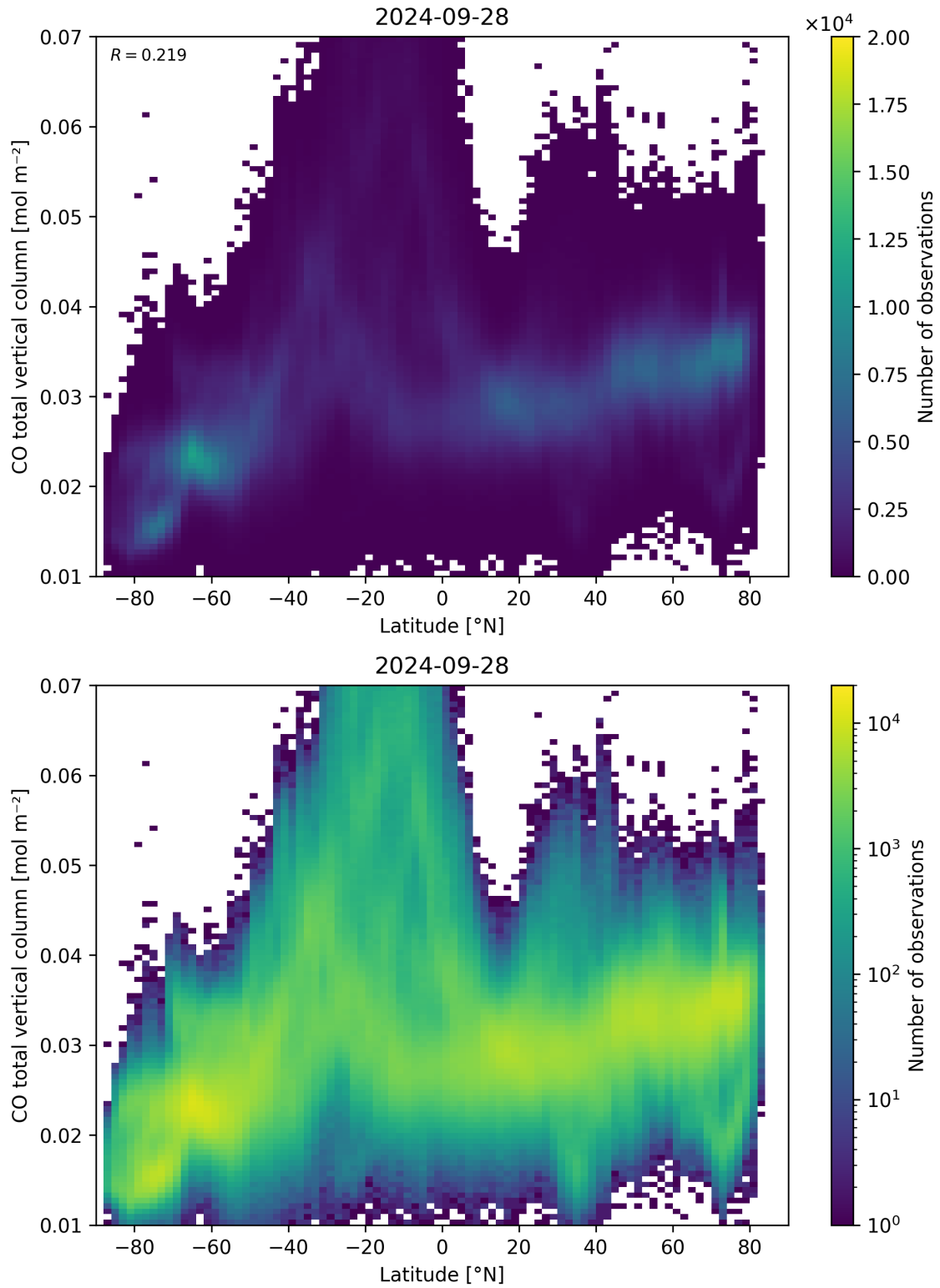
Figure 51: Scatter density plot of “Latitude” against “CO total vertical column” for 2024-09-28 to 2024-09-29.
