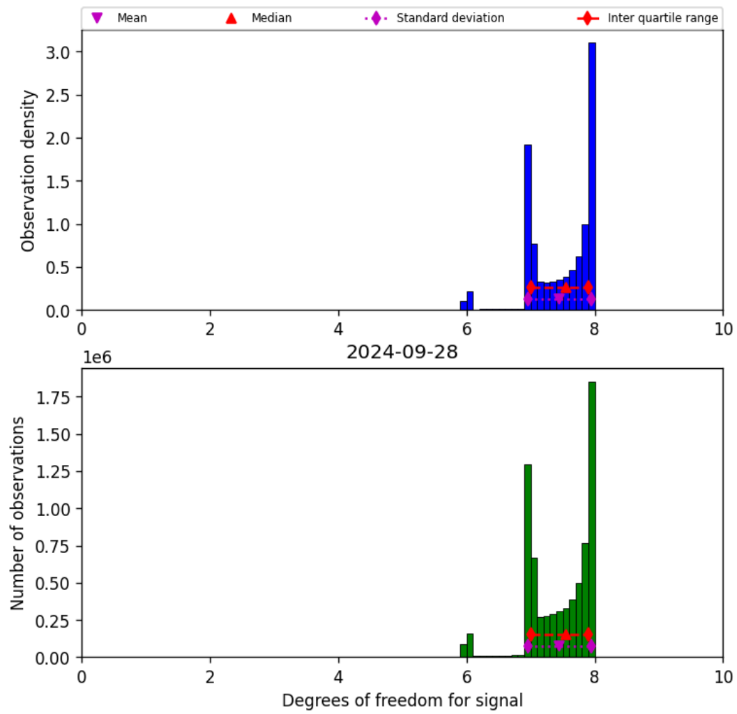
Figure 23: Histogram of “Degrees of freedom for signal” for 2024-09-28 to 2024-09-29
