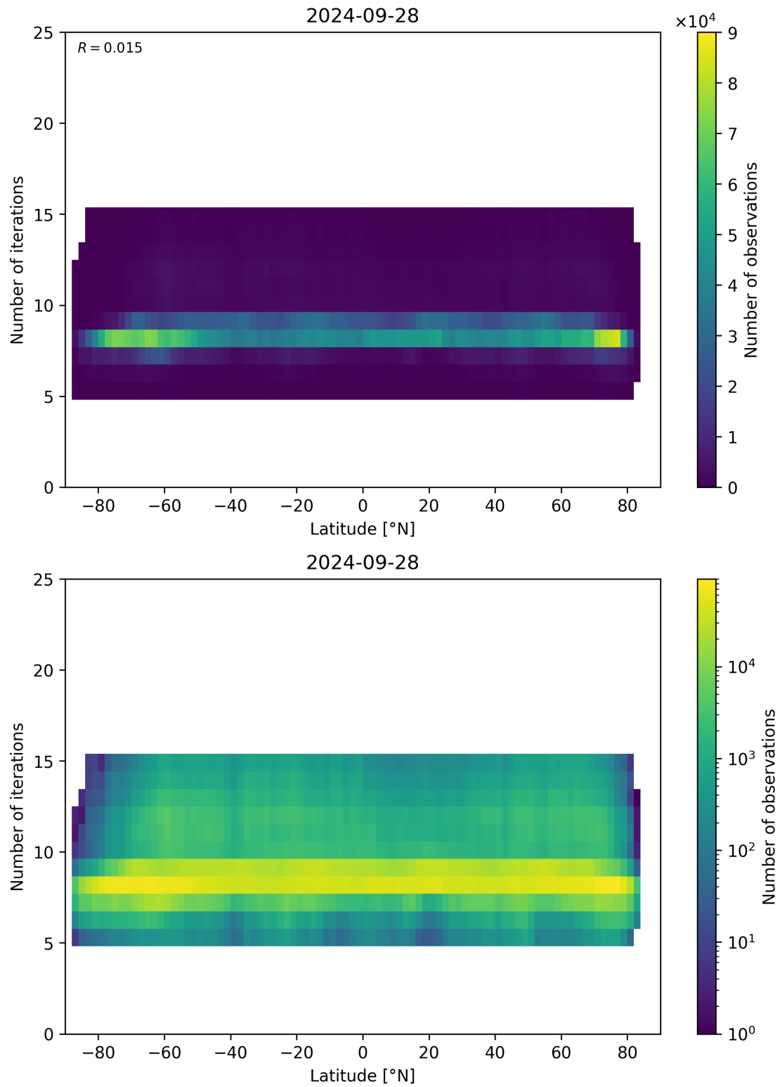
Figure 56: Scatter density plot of “Latitude” against “Number of iterations” for 2024-09-28 to 2024-09-29.
