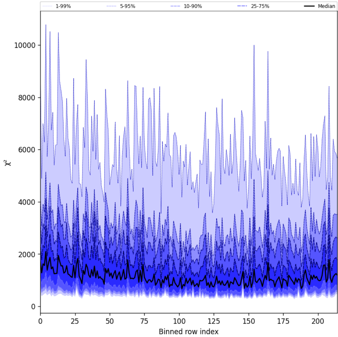
Figure 30: Along track statistics of “ \chi^2 ” for 2024-09-28 to 2024-09-29
