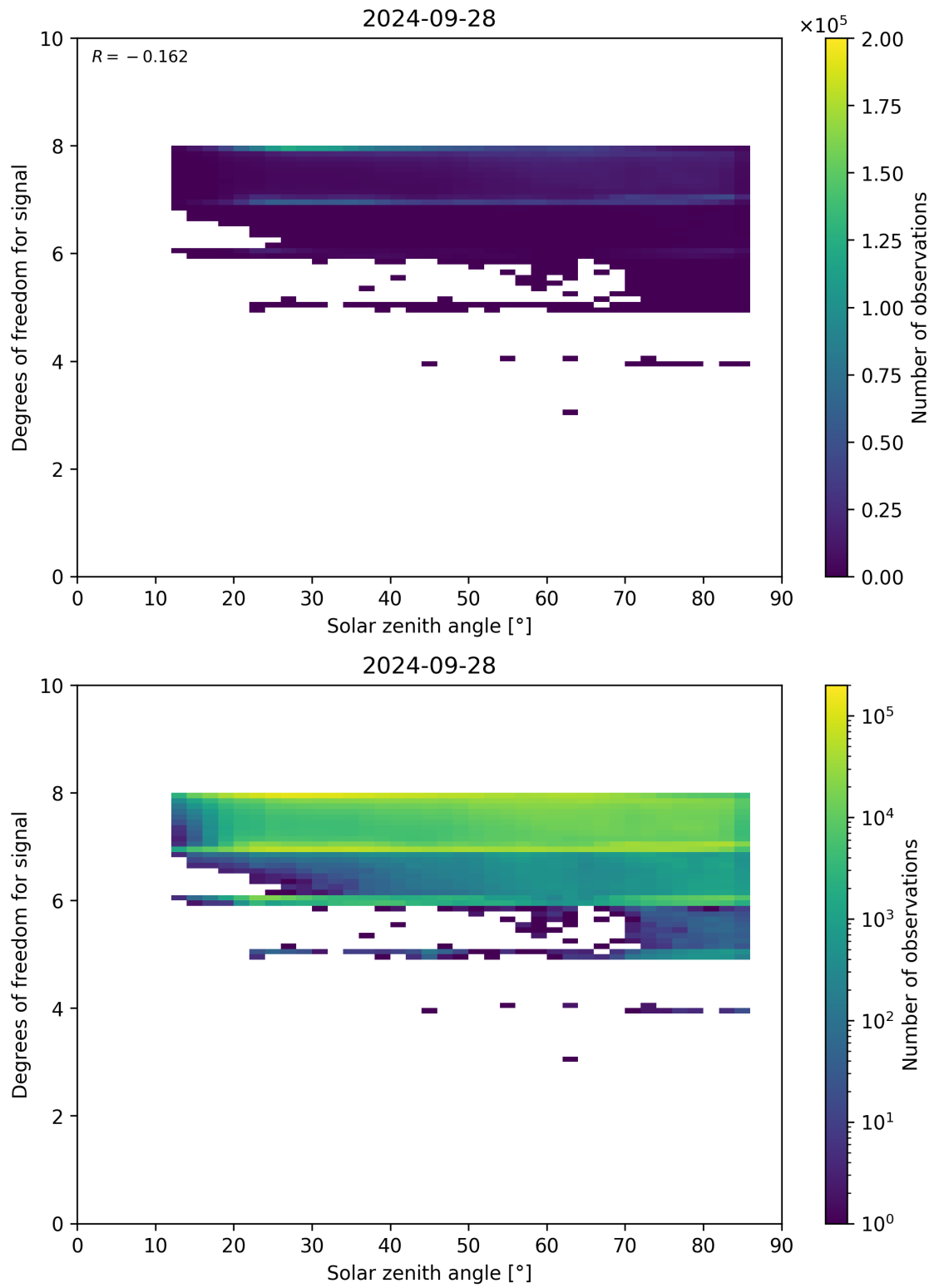
Figure 65: Scatter density plot of “Solar zenith angle” against “Degrees of freedom for signal” for 2024-09-28 to 2024-09-29.
