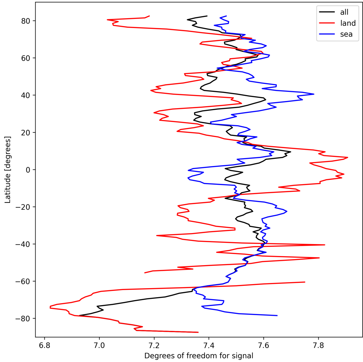
Figure 15: Zonal average of “Degrees of freedom for signal” for 2024-09-28 to 2024-09-29.
