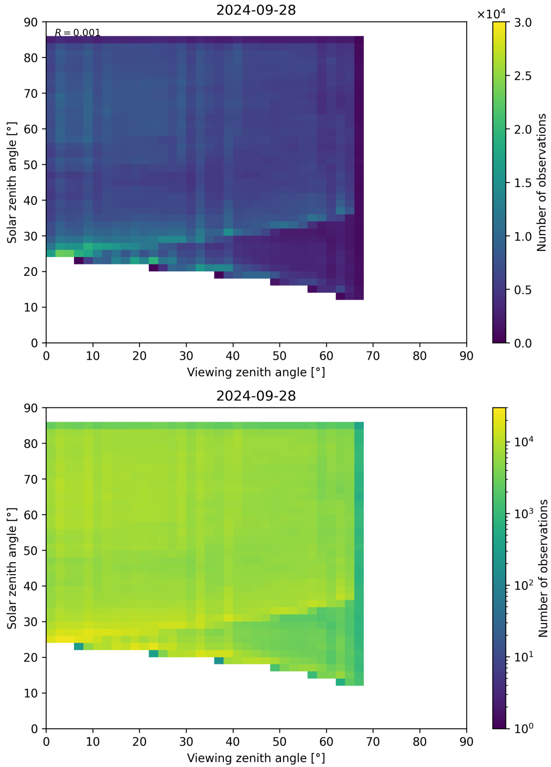
Figure 77: Scatter density plot of “Viewing zenith angle” against “Solar zenith angle” for 2024-09-28 to 2024-09-29.
