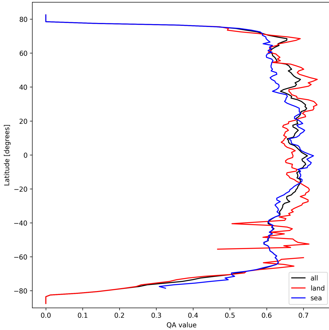
Figure 9: Zonal average of “QA value” for 2024-09-28 to 2024-09-29.
