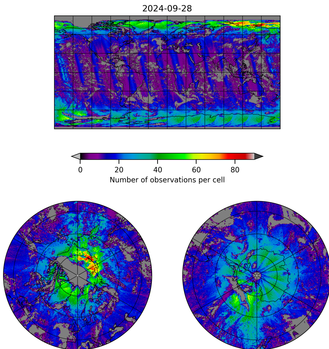
Figure 8: Map of the number of observations for 2024-09-28 to 2024-09-29
