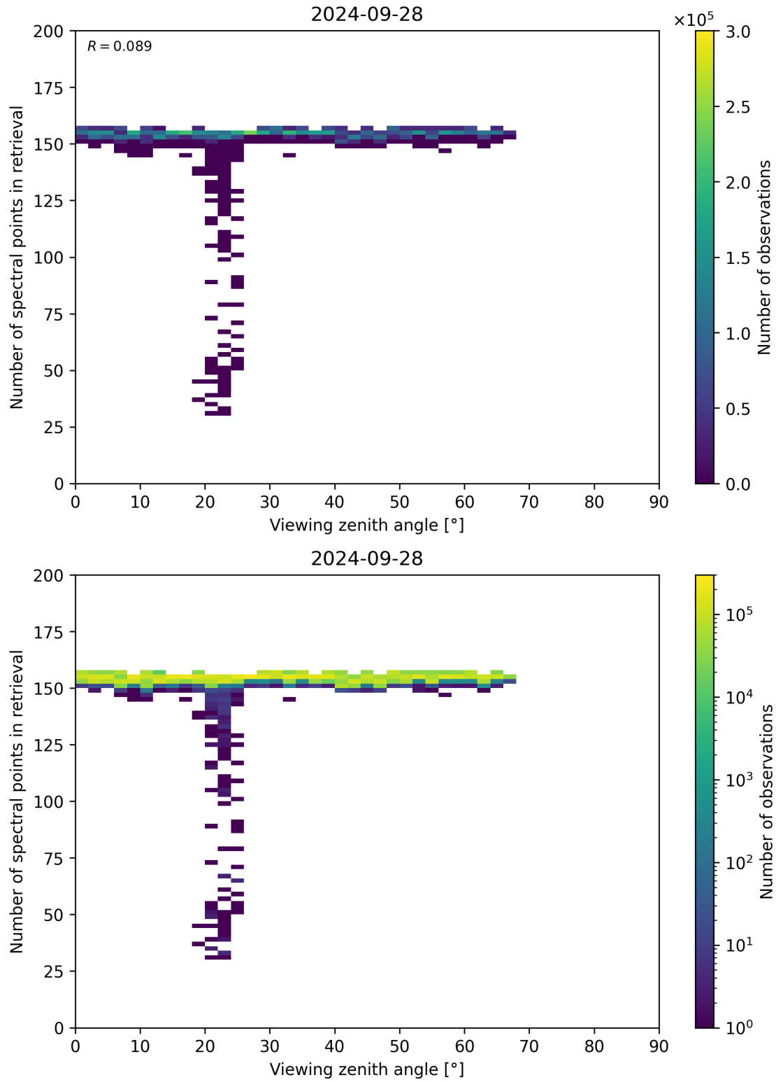
Figure 76: Scatter density plot of “Viewing zenith angle” against “Number of spectral points in retrieval” for 2024-09-28 to 2024-09-29.
