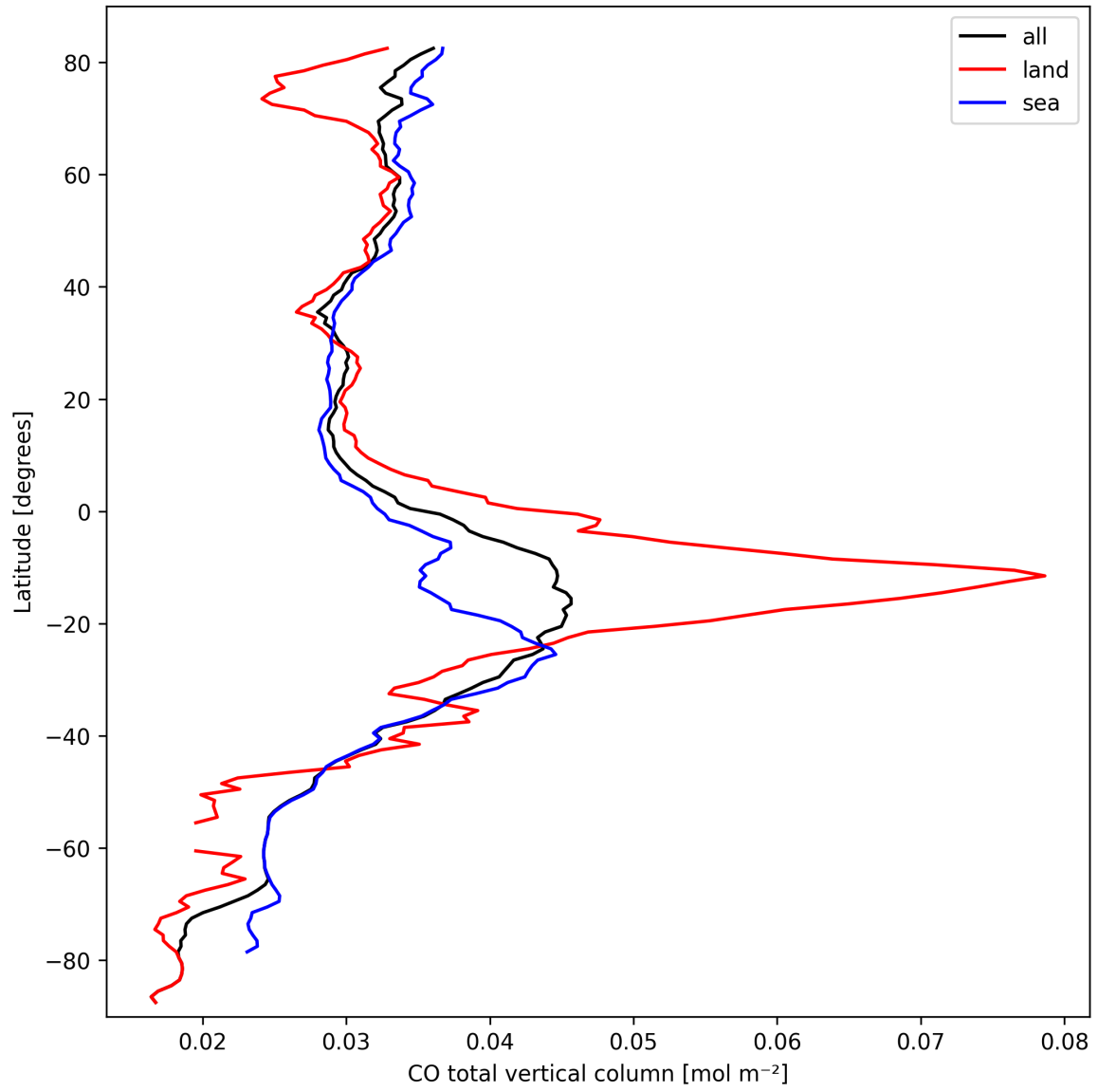
Figure 10: Zonal average of “CO total vertical column” for 2024-09-28 to 2024-09-29.
