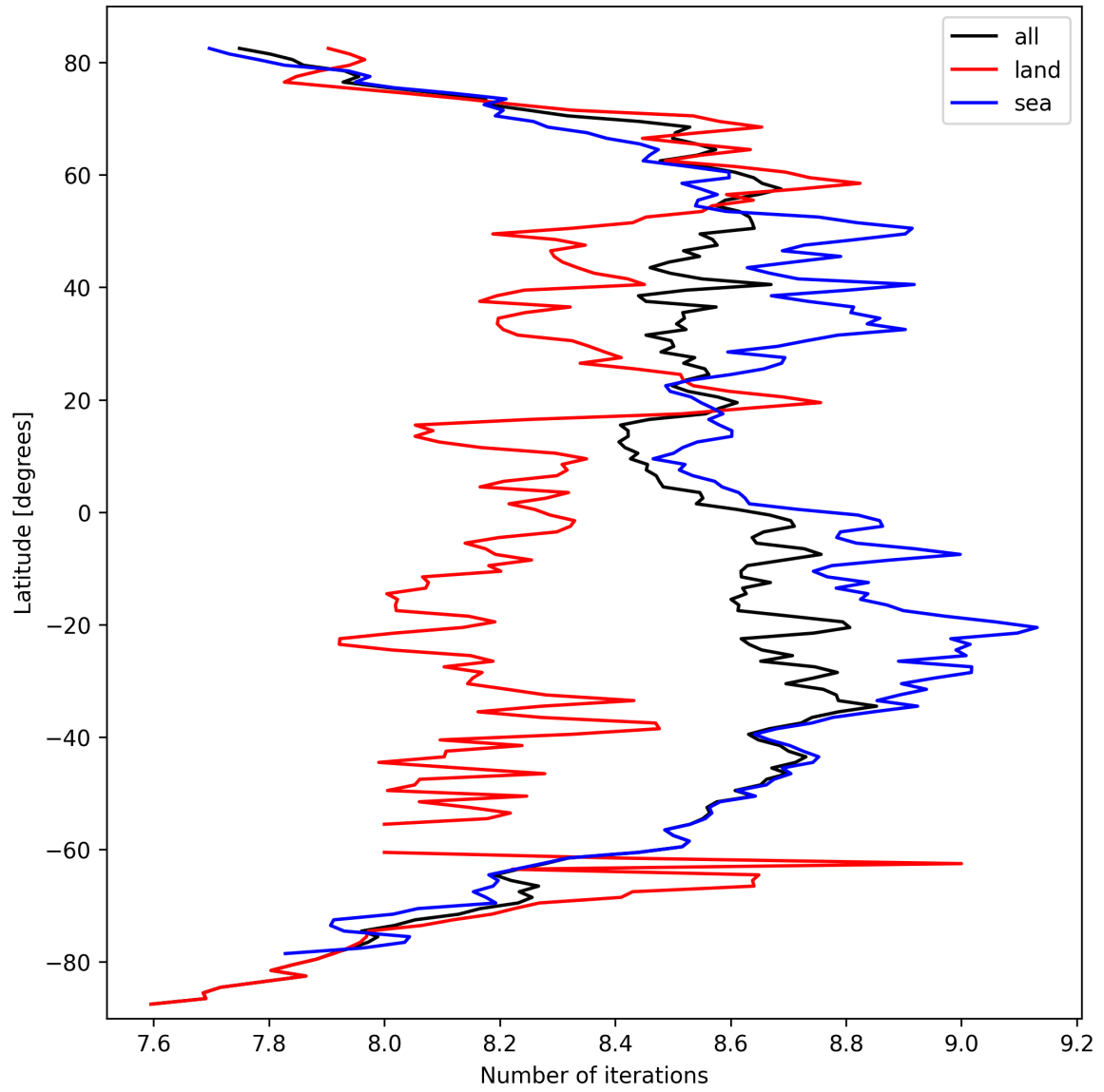
Figure 16: Zonal average of “Number of iterations” for 2024-09-28 to 2024-09-29.
