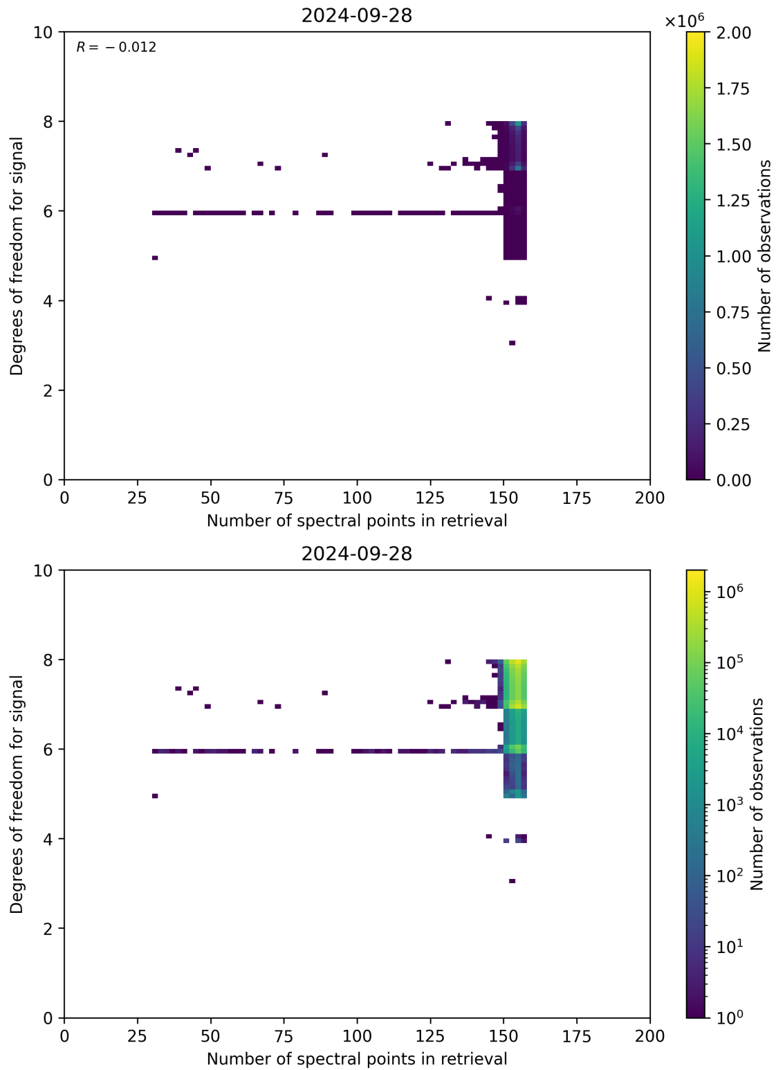
Figure 59: Scatter density plot of “Number of spectral points in retrieval” against “Degrees of freedom for signal” for 2024-09-28 to 2024-09-29.
