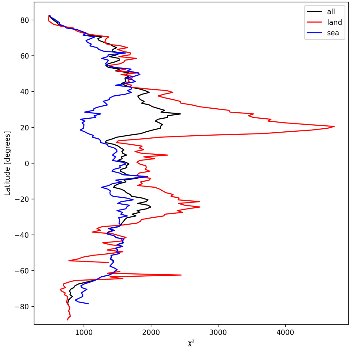
Figure 14: Zonal average of “ \chi^2 ” for 2024-09-28 to 2024-09-29.
