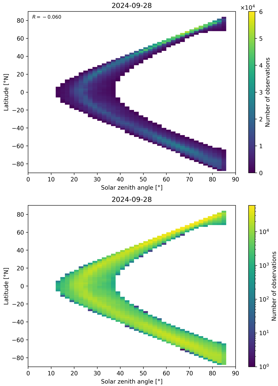
Figure 66: Scatter density plot of “Solar zenith angle” against “Latitude” for 2024-09-28 to 2024-09-29.
