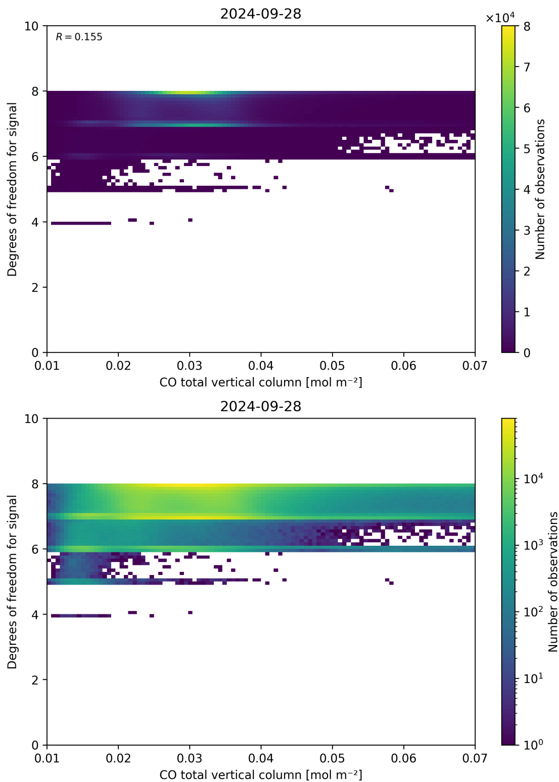
Figure 41: Scatter density plot of “CO total vertical column” against “Degrees of freedom for signal” for 2024-09-28 to 2024-09-29.
