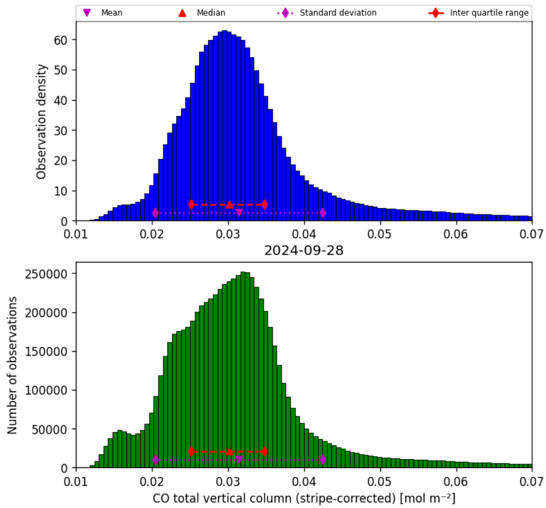
Figure 19: Histogram of “CO total vertical column (stripe-corrected)” for 2024-09-28 to 2024-09-29
