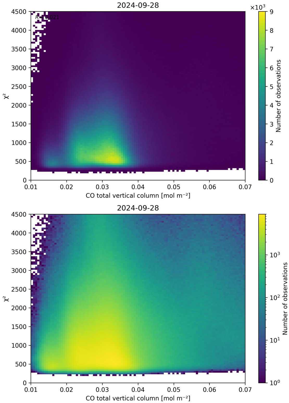
Figure 35: Scatter density plot of “CO total vertical column” against “ \chi^2 ” for 2024-09-28 to 2024-09-29.
