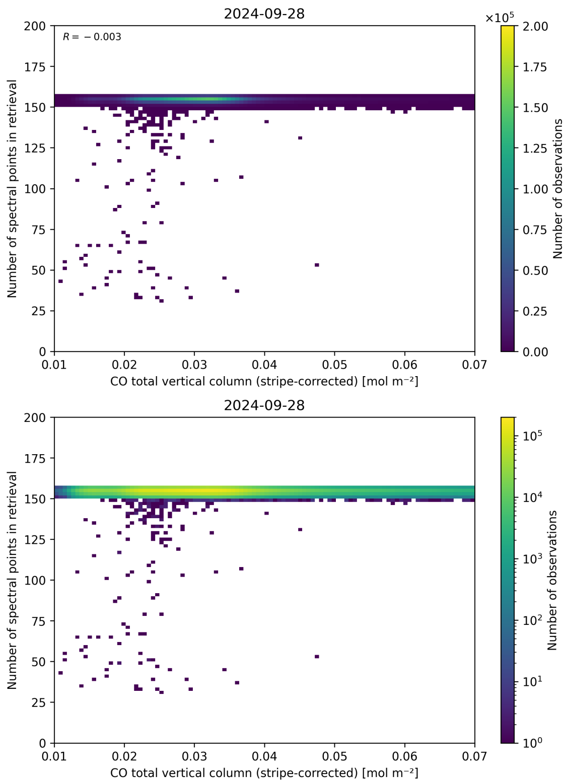
Figure 40: Scatter density plot of “CO total vertical column (stripe-corrected)” against “Number of spectral points in retrieval” for 2024-09-28 to 2024-09-29.
