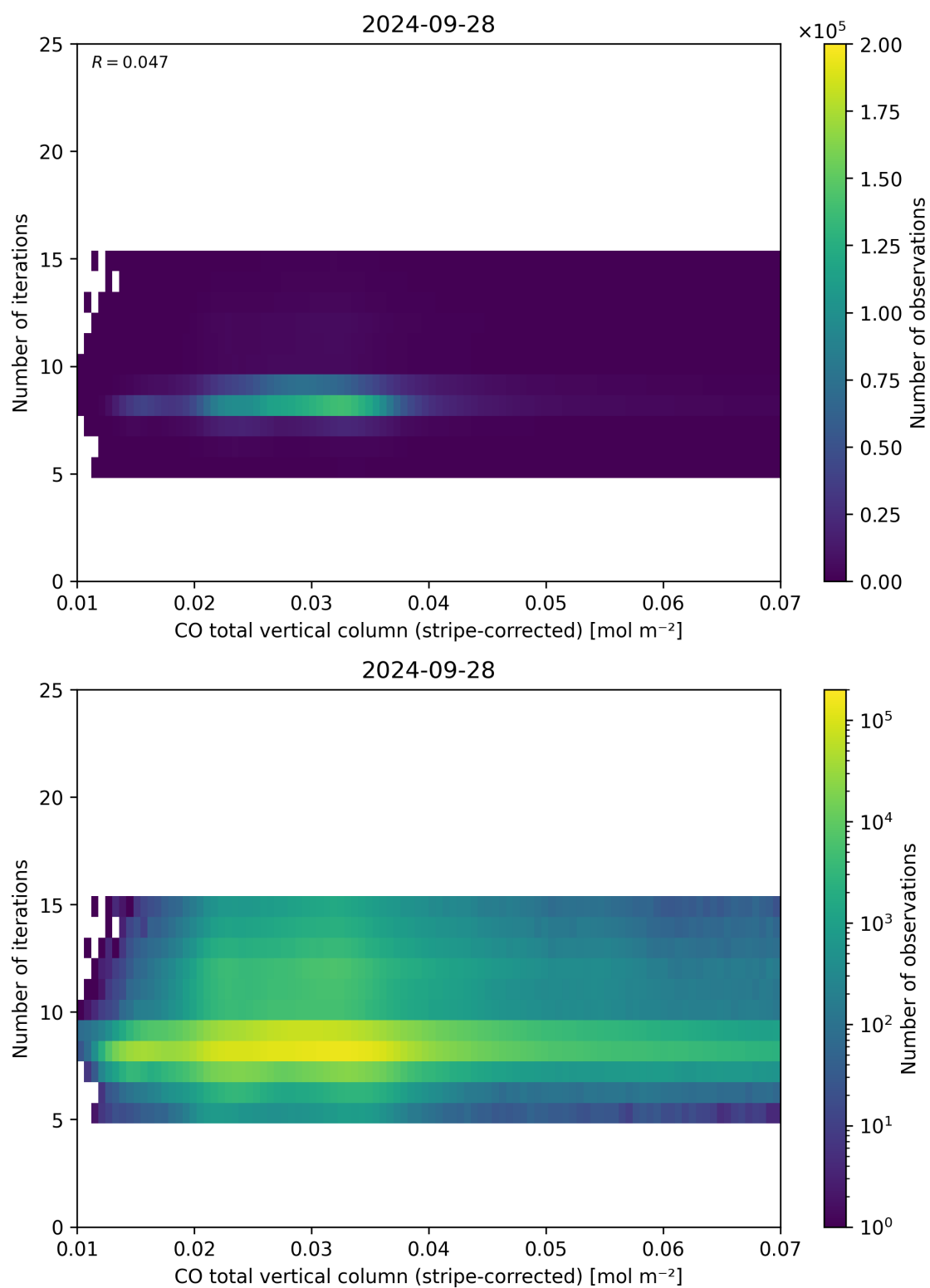
Figure 39: Scatter density plot of “CO total vertical column (stripe-corrected)” against “Number of iterations” for 2024-09-28 to 2024-09-29.
