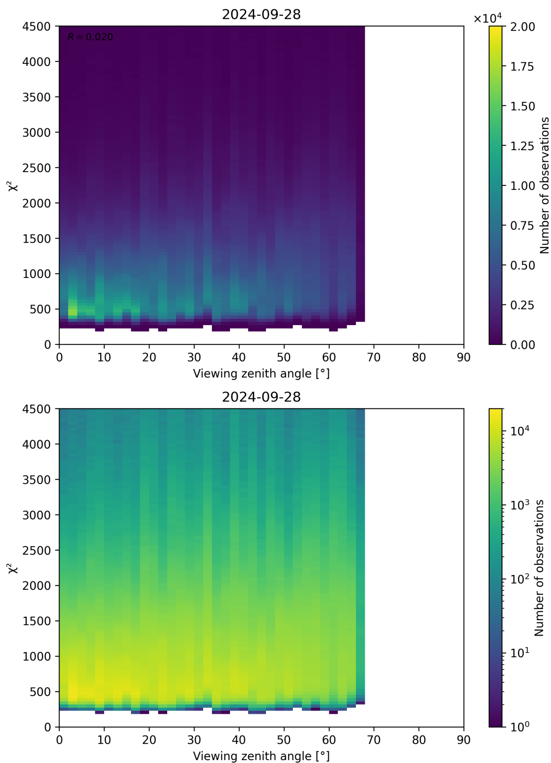
Figure 72: Scatter density plot of “Viewing zenith angle” against “ \chi^2 ” for 2024-09-28 to 2024-09-29.
