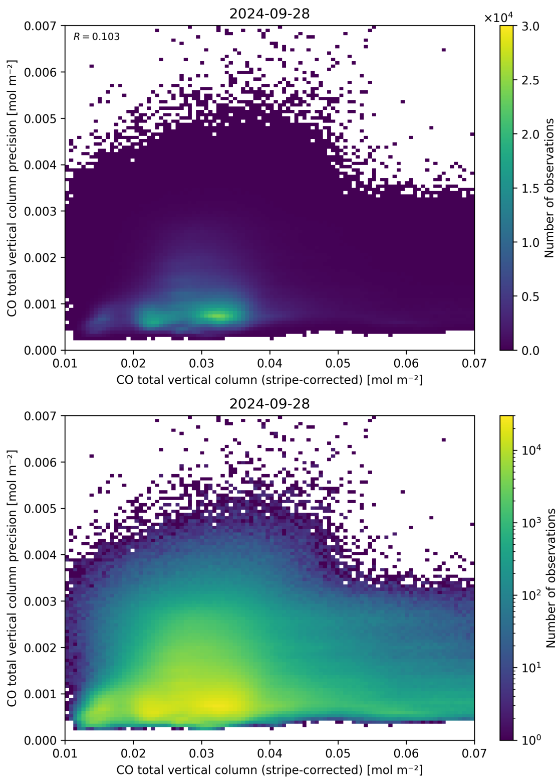
Figure 36: Scatter density plot of “CO total vertical column (stripe-corrected)” against “CO total vertical column precision” for 2024-09-28 to 2024-09-29.
