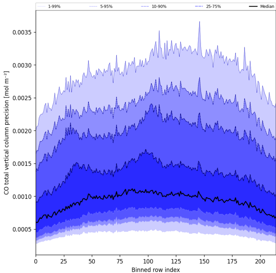
Figure 28: Along track statistics of “CO total vertical column precision” for 2024-09-28 to 2024-09-29
