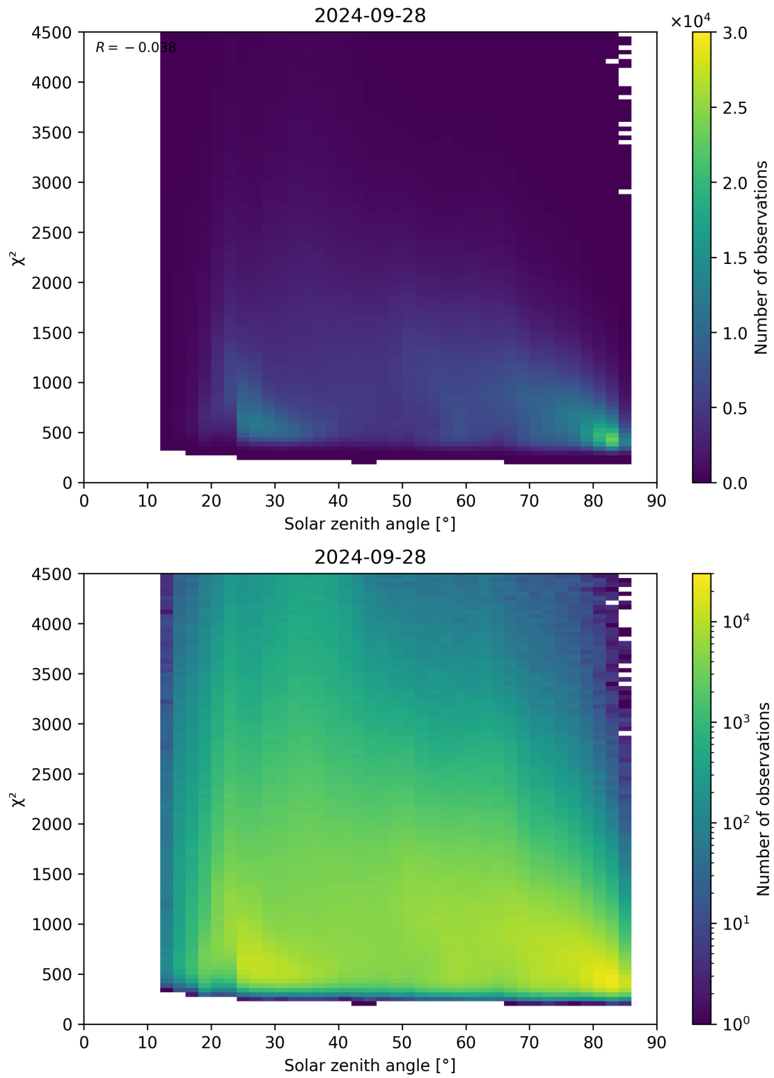
Figure 64: Scatter density plot of “Solar zenith angle” against “ \chi^2 ” for 2024-09-28 to 2024-09-29.
