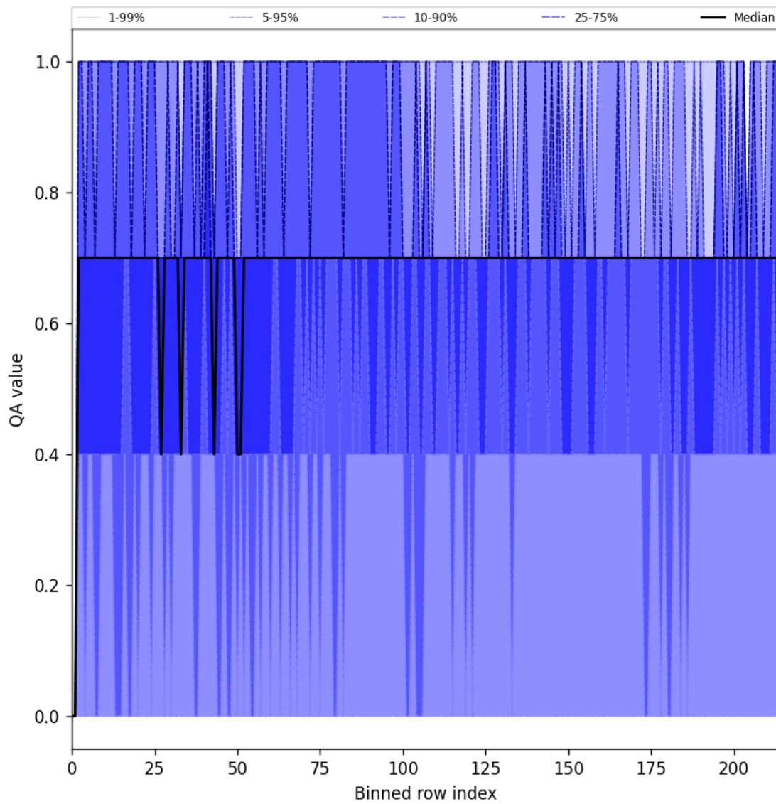
Figure 25: Along track statistics of “QA value” for 2024-09-28 to 2024-09-29
