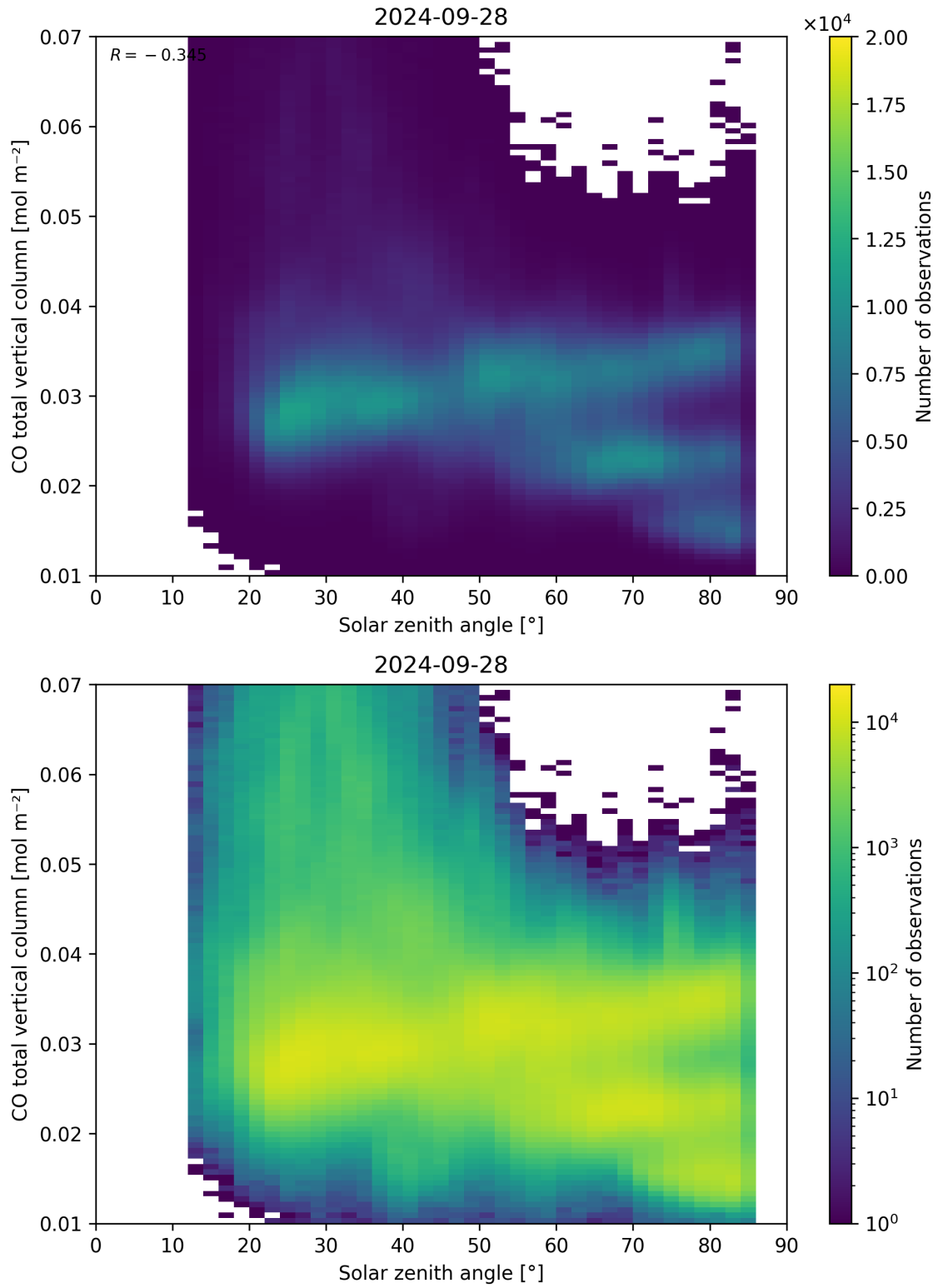
Figure 61: Scatter density plot of “Solar zenith angle” against “CO total vertical column” for 2024-09-28 to 2024-09-29.
