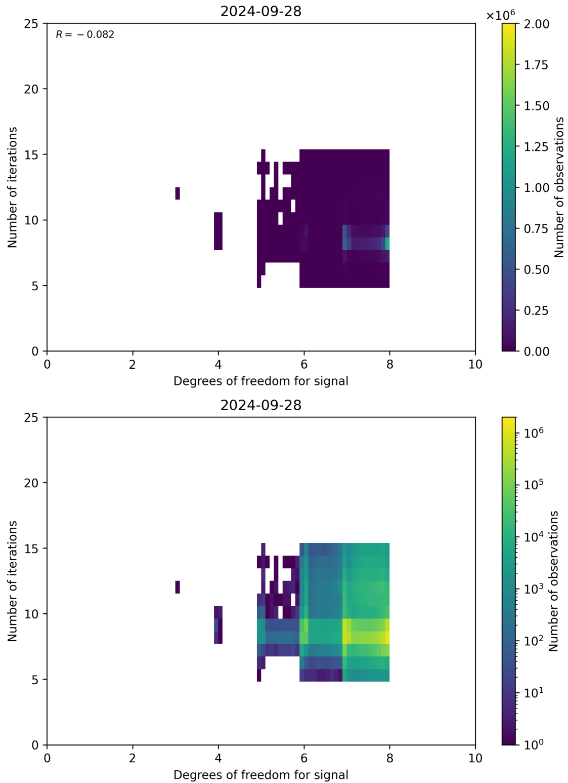
Figure 50: Scatter density plot of “Degrees of freedom for signal” against “Number of iterations” for 2024-09-28 to 2024-09-29.
