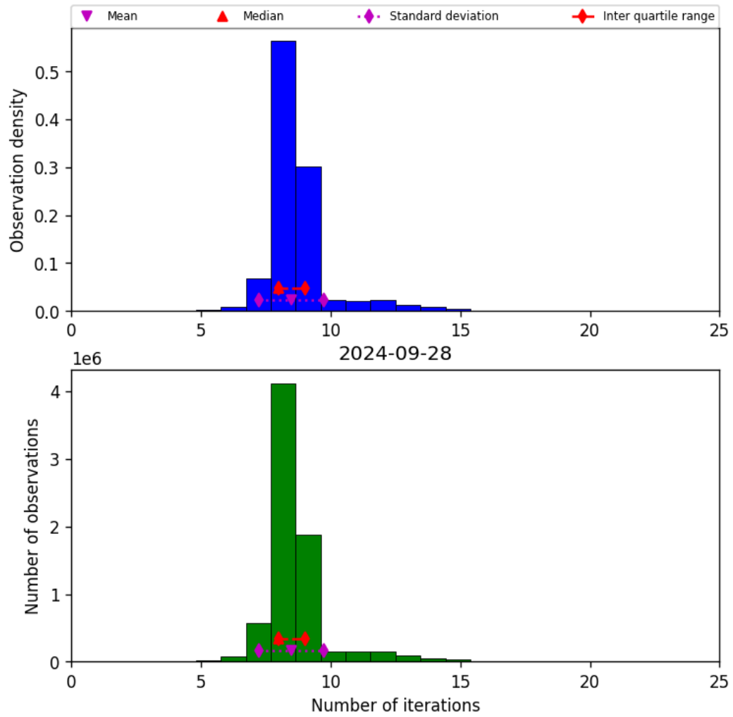
Figure 24: Histogram of “Number of iterations” for 2024-09-28 to 2024-09-29
