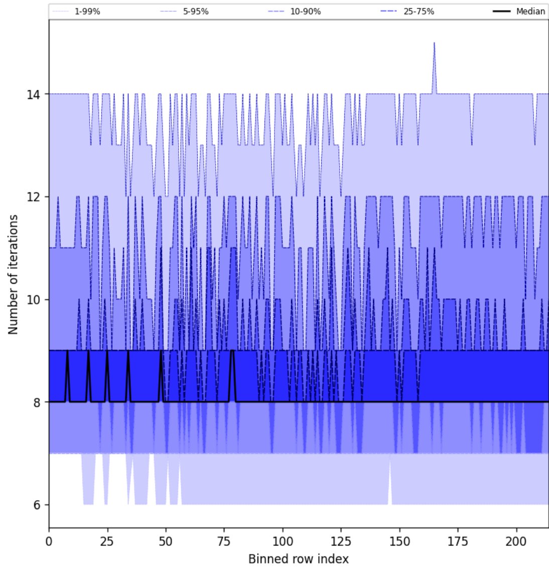
Figure 32: Along track statistics of “Number of iterations” for 2024-09-28 to 2024-09-29
