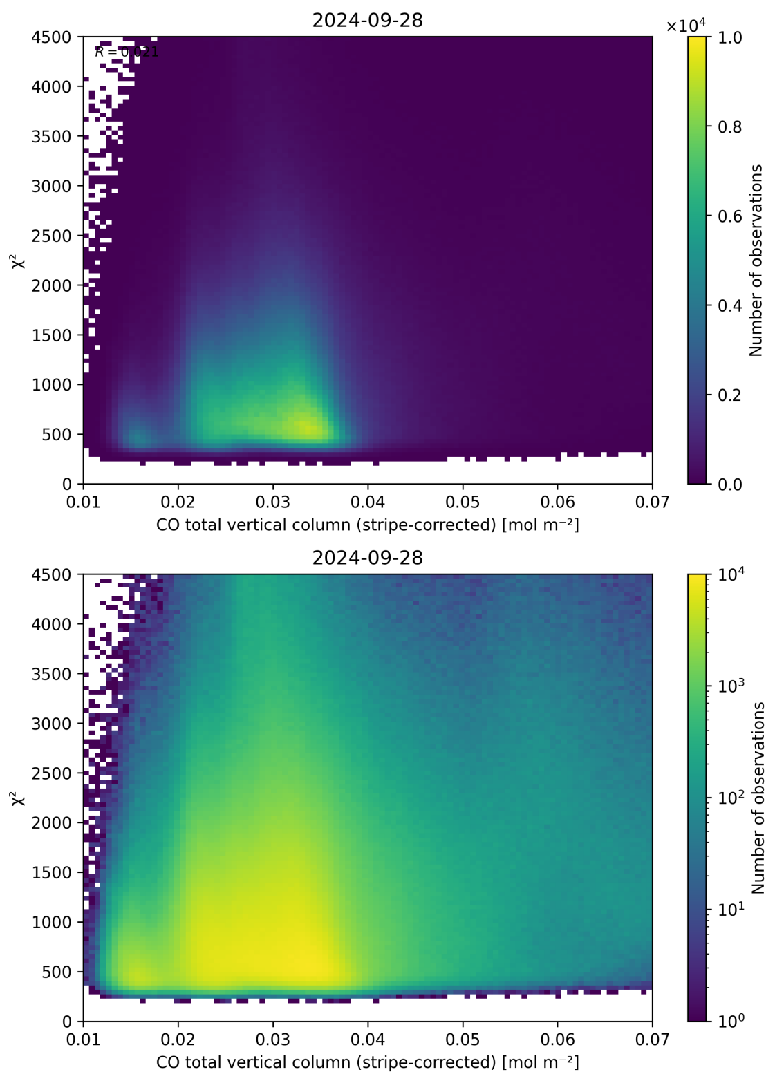
Figure 37: Scatter density plot of “CO total vertical column (stripe-corrected)” against “ \chi^2 ” for 2024-09-28 to 2024-09-29.
