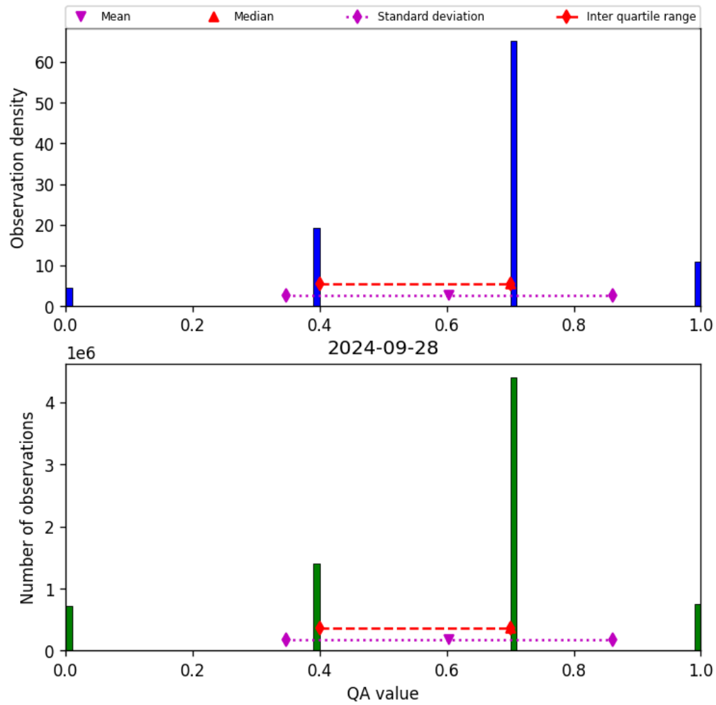
Figure 17: Histogram of “QA value” for 2024-09-28 to 2024-09-29
