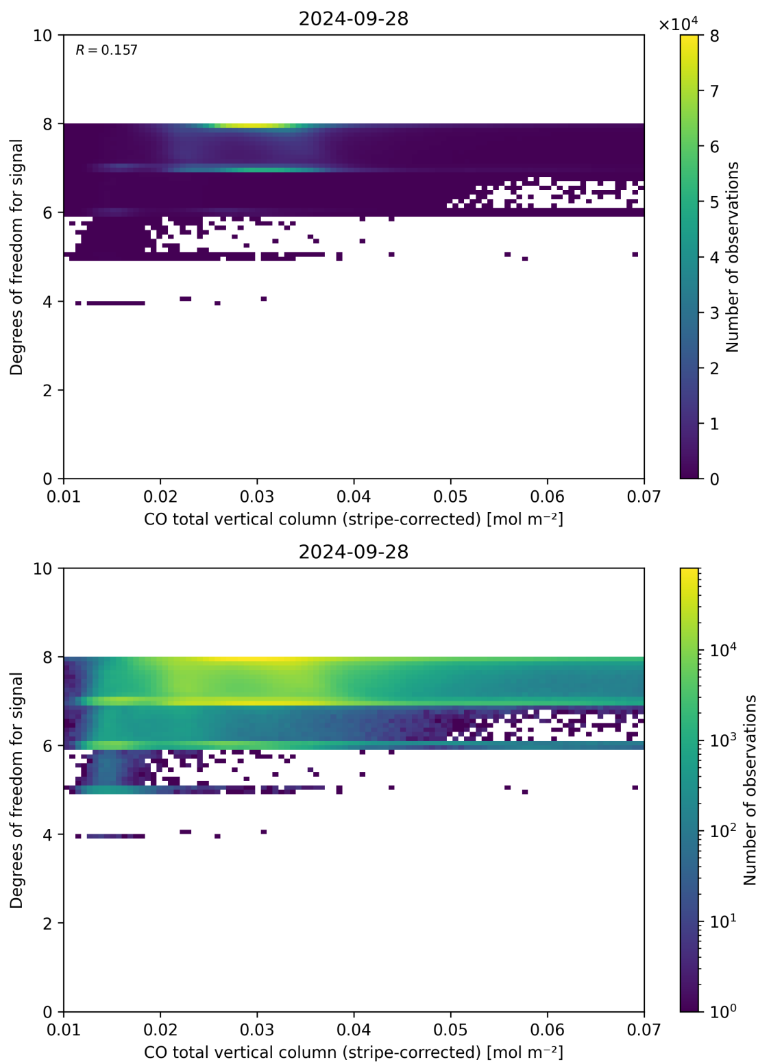
Figure 38: Scatter density plot of “CO total vertical column (stripe-corrected)” against “Degrees of freedom for signal” for 2024-09-28 to 2024-09-29.
