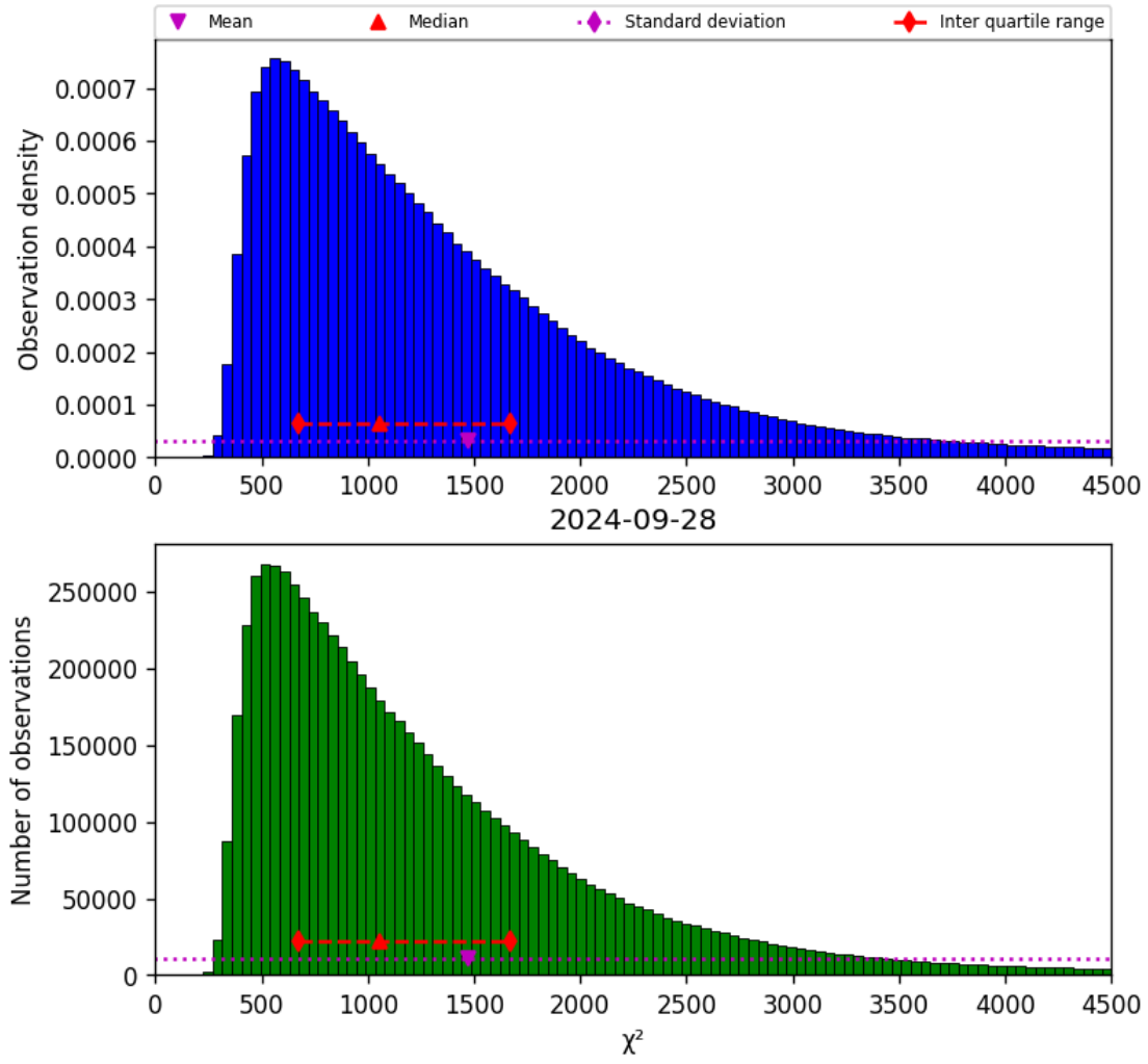
Figure 22: Histogram of “ \chi^2 ” for 2024-09-28 to 2024-09-29
