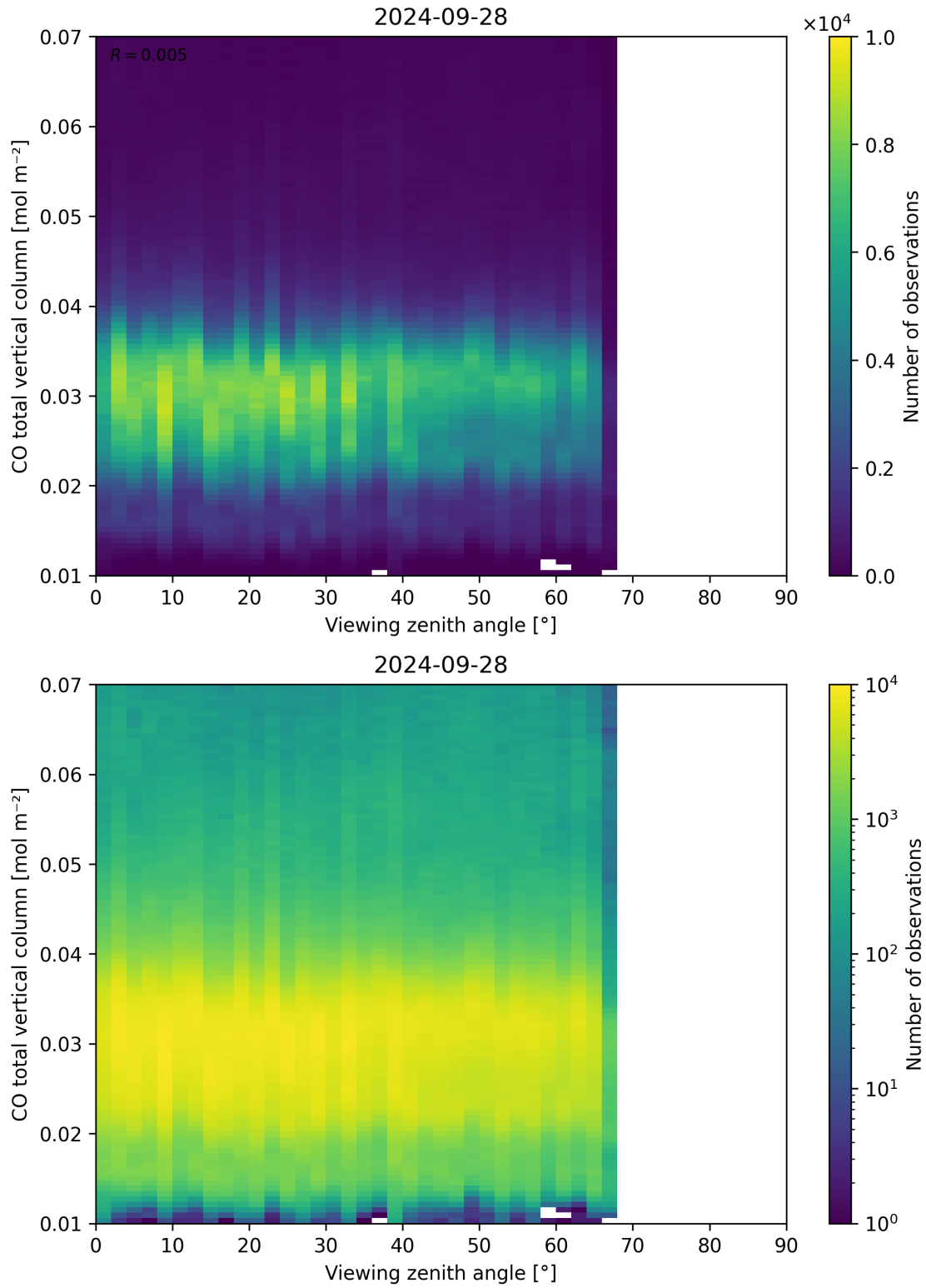
Figure 69: Scatter density plot of “Viewing zenith angle” against “CO total vertical column” for 2024-09-28 to 2024-09-29.
