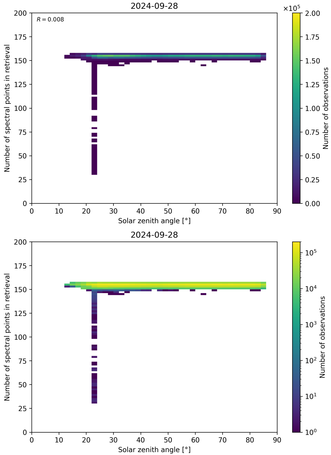
Figure 68: Scatter density plot of “Solar zenith angle” against “Number of spectral points in retrieval” for 2024-09-28 to 2024-09-29.
