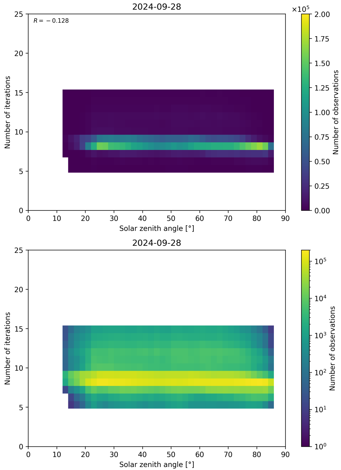
Figure 67: Scatter density plot of “Solar zenith angle” against “Number of iterations” for 2024-09-28 to 2024-09-29.
