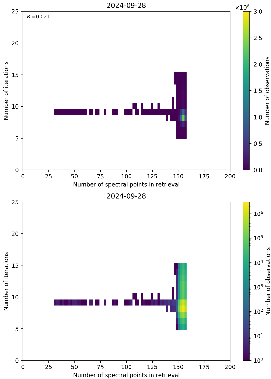
Figure 60: Scatter density plot of “Number of spectral points in retrieval” against “Number of iterations” for 2024-09-28 to 2024-09-29.
