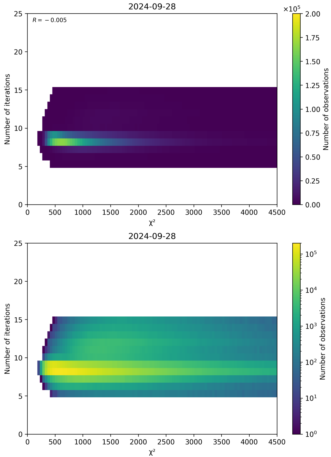
Figure 49: Scatter density plot of “ \chi^2 ” against “Number of iterations” for 2024-09-28 to 2024-09-29.
