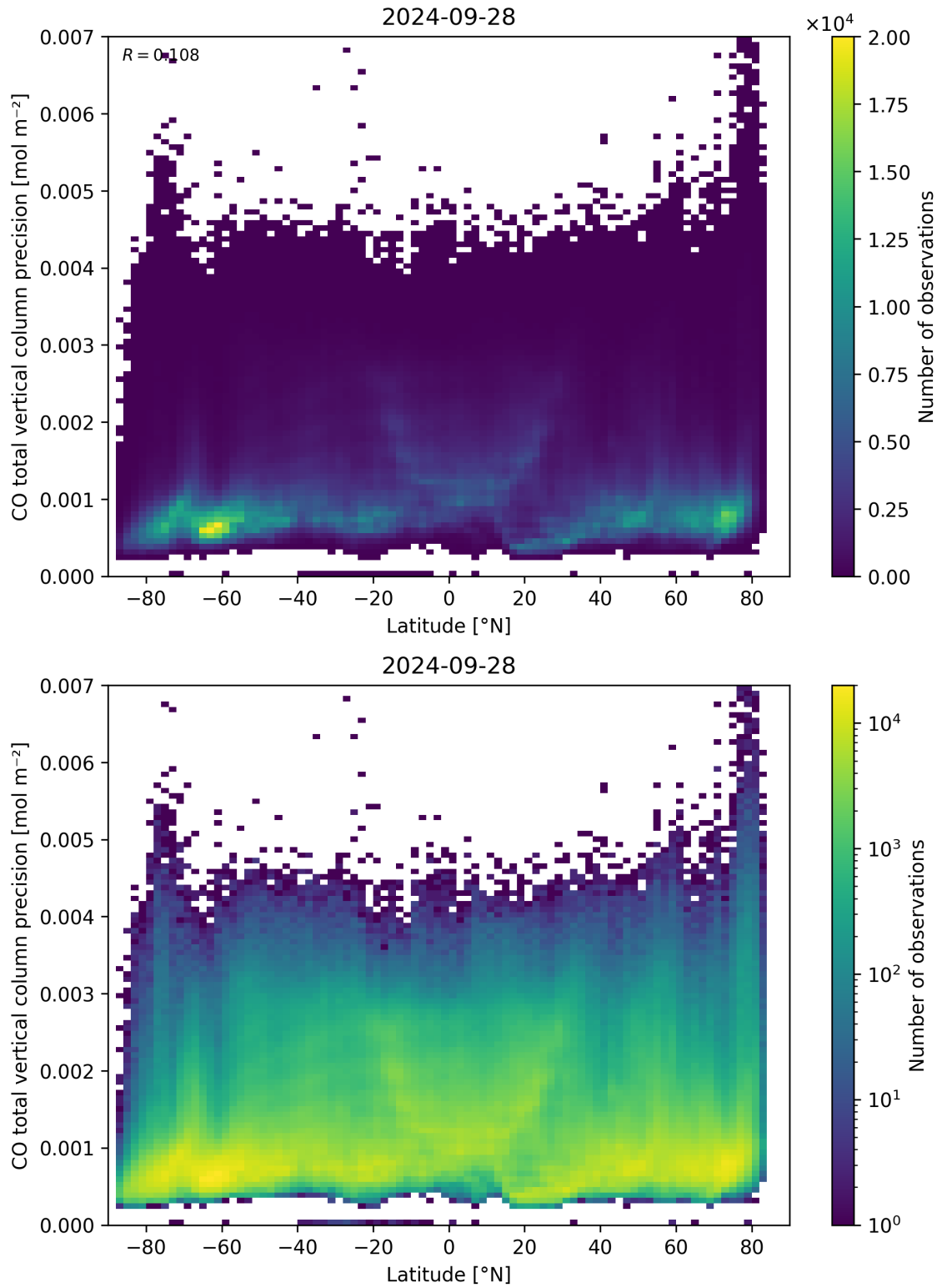
Figure 53: Scatter density plot of “Latitude” against “CO total vertical column precision” for 2024-09-28 to 2024-09-29.
