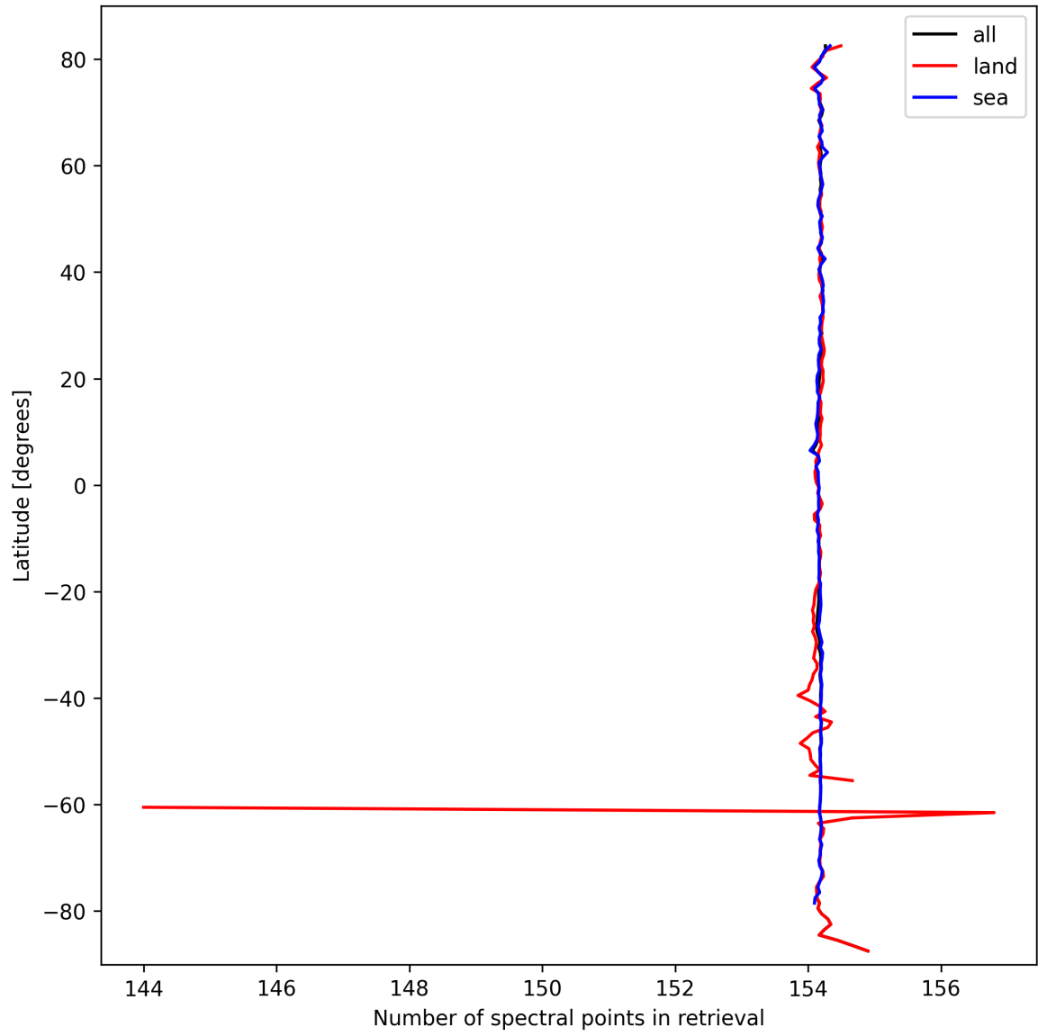
Figure 13: Zonal average of “Number of spectral points in retrieval” for 2024-09-28 to 2024-09-29.
