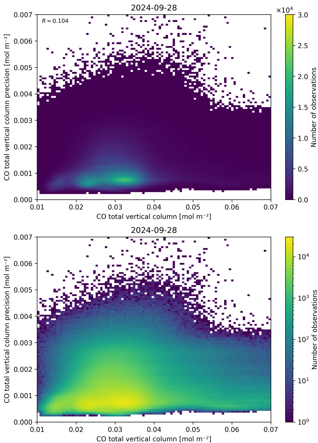
Figure 34: Scatter density plot of “CO total vertical column” against “CO total vertical column precision” for 2024-09-28 to 2024-09-29.
