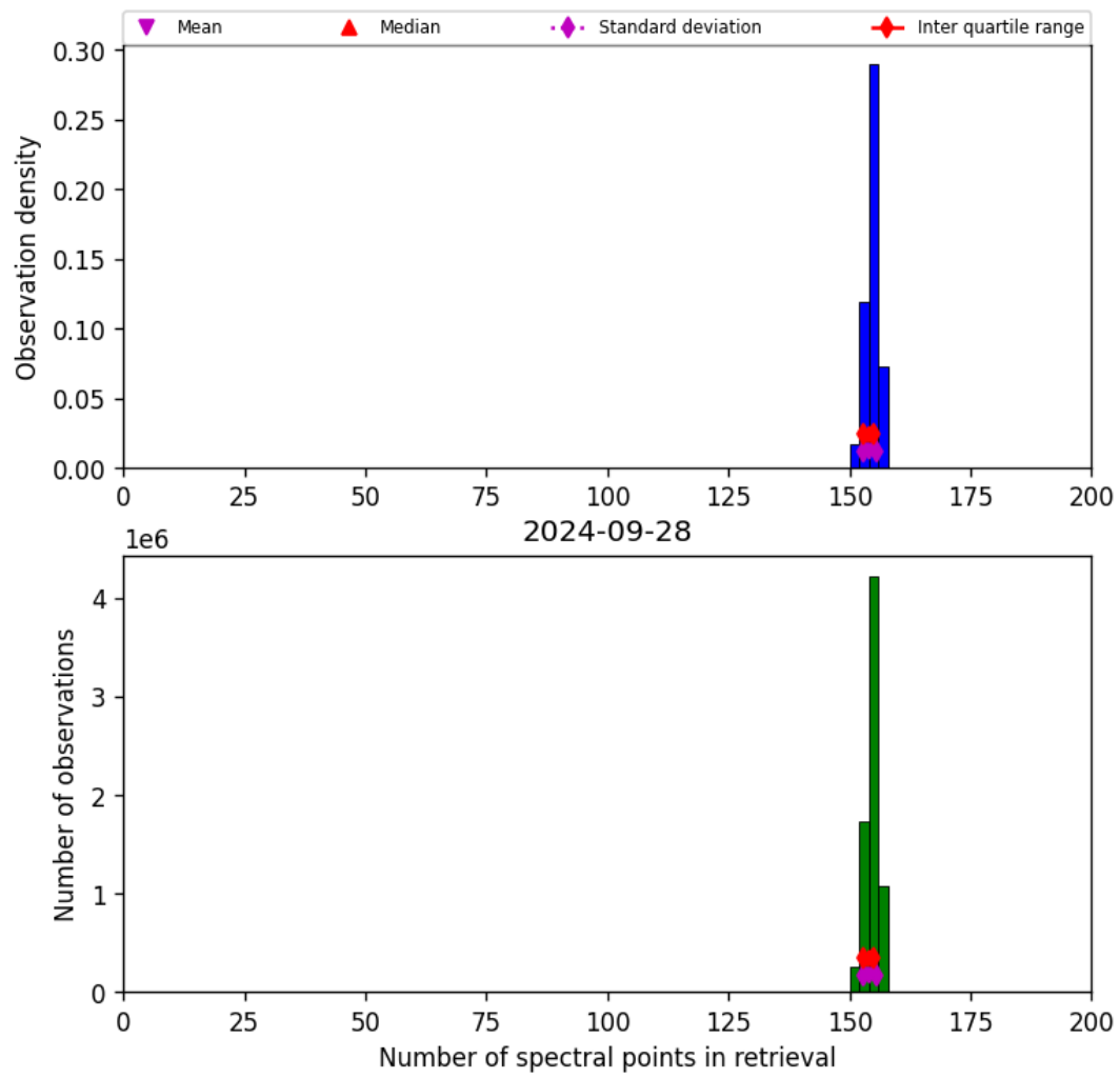
Figure 21: Histogram of “Number of spectral points in retrieval” for 2024-09-28 to 2024-09-29
