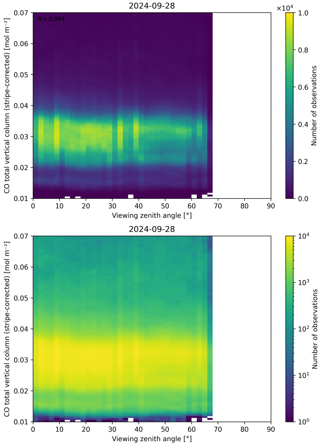
Figure 70: Scatter density plot of “Viewing zenith angle” against “CO total vertical column (stripe-corrected)” for 2024-09-28 to 2024-09-29.
