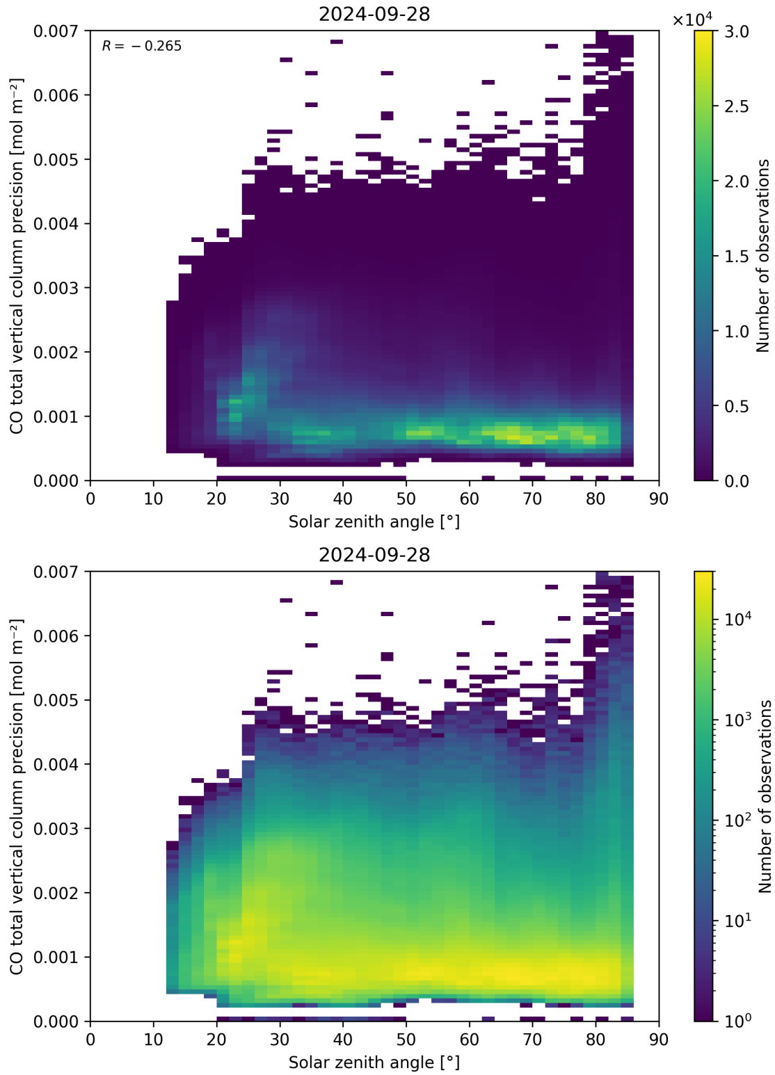
Figure 63: Scatter density plot of “Solar zenith angle” against “CO total vertical column precision” for 2024-09-28 to 2024-09-29.
