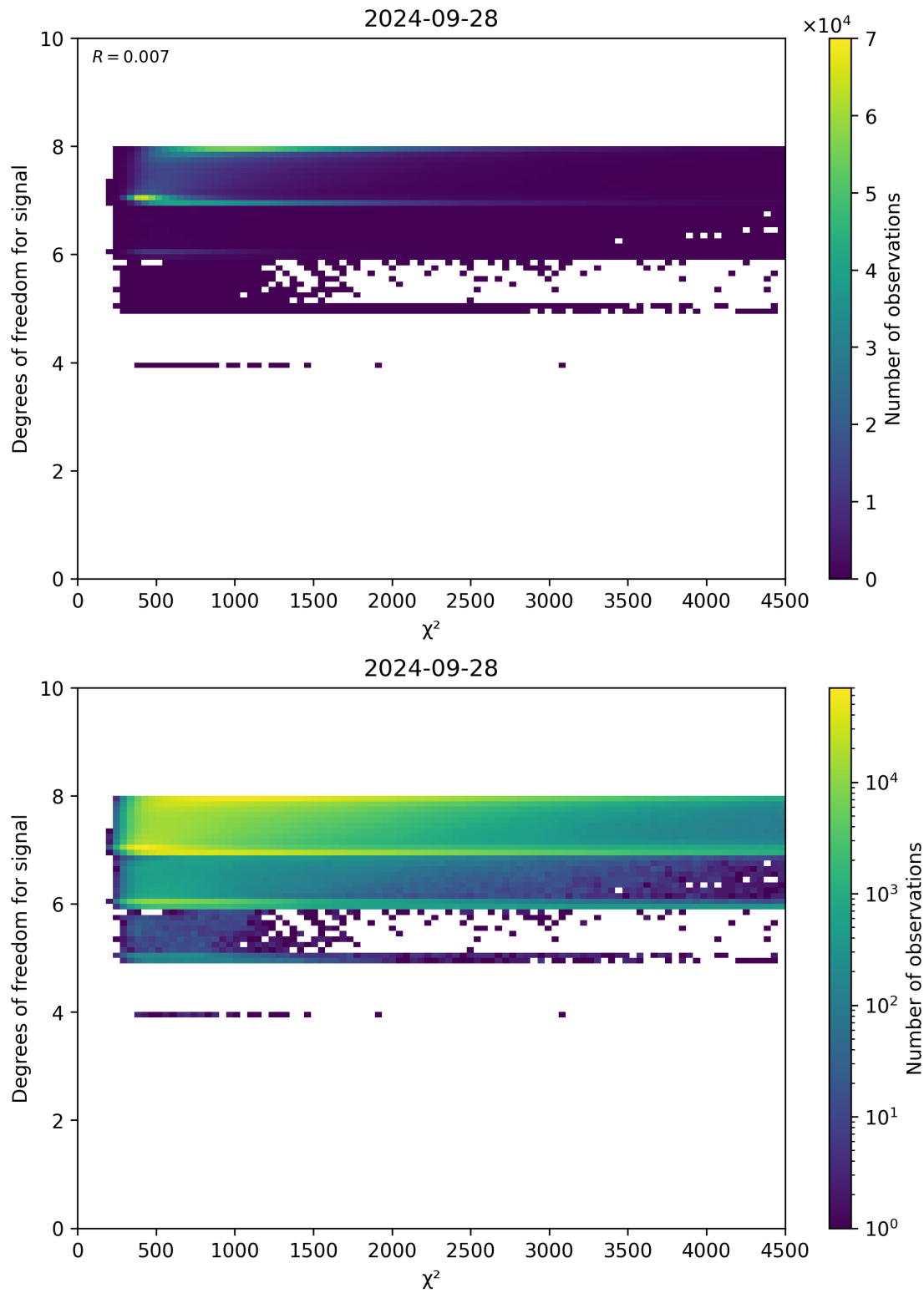
Figure 48: Scatter density plot of “ \chi^2 ” against “Degrees of freedom for signal” for 2024-09-28 to 2024-09-29.
