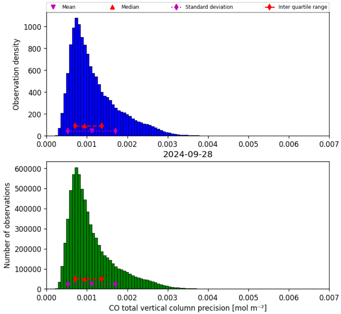
Figure 20: Histogram of “CO total vertical column precision” for 2024-09-28 to 2024-09-29
