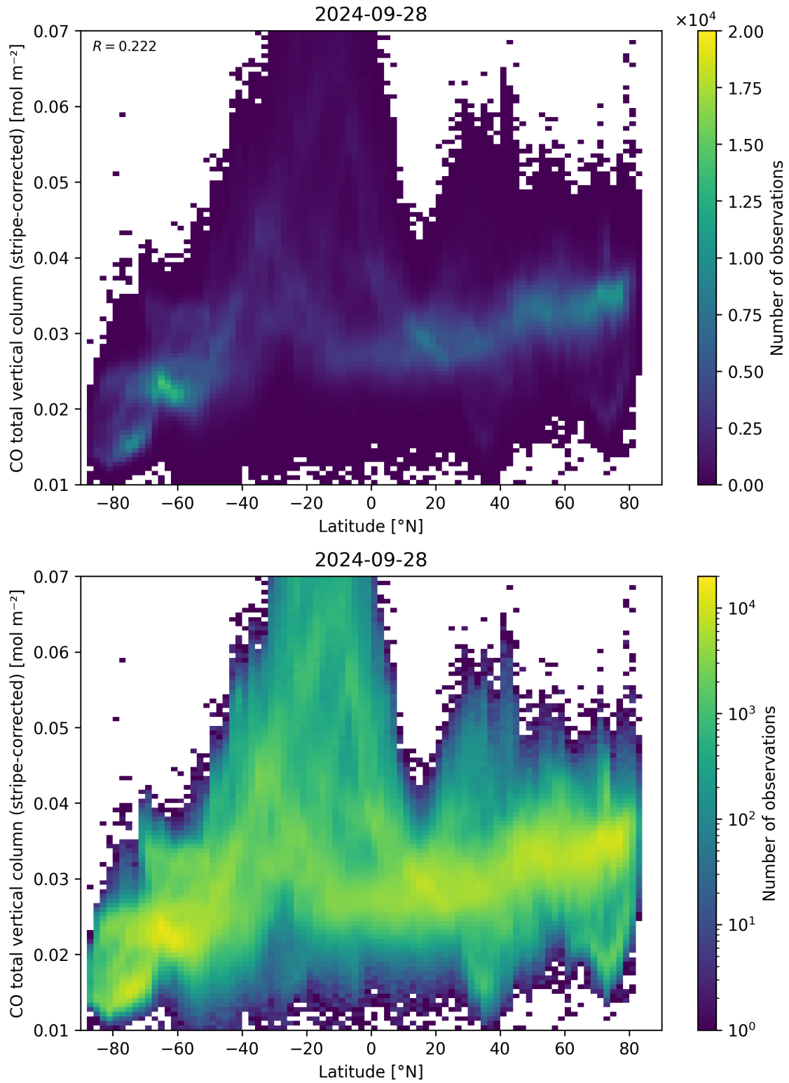
Figure 52: Scatter density plot of “Latitude” against “CO total vertical column (stripe-corrected)” for 2024-09-28 to 2024-09-29.
