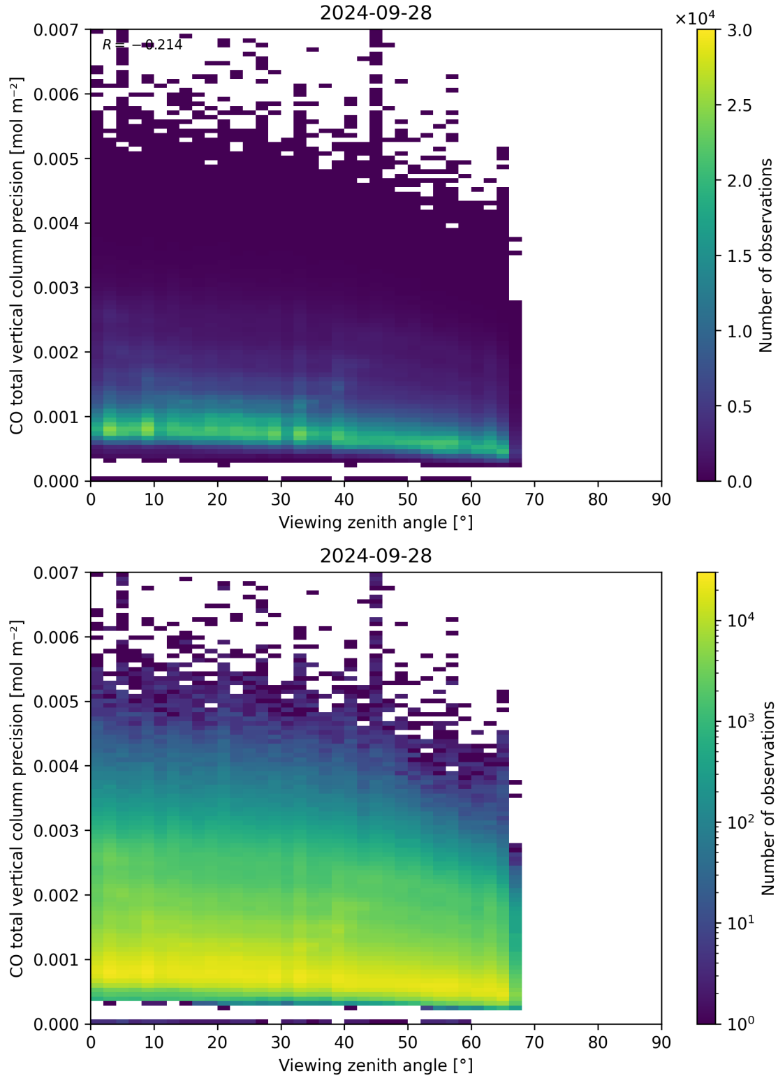
Figure 71: Scatter density plot of “Viewing zenith angle” against “CO total vertical column precision” for 2024-09-28 to 2024-09-29.
