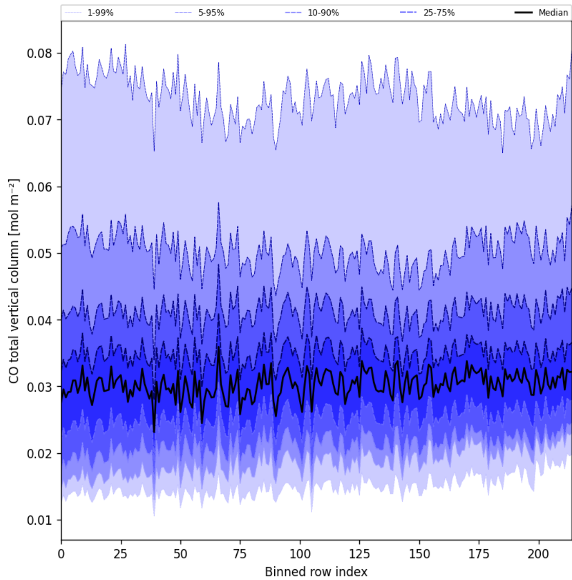
Figure 26: Along track statistics of “CO total vertical column” for 2024-09-28 to 2024-09-29
