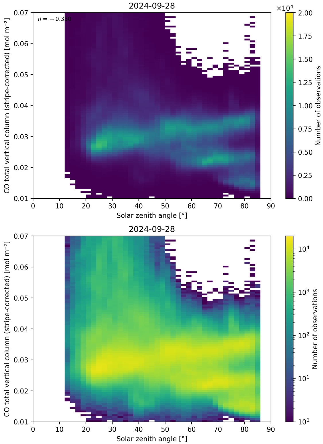
Figure 62: Scatter density plot of “Solar zenith angle” against “CO total vertical column (stripe-corrected)” for 2024-09-28 to 2024-09-29.
