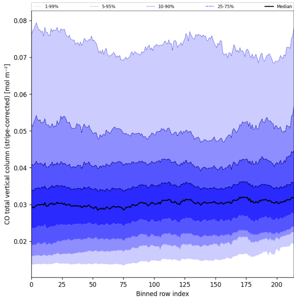
Figure 27: Along track statistics of “CO total vertical column (stripe-corrected)” for 2024-09-28 to 2024-09-29
