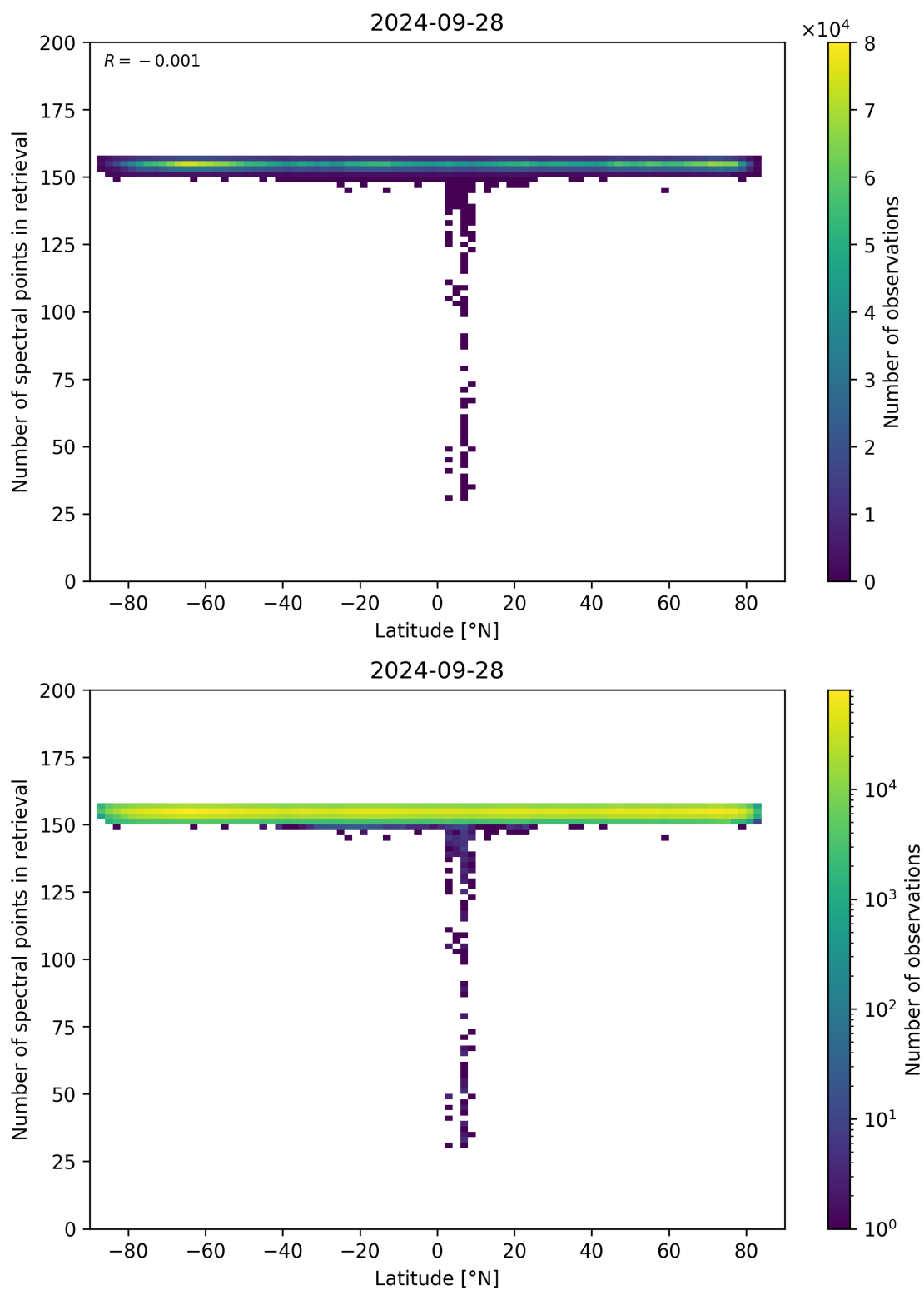
Figure 57: Scatter density plot of “Latitude” against “Number of spectral points in retrieval” for 2024-09-28 to 2024-09-29.
