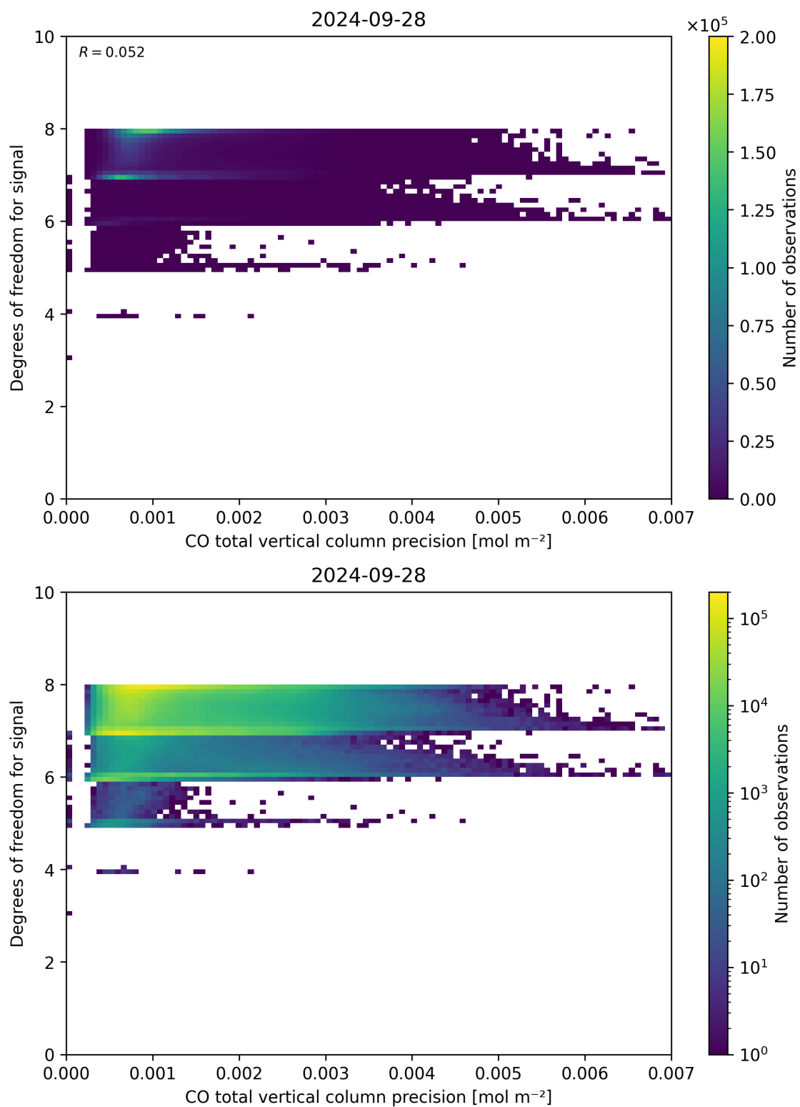
Figure 45: Scatter density plot of “CO total vertical column precision” against “Degrees of freedom for signal” for 2024-09-28 to 2024-09-29.
