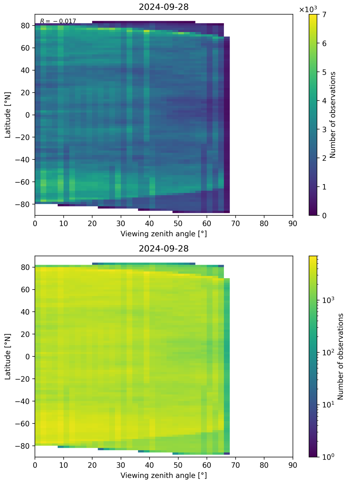
Figure 74: Scatter density plot of “Viewing zenith angle” against “Latitude” for 2024-09-28 to 2024-09-29.
