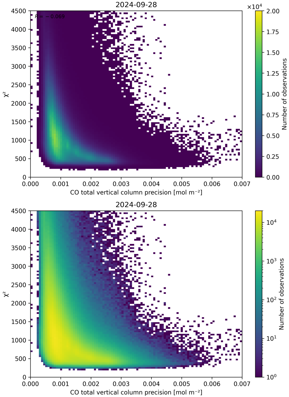
Figure 44: Scatter density plot of “CO total vertical column precision” against “ \chi^2 ” for 2024-09-28 to 2024-09-29.
