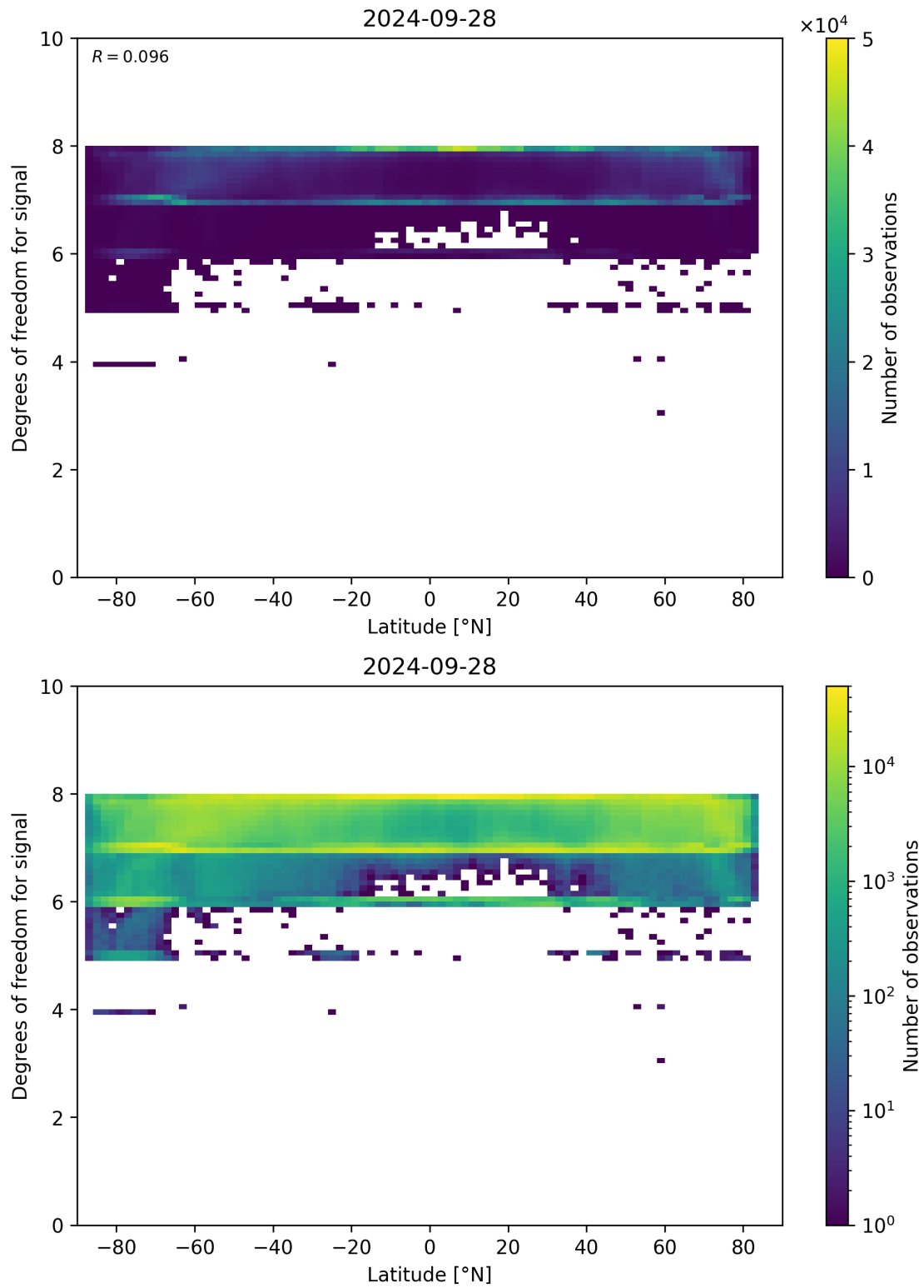
Figure 55: Scatter density plot of “Latitude” against “Degrees of freedom for signal” for 2024-09-28 to 2024-09-29.
