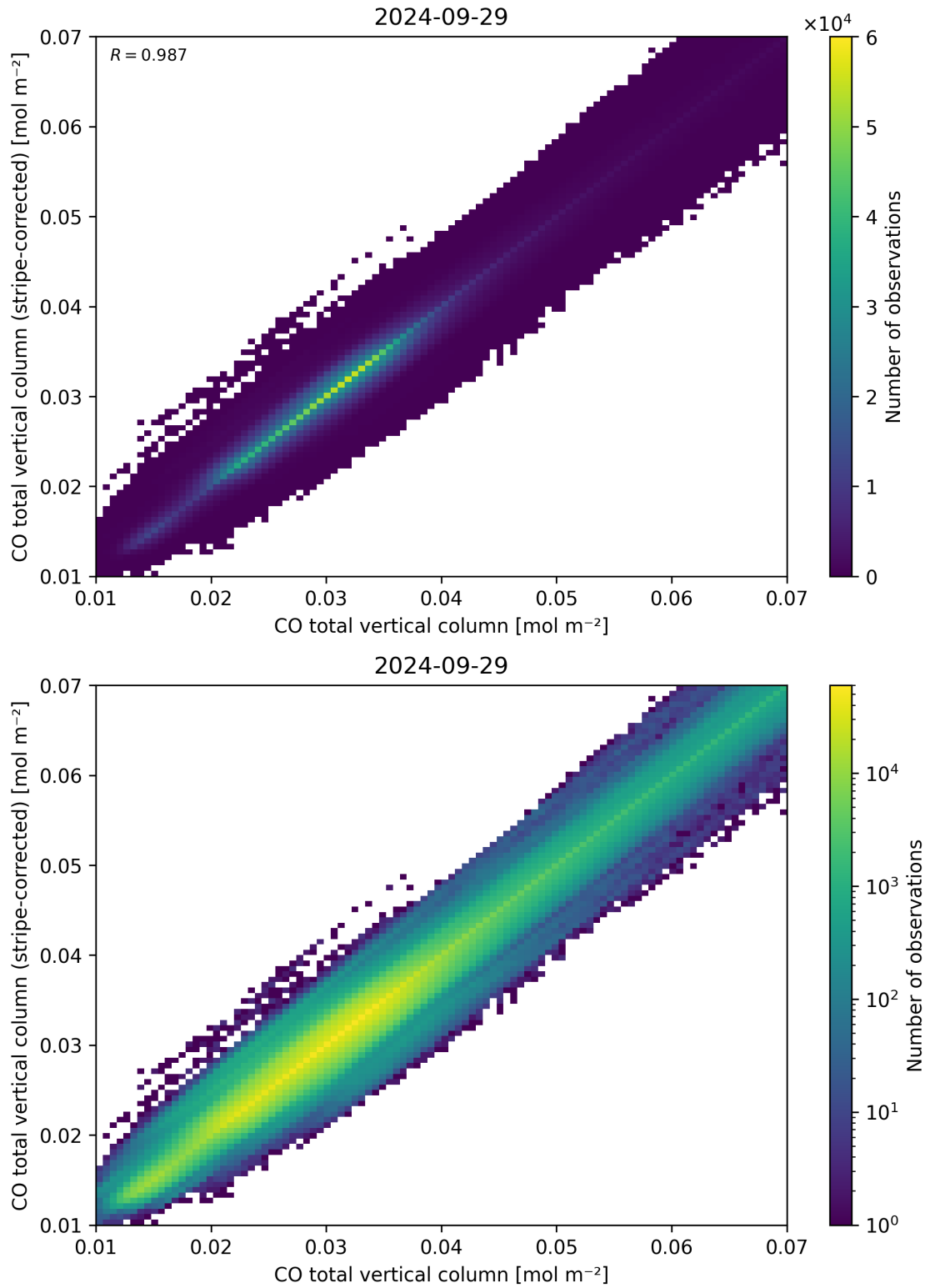
Figure 33: Scatter density plot of “CO total vertical column” against “CO total vertical column (stripe-corrected)” for 2024-09-28 to 2024-09-30.
