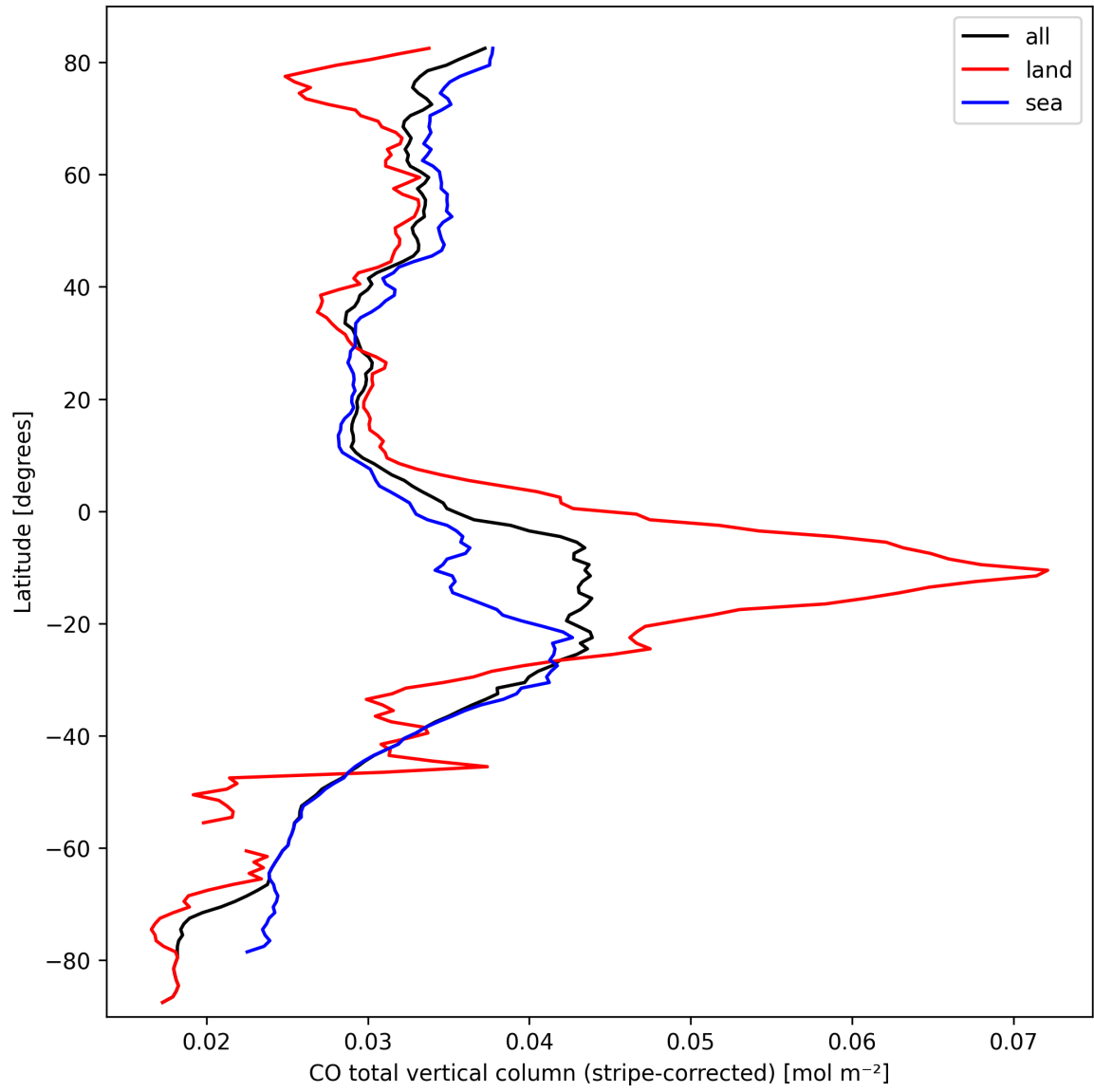
Figure 11: Zonal average of “CO total vertical column (stripe-corrected)” for 2024-09-28 to 2024-09-30.
