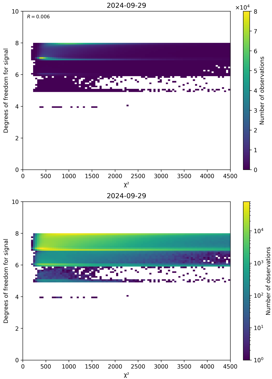
Figure 48: Scatter density plot of “ \chi^2 ” against “Degrees of freedom for signal” for 2024-09-28 to 2024-09-30.
