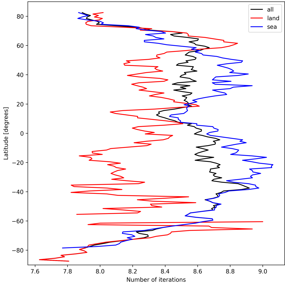
Figure 16: Zonal average of “Number of iterations” for 2024-09-28 to 2024-09-30.
