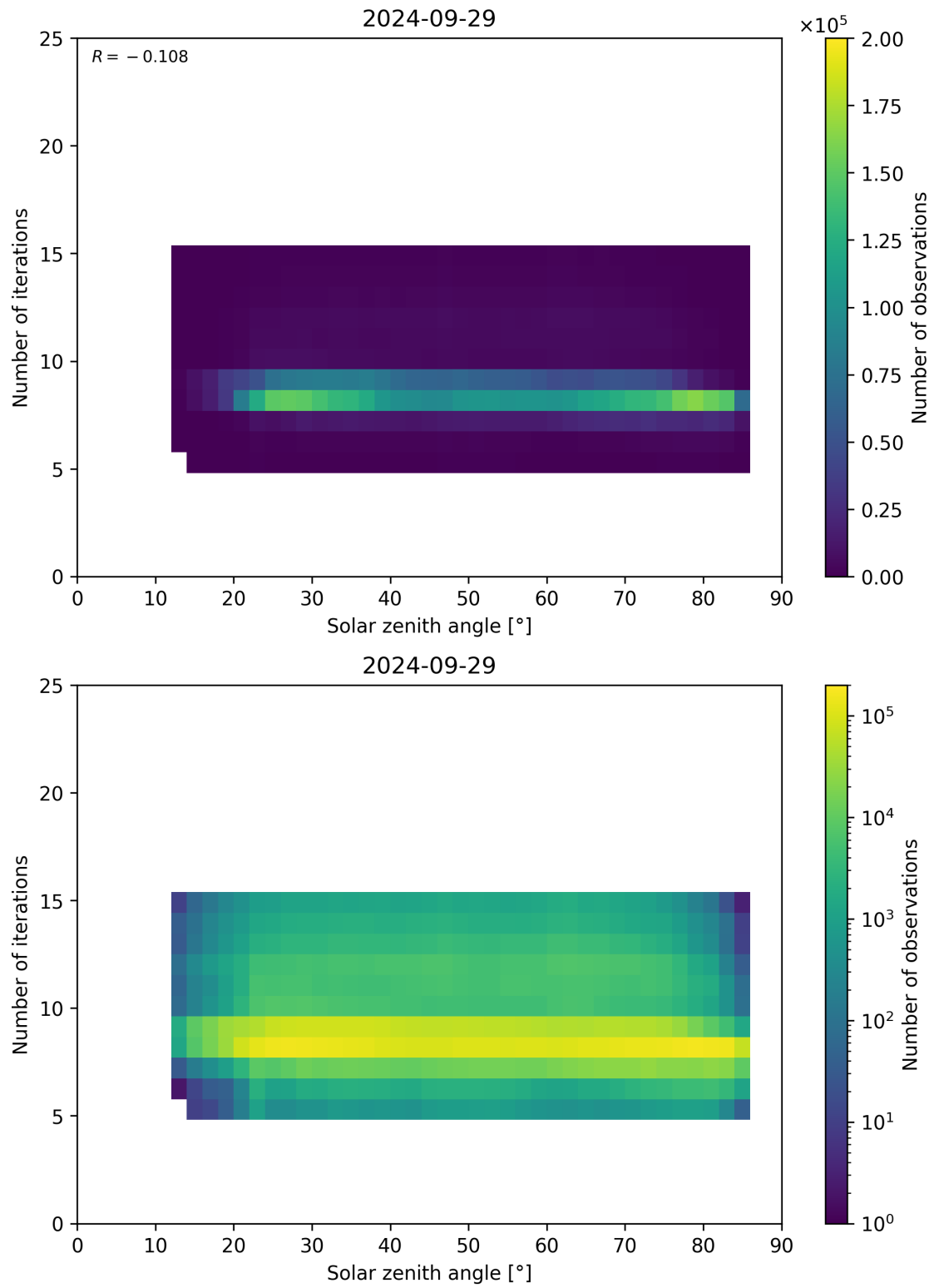
Figure 67: Scatter density plot of “Solar zenith angle” against “Number of iterations” for 2024-09-28 to 2024-09-30.
