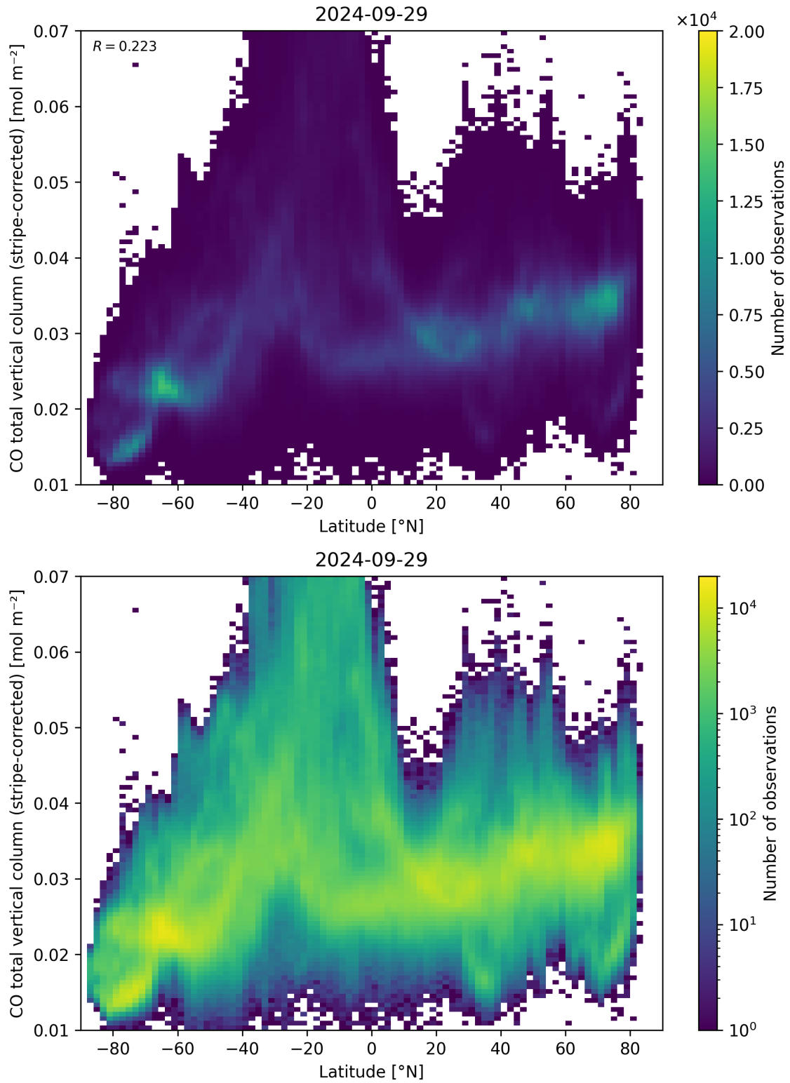
Figure 52: Scatter density plot of “Latitude” against “CO total vertical column (stripe-corrected)” for 2024-09-28 to 2024-09-30.
