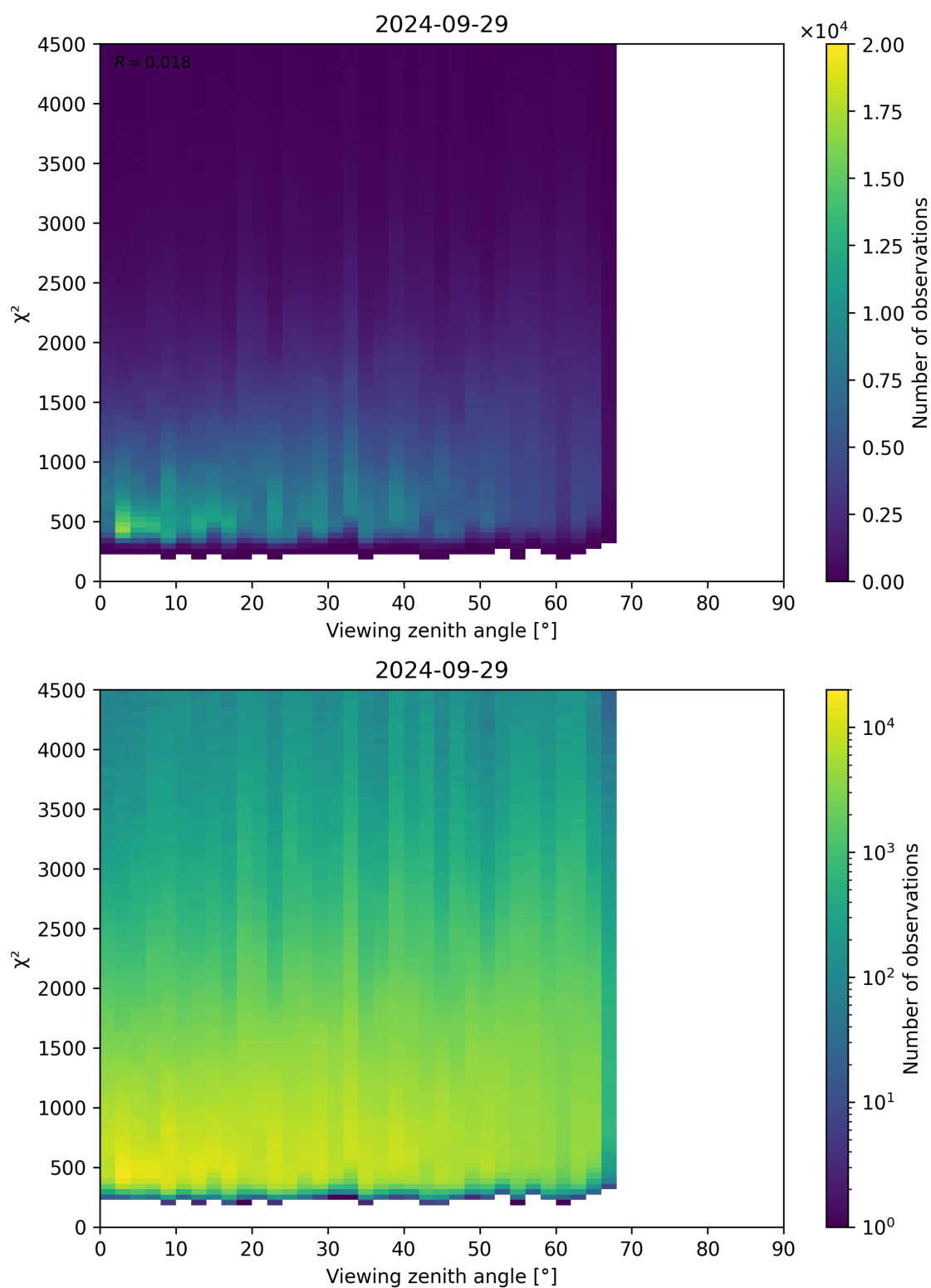
Figure 72: Scatter density plot of “Viewing zenith angle” against “ \chi^2 ” for 2024-09-28 to 2024-09-30.
