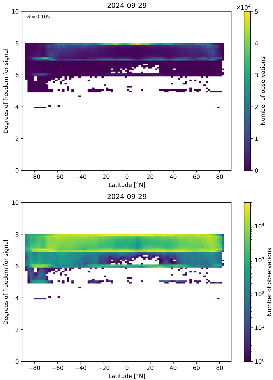
Figure 55: Scatter density plot of “Latitude” against “Degrees of freedom for signal” for 2024-09-28 to 2024-09-30.
