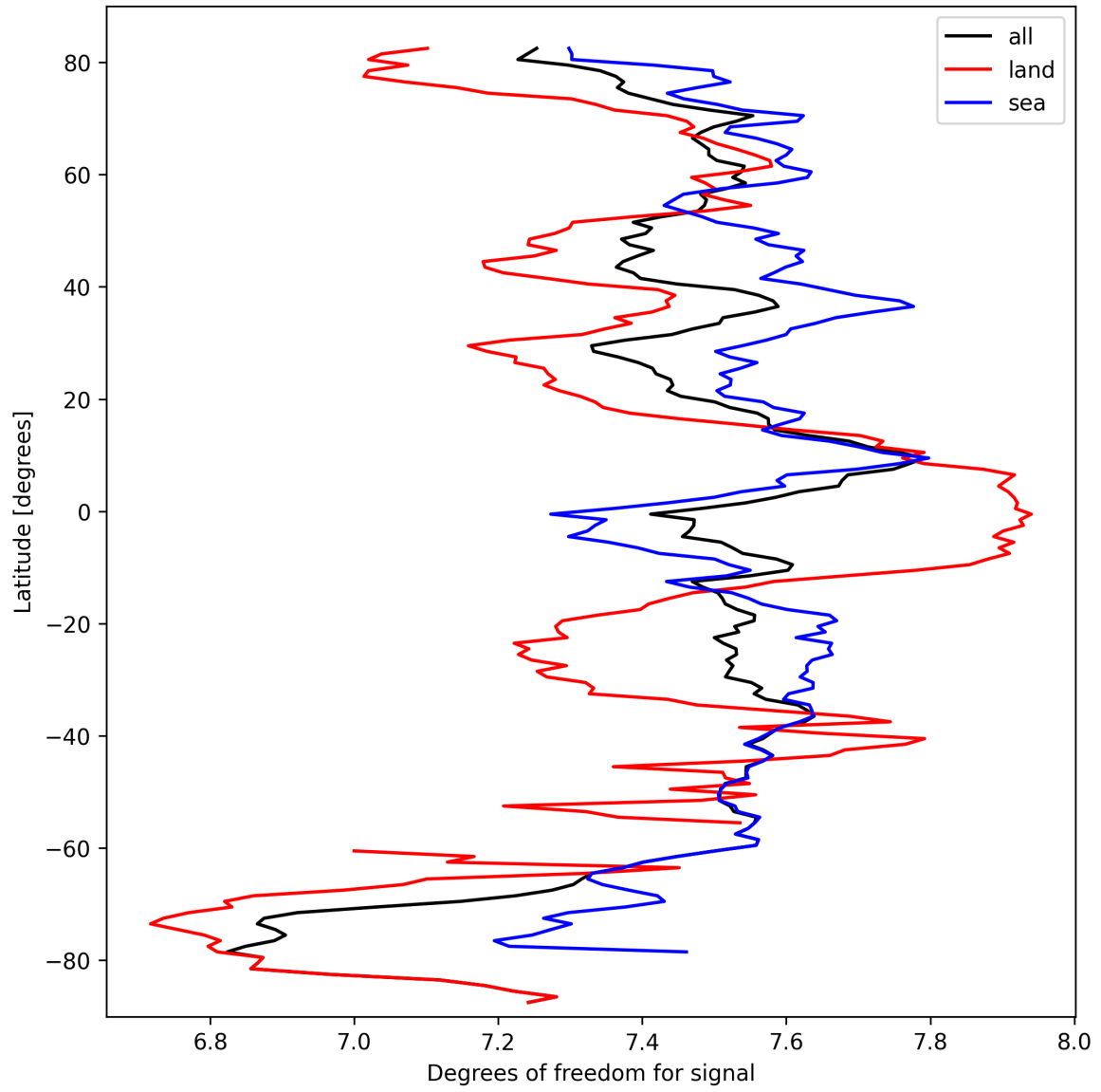
Figure 15: Zonal average of “Degrees of freedom for signal” for 2024-09-28 to 2024-09-30.
