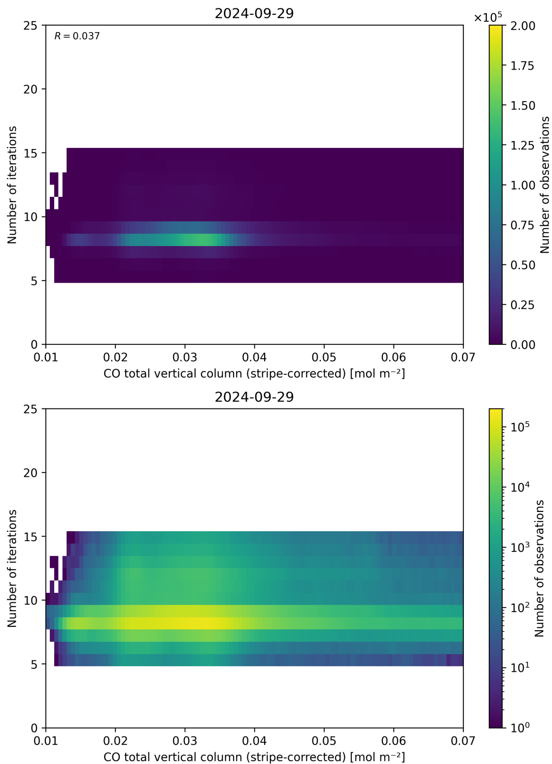
Figure 39: Scatter density plot of “CO total vertical column (stripe-corrected)” against “Number of iterations” for 2024-09-28 to 2024-09-30.
