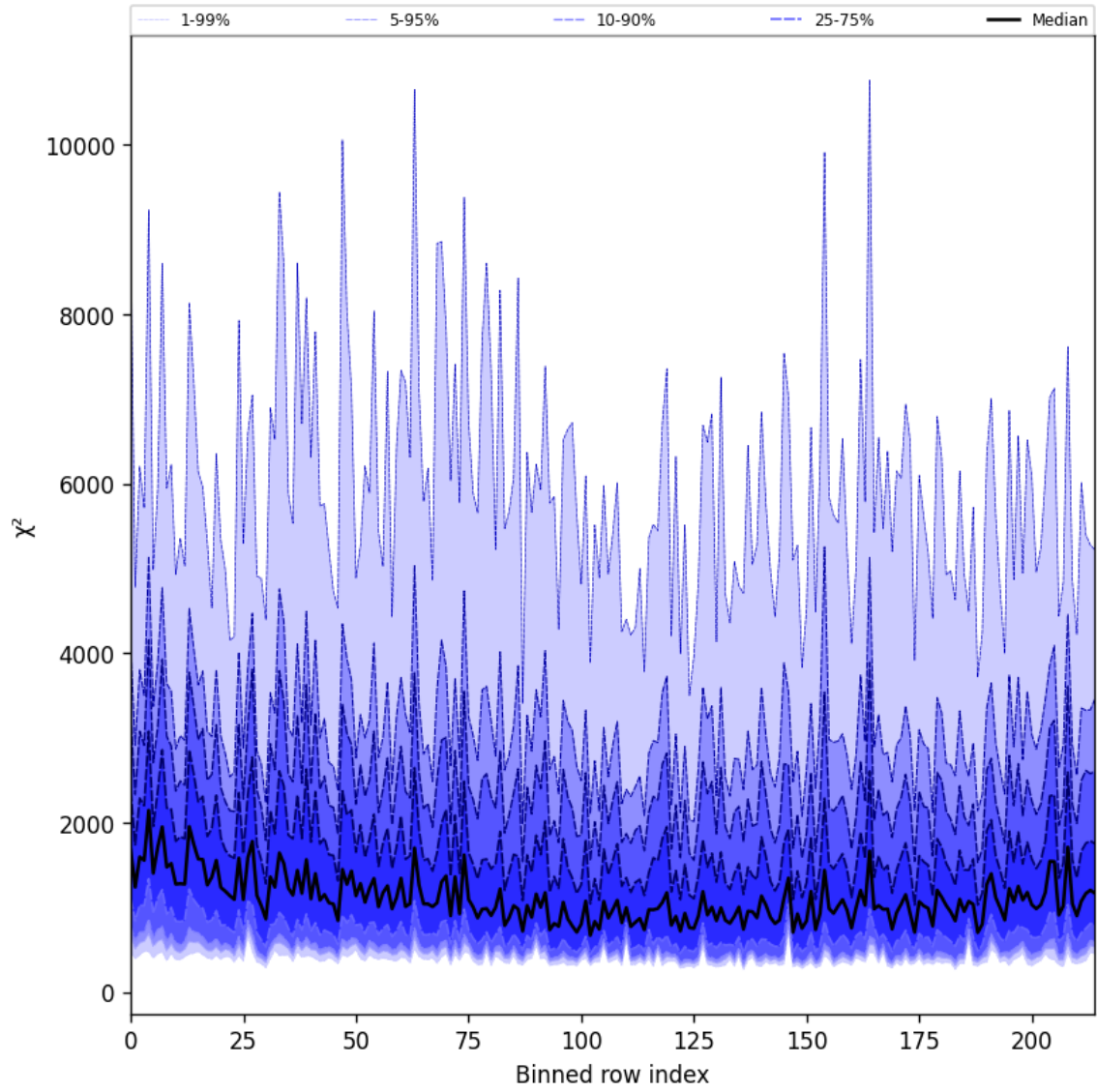
Figure 30: Along track statistics of “ \chi^2 ” for 2024-09-28 to 2024-09-30
