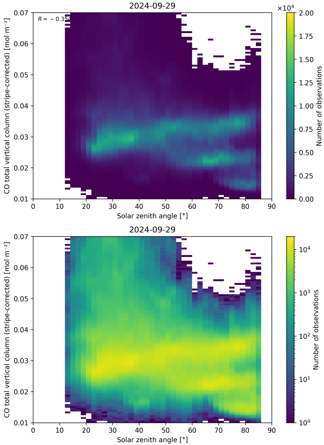
Figure 62: Scatter density plot of “Solar zenith angle” against “CO total vertical column (stripe-corrected)” for 2024-09-28 to 2024-09-30.
