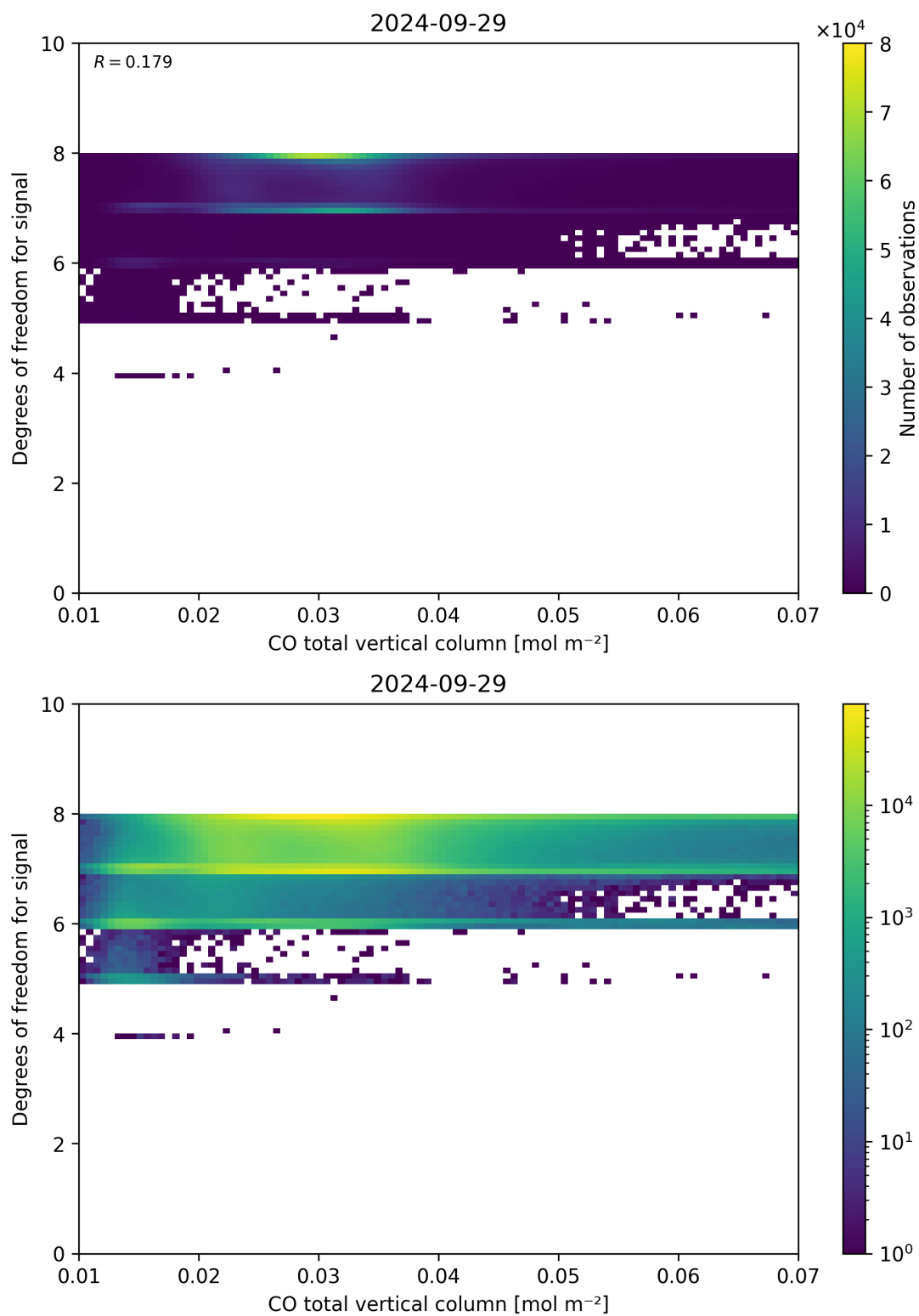
Figure 41: Scatter density plot of “CO total vertical column” against “Degrees of freedom for signal” for 2024-09-28 to 2024-09-30.
