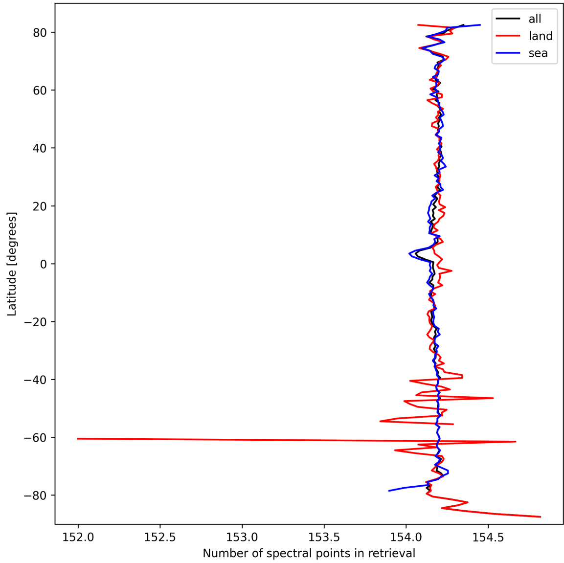
Figure 13: Zonal average of “Number of spectral points in retrieval” for 2024-09-28 to 2024-09-30.
