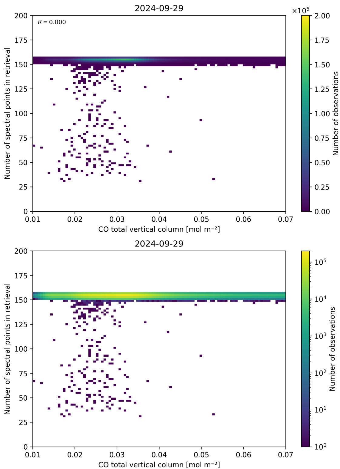
Figure 43: Scatter density plot of “CO total vertical column” against “Number of spectral points in retrieval” for 2024-09-28 to 2024-09-30.
