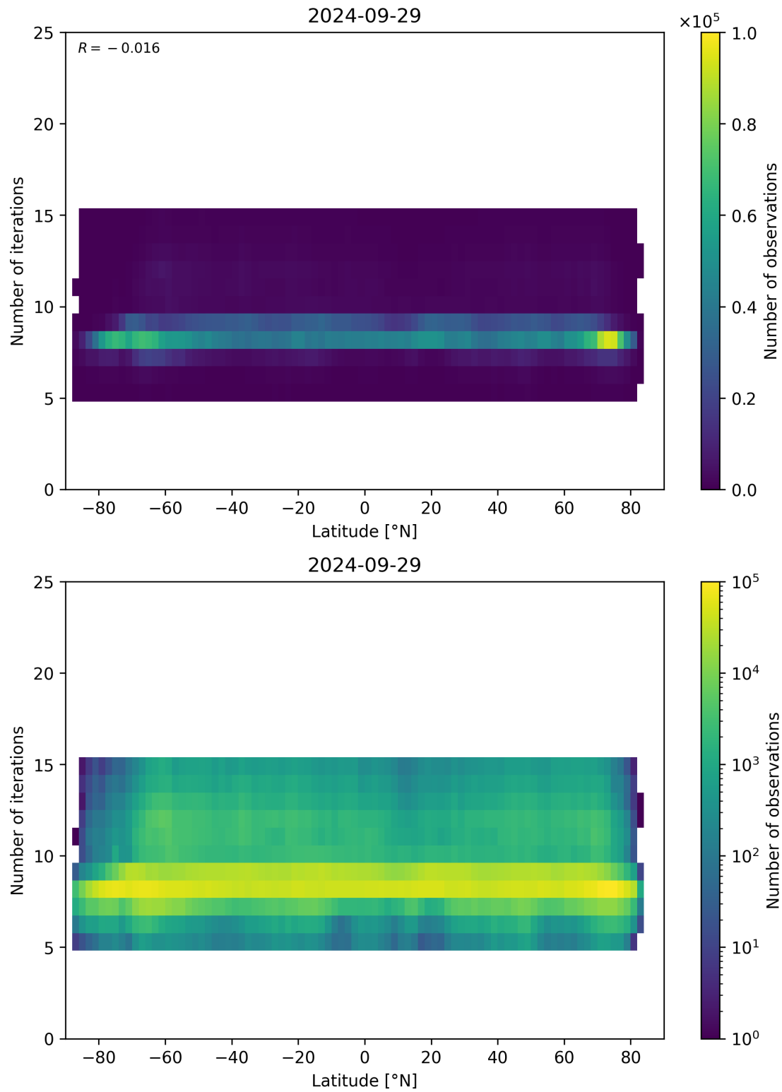
Figure 56: Scatter density plot of “Latitude” against “Number of iterations” for 2024-09-28 to 2024-09-30.
