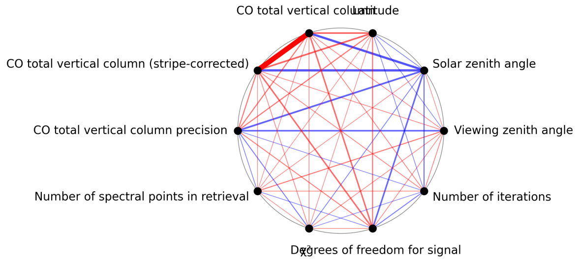
Figure 1: Map of correlation graph for 2024-09-28 to 2024-09-30.
