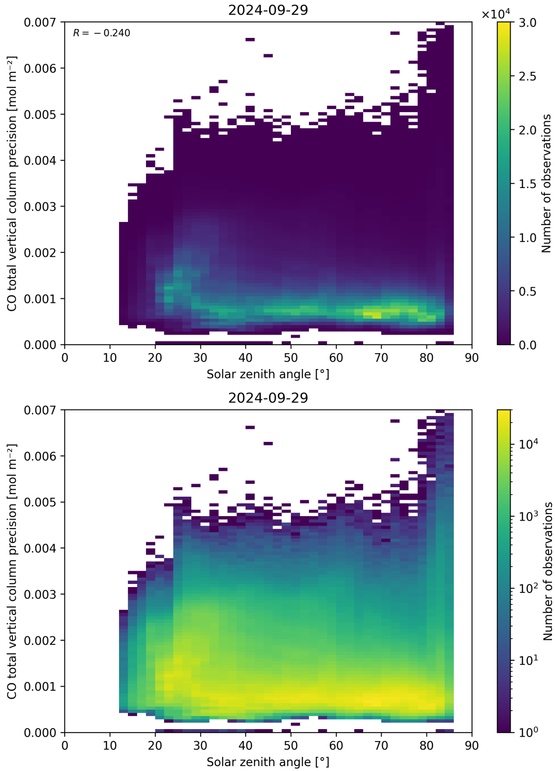
Figure 63: Scatter density plot of “Solar zenith angle” against “CO total vertical column precision” for 2024-09-28 to 2024-09-30.
