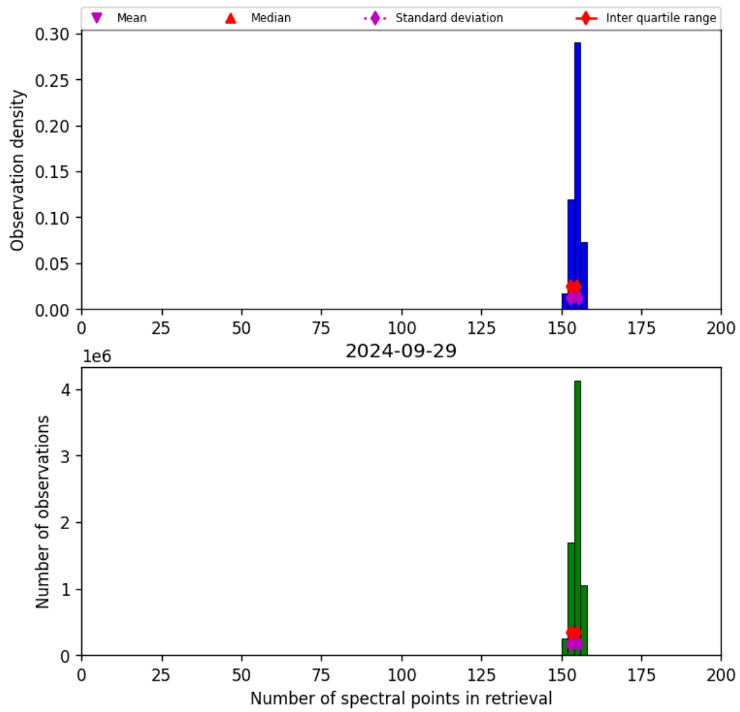
Figure 21: Histogram of “Number of spectral points in retrieval” for 2024-09-28 to 2024-09-30
