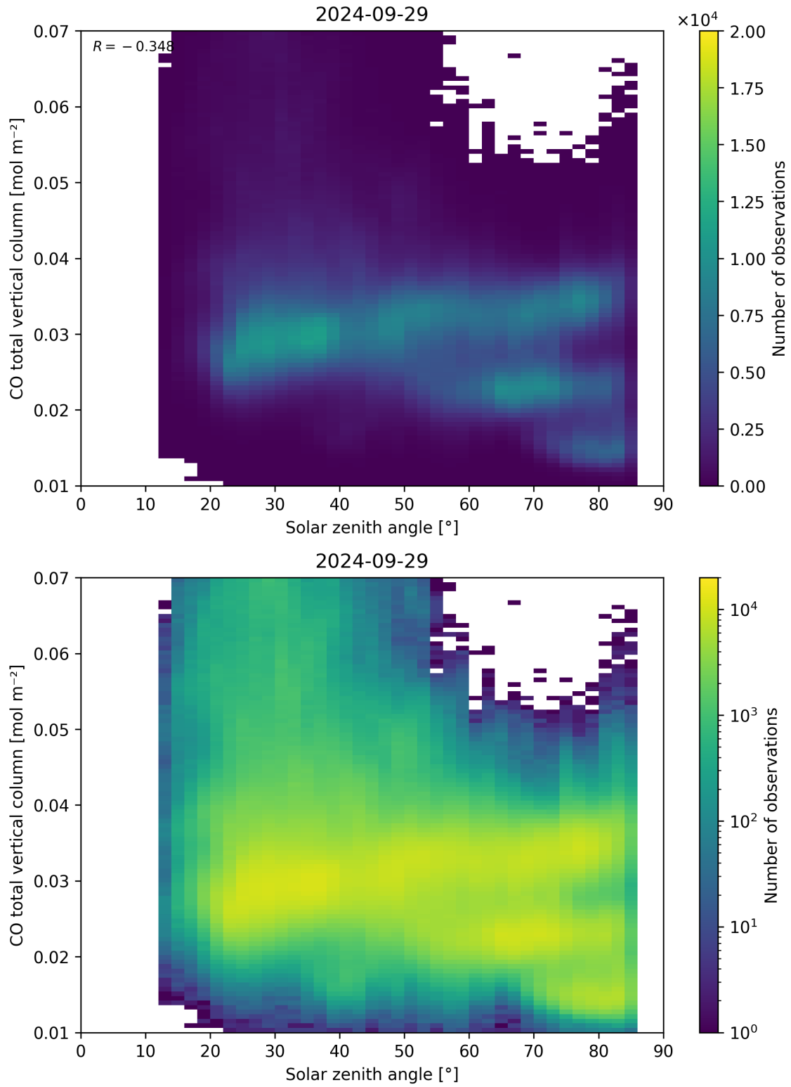
Figure 61: Scatter density plot of “Solar zenith angle” against “CO total vertical column” for 2024-09-28 to 2024-09-30.
