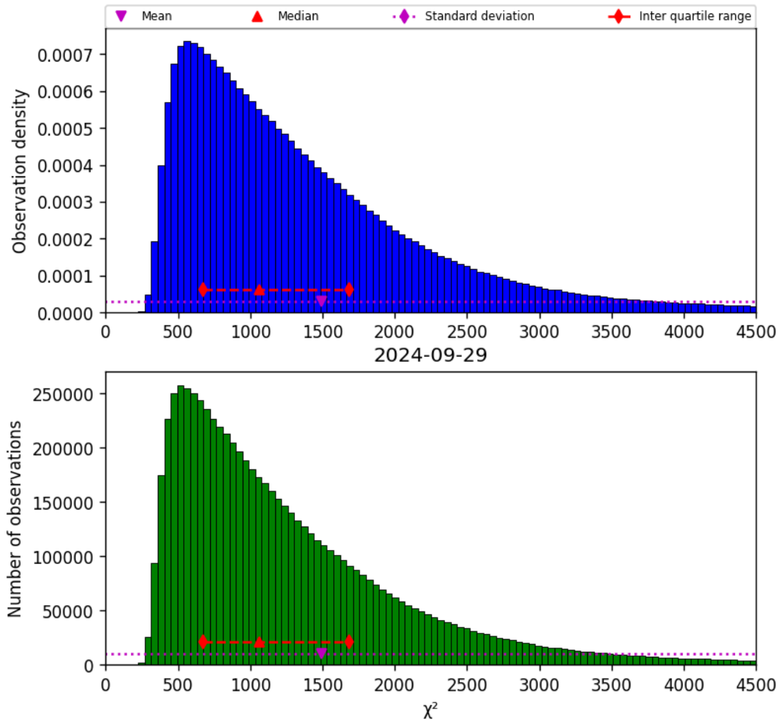
Figure 22: Histogram of " \chi^2 " for 2024-09-28 to 2024-09-30
