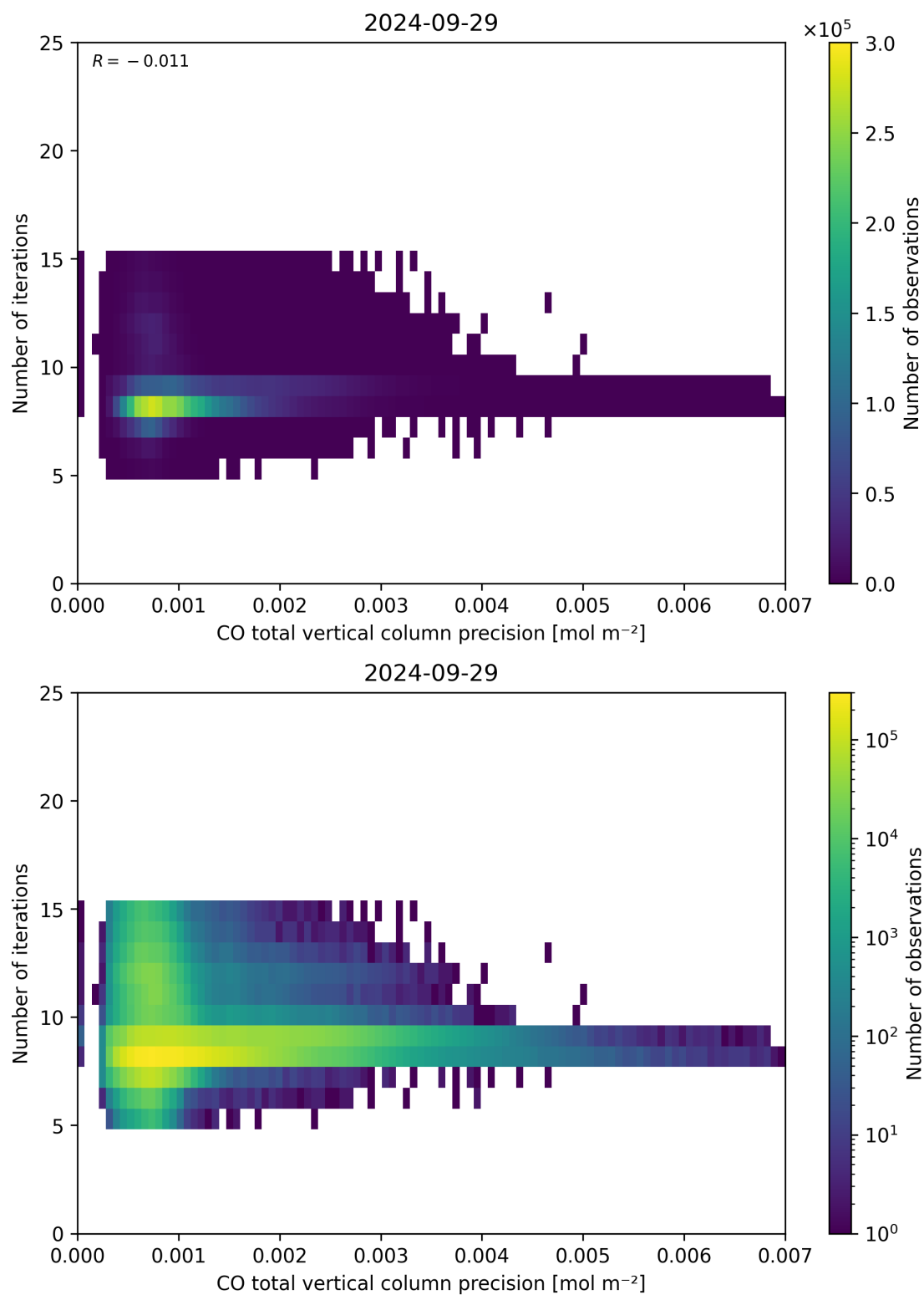
Figure 46: Scatter density plot of “CO total vertical column precision” against “Number of iterations” for 2024-09-28 to 2024-09-30.
