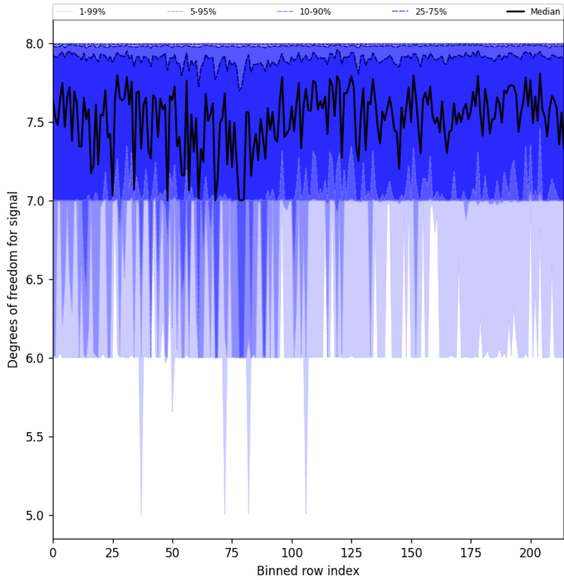
Figure 31: Along track statistics of “Degrees of freedom for signal” for 2024-09-28 to 2024-09-30
