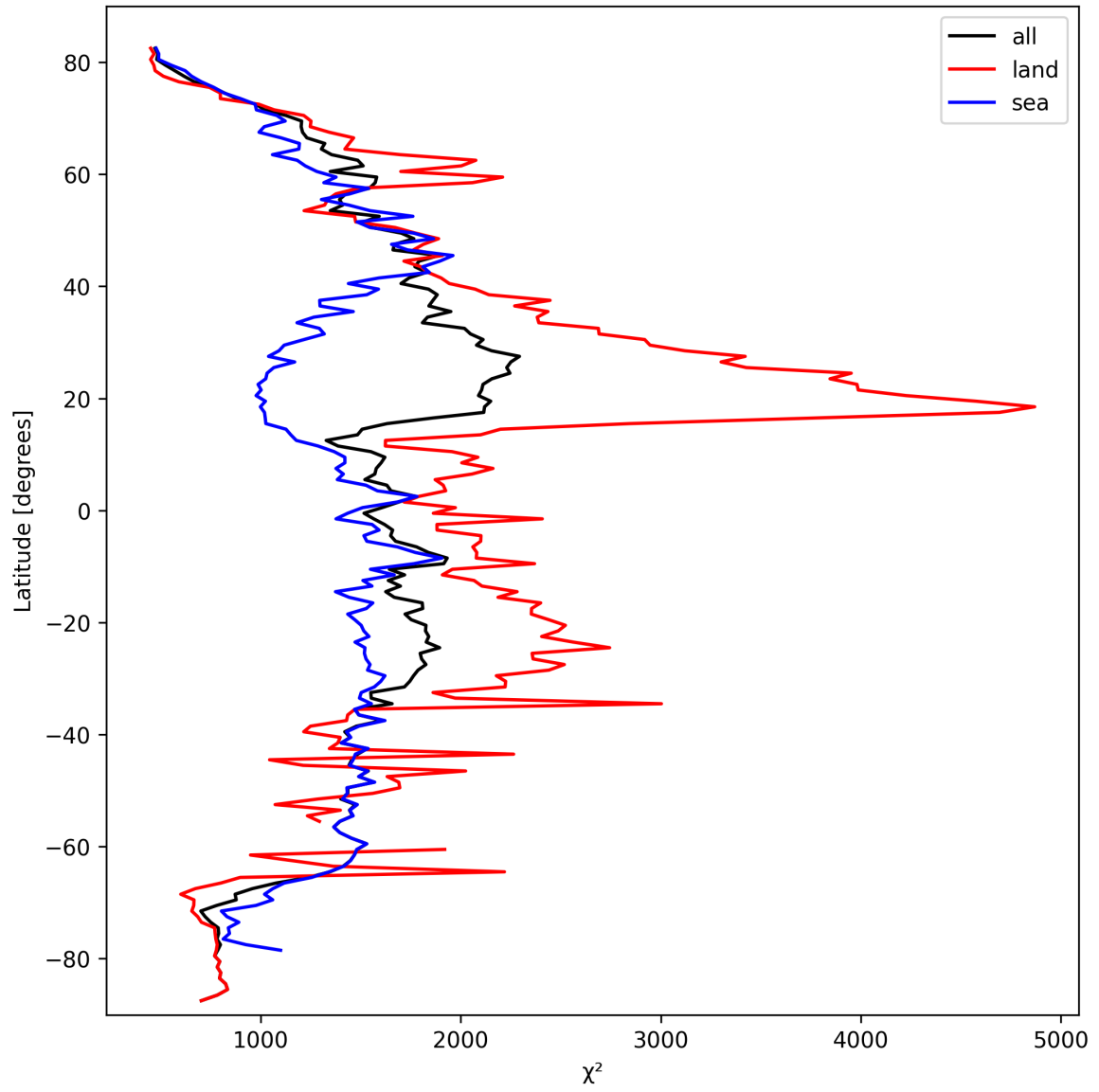
Figure 14: Zonal average of “ \chi^2 ” for 2024-09-28 to 2024-09-30.
