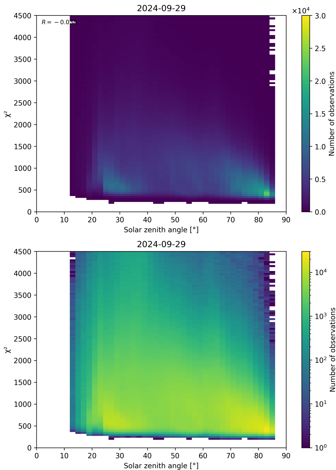
Figure 64: Scatter density plot of “Solar zenith angle” against “ \chi^2 ” for 2024-09-28 to 2024-09-30.
