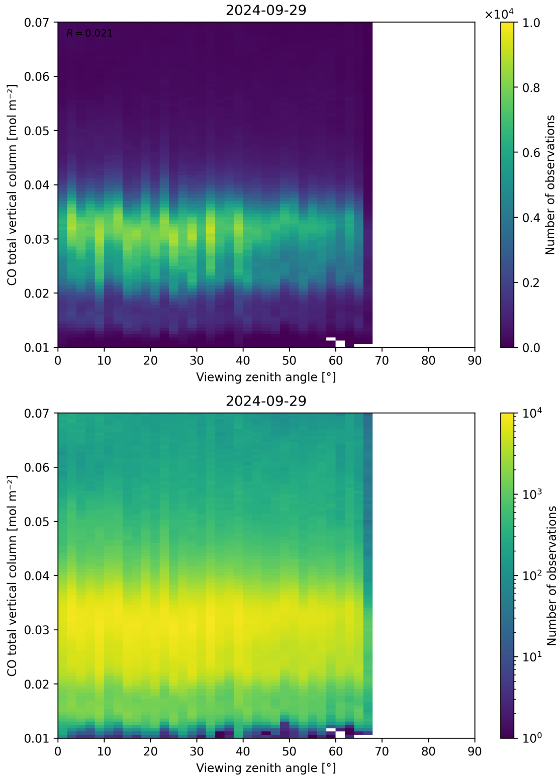
Figure 69: Scatter density plot of “Viewing zenith angle” against “CO total vertical column” for 2024-09-28 to 2024-09-30.
