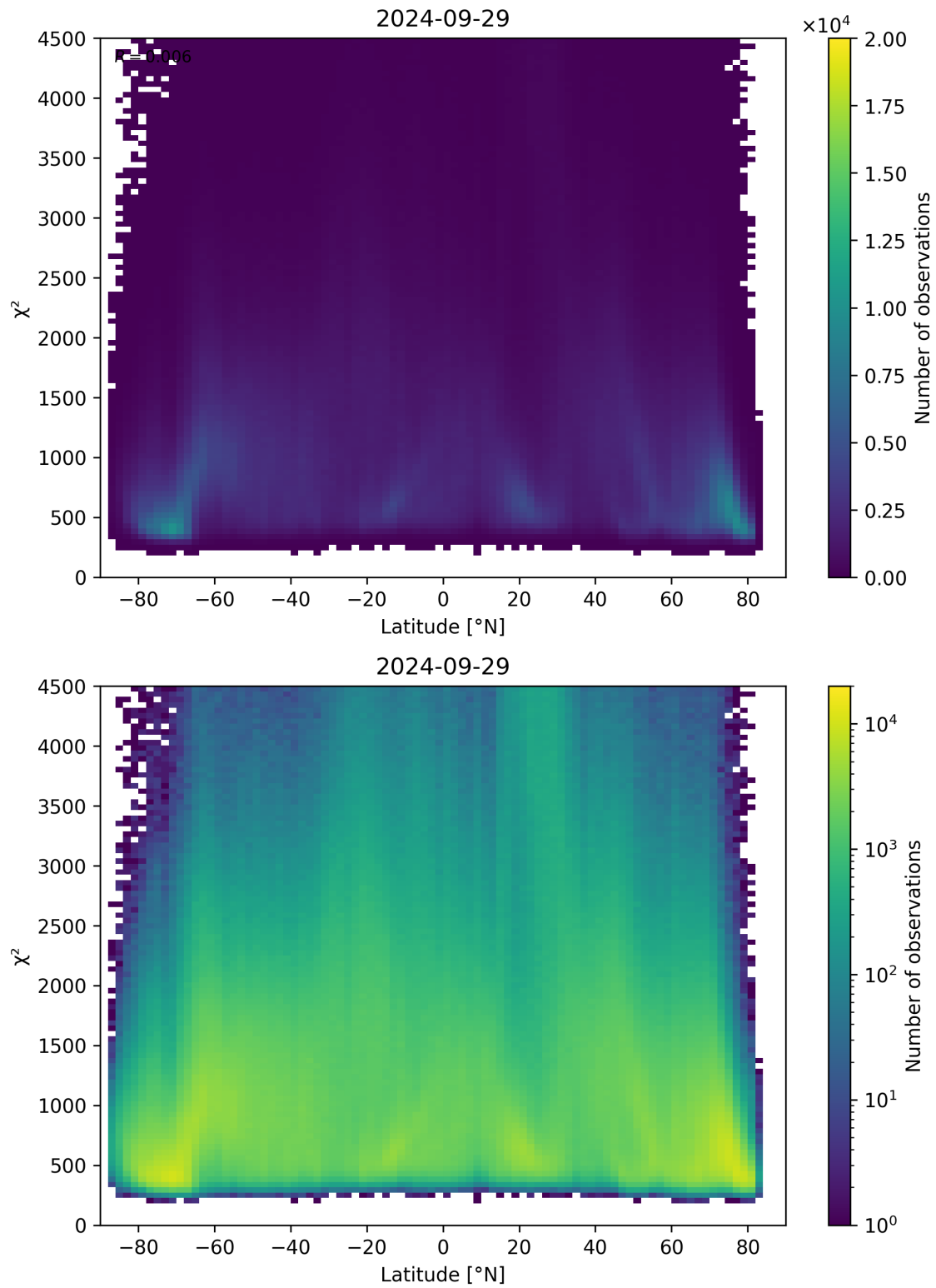
Figure 54: Scatter density plot of “Latitude” against “ \chi^2 ” for 2024-09-28 to 2024-09-30.
