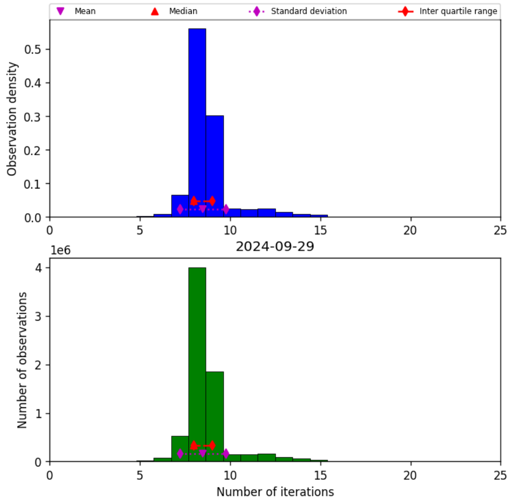
Figure 24: Histogram of “Number of iterations” for 2024-09-28 to 2024-09-30
