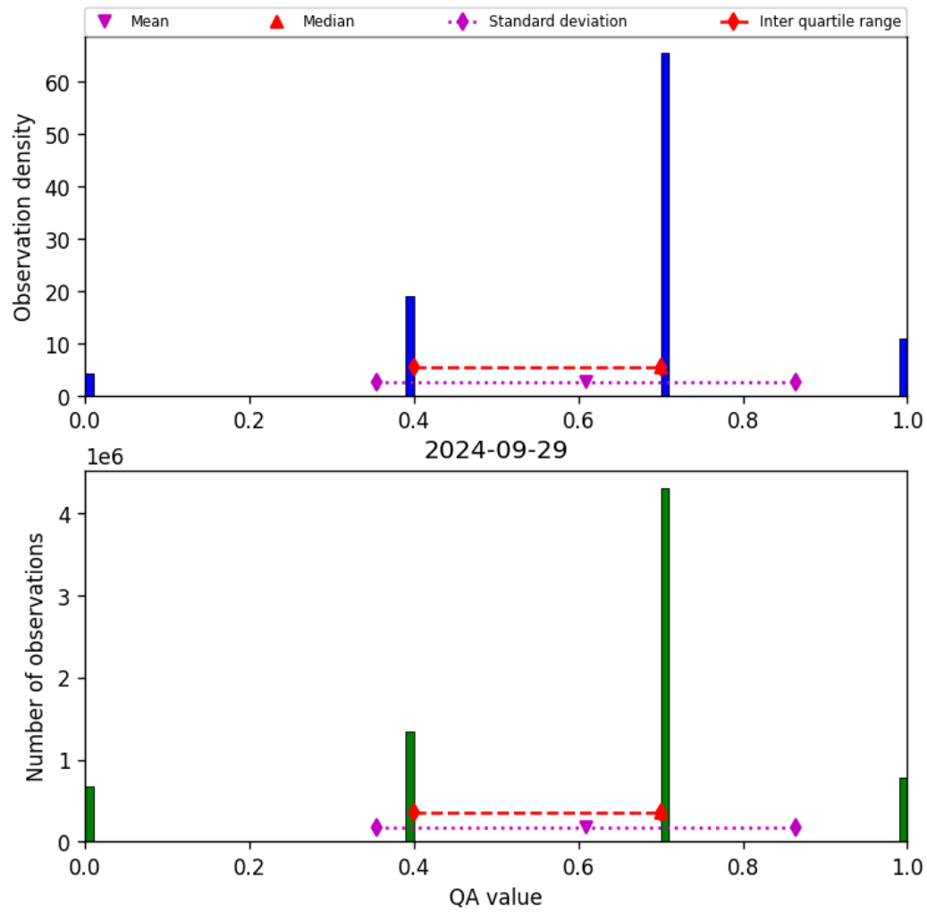
Figure 17: Histogram of “QA value” for 2024-09-28 to 2024-09-30
