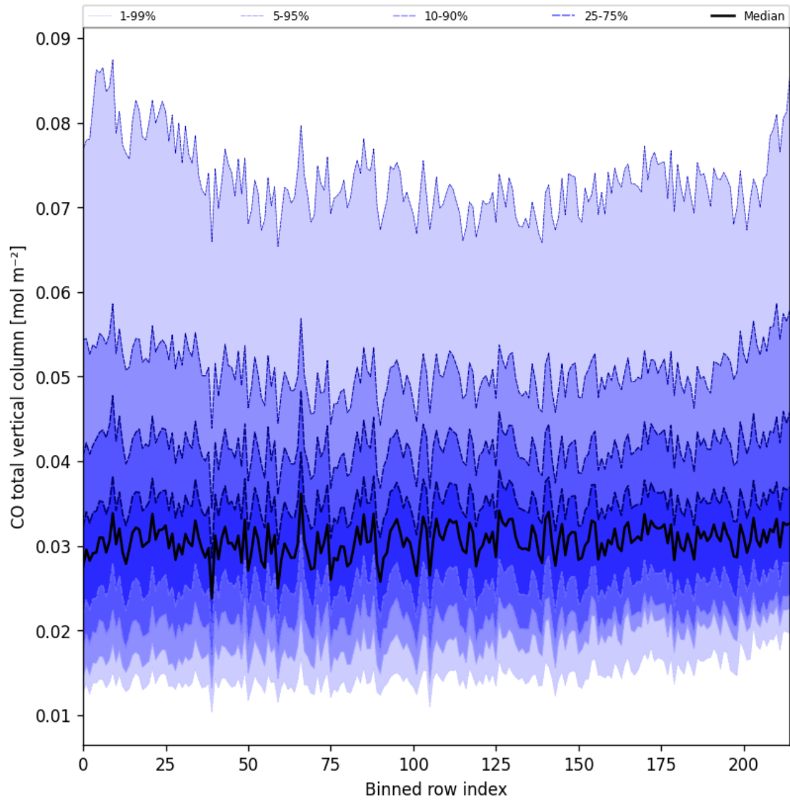
Figure 26: Along track statistics of “CO total vertical column” for 2024-09-28 to 2024-09-30
