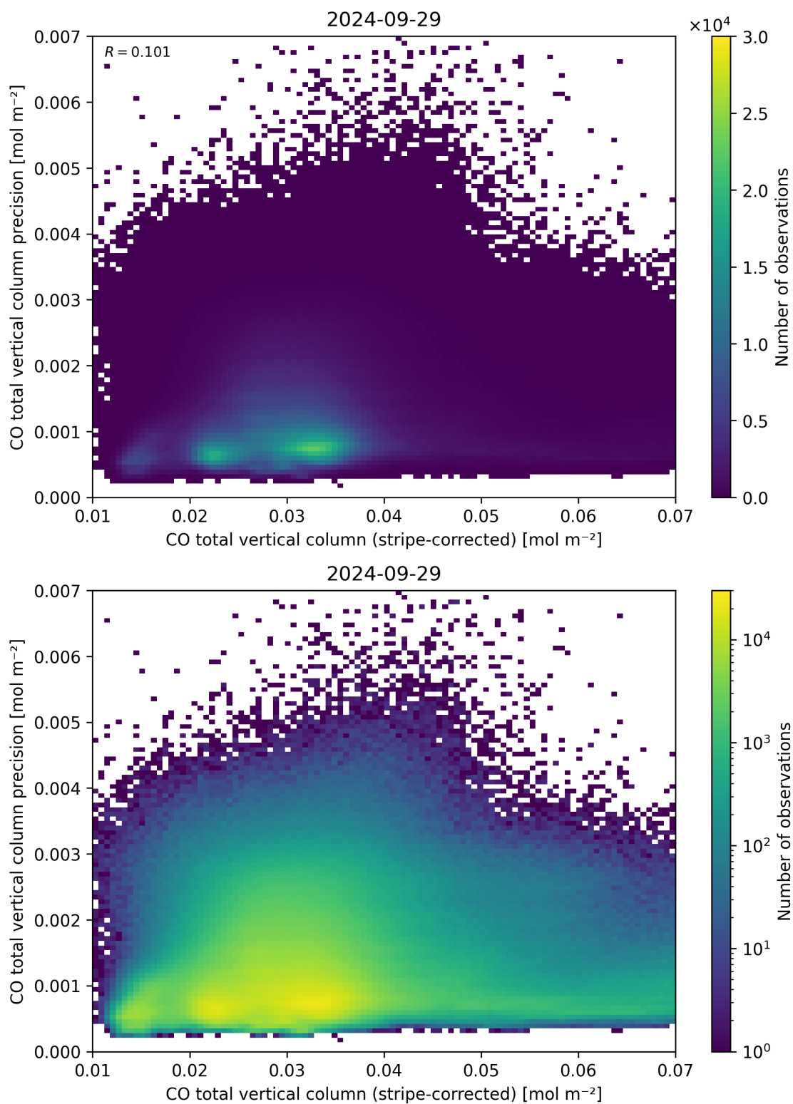
Figure 36: Scatter density plot of “CO total vertical column (stripe-corrected)” against “CO total vertical column precision” for 2024-09-28 to 2024-09-30.
