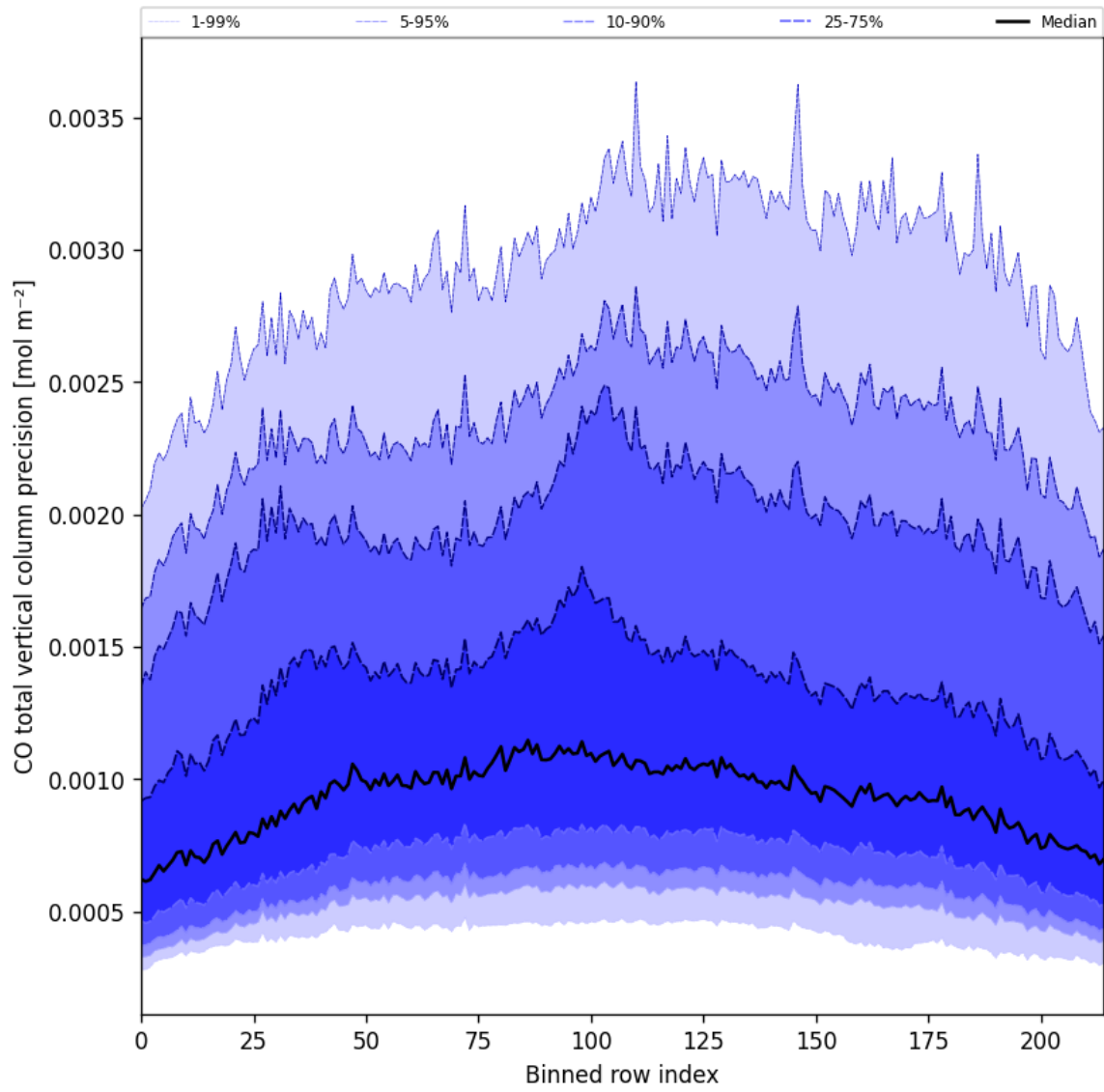
Figure 28: Along track statistics of “CO total vertical column precision” for 2024-09-28 to 2024-09-30
