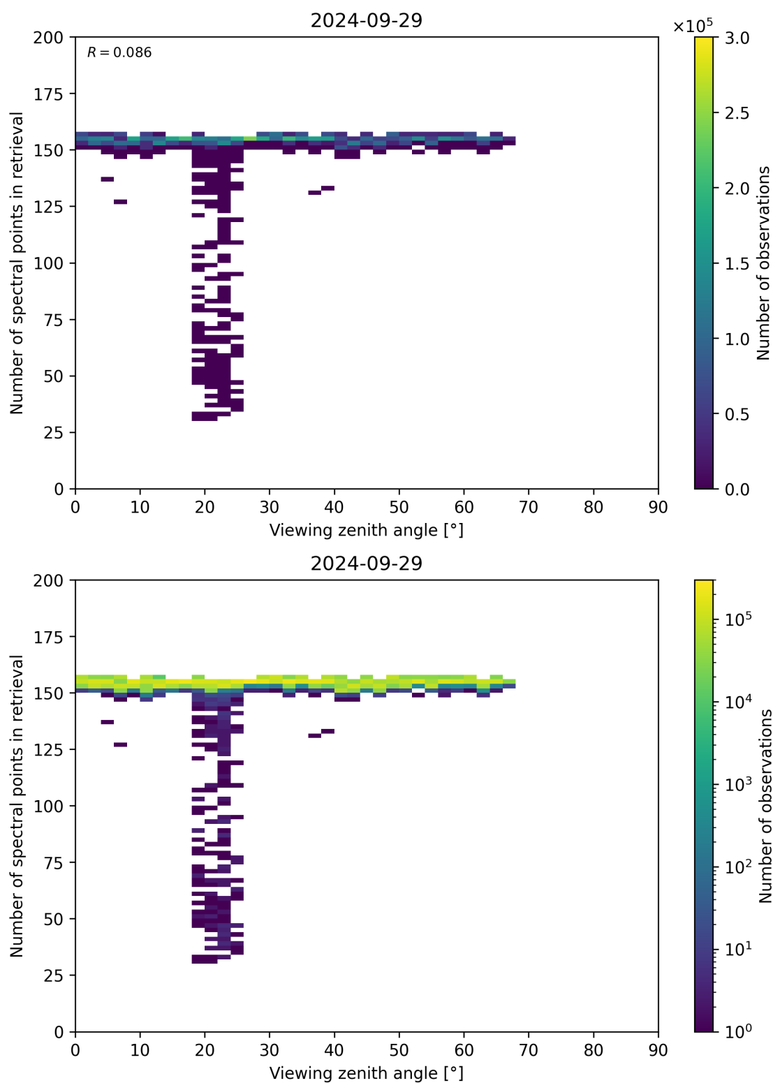
Figure 76: Scatter density plot of “Viewing zenith angle” against “Number of spectral points in retrieval” for 2024-09-28 to 2024-09-30.
