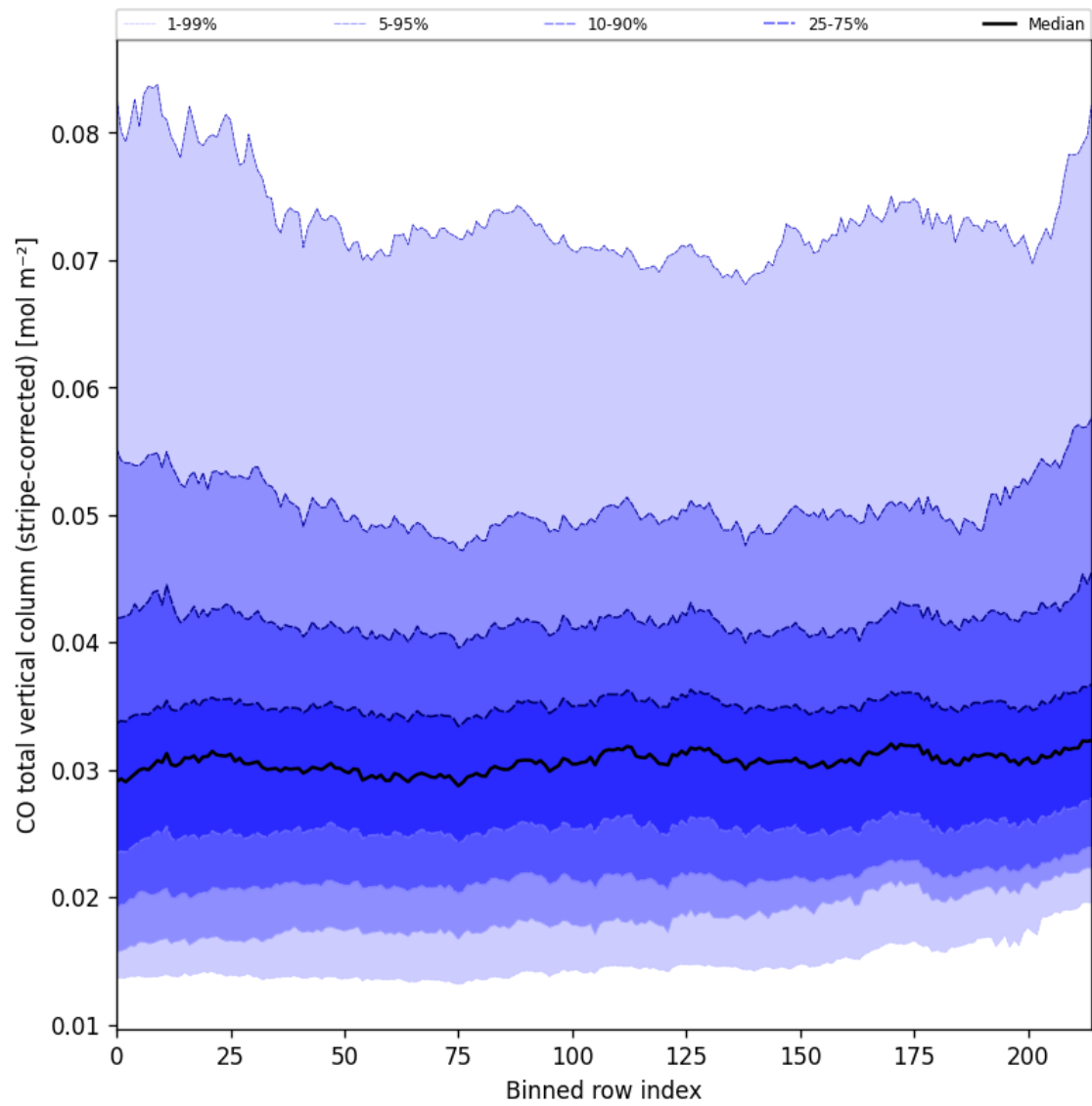
Figure 27: Along track statistics of “CO total vertical column (stripe-corrected)” for 2024-09-28 to 2024-09-30
