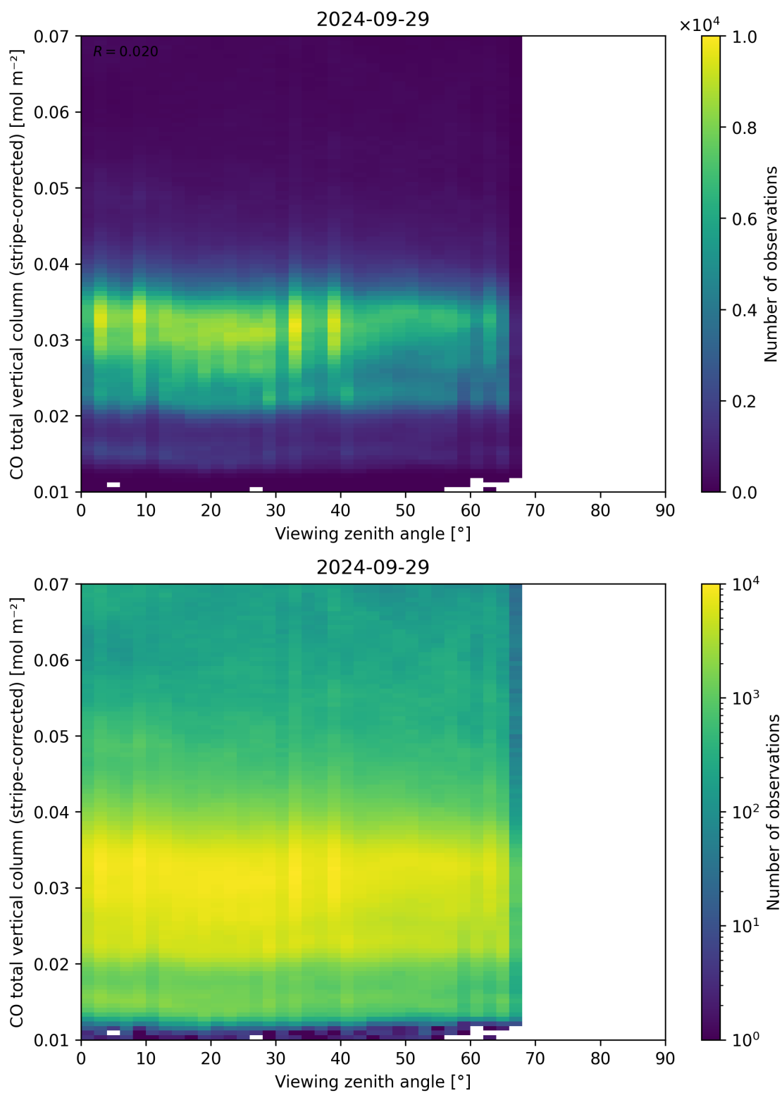
Figure 70: Scatter density plot of “Viewing zenith angle” against “CO total vertical column (stripe-corrected)” for 2024-09-28 to 2024-09-30.
