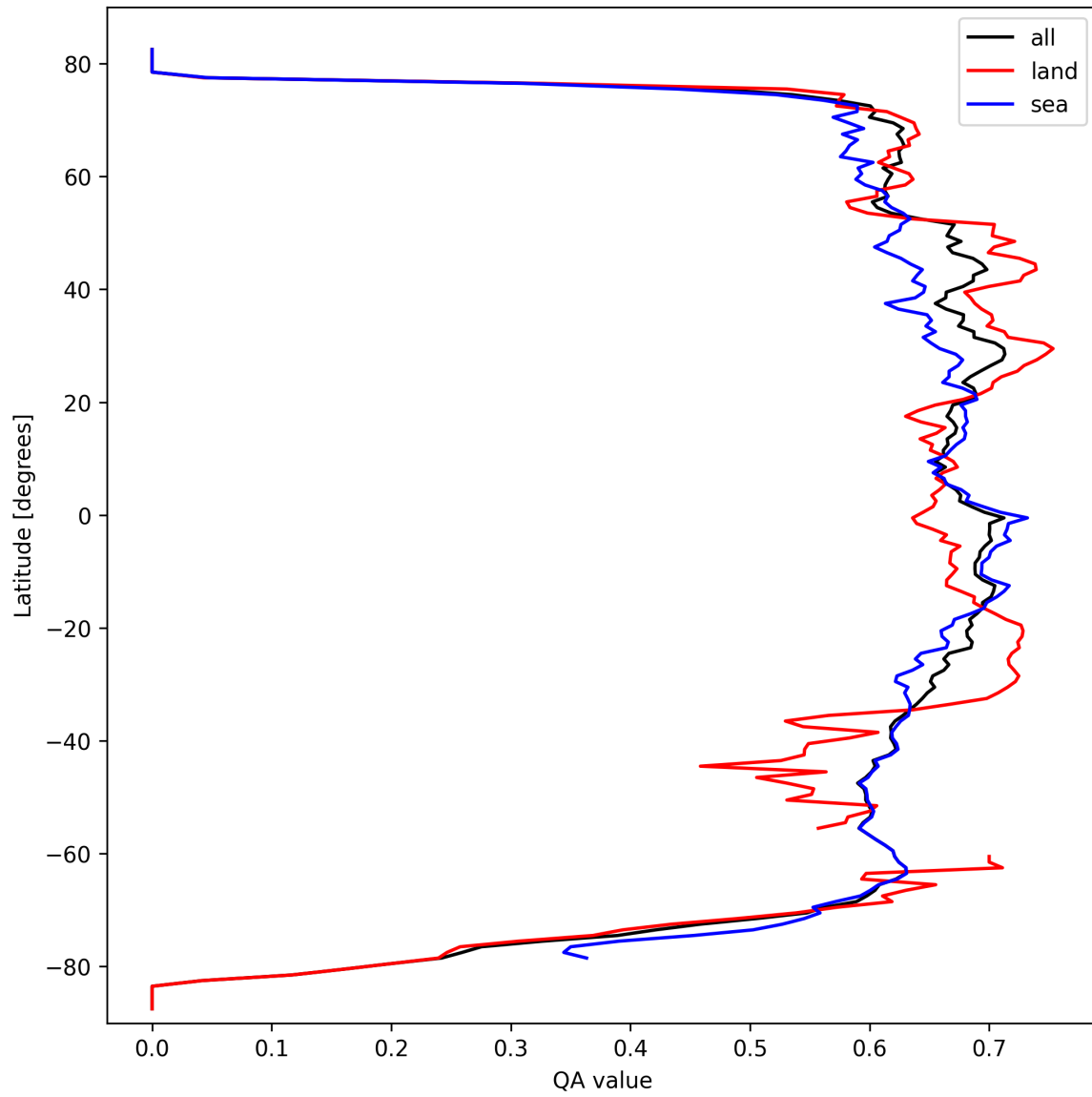
Figure 9: Zonal average of “QA value” for 2024-09-28 to 2024-09-30.
