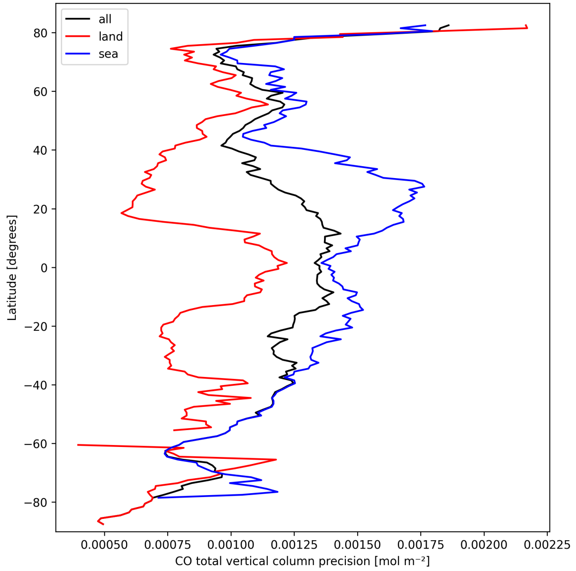
Figure 12: Zonal average of “CO total vertical column precision” for 2024-09-28 to 2024-09-30.
