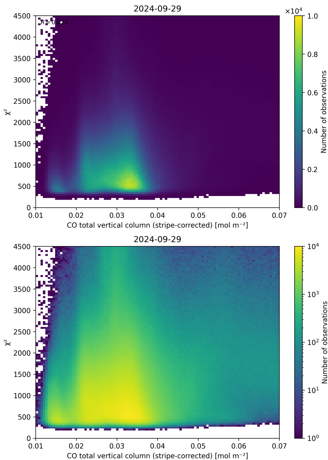
Figure 37: Scatter density plot of “CO total vertical column (stripe-corrected)” against “ \chi^2 ” for 2024-09-28 to 2024-09-30.
