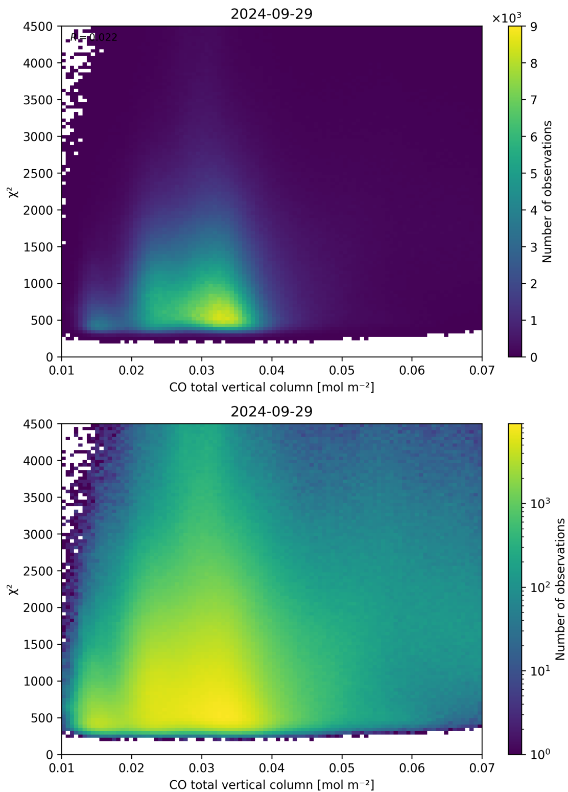
Figure 35: Scatter density plot of “CO total vertical column” against “ \chi^2 ” for 2024-09-28 to 2024-09-30.
