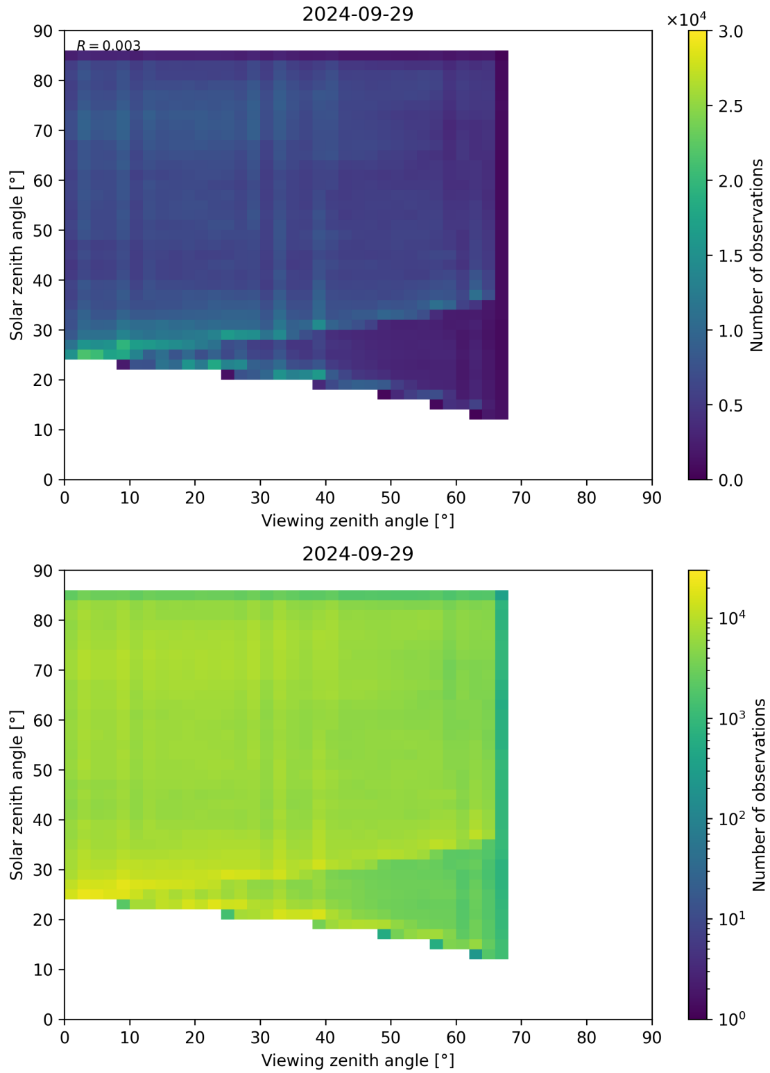
Figure 77: Scatter density plot of “Viewing zenith angle” against “Solar zenith angle” for 2024-09-28 to 2024-09-30.
