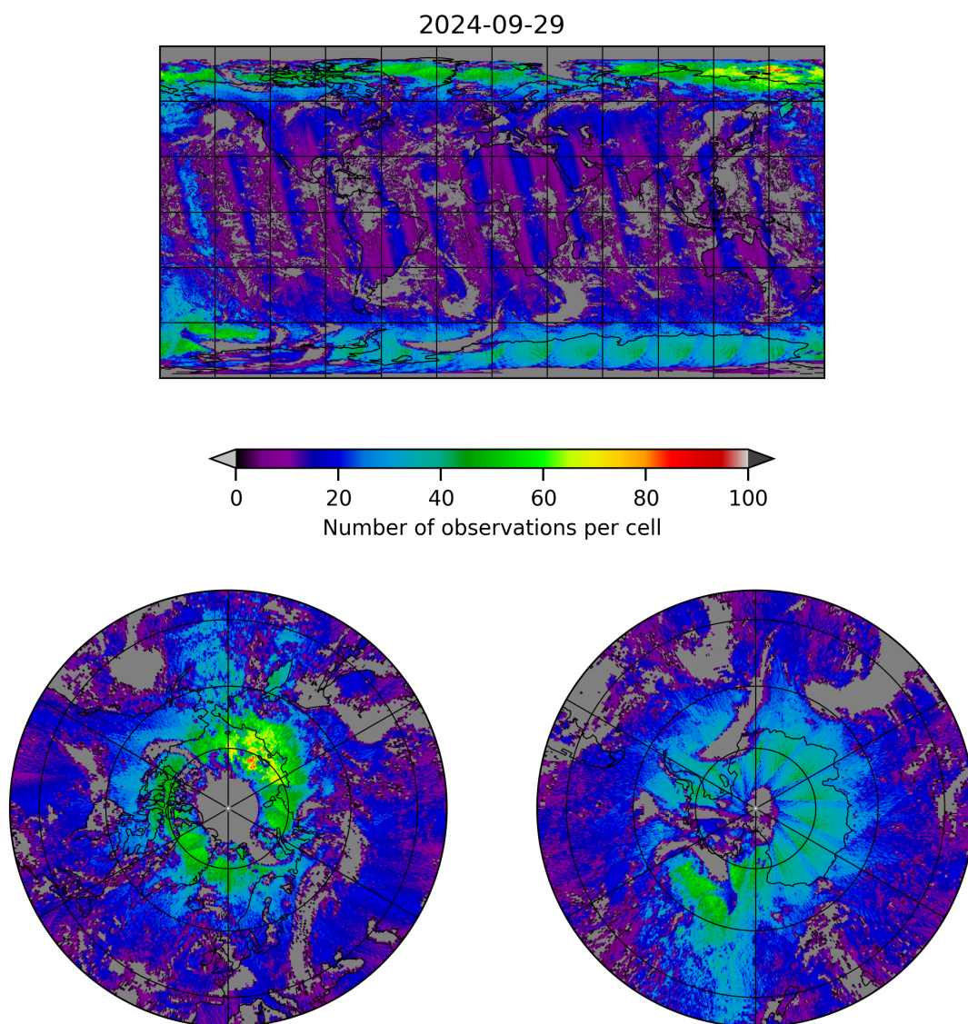
Figure 8: Map of the number of observations for 2024-09-28 to 2024-09-30
