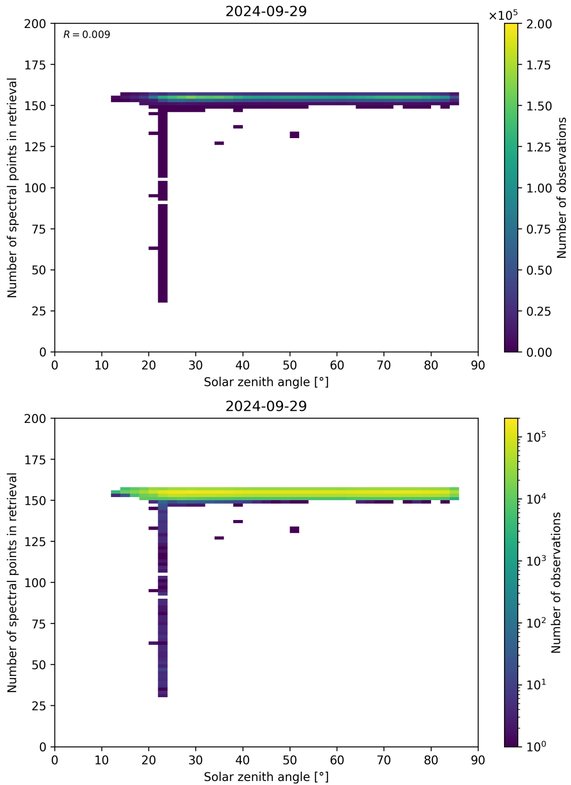
Figure 68: Scatter density plot of “Solar zenith angle” against “Number of spectral points in retrieval” for 2024-09-28 to 2024-09-30.
