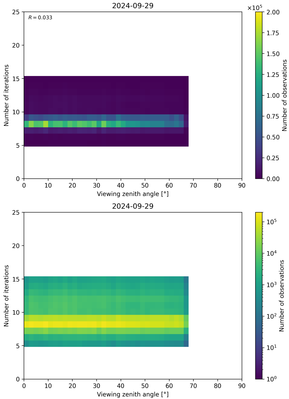
Figure 75: Scatter density plot of “Viewing zenith angle” against “Number of iterations” for 2024-09-28 to 2024-09-30.
