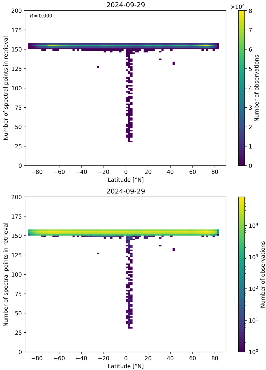
Figure 57: Scatter density plot of “Latitude” against “Number of spectral points in retrieval” for 2024-09-28 to 2024-09-30.
