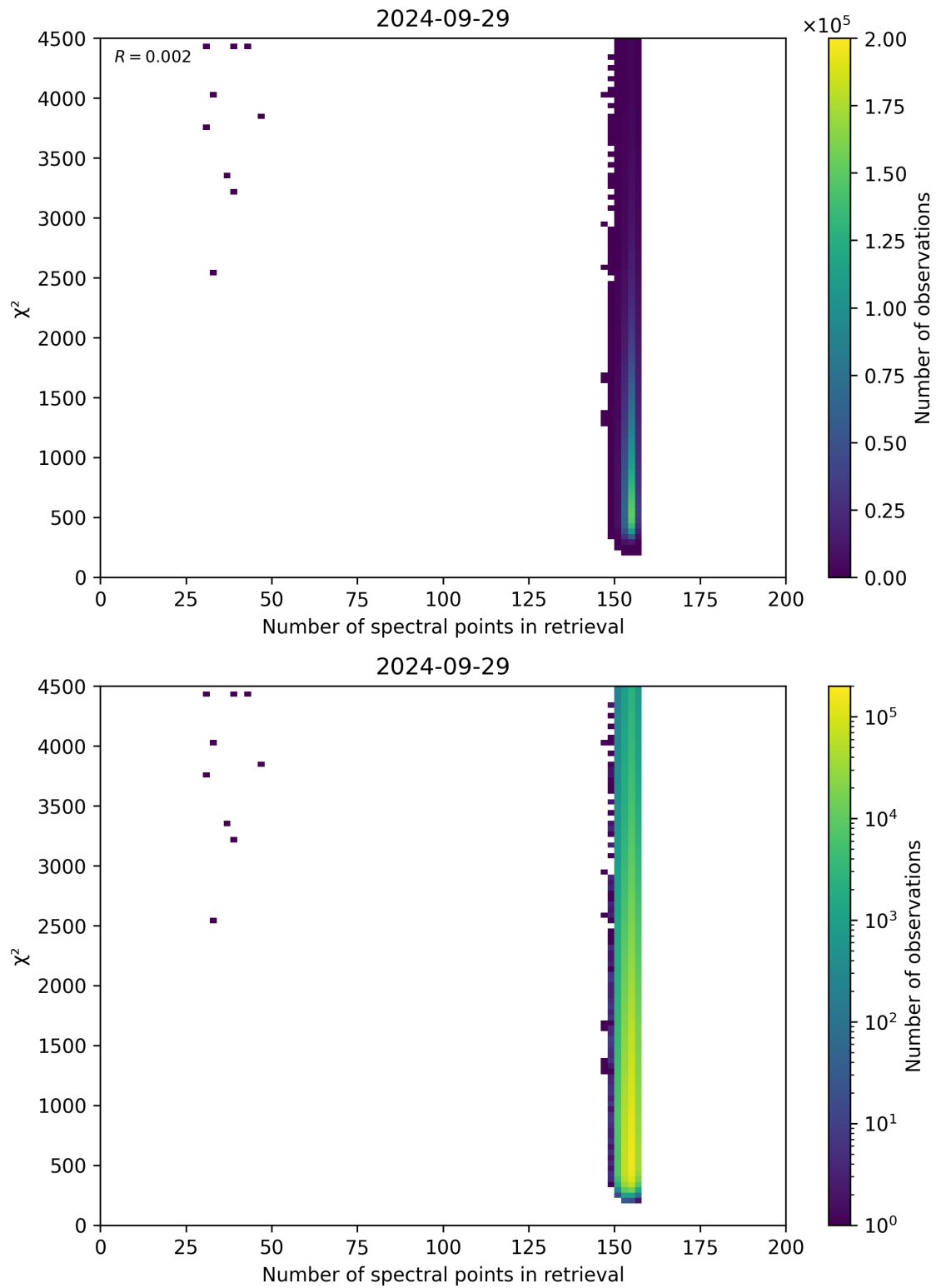
Figure 58: Scatter density plot of “Number of spectral points in retrieval” against “ \chi^2 ” for 2024-09-28 to 2024-09-30.
