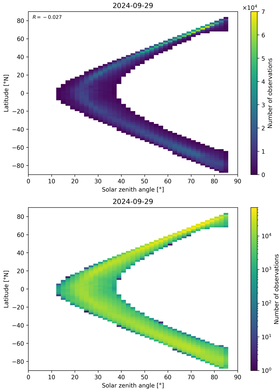
Figure 66: Scatter density plot of “Solar zenith angle” against “Latitude” for 2024-09-28 to 2024-09-30.
