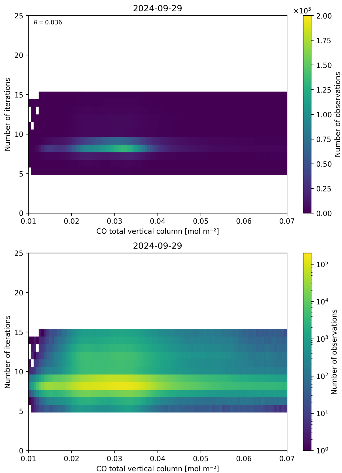
Figure 42: Scatter density plot of “CO total vertical column” against “Number of iterations” for 2024-09-28 to 2024-09-30.
