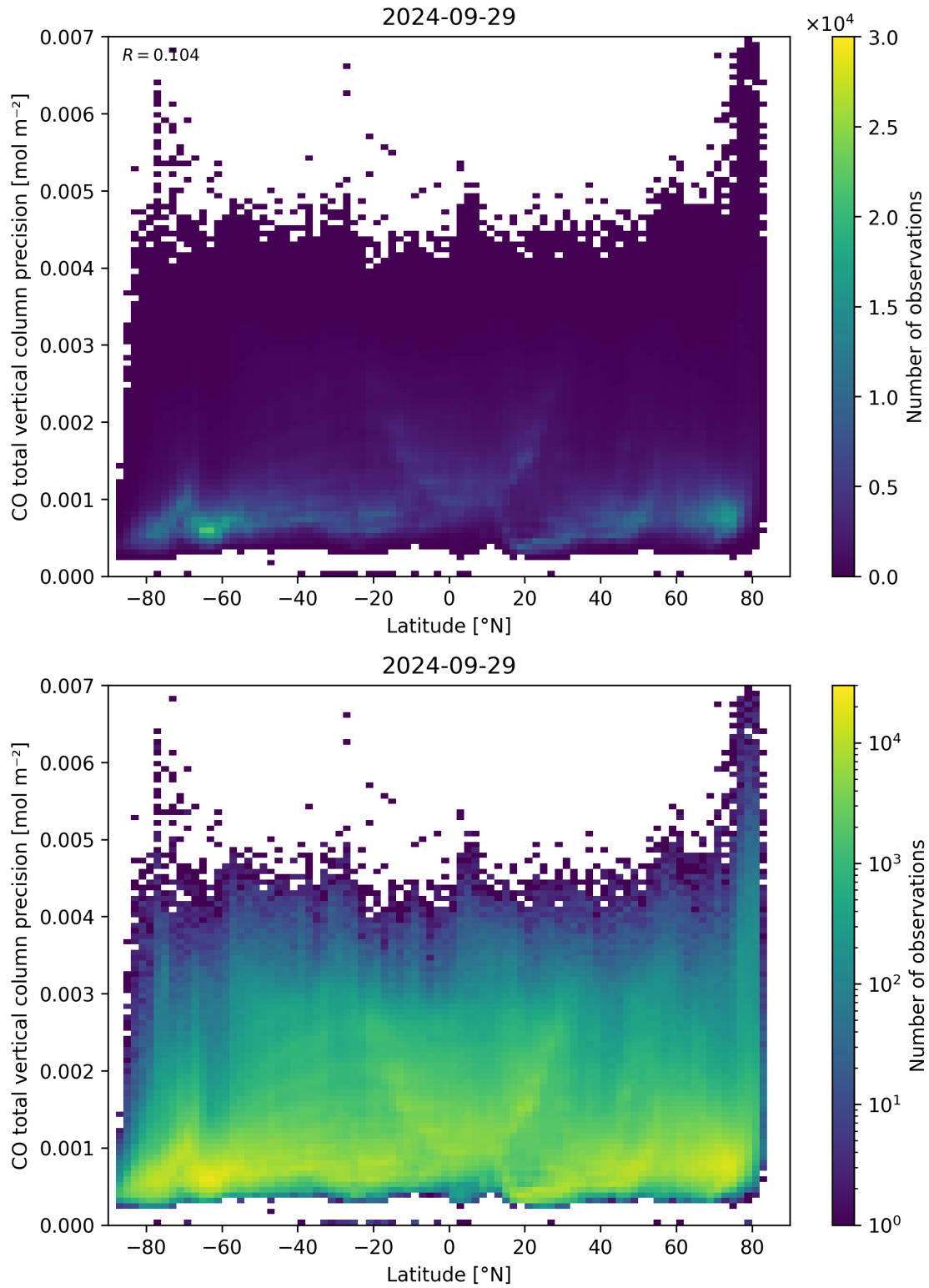
Figure 53: Scatter density plot of “Latitude” against “CO total vertical column precision” for 2024-09-28 to 2024-09-30.
