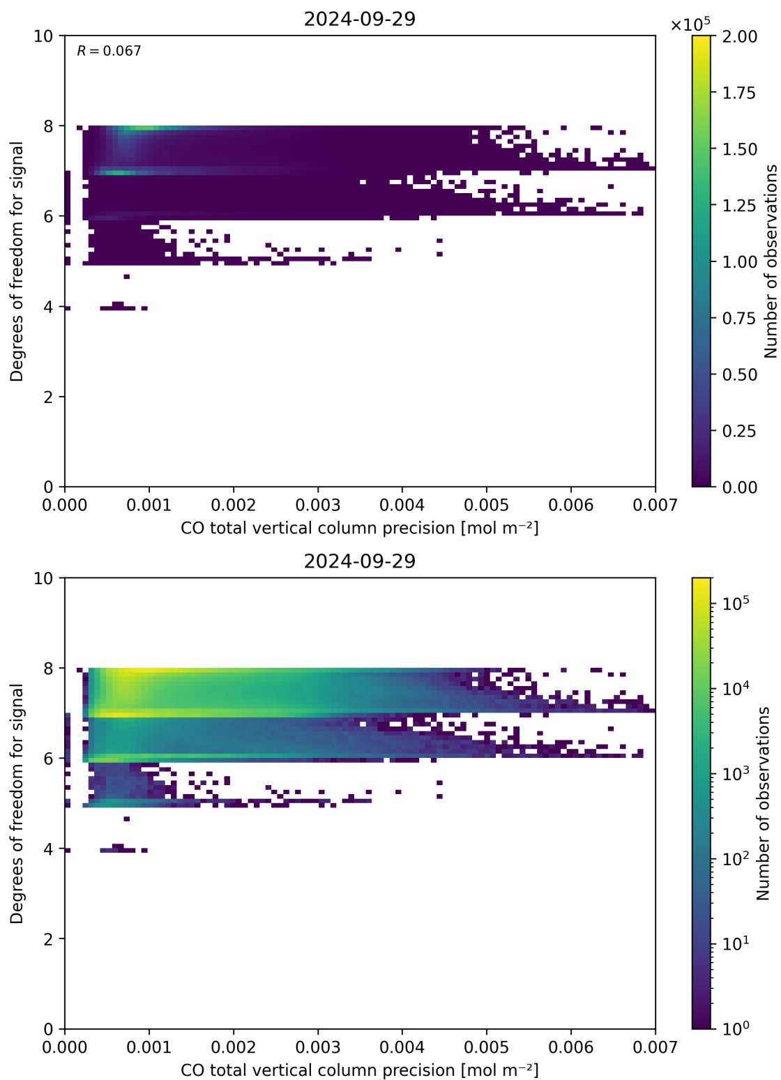
Figure 45: Scatter density plot of “CO total vertical column precision” against “Degrees of freedom for signal” for 2024-09-28 to 2024-09-30.
