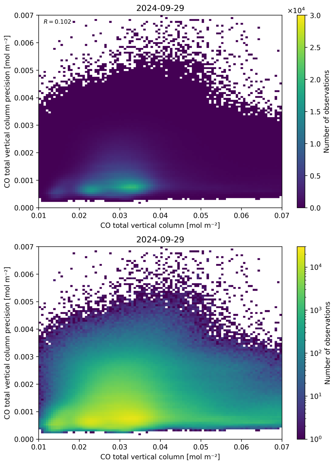
Figure 34: Scatter density plot of “CO total vertical column” against “CO total vertical column precision” for 2024-09-28 to 2024-09-30.
