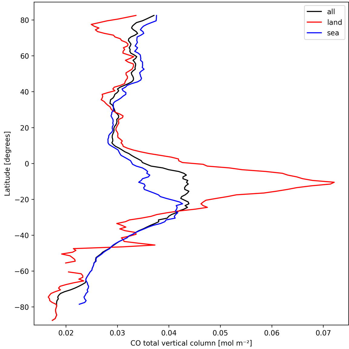
Figure 10: Zonal average of “CO total vertical column” for 2024-09-28 to 2024-09-30.
