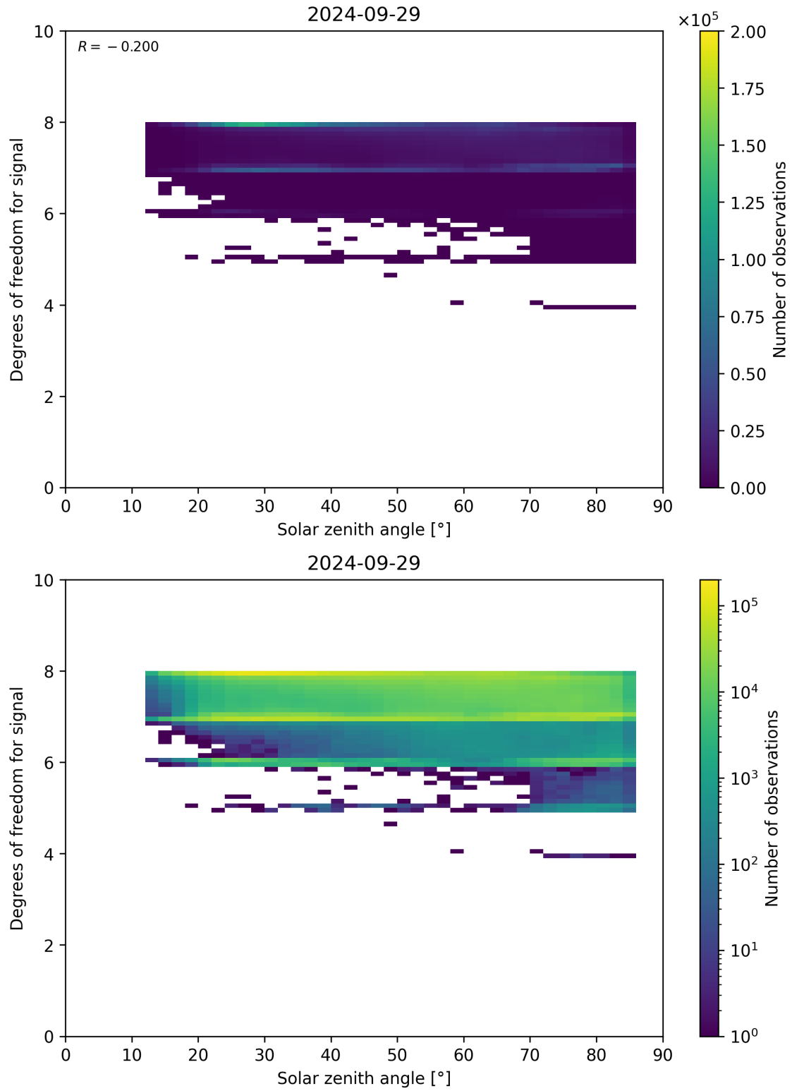
Figure 65: Scatter density plot of “Solar zenith angle” against “Degrees of freedom for signal” for 2024-09-28 to 2024-09-30.
