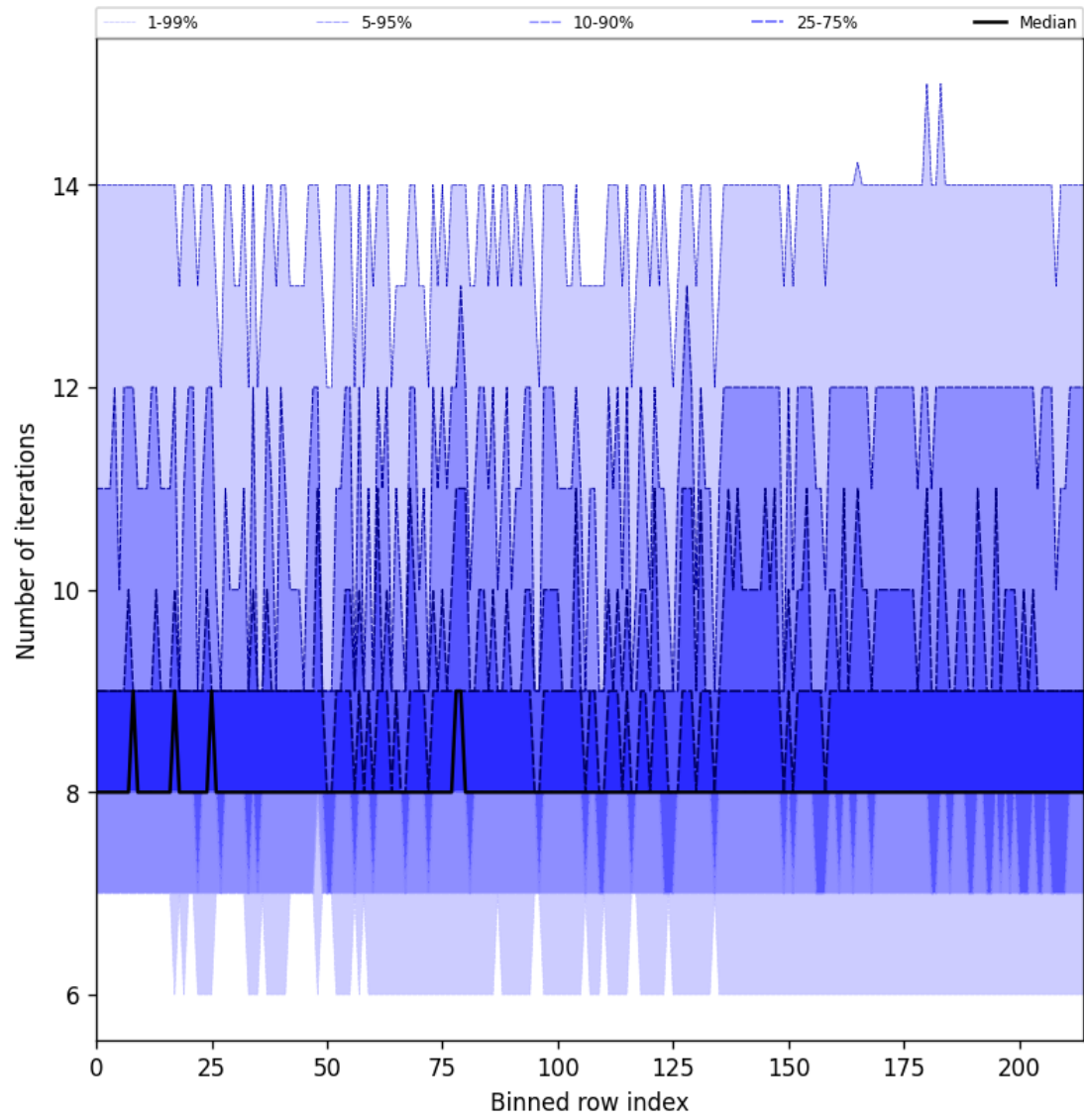
Figure 32: Along track statistics of “Number of iterations” for 2024-09-28 to 2024-09-30
