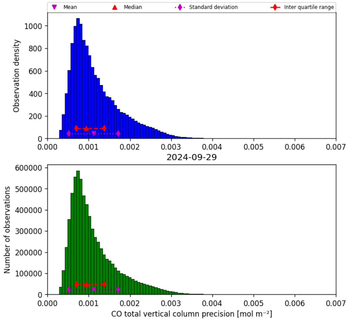
Figure 20: Histogram of “CO total vertical column precision” for 2024-09-28 to 2024-09-30
