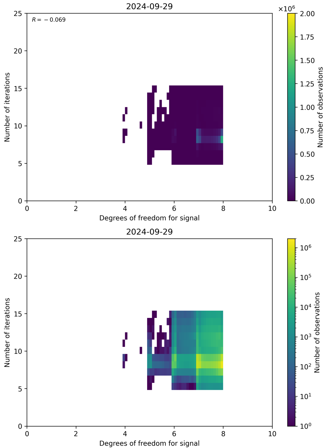
Figure 50: Scatter density plot of “Degrees of freedom for signal” against “Number of iterations” for 2024-09-28 to 2024-09-30.
