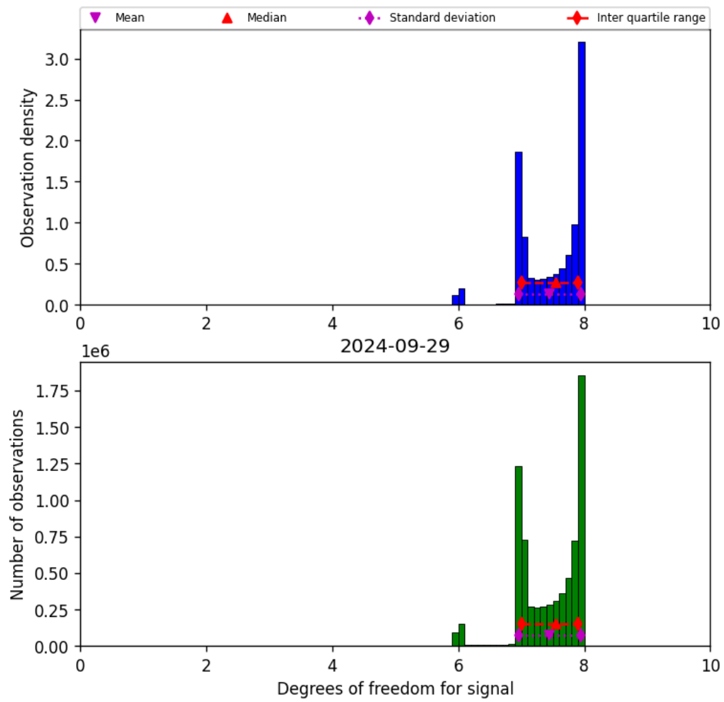
Figure 23: Histogram of “Degrees of freedom for signal” for 2024-09-28 to 2024-09-30
