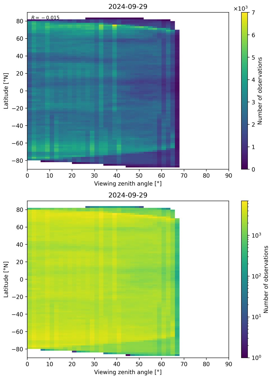
Figure 74: Scatter density plot of “Viewing zenith angle” against “Latitude” for 2024-09-28 to 2024-09-30.
