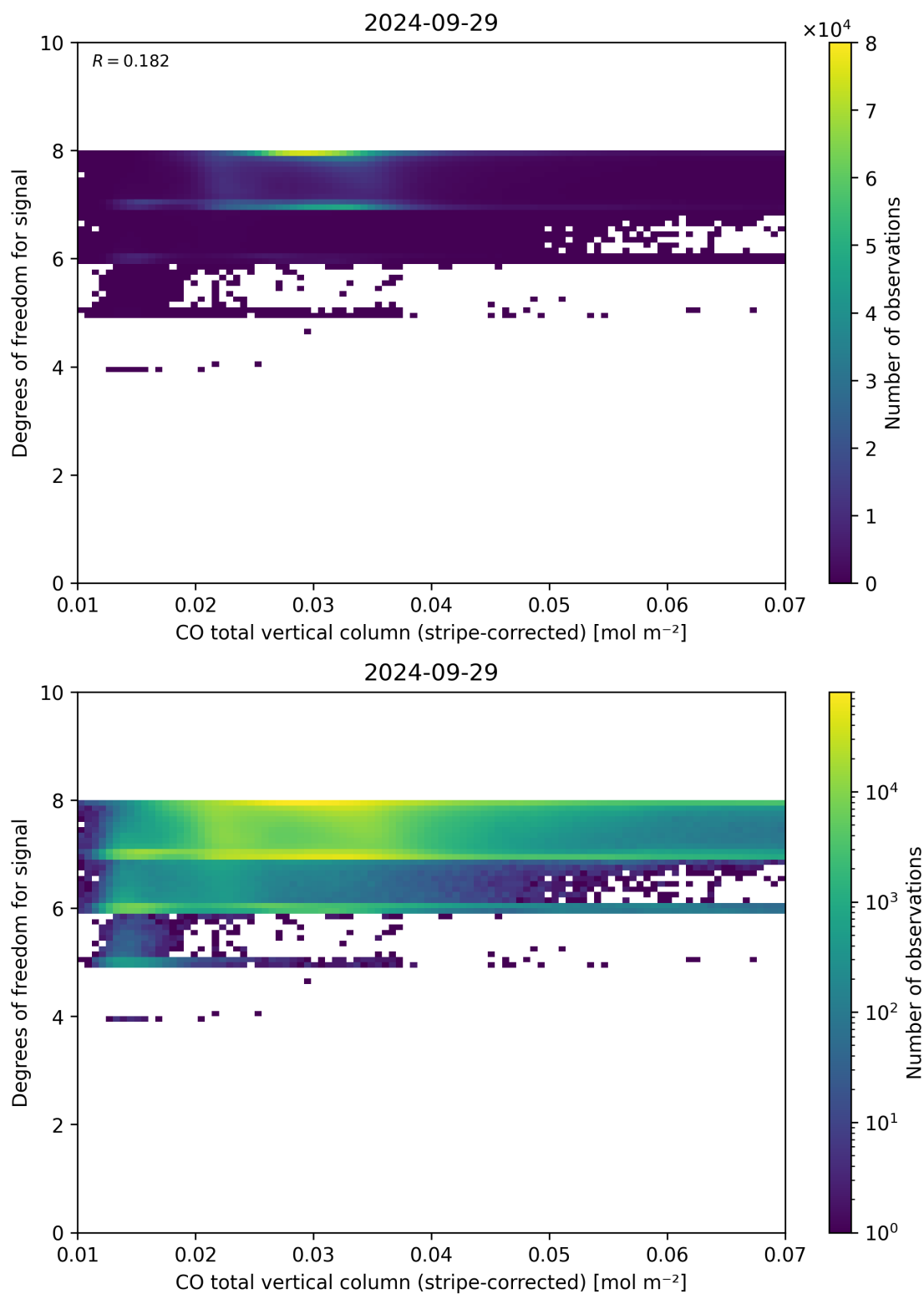
Figure 38: Scatter density plot of “CO total vertical column (stripe-corrected)” against “Degrees of freedom for signal” for 2024-09-28 to 2024-09-30.
