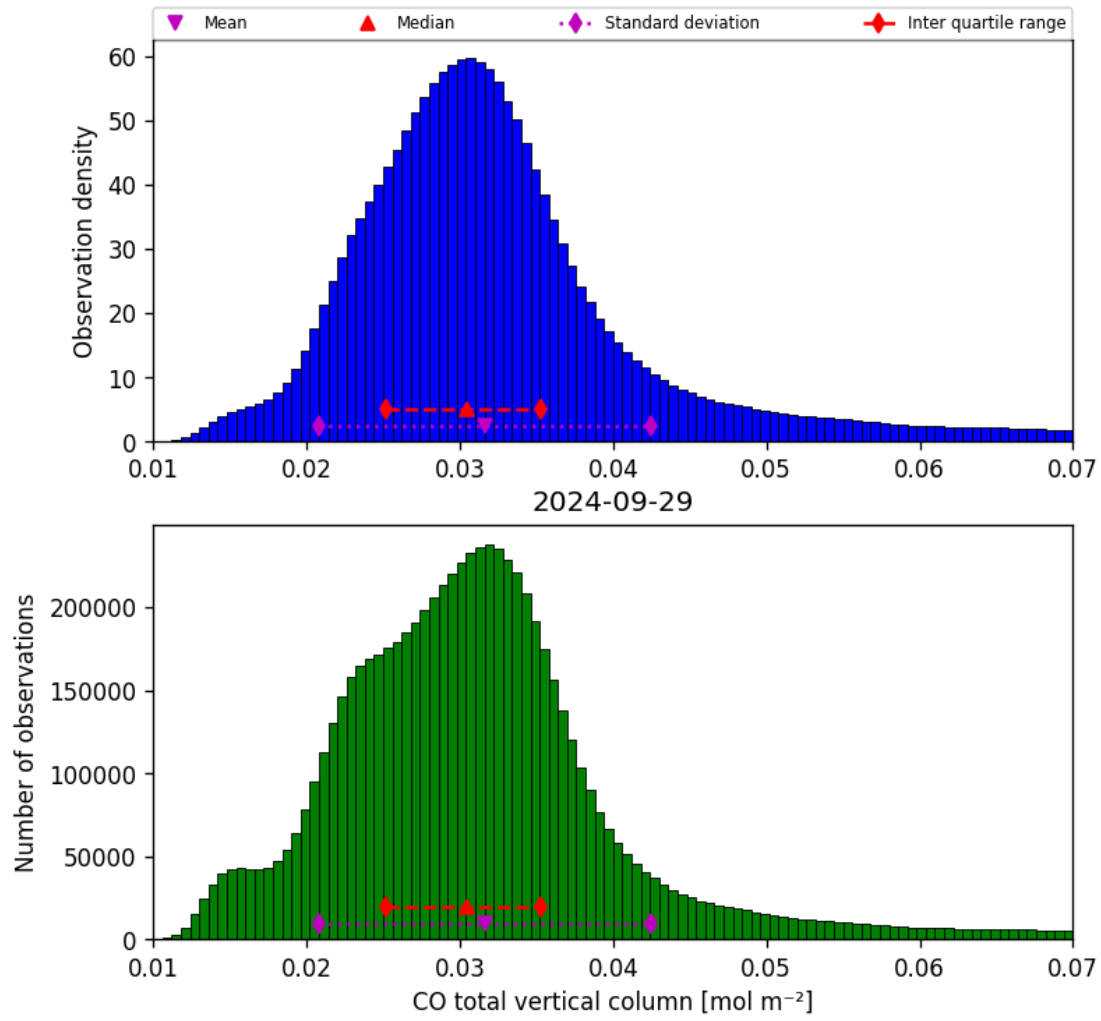
Figure 18: Histogram of “CO total vertical column” for 2024-09-28 to 2024-09-30
