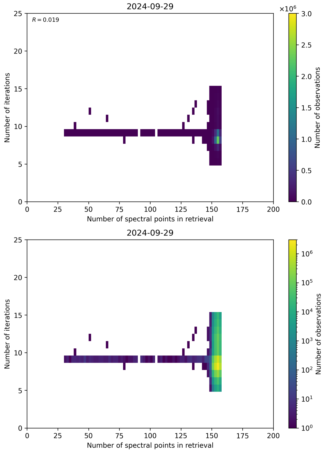
Figure 60: Scatter density plot of “Number of spectral points in retrieval” against “Number of iterations” for 2024-09-28 to 2024-09-30.
