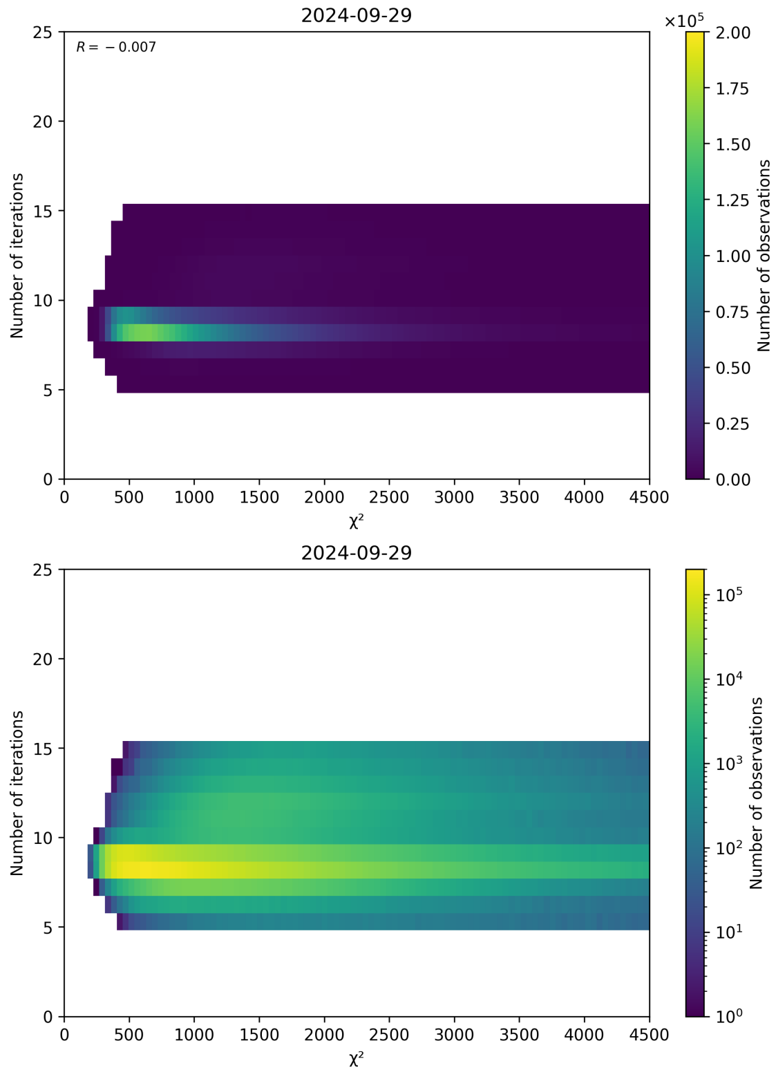
Figure 49: Scatter density plot of “ \chi^2 ” against “Number of iterations” for 2024-09-28 to 2024-09-30.
