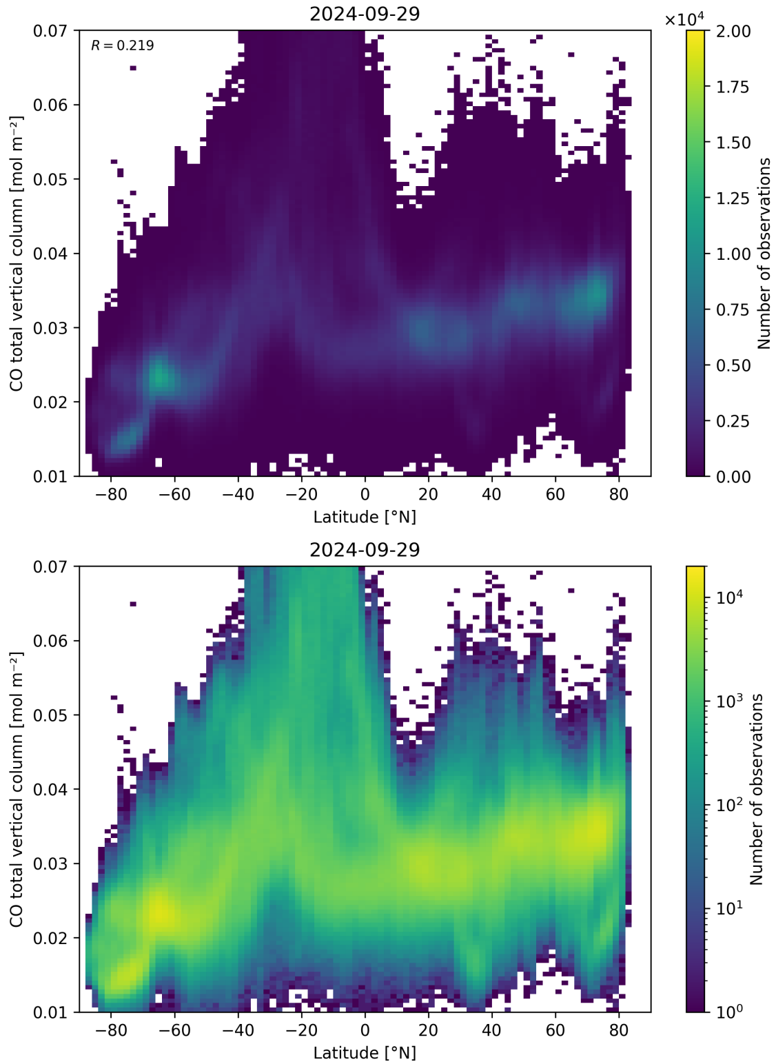
Figure 51: Scatter density plot of “Latitude” against “CO total vertical column” for 2024-09-28 to 2024-09-30.
