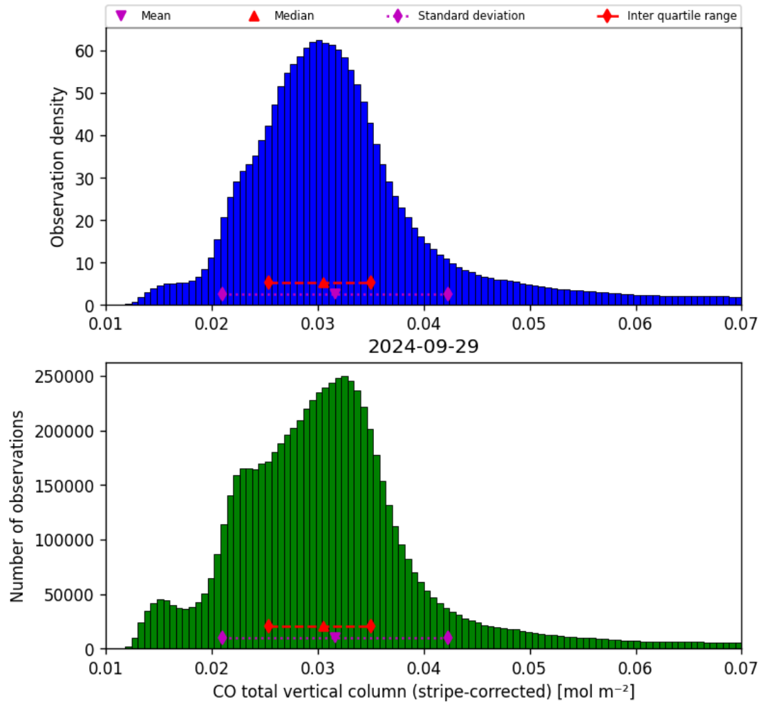
Figure 19: Histogram of “CO total vertical column (stripe-corrected)” for 2024-09-28 to 2024-09-30
