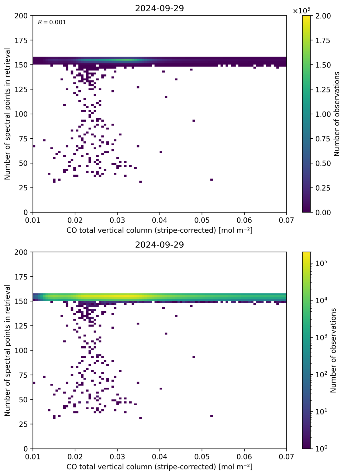
Figure 40: Scatter density plot of “CO total vertical column (stripe-corrected)” against “Number of spectral points in retrieval” for 2024-09-28 to 2024-09-30.
