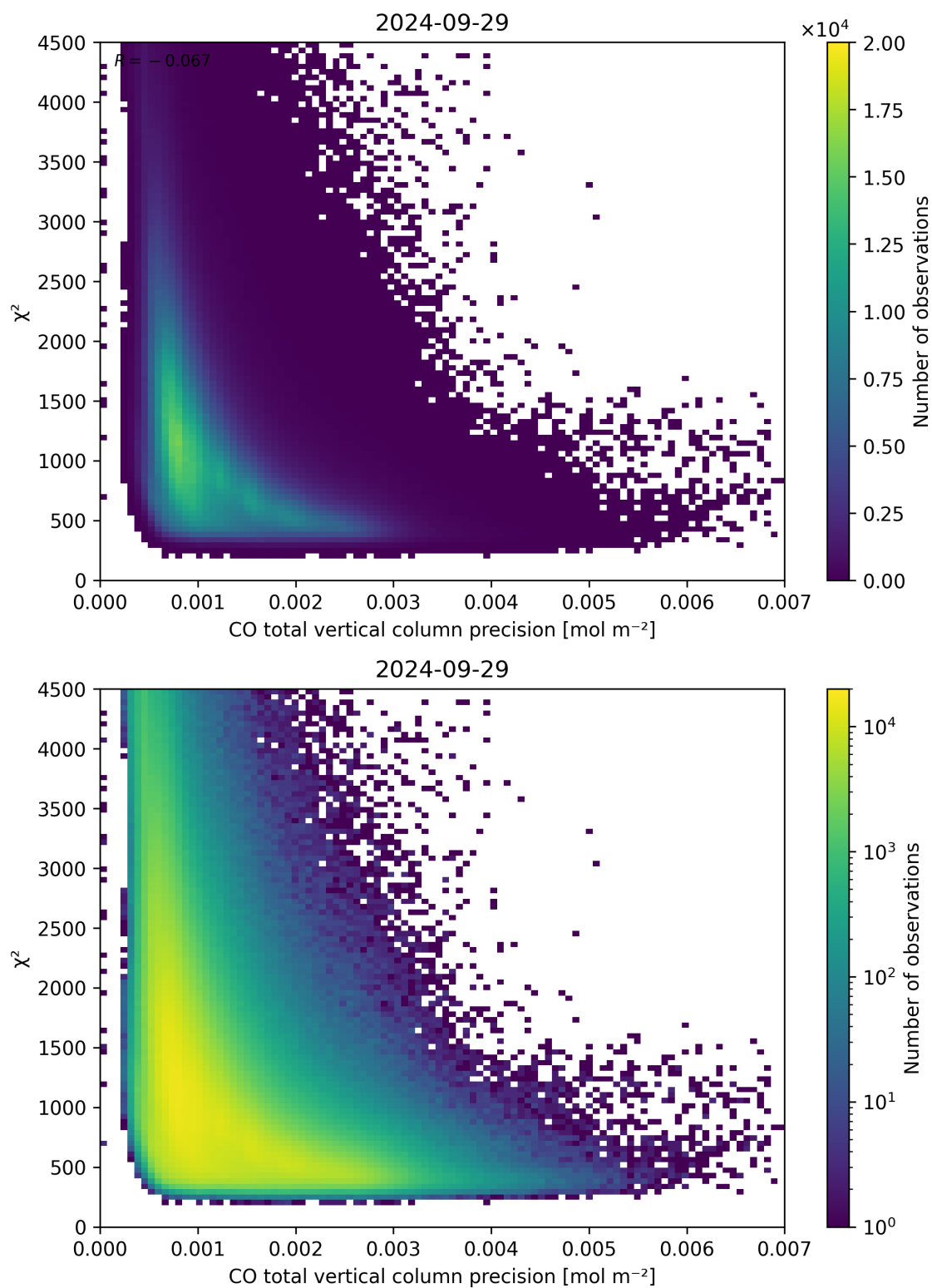
Figure 44: Scatter density plot of “CO total vertical column precision” against “ \chi^2 ” for 2024-09-28 to 2024-09-30.
