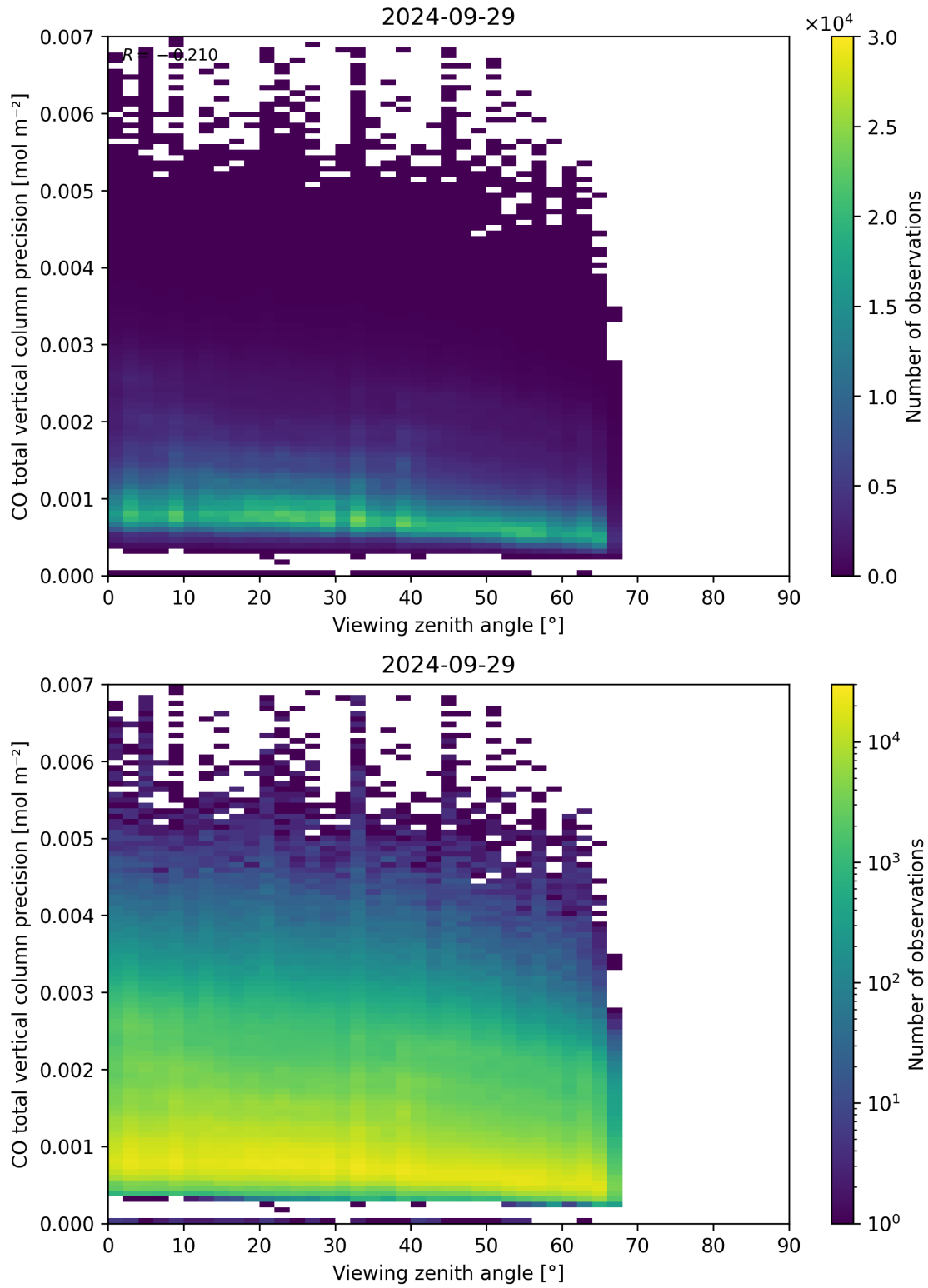
Figure 71: Scatter density plot of “Viewing zenith angle” against “CO total vertical column precision” for 2024-09-28 to 2024-09-30.
