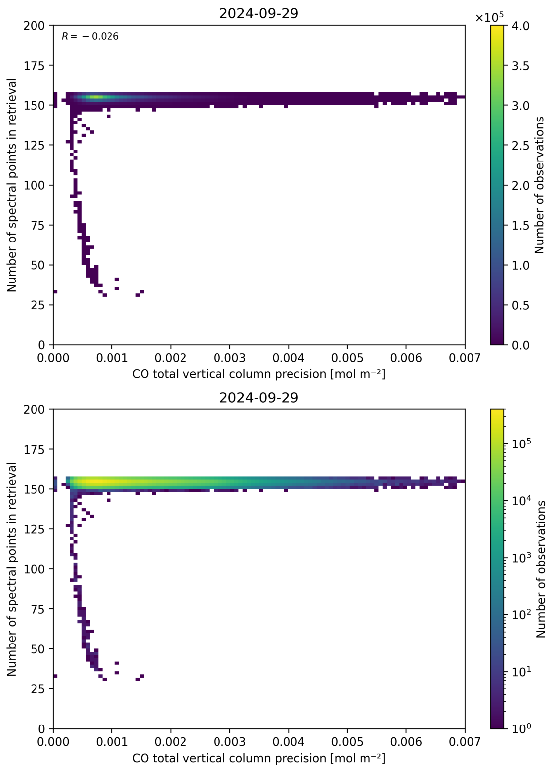
Figure 47: Scatter density plot of “CO total vertical column precision” against “Number of spectral points in retrieval” for 2024-09-28 to 2024-09-30.
