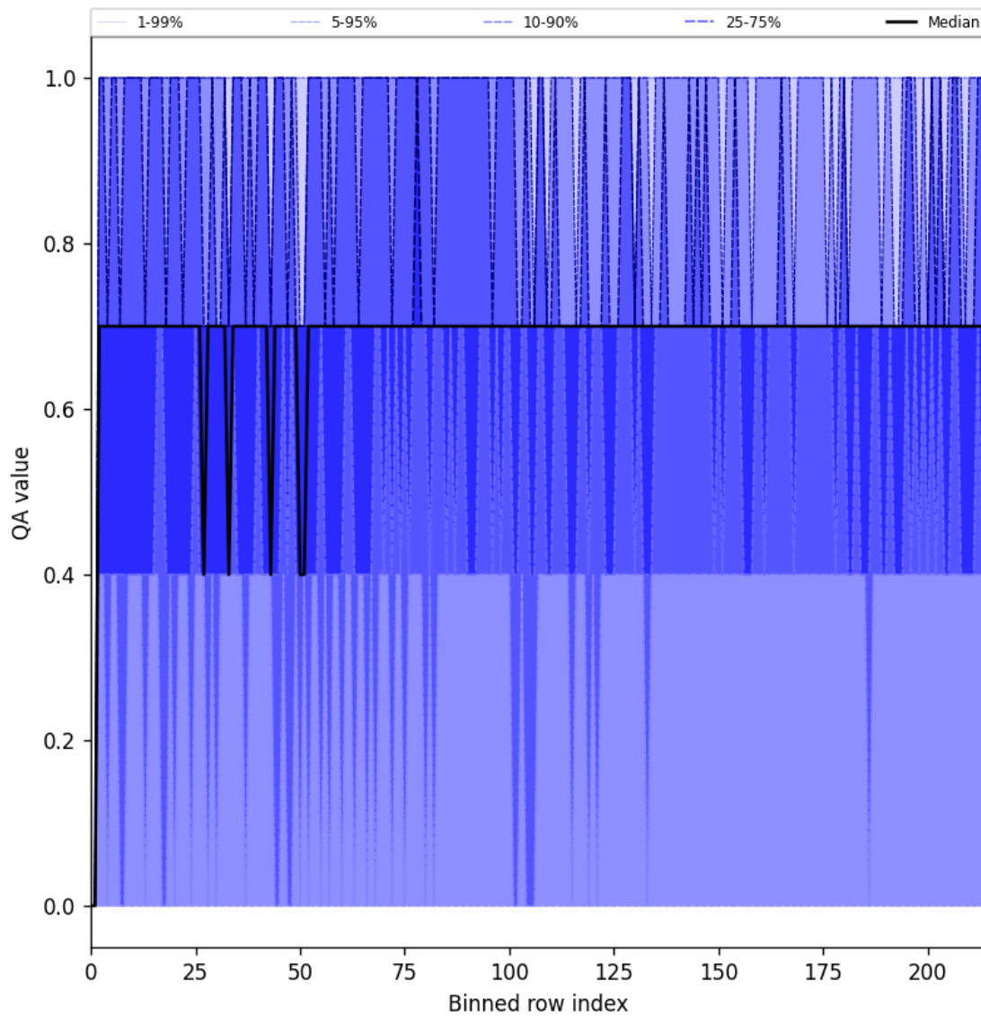
Figure 25: Along track statistics of “QA value” for 2024-09-28 to 2024-09-30
