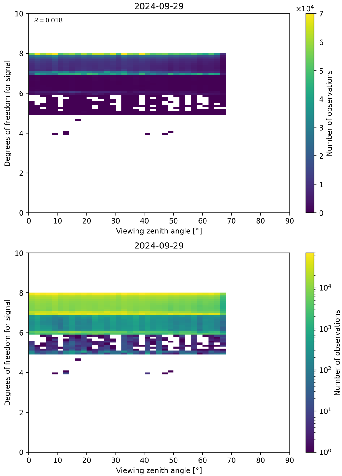
Figure 73: Scatter density plot of “Viewing zenith angle” against “Degrees of freedom for signal” for 2024-09-28 to 2024-09-30.
