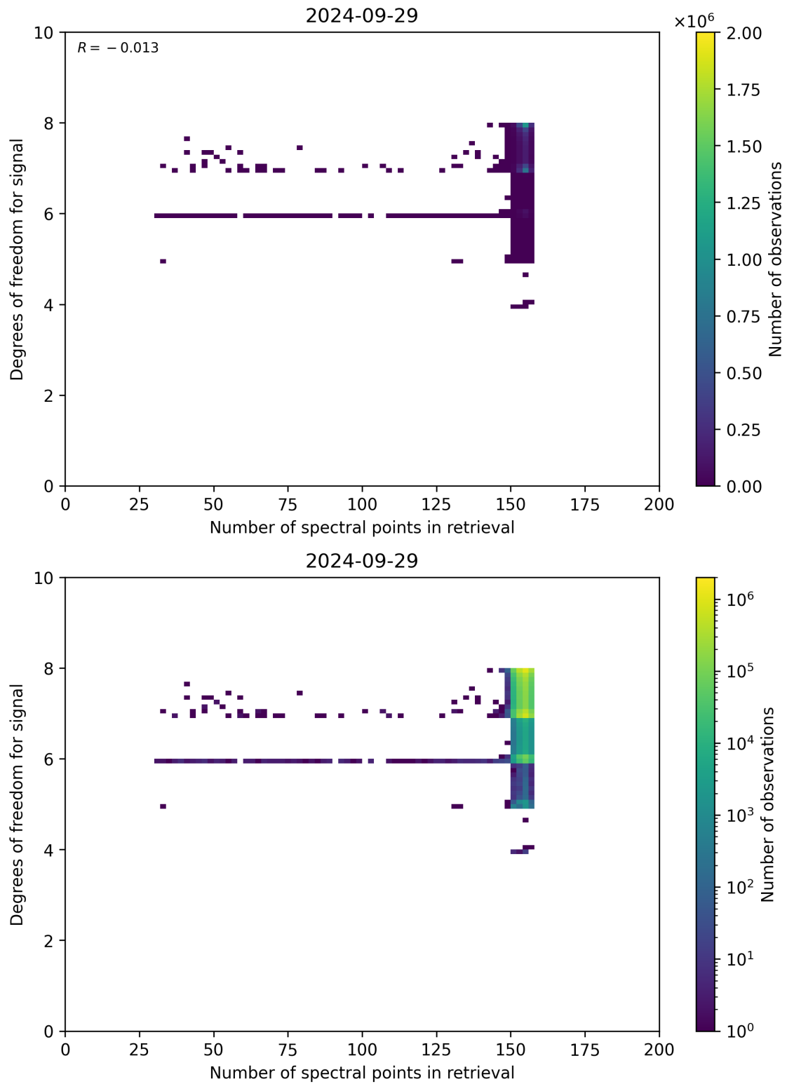
Figure 59: Scatter density plot of “Number of spectral points in retrieval” against “Degrees of freedom for signal” for 2024-09-28 to 2024-09-30.
